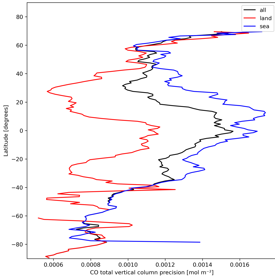
Figure 12: Zonal average of “CO total vertical column precision” for 2024-02-04 to 2024-02-06.
