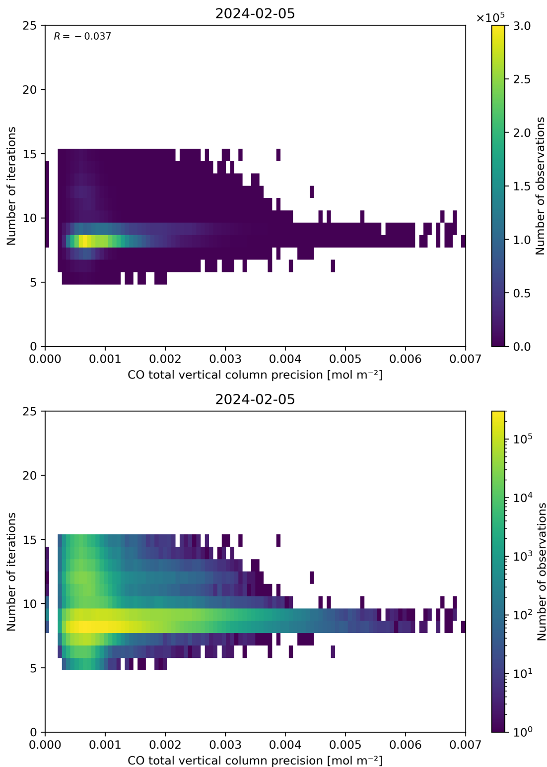
Figure 46: Scatter density plot of “CO total vertical column precision” against “Number of iterations” for 2024-02-04 to 2024-02-06.
