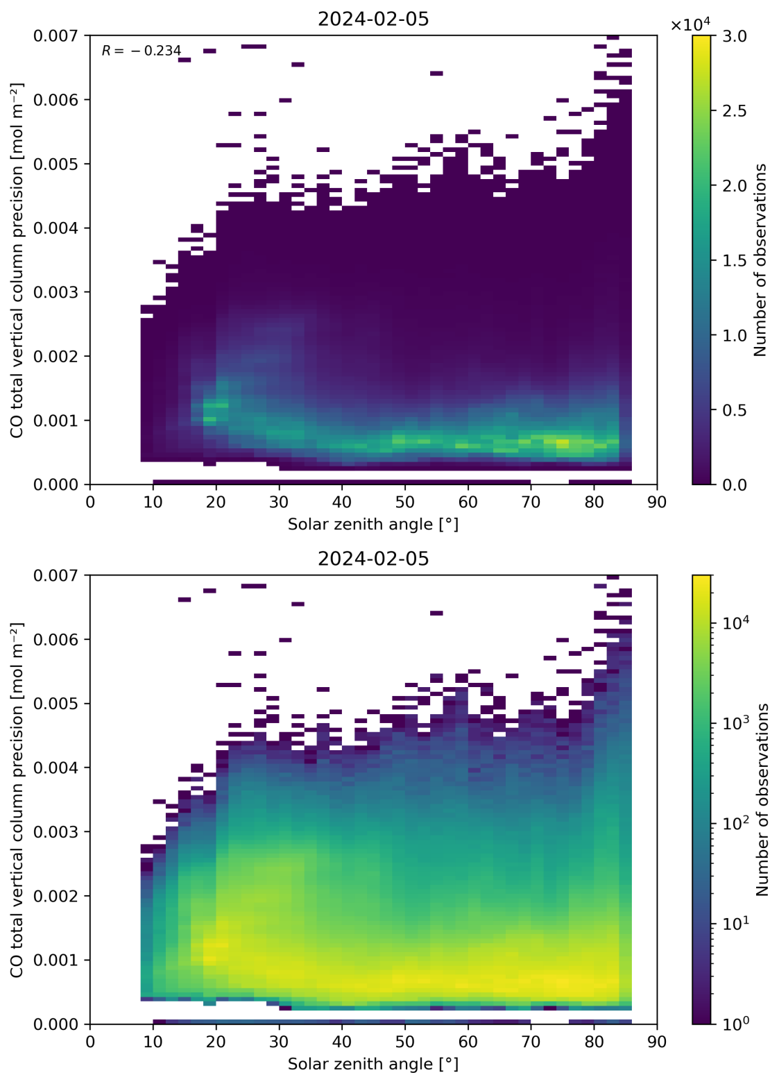
Figure 63: Scatter density plot of “Solar zenith angle” against “CO total vertical column precision” for 2024-02-04 to 2024-02-06.
