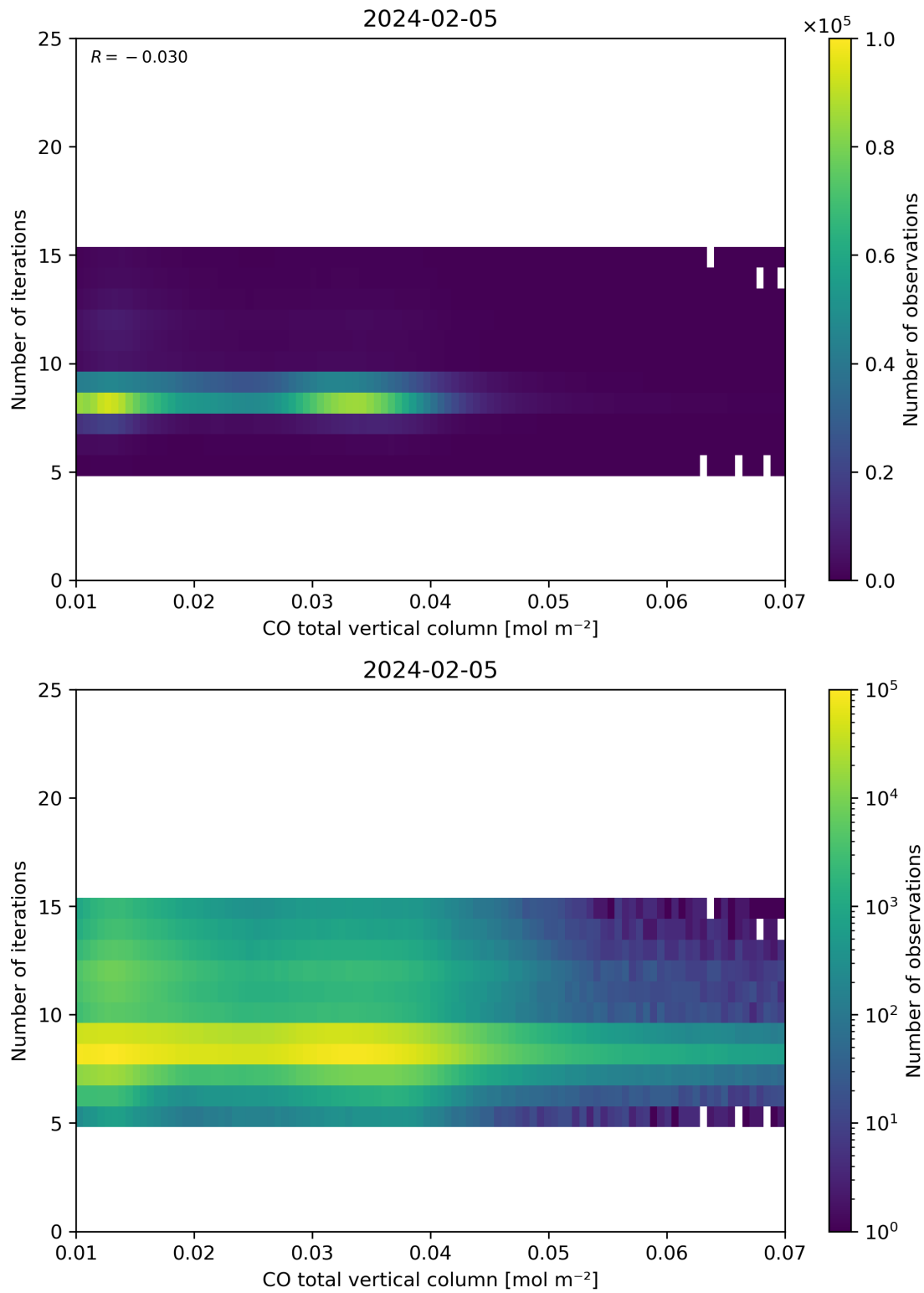
Figure 42: Scatter density plot of “CO total vertical column” against “Number of iterations” for 2024-02-04 to 2024-02-06.
