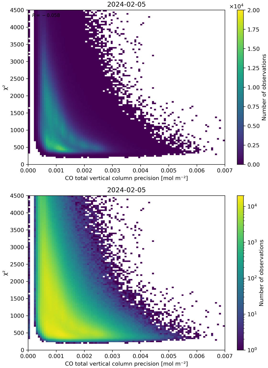
Figure 44: Scatter density plot of “CO total vertical column precision” against “ \chi^2 ” for 2024-02-04 to 2024-02-06.
