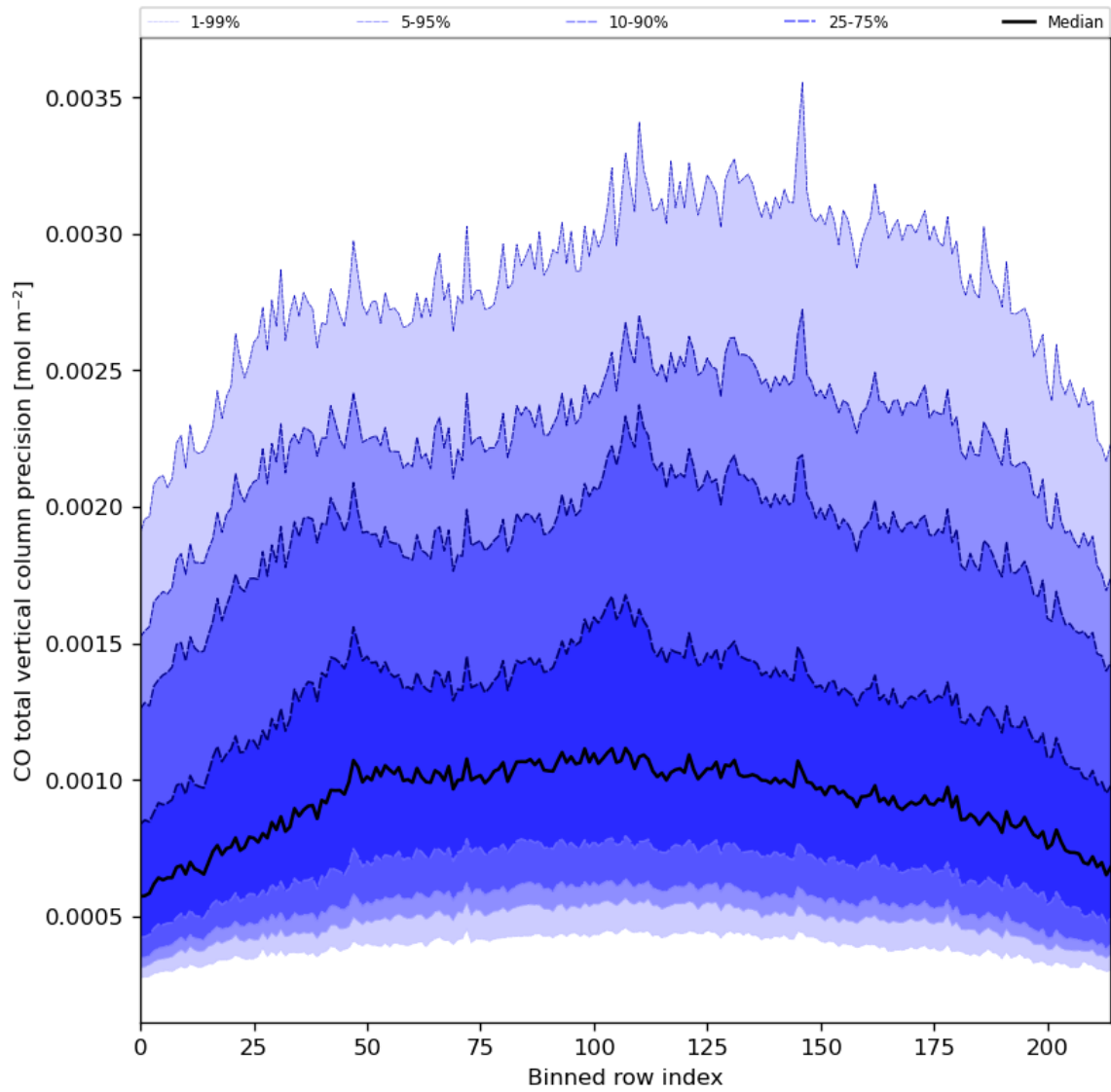
Figure 28: Along track statistics of “CO total vertical column precision” for 2024-02-04 to 2024-02-06
