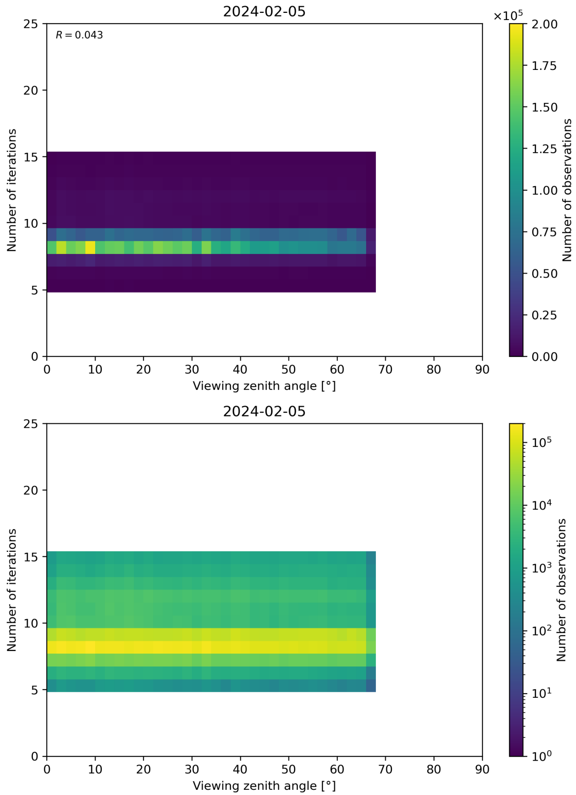
Figure 75: Scatter density plot of “Viewing zenith angle” against “Number of iterations” for 2024-02-04 to 2024-02-06.
