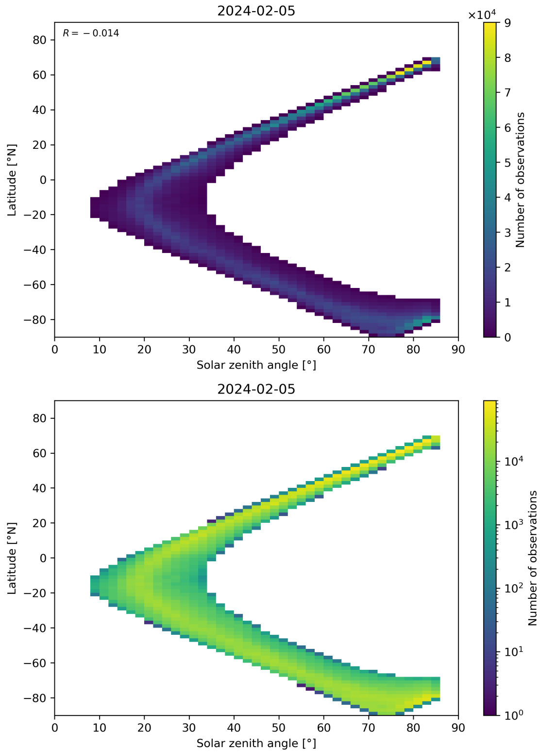
Figure 66: Scatter density plot of “Solar zenith angle” against “Latitude” for 2024-02-04 to 2024-02-06.
