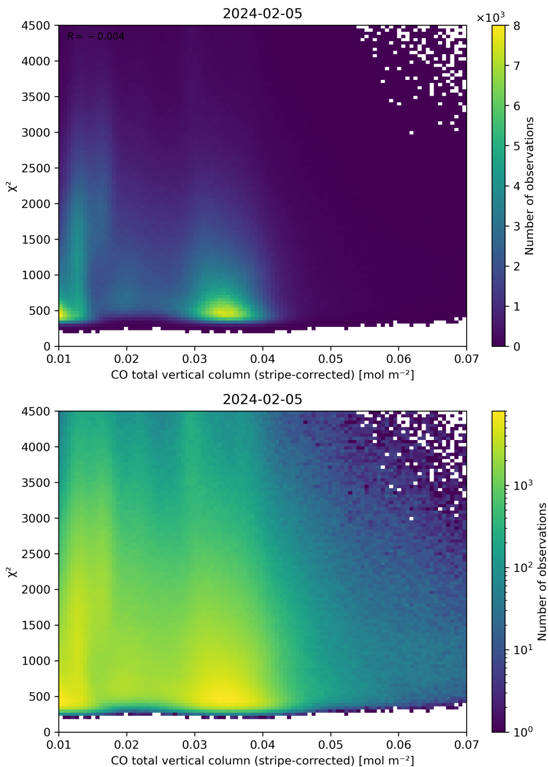
Figure 37: Scatter density plot of “CO total vertical column (stripe-corrected)” against “ \chi^2 ” for 2024-02-04 to 2024-02-06.
