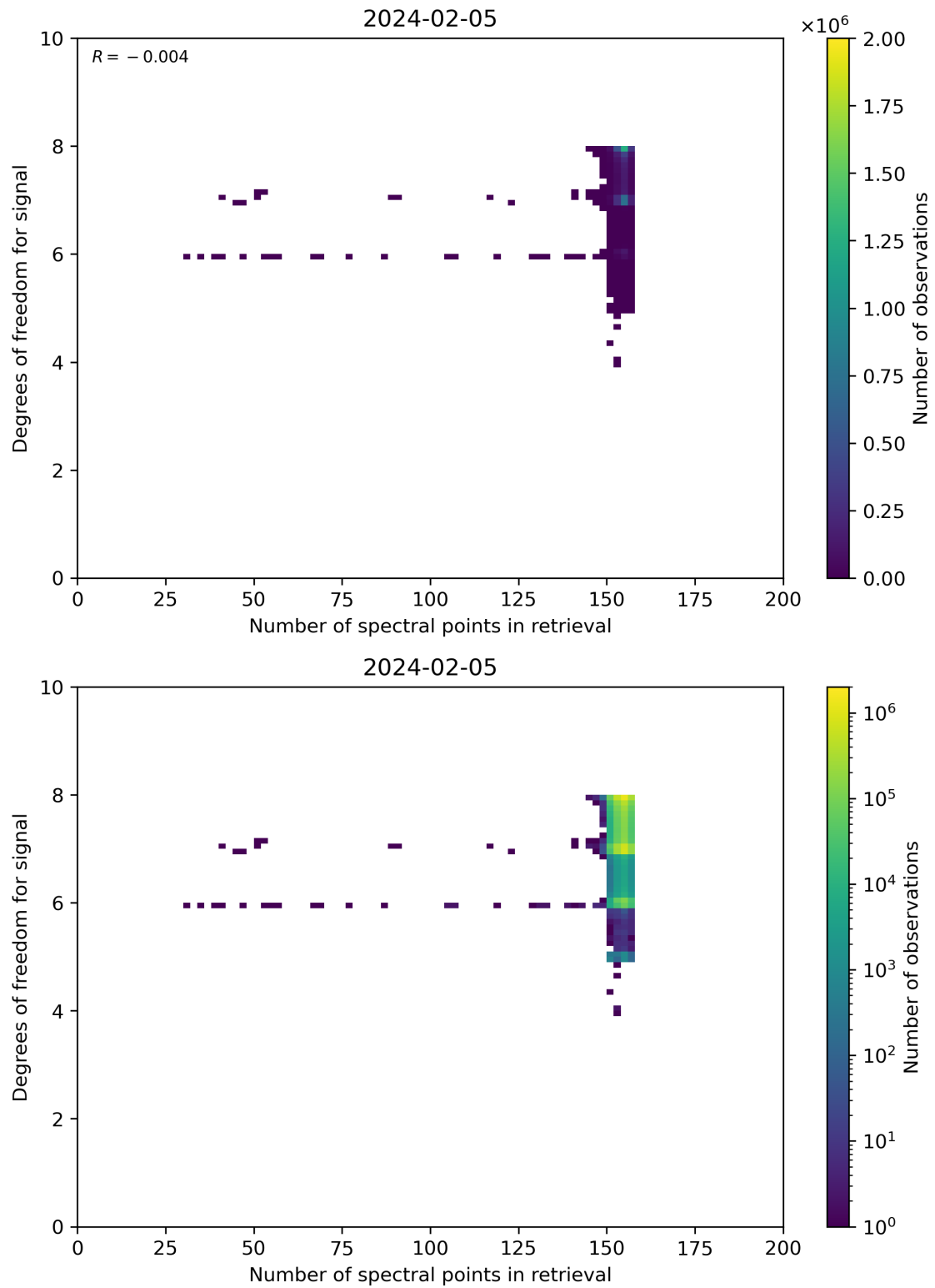
Figure 59: Scatter density plot of “Number of spectral points in retrieval” against “Degrees of freedom for signal” for 2024-02-04 to 2024-02-06.
