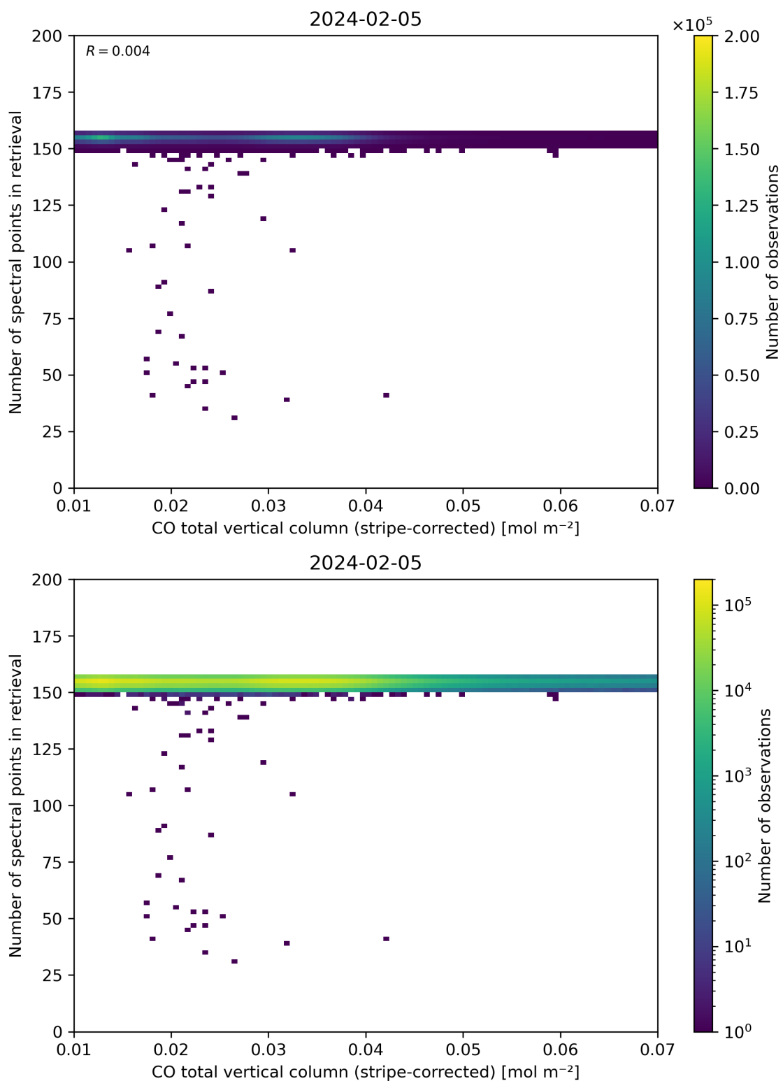
Figure 40: Scatter density plot of “CO total vertical column (stripe-corrected)” against “Number of spectral points in retrieval” for 2024-02-04 to 2024-02-06.
