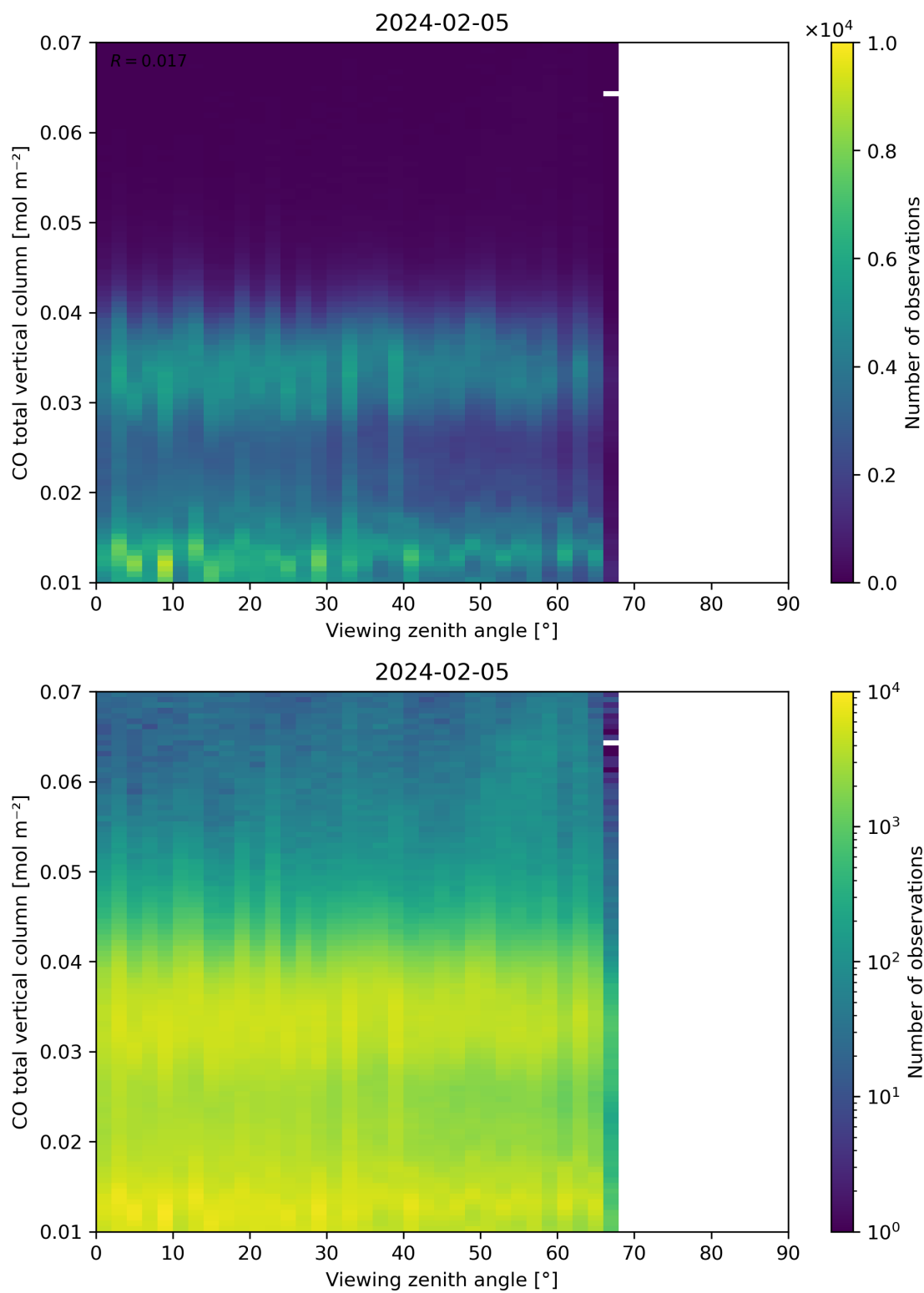
Figure 69: Scatter density plot of “Viewing zenith angle” against “CO total vertical column” for 2024-02-04 to 2024-02-06.
