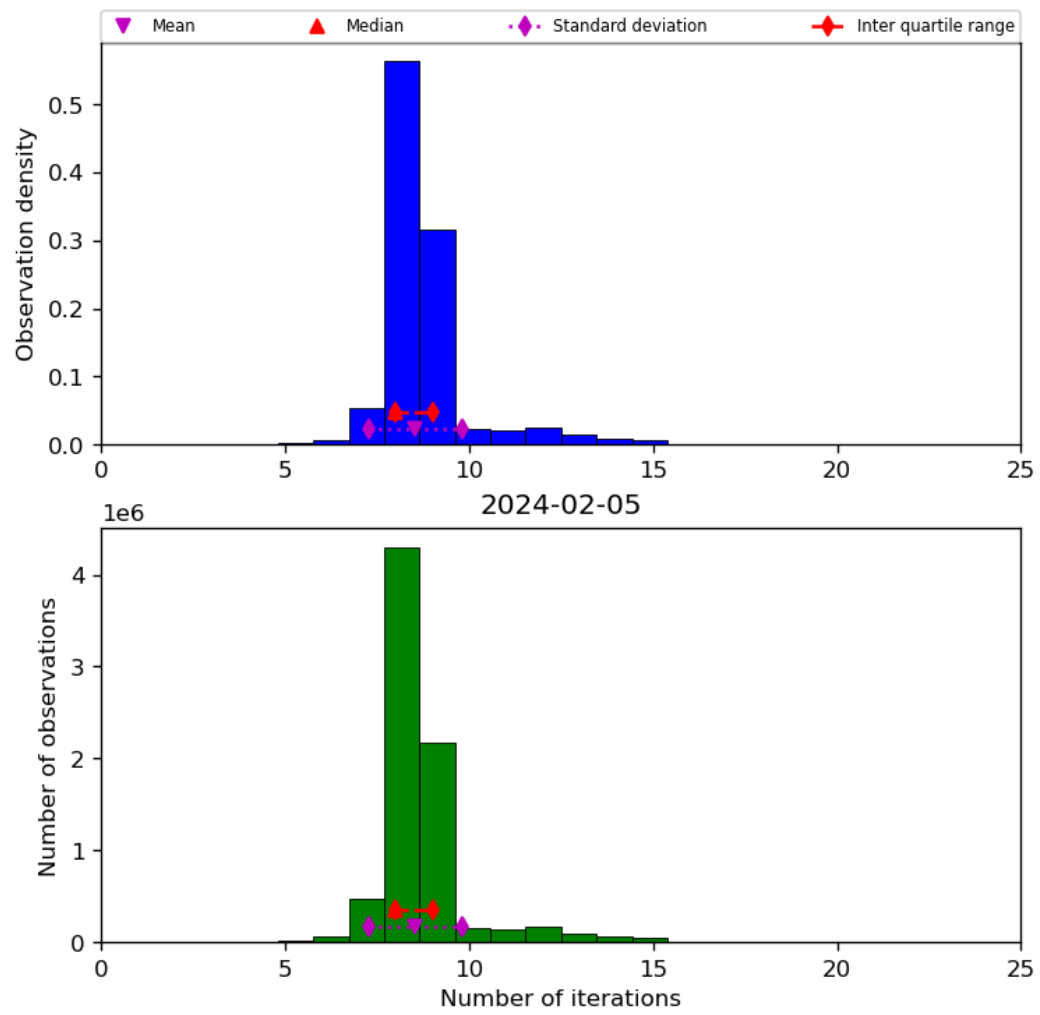
Figure 24: Histogram of “Number of iterations” for 2024-02-04 to 2024-02-06
