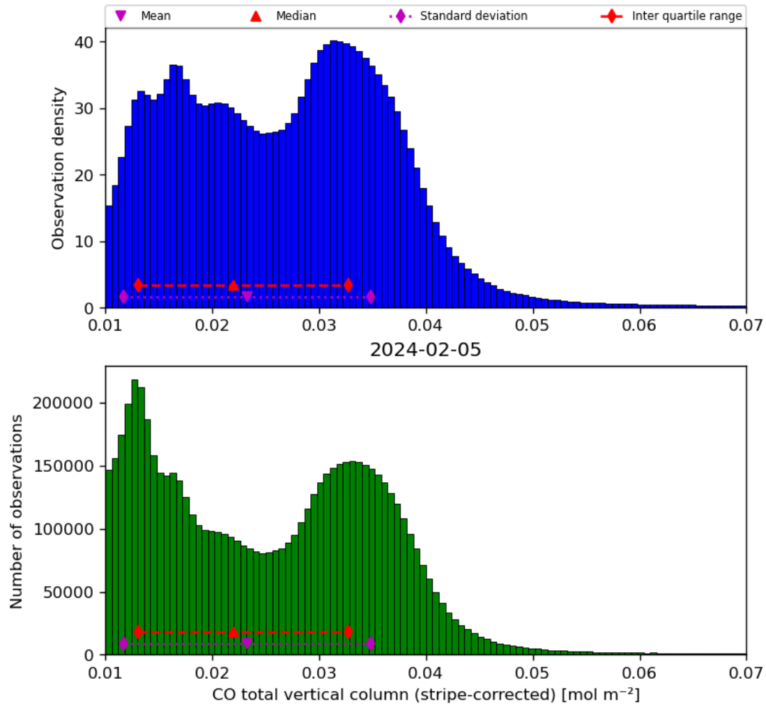
Figure 19: Histogram of “CO total vertical column (stripe-corrected)” for 2024-02-04 to 2024-02-06
