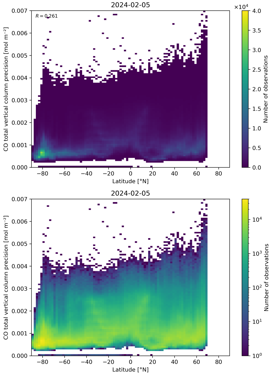
Figure 53: Scatter density plot of “Latitude” against “CO total vertical column precision” for 2024-02-04 to 2024-02-06.
