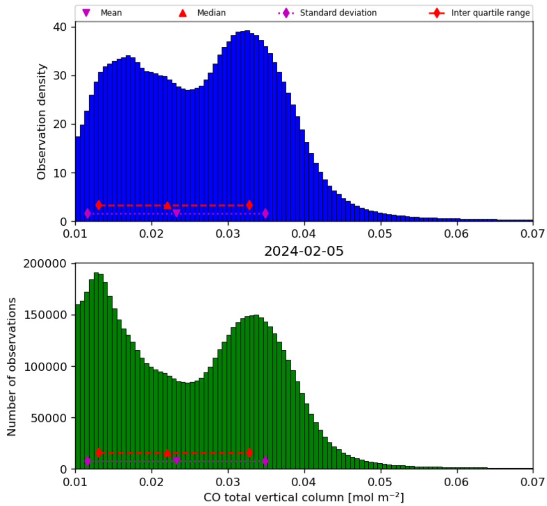
Figure 18: Histogram of “CO total vertical column” for 2024-02-04 to 2024-02-06
