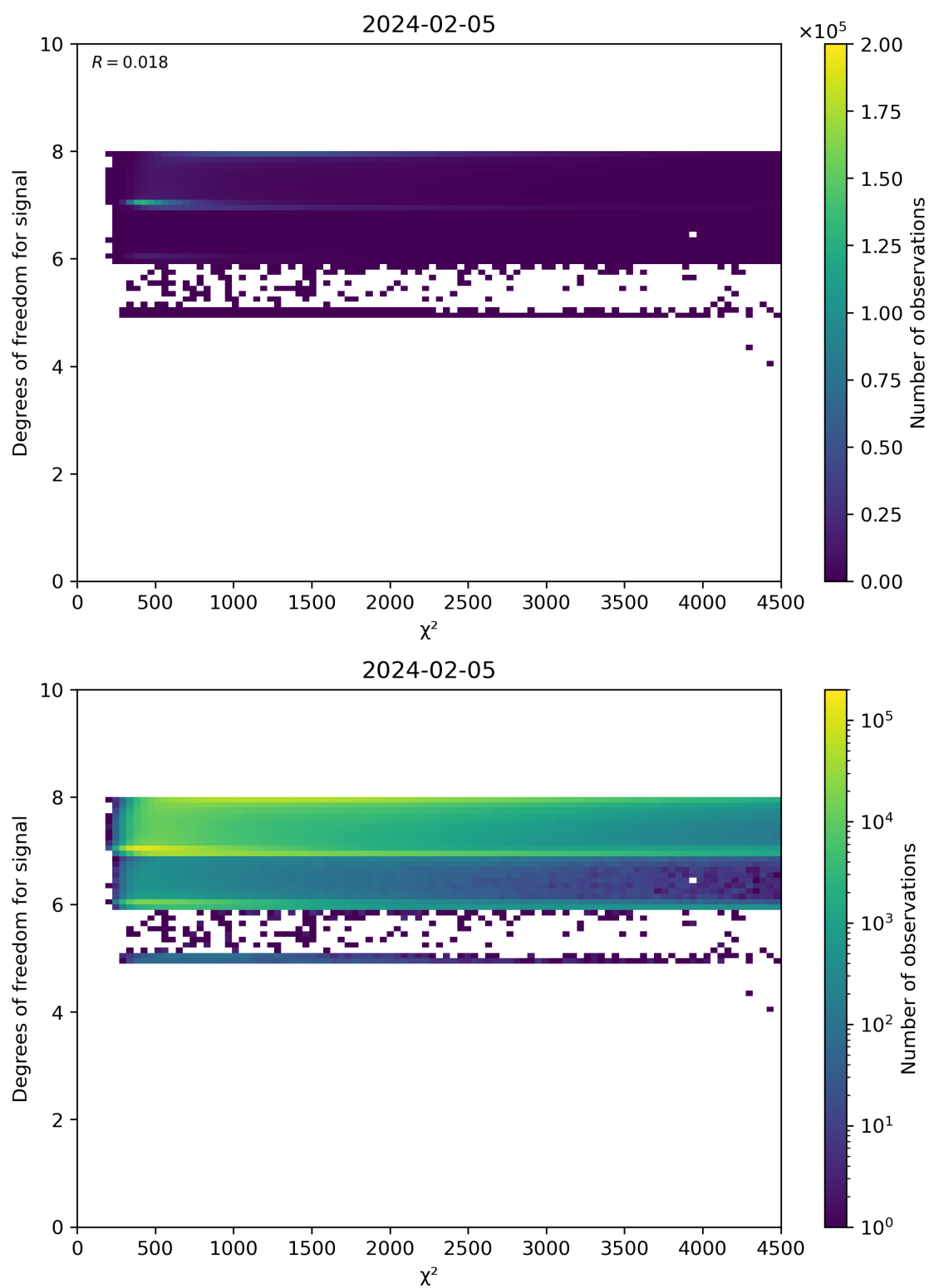
Figure 48: Scatter density plot of “ \chi^2 ” against “Degrees of freedom for signal” for 2024-02-04 to 2024-02-06.
