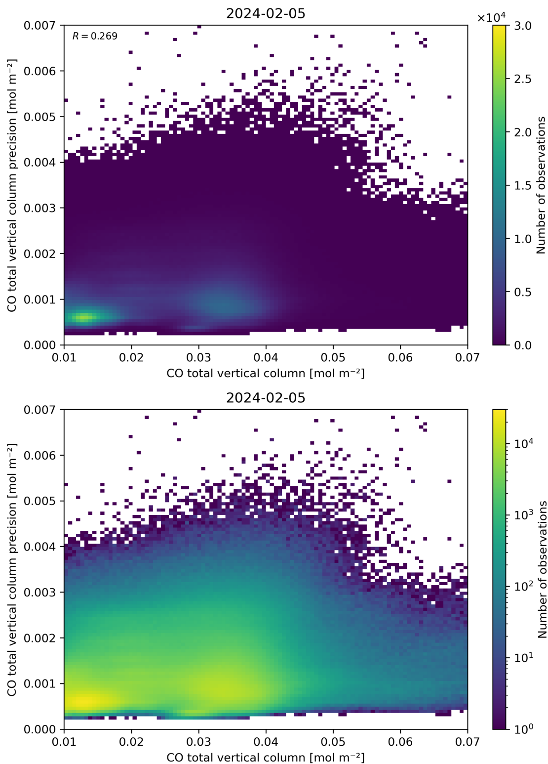
Figure 34: Scatter density plot of “CO total vertical column” against “CO total vertical column precision” for 2024-02-04 to 2024-02-06.
