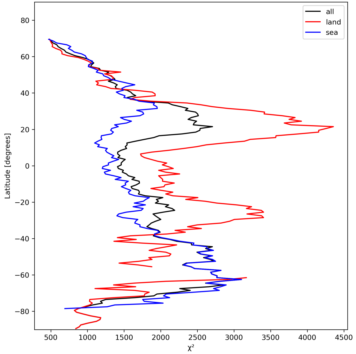
Figure 14: Zonal average of “ \chi^2 ” for 2024-02-04 to 2024-02-06.
