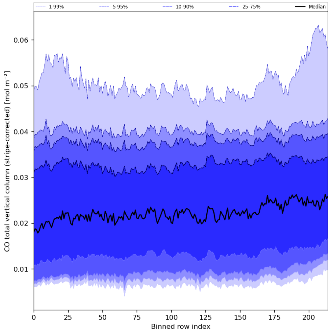
Figure 27: Along track statistics of “CO total vertical column (stripe-corrected)” for 2024-02-04 to 2024-02-06
