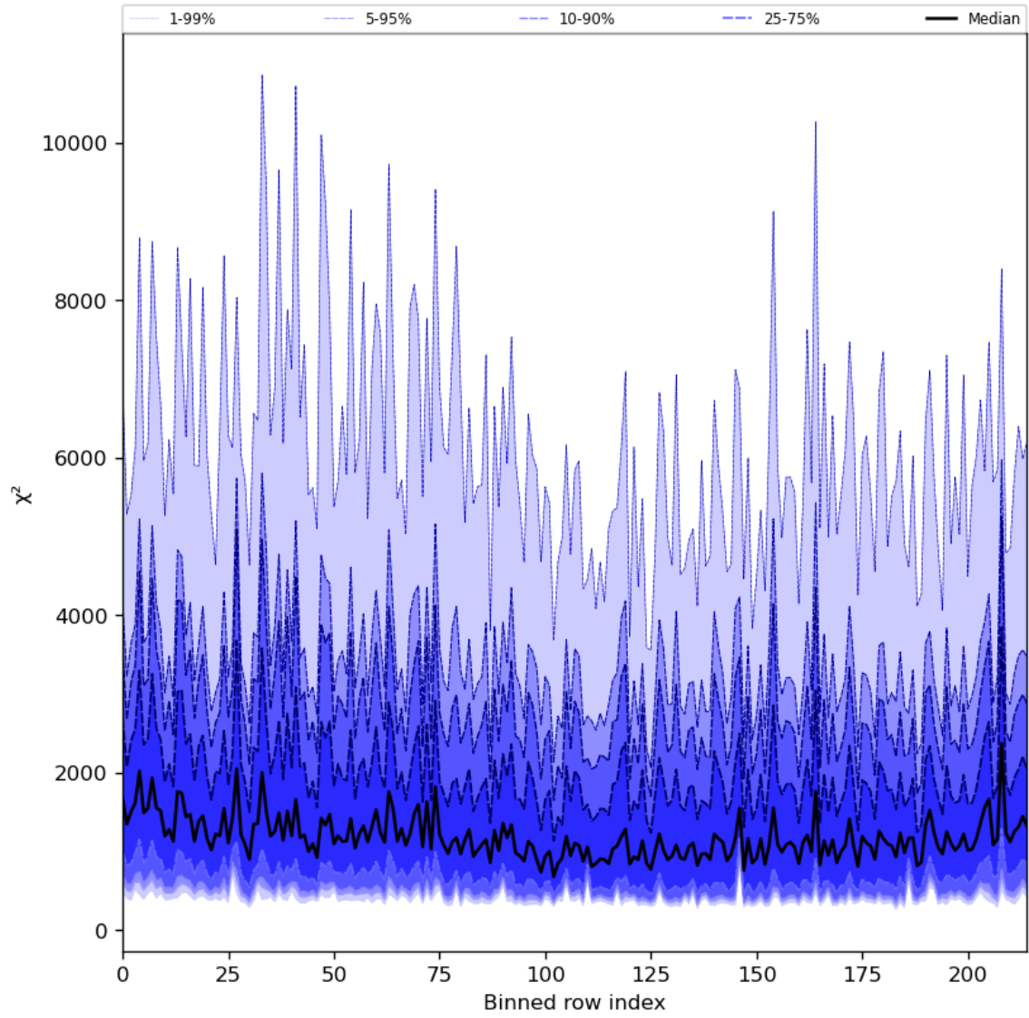
Figure 30: Along track statistics of “ \chi^2 ” for 2024-02-04 to 2024-02-06
