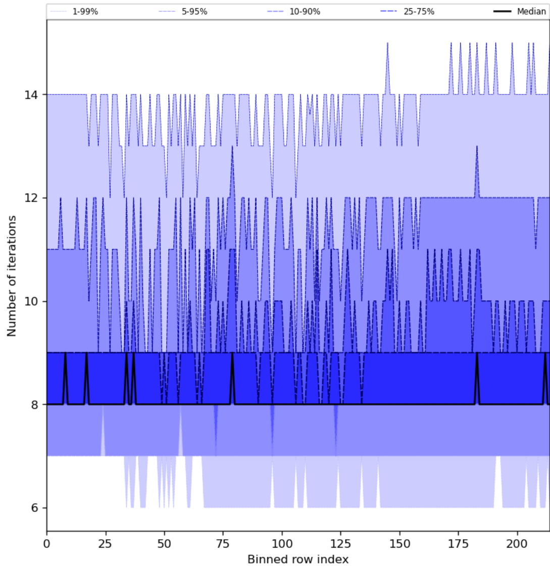
Figure 32: Along track statistics of “Number of iterations” for 2024-02-04 to 2024-02-06
