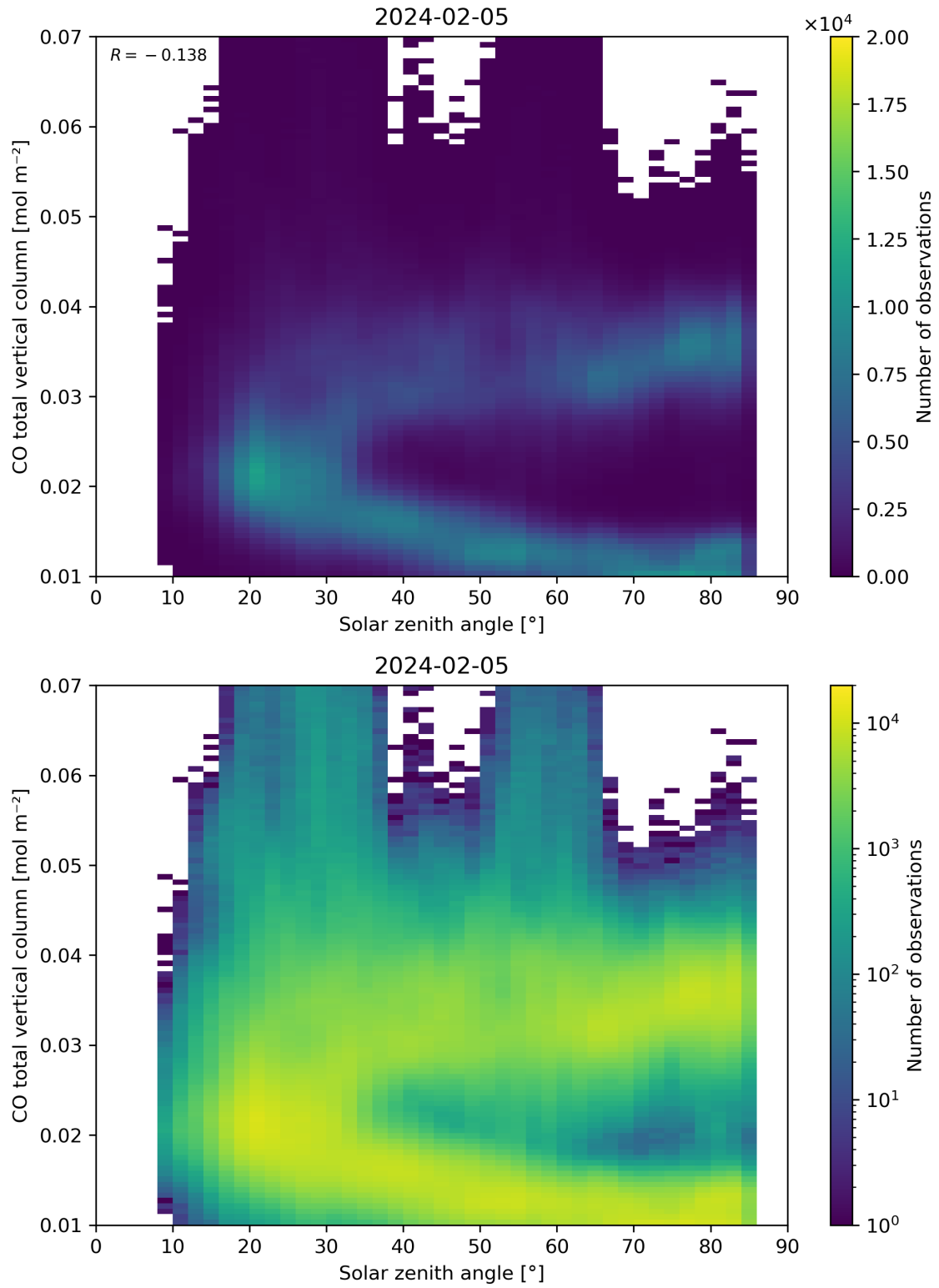
Figure 61: Scatter density plot of “Solar zenith angle” against “CO total vertical column” for 2024-02-04 to 2024-02-06.
