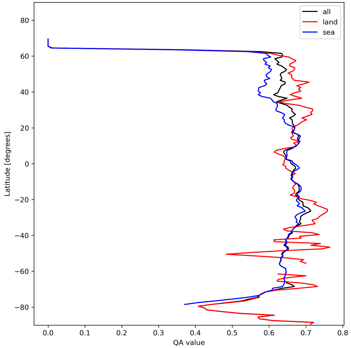
Figure 9: Zonal average of “QA value” for 2024-02-04 to 2024-02-06.
