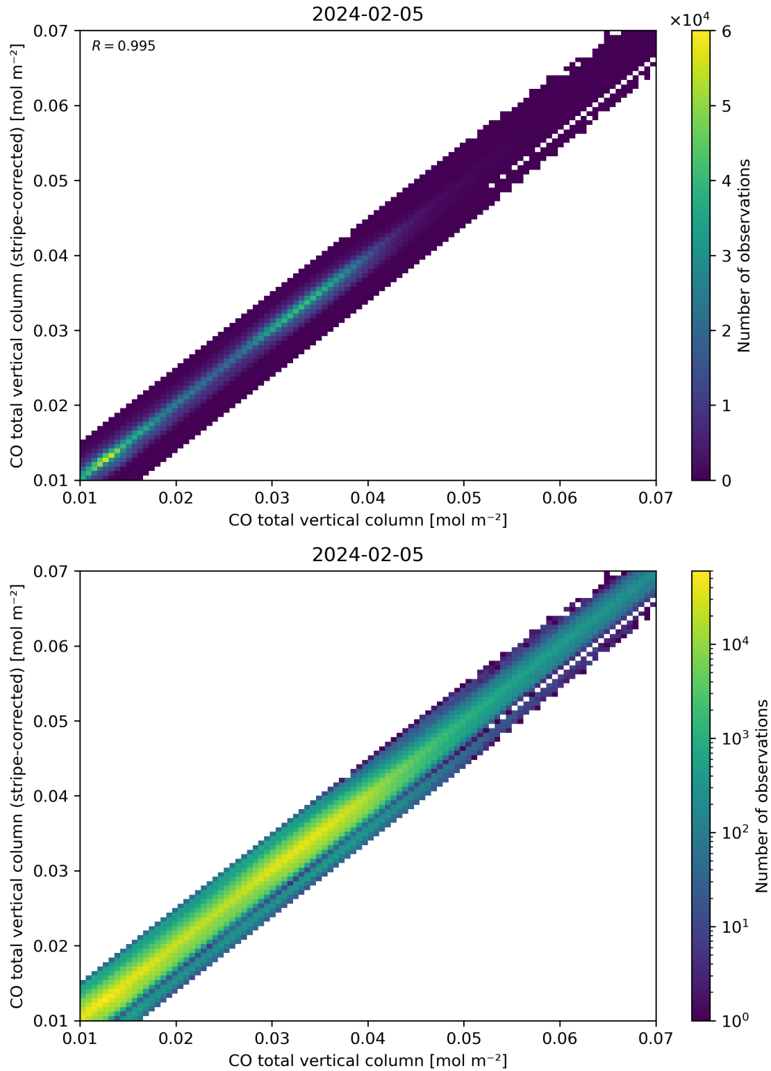
Figure 33: Scatter density plot of “CO total vertical column” against “CO total vertical column (stripe-corrected)” for 2024-02-04 to 2024-02-06.
