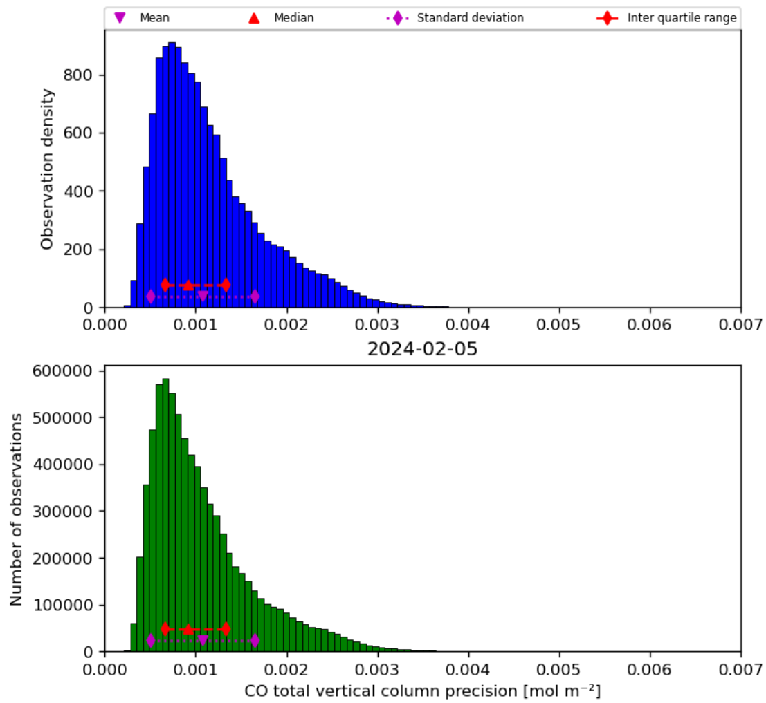
Figure 20: Histogram of “CO total vertical column precision” for 2024-02-04 to 2024-02-06
