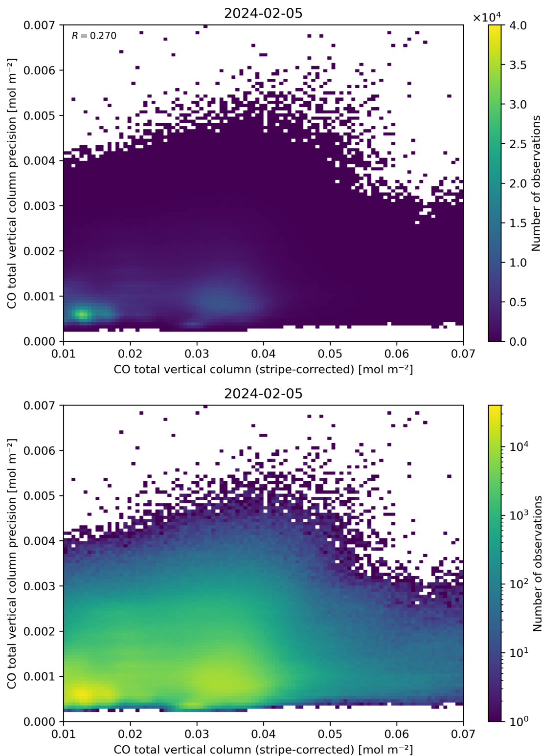
Figure 36: Scatter density plot of “CO total vertical column (stripe-corrected)” against “CO total vertical column precision” for 2024-02-04 to 2024-02-06.
