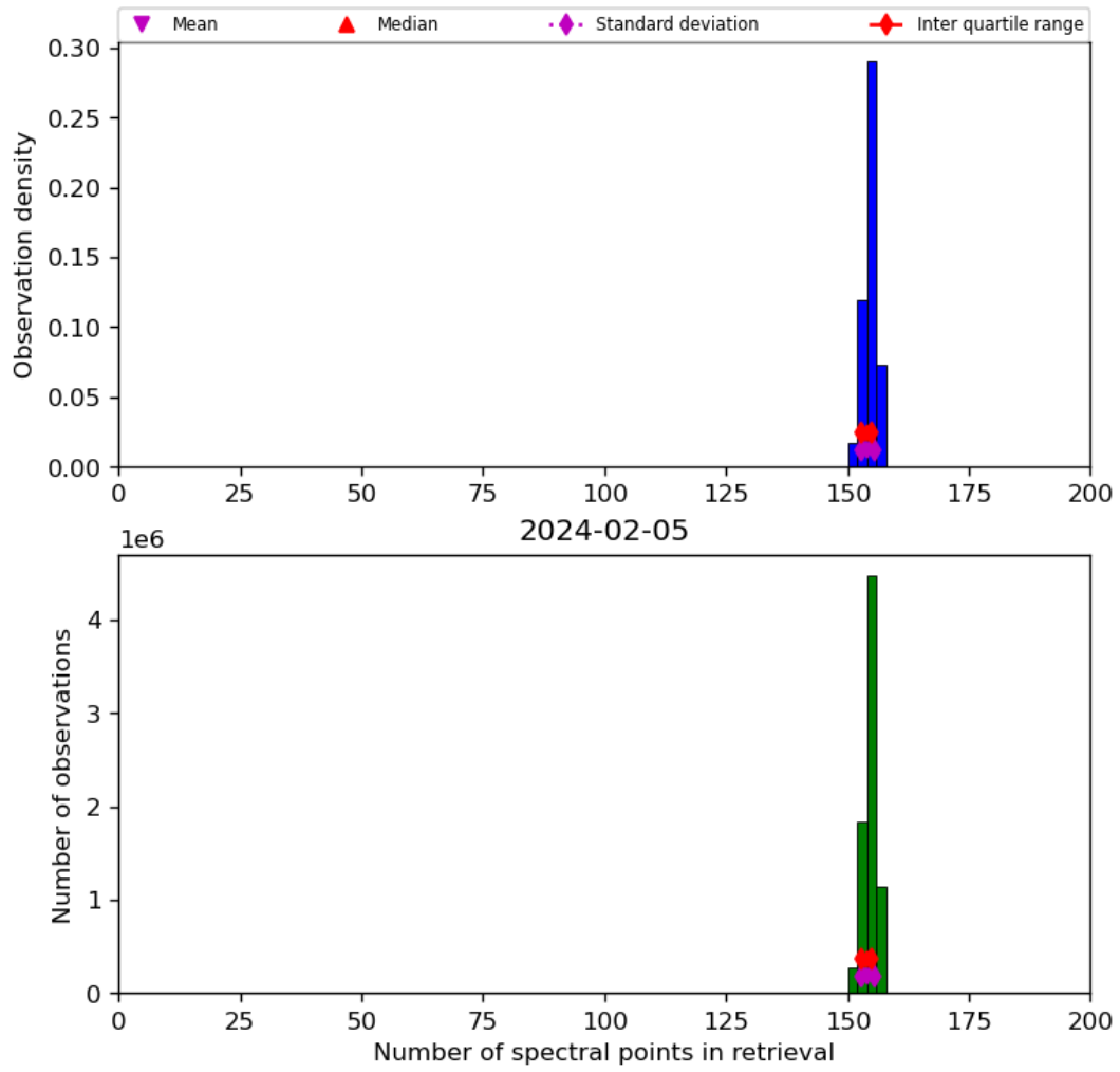
Figure 21: Histogram of “Number of spectral points in retrieval” for 2024-02-04 to 2024-02-06
