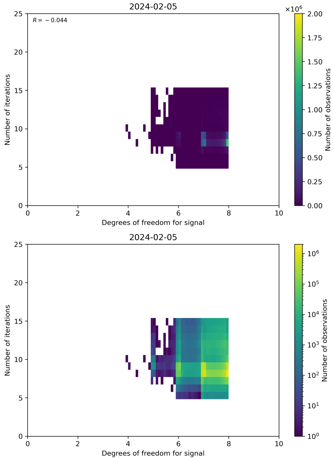
Figure 50: Scatter density plot of “Degrees of freedom for signal” against “Number of iterations” for 2024-02-04 to 2024-02-06.
