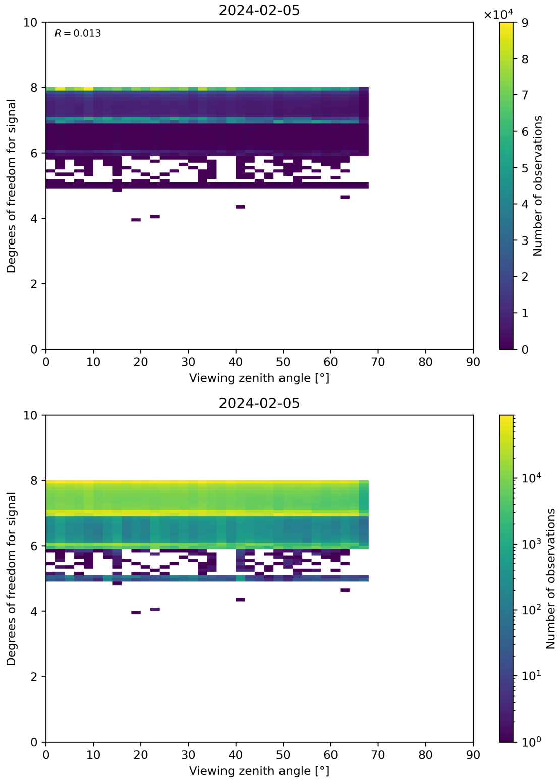
Figure 73: Scatter density plot of “Viewing zenith angle” against “Degrees of freedom for signal” for 2024-02-04 to 2024-02-06.
