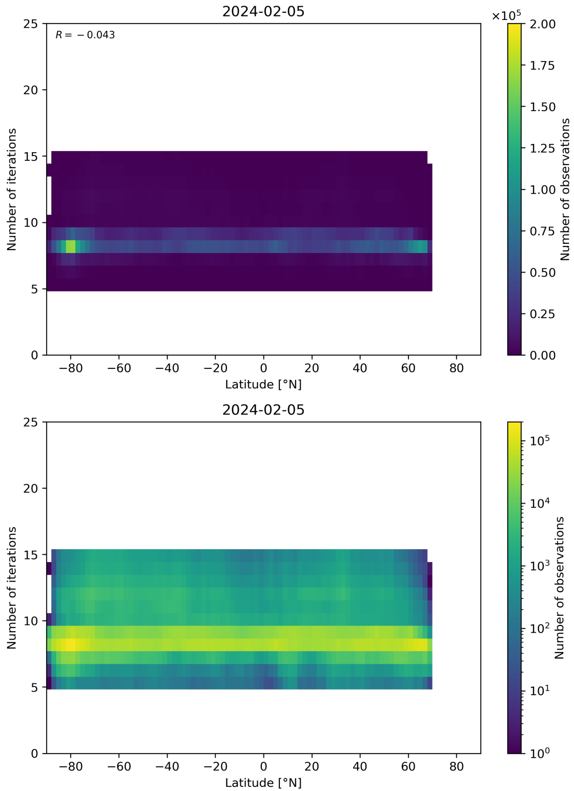
Figure 56: Scatter density plot of “Latitude” against “Number of iterations” for 2024-02-04 to 2024-02-06.
