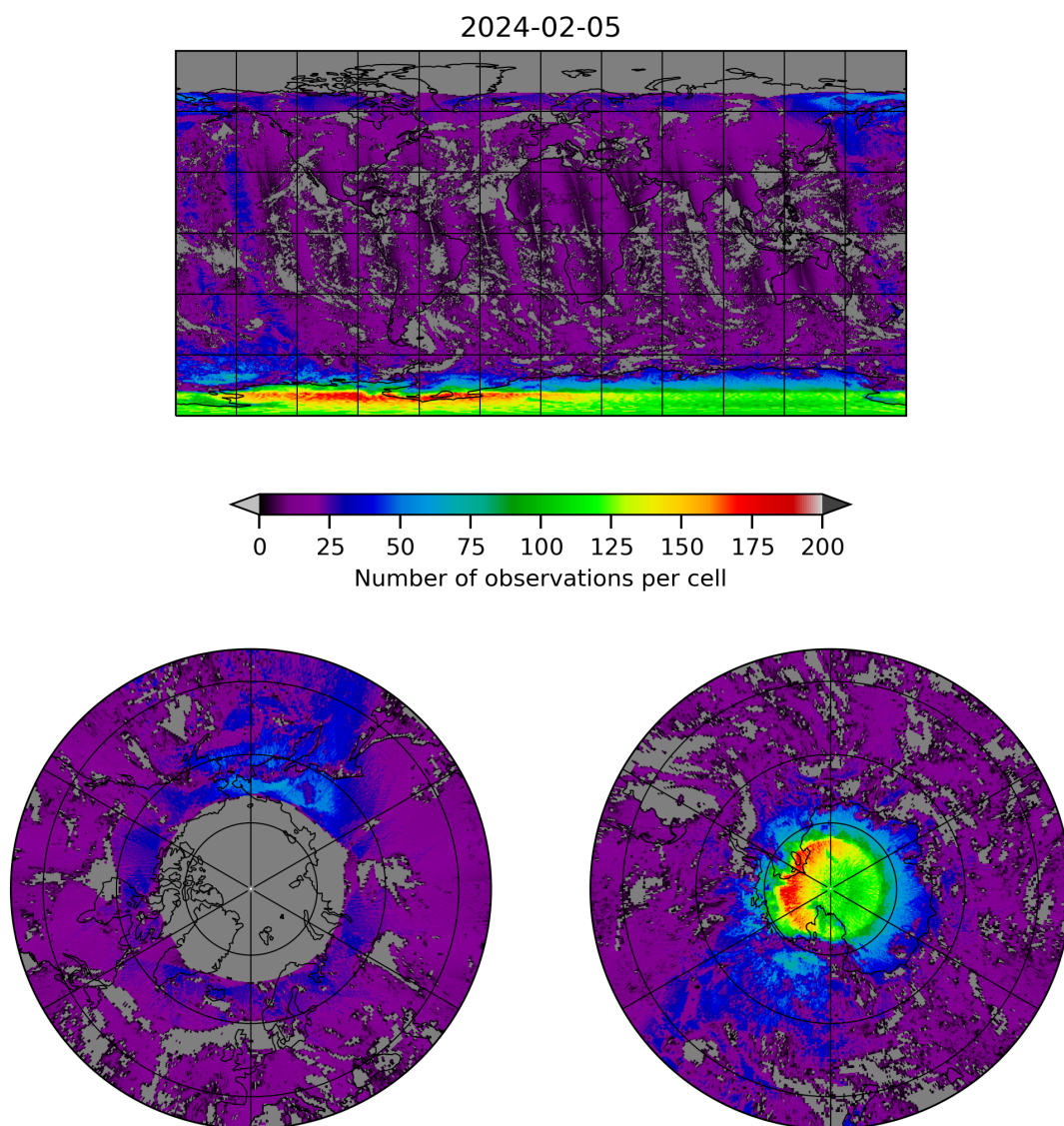
Figure 8: Map of the number of observations for 2024-02-04 to 2024-02-06
