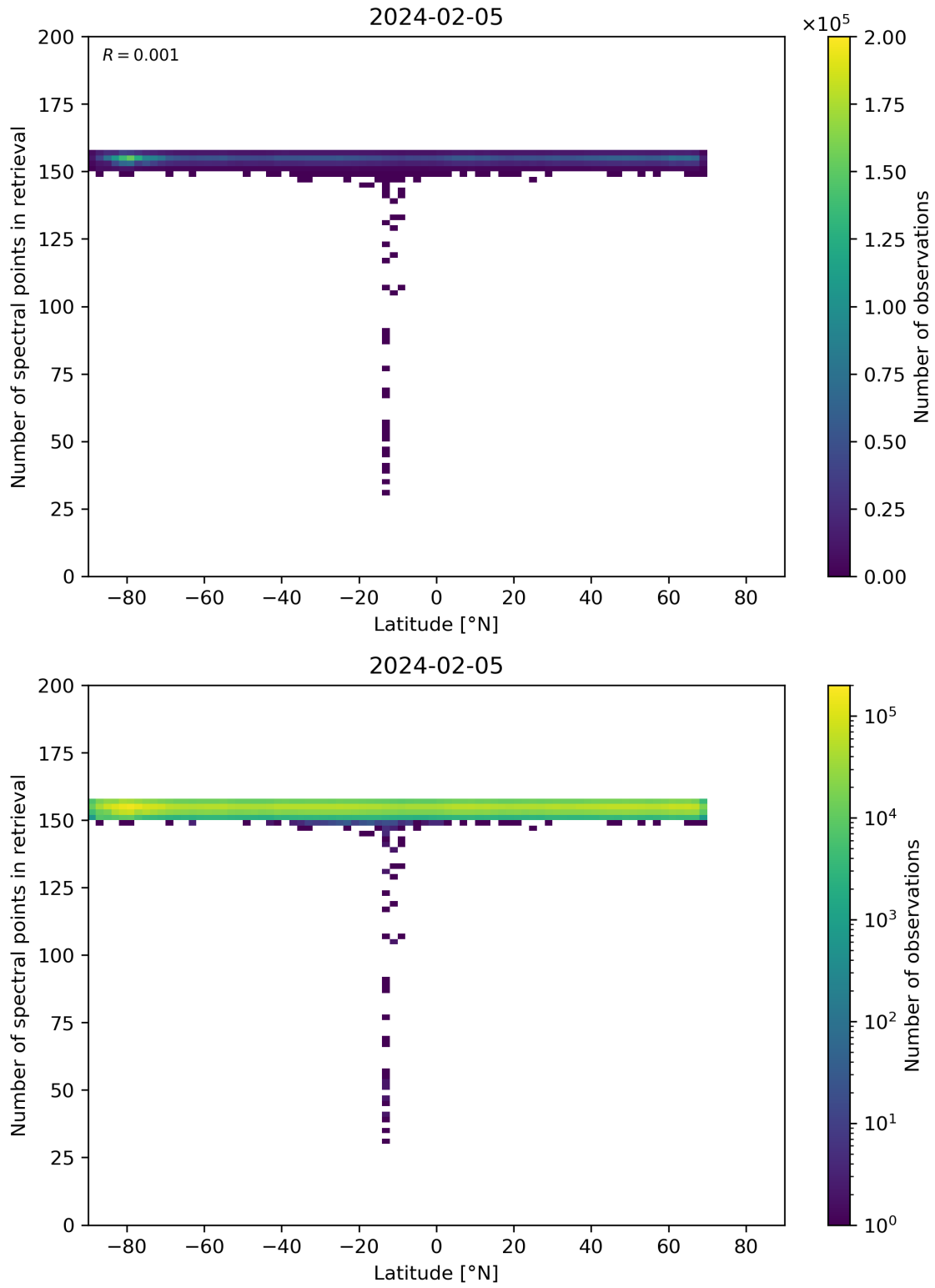
Figure 57: Scatter density plot of “Latitude” against “Number of spectral points in retrieval” for 2024-02-04 to 2024-02-06.
