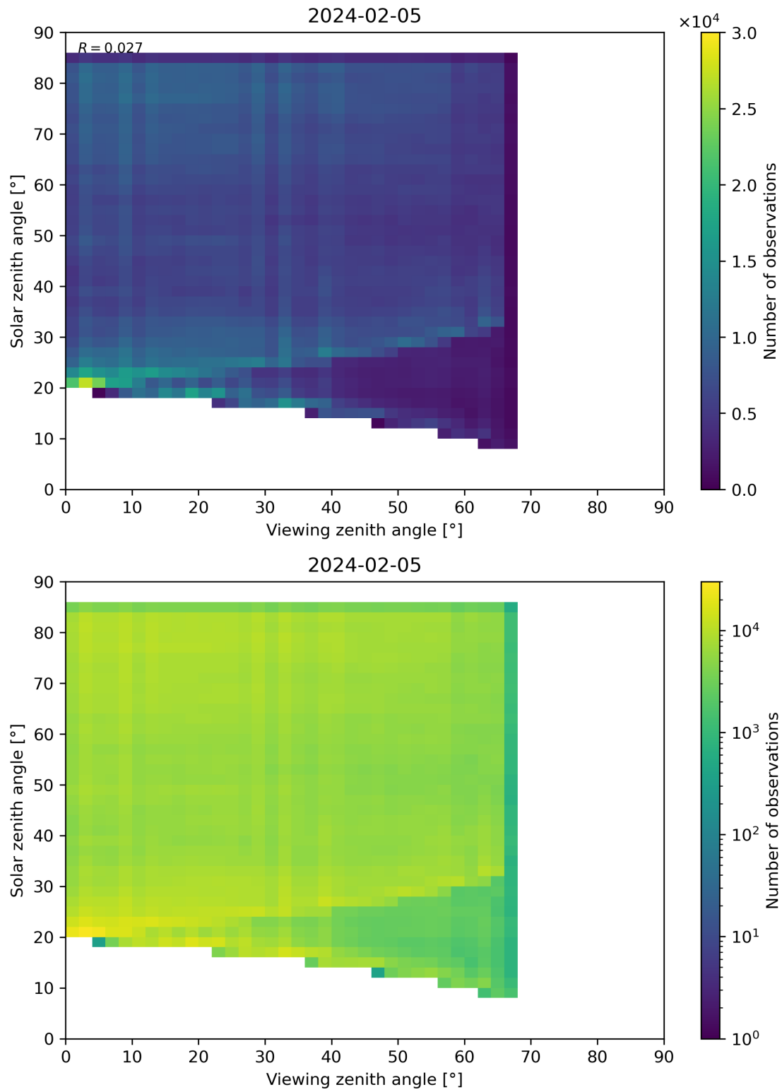
Figure 77: Scatter density plot of “Viewing zenith angle” against “Solar zenith angle” for 2024-02-04 to 2024-02-06.
