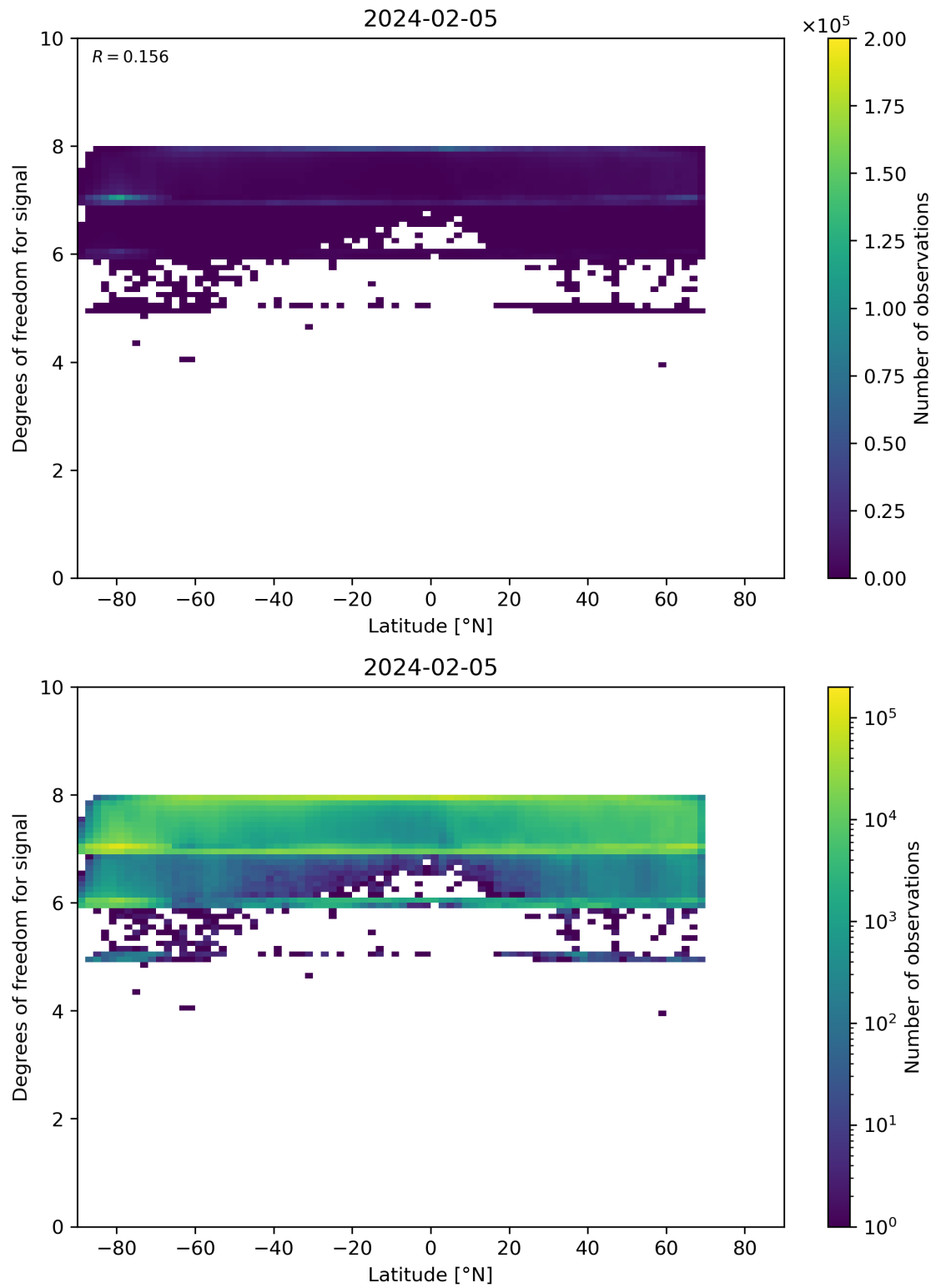
Figure 55: Scatter density plot of “Latitude” against “Degrees of freedom for signal” for 2024-02-04 to 2024-02-06.
