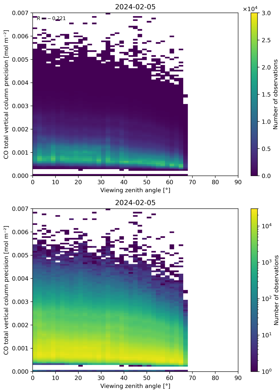
Figure 71: Scatter density plot of “Viewing zenith angle” against “CO total vertical column precision” for 2024-02-04 to 2024-02-06.
