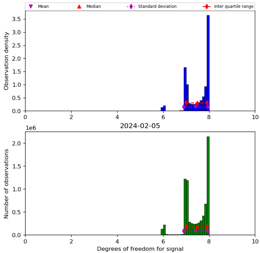
Figure 23: Histogram of “Degrees of freedom for signal” for 2024-02-04 to 2024-02-06
