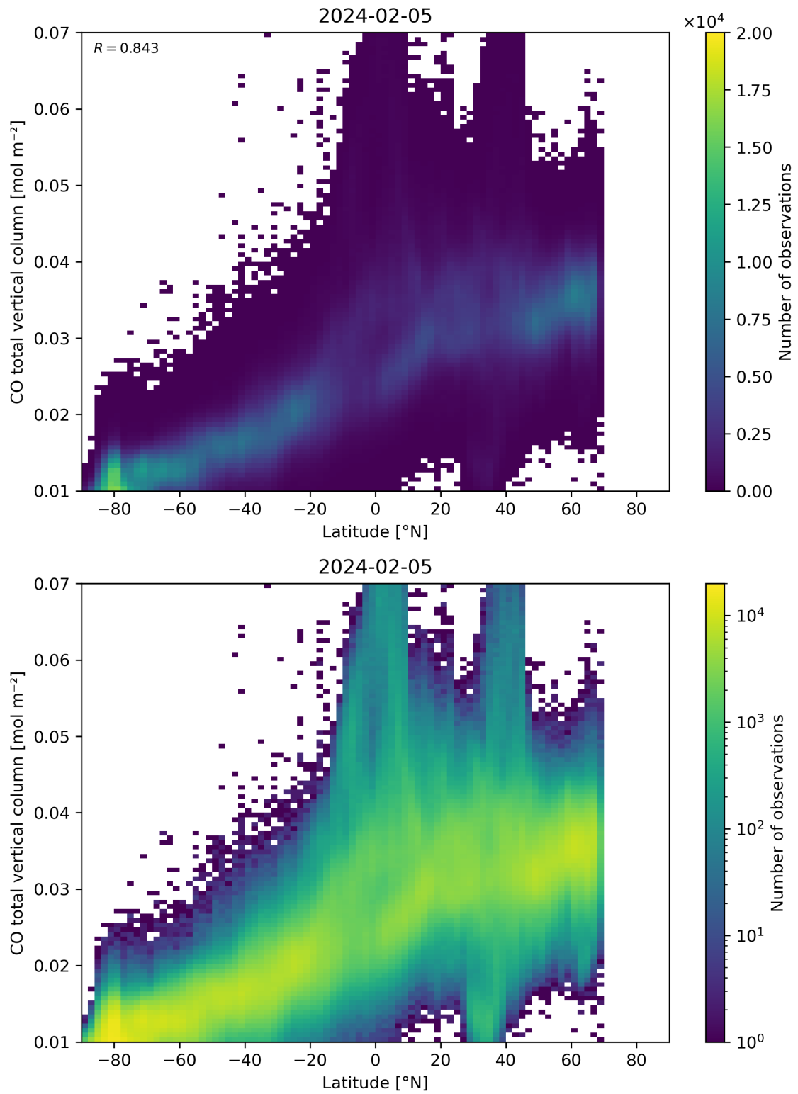
Figure 51: Scatter density plot of “Latitude” against “CO total vertical column” for 2024-02-04 to 2024-02-06.
