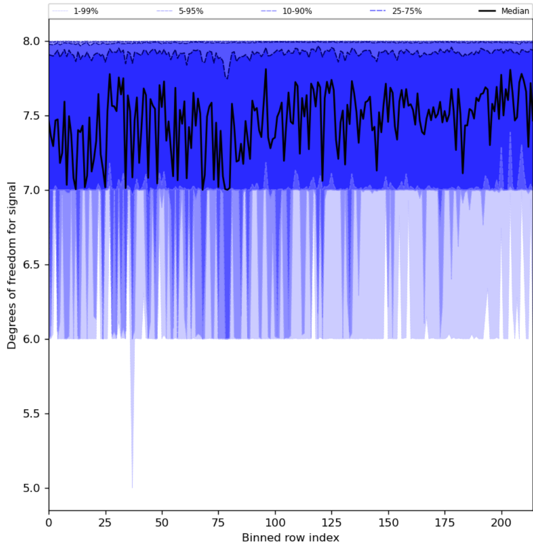
Figure 31: Along track statistics of “Degrees of freedom for signal” for 2024-02-04 to 2024-02-06
