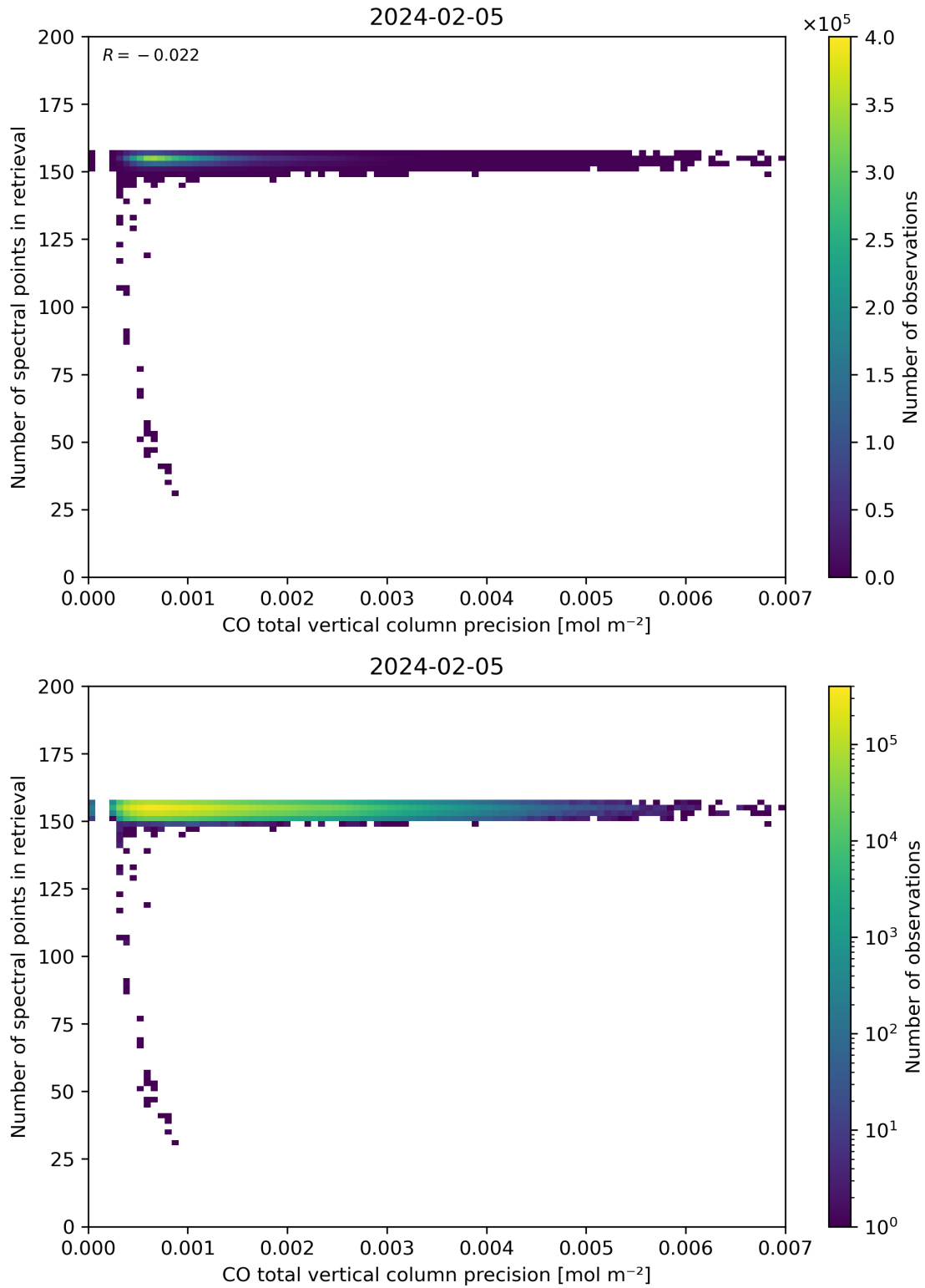
Figure 47: Scatter density plot of “CO total vertical column precision” against “Number of spectral points in retrieval” for 2024-02-04 to 2024-02-06.
