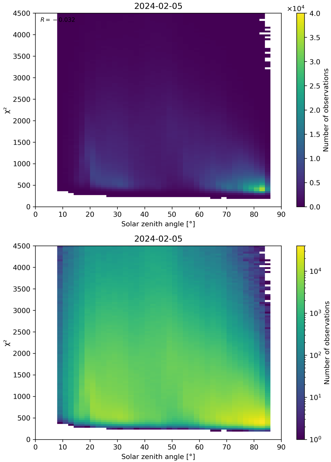
Figure 64: Scatter density plot of “Solar zenith angle” against “ \chi^2 ” for 2024-02-04 to 2024-02-06.
