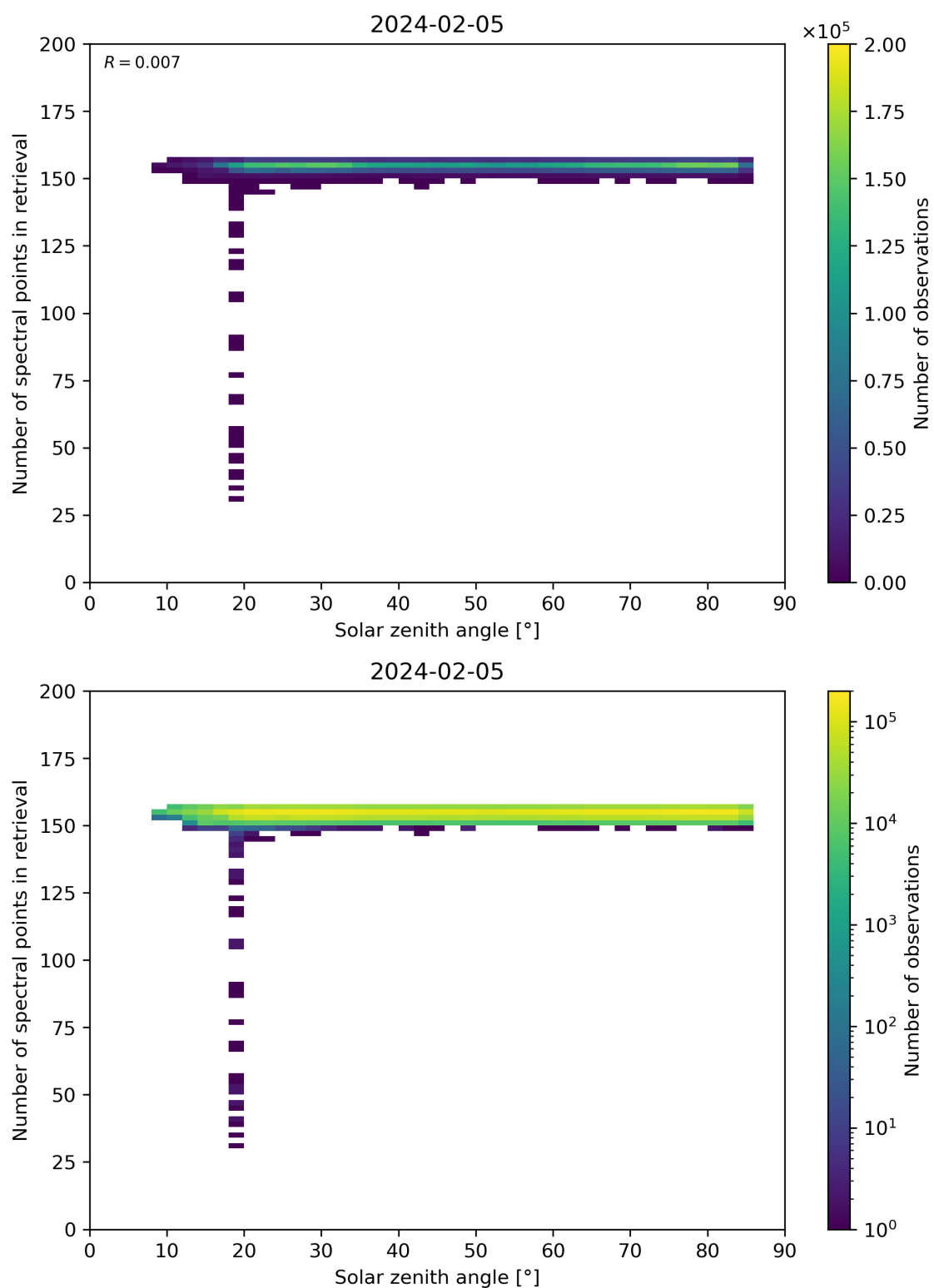
Figure 68: Scatter density plot of “Solar zenith angle” against “Number of spectral points in retrieval” for 2024-02-04 to 2024-02-06.
