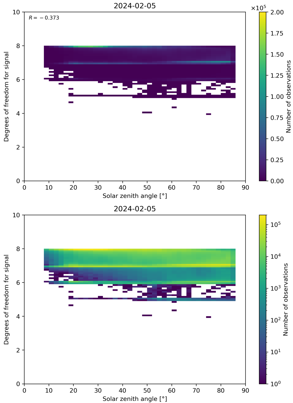
Figure 65: Scatter density plot of “Solar zenith angle” against “Degrees of freedom for signal” for 2024-02-04 to 2024-02-06.
