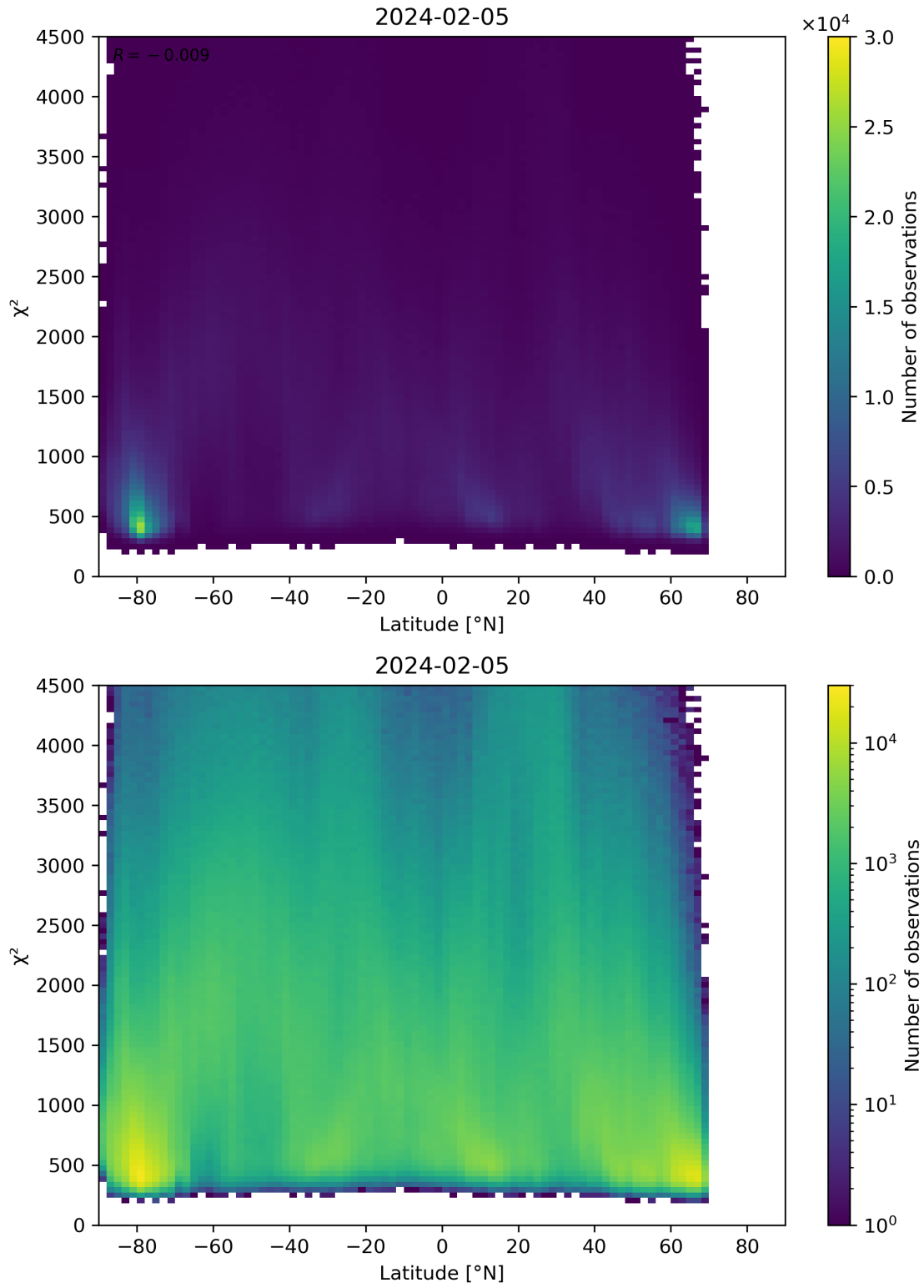
Figure 54: Scatter density plot of “Latitude” against “ \chi^2 ” for 2024-02-04 to 2024-02-06.
