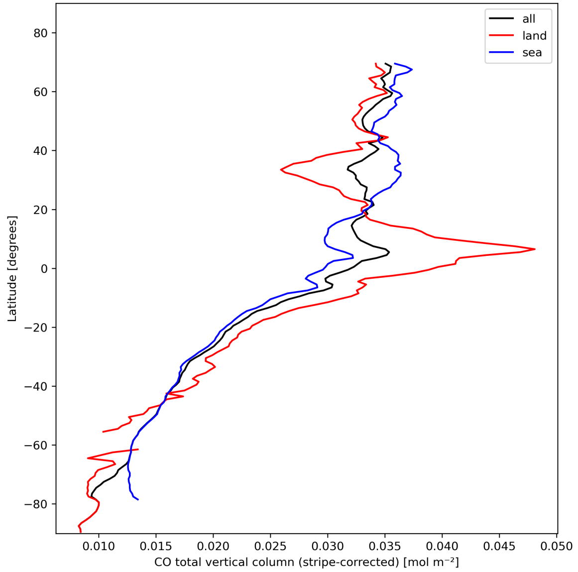
Figure 11: Zonal average of “CO total vertical column (stripe-corrected)” for 2024-02-04 to 2024-02-06.
