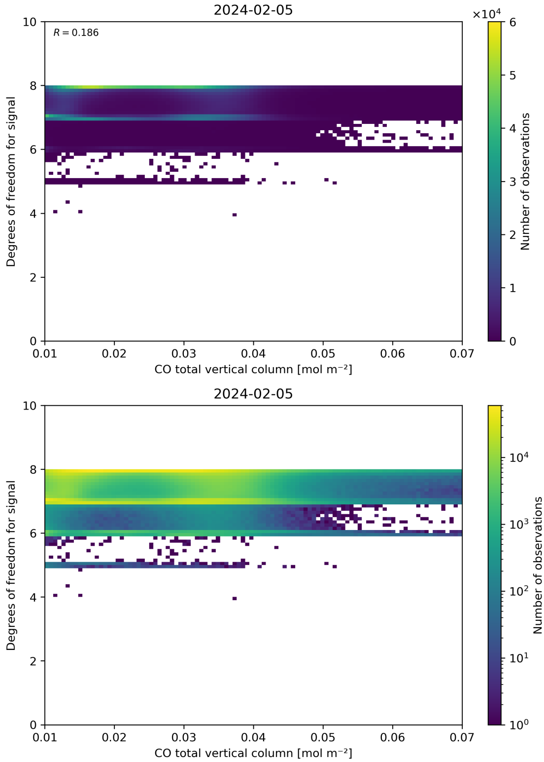
Figure 41: Scatter density plot of “CO total vertical column” against “Degrees of freedom for signal” for 2024-02-04 to 2024-02-06.
