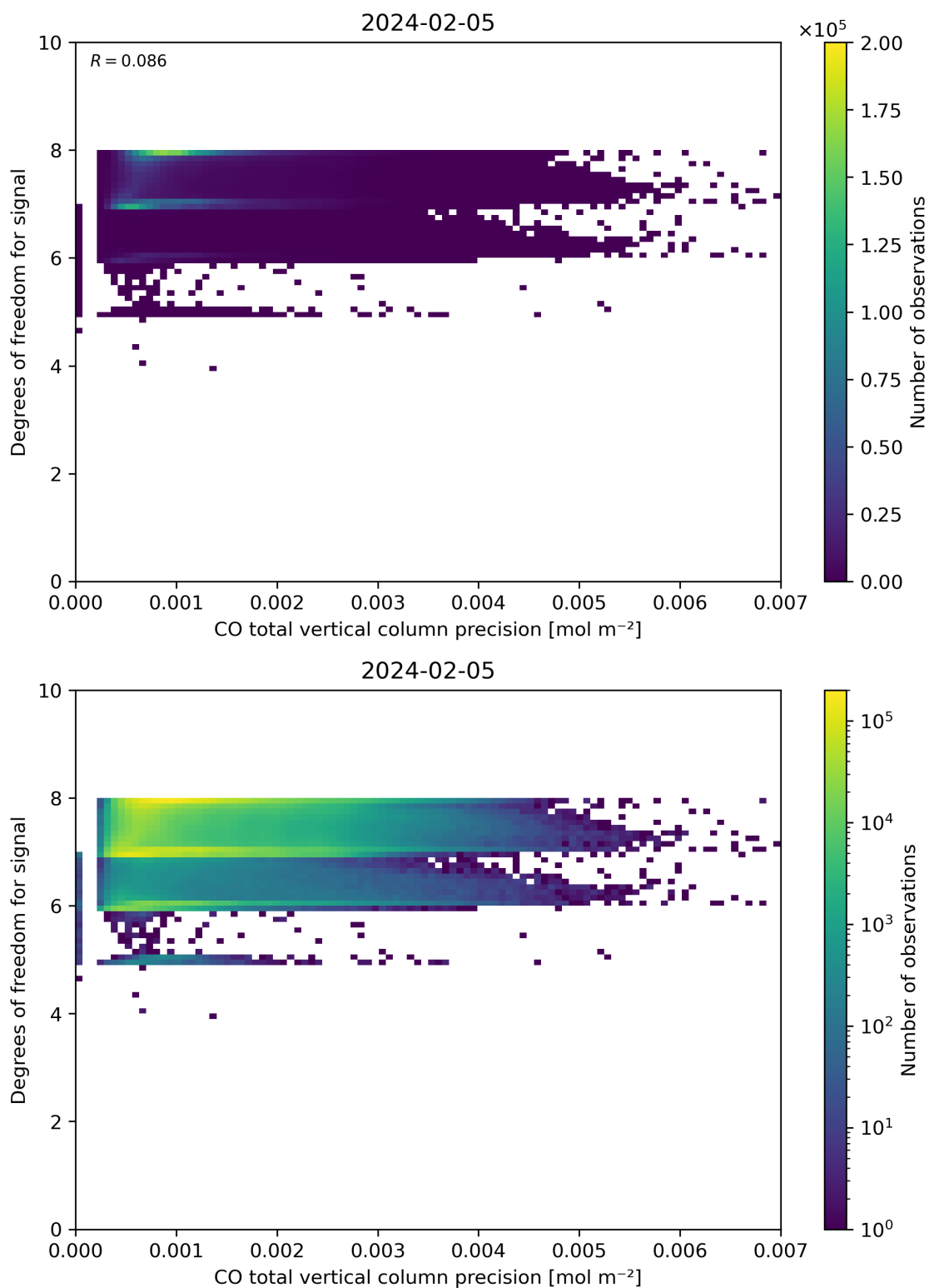
Figure 45: Scatter density plot of “CO total vertical column precision” against “Degrees of freedom for signal” for 2024-02-04 to 2024-02-06.
