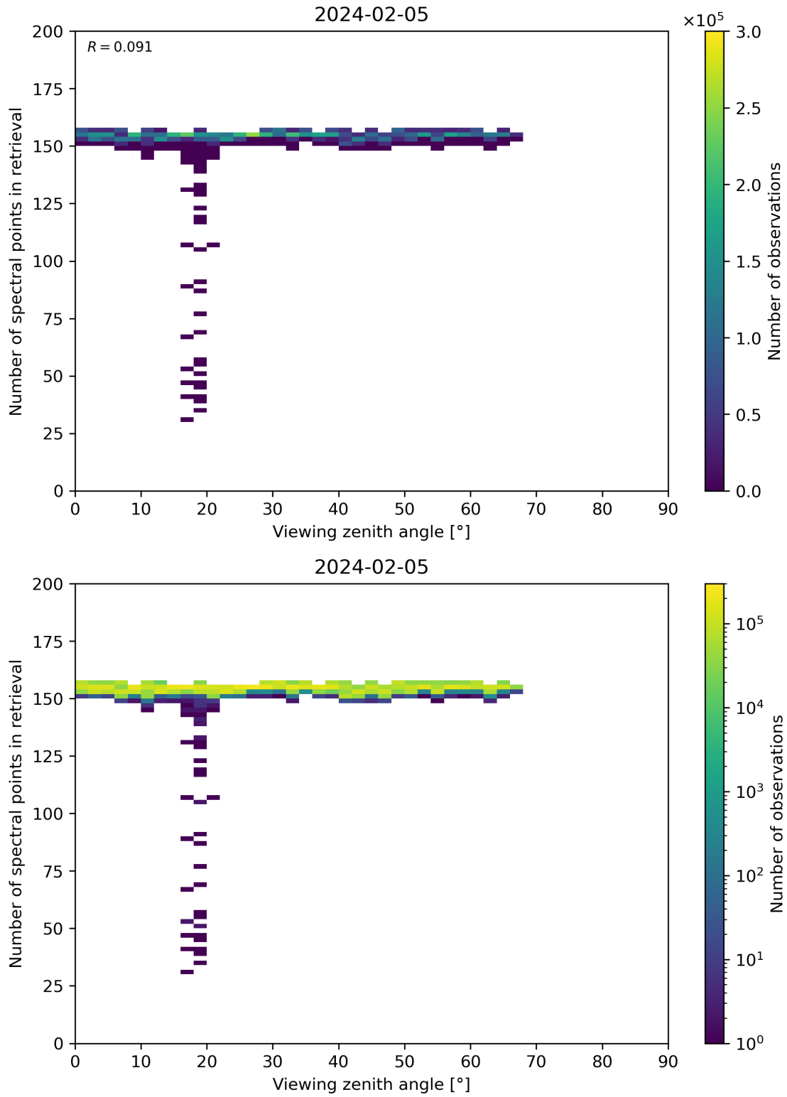
Figure 76: Scatter density plot of “Viewing zenith angle” against “Number of spectral points in retrieval” for 2024-02-04 to 2024-02-06.
