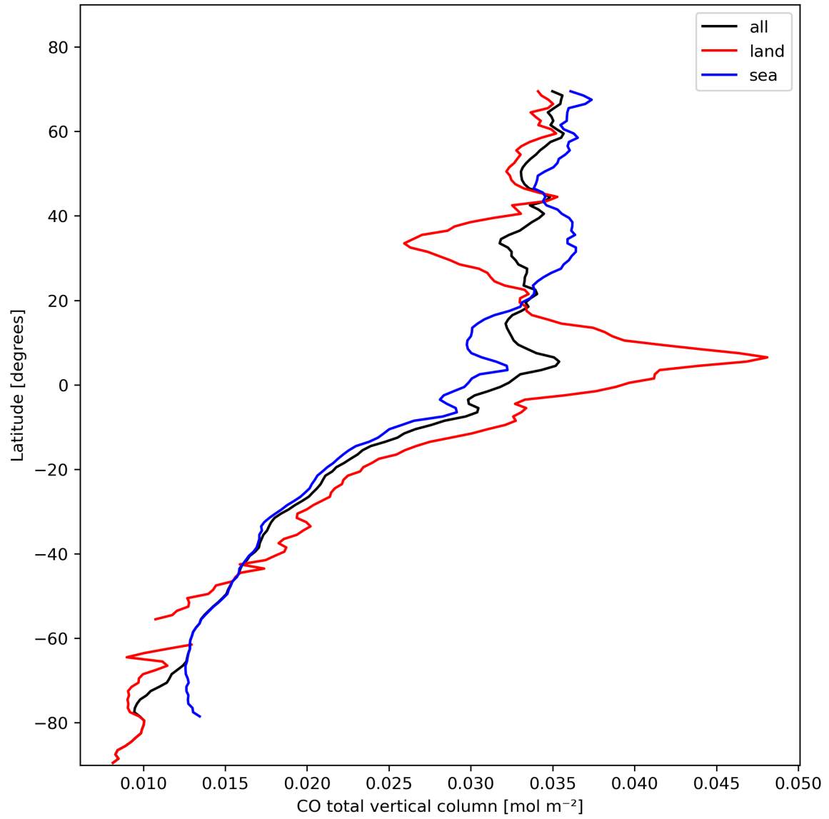
Figure 10: Zonal average of “CO total vertical column” for 2024-02-04 to 2024-02-06.
