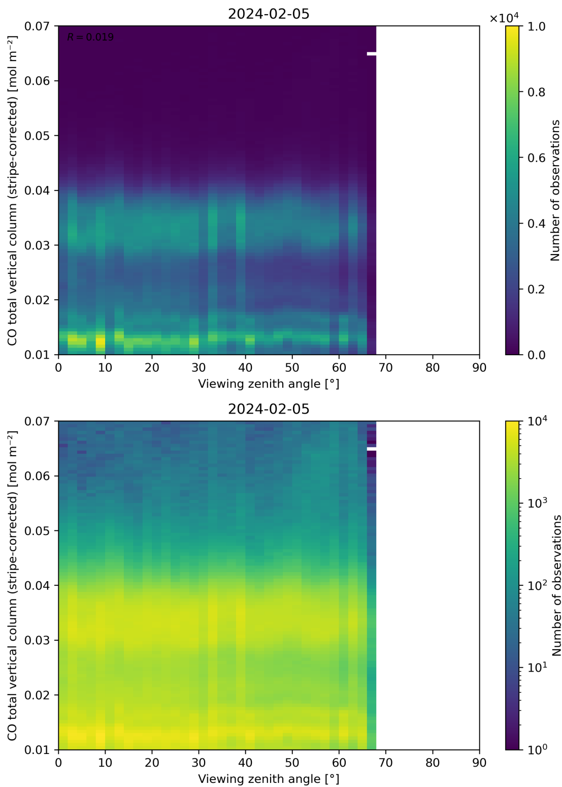
Figure 70: Scatter density plot of “Viewing zenith angle” against “CO total vertical column (stripe-corrected)” for 2024-02-04 to 2024-02-06.
