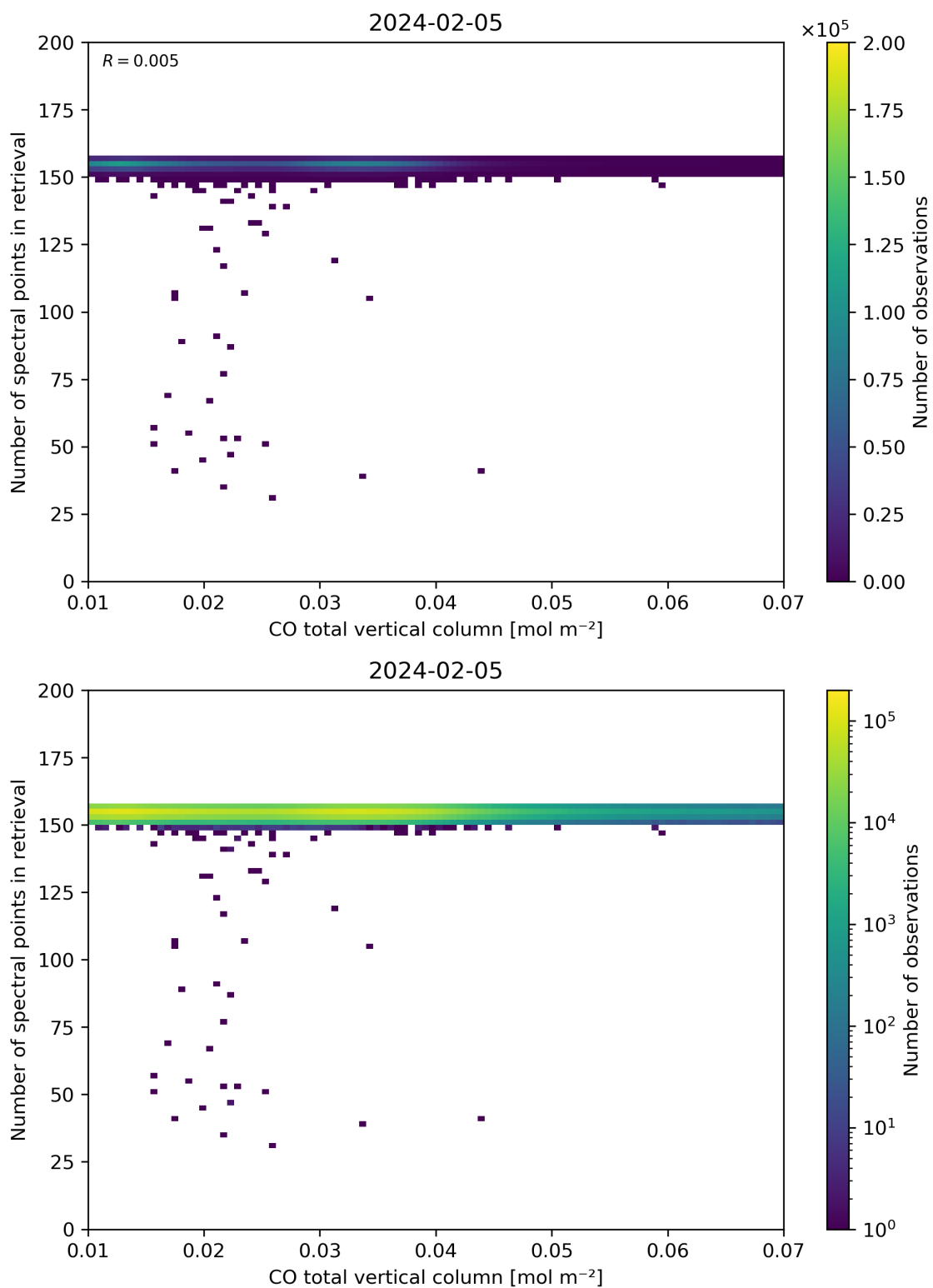
Figure 43: Scatter density plot of “CO total vertical column” against “Number of spectral points in retrieval” for 2024-02-04 to 2024-02-06.
