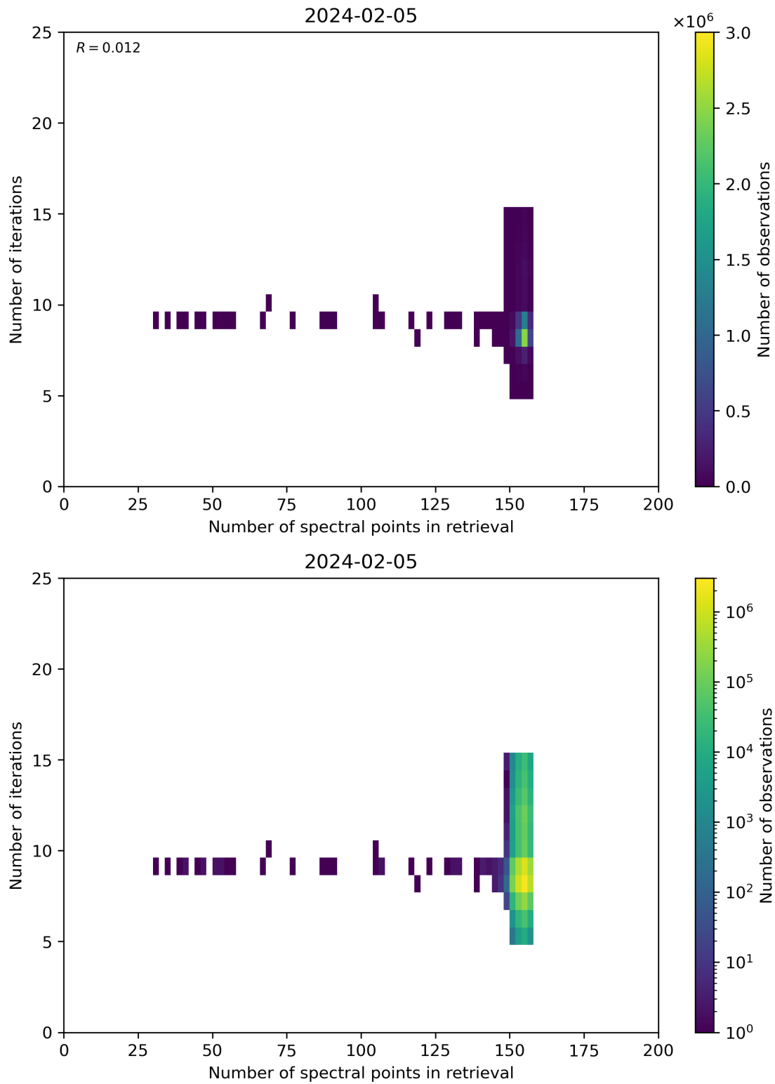
Figure 60: Scatter density plot of “Number of spectral points in retrieval” against “Number of iterations” for 2024-02-04 to 2024-02-06.
