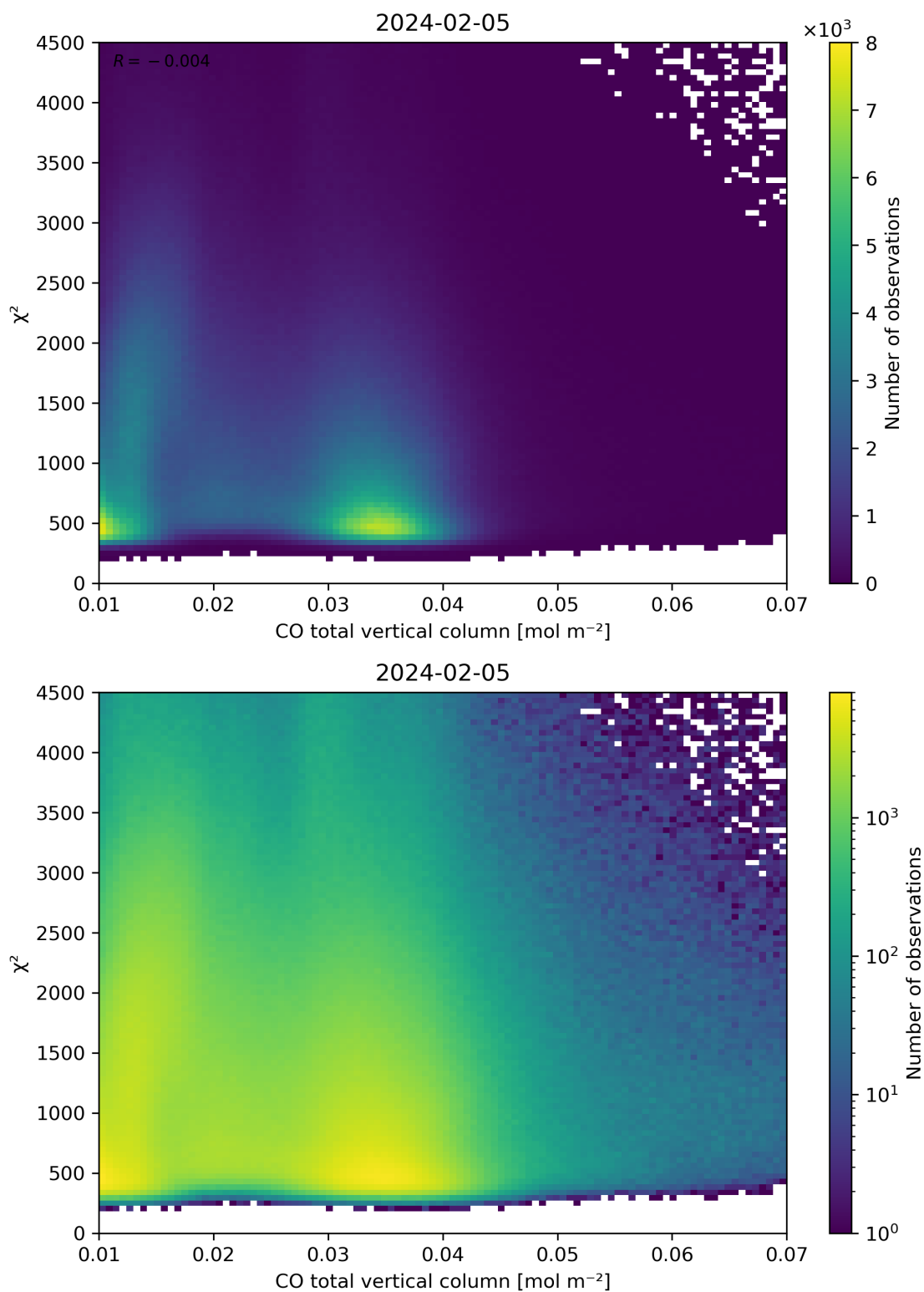
Figure 35: Scatter density plot of “CO total vertical column” against “ \chi^2 ” for 2024-02-04 to 2024-02-06.
