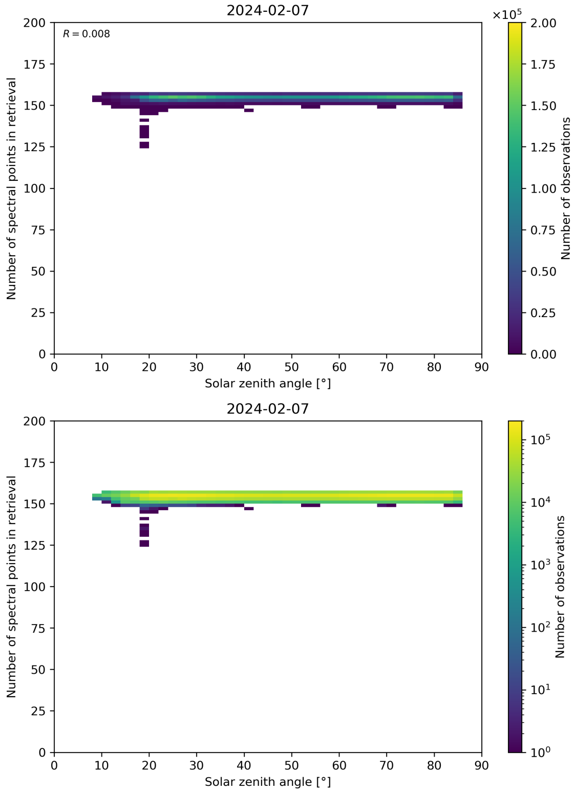
Figure 68: Scatter density plot of “Solar zenith angle” against “Number of spectral points in retrieval” for 2024-02-06 to 2024-02-08.
