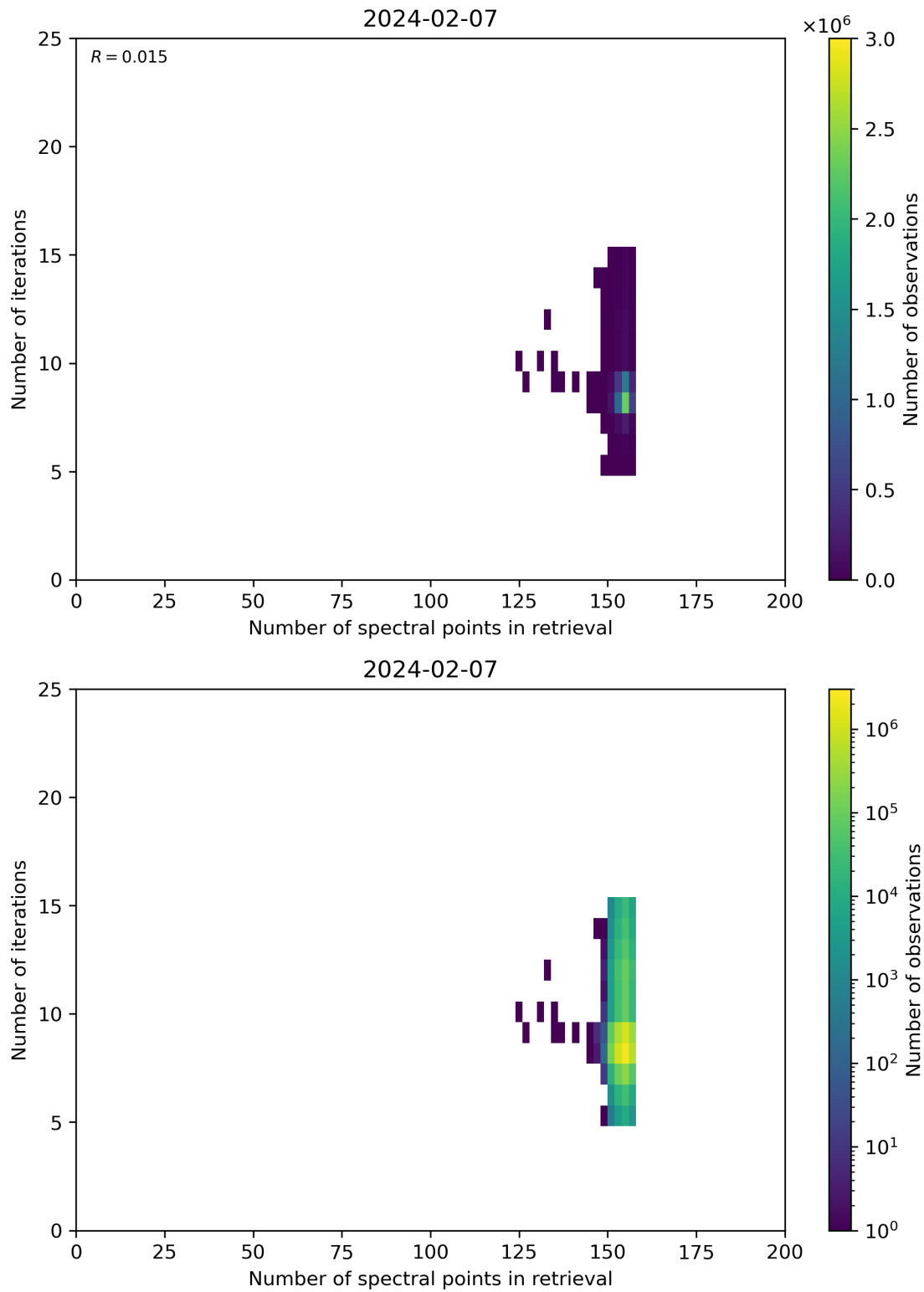
Figure 60: Scatter density plot of “Number of spectral points in retrieval” against “Number of iterations” for 2024-02-06 to 2024-02-08.
