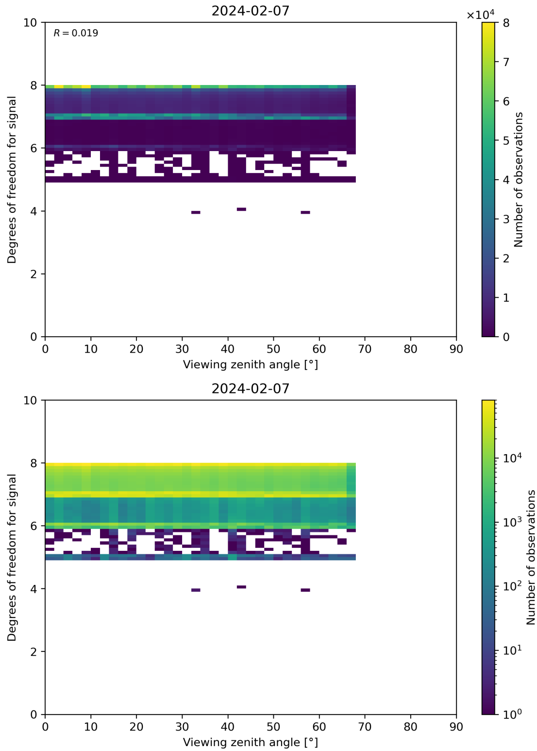
Figure 73: Scatter density plot of “Viewing zenith angle” against “Degrees of freedom for signal” for 2024-02-06 to 2024-02-08.
