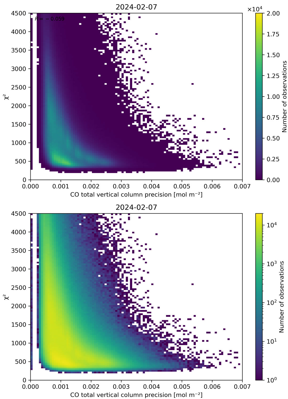
Figure 44: Scatter density plot of “CO total vertical column precision” against “ \chi^2 ” for 2024-02-06 to 2024-02-08.
