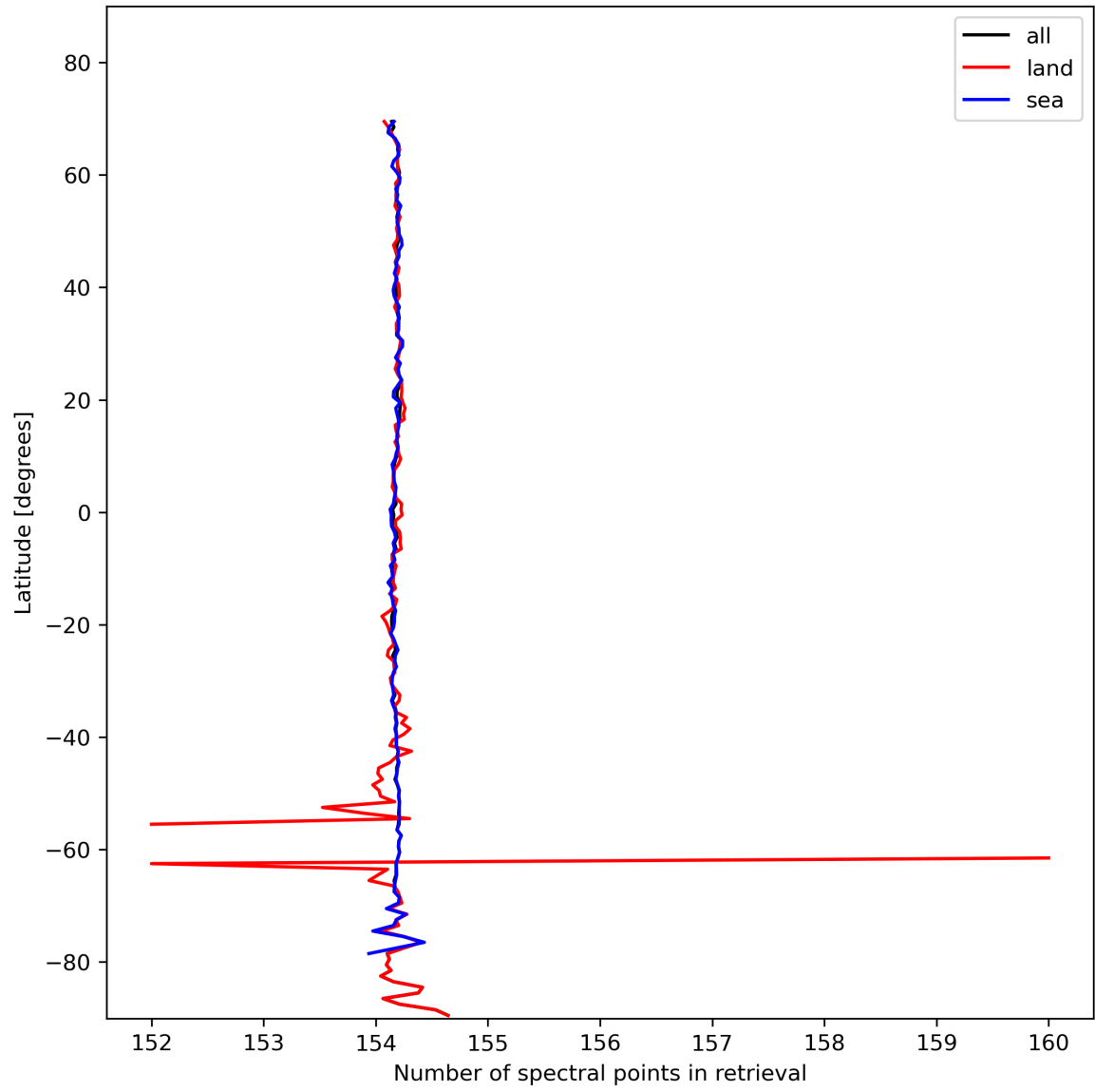
Figure 13: Zonal average of “Number of spectral points in retrieval” for 2024-02-06 to 2024-02-08.
