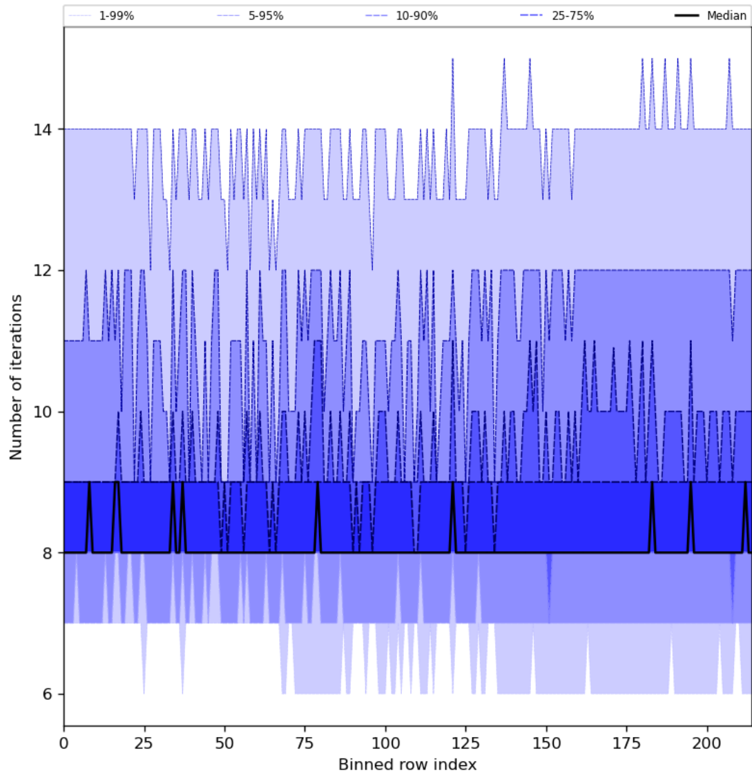
Figure 32: Along track statistics of “Number of iterations” for 2024-02-06 to 2024-02-08
