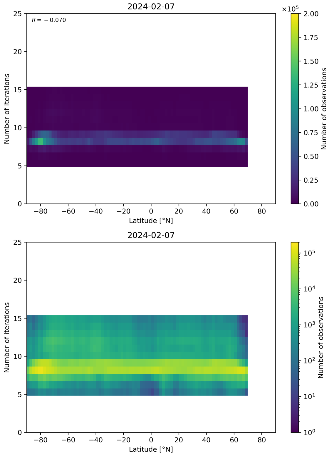
Figure 56: Scatter density plot of “Latitude” against “Number of iterations” for 2024-02-06 to 2024-02-08.
