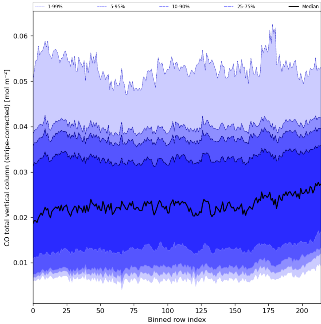
Figure 27: Along track statistics of “CO total vertical column (stripe-corrected)” for 2024-02-06 to 2024-02-08
