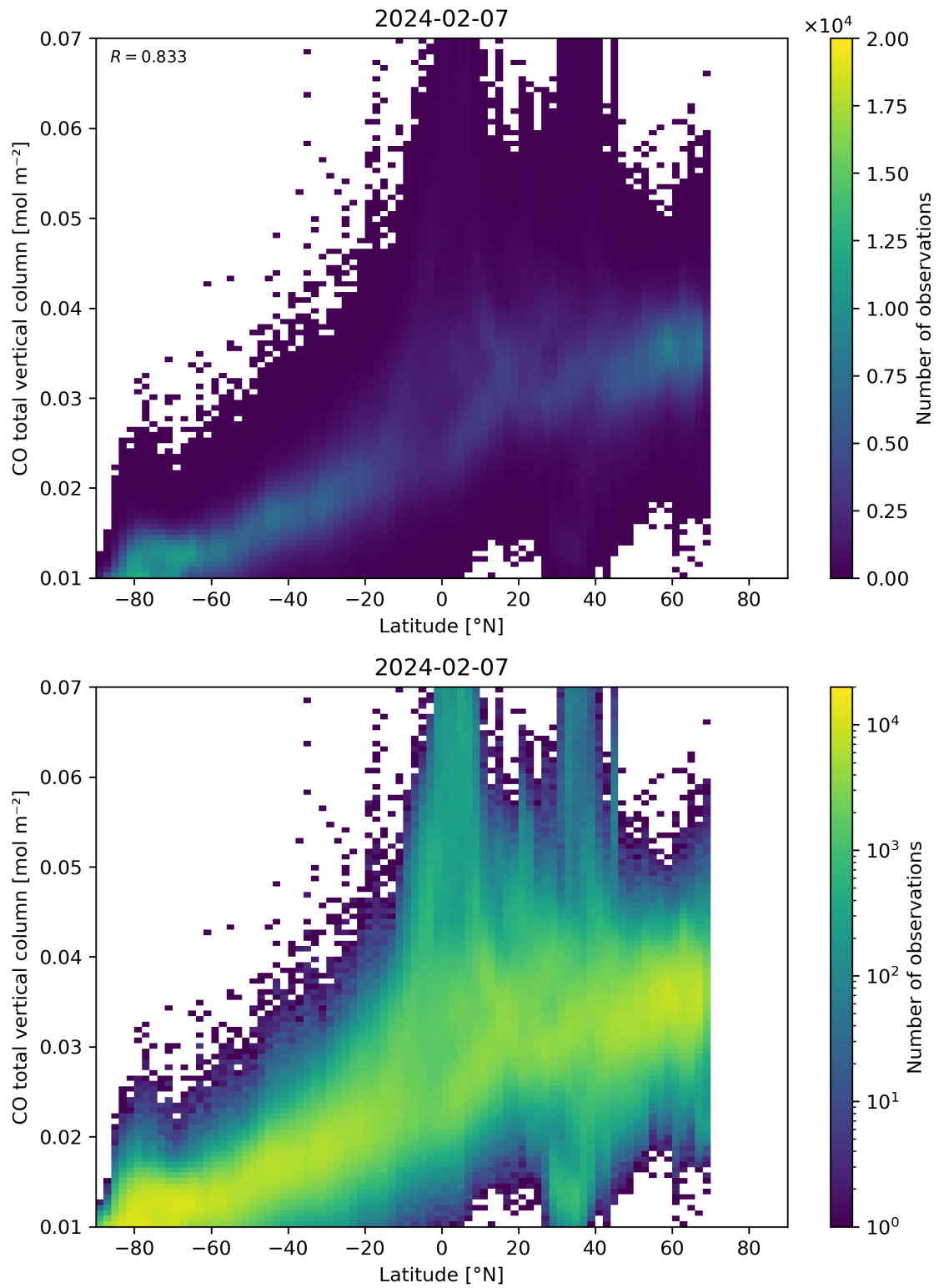
Figure 51: Scatter density plot of “Latitude” against “CO total vertical column” for 2024-02-06 to 2024-02-08.
