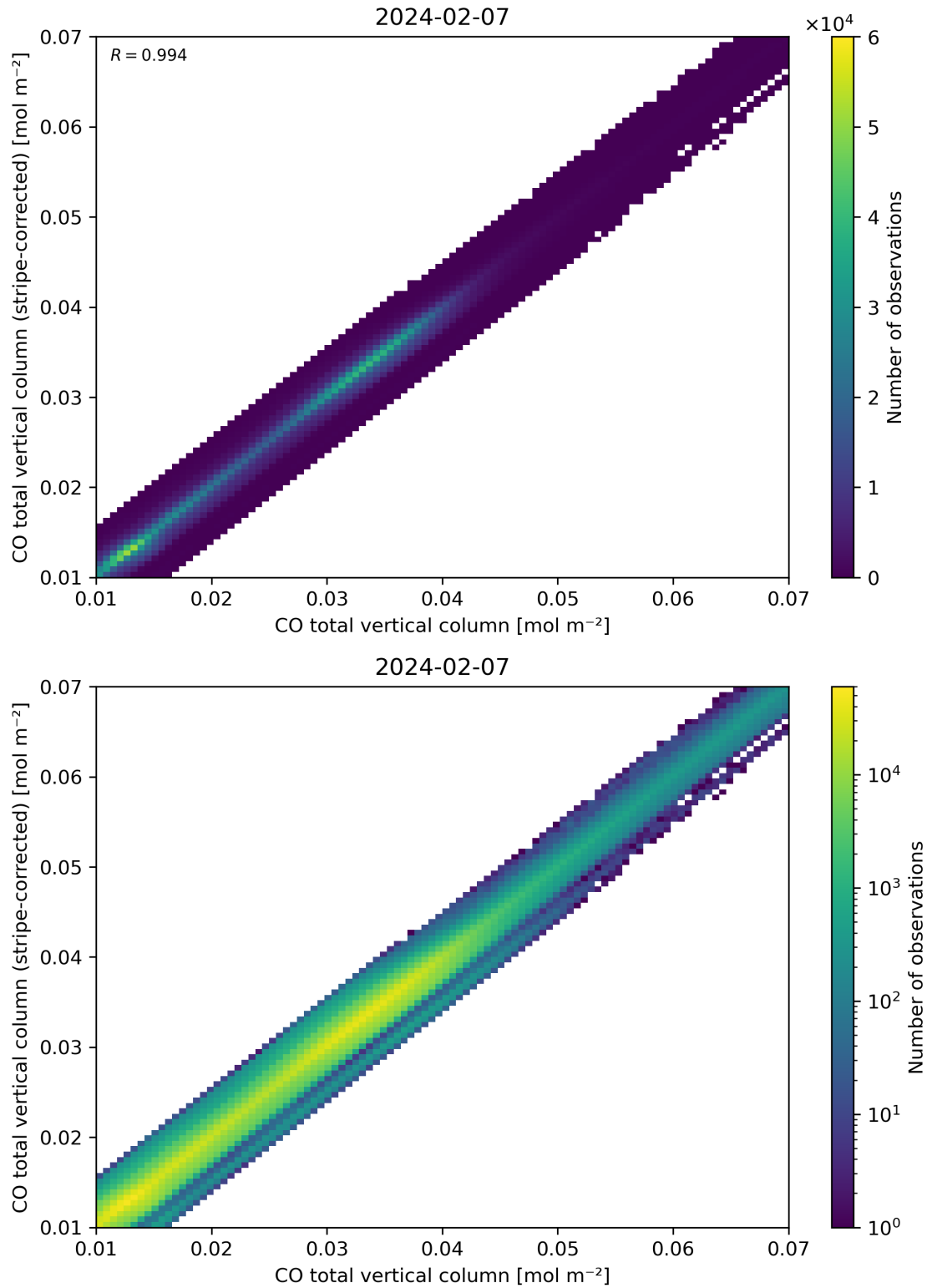
Figure 33: Scatter density plot of “CO total vertical column” against “CO total vertical column (stripe-corrected)” for 2024-02-06 to 2024-02-08.
