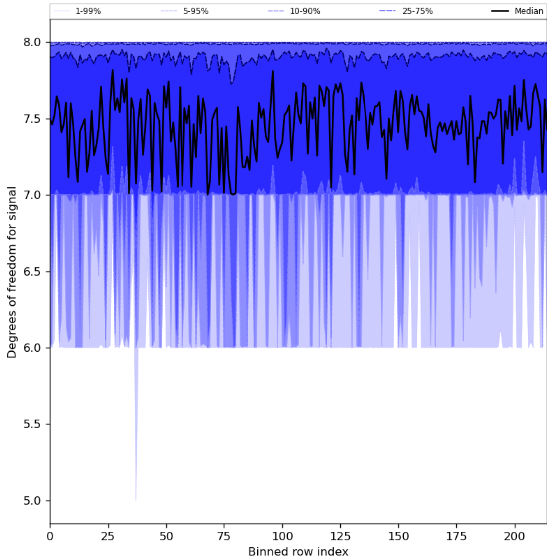
Figure 31: Along track statistics of “Degrees of freedom for signal” for 2024-02-06 to 2024-02-08
