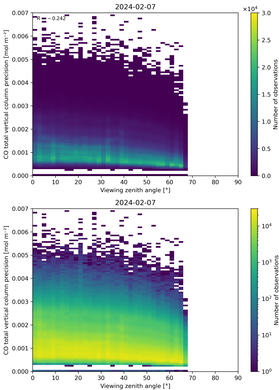
Figure 71: Scatter density plot of “Viewing zenith angle” against “CO total vertical column precision” for 2024-02-06 to 2024-02-08.
