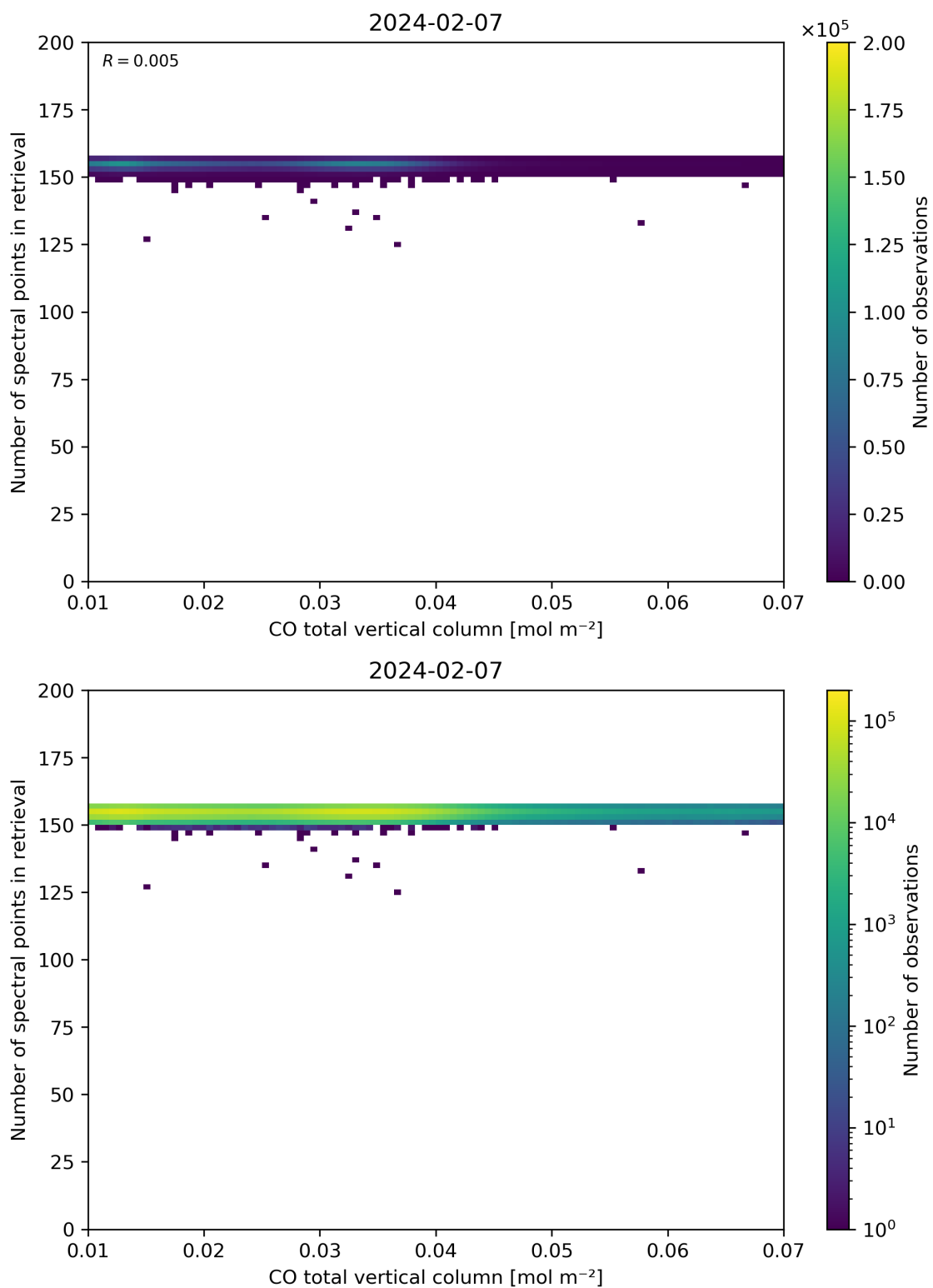
Figure 43: Scatter density plot of “CO total vertical column” against “Number of spectral points in retrieval” for 2024-02-06 to 2024-02-08.
