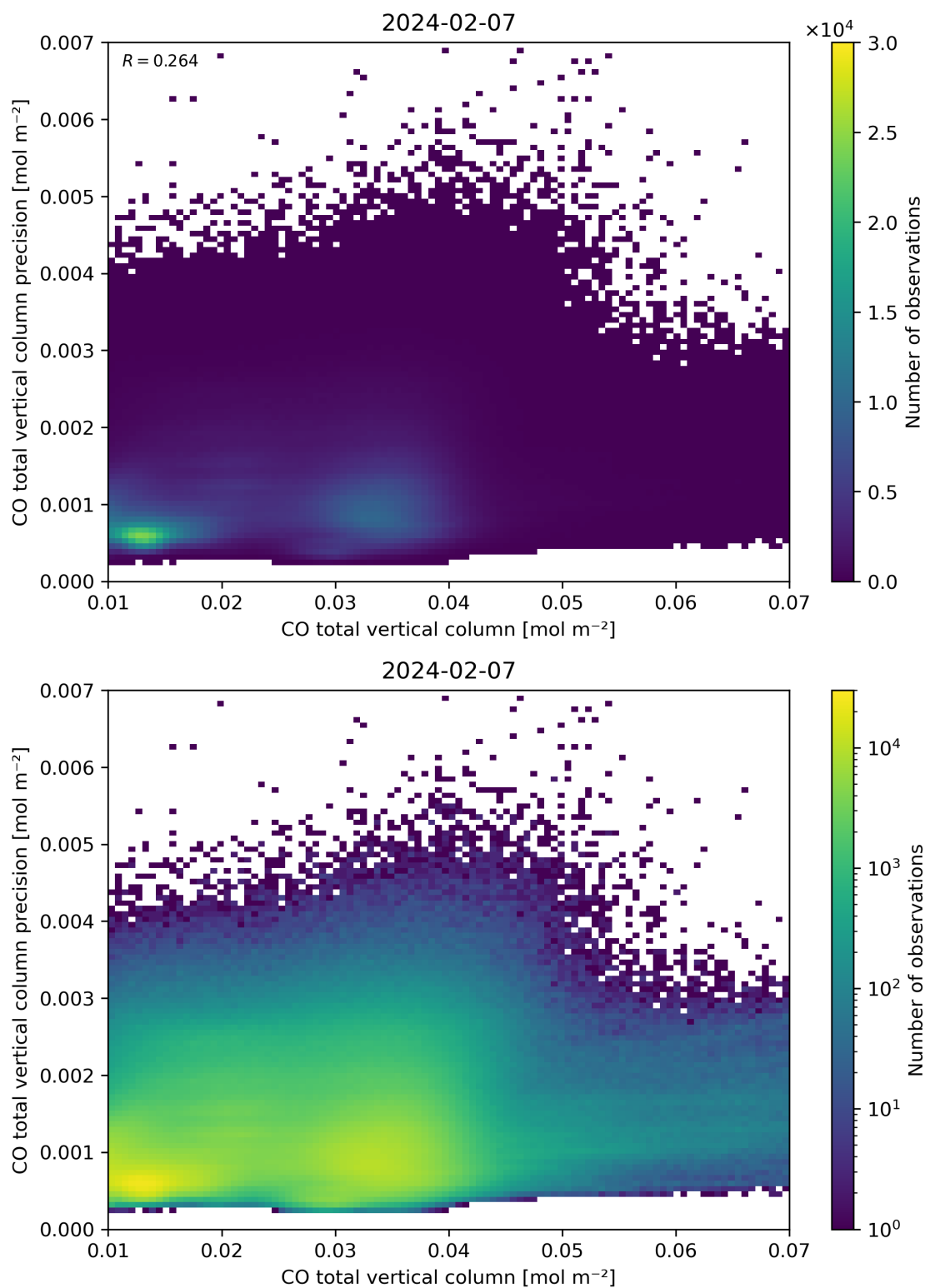
Figure 34: Scatter density plot of “CO total vertical column” against “CO total vertical column precision” for 2024-02-06 to 2024-02-08.
