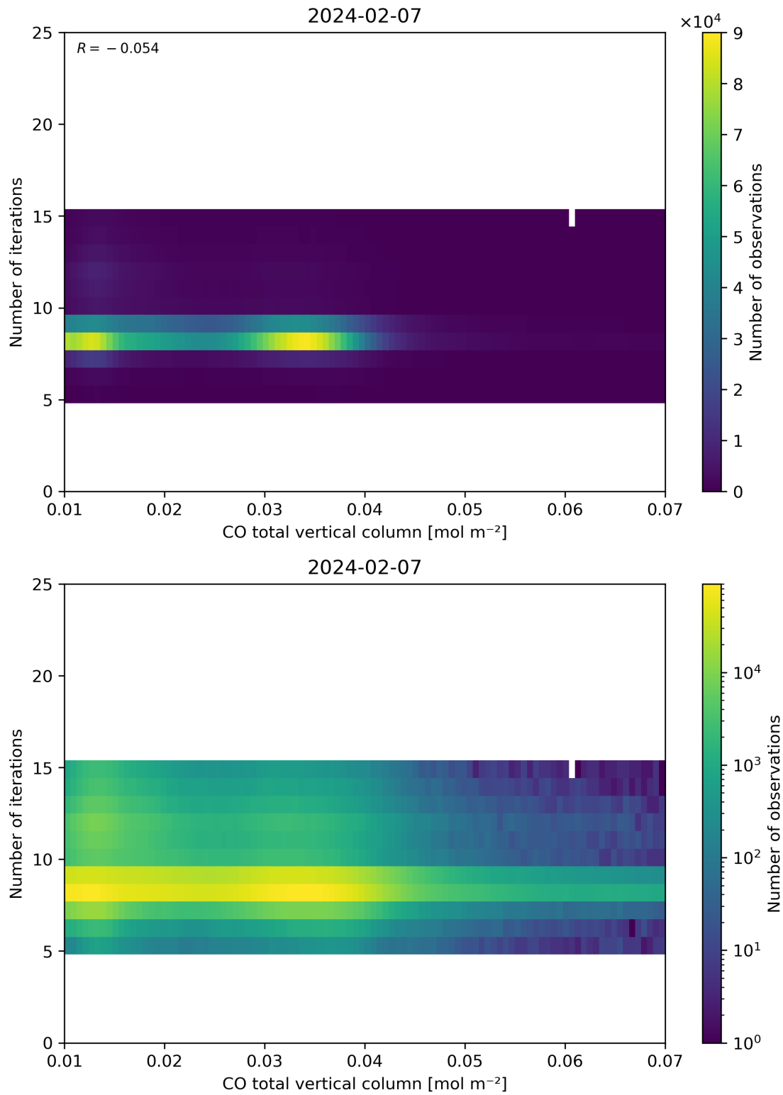
Figure 42: Scatter density plot of “CO total vertical column” against “Number of iterations” for 2024-02-06 to 2024-02-08.
