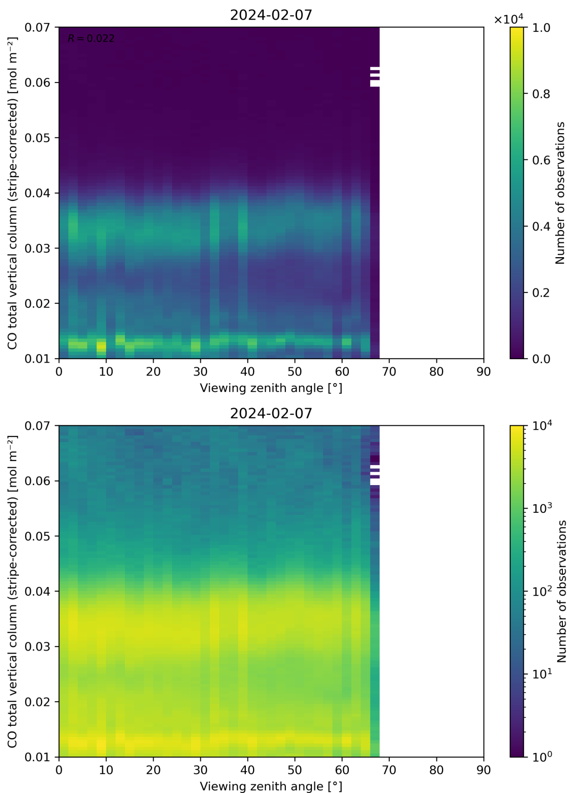
Figure 70: Scatter density plot of “Viewing zenith angle” against “CO total vertical column (stripe-corrected)” for 2024-02-06 to 2024-02-08.
