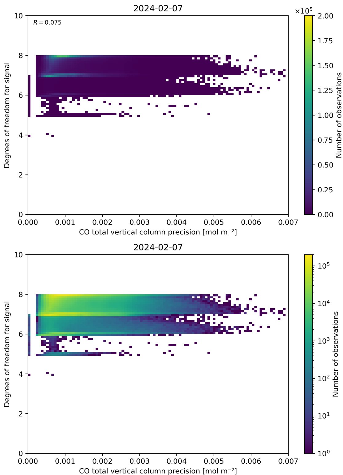
Figure 45: Scatter density plot of “CO total vertical column precision” against “Degrees of freedom for signal” for 2024-02-06 to 2024-02-08.
