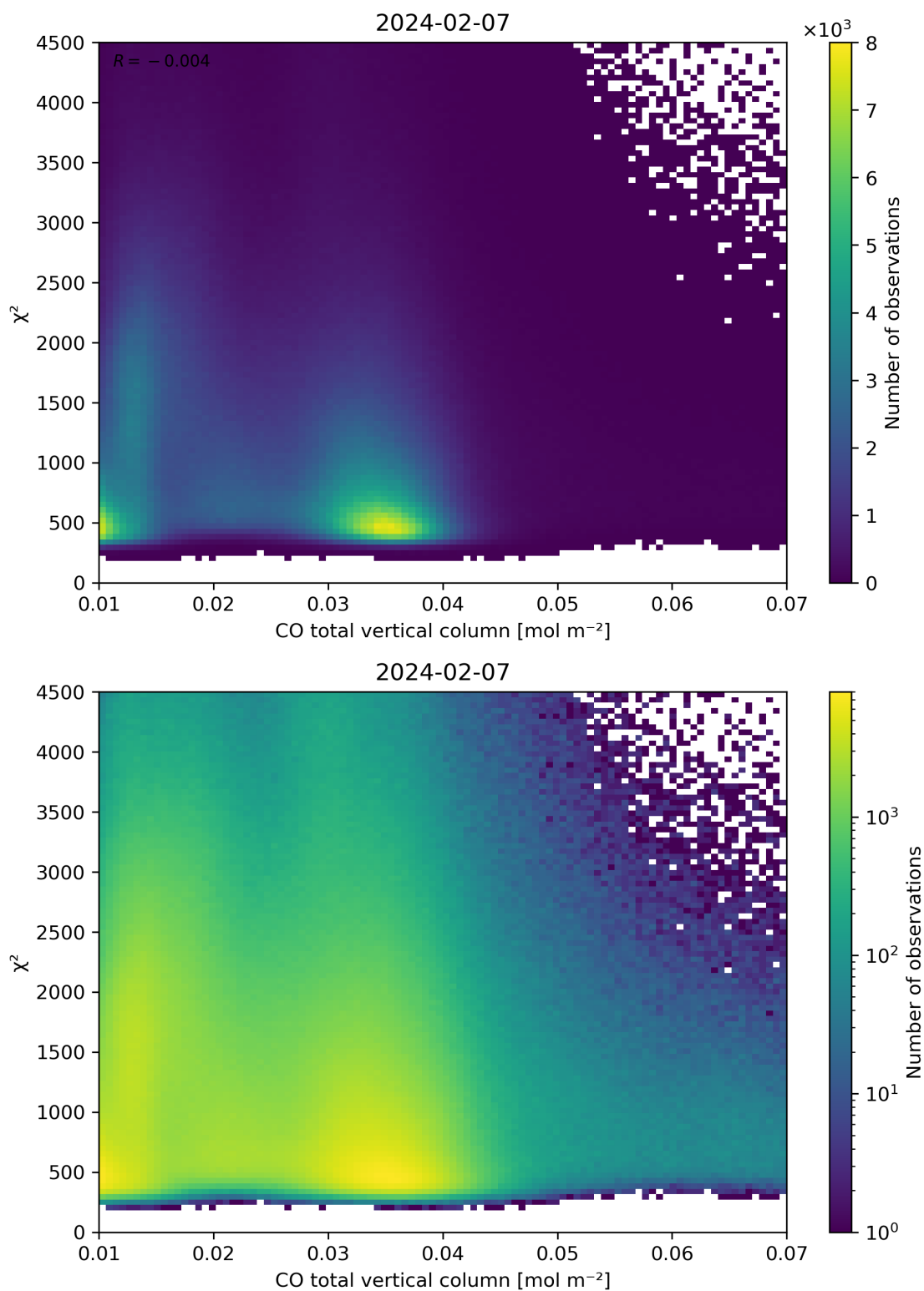
Figure 35: Scatter density plot of “CO total vertical column” against “ \chi^2 ” for 2024-02-06 to 2024-02-08.
