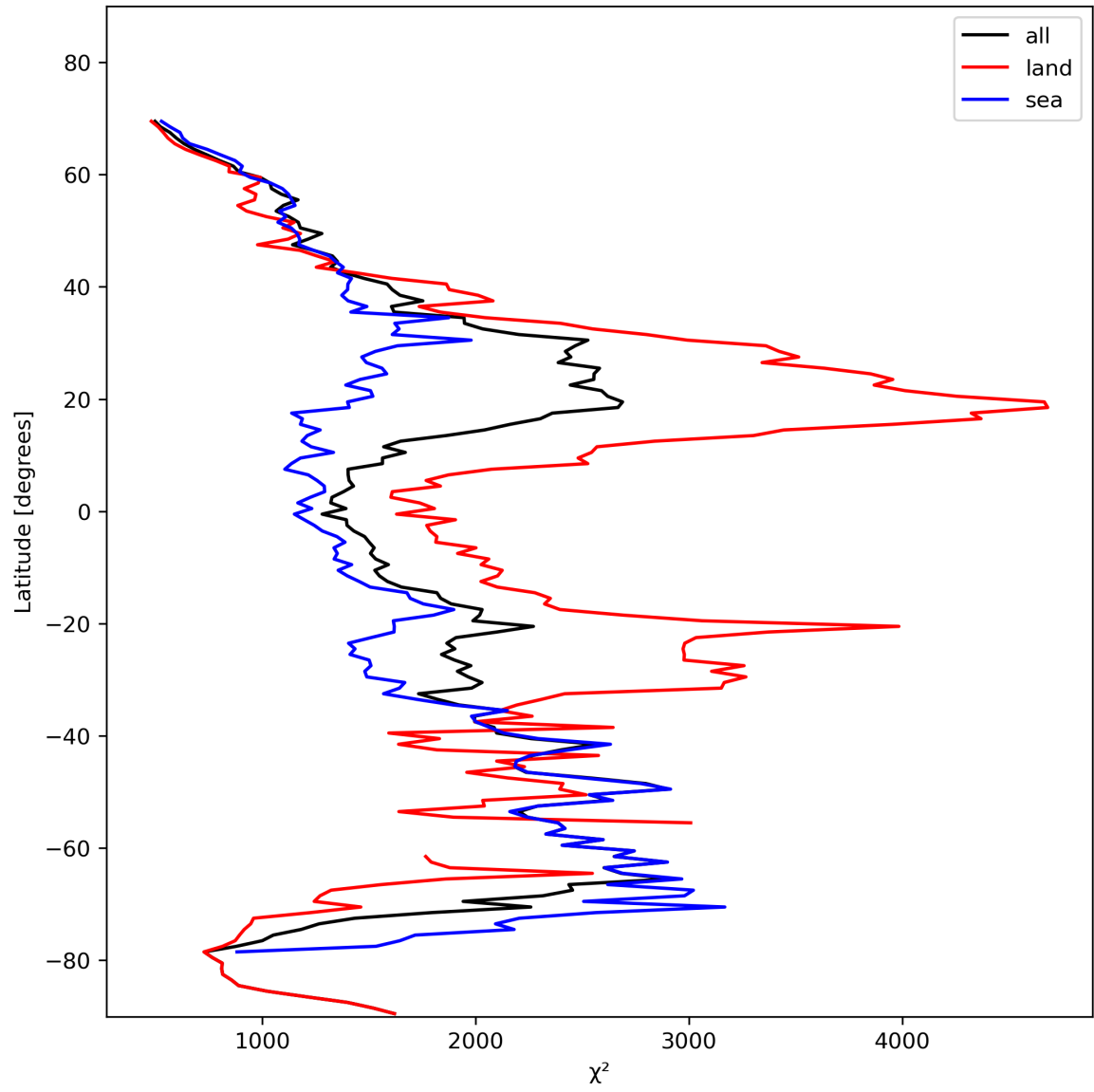
Figure 14: Zonal average of “ \chi^2 ” for 2024-02-06 to 2024-02-08.
