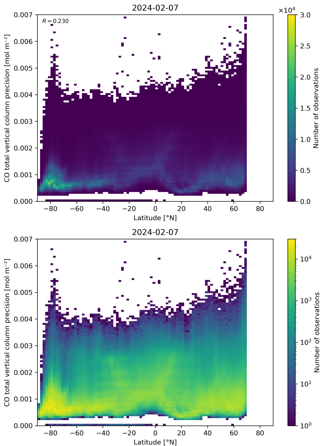
Figure 53: Scatter density plot of “Latitude” against “CO total vertical column precision” for 2024-02-06 to 2024-02-08.
