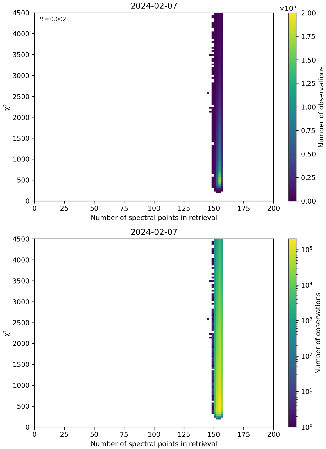
Figure 58: Scatter density plot of “Number of spectral points in retrieval” against “ \chi^2 ” for 2024-02-06 to 2024-02-08.
