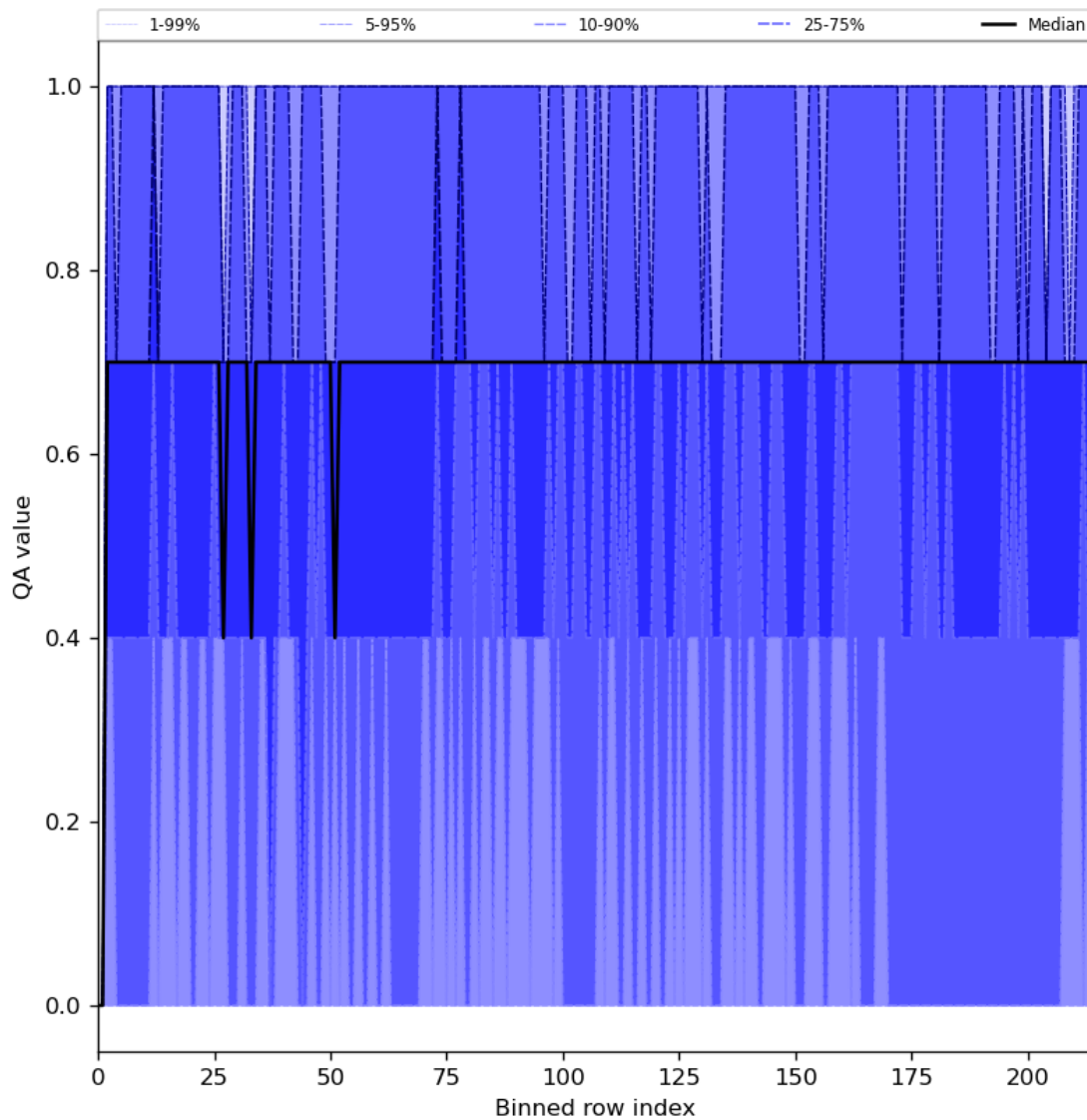
Figure 25: Along track statistics of “QA value” for 2024-02-06 to 2024-02-08
