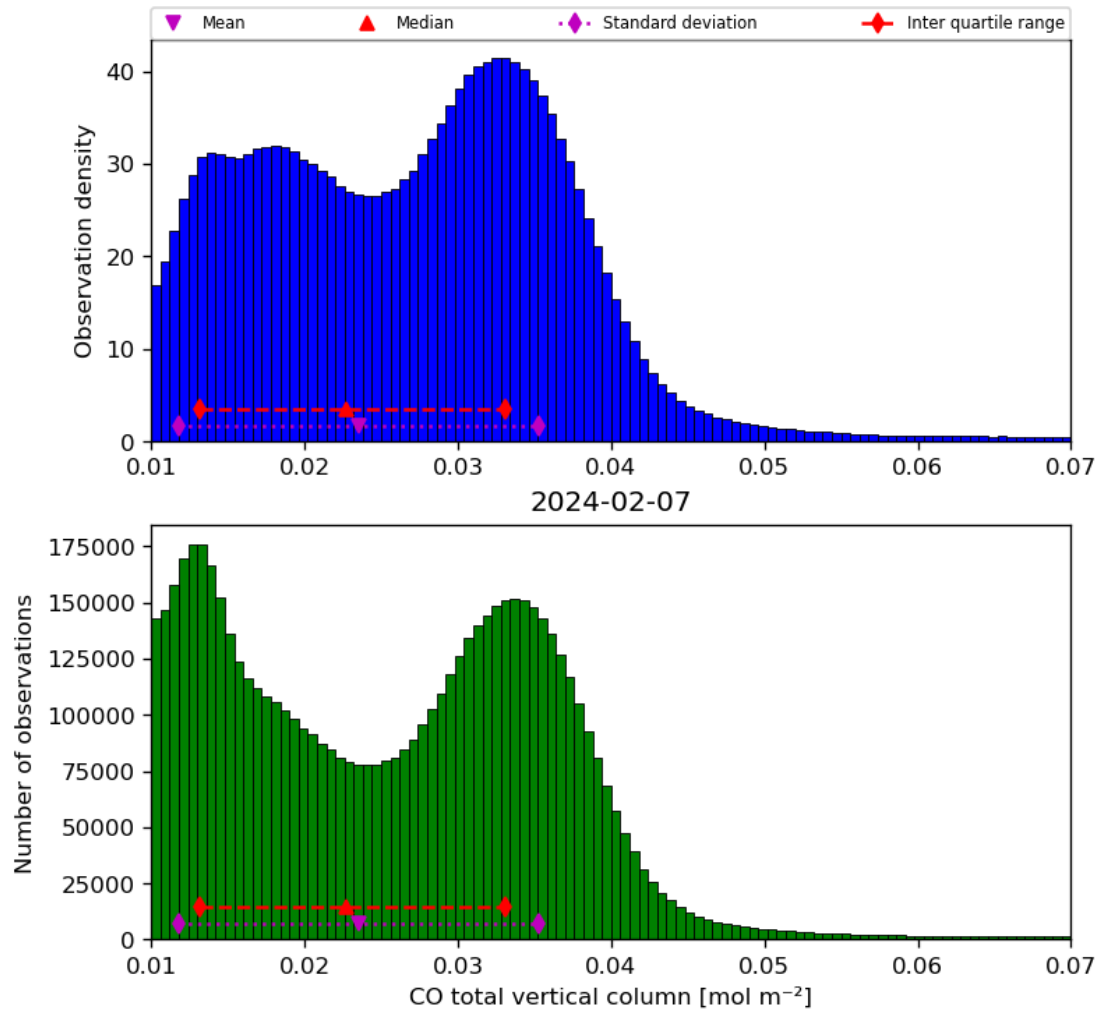
Figure 18: Histogram of “CO total vertical column” for 2024-02-06 to 2024-02-08
