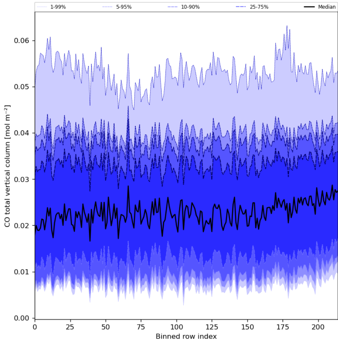
Figure 26: Along track statistics of “CO total vertical column” for 2024-02-06 to 2024-02-08
