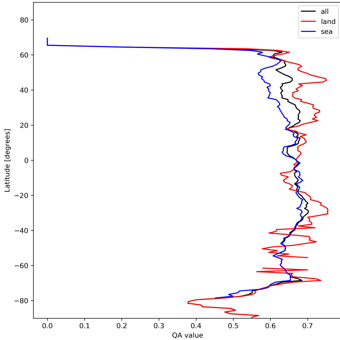
Figure 9: Zonal average of “QA value” for 2024-02-06 to 2024-02-08.
