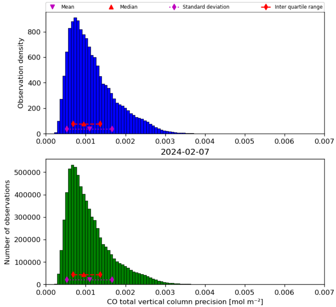
Figure 20: Histogram of “CO total vertical column precision” for 2024-02-06 to 2024-02-08
