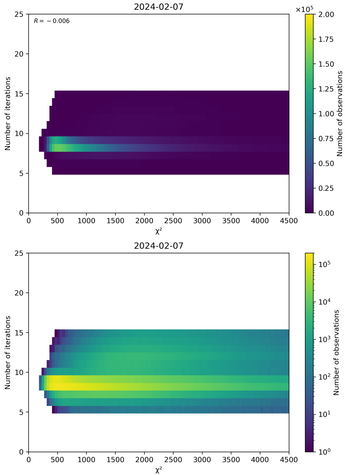
Figure 49: Scatter density plot of “ \chi^2 ” against “Number of iterations” for 2024-02-06 to 2024-02-08.
