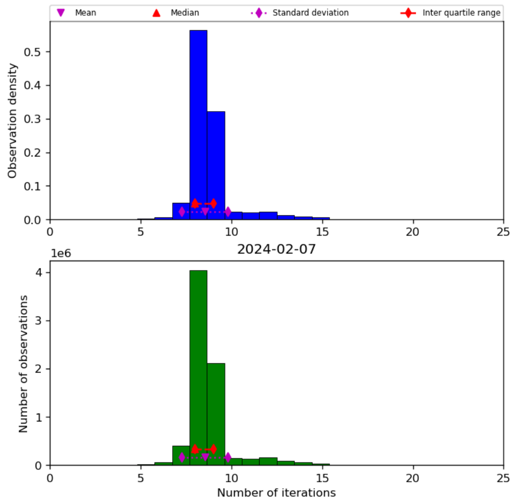
Figure 24: Histogram of “Number of iterations” for 2024-02-06 to 2024-02-08
