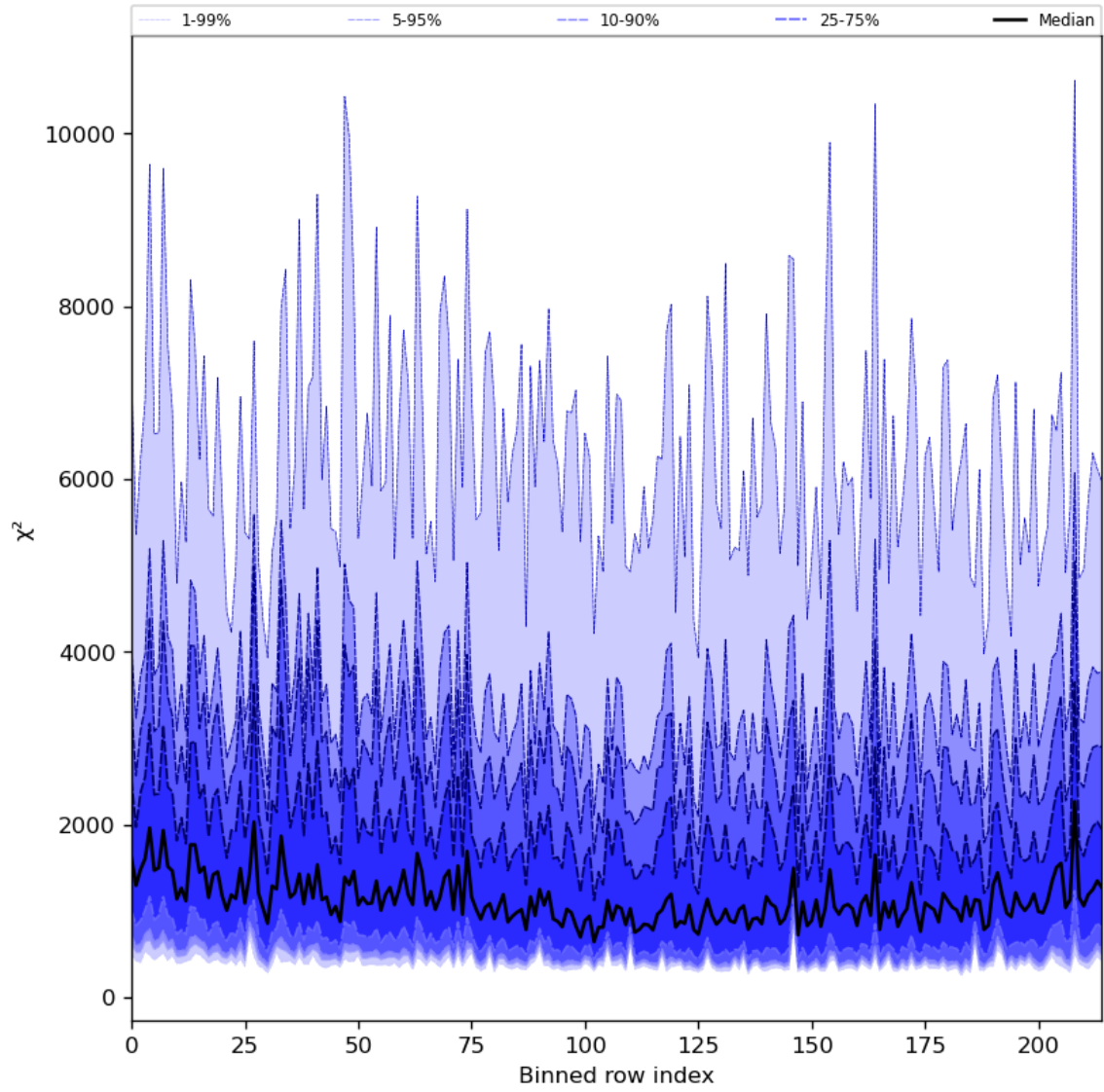
Figure 30: Along track statistics of “ \chi^2 ” for 2024-02-06 to 2024-02-08
