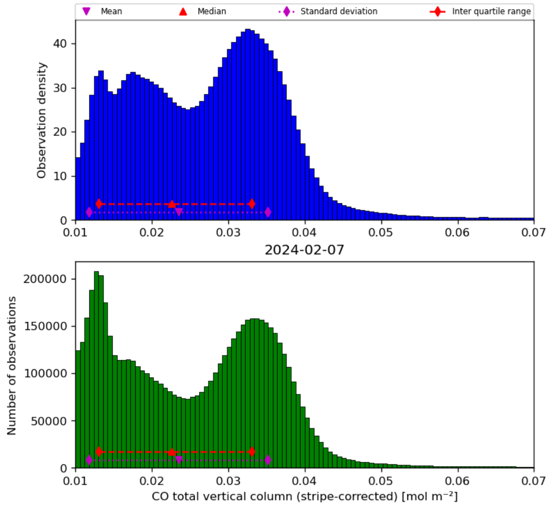
Figure 19: Histogram of “CO total vertical column (stripe-corrected)” for 2024-02-06 to 2024-02-08
