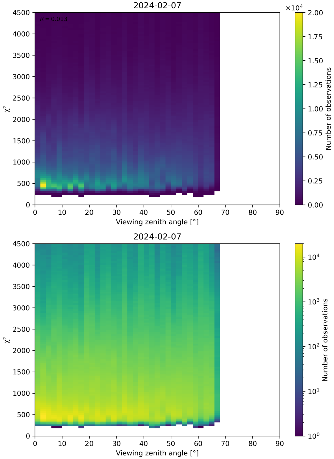
Figure 72: Scatter density plot of “Viewing zenith angle” against “ \chi^2 ” for 2024-02-06 to 2024-02-08.
