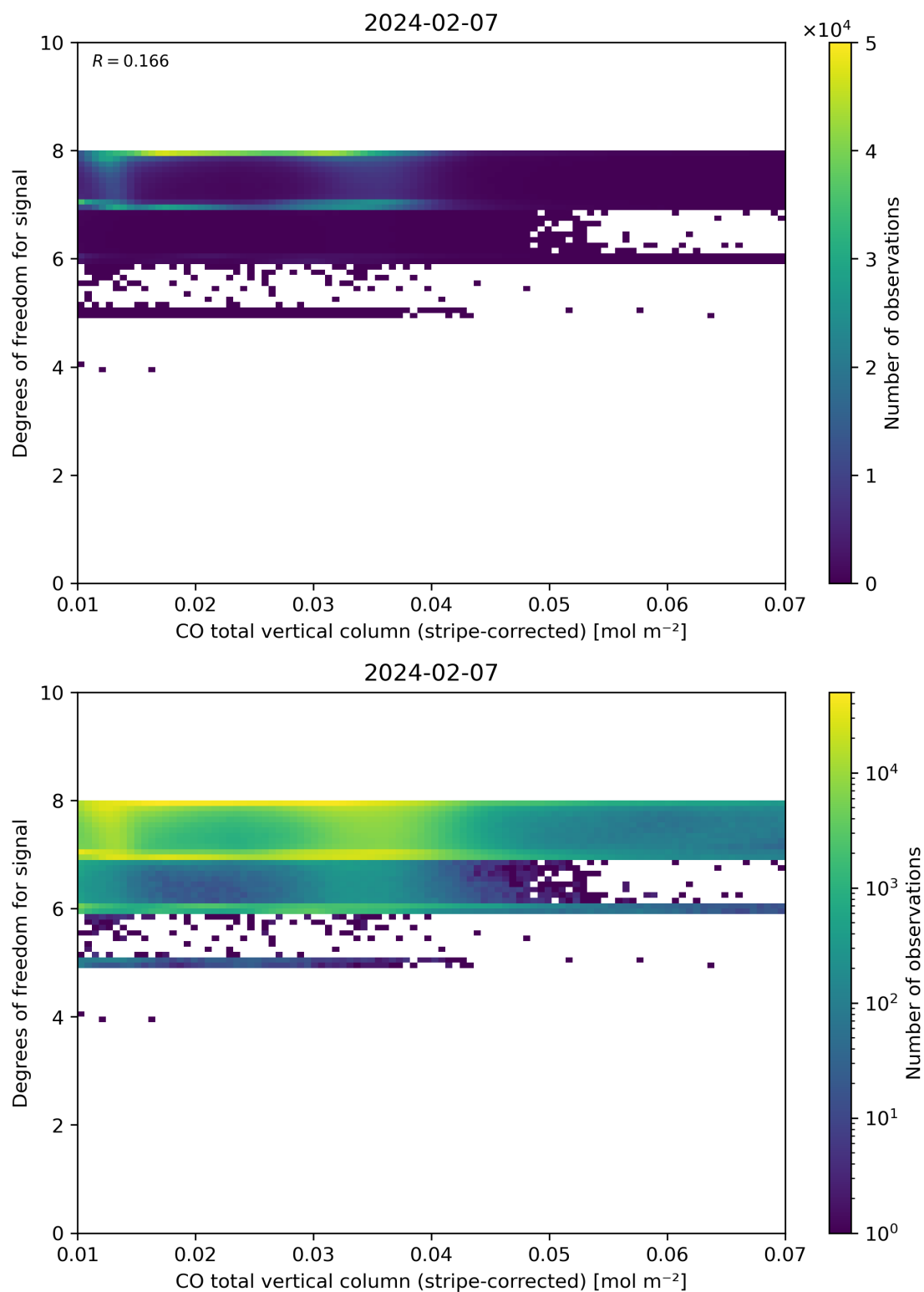
Figure 38: Scatter density plot of “CO total vertical column (stripe-corrected)” against “Degrees of freedom for signal” for 2024-02-06 to 2024-02-08.
