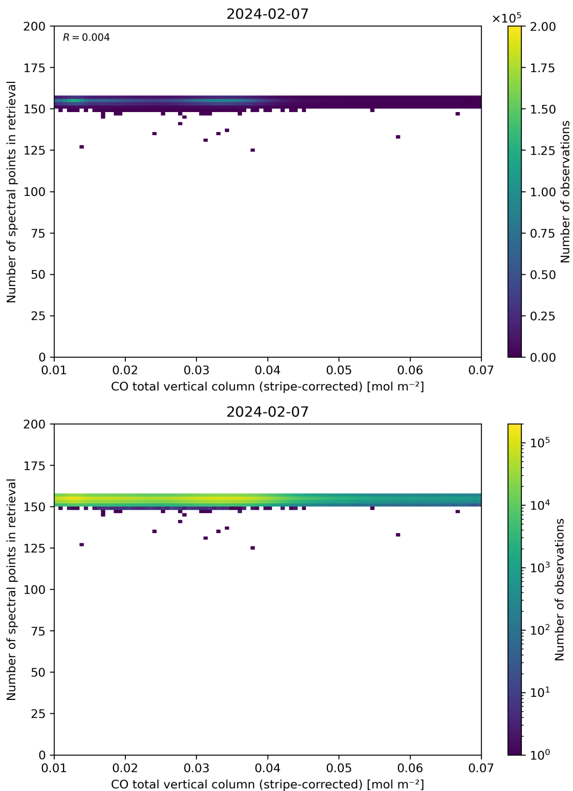
Figure 40: Scatter density plot of “CO total vertical column (stripe-corrected)” against “Number of spectral points in retrieval” for 2024-02-06 to 2024-02-08.
