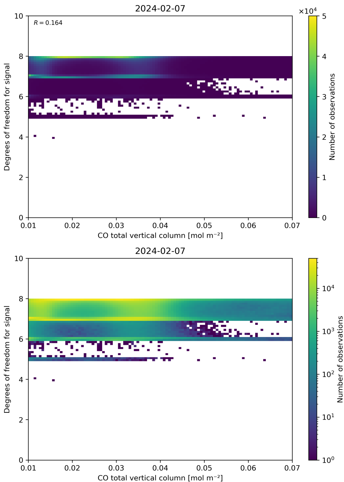
Figure 41: Scatter density plot of “CO total vertical column” against “Degrees of freedom for signal” for 2024-02-06 to 2024-02-08.
