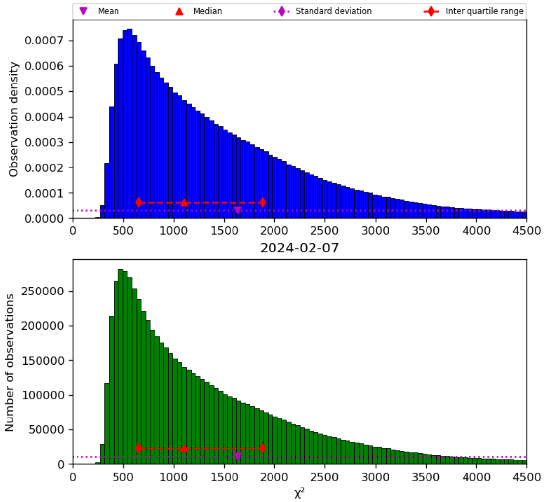
Figure 22: Histogram of “ \chi^2 ” for 2024-02-06 to 2024-02-08
