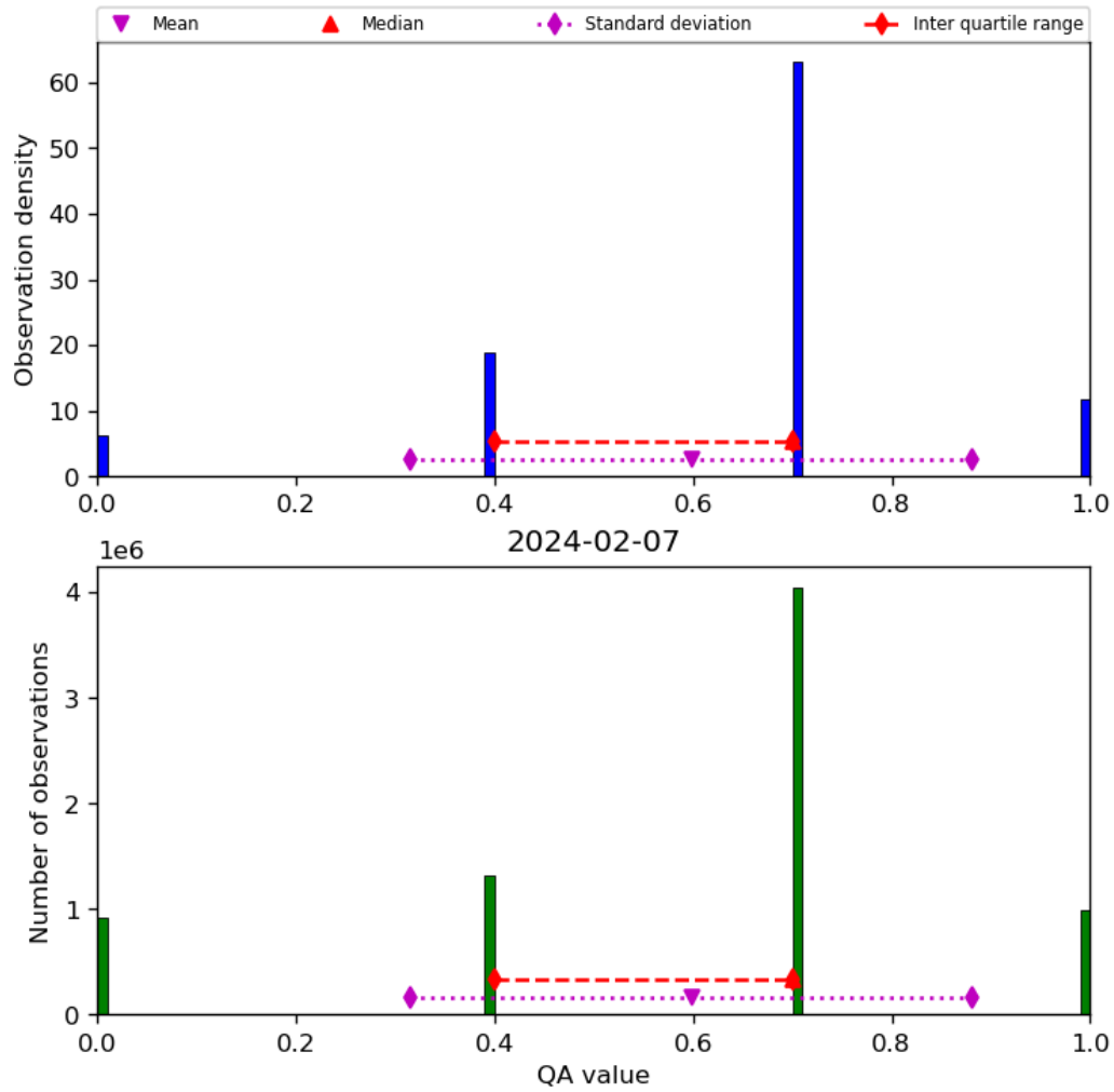
Figure 17: Histogram of “QA value” for 2024-02-06 to 2024-02-08
