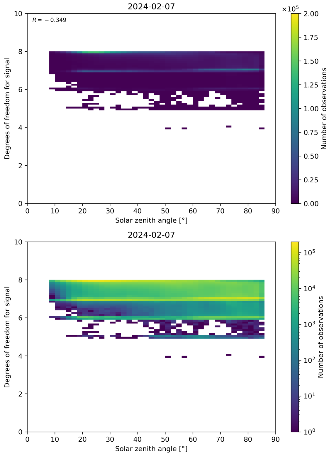
Figure 65: Scatter density plot of “Solar zenith angle” against “Degrees of freedom for signal” for 2024-02-06 to 2024-02-08.
