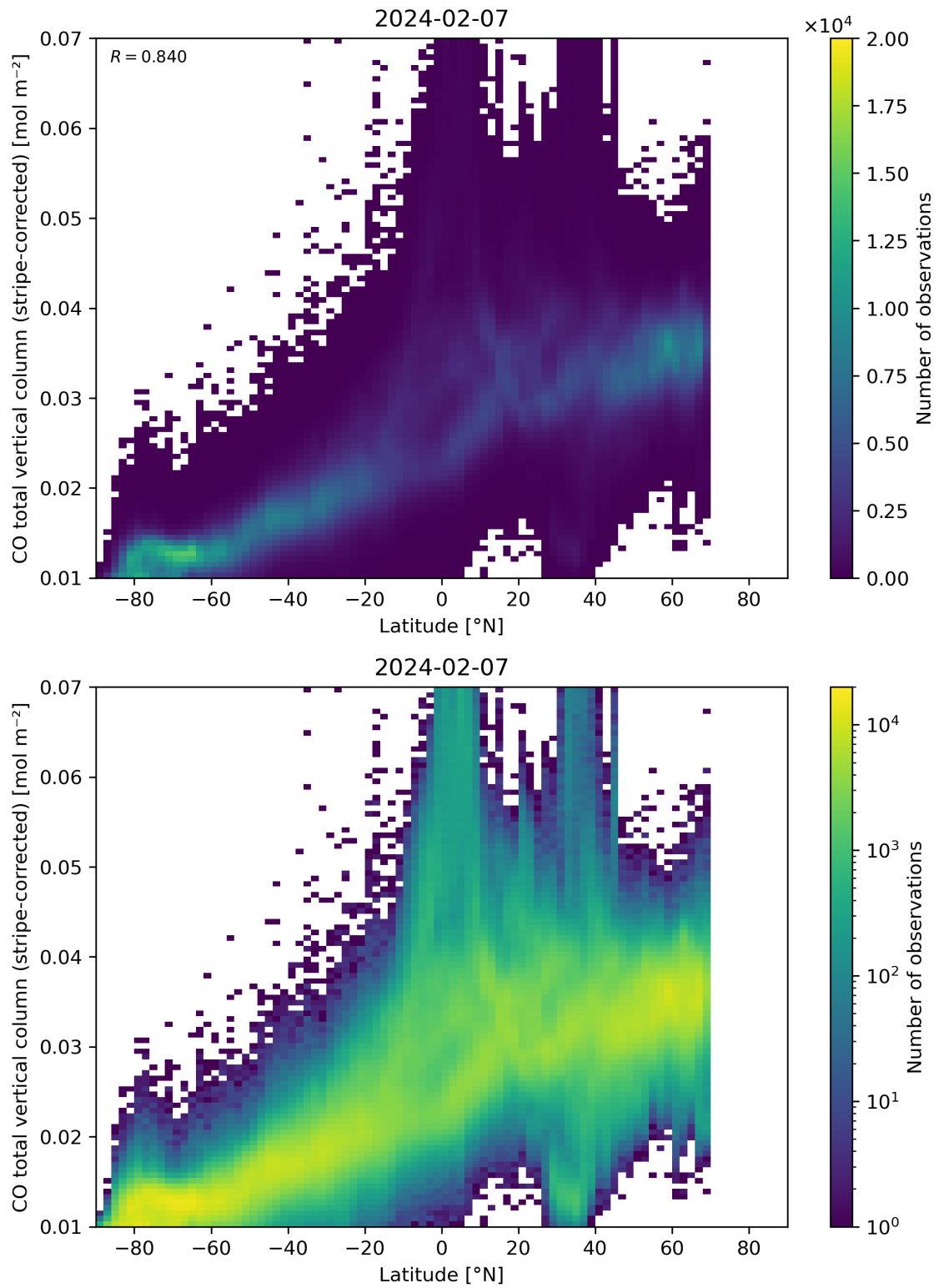
Figure 52: Scatter density plot of “Latitude” against “CO total vertical column (stripe-corrected)” for 2024-02-06 to 2024-02-08.
