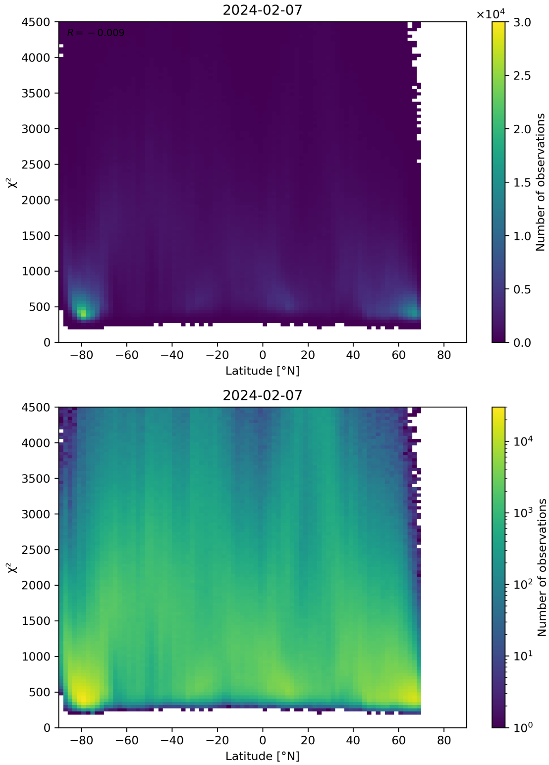
Figure 54: Scatter density plot of “Latitude” against “ \chi^2 ” for 2024-02-06 to 2024-02-08.
