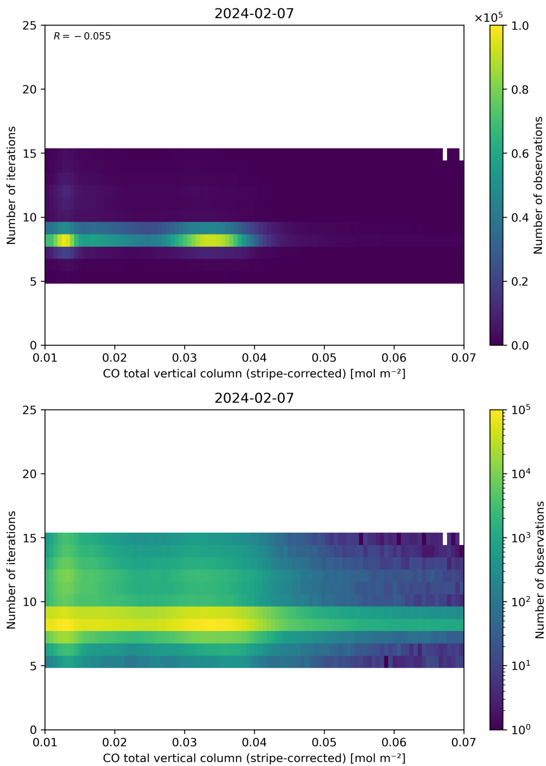
Figure 39: Scatter density plot of “CO total vertical column (stripe-corrected)” against “Number of iterations” for 2024-02-06 to 2024-02-08.
