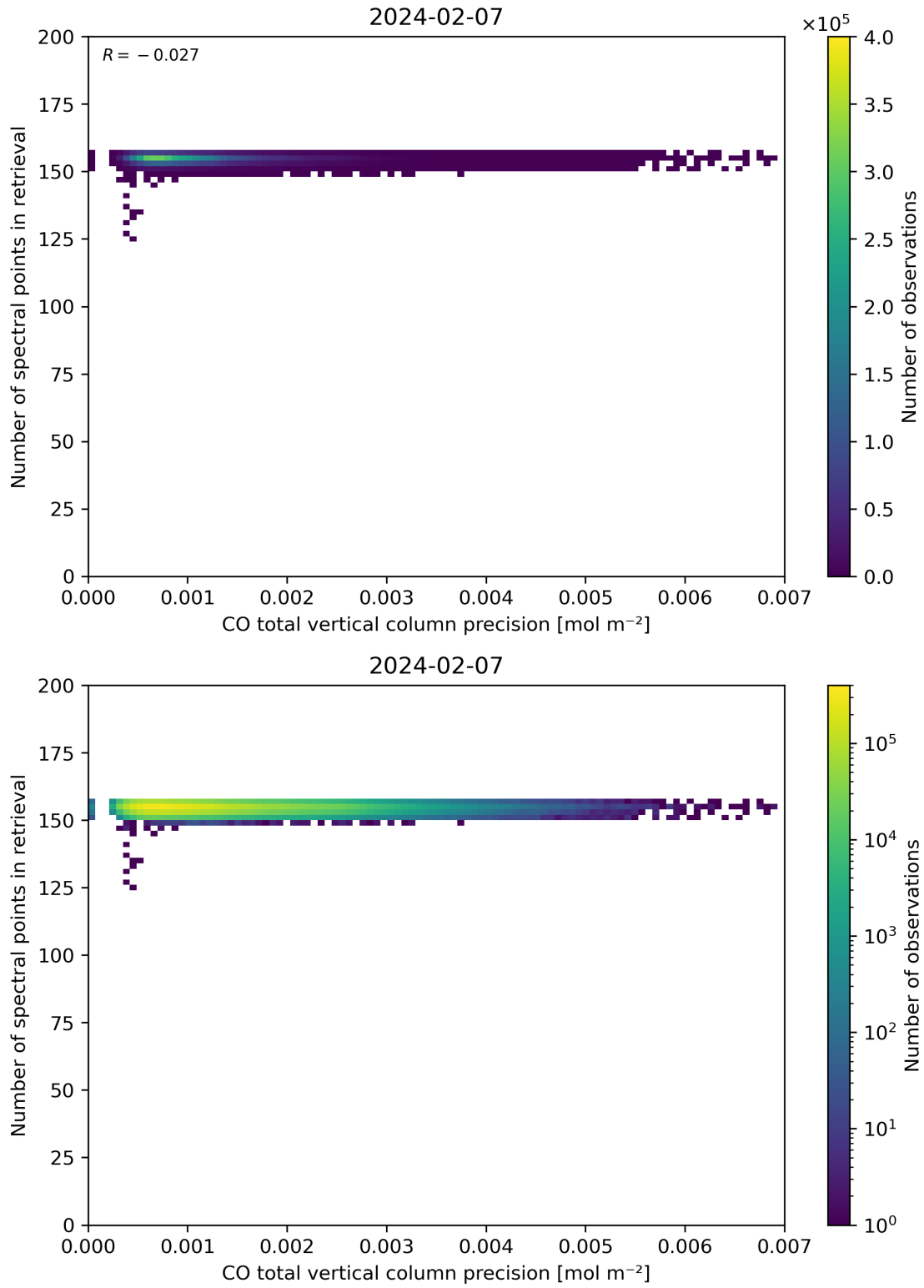
Figure 47: Scatter density plot of “CO total vertical column precision” against “Number of spectral points in retrieval” for 2024-02-06 to 2024-02-08.
