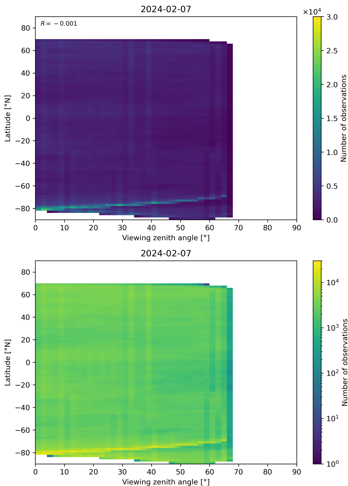
Figure 74: Scatter density plot of “Viewing zenith angle” against “Latitude” for 2024-02-06 to 2024-02-08.
