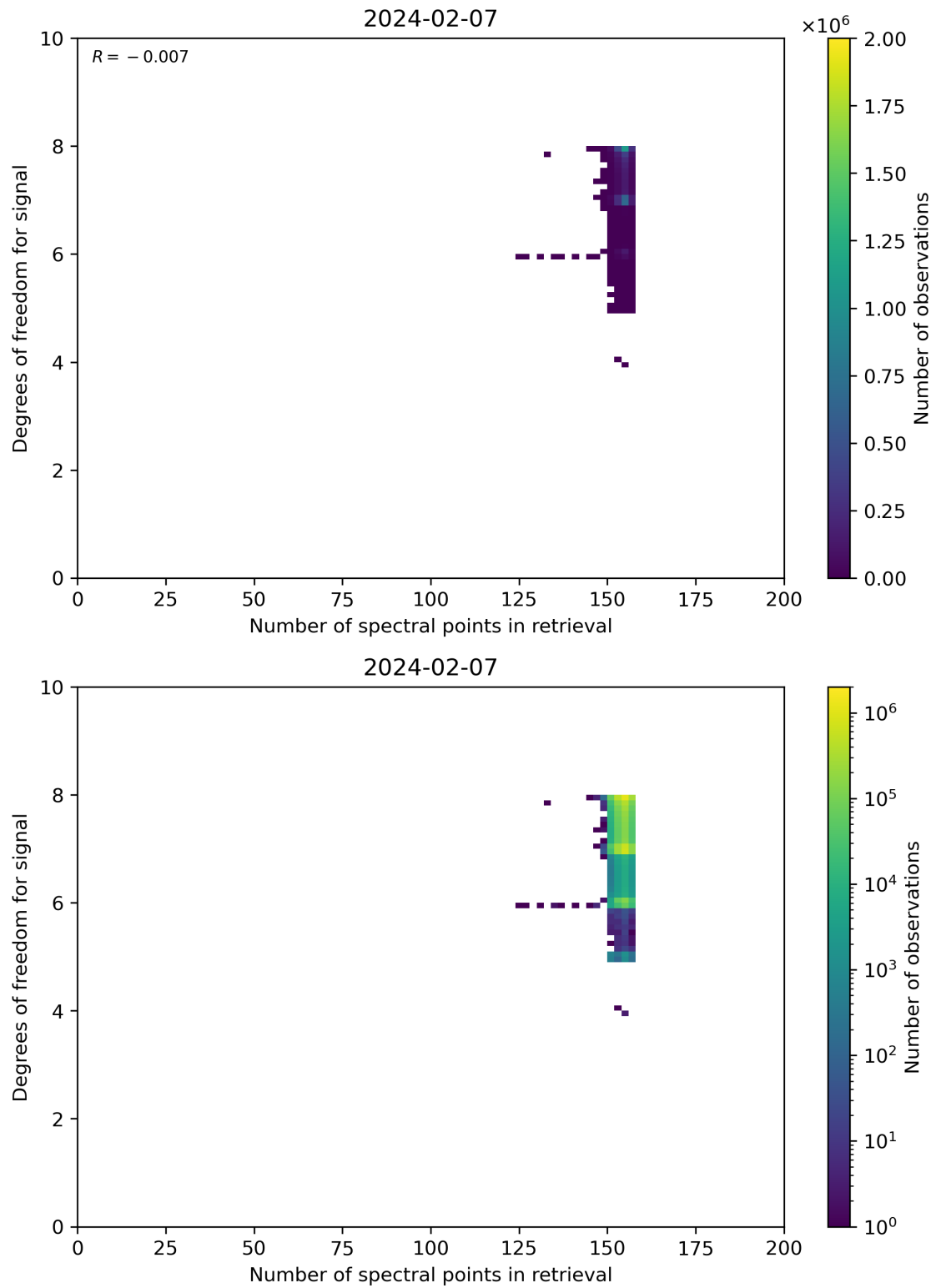
Figure 59: Scatter density plot of “Number of spectral points in retrieval” against “Degrees of freedom for signal” for 2024-02-06 to 2024-02-08.
