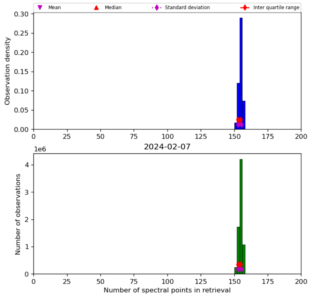
Figure 21: Histogram of “Number of spectral points in retrieval” for 2024-02-06 to 2024-02-08
