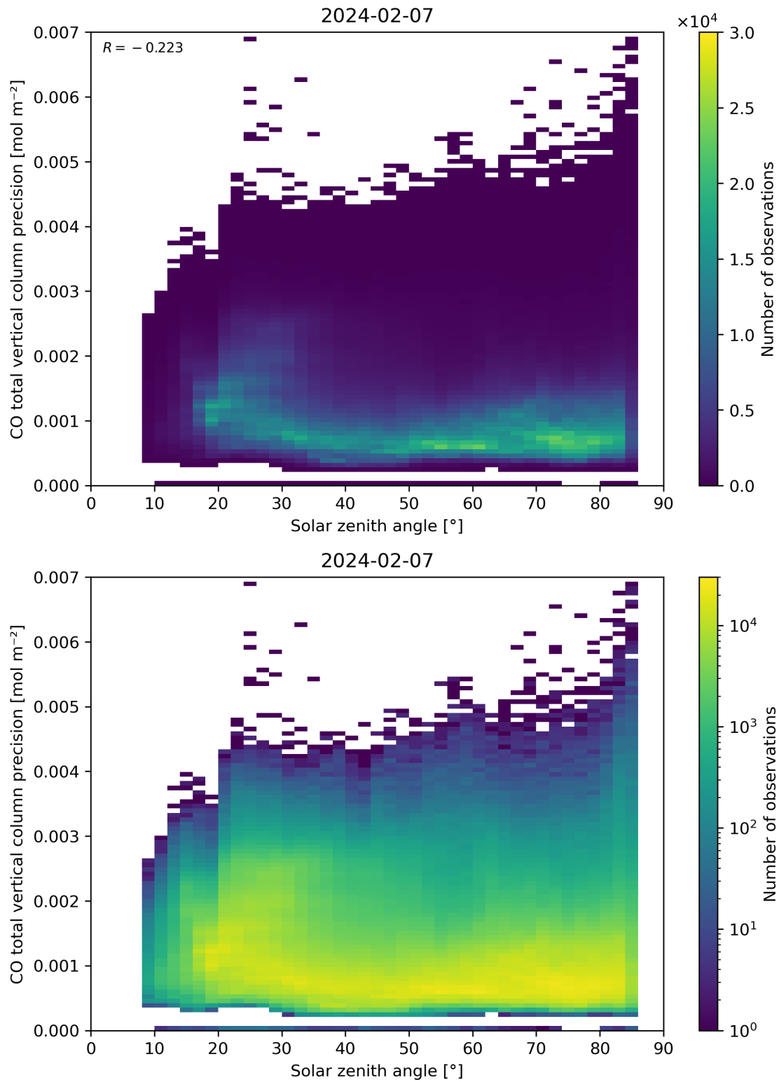
Figure 63: Scatter density plot of “Solar zenith angle” against “CO total vertical column precision” for 2024-02-06 to 2024-02-08.
