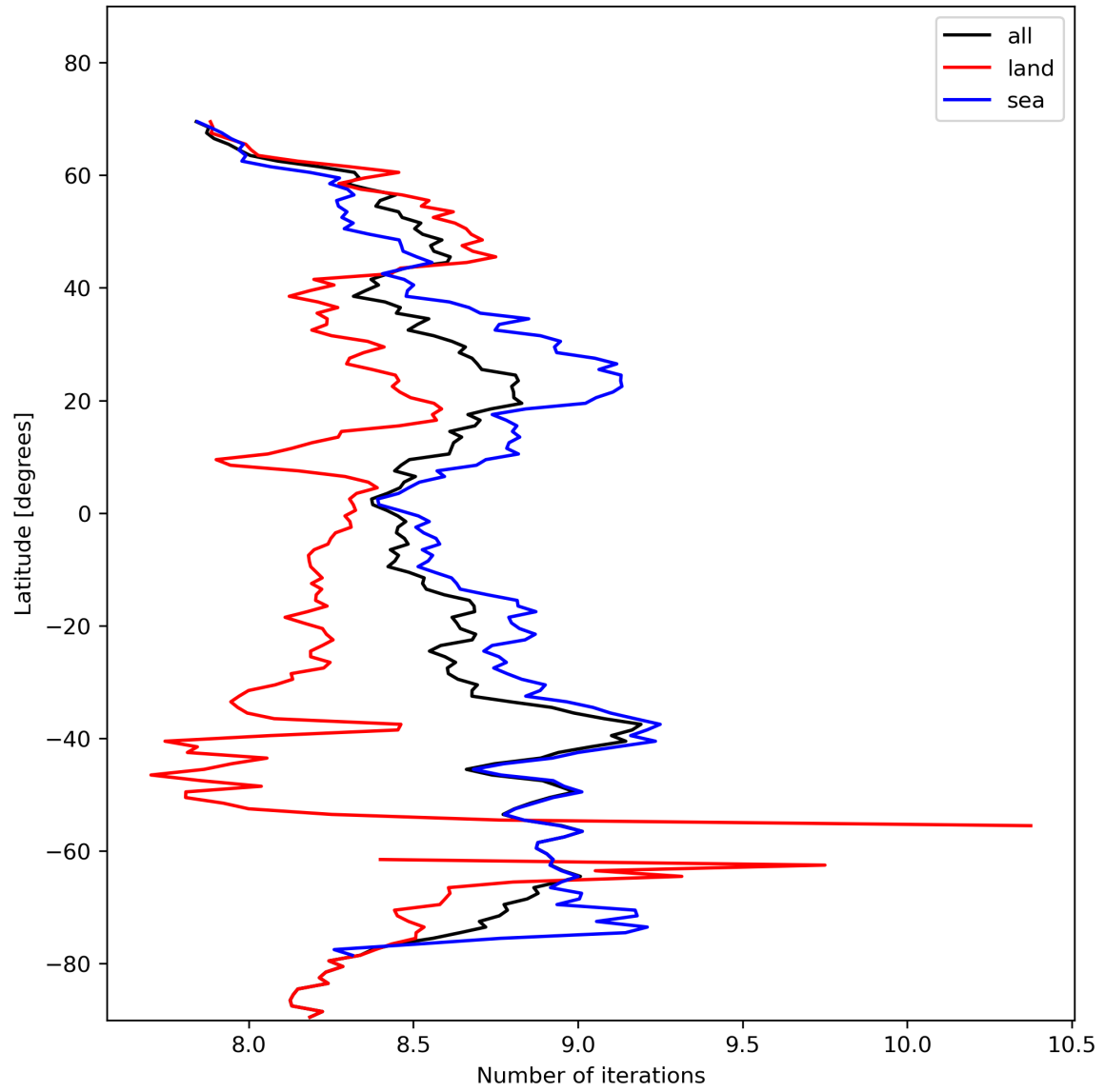
Figure 16: Zonal average of “Number of iterations” for 2024-02-06 to 2024-02-08.
