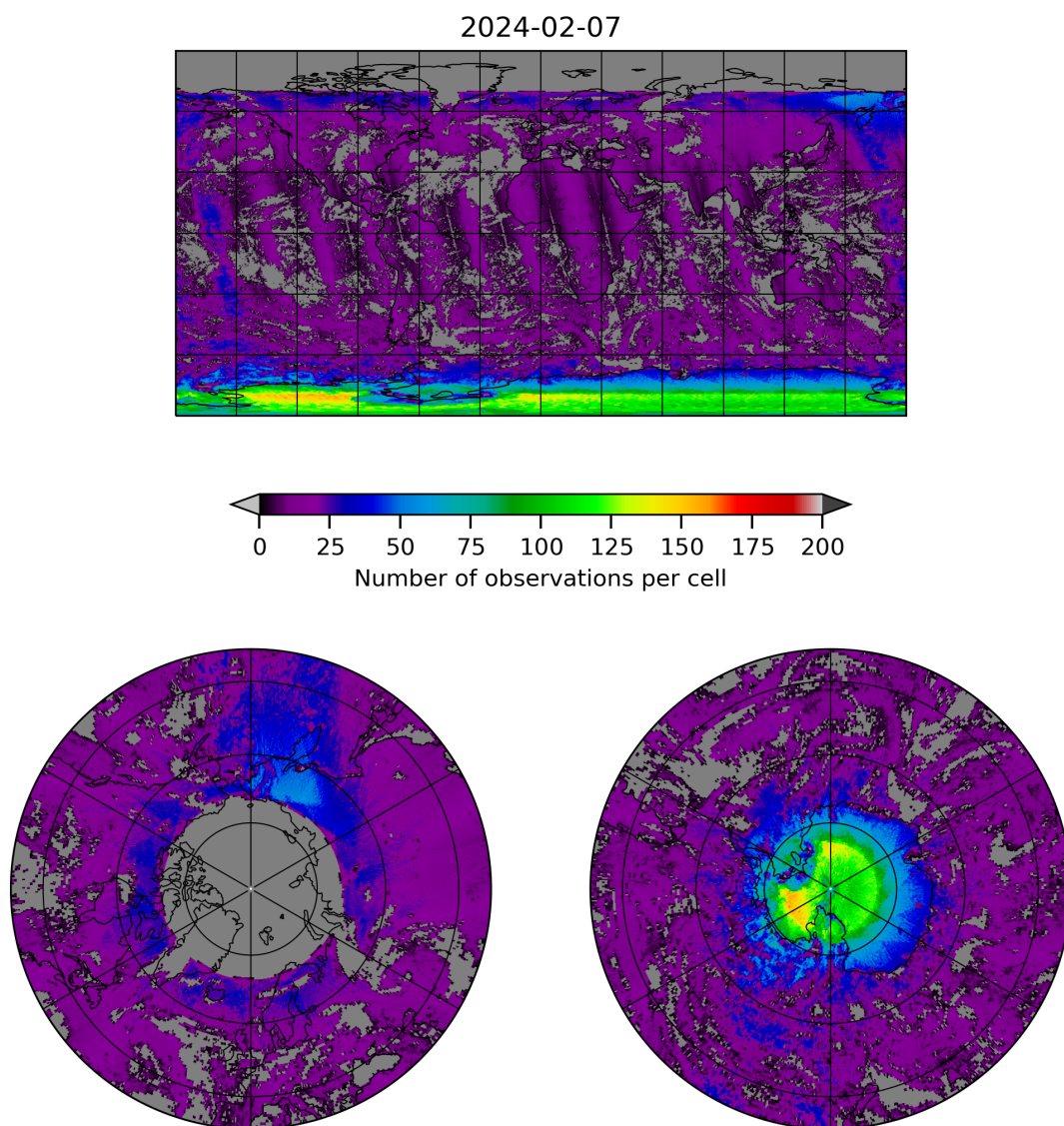
Figure 8: Map of the number of observations for 2024-02-06 to 2024-02-08
