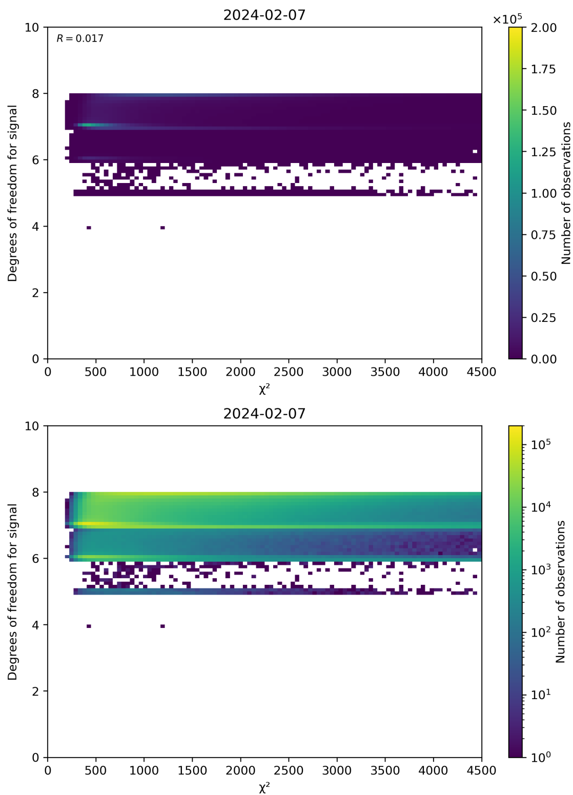
Figure 48: Scatter density plot of “ \chi^2 ” against “Degrees of freedom for signal” for 2024-02-06 to 2024-02-08.
