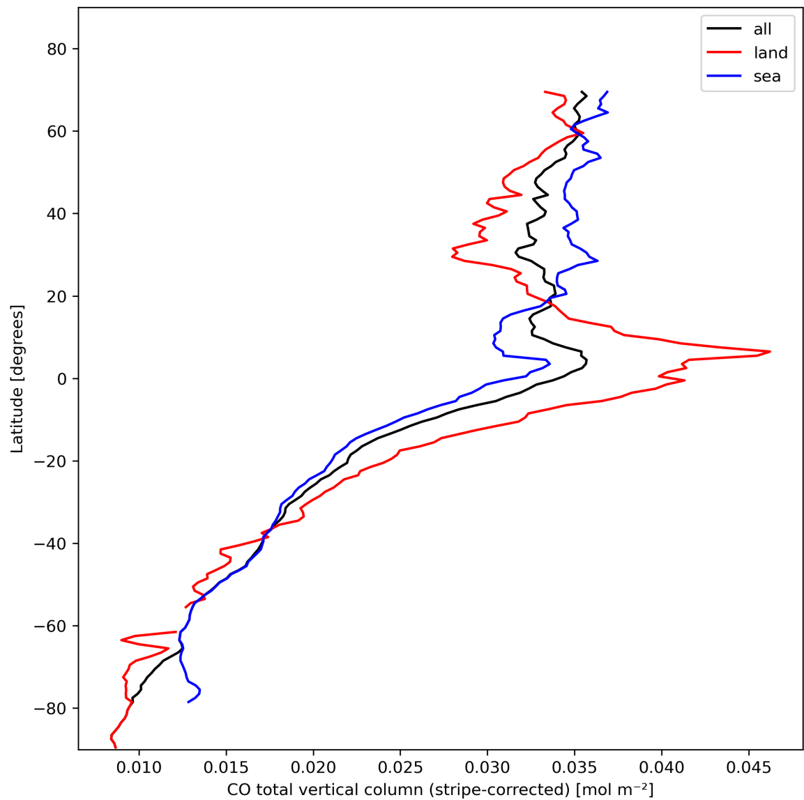
Figure 11: Zonal average of “CO total vertical column (stripe-corrected)” for 2024-02-06 to 2024-02-08.
