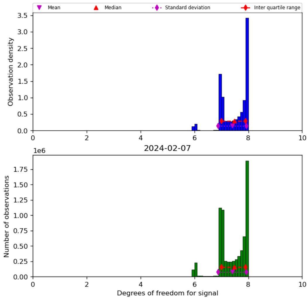
Figure 23: Histogram of “Degrees of freedom for signal” for 2024-02-06 to 2024-02-08
