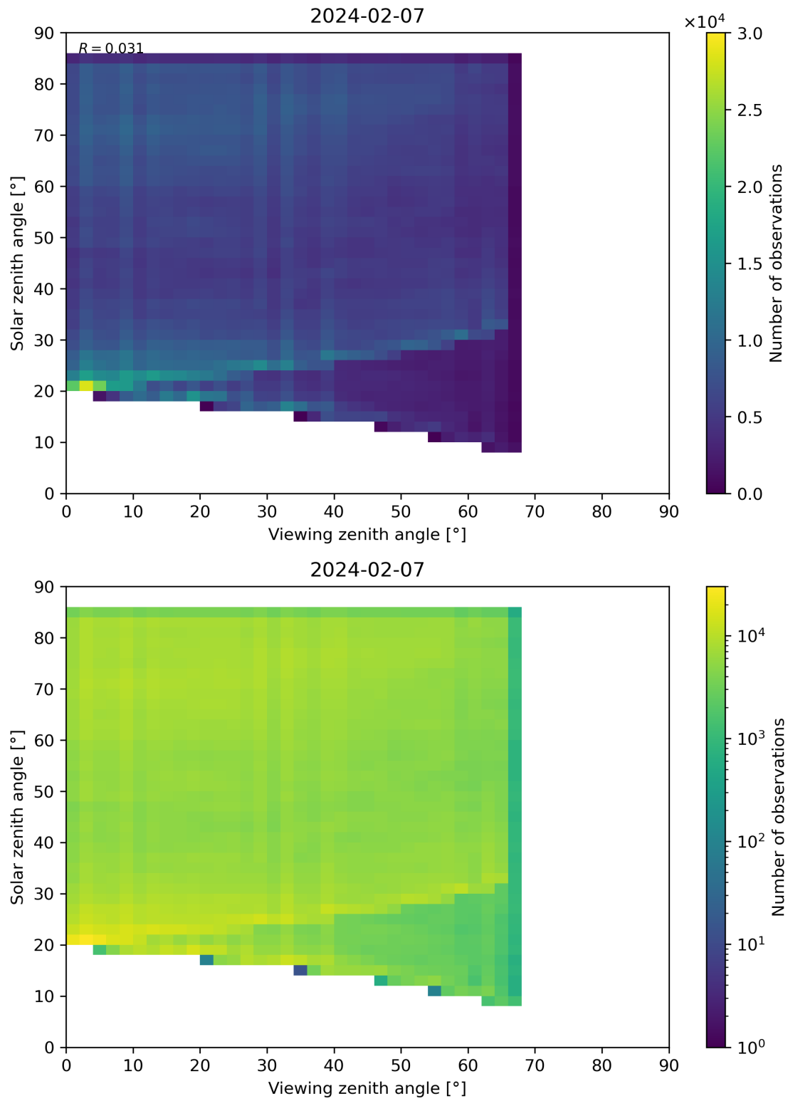
Figure 77: Scatter density plot of “Viewing zenith angle” against “Solar zenith angle” for 2024-02-06 to 2024-02-08.
