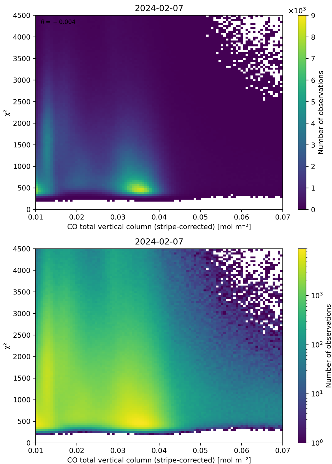
Figure 37: Scatter density plot of “CO total vertical column (stripe-corrected)” against “ \chi^2 ” for 2024-02-06 to 2024-02-08.
