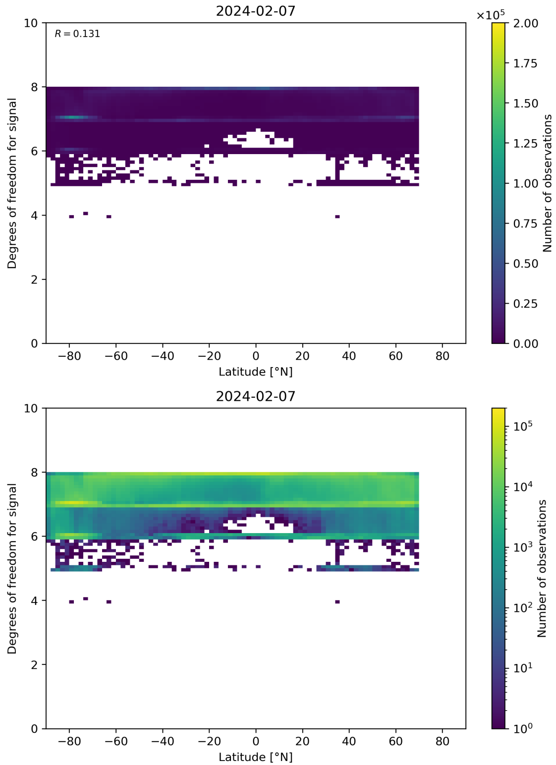
Figure 55: Scatter density plot of “Latitude” against “Degrees of freedom for signal” for 2024-02-06 to 2024-02-08.
