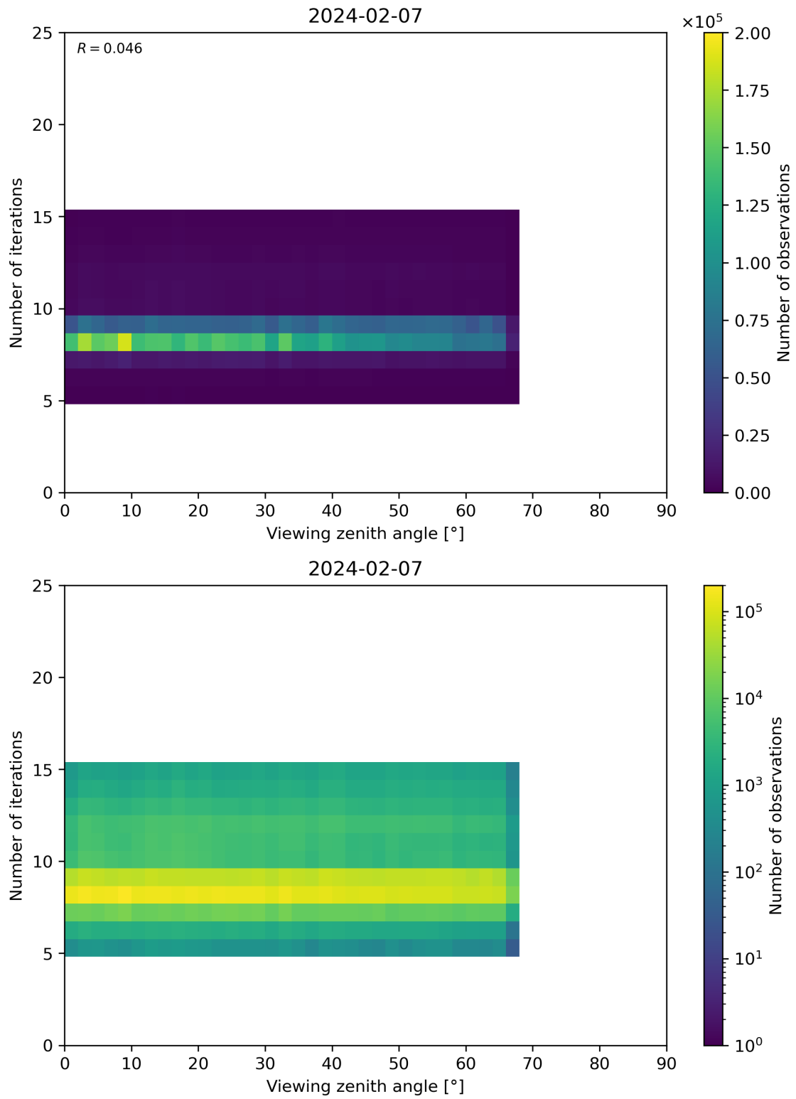
Figure 75: Scatter density plot of “Viewing zenith angle” against “Number of iterations” for 2024-02-06 to 2024-02-08.
