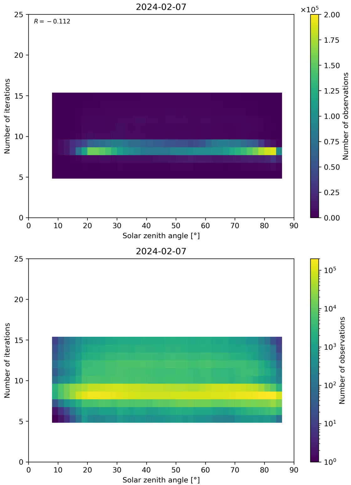
Figure 67: Scatter density plot of “Solar zenith angle” against “Number of iterations” for 2024-02-06 to 2024-02-08.
