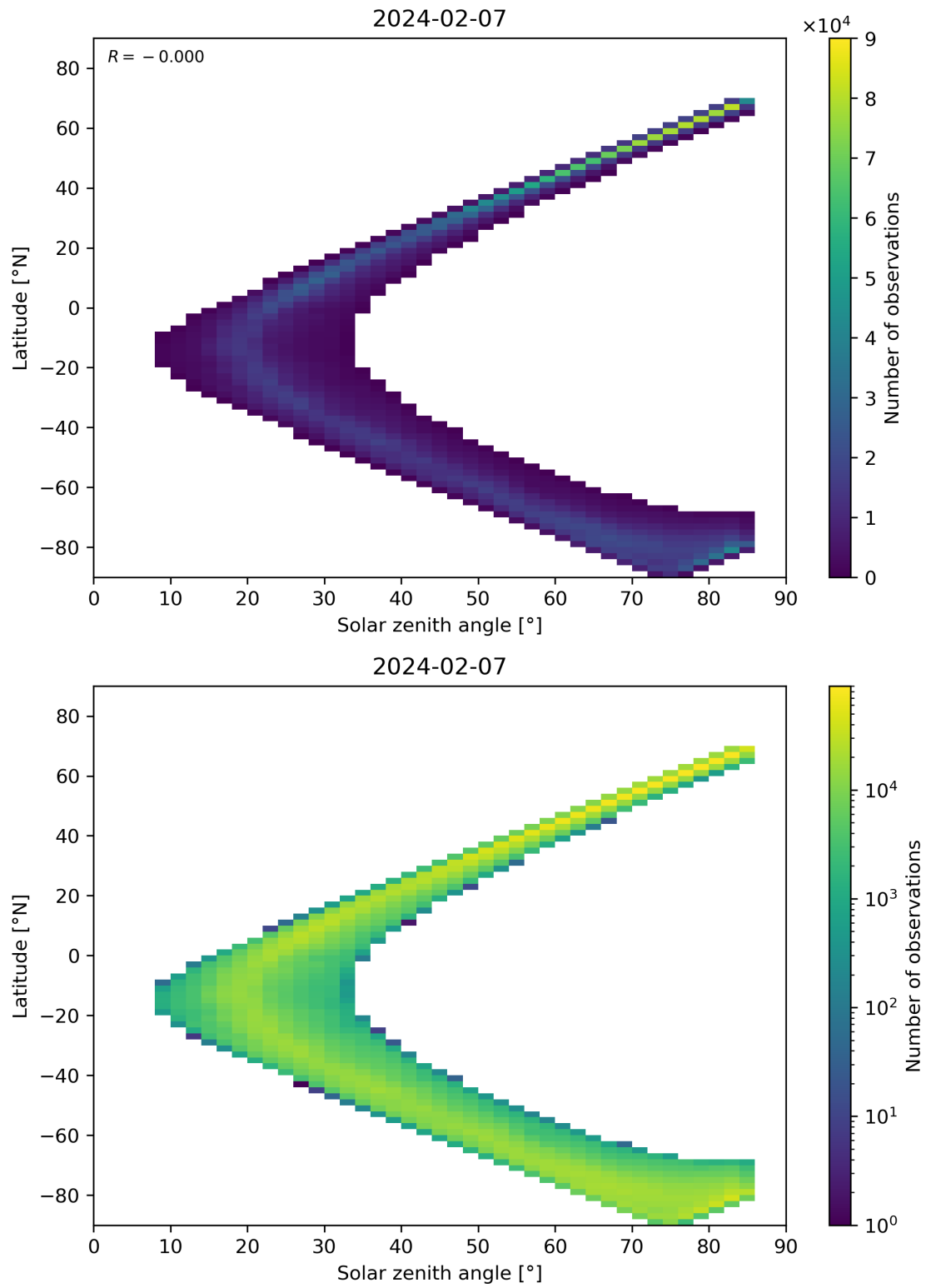
Figure 66: Scatter density plot of “Solar zenith angle” against “Latitude” for 2024-02-06 to 2024-02-08.
