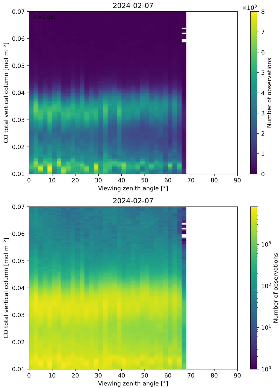
Figure 69: Scatter density plot of “Viewing zenith angle” against “CO total vertical column” for 2024-02-06 to 2024-02-08.
