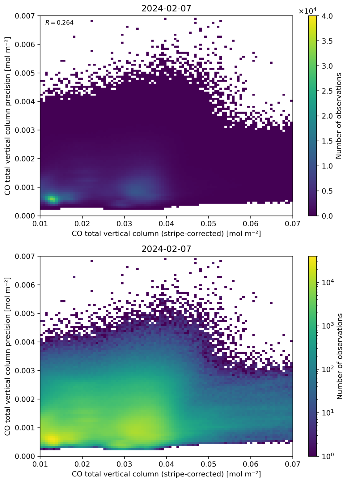
Figure 36: Scatter density plot of “CO total vertical column (stripe-corrected)” against “CO total vertical column precision” for 2024-02-06 to 2024-02-08.
