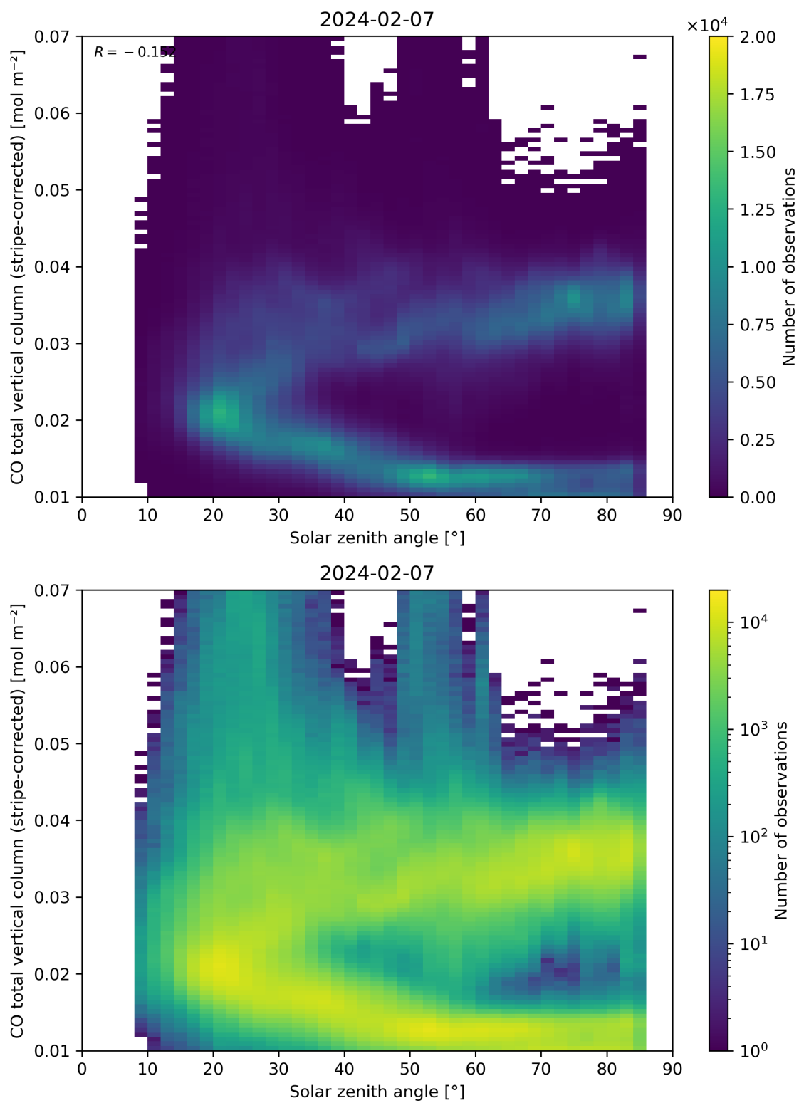
Figure 62: Scatter density plot of “Solar zenith angle” against “CO total vertical column (stripe-corrected)” for 2024-02-06 to 2024-02-08.
