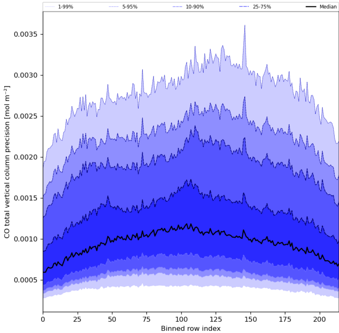
Figure 28: Along track statistics of “CO total vertical column precision” for 2024-02-06 to 2024-02-08
