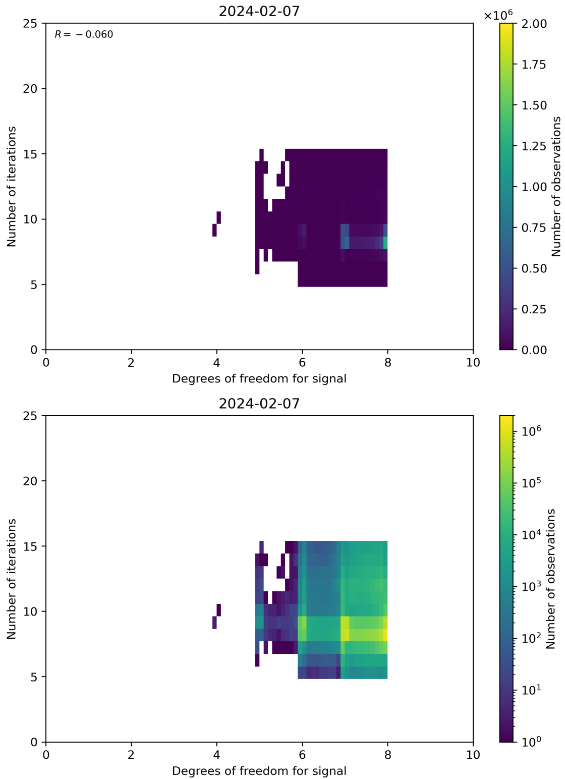
Figure 50: Scatter density plot of “Degrees of freedom for signal” against “Number of iterations” for 2024-02-06 to 2024-02-08.
