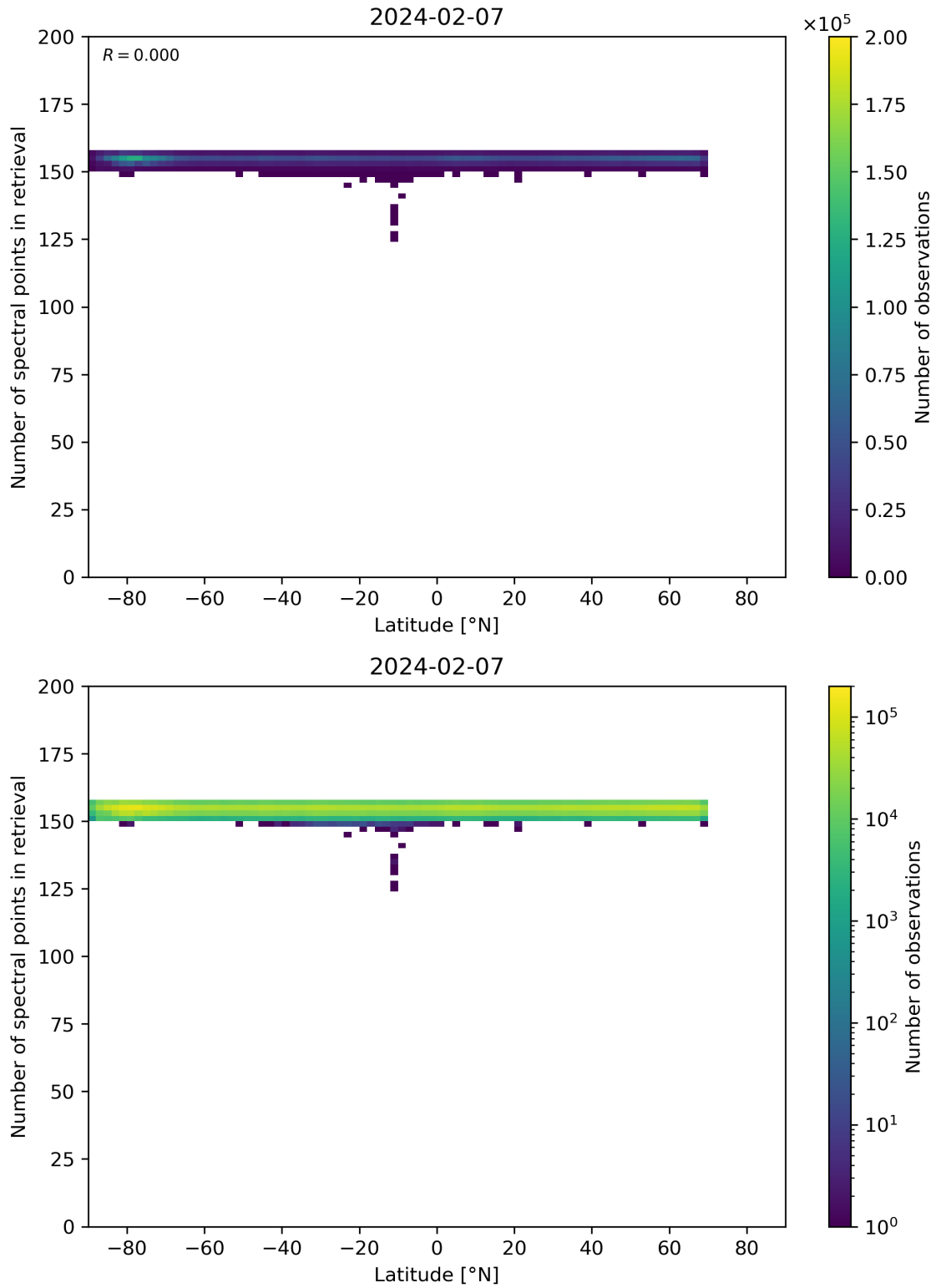
Figure 57: Scatter density plot of “Latitude” against “Number of spectral points in retrieval” for 2024-02-06 to 2024-02-08.
