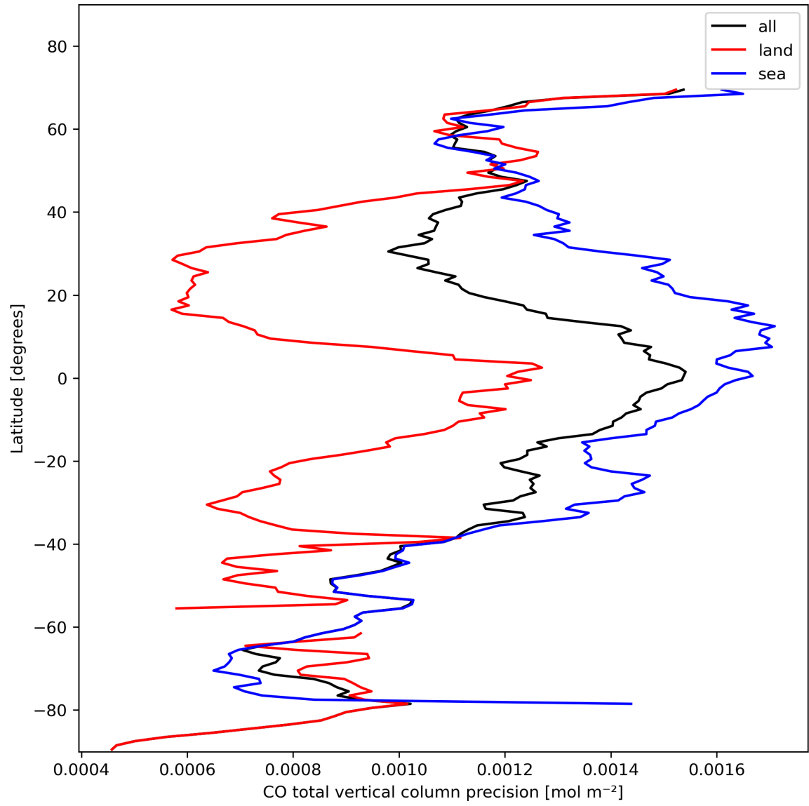
Figure 12: Zonal average of “CO total vertical column precision” for 2024-02-06 to 2024-02-08.
