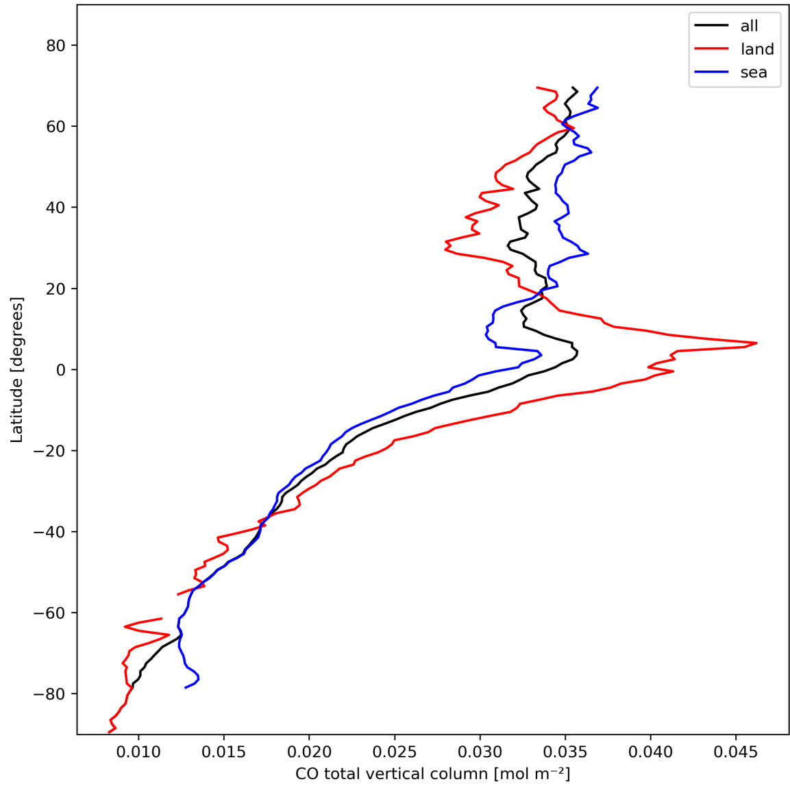
Figure 10: Zonal average of “CO total vertical column” for 2024-02-06 to 2024-02-08.
