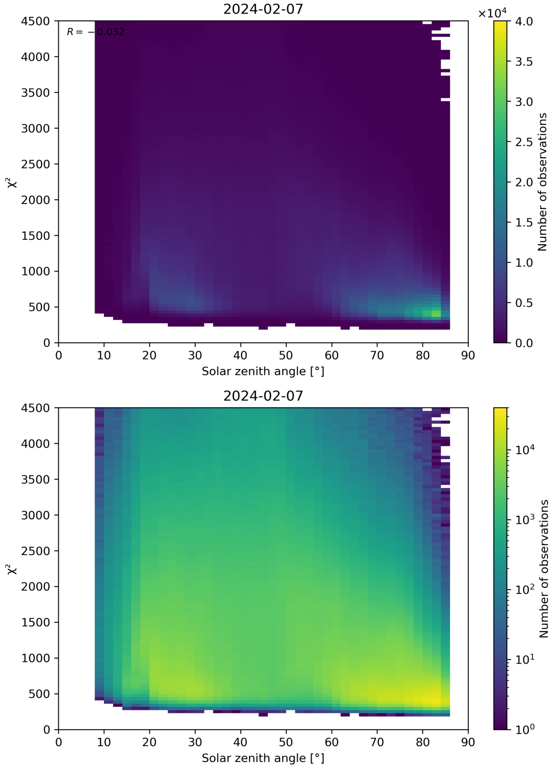
Figure 64: Scatter density plot of “Solar zenith angle” against “ \chi^2 ” for 2024-02-06 to 2024-02-08.
