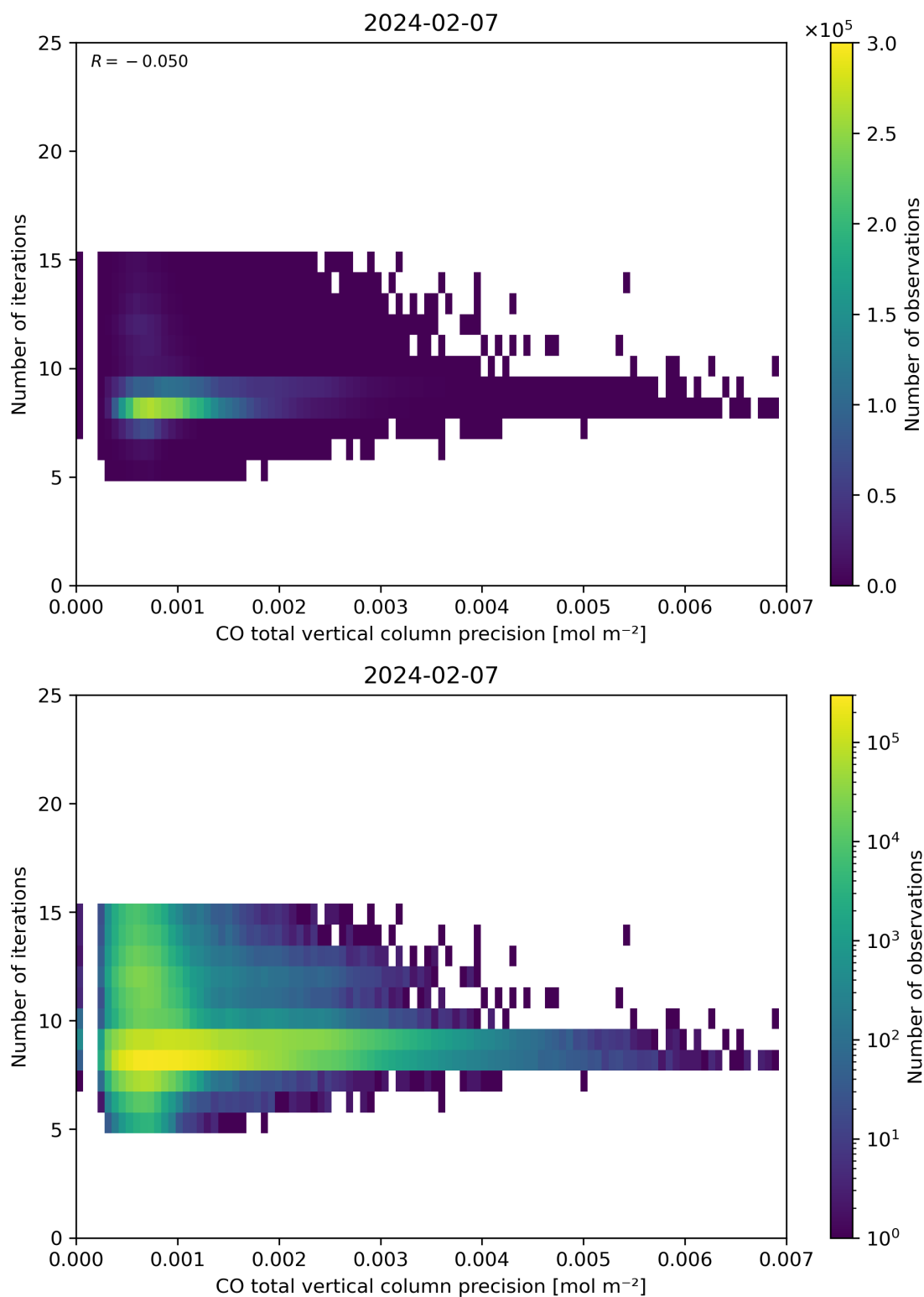
Figure 46: Scatter density plot of “CO total vertical column precision” against “Number of iterations” for 2024-02-06 to 2024-02-08.
