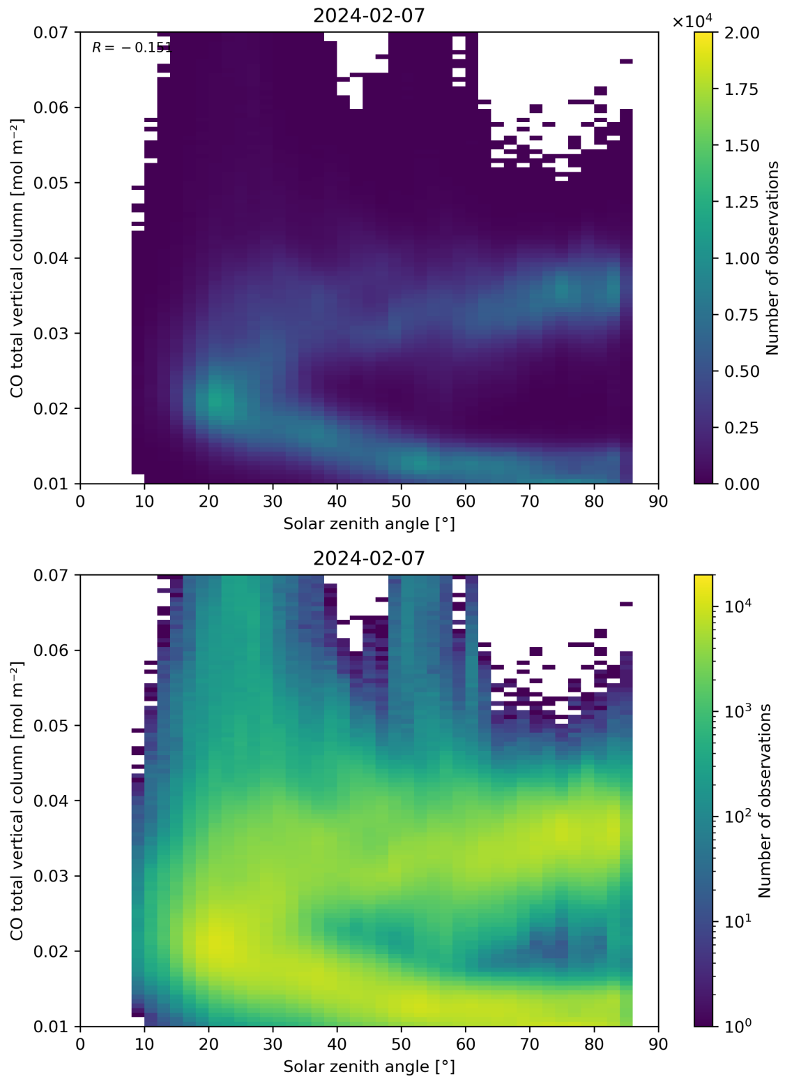
Figure 61: Scatter density plot of “Solar zenith angle” against “CO total vertical column” for 2024-02-06 to 2024-02-08.
