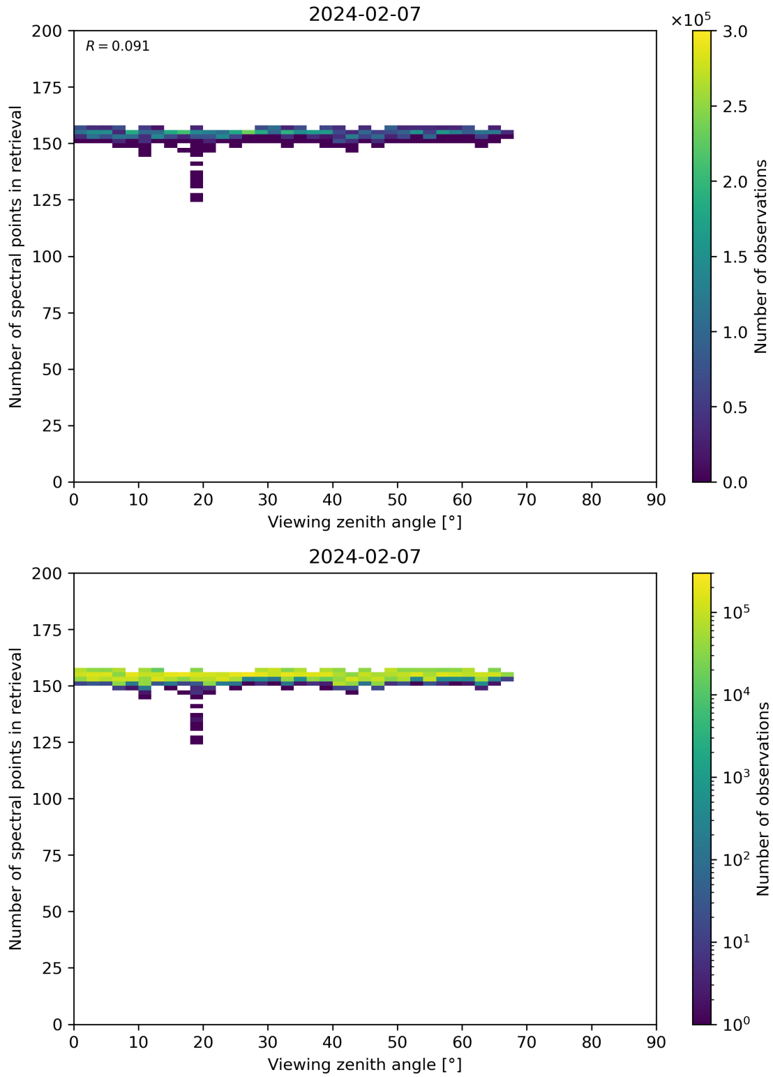
Figure 76: Scatter density plot of “Viewing zenith angle” against “Number of spectral points in retrieval” for 2024-02-06 to 2024-02-08.
