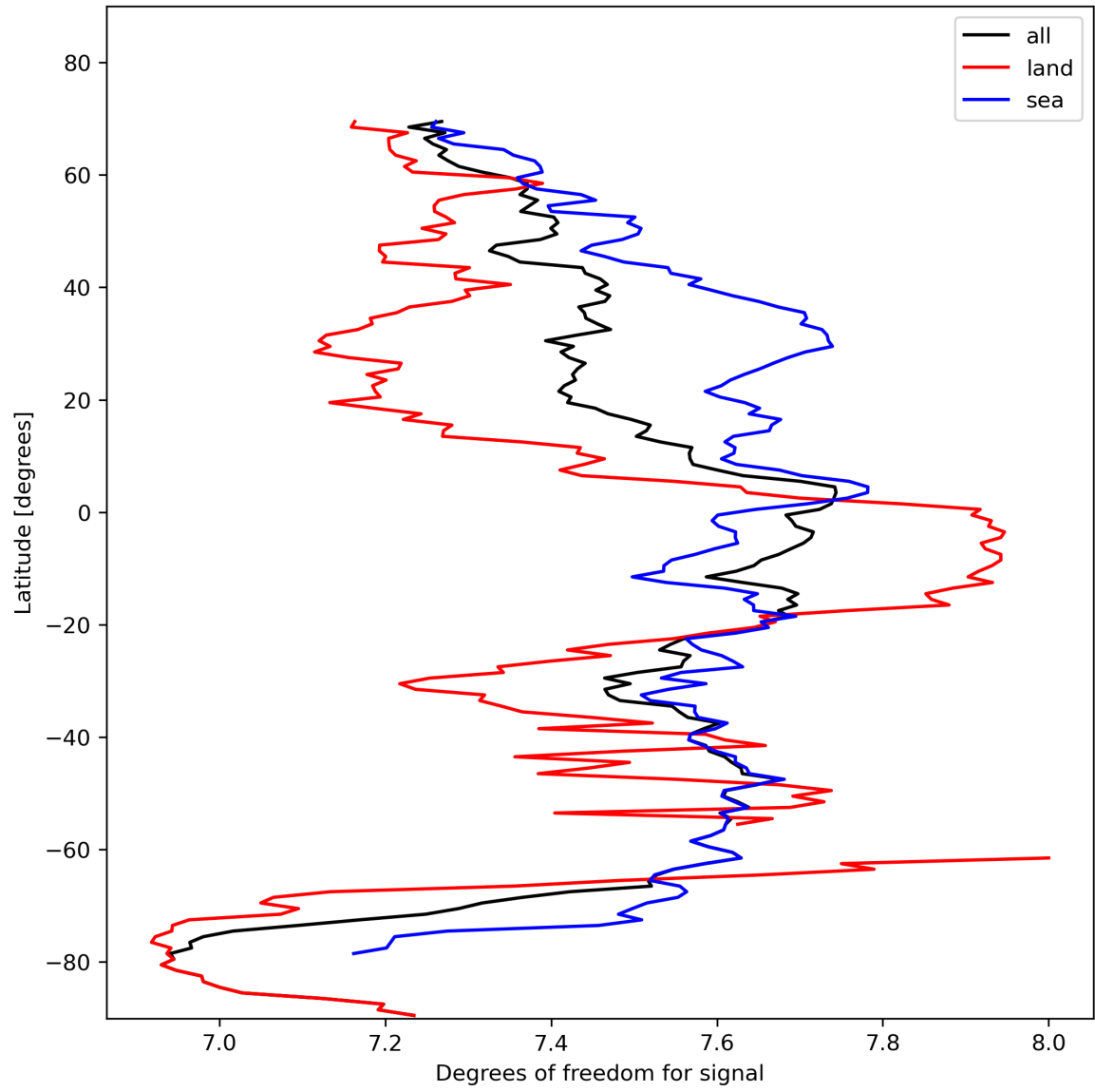
Figure 15: Zonal average of “Degrees of freedom for signal” for 2024-02-06 to 2024-02-08.
