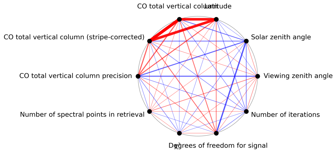
Figure 1: Map of correlation graph for 2024-02-06 to 2024-02-08.
