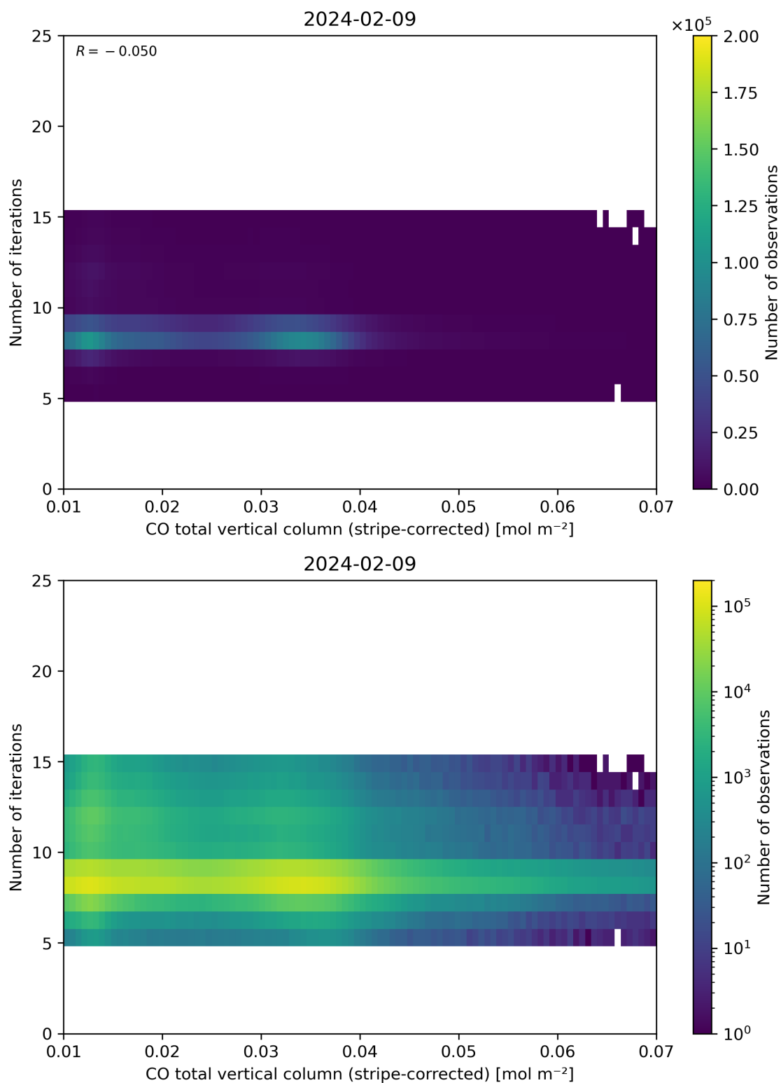
Figure 39: Scatter density plot of “CO total vertical column (stripe-corrected)” against “Number of iterations” for 2024-02-08 to 2024-02-10.
