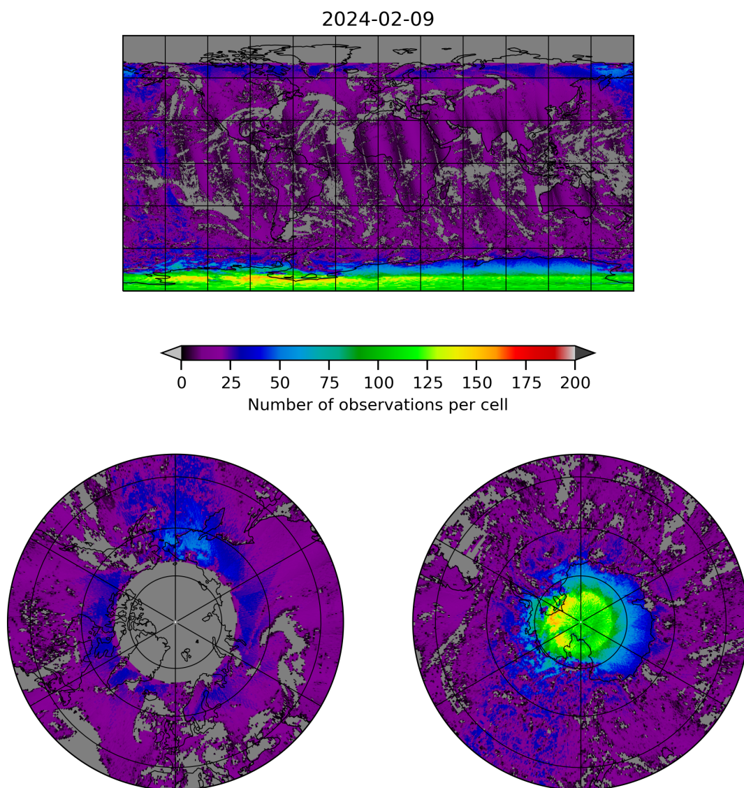
Figure 8: Map of the number of observations for 2024-02-08 to 2024-02-10
