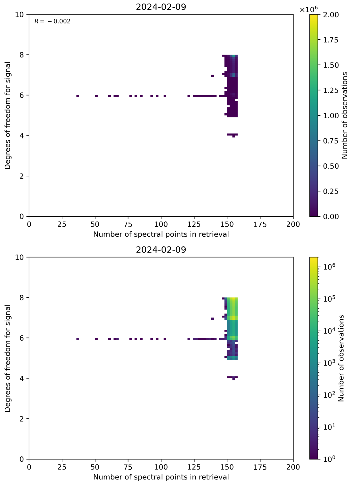
Figure 59: Scatter density plot of “Number of spectral points in retrieval” against “Degrees of freedom for signal” for 2024-02-08 to 2024-02-10.
