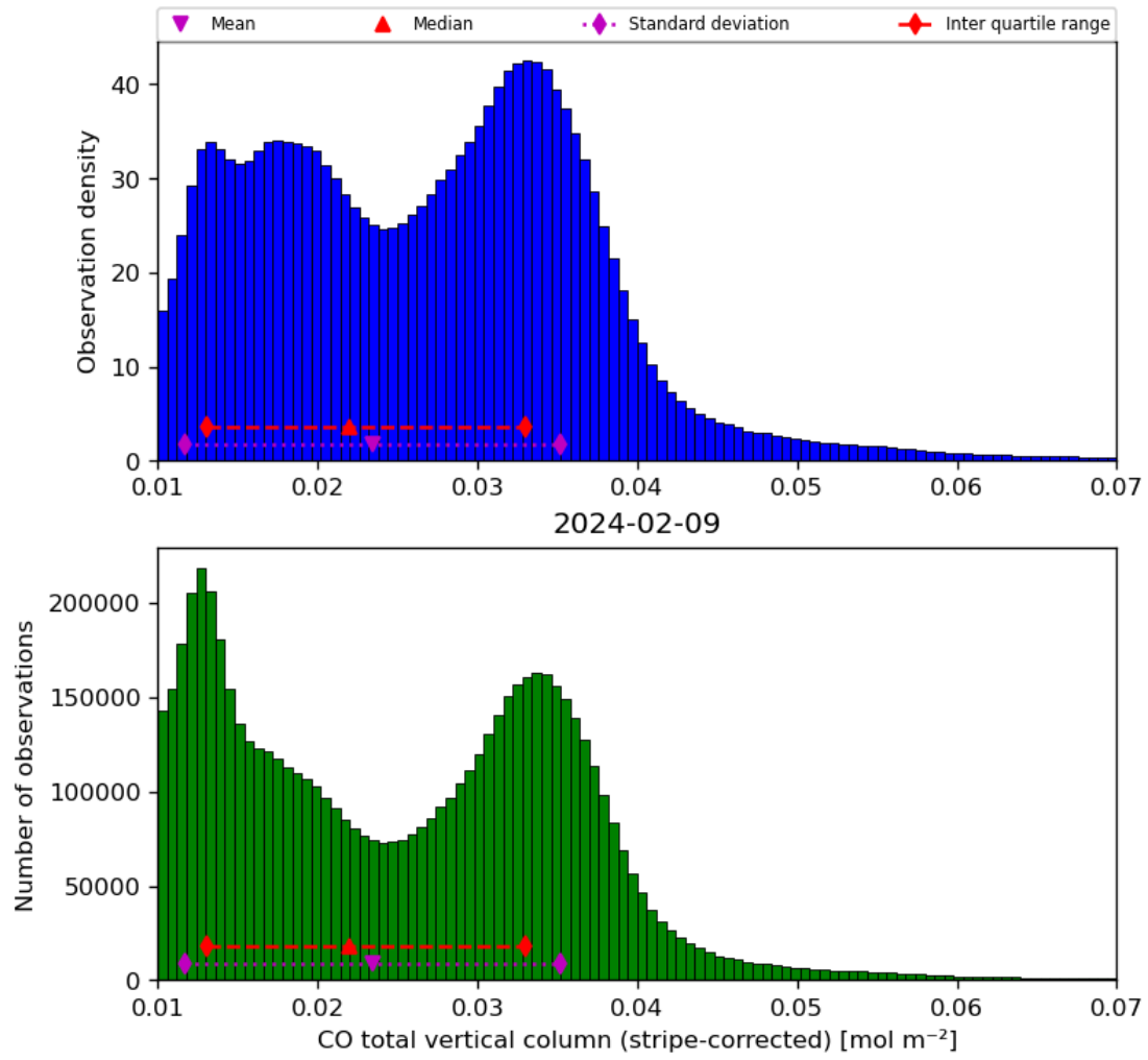
Figure 19: Histogram of “CO total vertical column (stripe-corrected)” for 2024-02-08 to 2024-02-10
