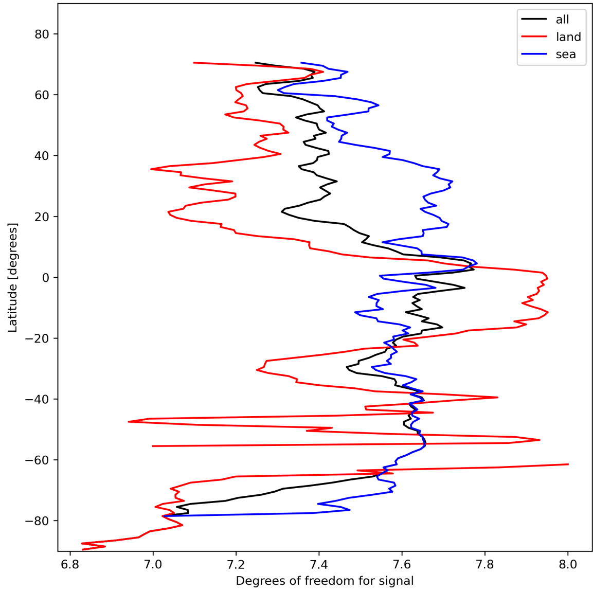
Figure 15: Zonal average of “Degrees of freedom for signal” for 2024-02-08 to 2024-02-10.
