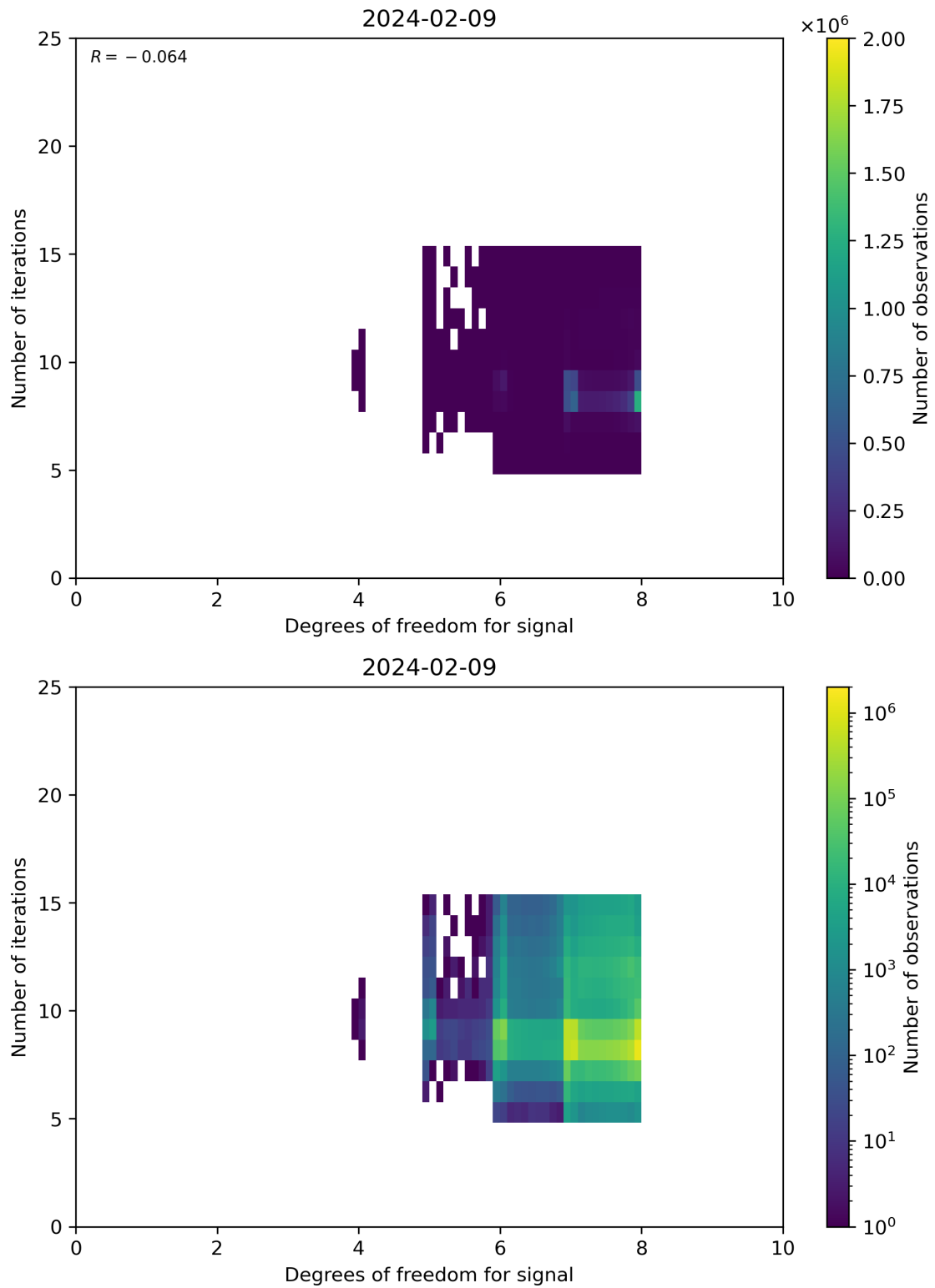
Figure 50: Scatter density plot of “Degrees of freedom for signal” against “Number of iterations” for 2024-02-08 to 2024-02-10.
