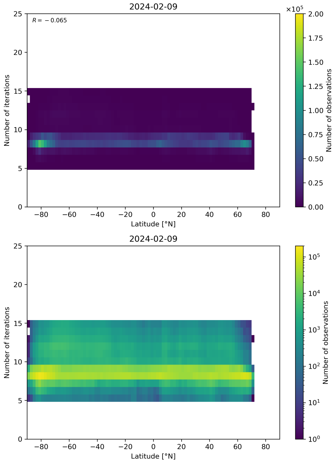
Figure 56: Scatter density plot of “Latitude” against “Number of iterations” for 2024-02-08 to 2024-02-10.
