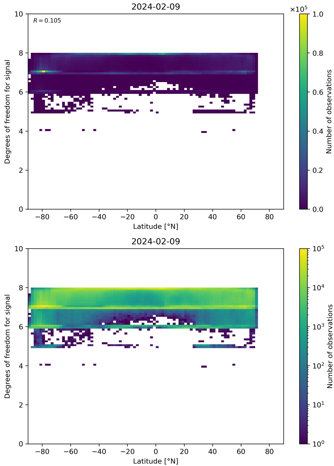
Figure 55: Scatter density plot of “Latitude” against “Degrees of freedom for signal” for 2024-02-08 to 2024-02-10.
