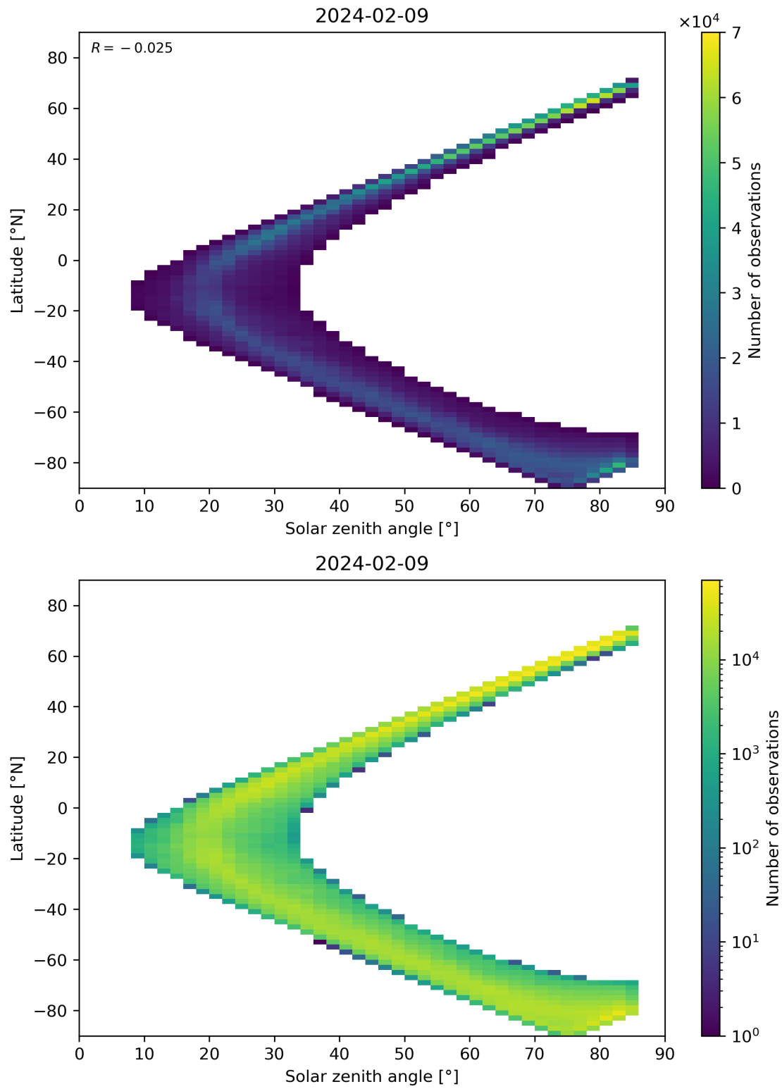
Figure 66: Scatter density plot of “Solar zenith angle” against “Latitude” for 2024-02-08 to 2024-02-10.
