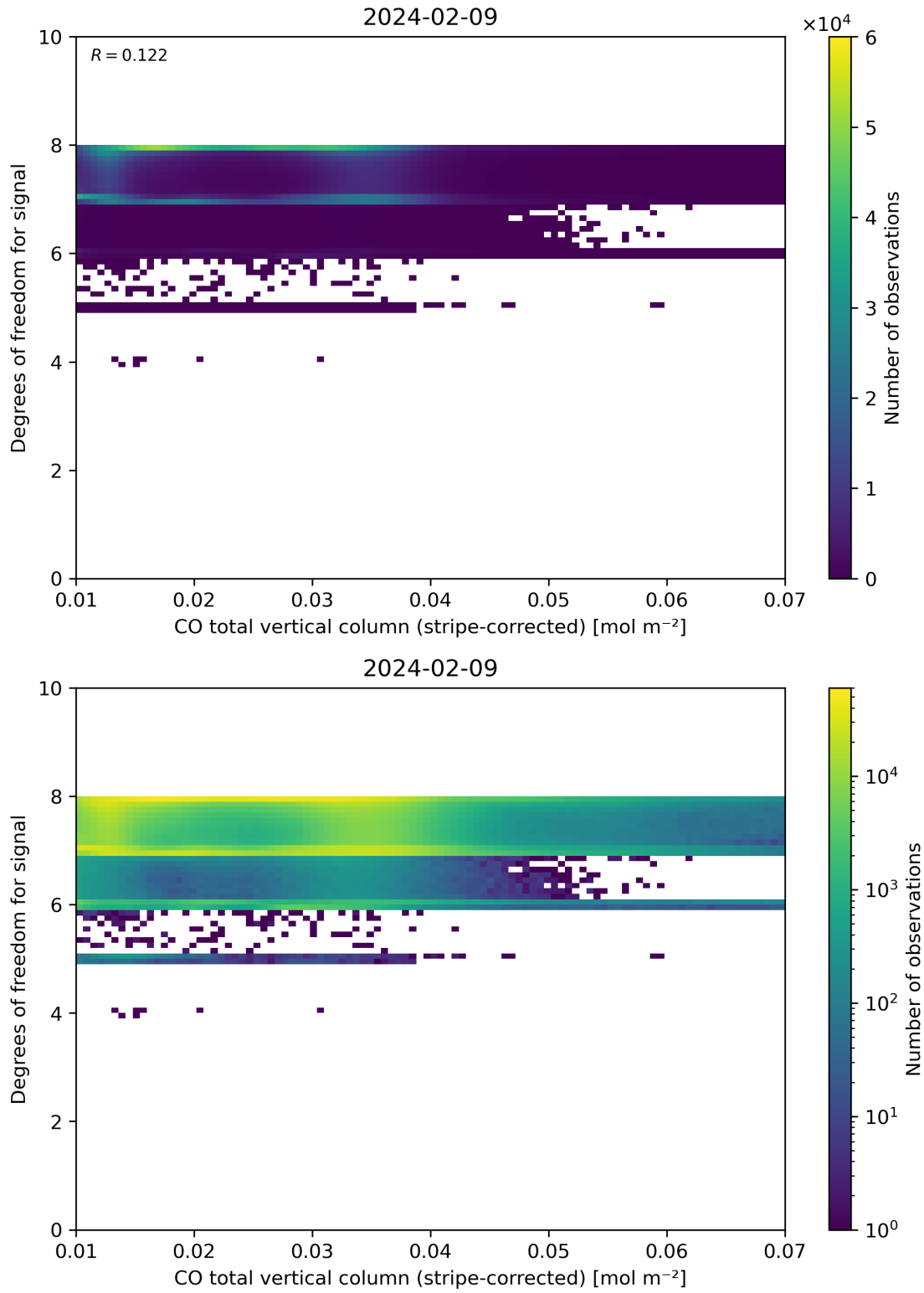
Figure 38: Scatter density plot of “CO total vertical column (stripe-corrected)” against “Degrees of freedom for signal” for 2024-02-08 to 2024-02-10.
