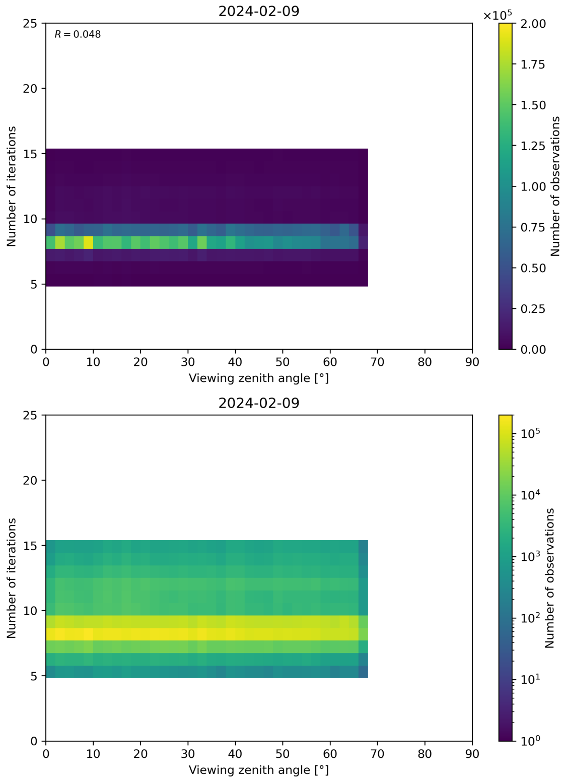
Figure 75: Scatter density plot of “Viewing zenith angle” against “Number of iterations” for 2024-02-08 to 2024-02-10.
