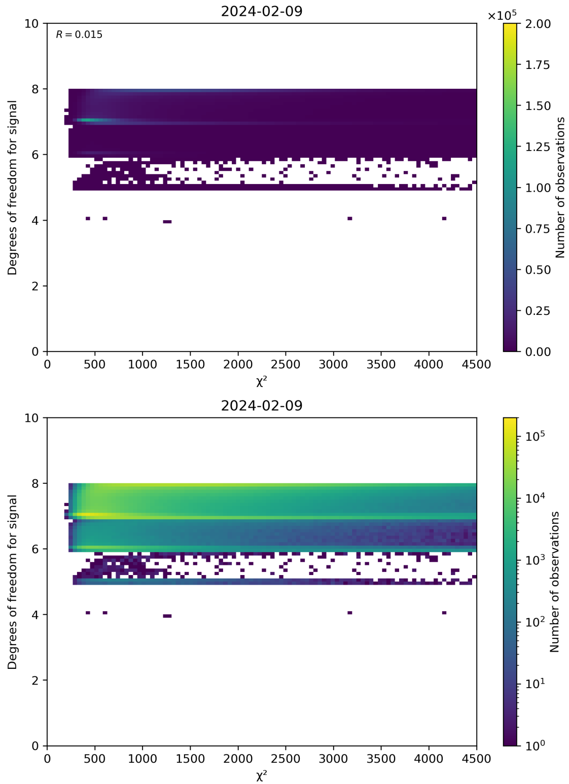
Figure 48: Scatter density plot of “ \chi^2 ” against “Degrees of freedom for signal” for 2024-02-08 to 2024-02-10.
