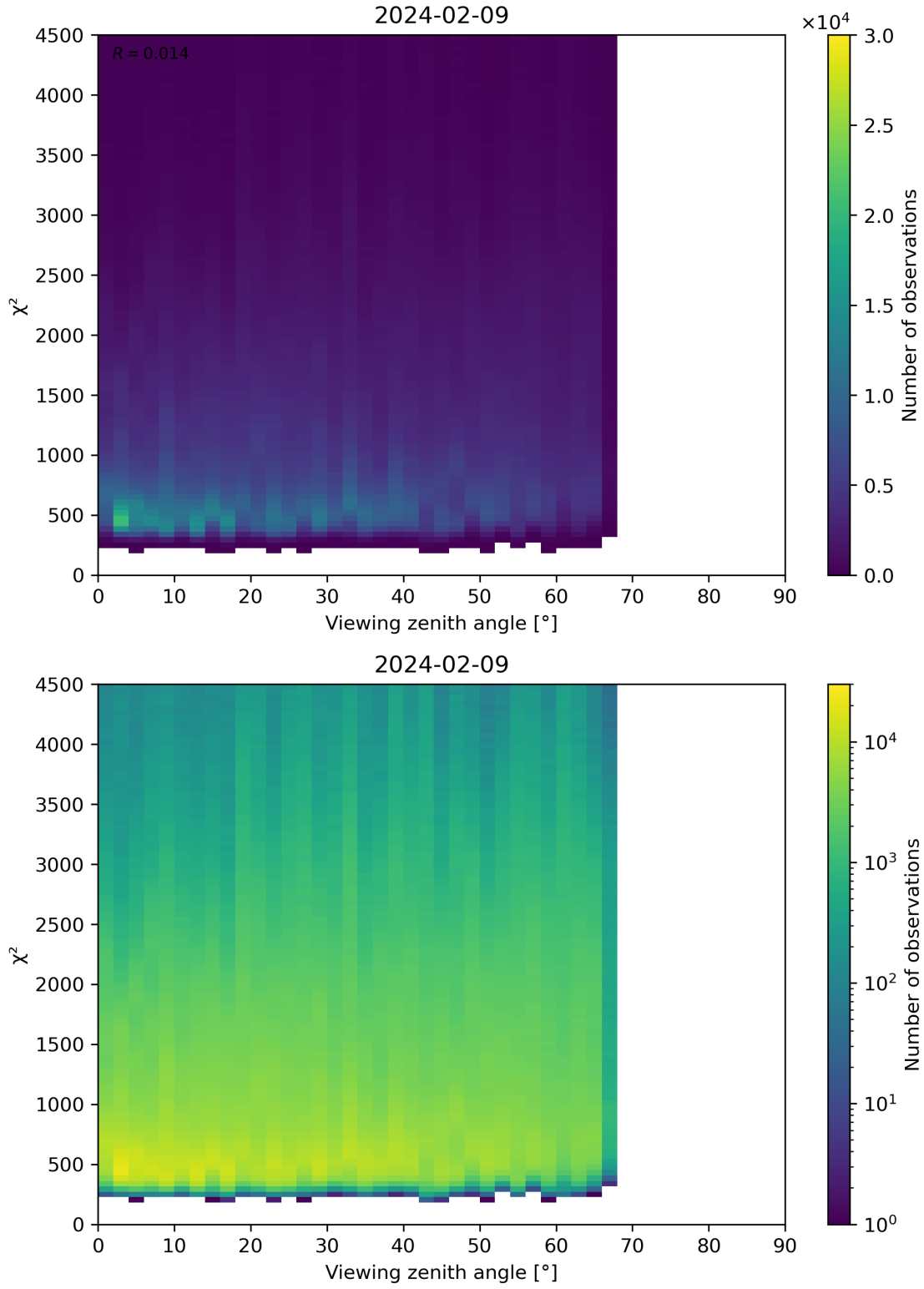
Figure 72: Scatter density plot of “Viewing zenith angle” against “ \chi^2 ” for 2024-02-08 to 2024-02-10.
