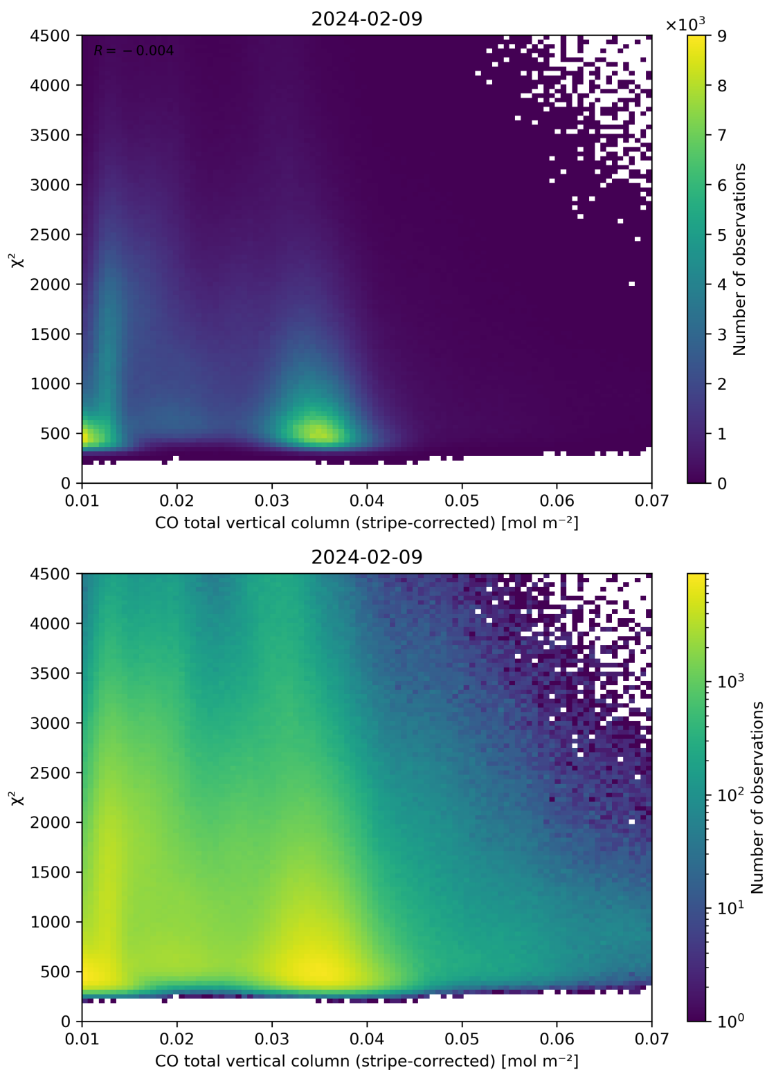
Figure 37: Scatter density plot of “CO total vertical column (stripe-corrected)” against “ \chi^2 ” for 2024-02-08 to 2024-02-10.
