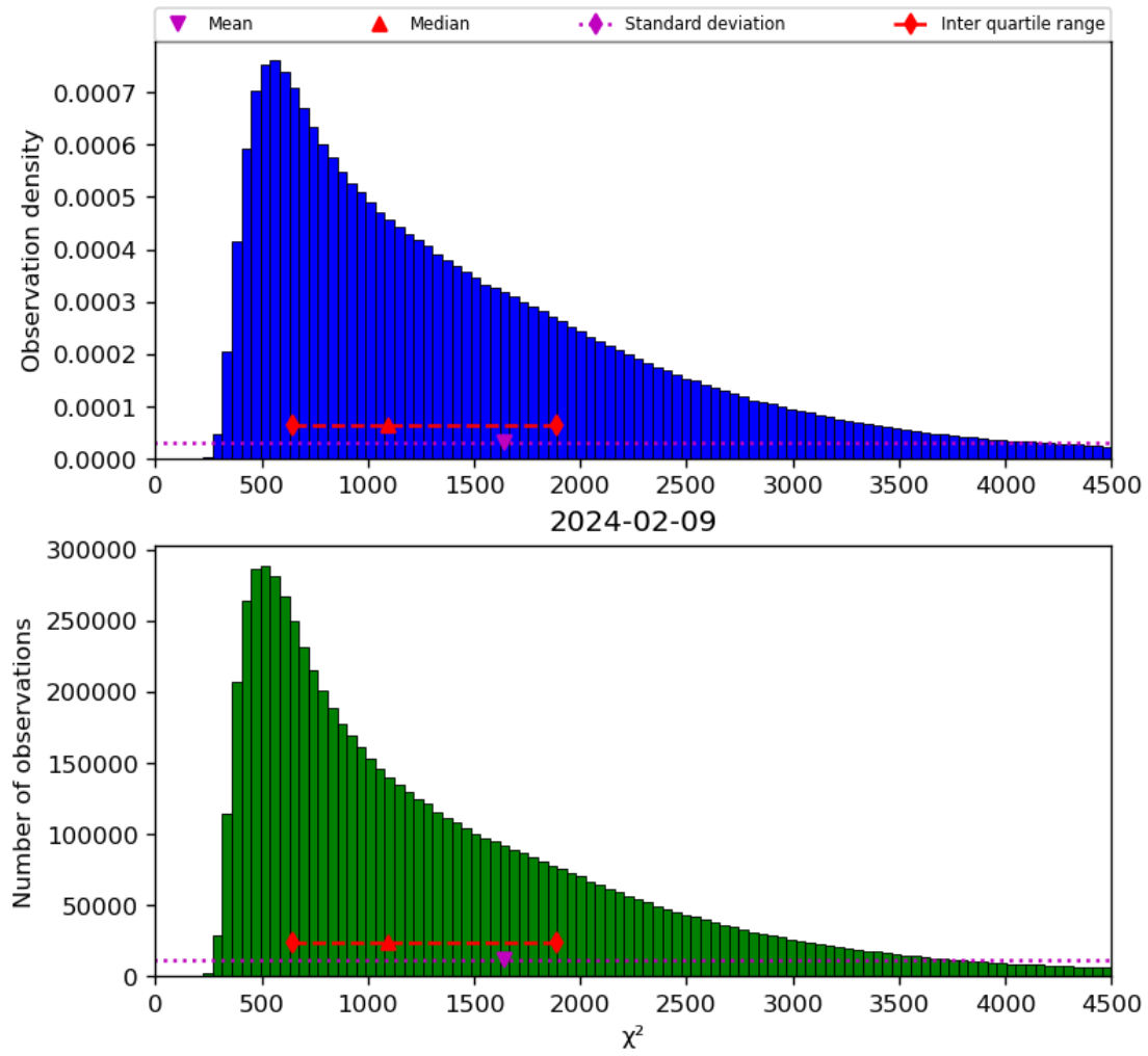
Figure 22: Histogram of " \chi^2 " for 2024-02-08 to 2024-02-10
