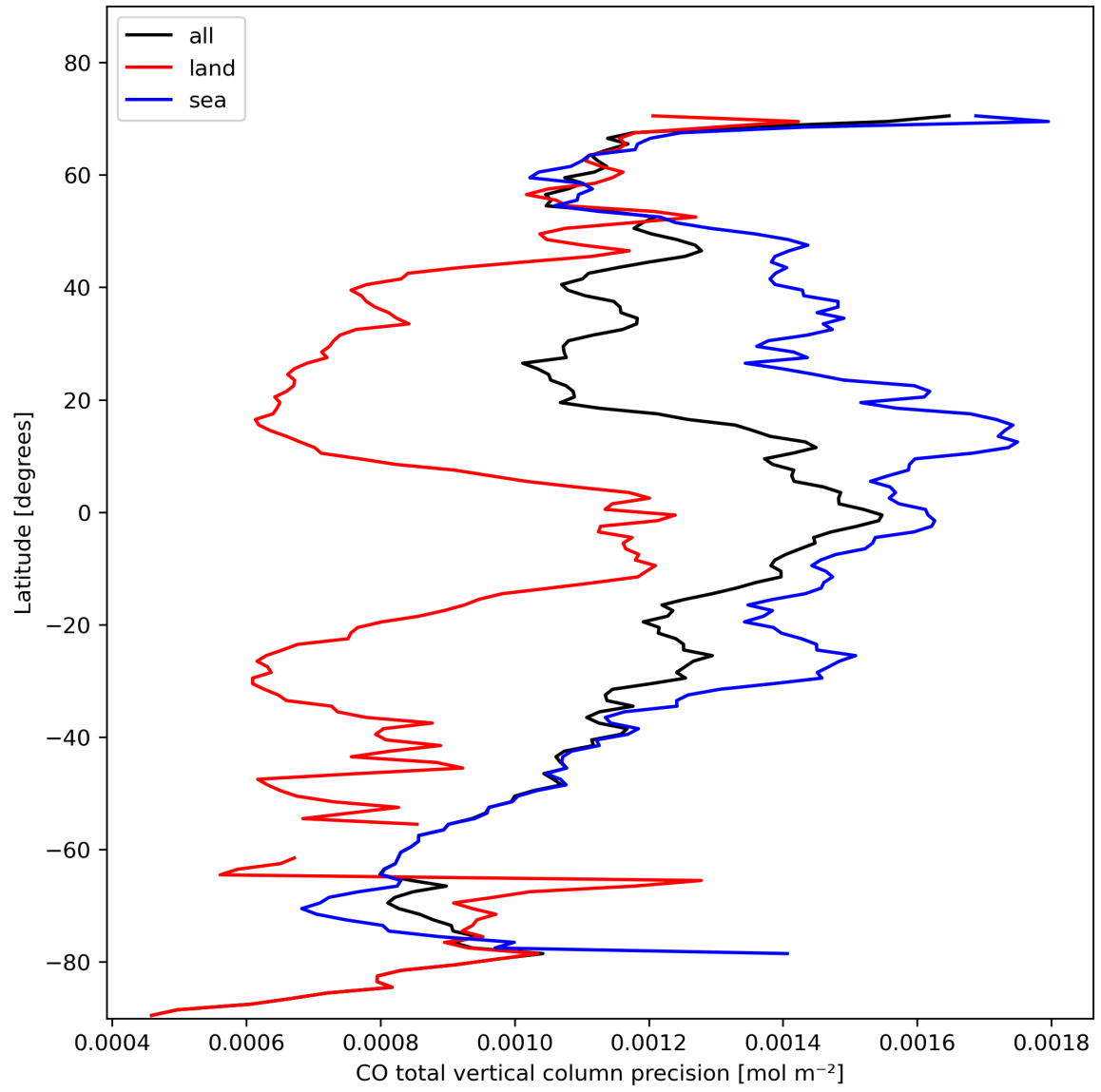
Figure 12: Zonal average of “CO total vertical column precision” for 2024-02-08 to 2024-02-10.
