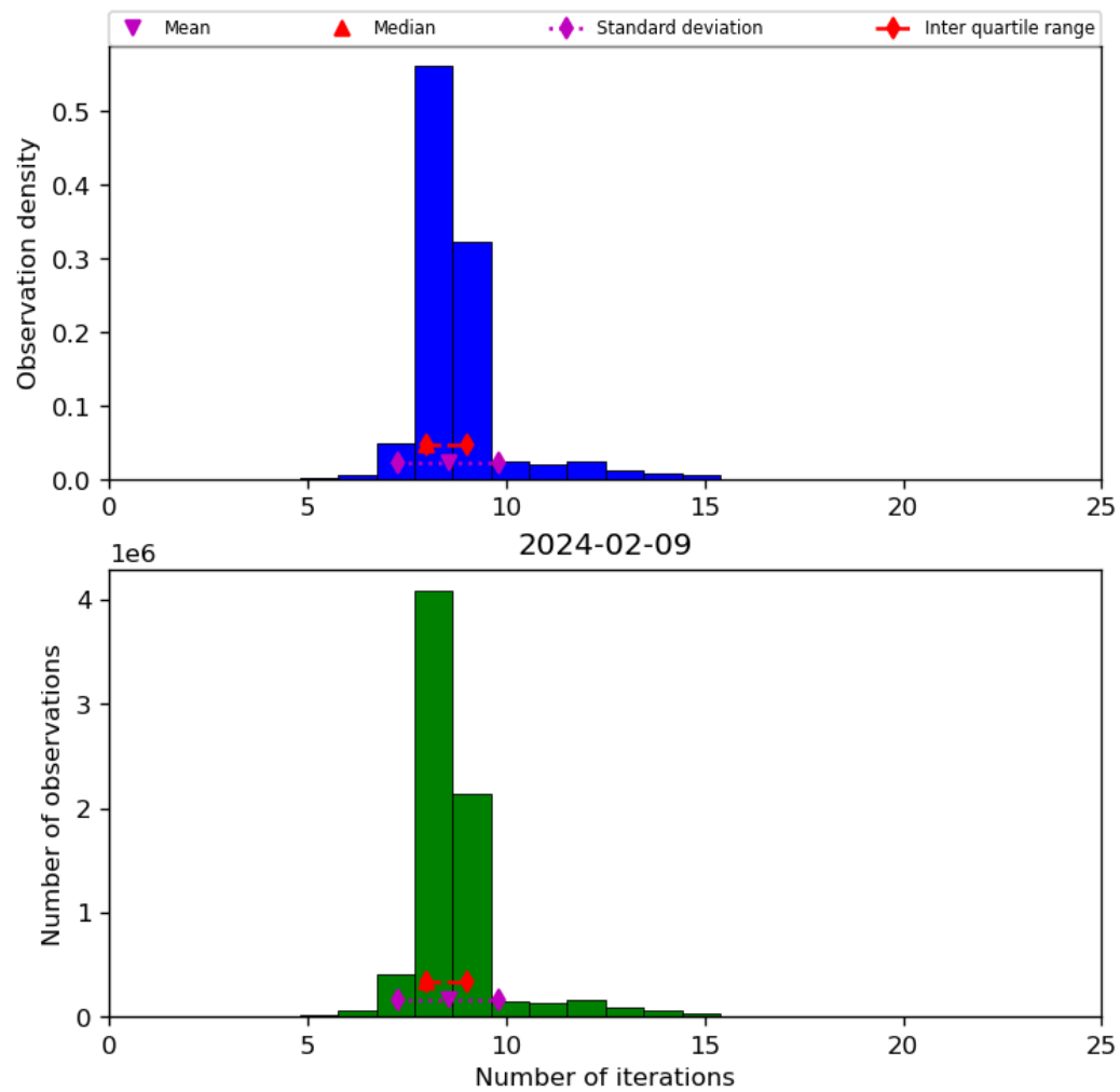
Figure 24: Histogram of “Number of iterations” for 2024-02-08 to 2024-02-10
