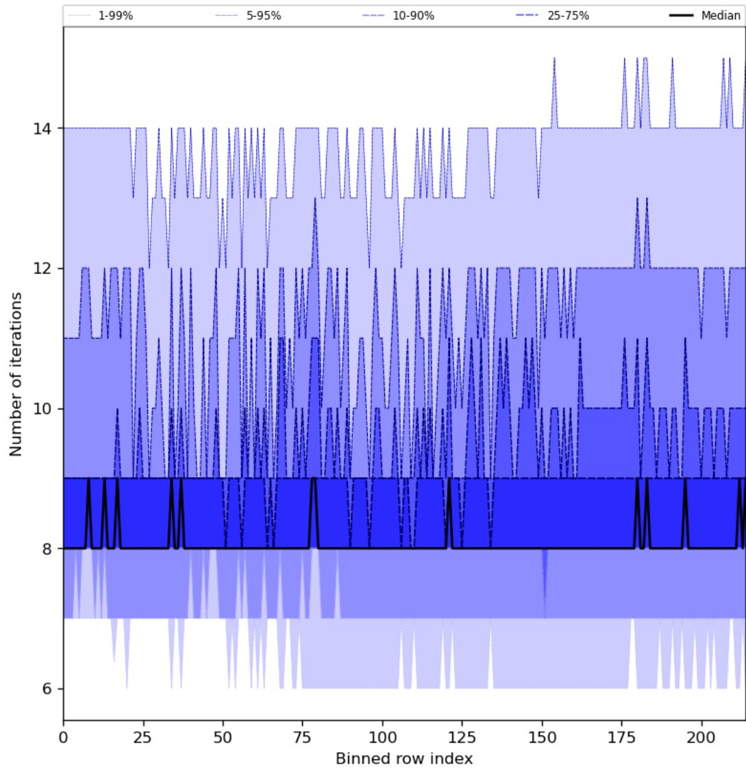
Figure 32: Along track statistics of “Number of iterations” for 2024-02-08 to 2024-02-10
