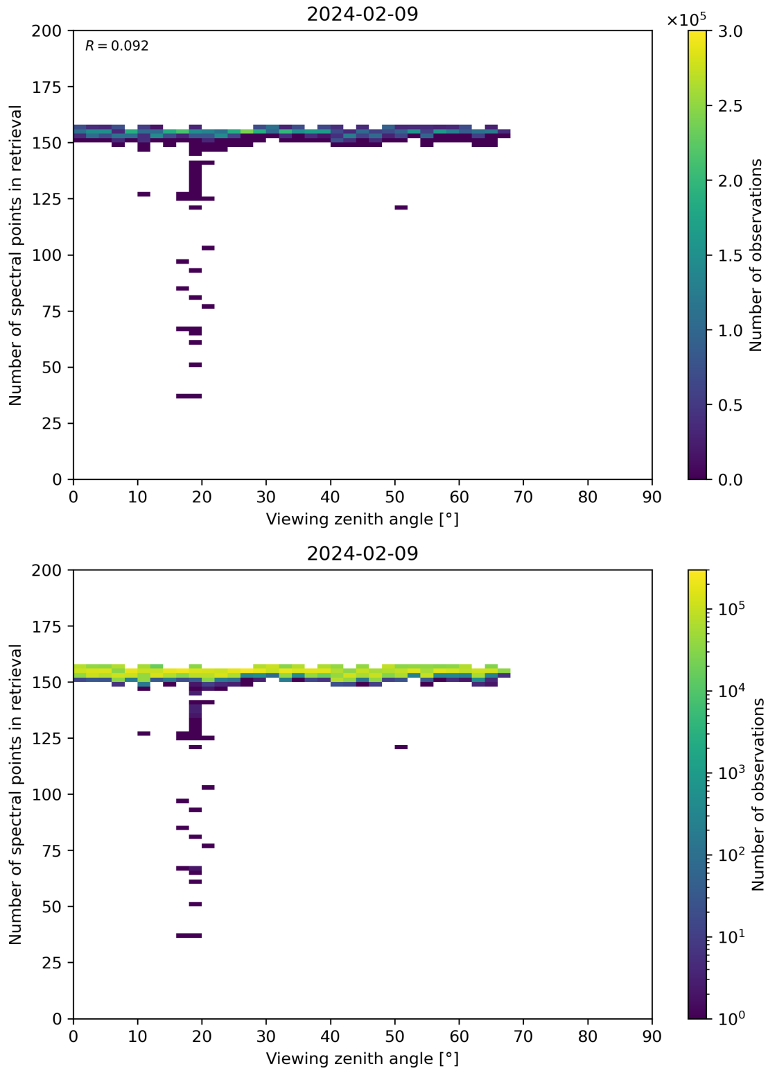
Figure 76: Scatter density plot of “Viewing zenith angle” against “Number of spectral points in retrieval” for 2024-02-08 to 2024-02-10.
