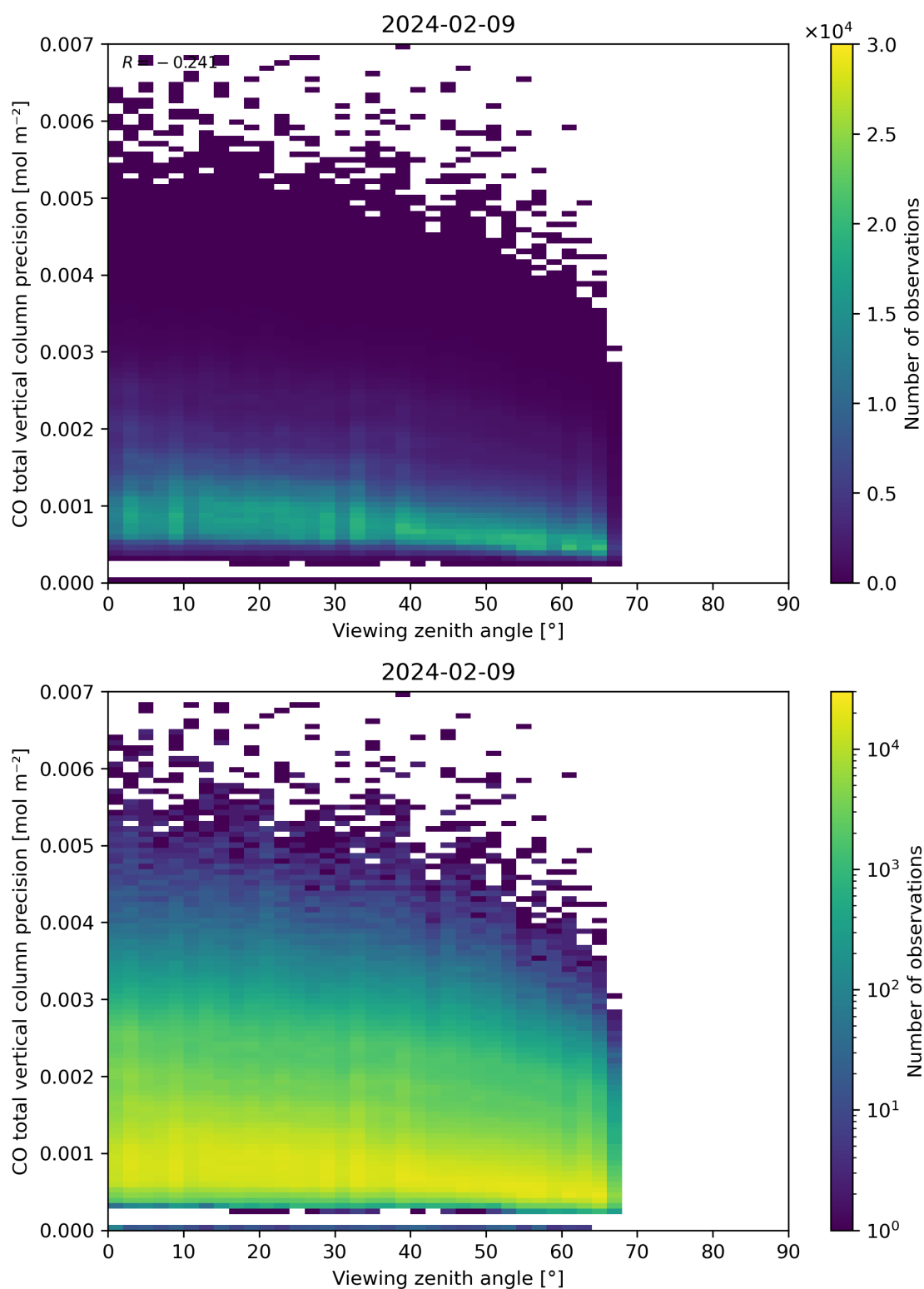
Figure 71: Scatter density plot of “Viewing zenith angle” against “CO total vertical column precision” for 2024-02-08 to 2024-02-10.
