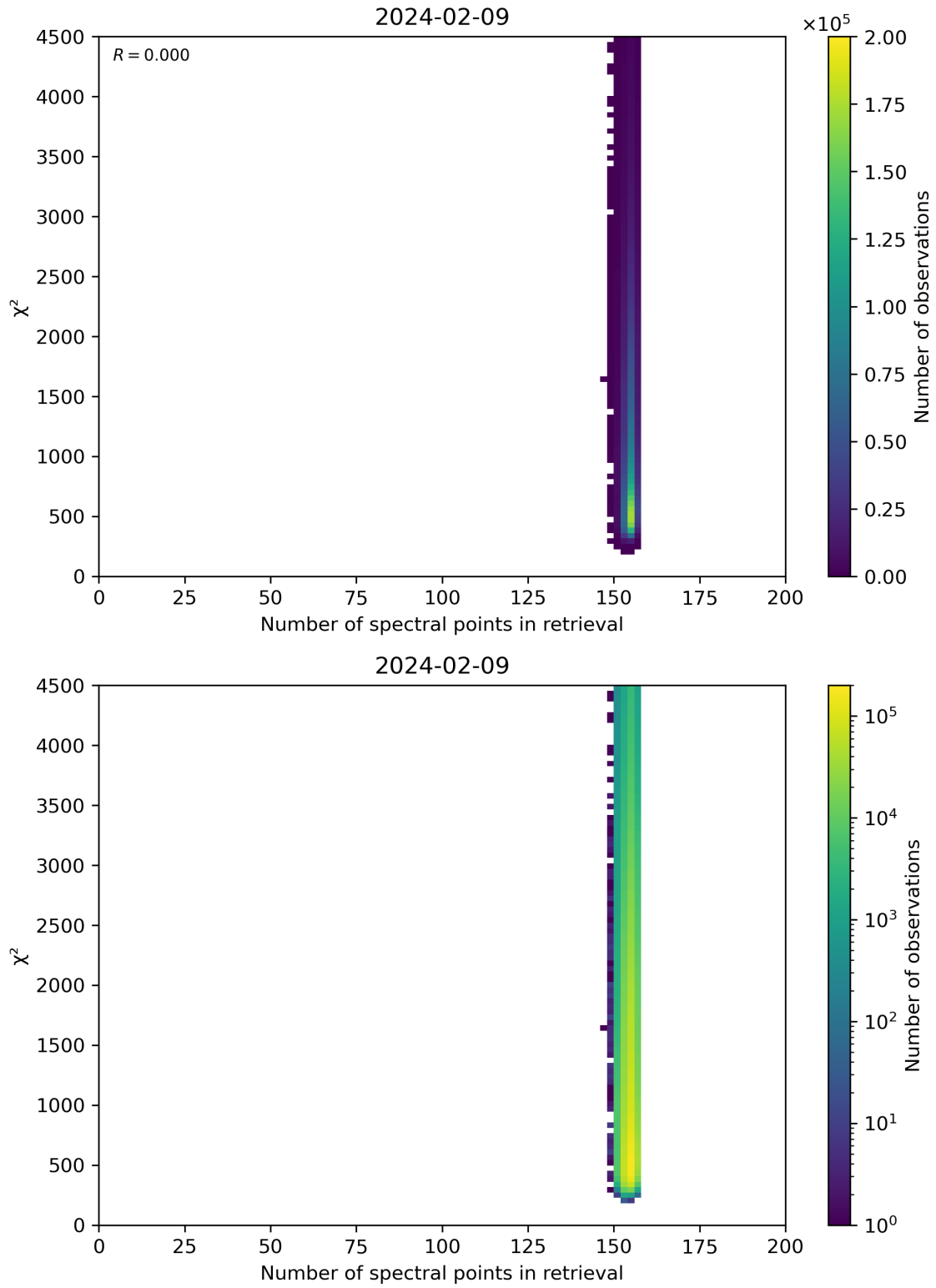
Figure 58: Scatter density plot of “Number of spectral points in retrieval” against “ \chi^2 ” for 2024-02-08 to 2024-02-10.
