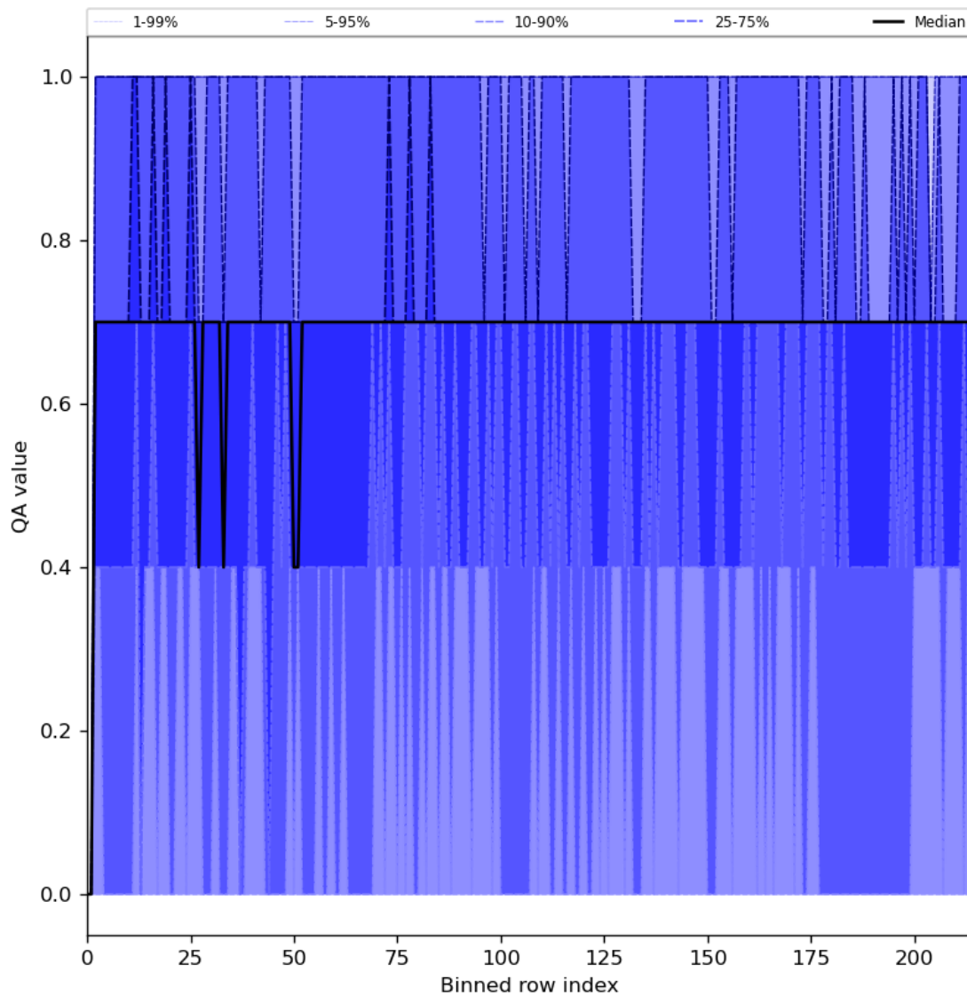
Figure 25: Along track statistics of “QA value” for 2024-02-08 to 2024-02-10
