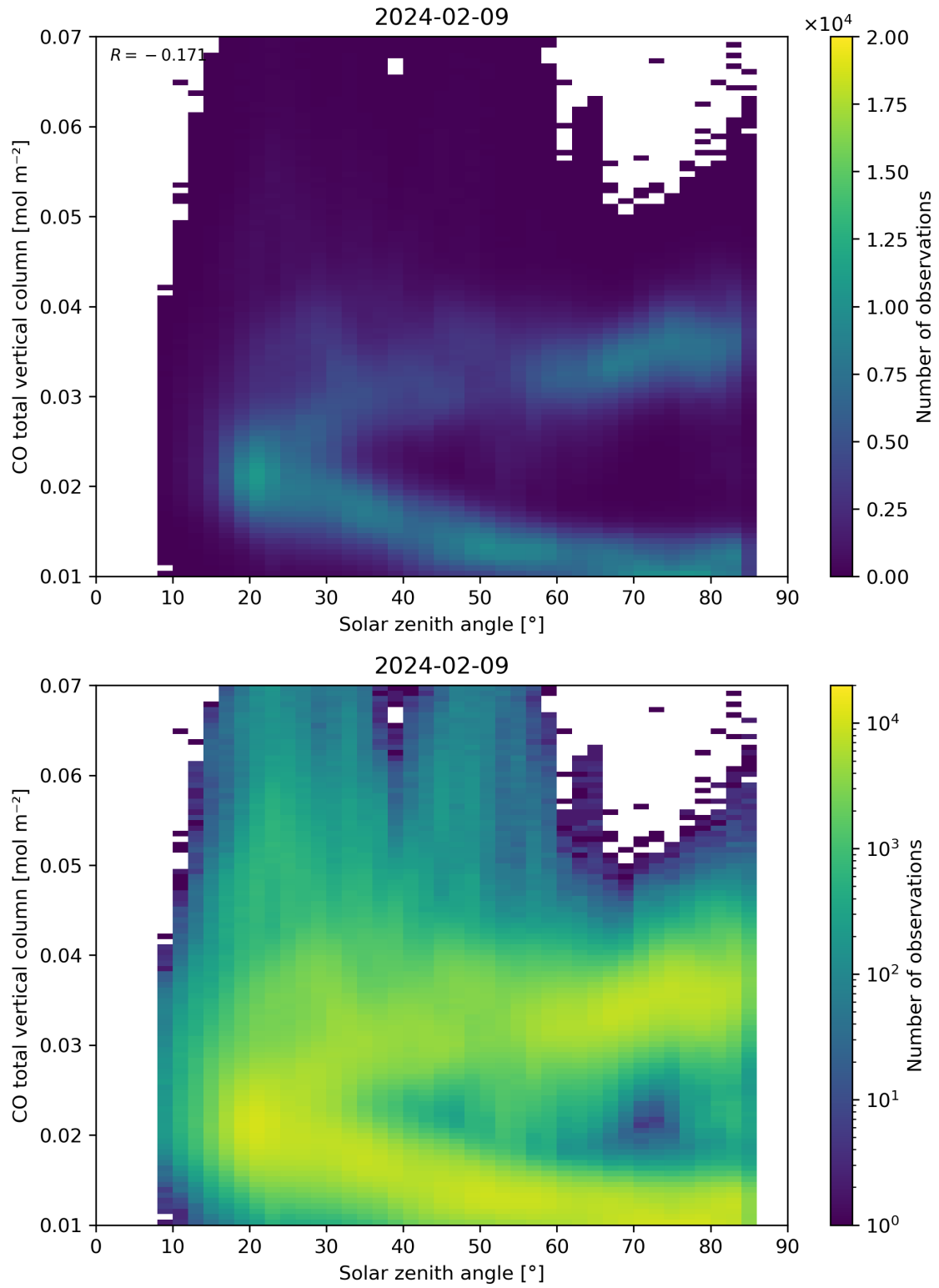
Figure 61: Scatter density plot of “Solar zenith angle” against “CO total vertical column” for 2024-02-08 to 2024-02-10.
