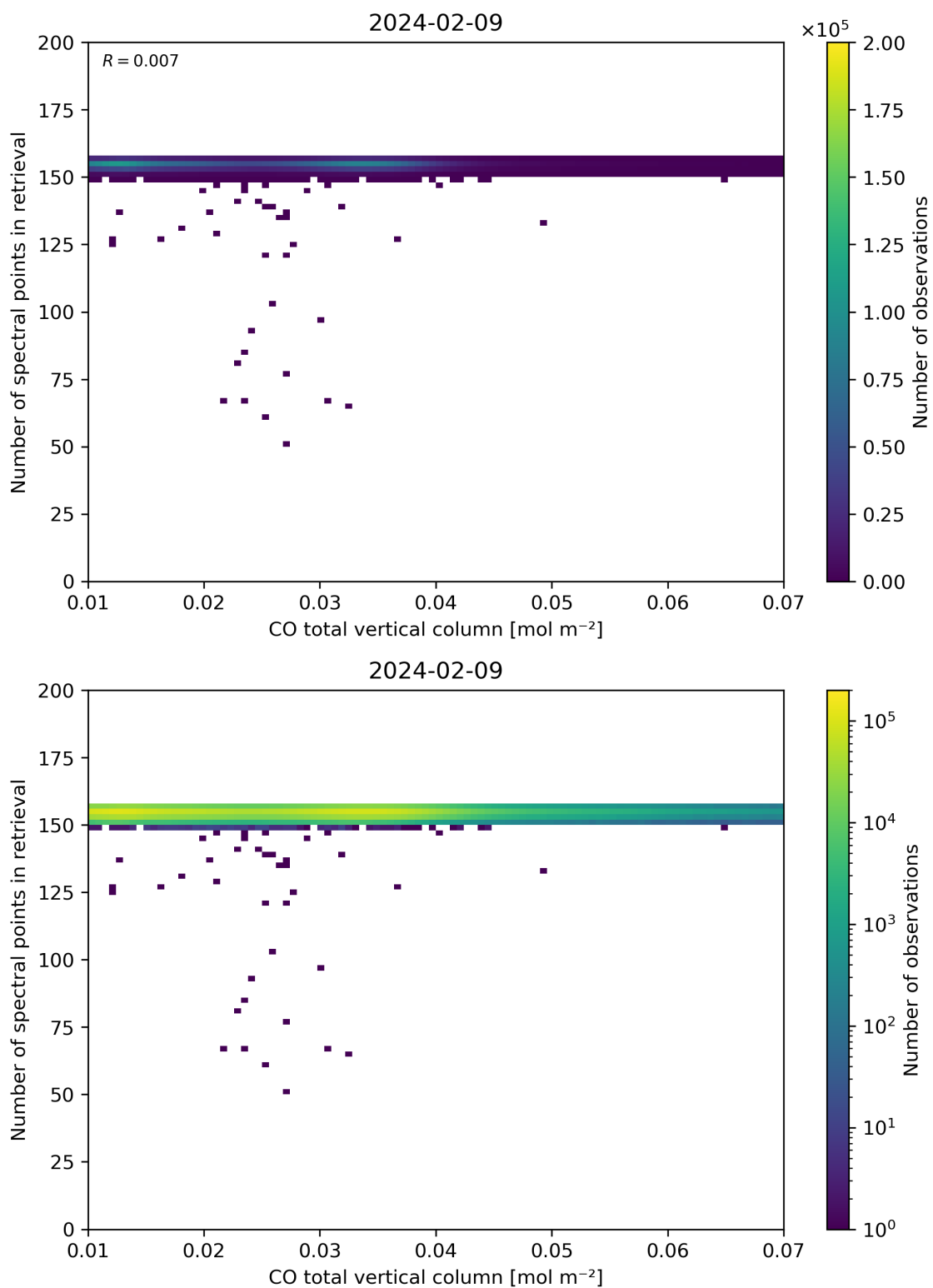
Figure 43: Scatter density plot of “CO total vertical column” against “Number of spectral points in retrieval” for 2024-02-08 to 2024-02-10.
