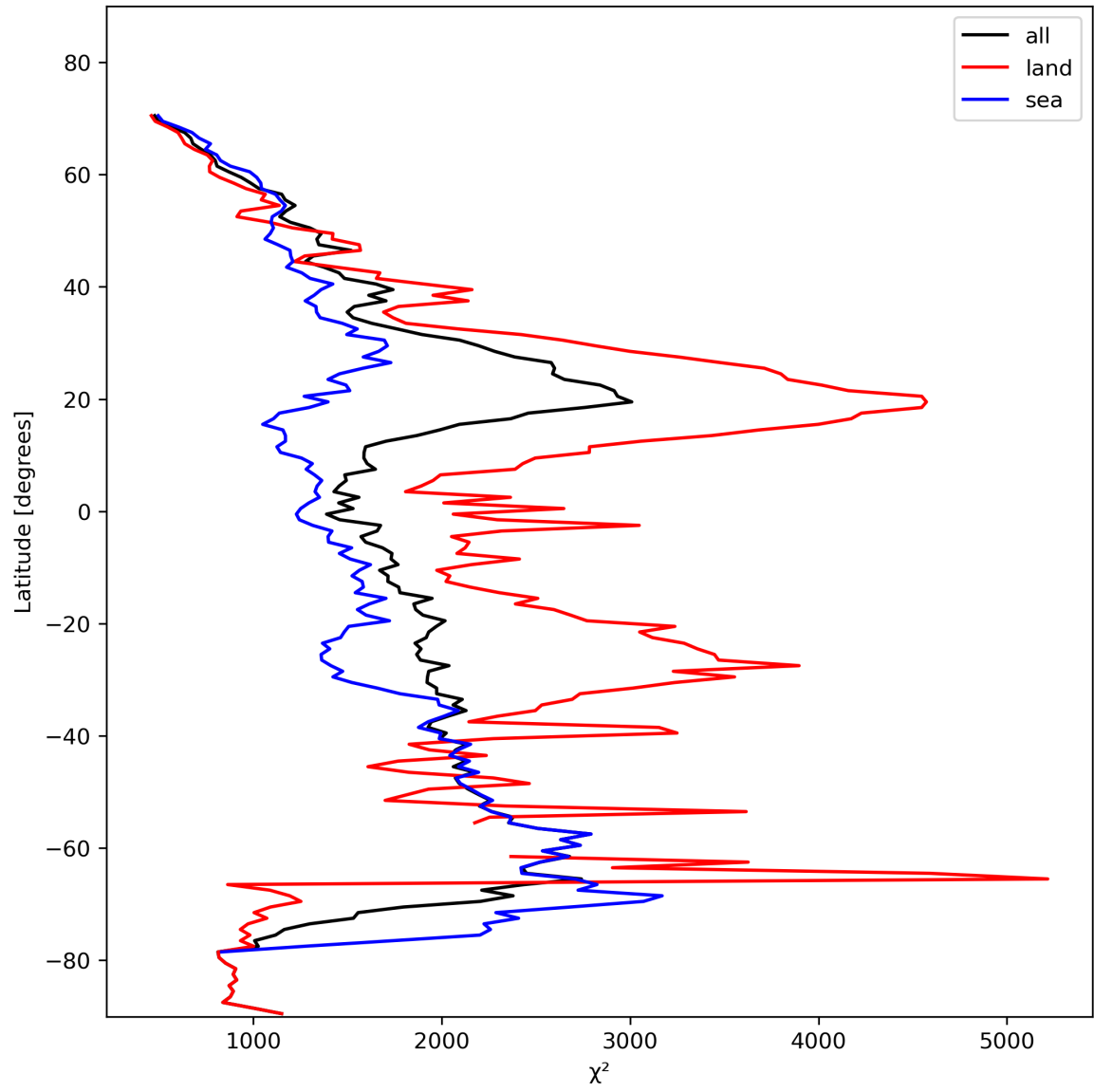
Figure 14: Zonal average of “ \chi^2 ” for 2024-02-08 to 2024-02-10.
