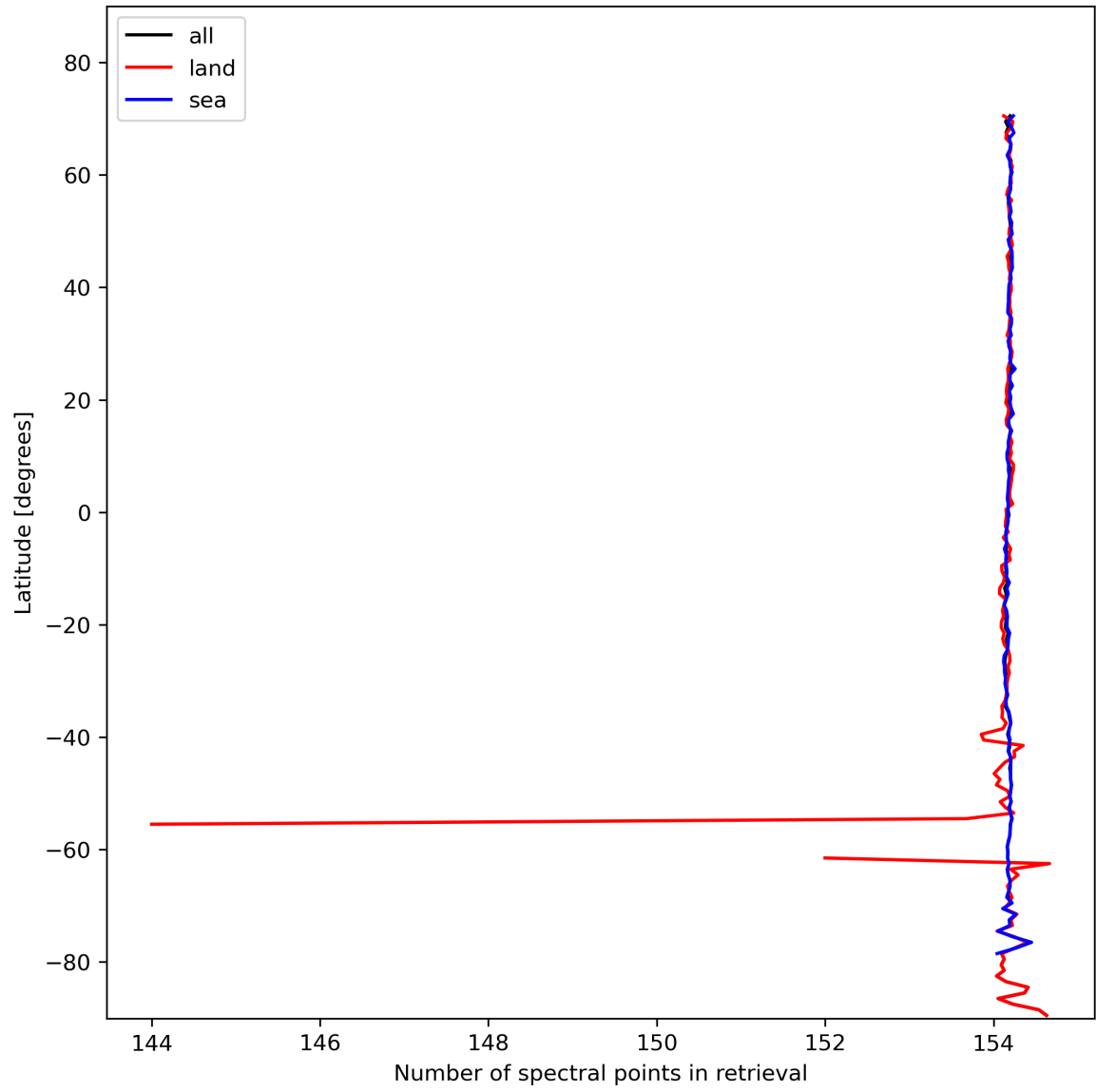
Figure 13: Zonal average of “Number of spectral points in retrieval” for 2024-02-08 to 2024-02-10.
