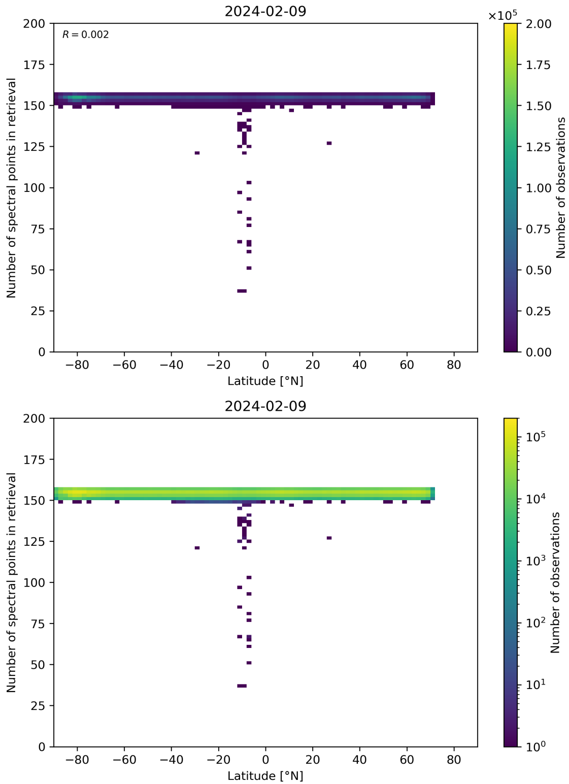
Figure 57: Scatter density plot of “Latitude” against “Number of spectral points in retrieval” for 2024-02-08 to 2024-02-10.
