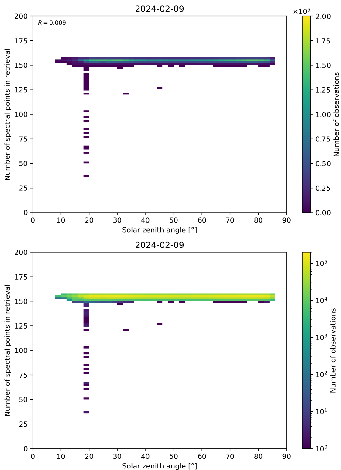
Figure 68: Scatter density plot of “Solar zenith angle” against “Number of spectral points in retrieval” for 2024-02-08 to 2024-02-10.
