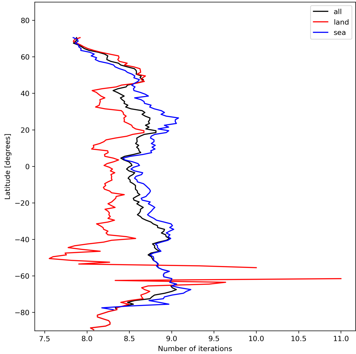
Figure 16: Zonal average of “Number of iterations” for 2024-02-08 to 2024-02-10.
