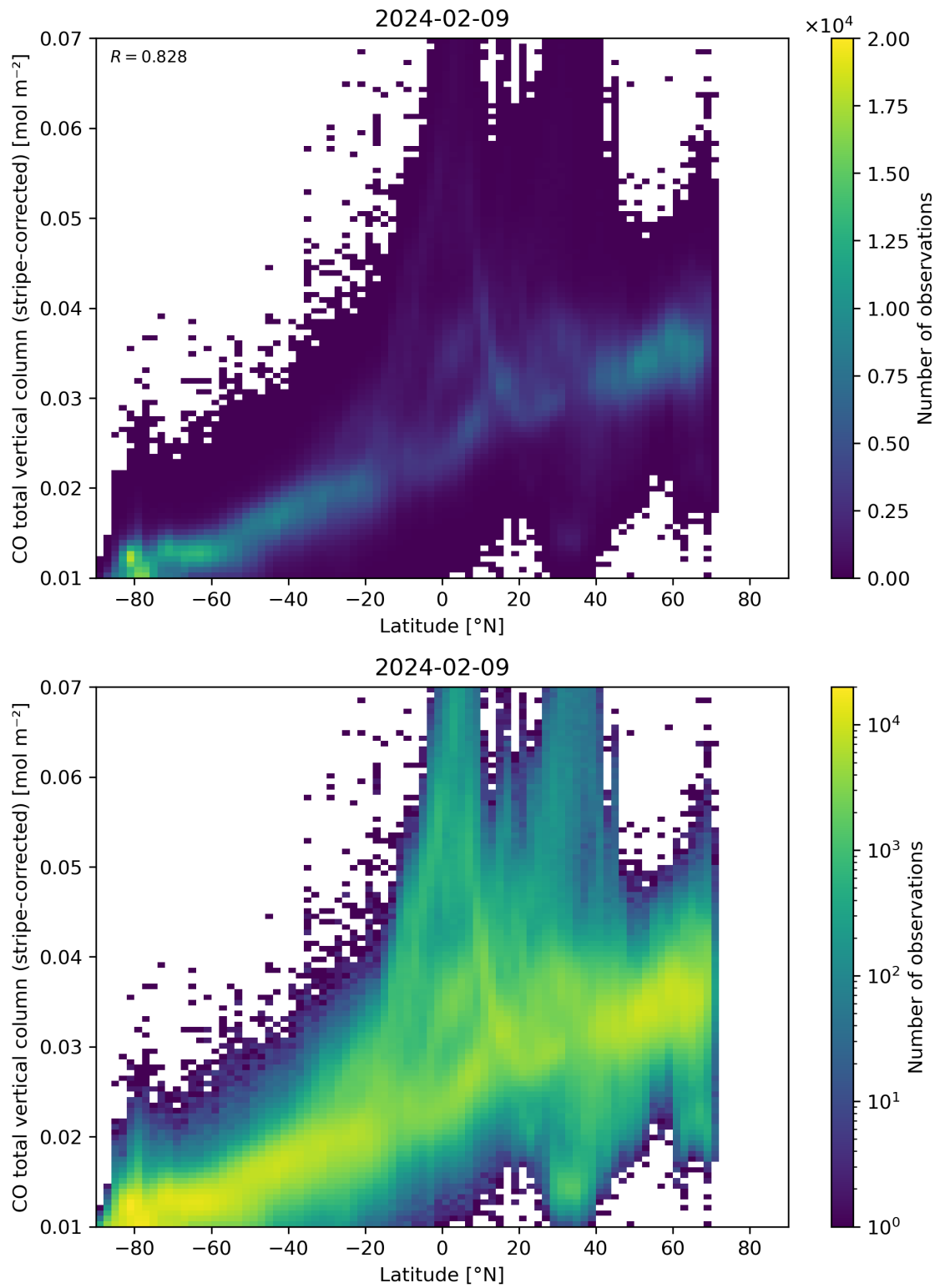
Figure 52: Scatter density plot of “Latitude” against “CO total vertical column (stripe-corrected)” for 2024-02-08 to 2024-02-10.
