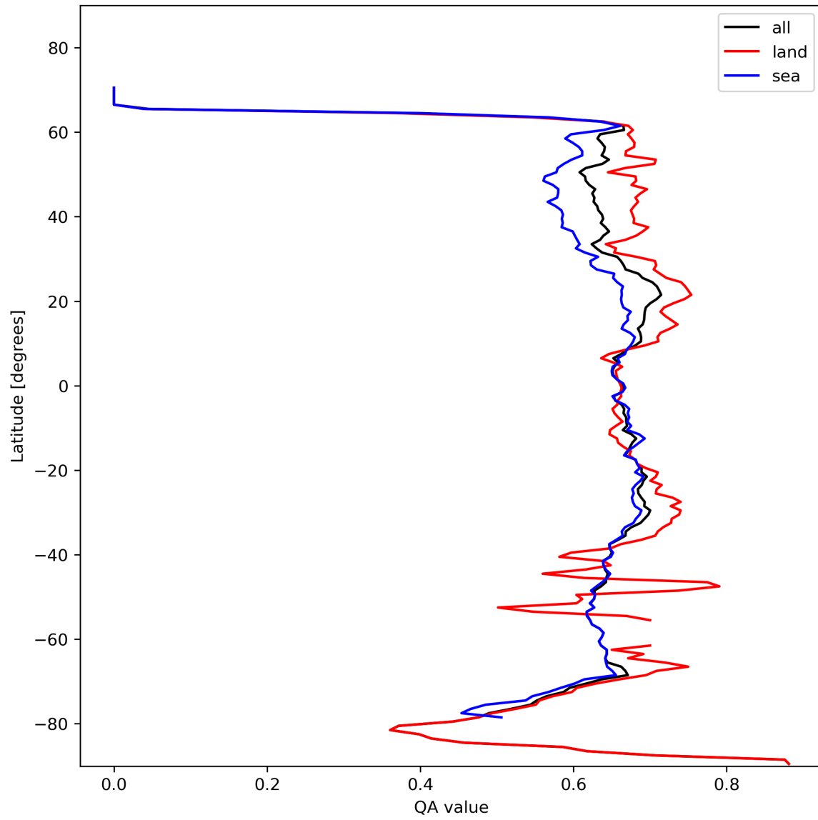
Figure 9: Zonal average of “QA value” for 2024-02-08 to 2024-02-10.
