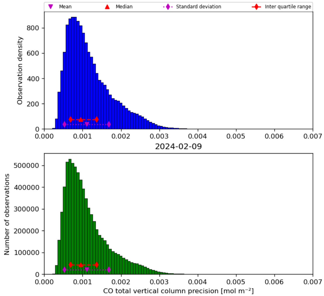
Figure 20: Histogram of “CO total vertical column precision” for 2024-02-08 to 2024-02-10
