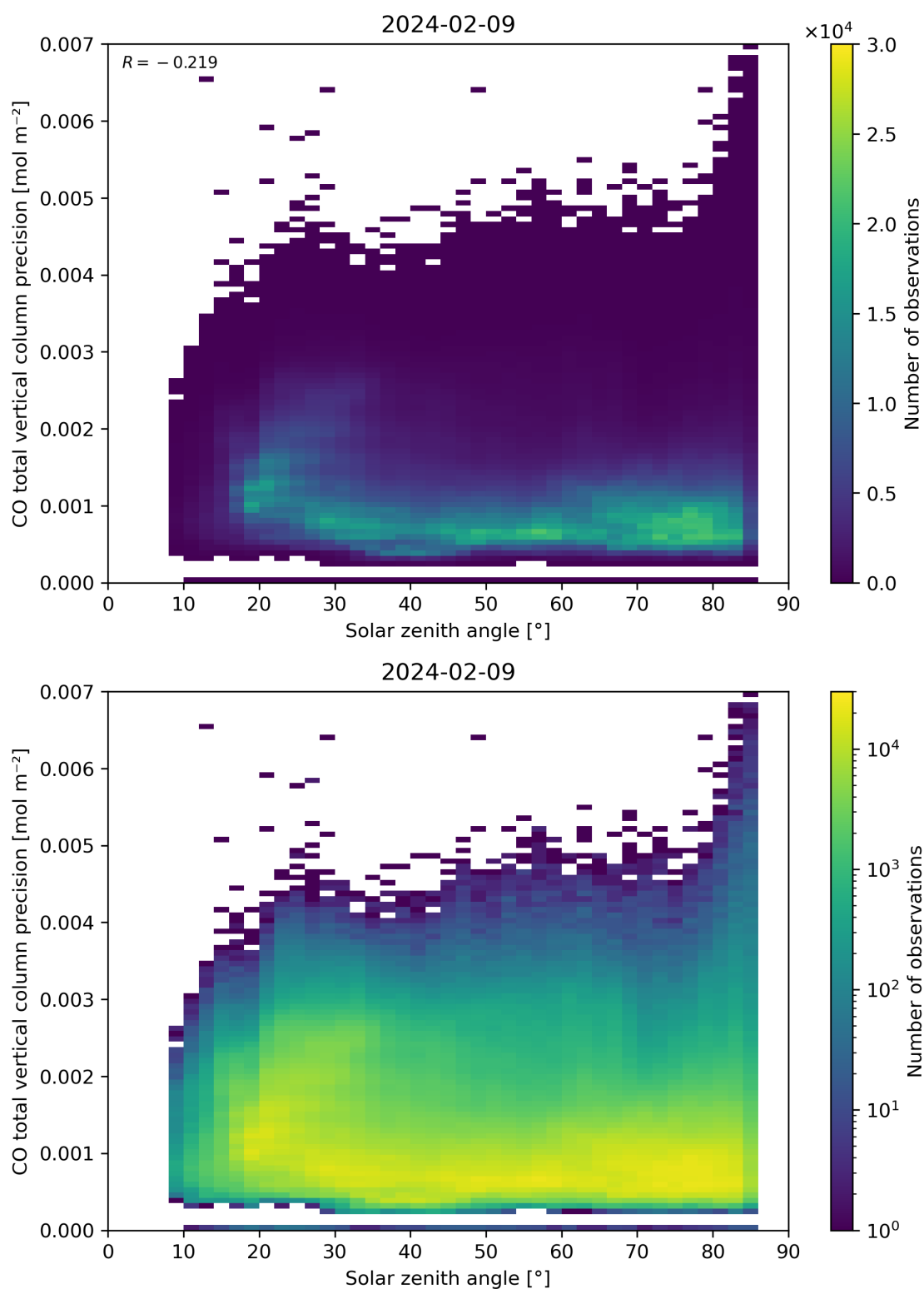
Figure 63: Scatter density plot of “Solar zenith angle” against “CO total vertical column precision” for 2024-02-08 to 2024-02-10.
