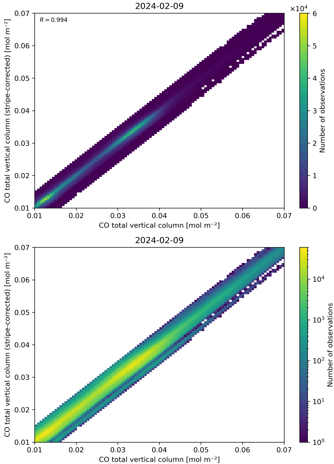
Figure 33: Scatter density plot of “CO total vertical column” against “CO total vertical column (stripe-corrected)” for 2024-02-08 to 2024-02-10.
