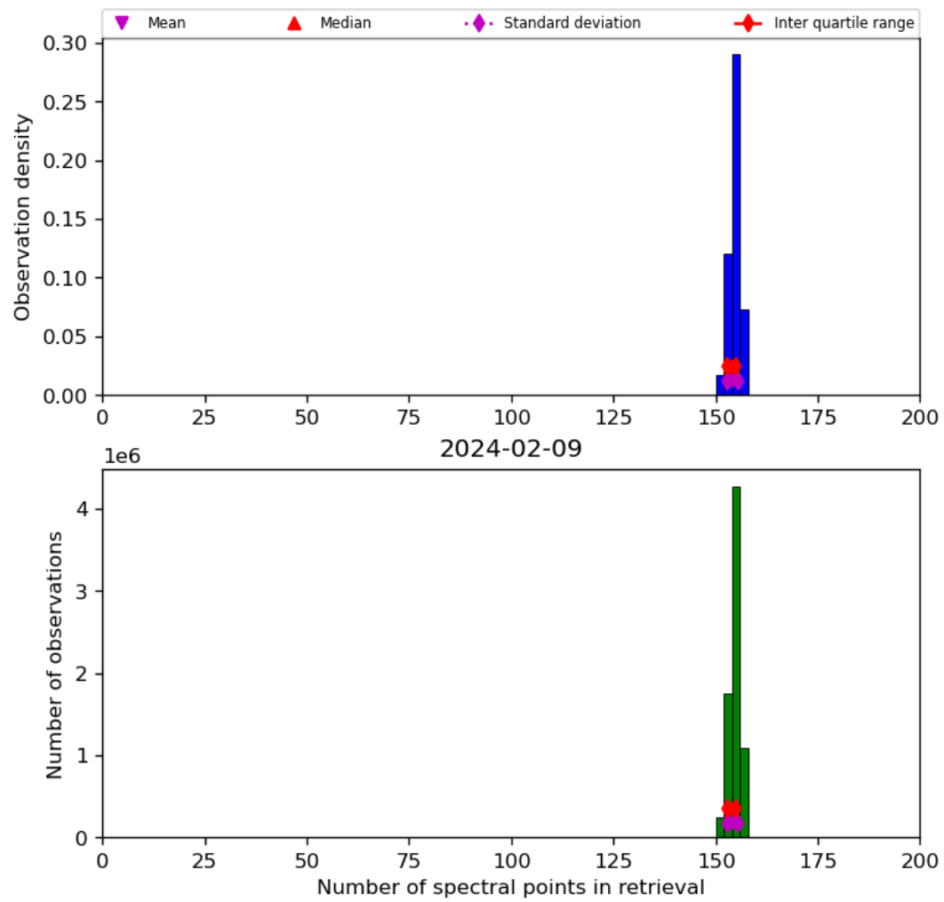
Figure 21: Histogram of “Number of spectral points in retrieval” for 2024-02-08 to 2024-02-10
