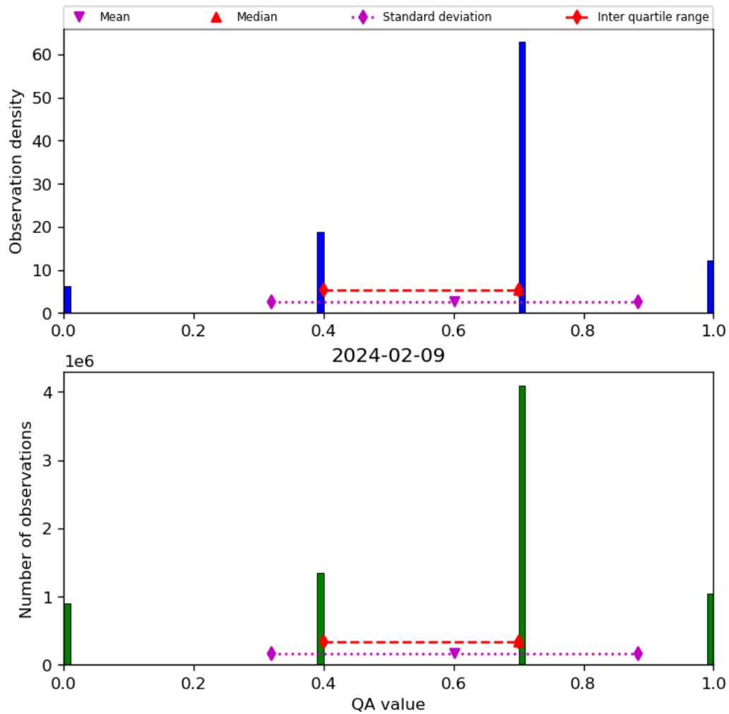
Figure 17: Histogram of “QA value” for 2024-02-08 to 2024-02-10
