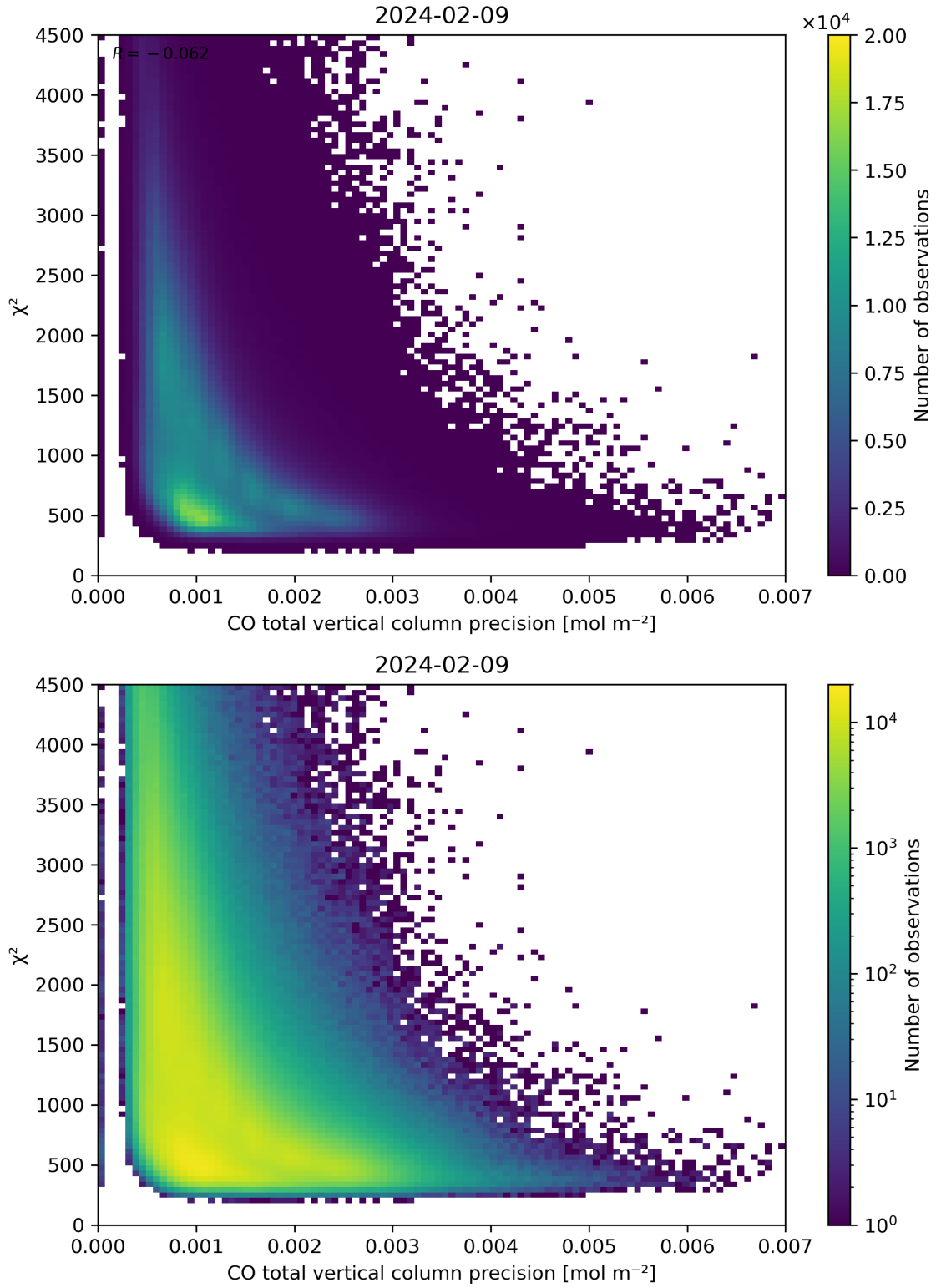
Figure 44: Scatter density plot of “CO total vertical column precision” against “ \chi^2 ” for 2024-02-08 to 2024-02-10.
