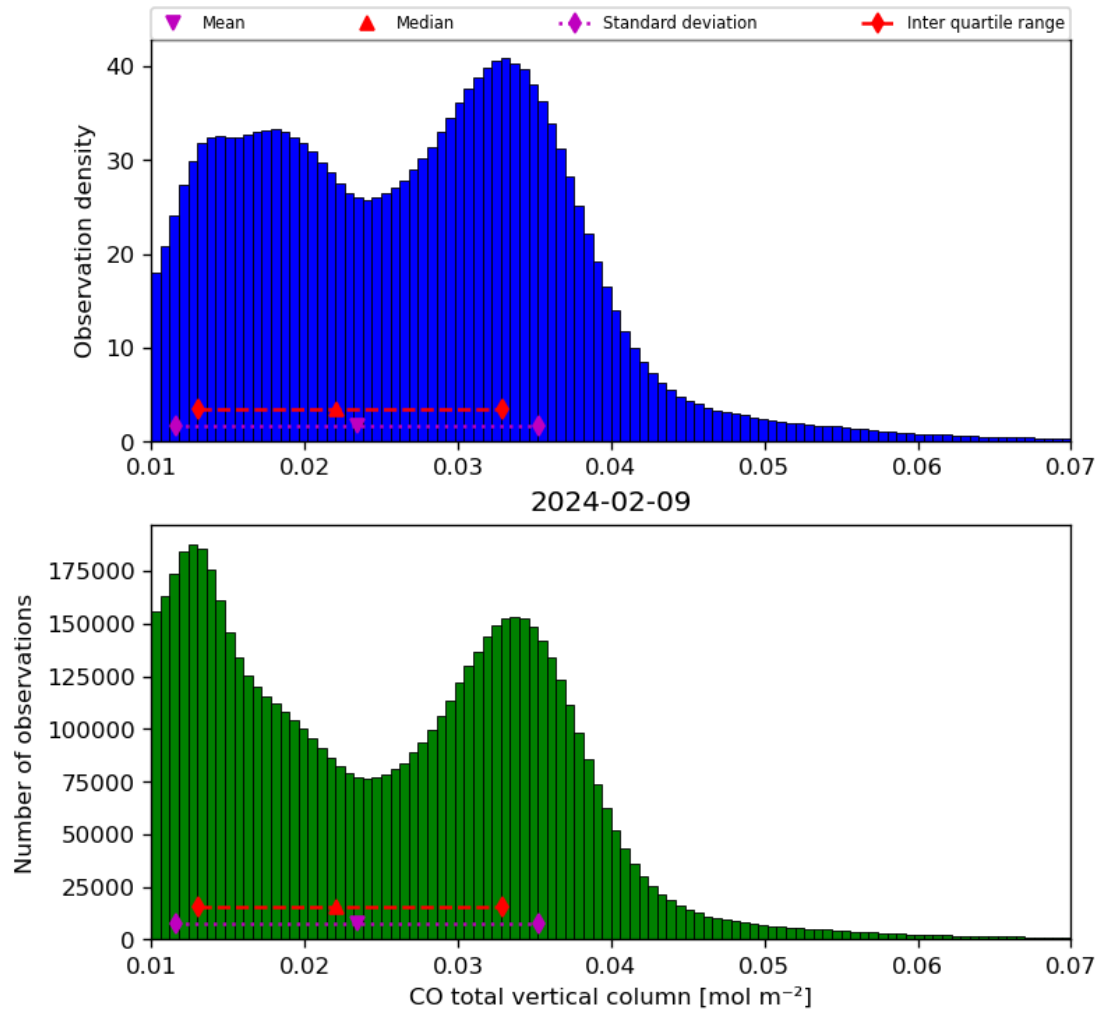
Figure 18: Histogram of “CO total vertical column” for 2024-02-08 to 2024-02-10
