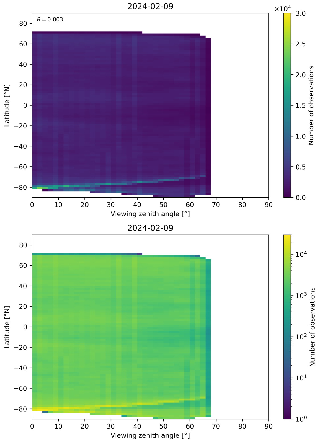
Figure 74: Scatter density plot of “Viewing zenith angle” against “Latitude” for 2024-02-08 to 2024-02-10.
