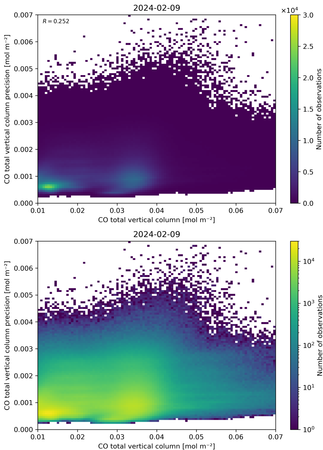
Figure 34: Scatter density plot of “CO total vertical column” against “CO total vertical column precision” for 2024-02-08 to 2024-02-10.
