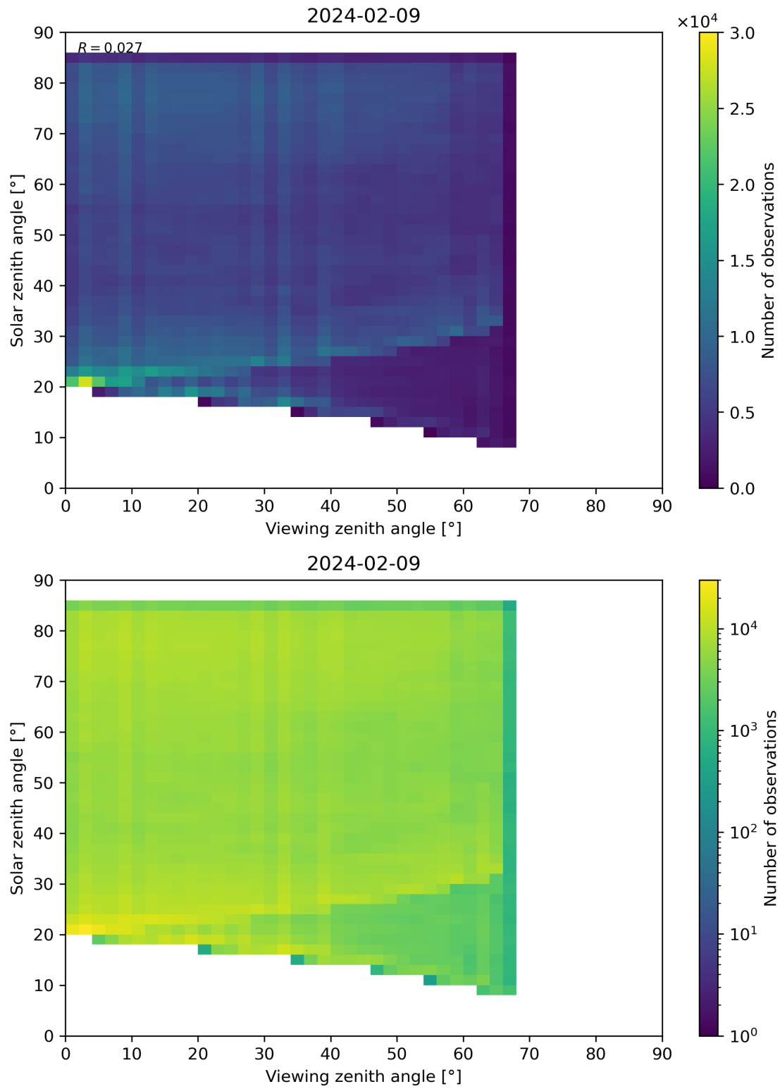
Figure 77: Scatter density plot of “Viewing zenith angle” against “Solar zenith angle” for 2024-02-08 to 2024-02-10.
