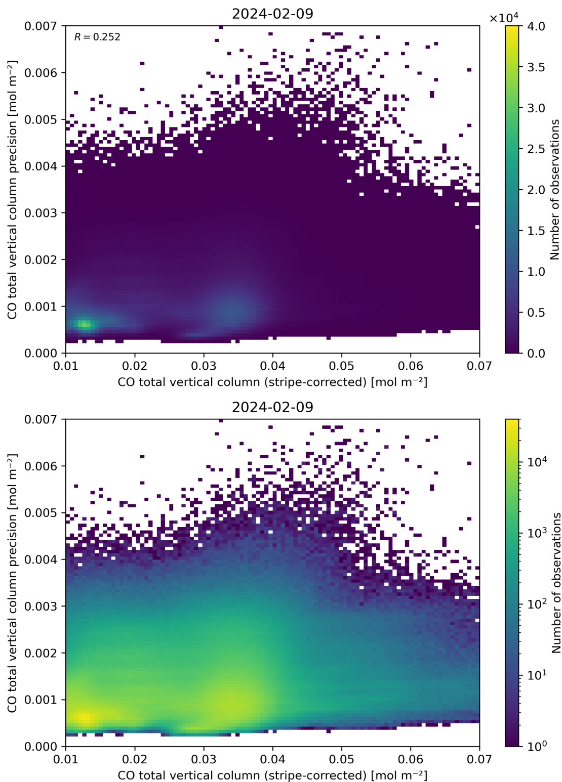
Figure 36: Scatter density plot of “CO total vertical column (stripe-corrected)” against “CO total vertical column precision” for 2024-02-08 to 2024-02-10.
