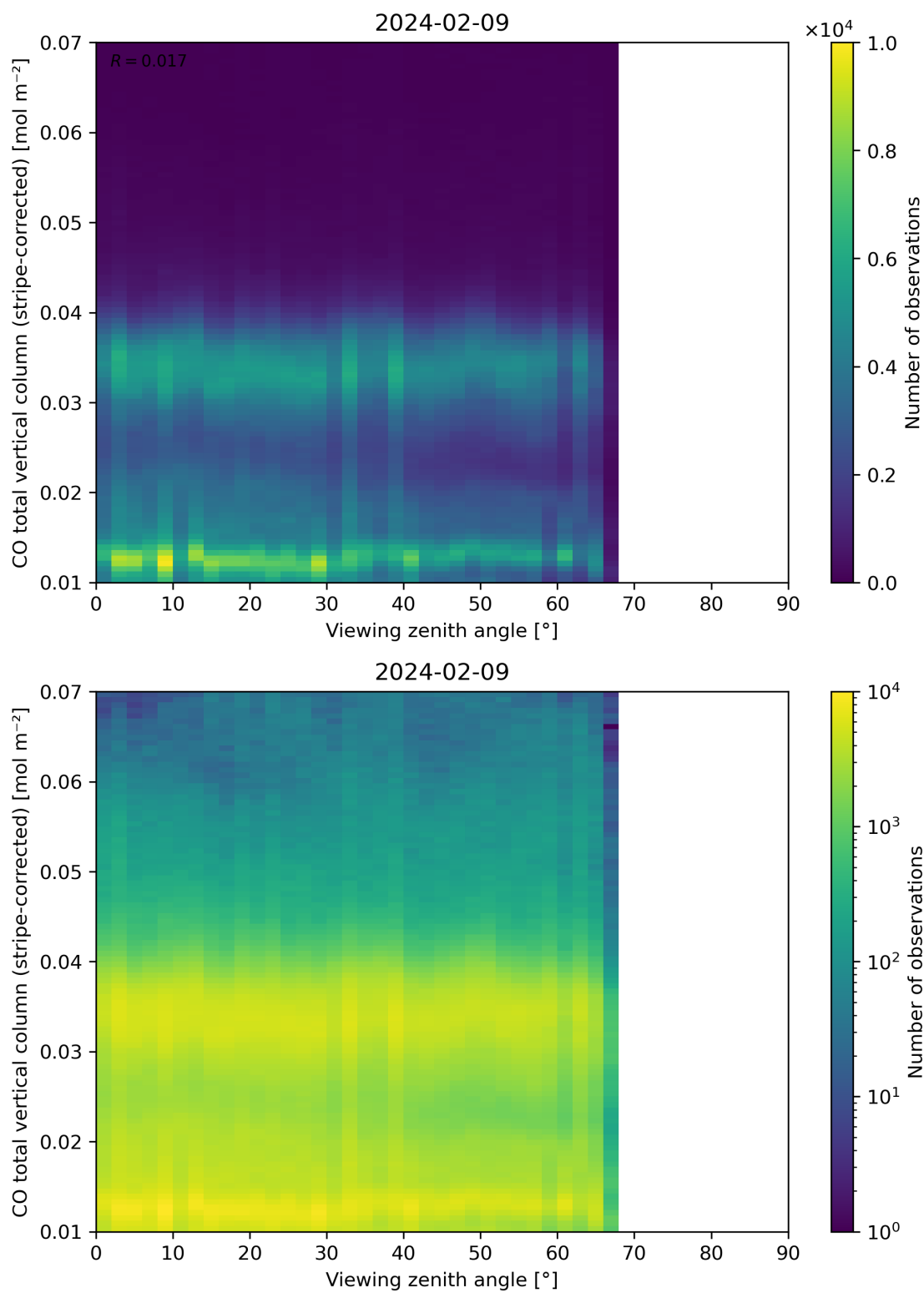
Figure 70: Scatter density plot of “Viewing zenith angle” against “CO total vertical column (stripe-corrected)” for 2024-02-08 to 2024-02-10.
