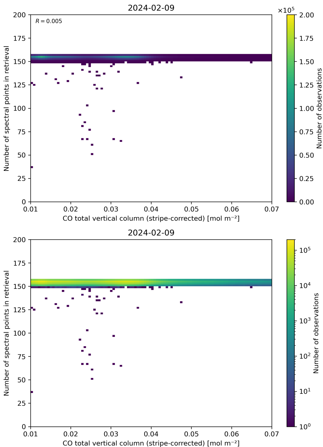
Figure 40: Scatter density plot of “CO total vertical column (stripe-corrected)” against “Number of spectral points in retrieval” for 2024-02-08 to 2024-02-10.
