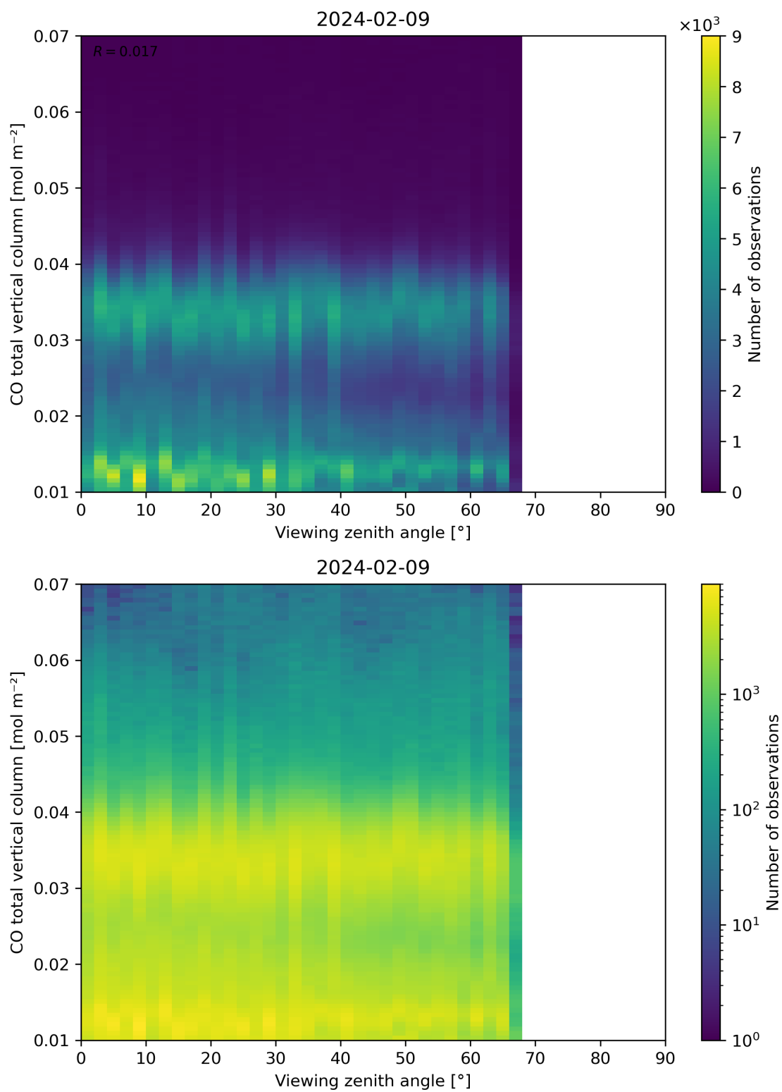
Figure 69: Scatter density plot of “Viewing zenith angle” against “CO total vertical column” for 2024-02-08 to 2024-02-10.
