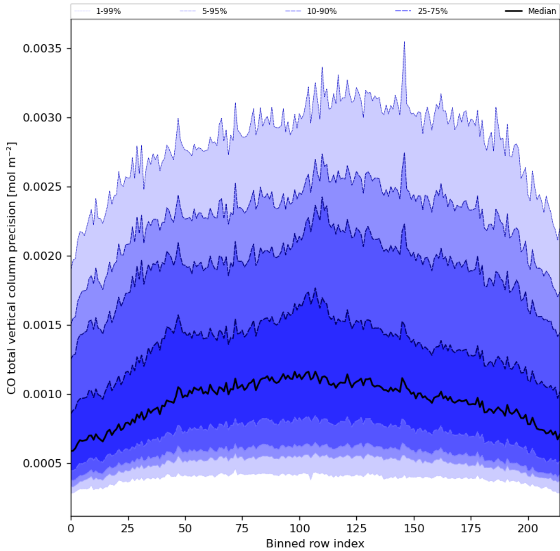
Figure 28: Along track statistics of “CO total vertical column precision” for 2024-02-08 to 2024-02-10
