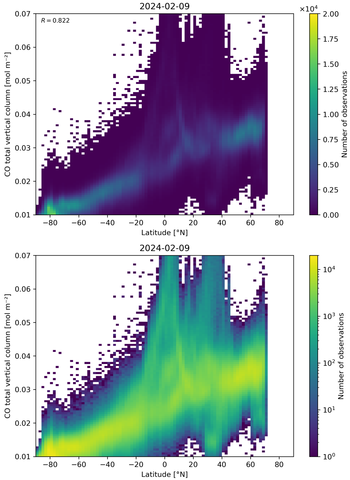
Figure 51: Scatter density plot of “Latitude” against “CO total vertical column” for 2024-02-08 to 2024-02-10.
