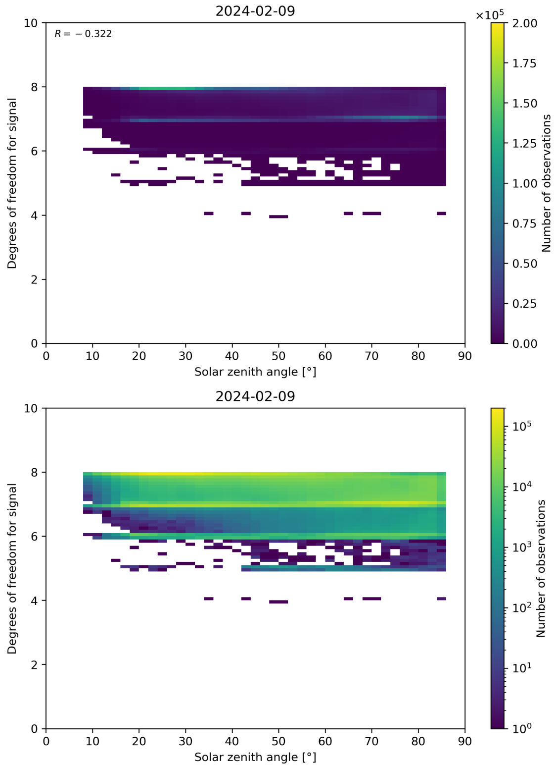
Figure 65: Scatter density plot of “Solar zenith angle” against “Degrees of freedom for signal” for 2024-02-08 to 2024-02-10.
