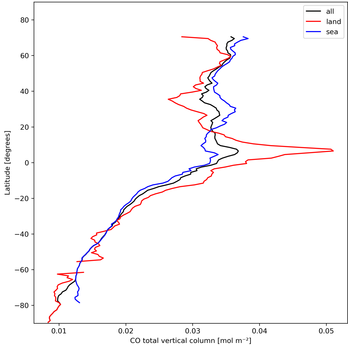
Figure 10: Zonal average of “CO total vertical column” for 2024-02-08 to 2024-02-10.
