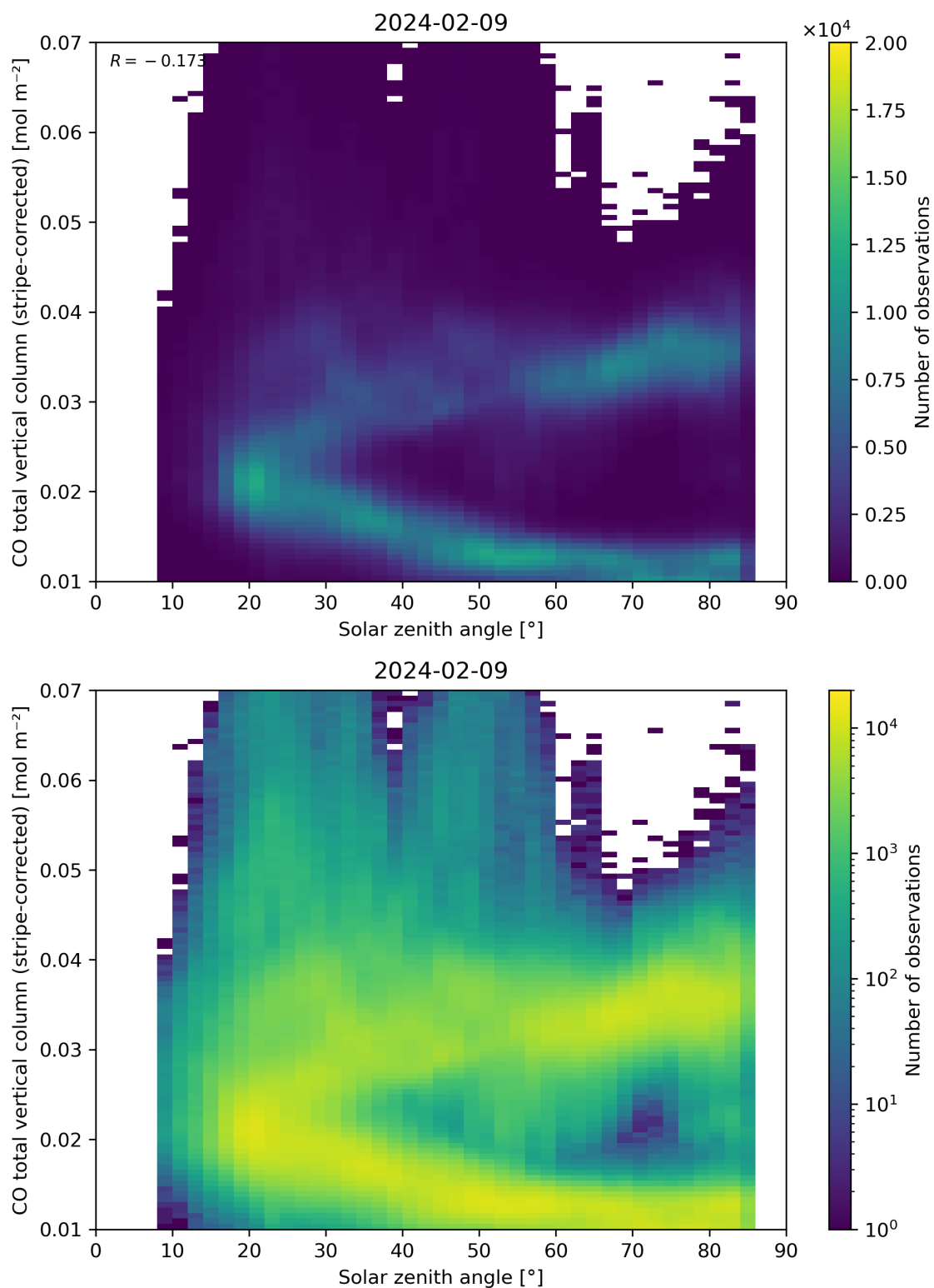
Figure 62: Scatter density plot of “Solar zenith angle” against “CO total vertical column (stripe-corrected)” for 2024-02-08 to 2024-02-10.
