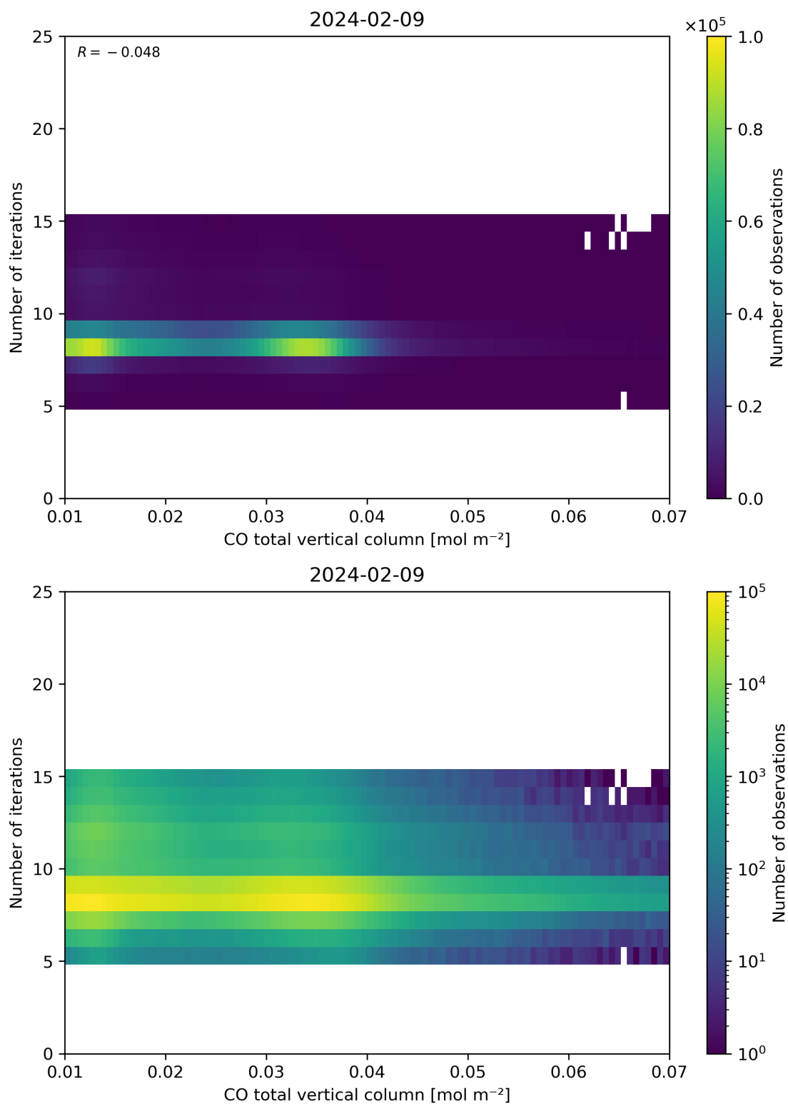
Figure 42: Scatter density plot of “CO total vertical column” against “Number of iterations” for 2024-02-08 to 2024-02-10.
