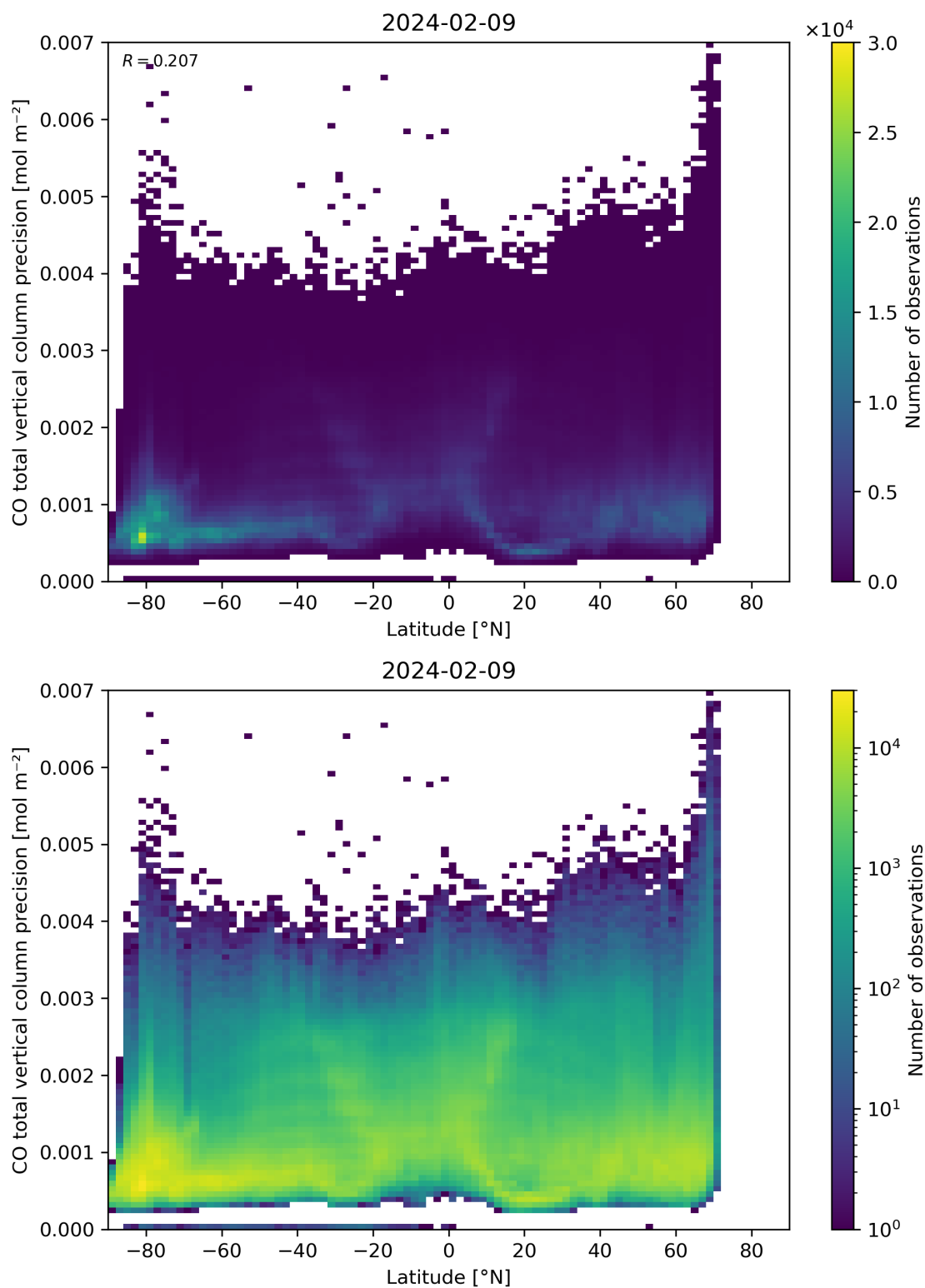
Figure 53: Scatter density plot of “Latitude” against “CO total vertical column precision” for 2024-02-08 to 2024-02-10.
