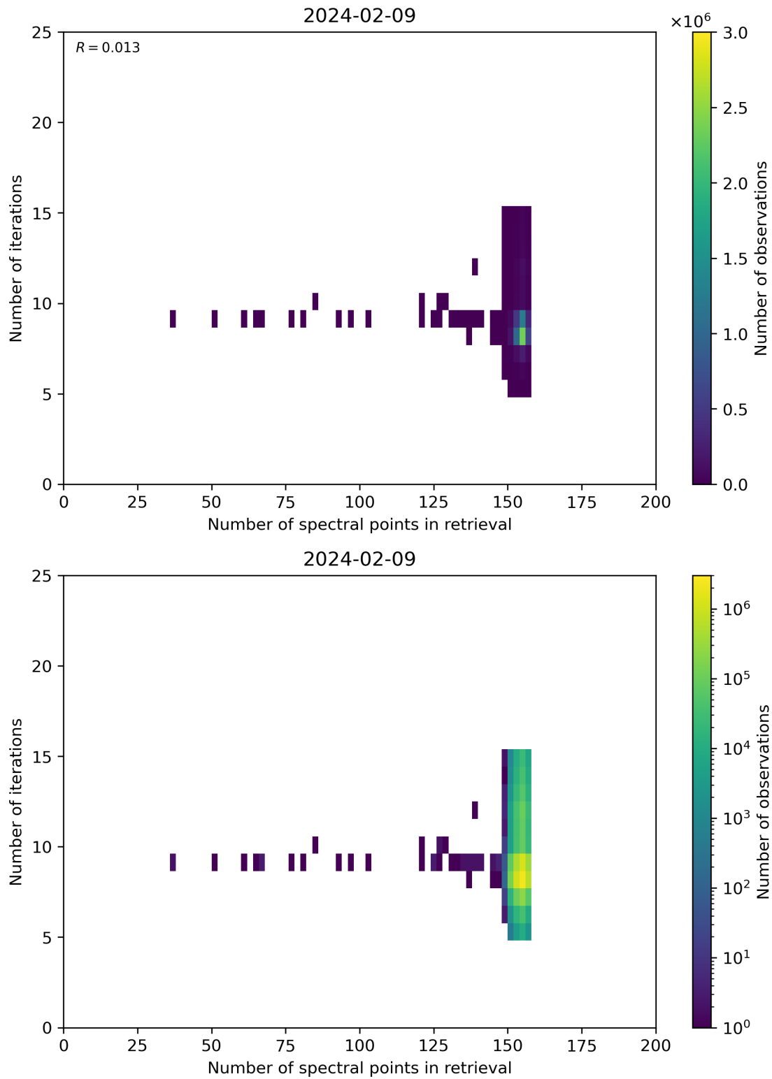
Figure 60: Scatter density plot of “Number of spectral points in retrieval” against “Number of iterations” for 2024-02-08 to 2024-02-10.
