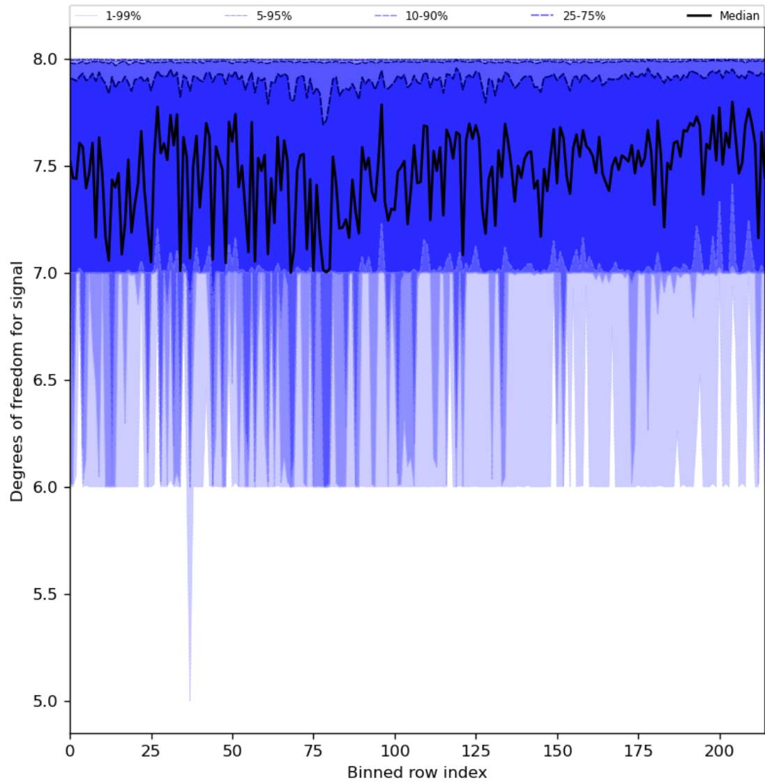
Figure 31: Along track statistics of “Degrees of freedom for signal” for 2024-02-08 to 2024-02-10
