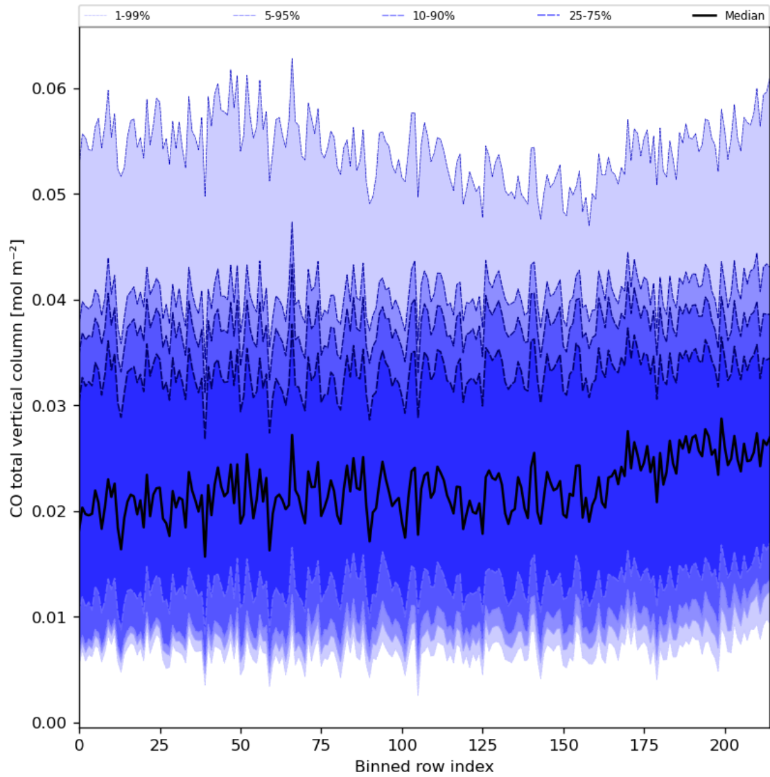
Figure 26: Along track statistics of “CO total vertical column” for 2024-02-08 to 2024-02-10
