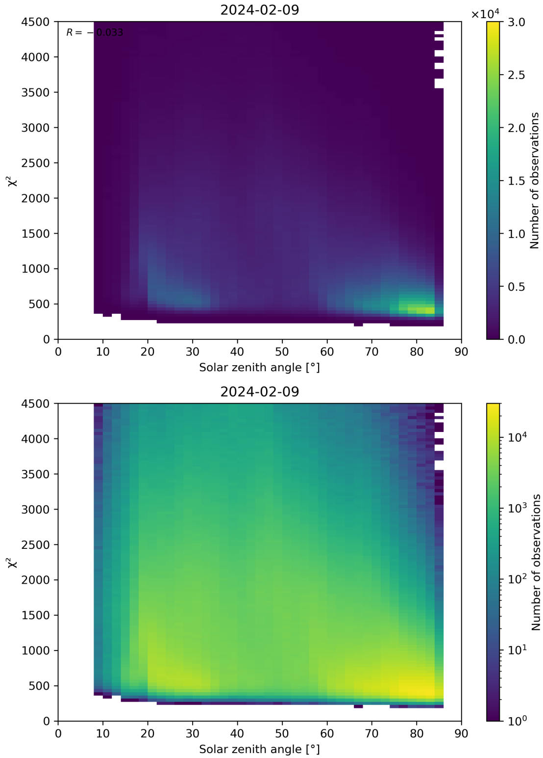
Figure 64: Scatter density plot of “Solar zenith angle” against “ \chi^2 ” for 2024-02-08 to 2024-02-10.
