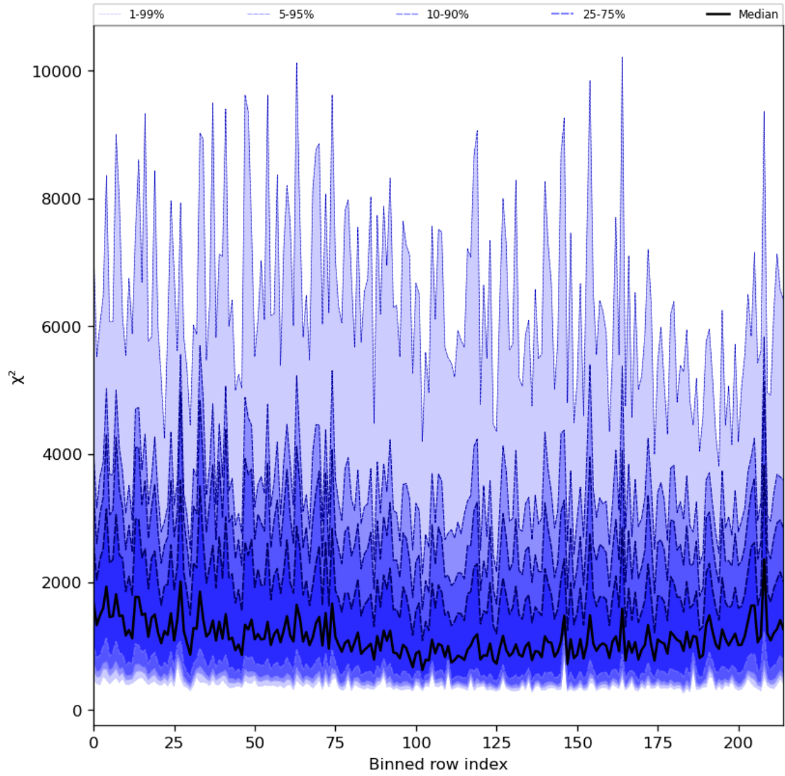
Figure 30: Along track statistics of “ \chi^2 ” for 2024-02-08 to 2024-02-10
