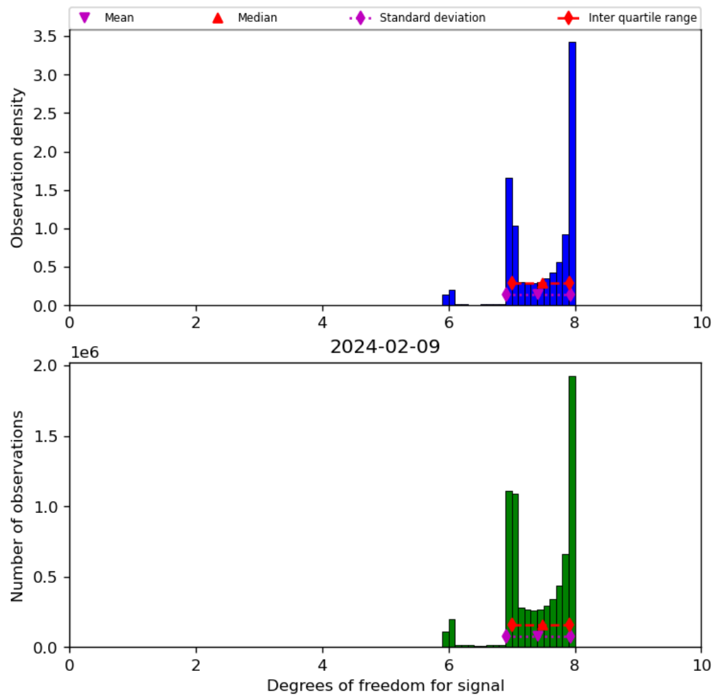
Figure 23: Histogram of “Degrees of freedom for signal” for 2024-02-08 to 2024-02-10
