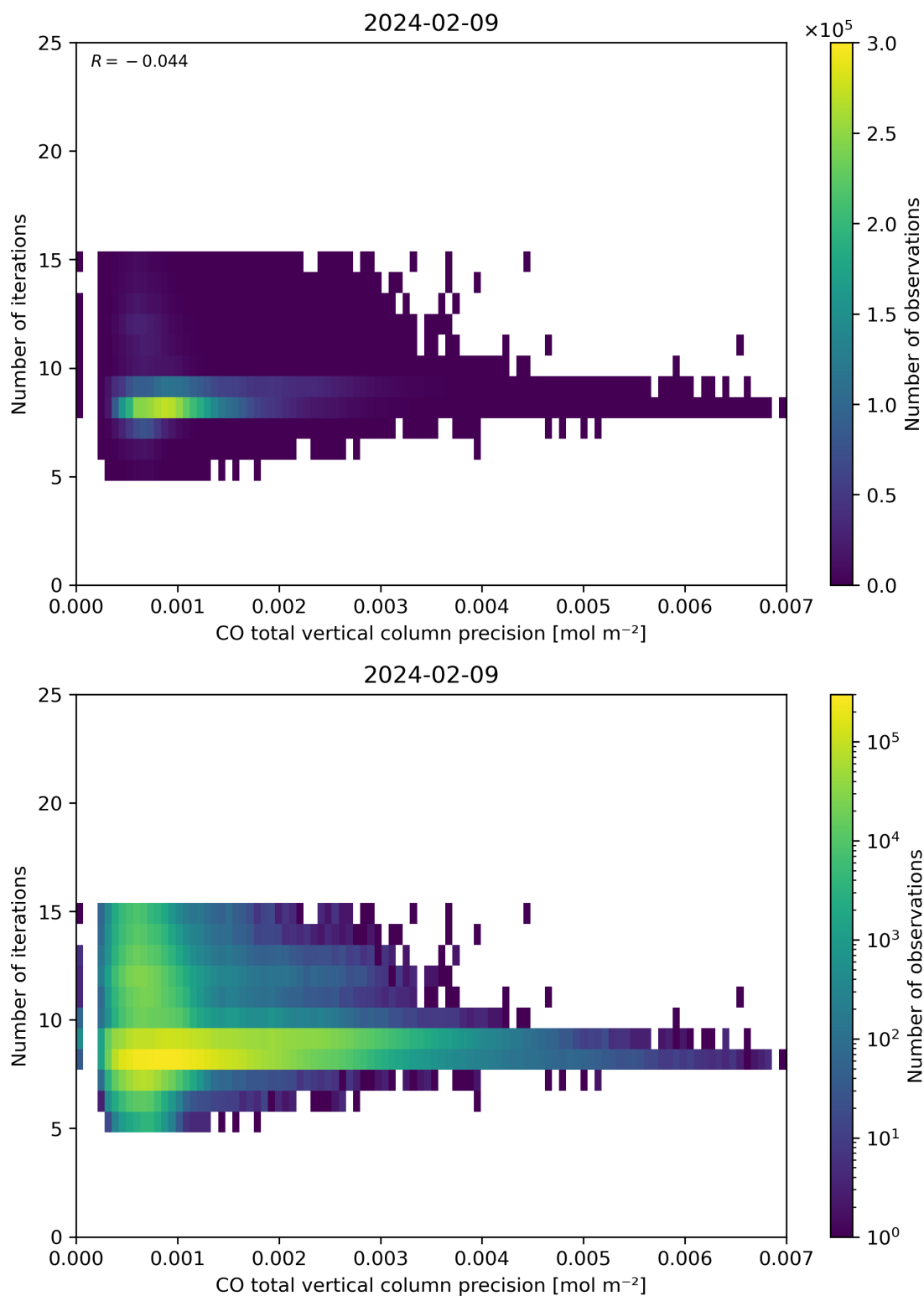
Figure 46: Scatter density plot of “CO total vertical column precision” against “Number of iterations” for 2024-02-08 to 2024-02-10.
