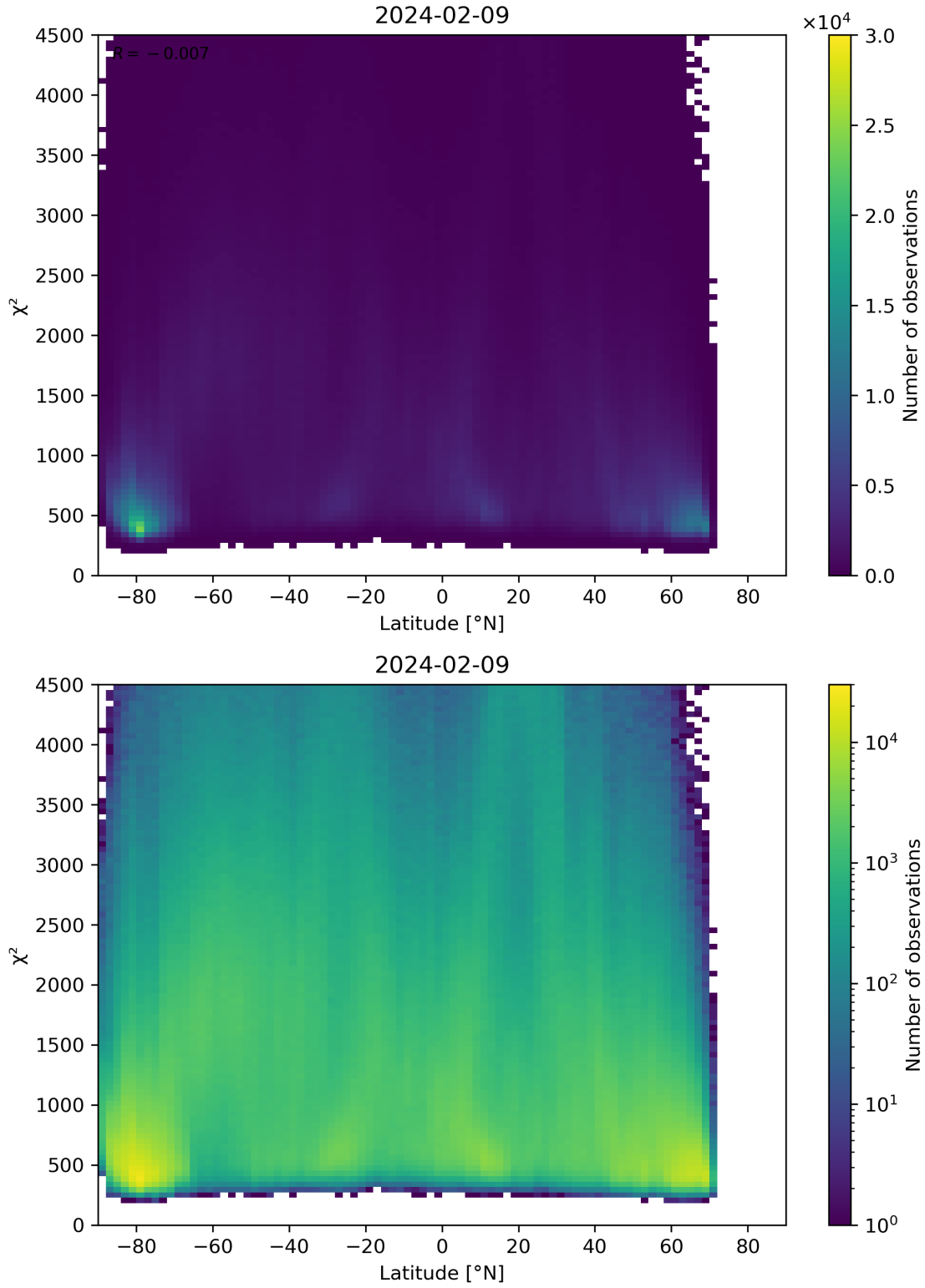
Figure 54: Scatter density plot of “Latitude” against “ \chi^2 ” for 2024-02-08 to 2024-02-10.
