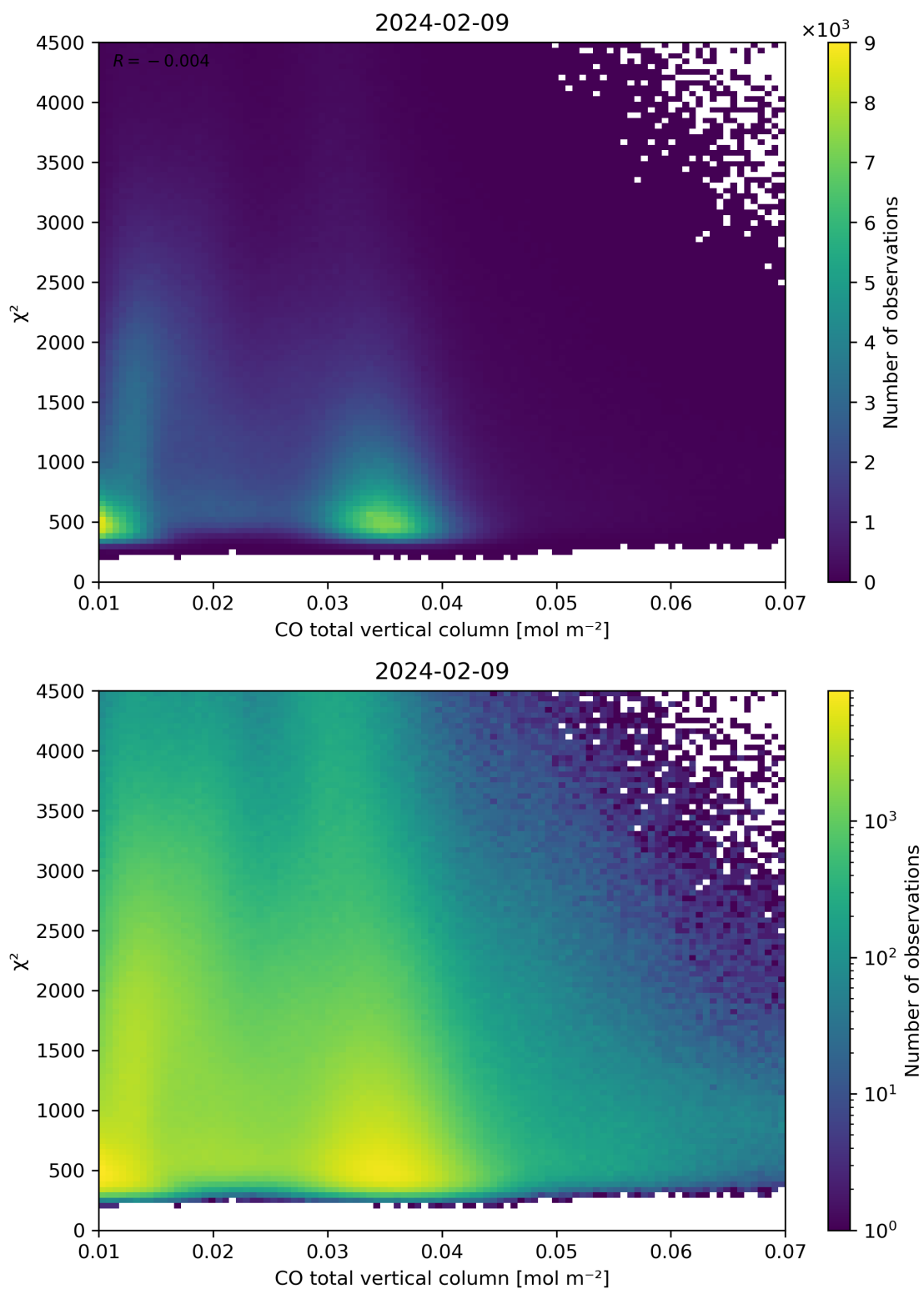
Figure 35: Scatter density plot of “CO total vertical column” against “ \chi^2 ” for 2024-02-08 to 2024-02-10.
