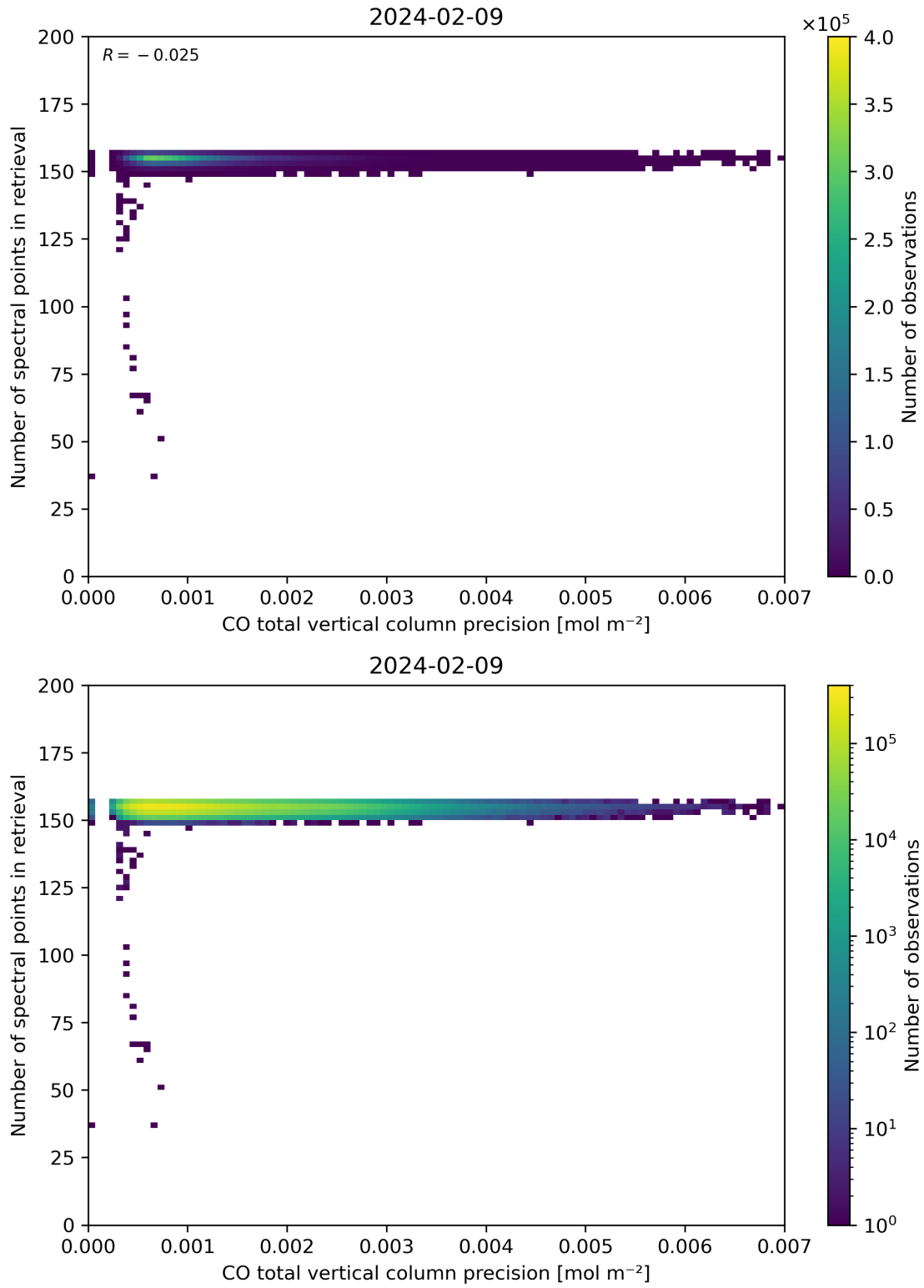
Figure 47: Scatter density plot of “CO total vertical column precision” against “Number of spectral points in retrieval” for 2024-02-08 to 2024-02-10.
