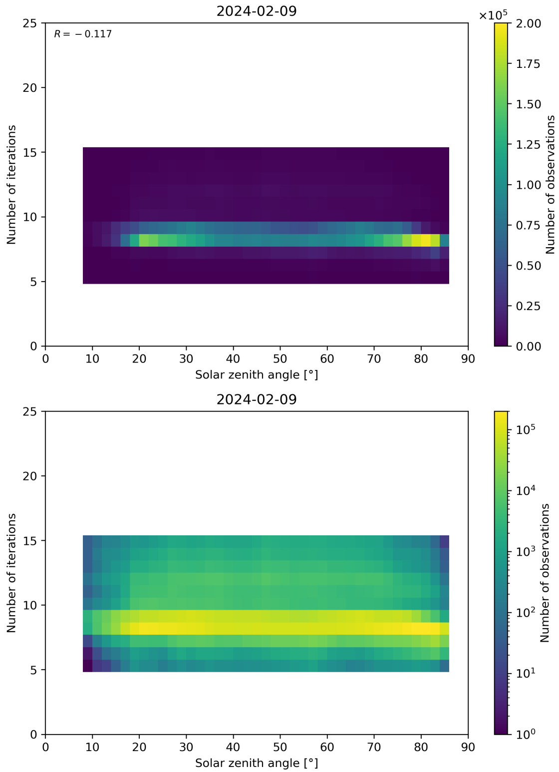
Figure 67: Scatter density plot of “Solar zenith angle” against “Number of iterations” for 2024-02-08 to 2024-02-10.
