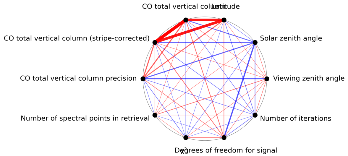
Figure 1: Map of correlation graph for 2024-02-08 to 2024-02-10.
