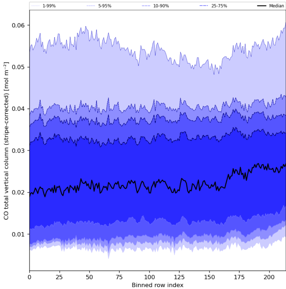
Figure 27: Along track statistics of “CO total vertical column (stripe-corrected)” for 2024-02-08 to 2024-02-10
