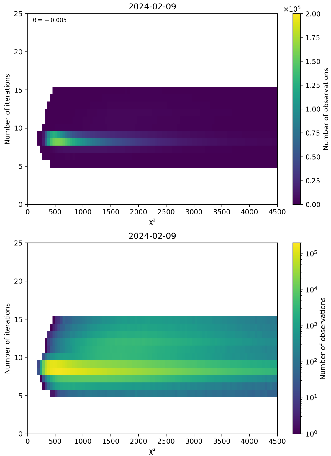
Figure 49: Scatter density plot of “ \chi^2 ” against “Number of iterations” for 2024-02-08 to 2024-02-10.
