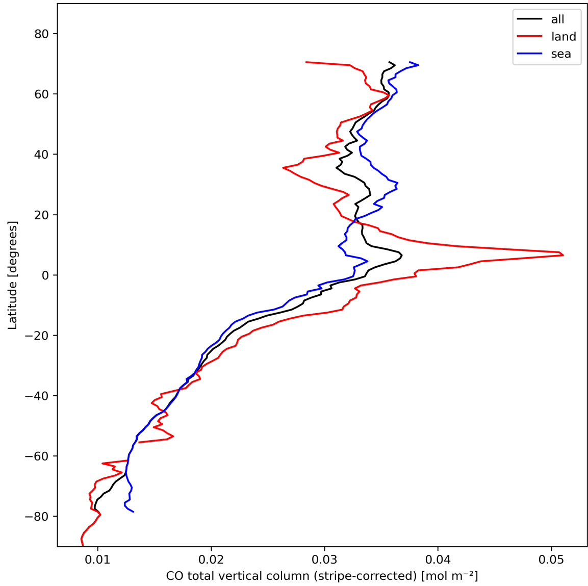
Figure 11: Zonal average of “CO total vertical column (stripe-corrected)” for 2024-02-08 to 2024-02-10.
