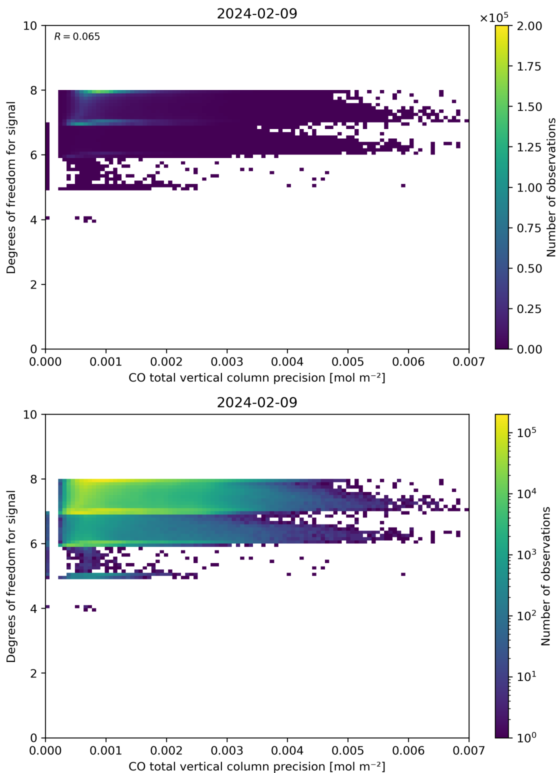
Figure 45: Scatter density plot of “CO total vertical column precision” against “Degrees of freedom for signal” for 2024-02-08 to 2024-02-10.
