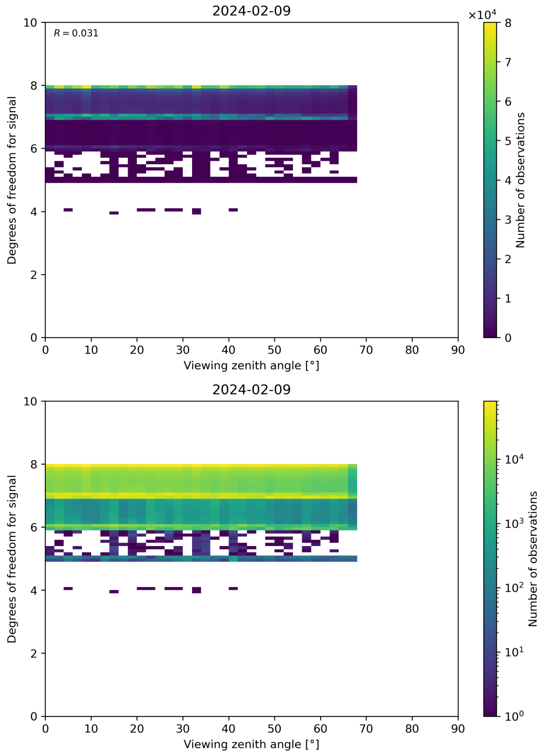
Figure 73: Scatter density plot of “Viewing zenith angle” against “Degrees of freedom for signal” for 2024-02-08 to 2024-02-10.
