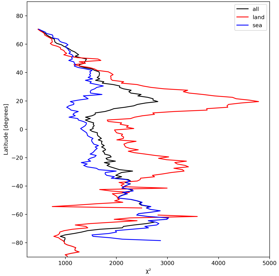
Figure 14: Zonal average of “ \chi^2 ” for 2024-02-09 to 2024-02-11.
