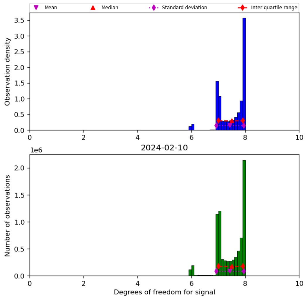
Figure 23: Histogram of “Degrees of freedom for signal” for 2024-02-09 to 2024-02-11
