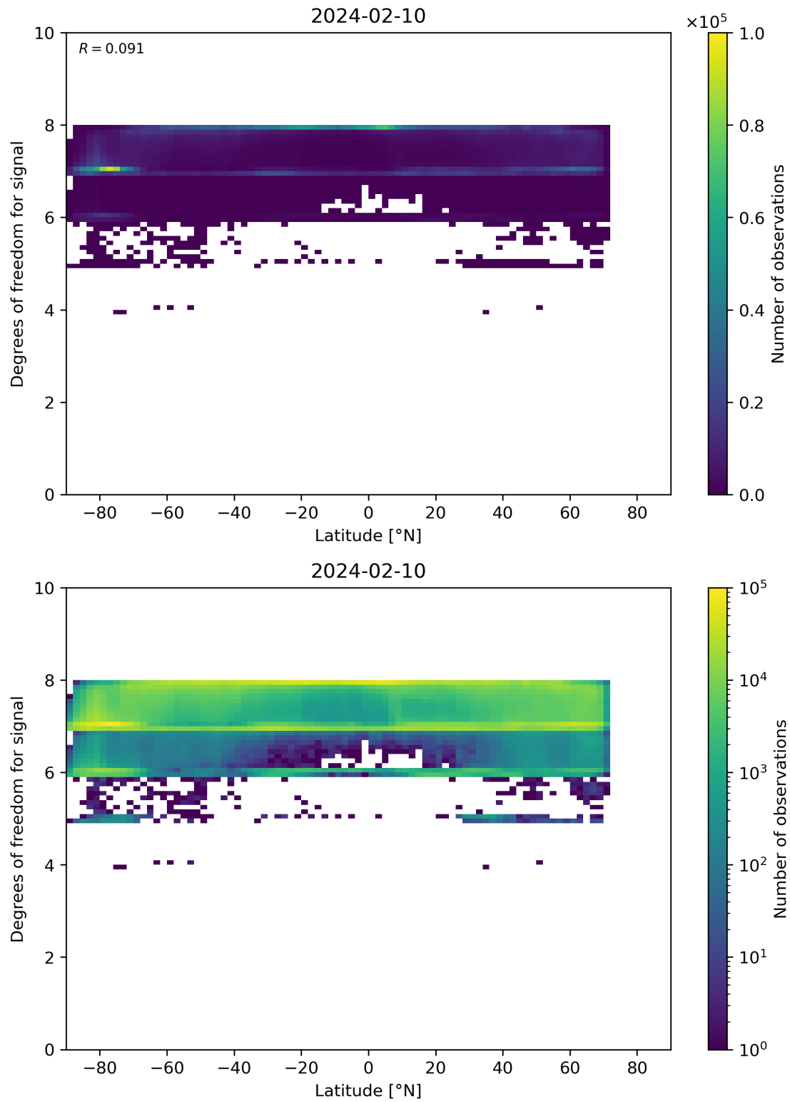
Figure 55: Scatter density plot of “Latitude” against “Degrees of freedom for signal” for 2024-02-09 to 2024-02-11.
