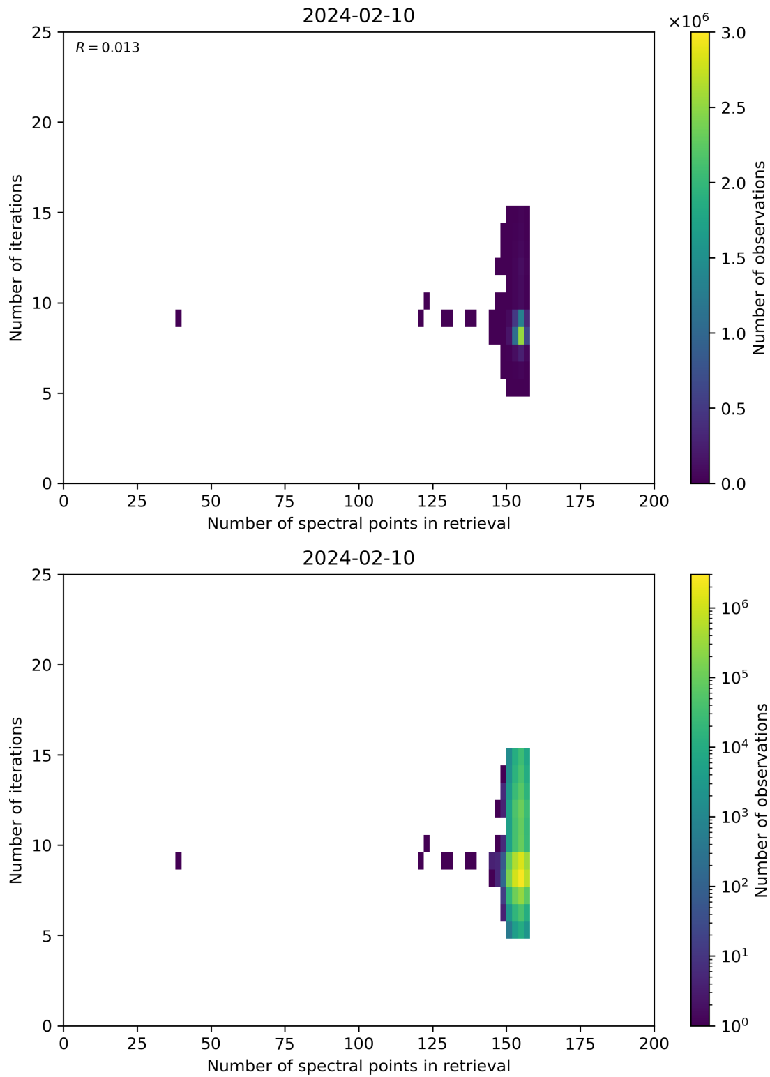
Figure 60: Scatter density plot of “Number of spectral points in retrieval” against “Number of iterations” for 2024-02-09 to 2024-02-11.
