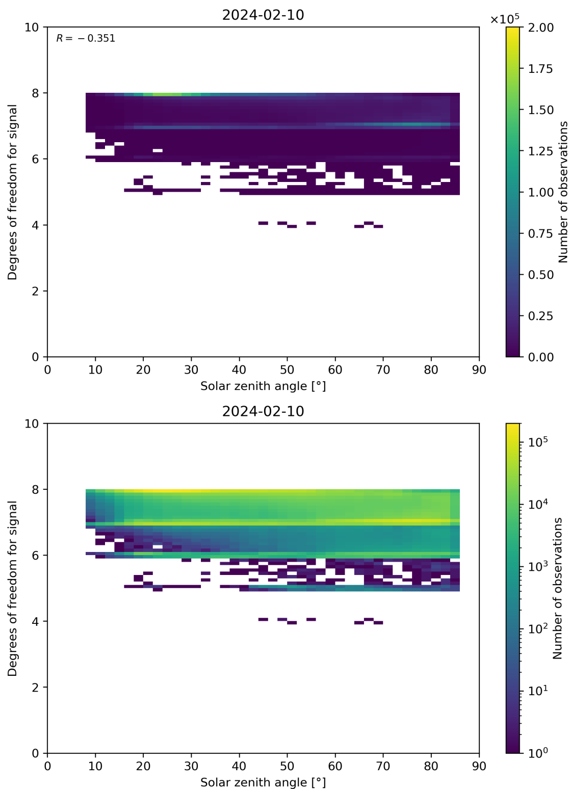
Figure 65: Scatter density plot of “Solar zenith angle” against “Degrees of freedom for signal” for 2024-02-09 to 2024-02-11.
