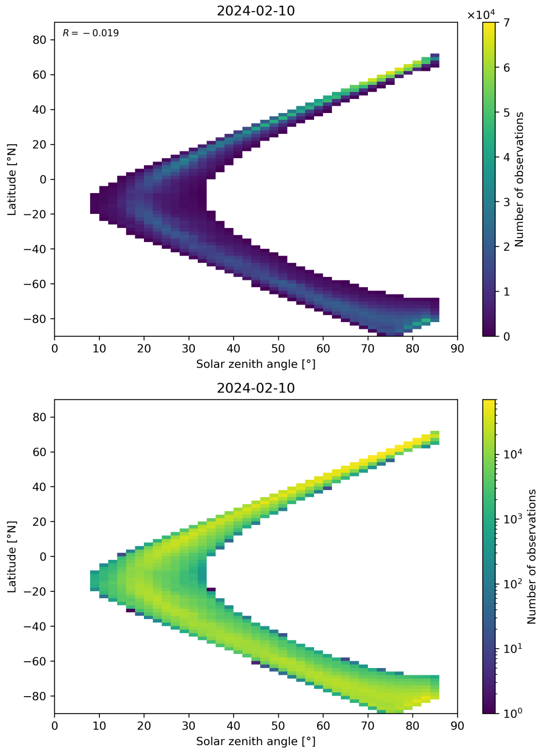
Figure 66: Scatter density plot of “Solar zenith angle” against “Latitude” for 2024-02-09 to 2024-02-11.
