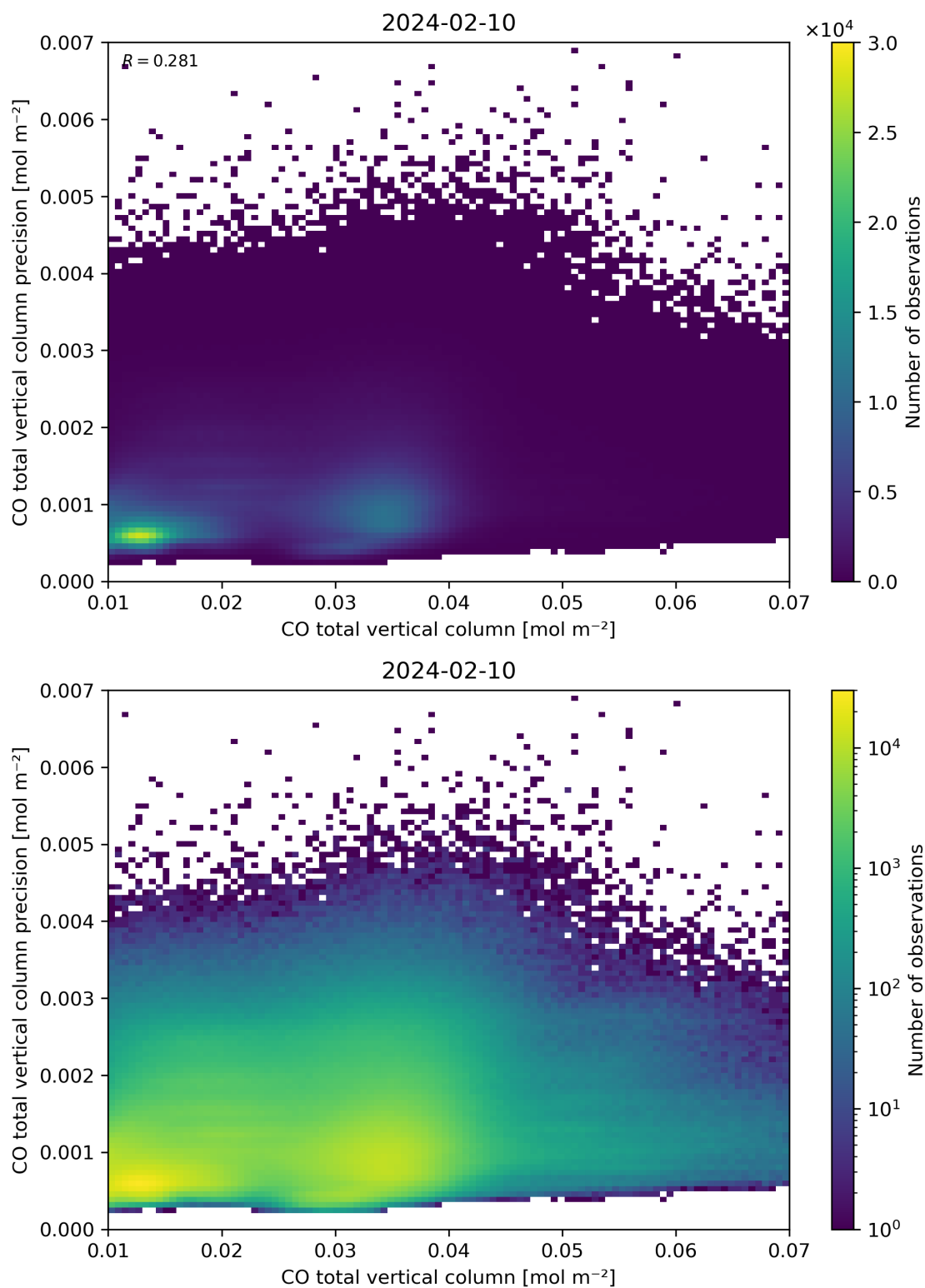
Figure 34: Scatter density plot of “CO total vertical column” against “CO total vertical column precision” for 2024-02-09 to 2024-02-11.
