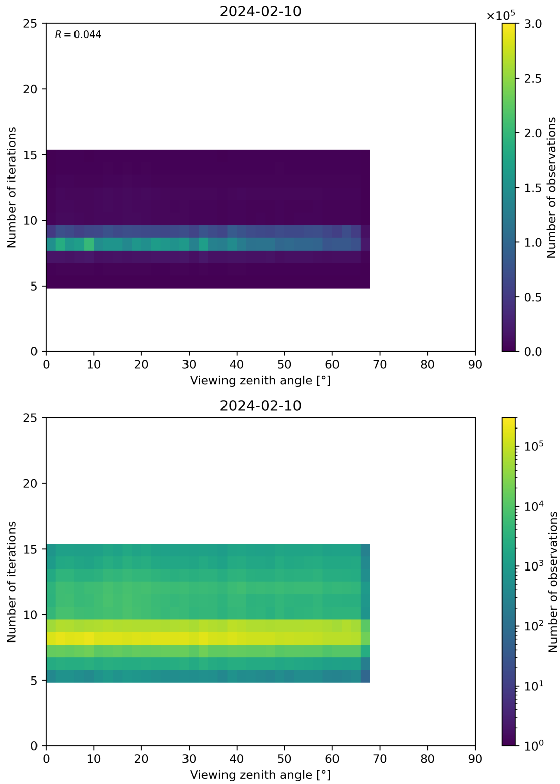
Figure 75: Scatter density plot of “Viewing zenith angle” against “Number of iterations” for 2024-02-09 to 2024-02-11.
