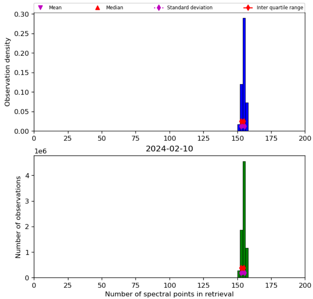
Figure 21: Histogram of “Number of spectral points in retrieval” for 2024-02-09 to 2024-02-11
