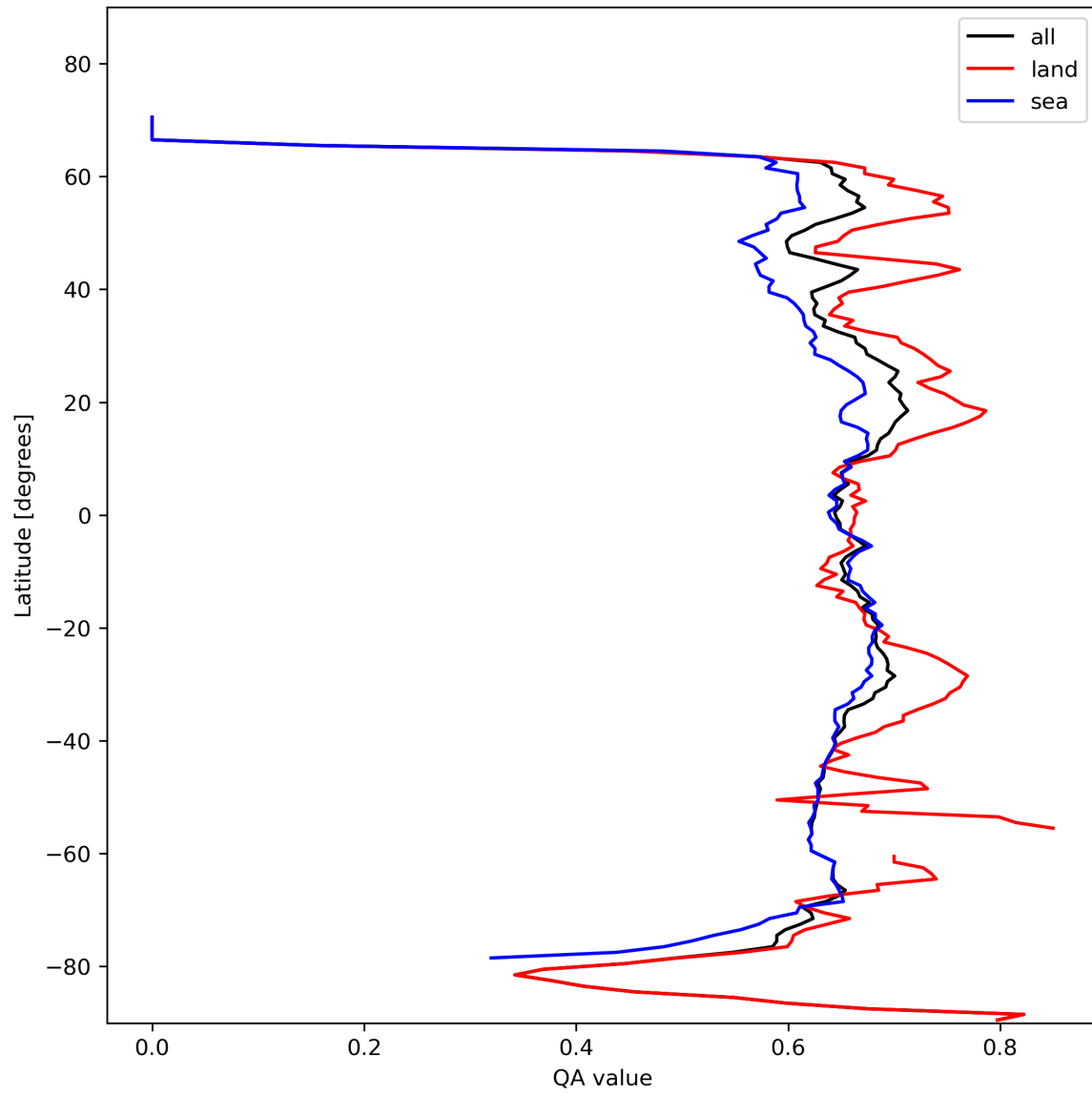
Figure 9: Zonal average of “QA value” for 2024-02-09 to 2024-02-11.
