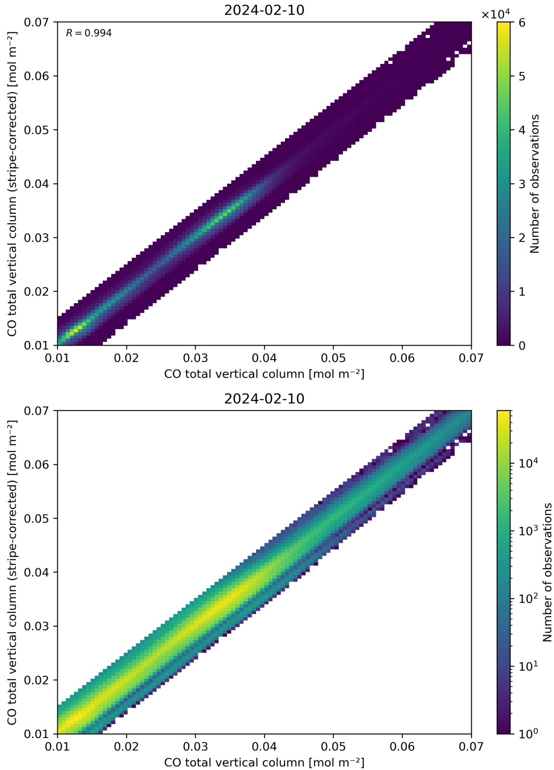
Figure 33: Scatter density plot of “CO total vertical column” against “CO total vertical column (stripe-corrected)” for 2024-02-09 to 2024-02-11.
