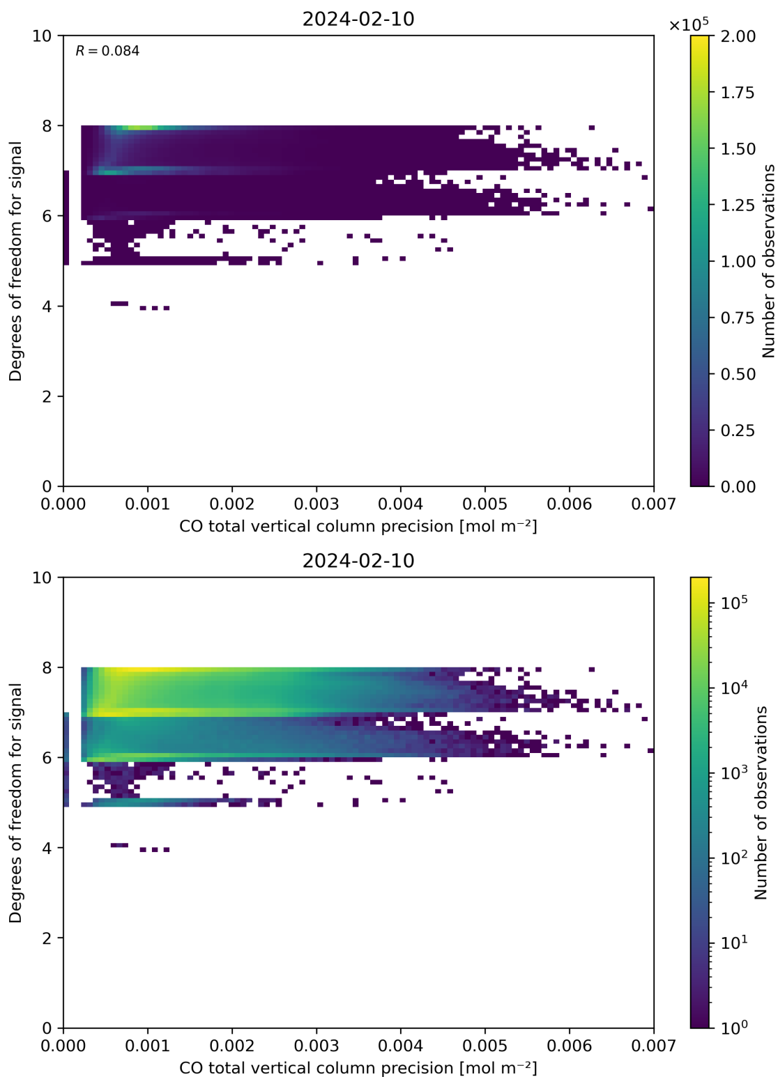
Figure 45: Scatter density plot of “CO total vertical column precision” against “Degrees of freedom for signal” for 2024-02-09 to 2024-02-11.
