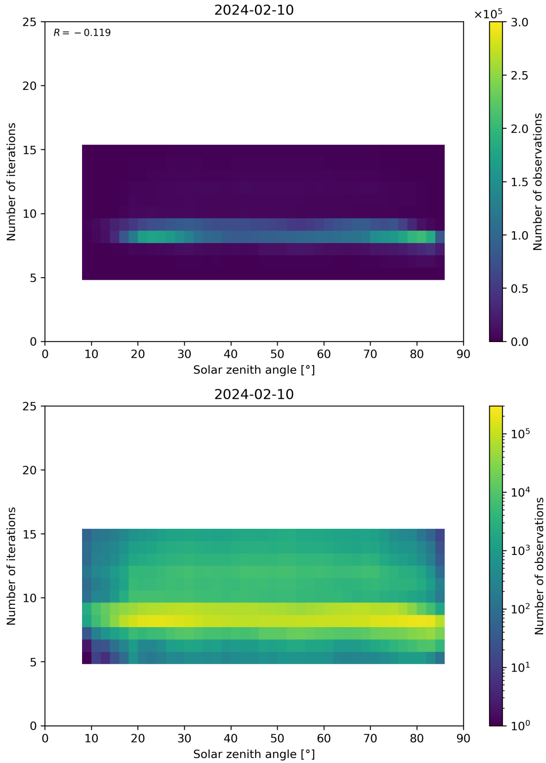
Figure 67: Scatter density plot of “Solar zenith angle” against “Number of iterations” for 2024-02-09 to 2024-02-11.
