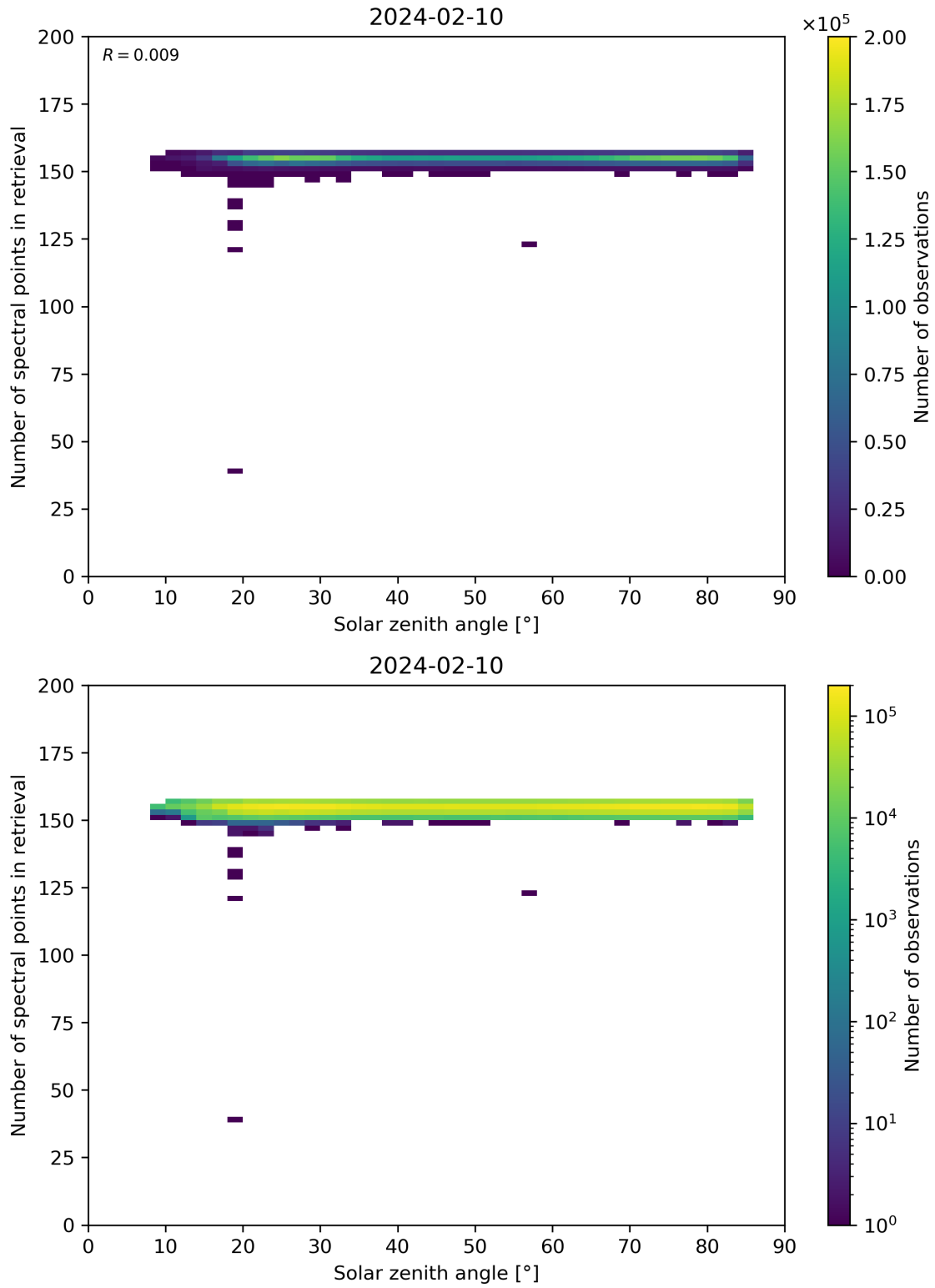
Figure 68: Scatter density plot of “Solar zenith angle” against “Number of spectral points in retrieval” for 2024-02-09 to 2024-02-11.
