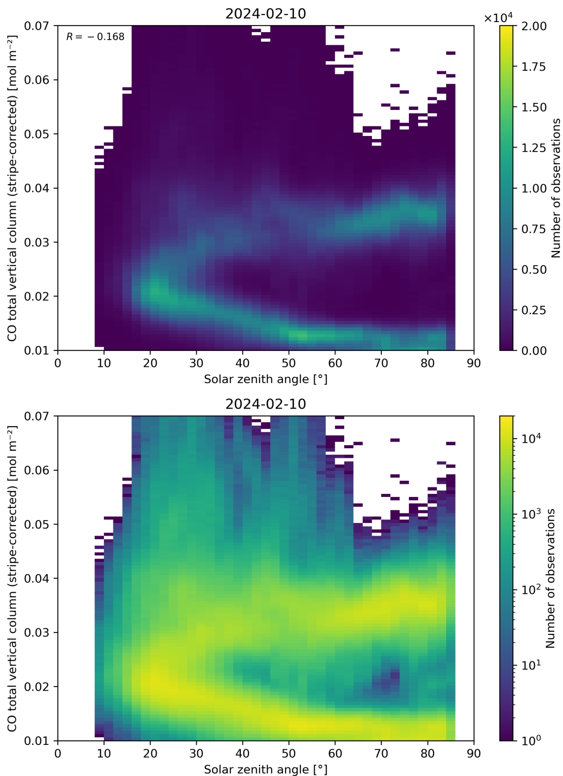
Figure 62: Scatter density plot of “Solar zenith angle” against “CO total vertical column (stripe-corrected)” for 2024-02-09 to 2024-02-11.
