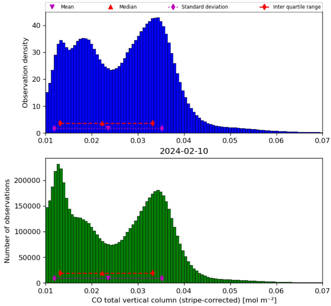
Figure 19: Histogram of “CO total vertical column (stripe-corrected)” for 2024-02-09 to 2024-02-11
