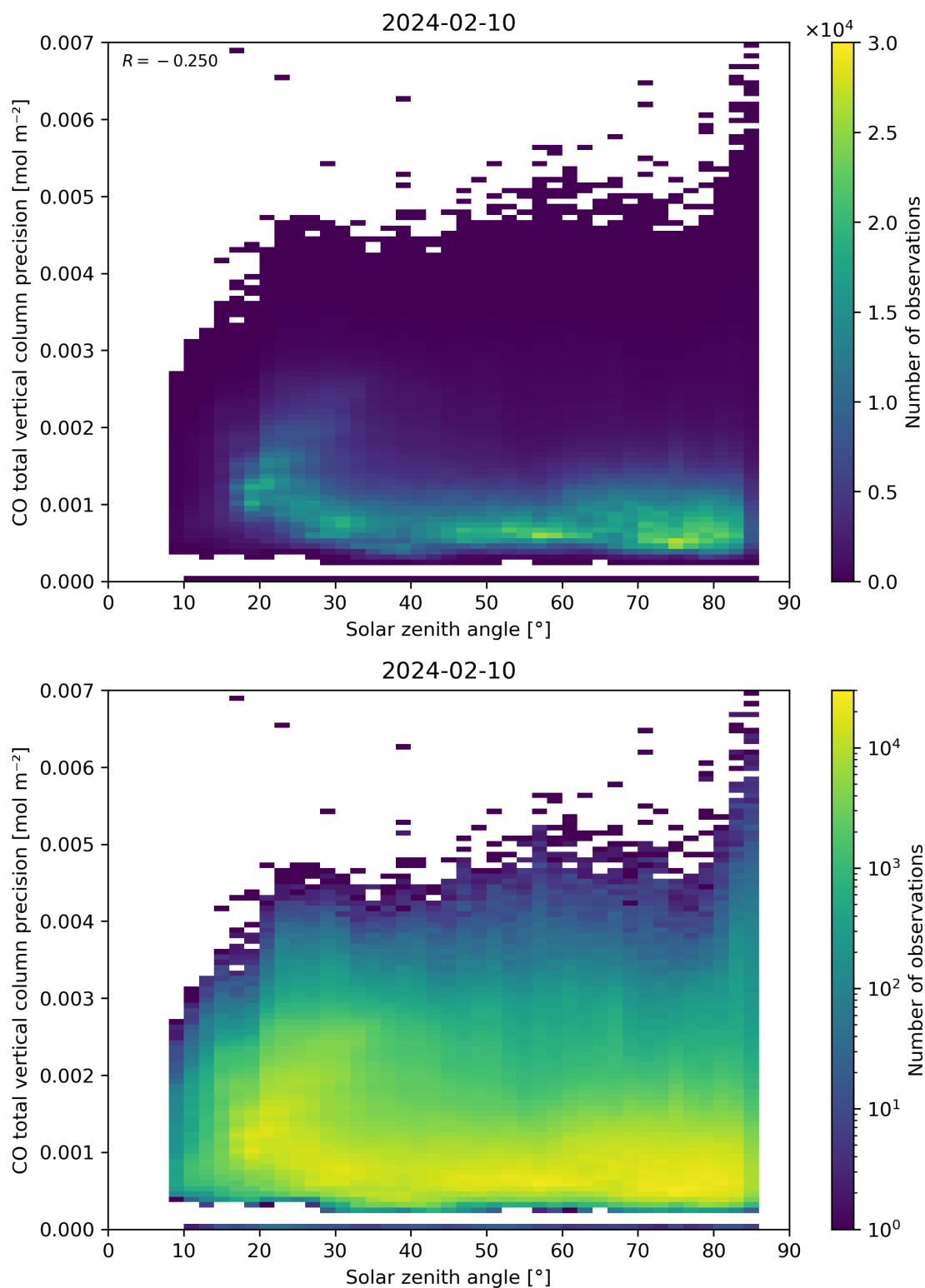
Figure 63: Scatter density plot of “Solar zenith angle” against “CO total vertical column precision” for 2024-02-09 to 2024-02-11.
