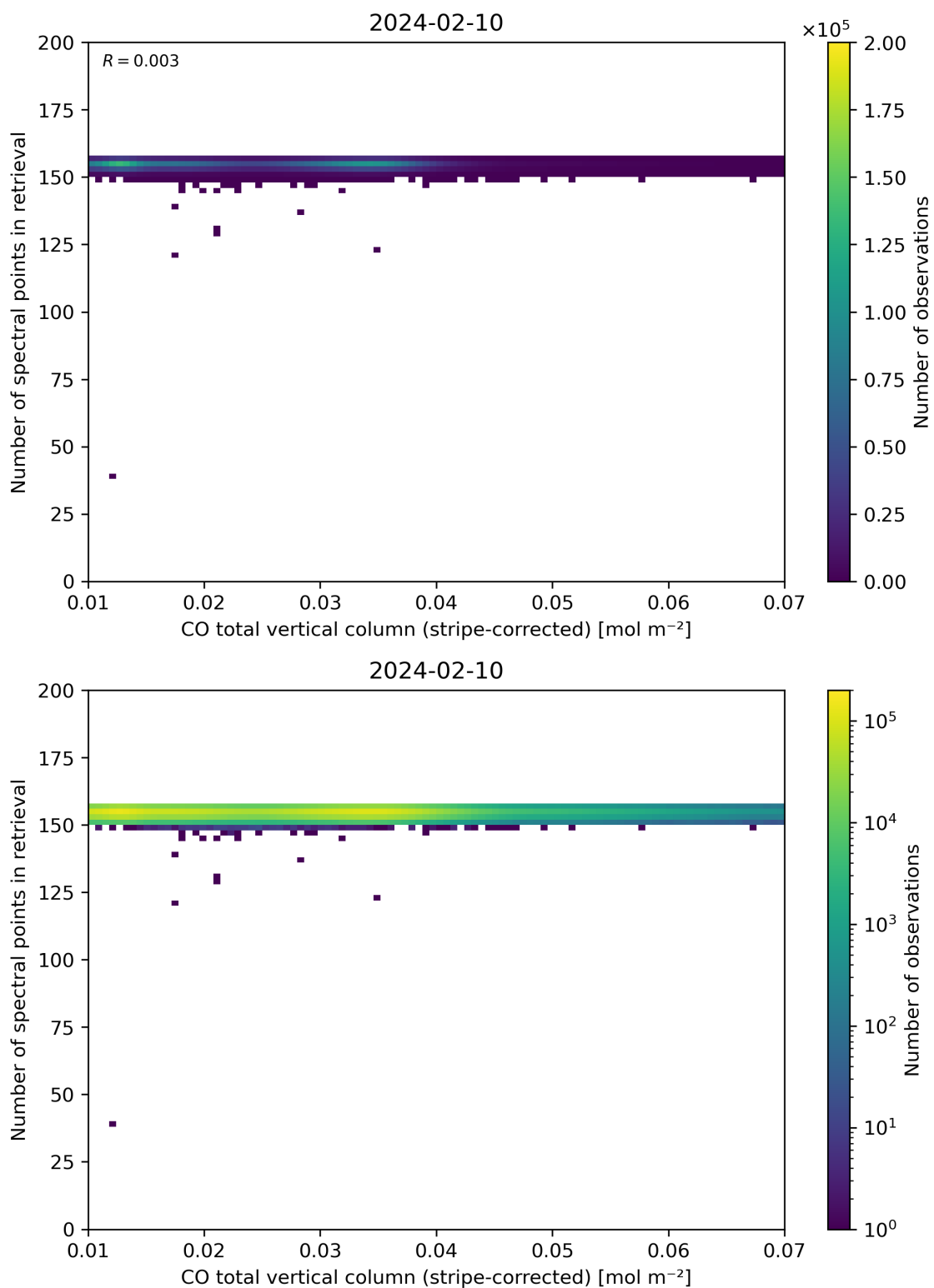
Figure 40: Scatter density plot of “CO total vertical column (stripe-corrected)” against “Number of spectral points in retrieval” for 2024-02-09 to 2024-02-11.
