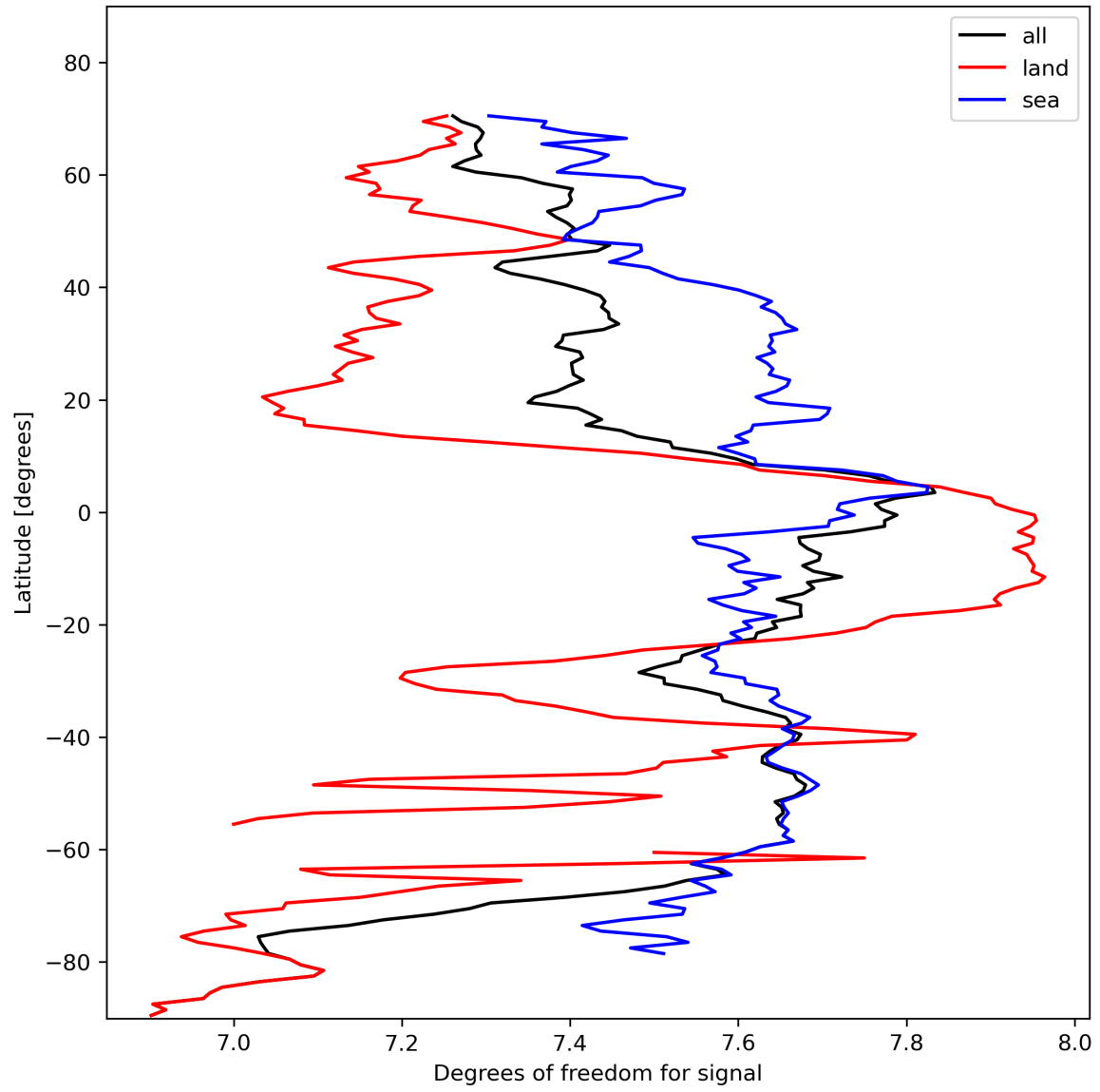
Figure 15: Zonal average of “Degrees of freedom for signal” for 2024-02-09 to 2024-02-11.
