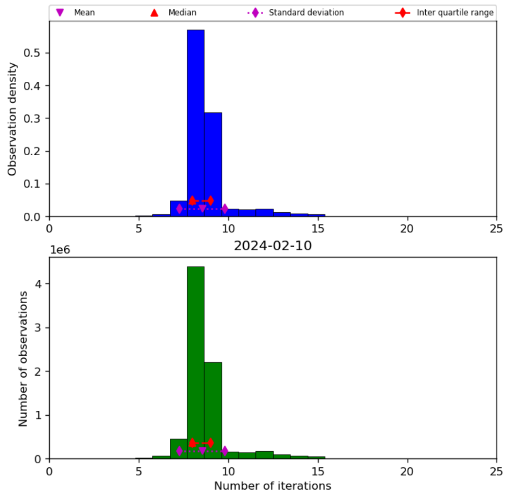
Figure 24: Histogram of “Number of iterations” for 2024-02-09 to 2024-02-11
