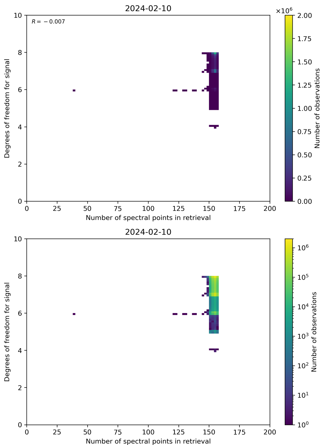
Figure 59: Scatter density plot of “Number of spectral points in retrieval” against “Degrees of freedom for signal” for 2024-02-09 to 2024-02-11.
