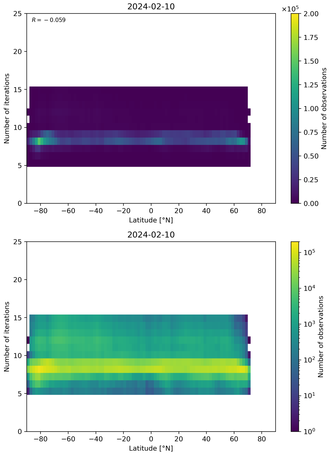
Figure 56: Scatter density plot of “Latitude” against “Number of iterations” for 2024-02-09 to 2024-02-11.
