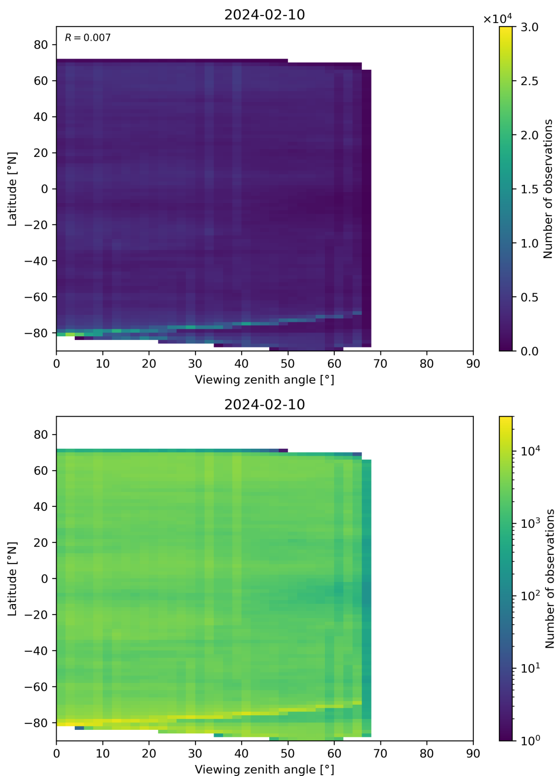
Figure 74: Scatter density plot of “Viewing zenith angle” against “Latitude” for 2024-02-09 to 2024-02-11.
