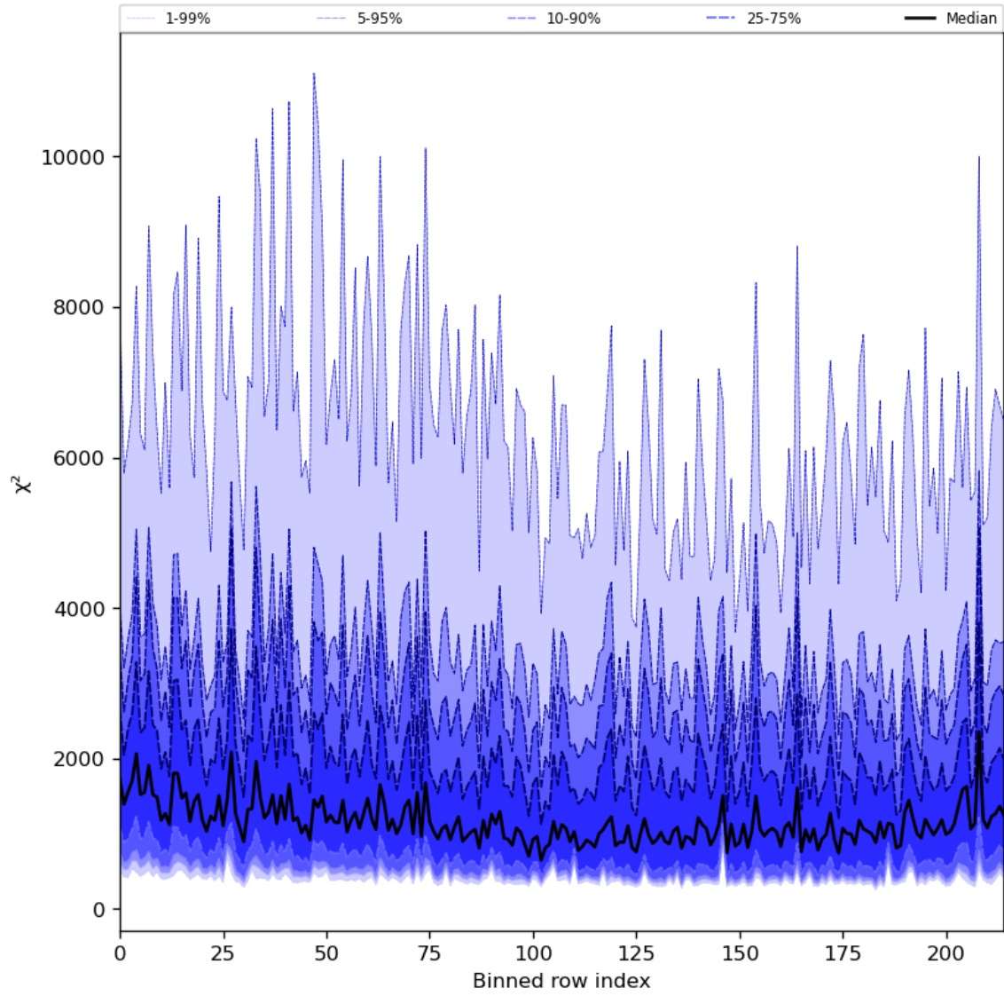
Figure 30: Along track statistics of “ \chi^2 ” for 2024-02-09 to 2024-02-11
