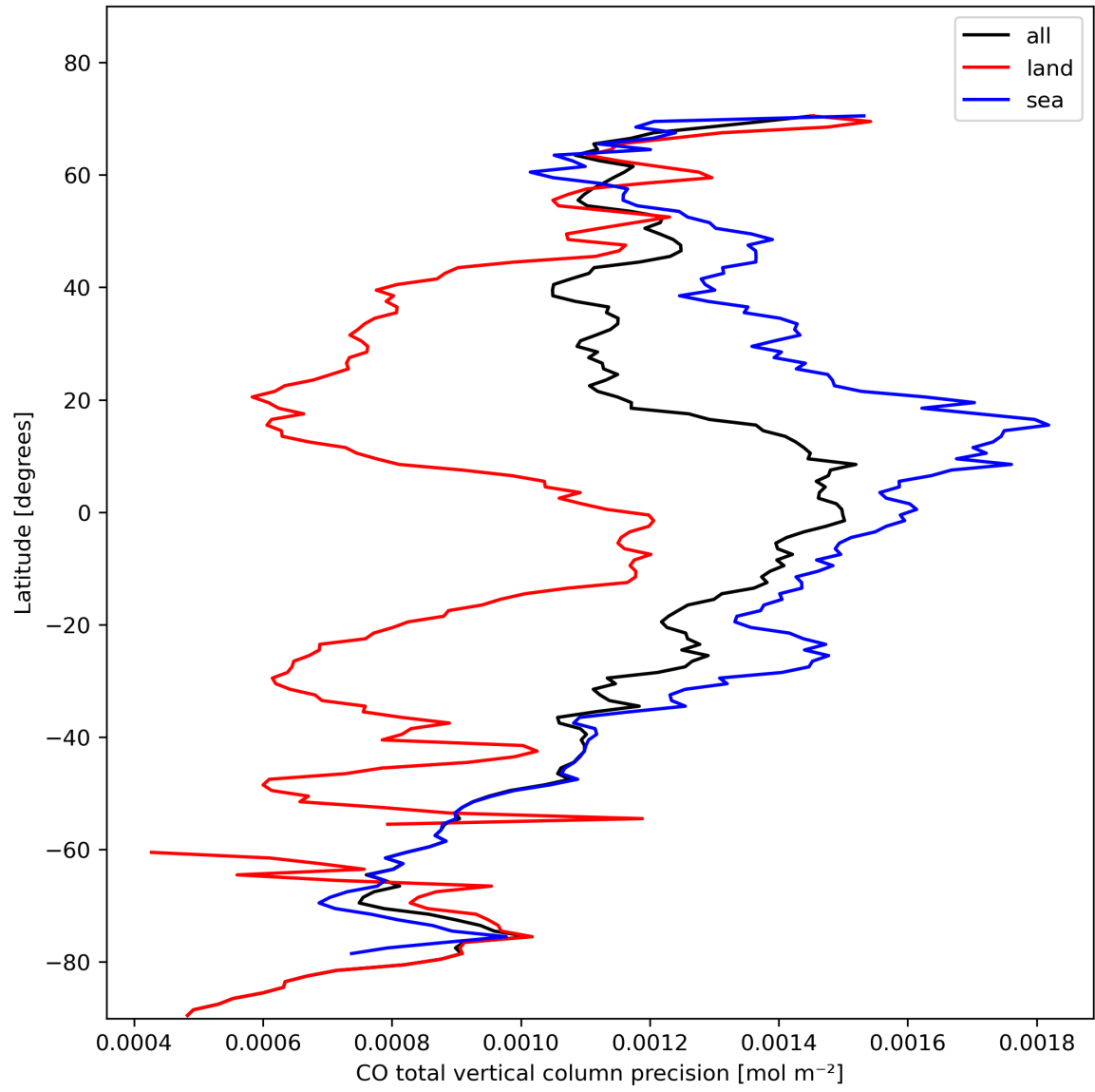
Figure 12: Zonal average of “CO total vertical column precision” for 2024-02-09 to 2024-02-11.
