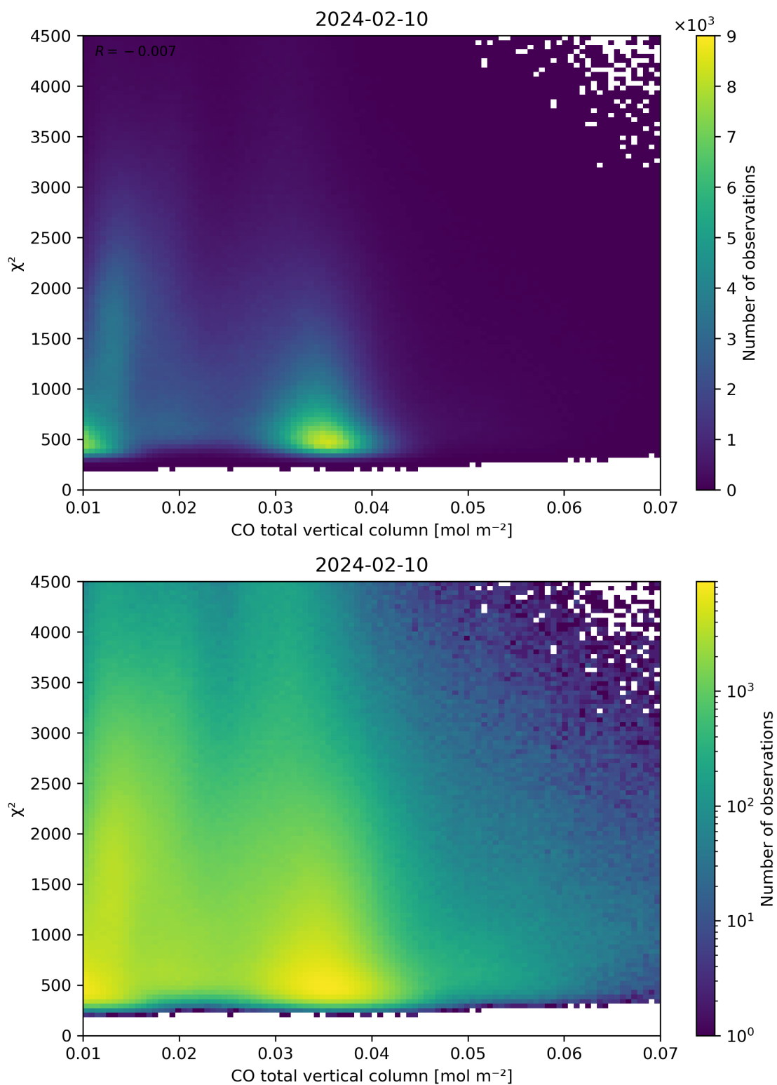
Figure 35: Scatter density plot of “CO total vertical column” against “ \chi^2 ” for 2024-02-09 to 2024-02-11.
