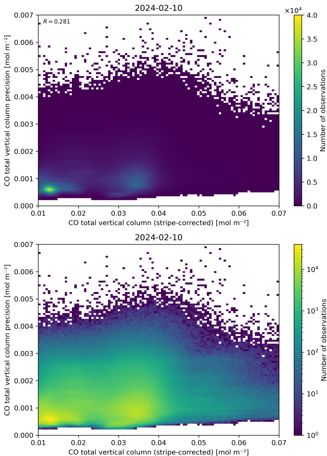
Figure 36: Scatter density plot of “CO total vertical column (stripe-corrected)” against “CO total vertical column precision” for 2024-02-09 to 2024-02-11.
