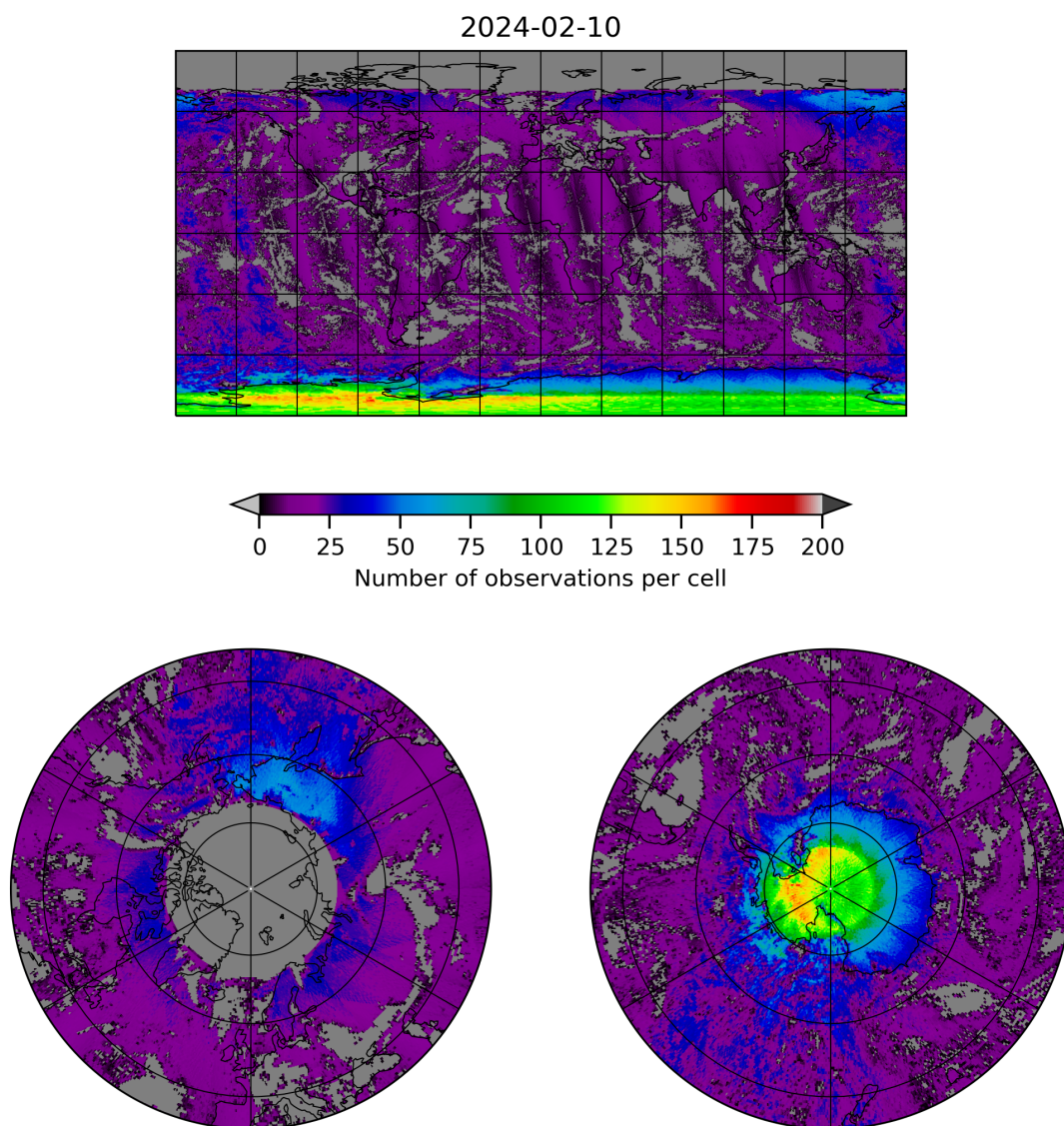
Figure 8: Map of the number of observations for 2024-02-09 to 2024-02-11
