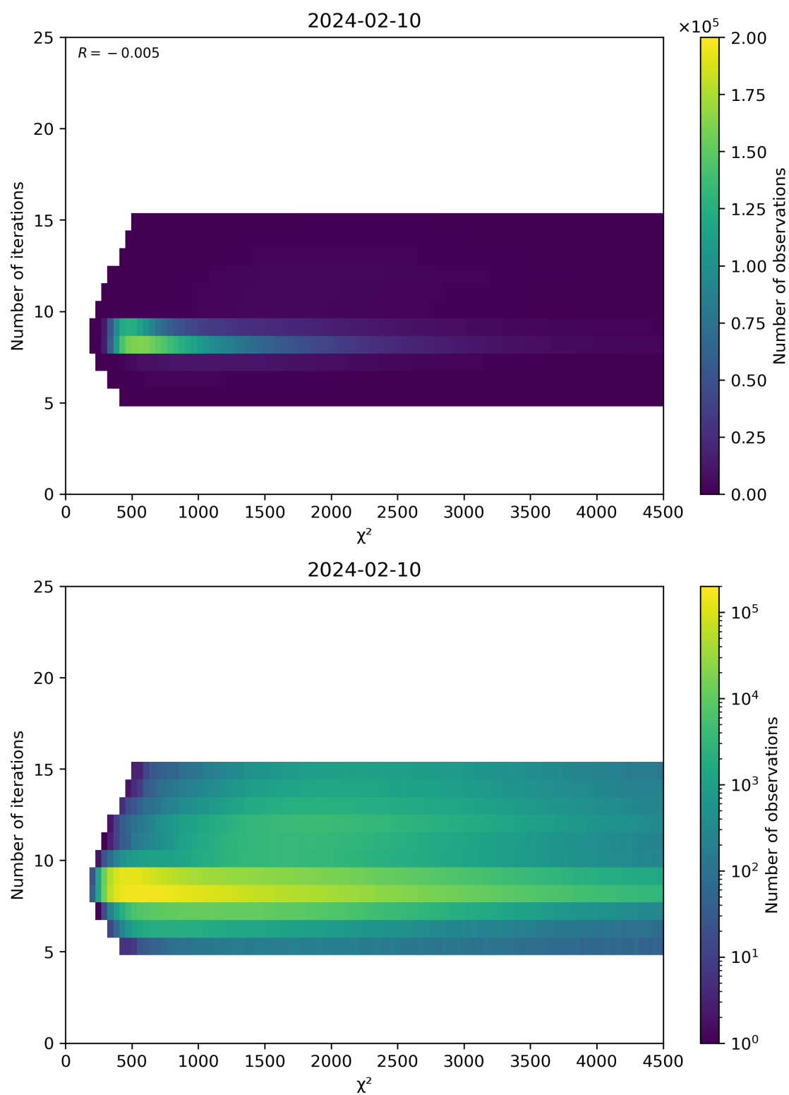
Figure 49: Scatter density plot of “ \chi^2 ” against “Number of iterations” for 2024-02-09 to 2024-02-11.
