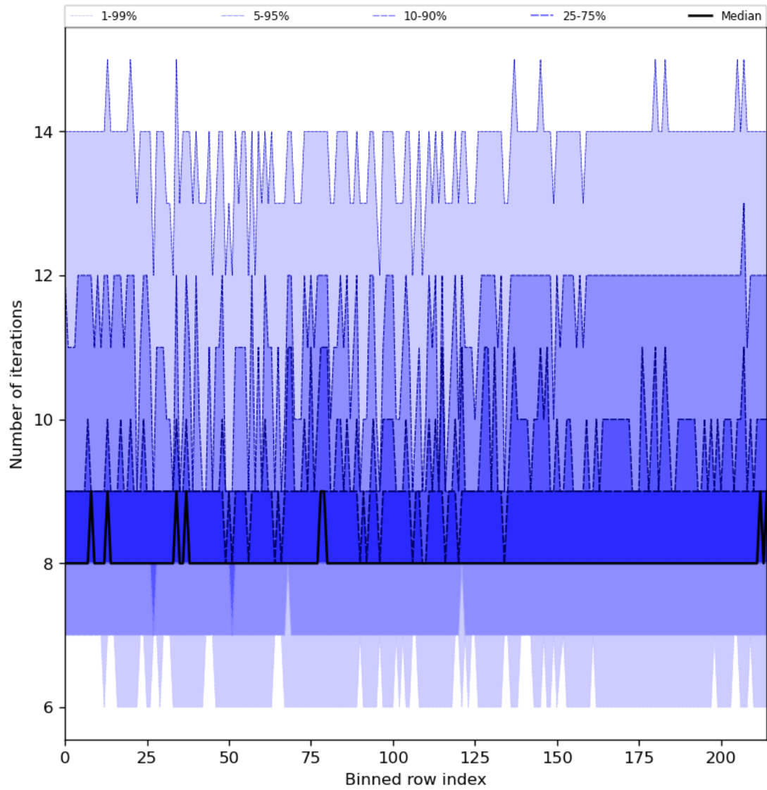
Figure 32: Along track statistics of “Number of iterations” for 2024-02-09 to 2024-02-11
