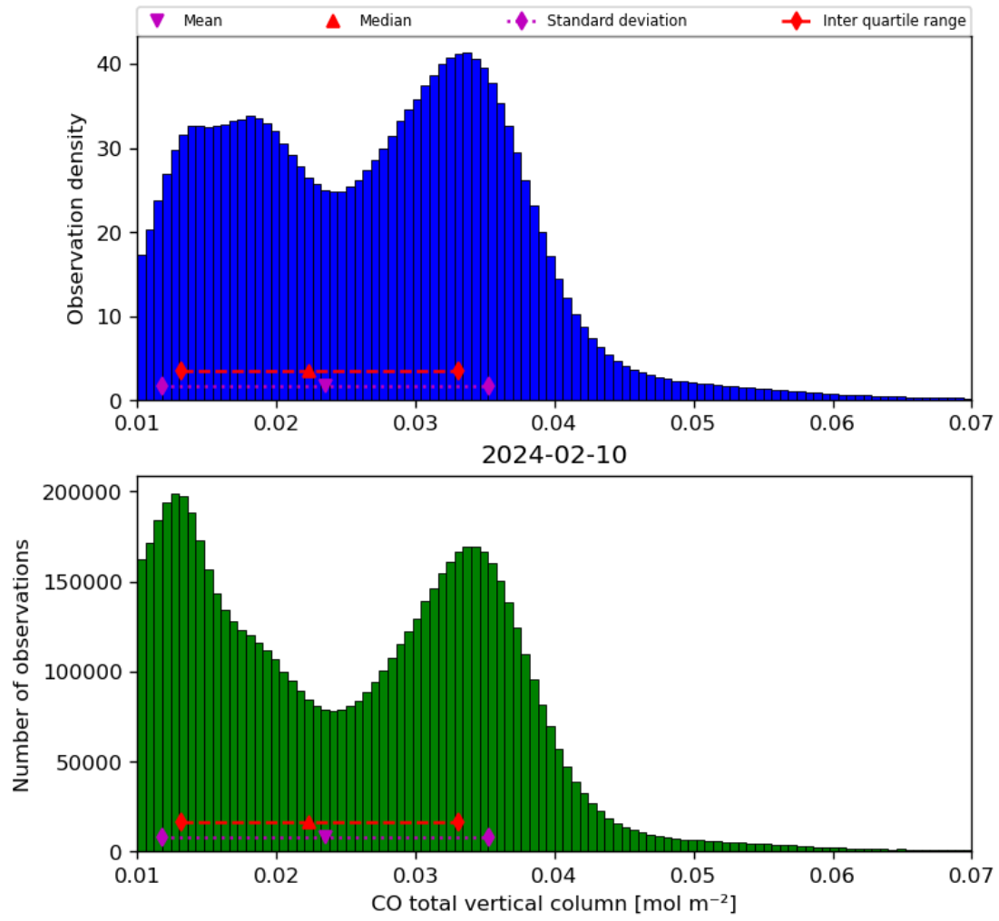
Figure 18: Histogram of “CO total vertical column” for 2024-02-09 to 2024-02-11
