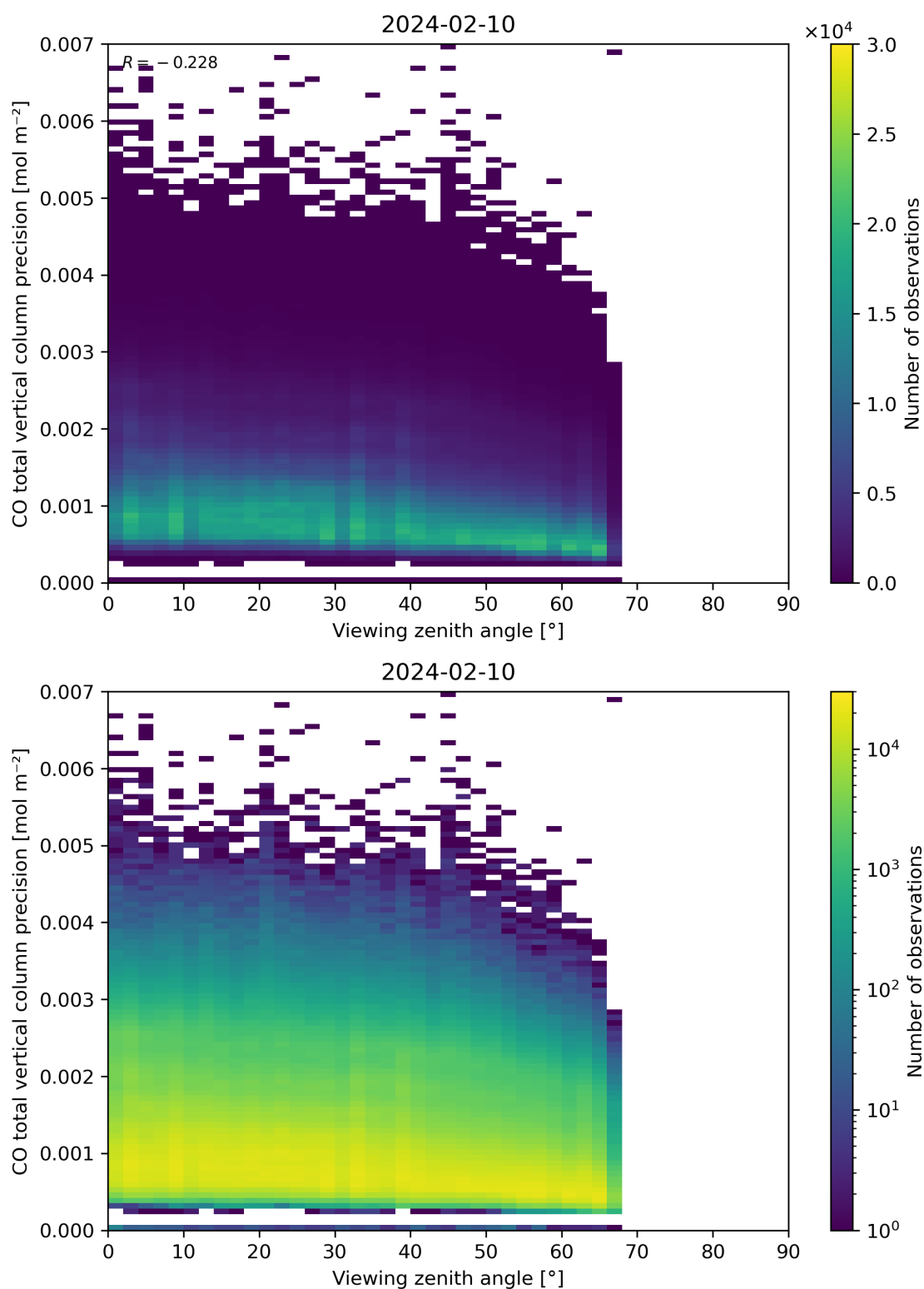
Figure 71: Scatter density plot of “Viewing zenith angle” against “CO total vertical column precision” for 2024-02-09 to 2024-02-11.
