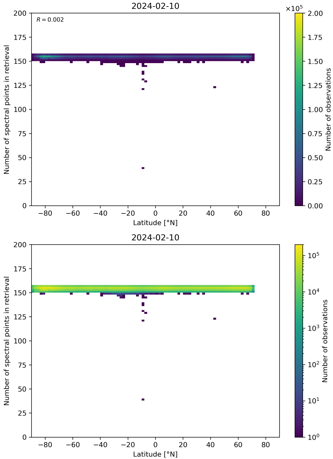
Figure 57: Scatter density plot of “Latitude” against “Number of spectral points in retrieval” for 2024-02-09 to 2024-02-11.
