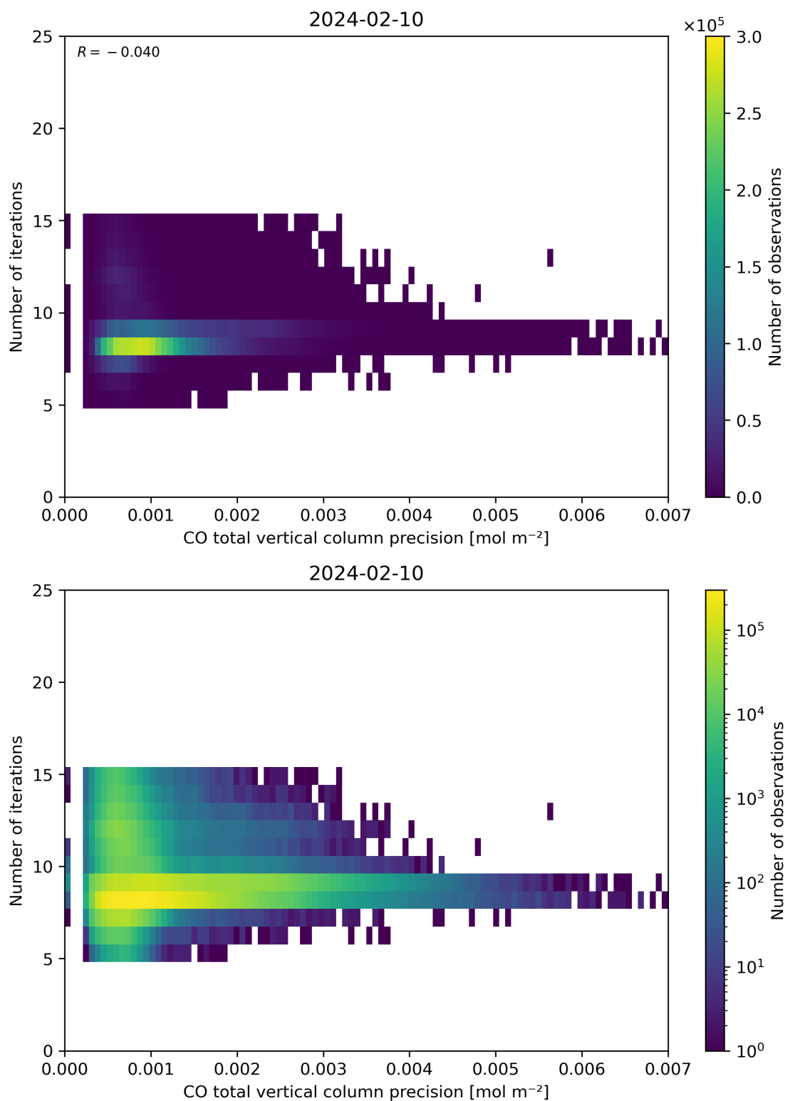
Figure 46: Scatter density plot of “CO total vertical column precision” against “Number of iterations” for 2024-02-09 to 2024-02-11.
