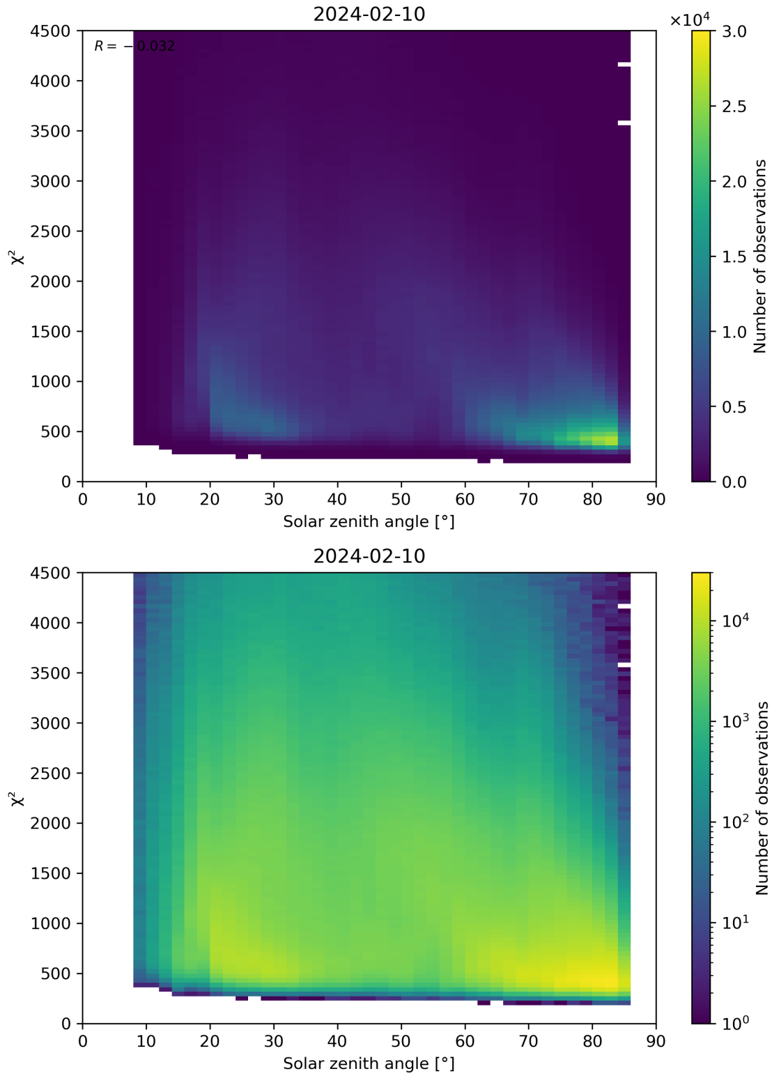
Figure 64: Scatter density plot of “Solar zenith angle” against “ \chi^2 ” for 2024-02-09 to 2024-02-11.
