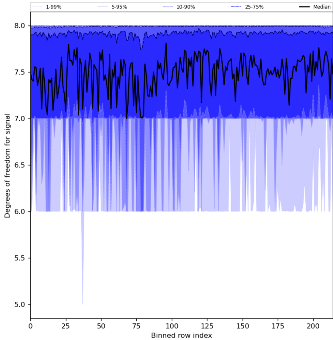
Figure 31: Along track statistics of “Degrees of freedom for signal” for 2024-02-09 to 2024-02-11
