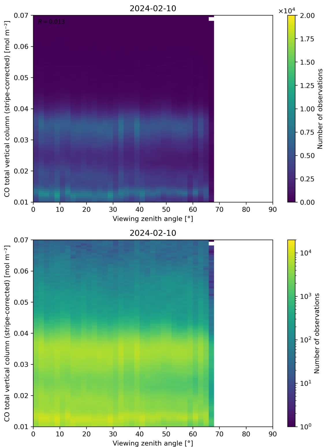
Figure 70: Scatter density plot of “Viewing zenith angle” against “CO total vertical column (stripe-corrected)” for 2024-02-09 to 2024-02-11.
