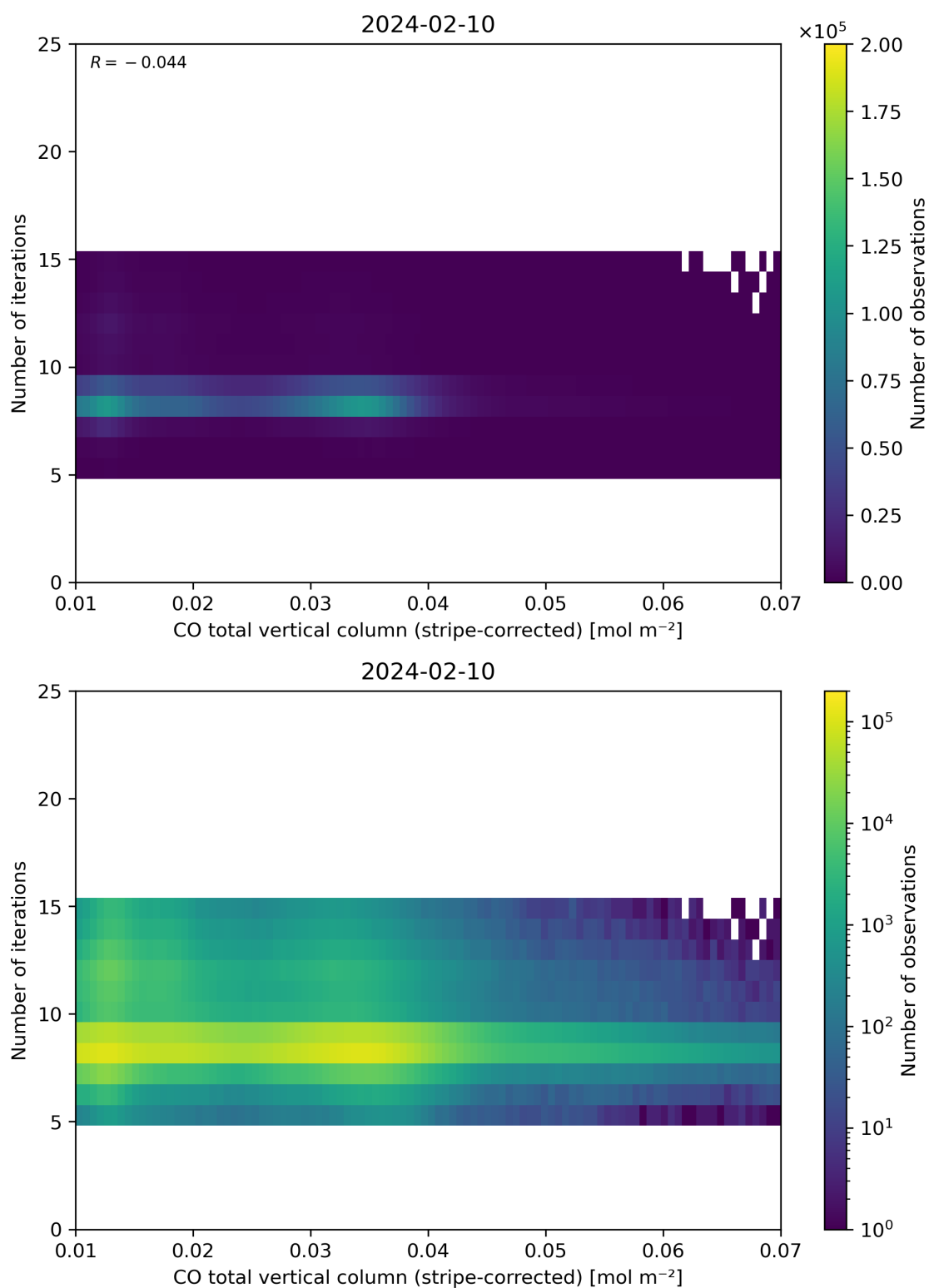
Figure 39: Scatter density plot of “CO total vertical column (stripe-corrected)” against “Number of iterations” for 2024-02-09 to 2024-02-11.
