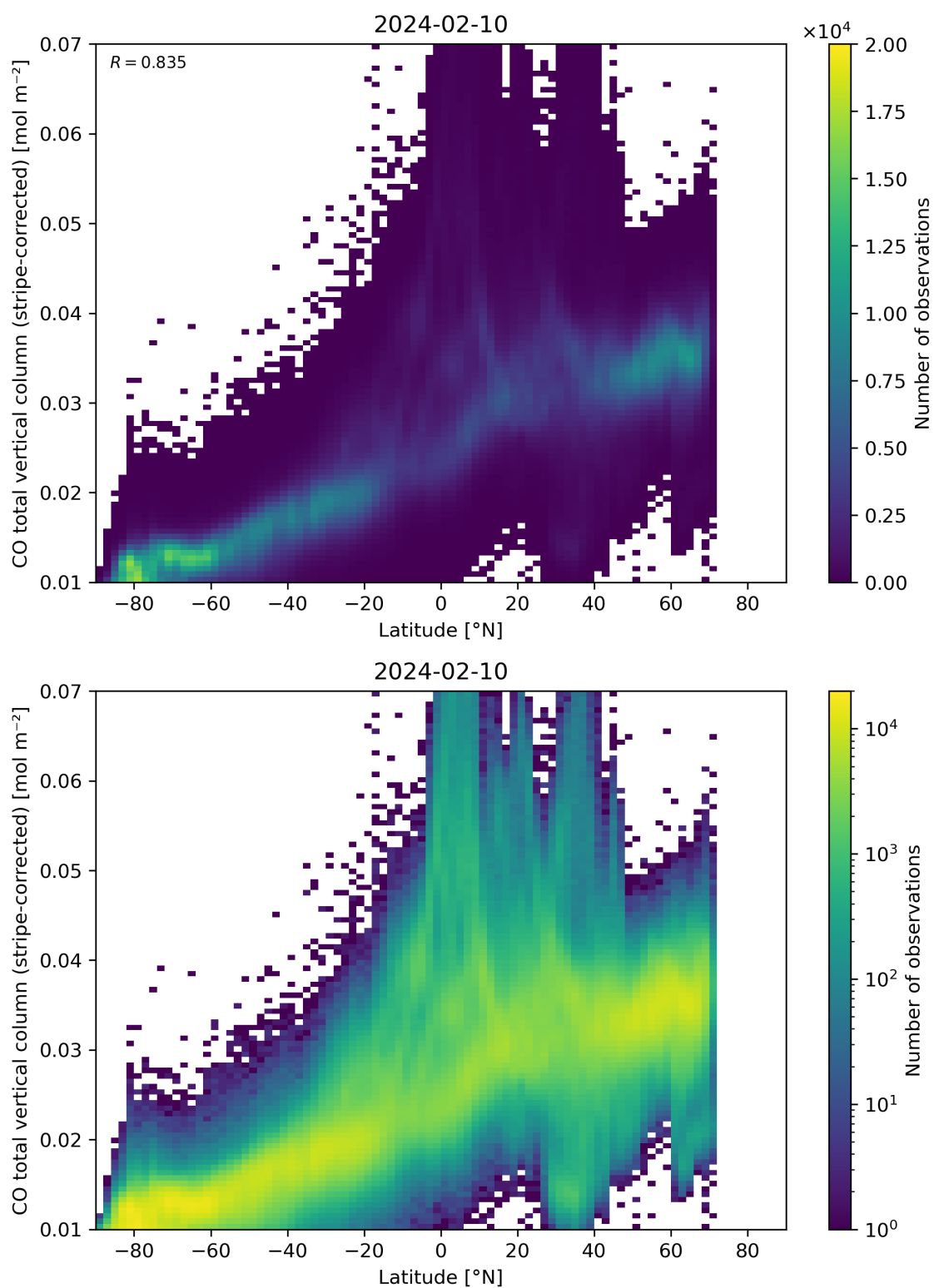
Figure 52: Scatter density plot of “Latitude” against “CO total vertical column (stripe-corrected)” for 2024-02-09 to 2024-02-11.
