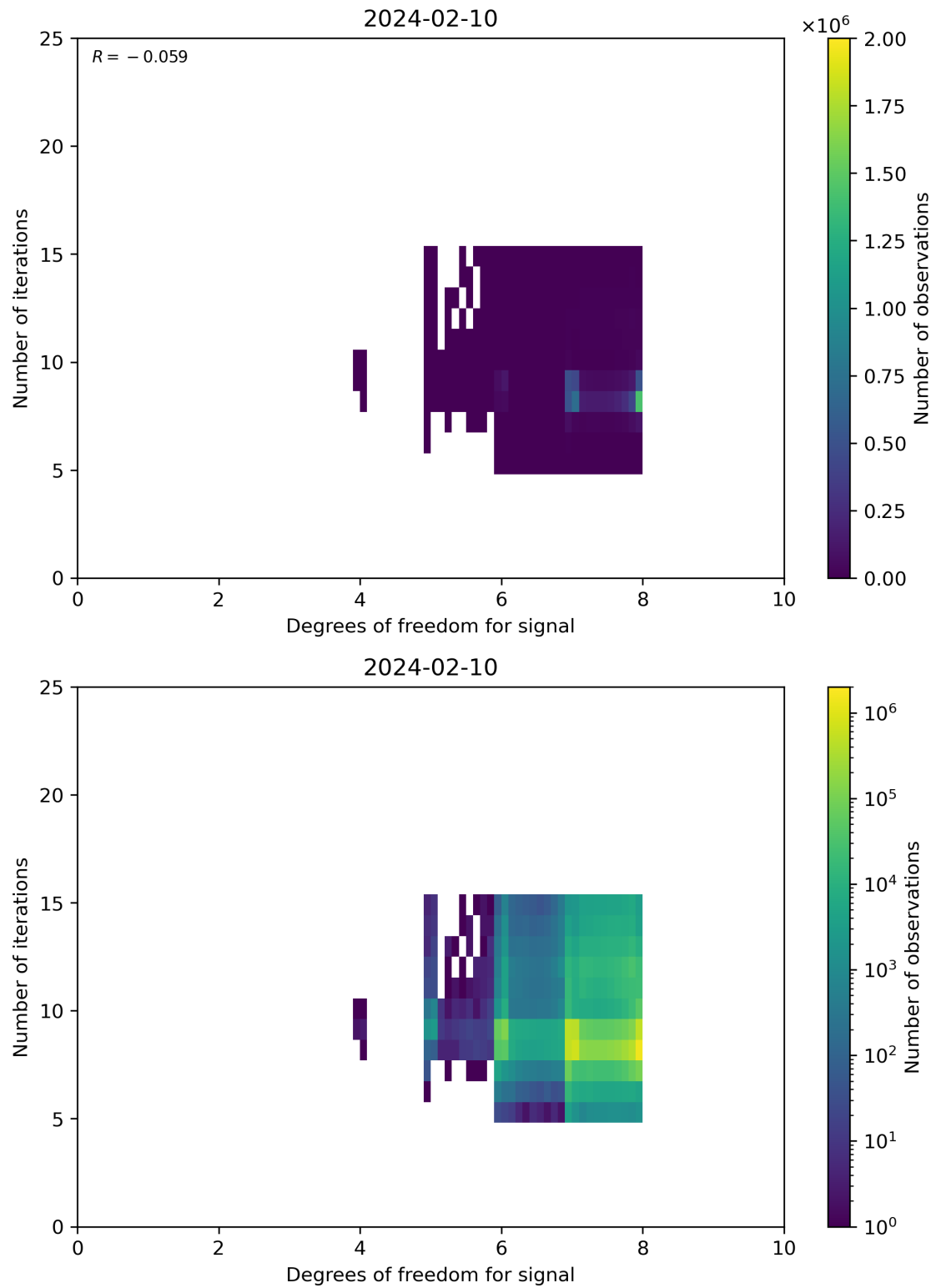
Figure 50: Scatter density plot of “Degrees of freedom for signal” against “Number of iterations” for 2024-02-09 to 2024-02-11.
