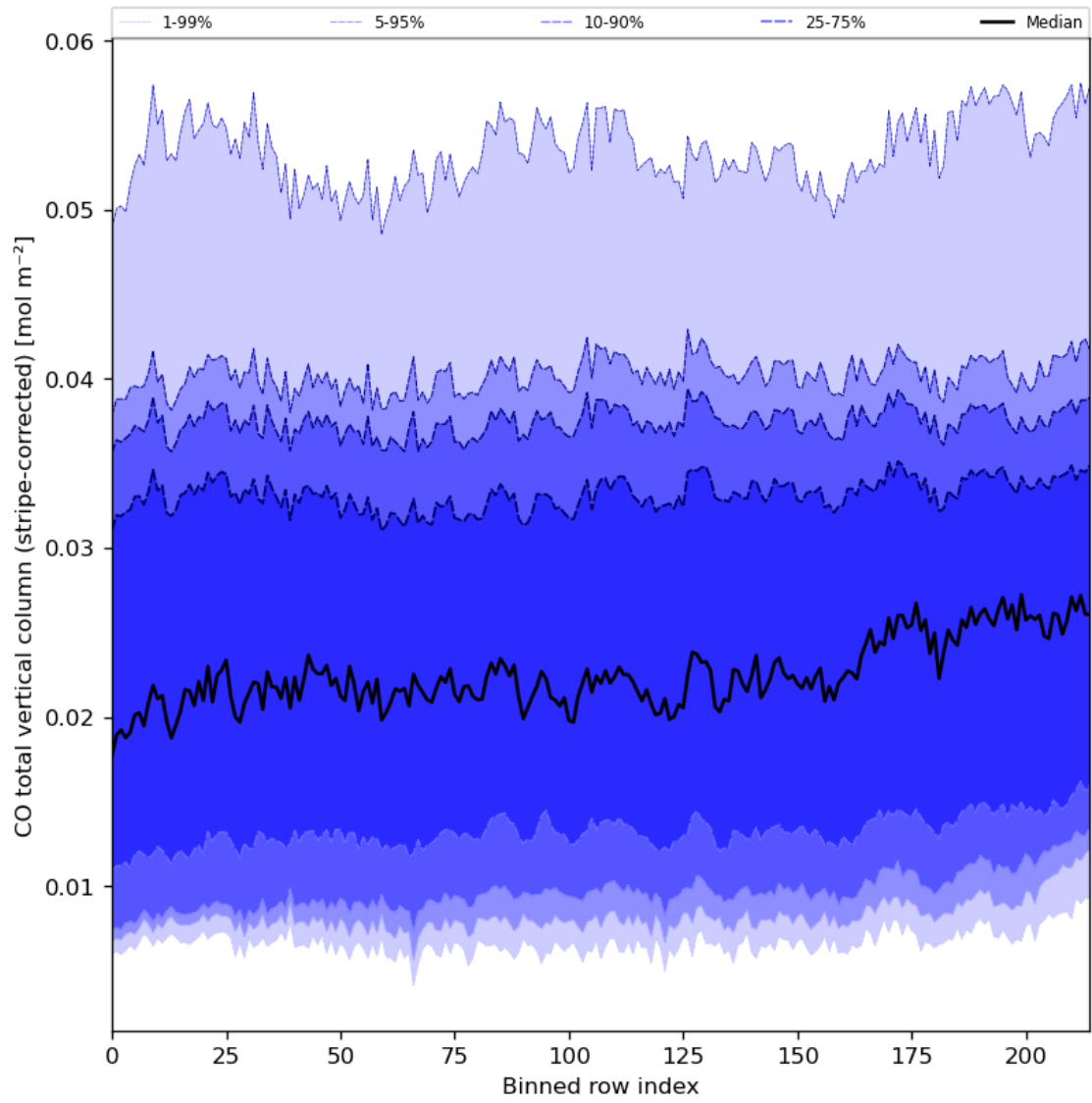
Figure 27: Along track statistics of “CO total vertical column (stripe-corrected)” for 2024-02-09 to 2024-02-11
