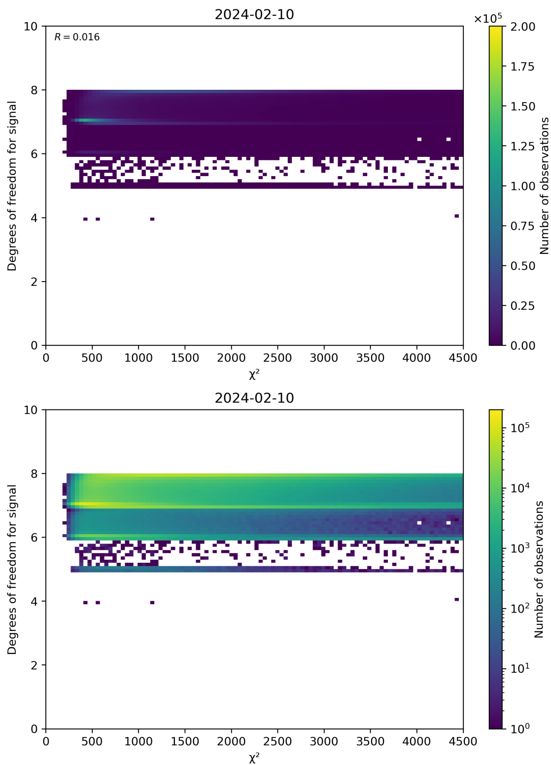
Figure 48: Scatter density plot of “ \chi^2 ” against “Degrees of freedom for signal” for 2024-02-09 to 2024-02-11.
