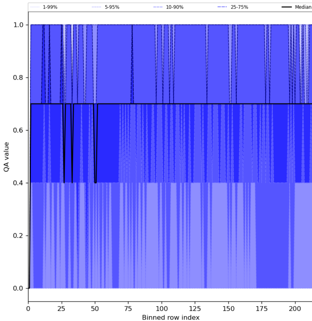
Figure 25: Along track statistics of “QA value” for 2024-02-09 to 2024-02-11
