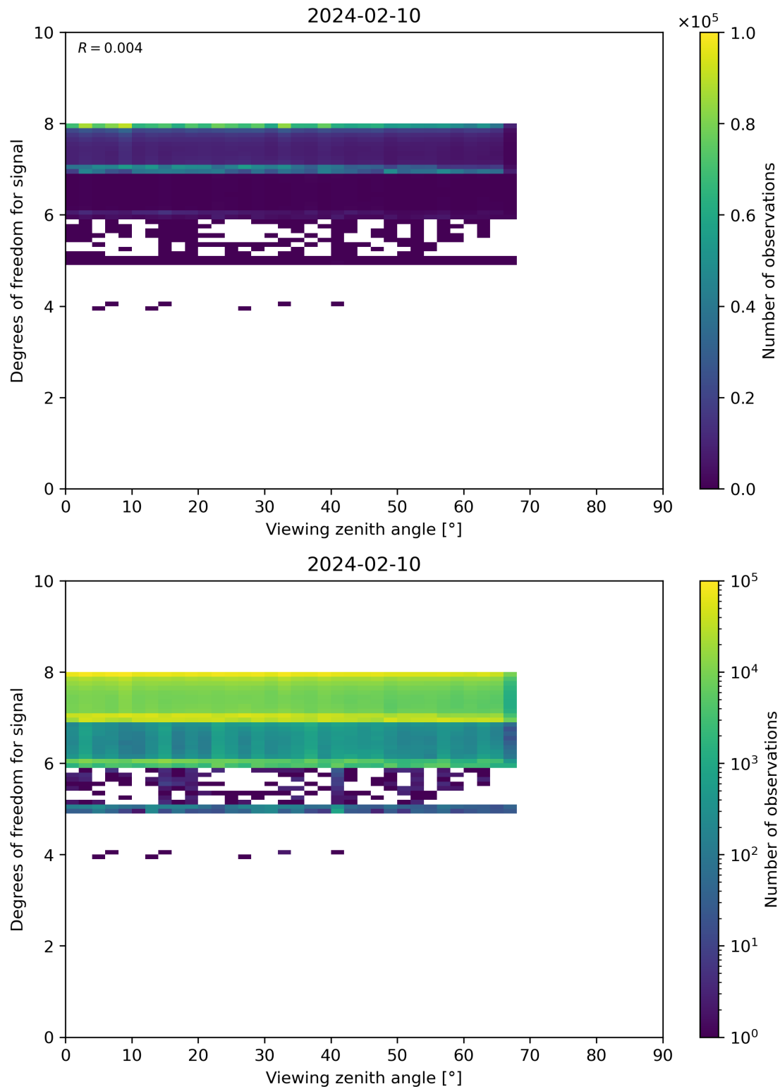
Figure 73: Scatter density plot of “Viewing zenith angle” against “Degrees of freedom for signal” for 2024-02-09 to 2024-02-11.
