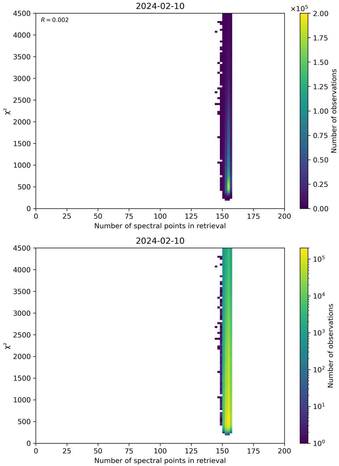
Figure 58: Scatter density plot of “Number of spectral points in retrieval” against “ \chi^2 ” for 2024-02-09 to 2024-02-11.
