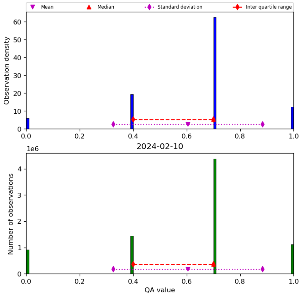
Figure 17: Histogram of “QA value” for 2024-02-09 to 2024-02-11
