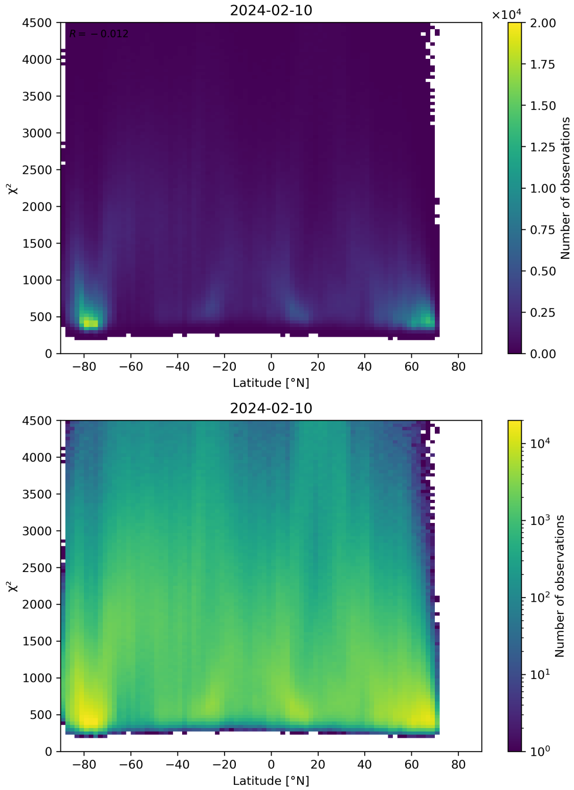
Figure 54: Scatter density plot of “Latitude” against “ \chi^2 ” for 2024-02-09 to 2024-02-11.
