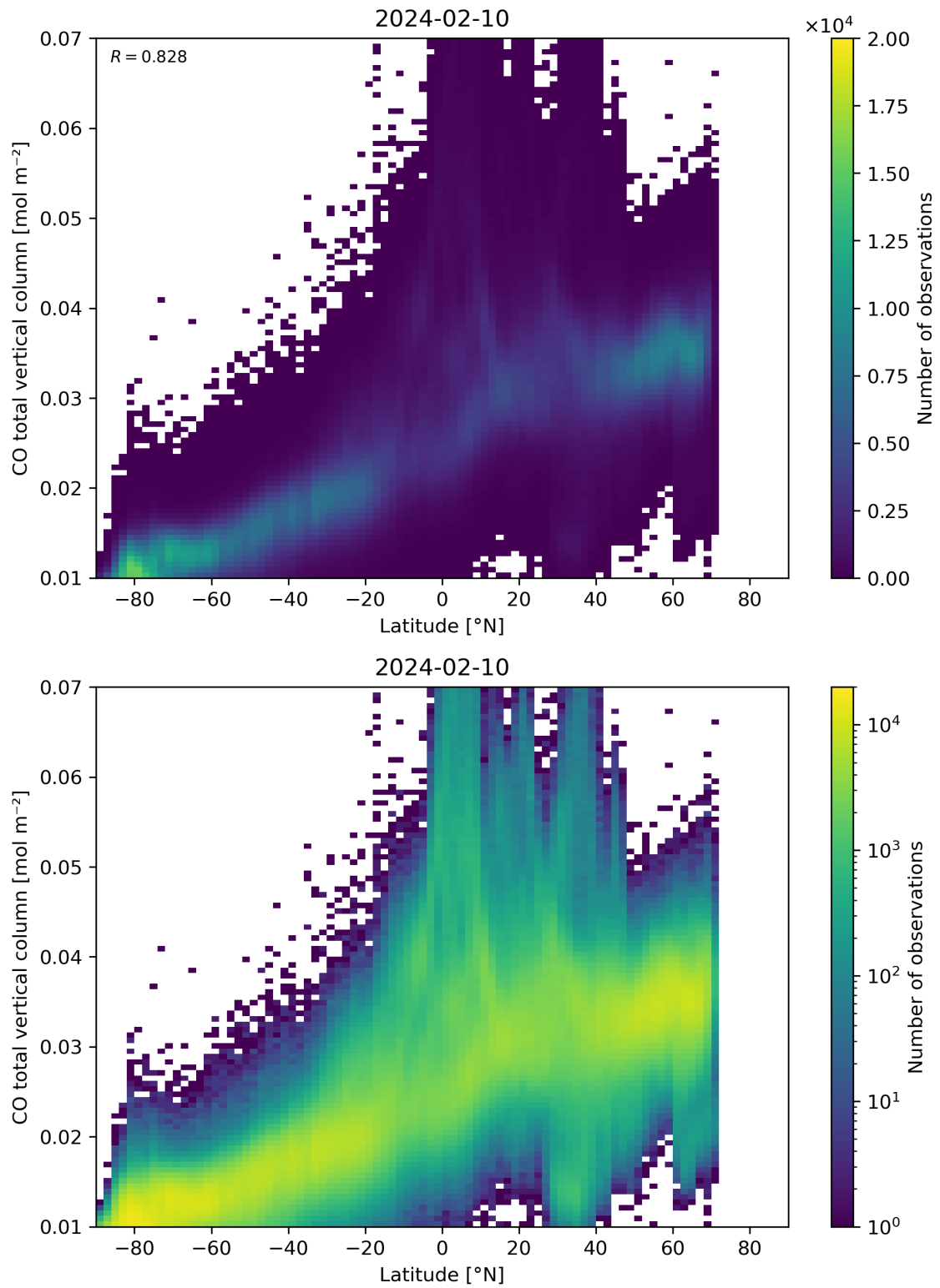
Figure 51: Scatter density plot of “Latitude” against “CO total vertical column” for 2024-02-09 to 2024-02-11.
