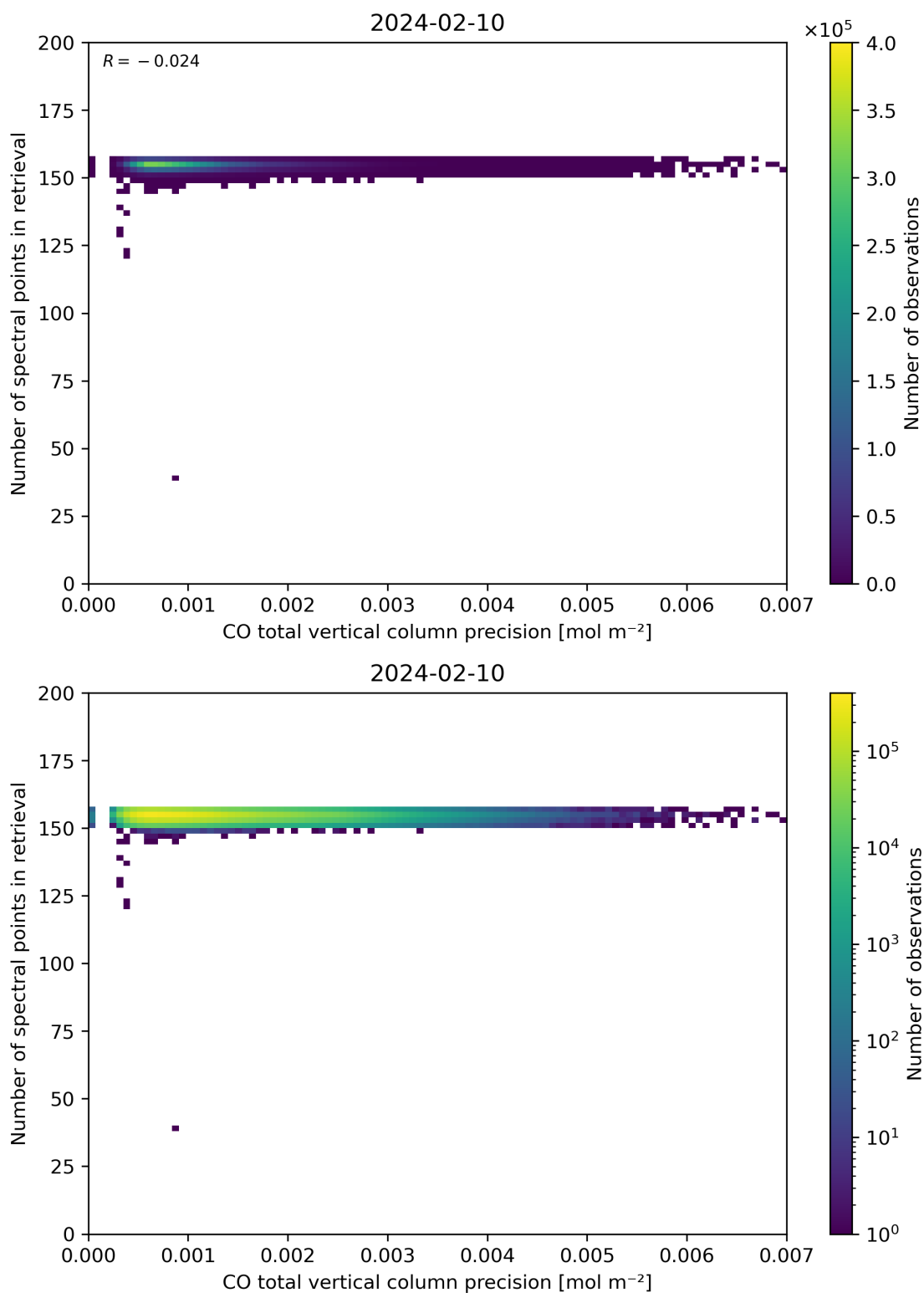
Figure 47: Scatter density plot of “CO total vertical column precision” against “Number of spectral points in retrieval” for 2024-02-09 to 2024-02-11.
