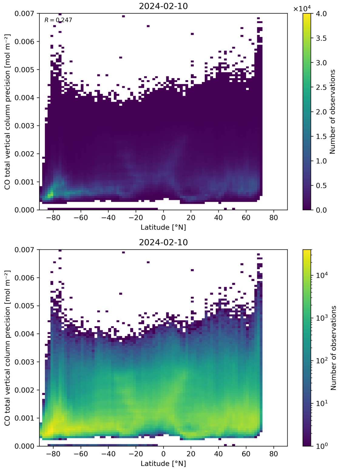
Figure 53: Scatter density plot of “Latitude” against “CO total vertical column precision” for 2024-02-09 to 2024-02-11.
