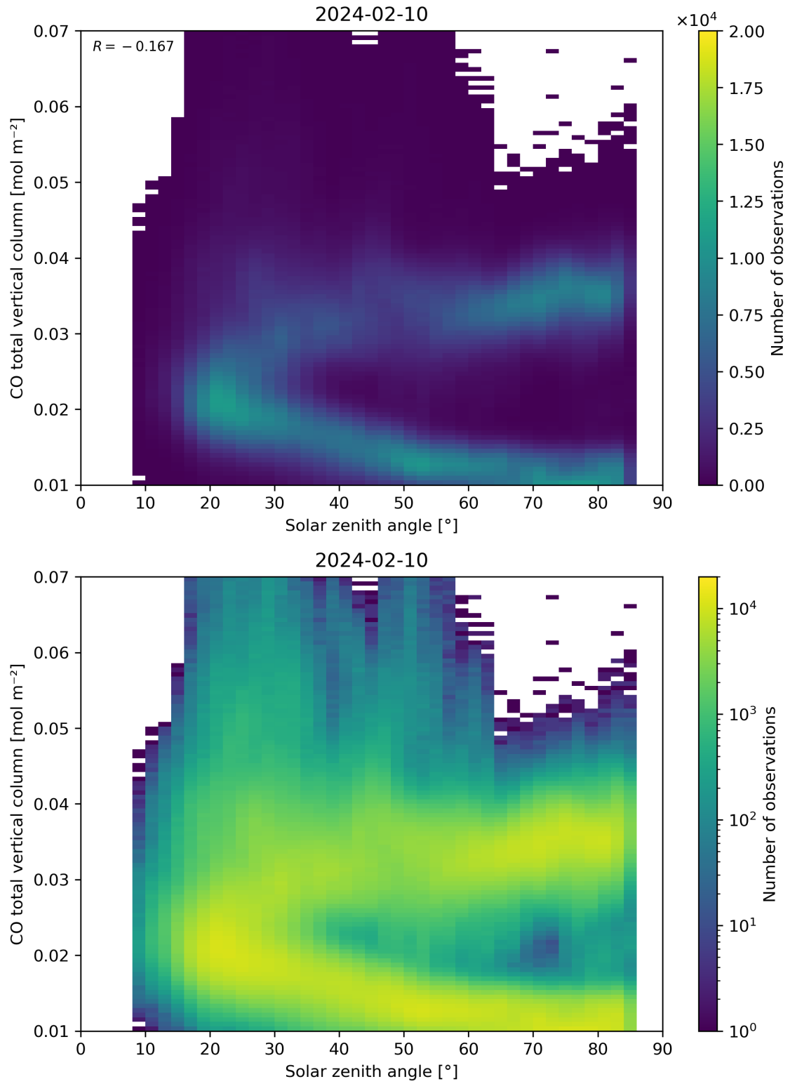
Figure 61: Scatter density plot of “Solar zenith angle” against “CO total vertical column” for 2024-02-09 to 2024-02-11.
