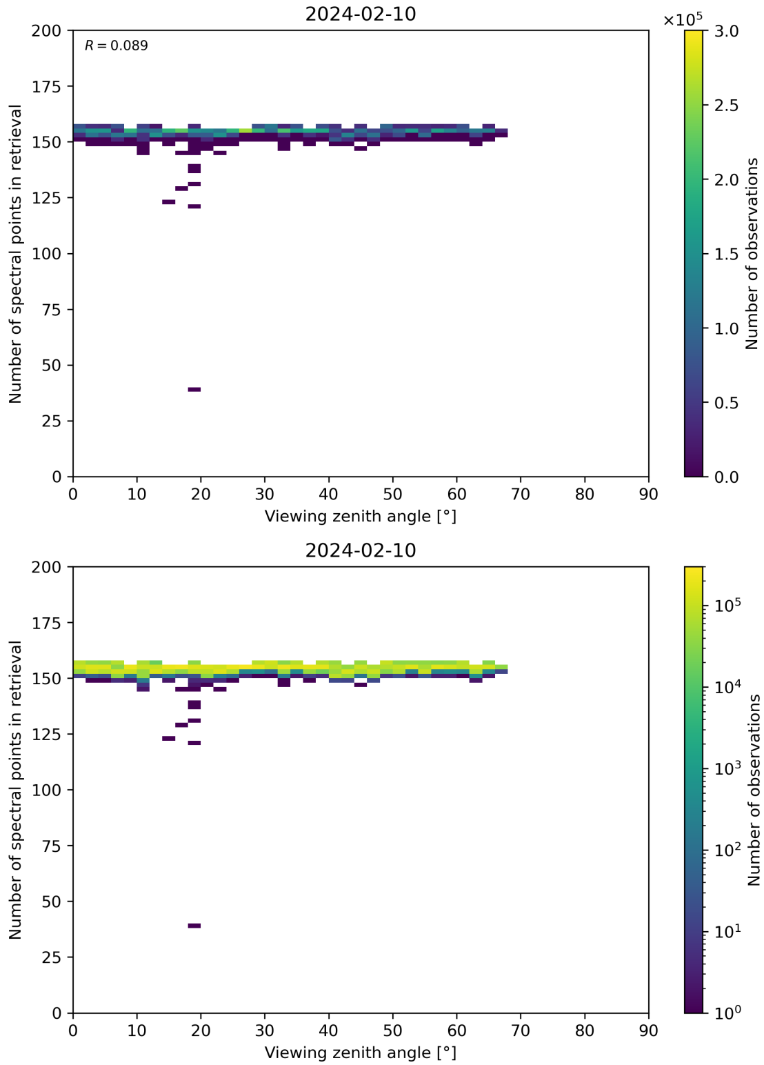
Figure 76: Scatter density plot of “Viewing zenith angle” against “Number of spectral points in retrieval” for 2024-02-09 to 2024-02-11.
