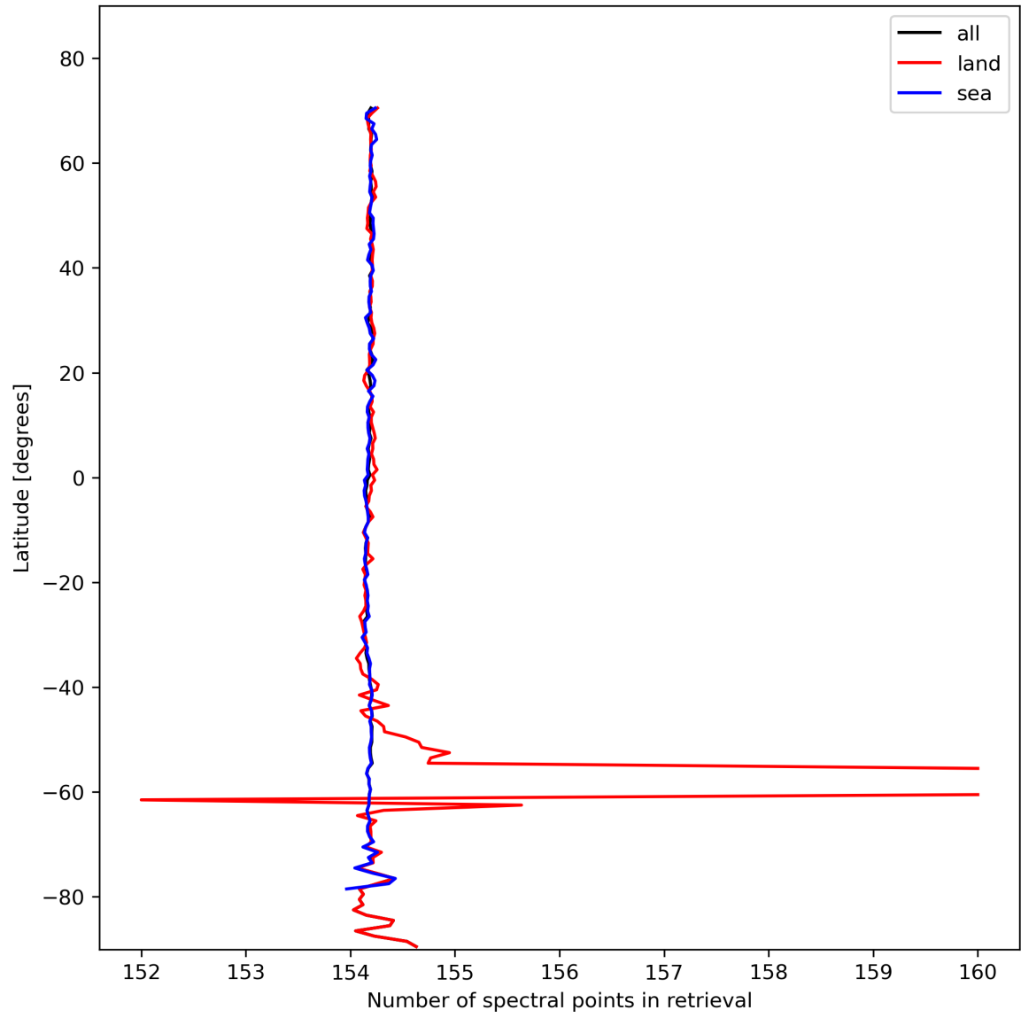
Figure 13: Zonal average of “Number of spectral points in retrieval” for 2024-02-09 to 2024-02-11.
