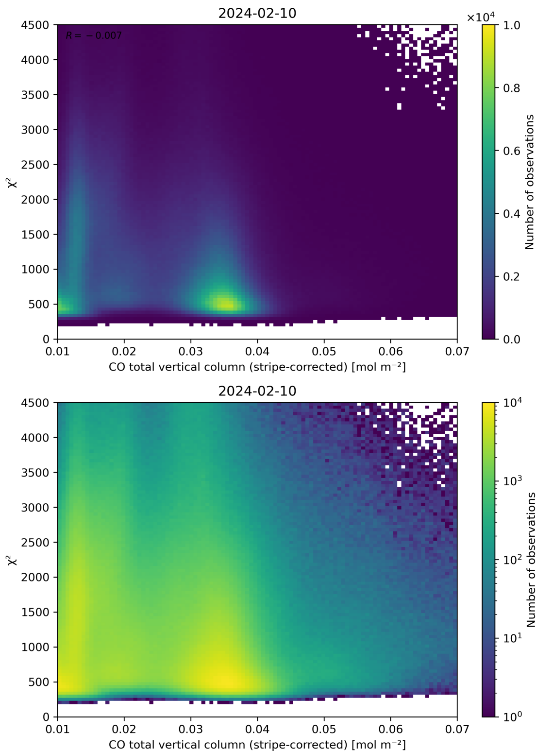
Figure 37: Scatter density plot of “CO total vertical column (stripe-corrected)” against “ \chi^2 ” for 2024-02-09 to 2024-02-11.
