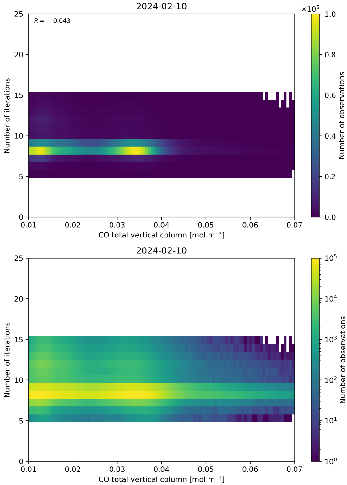
Figure 42: Scatter density plot of “CO total vertical column” against “Number of iterations” for 2024-02-09 to 2024-02-11.
