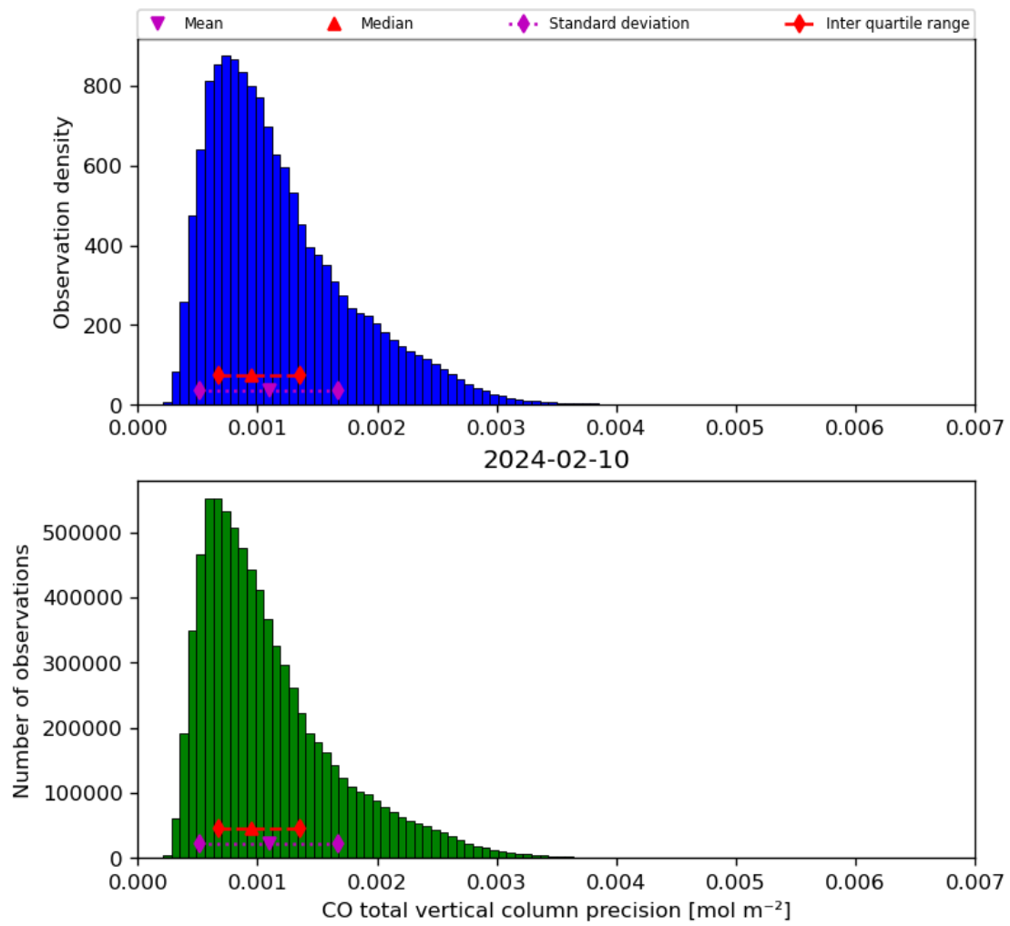
Figure 20: Histogram of “CO total vertical column precision” for 2024-02-09 to 2024-02-11
