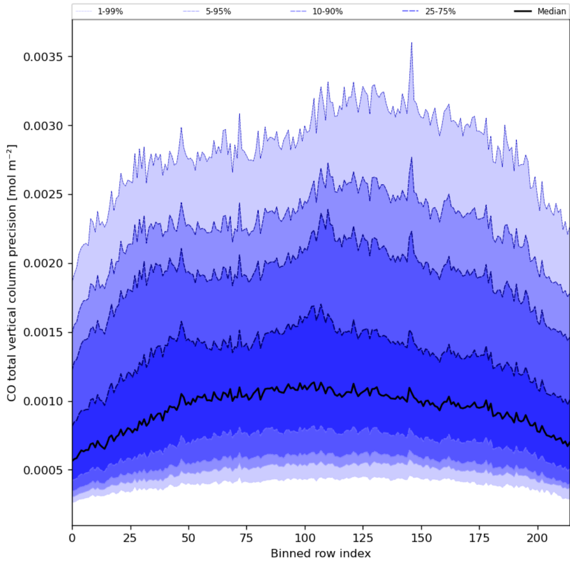
Figure 28: Along track statistics of “CO total vertical column precision” for 2024-02-09 to 2024-02-11
