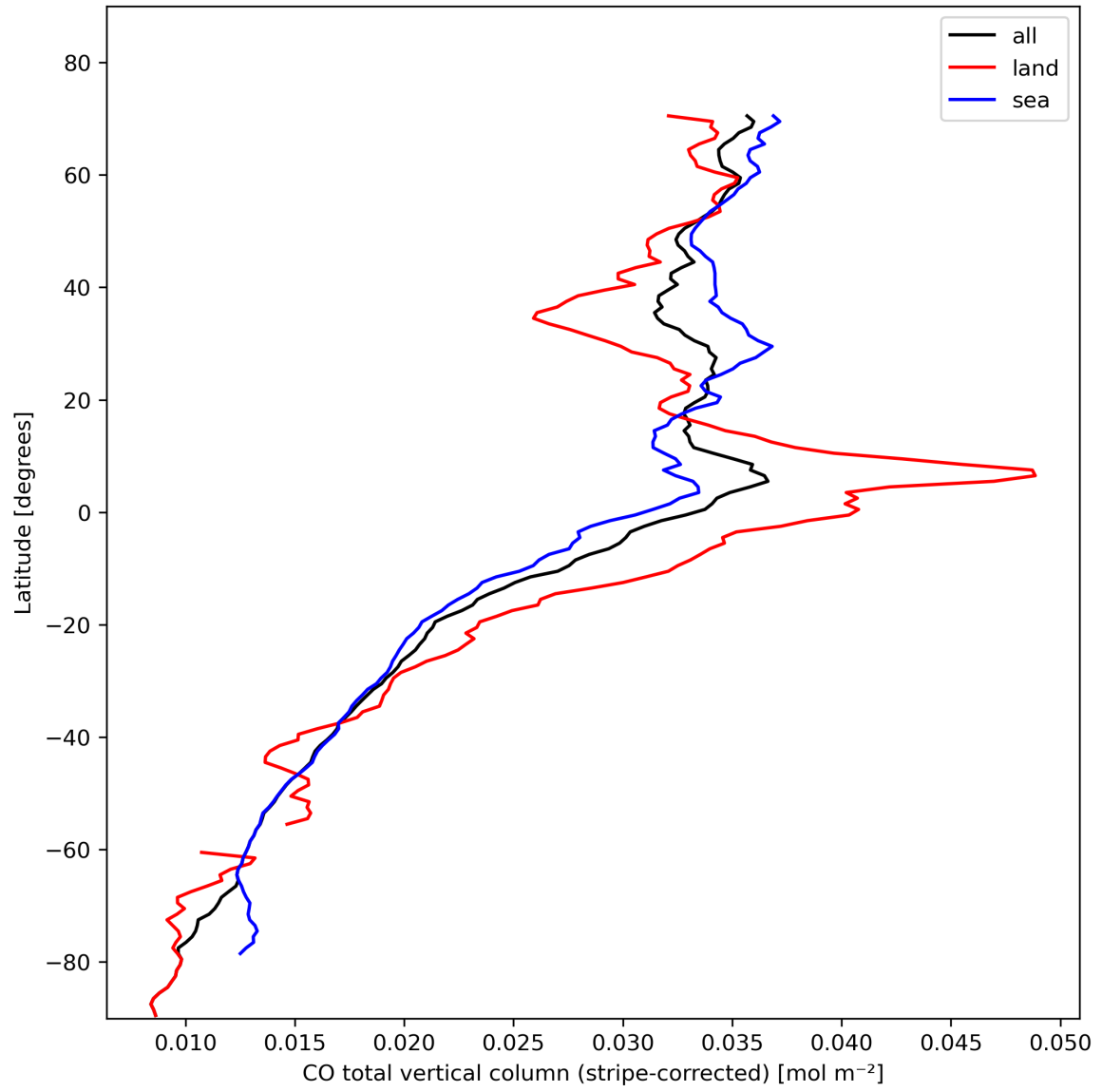
Figure 11: Zonal average of “CO total vertical column (stripe-corrected)” for 2024-02-09 to 2024-02-11.
