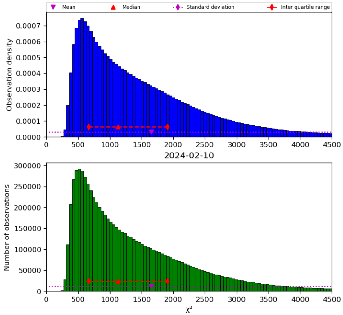
Figure 22: Histogram of “ \chi^2 ” for 2024-02-09 to 2024-02-11
