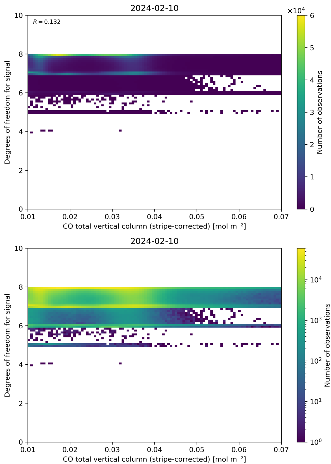
Figure 38: Scatter density plot of “CO total vertical column (stripe-corrected)” against “Degrees of freedom for signal” for 2024-02-09 to 2024-02-11.
