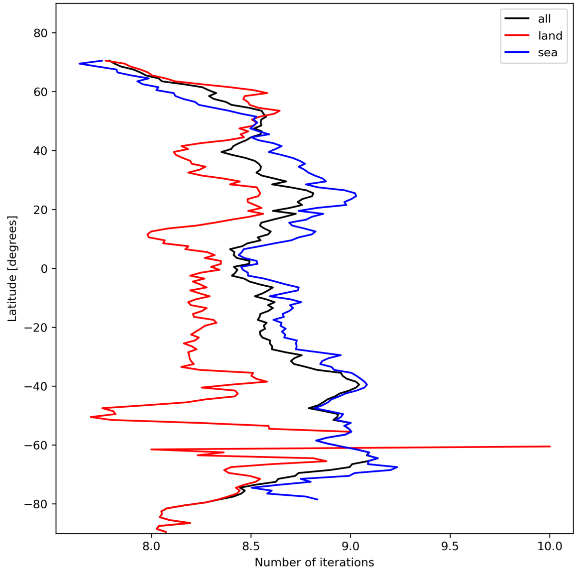
Figure 16: Zonal average of “Number of iterations” for 2024-02-09 to 2024-02-11.
