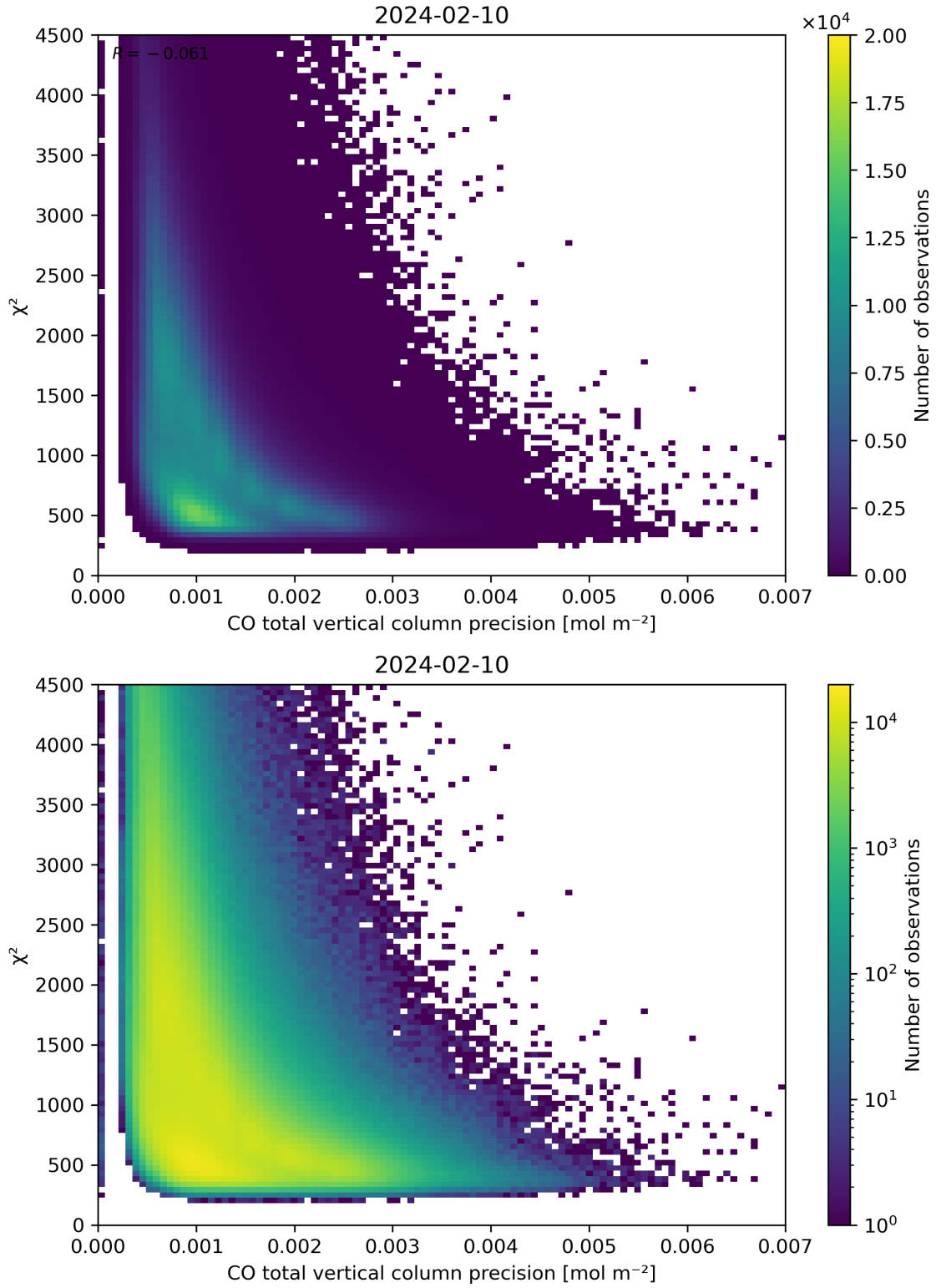
Figure 44: Scatter density plot of “CO total vertical column precision” against “ \chi^2 ” for 2024-02-09 to 2024-02-11.
