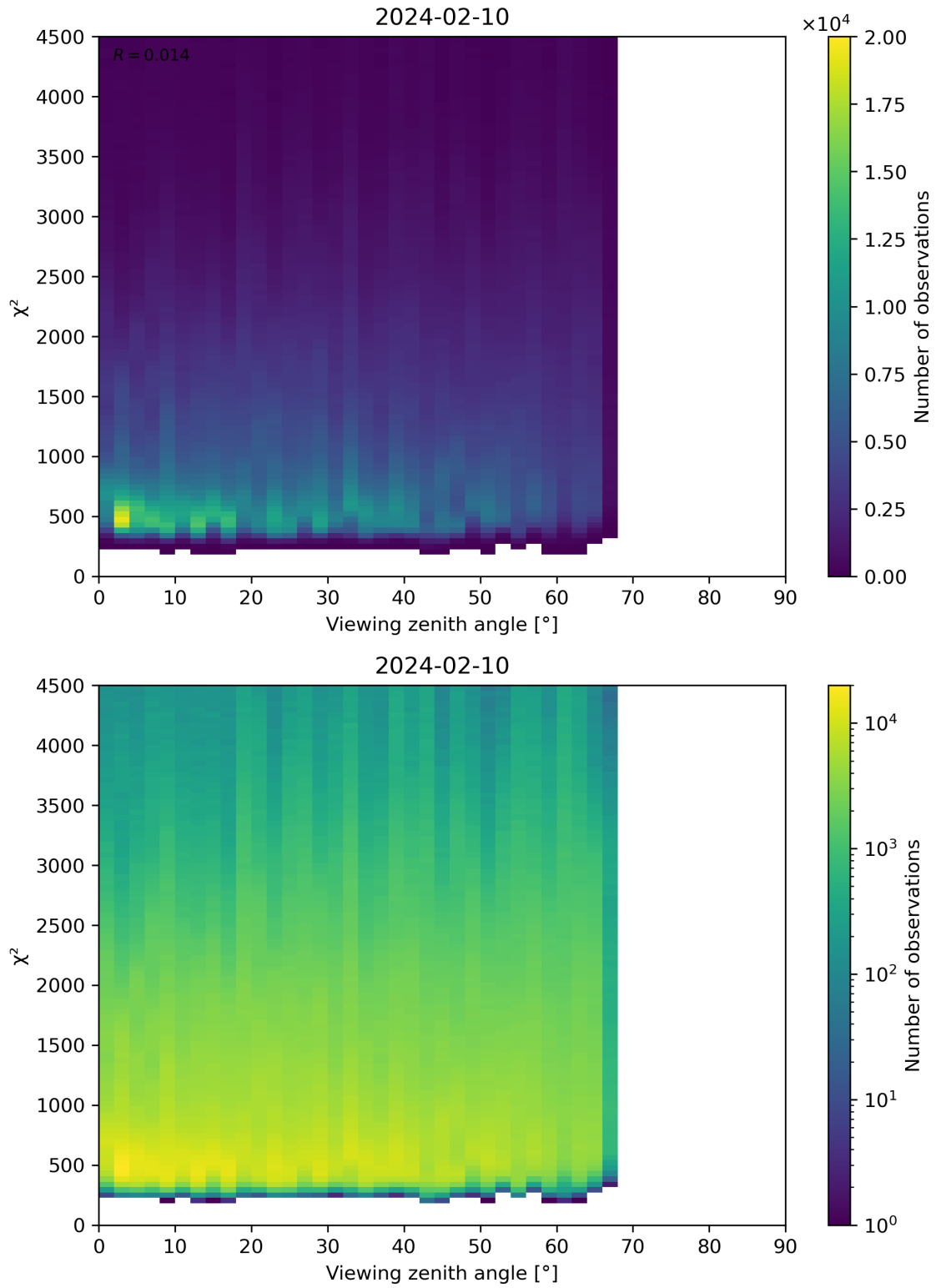
Figure 72: Scatter density plot of “Viewing zenith angle” against “ \chi^2 ” for 2024-02-09 to 2024-02-11.
