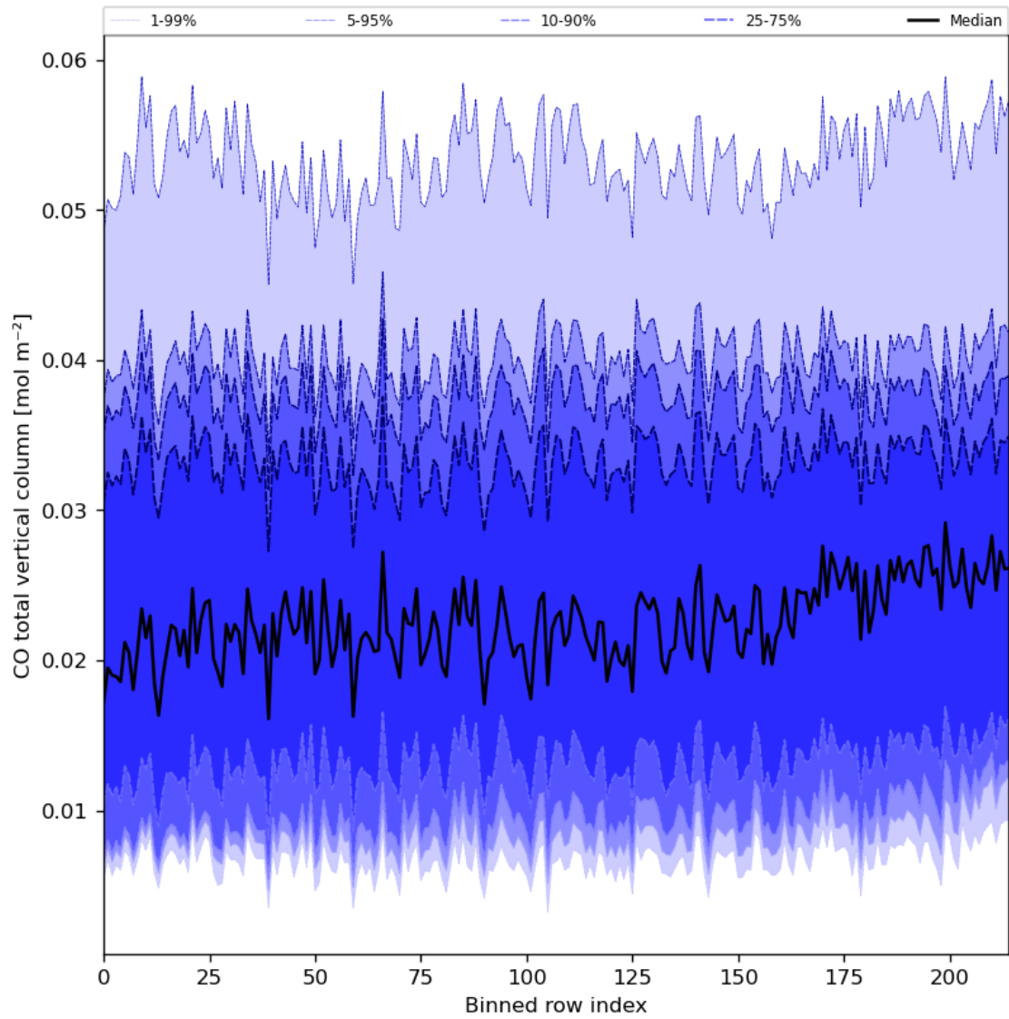
Figure 26: Along track statistics of “CO total vertical column” for 2024-02-09 to 2024-02-11
