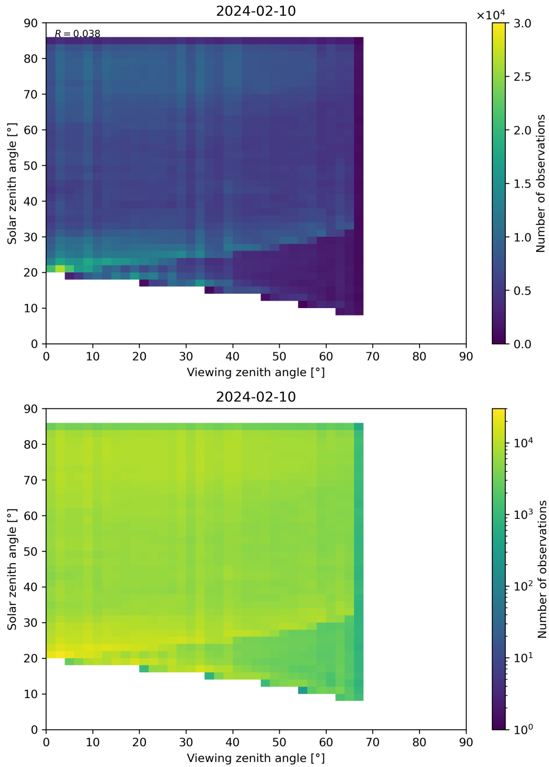
Figure 77: Scatter density plot of “Viewing zenith angle” against “Solar zenith angle” for 2024-02-09 to 2024-02-11.
