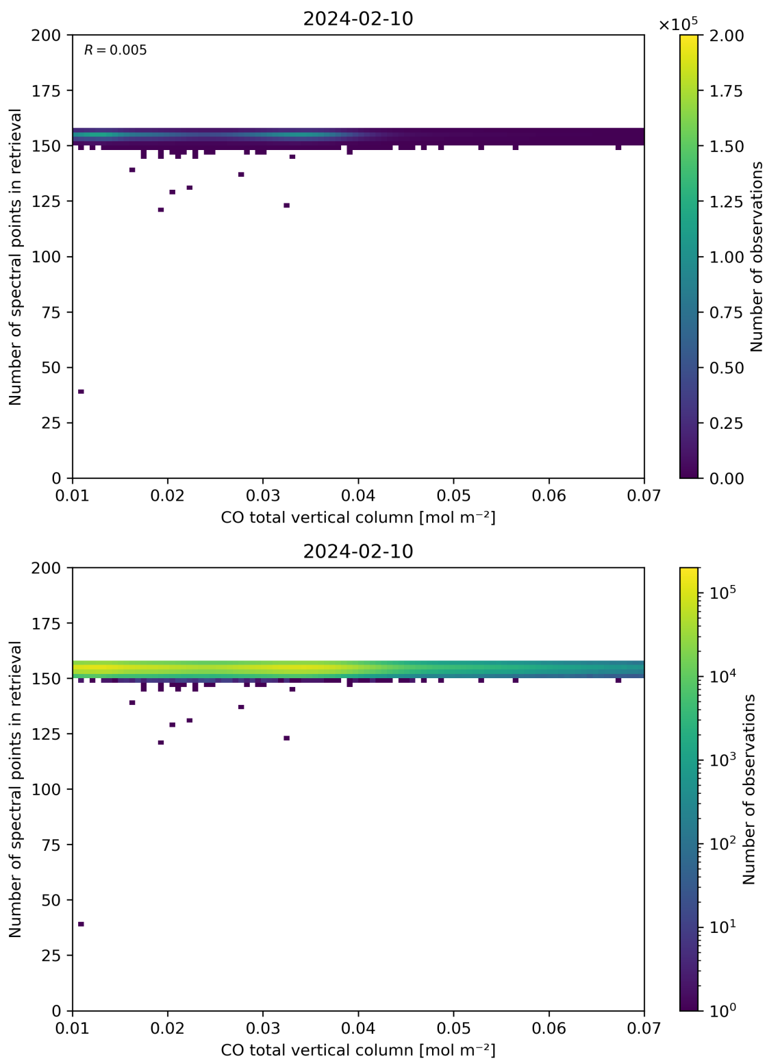
Figure 43: Scatter density plot of “CO total vertical column” against “Number of spectral points in retrieval” for 2024-02-09 to 2024-02-11.
