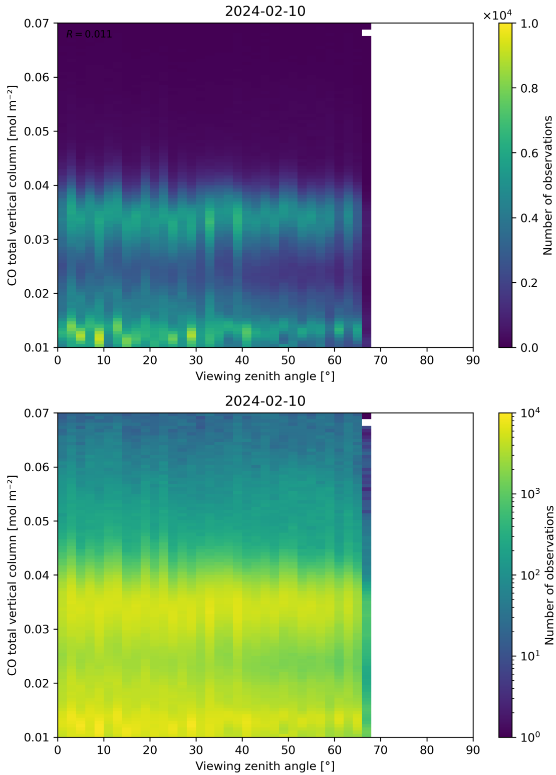
Figure 69: Scatter density plot of “Viewing zenith angle” against “CO total vertical column” for 2024-02-09 to 2024-02-11.
