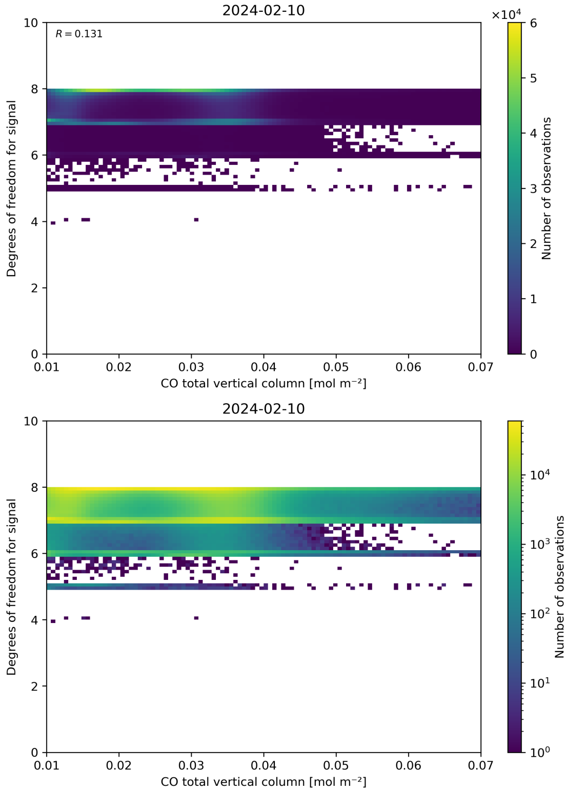
Figure 41: Scatter density plot of “CO total vertical column” against “Degrees of freedom for signal” for 2024-02-09 to 2024-02-11.
