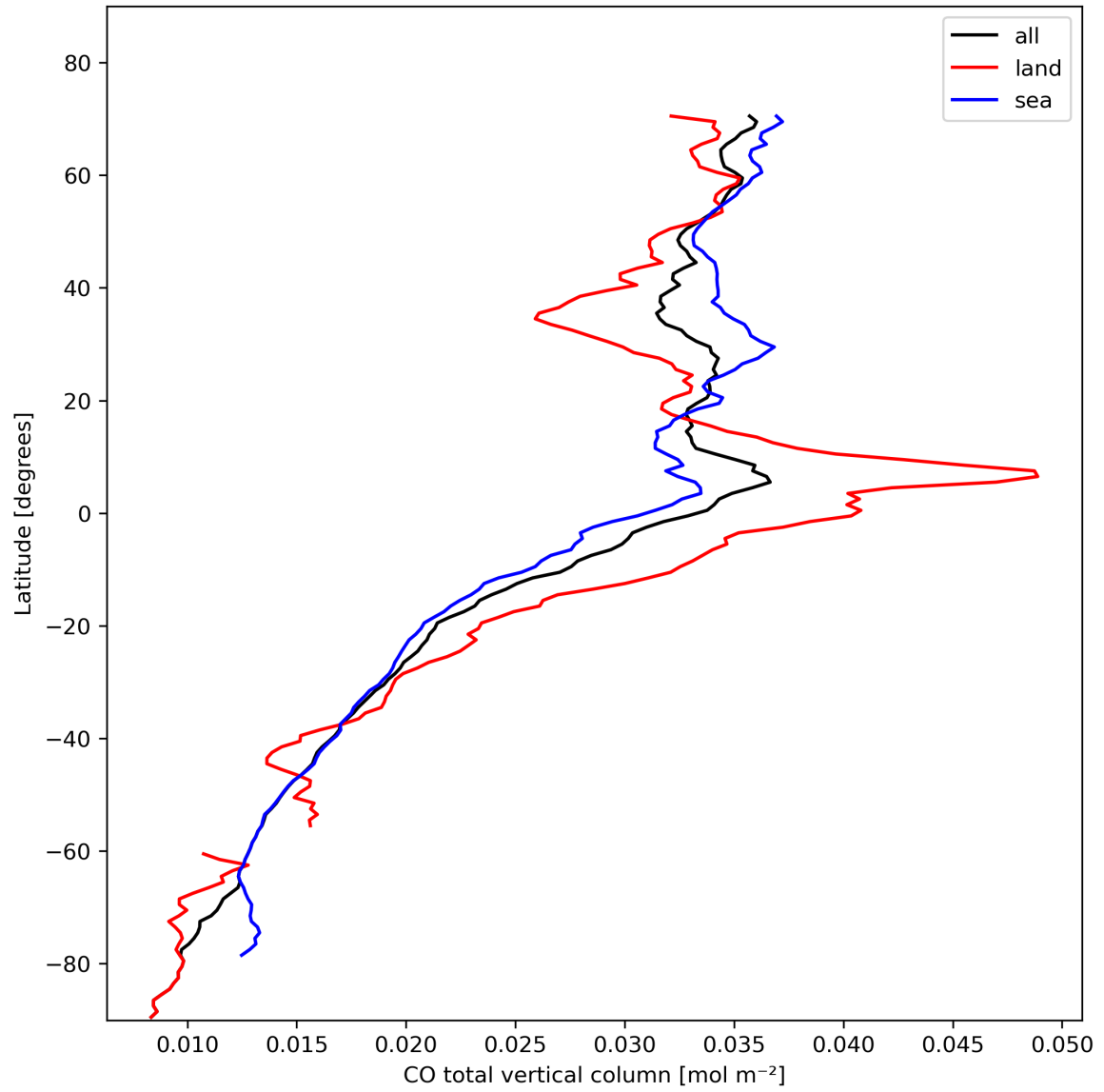
Figure 10: Zonal average of “CO total vertical column” for 2024-02-09 to 2024-02-11.
