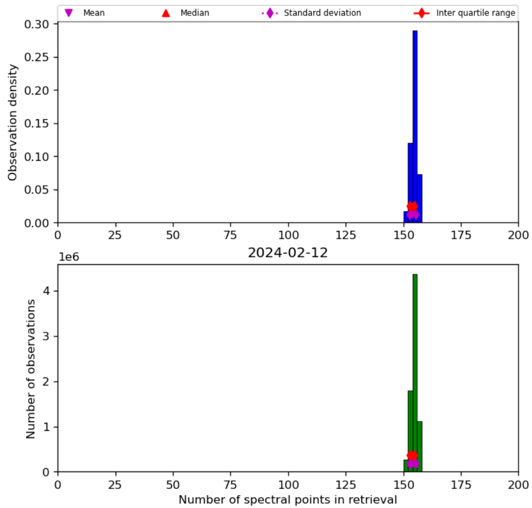
Figure 21: Histogram of “Number of spectral points in retrieval” for 2024-02-11 to 2024-02-13
