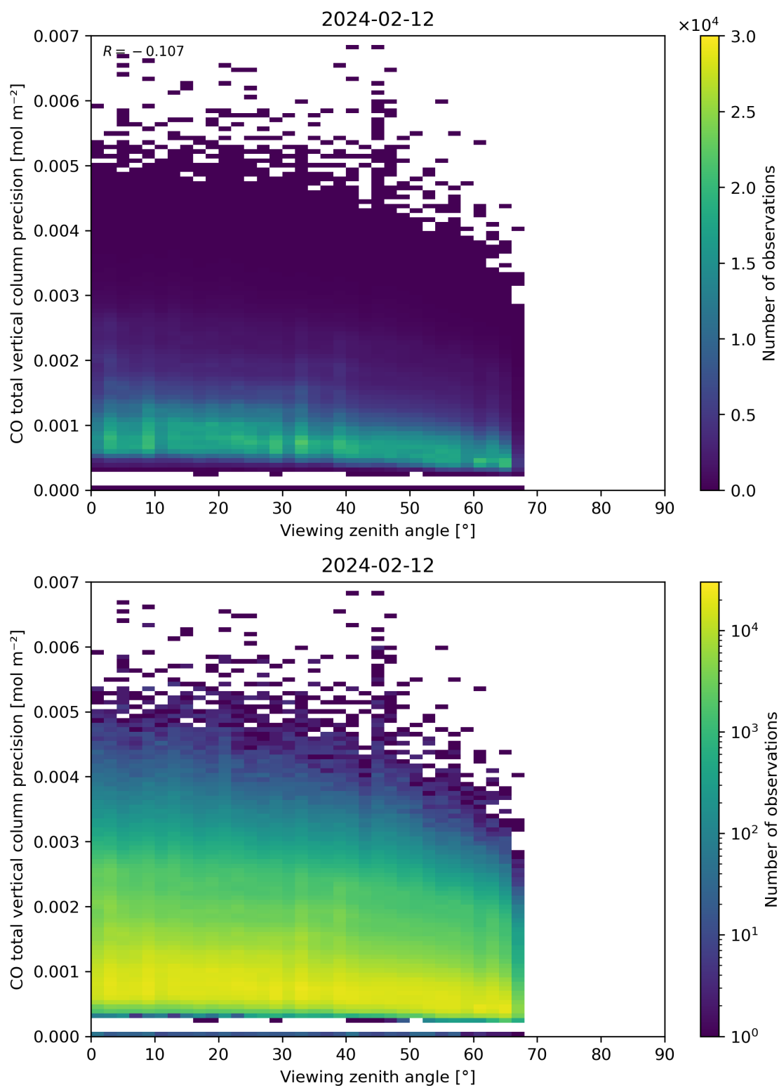
Figure 71: Scatter density plot of “Viewing zenith angle” against “CO total vertical column precision” for 2024-02-11 to 2024-02-13.
