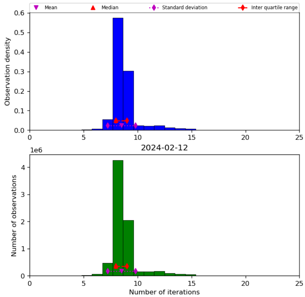
Figure 24: Histogram of “Number of iterations” for 2024-02-11 to 2024-02-13
