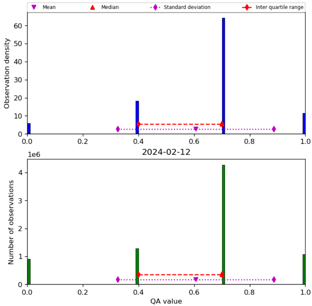
Figure 17: Histogram of “QA value” for 2024-02-11 to 2024-02-13
