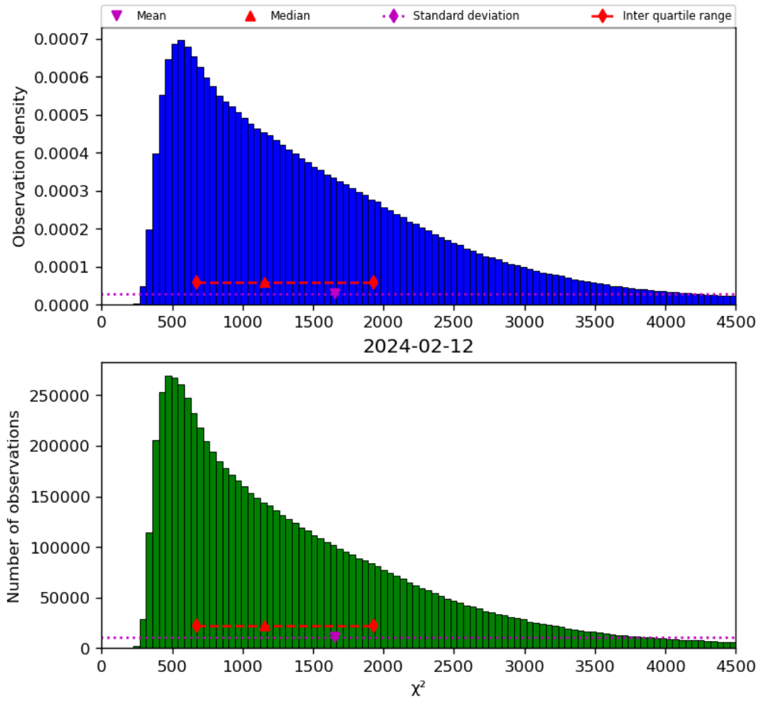
Figure 22: Histogram of “ \chi^2 ” for 2024-02-11 to 2024-02-13
