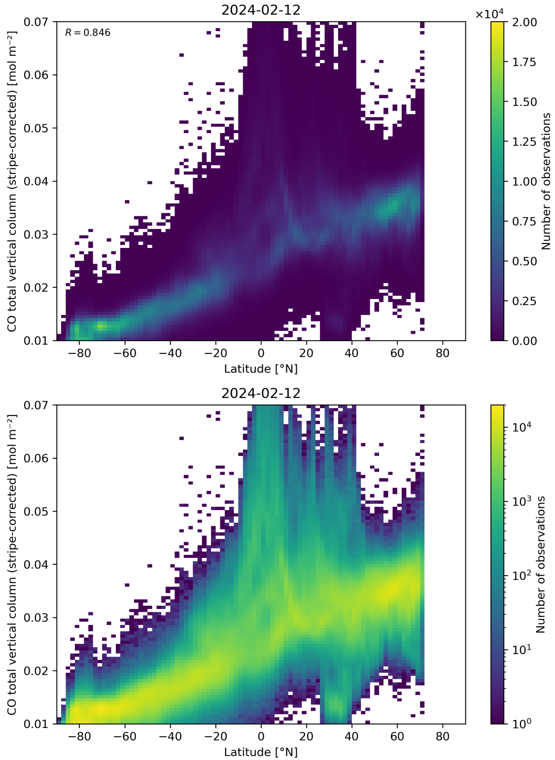
Figure 52: Scatter density plot of “Latitude” against “CO total vertical column (stripe-corrected)” for 2024-02-11 to 2024-02-13.
