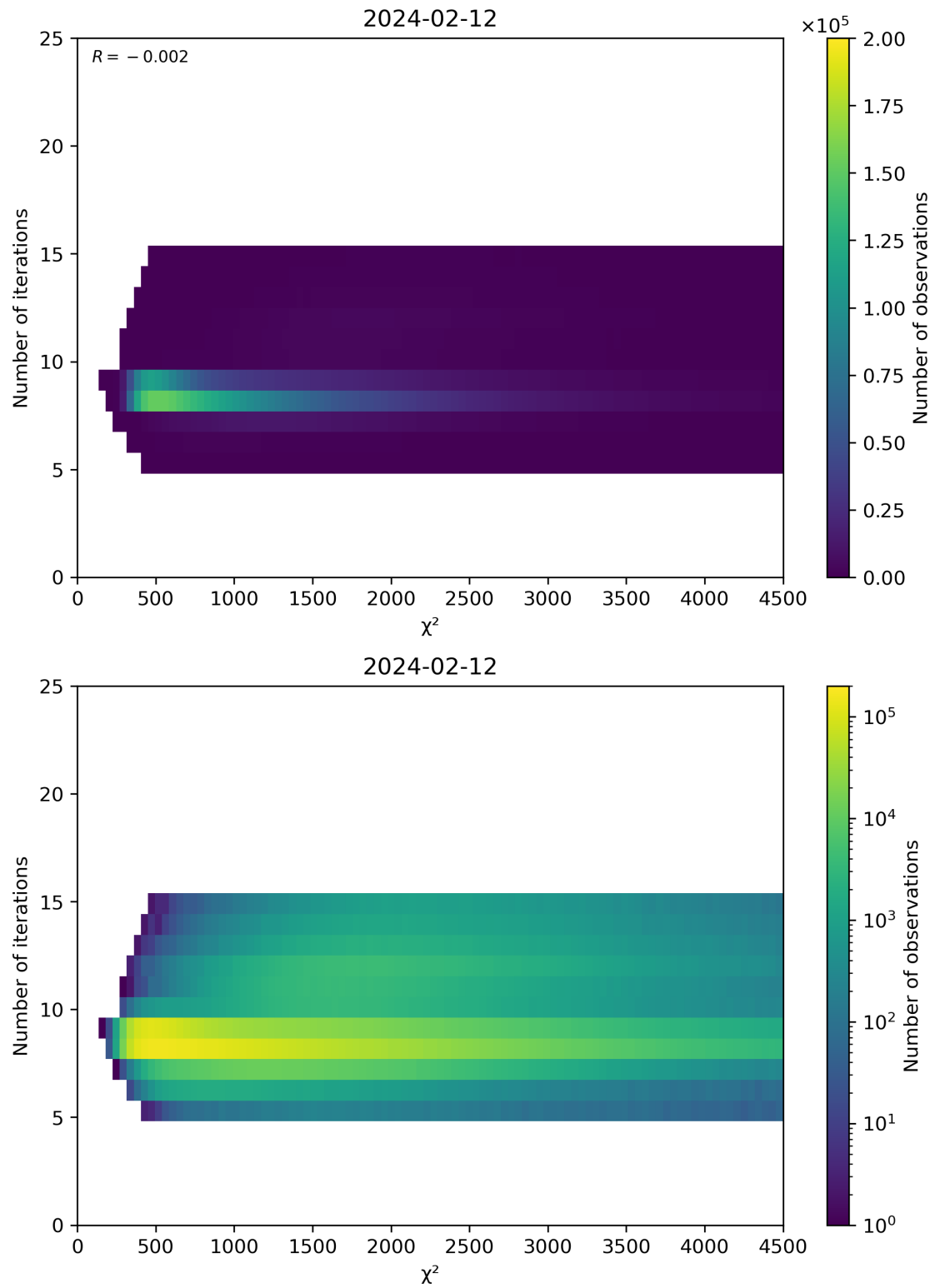
Figure 49: Scatter density plot of “ \chi^2 ” against “Number of iterations” for 2024-02-11 to 2024-02-13.
