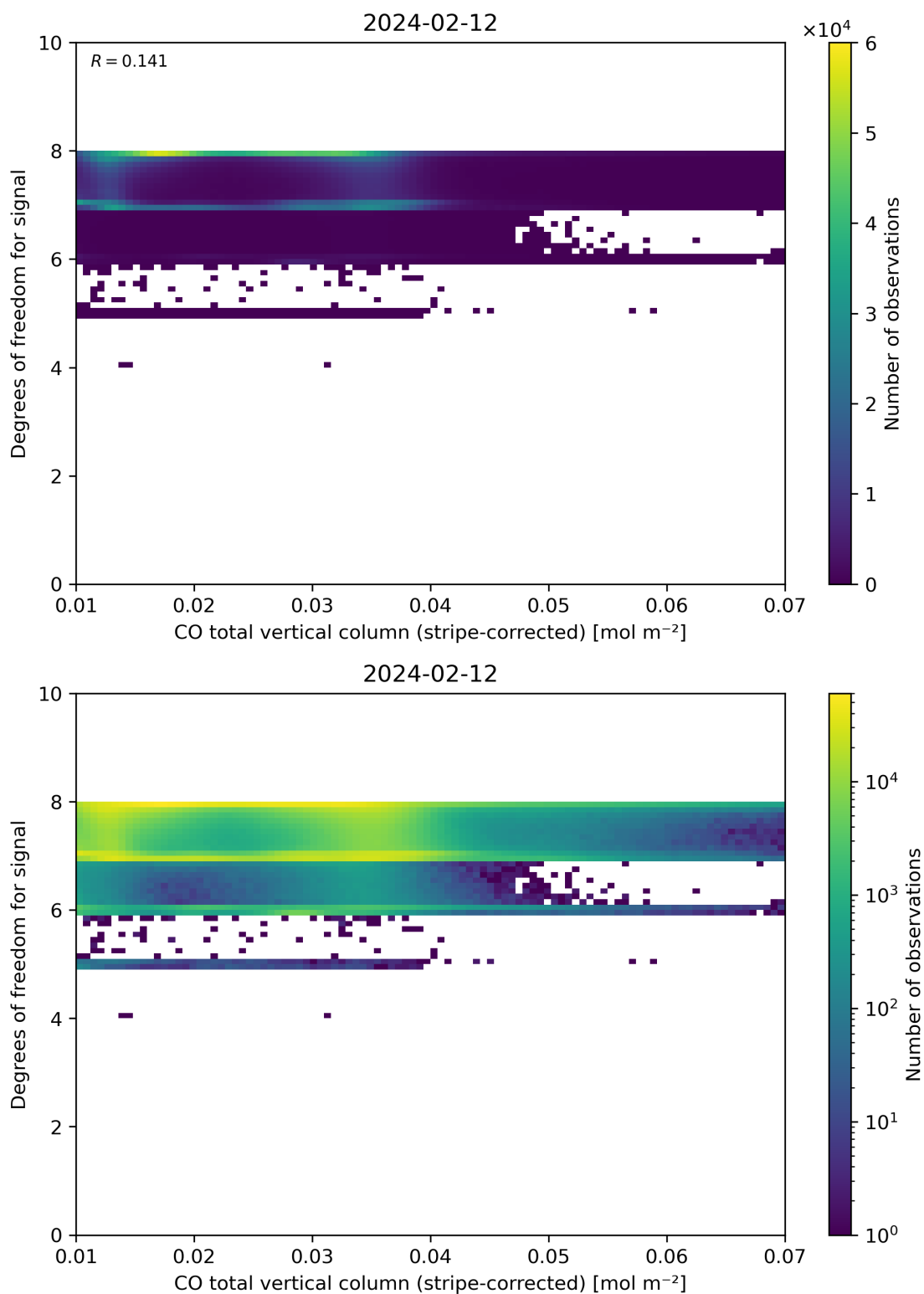
Figure 38: Scatter density plot of “CO total vertical column (stripe-corrected)” against “Degrees of freedom for signal” for 2024-02-11 to 2024-02-13.
