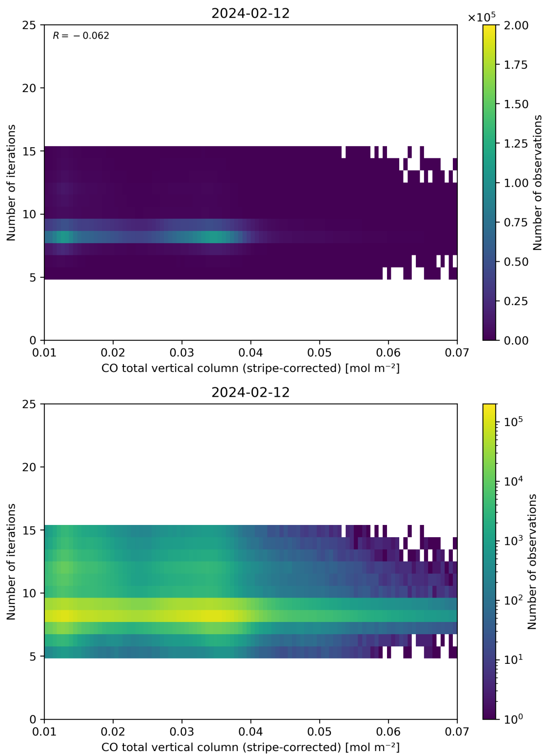
Figure 39: Scatter density plot of “CO total vertical column (stripe-corrected)” against “Number of iterations” for 2024-02-11 to 2024-02-13.
