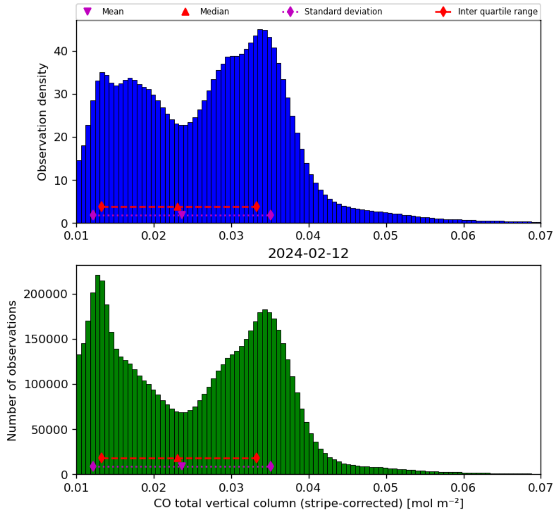
Figure 19: Histogram of “CO total vertical column (stripe-corrected)” for 2024-02-11 to 2024-02-13
