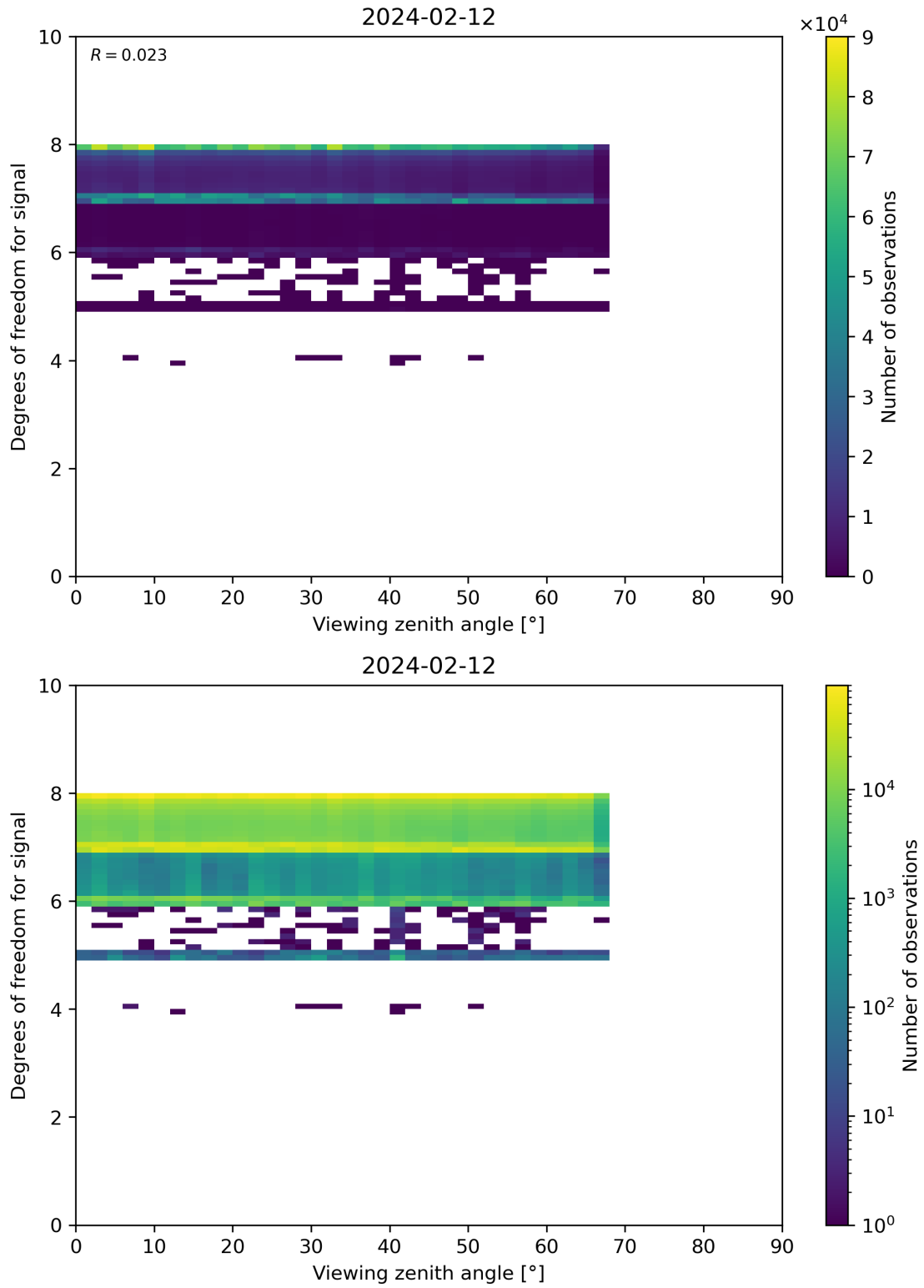
Figure 73: Scatter density plot of “Viewing zenith angle” against “Degrees of freedom for signal” for 2024-02-11 to 2024-02-13.
