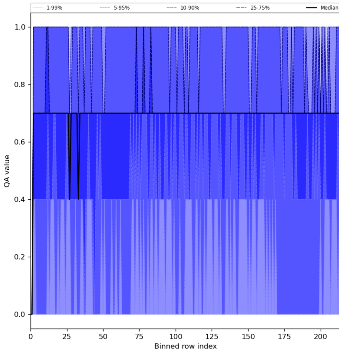
Figure 25: Along track statistics of “QA value” for 2024-02-11 to 2024-02-13
