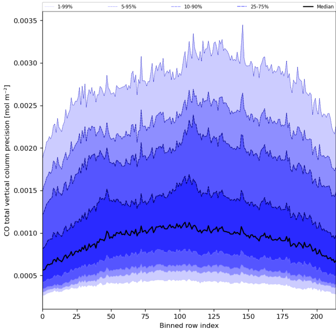
Figure 28: Along track statistics of “CO total vertical column precision” for 2024-02-11 to 2024-02-13
