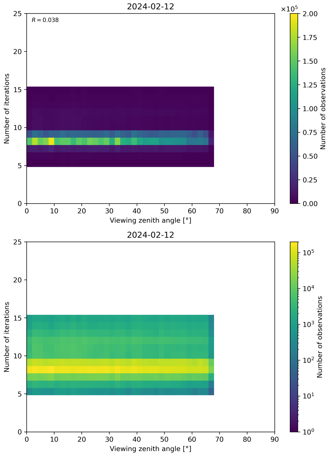
Figure 75: Scatter density plot of “Viewing zenith angle” against “Number of iterations” for 2024-02-11 to 2024-02-13.
