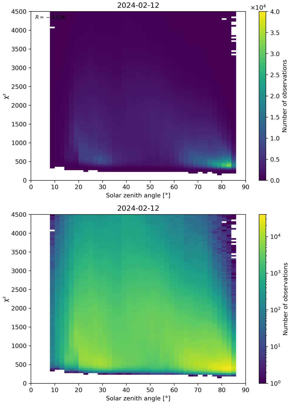
Figure 64: Scatter density plot of “Solar zenith angle” against “ \chi^2 ” for 2024-02-11 to 2024-02-13.
