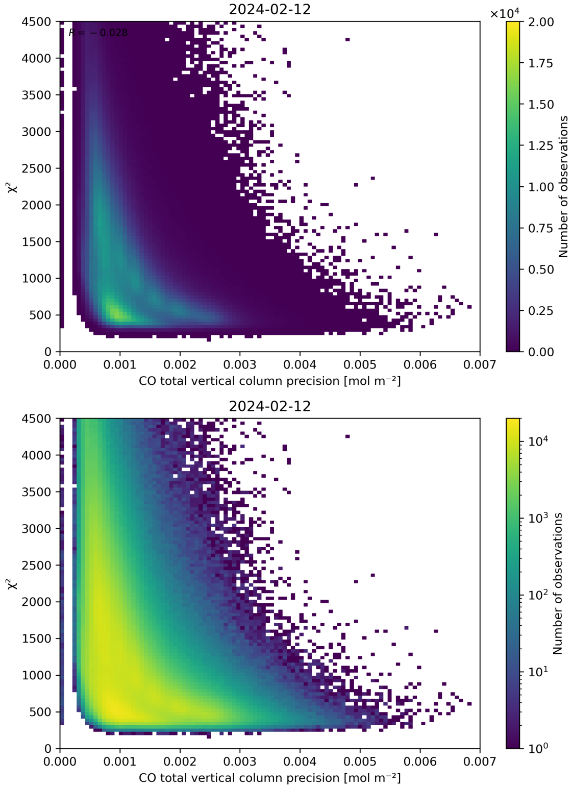
Figure 44: Scatter density plot of “CO total vertical column precision” against “ \chi^2 ” for 2024-02-11 to 2024-02-13.
