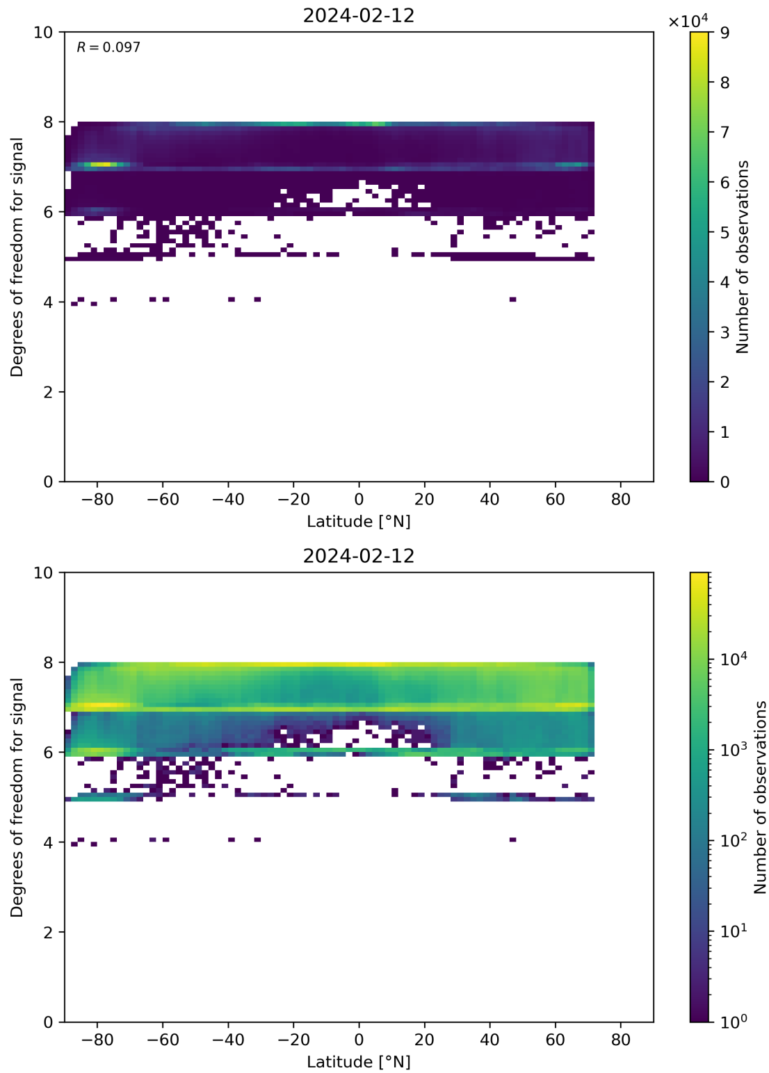
Figure 55: Scatter density plot of “Latitude” against “Degrees of freedom for signal” for 2024-02-11 to 2024-02-13.
