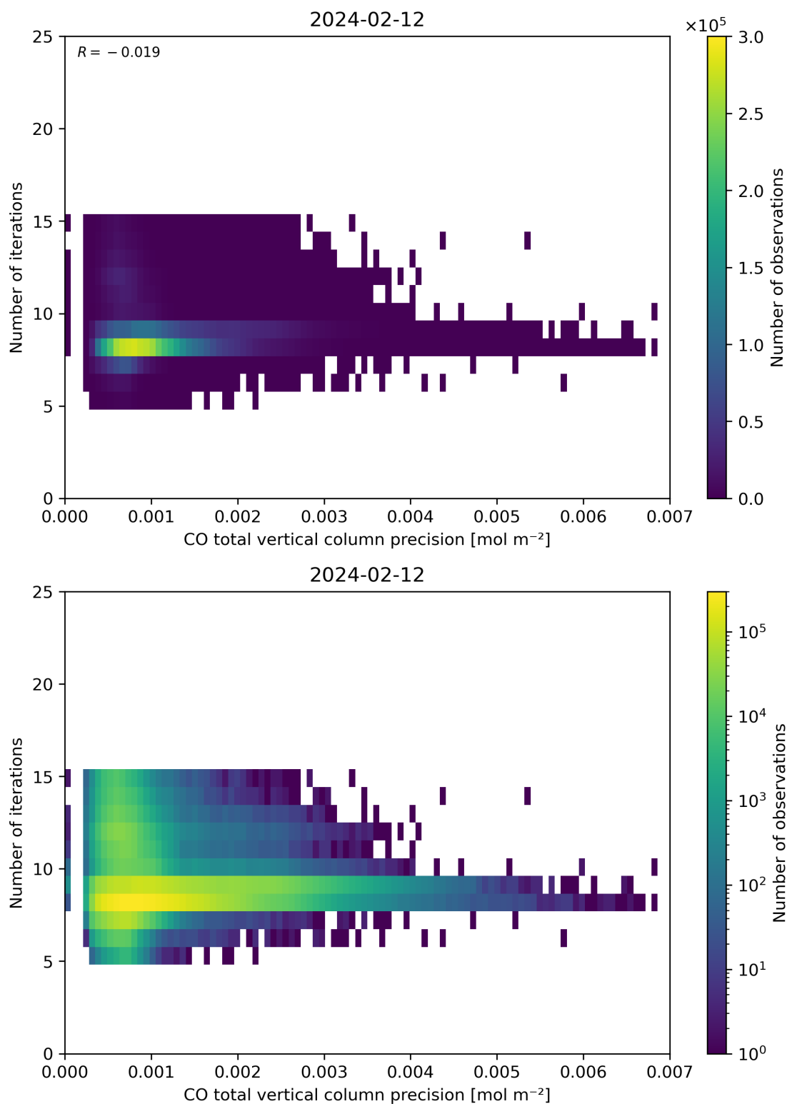
Figure 46: Scatter density plot of “CO total vertical column precision” against “Number of iterations” for 2024-02-11 to 2024-02-13.
