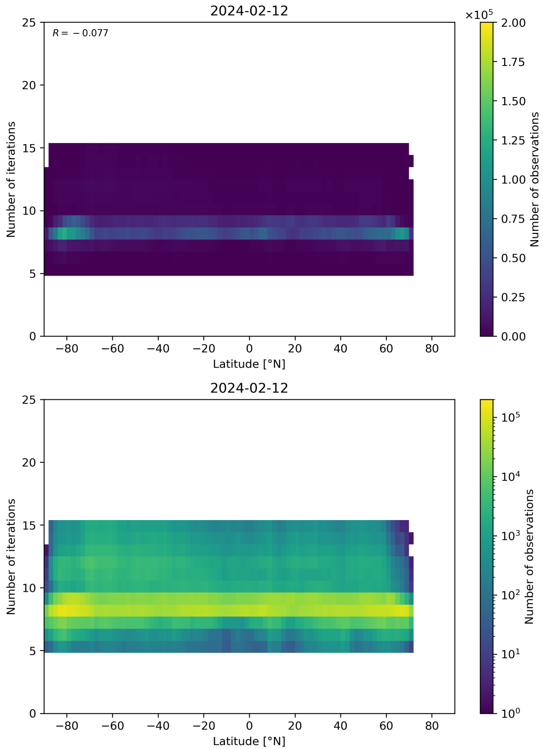
Figure 56: Scatter density plot of “Latitude” against “Number of iterations” for 2024-02-11 to 2024-02-13.
