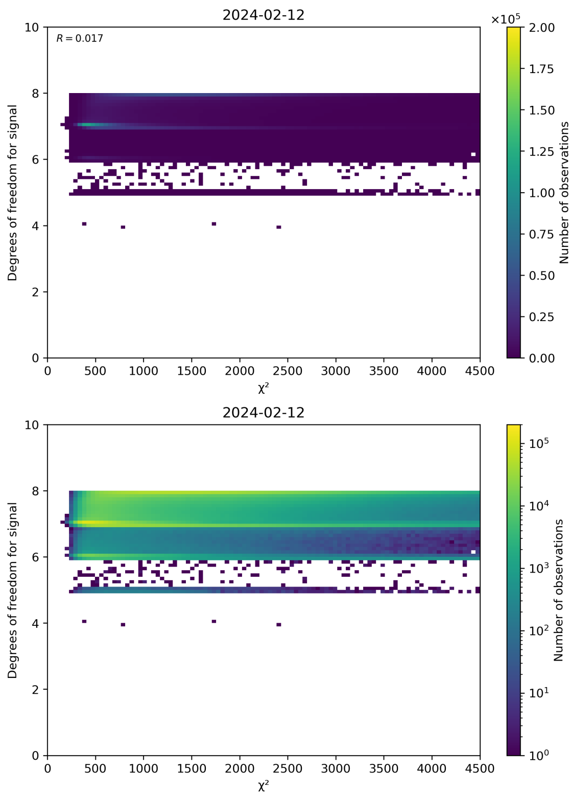
Figure 48: Scatter density plot of “ \chi^2 ” against “Degrees of freedom for signal” for 2024-02-11 to 2024-02-13.
