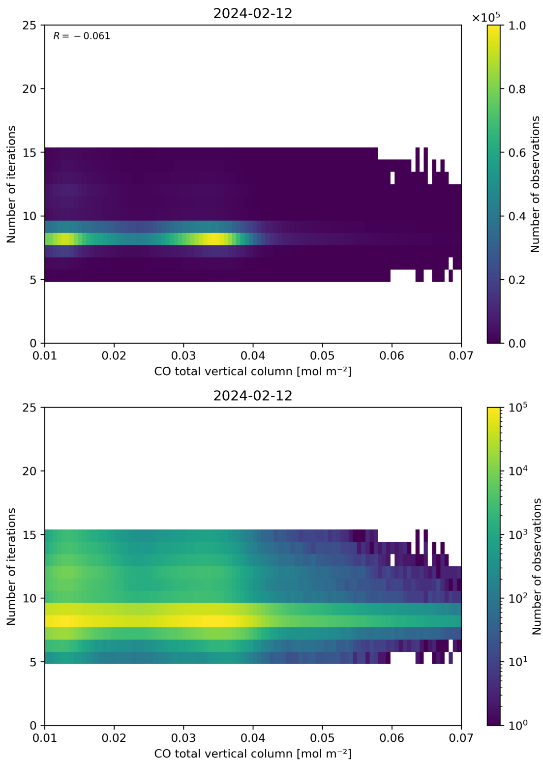
Figure 42: Scatter density plot of “CO total vertical column” against “Number of iterations” for 2024-02-11 to 2024-02-13.
