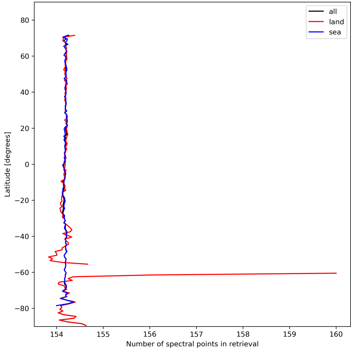
Figure 13: Zonal average of “Number of spectral points in retrieval” for 2024-02-11 to 2024-02-13.
