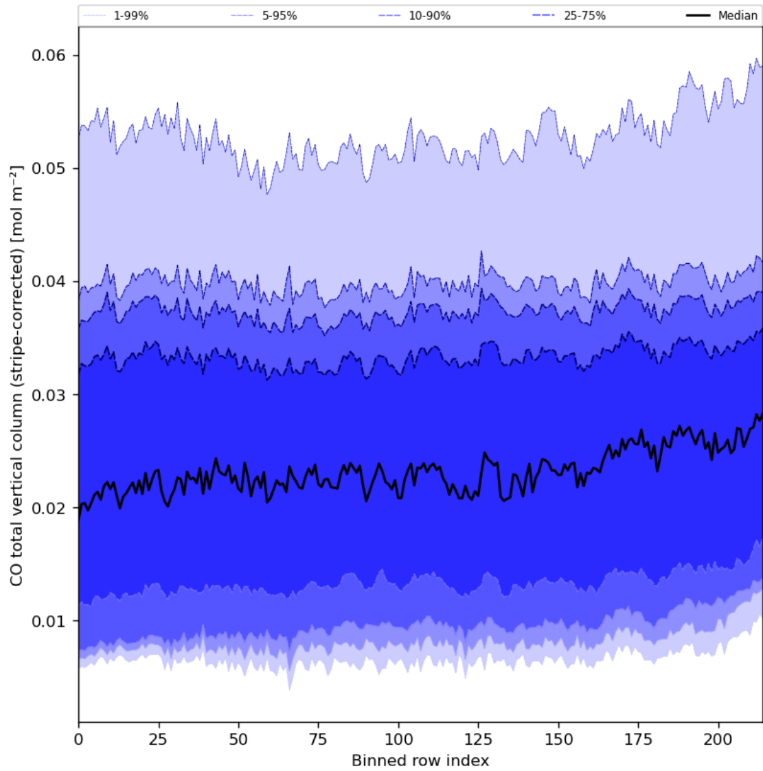
Figure 27: Along track statistics of “CO total vertical column (stripe-corrected)” for 2024-02-11 to 2024-02-13
