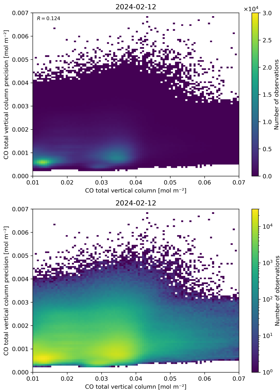
Figure 34: Scatter density plot of “CO total vertical column” against “CO total vertical column precision” for 2024-02-11 to 2024-02-13.
