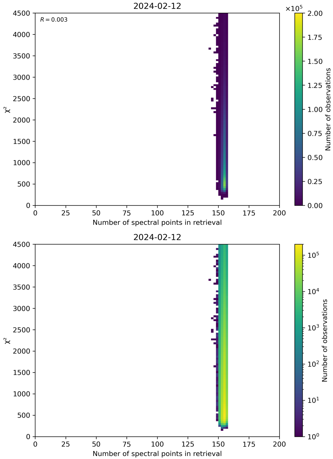
Figure 58: Scatter density plot of “Number of spectral points in retrieval” against “ \chi^2 ” for 2024-02-11 to 2024-02-13.
