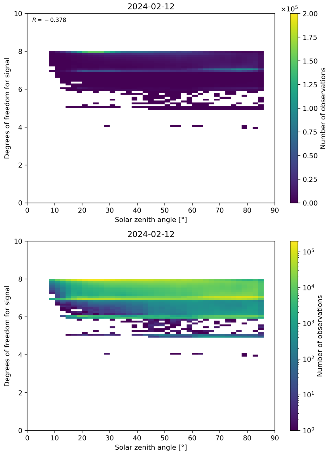
Figure 65: Scatter density plot of “Solar zenith angle” against “Degrees of freedom for signal” for 2024-02-11 to 2024-02-13.
