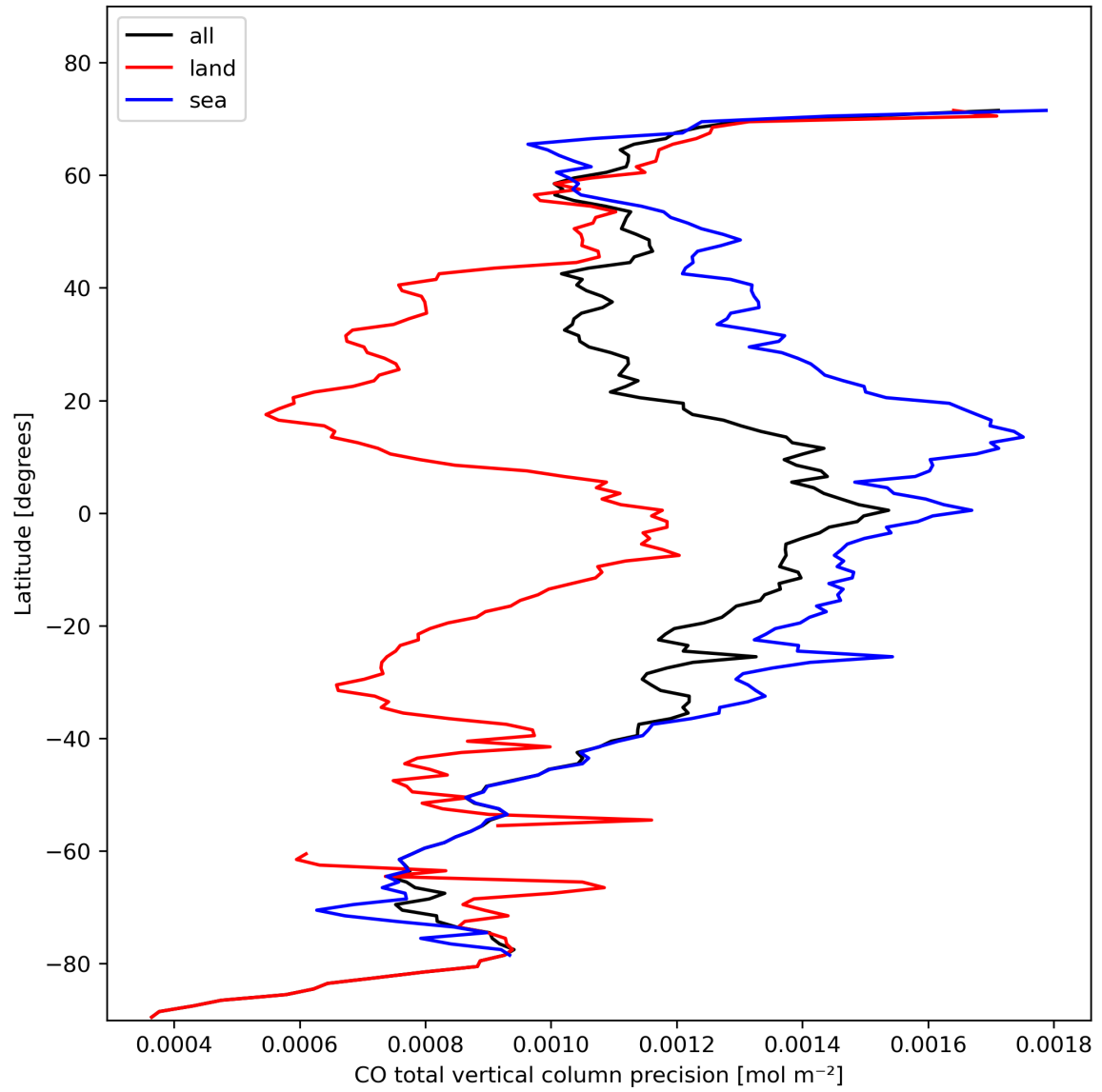
Figure 12: Zonal average of “CO total vertical column precision” for 2024-02-11 to 2024-02-13.
