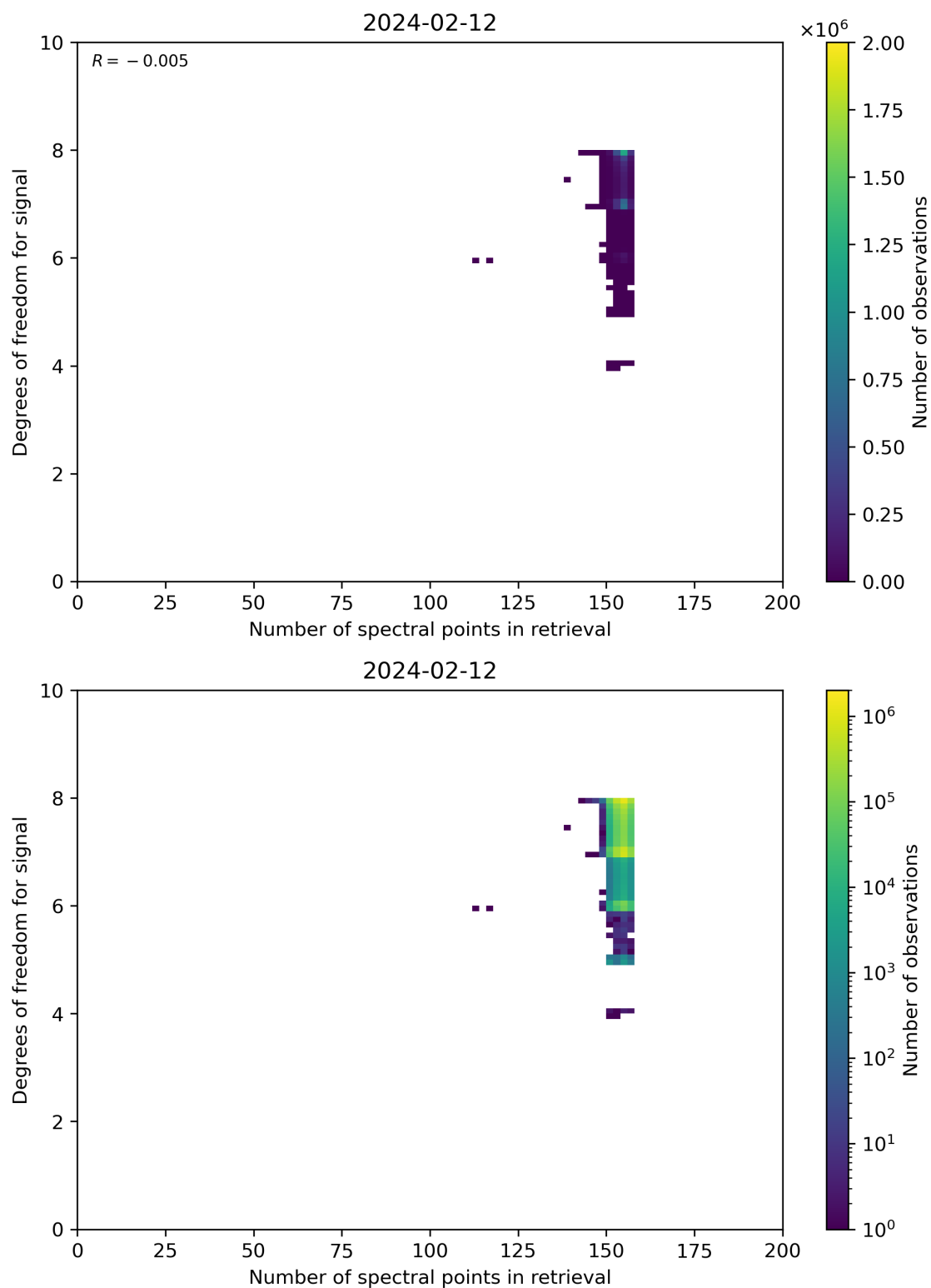
Figure 59: Scatter density plot of “Number of spectral points in retrieval” against “Degrees of freedom for signal” for 2024-02-11 to 2024-02-13.
