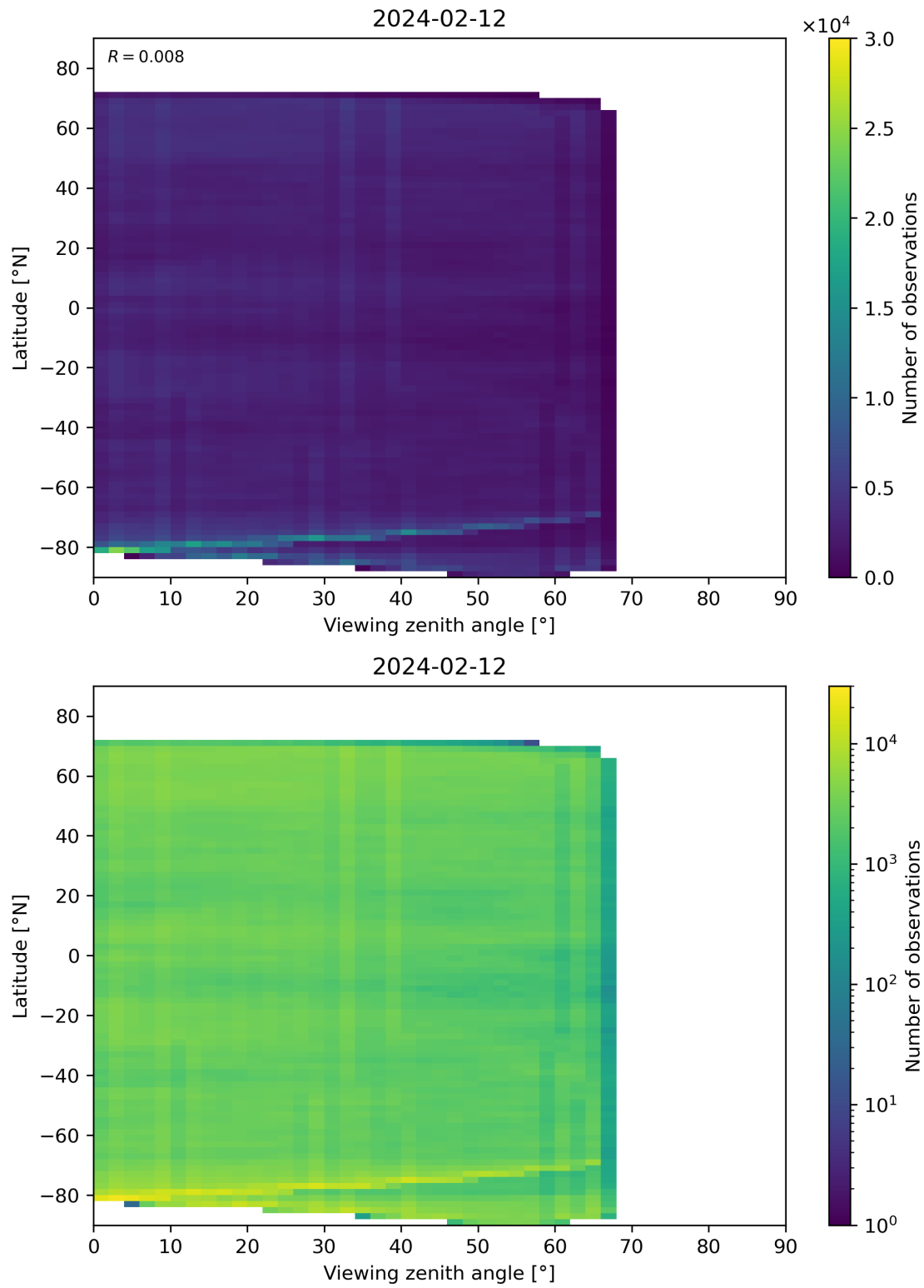
Figure 74: Scatter density plot of “Viewing zenith angle” against “Latitude” for 2024-02-11 to 2024-02-13.
