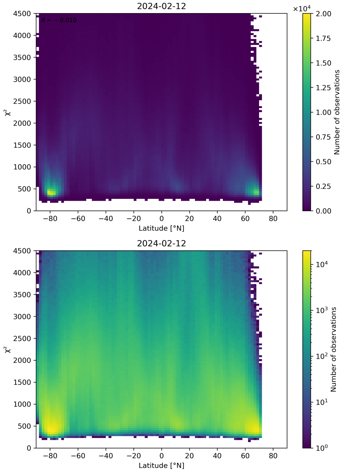
Figure 54: Scatter density plot of “Latitude” against “ \chi^2 ” for 2024-02-11 to 2024-02-13.
