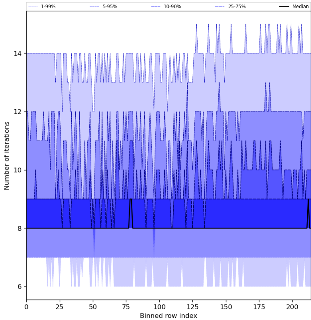
Figure 32: Along track statistics of “Number of iterations” for 2024-02-11 to 2024-02-13
