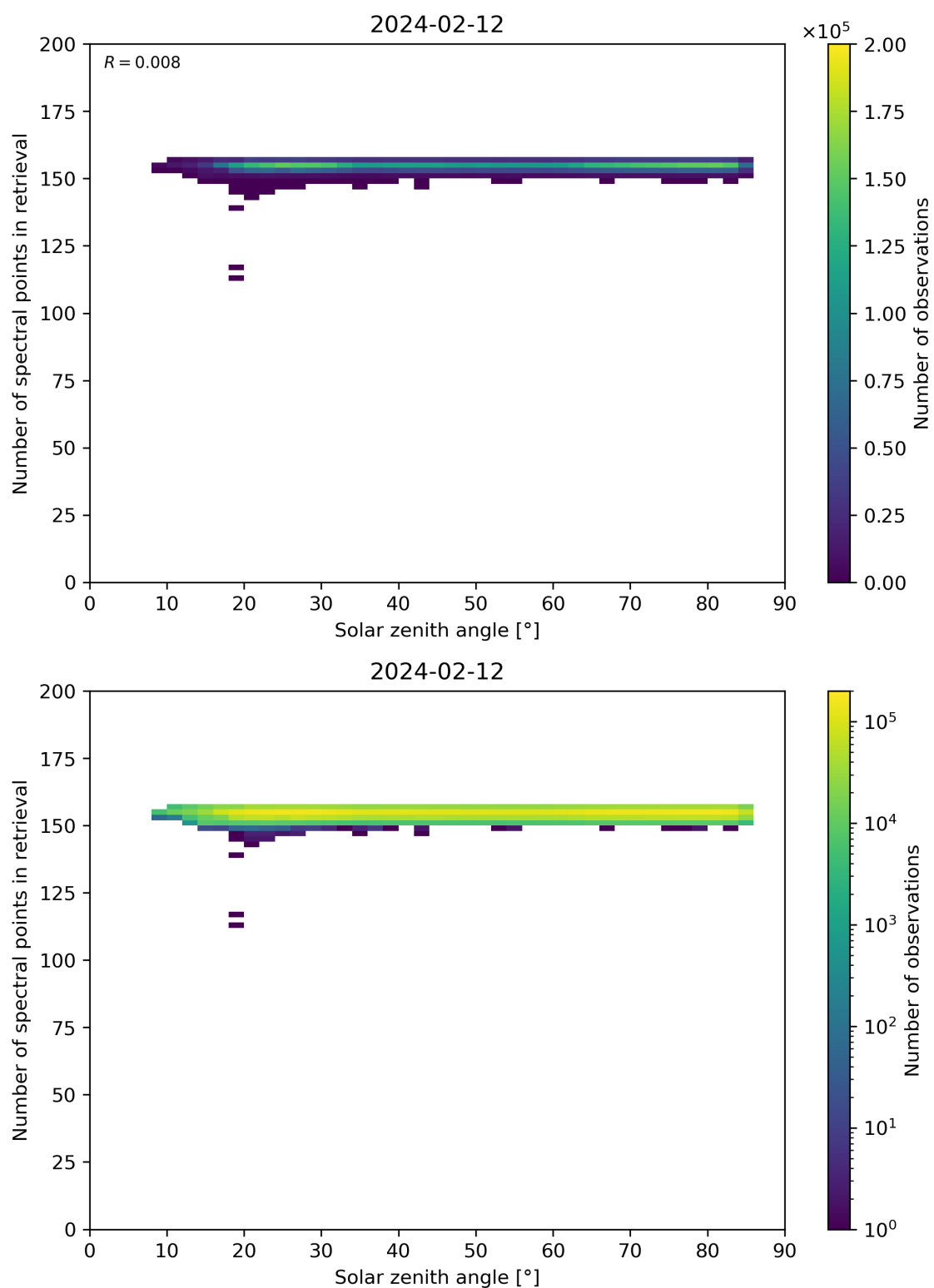
Figure 68: Scatter density plot of “Solar zenith angle” against “Number of spectral points in retrieval” for 2024-02-11 to 2024-02-13.
