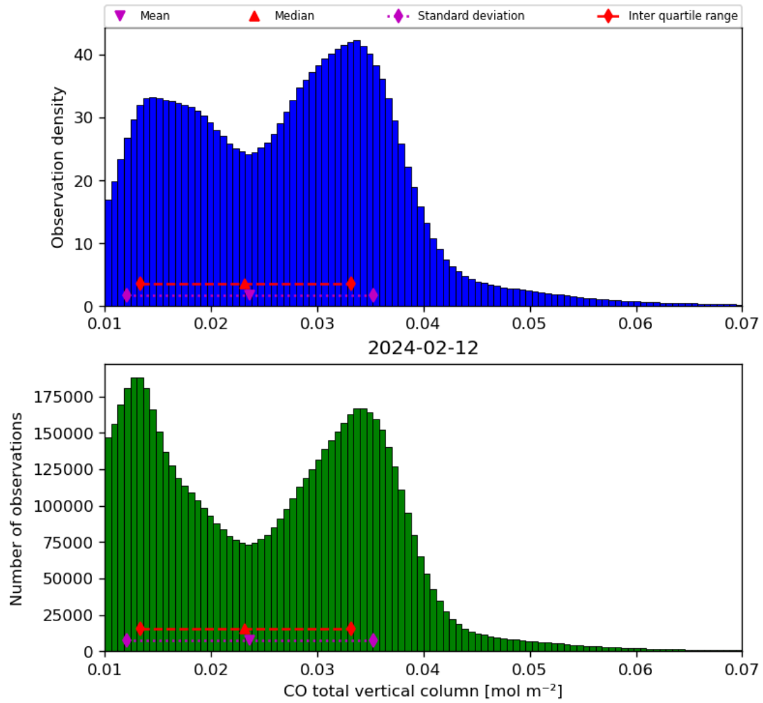
Figure 18: Histogram of “CO total vertical column” for 2024-02-11 to 2024-02-13
