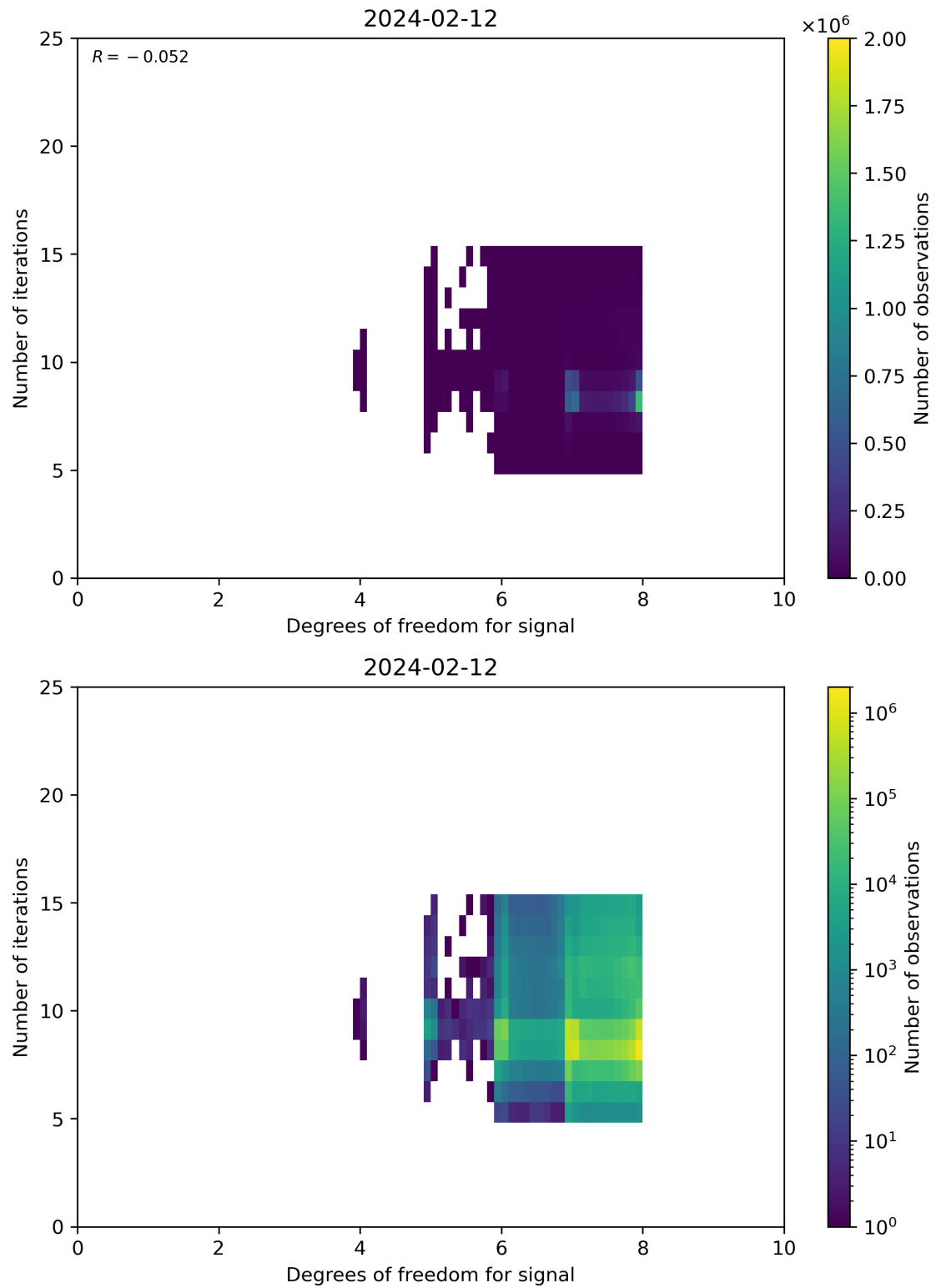
Figure 50: Scatter density plot of “Degrees of freedom for signal” against “Number of iterations” for 2024-02-11 to 2024-02-13.
