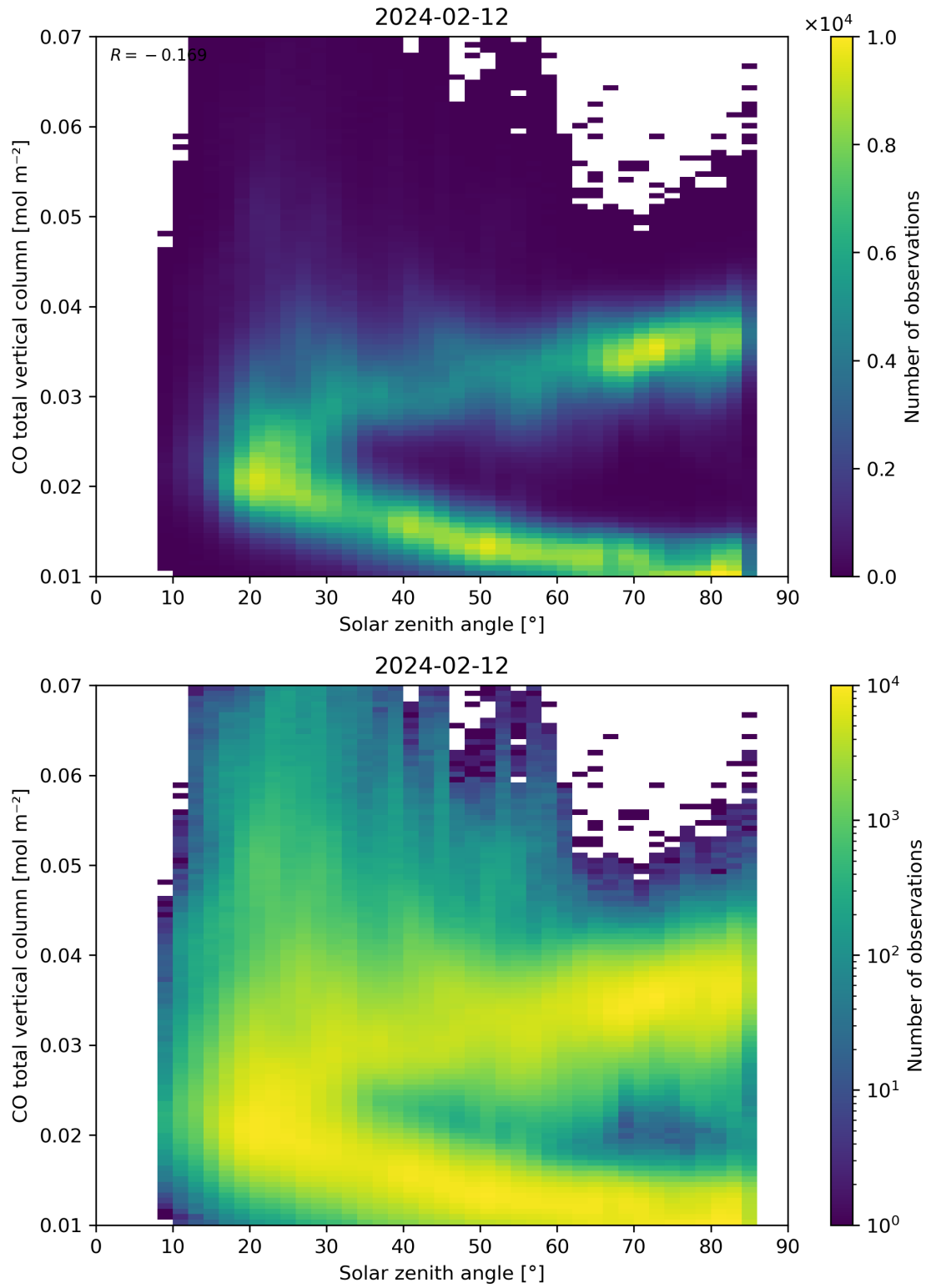
Figure 61: Scatter density plot of “Solar zenith angle” against “CO total vertical column” for 2024-02-11 to 2024-02-13.
