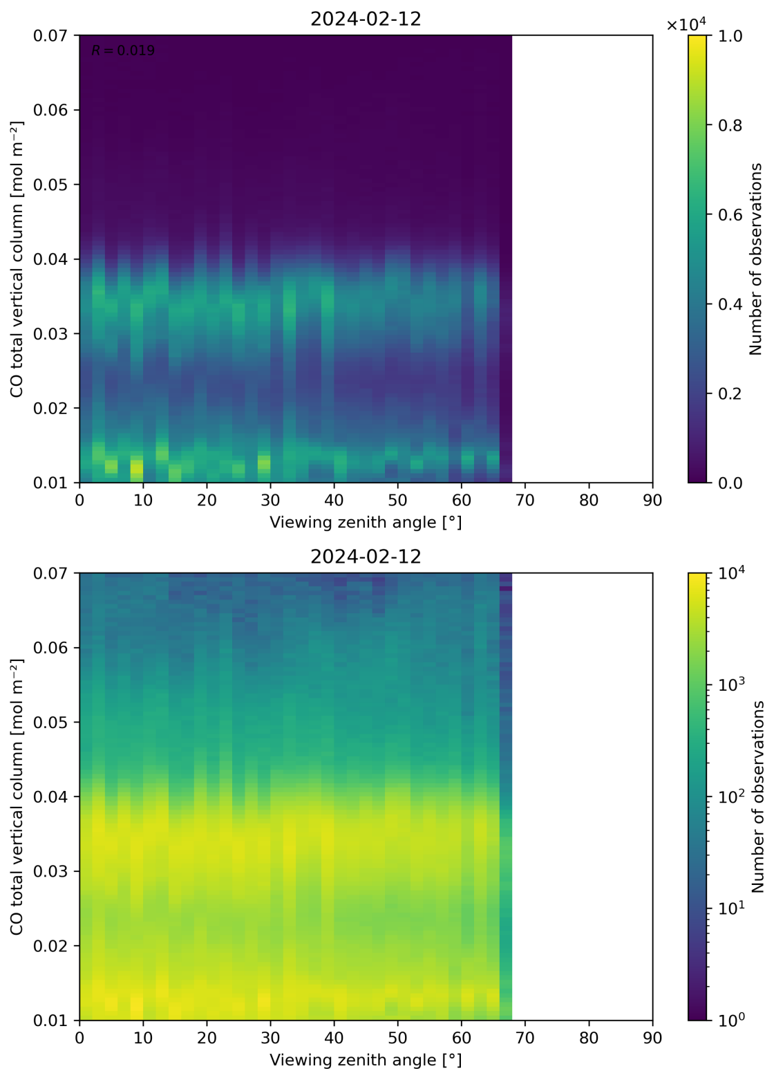
Figure 69: Scatter density plot of “Viewing zenith angle” against “CO total vertical column” for 2024-02-11 to 2024-02-13.
