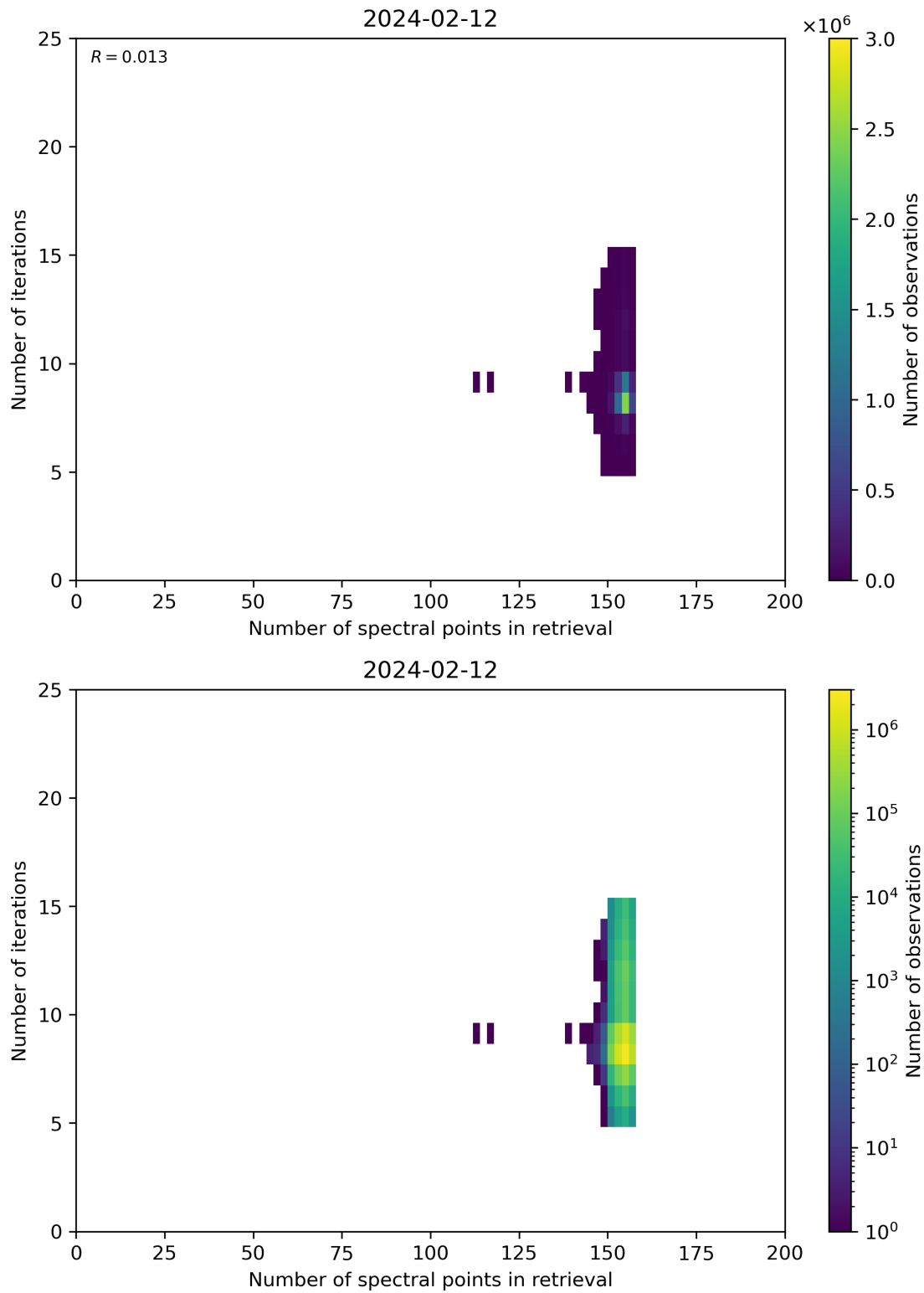
Figure 60: Scatter density plot of “Number of spectral points in retrieval” against “Number of iterations” for 2024-02-11 to 2024-02-13.
