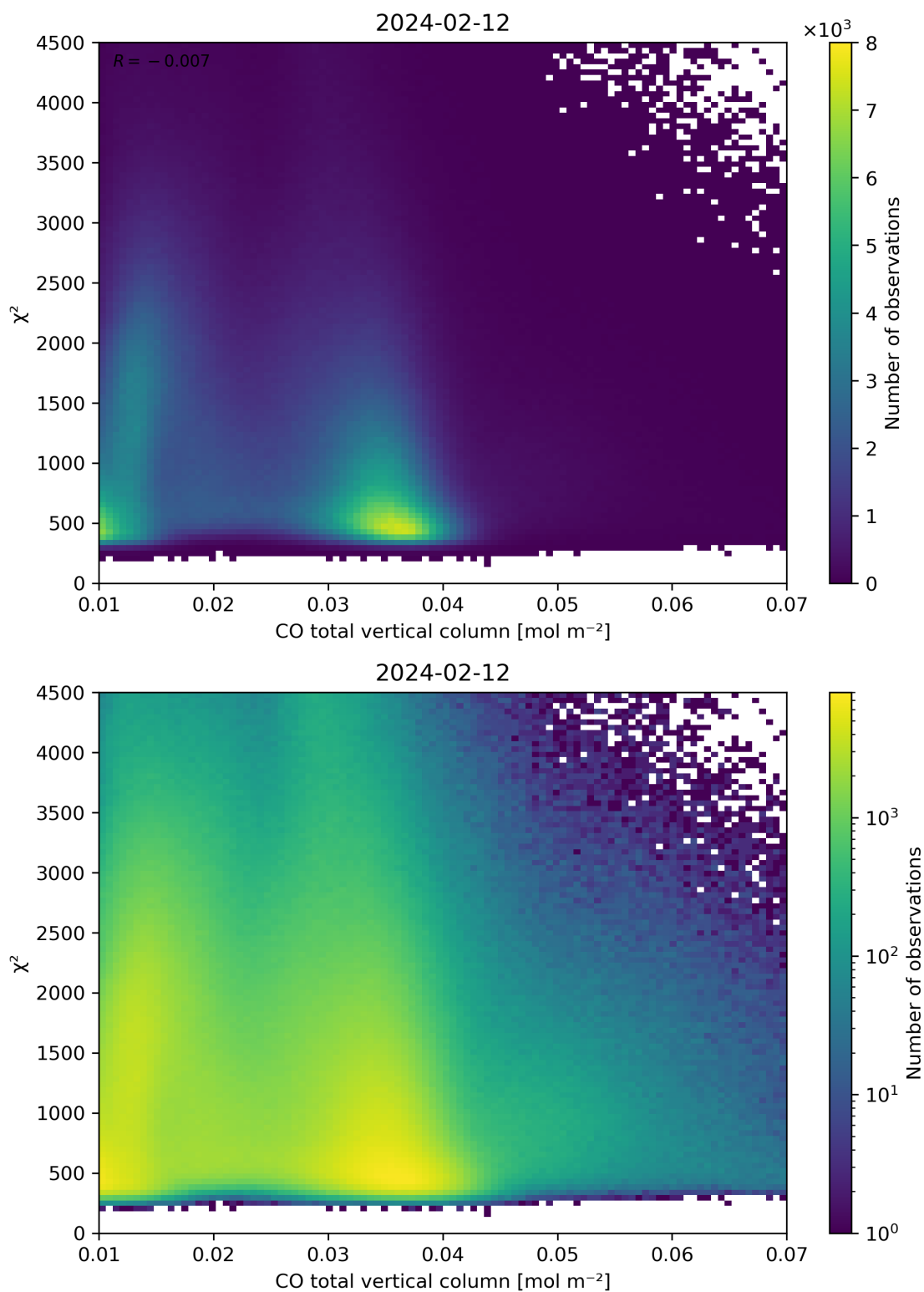
Figure 35: Scatter density plot of “CO total vertical column” against “ \chi^2 ” for 2024-02-11 to 2024-02-13.
