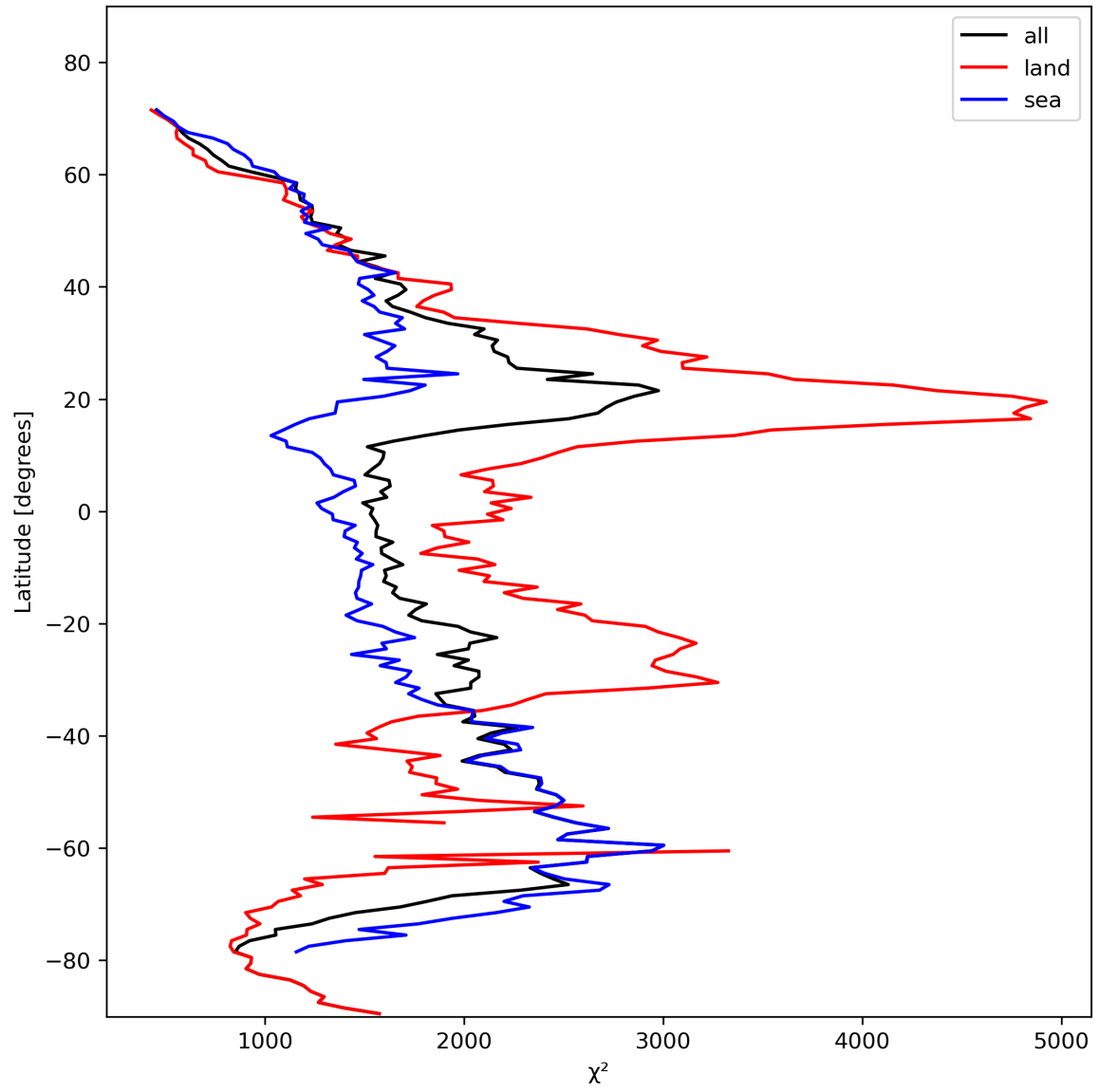
Figure 14: Zonal average of “ \chi^2 ” for 2024-02-11 to 2024-02-13.
