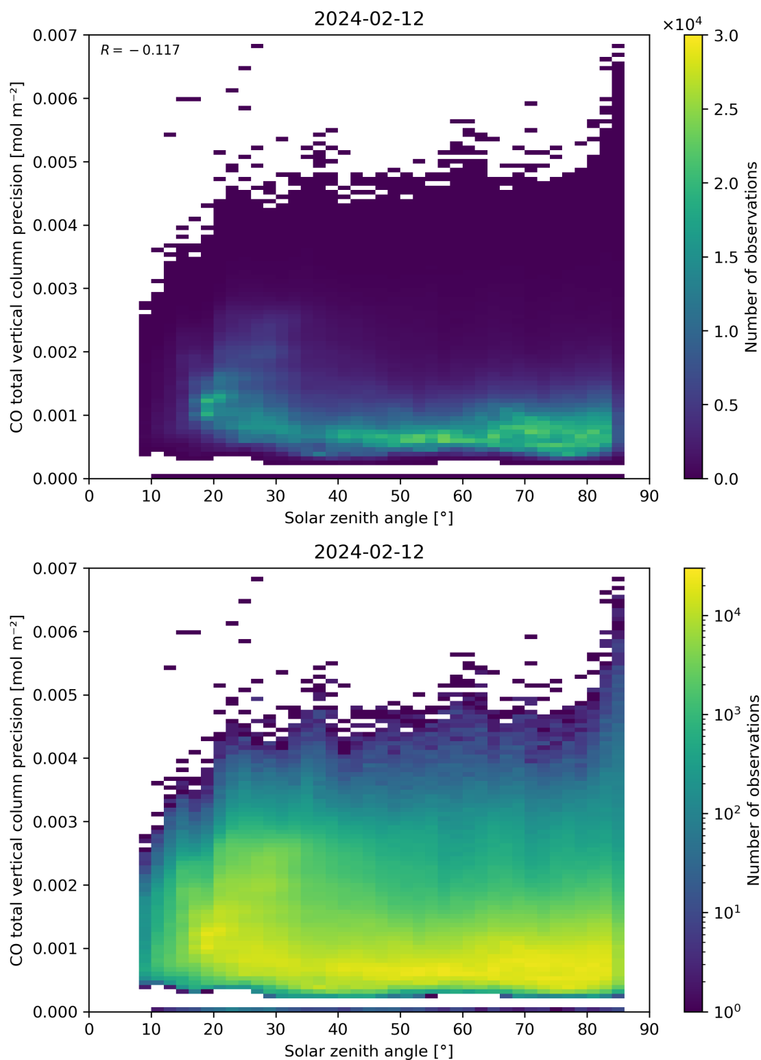
Figure 63: Scatter density plot of “Solar zenith angle” against “CO total vertical column precision” for 2024-02-11 to 2024-02-13.
