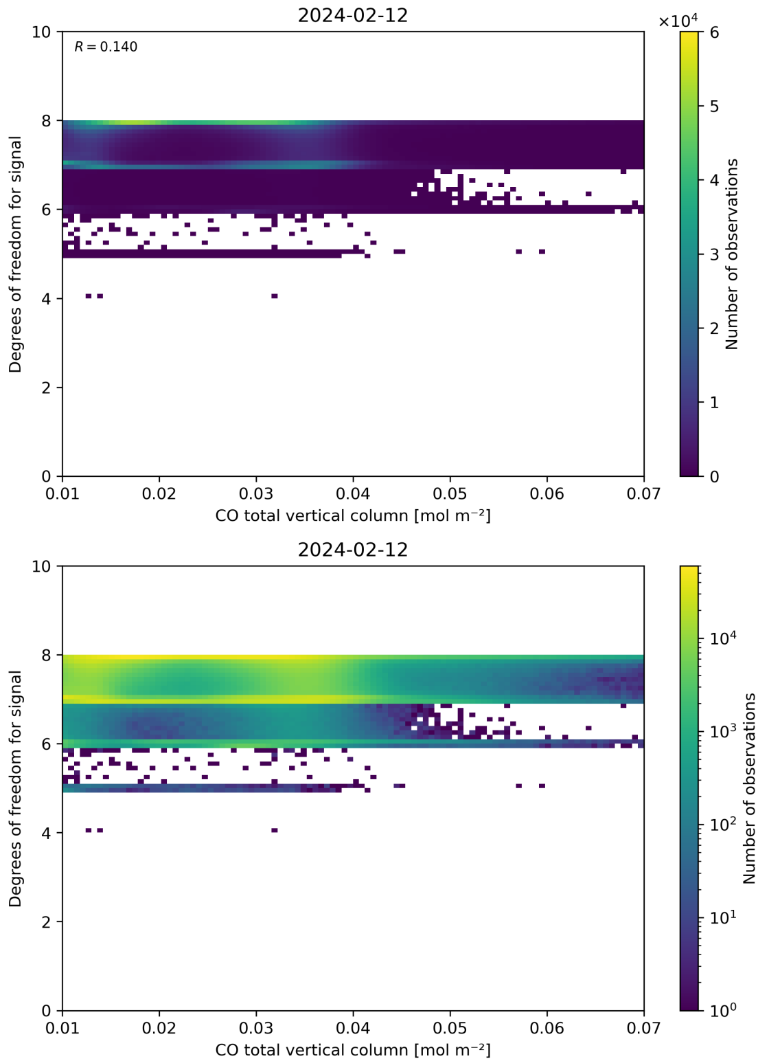
Figure 41: Scatter density plot of “CO total vertical column” against “Degrees of freedom for signal” for 2024-02-11 to 2024-02-13.
