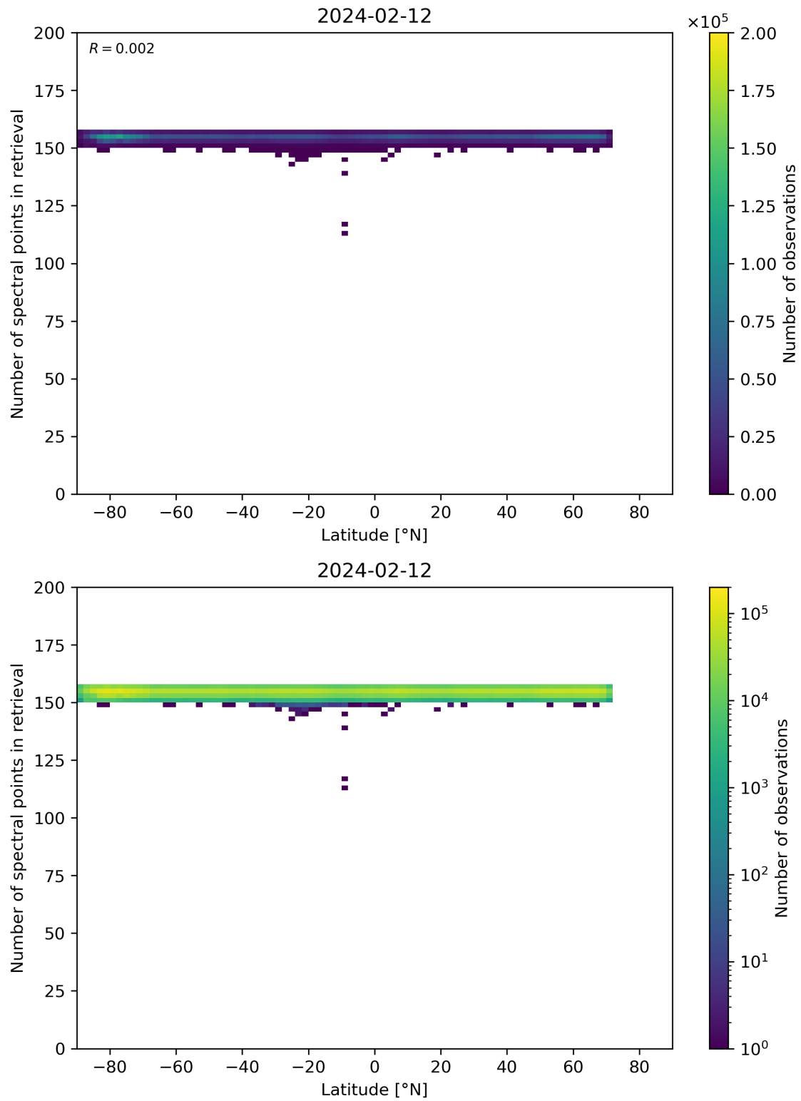
Figure 57: Scatter density plot of “Latitude” against “Number of spectral points in retrieval” for 2024-02-11 to 2024-02-13.
