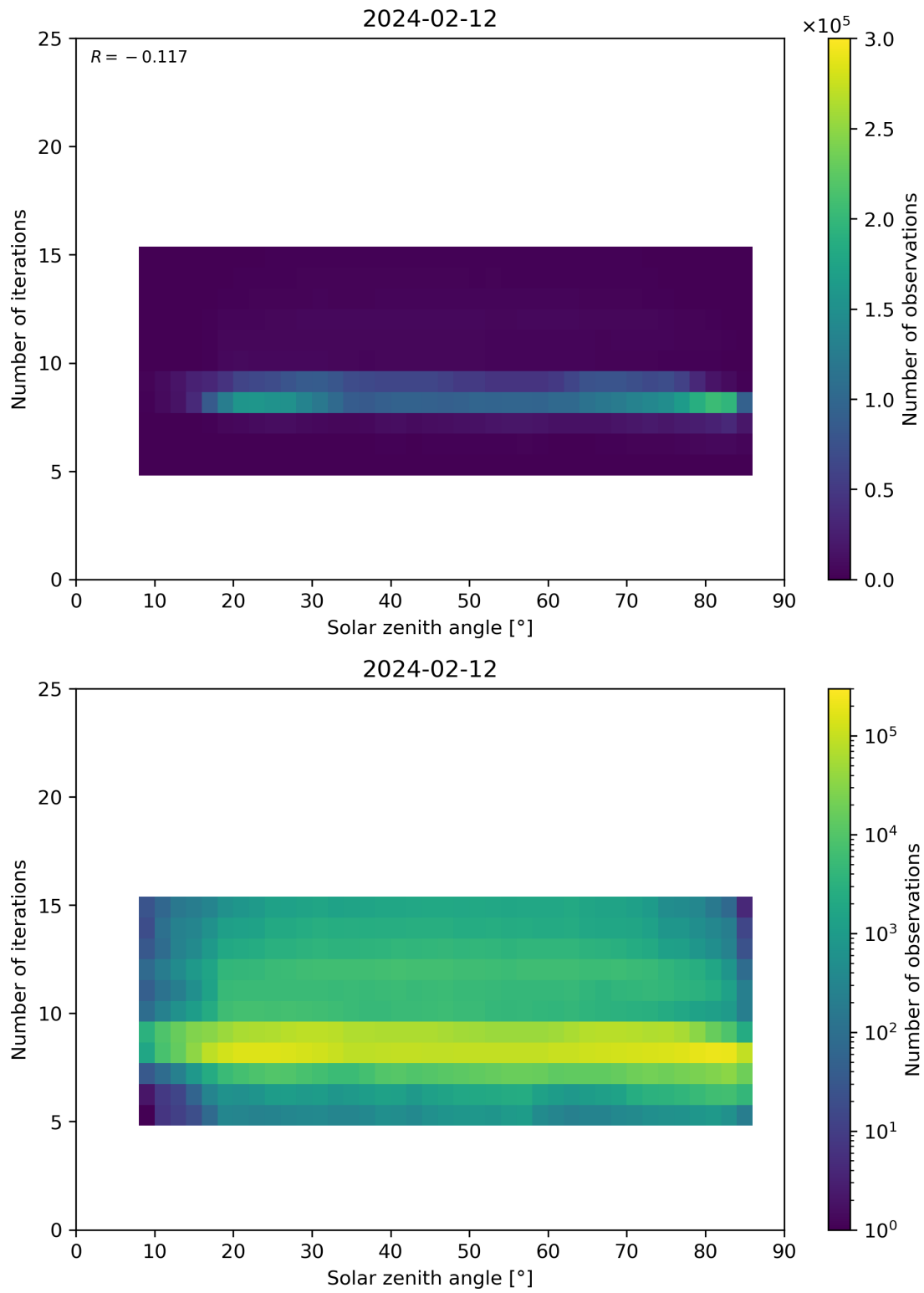
Figure 67: Scatter density plot of “Solar zenith angle” against “Number of iterations” for 2024-02-11 to 2024-02-13.
