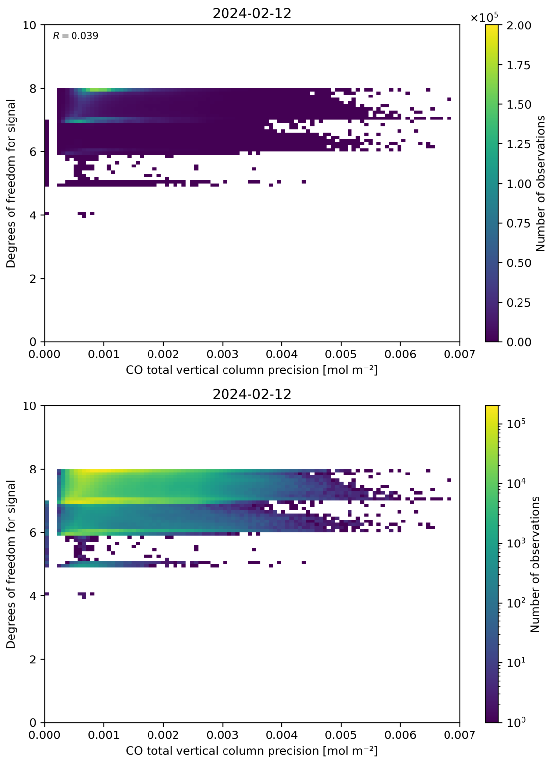
Figure 45: Scatter density plot of “CO total vertical column precision” against “Degrees of freedom for signal” for 2024-02-11 to 2024-02-13.
