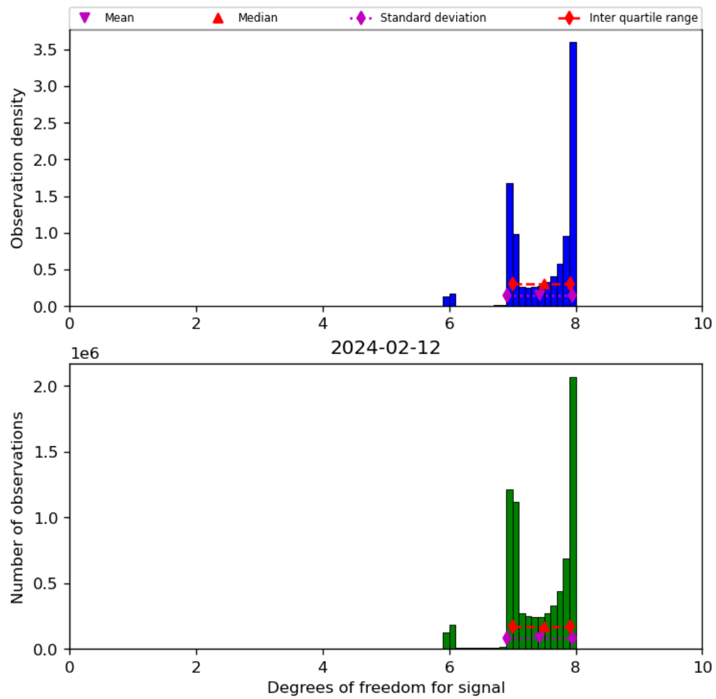
Figure 23: Histogram of “Degrees of freedom for signal” for 2024-02-11 to 2024-02-13
