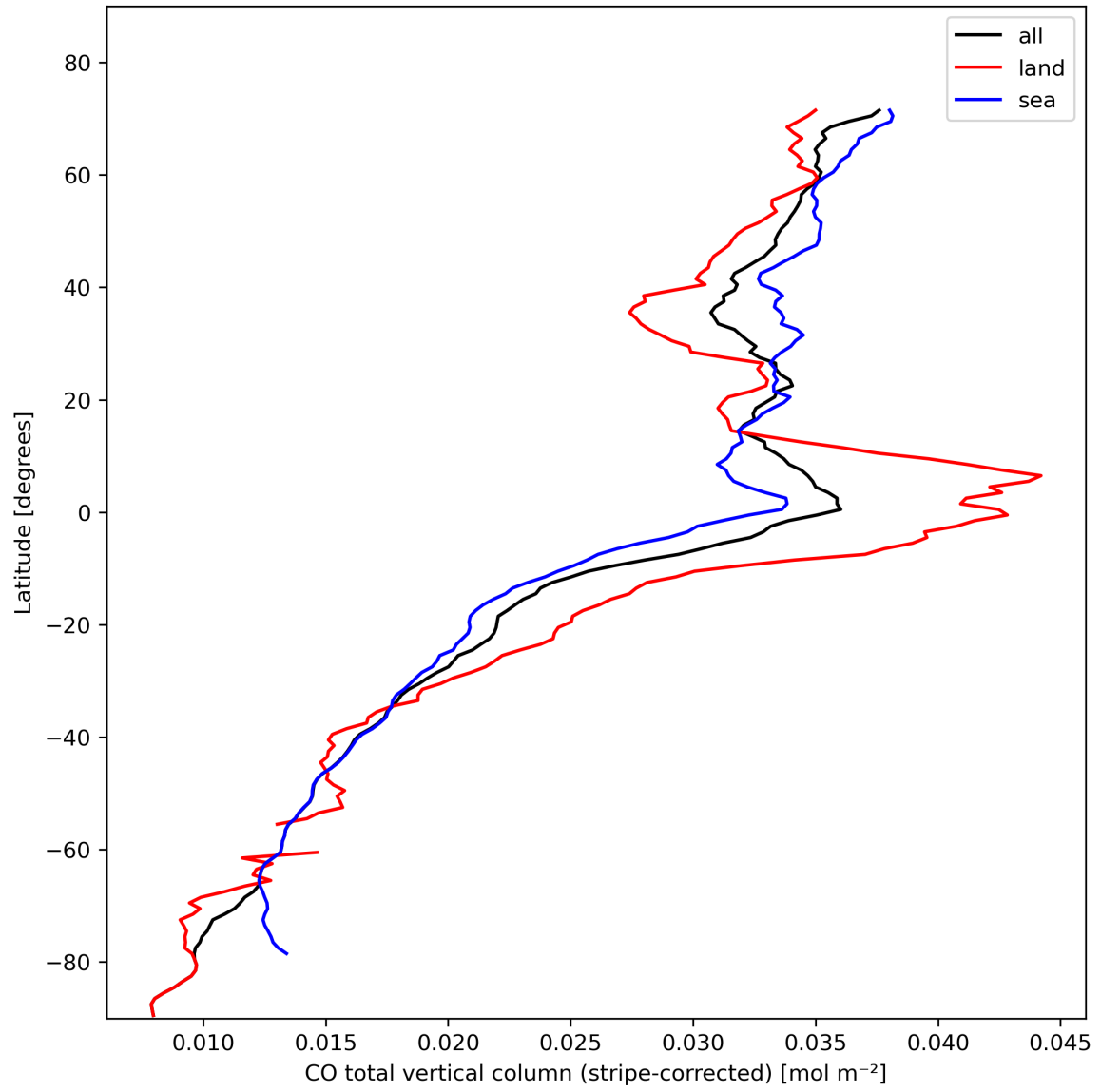
Figure 11: Zonal average of “CO total vertical column (stripe-corrected)” for 2024-02-11 to 2024-02-13.
