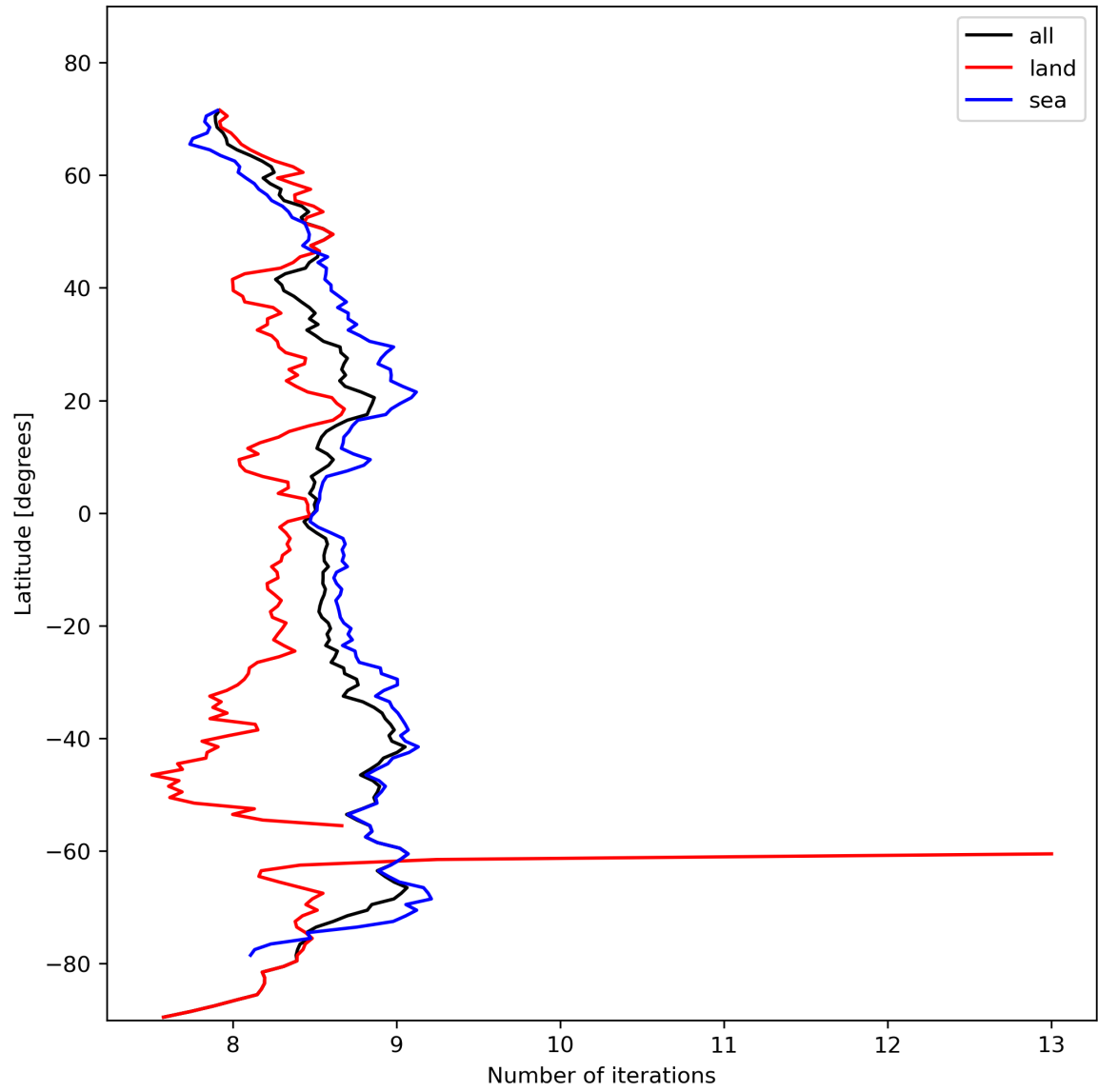
Figure 16: Zonal average of “Number of iterations” for 2024-02-11 to 2024-02-13.
