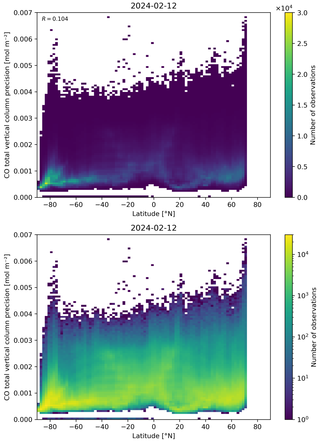
Figure 53: Scatter density plot of “Latitude” against “CO total vertical column precision” for 2024-02-11 to 2024-02-13.
