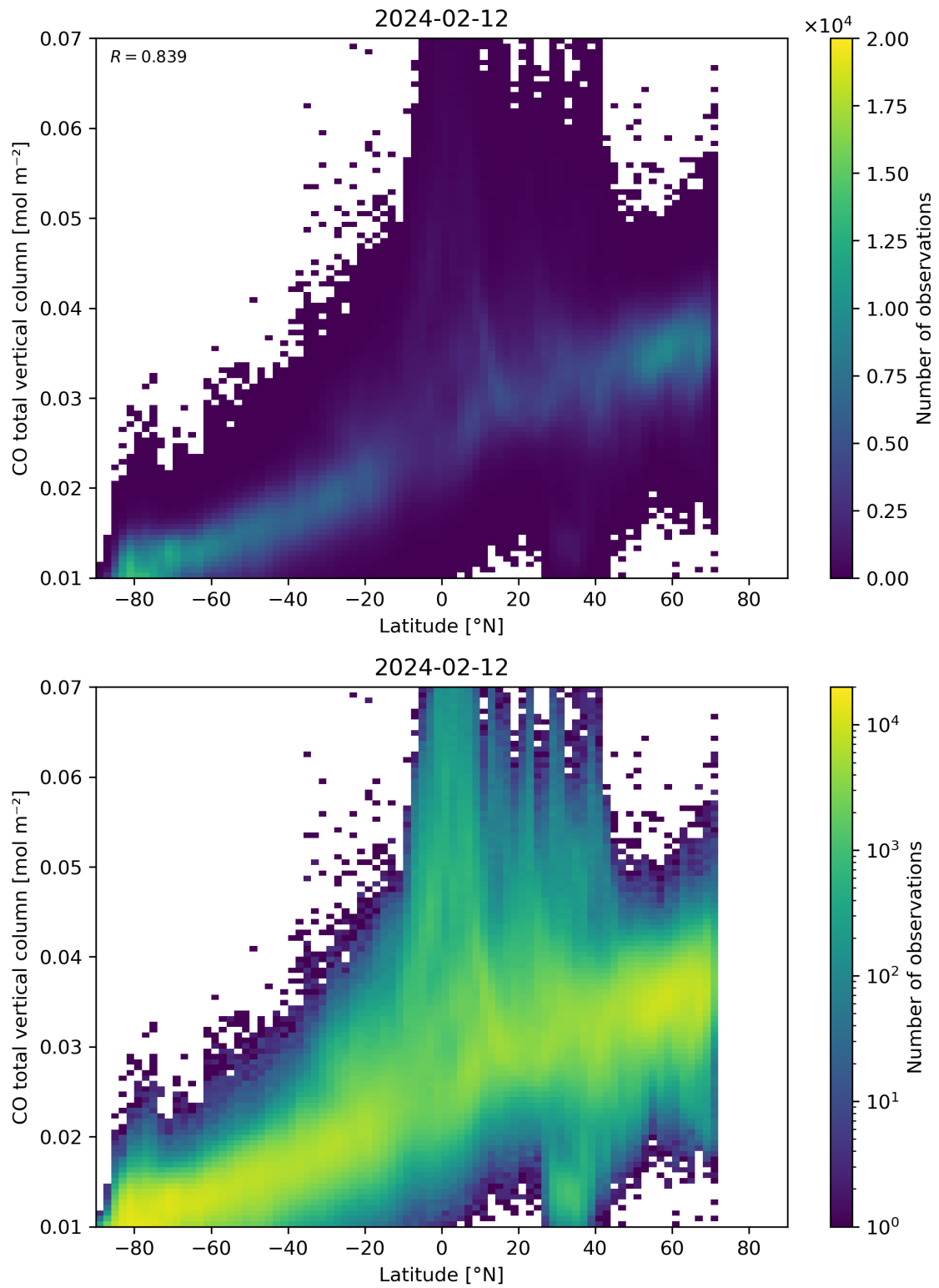
Figure 51: Scatter density plot of “Latitude” against “CO total vertical column” for 2024-02-11 to 2024-02-13.
