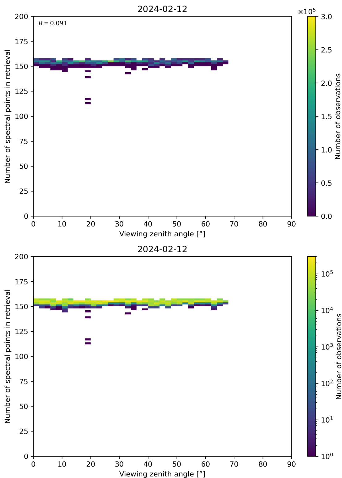
Figure 76: Scatter density plot of “Viewing zenith angle” against “Number of spectral points in retrieval” for 2024-02-11 to 2024-02-13.
