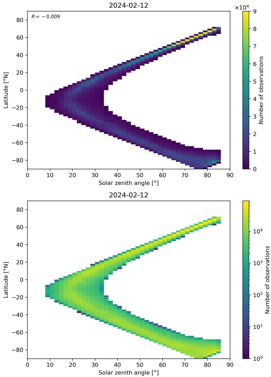
Figure 66: Scatter density plot of “Solar zenith angle” against “Latitude” for 2024-02-11 to 2024-02-13.
