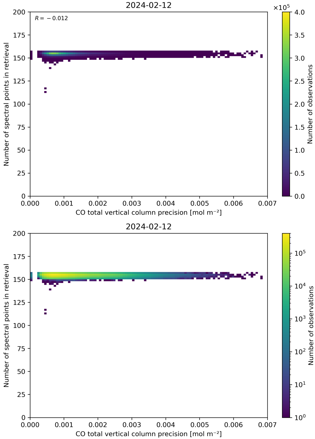
Figure 47: Scatter density plot of “CO total vertical column precision” against “Number of spectral points in retrieval” for 2024-02-11 to 2024-02-13.
