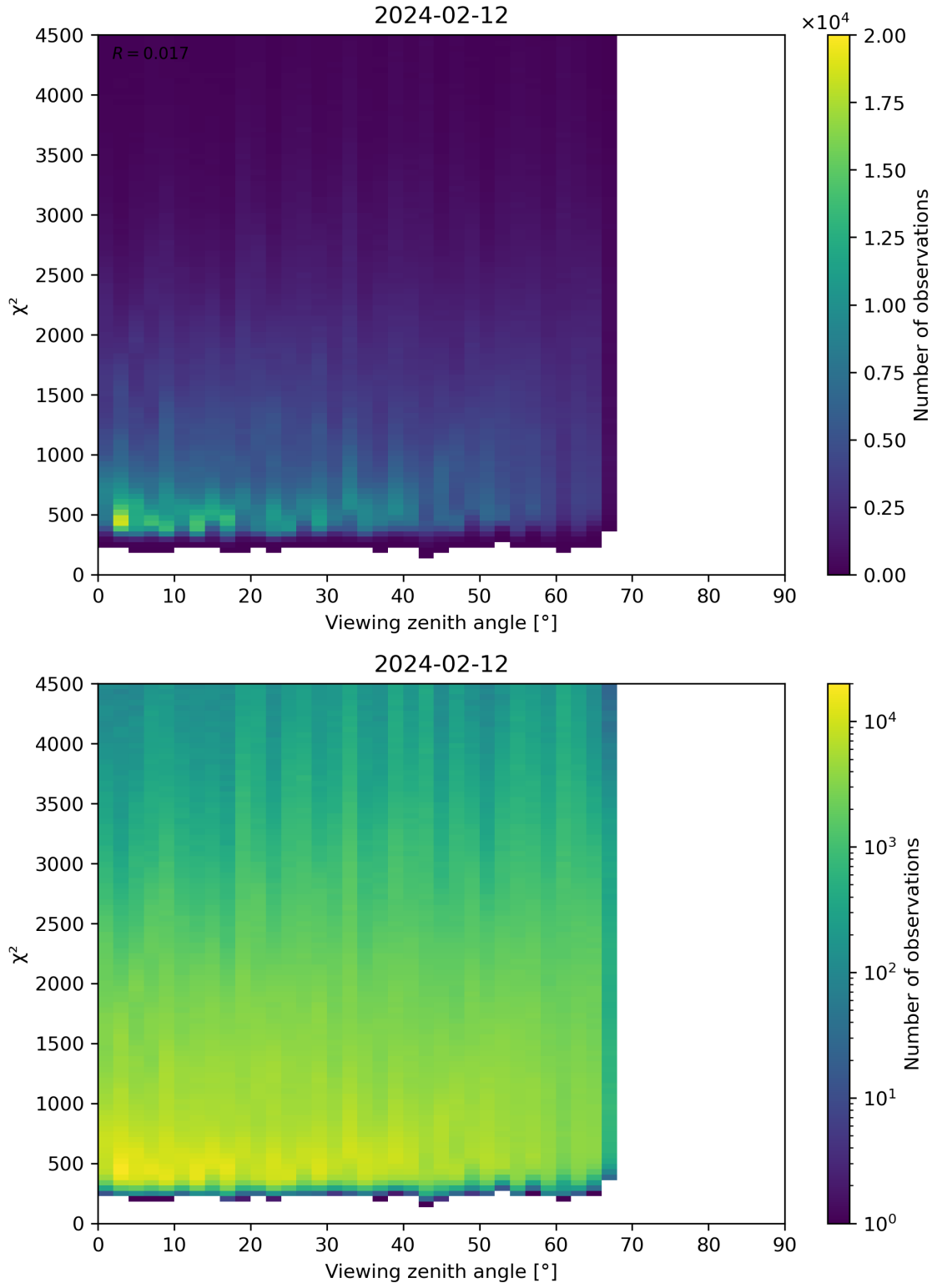
Figure 72: Scatter density plot of “Viewing zenith angle” against “ \chi^2 ” for 2024-02-11 to 2024-02-13.
