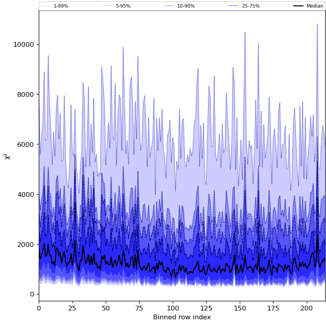
Figure 30: Along track statistics of “ \chi^2 ” for 2024-02-11 to 2024-02-13
