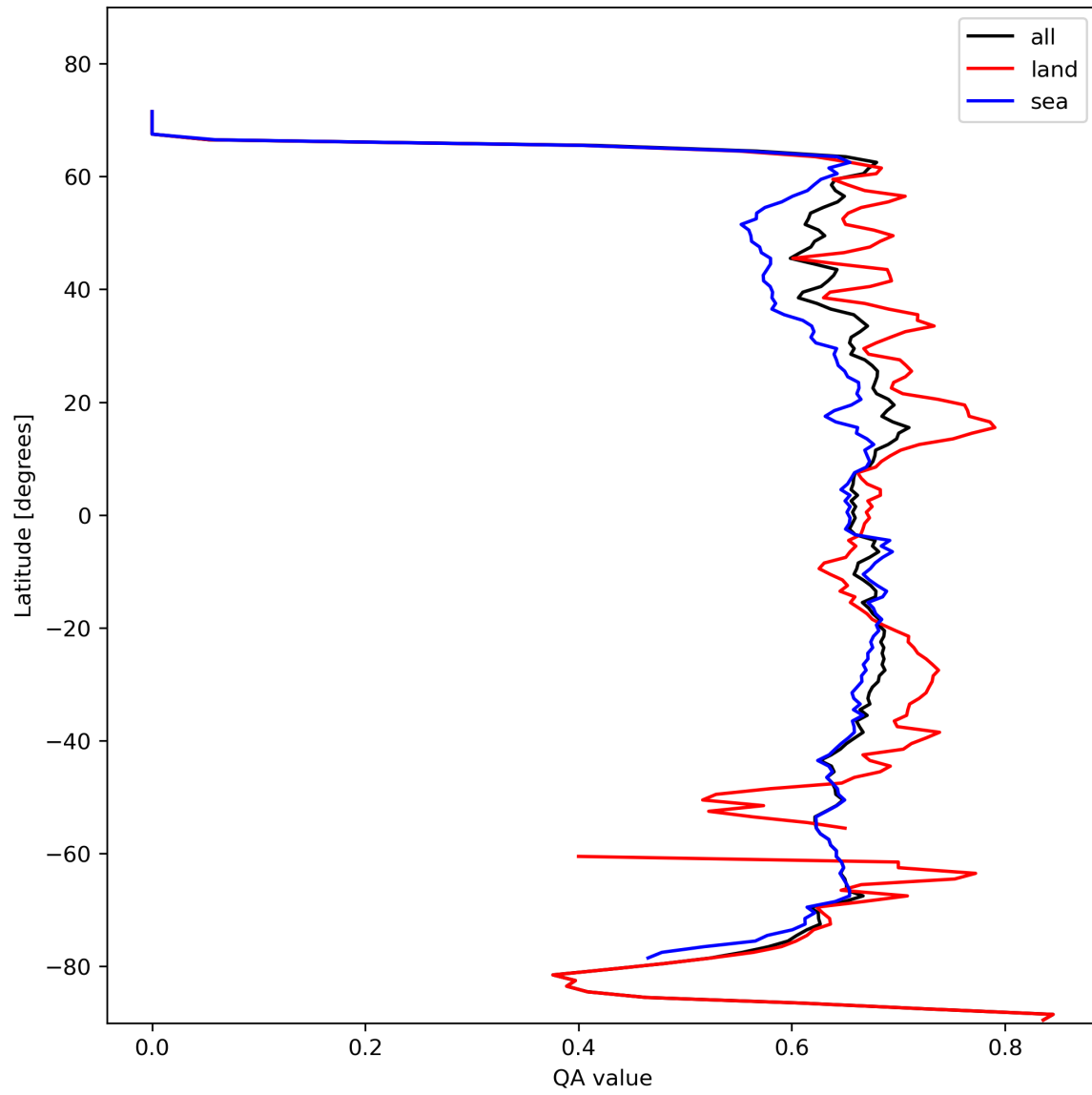
Figure 9: Zonal average of “QA value” for 2024-02-11 to 2024-02-13.
