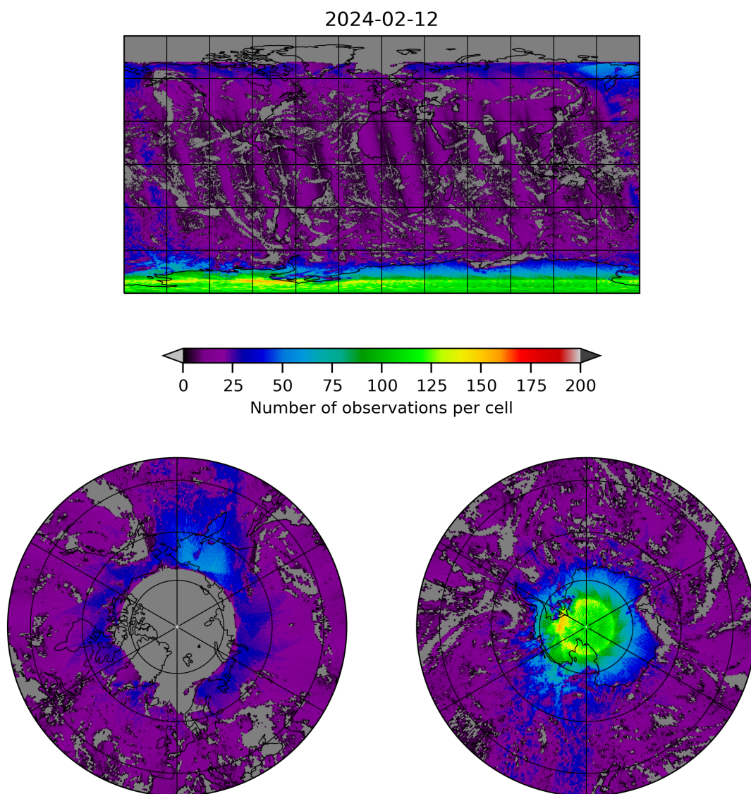
Figure 8: Map of the number of observations for 2024-02-11 to 2024-02-13
