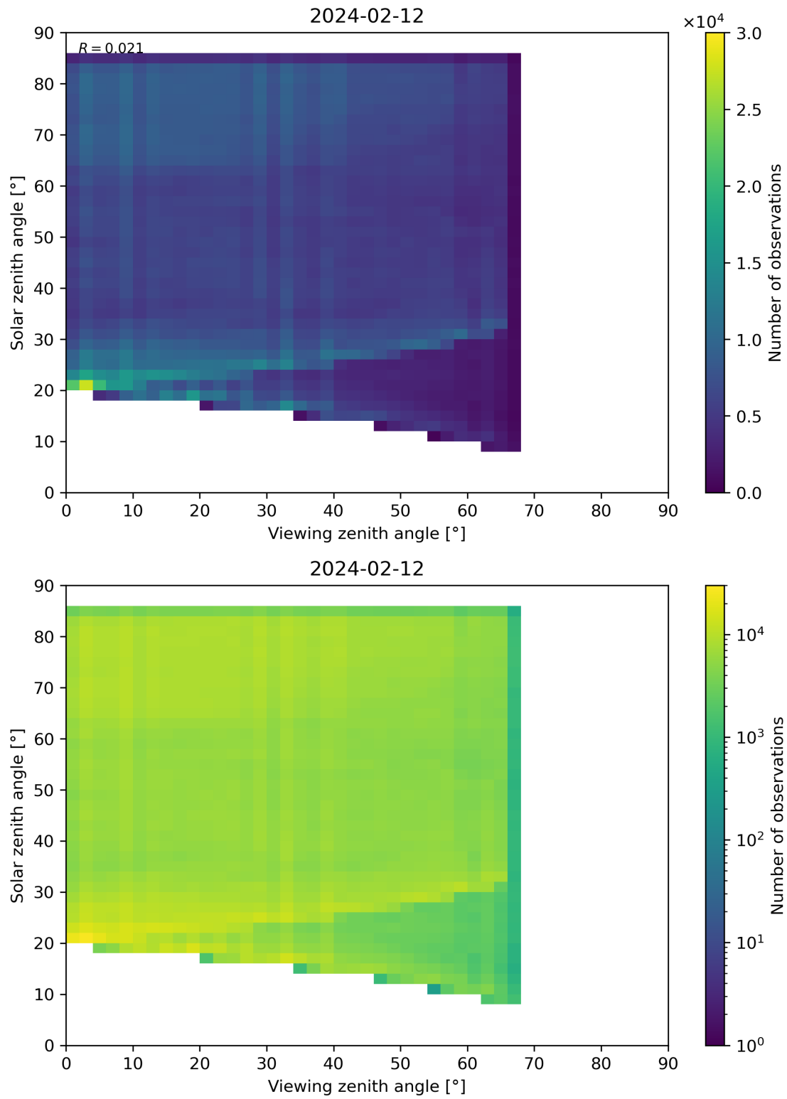
Figure 77: Scatter density plot of “Viewing zenith angle” against “Solar zenith angle” for 2024-02-11 to 2024-02-13.
