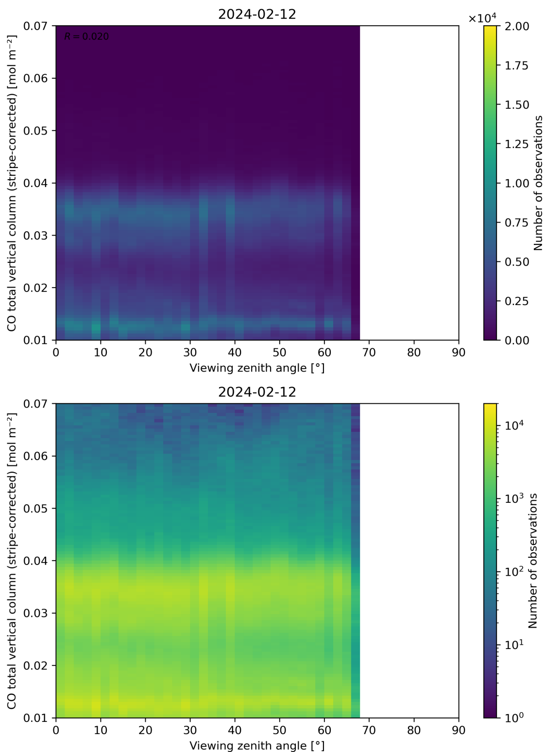
Figure 70: Scatter density plot of “Viewing zenith angle” against “CO total vertical column (stripe-corrected)” for 2024-02-11 to 2024-02-13.
