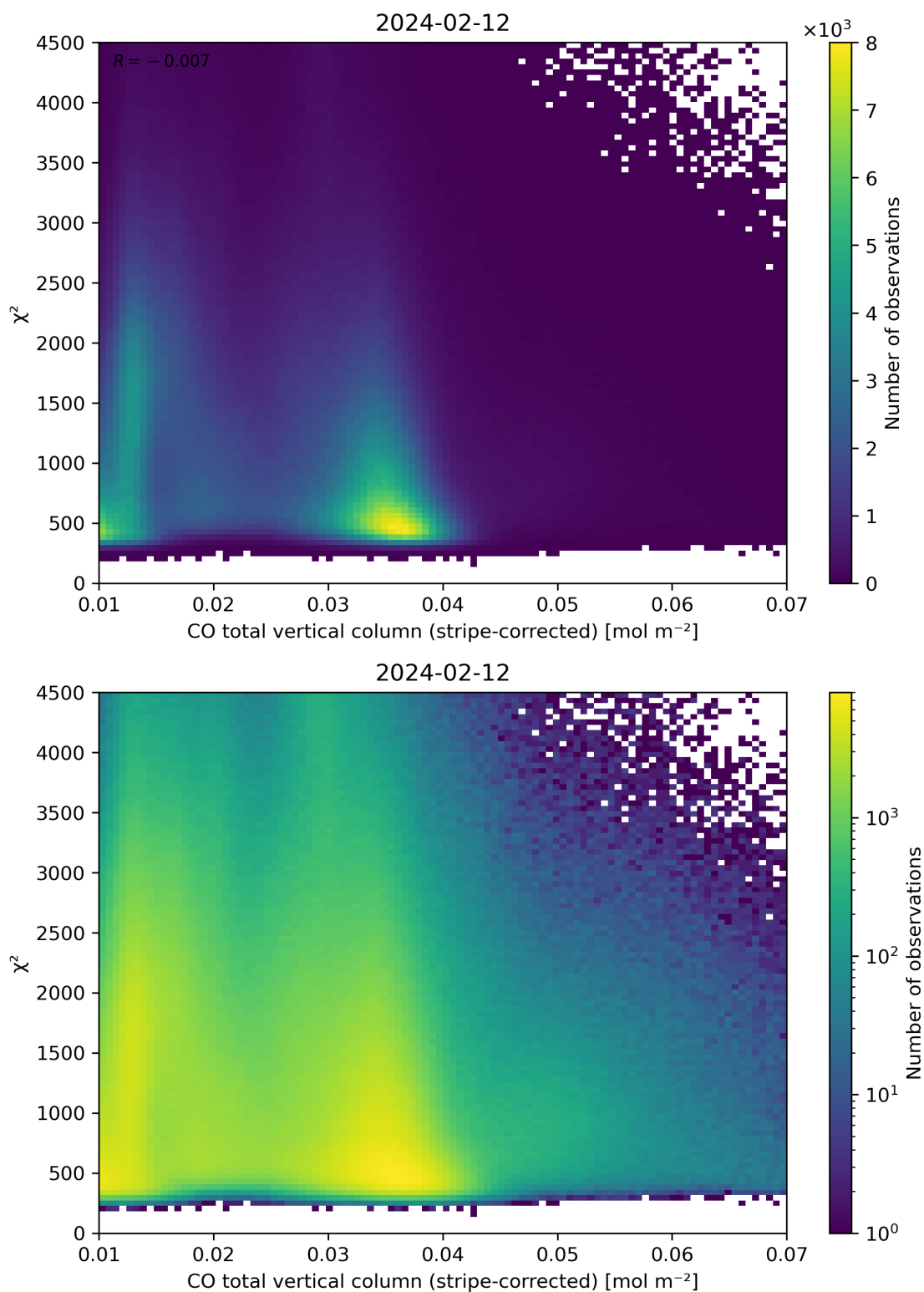
Figure 37: Scatter density plot of “CO total vertical column (stripe-corrected)” against “ \chi^2 ” for 2024-02-11 to 2024-02-13.
