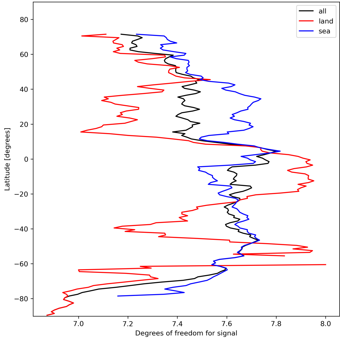
Figure 15: Zonal average of “Degrees of freedom for signal” for 2024-02-11 to 2024-02-13.
