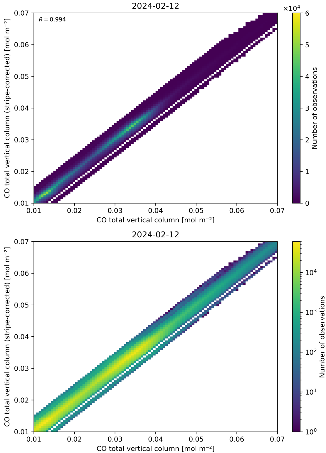
Figure 33: Scatter density plot of “CO total vertical column” against “CO total vertical column (stripe-corrected)” for 2024-02-11 to 2024-02-13.
