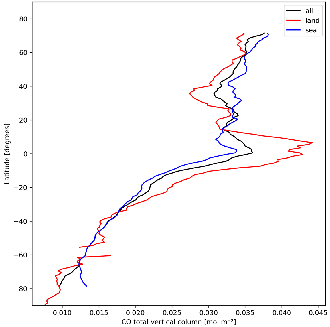
Figure 10: Zonal average of “CO total vertical column” for 2024-02-11 to 2024-02-13.
