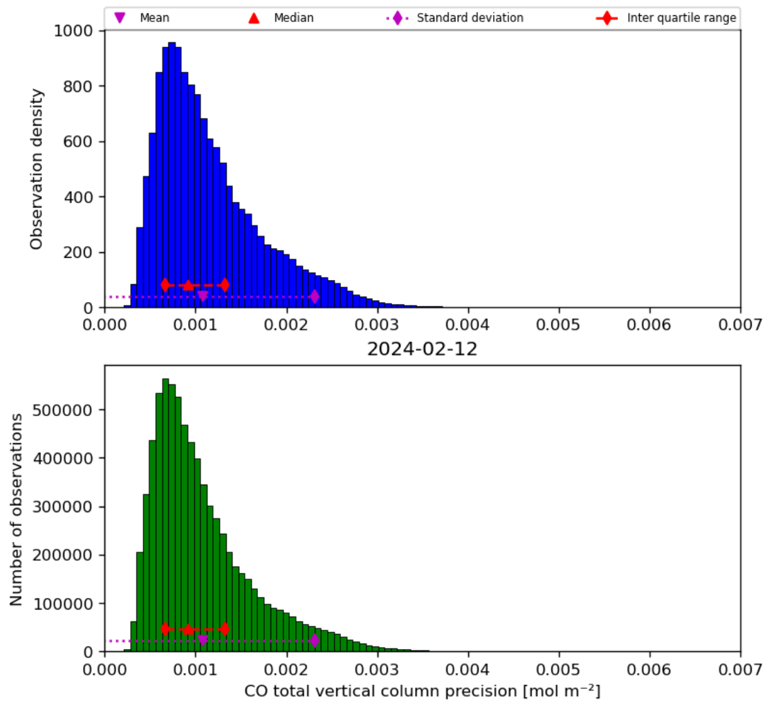
Figure 20: Histogram of “CO total vertical column precision” for 2024-02-11 to 2024-02-13
