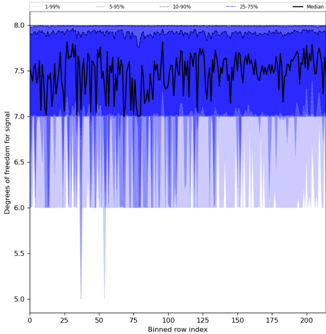
Figure 31: Along track statistics of “Degrees of freedom for signal” for 2024-02-11 to 2024-02-13
