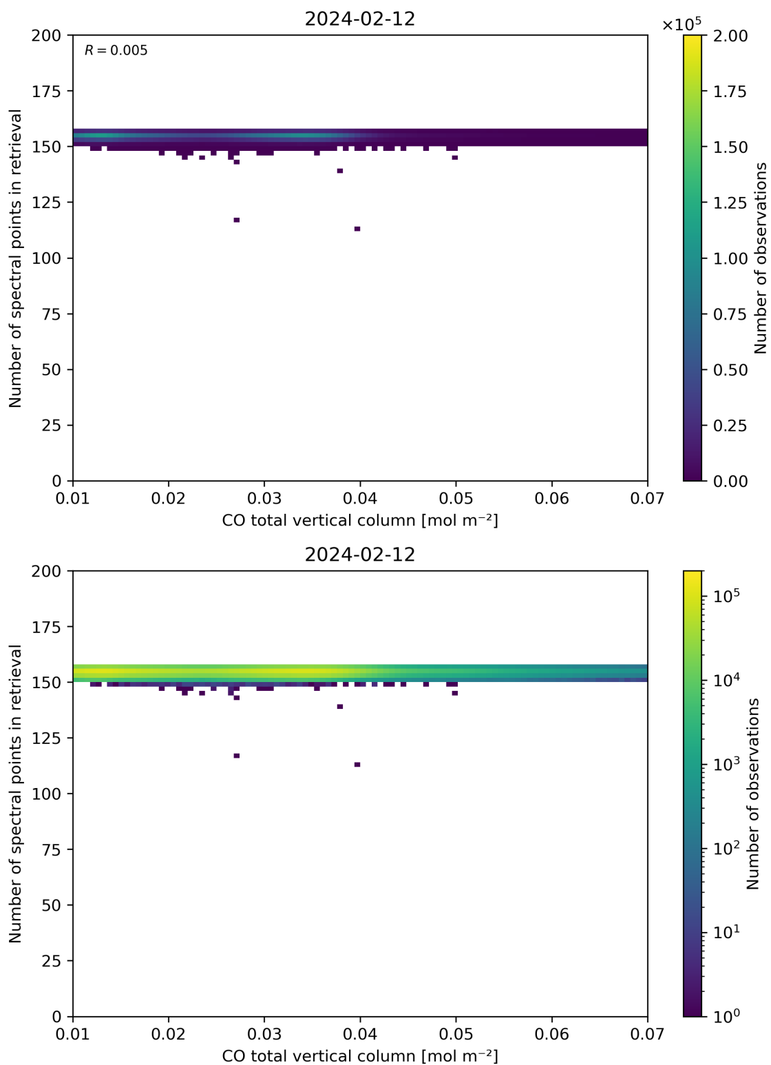
Figure 43: Scatter density plot of “CO total vertical column” against “Number of spectral points in retrieval” for 2024-02-11 to 2024-02-13.
