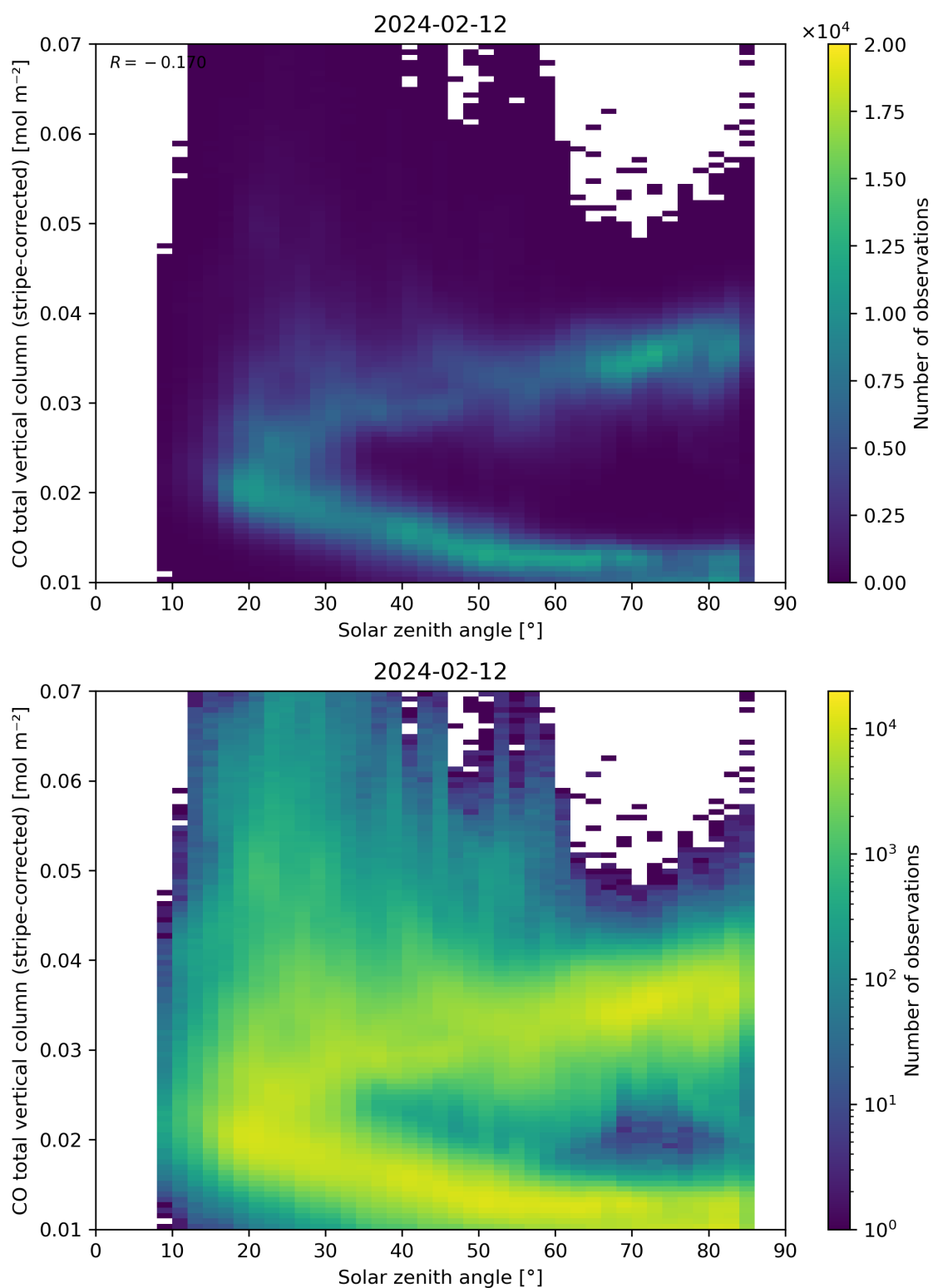
Figure 62: Scatter density plot of “Solar zenith angle” against “CO total vertical column (stripe-corrected)” for 2024-02-11 to 2024-02-13.
