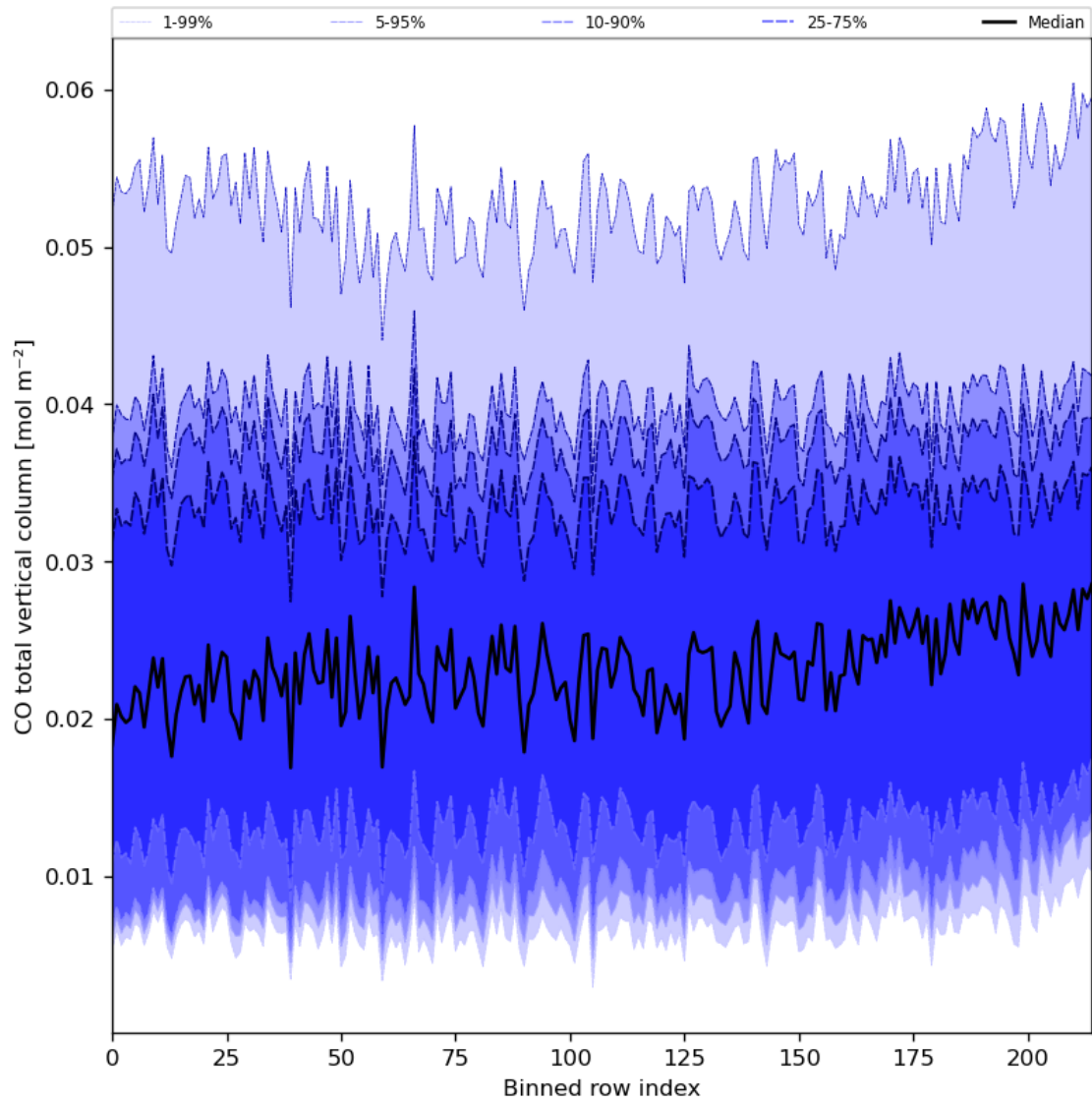
Figure 26: Along track statistics of “CO total vertical column” for 2024-02-11 to 2024-02-13
