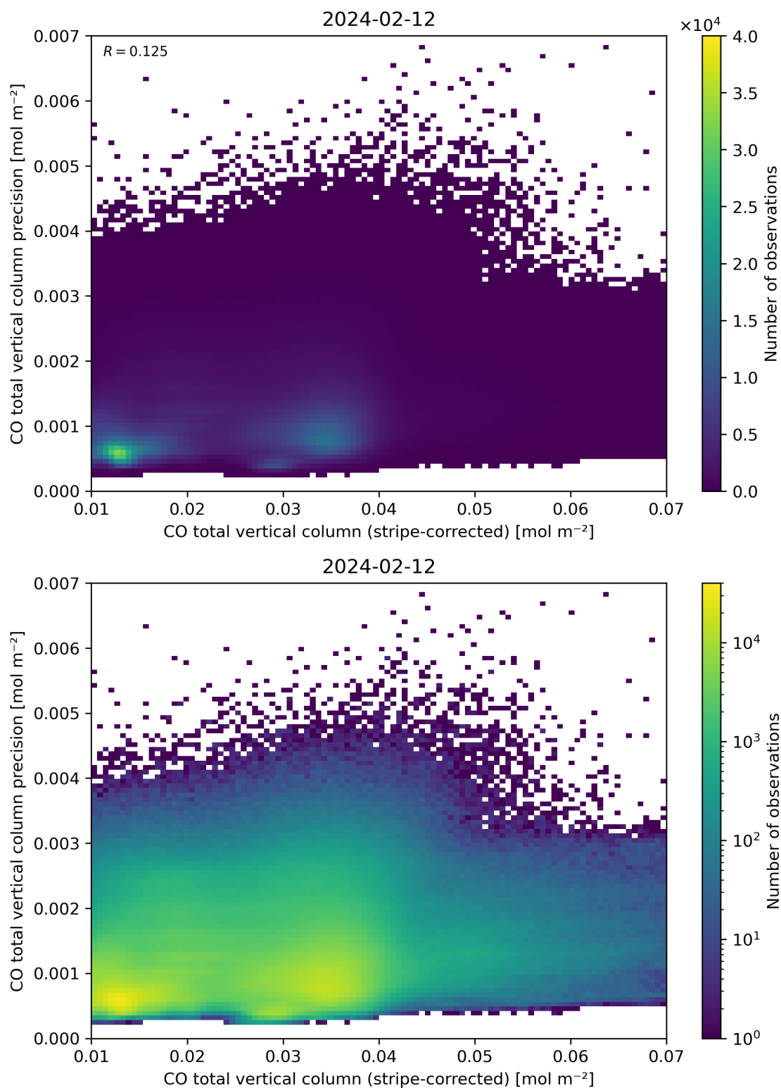
Figure 36: Scatter density plot of “CO total vertical column (stripe-corrected)” against “CO total vertical column precision” for 2024-02-11 to 2024-02-13.
