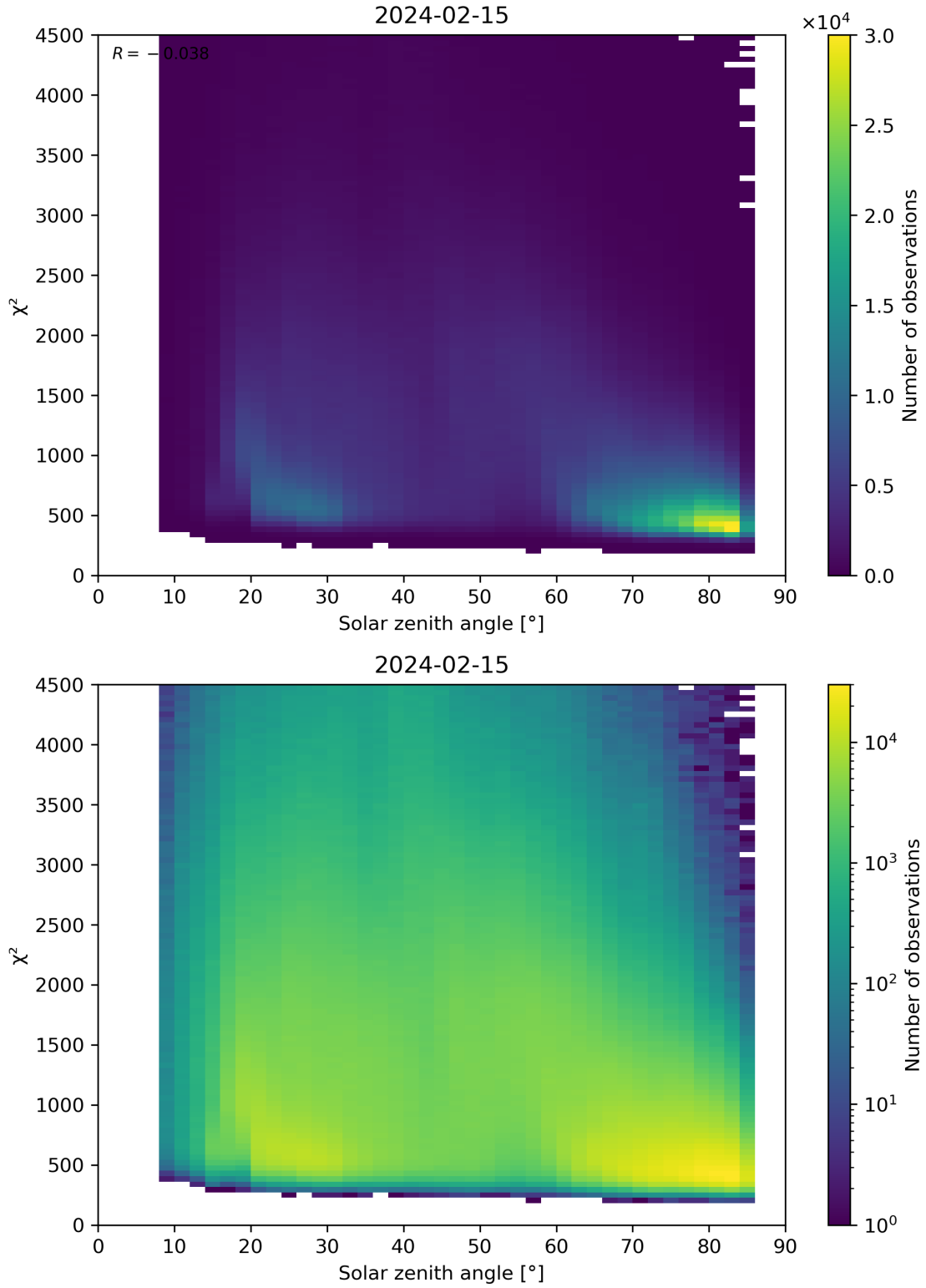
Figure 64: Scatter density plot of “Solar zenith angle” against “ \chi^2 ” for 2024-02-14 to 2024-02-16.
