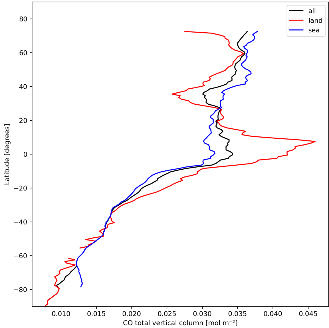
Figure 10: Zonal average of “CO total vertical column” for 2024-02-14 to 2024-02-16.
