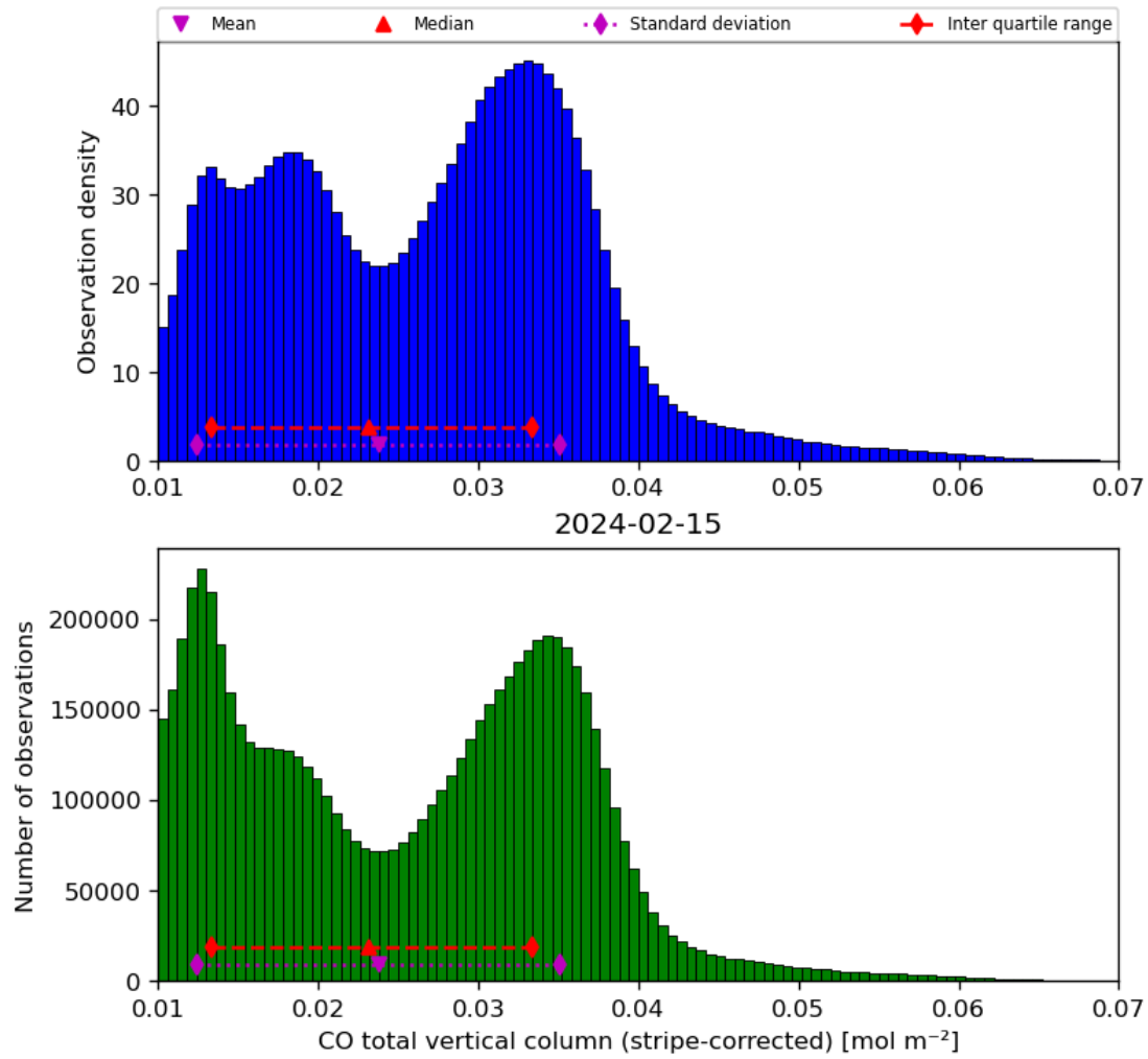
Figure 19: Histogram of “CO total vertical column (stripe-corrected)” for 2024-02-14 to 2024-02-16
