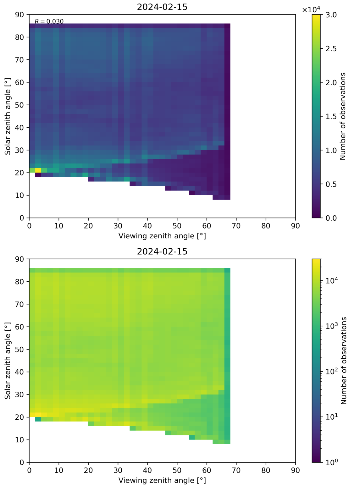
Figure 77: Scatter density plot of “Viewing zenith angle” against “Solar zenith angle” for 2024-02-14 to 2024-02-16.
