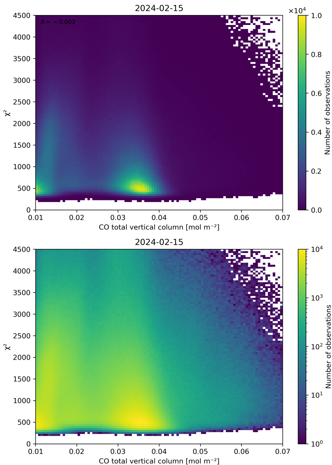
Figure 35: Scatter density plot of “CO total vertical column” against “ \chi^2 ” for 2024-02-14 to 2024-02-16.
