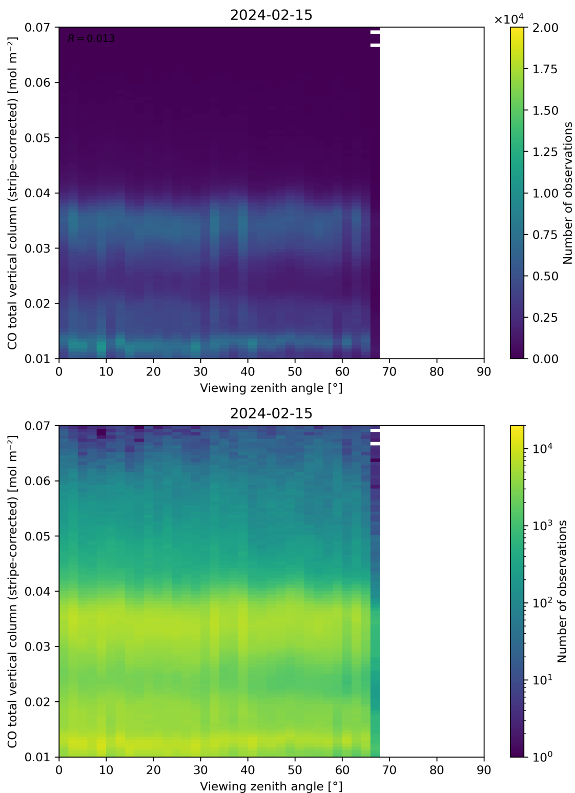
Figure 70: Scatter density plot of “Viewing zenith angle” against “CO total vertical column (stripe-corrected)” for 2024-02-14 to 2024-02-16.
