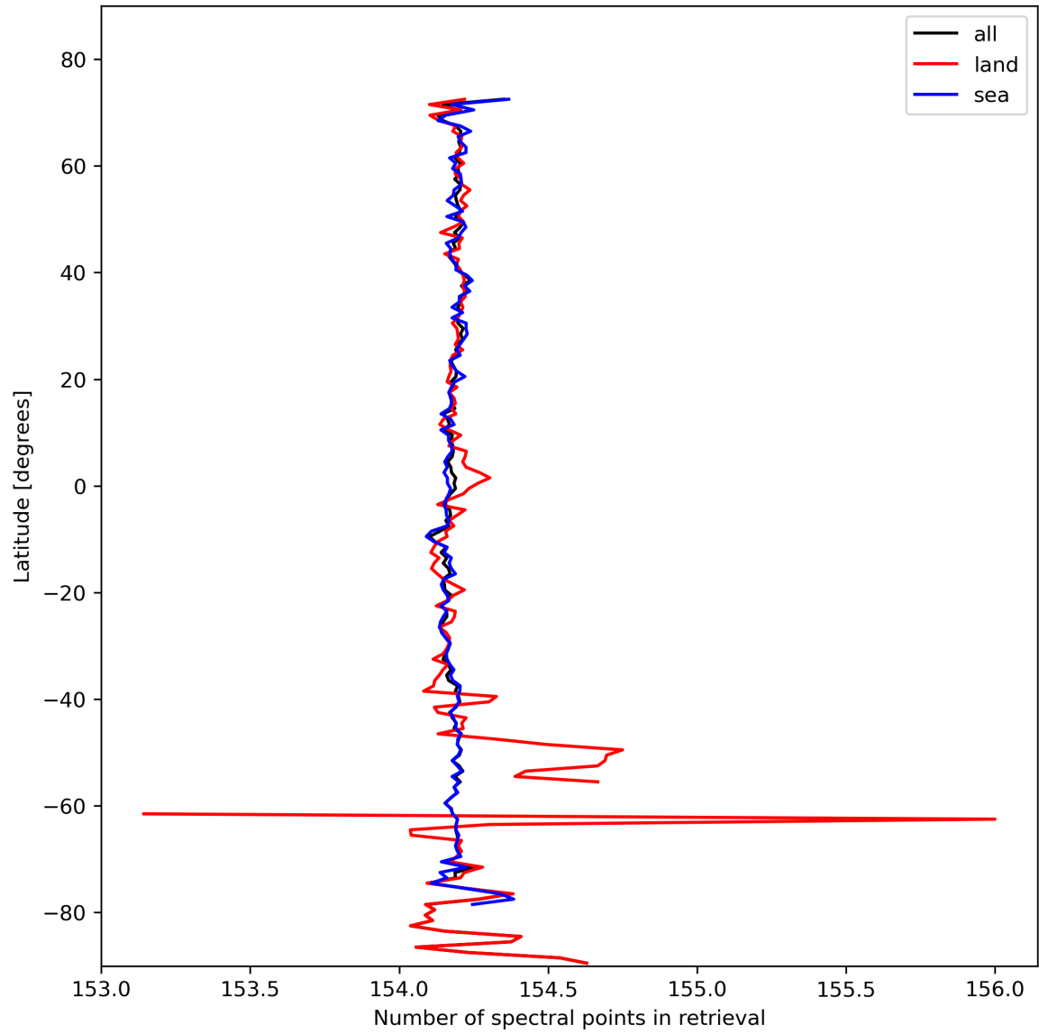
Figure 13: Zonal average of “Number of spectral points in retrieval” for 2024-02-14 to 2024-02-16.
