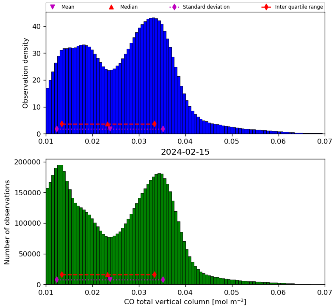
Figure 18: Histogram of “CO total vertical column” for 2024-02-14 to 2024-02-16
