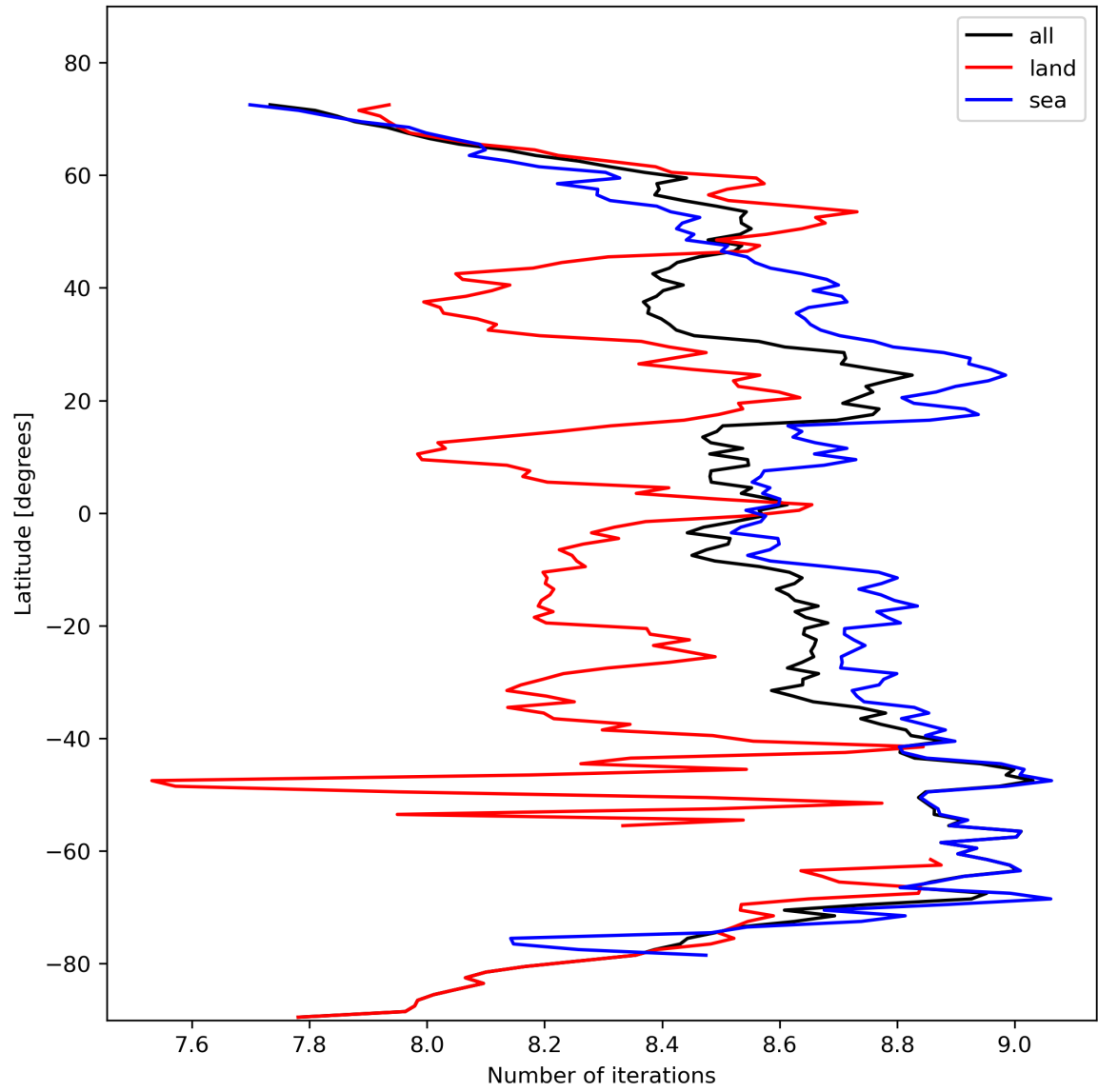
Figure 16: Zonal average of “Number of iterations” for 2024-02-14 to 2024-02-16.
