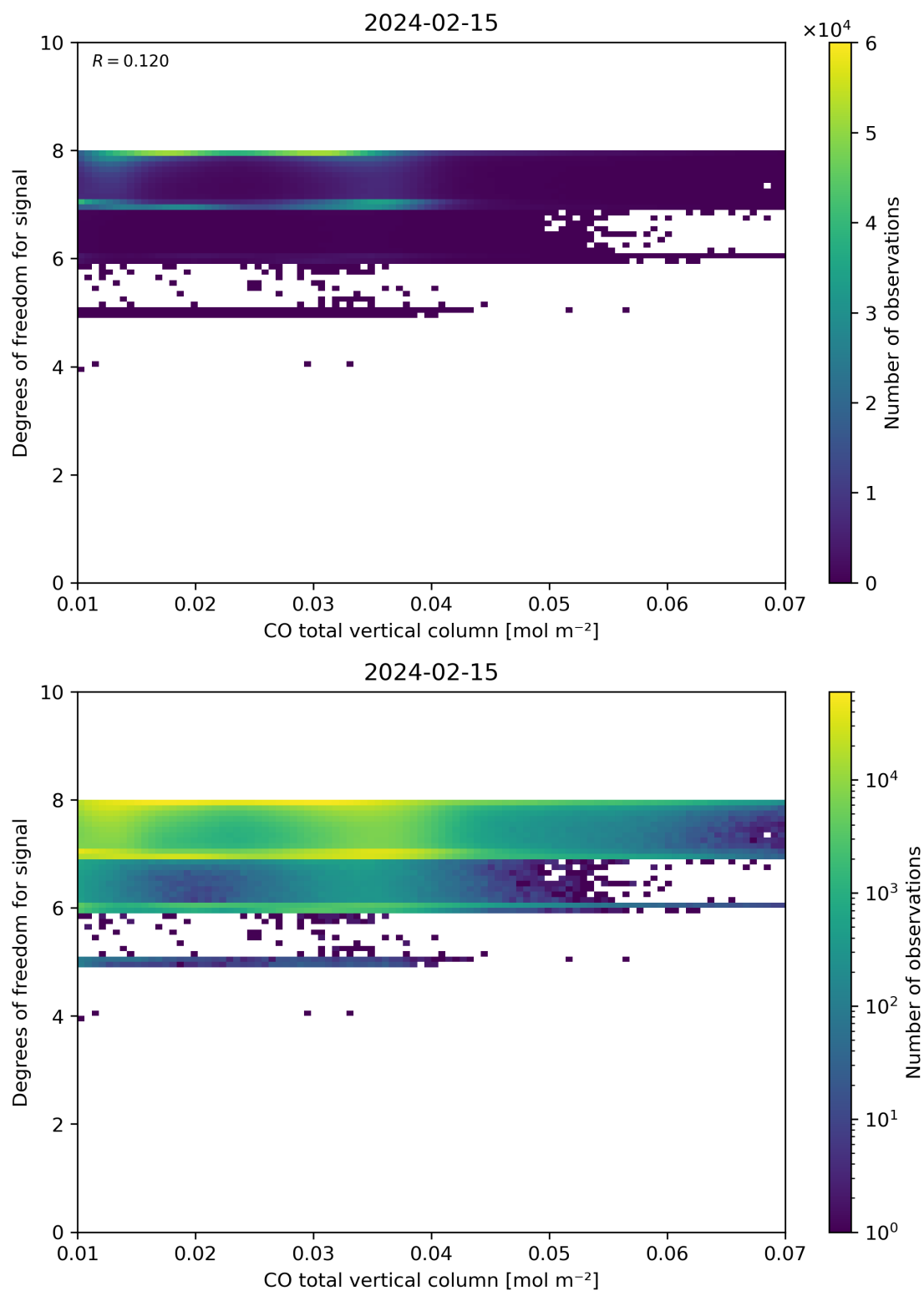
Figure 41: Scatter density plot of “CO total vertical column” against “Degrees of freedom for signal” for 2024-02-14 to 2024-02-16.
