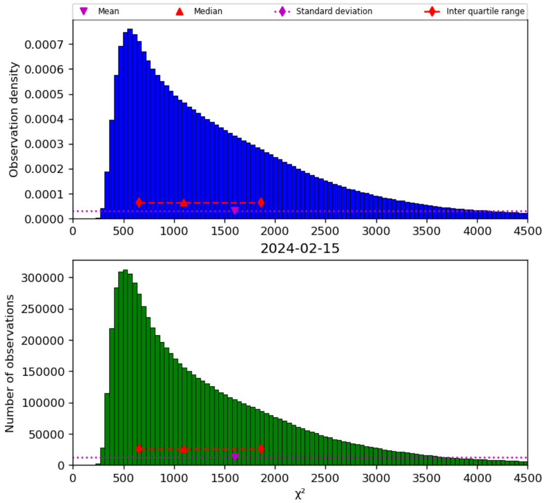
Figure 22: Histogram of “ \chi^2 ” for 2024-02-14 to 2024-02-16
