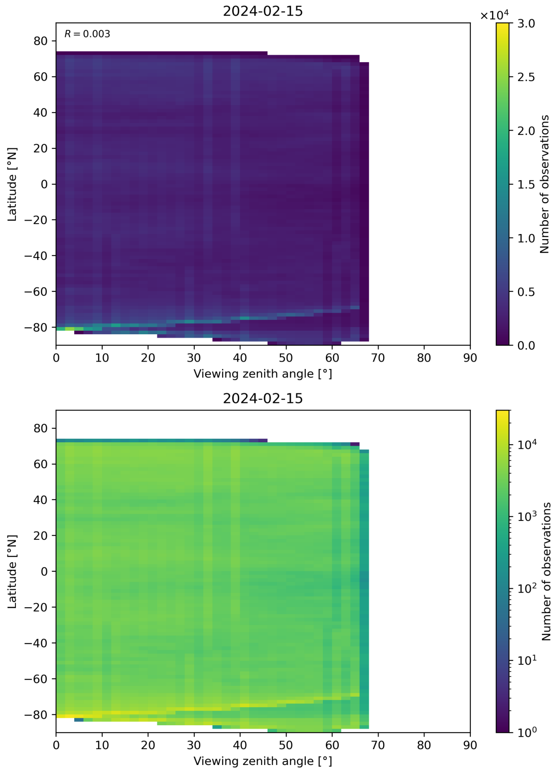
Figure 74: Scatter density plot of “Viewing zenith angle” against “Latitude” for 2024-02-14 to 2024-02-16.
