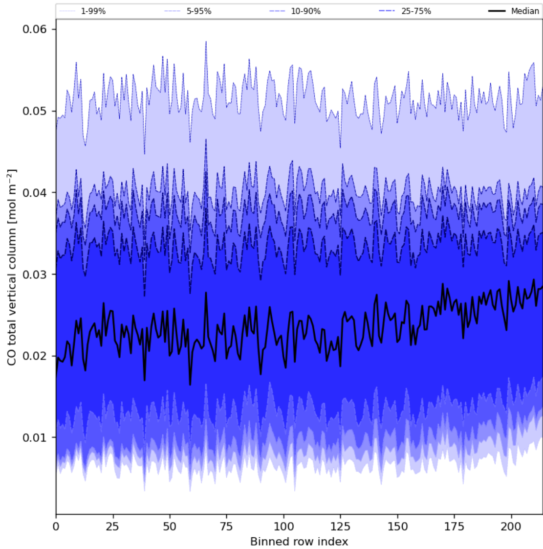
Figure 26: Along track statistics of “CO total vertical column” for 2024-02-14 to 2024-02-16
