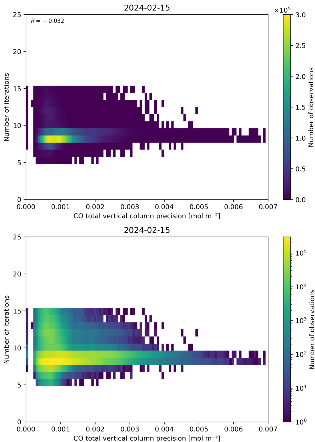
Figure 46: Scatter density plot of “CO total vertical column precision” against “Number of iterations” for 2024-02-14 to 2024-02-16.
