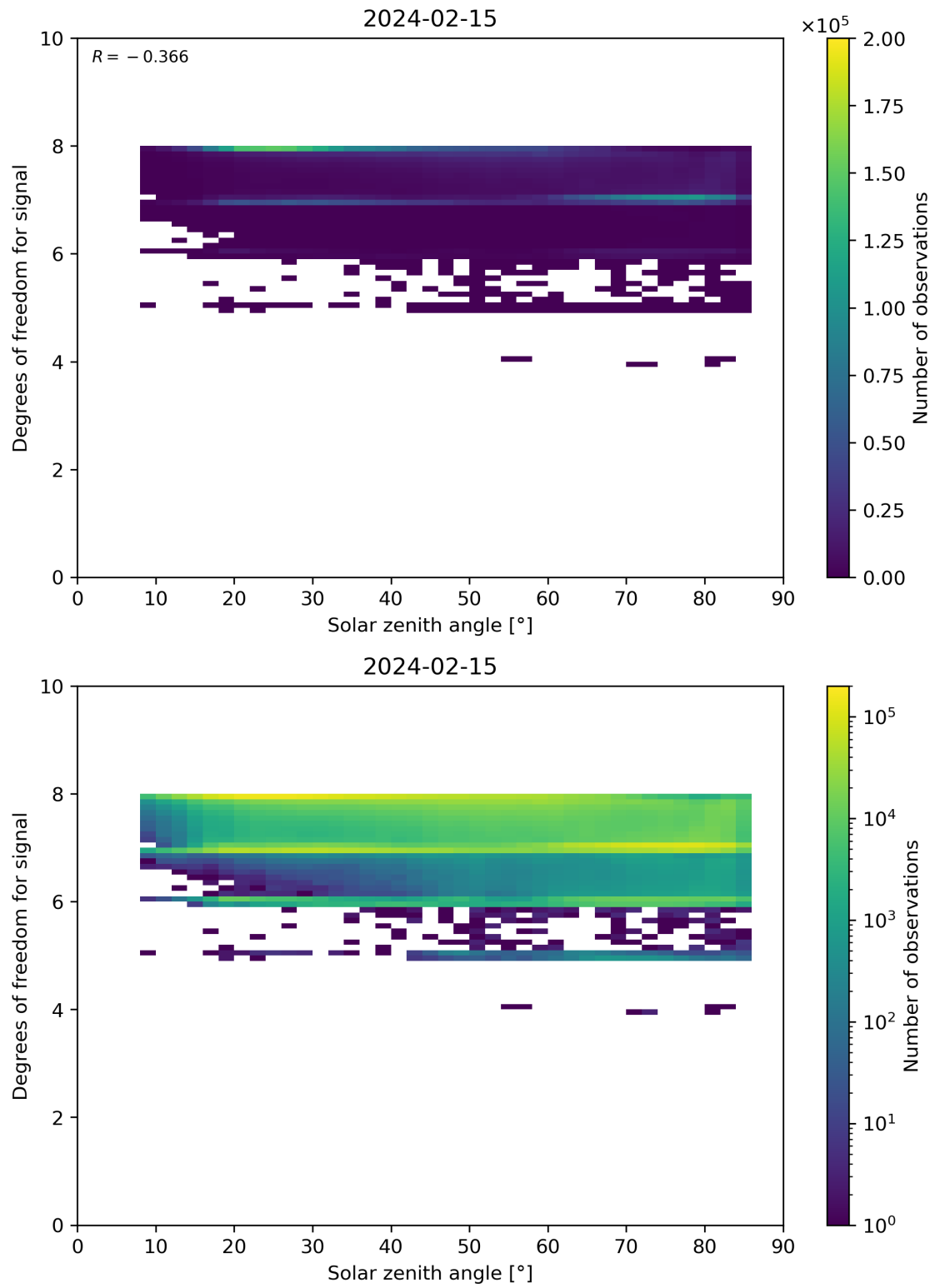
Figure 65: Scatter density plot of “Solar zenith angle” against “Degrees of freedom for signal” for 2024-02-14 to 2024-02-16.
