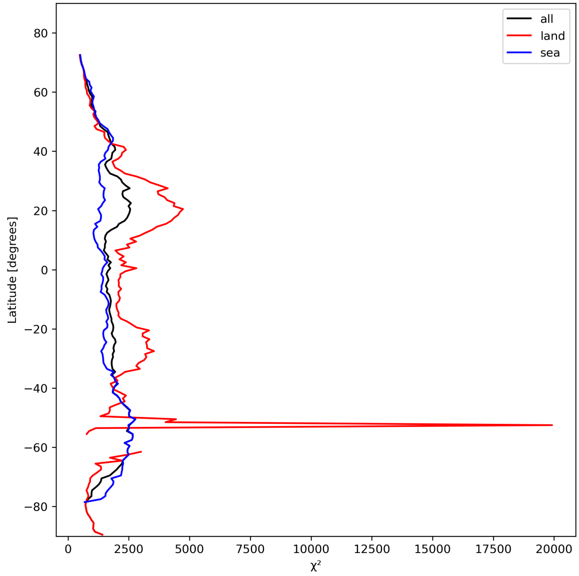
Figure 14: Zonal average of “ \chi^2 ” for 2024-02-14 to 2024-02-16.
