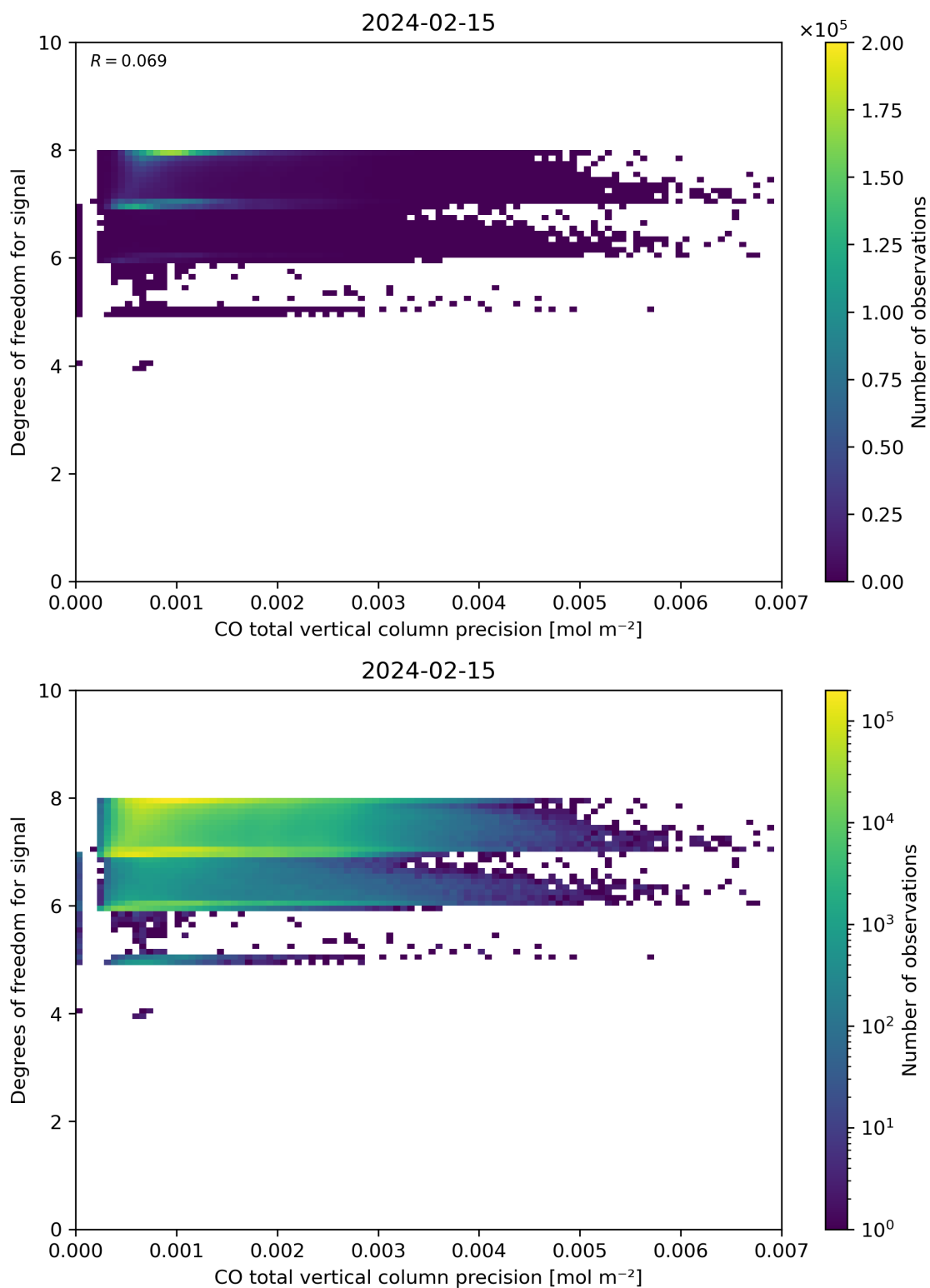
Figure 45: Scatter density plot of “CO total vertical column precision” against “Degrees of freedom for signal” for 2024-02-14 to 2024-02-16.
