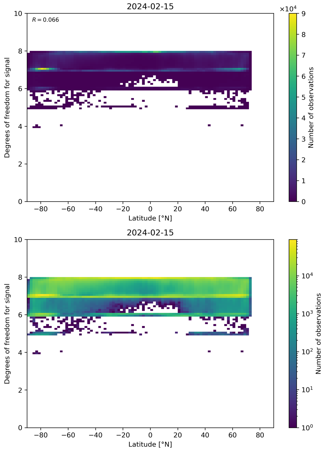
Figure 55: Scatter density plot of “Latitude” against “Degrees of freedom for signal” for 2024-02-14 to 2024-02-16.
