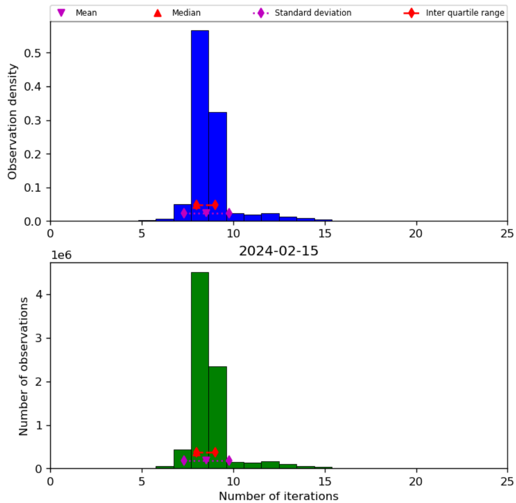
Figure 24: Histogram of “Number of iterations” for 2024-02-14 to 2024-02-16
