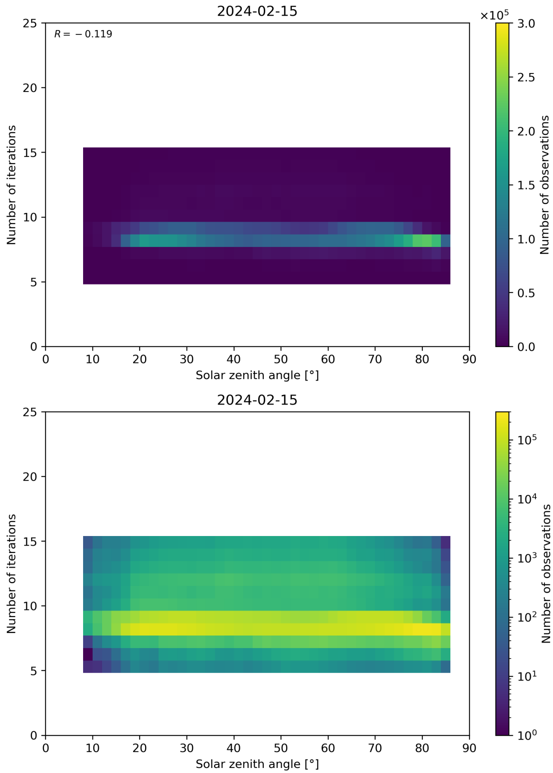
Figure 67: Scatter density plot of “Solar zenith angle” against “Number of iterations” for 2024-02-14 to 2024-02-16.
