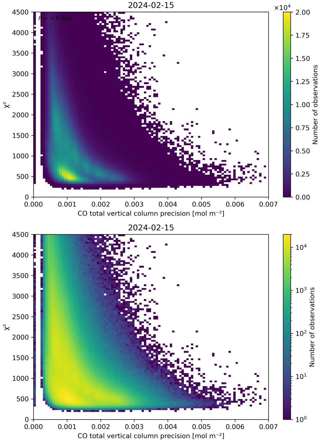
Figure 44: Scatter density plot of “CO total vertical column precision” against “ \chi^2 ” for 2024-02-14 to 2024-02-16.
