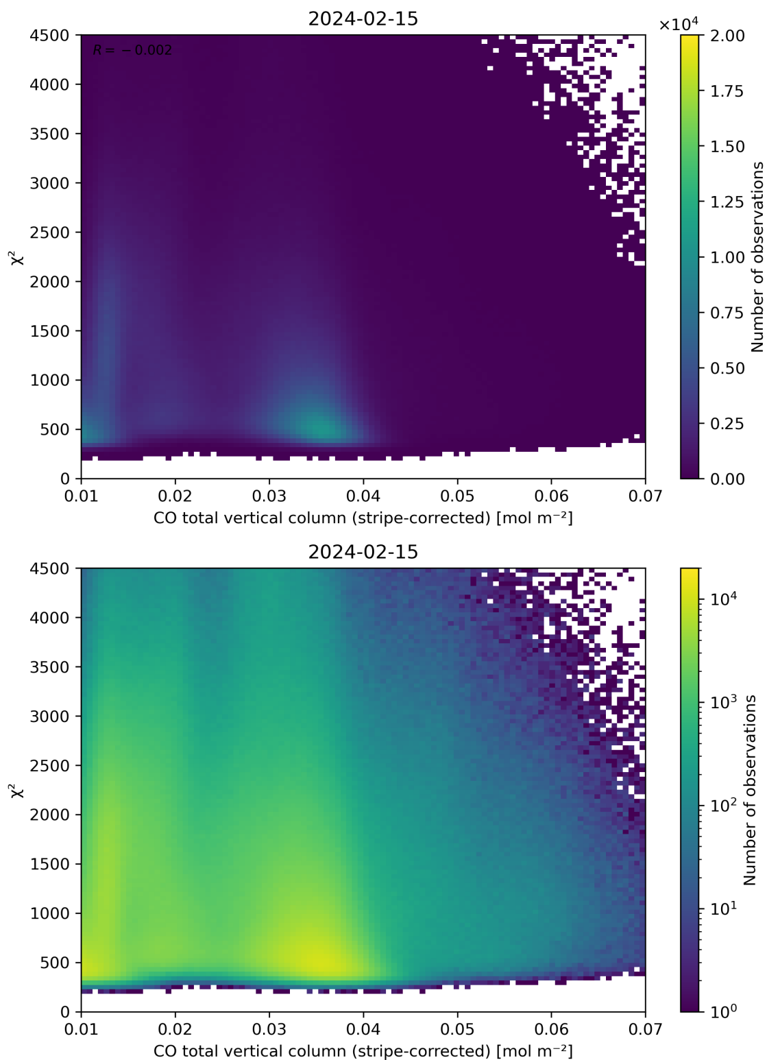
Figure 37: Scatter density plot of “CO total vertical column (stripe-corrected)” against “ \chi^2 ” for 2024-02-14 to 2024-02-16.
