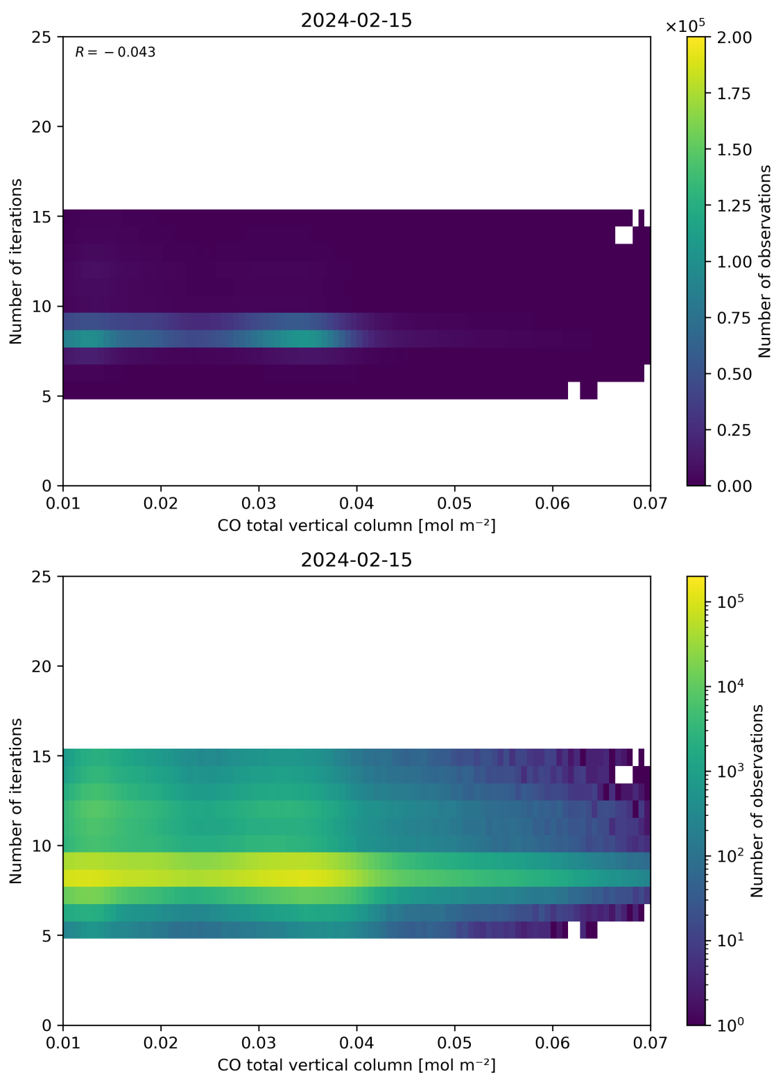
Figure 42: Scatter density plot of “CO total vertical column” against “Number of iterations” for 2024-02-14 to 2024-02-16.
