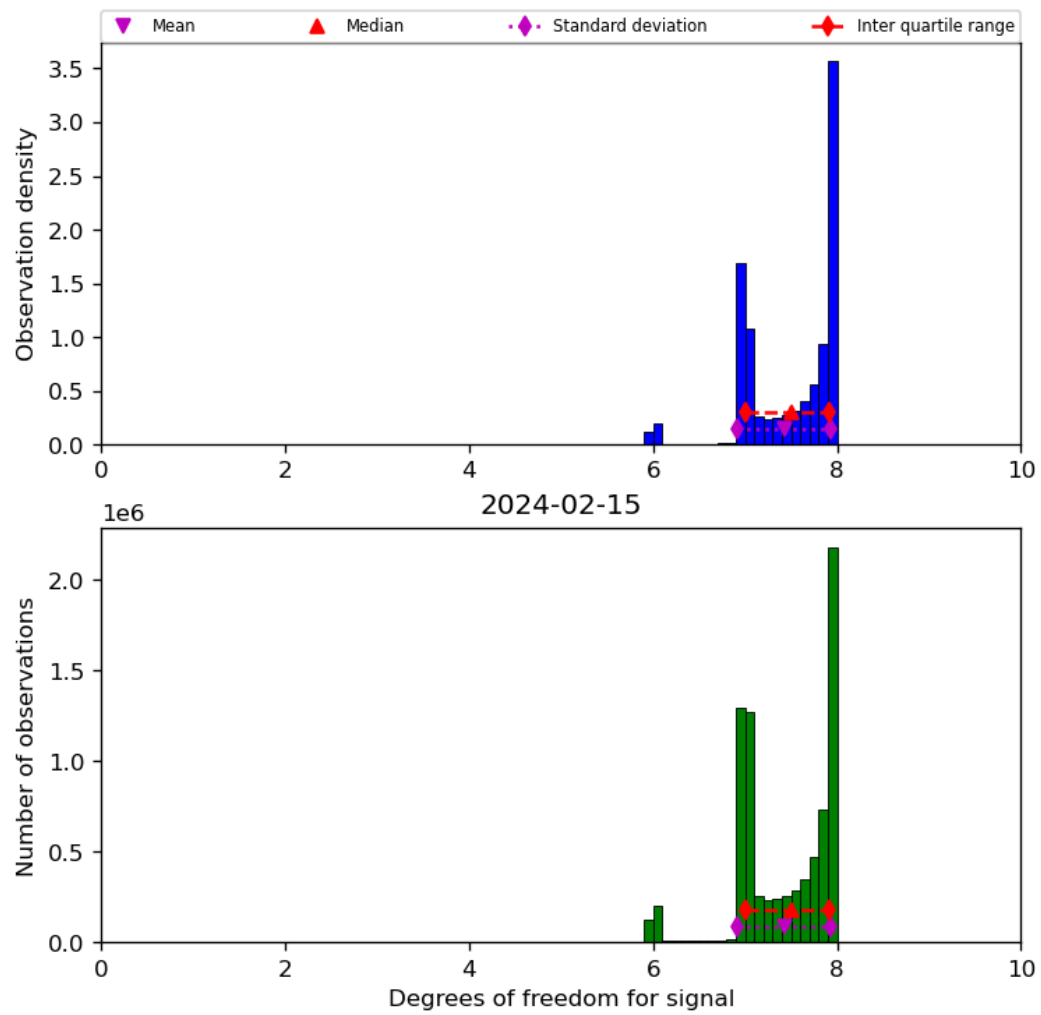
Figure 23: Histogram of “Degrees of freedom for signal” for 2024-02-14 to 2024-02-16
