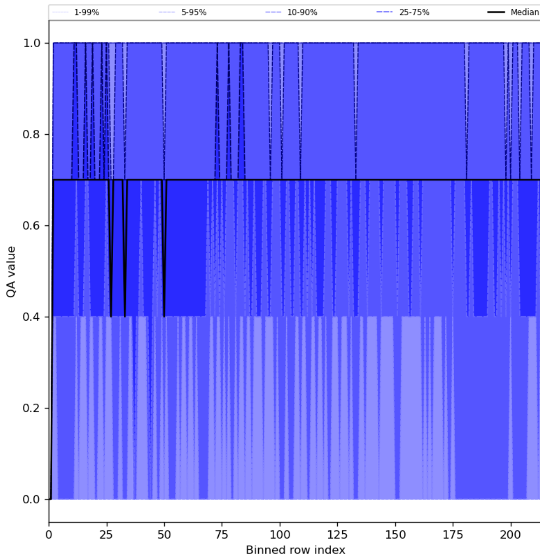
Figure 25: Along track statistics of “QA value” for 2024-02-14 to 2024-02-16
