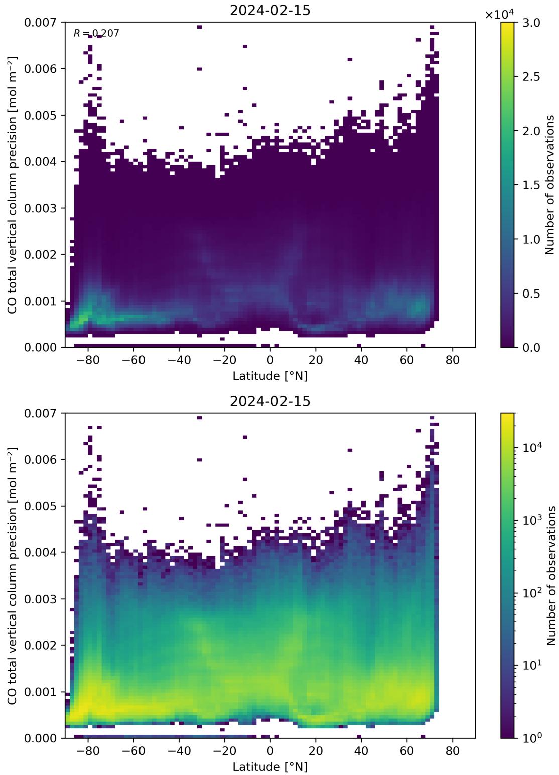
Figure 53: Scatter density plot of “Latitude” against “CO total vertical column precision” for 2024-02-14 to 2024-02-16.
