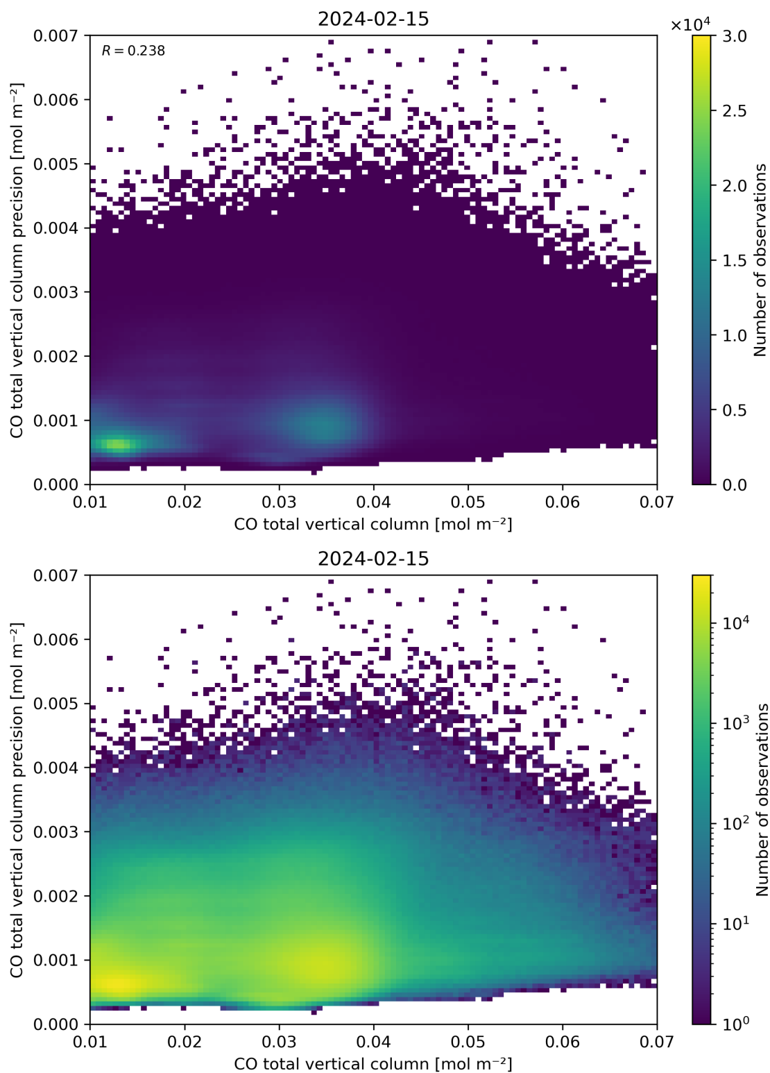
Figure 34: Scatter density plot of “CO total vertical column” against “CO total vertical column precision” for 2024-02-14 to 2024-02-16.
