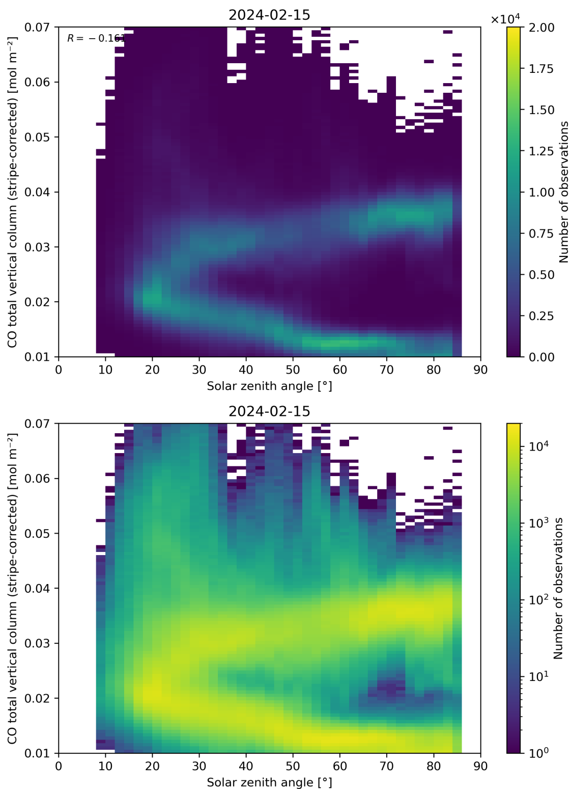
Figure 62: Scatter density plot of “Solar zenith angle” against “CO total vertical column (stripe-corrected)” for 2024-02-14 to 2024-02-16.
