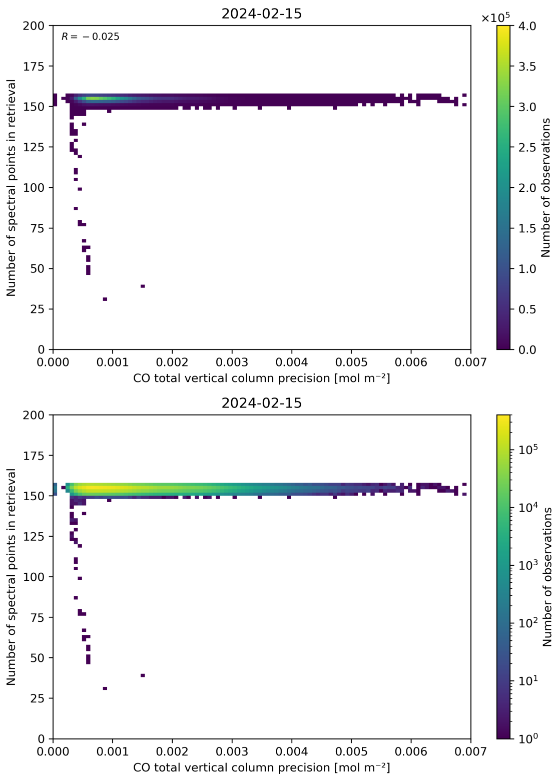
Figure 47: Scatter density plot of “CO total vertical column precision” against “Number of spectral points in retrieval” for 2024-02-14 to 2024-02-16.
