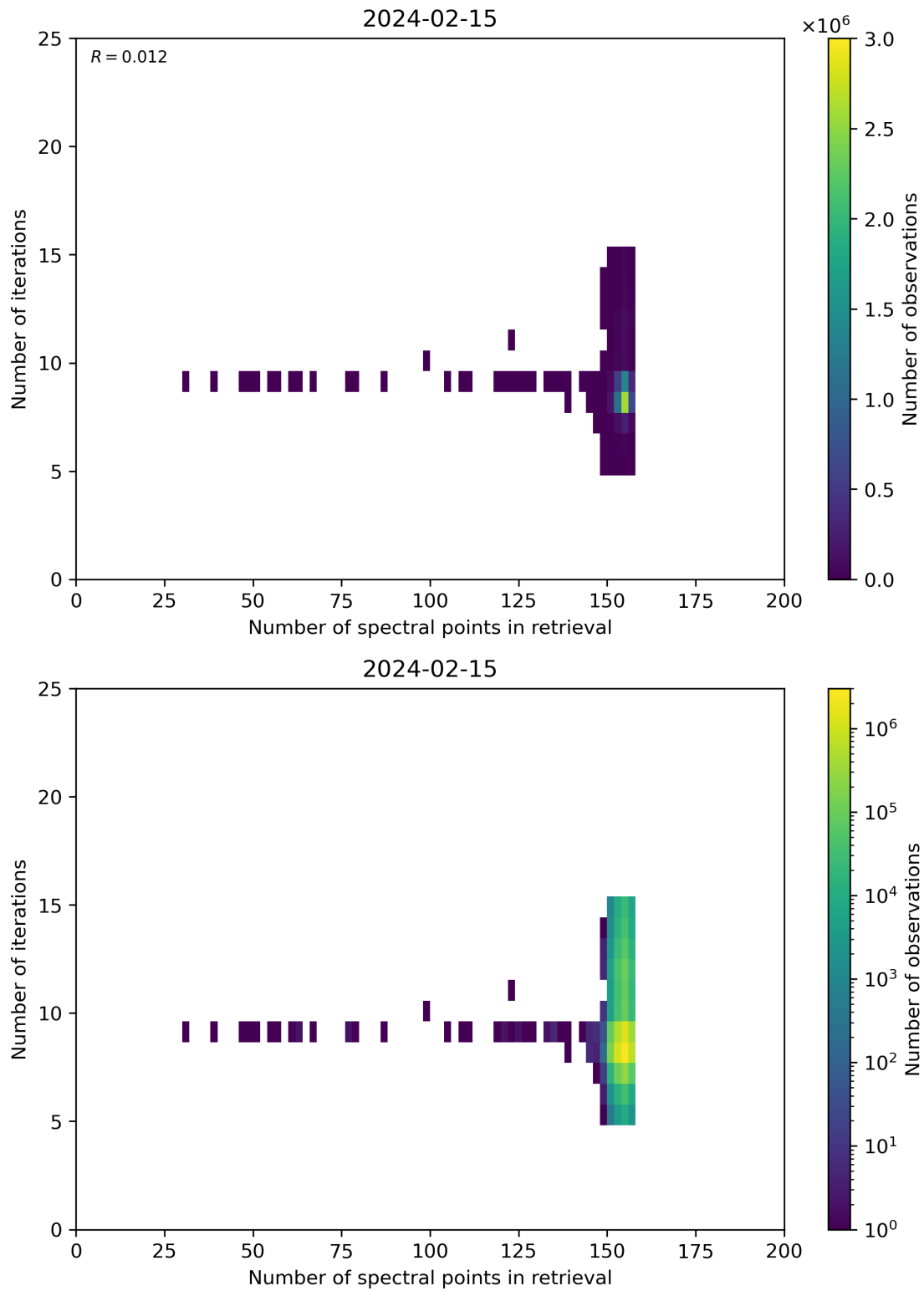
Figure 60: Scatter density plot of “Number of spectral points in retrieval” against “Number of iterations” for 2024-02-14 to 2024-02-16.
