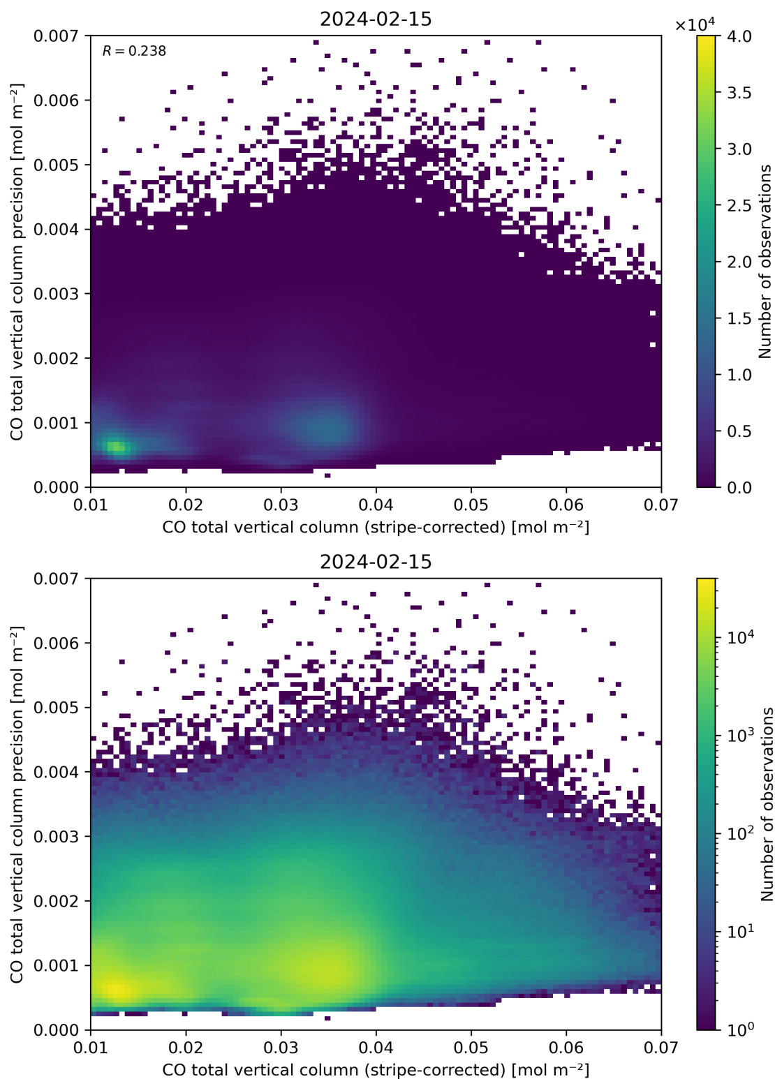
Figure 36: Scatter density plot of “CO total vertical column (stripe-corrected)” against “CO total vertical column precision” for 2024-02-14 to 2024-02-16.
