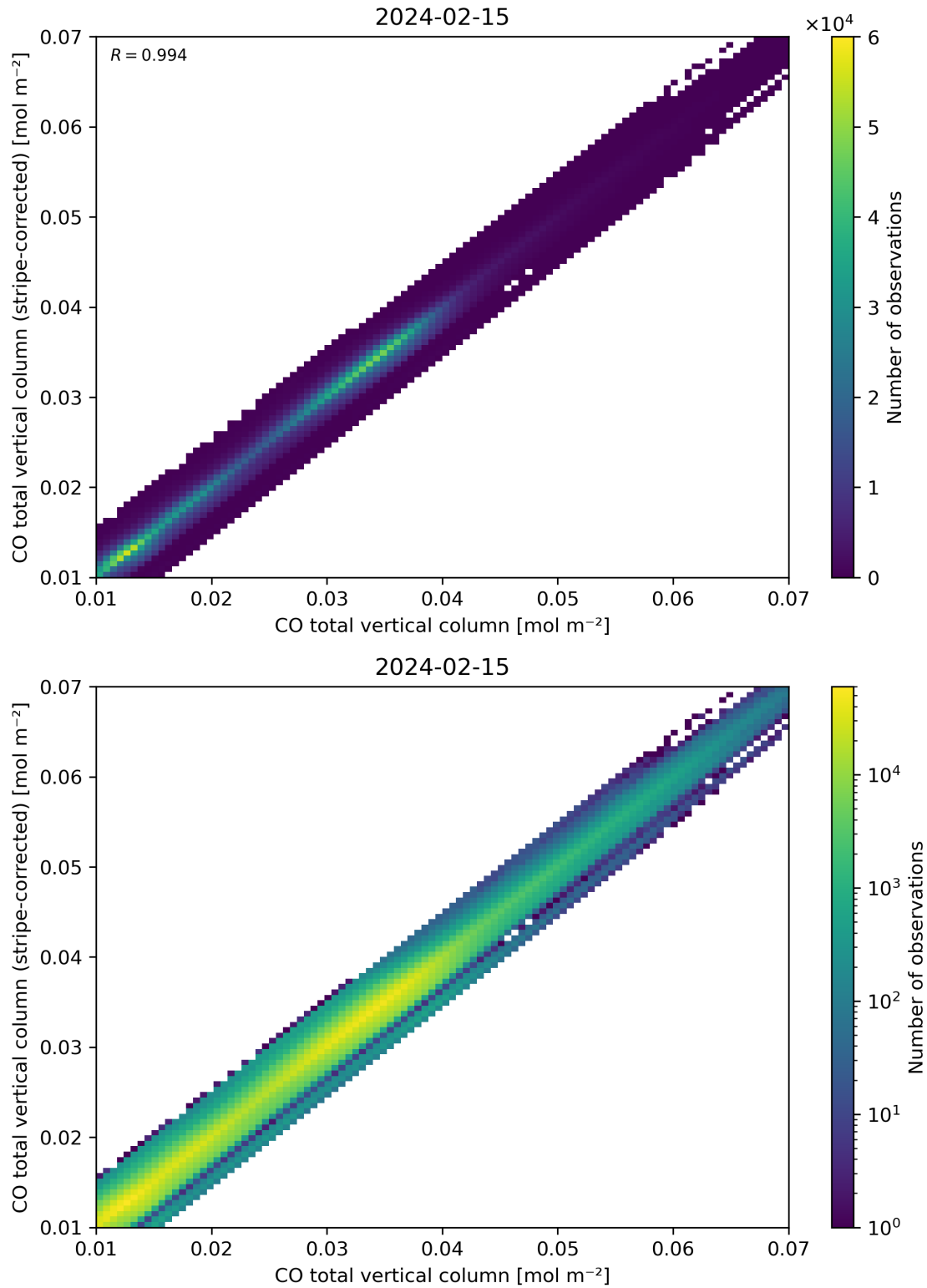
Figure 33: Scatter density plot of “CO total vertical column” against “CO total vertical column (stripe-corrected)” for 2024-02-14 to 2024-02-16.
