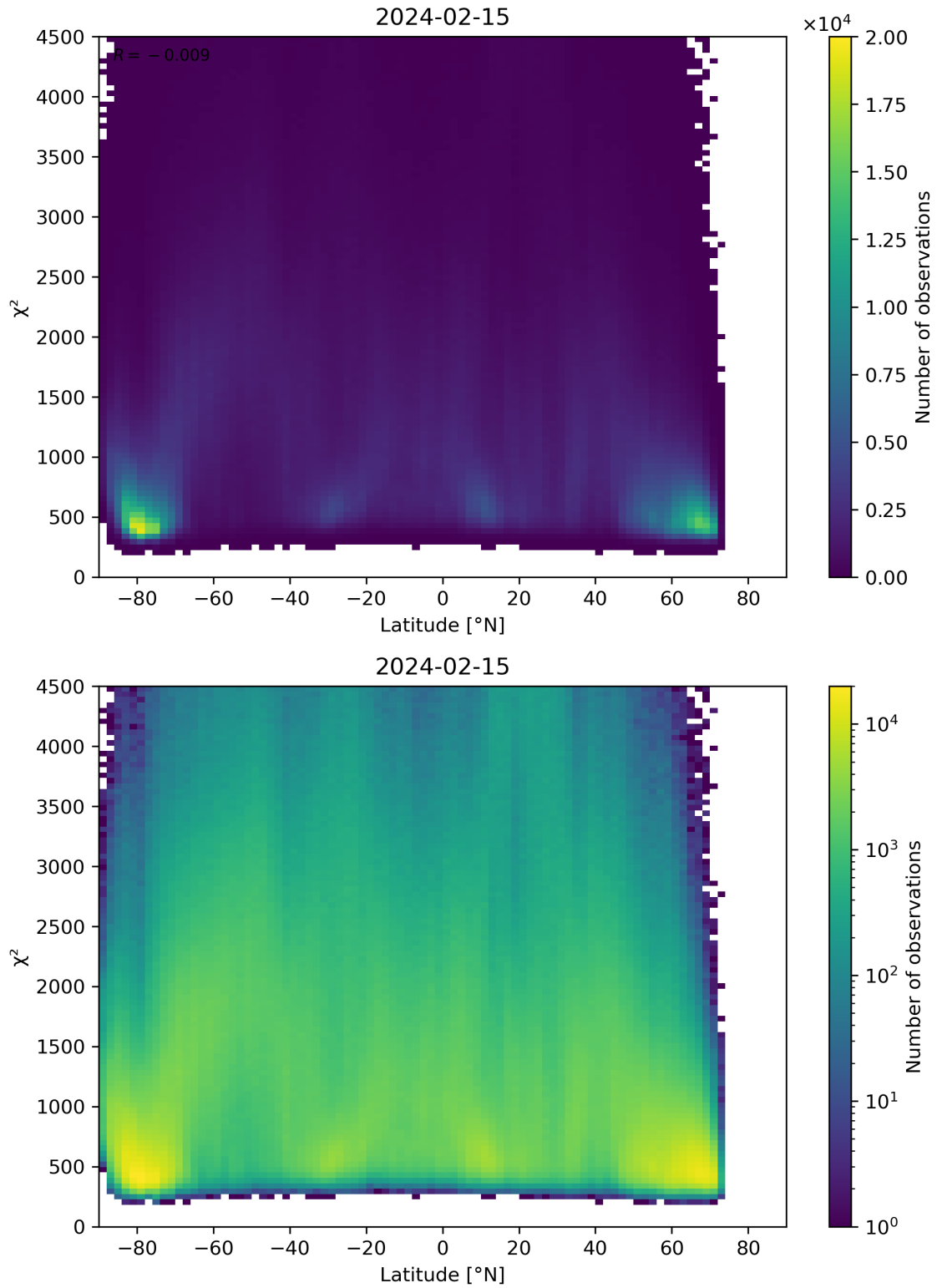
Figure 54: Scatter density plot of “Latitude” against “ \chi^2 ” for 2024-02-14 to 2024-02-16.
