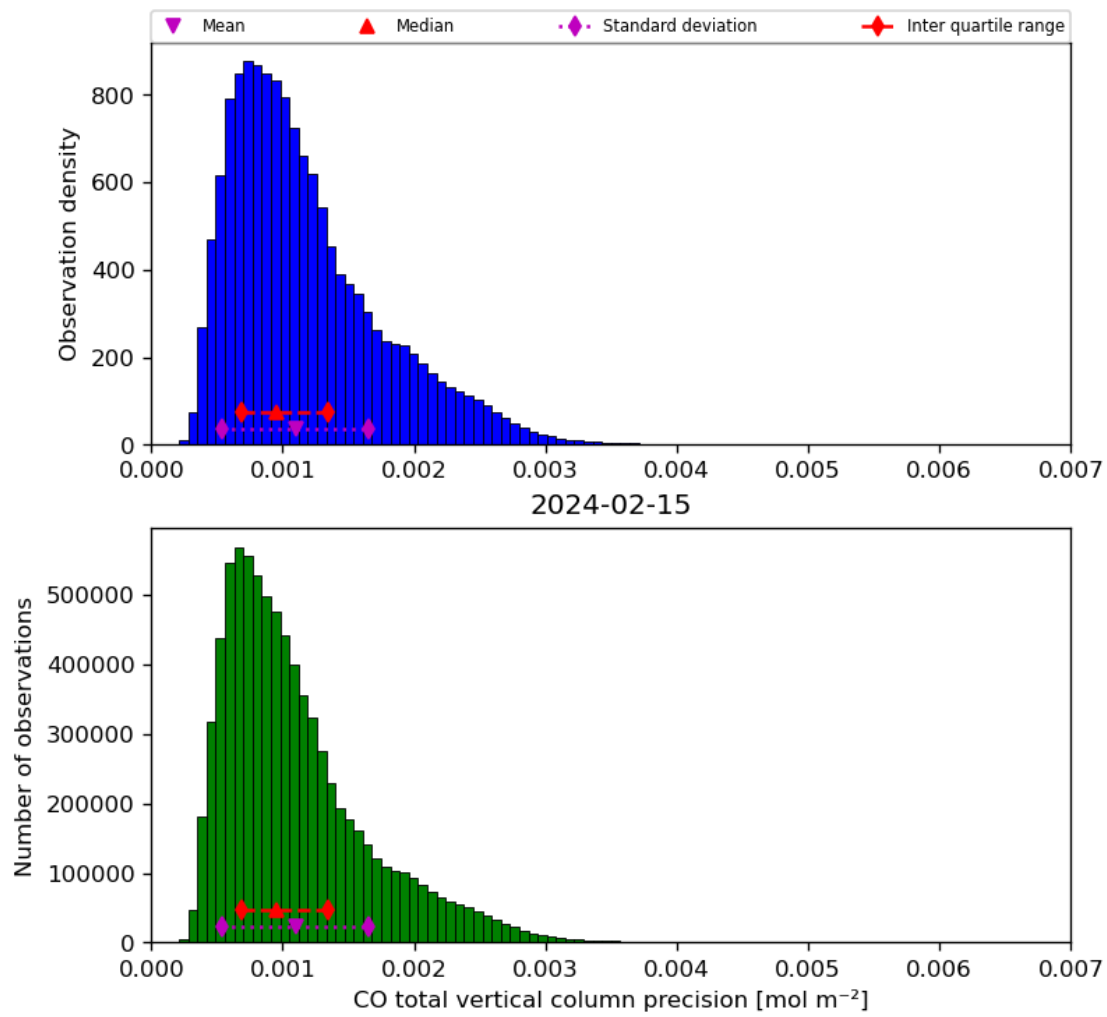
Figure 20: Histogram of “CO total vertical column precision” for 2024-02-14 to 2024-02-16
