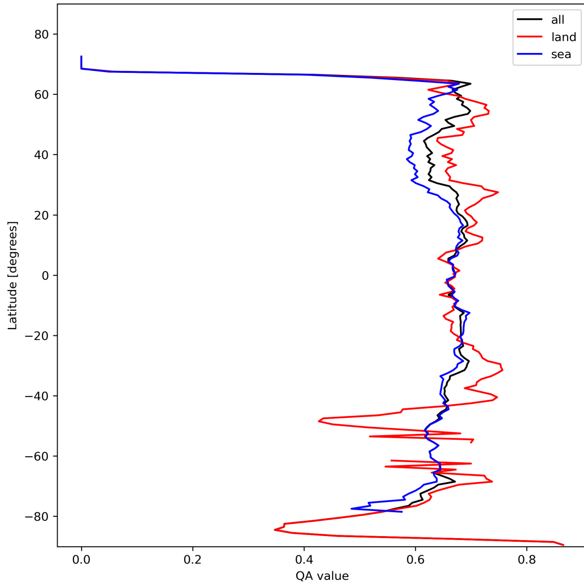
Figure 9: Zonal average of “QA value” for 2024-02-14 to 2024-02-16.
