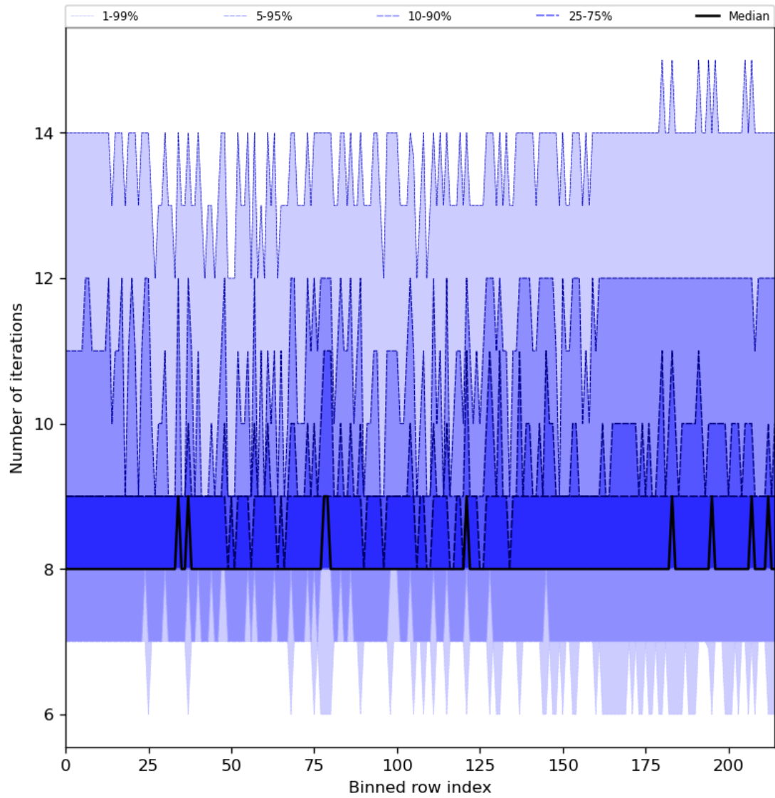
Figure 32: Along track statistics of “Number of iterations” for 2024-02-14 to 2024-02-16
