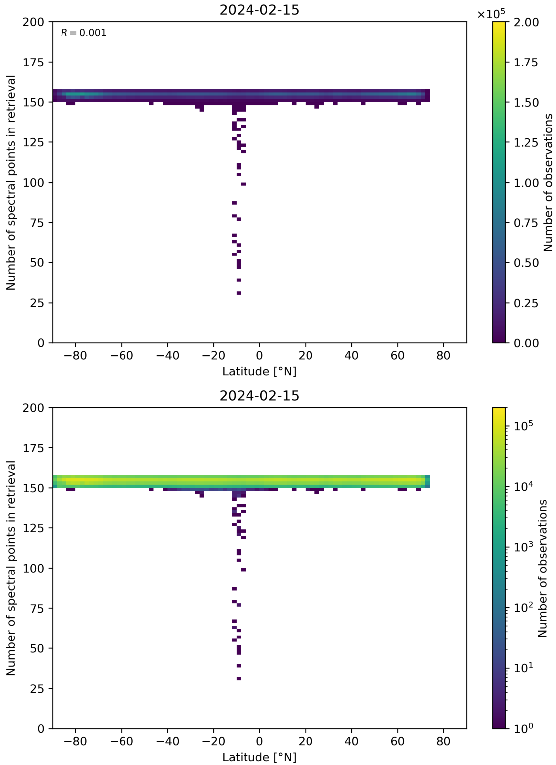
Figure 57: Scatter density plot of “Latitude” against “Number of spectral points in retrieval” for 2024-02-14 to 2024-02-16.
