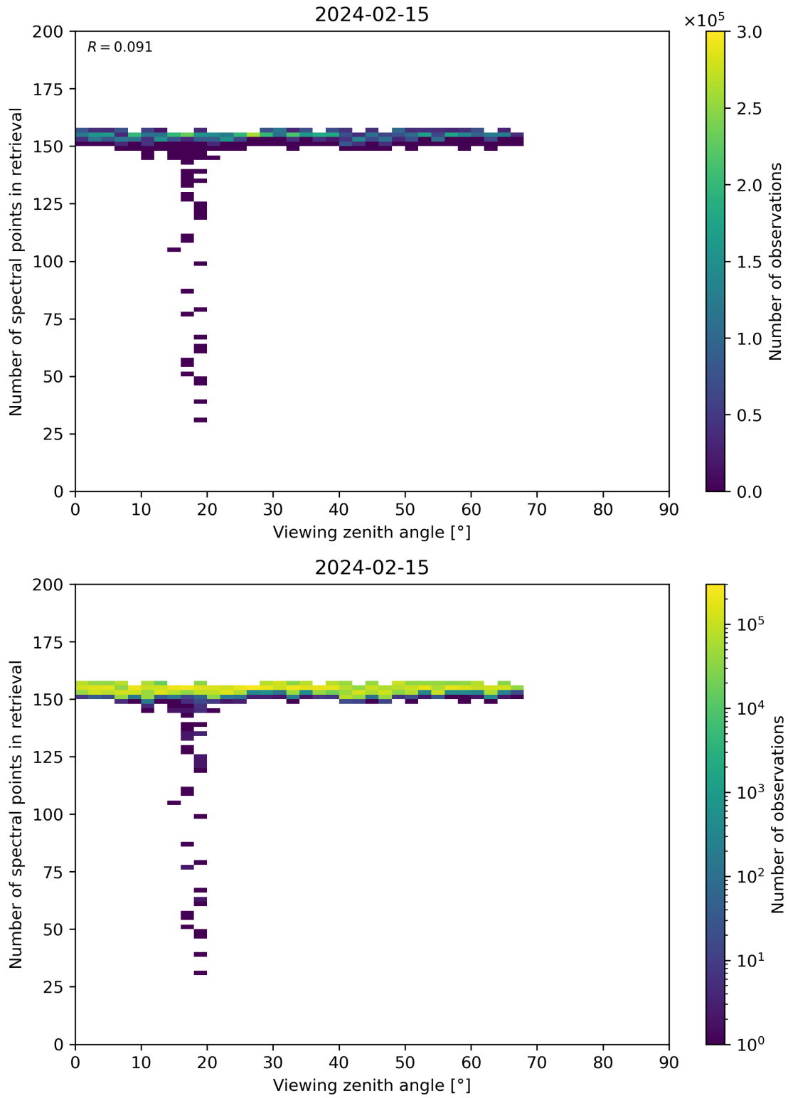
Figure 76: Scatter density plot of “Viewing zenith angle” against “Number of spectral points in retrieval” for 2024-02-14 to 2024-02-16.
