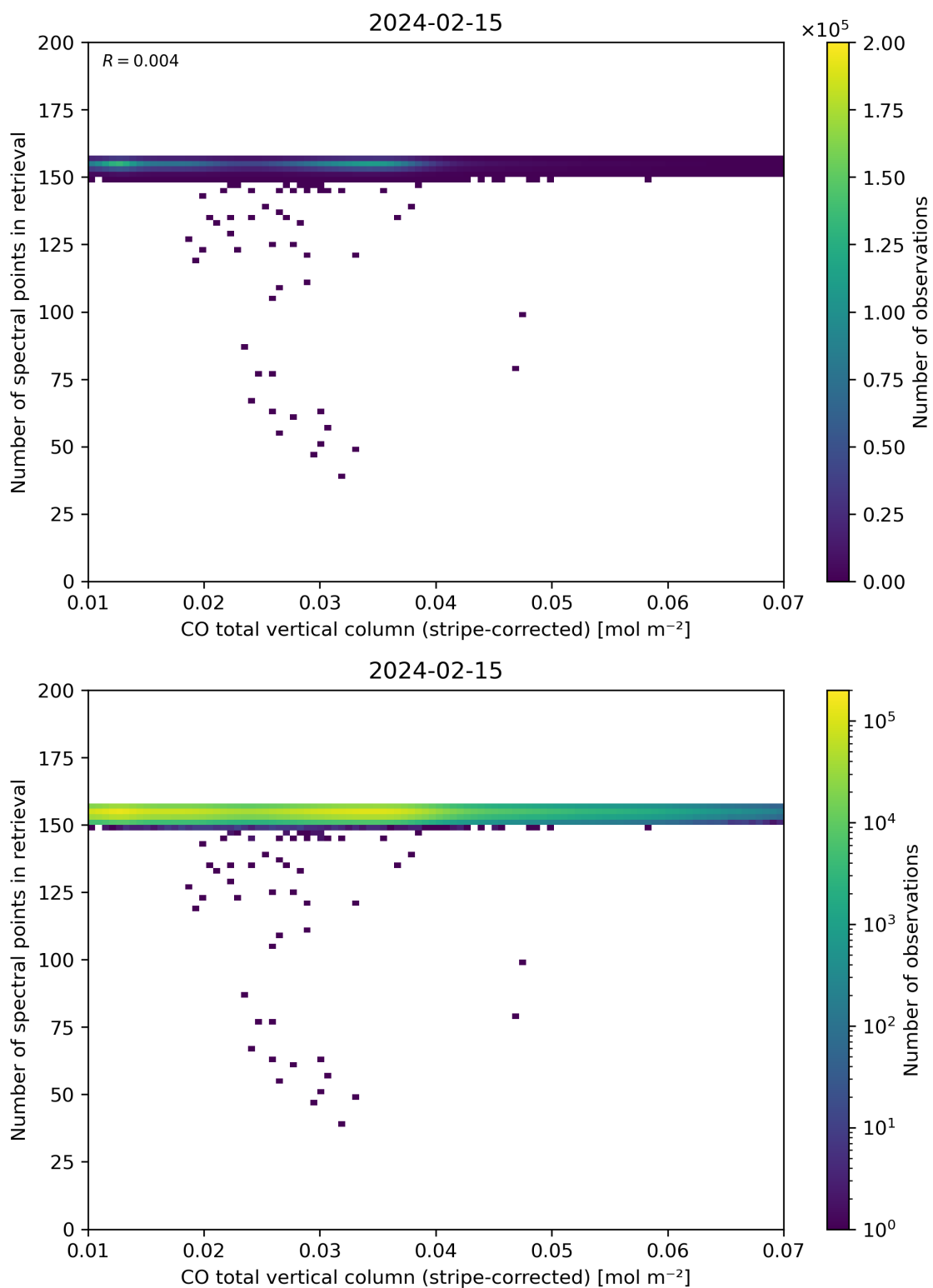
Figure 40: Scatter density plot of “CO total vertical column (stripe-corrected)” against “Number of spectral points in retrieval” for 2024-02-14 to 2024-02-16.
