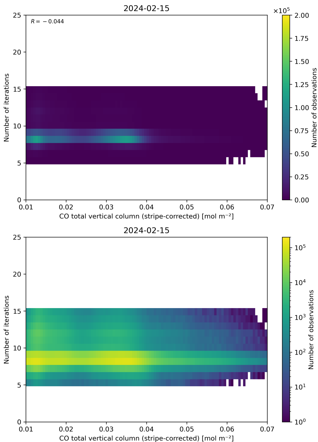
Figure 39: Scatter density plot of “CO total vertical column (stripe-corrected)” against “Number of iterations” for 2024-02-14 to 2024-02-16.
