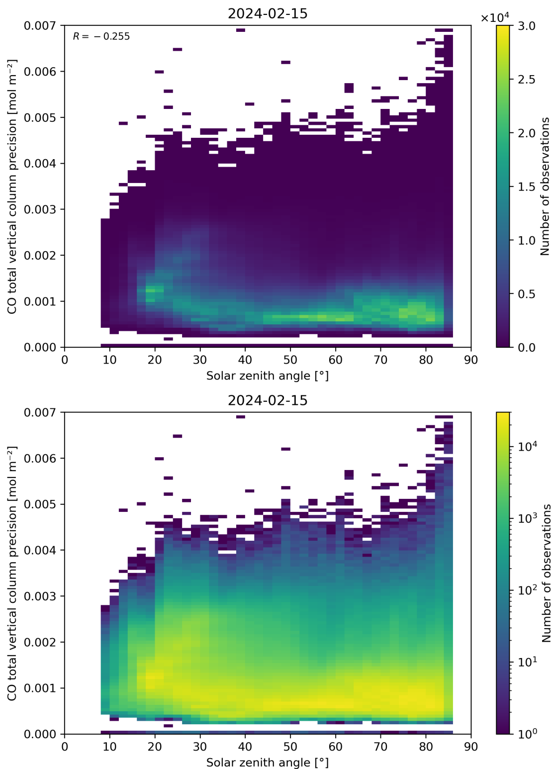
Figure 63: Scatter density plot of “Solar zenith angle” against “CO total vertical column precision” for 2024-02-14 to 2024-02-16.
