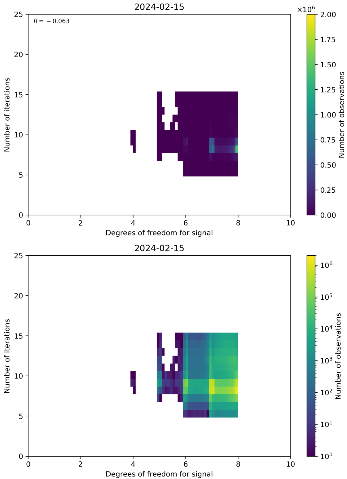
Figure 50: Scatter density plot of “Degrees of freedom for signal” against “Number of iterations” for 2024-02-14 to 2024-02-16.
