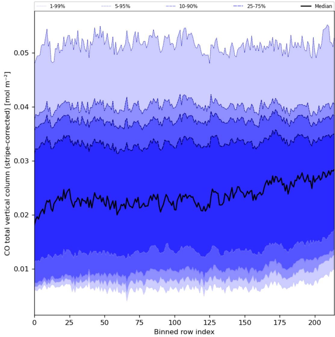
Figure 27: Along track statistics of “CO total vertical column (stripe-corrected)” for 2024-02-14 to 2024-02-16
