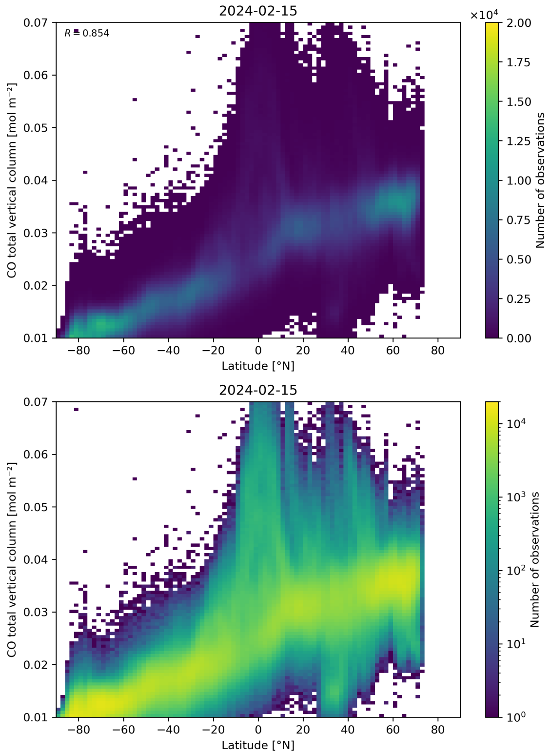
Figure 51: Scatter density plot of “Latitude” against “CO total vertical column” for 2024-02-14 to 2024-02-16.
