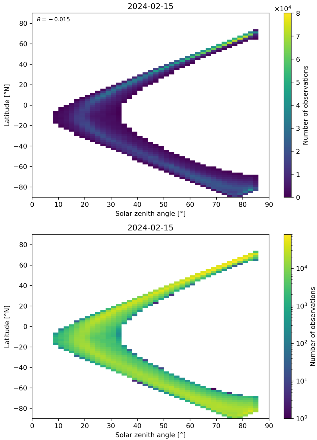
Figure 66: Scatter density plot of “Solar zenith angle” against “Latitude” for 2024-02-14 to 2024-02-16.
