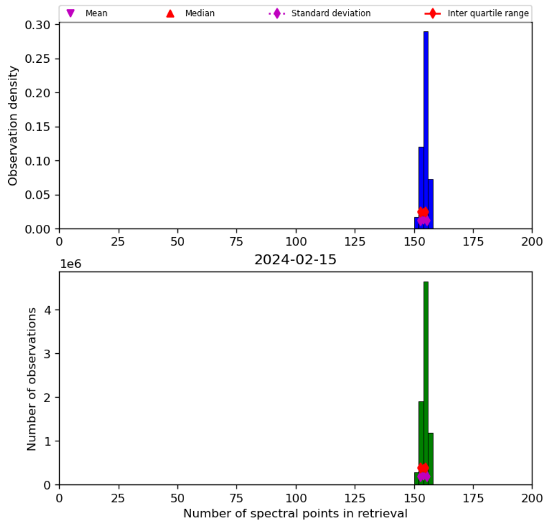
Figure 21: Histogram of “Number of spectral points in retrieval” for 2024-02-14 to 2024-02-16
