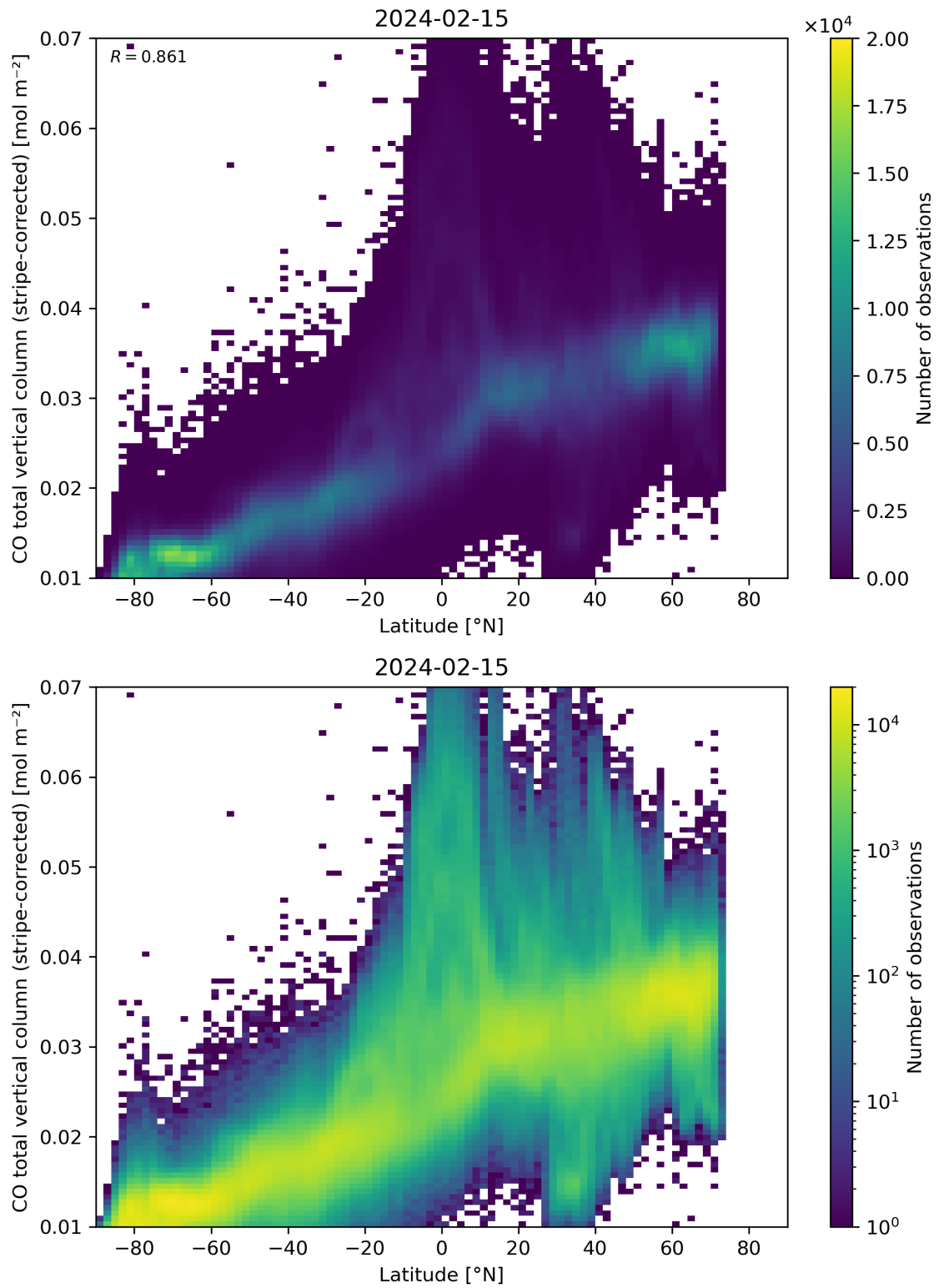
Figure 52: Scatter density plot of “Latitude” against “CO total vertical column (stripe-corrected)” for 2024-02-14 to 2024-02-16.
