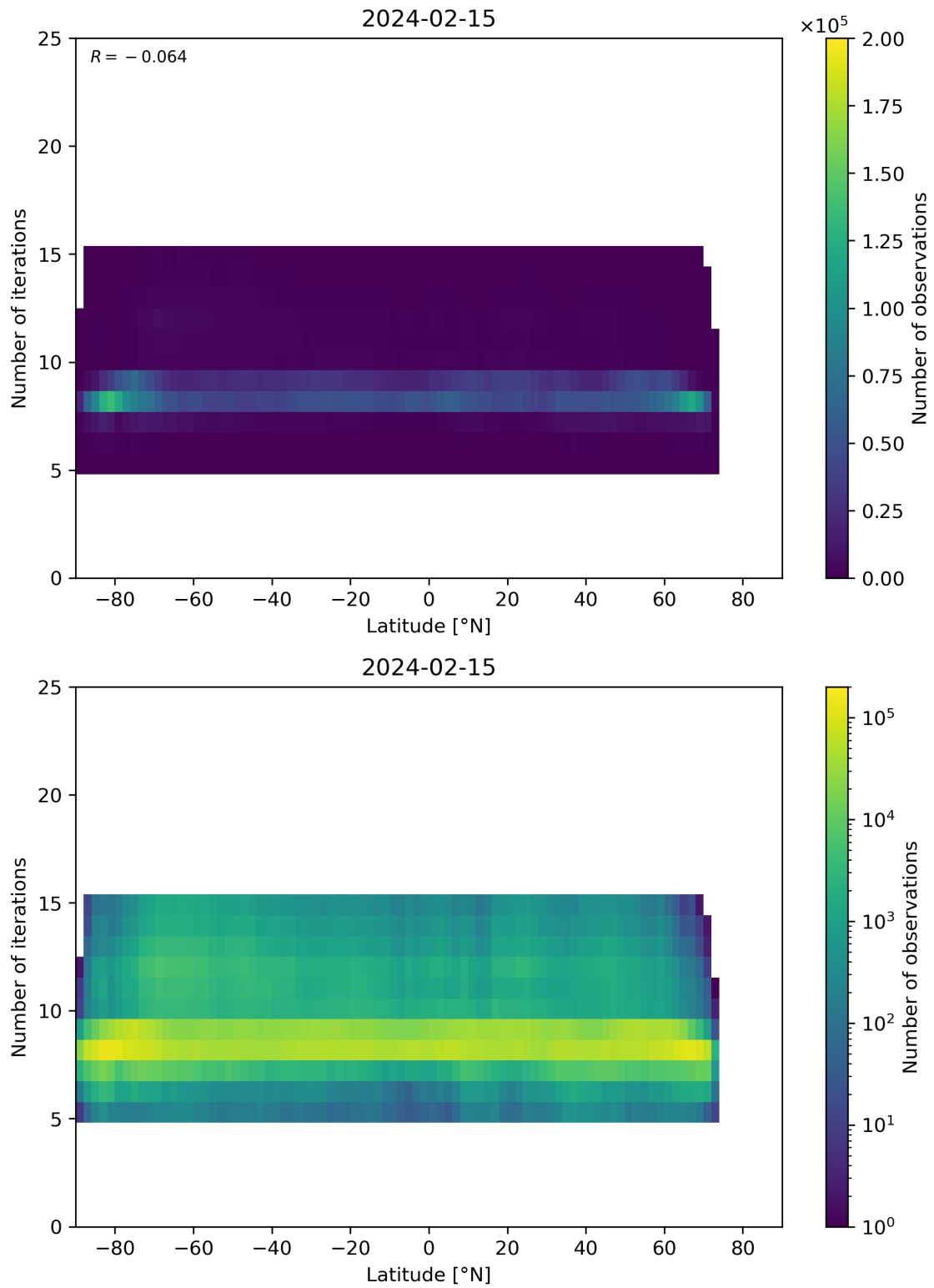
Figure 56: Scatter density plot of “Latitude” against “Number of iterations” for 2024-02-14 to 2024-02-16.
