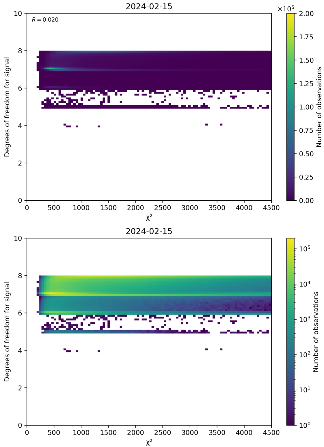
Figure 48: Scatter density plot of “ \chi^2 ” against “Degrees of freedom for signal” for 2024-02-14 to 2024-02-16.
