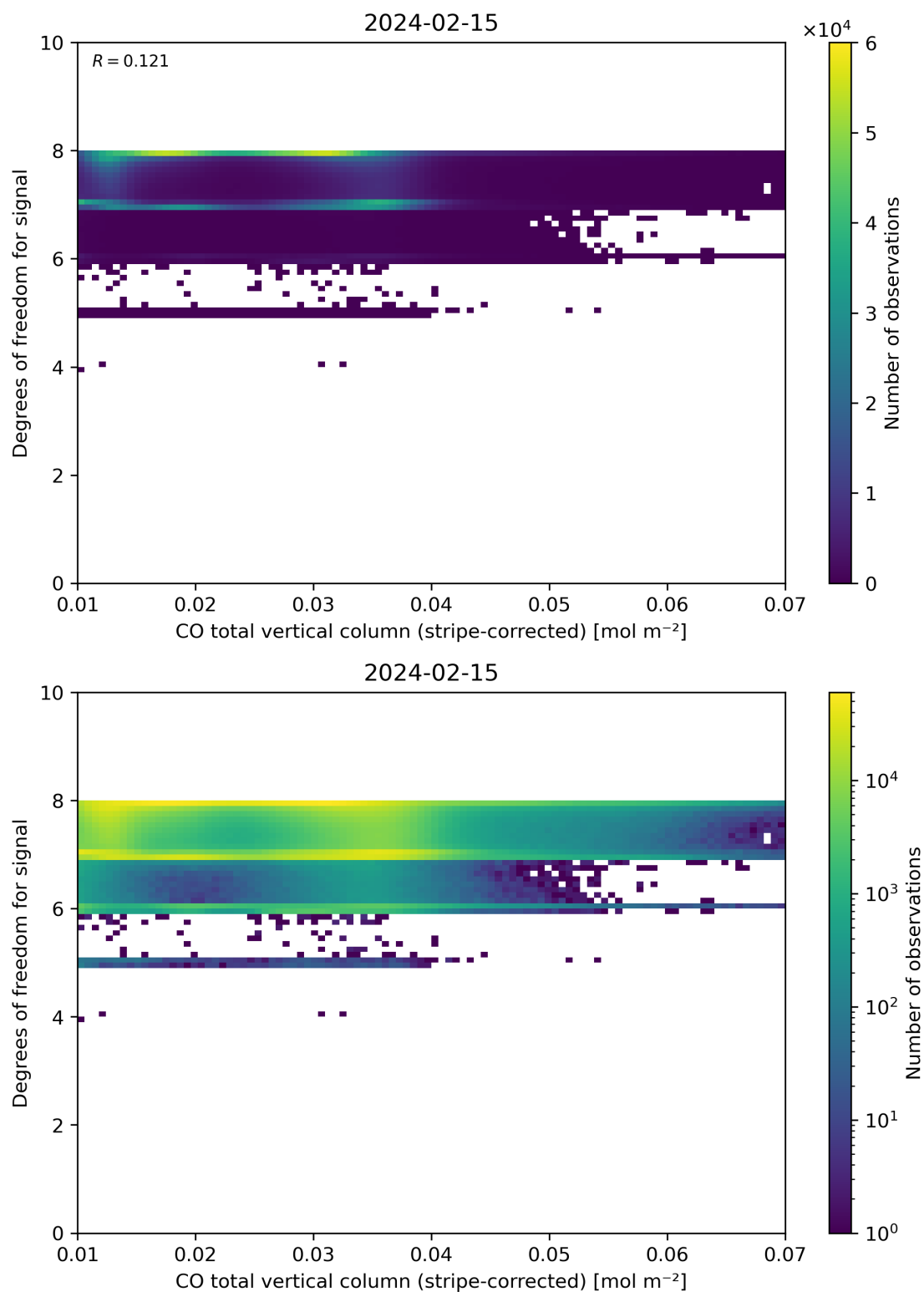
Figure 38: Scatter density plot of “CO total vertical column (stripe-corrected)” against “Degrees of freedom for signal” for 2024-02-14 to 2024-02-16.
