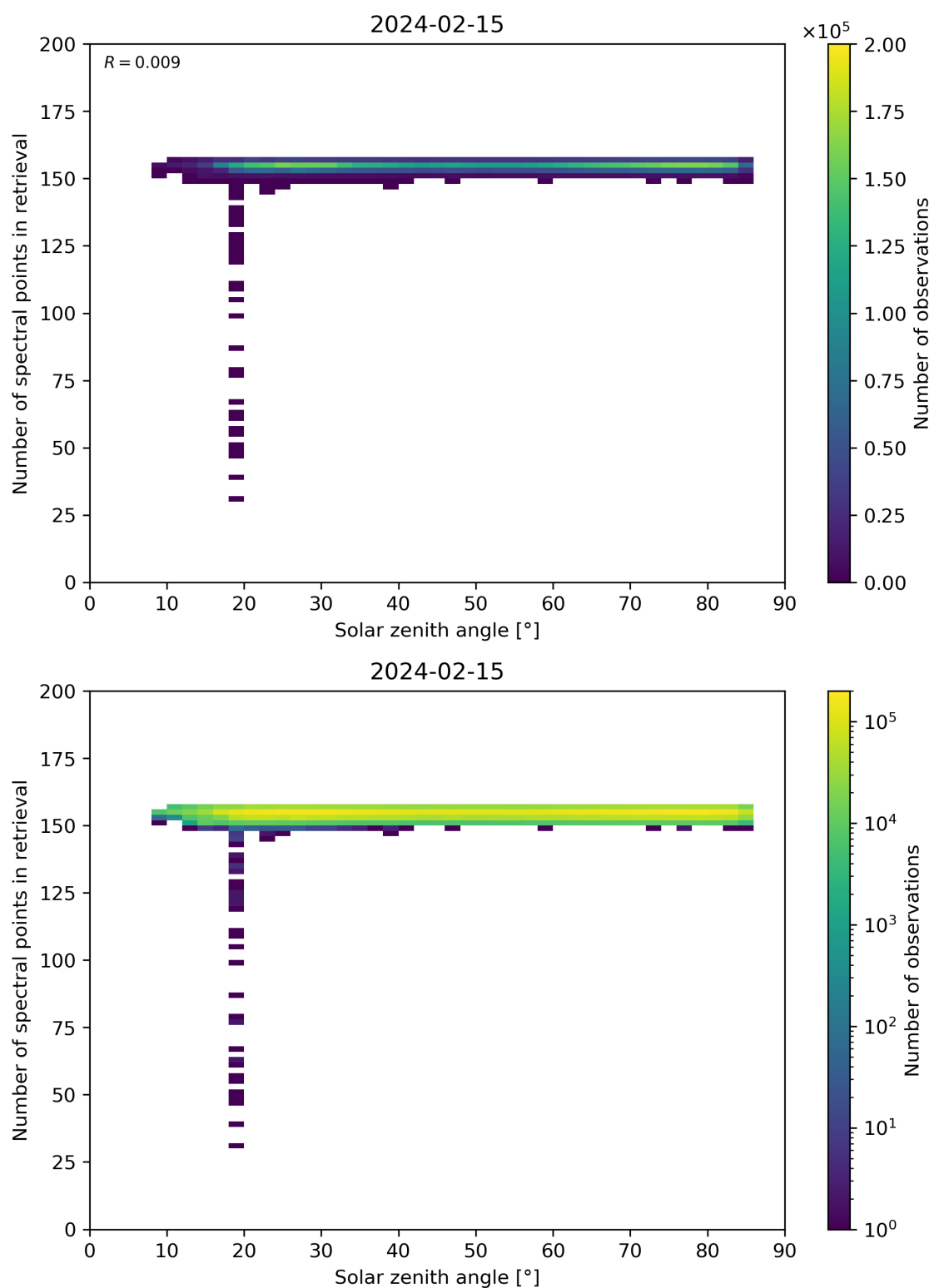
Figure 68: Scatter density plot of “Solar zenith angle” against “Number of spectral points in retrieval” for 2024-02-14 to 2024-02-16.
