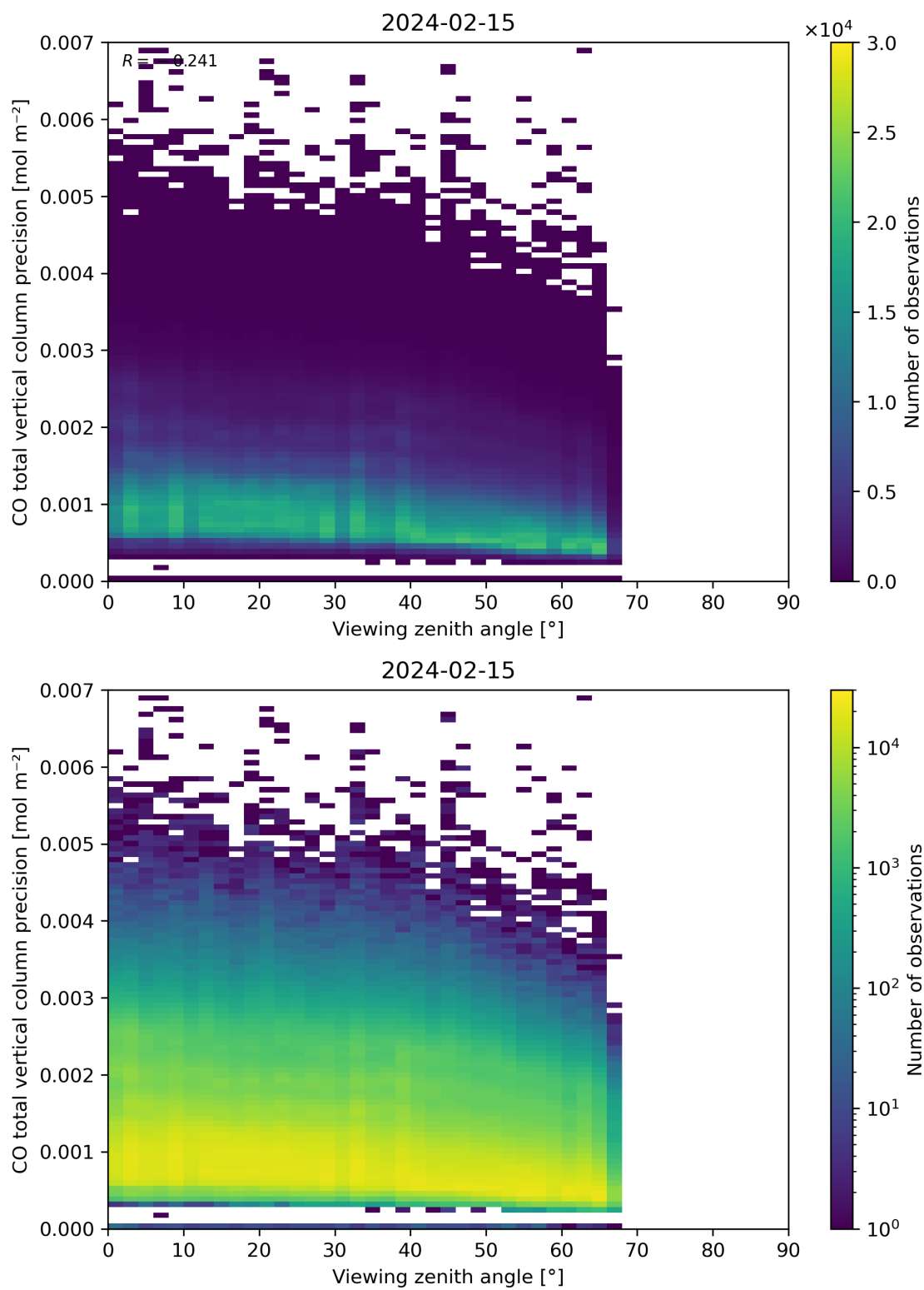
Figure 71: Scatter density plot of “Viewing zenith angle” against “CO total vertical column precision” for 2024-02-14 to 2024-02-16.
