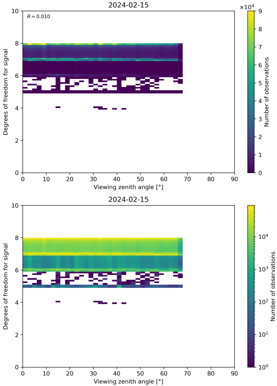
Figure 73: Scatter density plot of “Viewing zenith angle” against “Degrees of freedom for signal” for 2024-02-14 to 2024-02-16.
