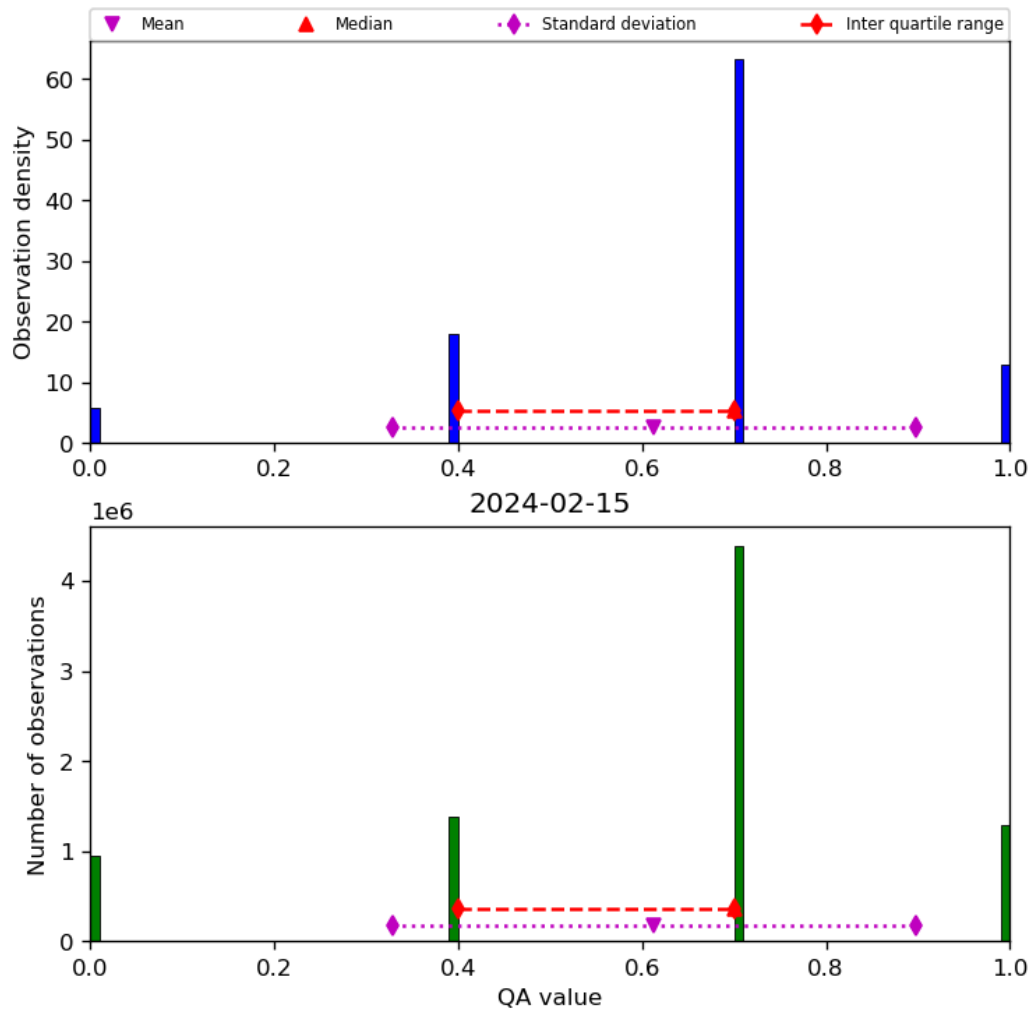
Figure 17: Histogram of “QA value” for 2024-02-14 to 2024-02-16
