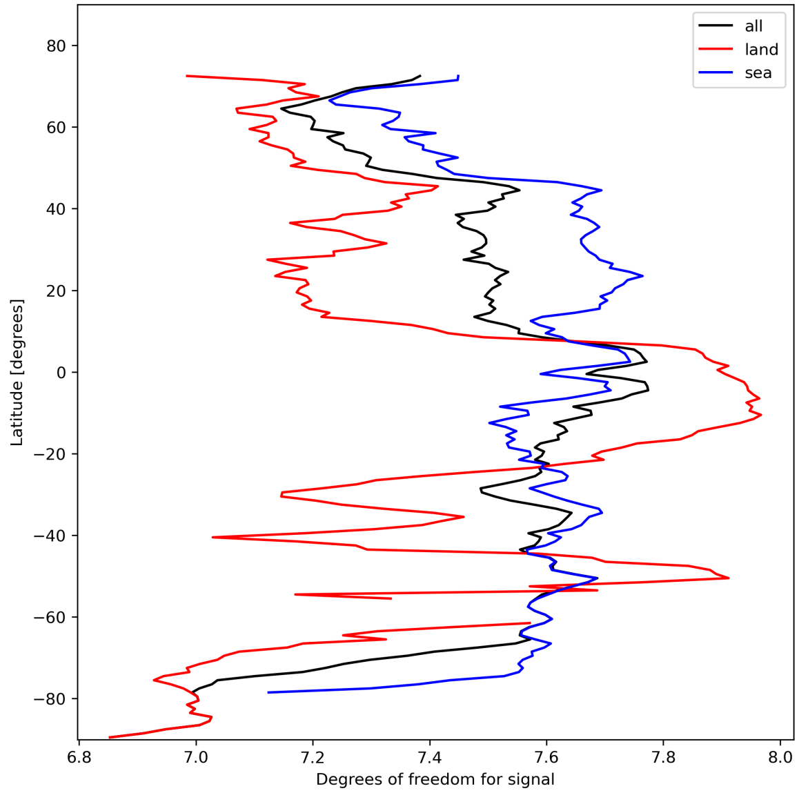
Figure 15: Zonal average of “Degrees of freedom for signal” for 2024-02-14 to 2024-02-16.
