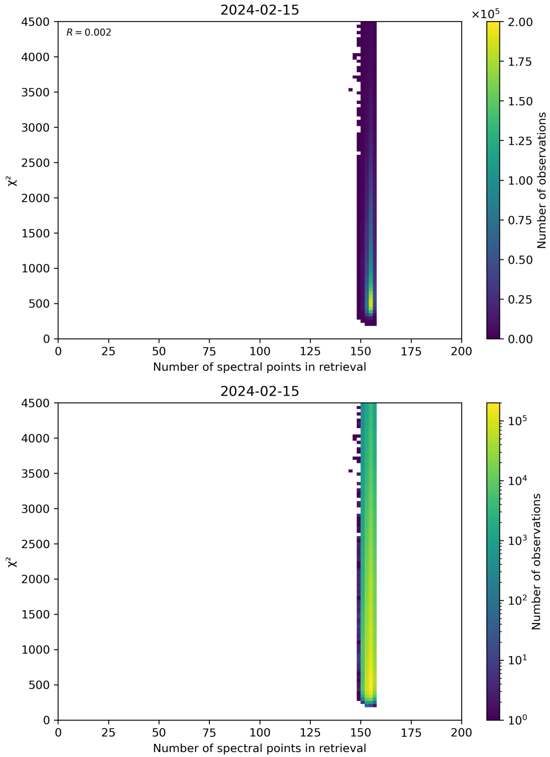
Figure 58: Scatter density plot of “Number of spectral points in retrieval” against “ \chi^2 ” for 2024-02-14 to 2024-02-16.
