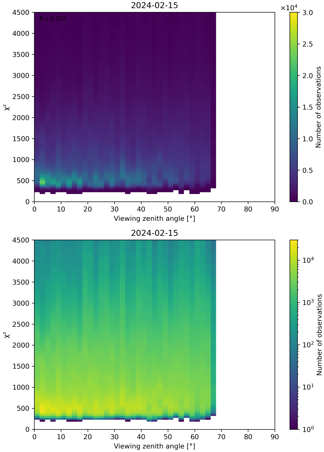
Figure 72: Scatter density plot of “Viewing zenith angle” against “ \chi^2 ” for 2024-02-14 to 2024-02-16.
