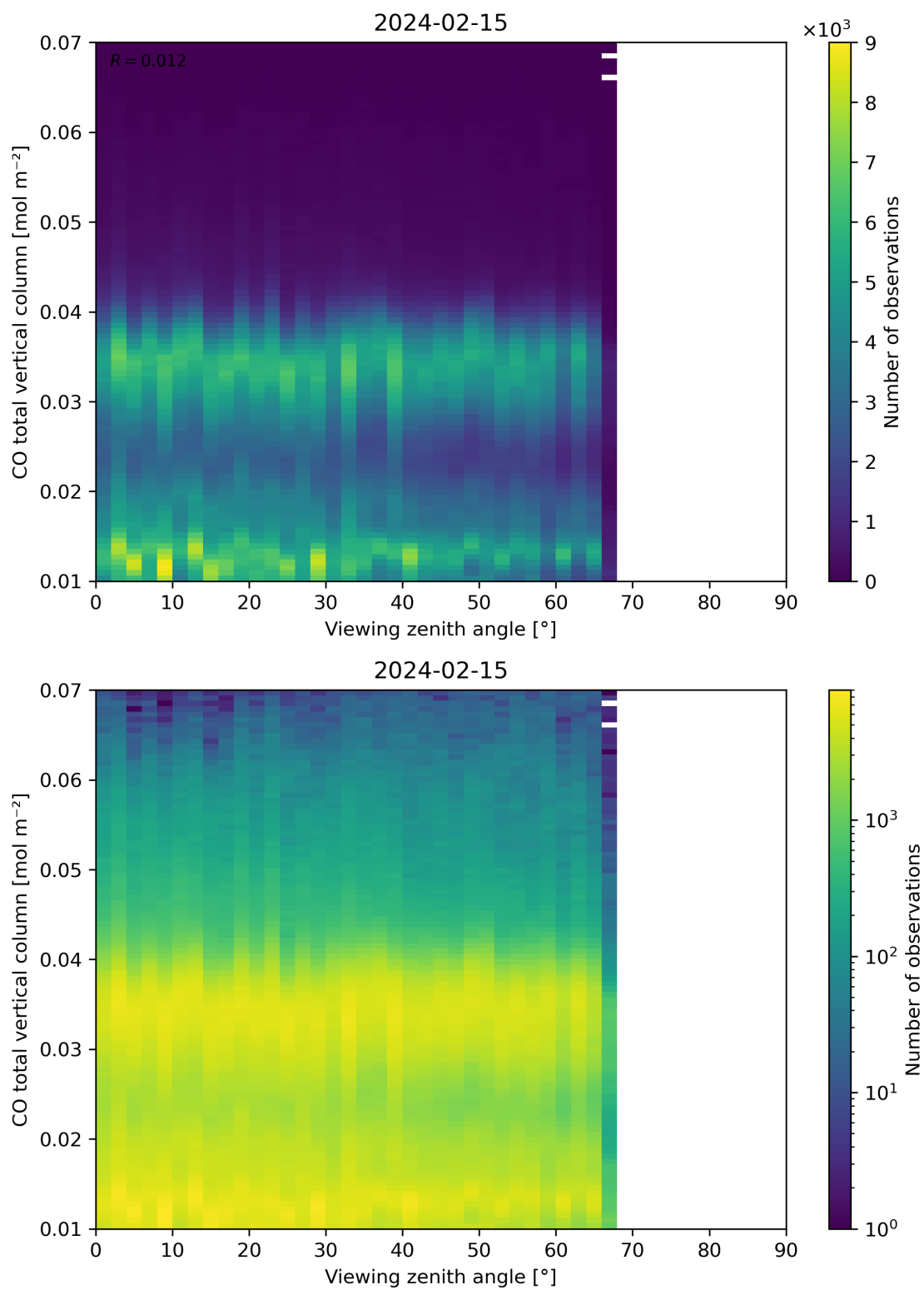
Figure 69: Scatter density plot of “Viewing zenith angle” against “CO total vertical column” for 2024-02-14 to 2024-02-16.
