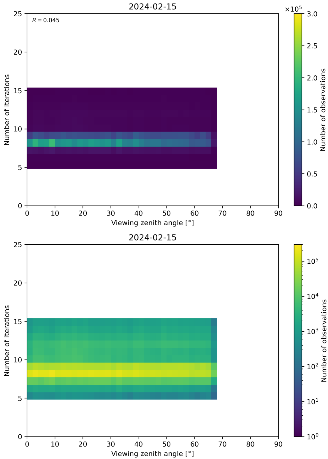
Figure 75: Scatter density plot of “Viewing zenith angle” against “Number of iterations” for 2024-02-14 to 2024-02-16.
