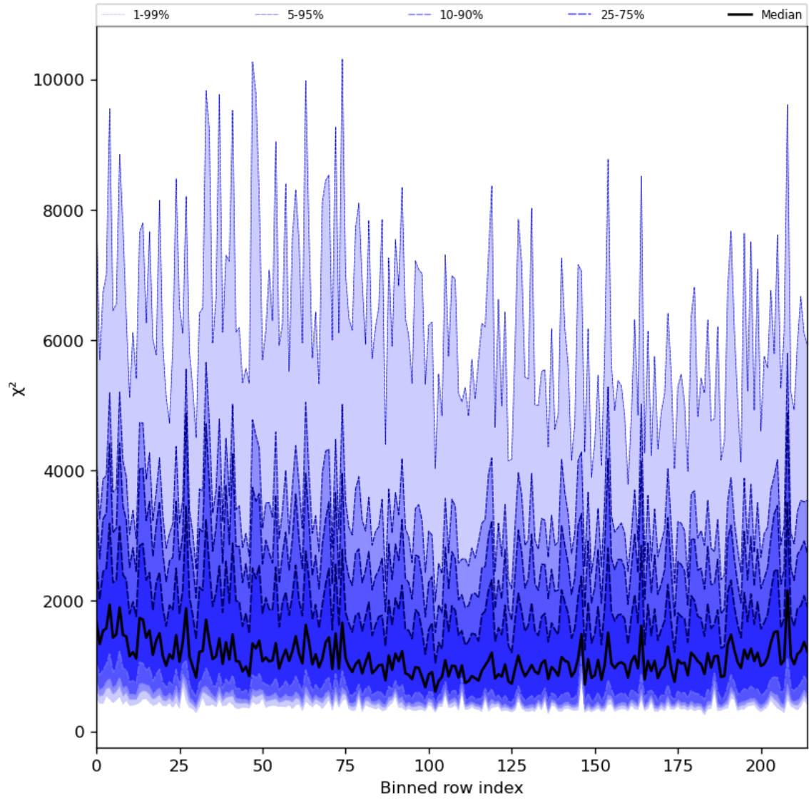
Figure 30: Along track statistics of “ \chi^2 ” for 2024-02-14 to 2024-02-16
