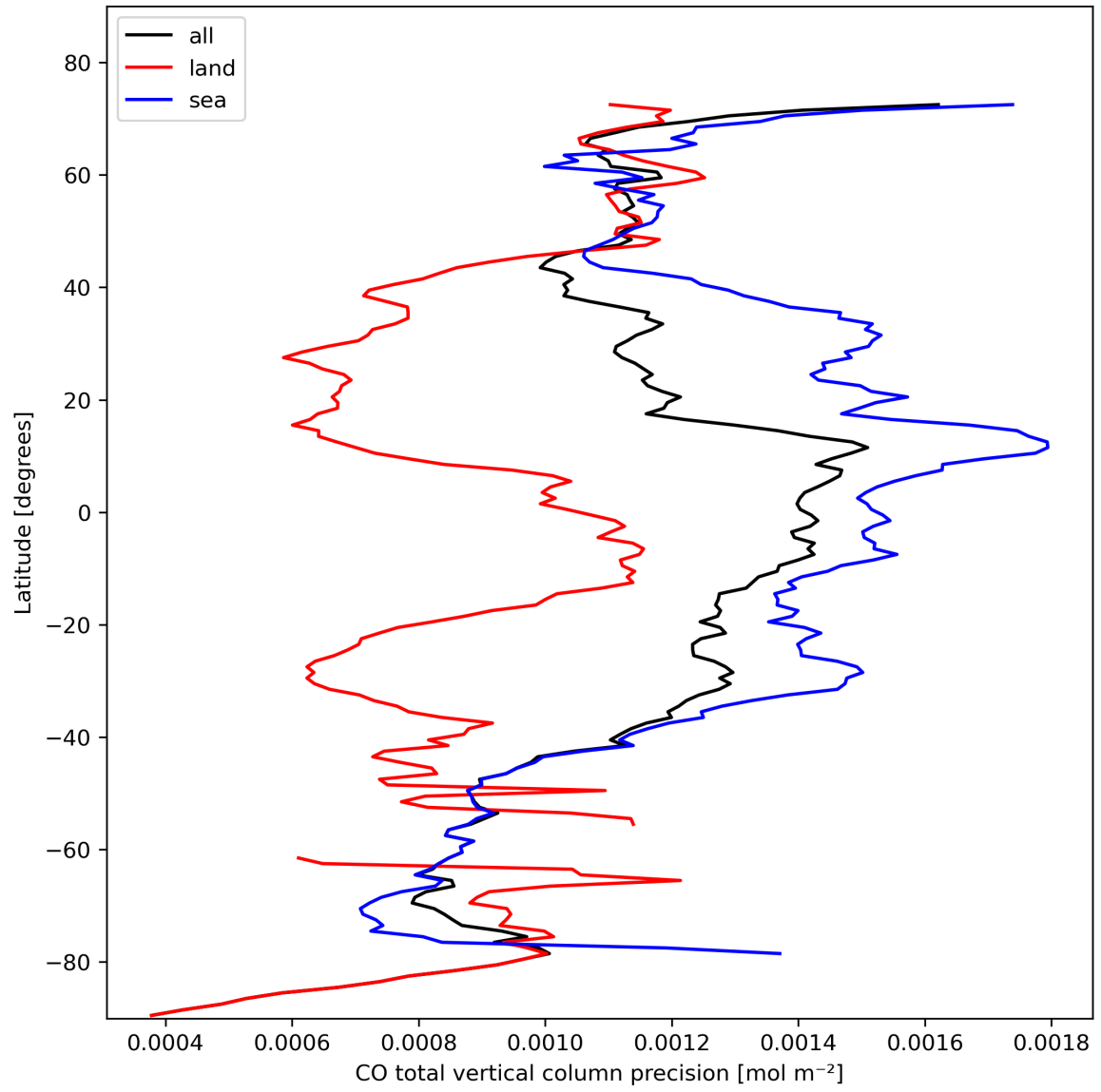
Figure 12: Zonal average of “CO total vertical column precision” for 2024-02-14 to 2024-02-16.
