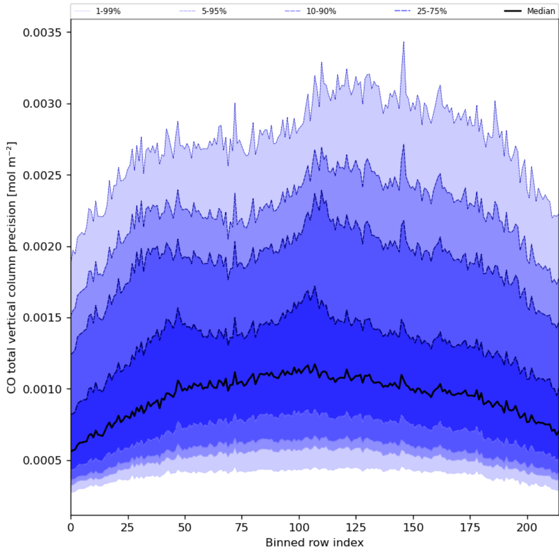
Figure 28: Along track statistics of “CO total vertical column precision” for 2024-02-14 to 2024-02-16
