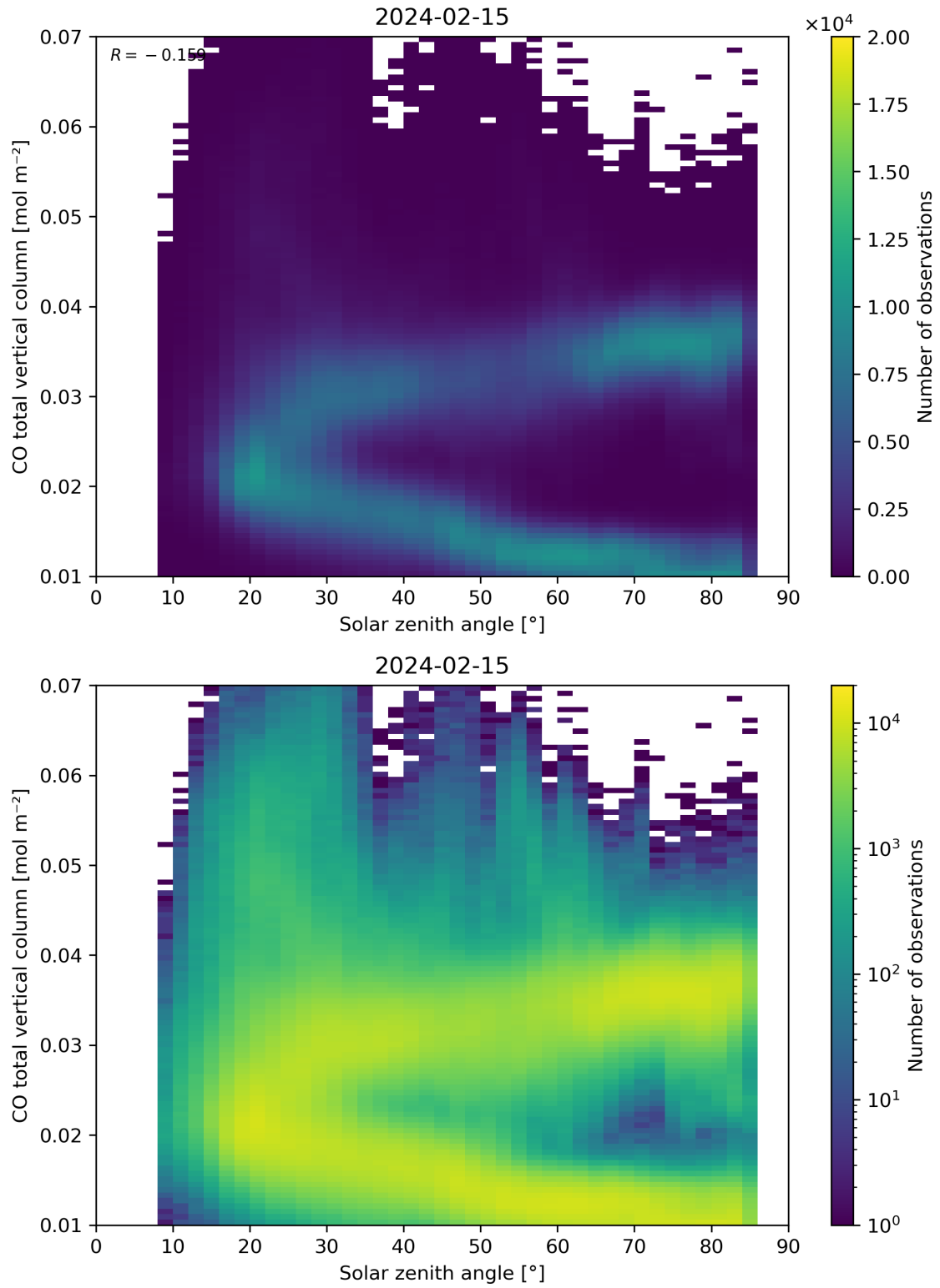
Figure 61: Scatter density plot of “Solar zenith angle” against “CO total vertical column” for 2024-02-14 to 2024-02-16.
