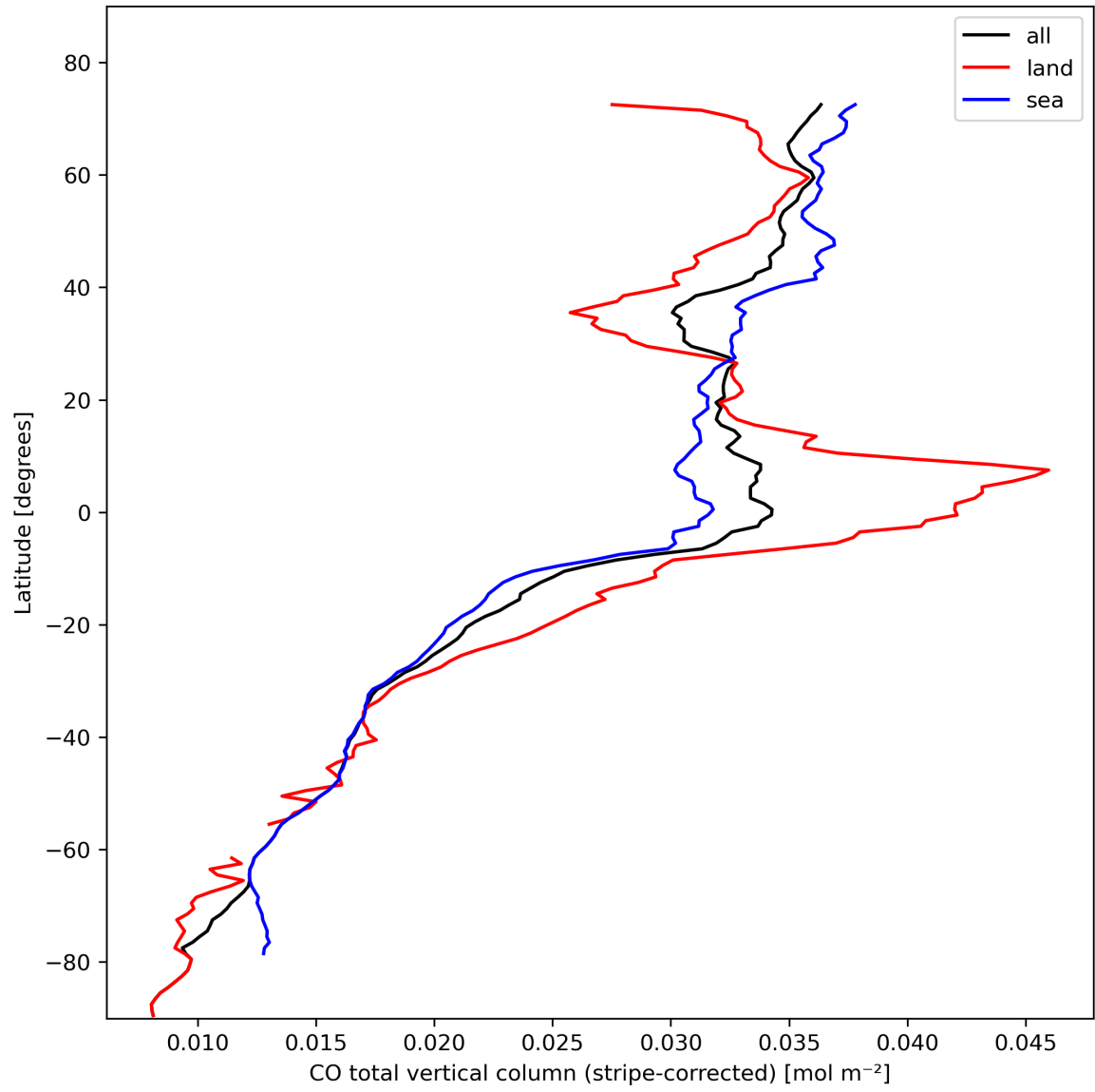
Figure 11: Zonal average of “CO total vertical column (stripe-corrected)” for 2024-02-14 to 2024-02-16.
