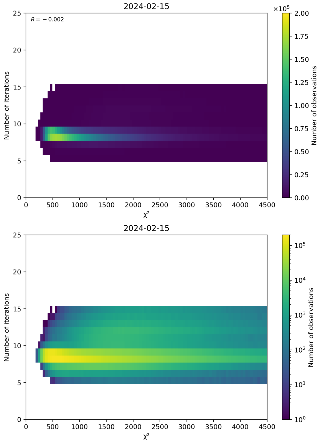
Figure 49: Scatter density plot of “ \chi^2 ” against “Number of iterations” for 2024-02-14 to 2024-02-16.
