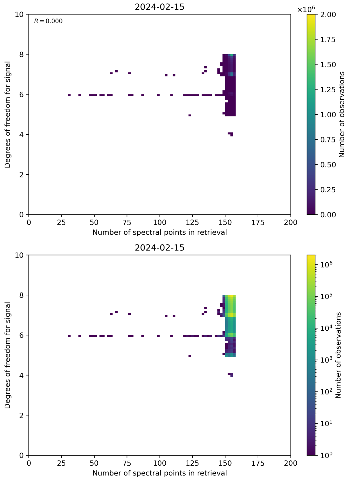
Figure 59: Scatter density plot of “Number of spectral points in retrieval” against “Degrees of freedom for signal” for 2024-02-14 to 2024-02-16.
