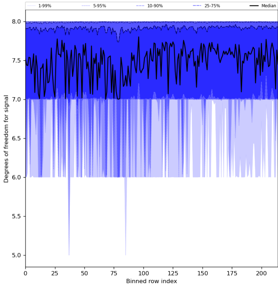
Figure 31: Along track statistics of “Degrees of freedom for signal” for 2024-02-14 to 2024-02-16
