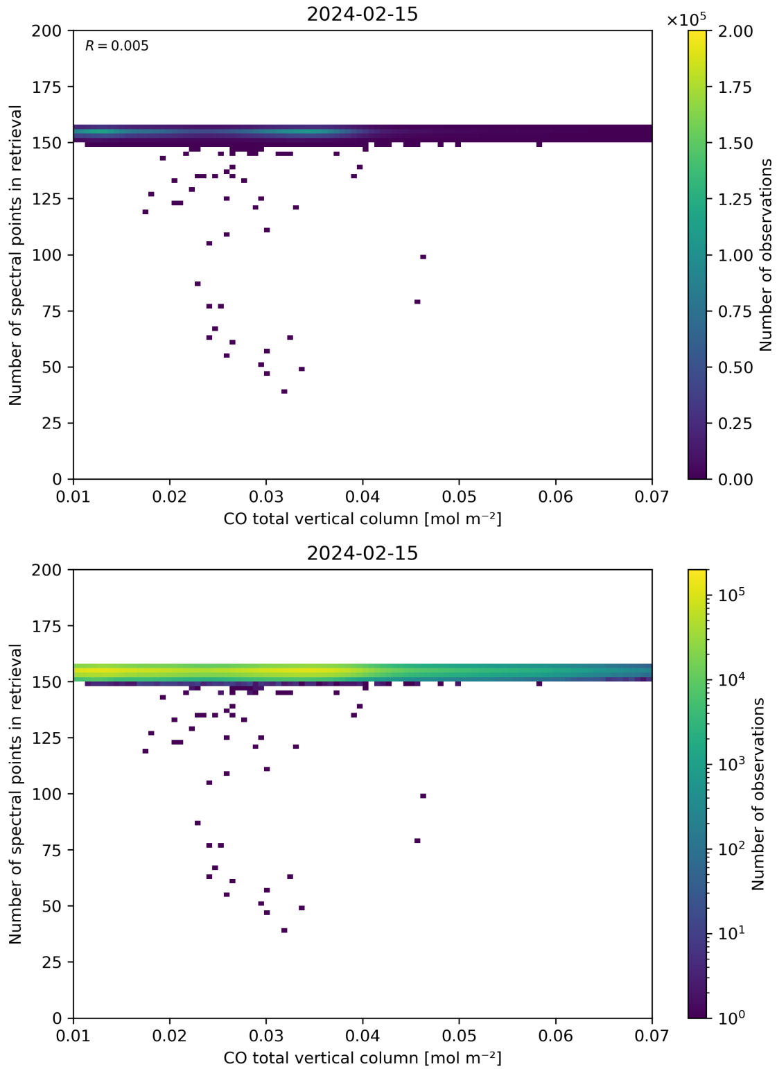
Figure 43: Scatter density plot of “CO total vertical column” against “Number of spectral points in retrieval” for 2024-02-14 to 2024-02-16.
