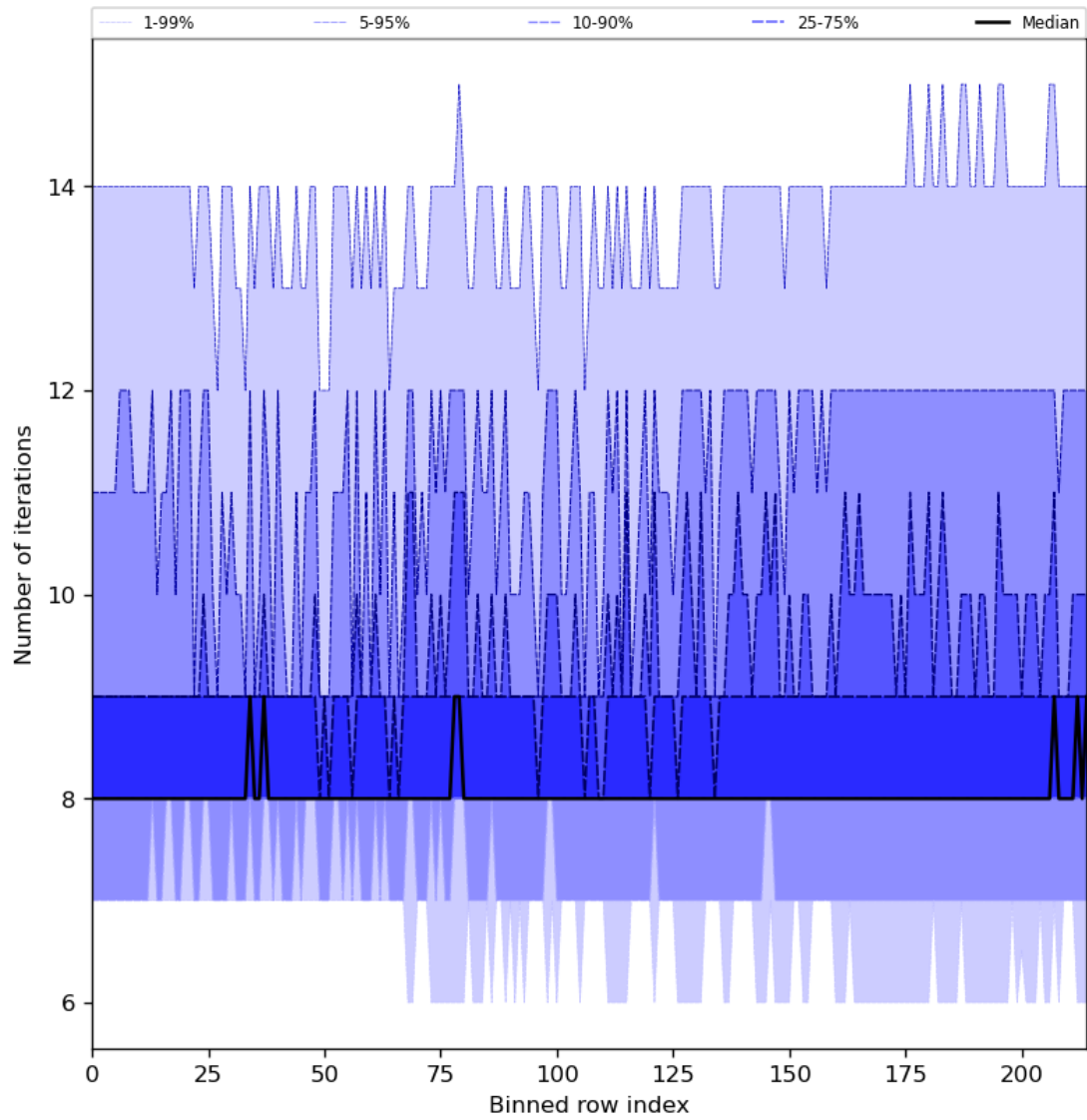
Figure 32: Along track statistics of “Number of iterations” for 2024-02-16 to 2024-02-17
