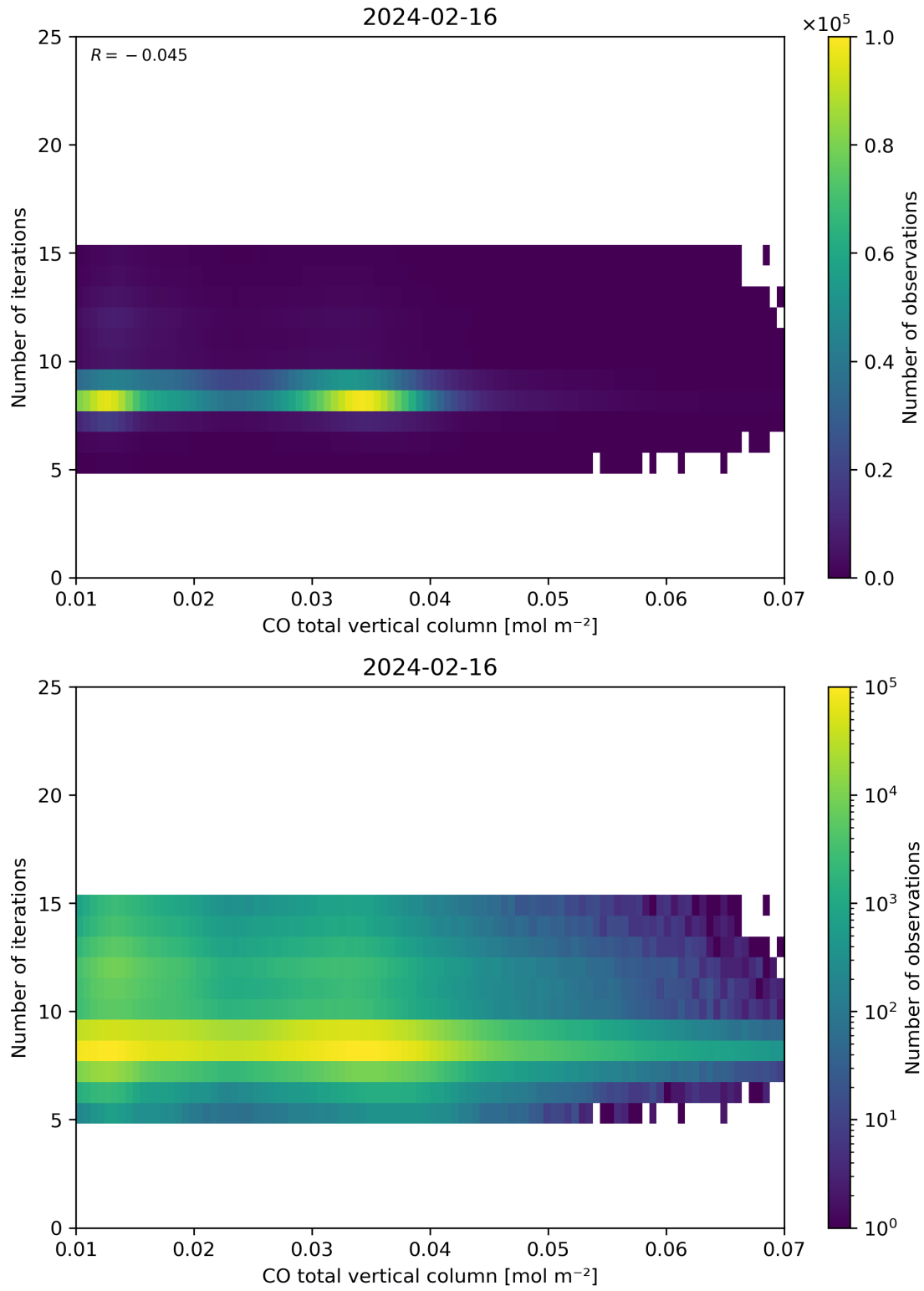
Figure 42: Scatter density plot of “CO total vertical column” against “Number of iterations” for 2024-02-16 to 2024-02-17.
