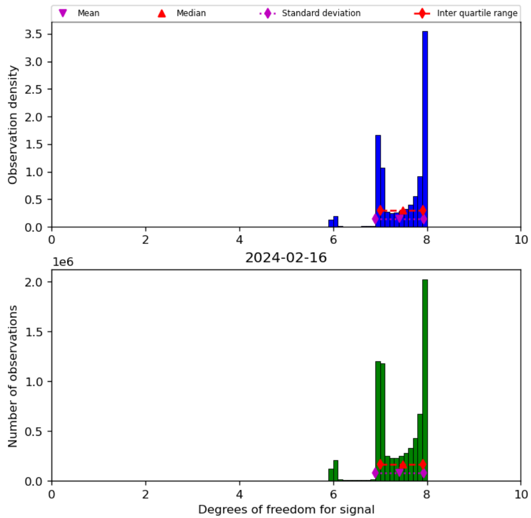
Figure 23: Histogram of “Degrees of freedom for signal” for 2024-02-16 to 2024-02-17
