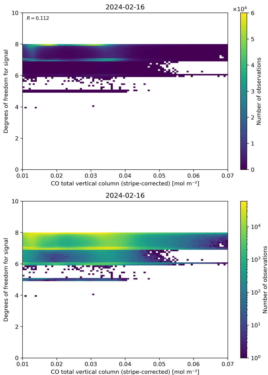
Figure 38: Scatter density plot of “CO total vertical column (stripe-corrected)” against “Degrees of freedom for signal” for 2024-02-16 to 2024-02-17.
