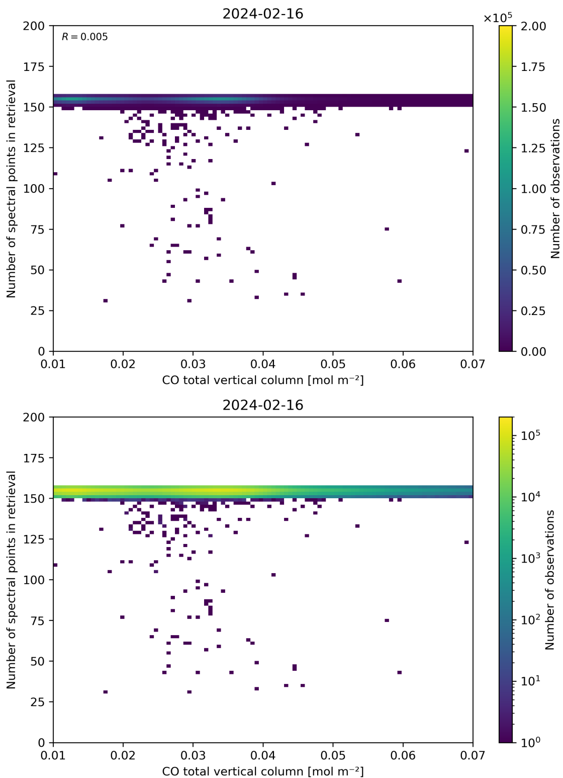
Figure 43: Scatter density plot of “CO total vertical column” against “Number of spectral points in retrieval” for 2024-02-16 to 2024-02-17.
