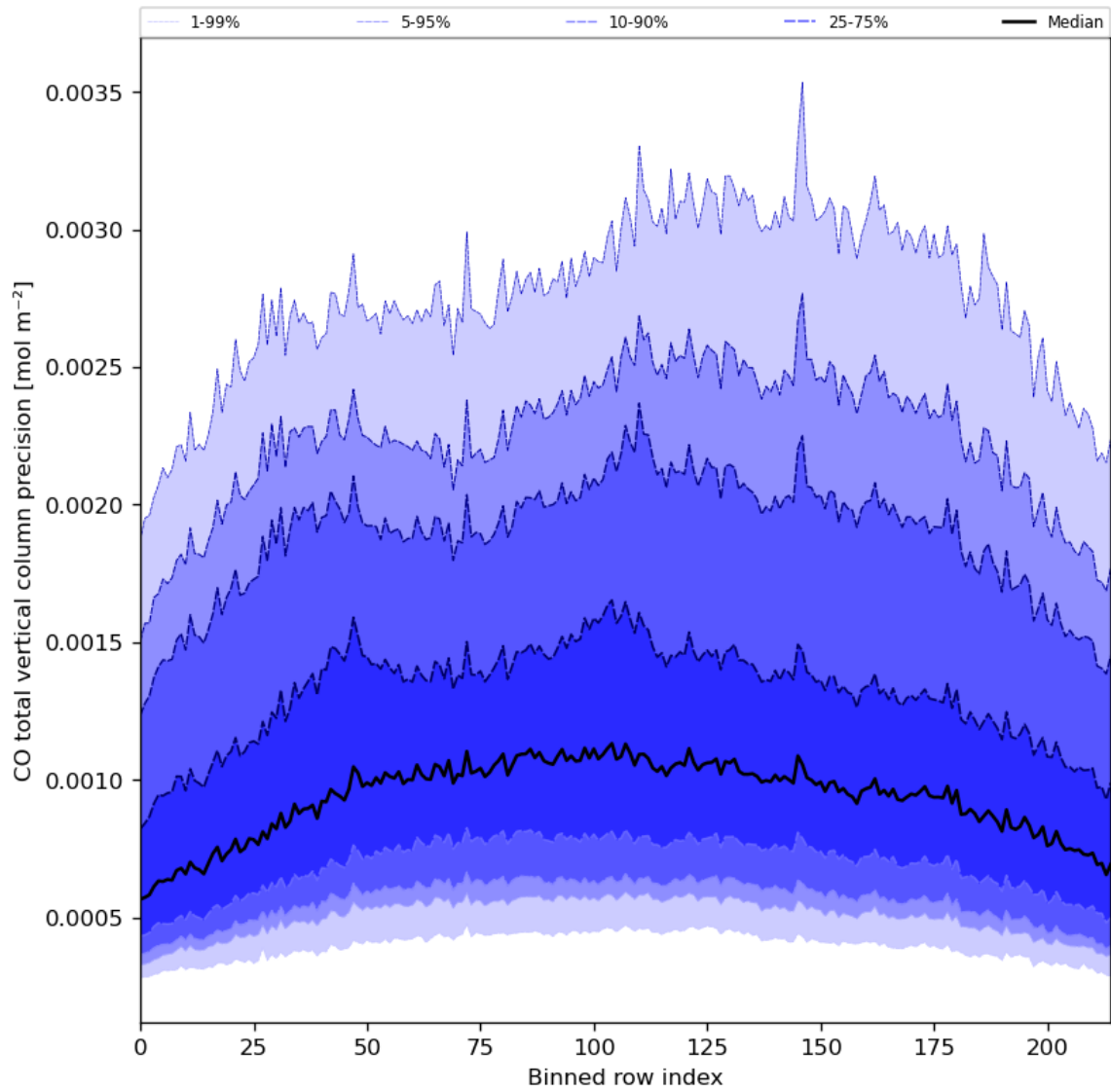
Figure 28: Along track statistics of “CO total vertical column precision” for 2024-02-16 to 2024-02-17
