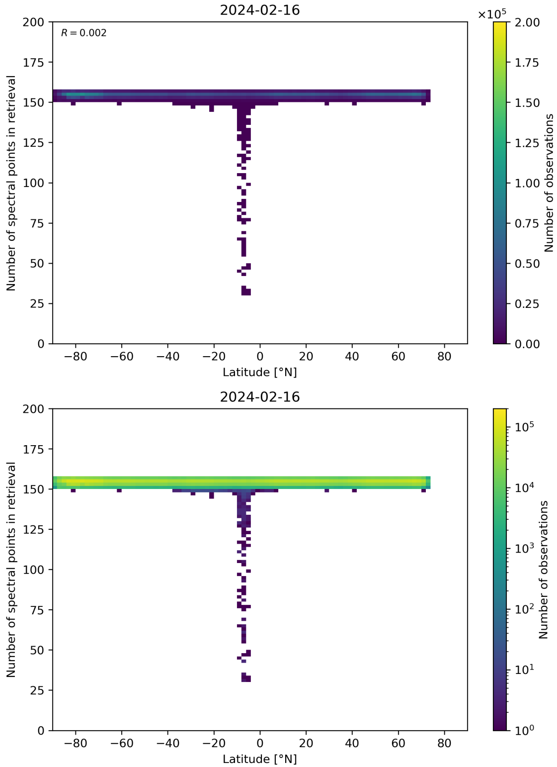
Figure 57: Scatter density plot of “Latitude” against “Number of spectral points in retrieval” for 2024-02-16 to 2024-02-17.
