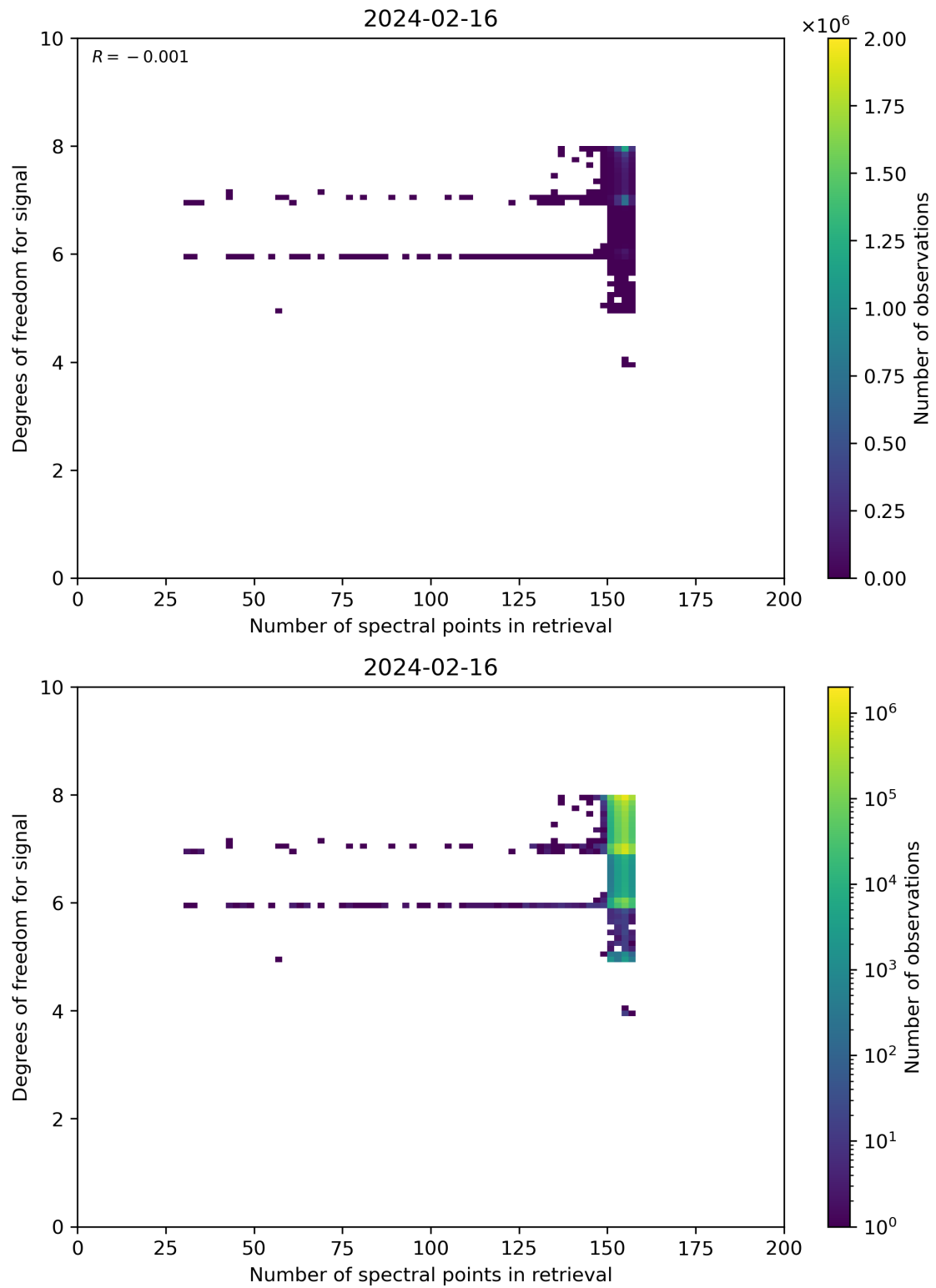
Figure 59: Scatter density plot of “Number of spectral points in retrieval” against “Degrees of freedom for signal” for 2024-02-16 to 2024-02-17.
