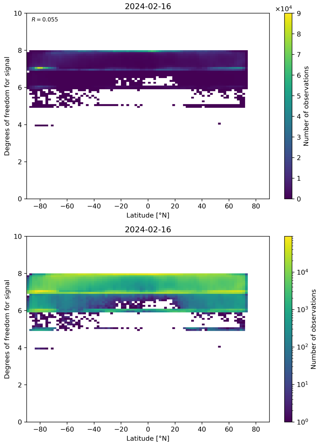
Figure 55: Scatter density plot of “Latitude” against “Degrees of freedom for signal” for 2024-02-16 to 2024-02-17.
