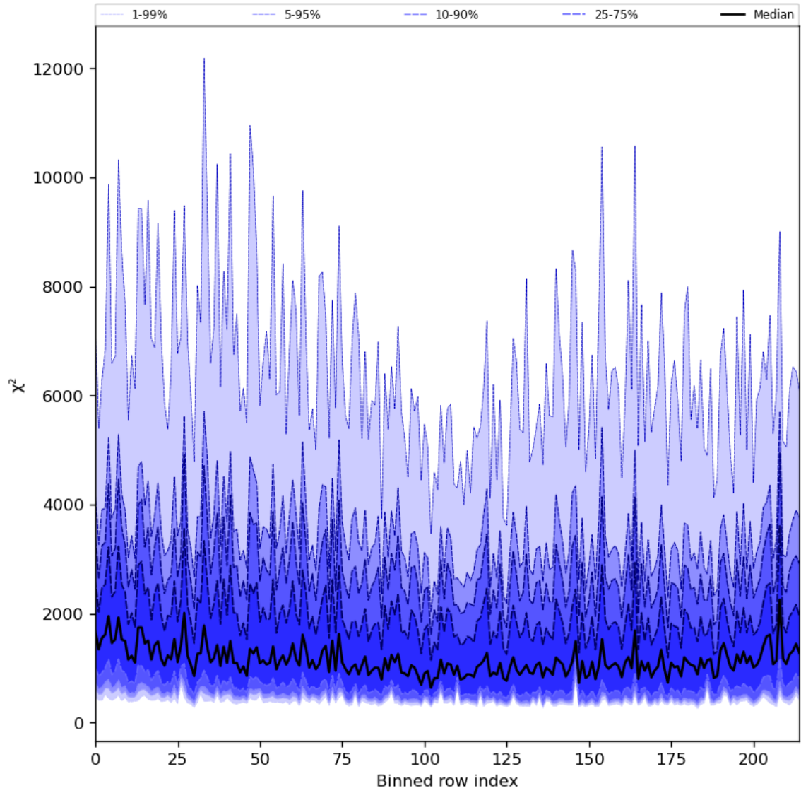
Figure 30: Along track statistics of “ \chi^2 ” for 2024-02-16 to 2024-02-17
