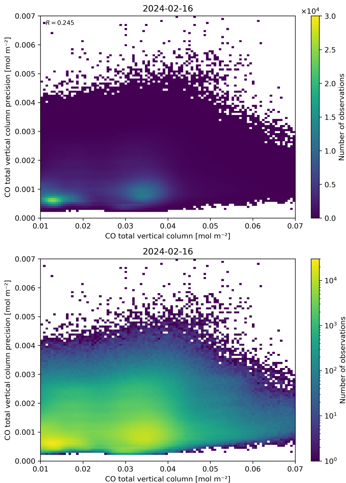
Figure 34: Scatter density plot of “CO total vertical column” against “CO total vertical column precision” for 2024-02-16 to 2024-02-17.
