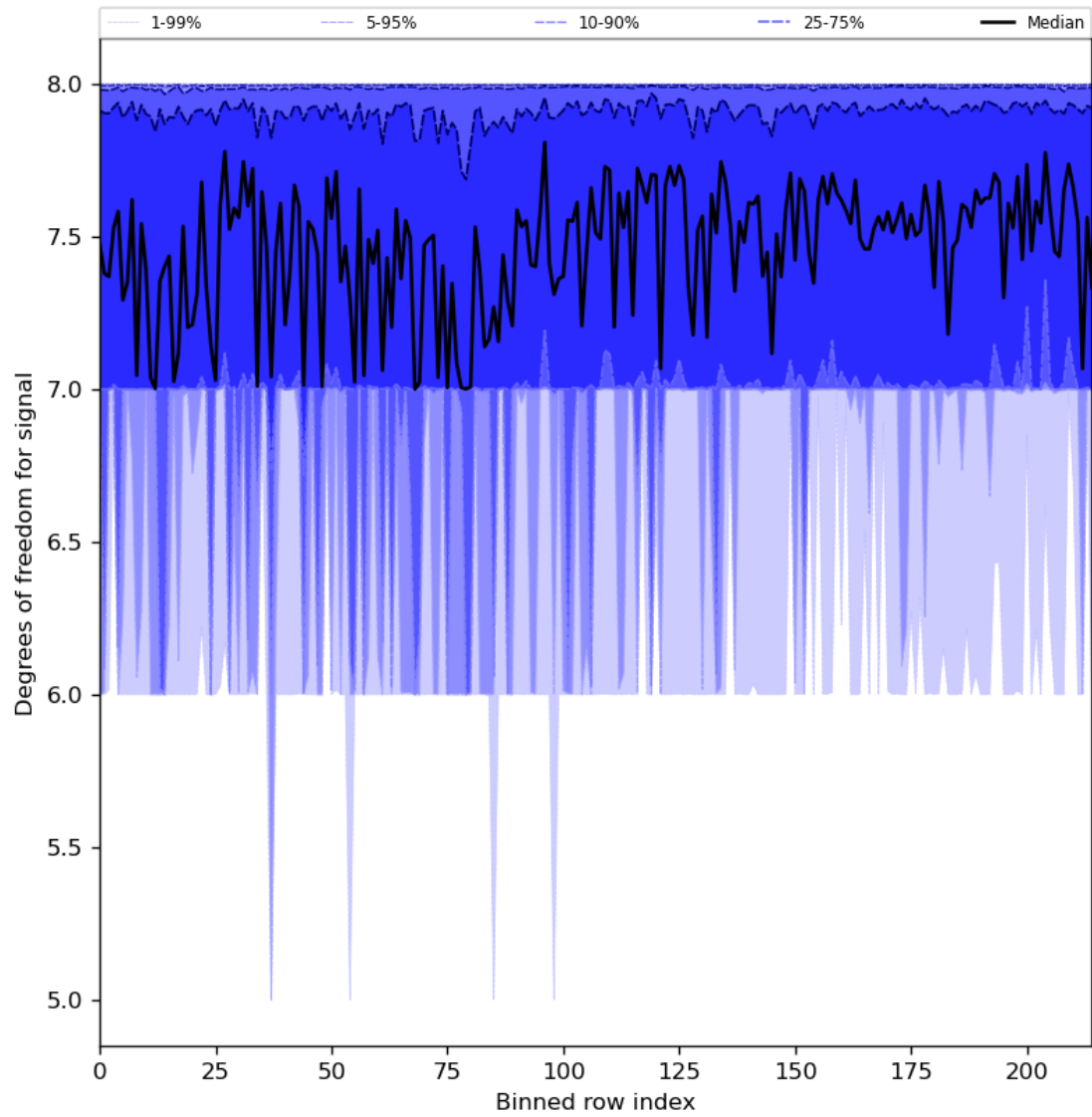
Figure 31: Along track statistics of “Degrees of freedom for signal” for 2024-02-16 to 2024-02-17
