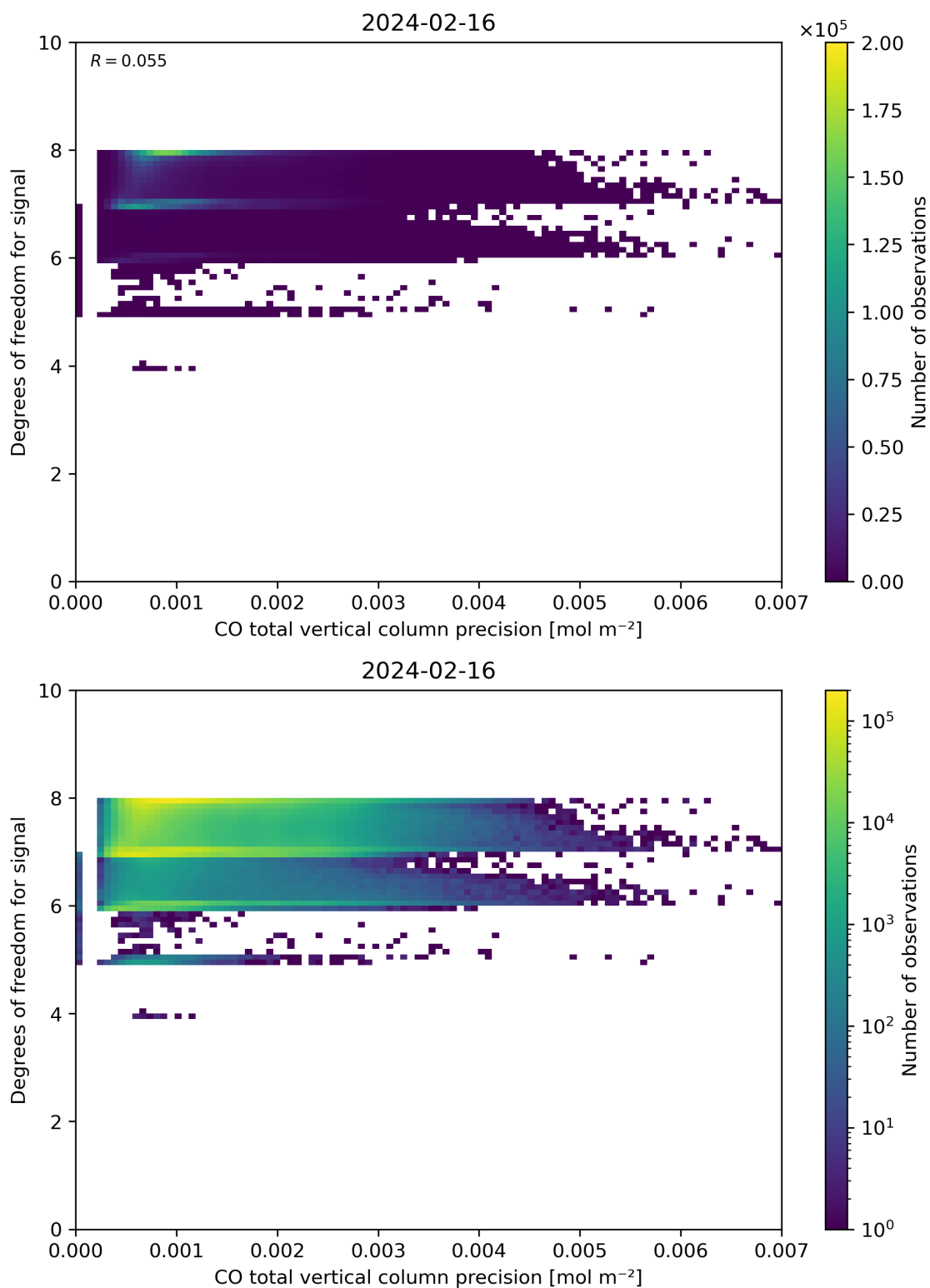
Figure 45: Scatter density plot of “CO total vertical column precision” against “Degrees of freedom for signal” for 2024-02-16 to 2024-02-17.
