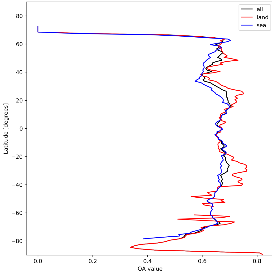
Figure 9: Zonal average of “QA value” for 2024-02-16 to 2024-02-17.
