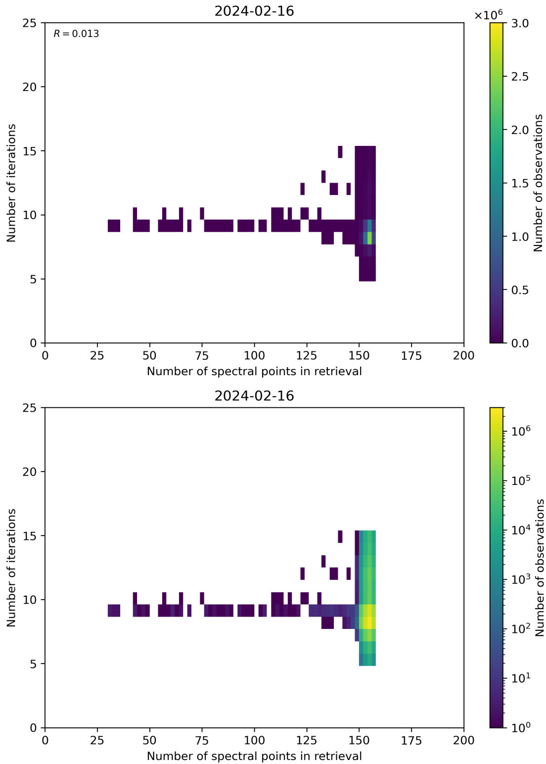
Figure 60: Scatter density plot of “Number of spectral points in retrieval” against “Number of iterations” for 2024-02-16 to 2024-02-17.
