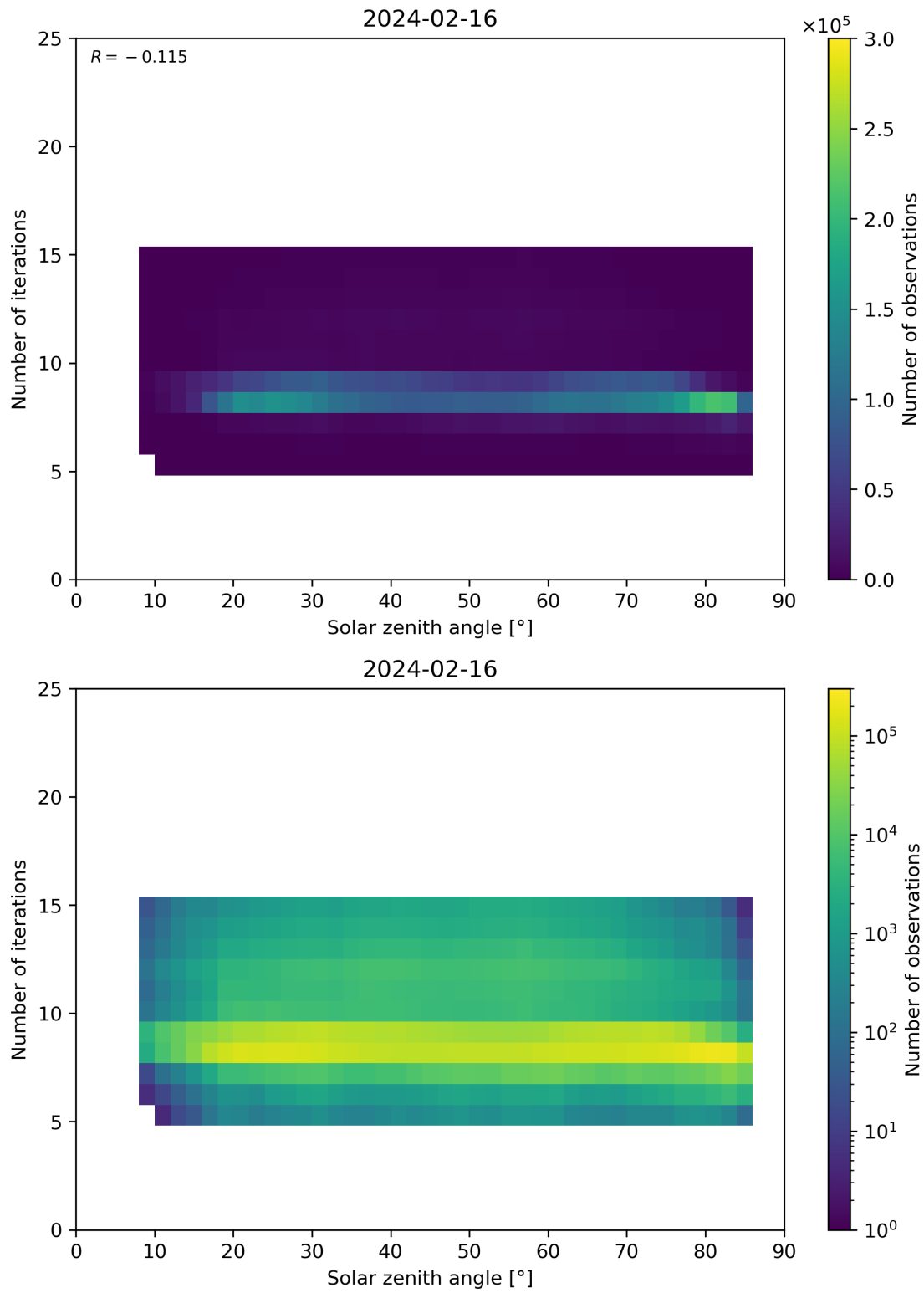
Figure 67: Scatter density plot of “Solar zenith angle” against “Number of iterations” for 2024-02-16 to 2024-02-17.
