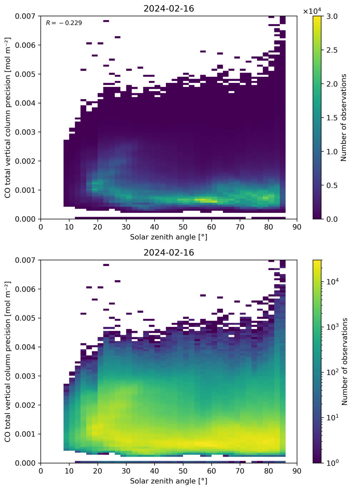
Figure 63: Scatter density plot of “Solar zenith angle” against “CO total vertical column precision” for 2024-02-16 to 2024-02-17.
