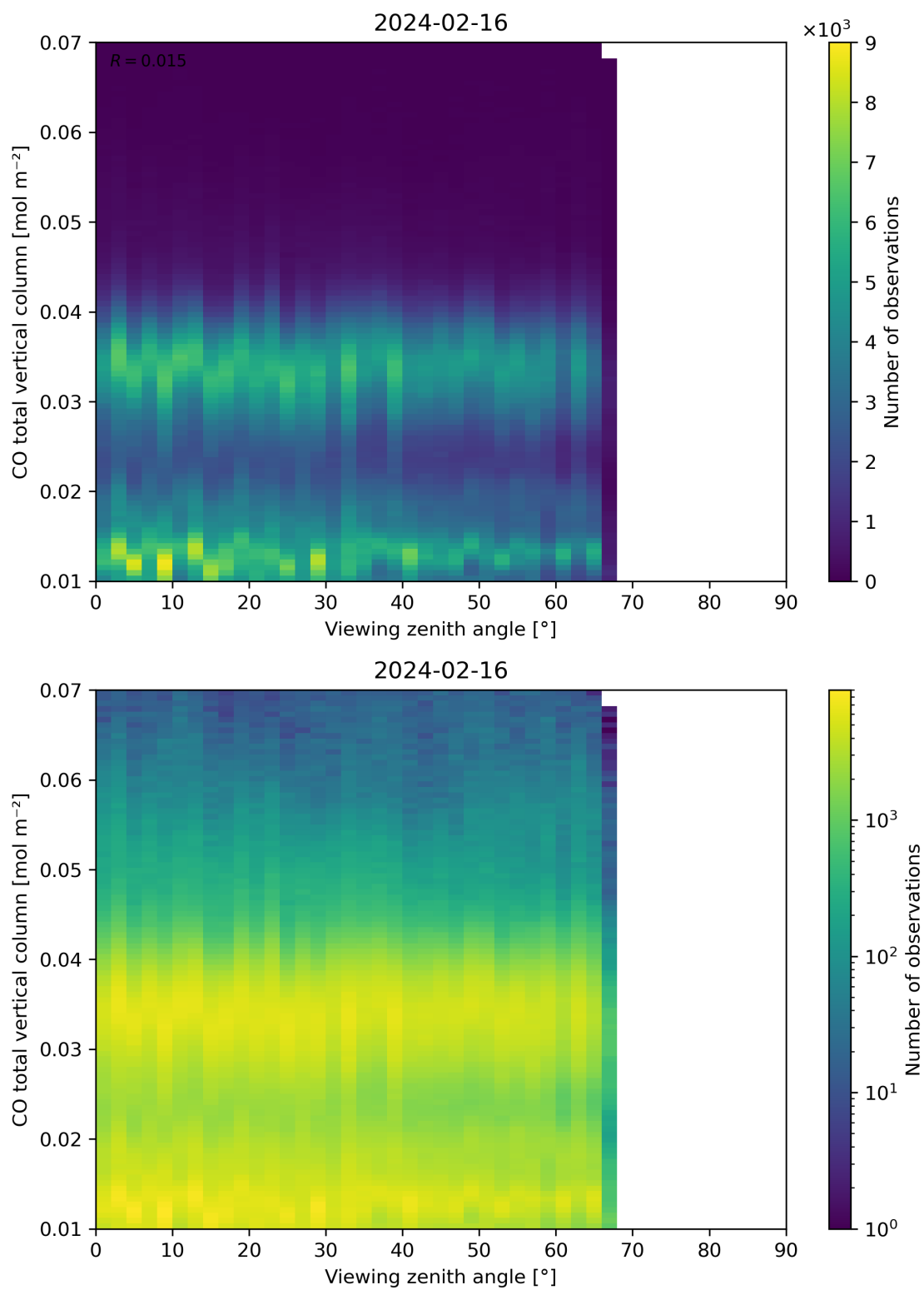
Figure 69: Scatter density plot of “Viewing zenith angle” against “CO total vertical column” for 2024-02-16 to 2024-02-17.
