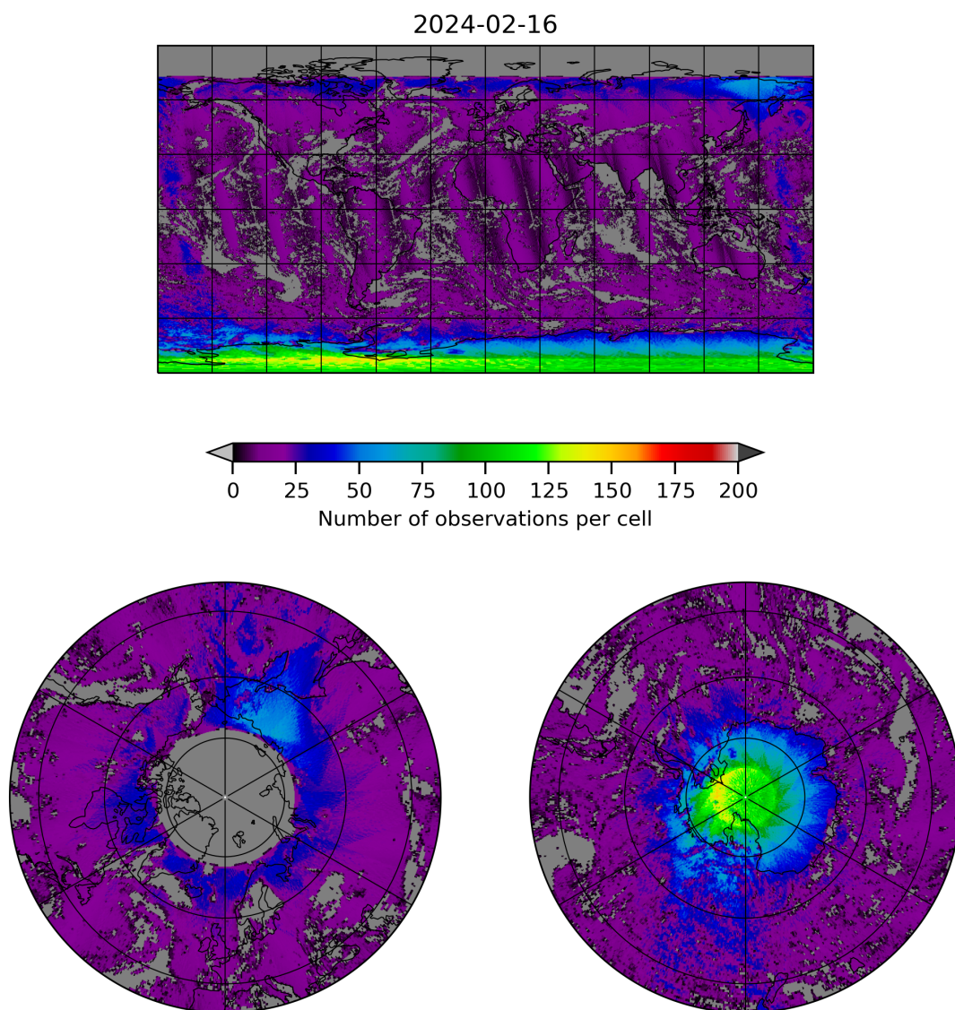
Figure 8: Map of the number of observations for 2024-02-16 to 2024-02-17
