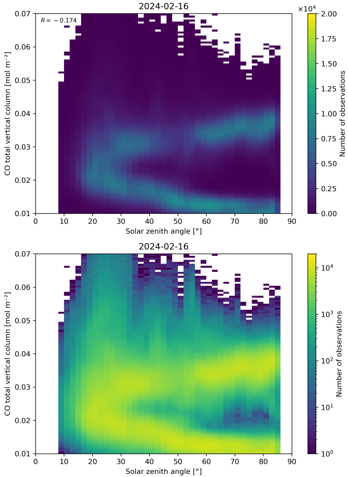
Figure 61: Scatter density plot of “Solar zenith angle” against “CO total vertical column” for 2024-02-16 to 2024-02-17.
