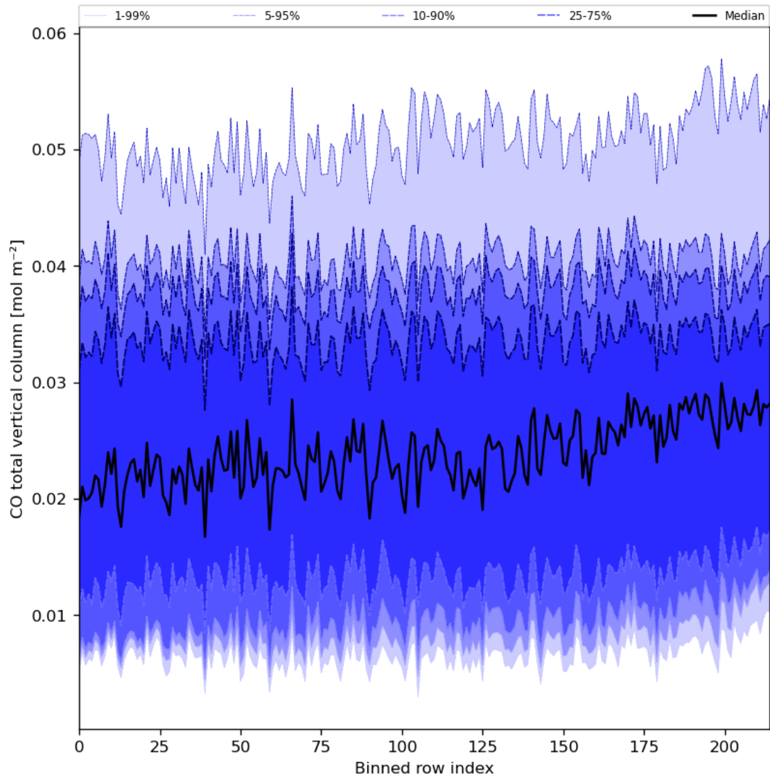
Figure 26: Along track statistics of “CO total vertical column” for 2024-02-16 to 2024-02-17
