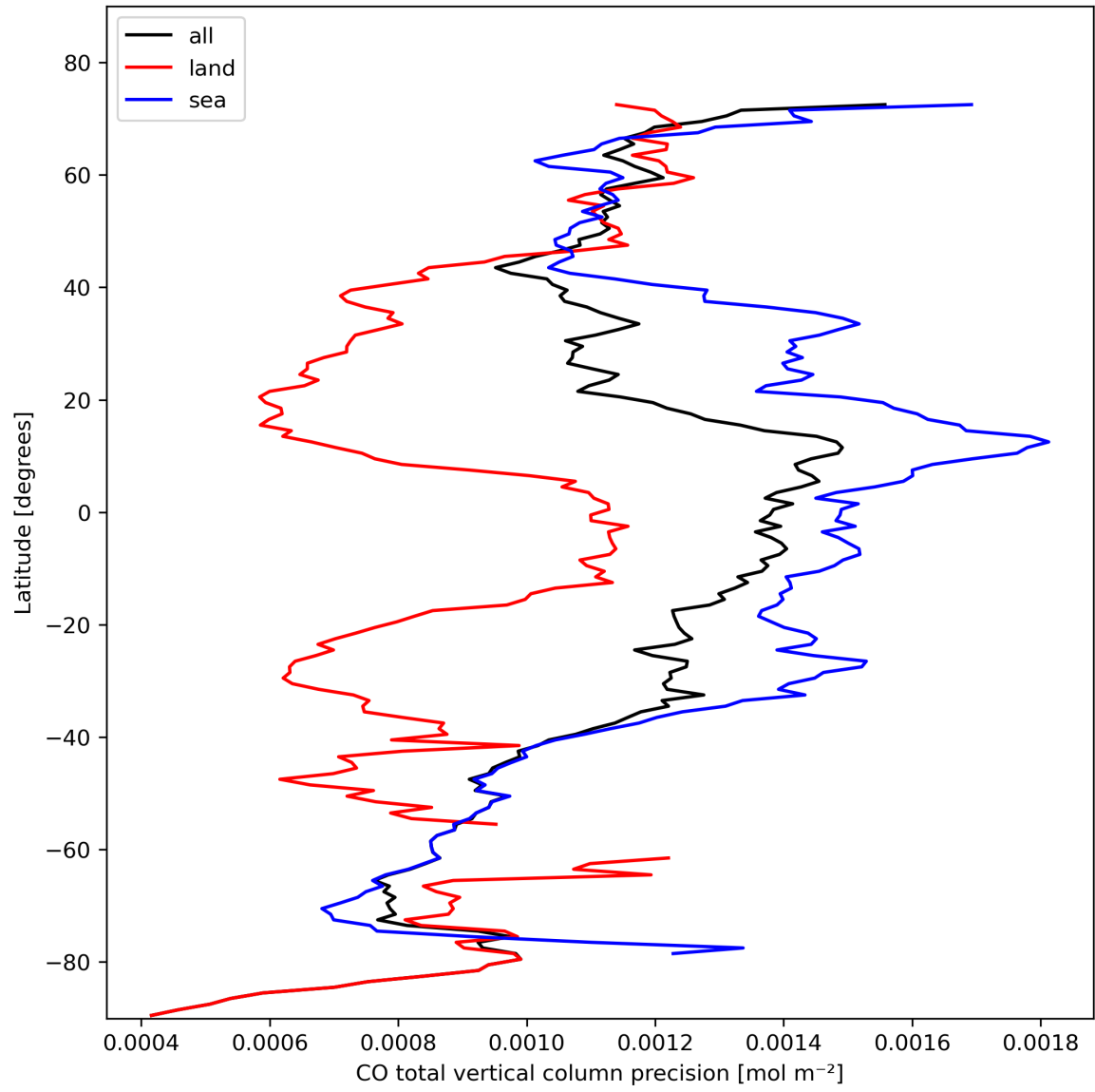
Figure 12: Zonal average of “CO total vertical column precision” for 2024-02-16 to 2024-02-17.
