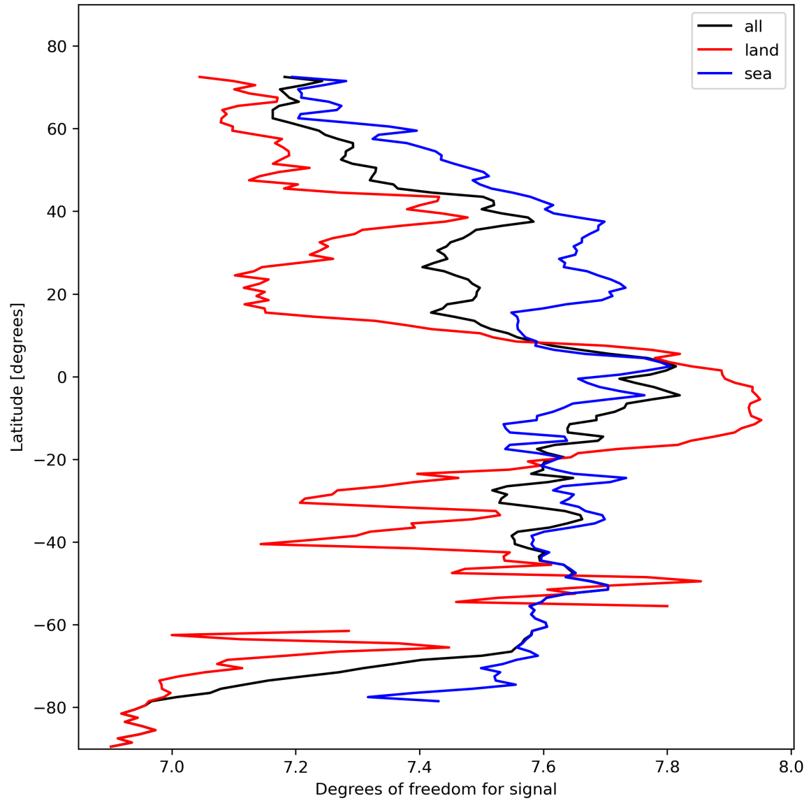
Figure 15: Zonal average of “Degrees of freedom for signal” for 2024-02-16 to 2024-02-17.
