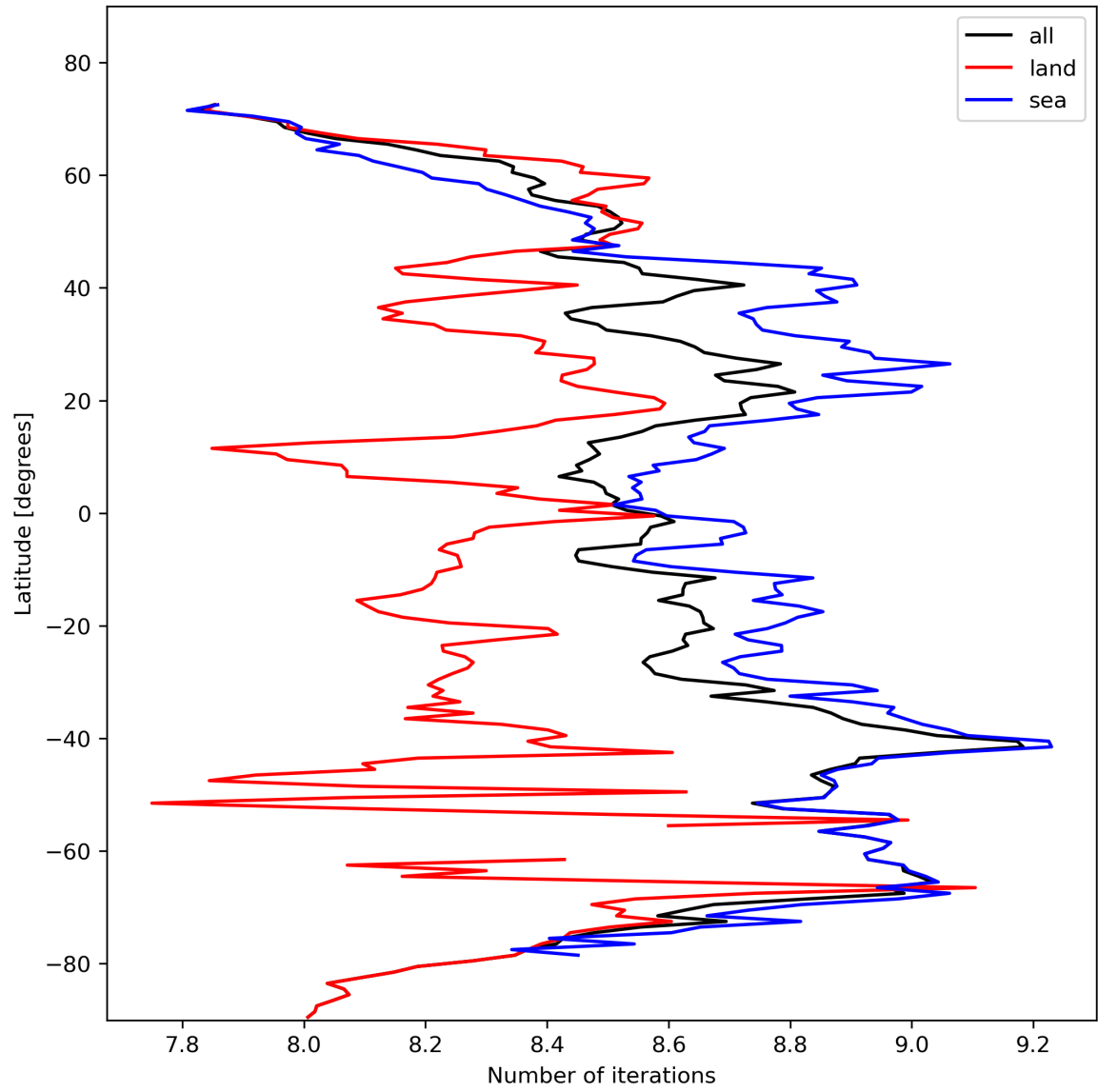
Figure 16: Zonal average of “Number of iterations” for 2024-02-16 to 2024-02-17.
