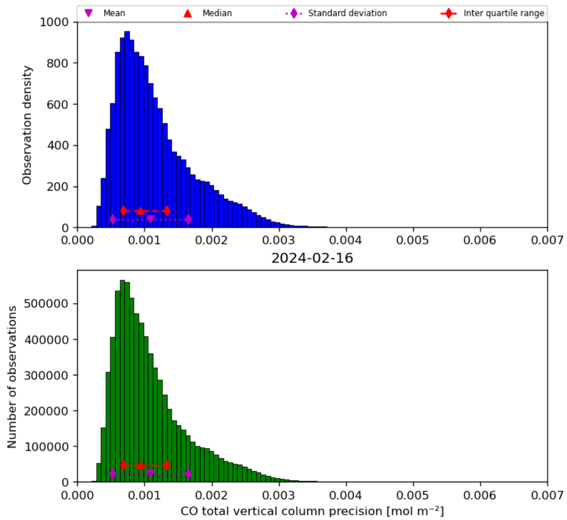
Figure 20: Histogram of “CO total vertical column precision” for 2024-02-16 to 2024-02-17
