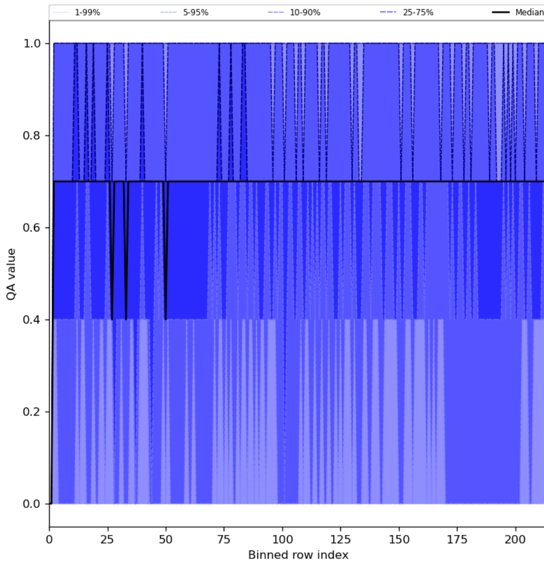
Figure 25: Along track statistics of “QA value” for 2024-02-16 to 2024-02-17
