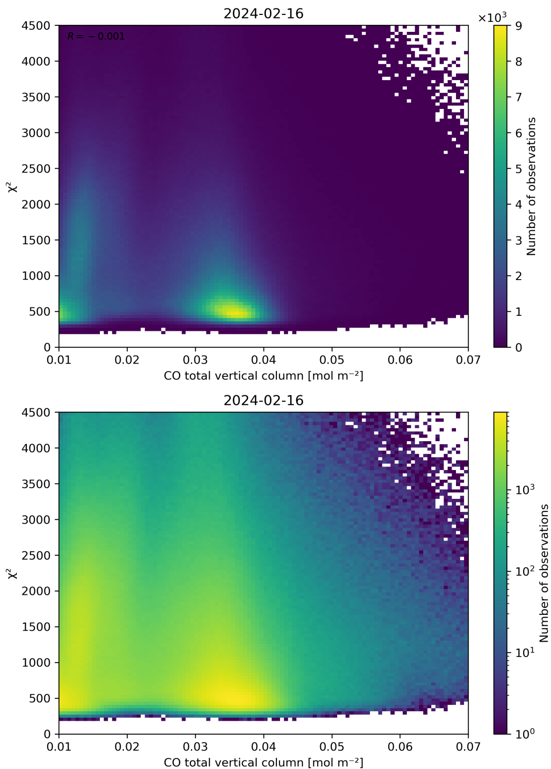
Figure 35: Scatter density plot of “CO total vertical column” against “ \chi^2 ” for 2024-02-16 to 2024-02-17.
