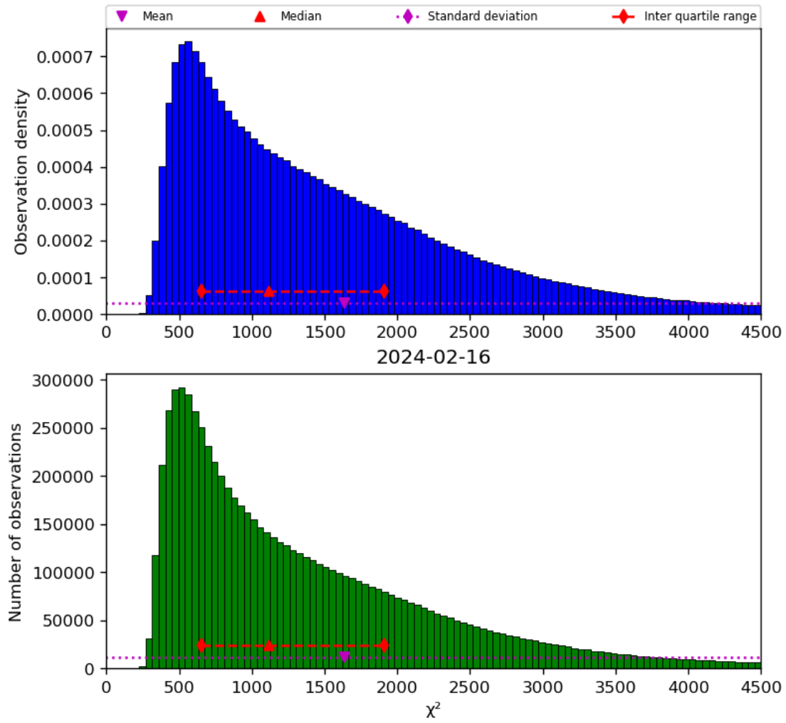
Figure 22: Histogram of “ \chi^2 ” for 2024-02-16 to 2024-02-17
