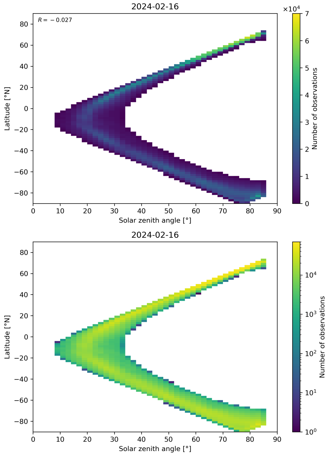
Figure 66: Scatter density plot of “Solar zenith angle” against “Latitude” for 2024-02-16 to 2024-02-17.
