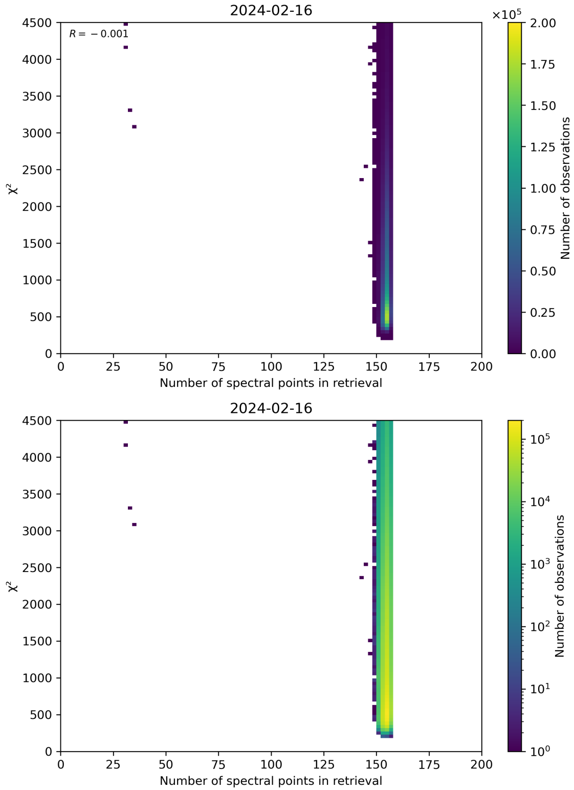
Figure 58: Scatter density plot of “Number of spectral points in retrieval” against “ \chi^2 ” for 2024-02-16 to 2024-02-17.
