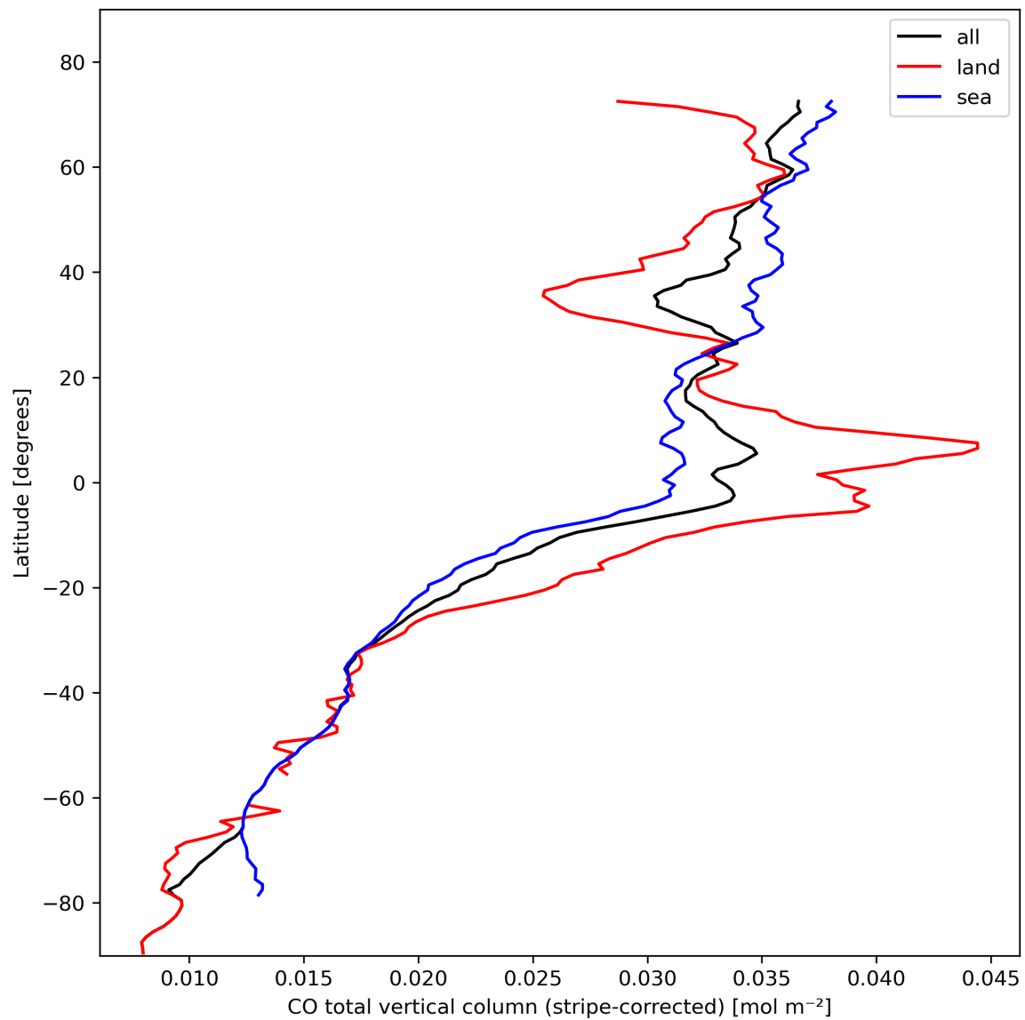
Figure 11: Zonal average of “CO total vertical column (stripe-corrected)” for 2024-02-16 to 2024-02-17.
