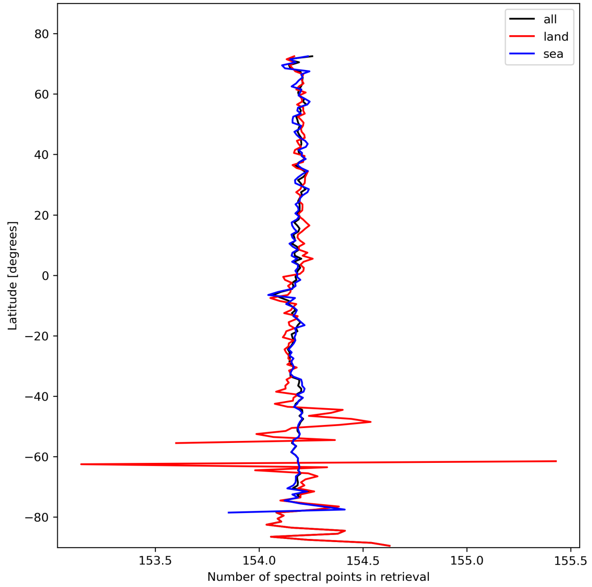
Figure 13: Zonal average of “Number of spectral points in retrieval” for 2024-02-16 to 2024-02-17.
