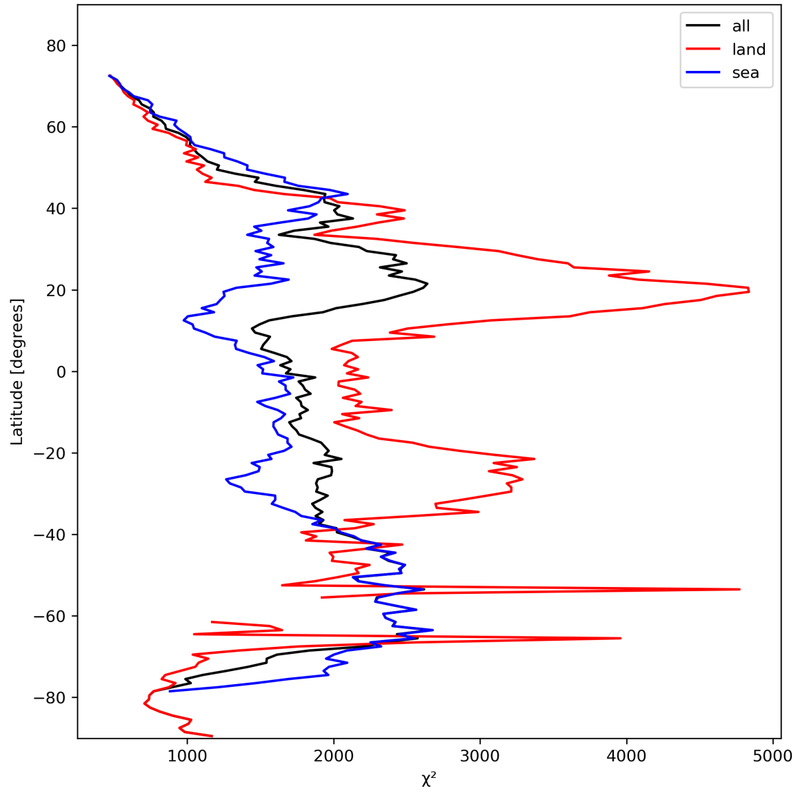
Figure 14: Zonal average of “ \chi^2 ” for 2024-02-16 to 2024-02-17.
