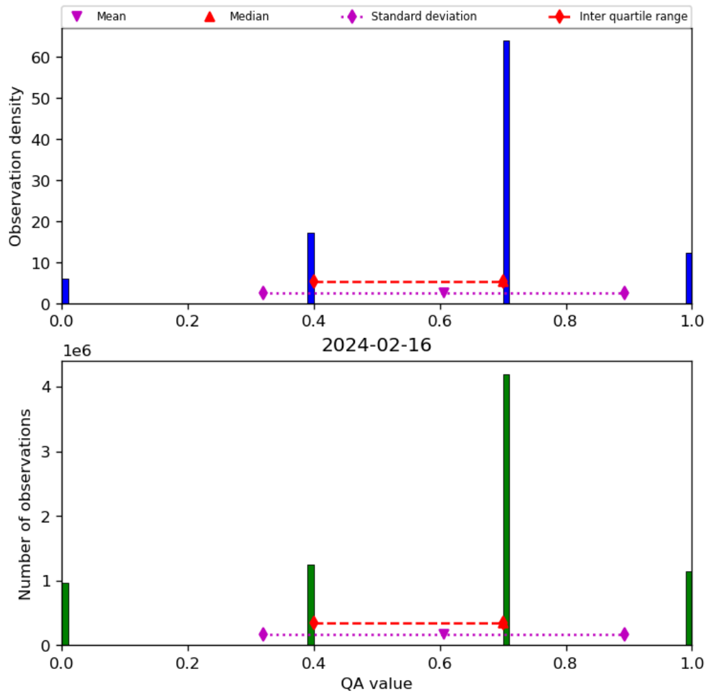
Figure 17: Histogram of “QA value” for 2024-02-16 to 2024-02-17
