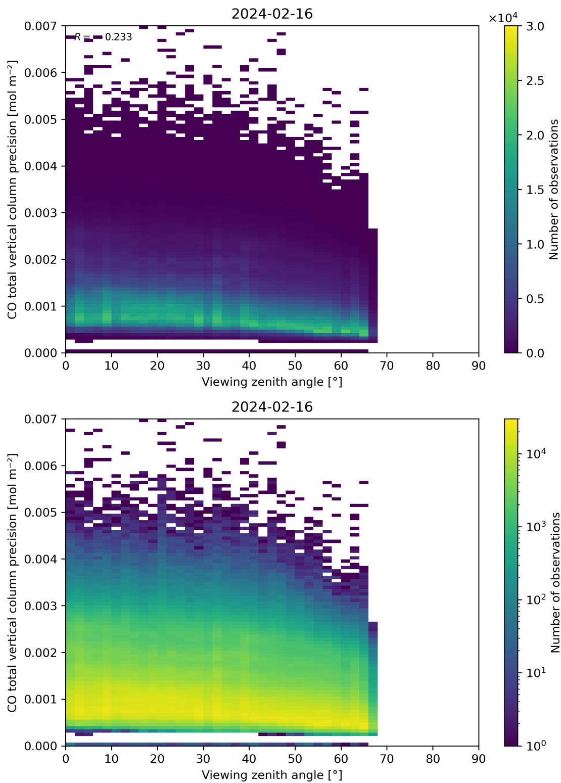
Figure 71: Scatter density plot of “Viewing zenith angle” against “CO total vertical column precision” for 2024-02-16 to 2024-02-17.
