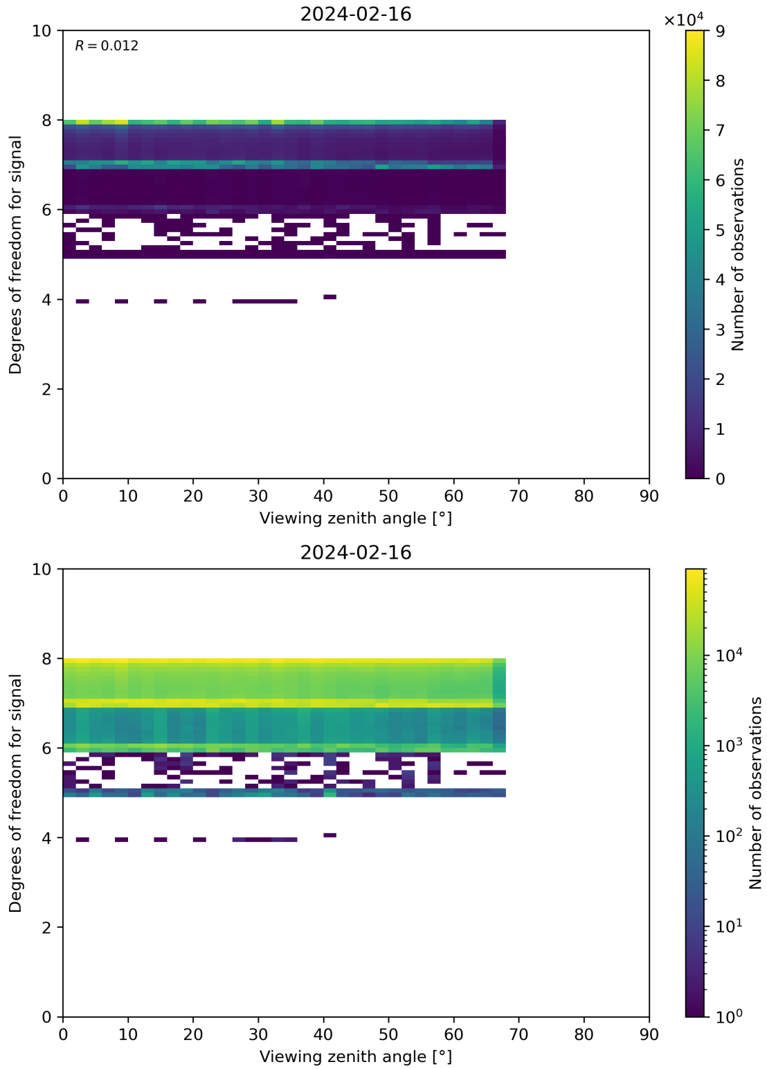
Figure 73: Scatter density plot of “Viewing zenith angle” against “Degrees of freedom for signal” for 2024-02-16 to 2024-02-17.
