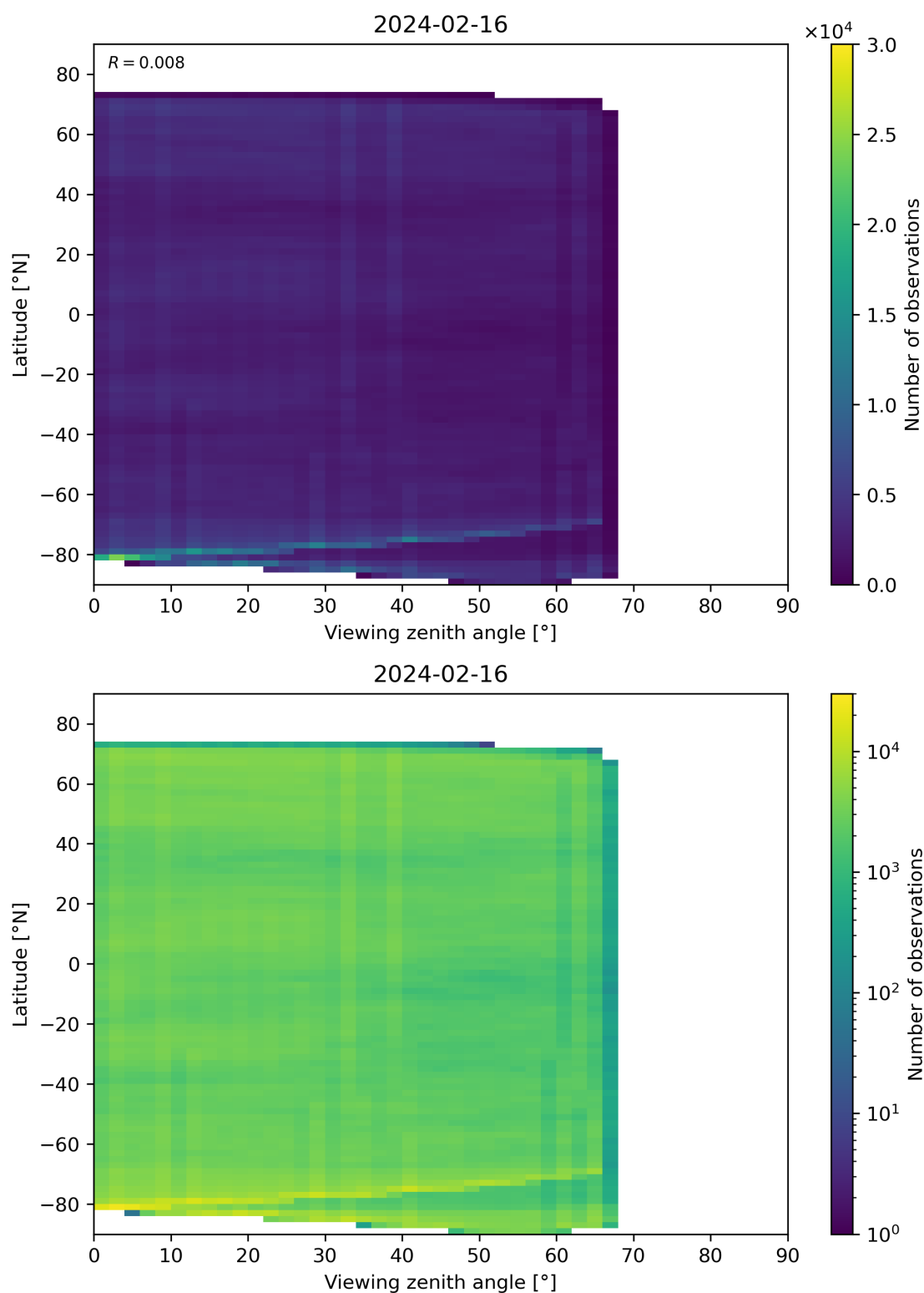
Figure 74: Scatter density plot of “Viewing zenith angle” against “Latitude” for 2024-02-16 to 2024-02-17.
