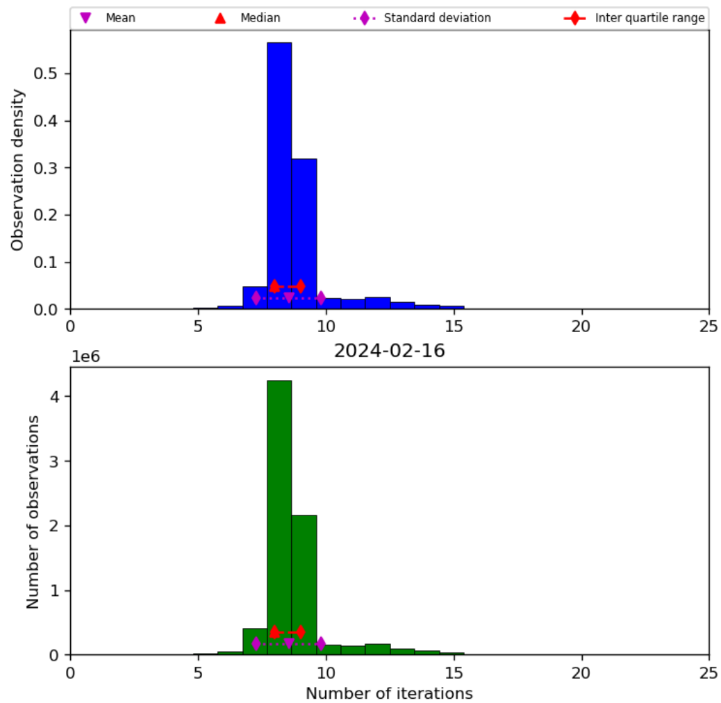
Figure 24: Histogram of “Number of iterations” for 2024-02-16 to 2024-02-17
