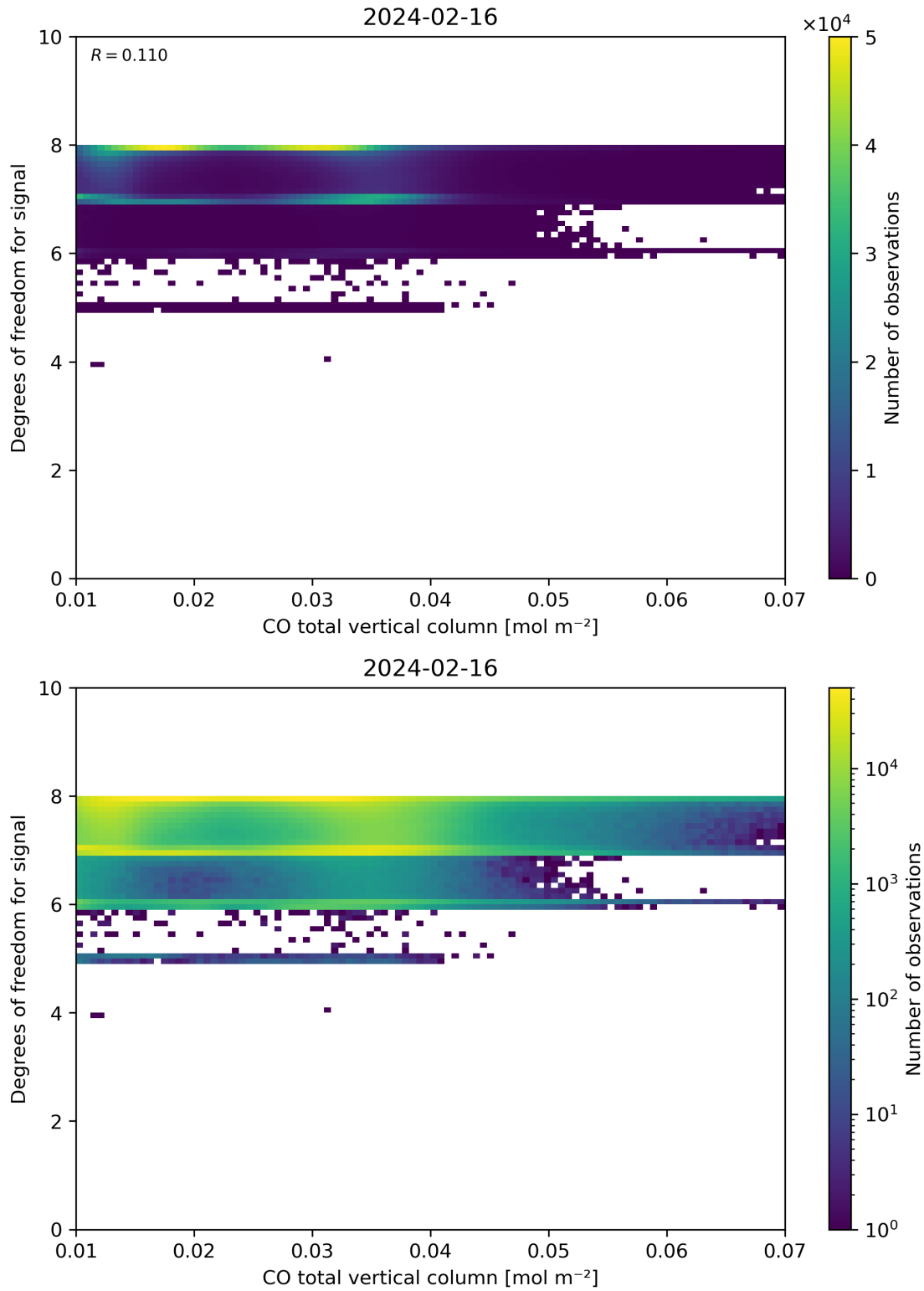
Figure 41: Scatter density plot of “CO total vertical column” against “Degrees of freedom for signal” for 2024-02-16 to 2024-02-17.
