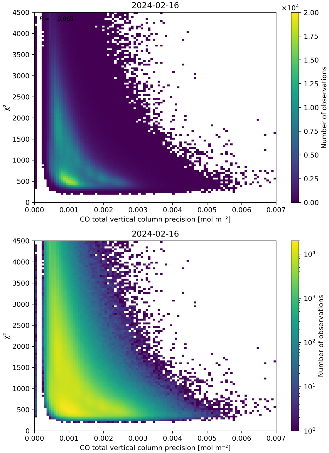
Figure 44: Scatter density plot of “CO total vertical column precision” against “ \chi^2 ” for 2024-02-16 to 2024-02-17.
