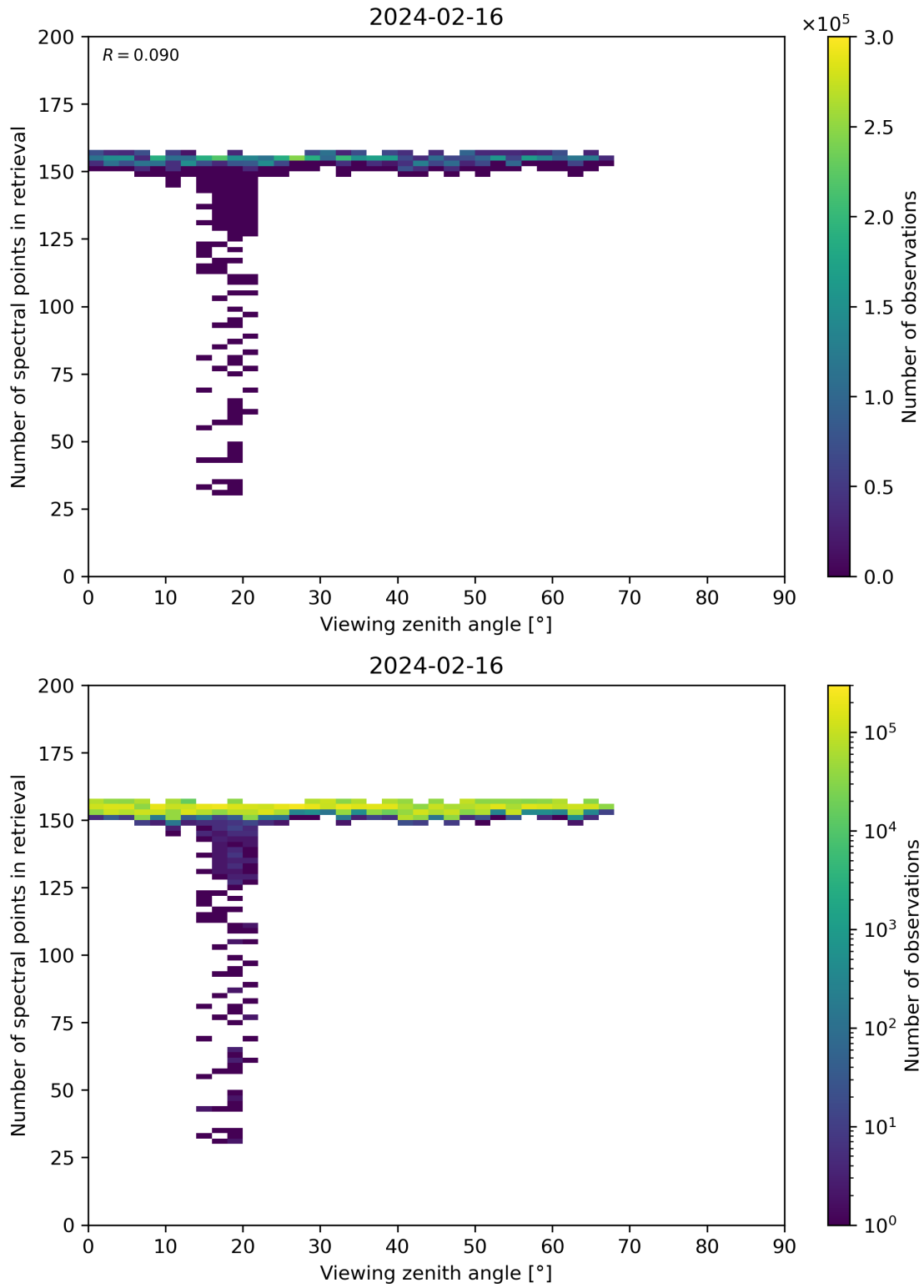
Figure 76: Scatter density plot of “Viewing zenith angle” against “Number of spectral points in retrieval” for 2024-02-16 to 2024-02-17.
