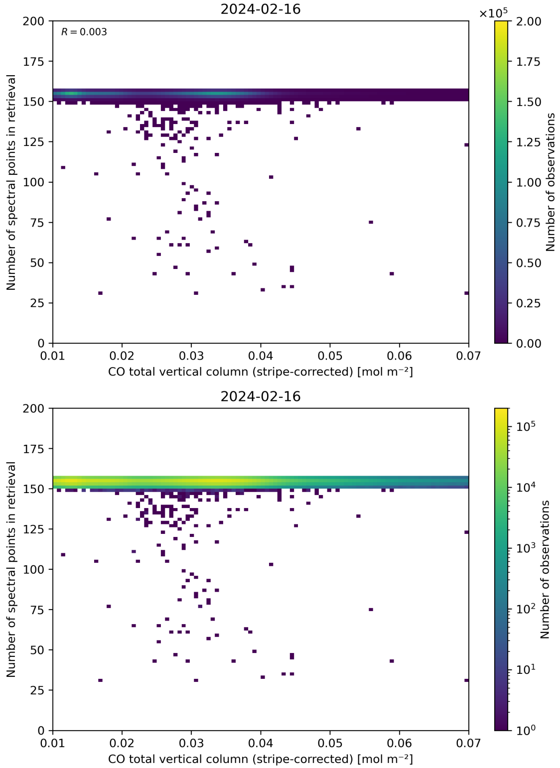
Figure 40: Scatter density plot of “CO total vertical column (stripe-corrected)” against “Number of spectral points in retrieval” for 2024-02-16 to 2024-02-17.
