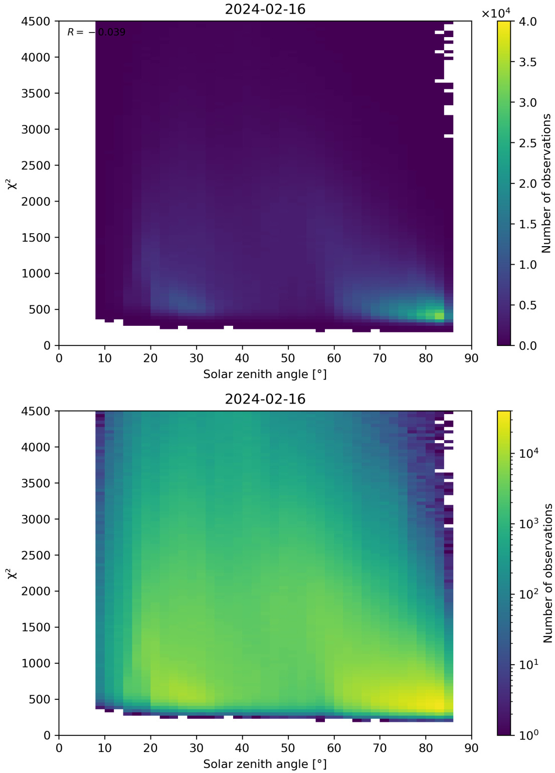
Figure 64: Scatter density plot of “Solar zenith angle” against “ \chi^2 ” for 2024-02-16 to 2024-02-17.
