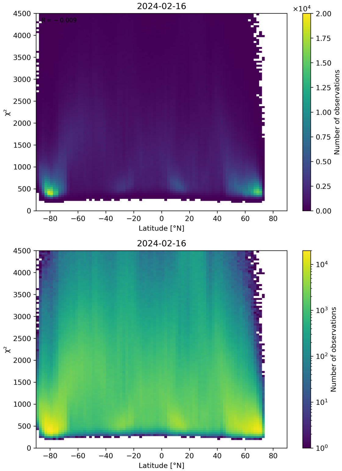
Figure 54: Scatter density plot of “Latitude” against “ \chi^2 ” for 2024-02-16 to 2024-02-17.
