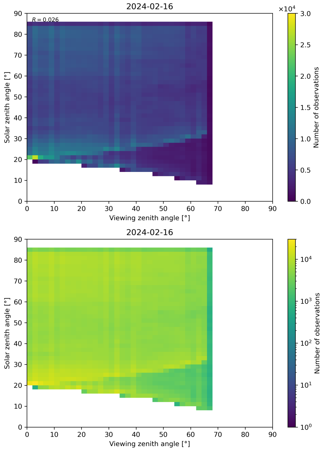
Figure 77: Scatter density plot of “Viewing zenith angle” against “Solar zenith angle” for 2024-02-16 to 2024-02-17.
