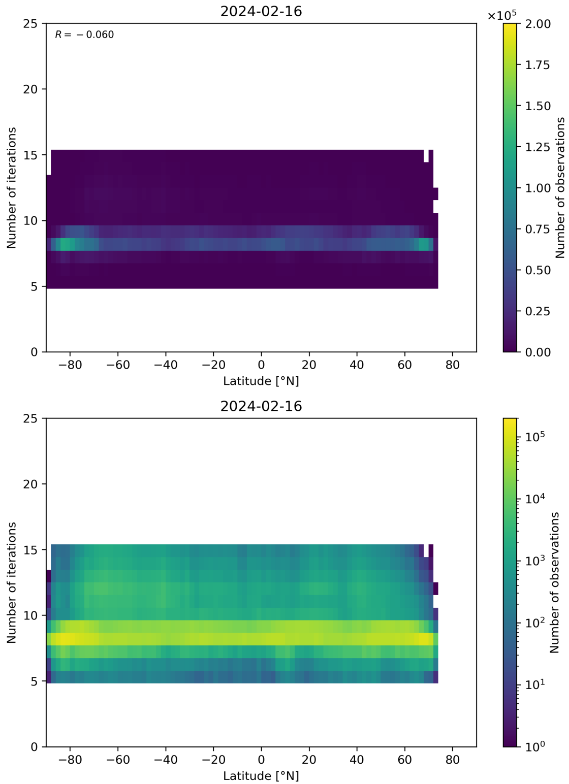
Figure 56: Scatter density plot of “Latitude” against “Number of iterations” for 2024-02-16 to 2024-02-17.
