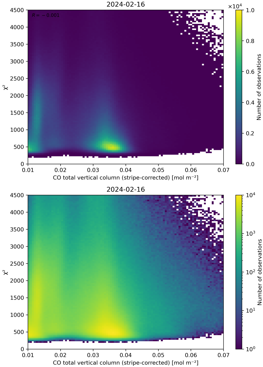
Figure 37: Scatter density plot of “CO total vertical column (stripe-corrected)” against “ \chi^2 ” for 2024-02-16 to 2024-02-17.
