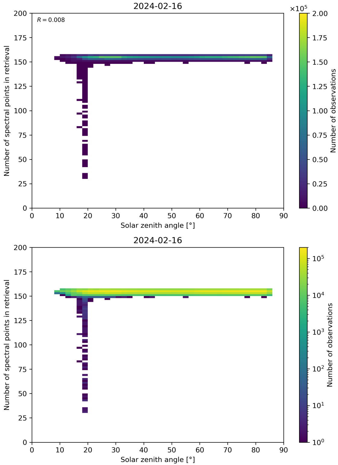
Figure 68: Scatter density plot of “Solar zenith angle” against “Number of spectral points in retrieval” for 2024-02-16 to 2024-02-17.
