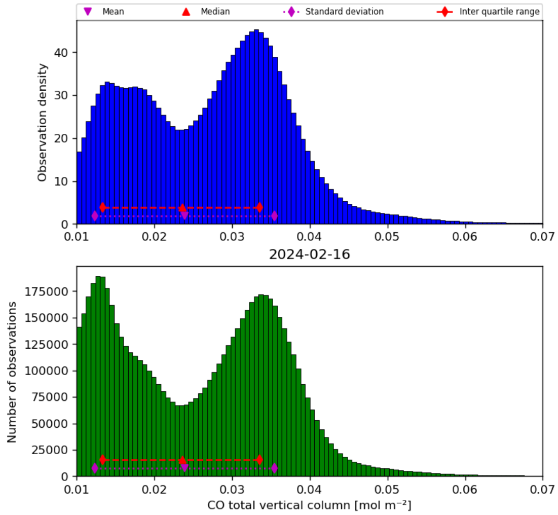
Figure 18: Histogram of “CO total vertical column” for 2024-02-16 to 2024-02-17
