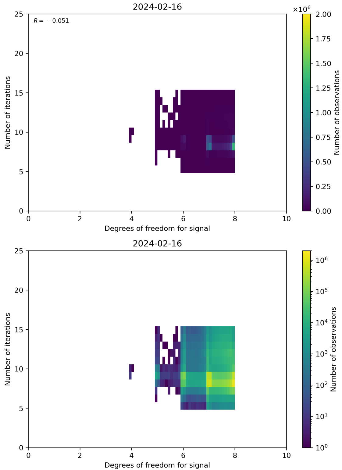
Figure 50: Scatter density plot of “Degrees of freedom for signal” against “Number of iterations” for 2024-02-16 to 2024-02-17.
