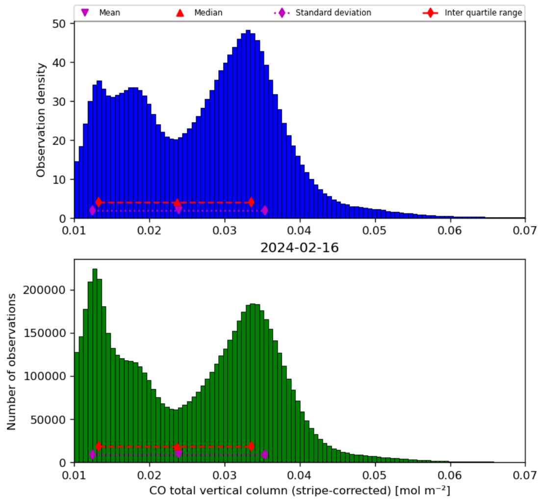
Figure 19: Histogram of “CO total vertical column (stripe-corrected)” for 2024-02-16 to 2024-02-17
