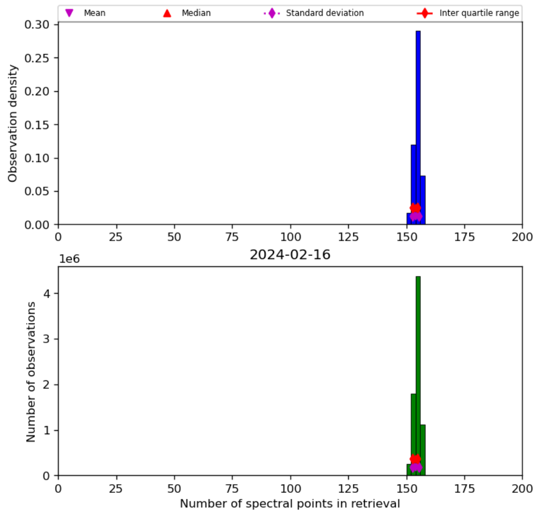
Figure 21: Histogram of “Number of spectral points in retrieval” for 2024-02-16 to 2024-02-17
