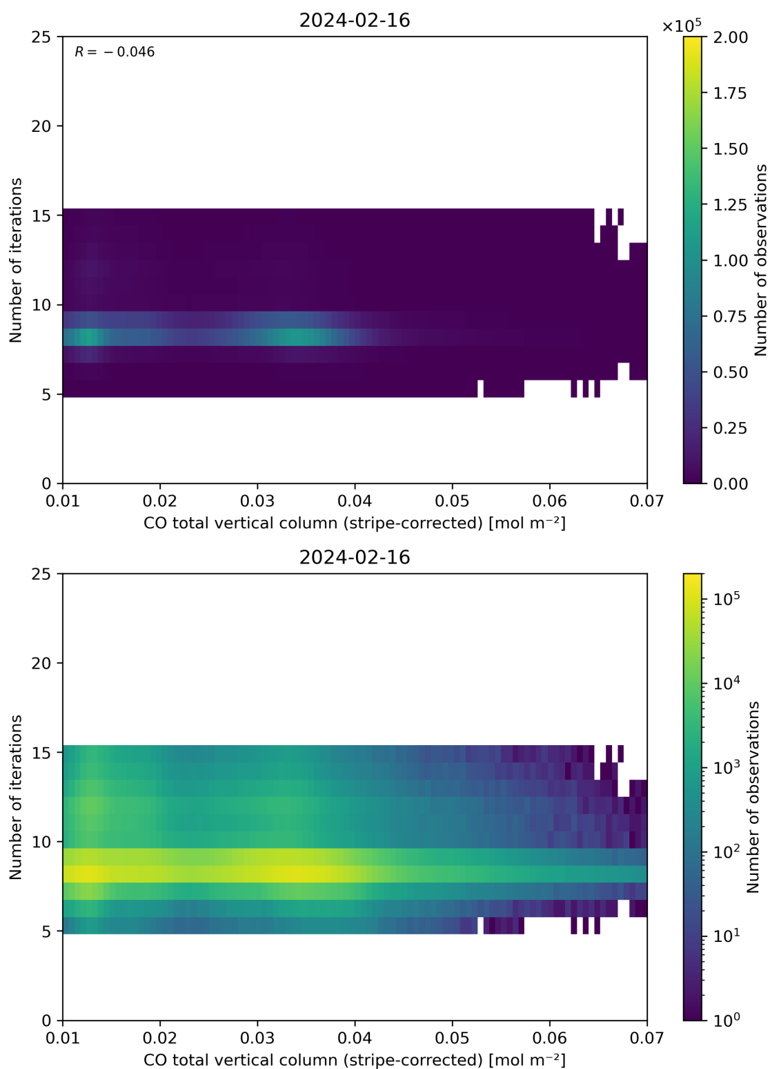
Figure 39: Scatter density plot of “CO total vertical column (stripe-corrected)” against “Number of iterations” for 2024-02-16 to 2024-02-17.
