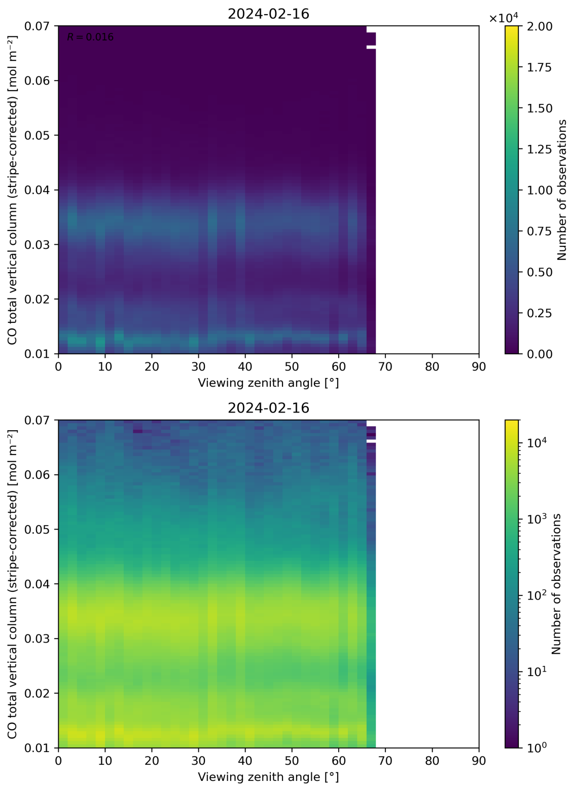
Figure 70: Scatter density plot of “Viewing zenith angle” against “CO total vertical column (stripe-corrected)” for 2024-02-16 to 2024-02-17.
