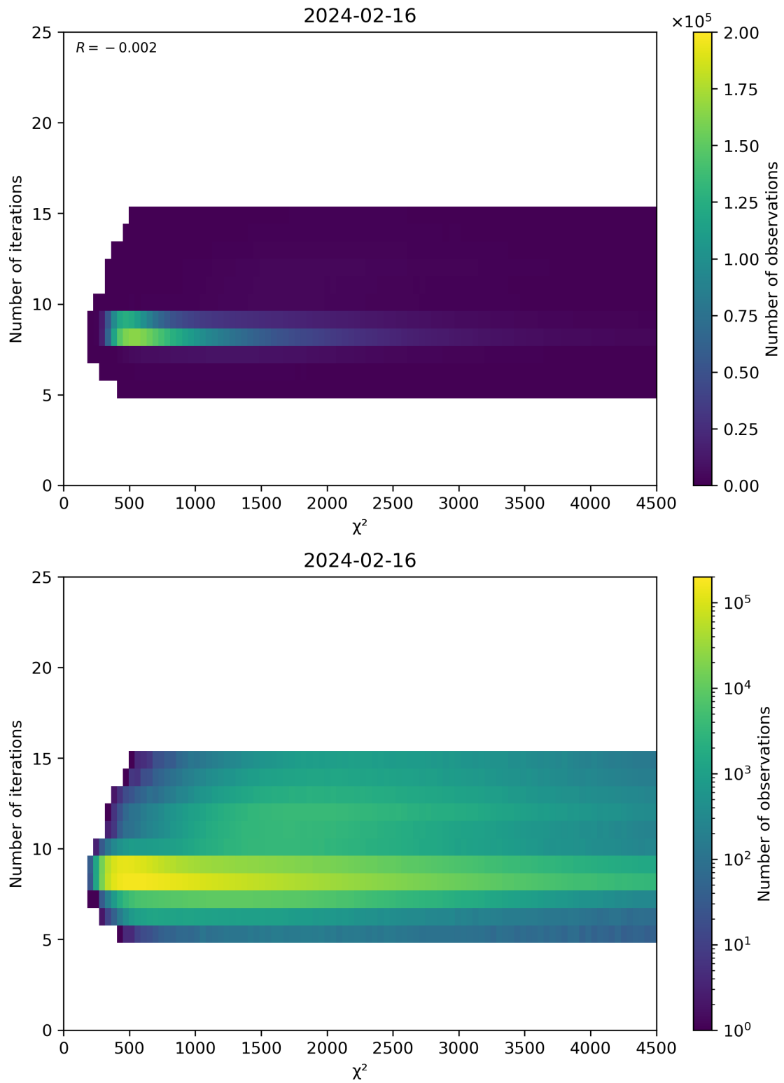
Figure 49: Scatter density plot of “ \chi^2 ” against “Number of iterations” for 2024-02-16 to 2024-02-17.
