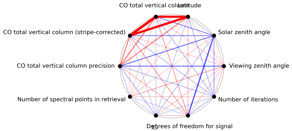
Figure 1: Map of correlation graph for 2024-02-16 to 2024-02-17.
