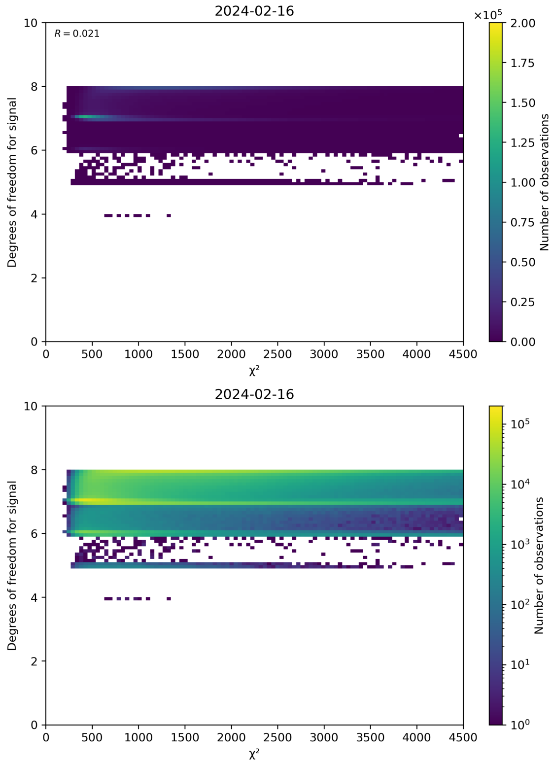
Figure 48: Scatter density plot of “ \chi^2 ” against “Degrees of freedom for signal” for 2024-02-16 to 2024-02-17.
