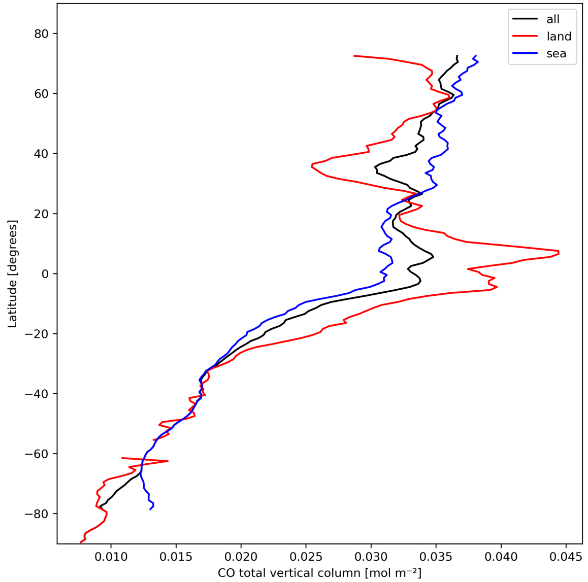
Figure 10: Zonal average of “CO total vertical column” for 2024-02-16 to 2024-02-17.
