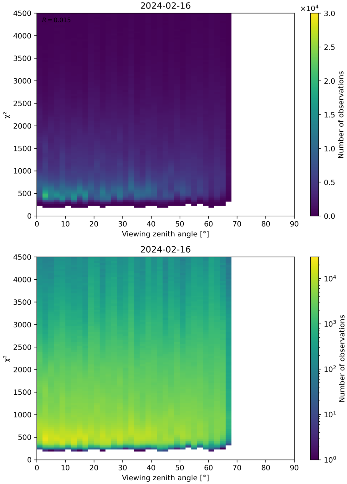
Figure 72: Scatter density plot of “Viewing zenith angle” against “ \chi^2 ” for 2024-02-16 to 2024-02-17.
