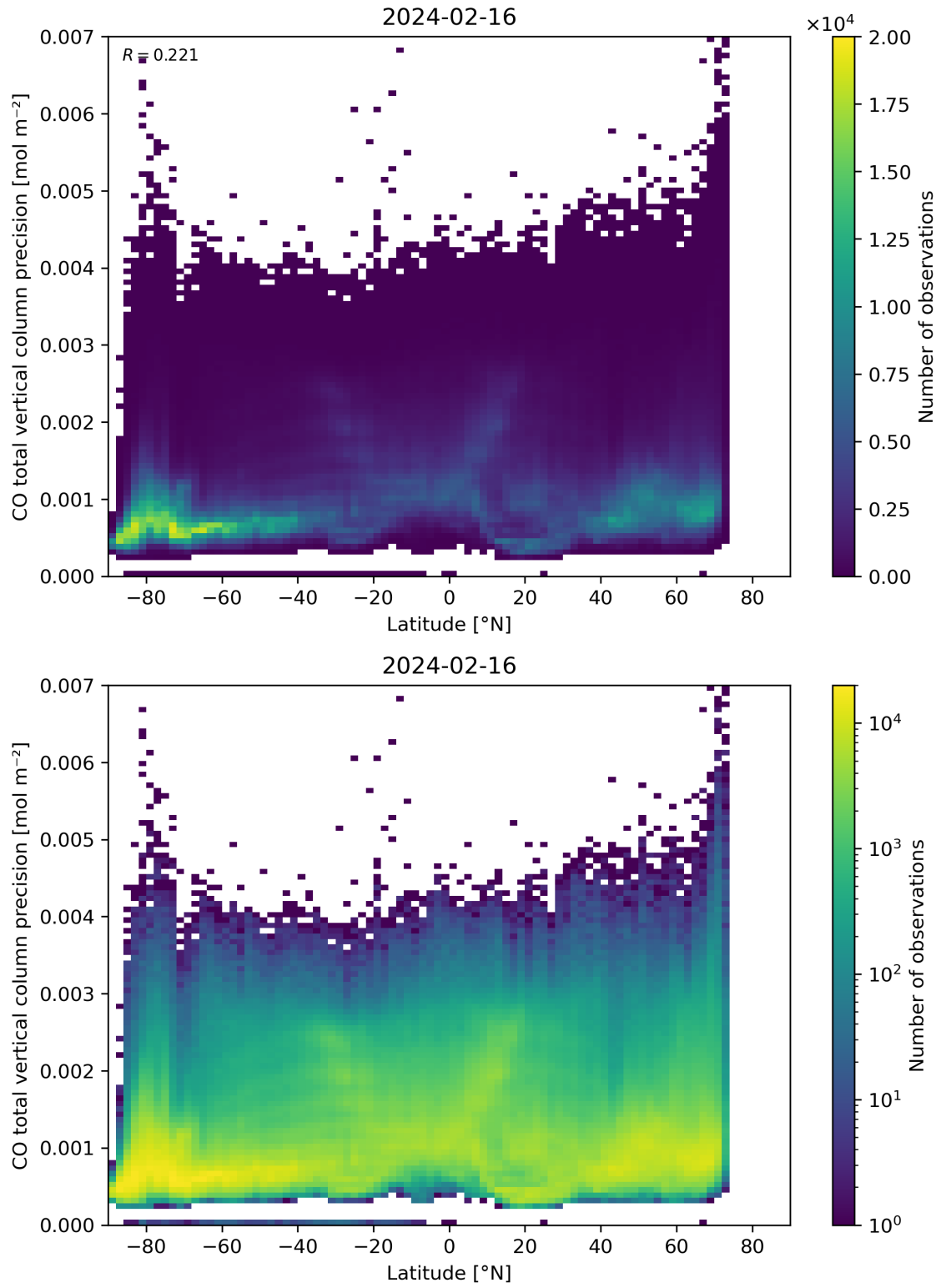
Figure 53: Scatter density plot of “Latitude” against “CO total vertical column precision” for 2024-02-16 to 2024-02-17.
