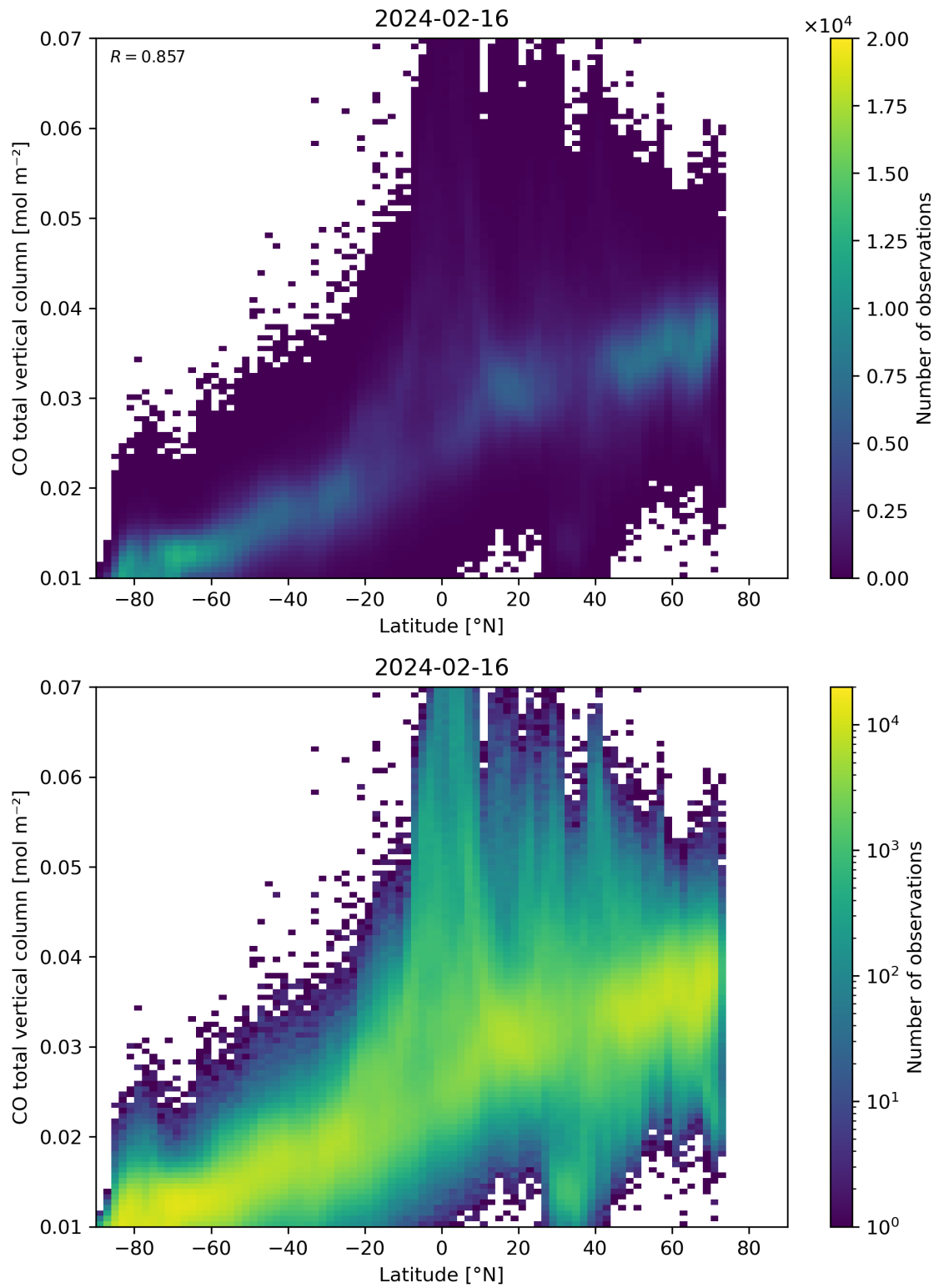
Figure 51: Scatter density plot of “Latitude” against “CO total vertical column” for 2024-02-16 to 2024-02-17.
