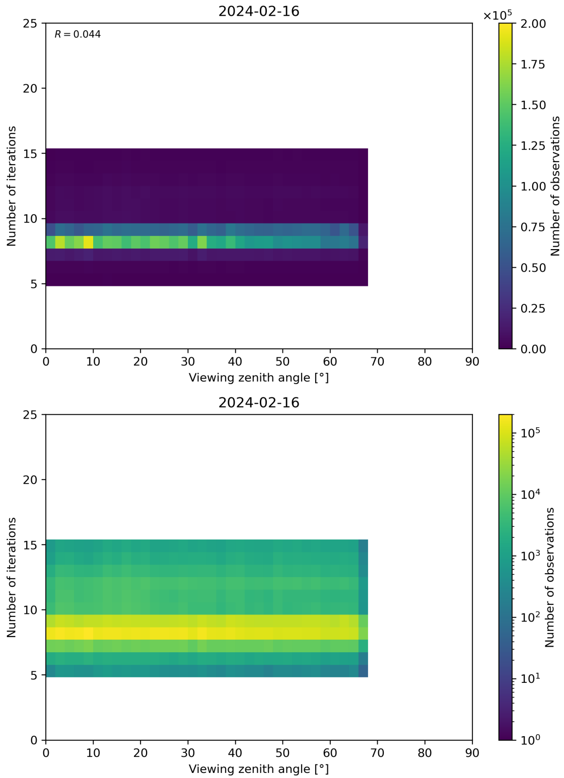
Figure 75: Scatter density plot of “Viewing zenith angle” against “Number of iterations” for 2024-02-16 to 2024-02-17.
