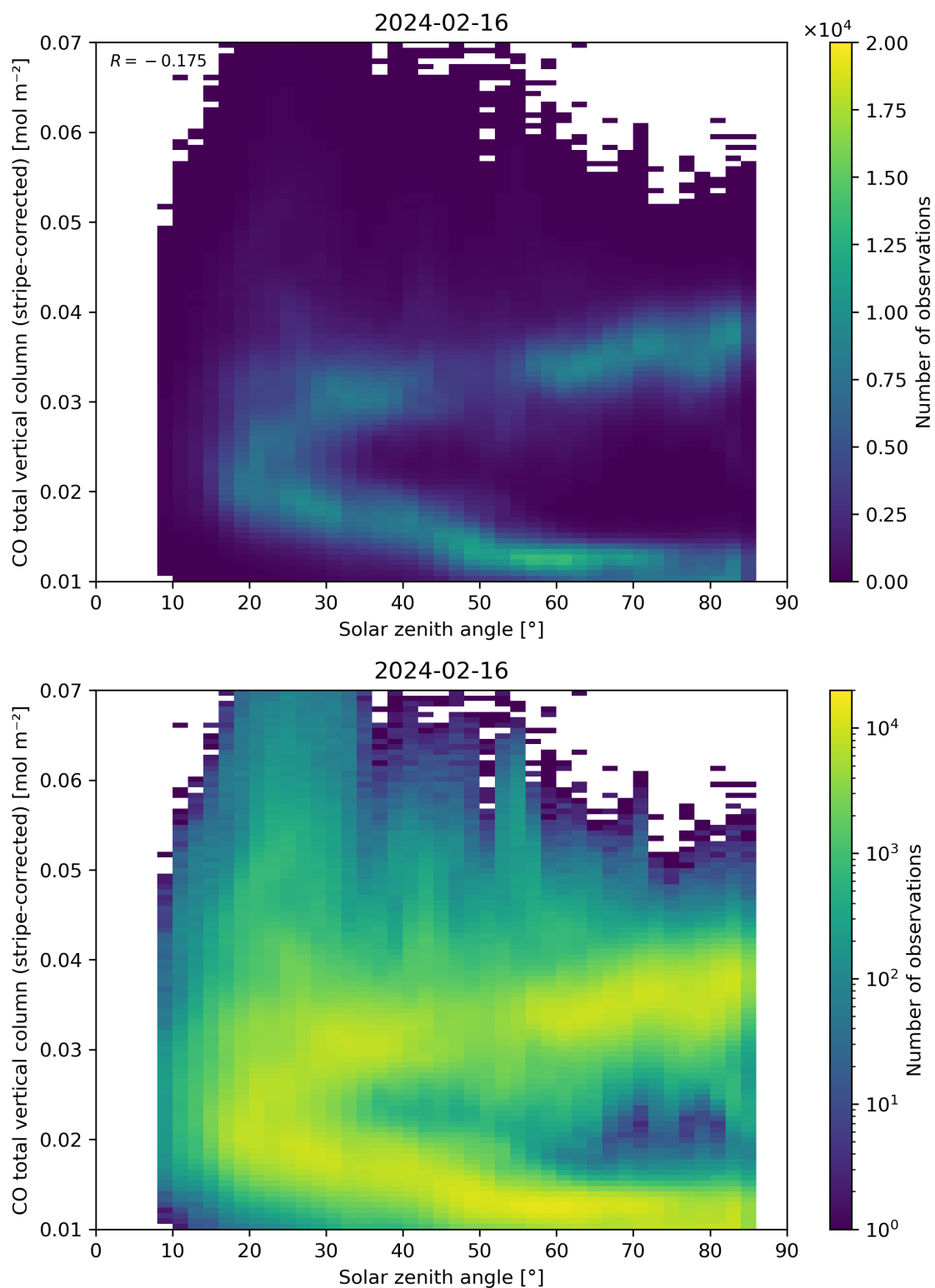
Figure 62: Scatter density plot of “Solar zenith angle” against “CO total vertical column (stripe-corrected)” for 2024-02-16 to 2024-02-17.
