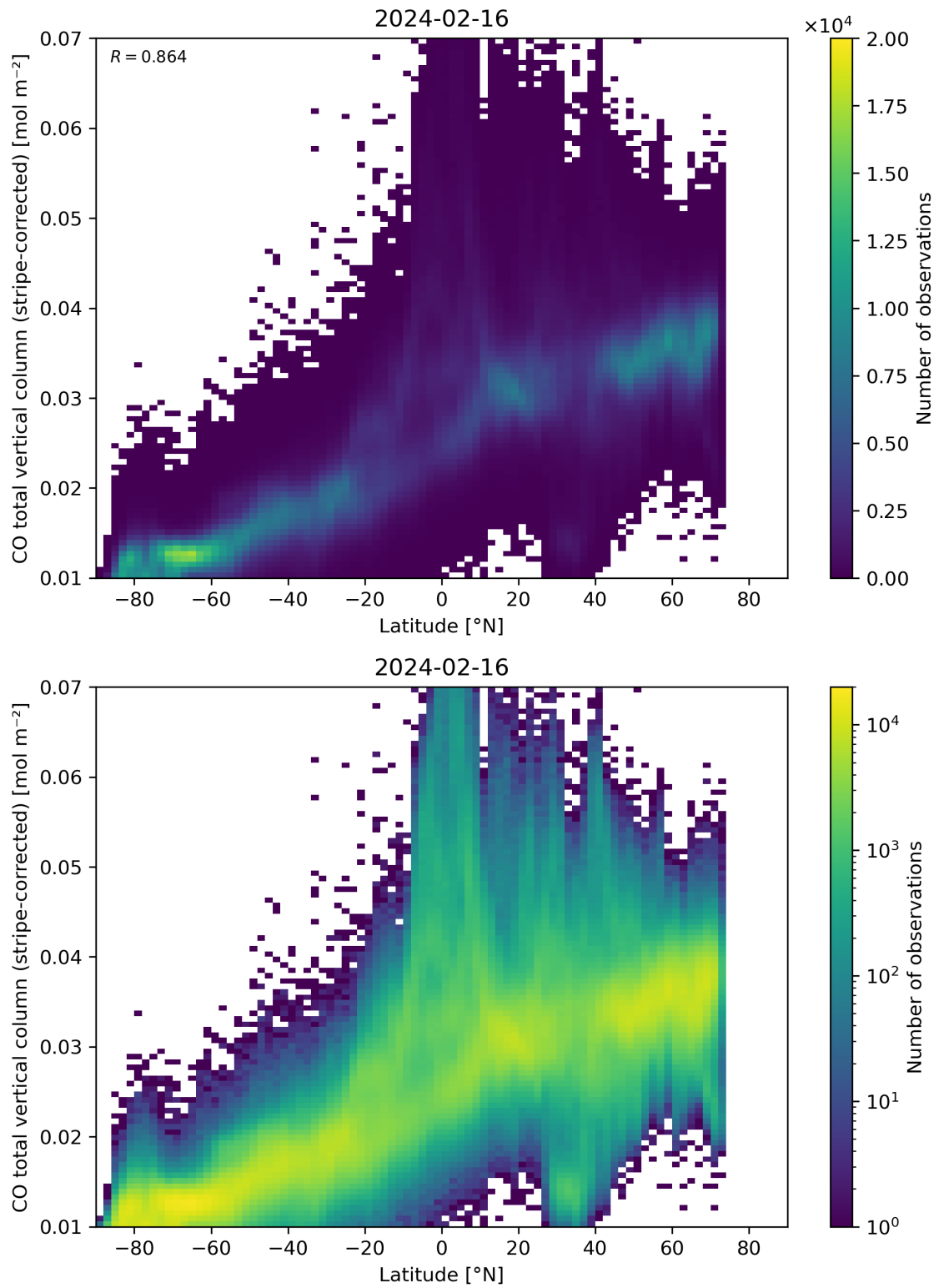
Figure 52: Scatter density plot of “Latitude” against “CO total vertical column (stripe-corrected)” for 2024-02-16 to 2024-02-17.
