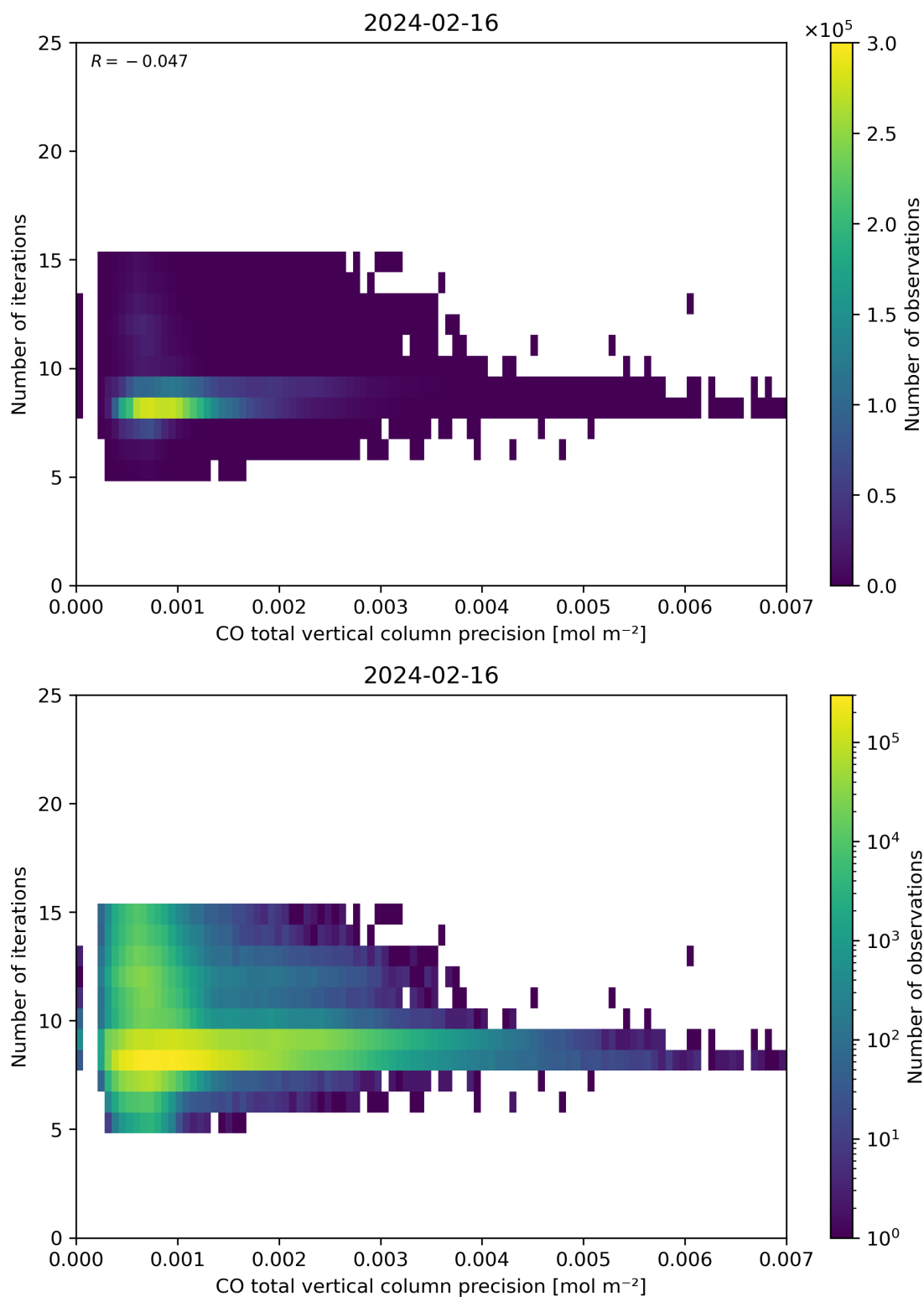
Figure 46: Scatter density plot of “CO total vertical column precision” against “Number of iterations” for 2024-02-16 to 2024-02-17.
