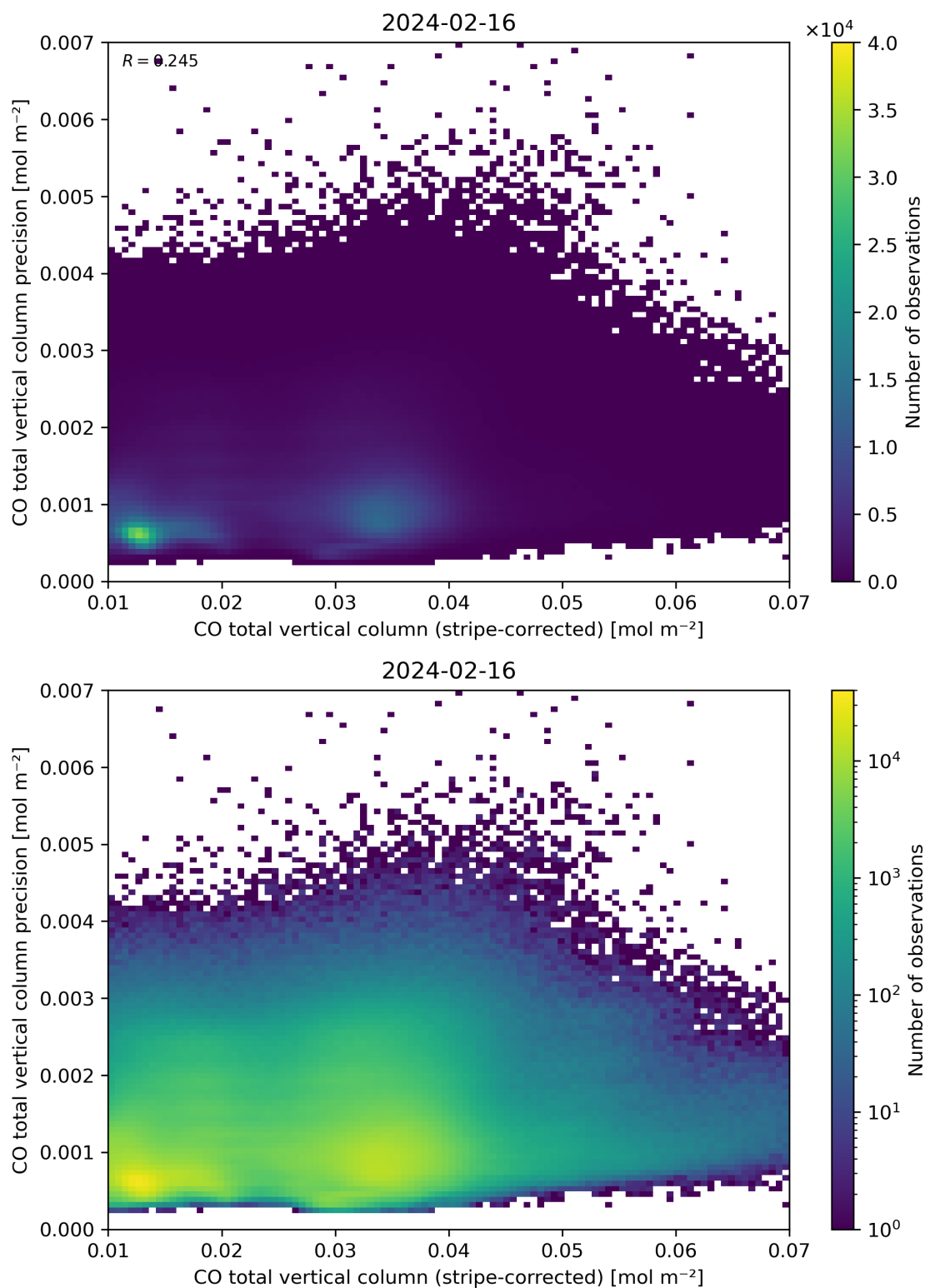
Figure 36: Scatter density plot of “CO total vertical column (stripe-corrected)” against “CO total vertical column precision” for 2024-02-16 to 2024-02-17.
