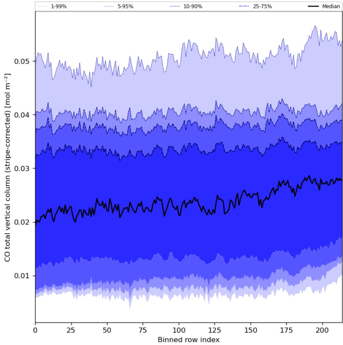
Figure 27: Along track statistics of “CO total vertical column (stripe-corrected)” for 2024-02-16 to 2024-02-17
