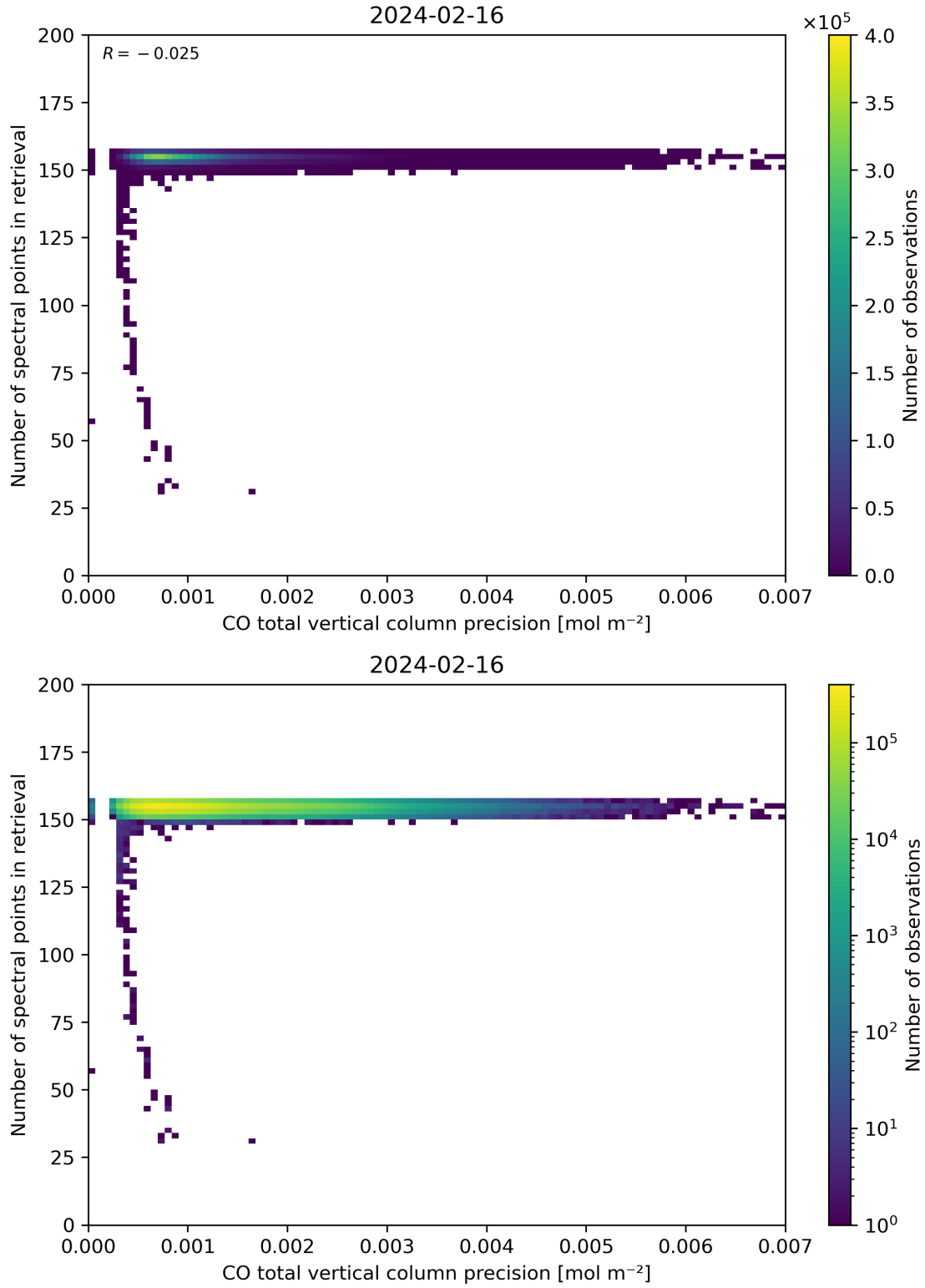
Figure 47: Scatter density plot of “CO total vertical column precision” against “Number of spectral points in retrieval” for 2024-02-16 to 2024-02-17.
