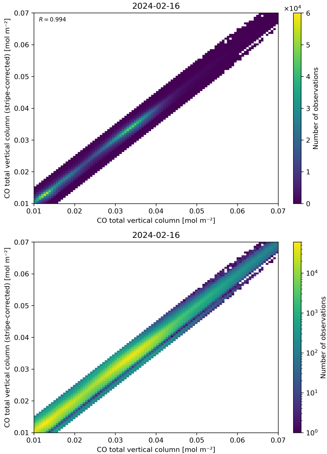
Figure 33: Scatter density plot of “CO total vertical column” against “CO total vertical column (stripe-corrected)” for 2024-02-16 to 2024-02-17.
