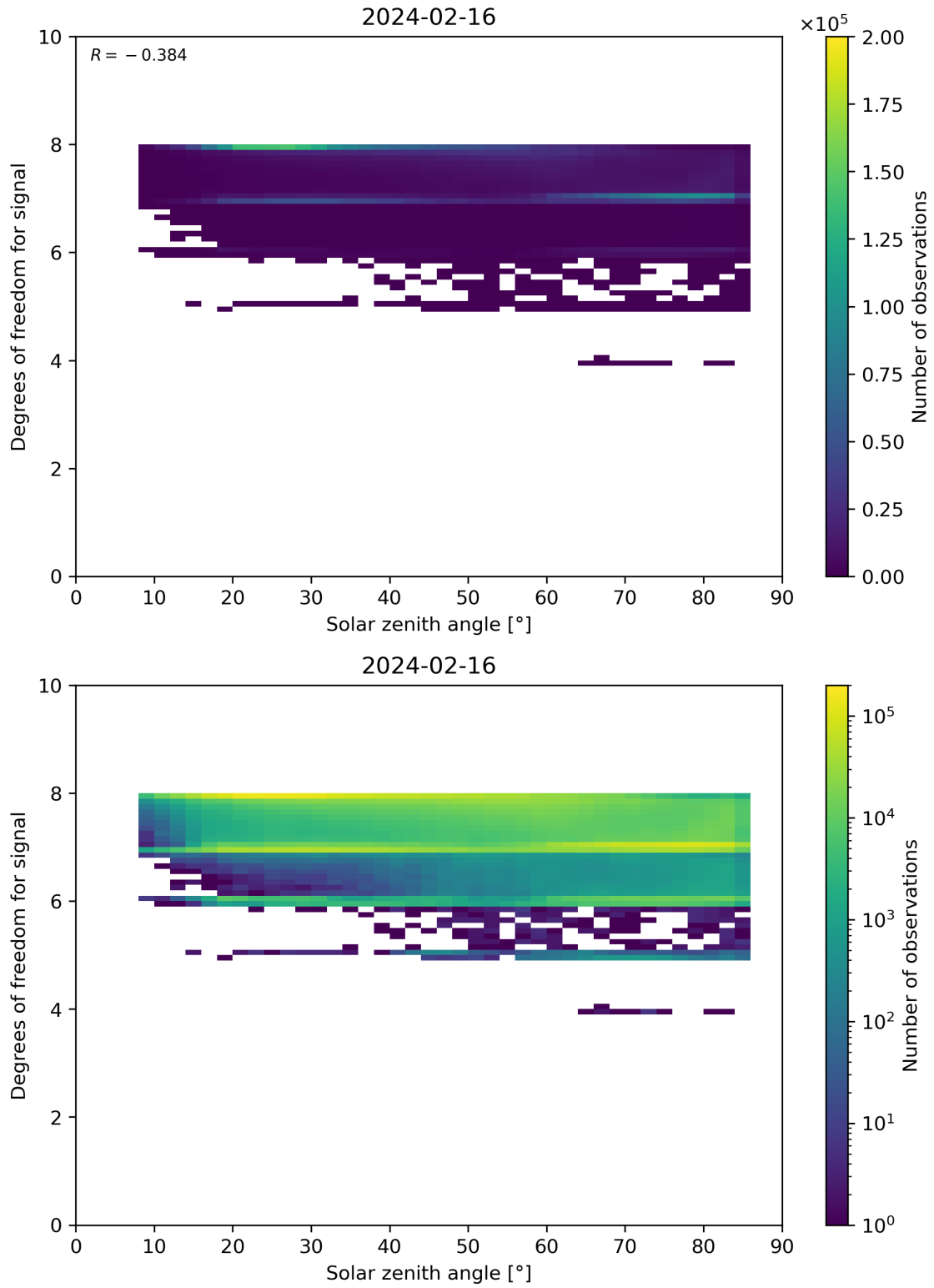
Figure 65: Scatter density plot of “Solar zenith angle” against “Degrees of freedom for signal” for 2024-02-16 to 2024-02-17.
