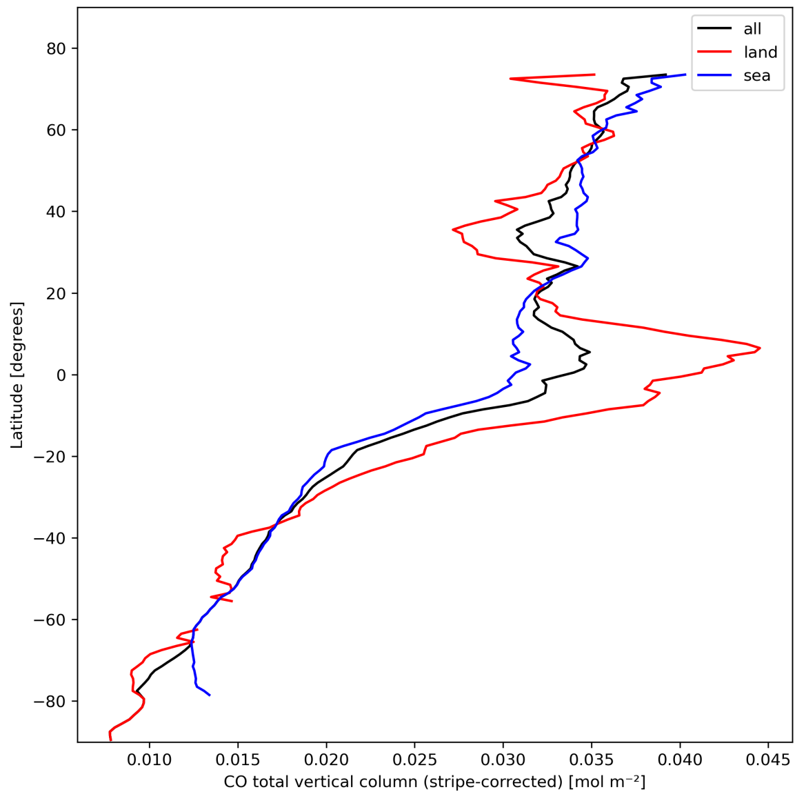
Figure 11: Zonal average of “CO total vertical column (stripe-corrected)” for 2024-02-17 to 2024-02-18.
