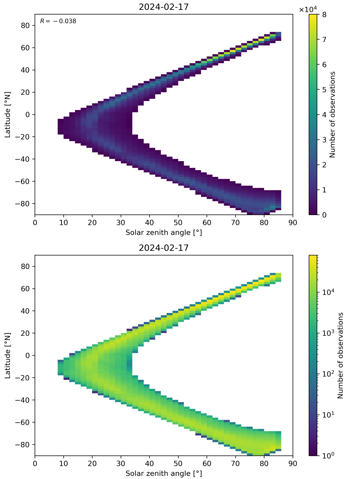
Figure 66: Scatter density plot of “Solar zenith angle” against “Latitude” for 2024-02-17 to 2024-02-18.
