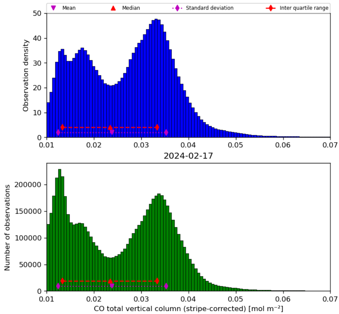
Figure 19: Histogram of “CO total vertical column (stripe-corrected)” for 2024-02-17 to 2024-02-18
