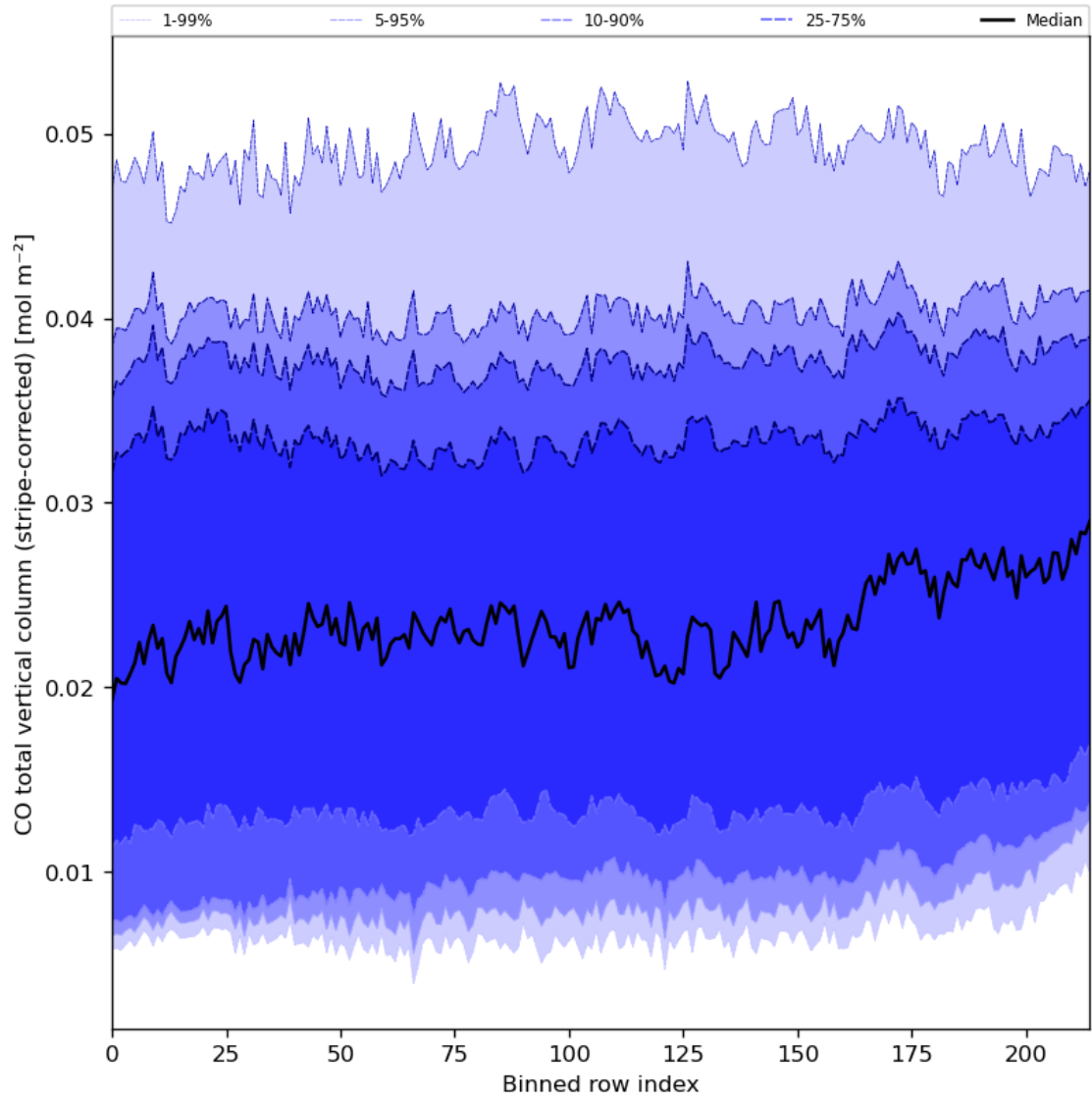
Figure 27: Along track statistics of “CO total vertical column (stripe-corrected)” for 2024-02-17 to 2024-02-18
