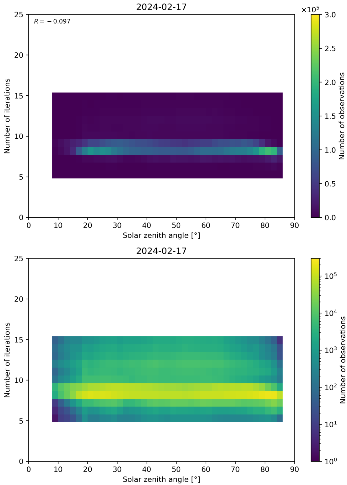
Figure 67: Scatter density plot of “Solar zenith angle” against “Number of iterations” for 2024-02-17 to 2024-02-18.
