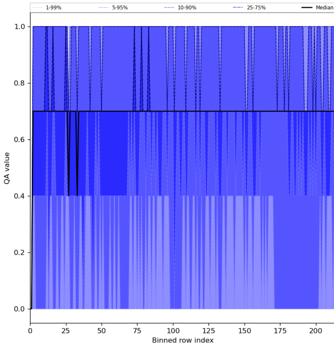
Figure 25: Along track statistics of “QA value” for 2024-02-17 to 2024-02-18
