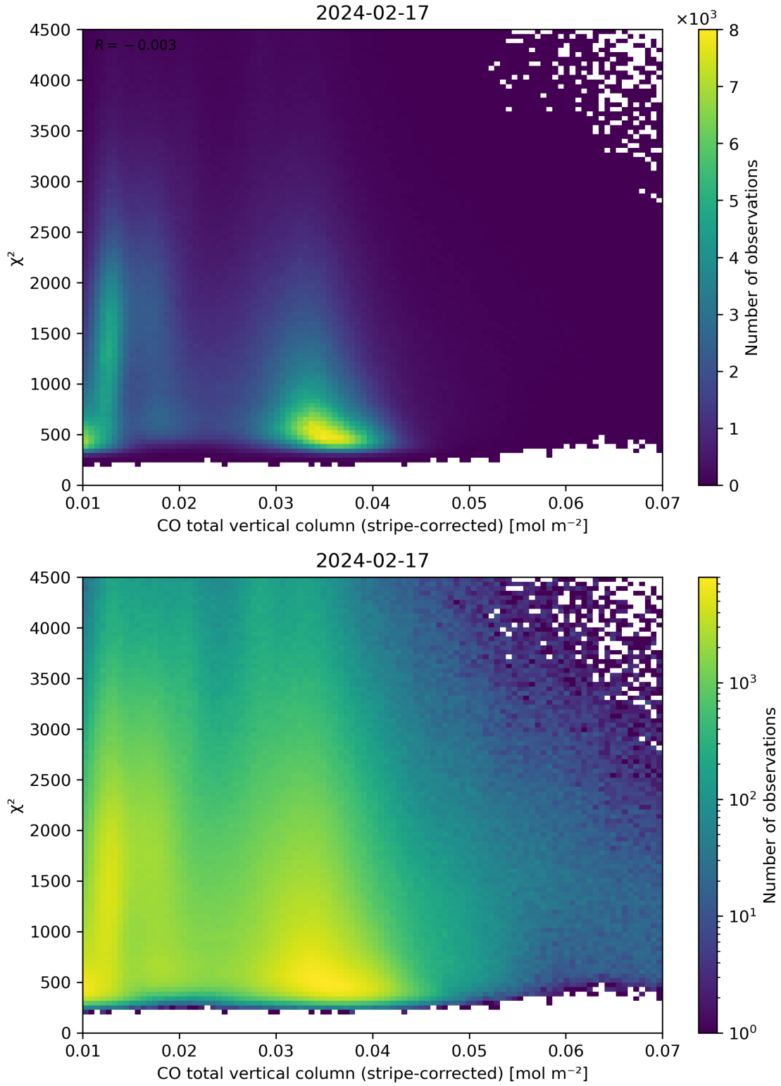
Figure 37: Scatter density plot of “CO total vertical column (stripe-corrected)” against “ \chi^2 ” for 2024-02-17 to 2024-02-18.
