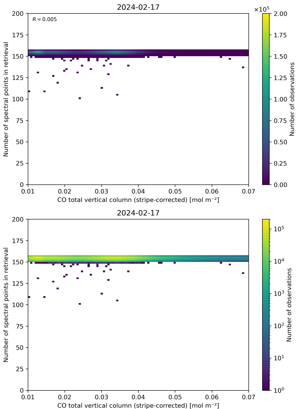
Figure 40: Scatter density plot of “CO total vertical column (stripe-corrected)” against “Number of spectral points in retrieval” for 2024-02-17 to 2024-02-18.
