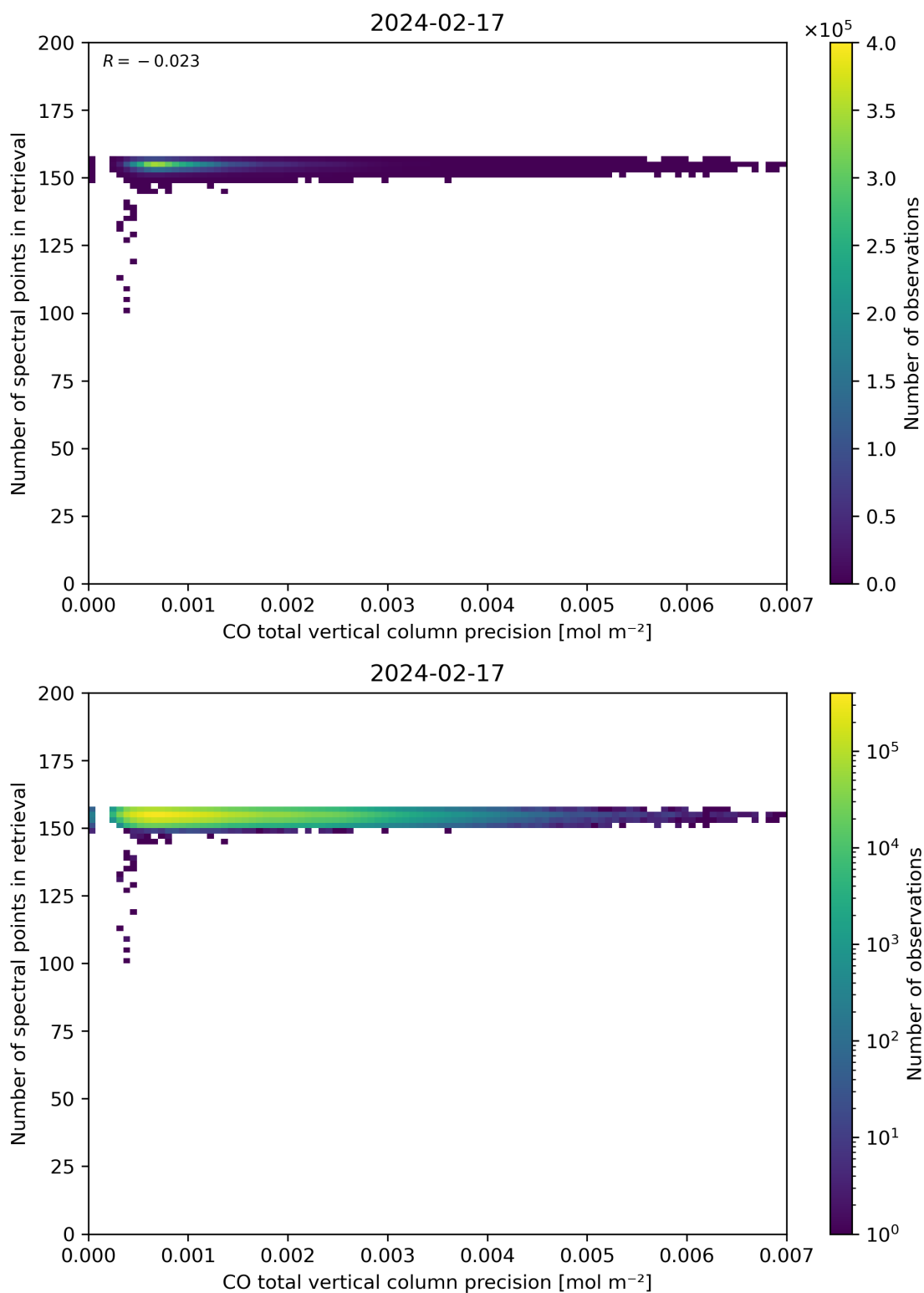
Figure 47: Scatter density plot of “CO total vertical column precision” against “Number of spectral points in retrieval” for 2024-02-17 to 2024-02-18.
