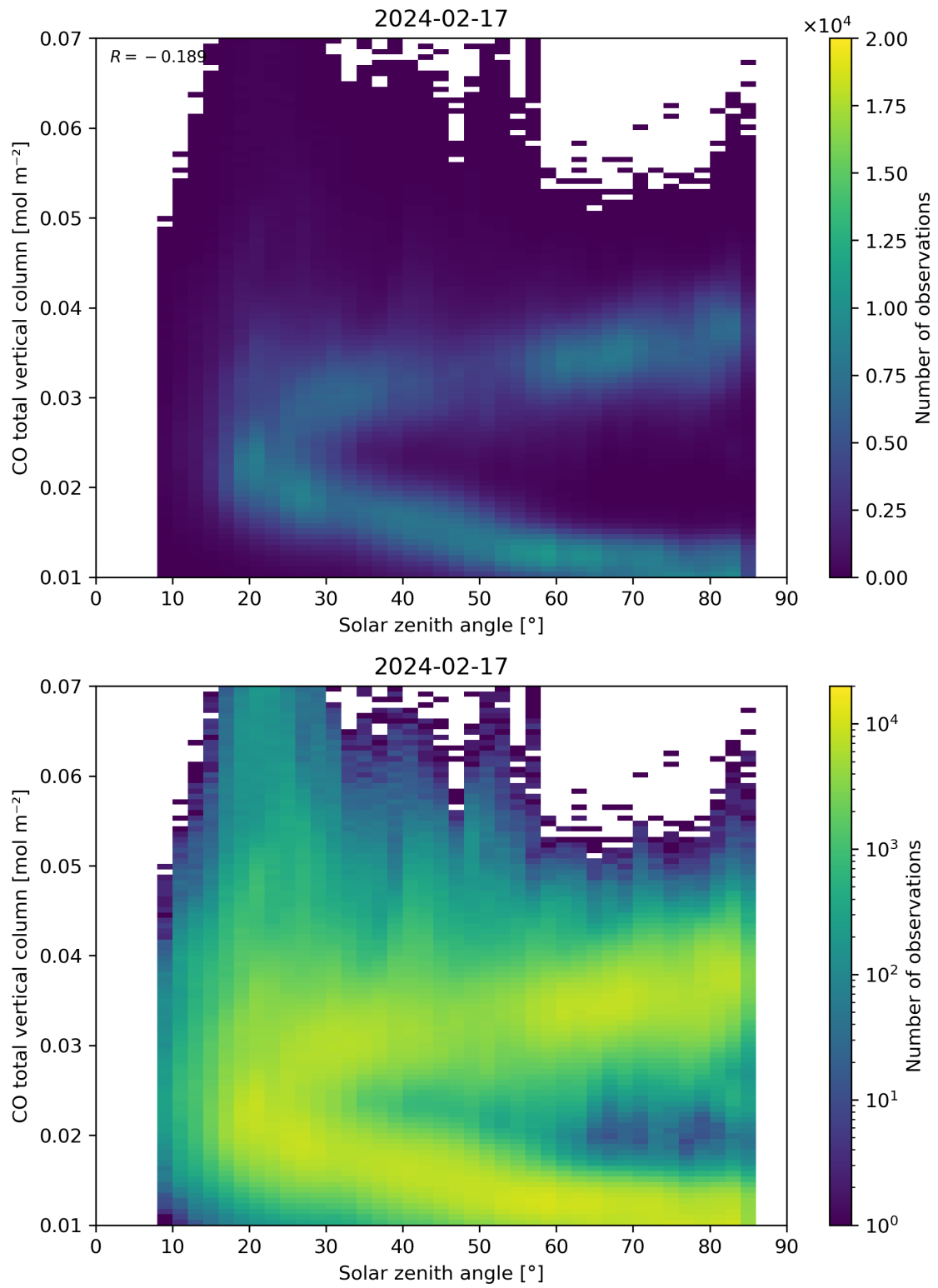
Figure 61: Scatter density plot of “Solar zenith angle” against “CO total vertical column” for 2024-02-17 to 2024-02-18.
