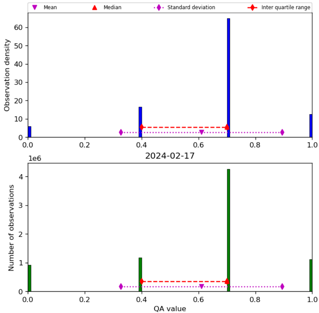
Figure 17: Histogram of “QA value” for 2024-02-17 to 2024-02-18
