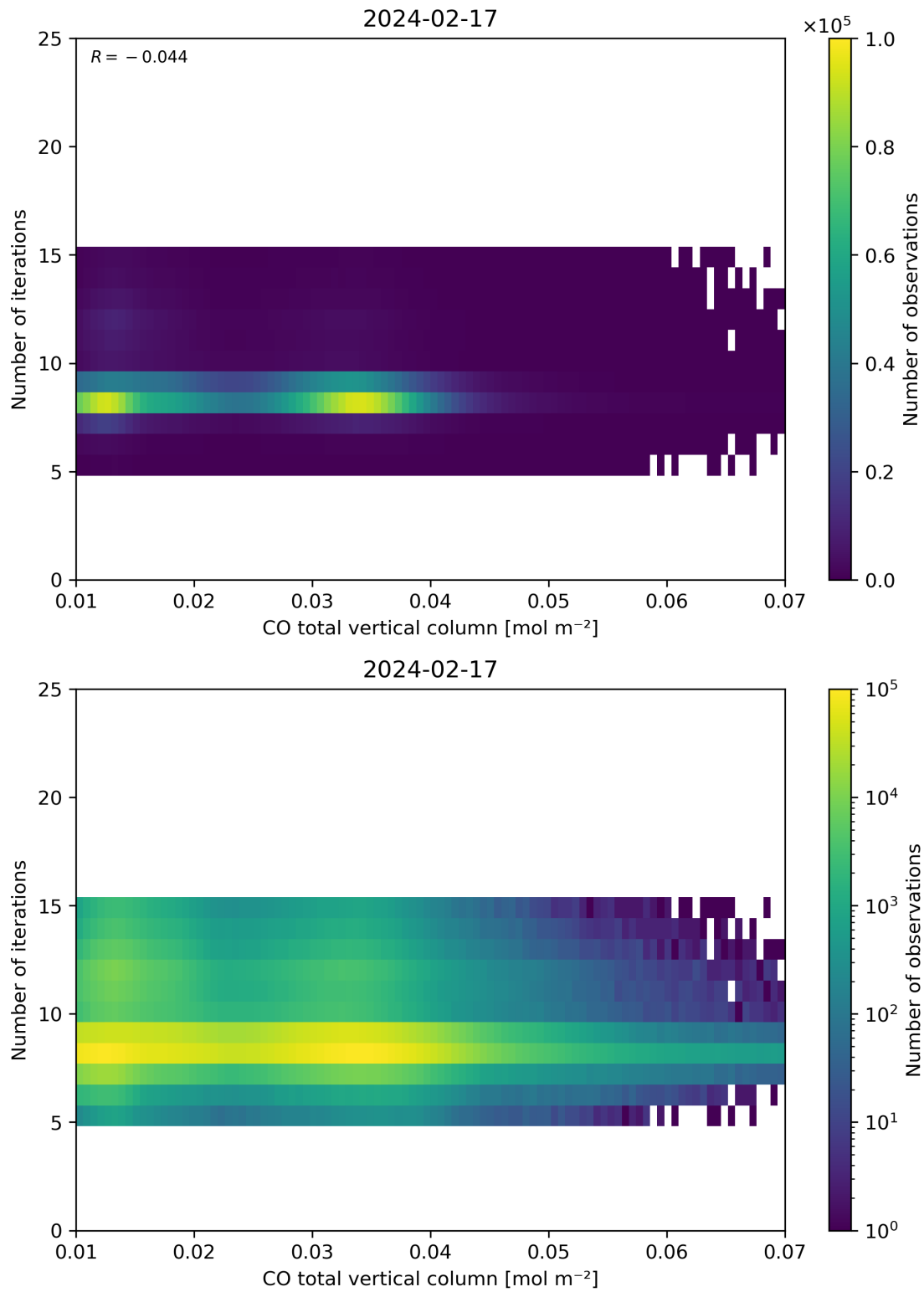
Figure 42: Scatter density plot of “CO total vertical column” against “Number of iterations” for 2024-02-17 to 2024-02-18.
