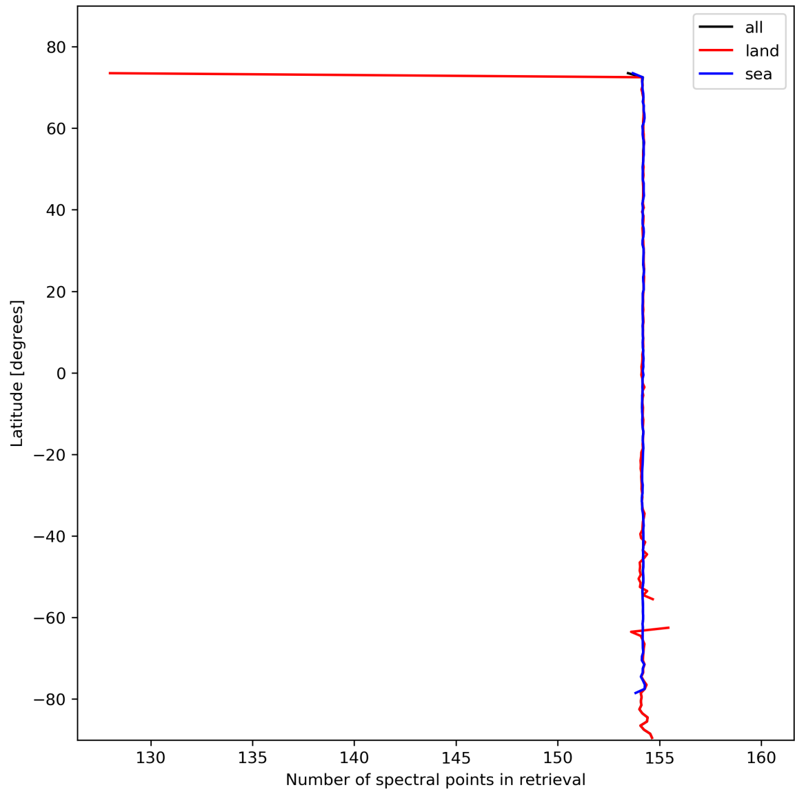
Figure 13: Zonal average of “Number of spectral points in retrieval” for 2024-02-17 to 2024-02-18.
