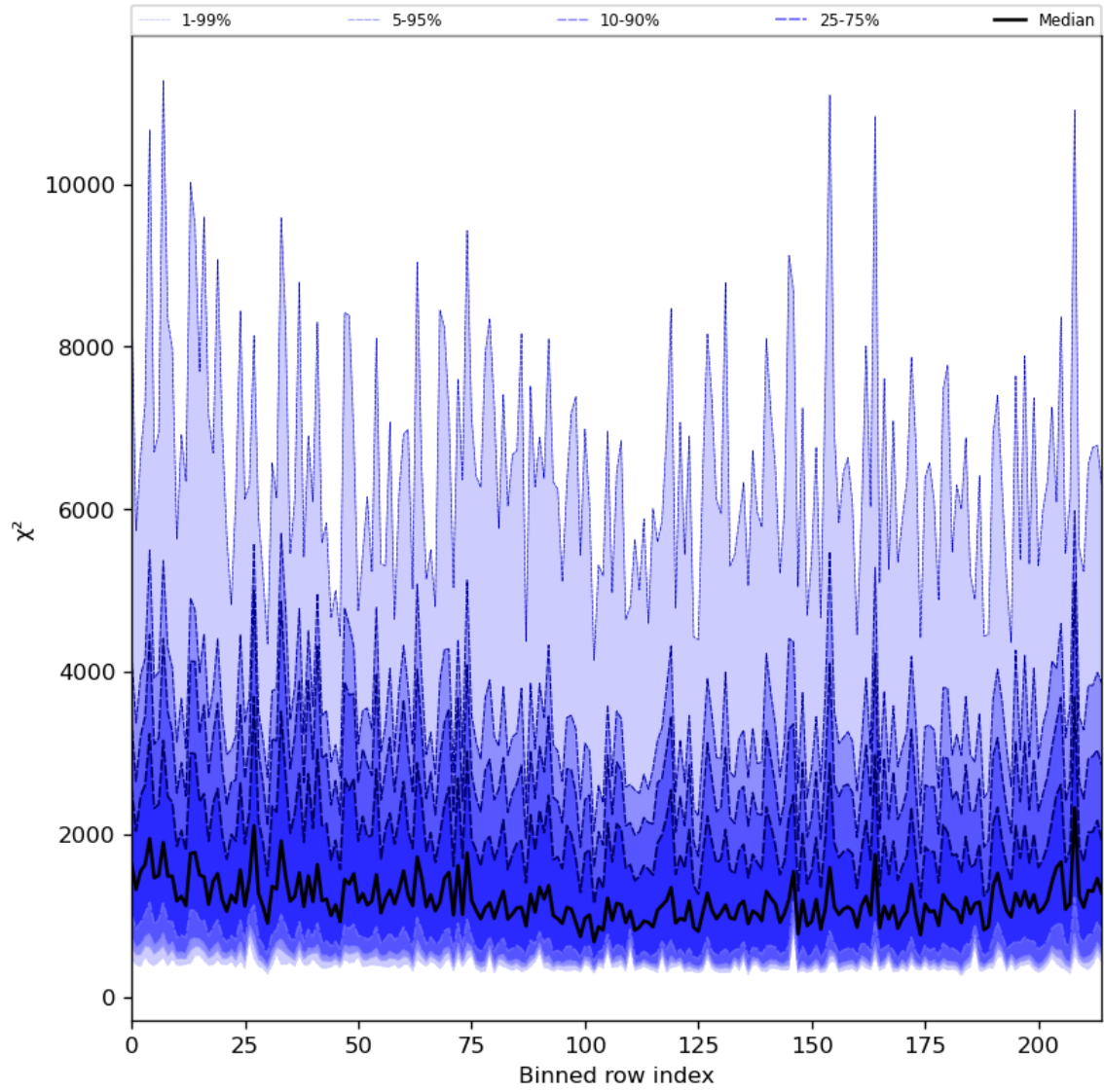
Figure 30: Along track statistics of “ \chi^2 ” for 2024-02-17 to 2024-02-18
