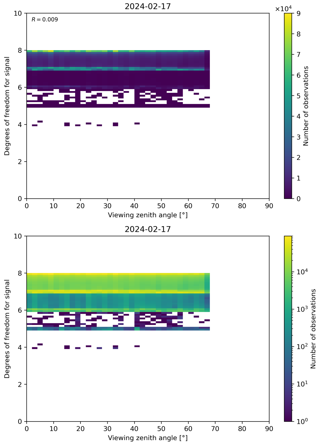
Figure 73: Scatter density plot of “Viewing zenith angle” against “Degrees of freedom for signal” for 2024-02-17 to 2024-02-18.
