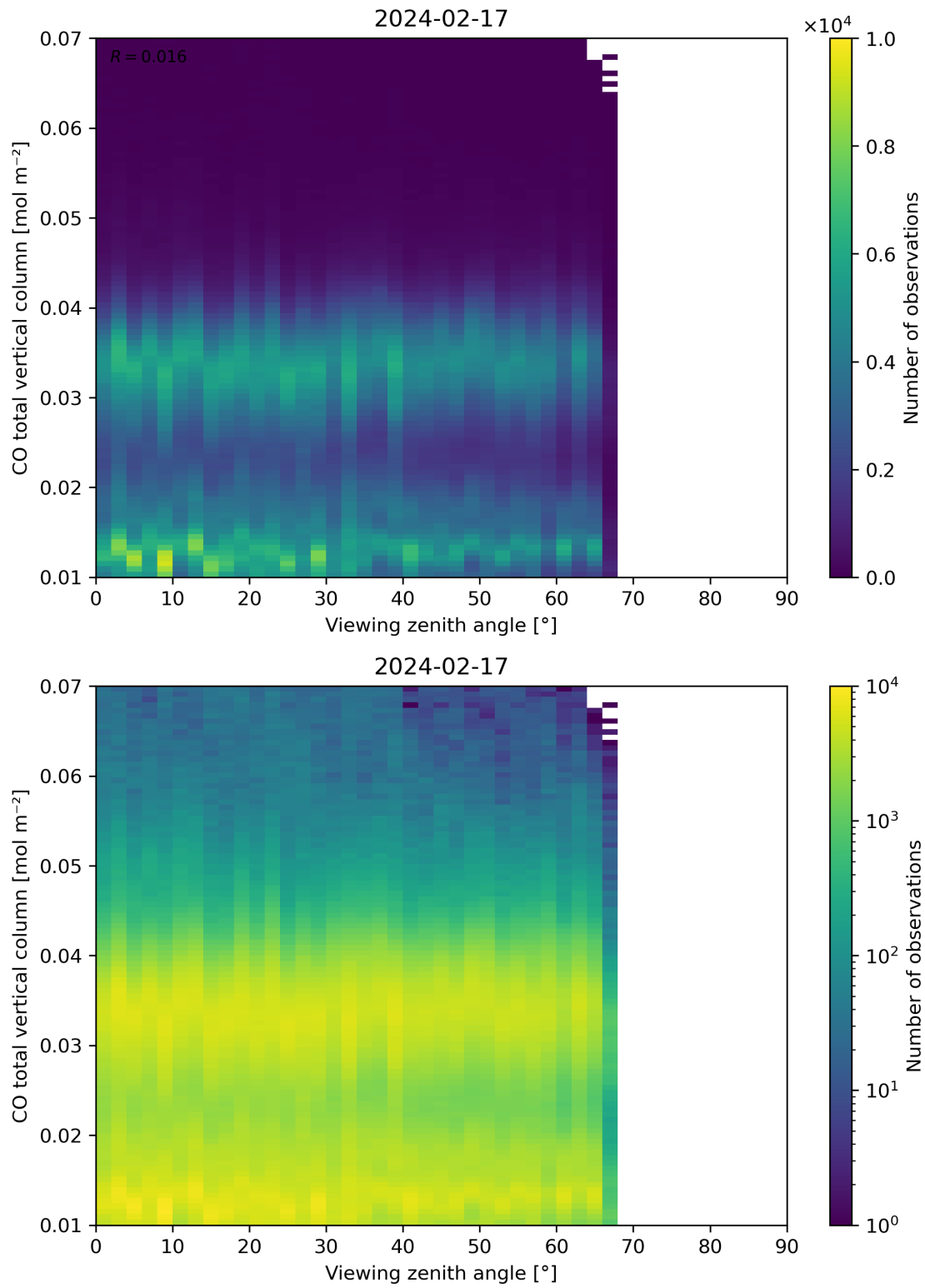
Figure 69: Scatter density plot of “Viewing zenith angle” against “CO total vertical column” for 2024-02-17 to 2024-02-18.
