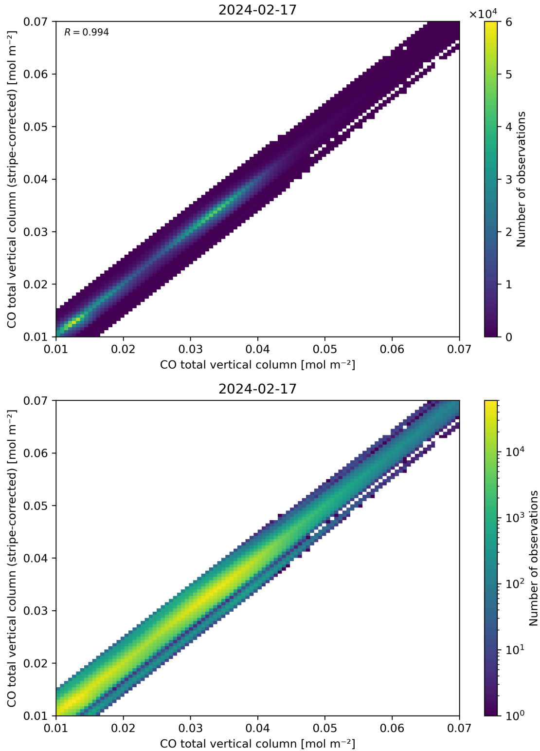
Figure 33: Scatter density plot of “CO total vertical column” against “CO total vertical column (stripe-corrected)” for 2024-02-17 to 2024-02-18.
