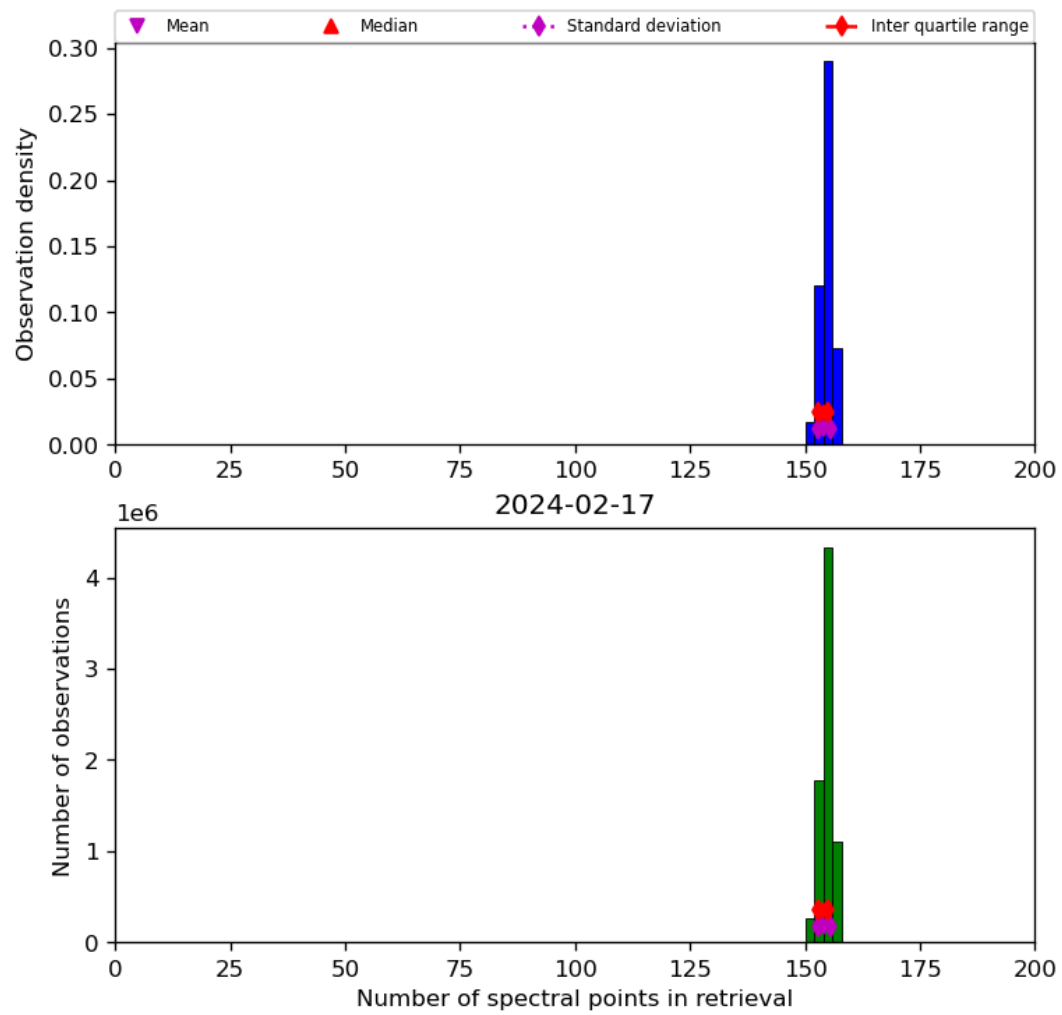
Figure 21: Histogram of “Number of spectral points in retrieval” for 2024-02-17 to 2024-02-18
