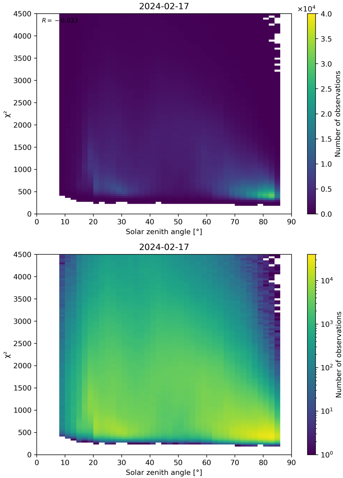
Figure 64: Scatter density plot of “Solar zenith angle” against “ \chi^2 ” for 2024-02-17 to 2024-02-18.
