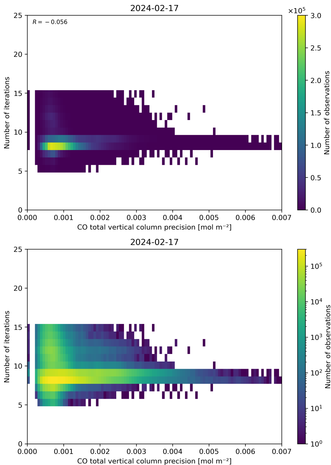
Figure 46: Scatter density plot of “CO total vertical column precision” against “Number of iterations” for 2024-02-17 to 2024-02-18.
