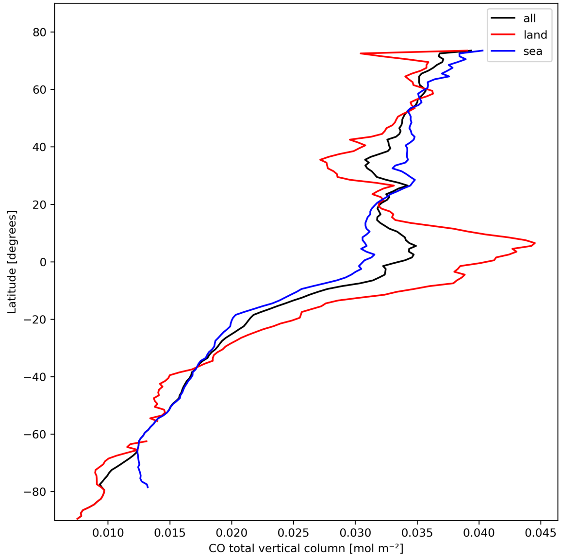
Figure 10: Zonal average of “CO total vertical column” for 2024-02-17 to 2024-02-18.
