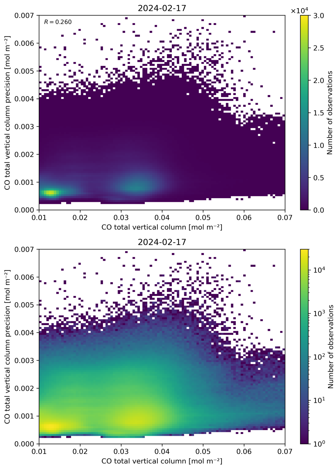
Figure 34: Scatter density plot of “CO total vertical column” against “CO total vertical column precision” for 2024-02-17 to 2024-02-18.
