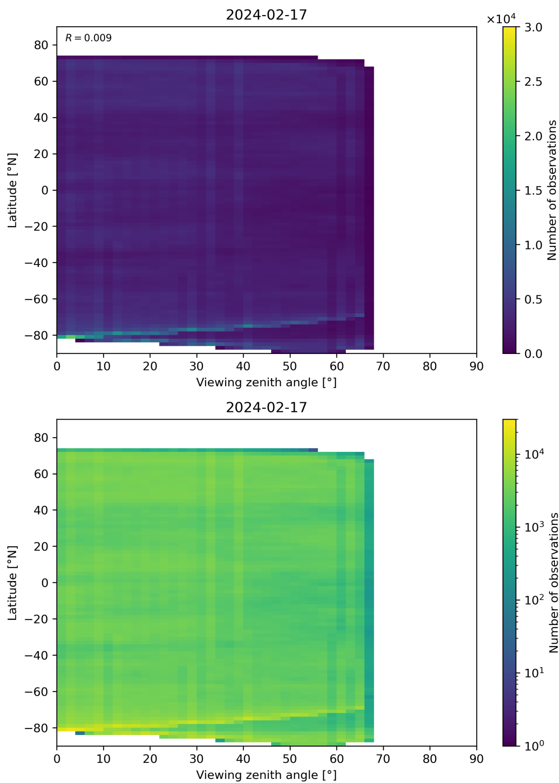
Figure 74: Scatter density plot of “Viewing zenith angle” against “Latitude” for 2024-02-17 to 2024-02-18.
