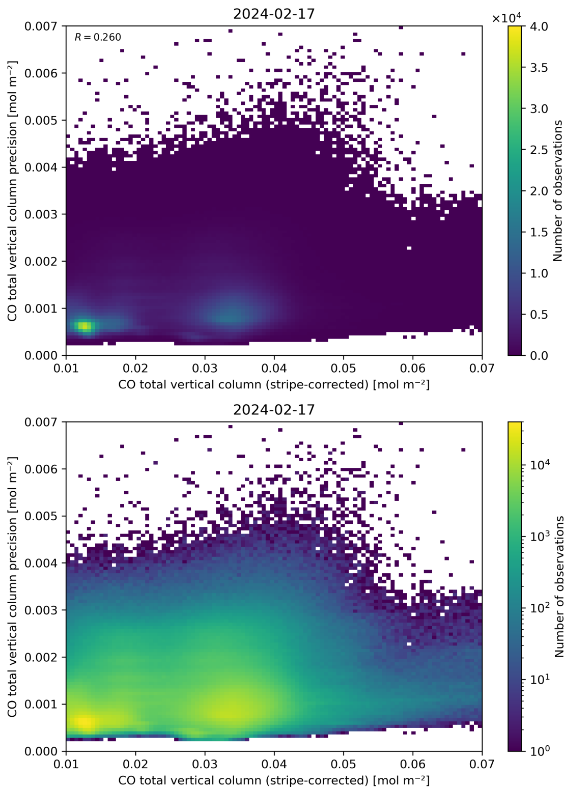
Figure 36: Scatter density plot of “CO total vertical column (stripe-corrected)” against “CO total vertical column precision” for 2024-02-17 to 2024-02-18.
