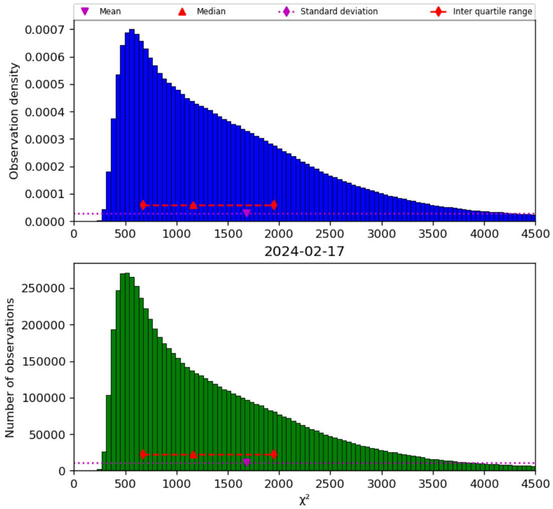
Figure 22: Histogram of “ \chi^2 ” for 2024-02-17 to 2024-02-18
