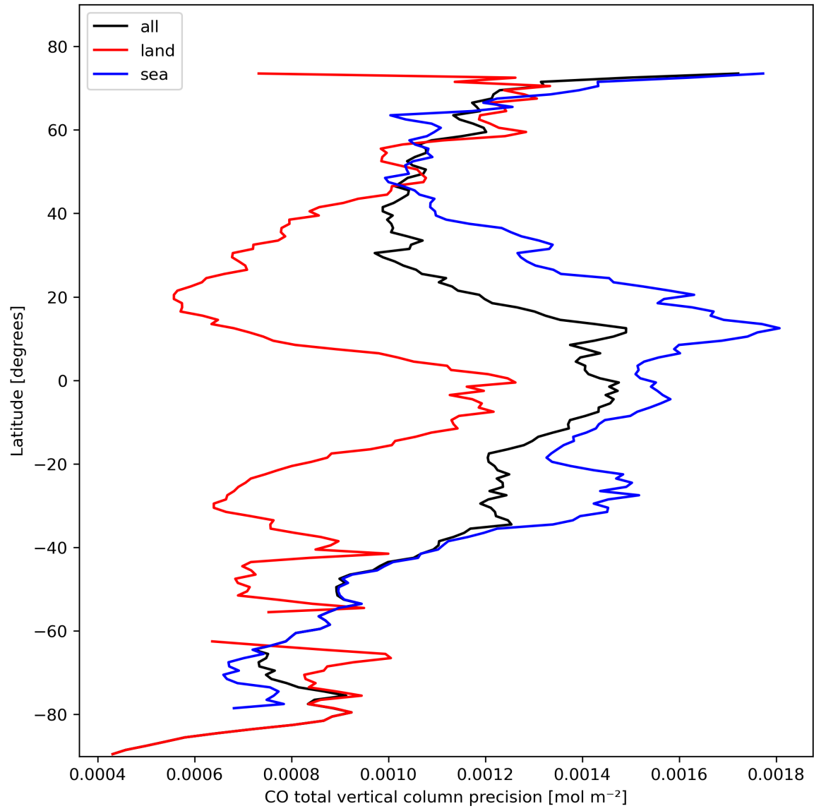
Figure 12: Zonal average of “CO total vertical column precision” for 2024-02-17 to 2024-02-18.
