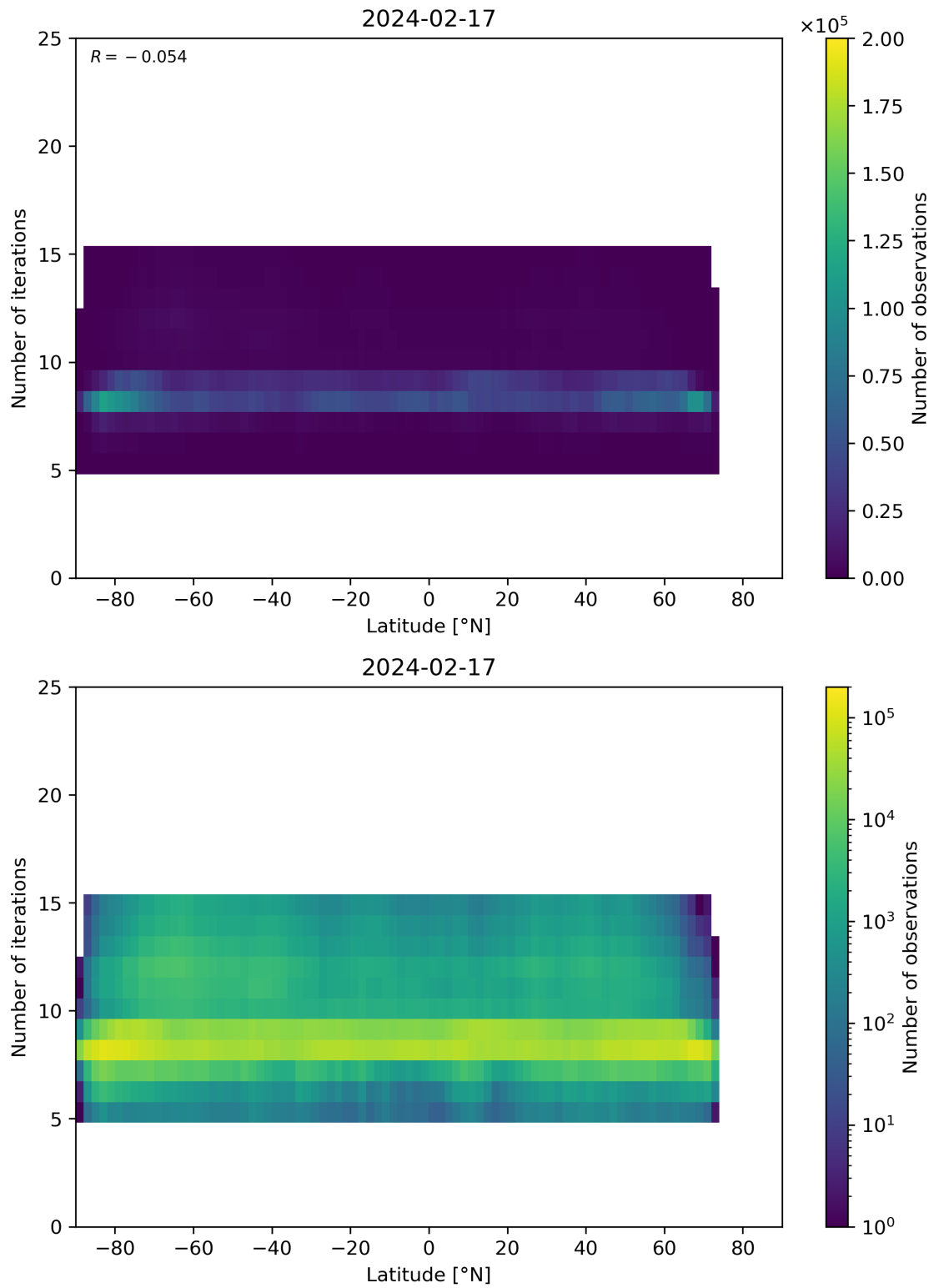
Figure 56: Scatter density plot of “Latitude” against “Number of iterations” for 2024-02-17 to 2024-02-18.
