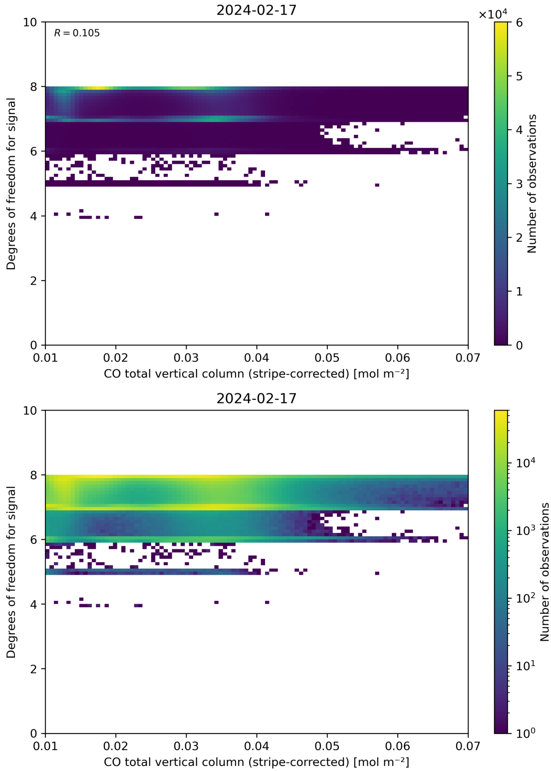
Figure 38: Scatter density plot of “CO total vertical column (stripe-corrected)” against “Degrees of freedom for signal” for 2024-02-17 to 2024-02-18.
