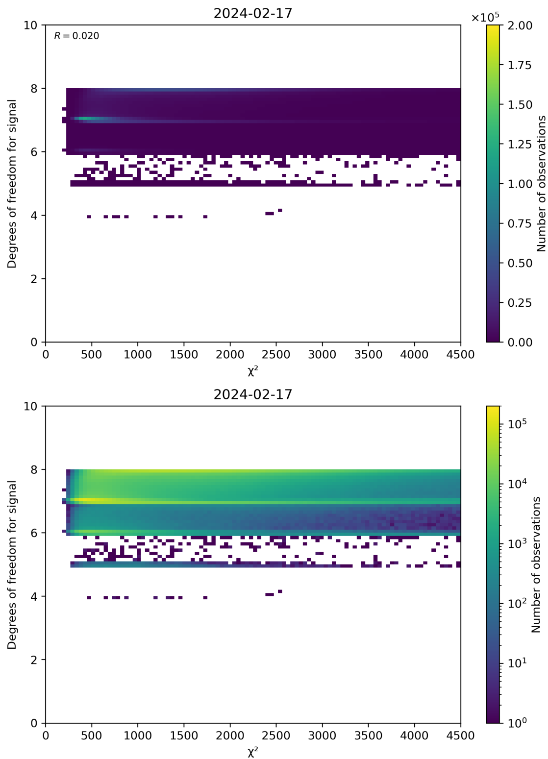
Figure 48: Scatter density plot of “ \chi^2 ” against “Degrees of freedom for signal” for 2024-02-17 to 2024-02-18.
