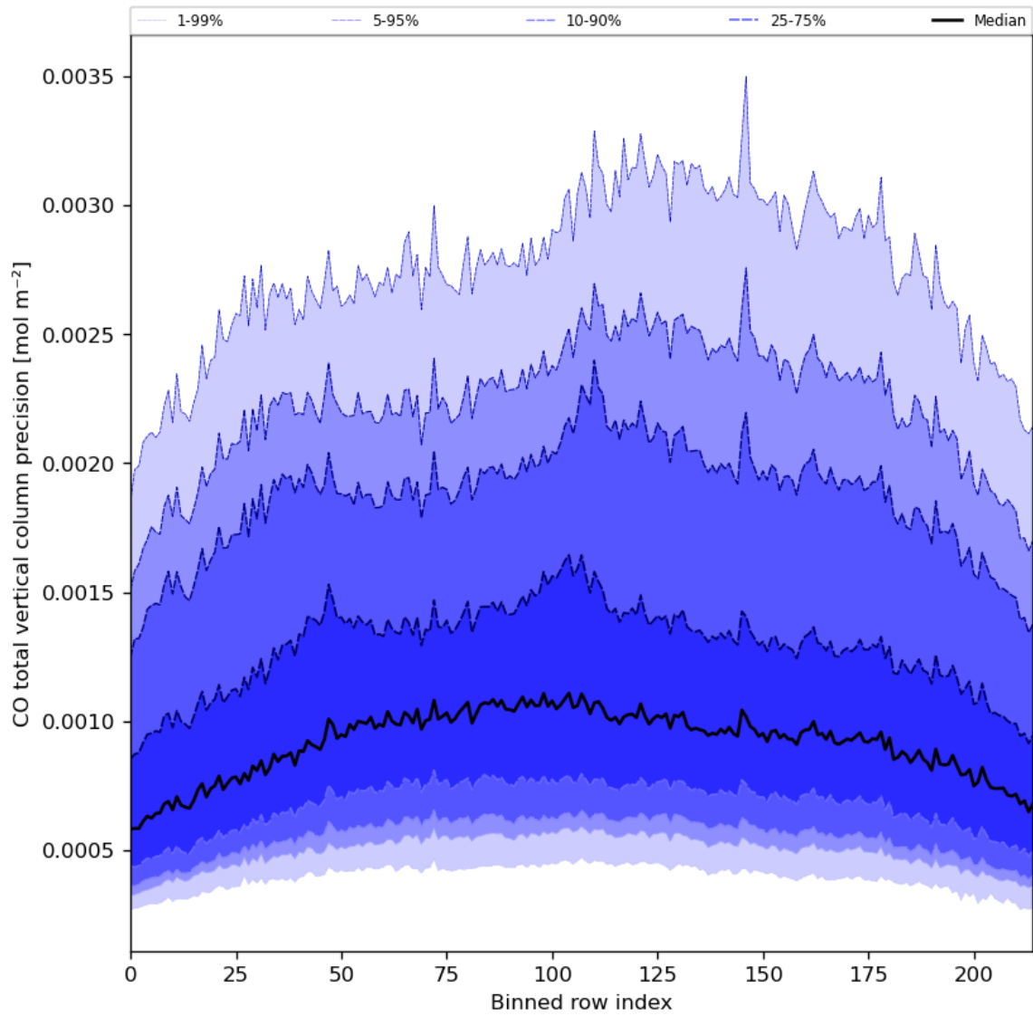
Figure 28: Along track statistics of “CO total vertical column precision” for 2024-02-17 to 2024-02-18
