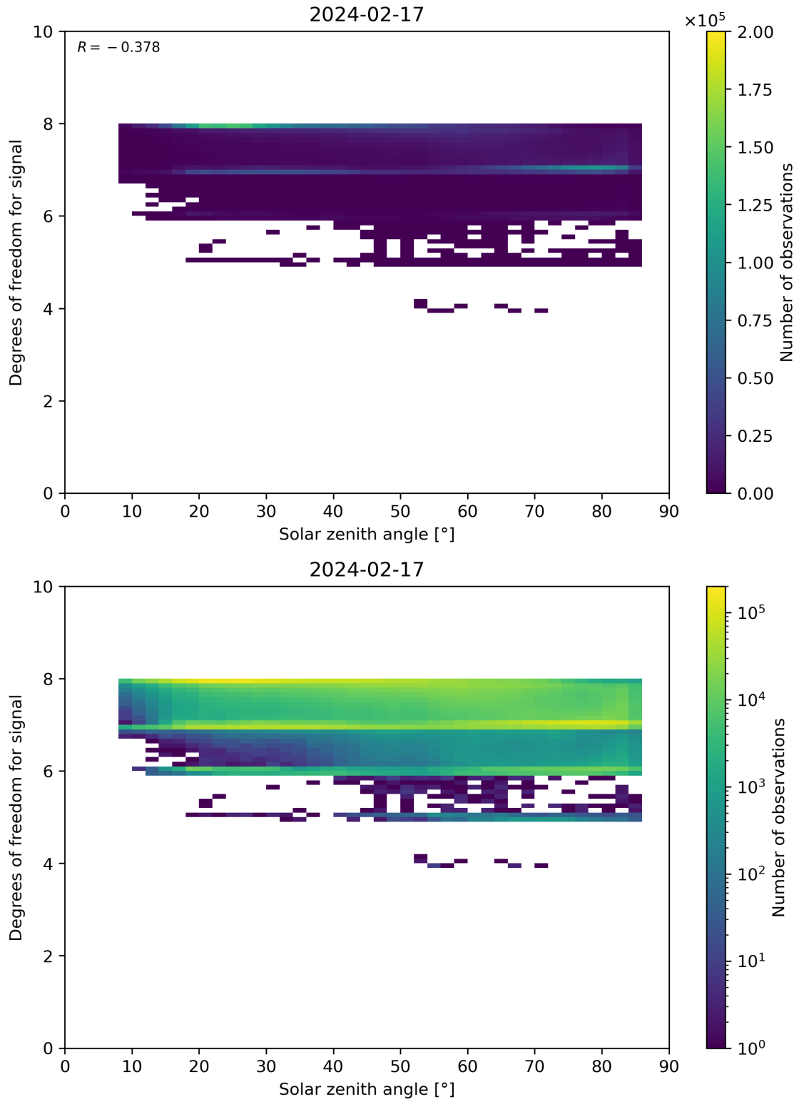
Figure 65: Scatter density plot of “Solar zenith angle” against “Degrees of freedom for signal” for 2024-02-17 to 2024-02-18.
