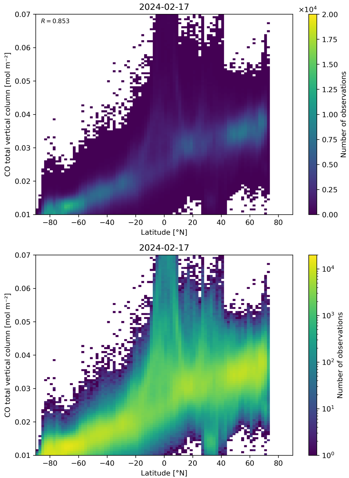
Figure 51: Scatter density plot of “Latitude” against “CO total vertical column” for 2024-02-17 to 2024-02-18.
