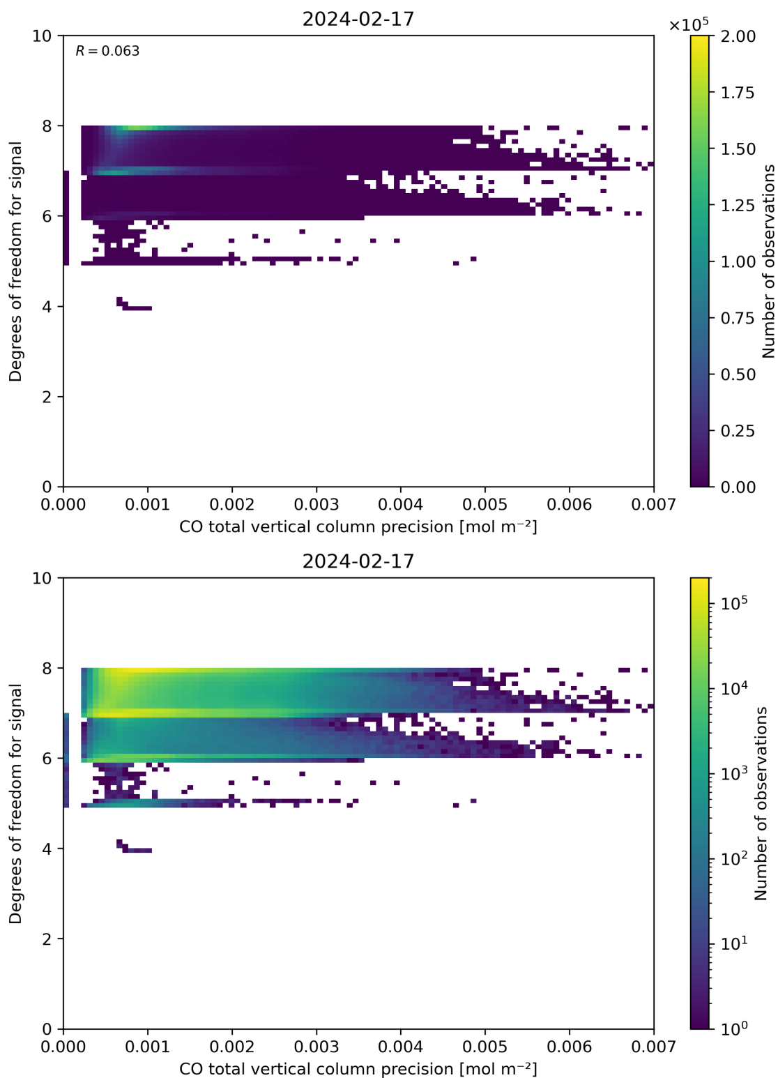
Figure 45: Scatter density plot of “CO total vertical column precision” against “Degrees of freedom for signal” for 2024-02-17 to 2024-02-18.
