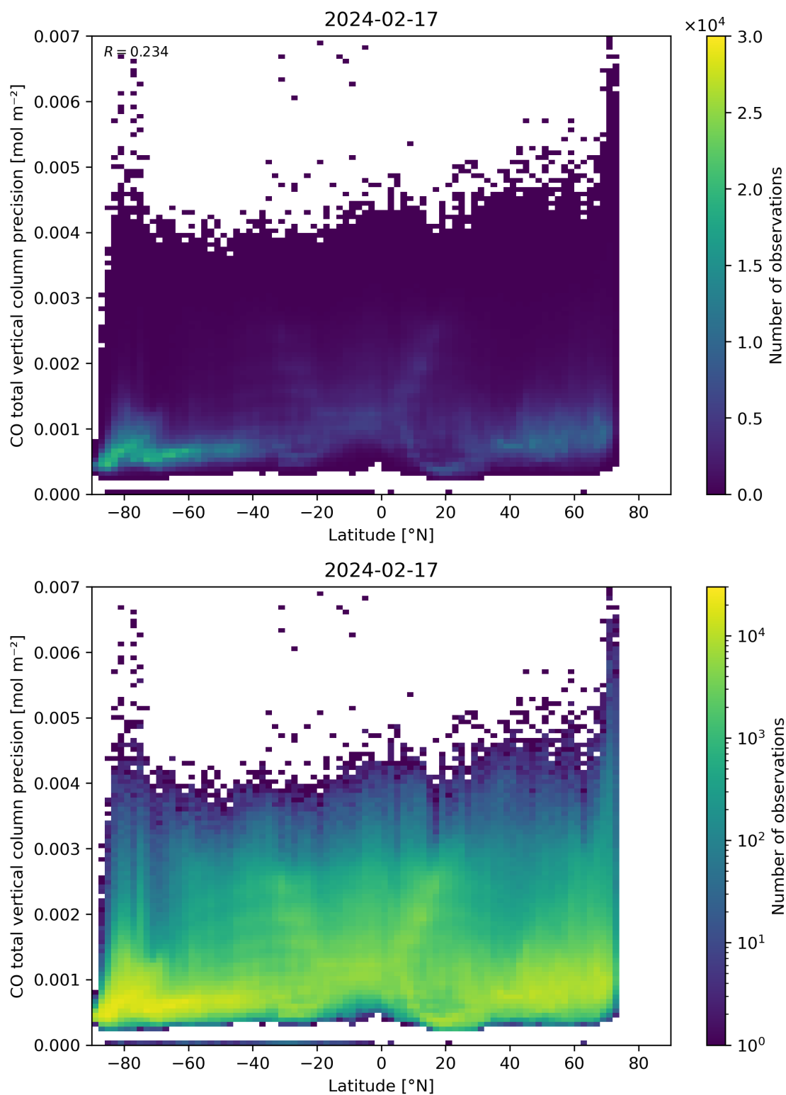
Figure 53: Scatter density plot of “Latitude” against “CO total vertical column precision” for 2024-02-17 to 2024-02-18.
