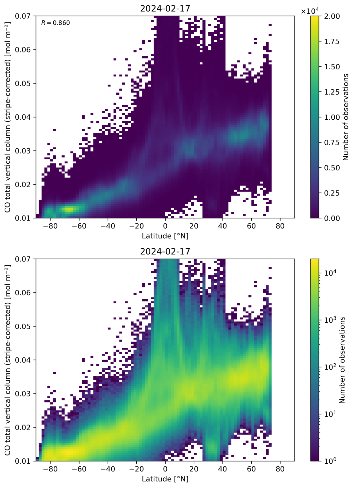
Figure 52: Scatter density plot of “Latitude” against “CO total vertical column (stripe-corrected)” for 2024-02-17 to 2024-02-18.
