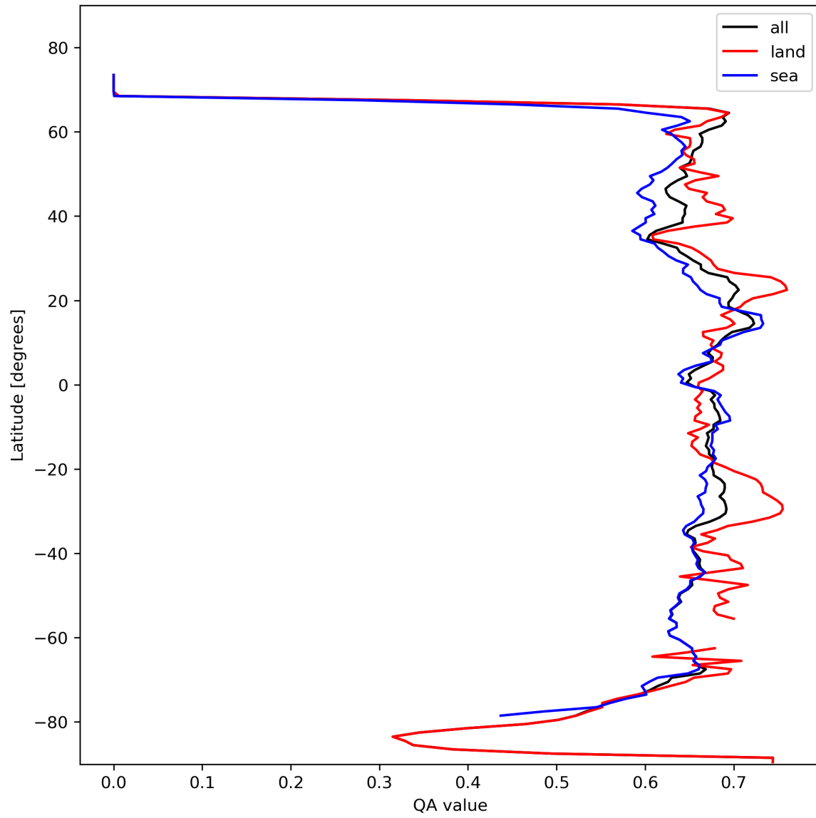
Figure 9: Zonal average of “QA value” for 2024-02-17 to 2024-02-18.
