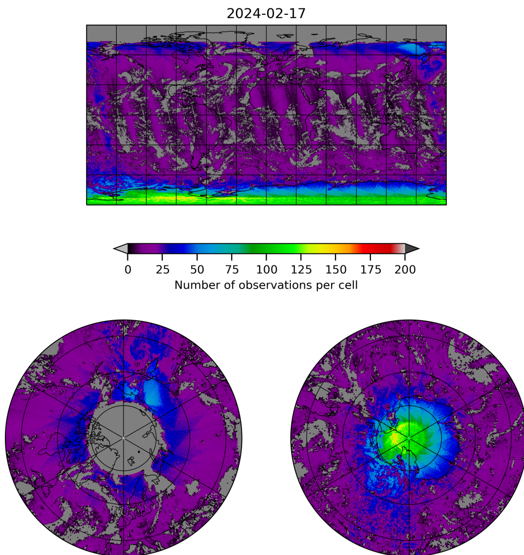
Figure 8: Map of the number of observations for 2024-02-17 to 2024-02-18
