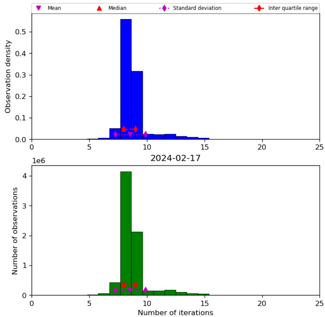
Figure 24: Histogram of “Number of iterations” for 2024-02-17 to 2024-02-18
