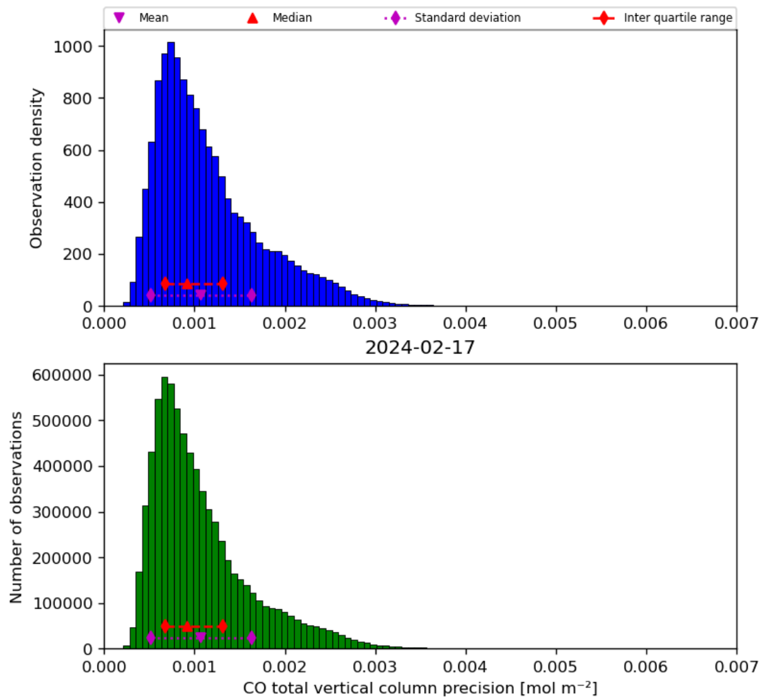
Figure 20: Histogram of “CO total vertical column precision” for 2024-02-17 to 2024-02-18
