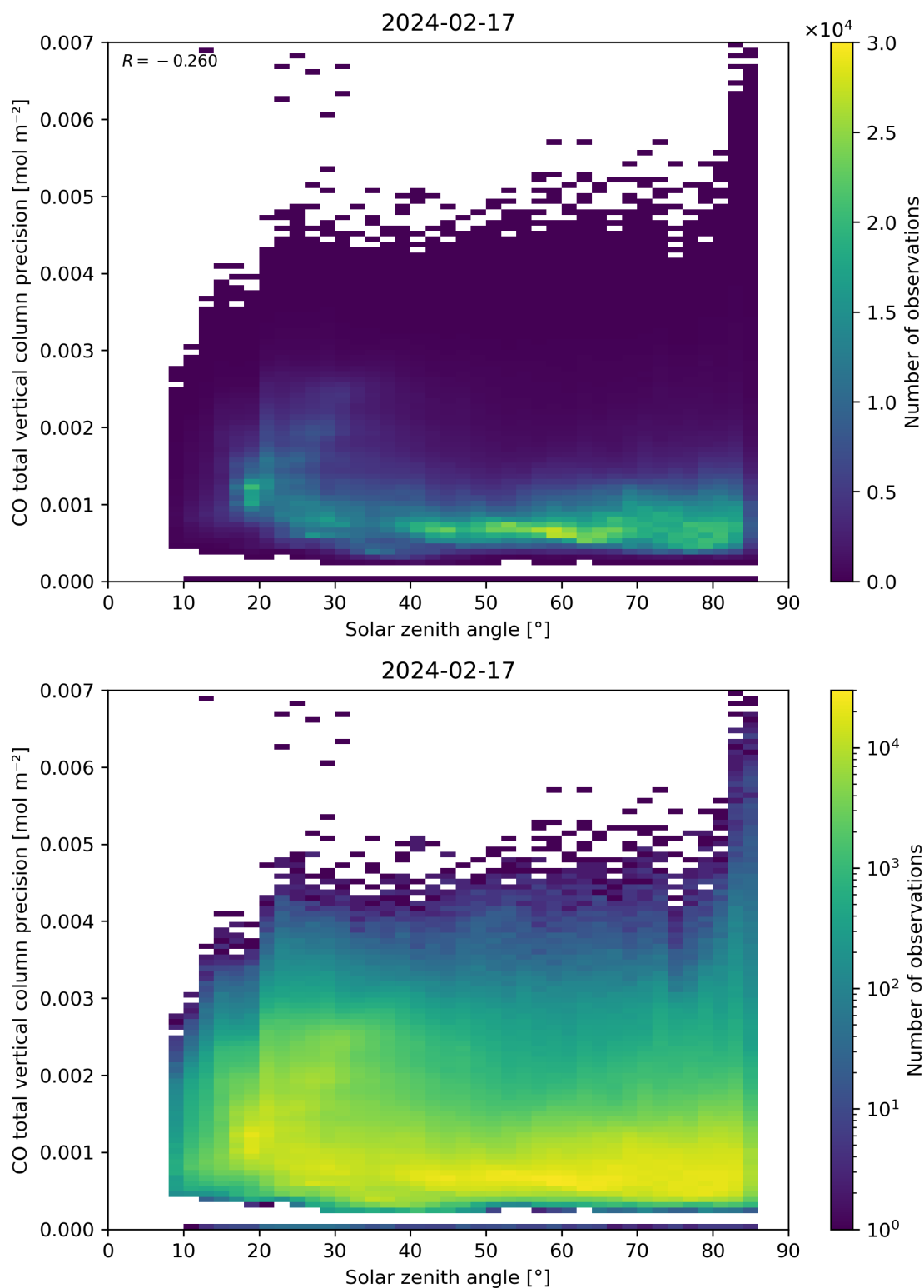
Figure 63: Scatter density plot of “Solar zenith angle” against “CO total vertical column precision” for 2024-02-17 to 2024-02-18.
