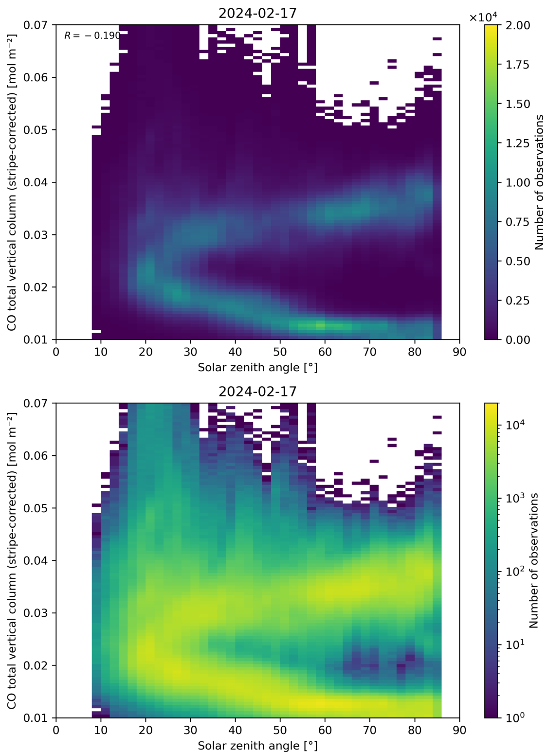
Figure 62: Scatter density plot of “Solar zenith angle” against “CO total vertical column (stripe-corrected)” for 2024-02-17 to 2024-02-18.
