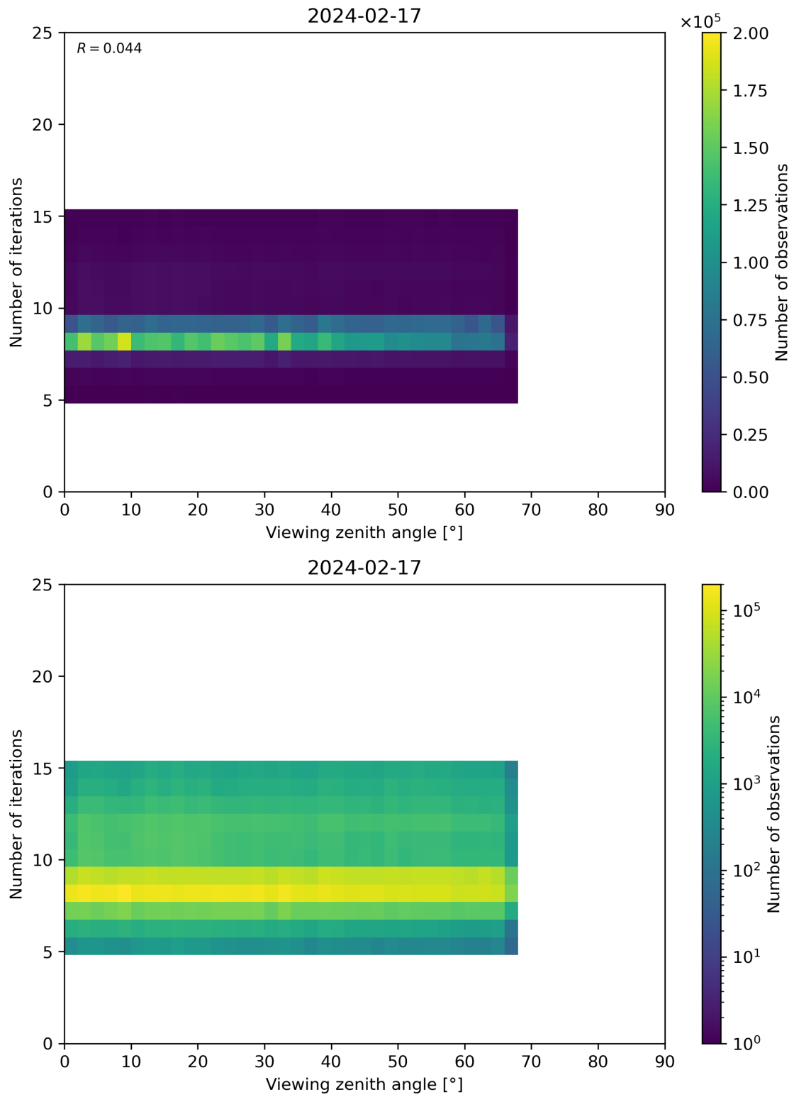
Figure 75: Scatter density plot of “Viewing zenith angle” against “Number of iterations” for 2024-02-17 to 2024-02-18.
