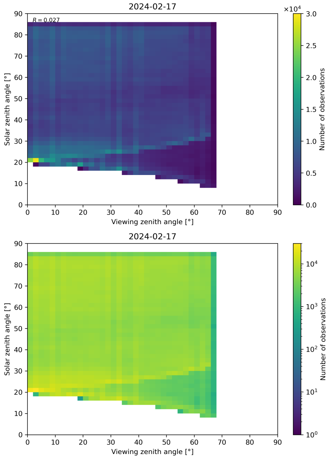
Figure 77: Scatter density plot of “Viewing zenith angle” against “Solar zenith angle” for 2024-02-17 to 2024-02-18.
