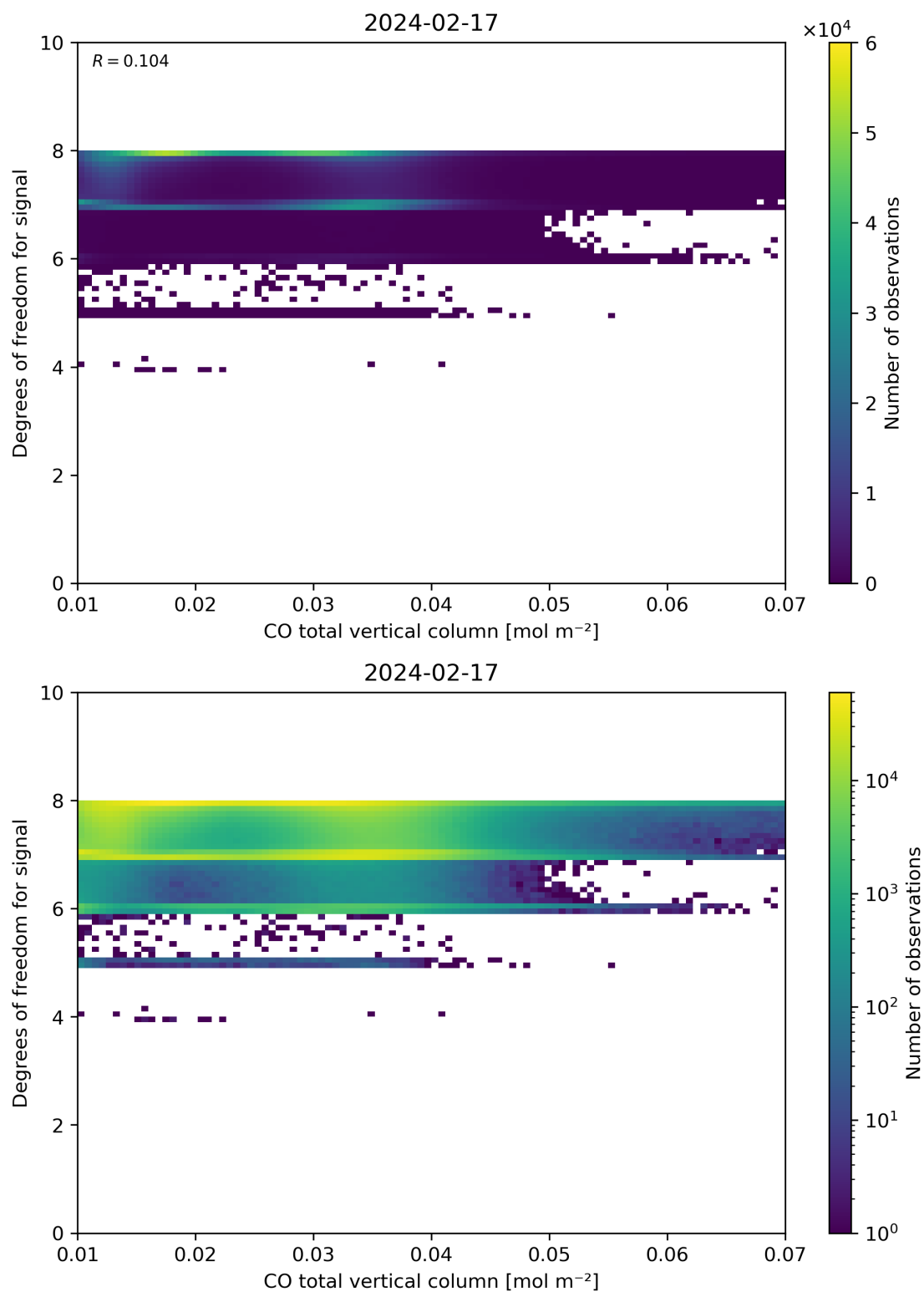
Figure 41: Scatter density plot of “CO total vertical column” against “Degrees of freedom for signal” for 2024-02-17 to 2024-02-18.
