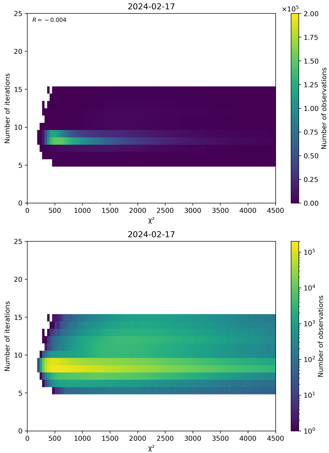
Figure 49: Scatter density plot of “ \chi^2 ” against “Number of iterations” for 2024-02-17 to 2024-02-18.
