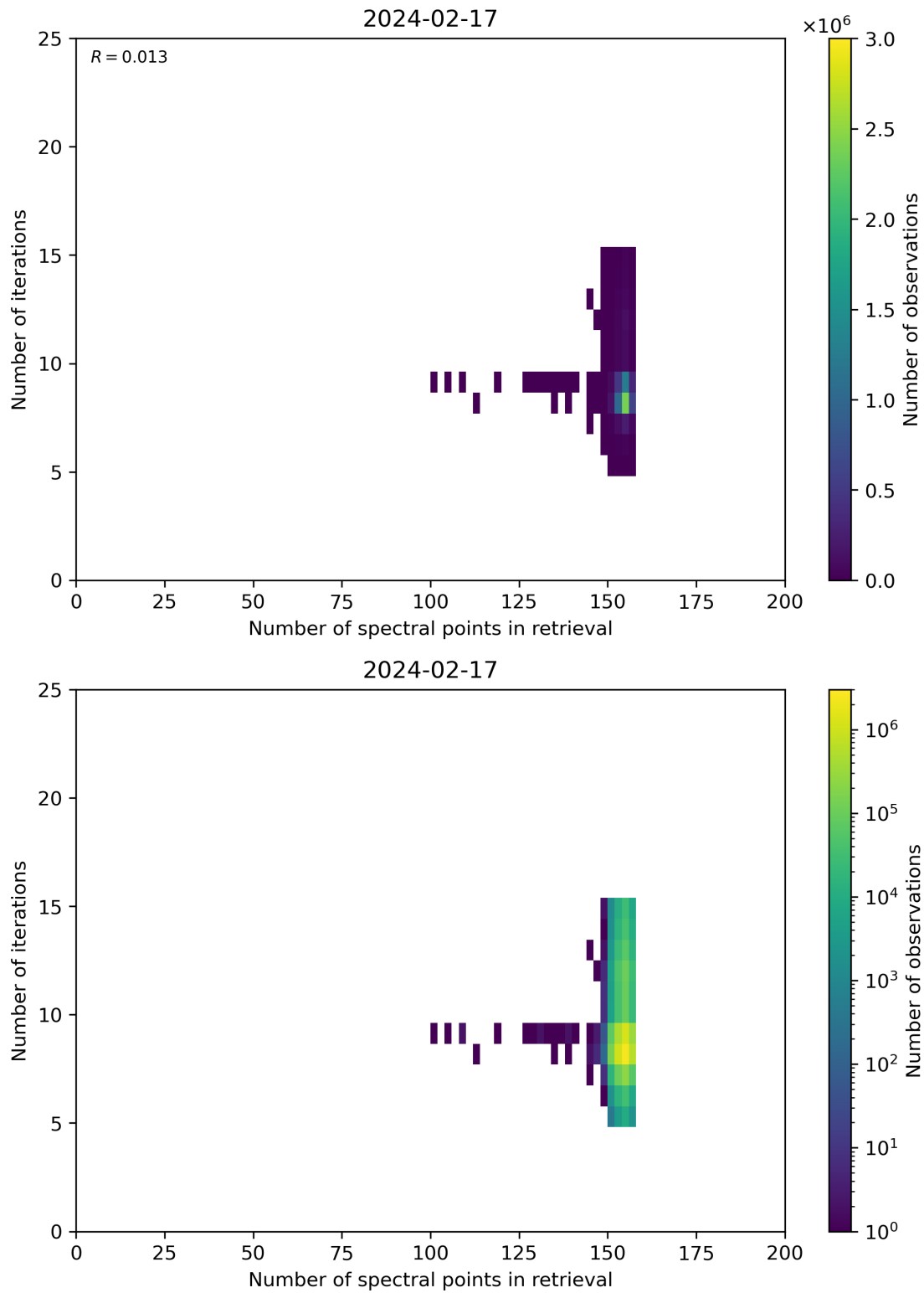
Figure 60: Scatter density plot of “Number of spectral points in retrieval” against “Number of iterations” for 2024-02-17 to 2024-02-18.
