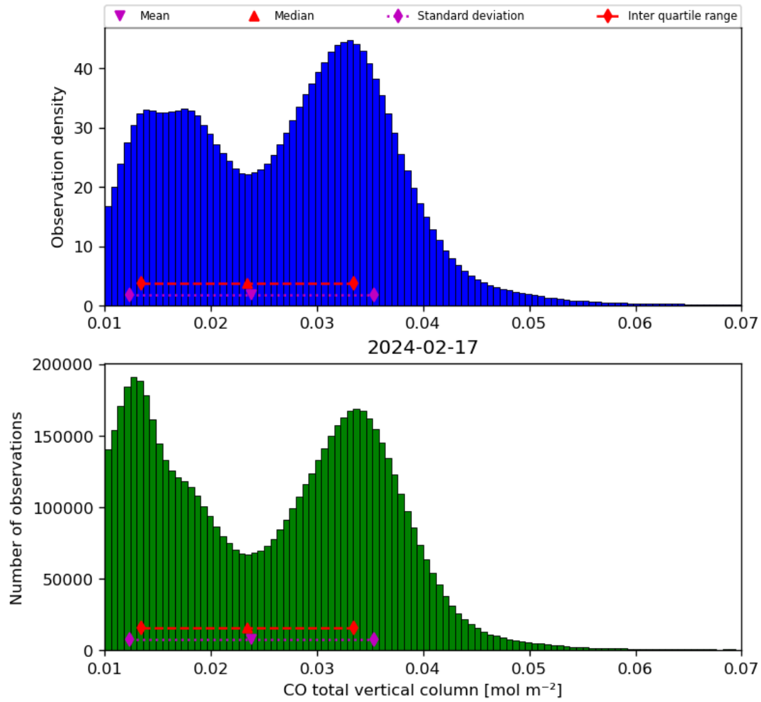
Figure 18: Histogram of “CO total vertical column” for 2024-02-17 to 2024-02-18
