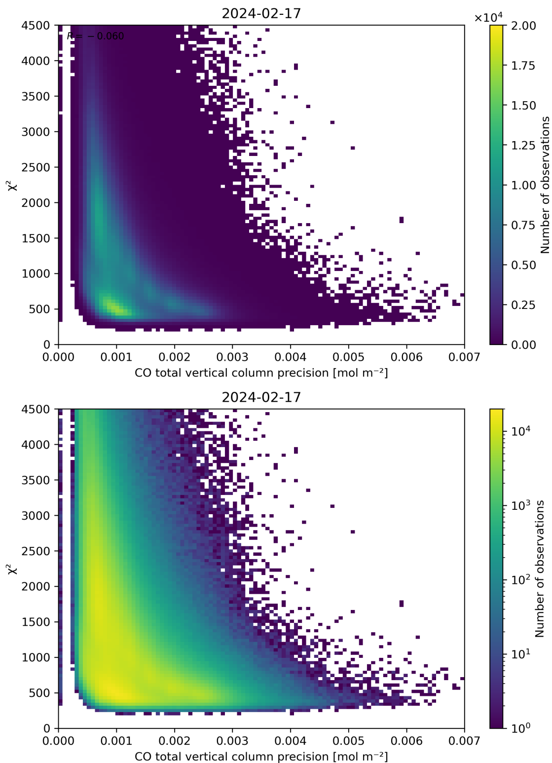
Figure 44: Scatter density plot of “CO total vertical column precision” against “ \chi^2 ” for 2024-02-17 to 2024-02-18.
