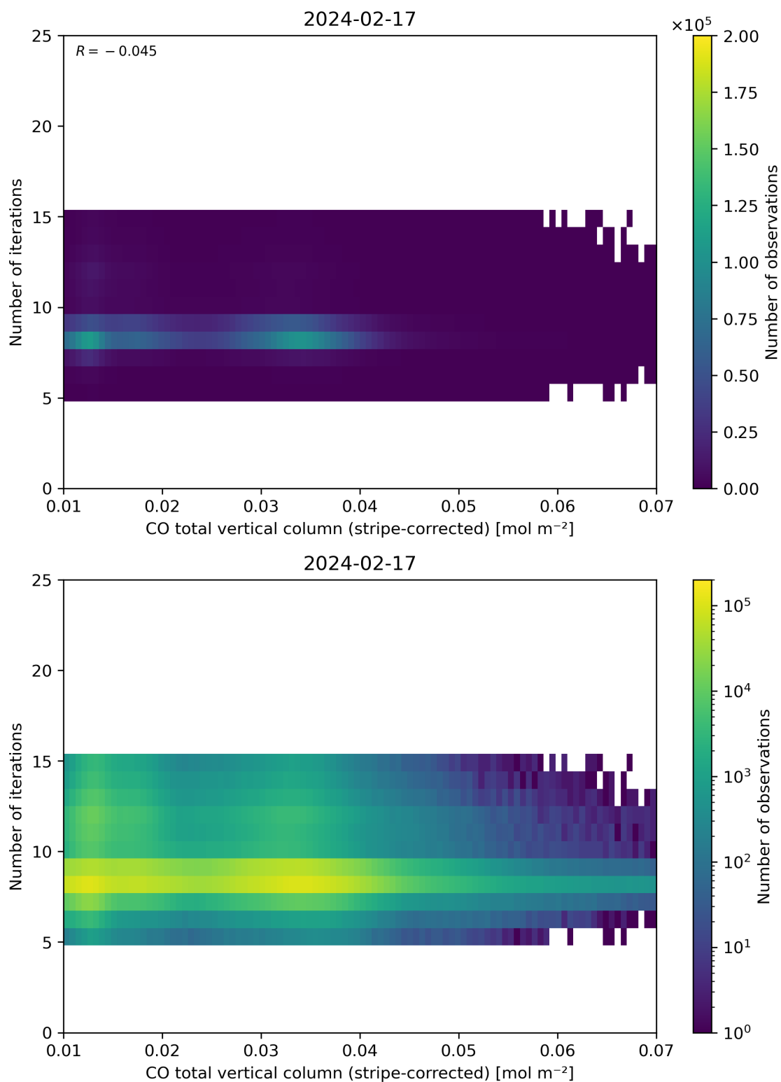
Figure 39: Scatter density plot of “CO total vertical column (stripe-corrected)” against “Number of iterations” for 2024-02-17 to 2024-02-18.
