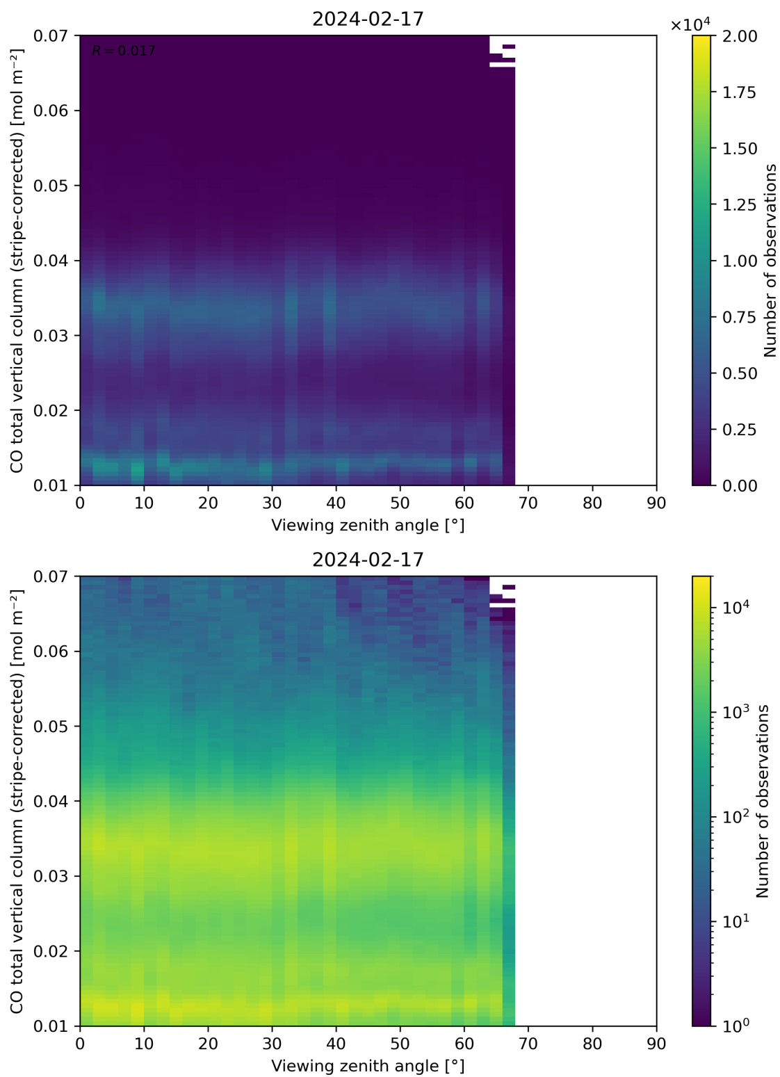
Figure 70: Scatter density plot of “Viewing zenith angle” against “CO total vertical column (stripe-corrected)” for 2024-02-17 to 2024-02-18.
