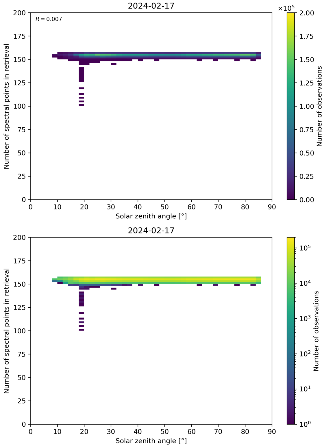
Figure 68: Scatter density plot of “Solar zenith angle” against “Number of spectral points in retrieval” for 2024-02-17 to 2024-02-18.
