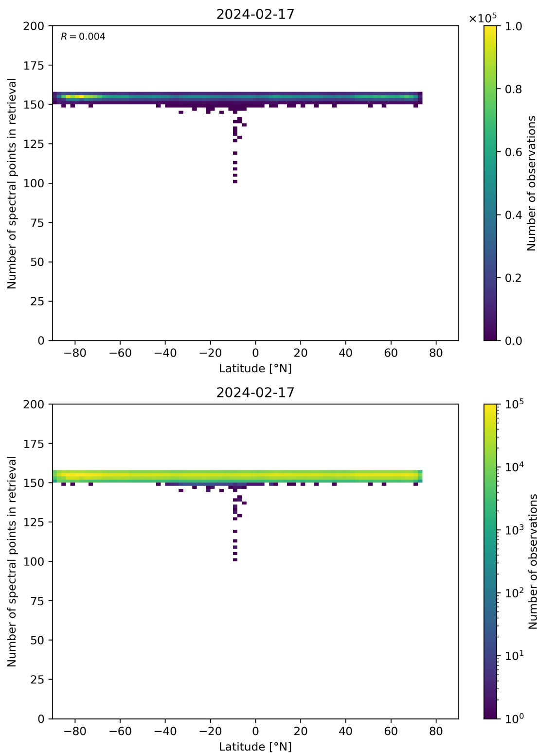
Figure 57: Scatter density plot of “Latitude” against “Number of spectral points in retrieval” for 2024-02-17 to 2024-02-18.
