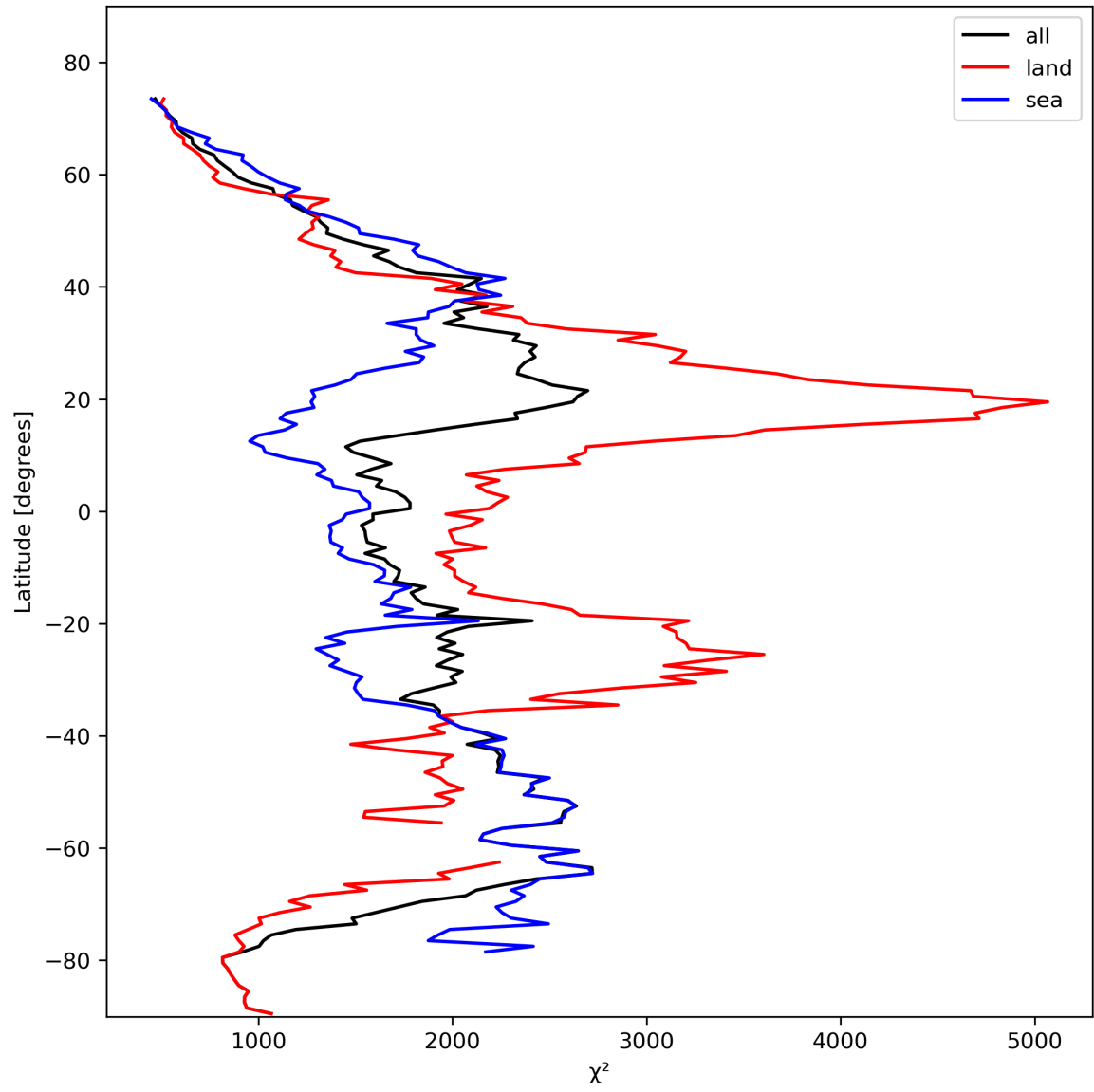
Figure 14: Zonal average of “ \chi^2 ” for 2024-02-17 to 2024-02-18.
