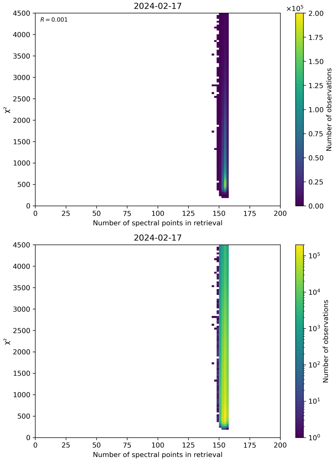
Figure 58: Scatter density plot of “Number of spectral points in retrieval” against “ \chi^2 ” for 2024-02-17 to 2024-02-18.
