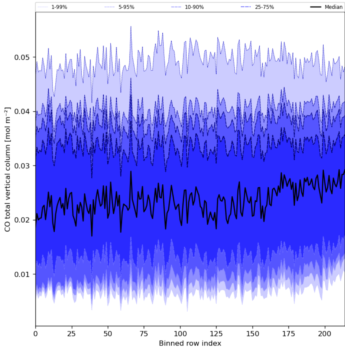
Figure 26: Along track statistics of “CO total vertical column” for 2024-02-17 to 2024-02-18
