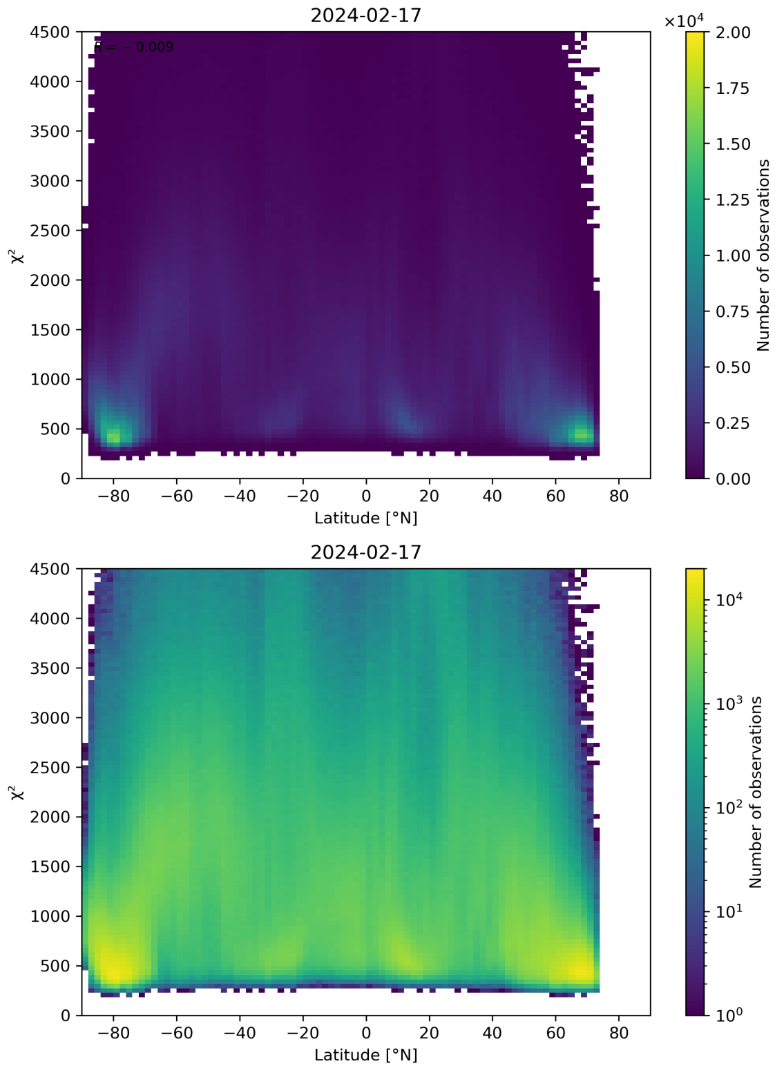
Figure 54: Scatter density plot of “Latitude” against “ \chi^2 ” for 2024-02-17 to 2024-02-18.
