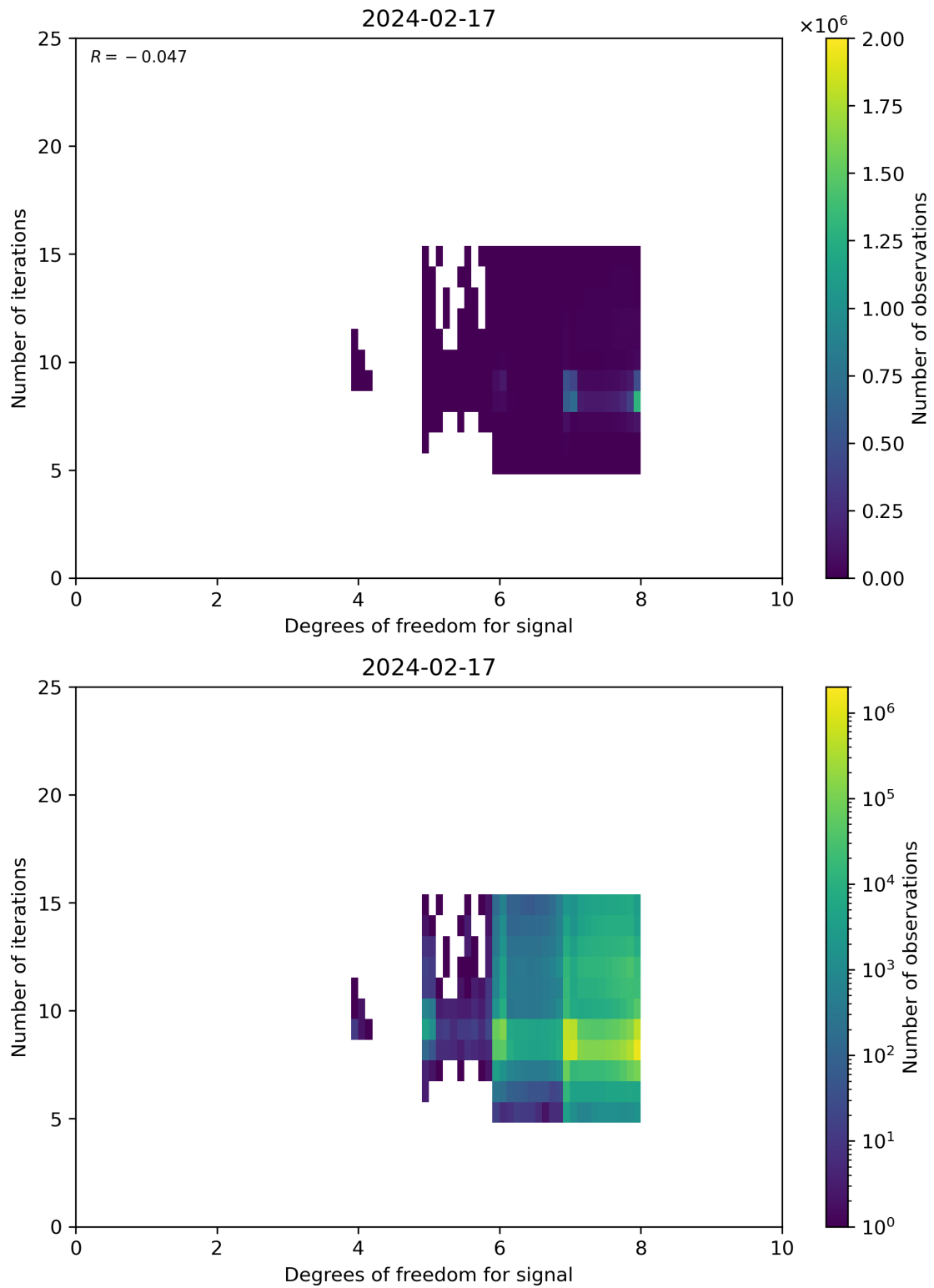
Figure 50: Scatter density plot of “Degrees of freedom for signal” against “Number of iterations” for 2024-02-17 to 2024-02-18.
