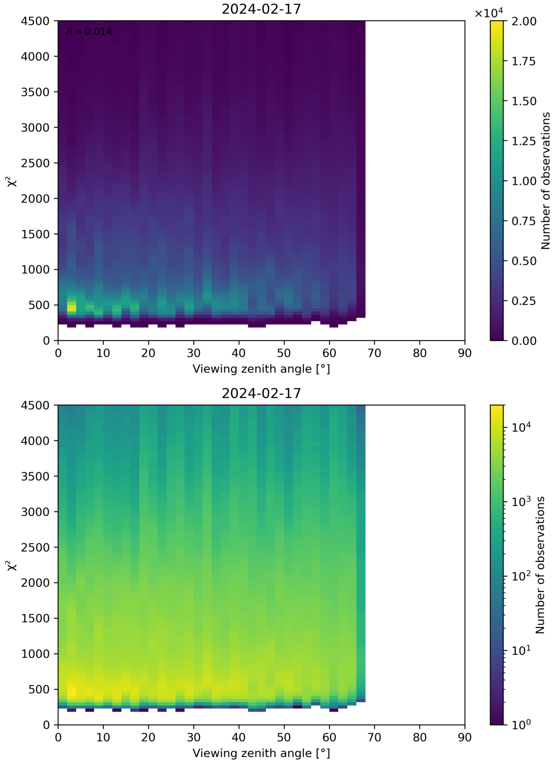
Figure 72: Scatter density plot of “Viewing zenith angle” against “ \chi^2 ” for 2024-02-17 to 2024-02-18.
