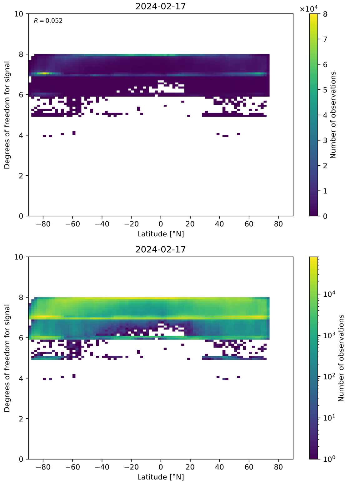
Figure 55: Scatter density plot of “Latitude” against “Degrees of freedom for signal” for 2024-02-17 to 2024-02-18.
