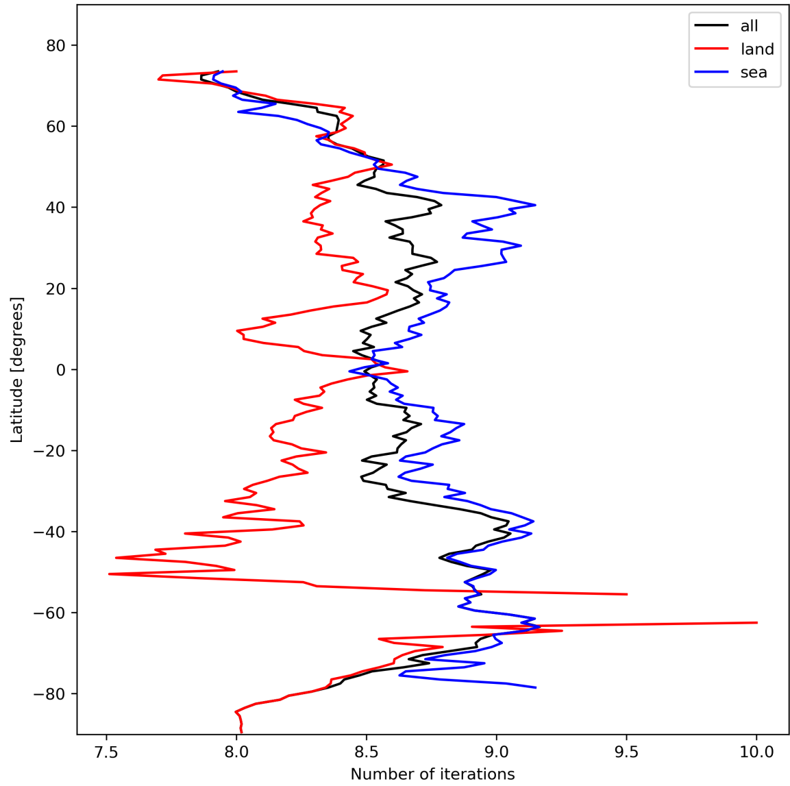
Figure 16: Zonal average of “Number of iterations” for 2024-02-17 to 2024-02-18.
