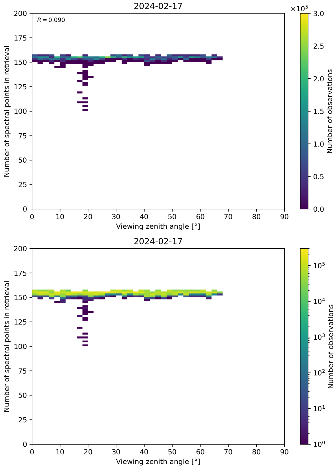
Figure 76: Scatter density plot of “Viewing zenith angle” against “Number of spectral points in retrieval” for 2024-02-17 to 2024-02-18.
