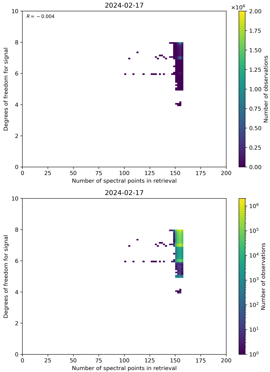
Figure 59: Scatter density plot of “Number of spectral points in retrieval” against “Degrees of freedom for signal” for 2024-02-17 to 2024-02-18.
