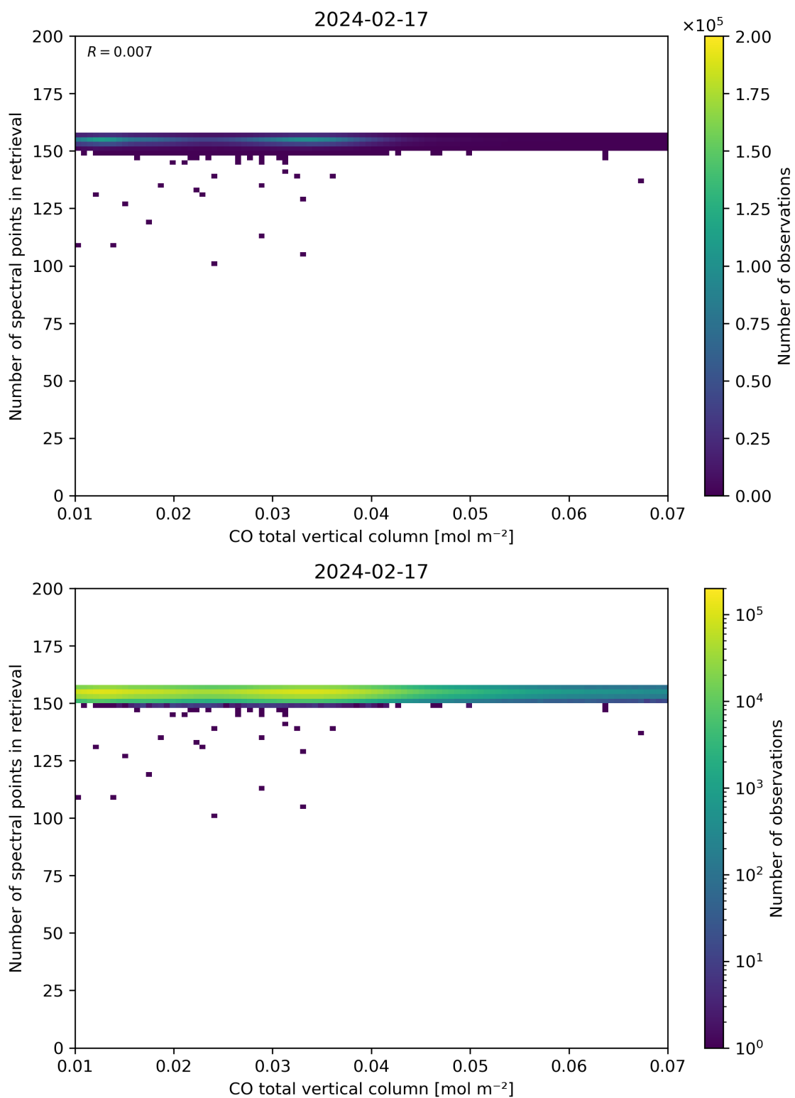
Figure 43: Scatter density plot of “CO total vertical column” against “Number of spectral points in retrieval” for 2024-02-17 to 2024-02-18.
