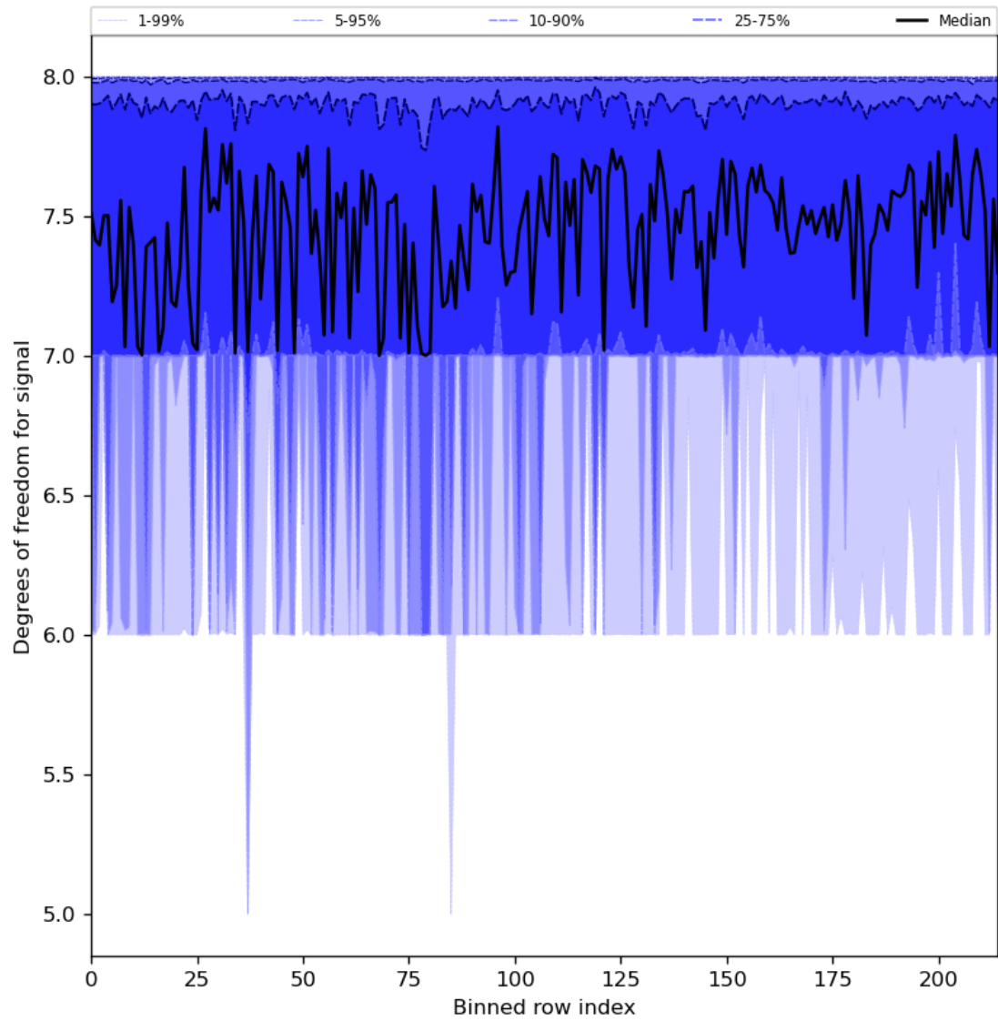
Figure 31: Along track statistics of “Degrees of freedom for signal” for 2024-02-17 to 2024-02-18
