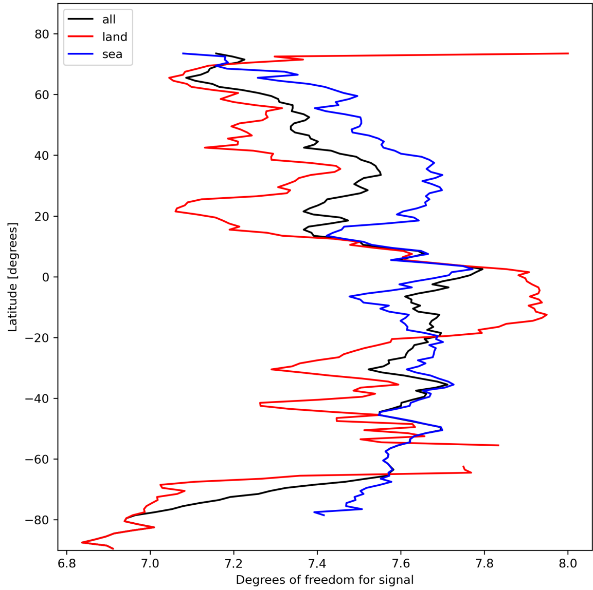
Figure 15: Zonal average of “Degrees of freedom for signal” for 2024-02-17 to 2024-02-18.
