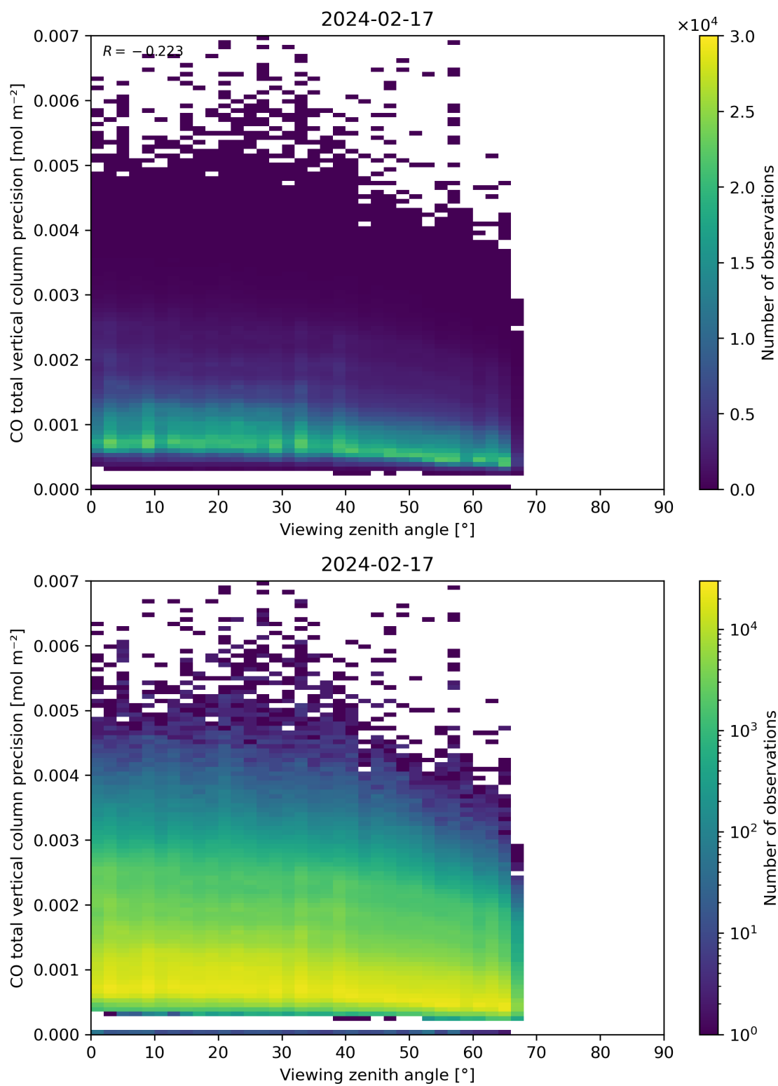
Figure 71: Scatter density plot of “Viewing zenith angle” against “CO total vertical column precision” for 2024-02-17 to 2024-02-18.
