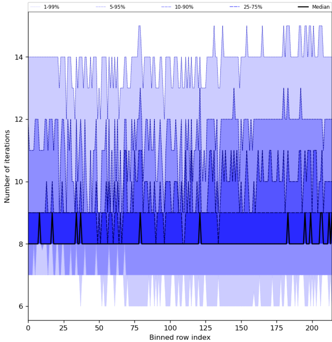
Figure 32: Along track statistics of “Number of iterations” for 2024-02-17 to 2024-02-18
