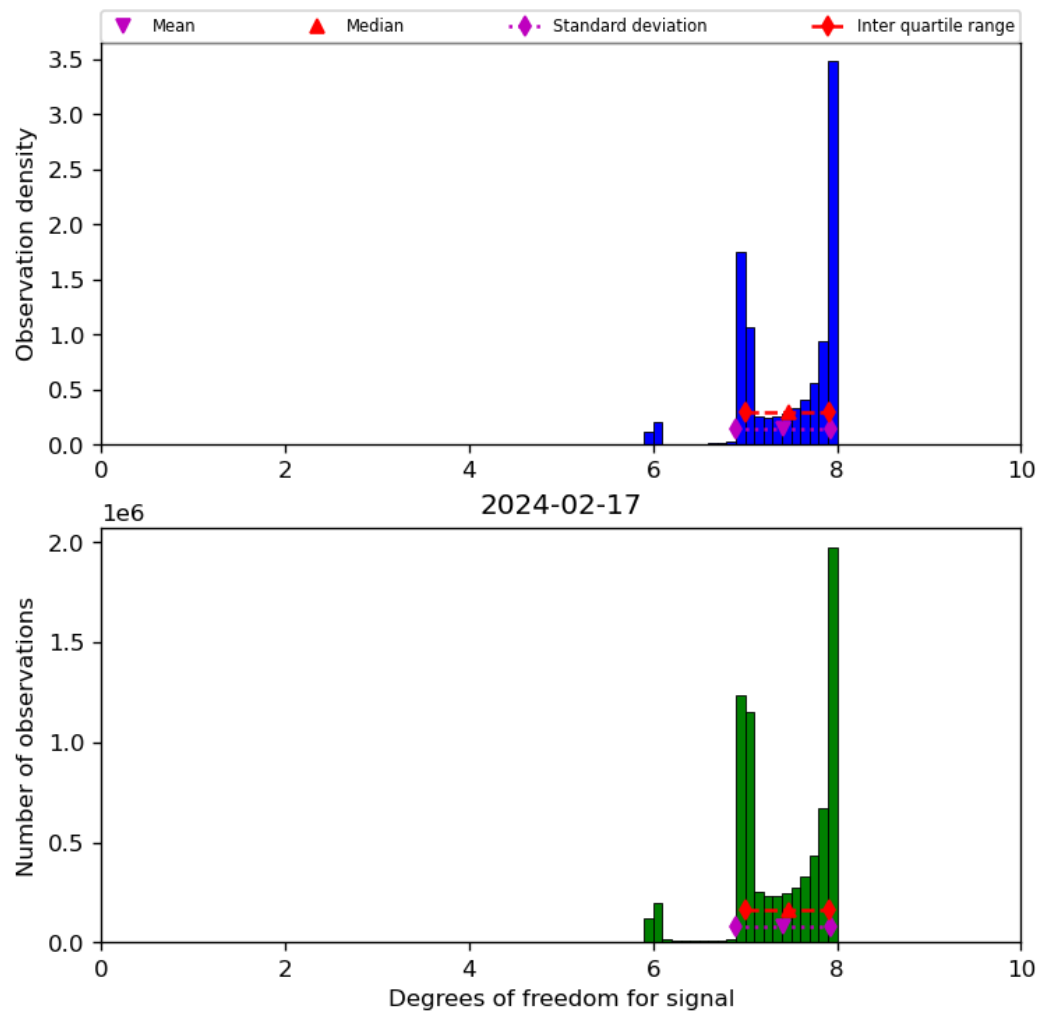
Figure 23: Histogram of “Degrees of freedom for signal” for 2024-02-17 to 2024-02-18
