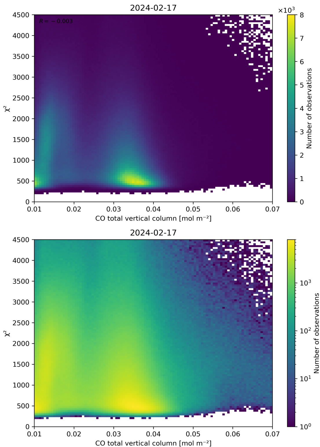
Figure 35: Scatter density plot of “CO total vertical column” against “ \chi^2 ” for 2024-02-17 to 2024-02-18.
