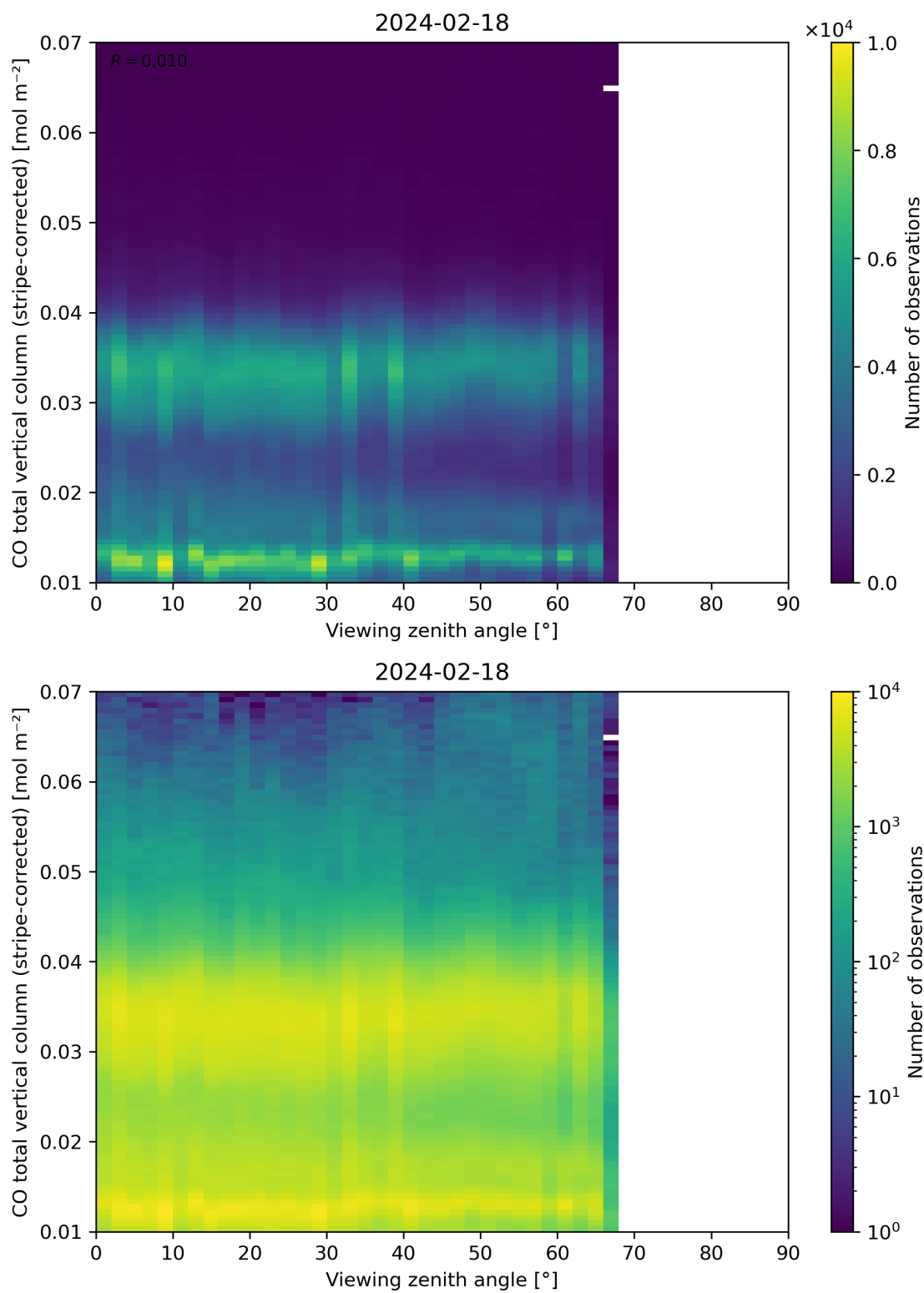
Figure 70: Scatter density plot of “Viewing zenith angle” against “CO total vertical column (stripe-corrected)” for 2024-02-17 to 2024-02-19.
