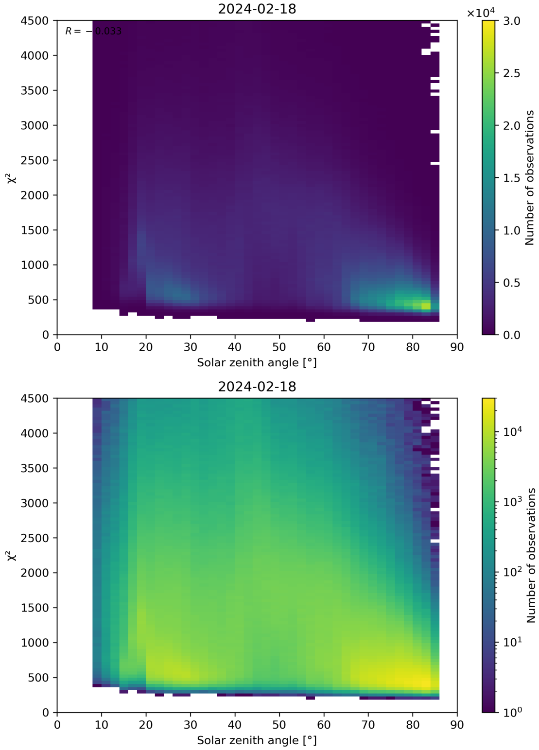
Figure 64: Scatter density plot of “Solar zenith angle” against “ \chi^2 ” for 2024-02-17 to 2024-02-19.
