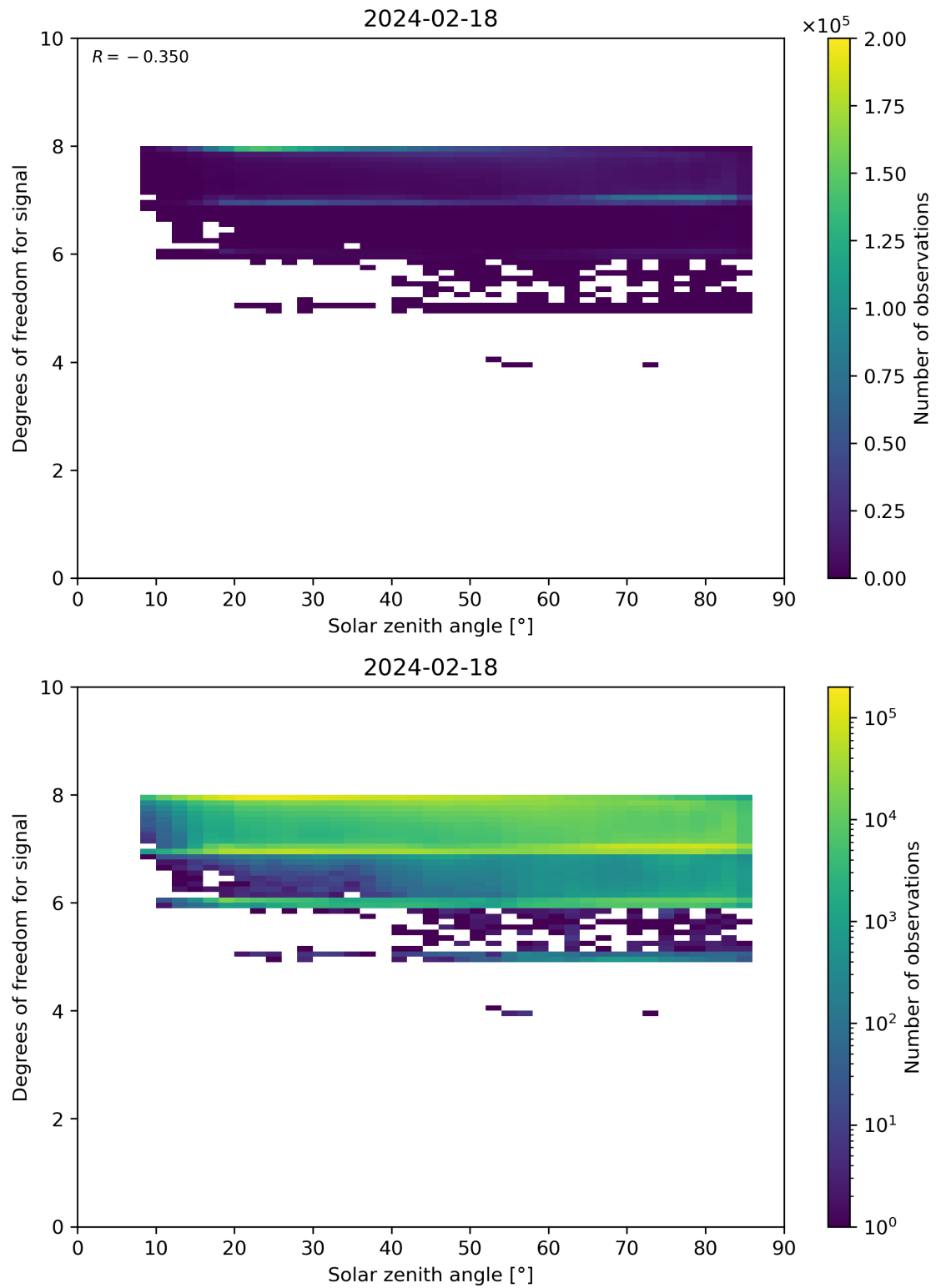
Figure 65: Scatter density plot of “Solar zenith angle” against “Degrees of freedom for signal” for 2024-02-17 to 2024-02-19.
