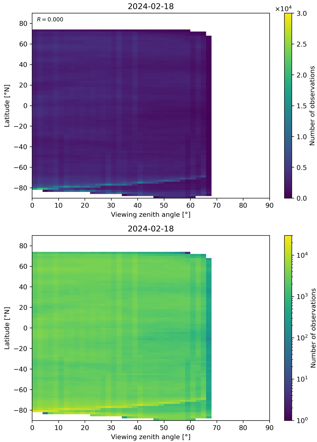
Figure 74: Scatter density plot of “Viewing zenith angle” against “Latitude” for 2024-02-17 to 2024-02-19.
