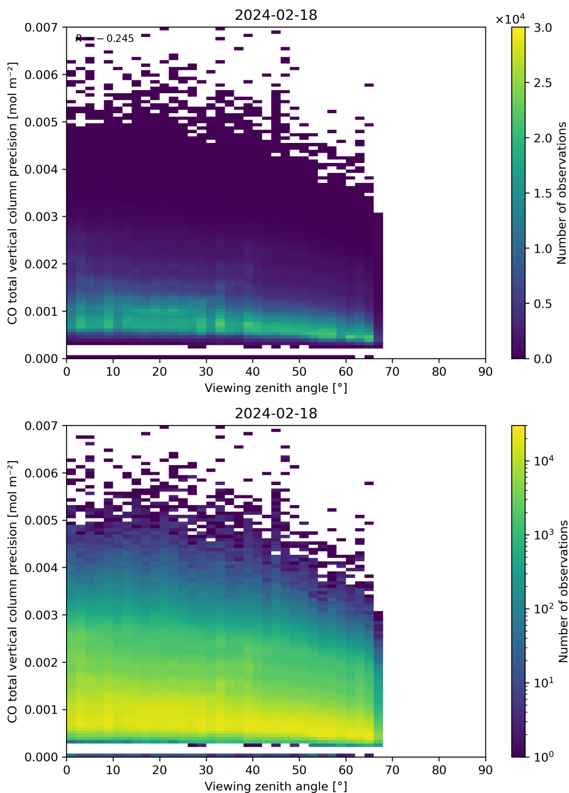
Figure 71: Scatter density plot of “Viewing zenith angle” against “CO total vertical column precision” for 2024-02-17 to 2024-02-19.
