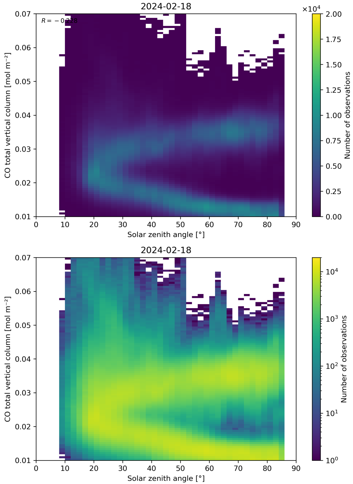
Figure 61: Scatter density plot of “Solar zenith angle” against “CO total vertical column” for 2024-02-17 to 2024-02-19.
