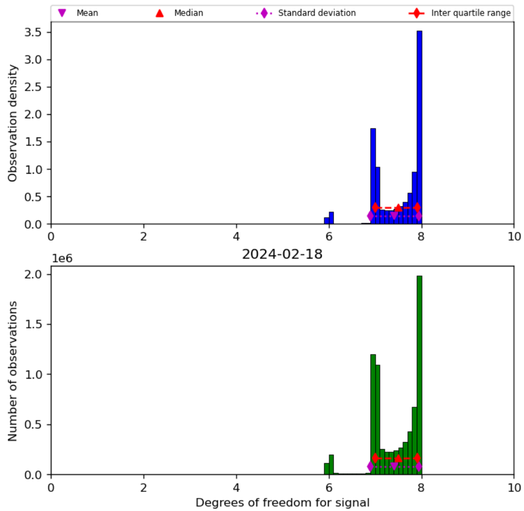
Figure 23: Histogram of “Degrees of freedom for signal” for 2024-02-17 to 2024-02-19
