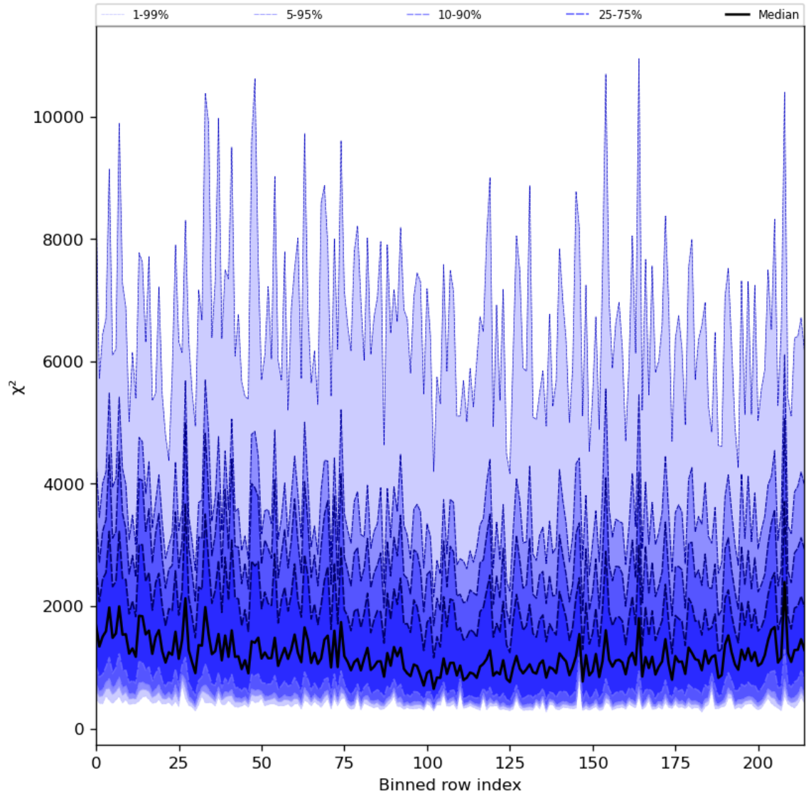
Figure 30: Along track statistics of “ \chi^2 ” for 2024-02-17 to 2024-02-19
