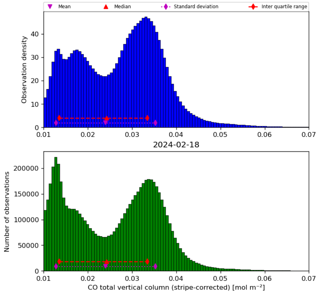
Figure 19: Histogram of “CO total vertical column (stripe-corrected)” for 2024-02-17 to 2024-02-19
