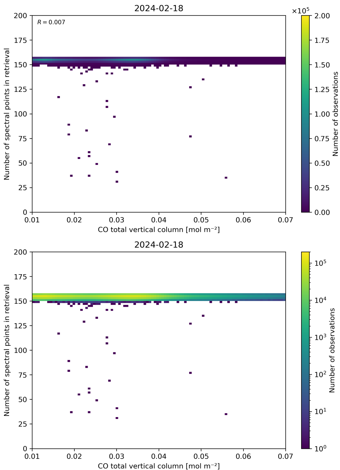
Figure 43: Scatter density plot of “CO total vertical column” against “Number of spectral points in retrieval” for 2024-02-17 to 2024-02-19.
