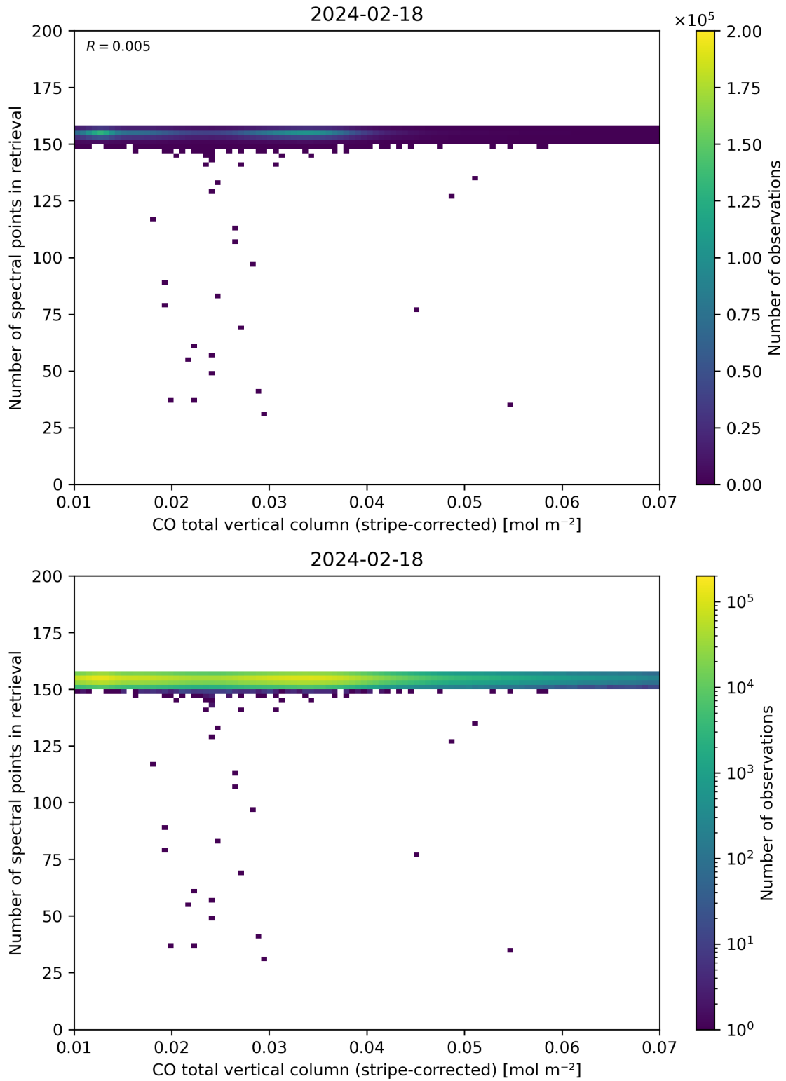
Figure 40: Scatter density plot of “CO total vertical column (stripe-corrected)” against “Number of spectral points in retrieval” for 2024-02-17 to 2024-02-19.
