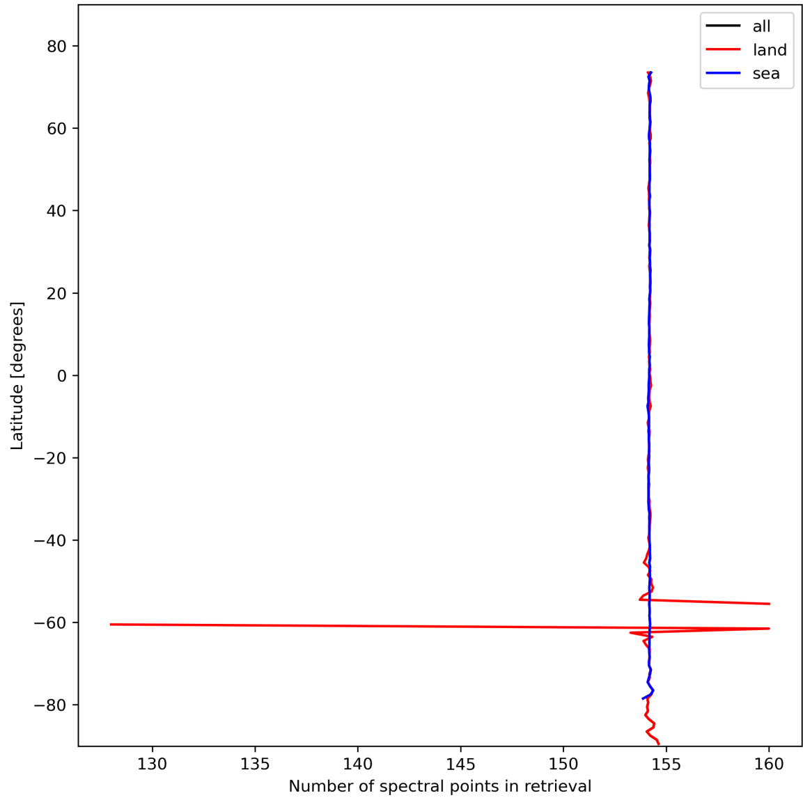
Figure 13: Zonal average of “Number of spectral points in retrieval” for 2024-02-17 to 2024-02-19.
