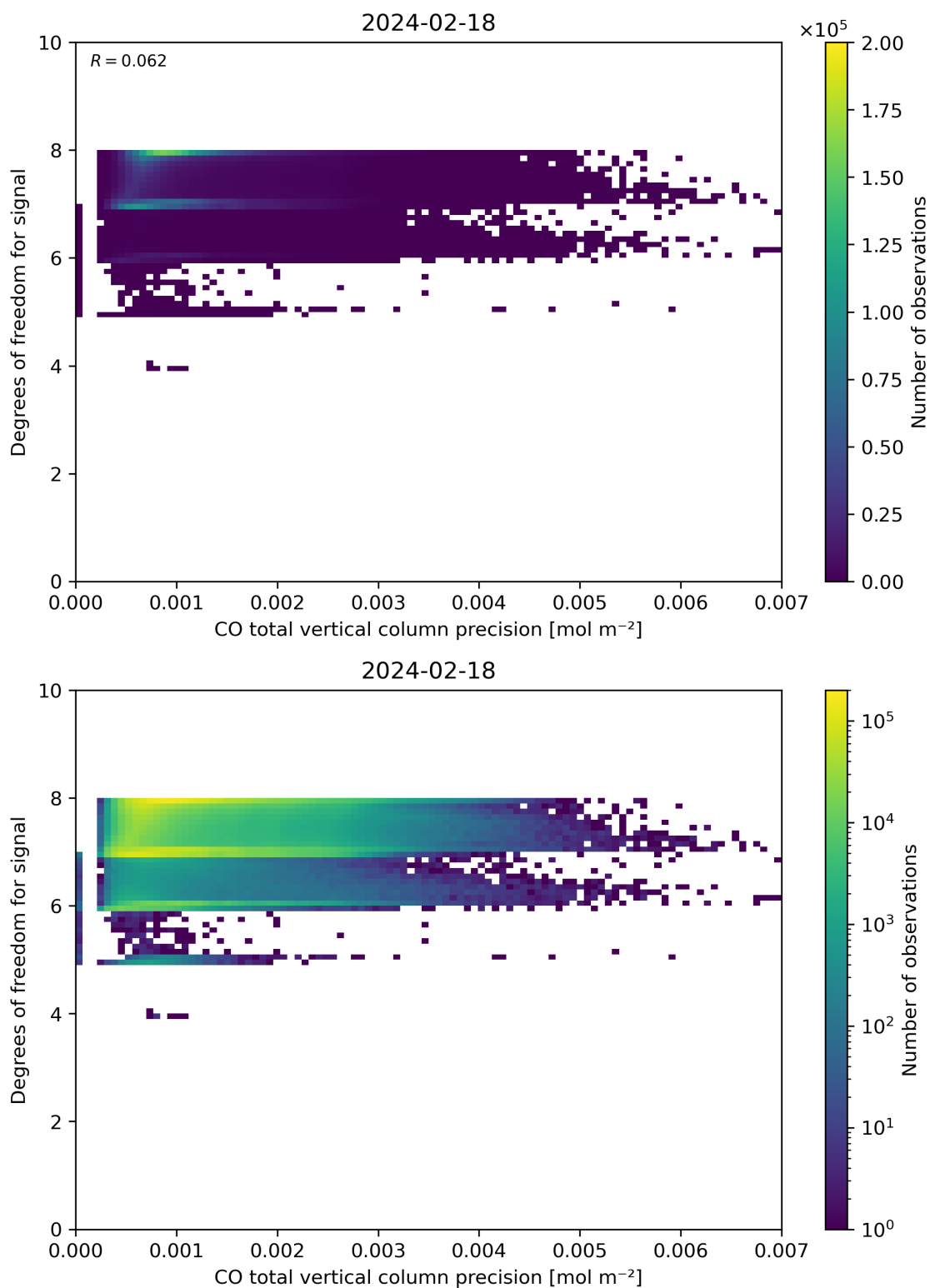
Figure 45: Scatter density plot of “CO total vertical column precision” against “Degrees of freedom for signal” for 2024-02-17 to 2024-02-19.
