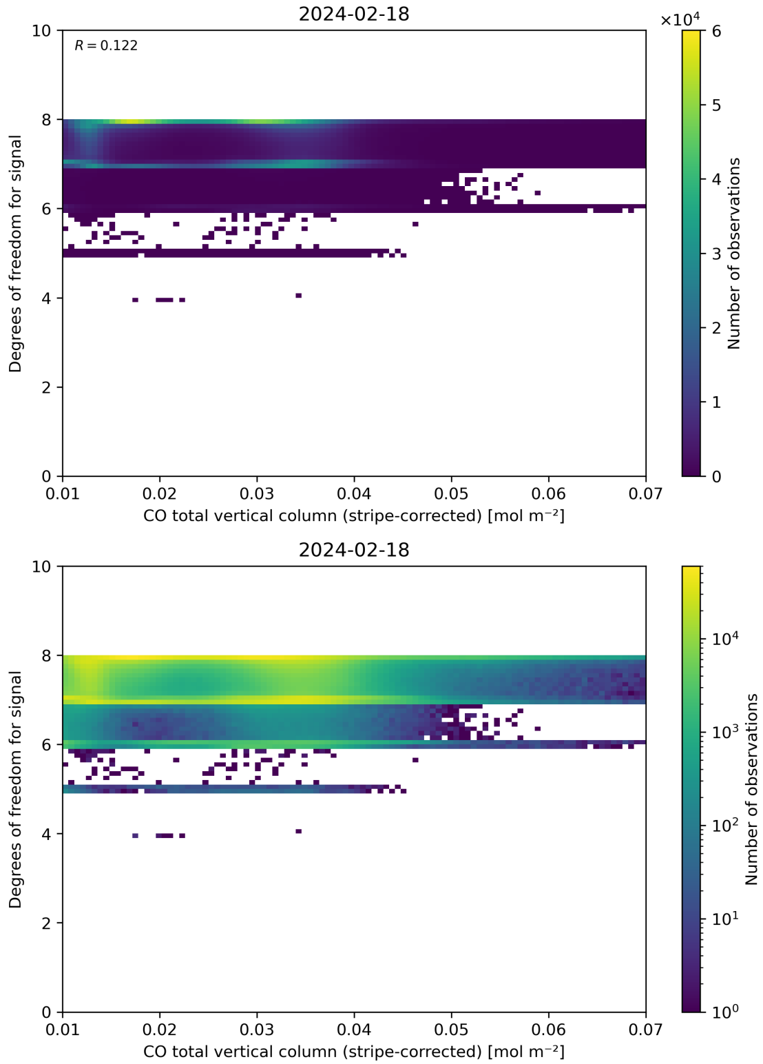
Figure 38: Scatter density plot of “CO total vertical column (stripe-corrected)” against “Degrees of freedom for signal” for 2024-02-17 to 2024-02-19.
