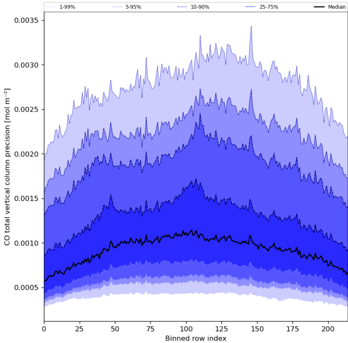
Figure 28: Along track statistics of “CO total vertical column precision” for 2024-02-17 to 2024-02-19
