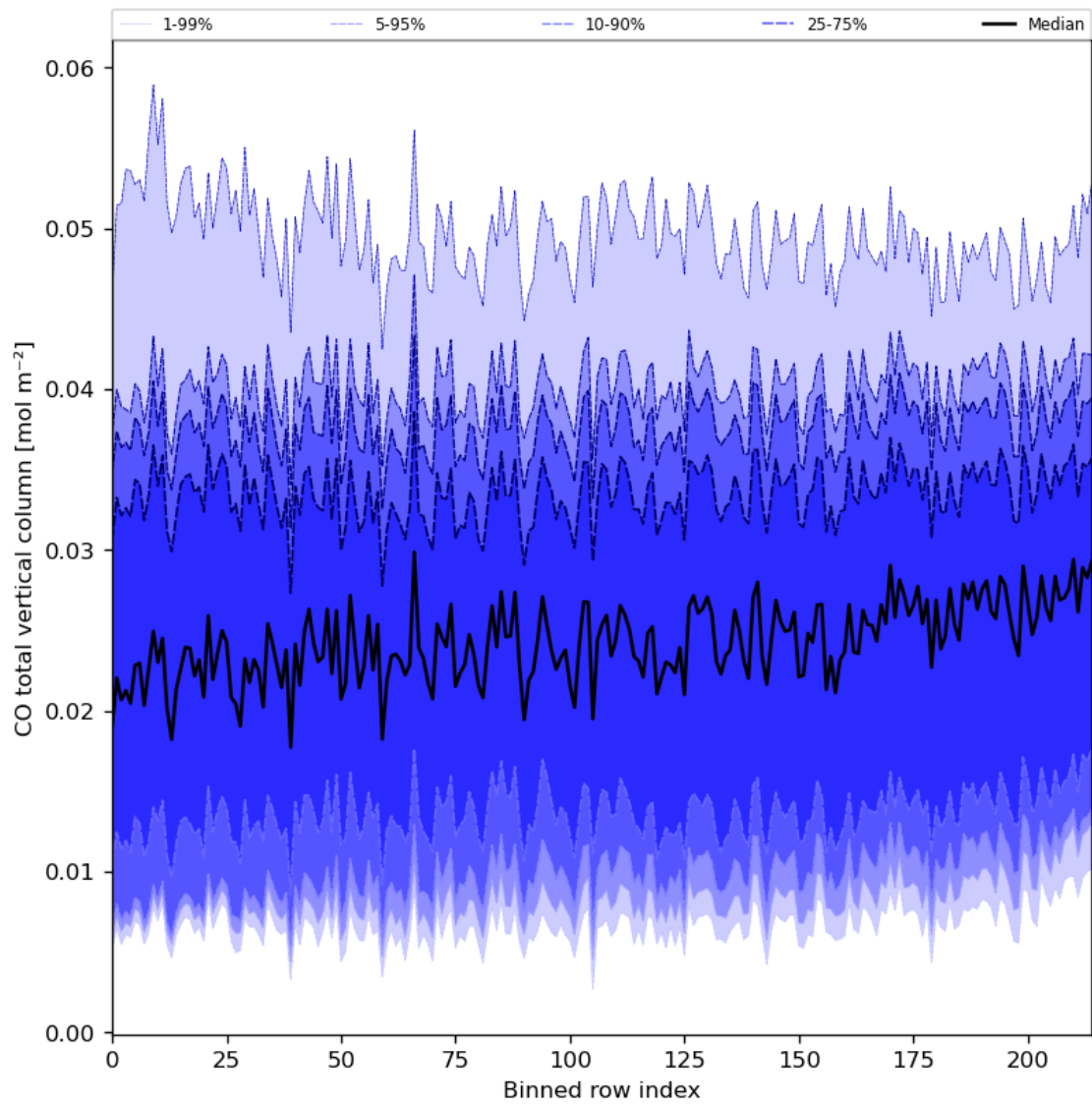
Figure 26: Along track statistics of “CO total vertical column” for 2024-02-17 to 2024-02-19
