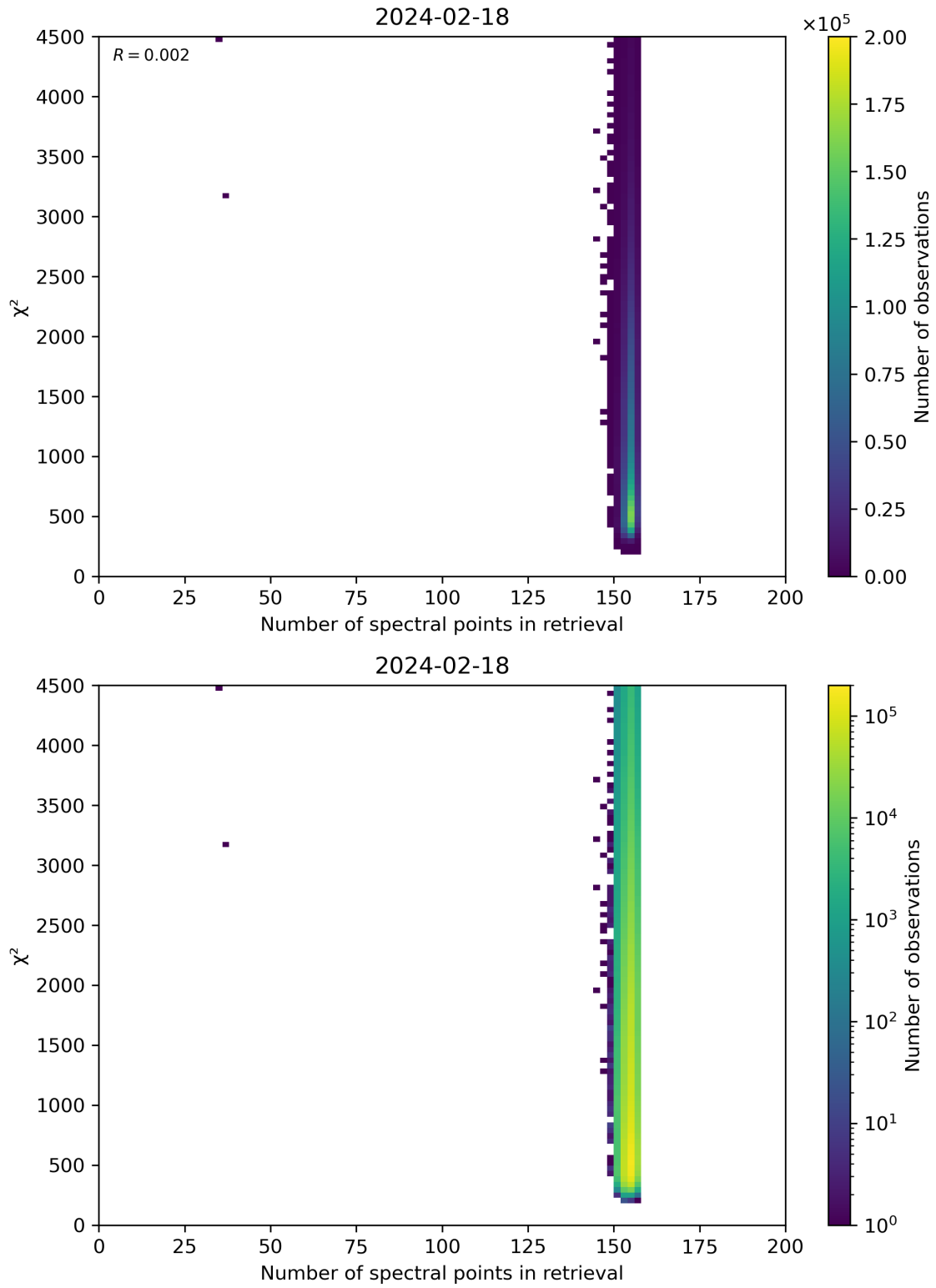
Figure 58: Scatter density plot of “Number of spectral points in retrieval” against “ \chi^2 ” for 2024-02-17 to 2024-02-19.
