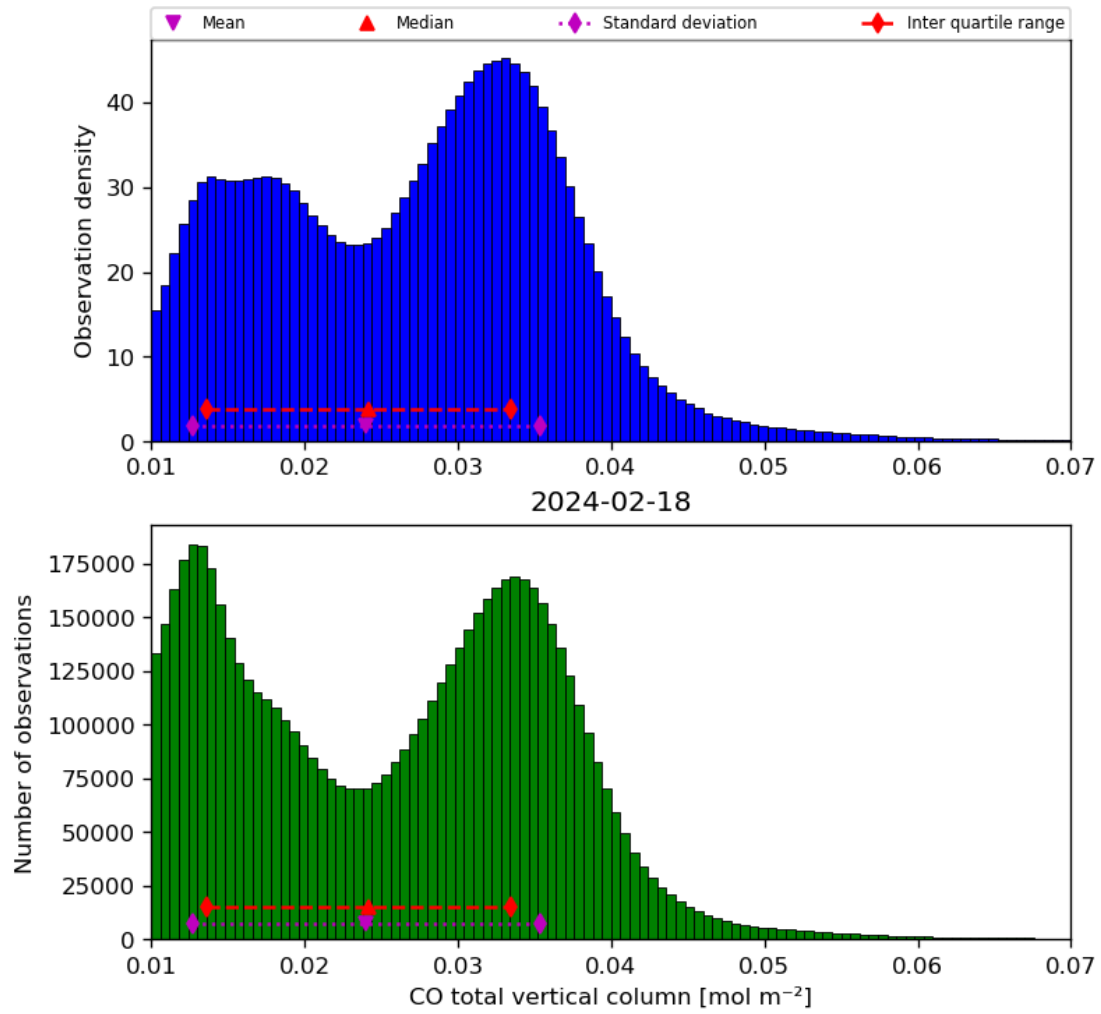
Figure 18: Histogram of “CO total vertical column” for 2024-02-17 to 2024-02-19
