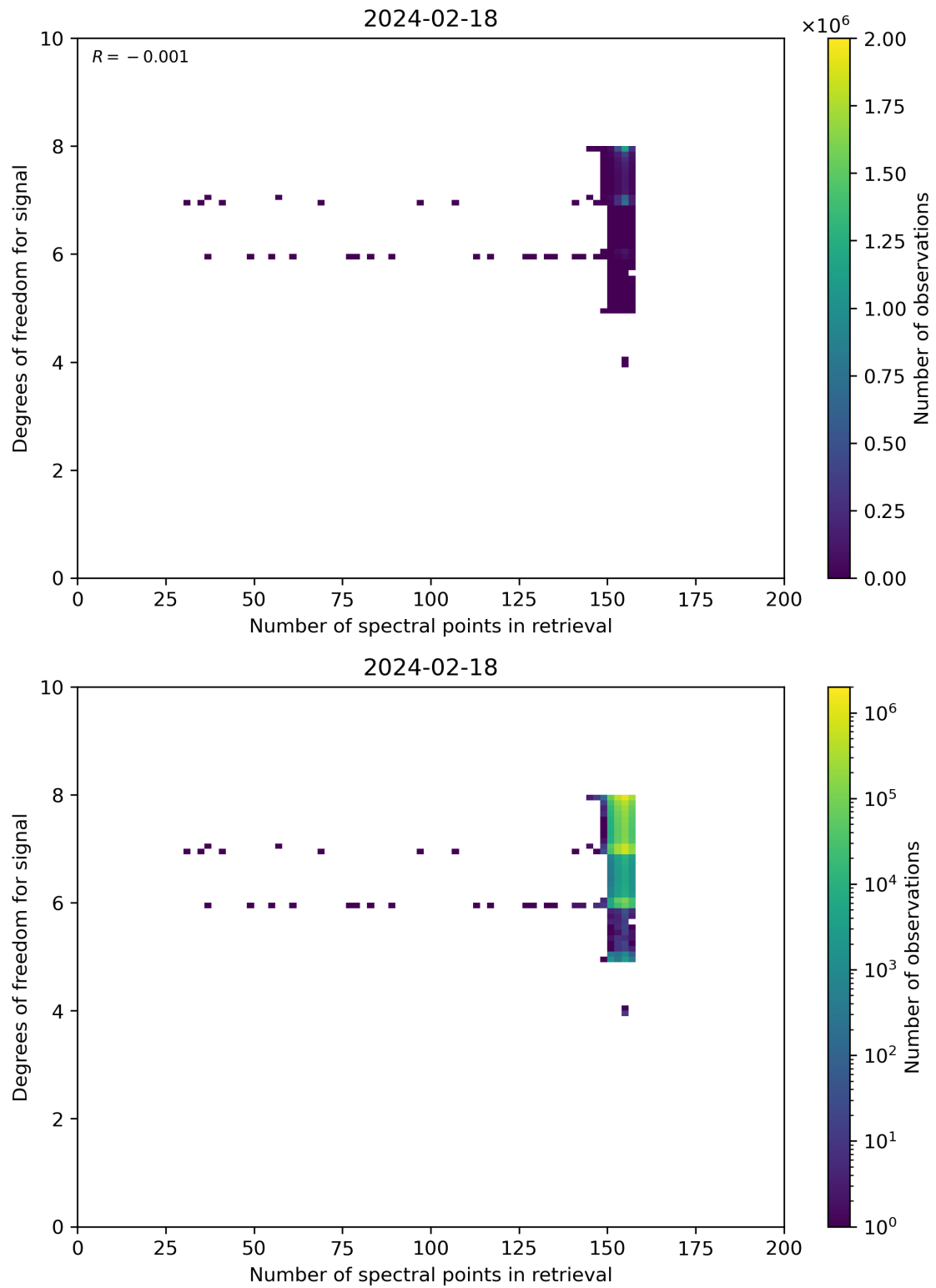
Figure 59: Scatter density plot of “Number of spectral points in retrieval” against “Degrees of freedom for signal” for 2024-02-17 to 2024-02-19.
