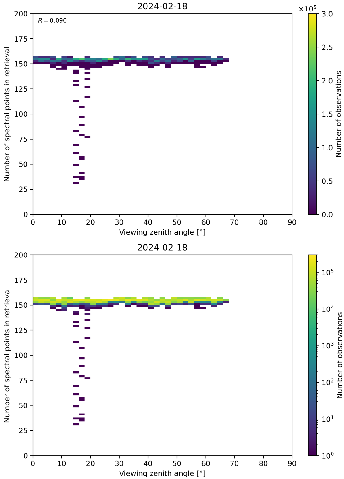
Figure 76: Scatter density plot of “Viewing zenith angle” against “Number of spectral points in retrieval” for 2024-02-17 to 2024-02-19.
