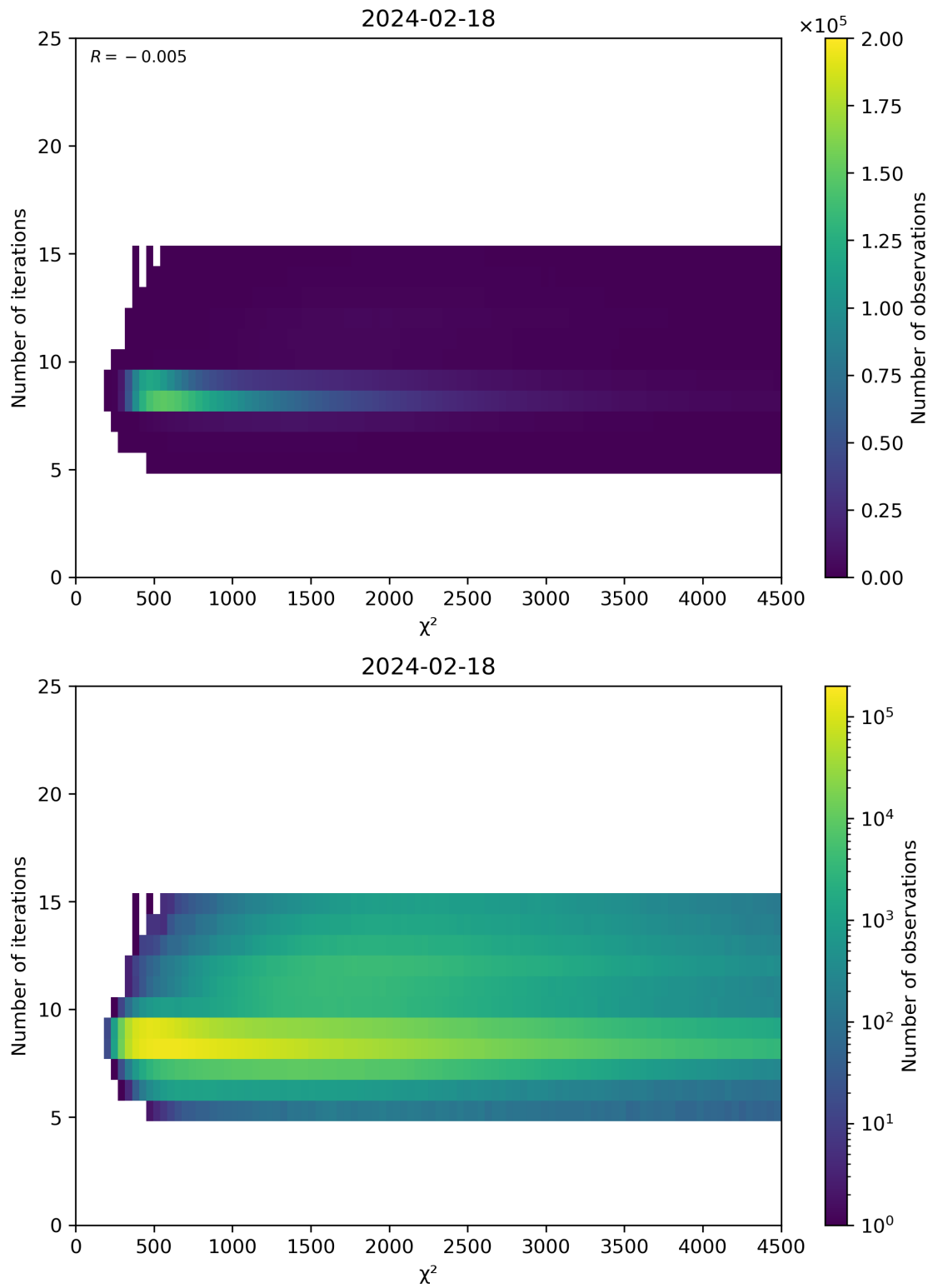
Figure 49: Scatter density plot of “ \chi^2 ” against “Number of iterations” for 2024-02-17 to 2024-02-19.
