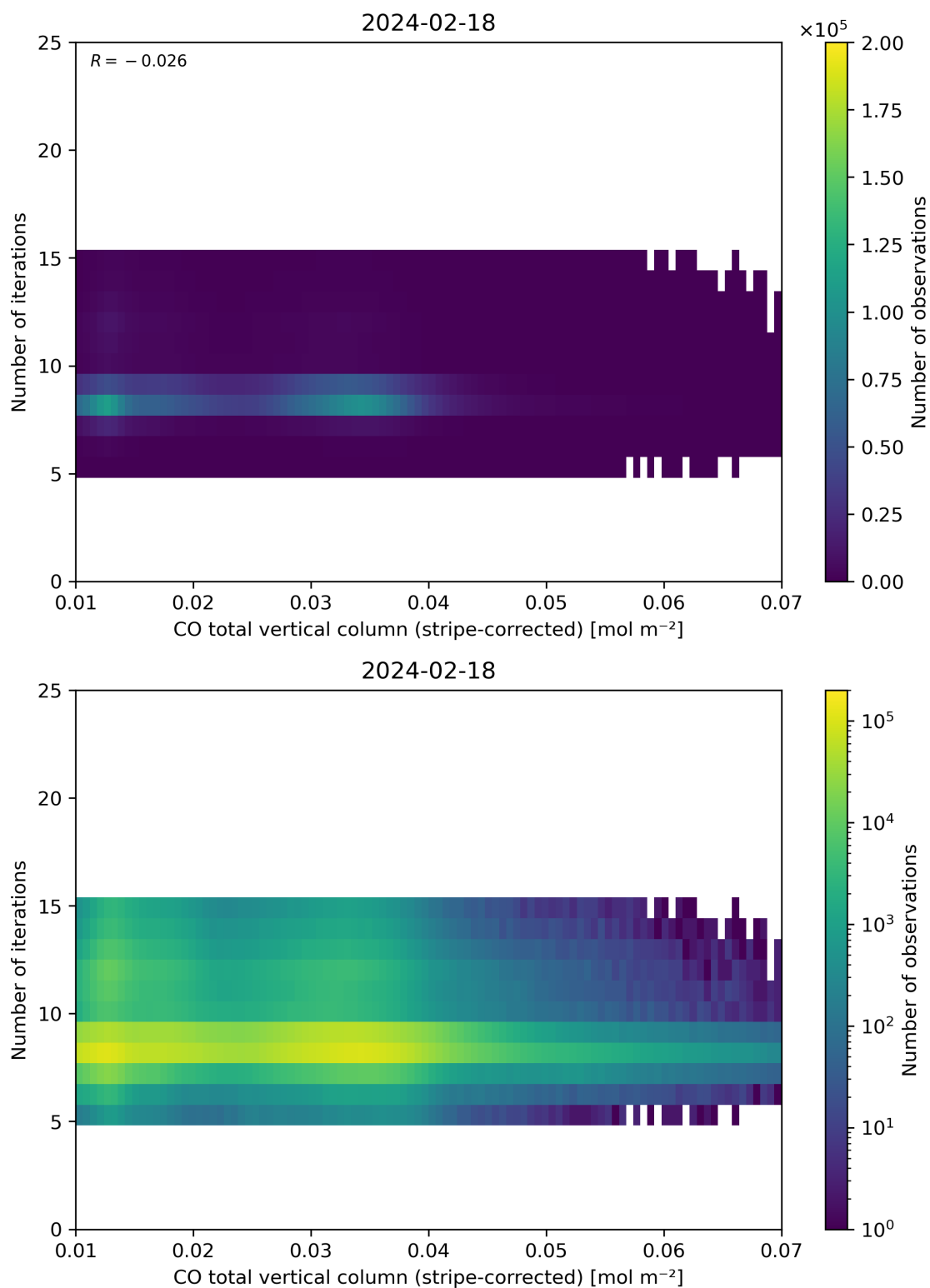
Figure 39: Scatter density plot of “CO total vertical column (stripe-corrected)” against “Number of iterations” for 2024-02-17 to 2024-02-19.
