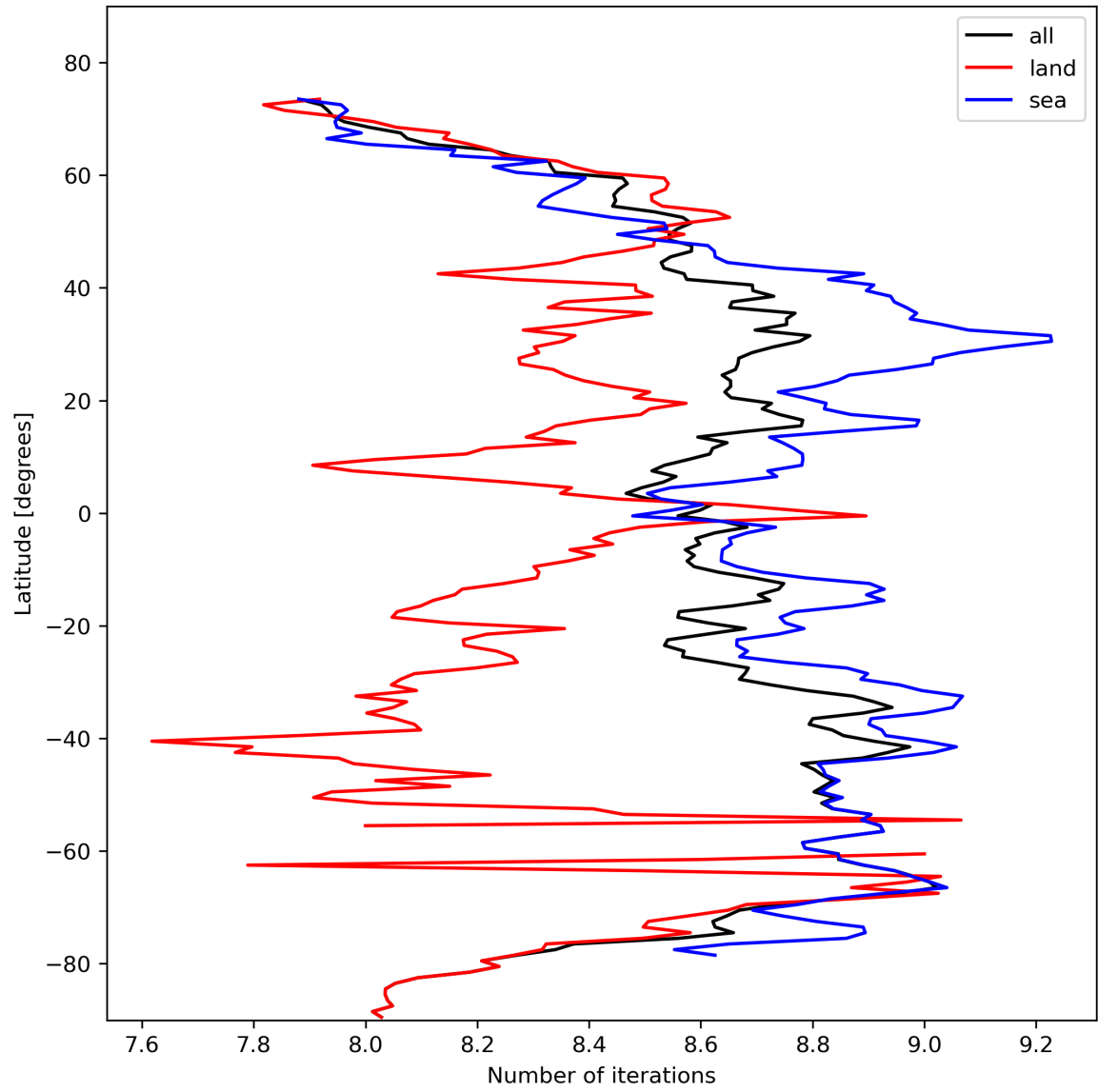
Figure 16: Zonal average of “Number of iterations” for 2024-02-17 to 2024-02-19.
