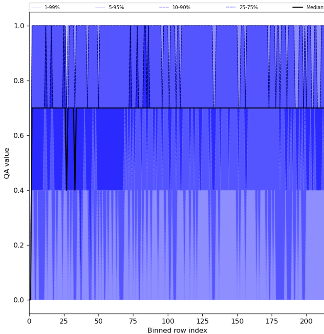
Figure 25: Along track statistics of “QA value” for 2024-02-17 to 2024-02-19
