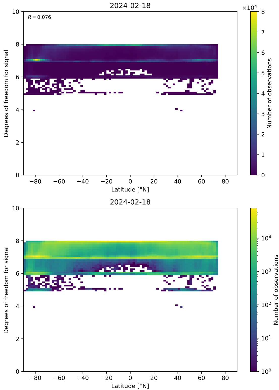
Figure 55: Scatter density plot of “Latitude” against “Degrees of freedom for signal” for 2024-02-17 to 2024-02-19.
