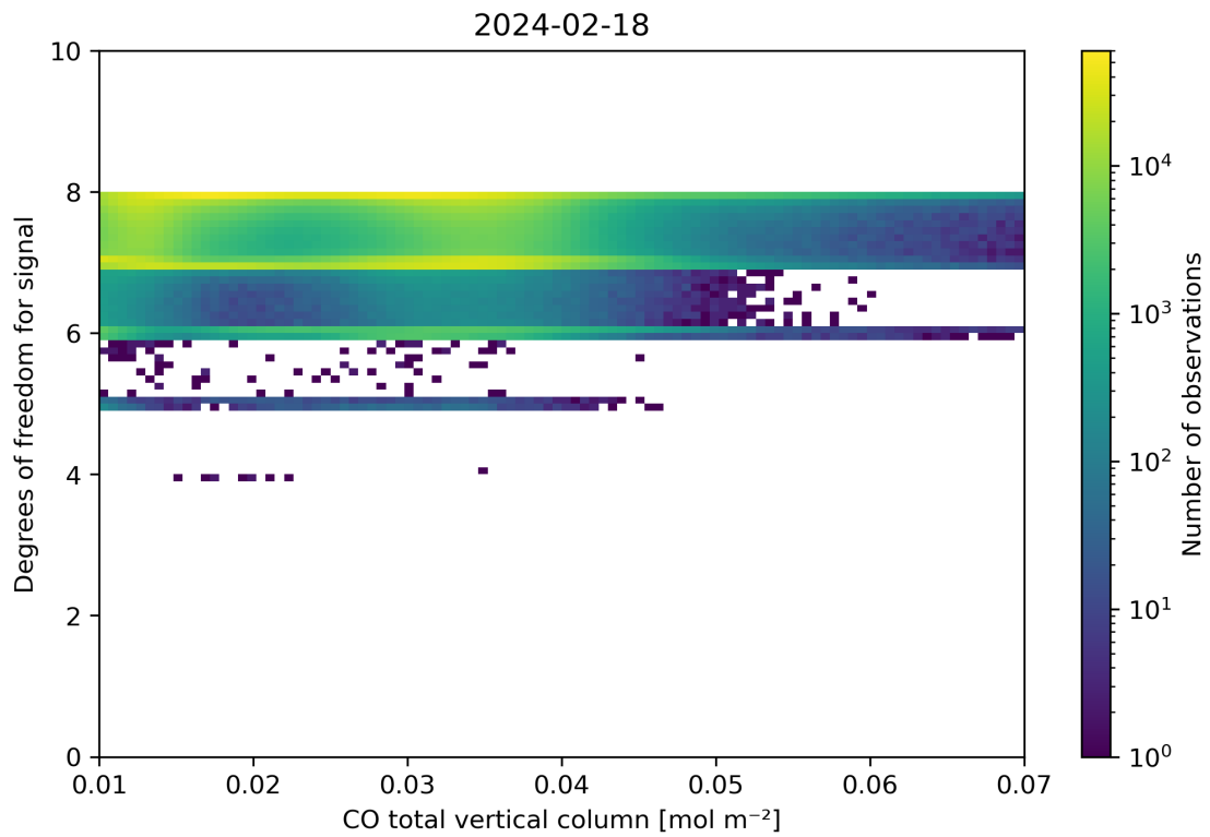
Figure 41: Scatter density plot of “CO total vertical column” against “Degrees of freedom for signal” for 2024-02-17 to 2024-02-19.
