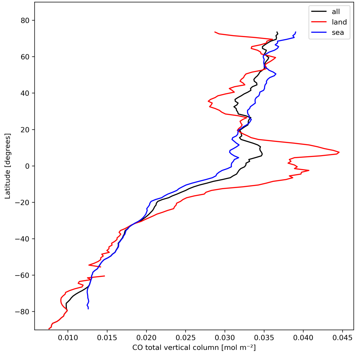
Figure 10: Zonal average of “CO total vertical column” for 2024-02-17 to 2024-02-19.
