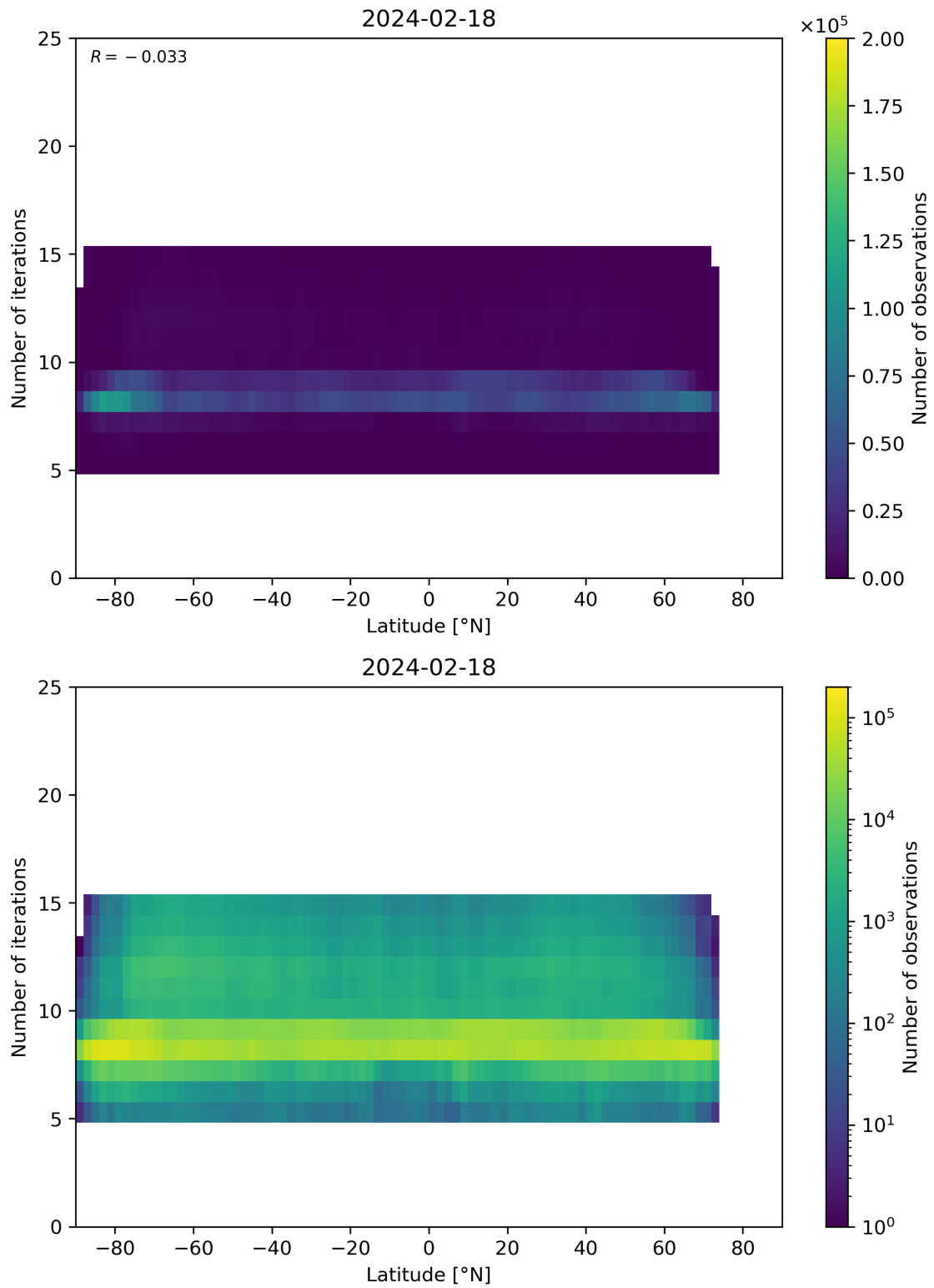
Figure 56: Scatter density plot of “Latitude” against “Number of iterations” for 2024-02-17 to 2024-02-19.
