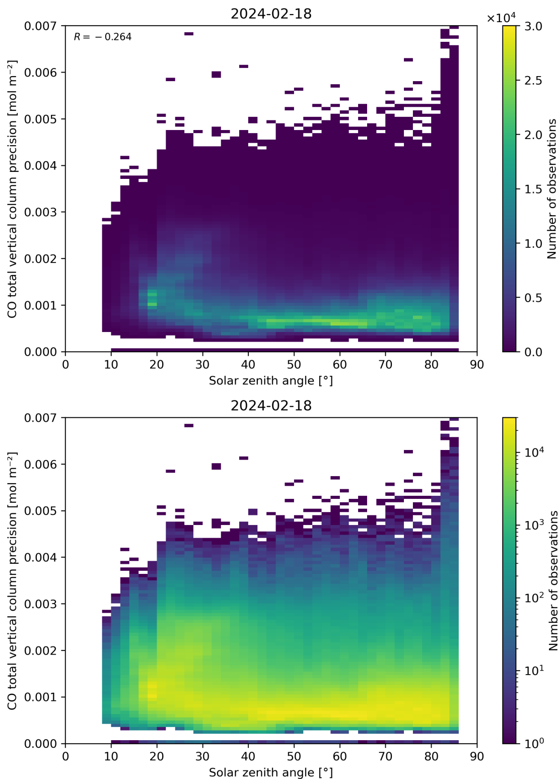
Figure 63: Scatter density plot of “Solar zenith angle” against “CO total vertical column precision” for 2024-02-17 to 2024-02-19.
