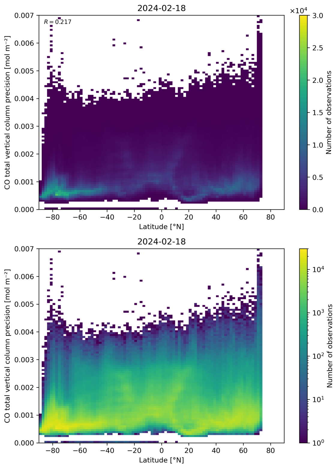
Figure 53: Scatter density plot of “Latitude” against “CO total vertical column precision” for 2024-02-17 to 2024-02-19.
