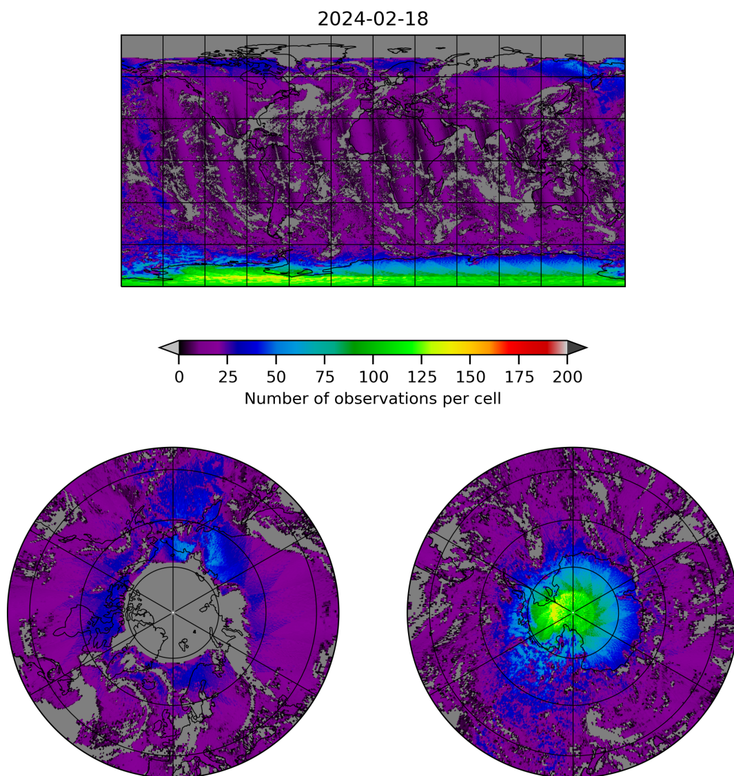
Figure 8: Map of the number of observations for 2024-02-17 to 2024-02-19
