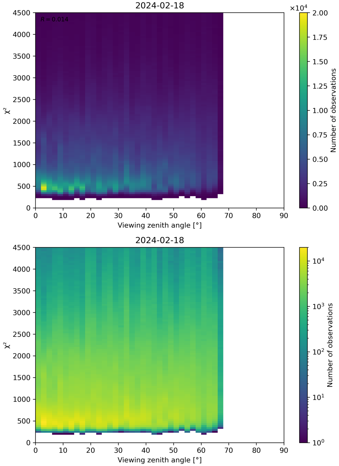
Figure 72: Scatter density plot of “Viewing zenith angle” against “ \chi^2 ” for 2024-02-17 to 2024-02-19.
