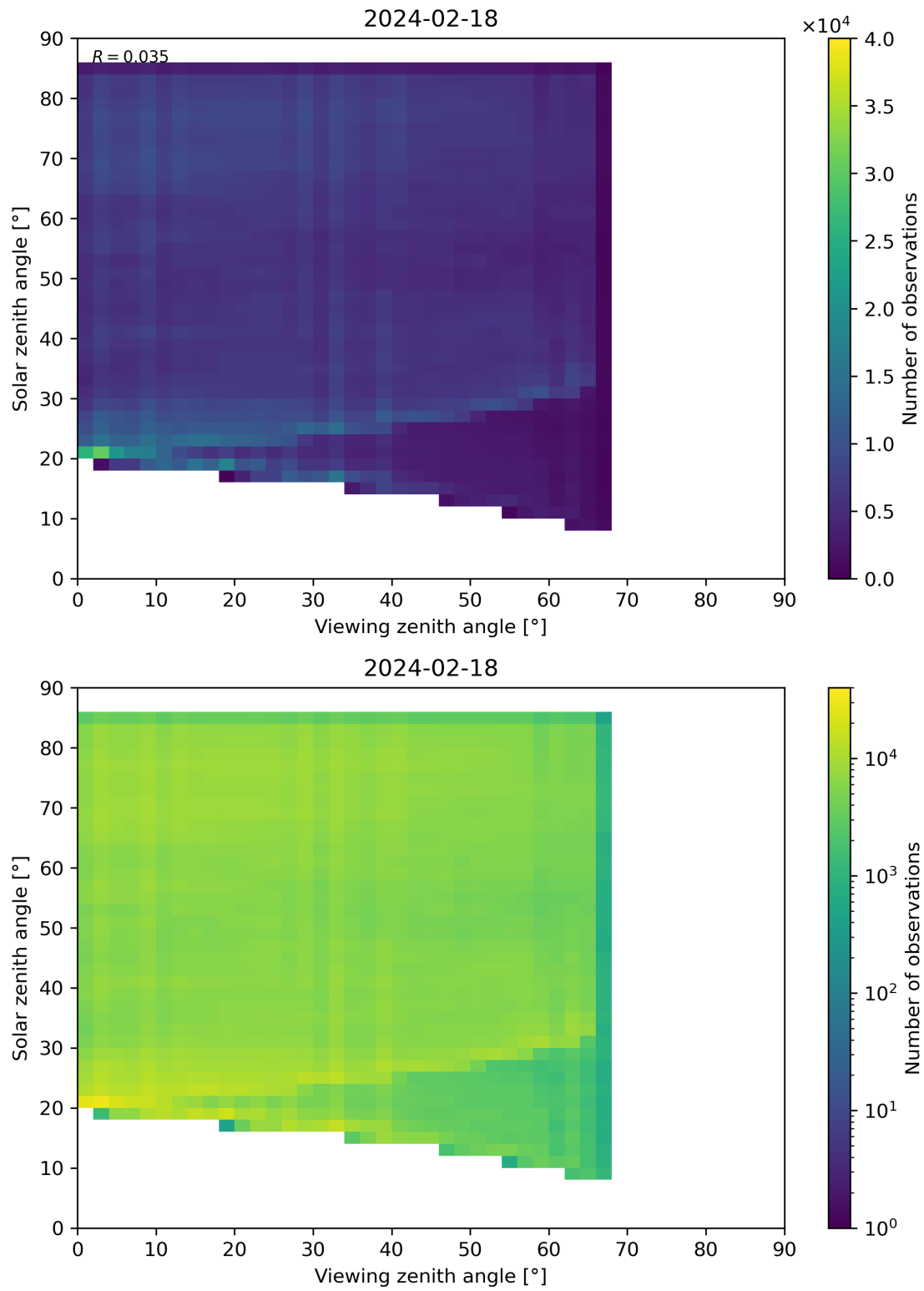
Figure 77: Scatter density plot of “Viewing zenith angle” against “Solar zenith angle” for 2024-02-17 to 2024-02-19.
