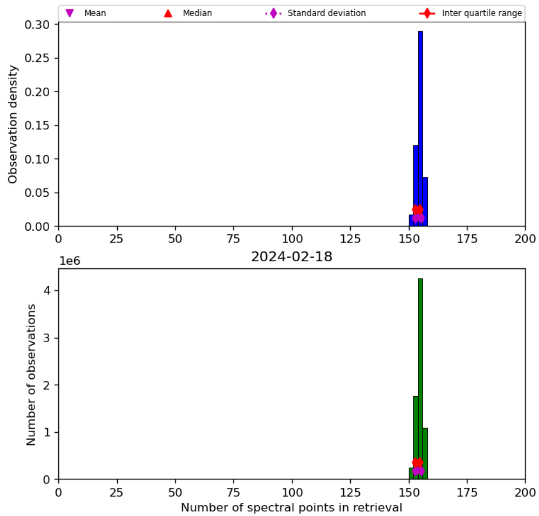
Figure 21: Histogram of “Number of spectral points in retrieval” for 2024-02-17 to 2024-02-19
