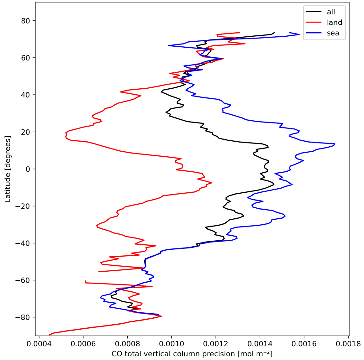
Figure 12: Zonal average of “CO total vertical column precision” for 2024-02-17 to 2024-02-19.
