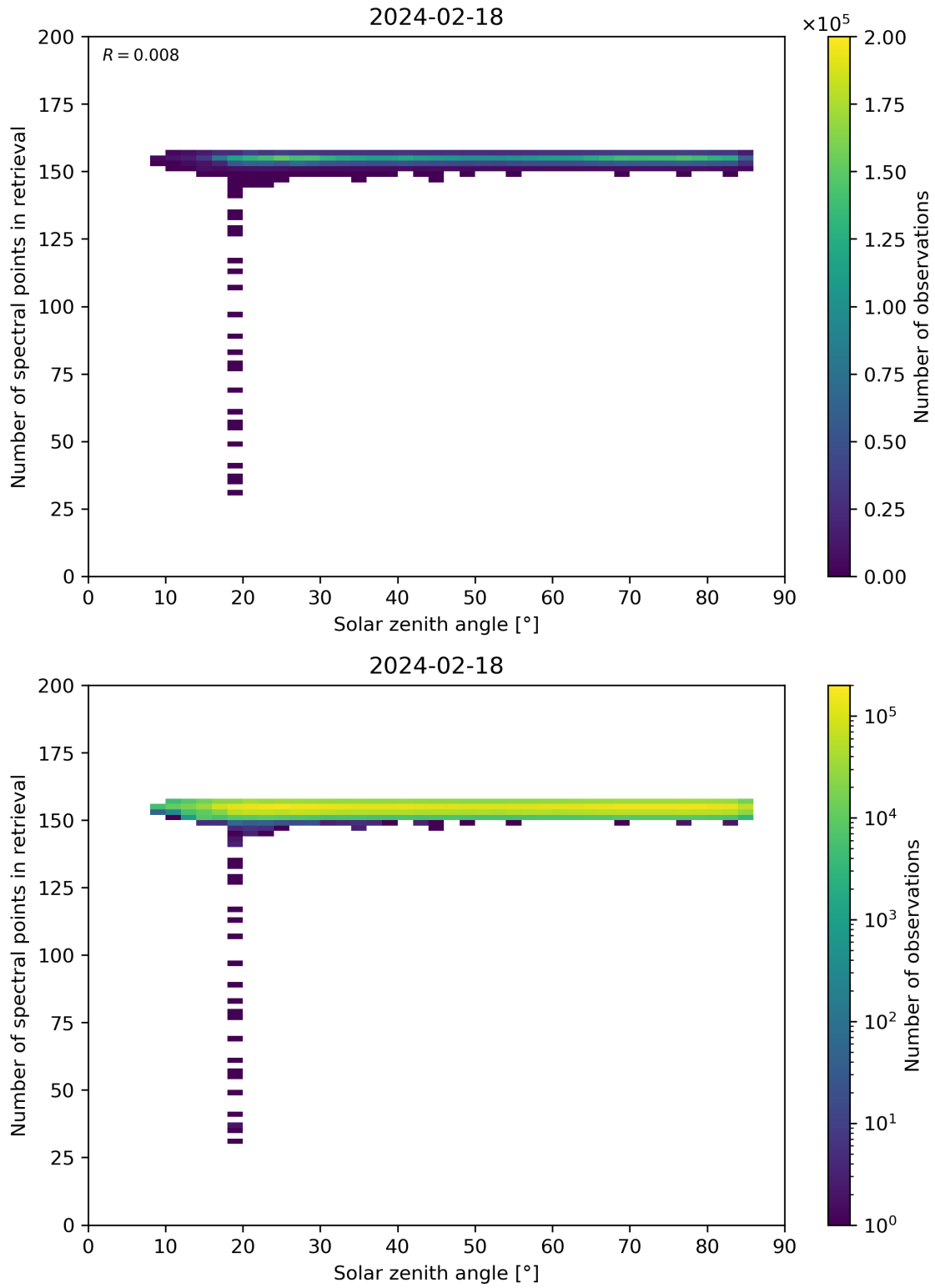
Figure 68: Scatter density plot of “Solar zenith angle” against “Number of spectral points in retrieval” for 2024-02-17 to 2024-02-19.
