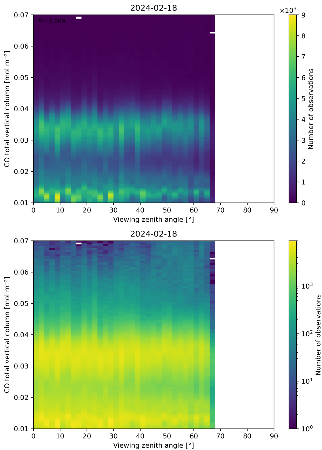
Figure 69: Scatter density plot of “Viewing zenith angle” against “CO total vertical column” for 2024-02-17 to 2024-02-19.
