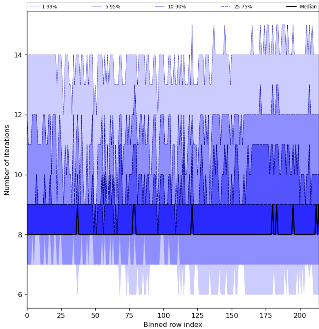
Figure 32: Along track statistics of “Number of iterations” for 2024-02-17 to 2024-02-19
