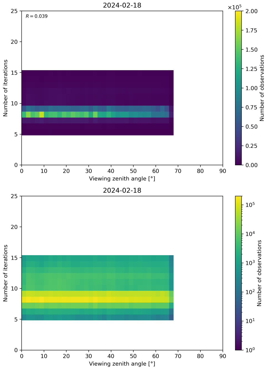
Figure 75: Scatter density plot of “Viewing zenith angle” against “Number of iterations” for 2024-02-17 to 2024-02-19.
