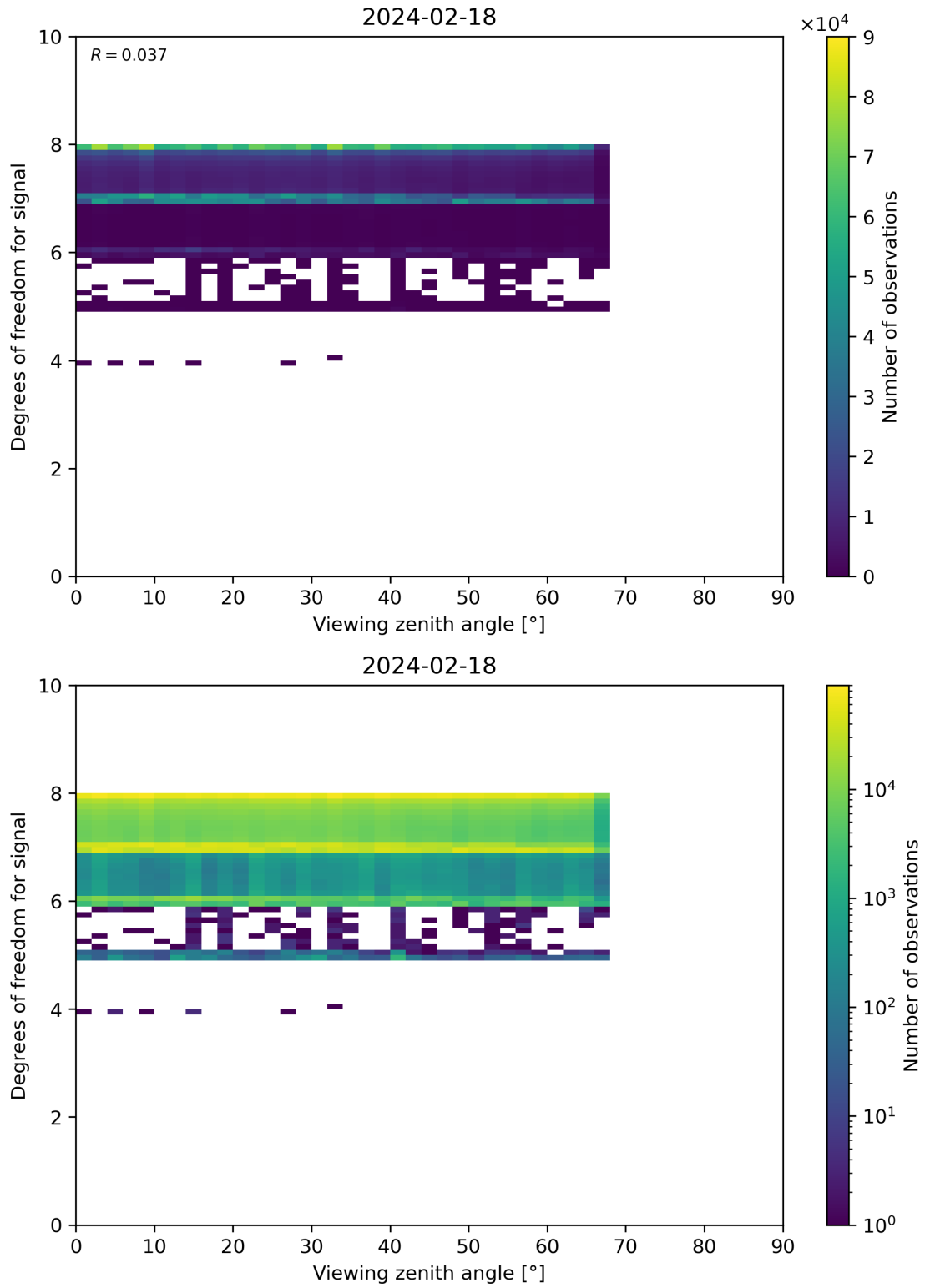
Figure 73: Scatter density plot of “Viewing zenith angle” against “Degrees of freedom for signal” for 2024-02-17 to 2024-02-19.
