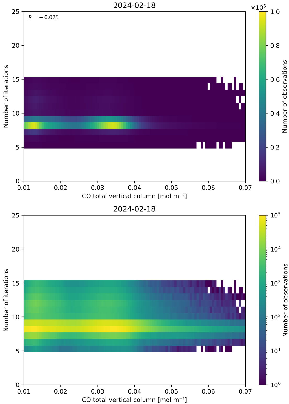
Figure 42: Scatter density plot of “CO total vertical column” against “Number of iterations” for 2024-02-17 to 2024-02-19.
