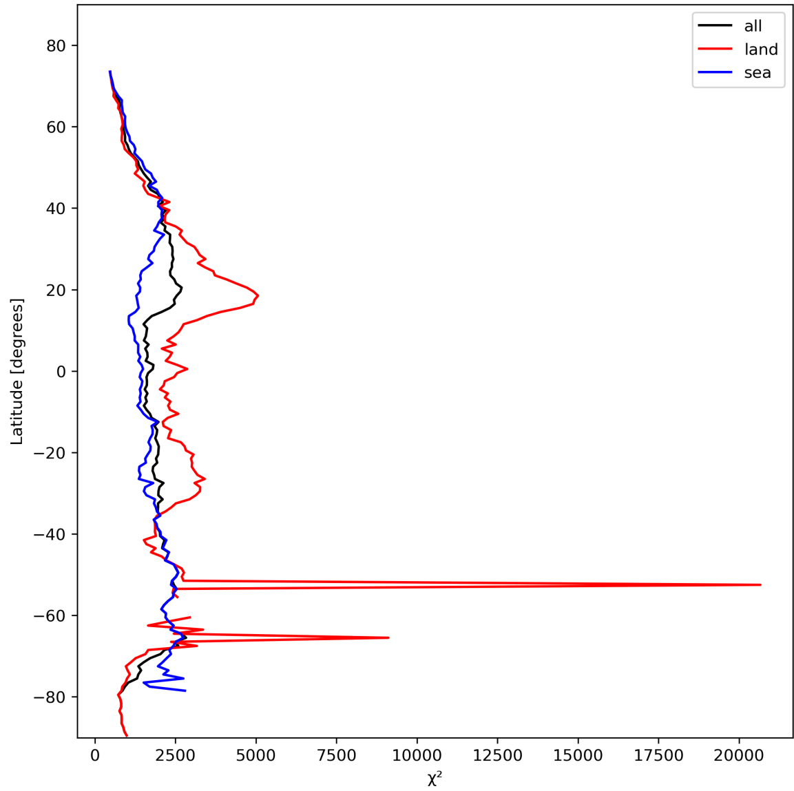
Figure 14: Zonal average of “ \chi^2 ” for 2024-02-17 to 2024-02-19.
