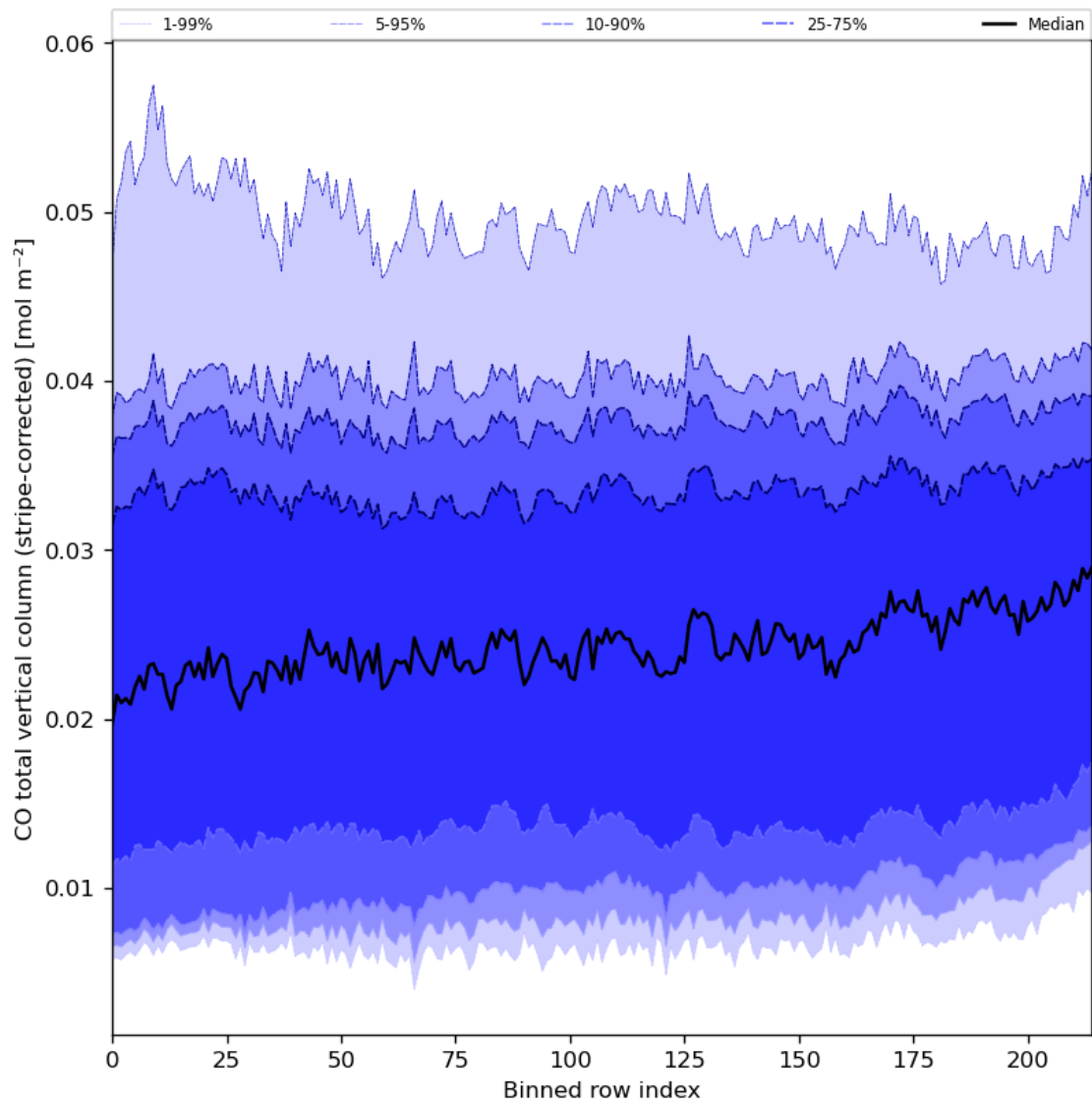
Figure 27: Along track statistics of “CO total vertical column (stripe-corrected)” for 2024-02-17 to 2024-02-19
