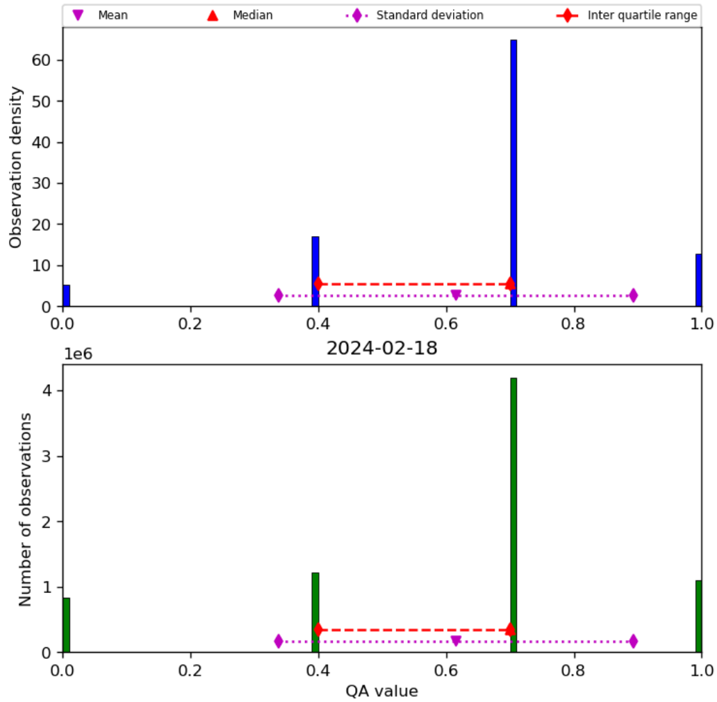
Figure 17: Histogram of “QA value” for 2024-02-17 to 2024-02-19
