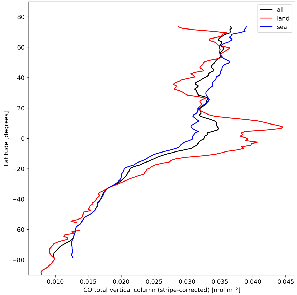
Figure 11: Zonal average of “CO total vertical column (stripe-corrected)” for 2024-02-17 to 2024-02-19.
