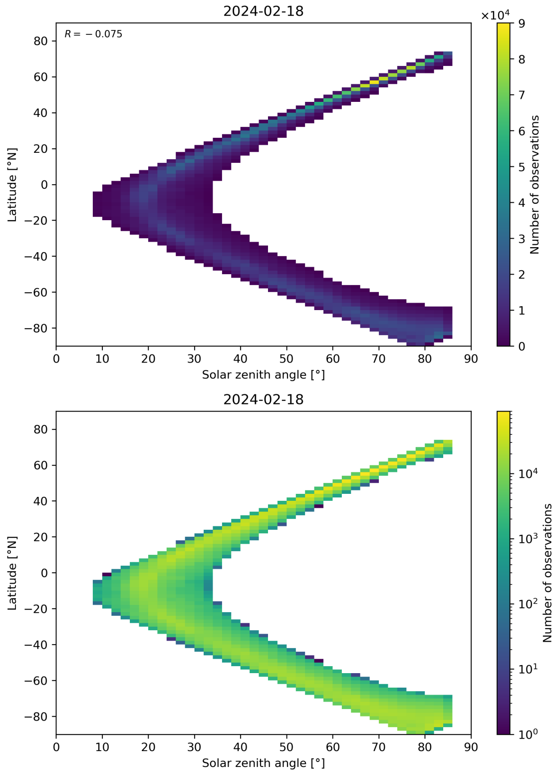
Figure 66: Scatter density plot of “Solar zenith angle” against “Latitude” for 2024-02-17 to 2024-02-19.
