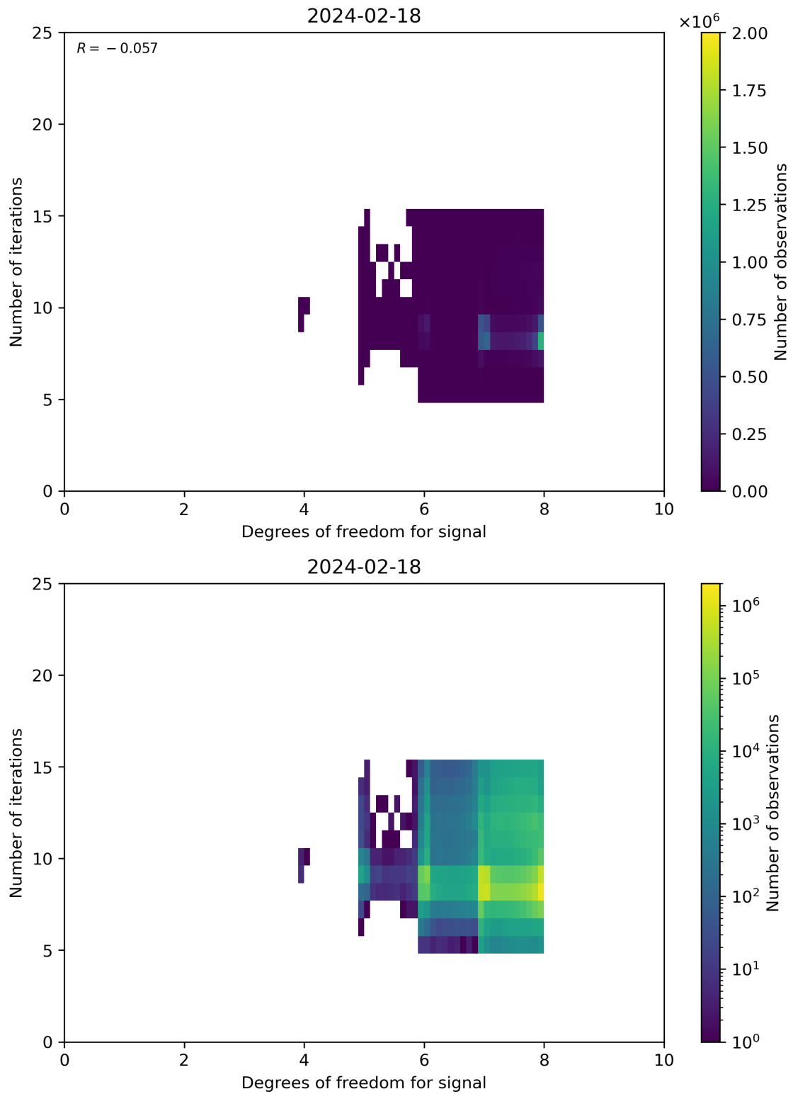
Figure 50: Scatter density plot of “Degrees of freedom for signal” against “Number of iterations” for 2024-02-17 to 2024-02-19.
