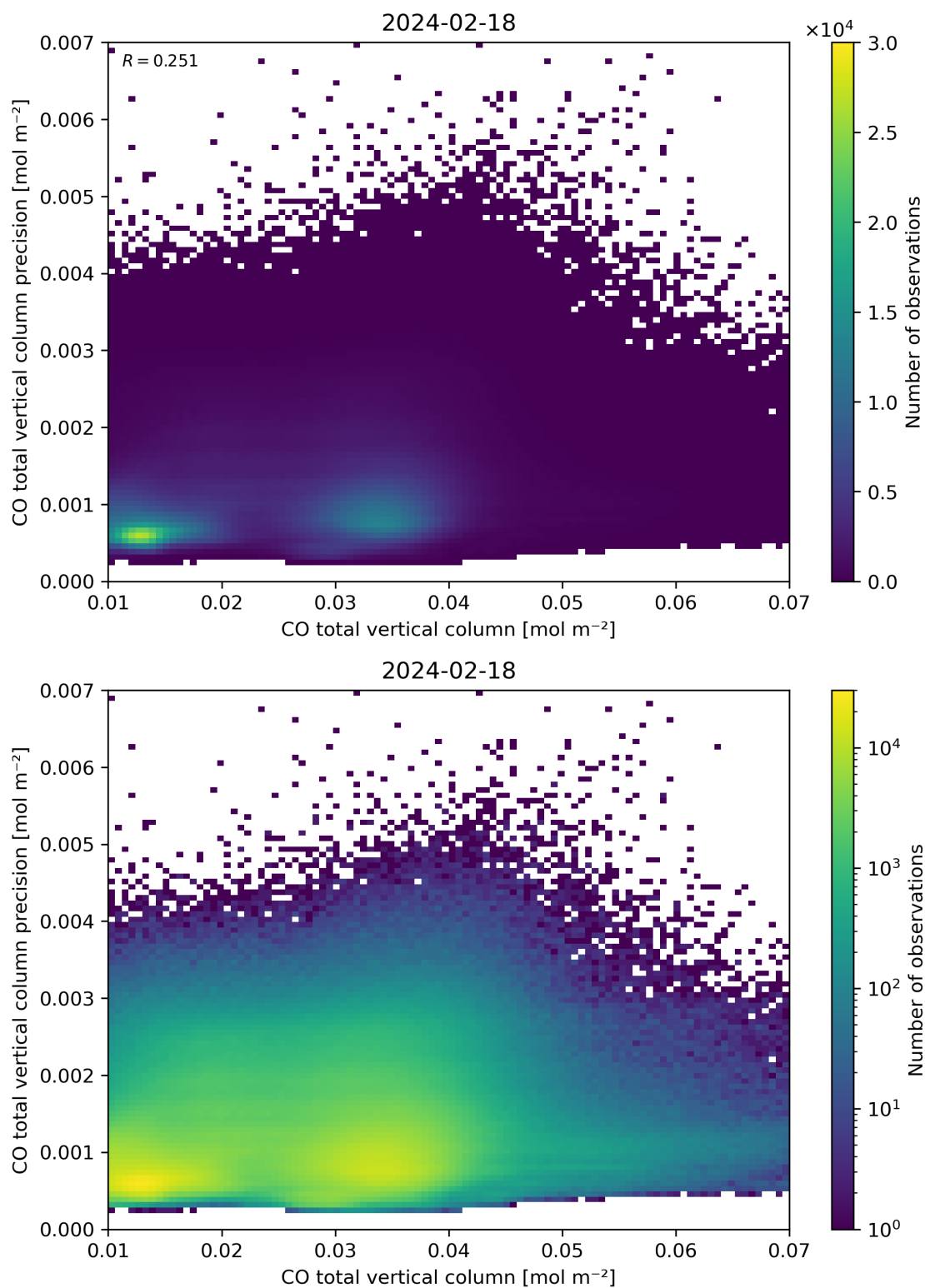
Figure 34: Scatter density plot of “CO total vertical column” against “CO total vertical column precision” for 2024-02-17 to 2024-02-19.
