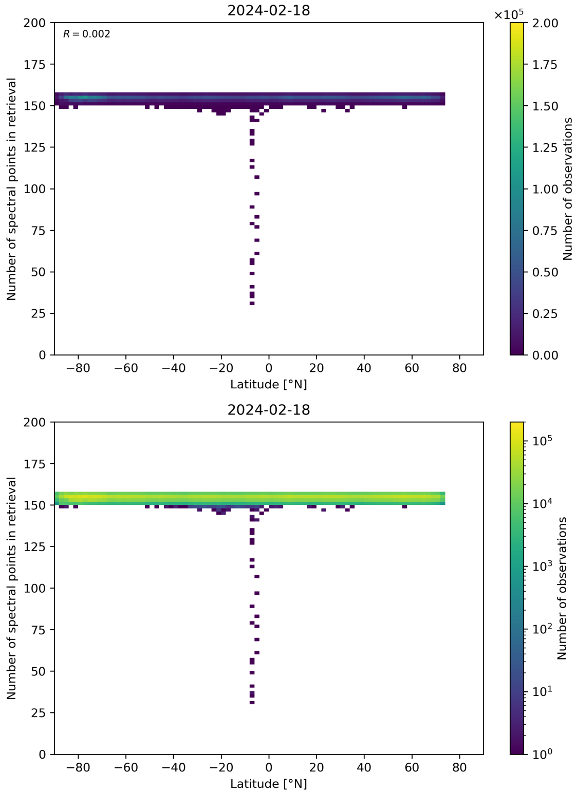
Figure 57: Scatter density plot of “Latitude” against “Number of spectral points in retrieval” for 2024-02-17 to 2024-02-19.
