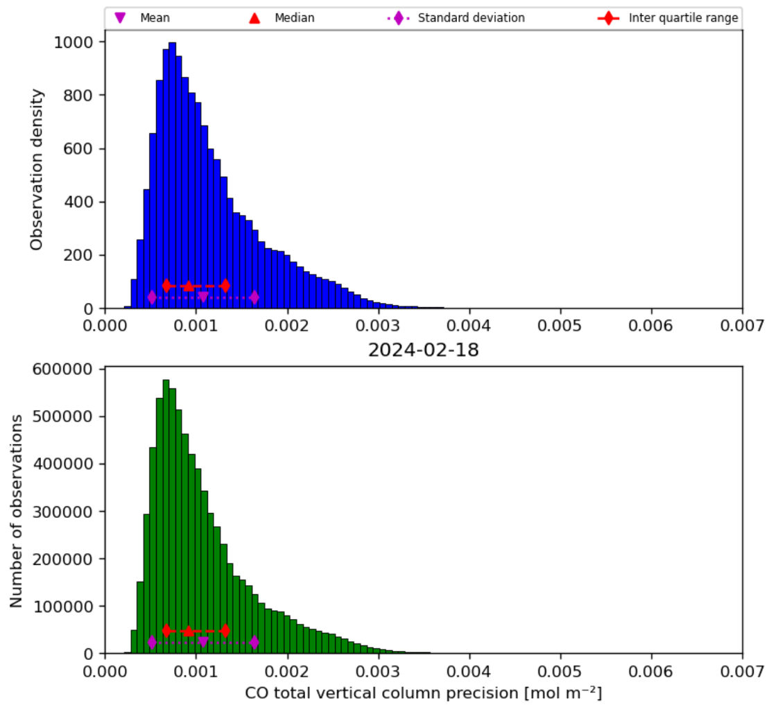
Figure 20: Histogram of “CO total vertical column precision” for 2024-02-17 to 2024-02-19
