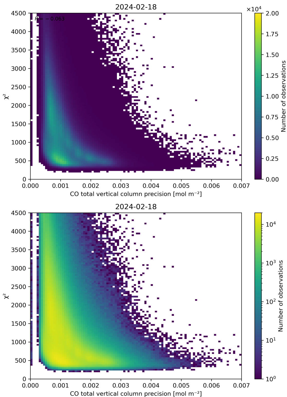
Figure 44: Scatter density plot of “CO total vertical column precision” against “ \chi^2 ” for 2024-02-17 to 2024-02-19.
