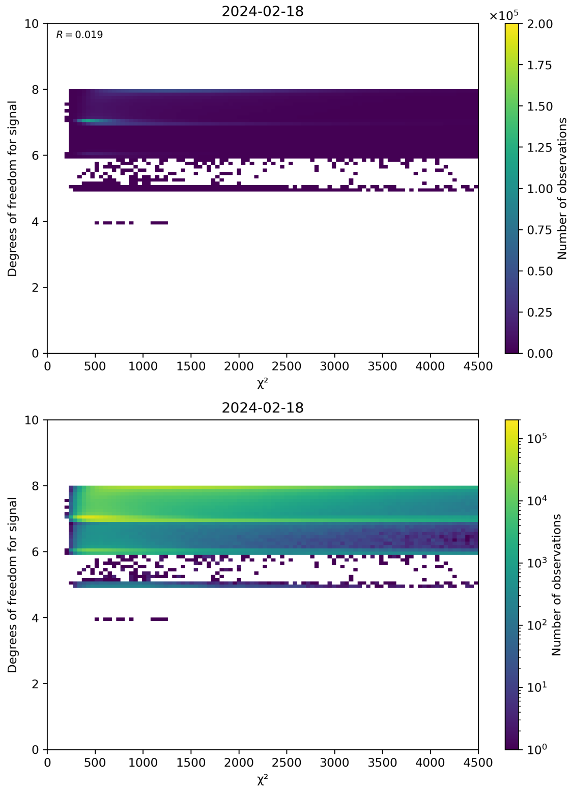
Figure 48: Scatter density plot of “ \chi^2 ” against “Degrees of freedom for signal” for 2024-02-17 to 2024-02-19.
