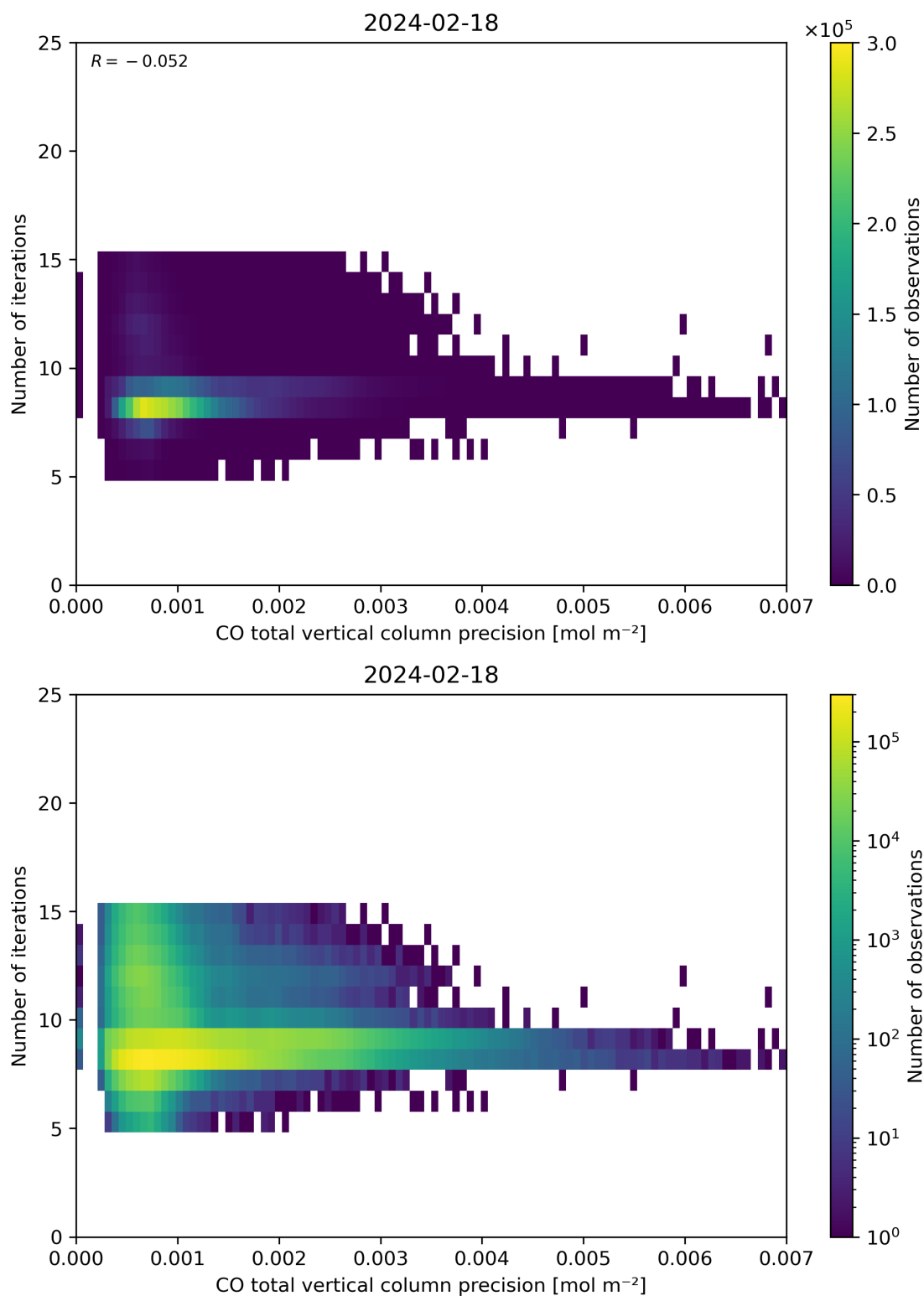
Figure 46: Scatter density plot of “CO total vertical column precision” against “Number of iterations” for 2024-02-17 to 2024-02-19.
