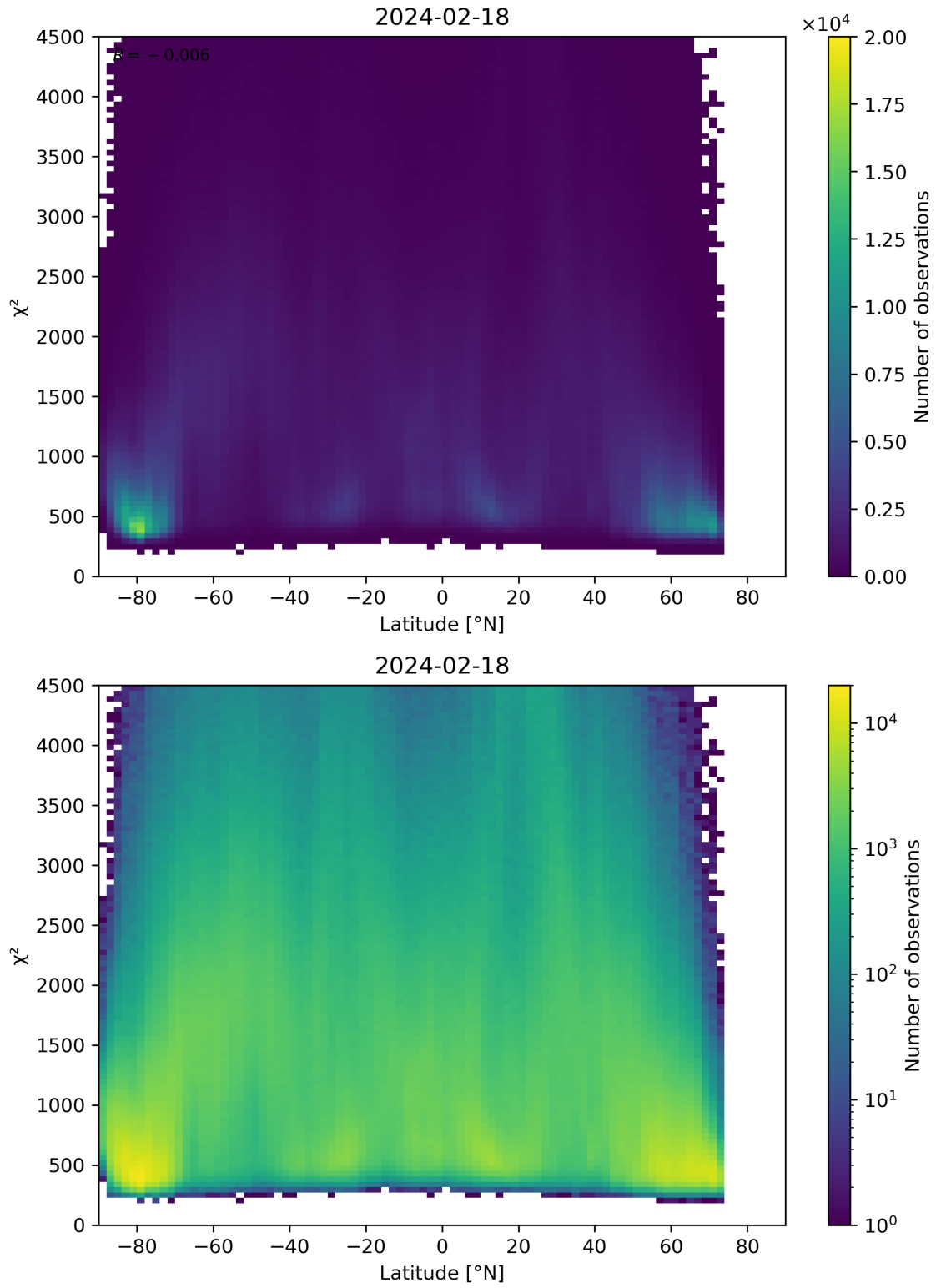
Figure 54: Scatter density plot of “Latitude” against “ \chi^2 ” for 2024-02-17 to 2024-02-19.
