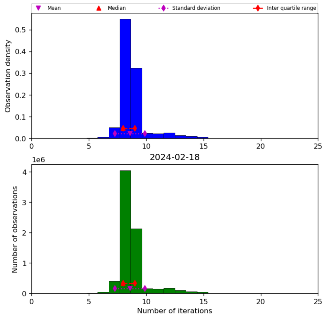
Figure 24: Histogram of “Number of iterations” for 2024-02-17 to 2024-02-19
