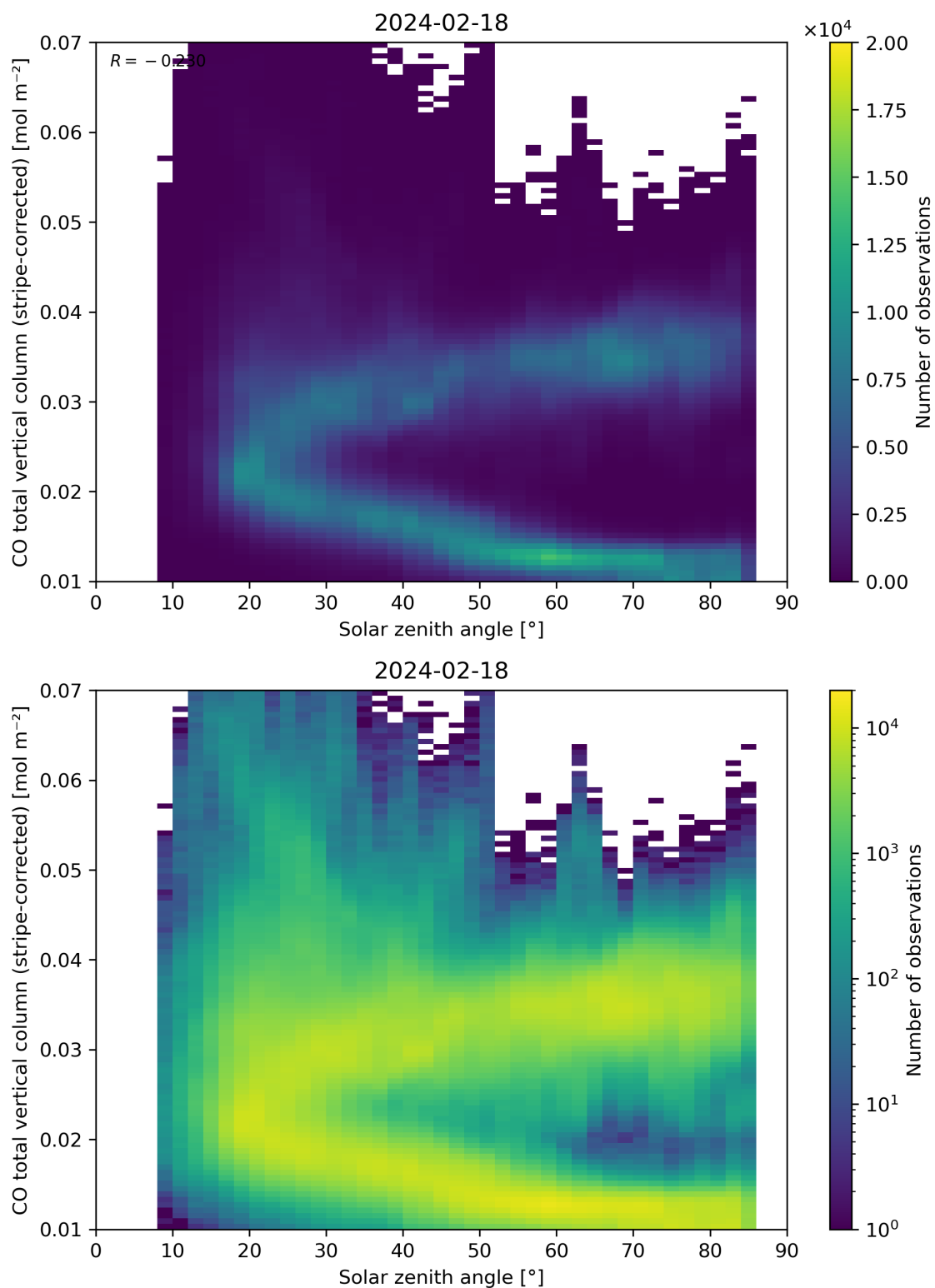
Figure 62: Scatter density plot of “Solar zenith angle” against “CO total vertical column (stripe-corrected)” for 2024-02-17 to 2024-02-19.
