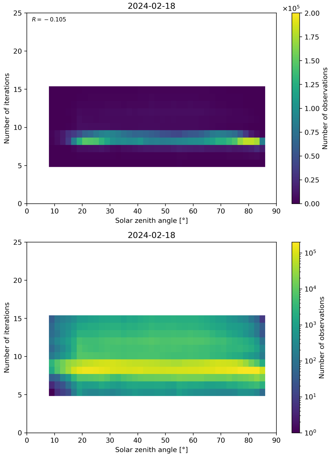
Figure 67: Scatter density plot of “Solar zenith angle” against “Number of iterations” for 2024-02-17 to 2024-02-19.
