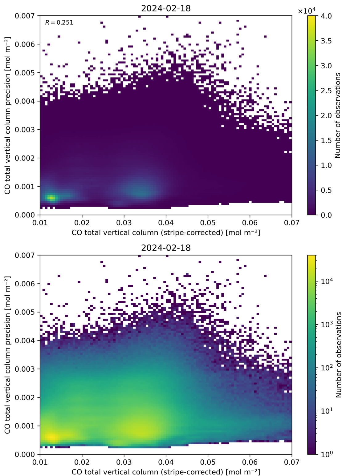
Figure 36: Scatter density plot of “CO total vertical column (stripe-corrected)” against “CO total vertical column precision” for 2024-02-17 to 2024-02-19.
