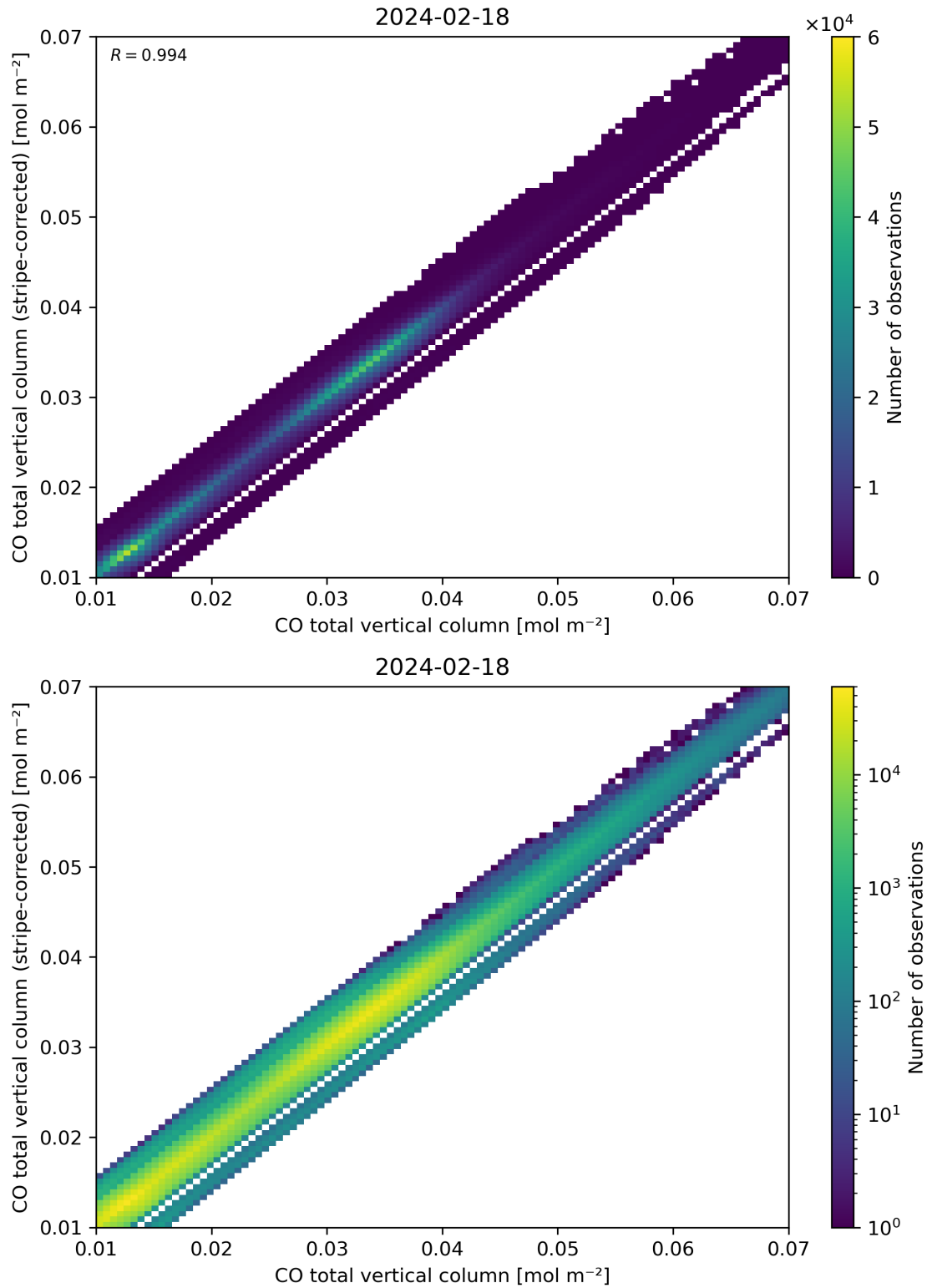
Figure 33: Scatter density plot of “CO total vertical column” against “CO total vertical column (stripe-corrected)” for 2024-02-17 to 2024-02-19.
