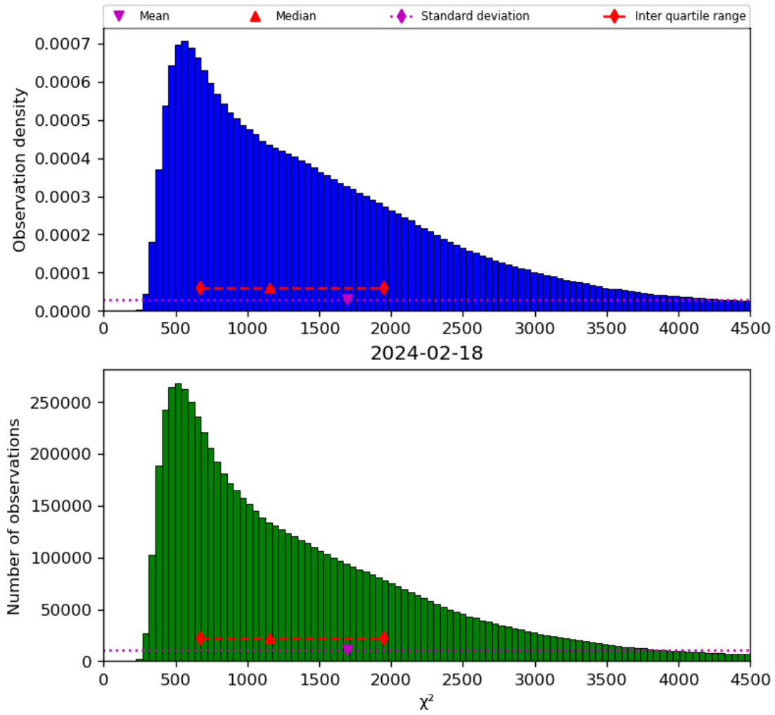
Figure 22: Histogram of “ \chi^2 ” for 2024-02-17 to 2024-02-19
