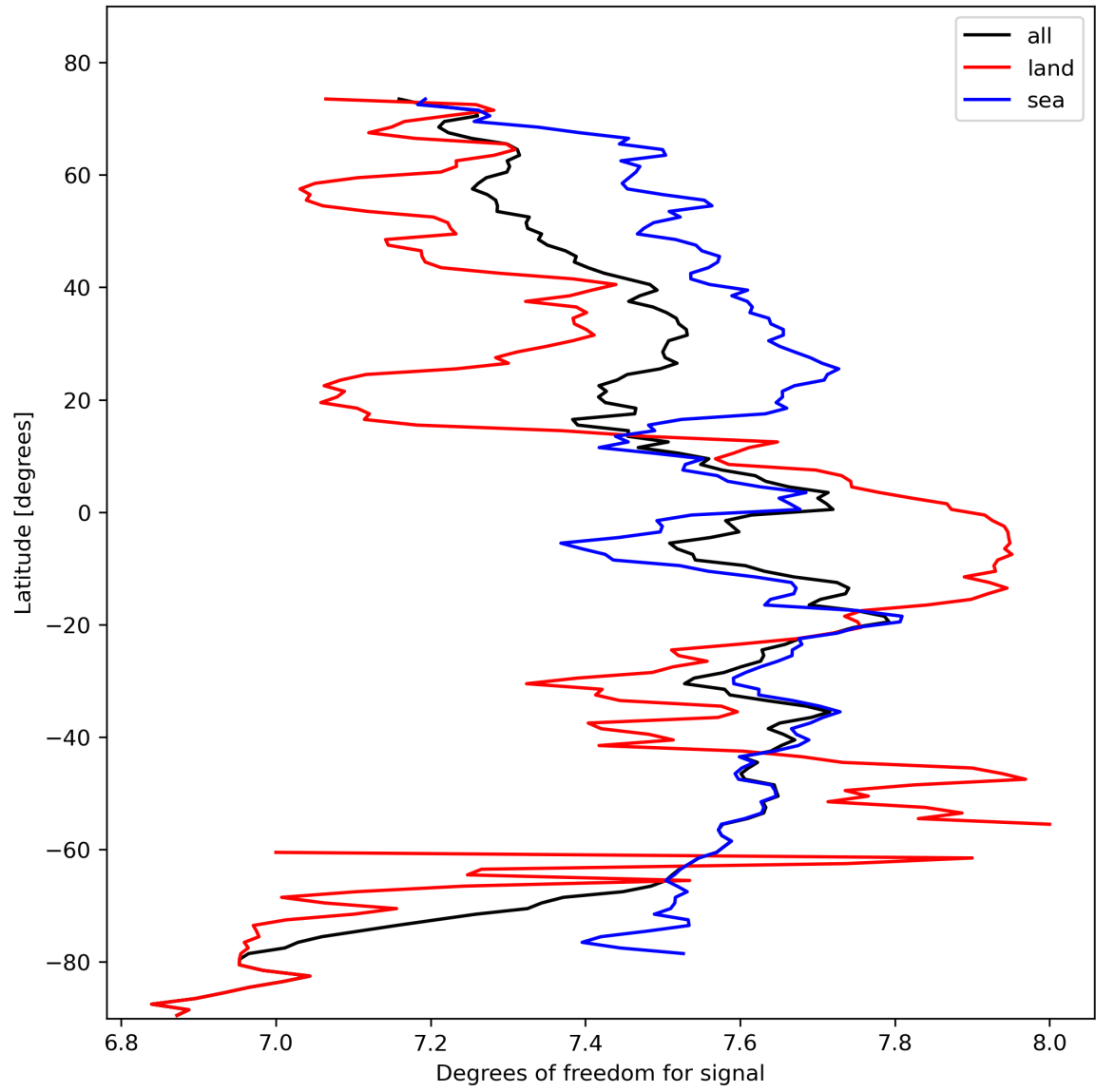
Figure 15: Zonal average of “Degrees of freedom for signal” for 2024-02-17 to 2024-02-19.
