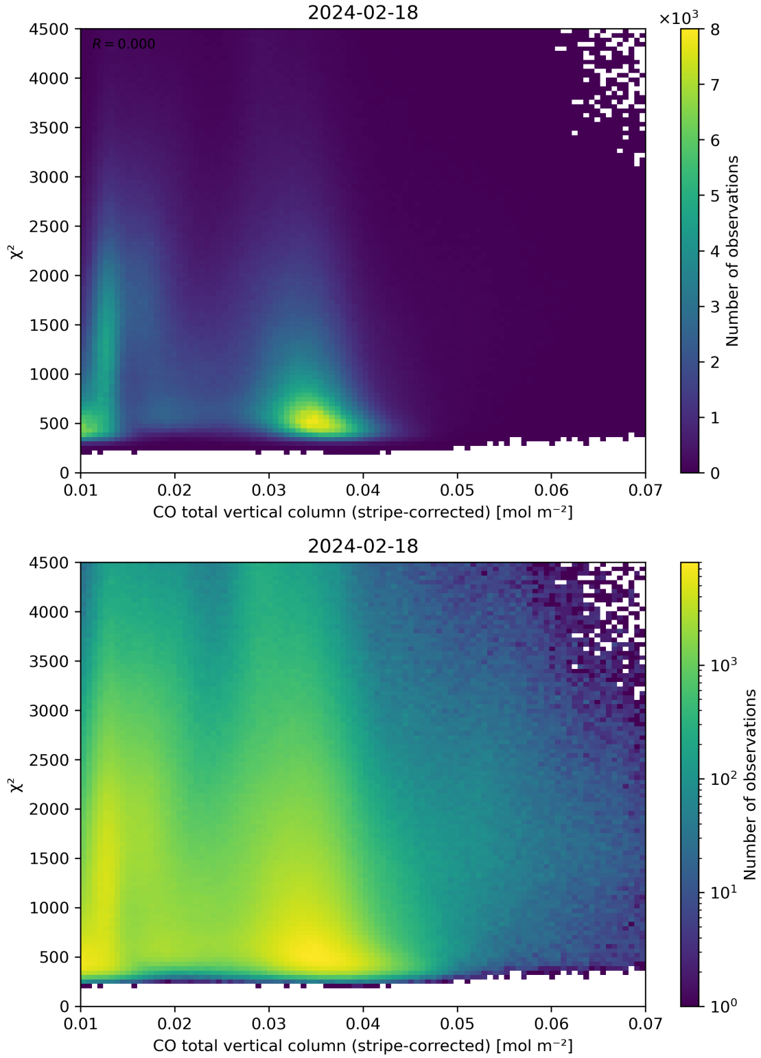
Figure 37: Scatter density plot of “CO total vertical column (stripe-corrected)” against “ \chi^2 ” for 2024-02-17 to 2024-02-19.
