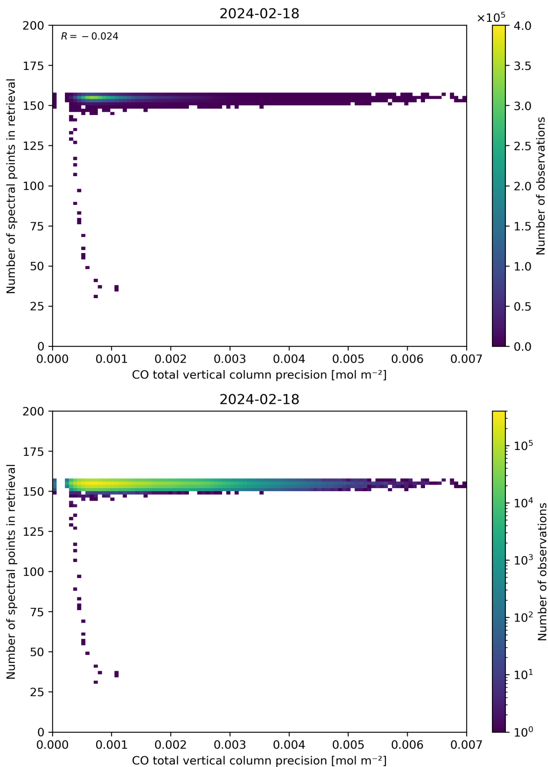
Figure 47: Scatter density plot of “CO total vertical column precision” against “Number of spectral points in retrieval” for 2024-02-17 to 2024-02-19.
