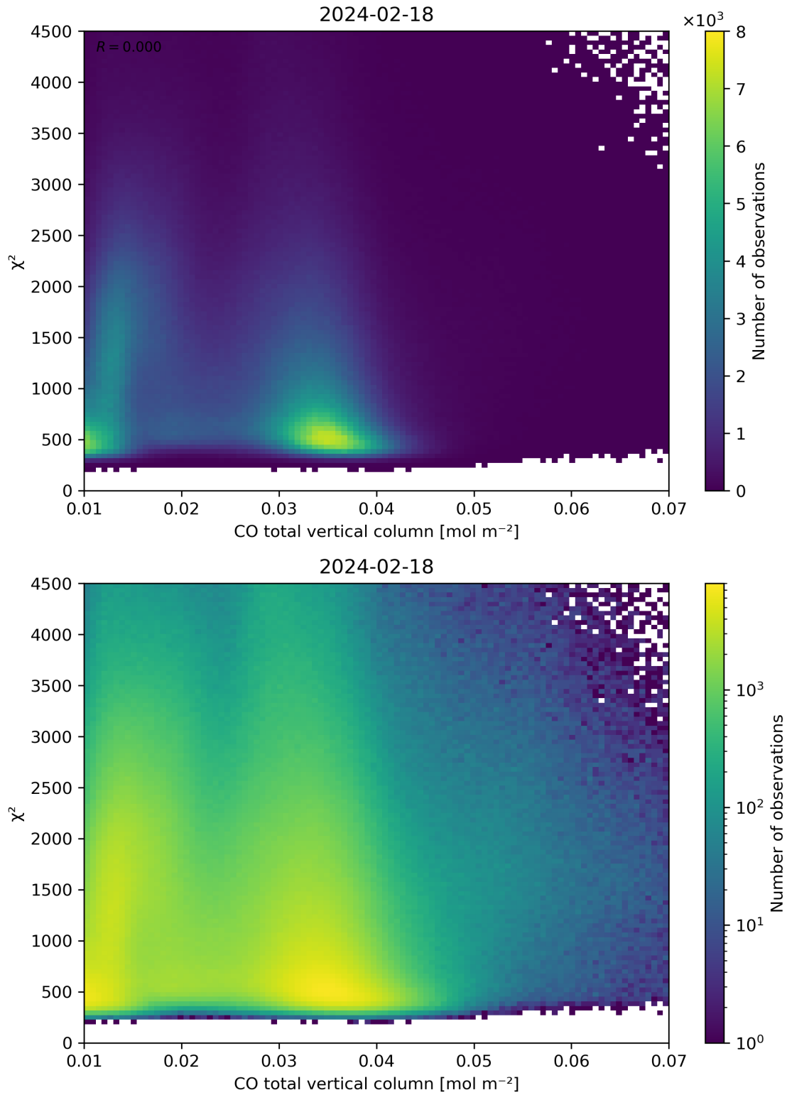
Figure 35: Scatter density plot of “CO total vertical column” against “ \chi^2 ” for 2024-02-17 to 2024-02-19.
