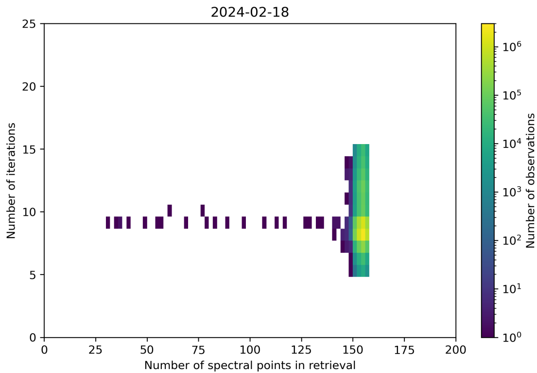
Figure 60: Scatter density plot of “Number of spectral points in retrieval” against “Number of iterations” for 2024-02-17 to 2024-02-19.
