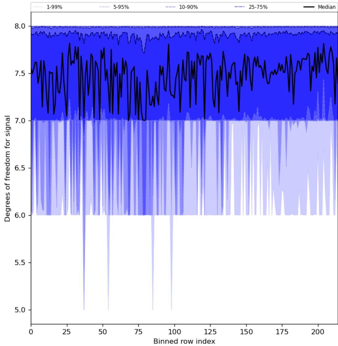
Figure 31: Along track statistics of “Degrees of freedom for signal” for 2024-02-17 to 2024-02-19
