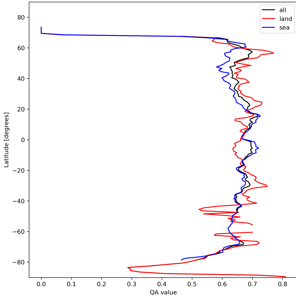
Figure 9: Zonal average of “QA value” for 2024-02-17 to 2024-02-19.
