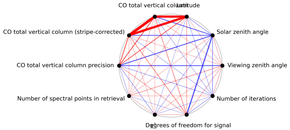
Figure 1: Map of correlation graph for 2024-02-17 to 2024-02-19.
