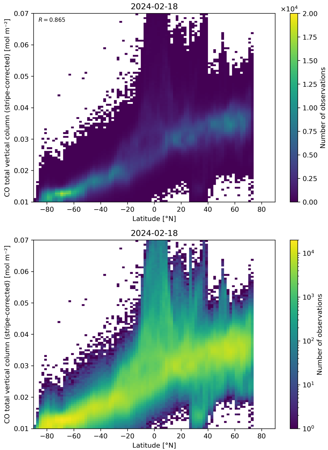
Figure 52: Scatter density plot of “Latitude” against “CO total vertical column (stripe-corrected)” for 2024-02-17 to 2024-02-19.
