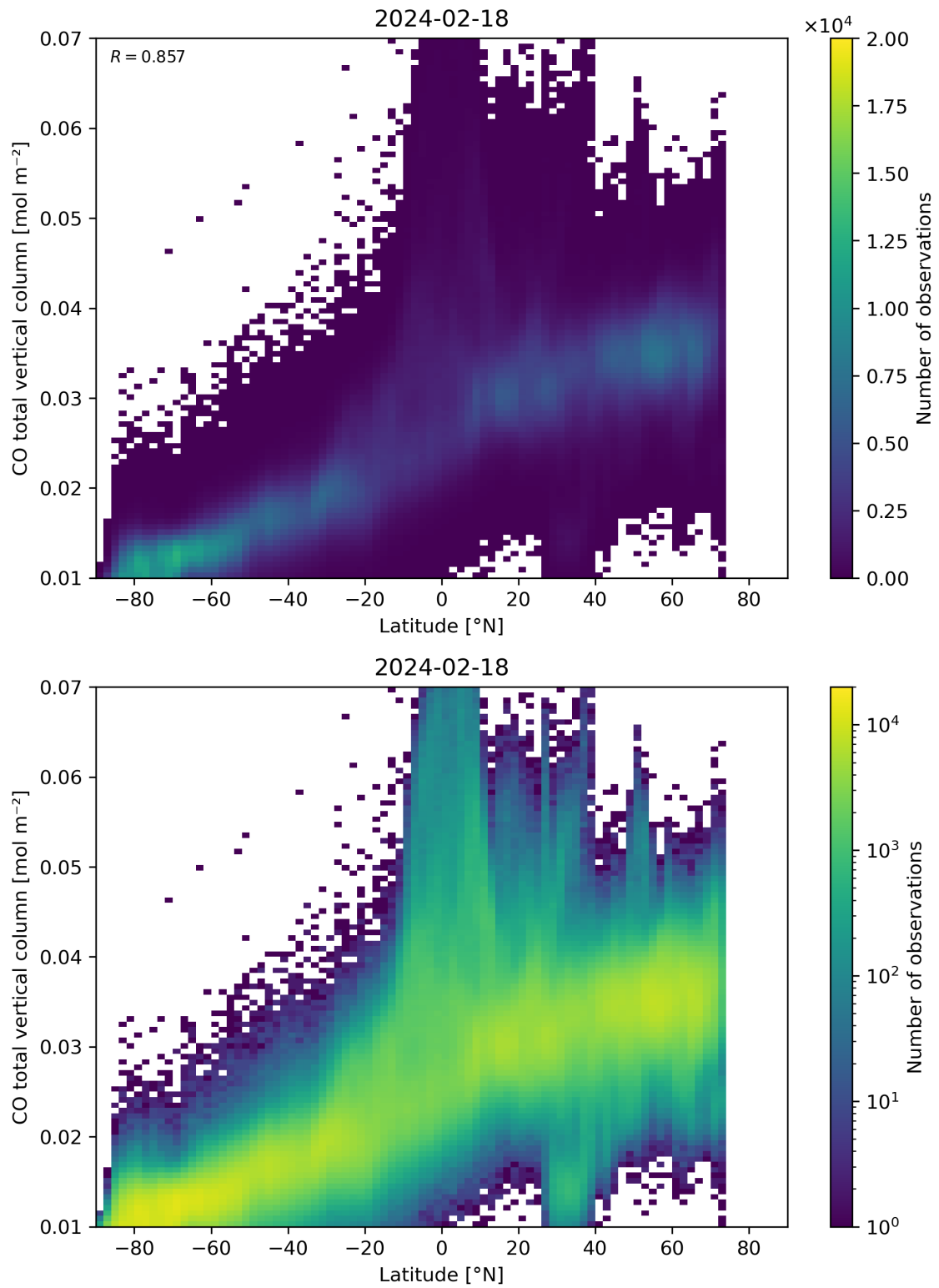
Figure 51: Scatter density plot of “Latitude” against “CO total vertical column” for 2024-02-17 to 2024-02-19.
