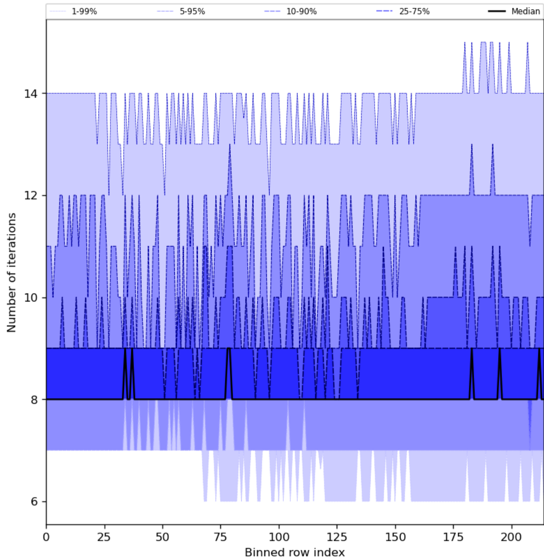
Figure 32: Along track statistics of “Number of iterations” for 2024-02-18 to 2024-02-20
