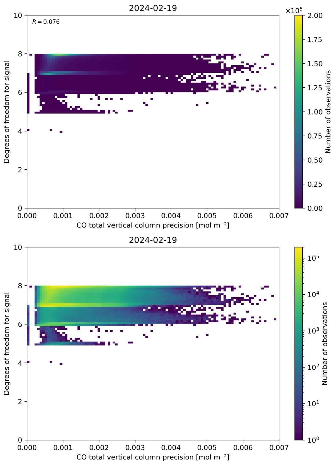
Figure 45: Scatter density plot of “CO total vertical column precision” against “Degrees of freedom for signal” for 2024-02-18 to 2024-02-20.
