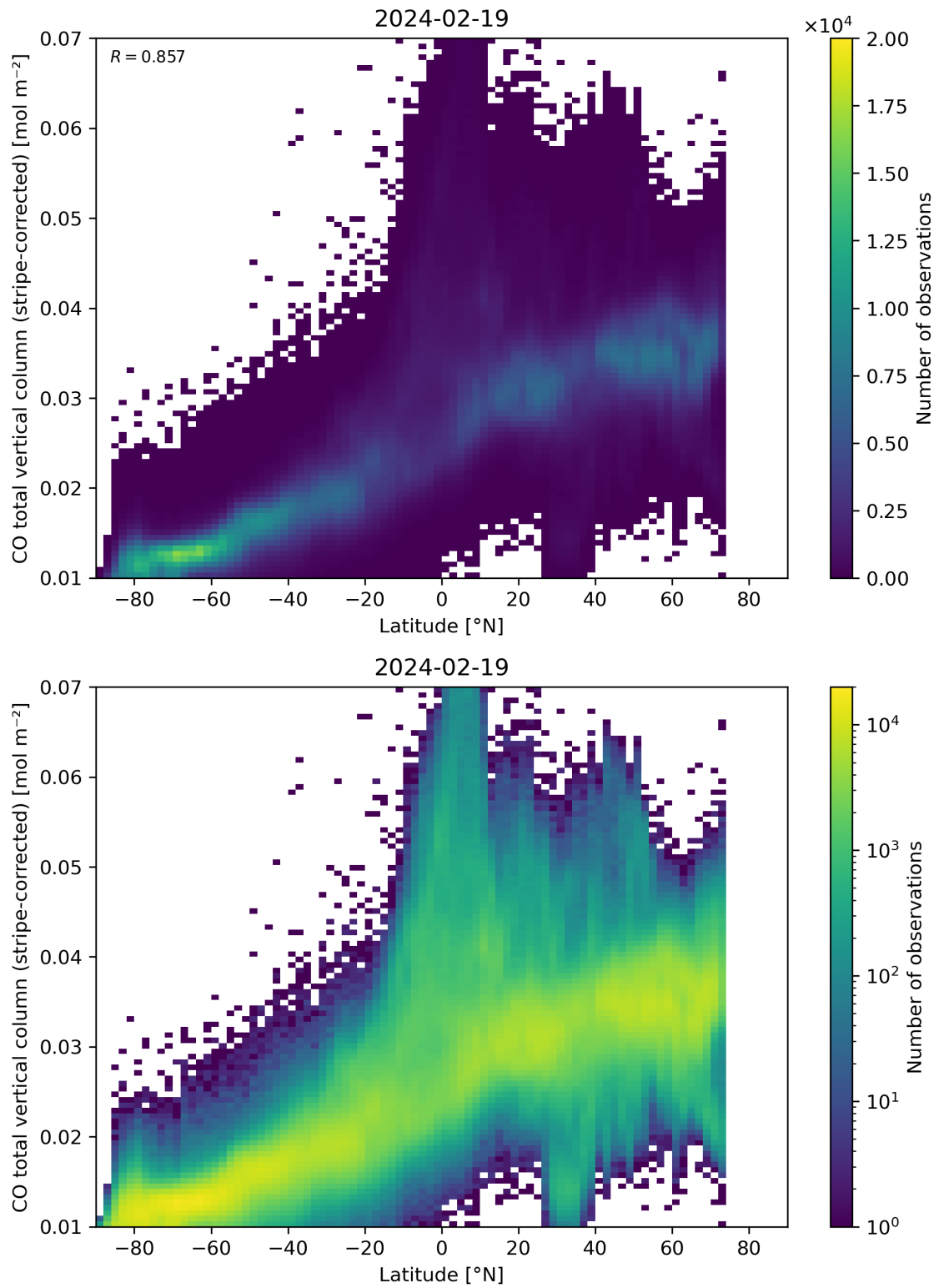
Figure 52: Scatter density plot of “Latitude” against “CO total vertical column (stripe-corrected)” for 2024-02-18 to 2024-02-20.
