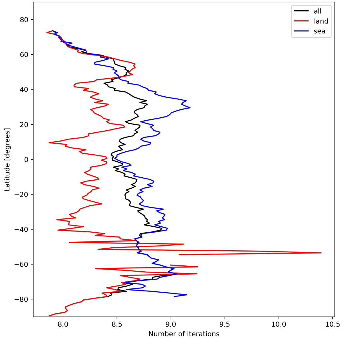
Figure 16: Zonal average of “Number of iterations” for 2024-02-18 to 2024-02-20.
