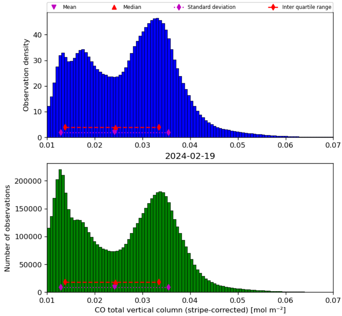
Figure 19: Histogram of “CO total vertical column (stripe-corrected)” for 2024-02-18 to 2024-02-20
