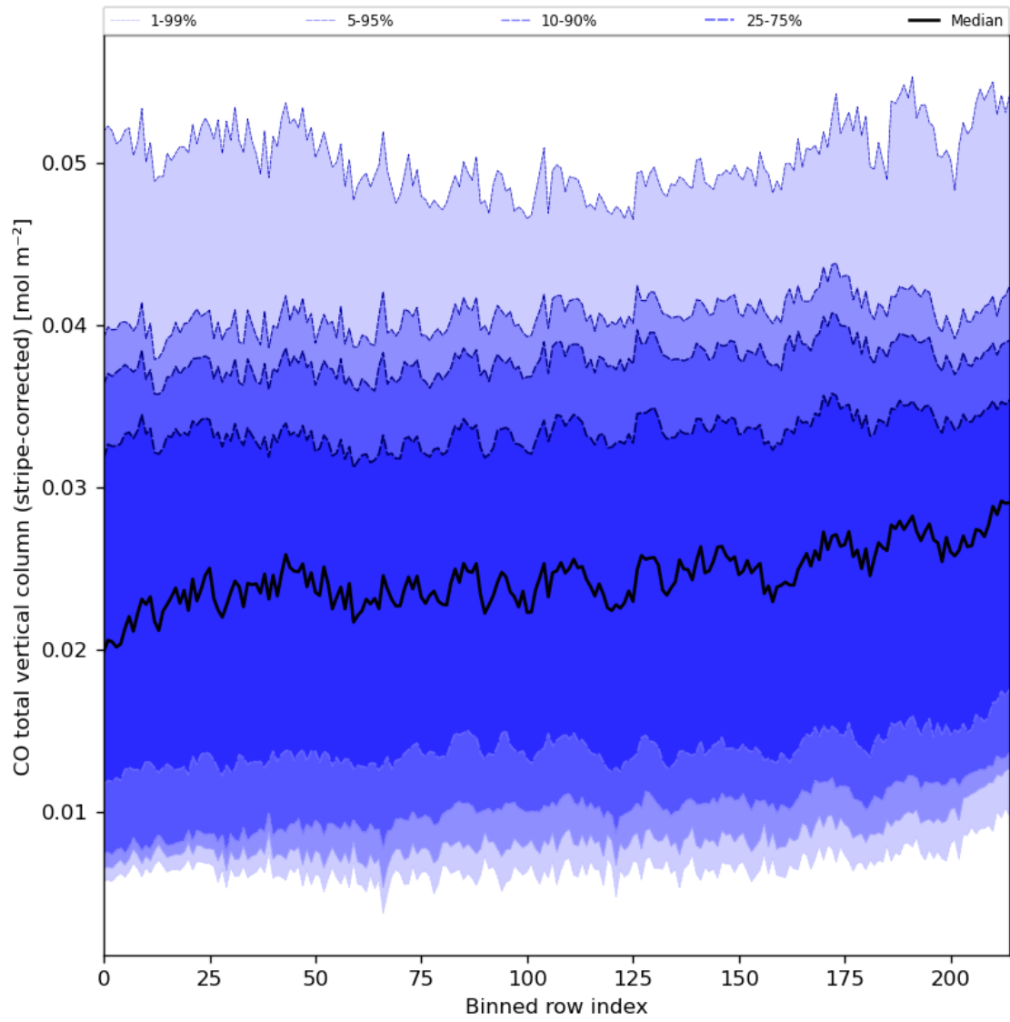
Figure 27: Along track statistics of “CO total vertical column (stripe-corrected)” for 2024-02-18 to 2024-02-20
