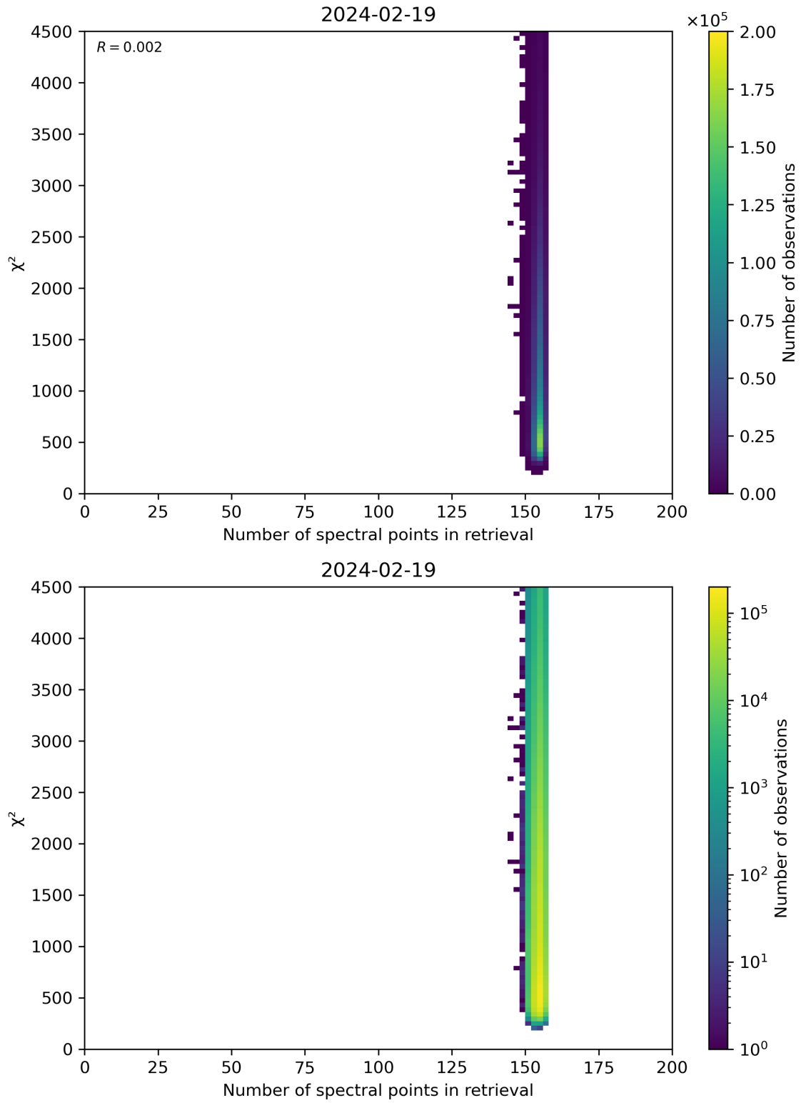
Figure 58: Scatter density plot of “Number of spectral points in retrieval” against “ \chi^2 ” for 2024-02-18 to 2024-02-20.
