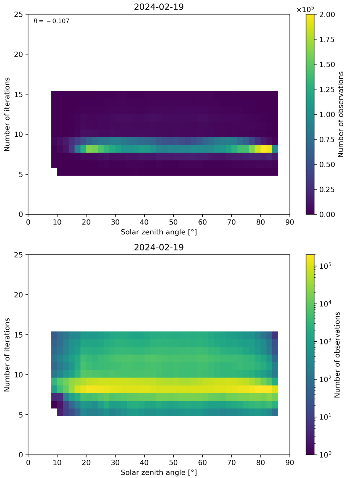
Figure 67: Scatter density plot of “Solar zenith angle” against “Number of iterations” for 2024-02-18 to 2024-02-20.
