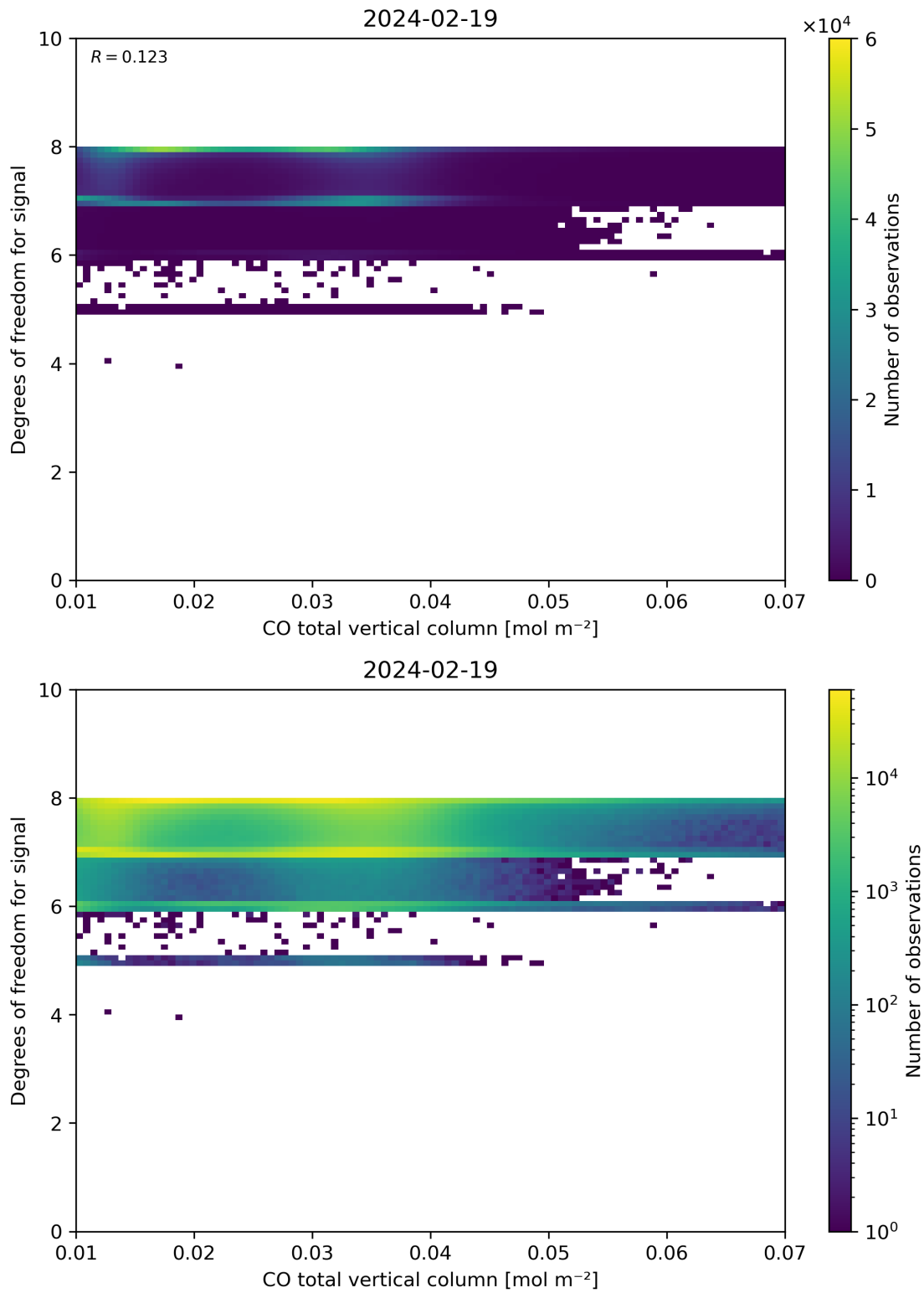
Figure 41: Scatter density plot of “CO total vertical column” against “Degrees of freedom for signal” for 2024-02-18 to 2024-02-20.
