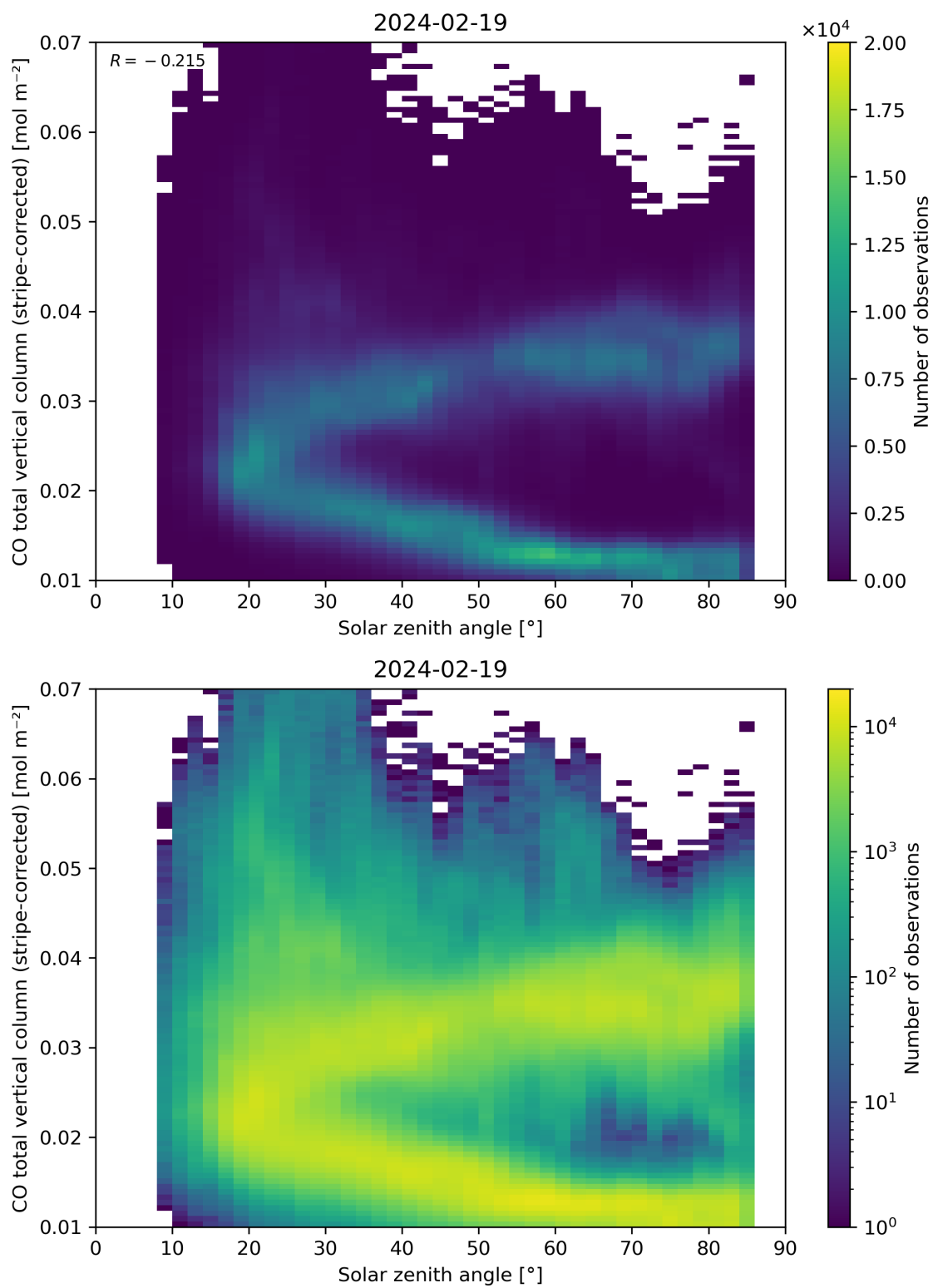
Figure 62: Scatter density plot of “Solar zenith angle” against “CO total vertical column (stripe-corrected)” for 2024-02-18 to 2024-02-20.
