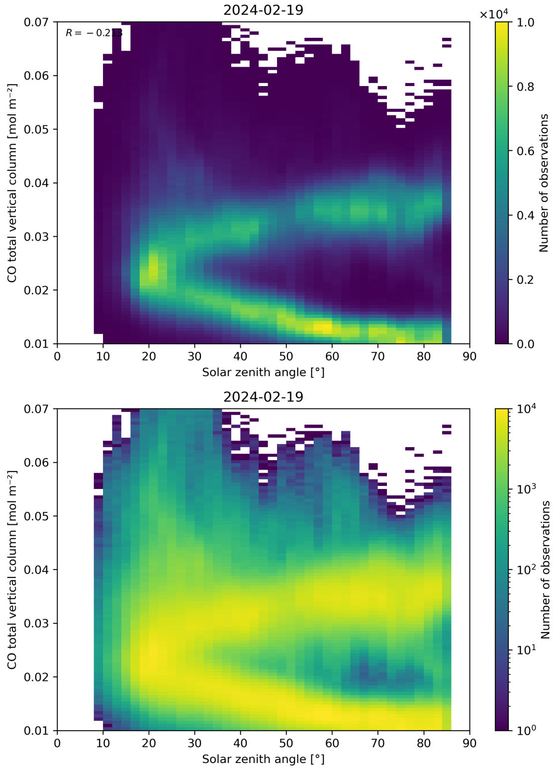
Figure 61: Scatter density plot of “Solar zenith angle” against “CO total vertical column” for 2024-02-18 to 2024-02-20.
