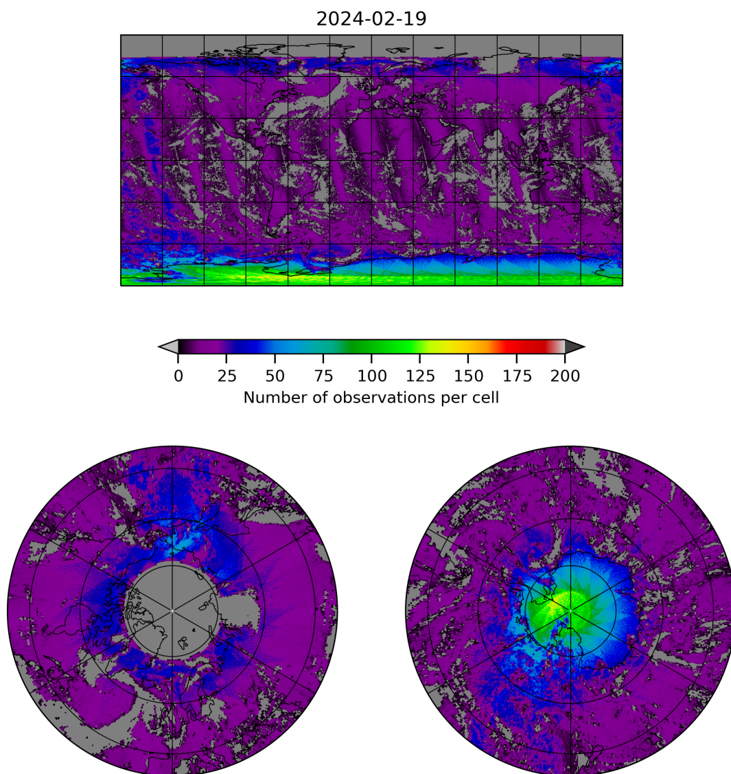
Figure 8: Map of the number of observations for 2024-02-18 to 2024-02-20
