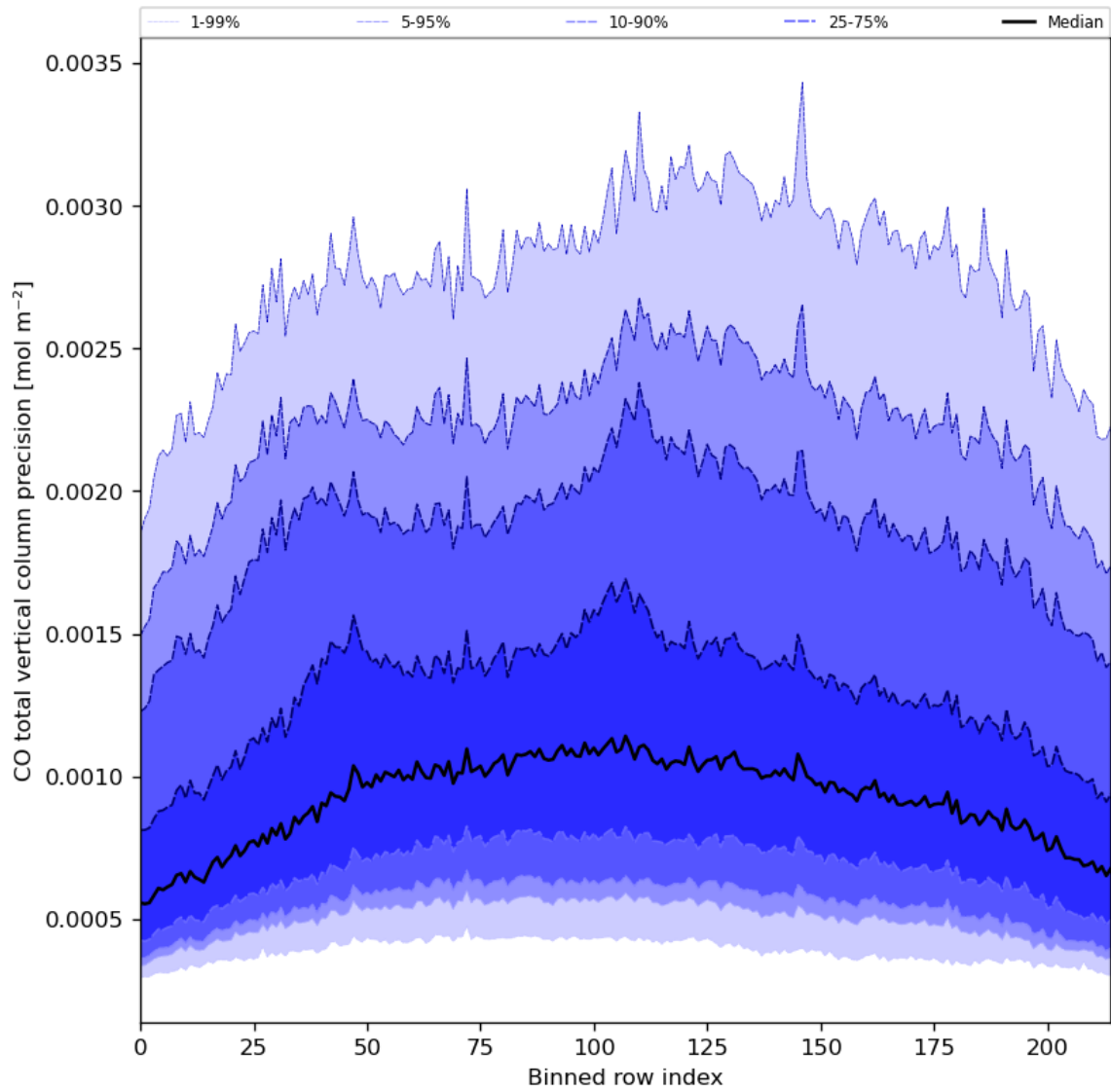
Figure 28: Along track statistics of “CO total vertical column precision” for 2024-02-18 to 2024-02-20
