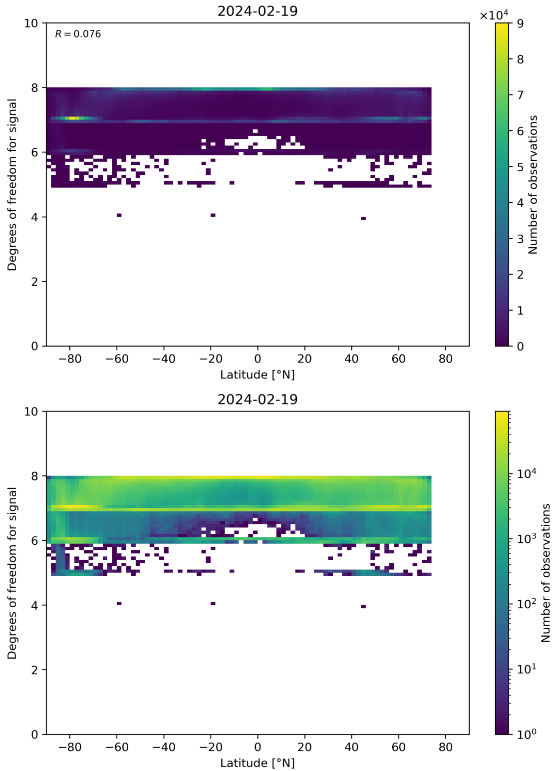
Figure 55: Scatter density plot of “Latitude” against “Degrees of freedom for signal” for 2024-02-18 to 2024-02-20.
