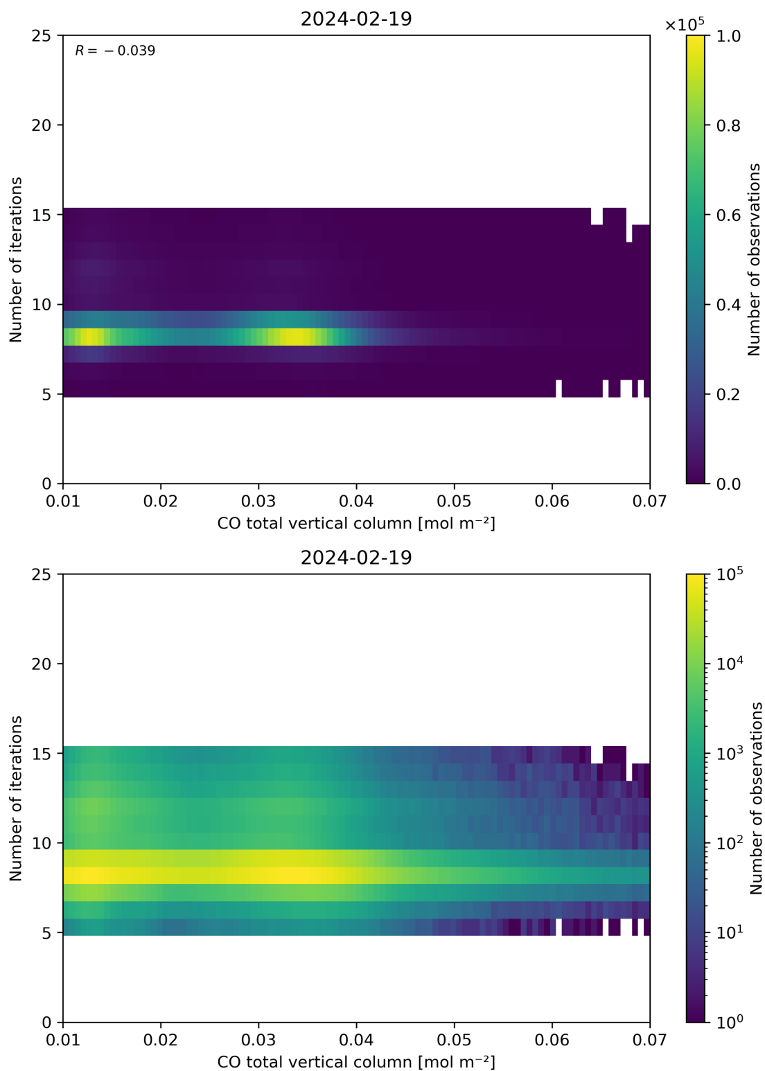
Figure 42: Scatter density plot of “CO total vertical column” against “Number of iterations” for 2024-02-18 to 2024-02-20.
