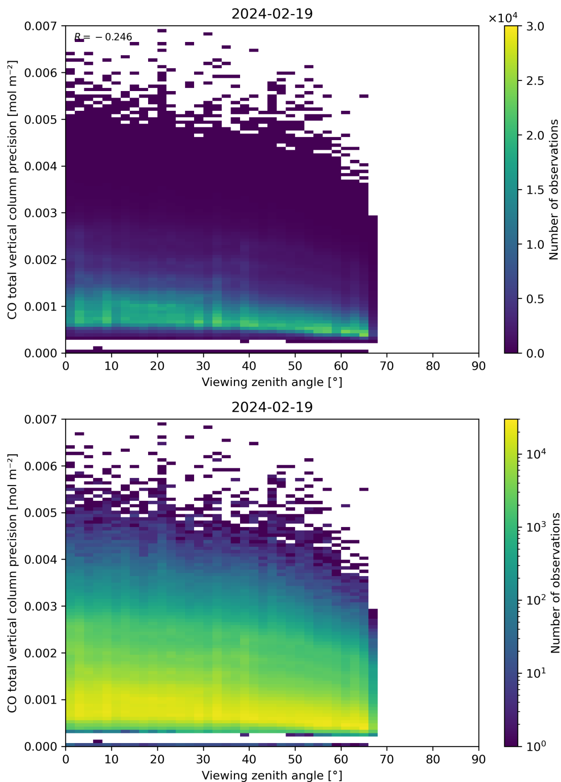
Figure 71: Scatter density plot of “Viewing zenith angle” against “CO total vertical column precision” for 2024-02-18 to 2024-02-20.
