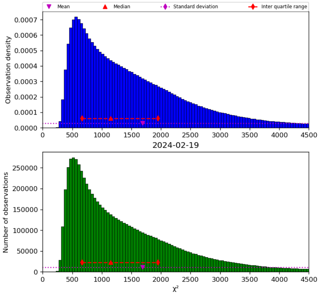
Figure 22: Histogram of “ \chi^2 ” for 2024-02-18 to 2024-02-20
