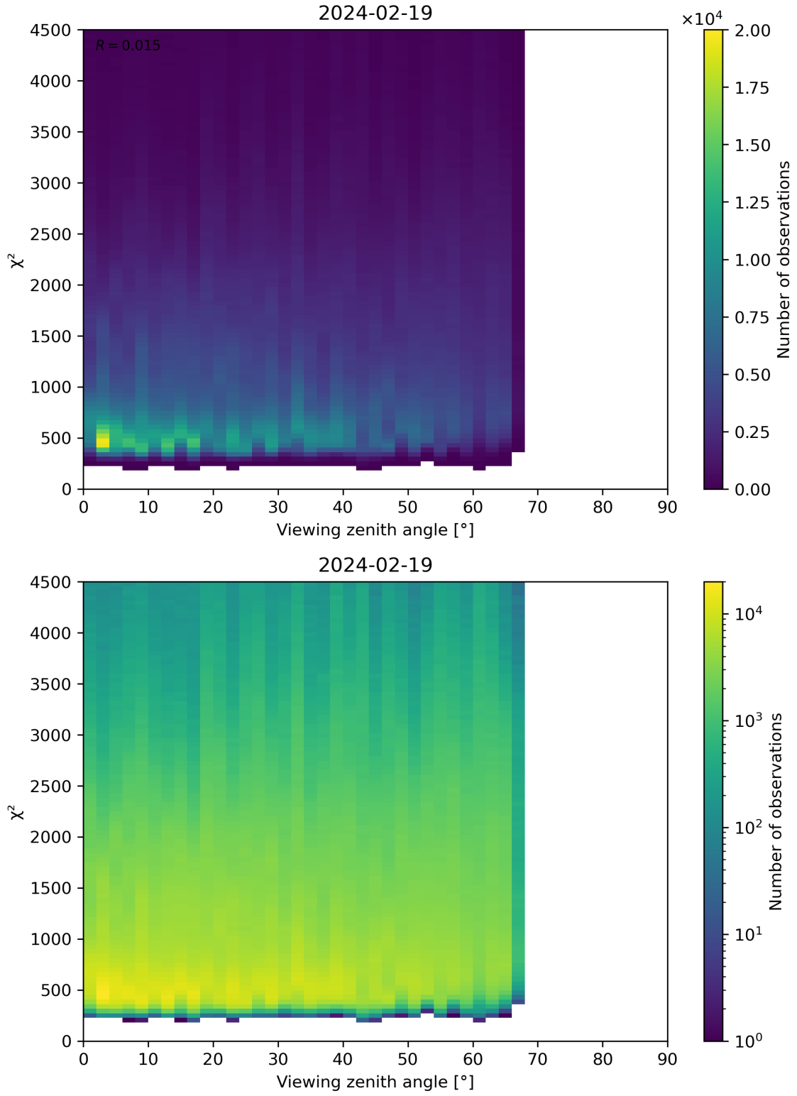
Figure 72: Scatter density plot of “Viewing zenith angle” against “ \chi^2 ” for 2024-02-18 to 2024-02-20.
