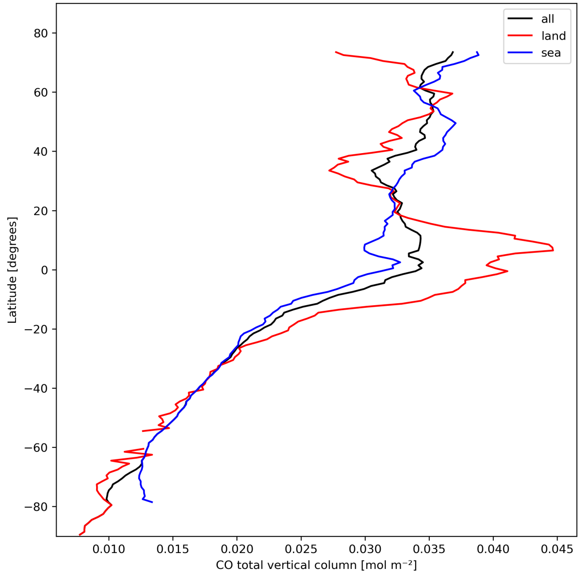
Figure 10: Zonal average of “CO total vertical column” for 2024-02-18 to 2024-02-20.
