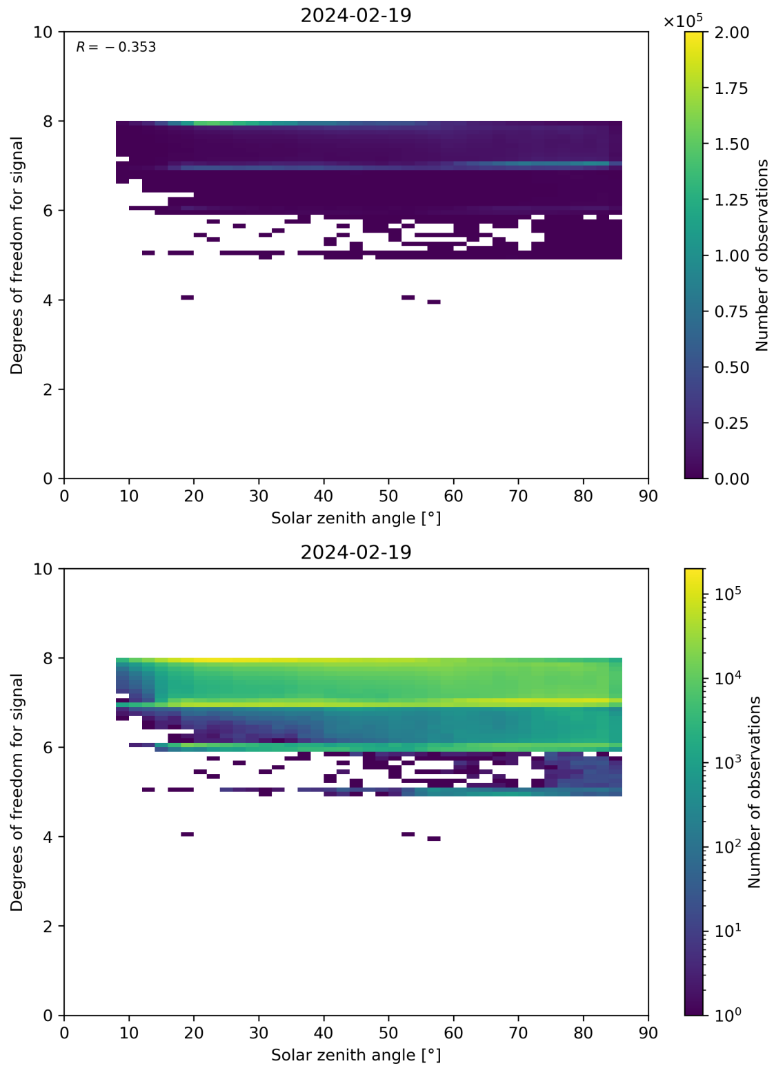
Figure 65: Scatter density plot of “Solar zenith angle” against “Degrees of freedom for signal” for 2024-02-18 to 2024-02-20.
