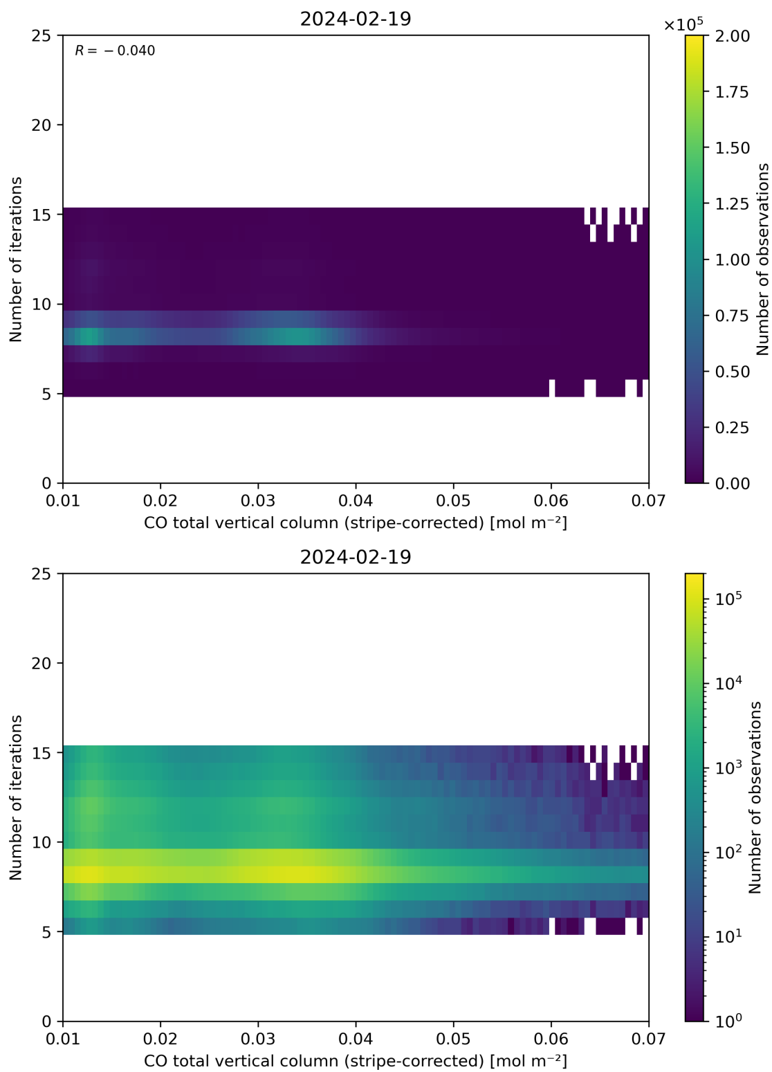
Figure 39: Scatter density plot of “CO total vertical column (stripe-corrected)” against “Number of iterations” for 2024-02-18 to 2024-02-20.
