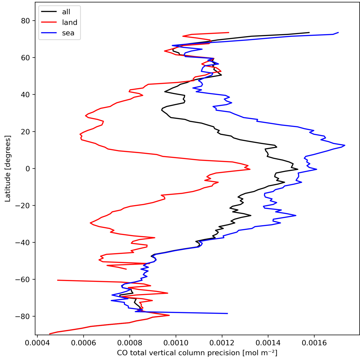
Figure 12: Zonal average of “CO total vertical column precision” for 2024-02-18 to 2024-02-20.
