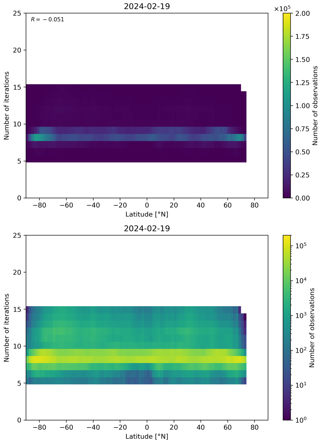
Figure 56: Scatter density plot of “Latitude” against “Number of iterations” for 2024-02-18 to 2024-02-20.
