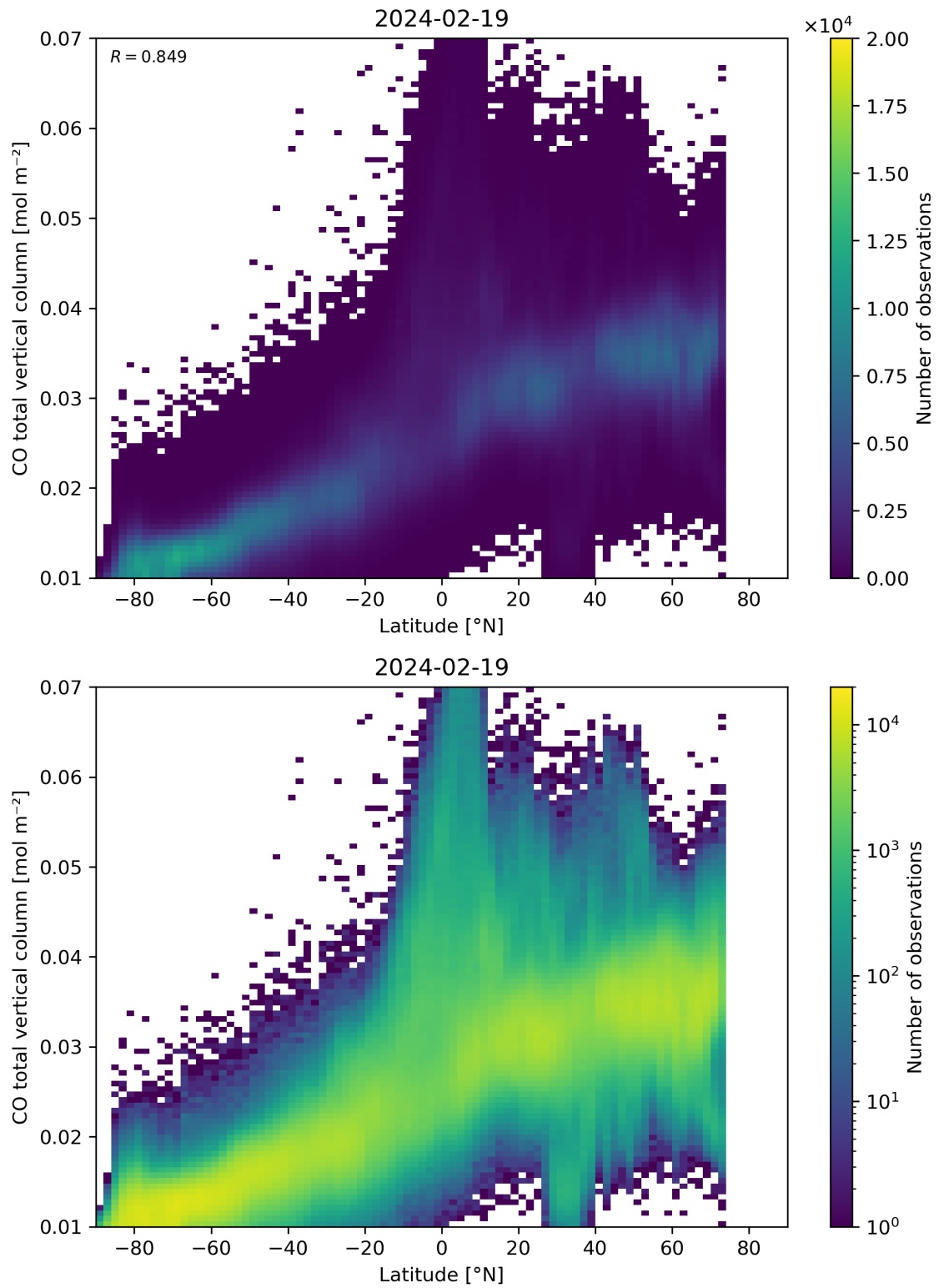
Figure 51: Scatter density plot of “Latitude” against “CO total vertical column” for 2024-02-18 to 2024-02-20.
