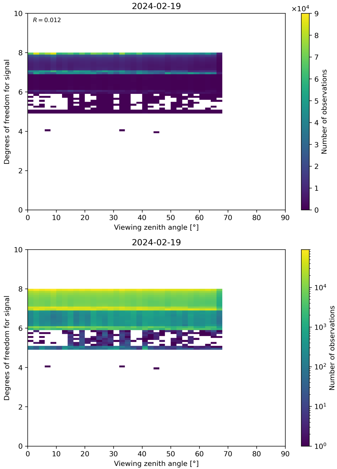
Figure 73: Scatter density plot of “Viewing zenith angle” against “Degrees of freedom for signal” for 2024-02-18 to 2024-02-20.
