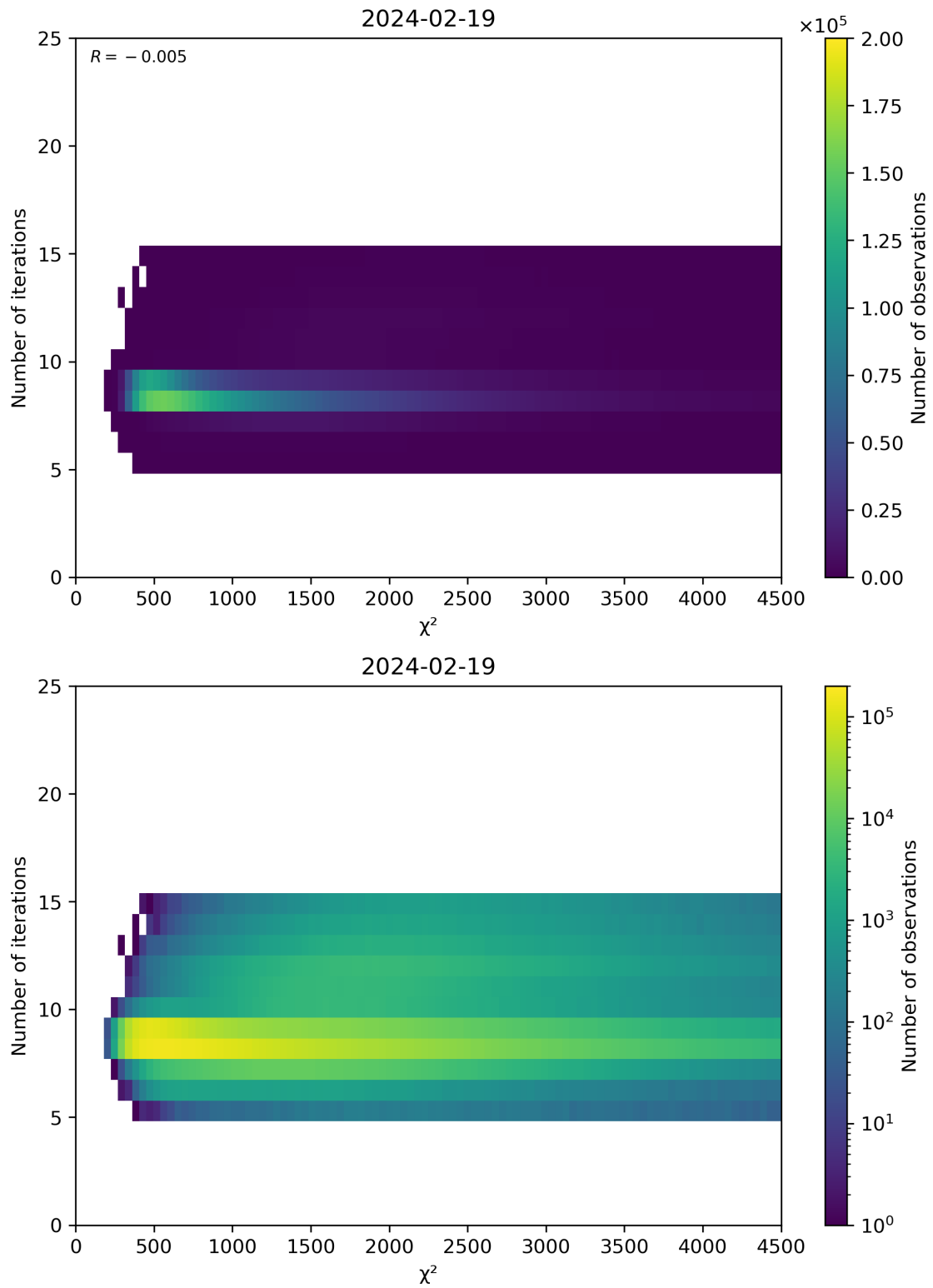
Figure 49: Scatter density plot of “ \chi^2 ” against “Number of iterations” for 2024-02-18 to 2024-02-20.
