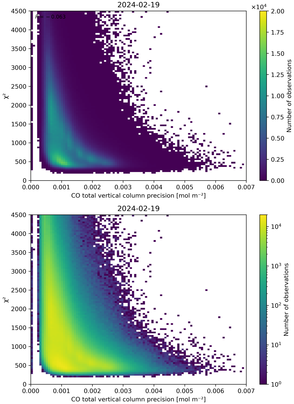
Figure 44: Scatter density plot of “CO total vertical column precision” against “ \chi^2 ” for 2024-02-18 to 2024-02-20.
