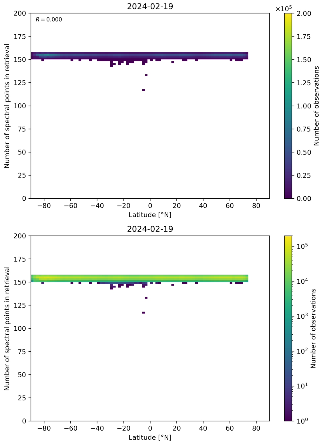
Figure 57: Scatter density plot of “Latitude” against “Number of spectral points in retrieval” for 2024-02-18 to 2024-02-20.
