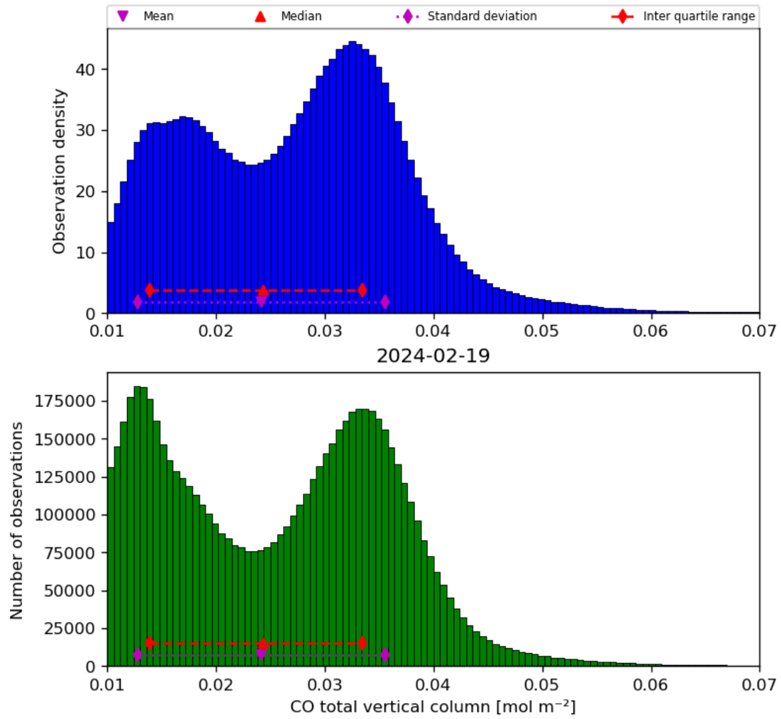
Figure 18: Histogram of “CO total vertical column” for 2024-02-18 to 2024-02-20
