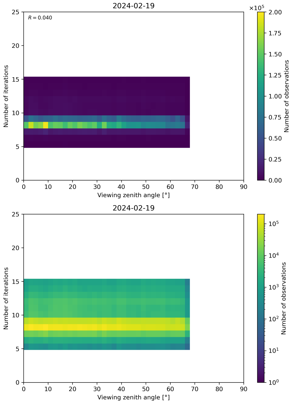
Figure 75: Scatter density plot of “Viewing zenith angle” against “Number of iterations” for 2024-02-18 to 2024-02-20.
