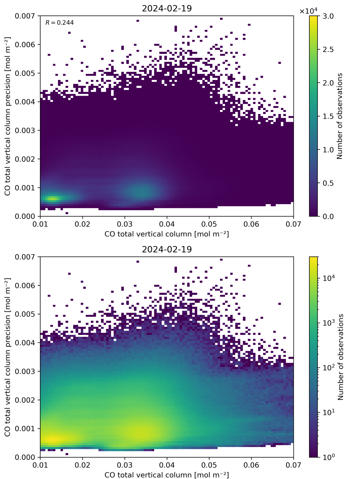
Figure 34: Scatter density plot of “CO total vertical column” against “CO total vertical column precision” for 2024-02-18 to 2024-02-20.
