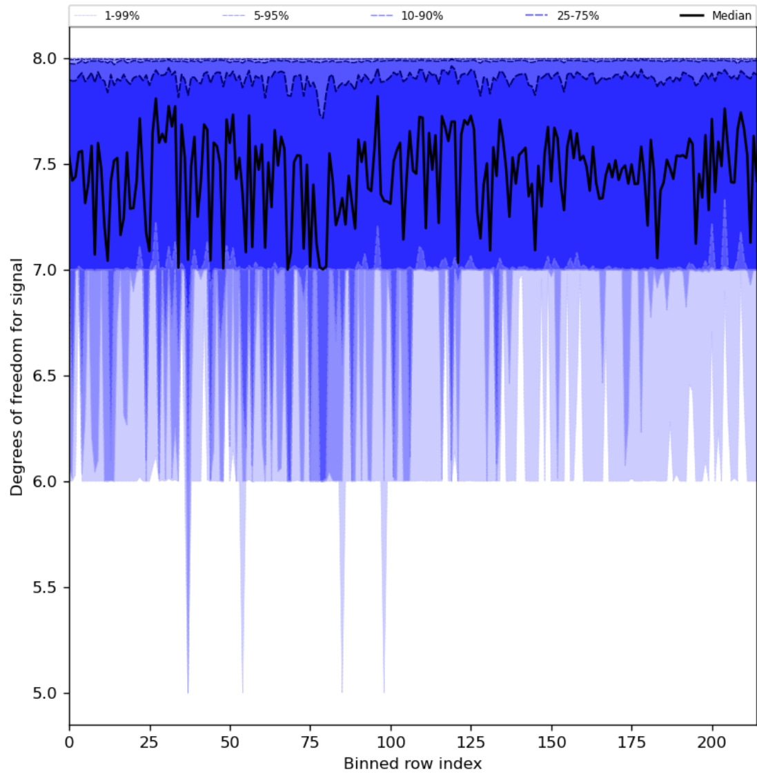
Figure 31: Along track statistics of “Degrees of freedom for signal” for 2024-02-18 to 2024-02-20
