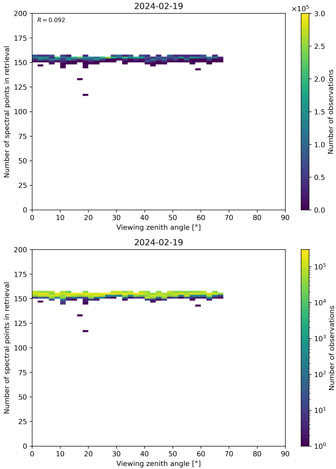
Figure 76: Scatter density plot of “Viewing zenith angle” against “Number of spectral points in retrieval” for 2024-02-18 to 2024-02-20.
