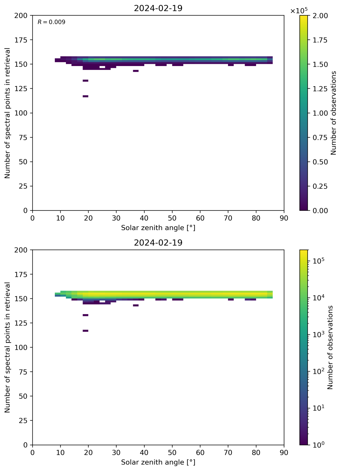
Figure 68: Scatter density plot of “Solar zenith angle” against “Number of spectral points in retrieval” for 2024-02-18 to 2024-02-20.
