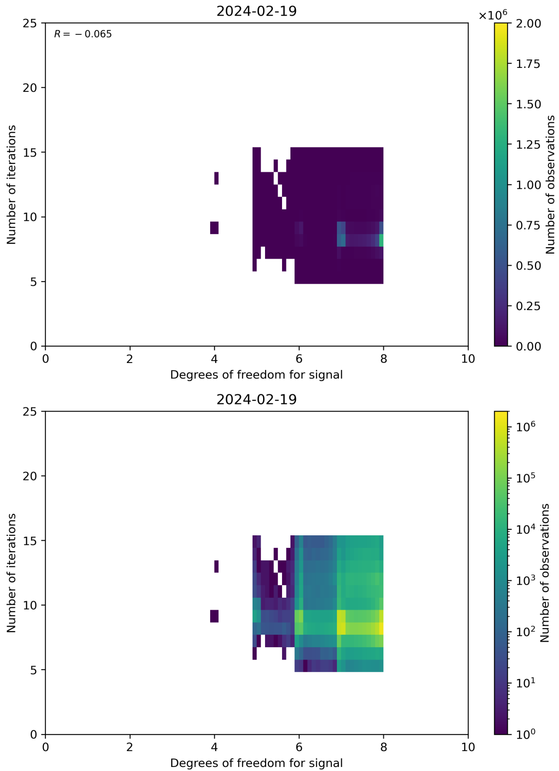
Figure 50: Scatter density plot of “Degrees of freedom for signal” against “Number of iterations” for 2024-02-18 to 2024-02-20.
