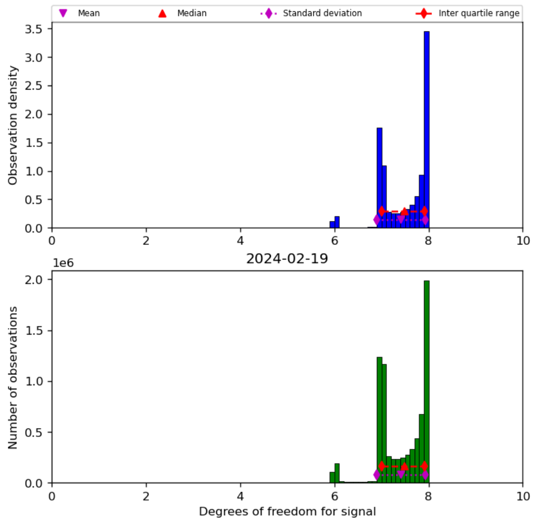
Figure 23: Histogram of “Degrees of freedom for signal” for 2024-02-18 to 2024-02-20
