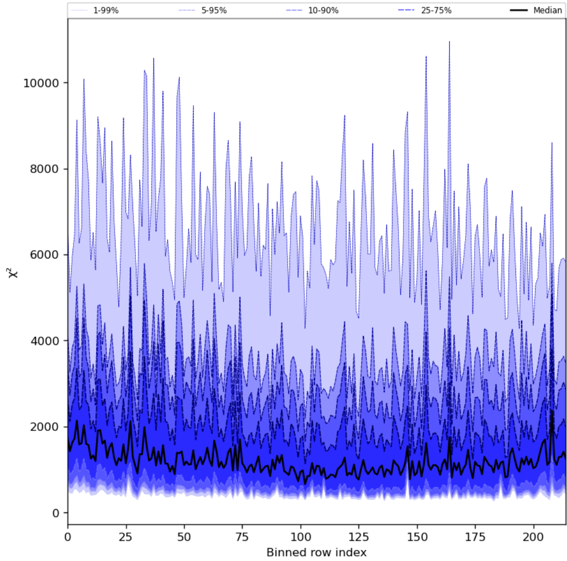
Figure 30: Along track statistics of “ \chi^2 ” for 2024-02-18 to 2024-02-20
