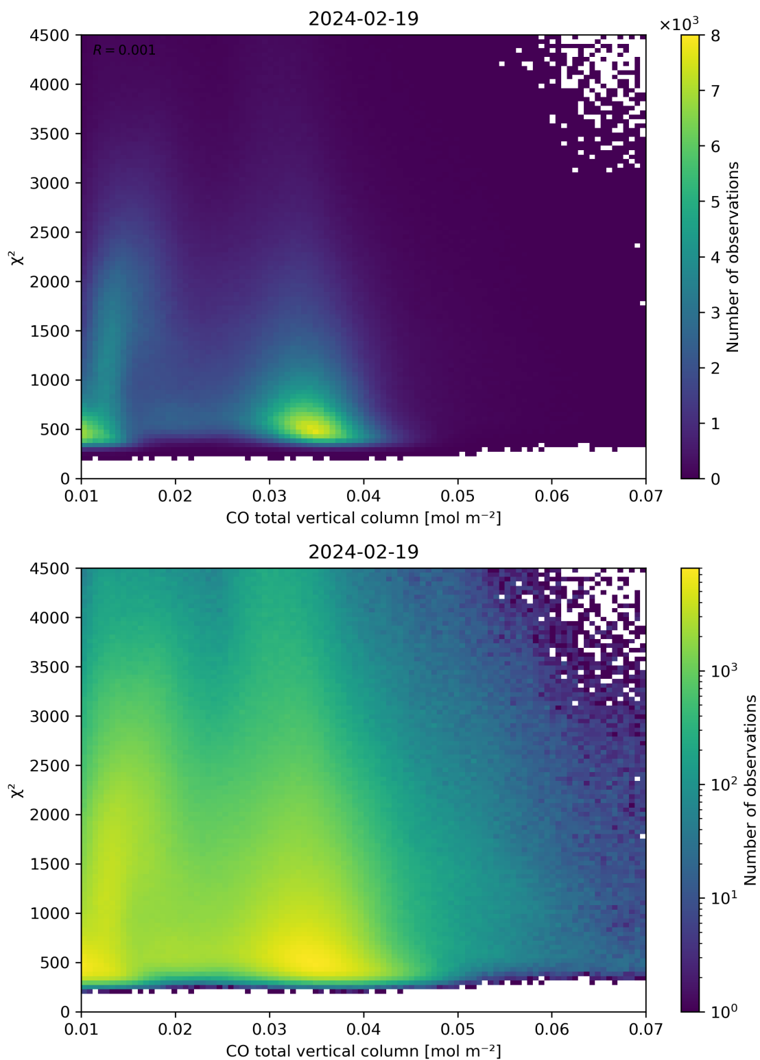
Figure 35: Scatter density plot of “CO total vertical column” against “ \chi^2 ” for 2024-02-18 to 2024-02-20.
