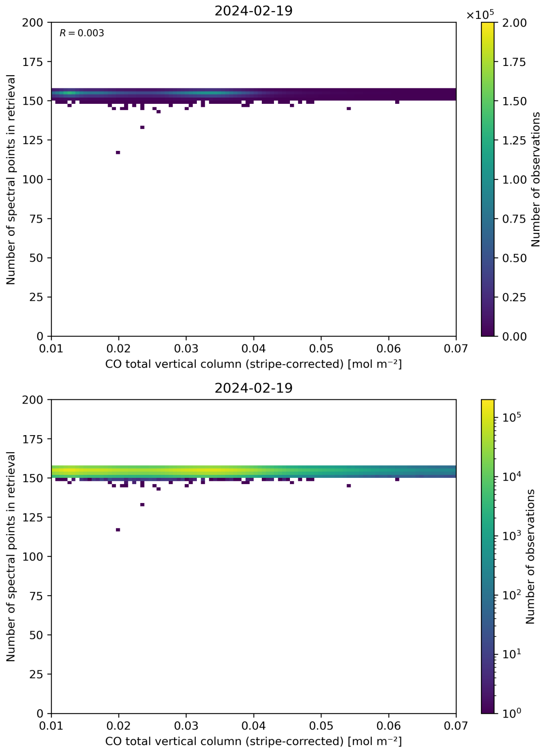
Figure 40: Scatter density plot of “CO total vertical column (stripe-corrected)” against “Number of spectral points in retrieval” for 2024-02-18 to 2024-02-20.
