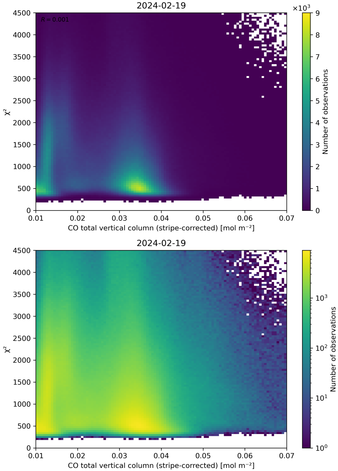
Figure 37: Scatter density plot of “CO total vertical column (stripe-corrected)” against “ \chi^2 ” for 2024-02-18 to 2024-02-20.
