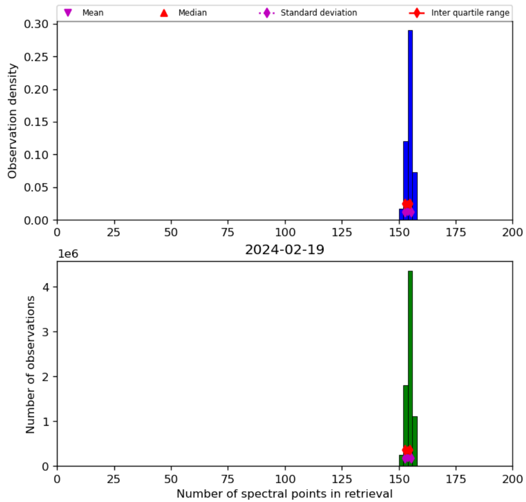
Figure 21: Histogram of “Number of spectral points in retrieval” for 2024-02-18 to 2024-02-20
