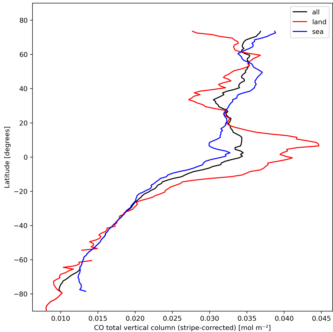
Figure 11: Zonal average of “CO total vertical column (stripe-corrected)” for 2024-02-18 to 2024-02-20.
