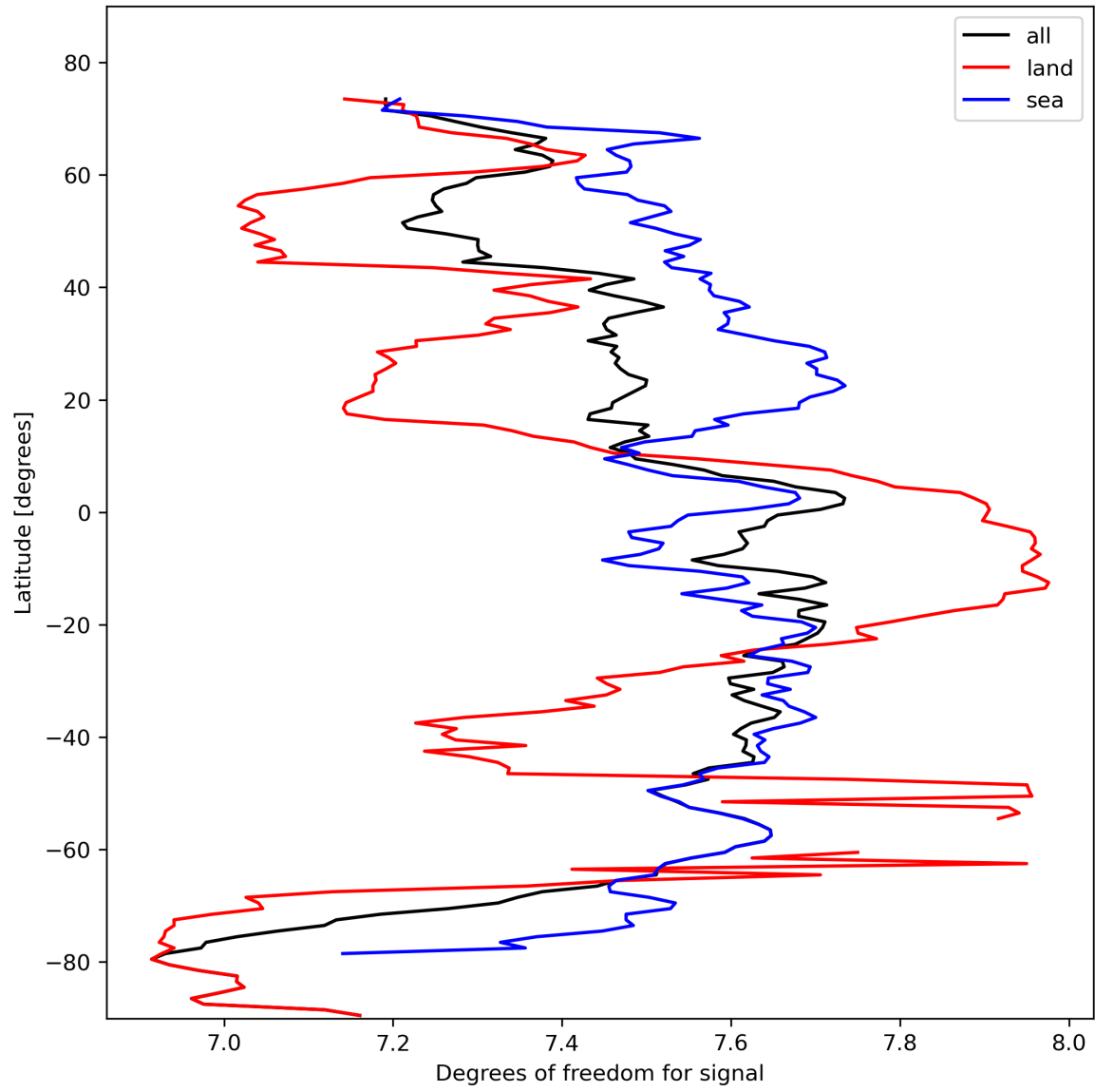
Figure 15: Zonal average of “Degrees of freedom for signal” for 2024-02-18 to 2024-02-20.
