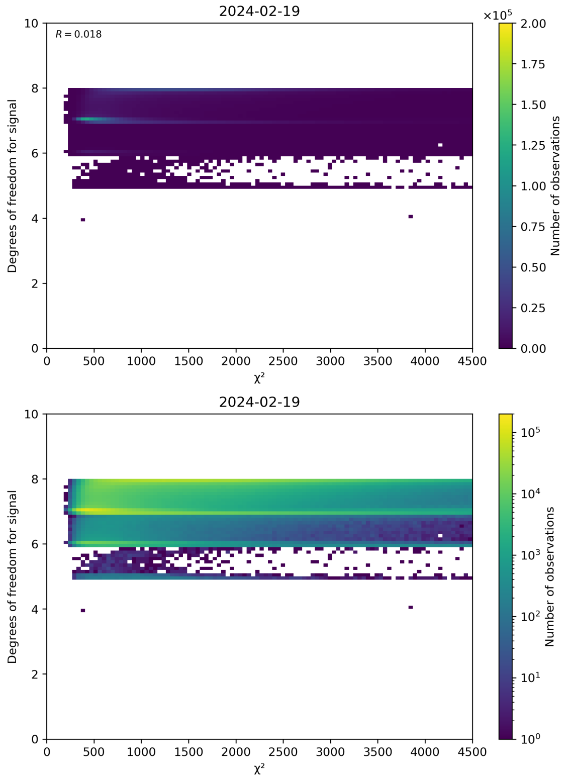
Figure 48: Scatter density plot of “ \chi^2 ” against “Degrees of freedom for signal” for 2024-02-18 to 2024-02-20.
