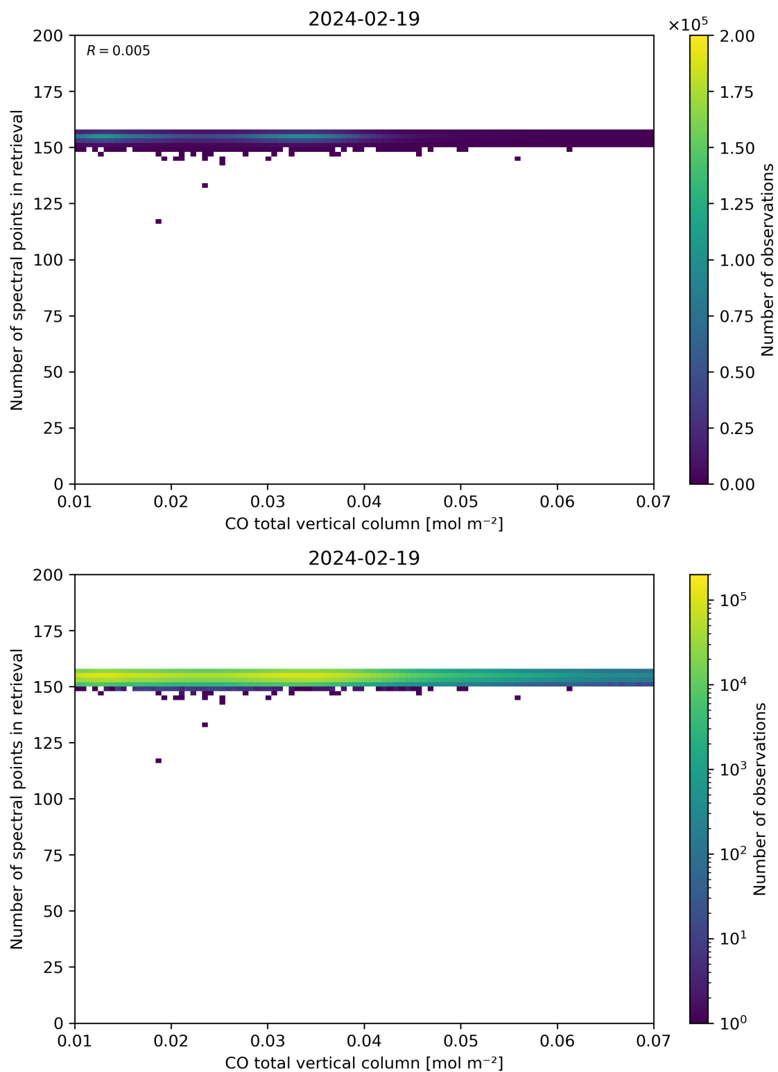
Figure 43: Scatter density plot of “CO total vertical column” against “Number of spectral points in retrieval” for 2024-02-18 to 2024-02-20.
