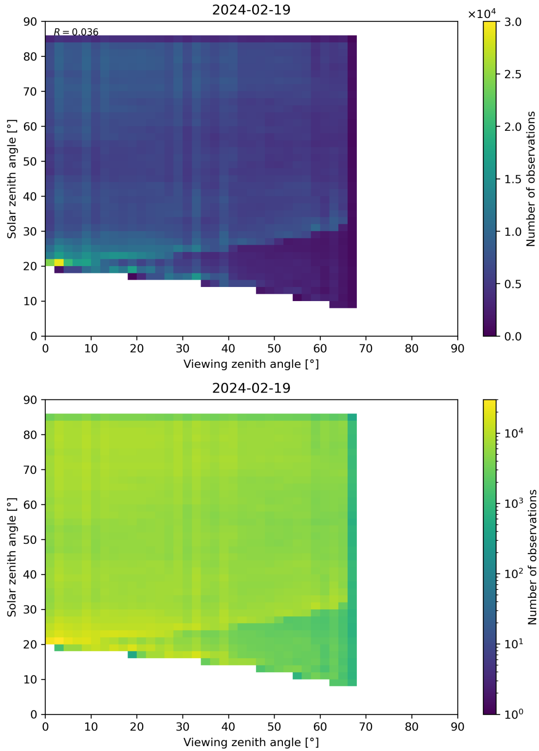
Figure 77: Scatter density plot of “Viewing zenith angle” against “Solar zenith angle” for 2024-02-18 to 2024-02-20.
