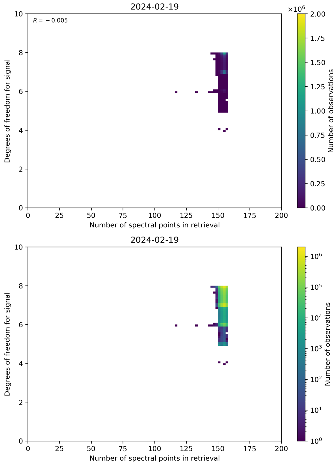
Figure 59: Scatter density plot of “Number of spectral points in retrieval” against “Degrees of freedom for signal” for 2024-02-18 to 2024-02-20.
