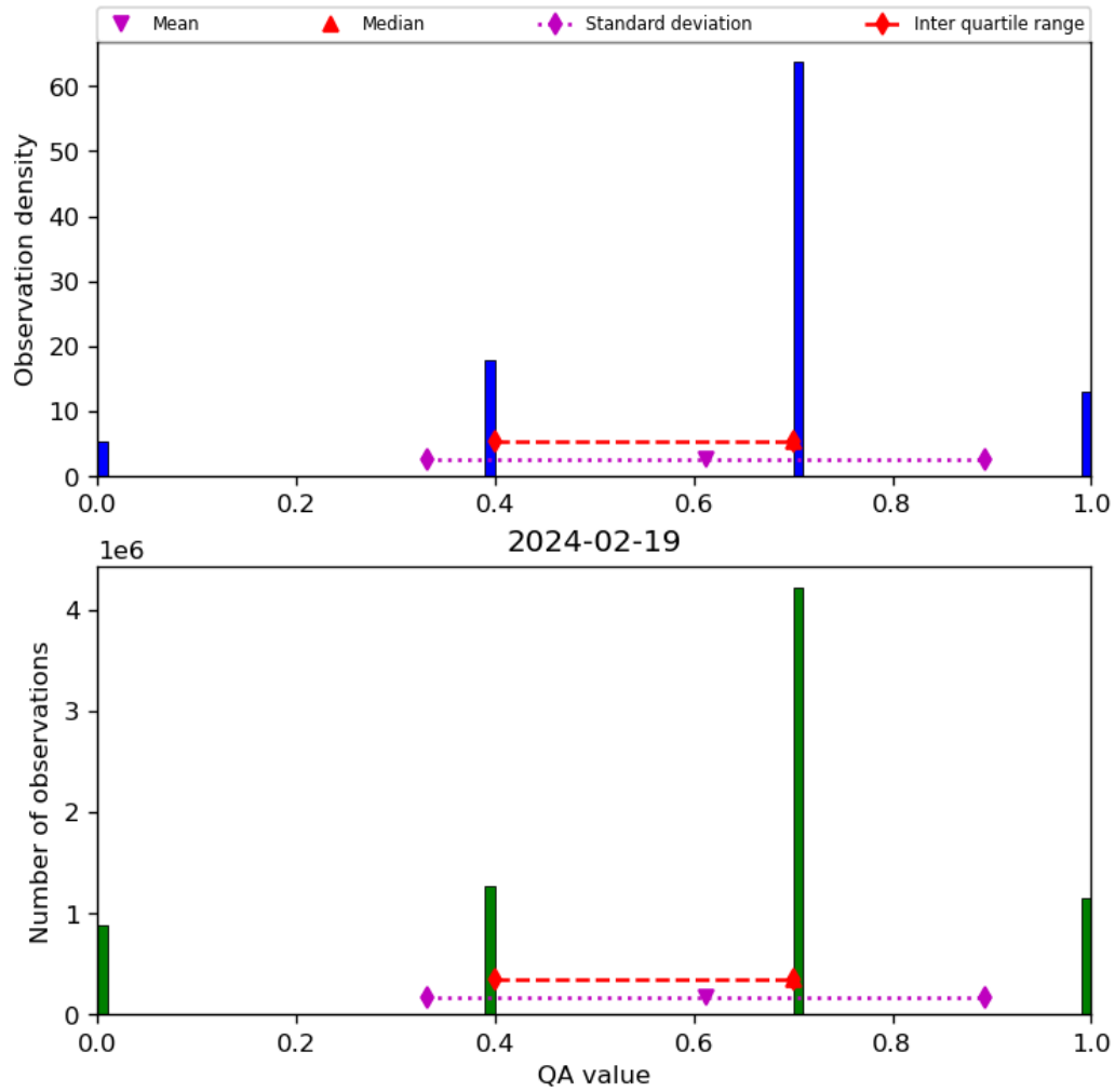
Figure 17: Histogram of “QA value” for 2024-02-18 to 2024-02-20
