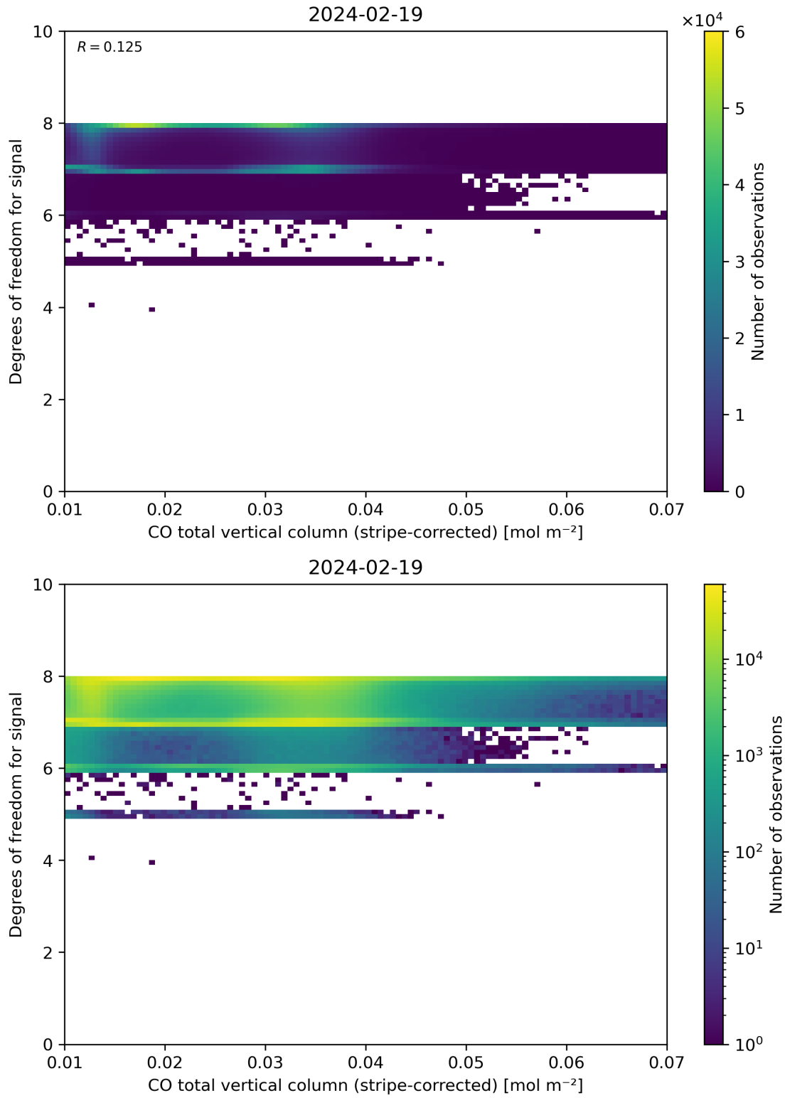
Figure 38: Scatter density plot of “CO total vertical column (stripe-corrected)” against “Degrees of freedom for signal” for 2024-02-18 to 2024-02-20.
