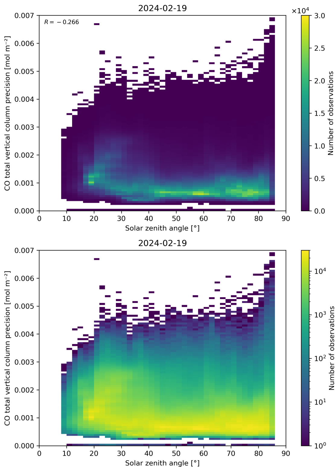
Figure 63: Scatter density plot of “Solar zenith angle” against “CO total vertical column precision” for 2024-02-18 to 2024-02-20.
