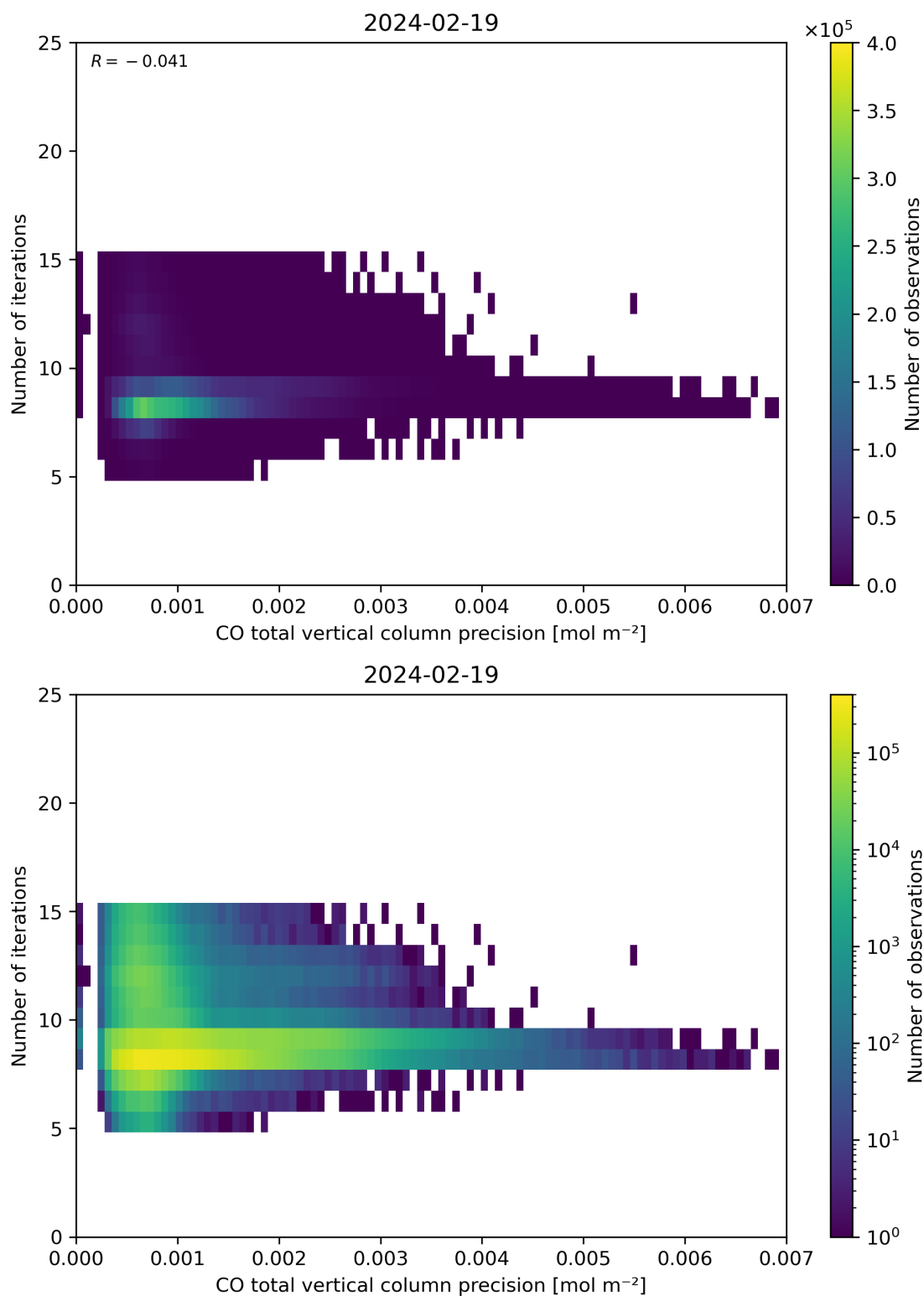
Figure 46: Scatter density plot of “CO total vertical column precision” against “Number of iterations” for 2024-02-18 to 2024-02-20.
