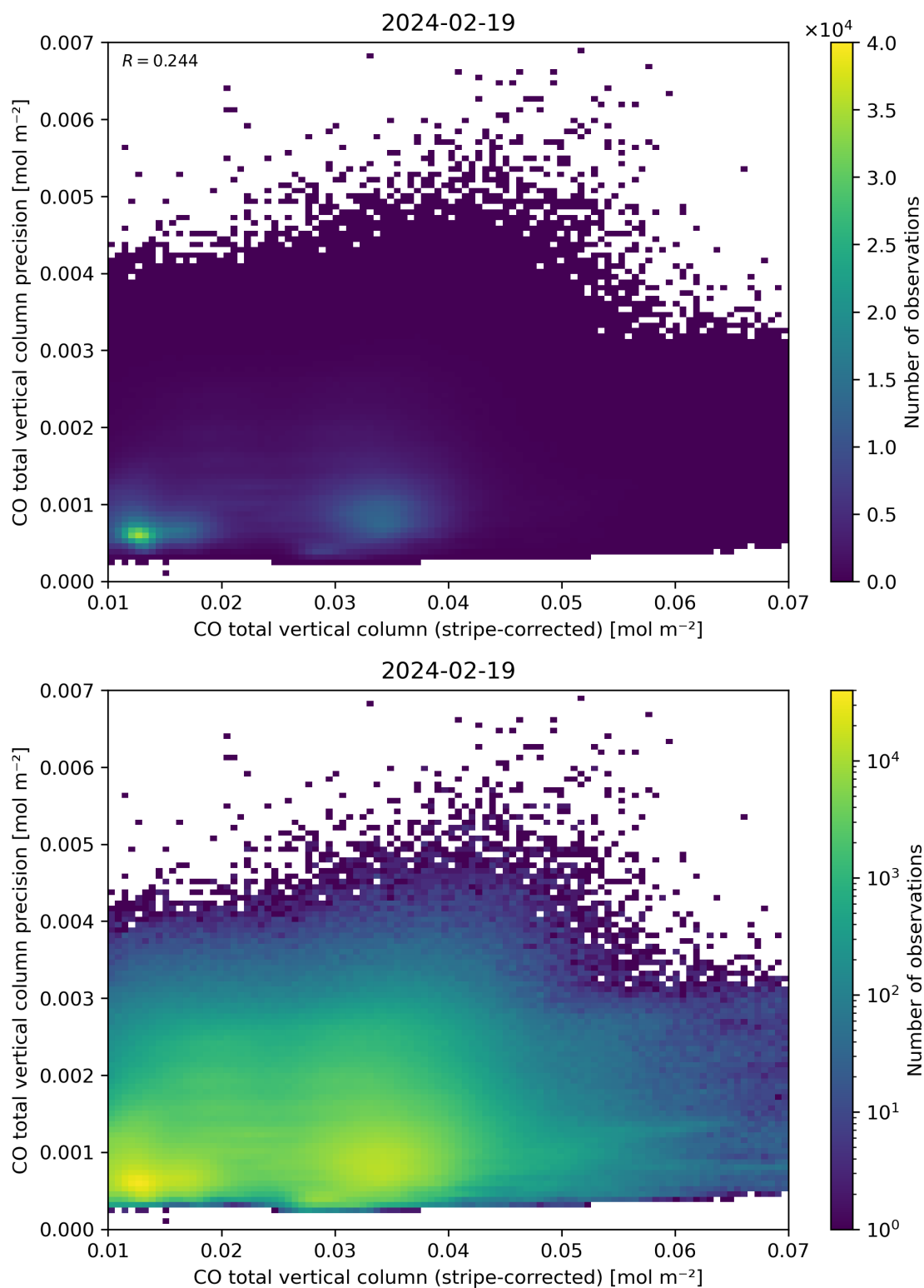
Figure 36: Scatter density plot of “CO total vertical column (stripe-corrected)” against “CO total vertical column precision” for 2024-02-18 to 2024-02-20.
