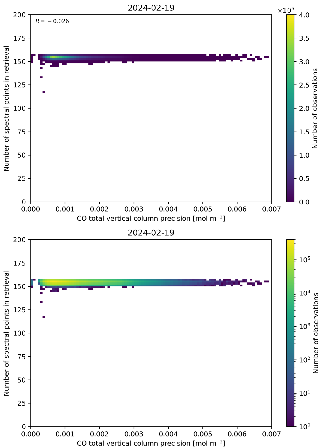
Figure 47: Scatter density plot of “CO total vertical column precision” against “Number of spectral points in retrieval” for 2024-02-18 to 2024-02-20.
