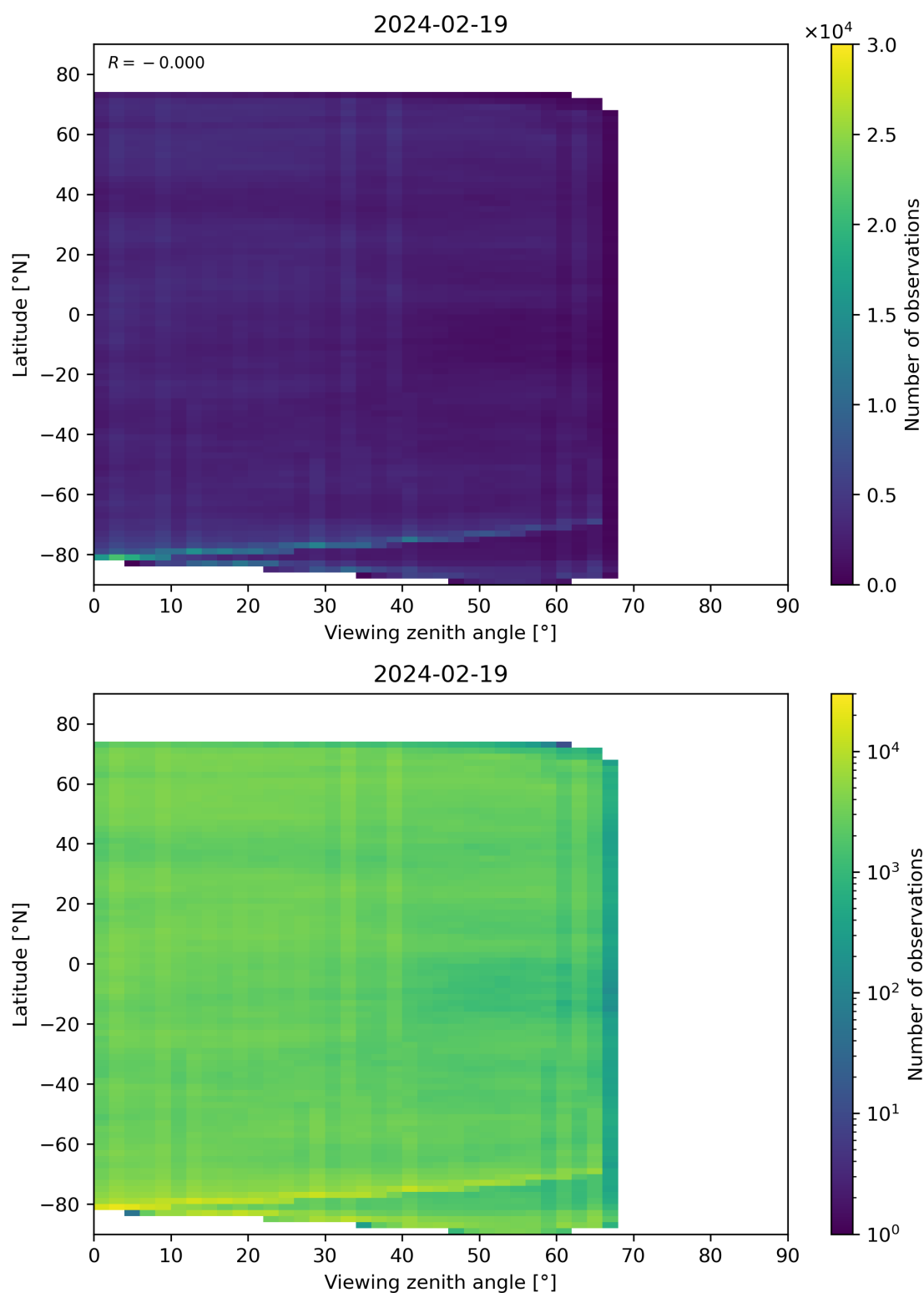
Figure 74: Scatter density plot of “Viewing zenith angle” against “Latitude” for 2024-02-18 to 2024-02-20.
