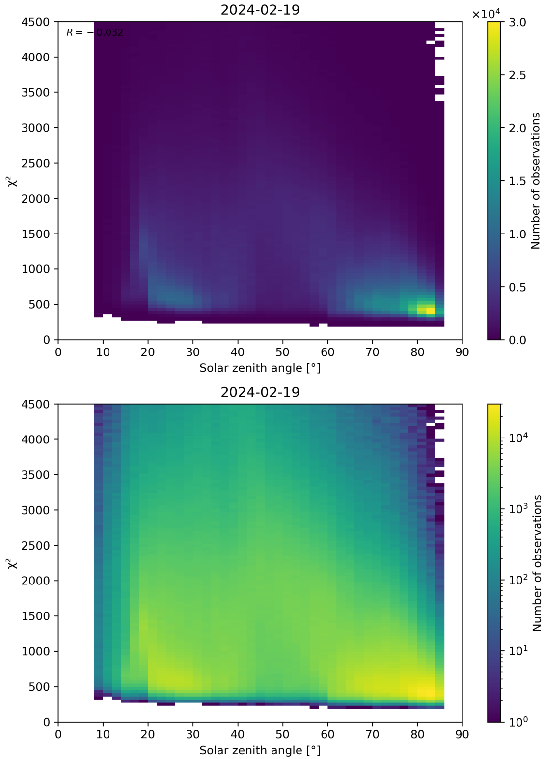
Figure 64: Scatter density plot of “Solar zenith angle” against “ \chi^2 ” for 2024-02-18 to 2024-02-20.
