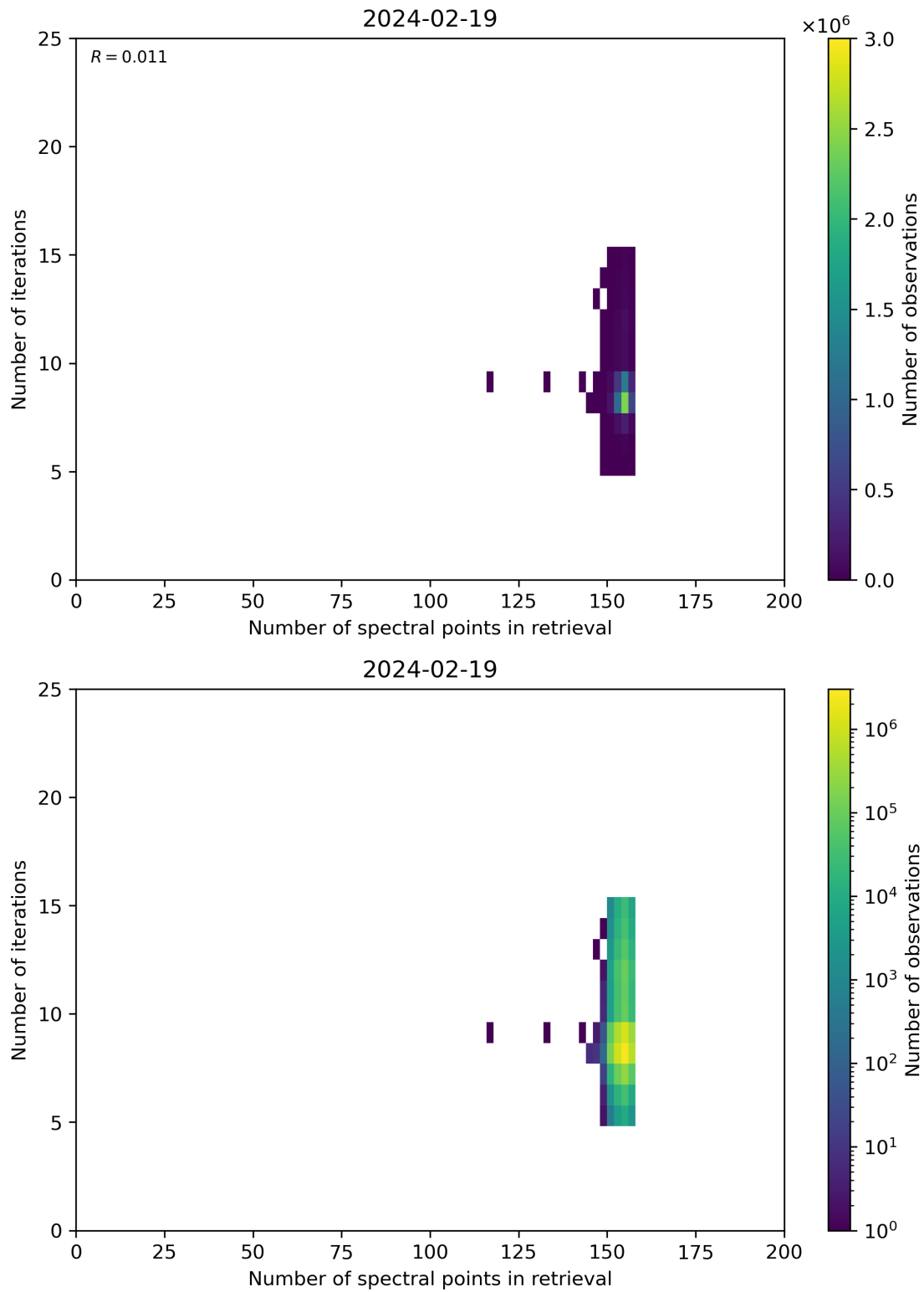
Figure 60: Scatter density plot of “Number of spectral points in retrieval” against “Number of iterations” for 2024-02-18 to 2024-02-20.
