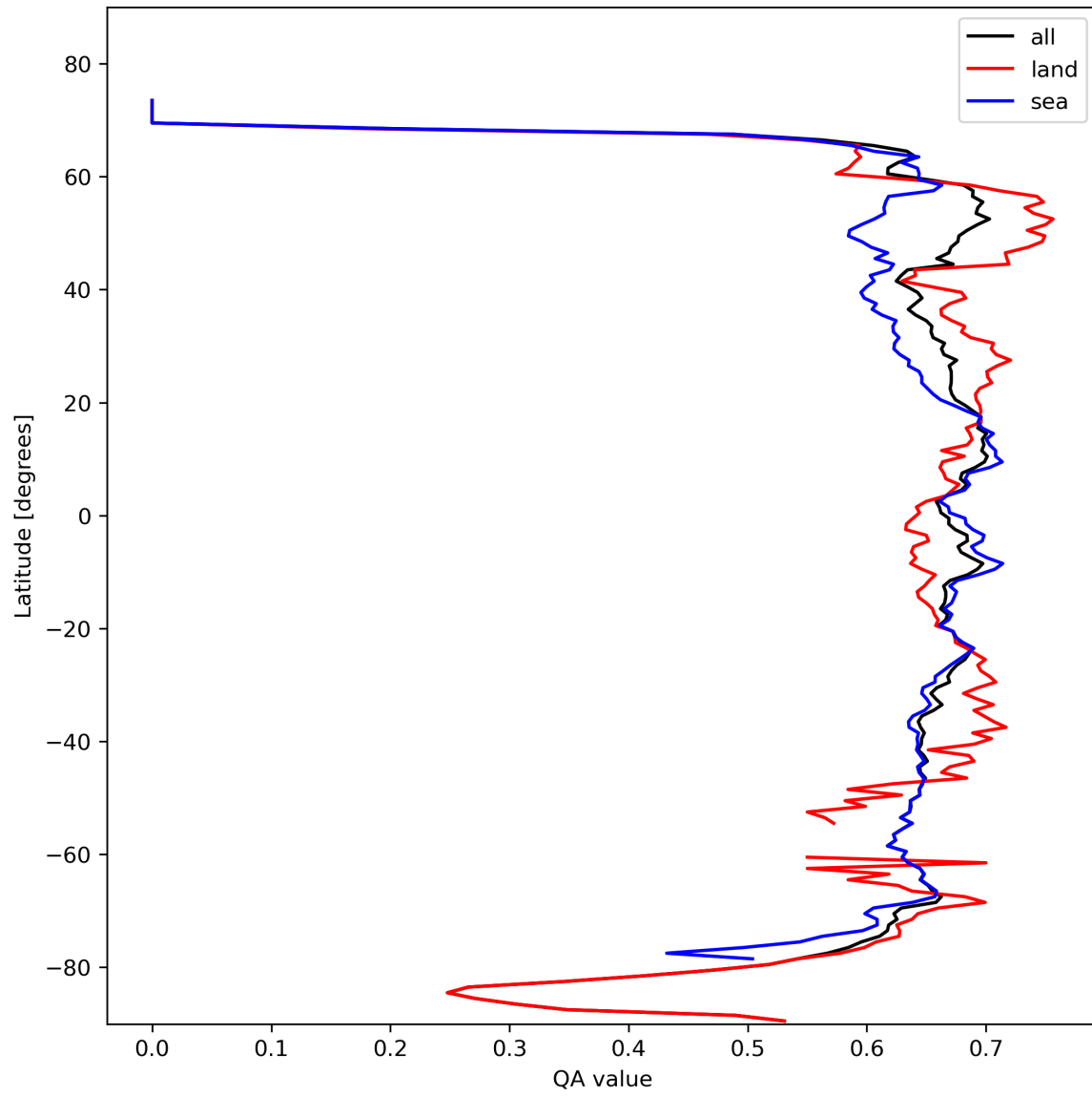
Figure 9: Zonal average of “QA value” for 2024-02-18 to 2024-02-20.
