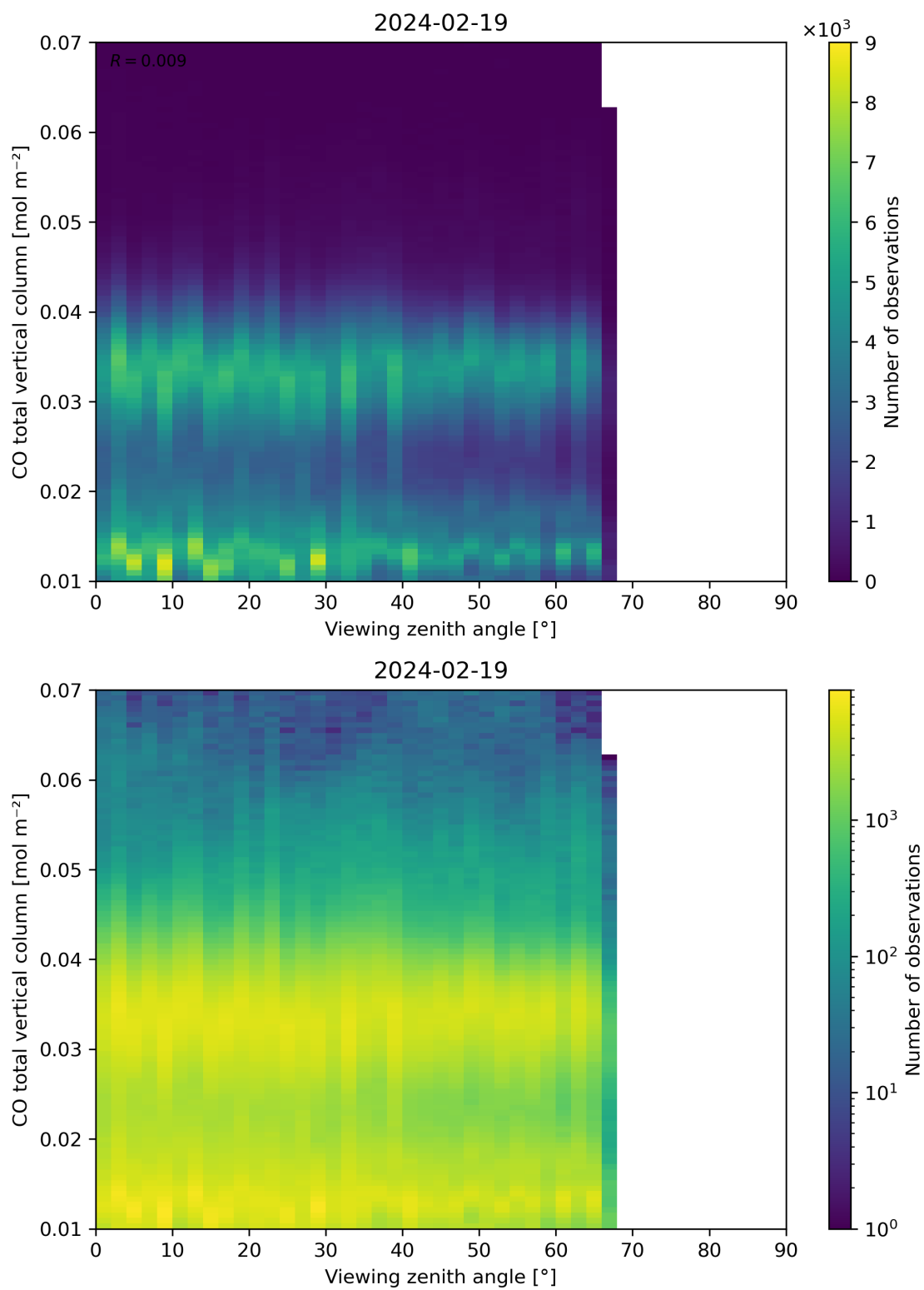
Figure 69: Scatter density plot of “Viewing zenith angle” against “CO total vertical column” for 2024-02-18 to 2024-02-20.
