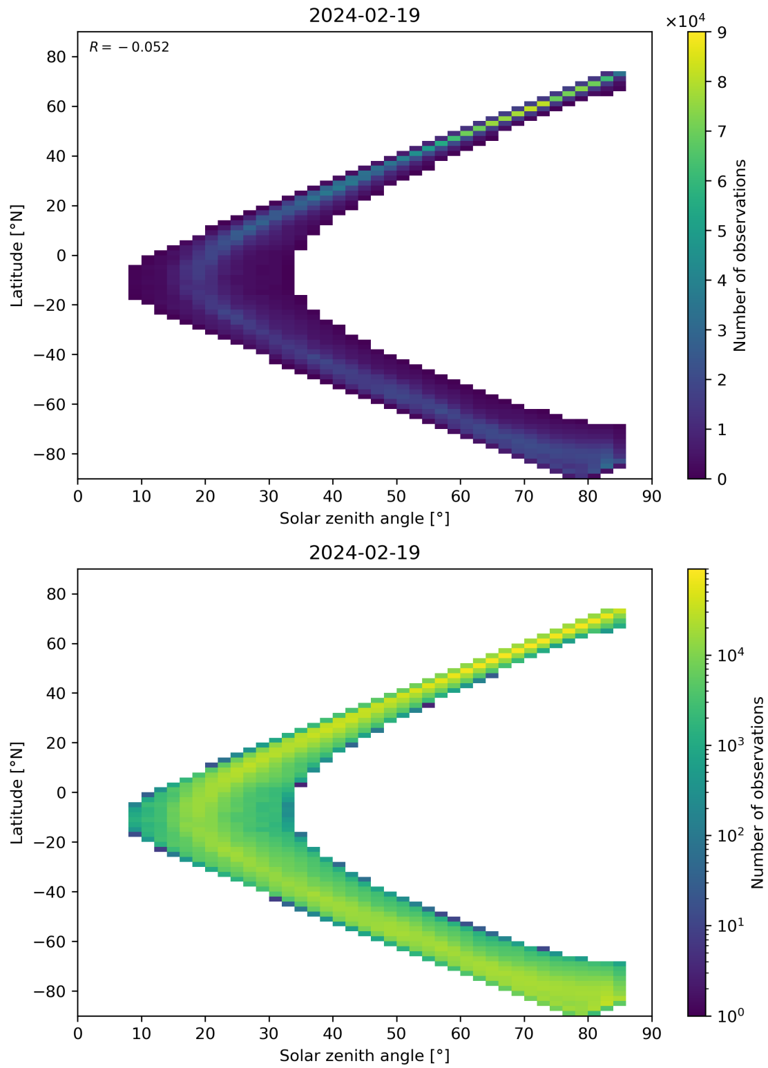
Figure 66: Scatter density plot of “Solar zenith angle” against “Latitude” for 2024-02-18 to 2024-02-20.
