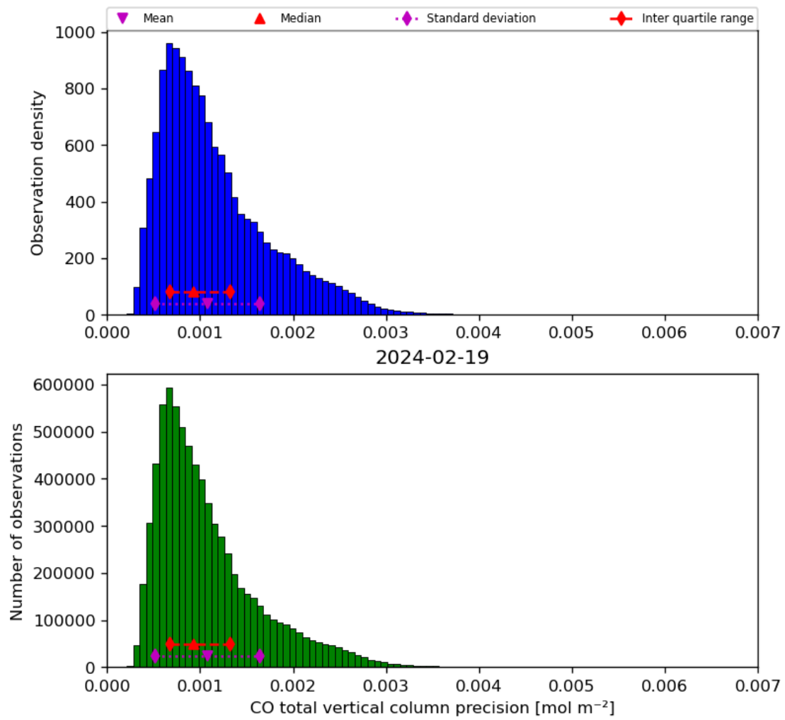
Figure 20: Histogram of “CO total vertical column precision” for 2024-02-18 to 2024-02-20
