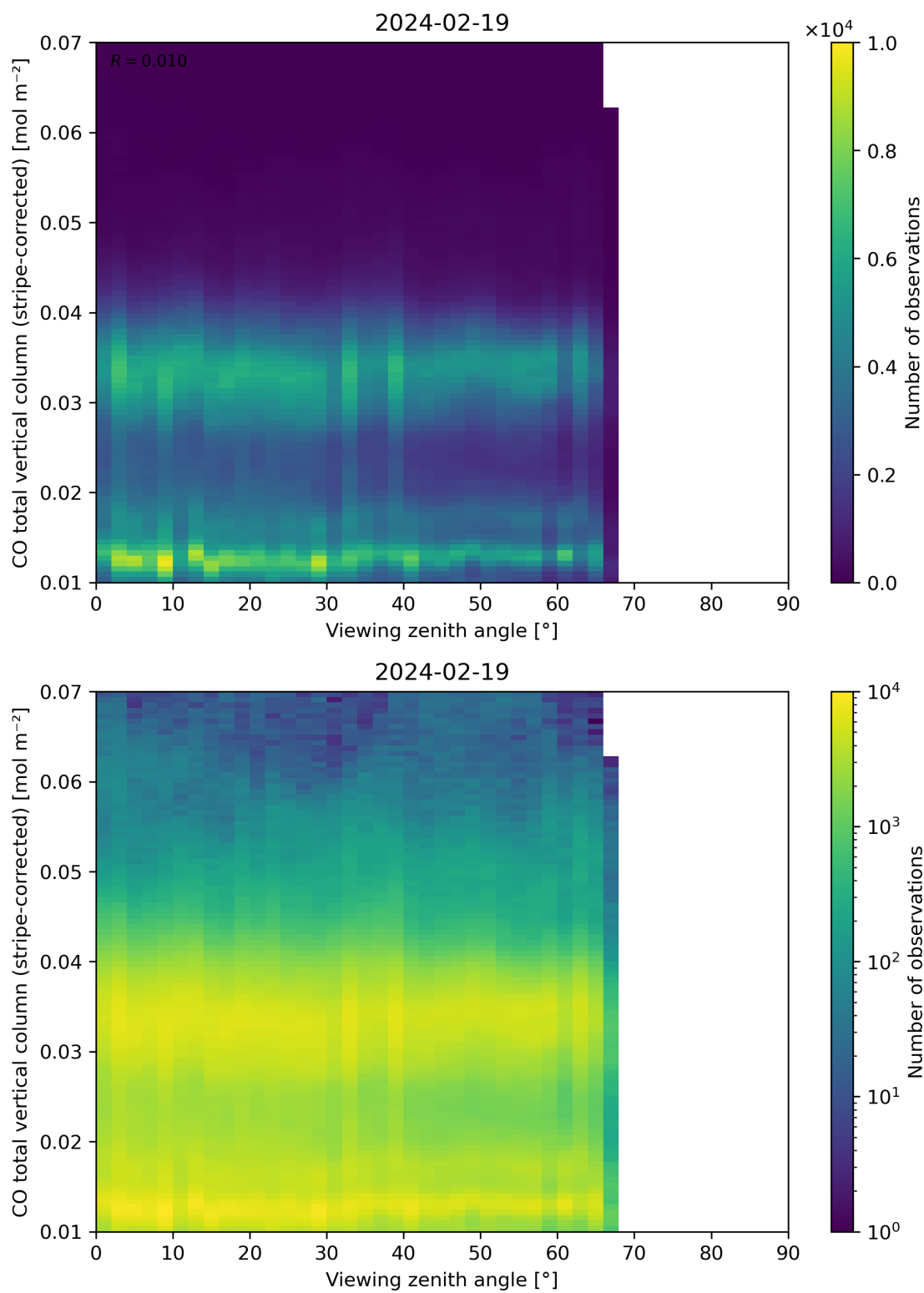
Figure 70: Scatter density plot of “Viewing zenith angle” against “CO total vertical column (stripe-corrected)” for 2024-02-18 to 2024-02-20.
