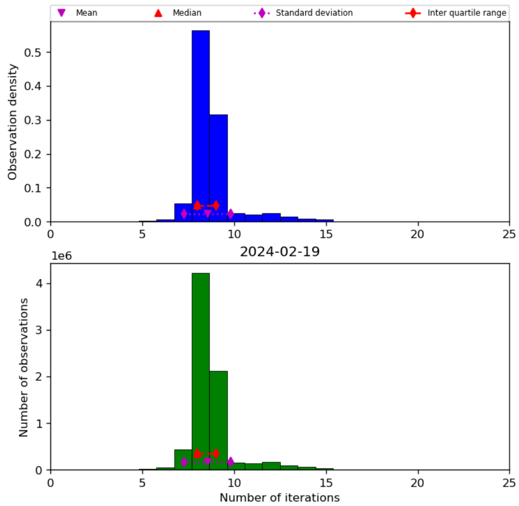
Figure 24: Histogram of "Number of iterations" for 2024-02-18 to 2024-02-20
