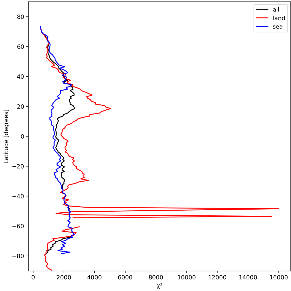
Figure 14: Zonal average of “ \chi^2 ” for 2024-02-18 to 2024-02-20.
