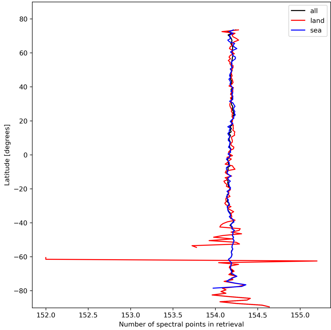
Figure 13: Zonal average of “Number of spectral points in retrieval” for 2024-02-18 to 2024-02-20.
