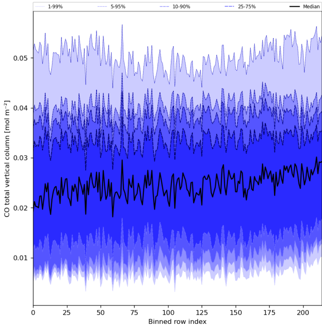
Figure 26: Along track statistics of “CO total vertical column” for 2024-02-18 to 2024-02-20
