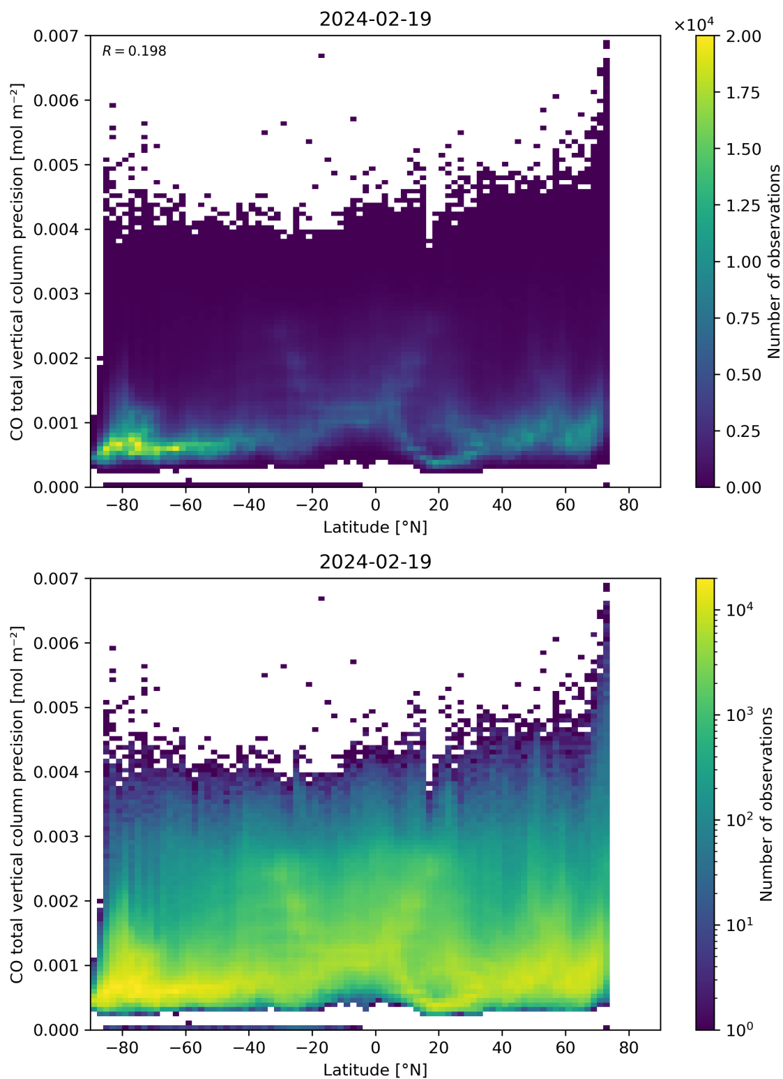
Figure 53: Scatter density plot of “Latitude” against “CO total vertical column precision” for 2024-02-18 to 2024-02-20.
