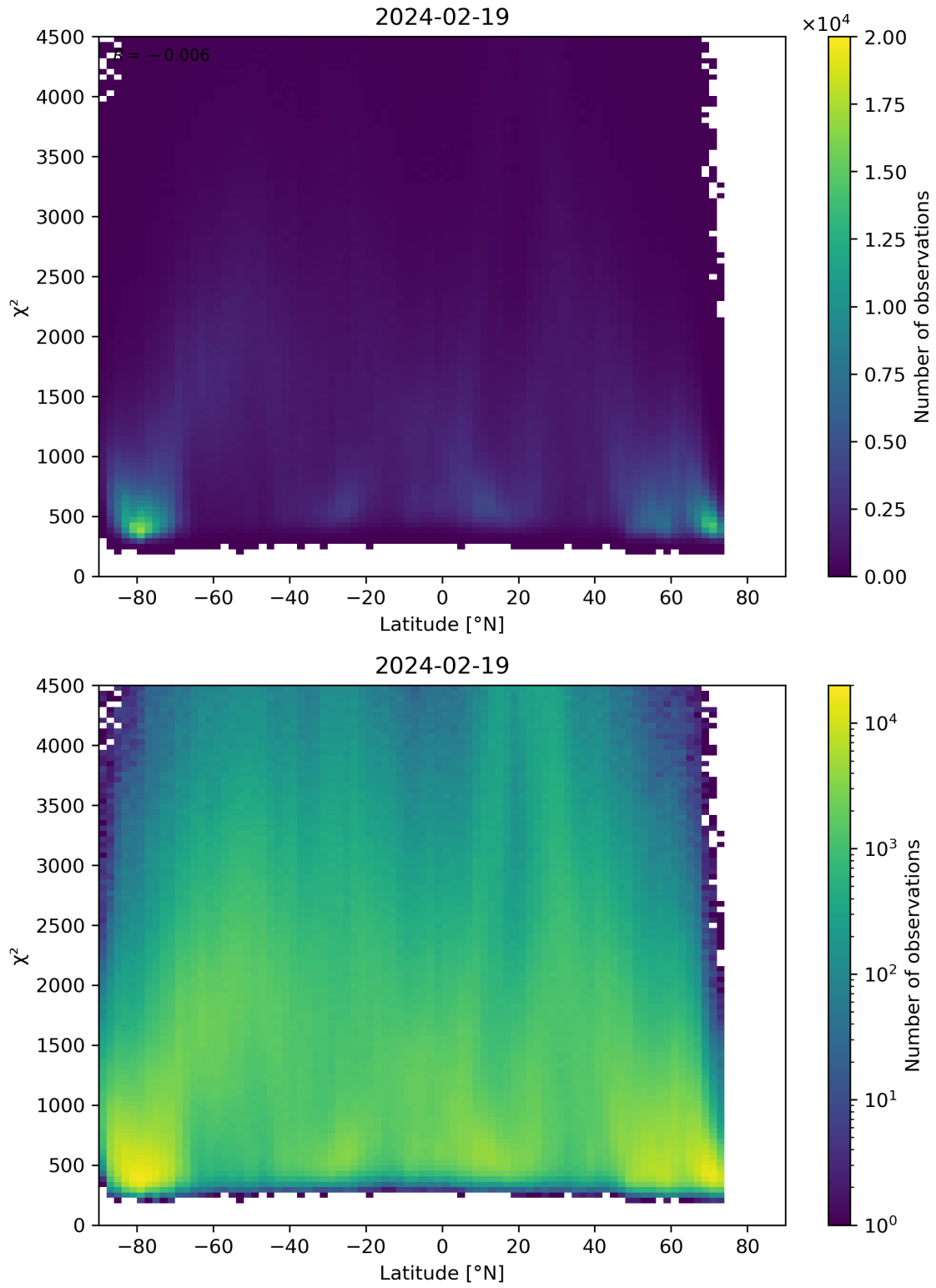
Figure 54: Scatter density plot of “Latitude” against “ \chi^2 ” for 2024-02-18 to 2024-02-20.
