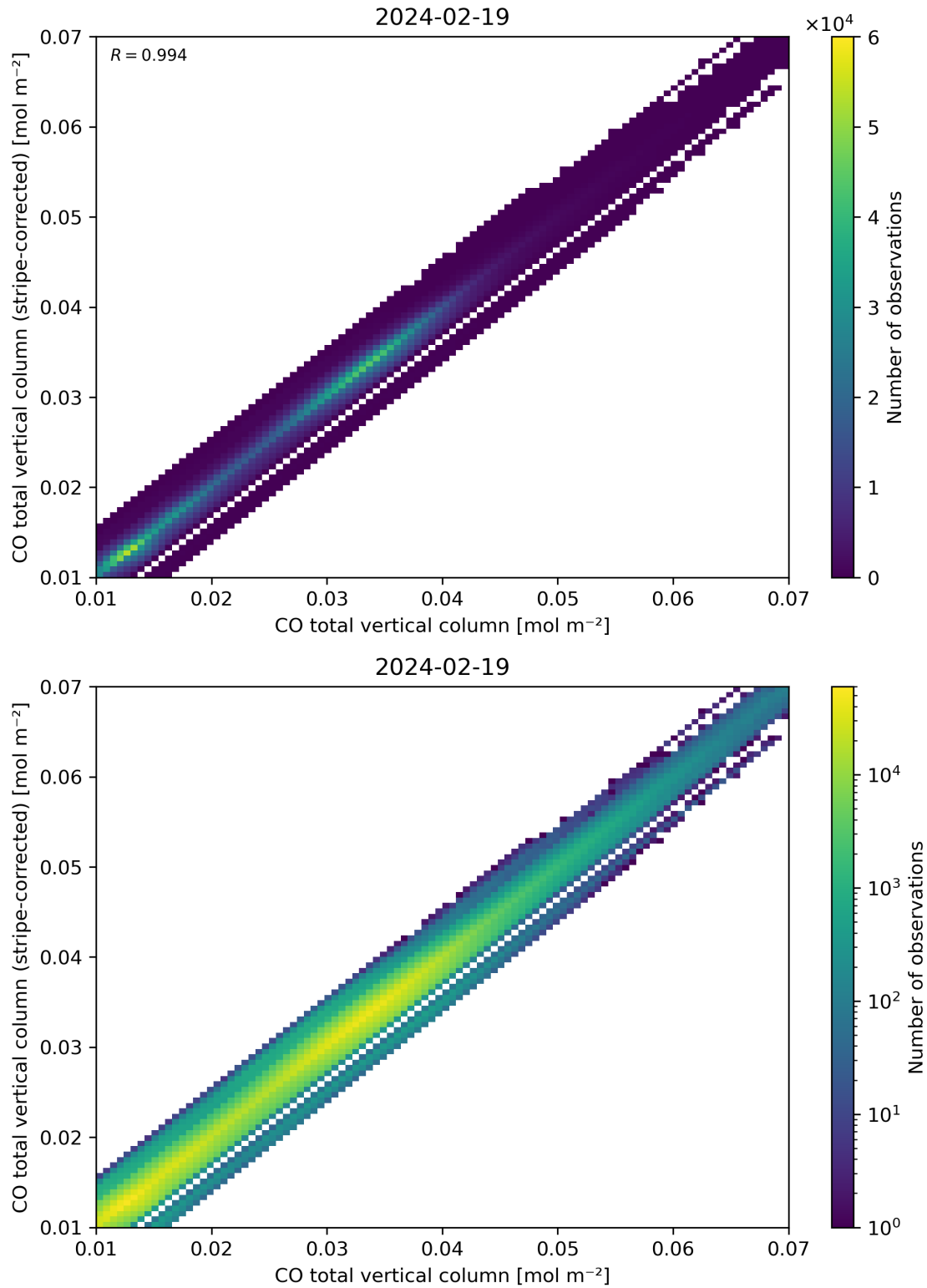
Figure 33: Scatter density plot of “CO total vertical column” against “CO total vertical column (stripe-corrected)” for 2024-02-18 to 2024-02-20.
