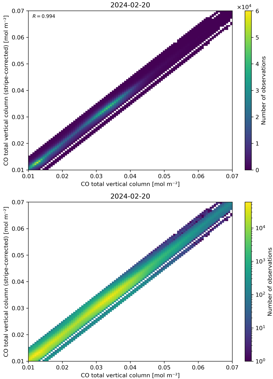
Figure 33: Scatter density plot of “CO total vertical column” against “CO total vertical column (stripe-corrected)” for 2024-02-19 to 2024-02-21.
