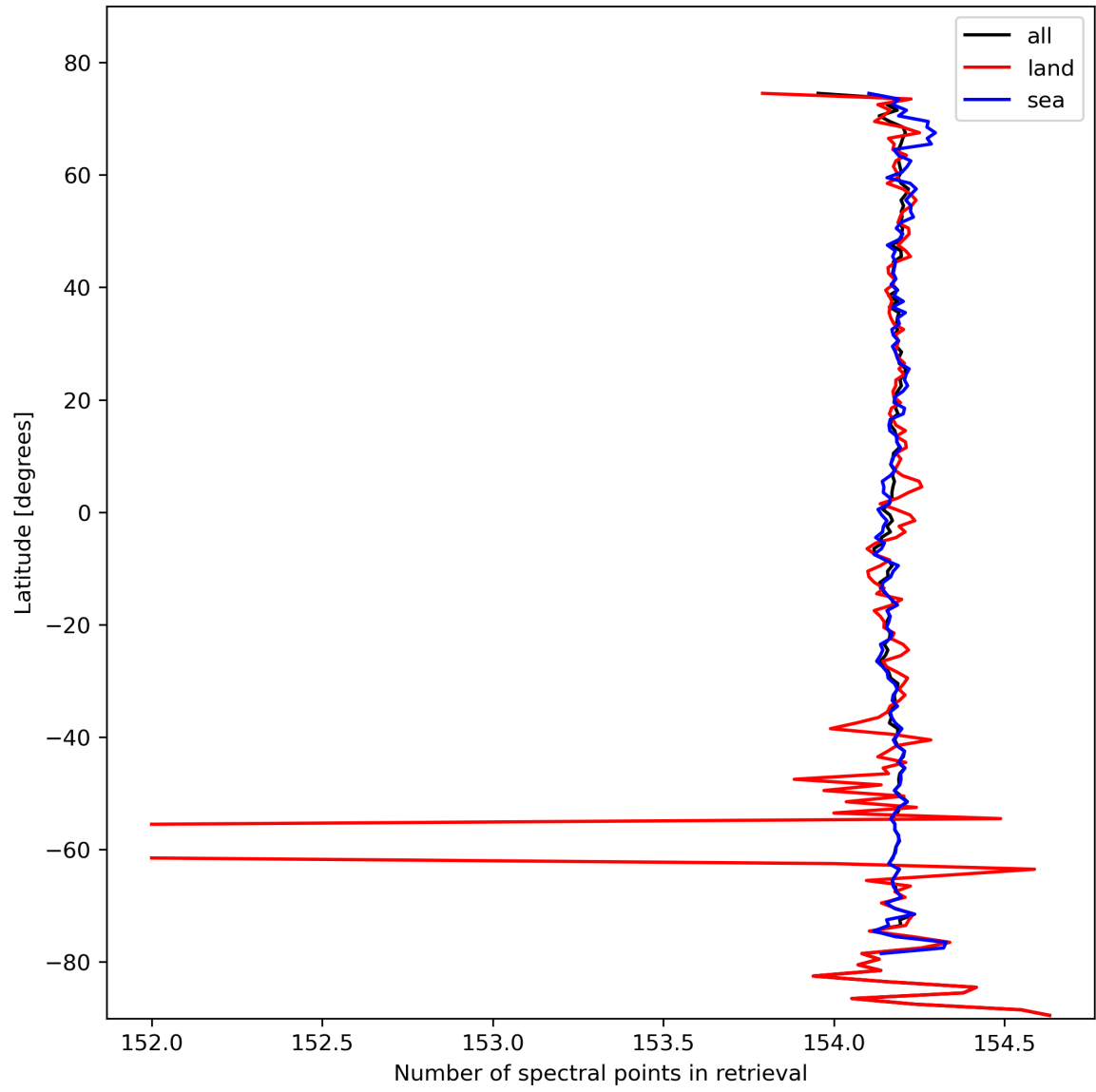
Figure 13: Zonal average of “Number of spectral points in retrieval” for 2024-02-19 to 2024-02-21.
