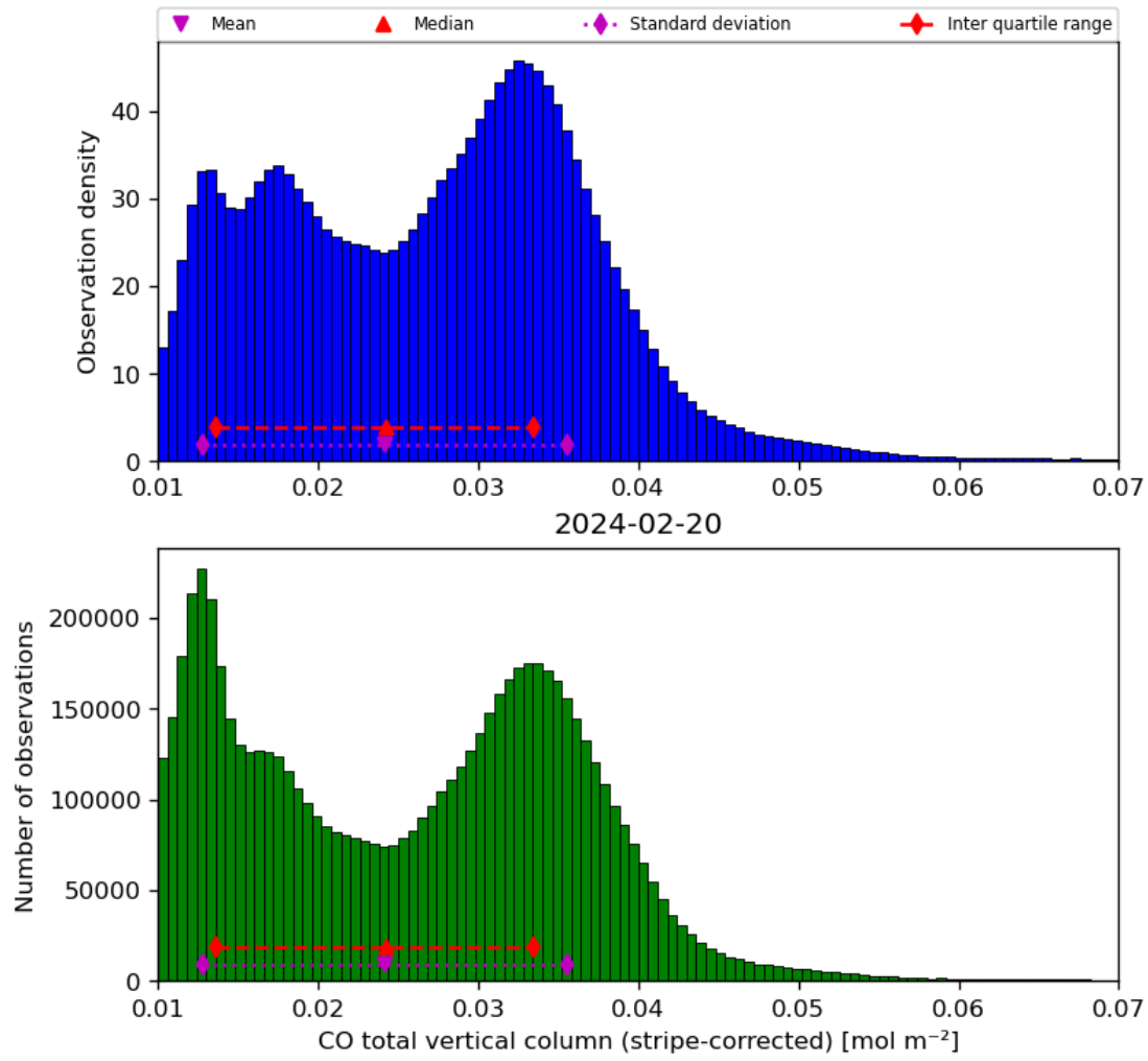
Figure 19: Histogram of “CO total vertical column (stripe-corrected)” for 2024-02-19 to 2024-02-21
