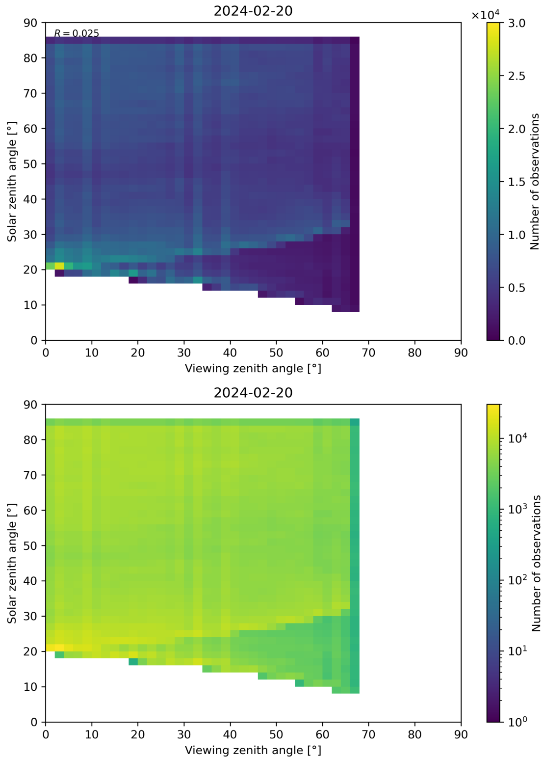
Figure 77: Scatter density plot of “Viewing zenith angle” against “Solar zenith angle” for 2024-02-19 to 2024-02-21.
