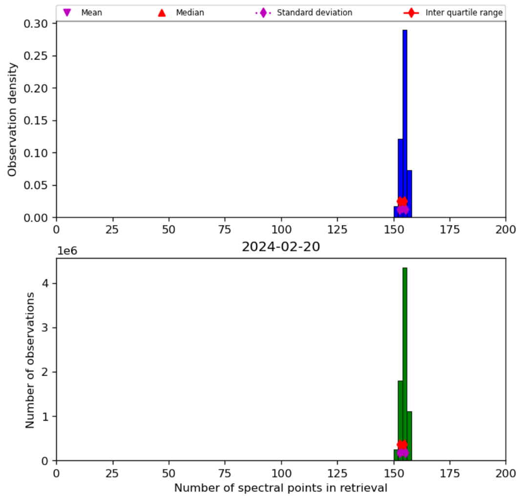
Figure 21: Histogram of “Number of spectral points in retrieval” for 2024-02-19 to 2024-02-21
