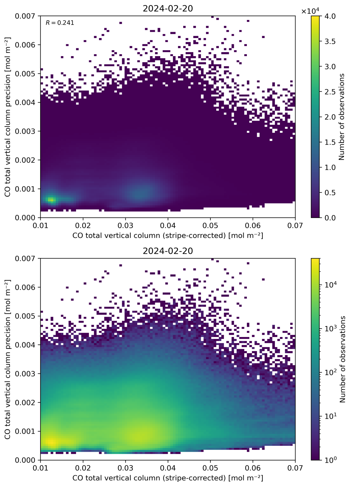
Figure 36: Scatter density plot of “CO total vertical column (stripe-corrected)” against “CO total vertical column precision” for 2024-02-19 to 2024-02-21.
