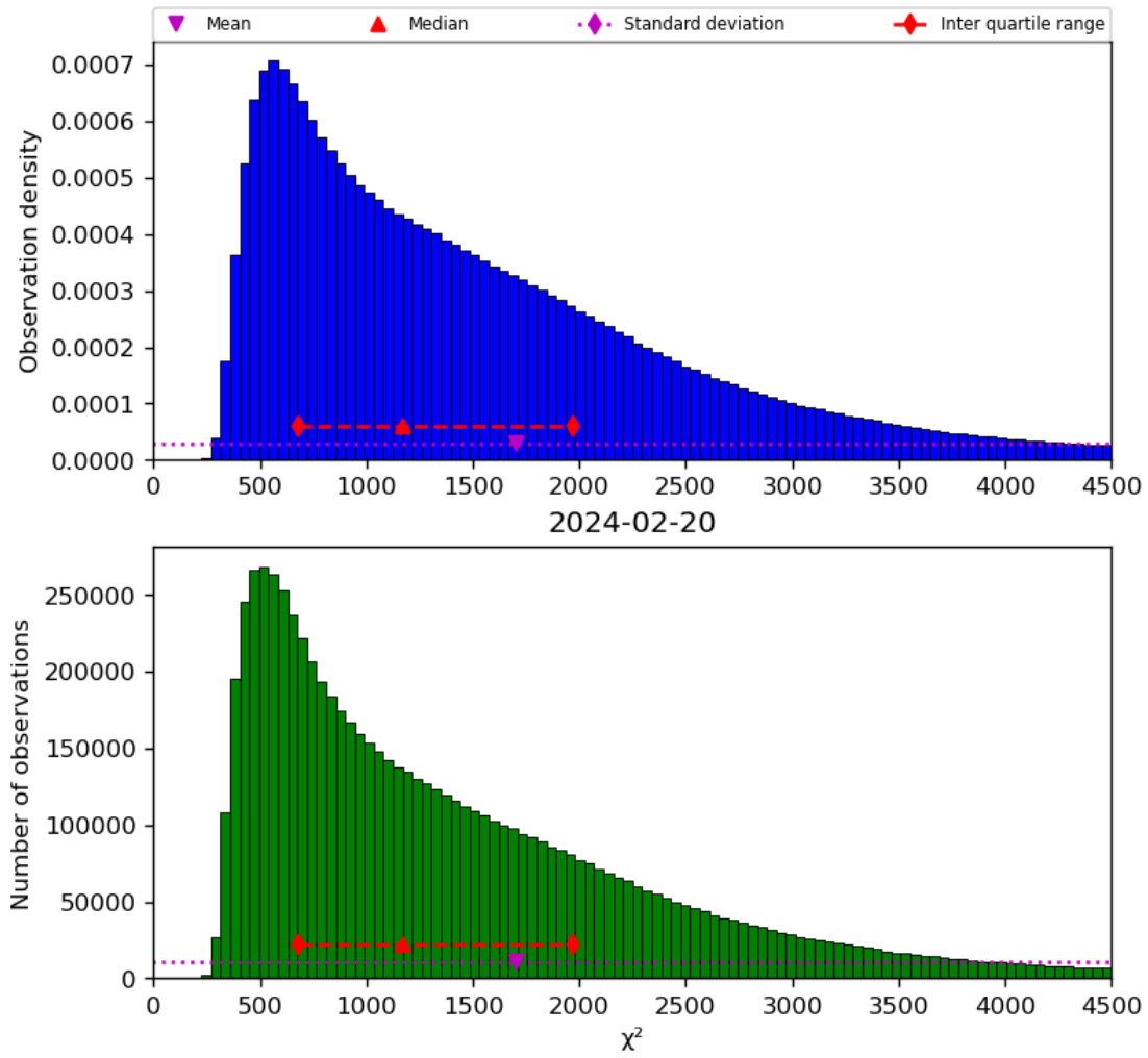
Figure 22: Histogram of “ \chi^2 ” for 2024-02-19 to 2024-02-21
