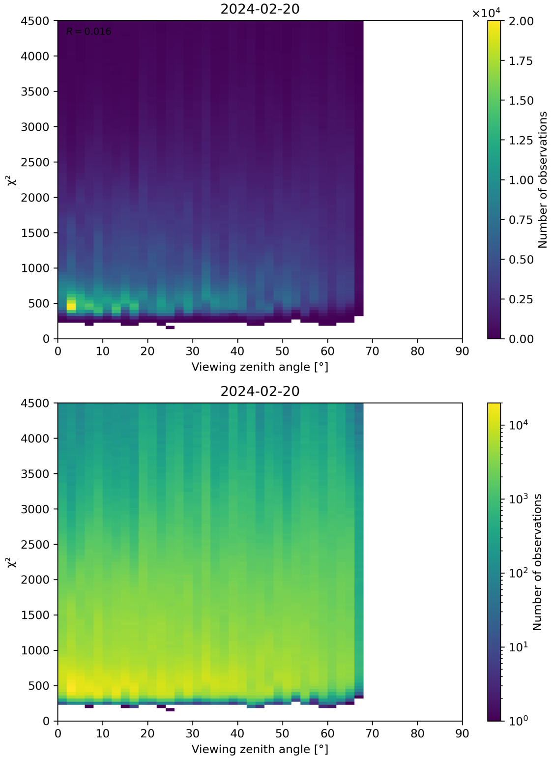
Figure 72: Scatter density plot of “Viewing zenith angle” against “ \chi^2 ” for 2024-02-19 to 2024-02-21.
