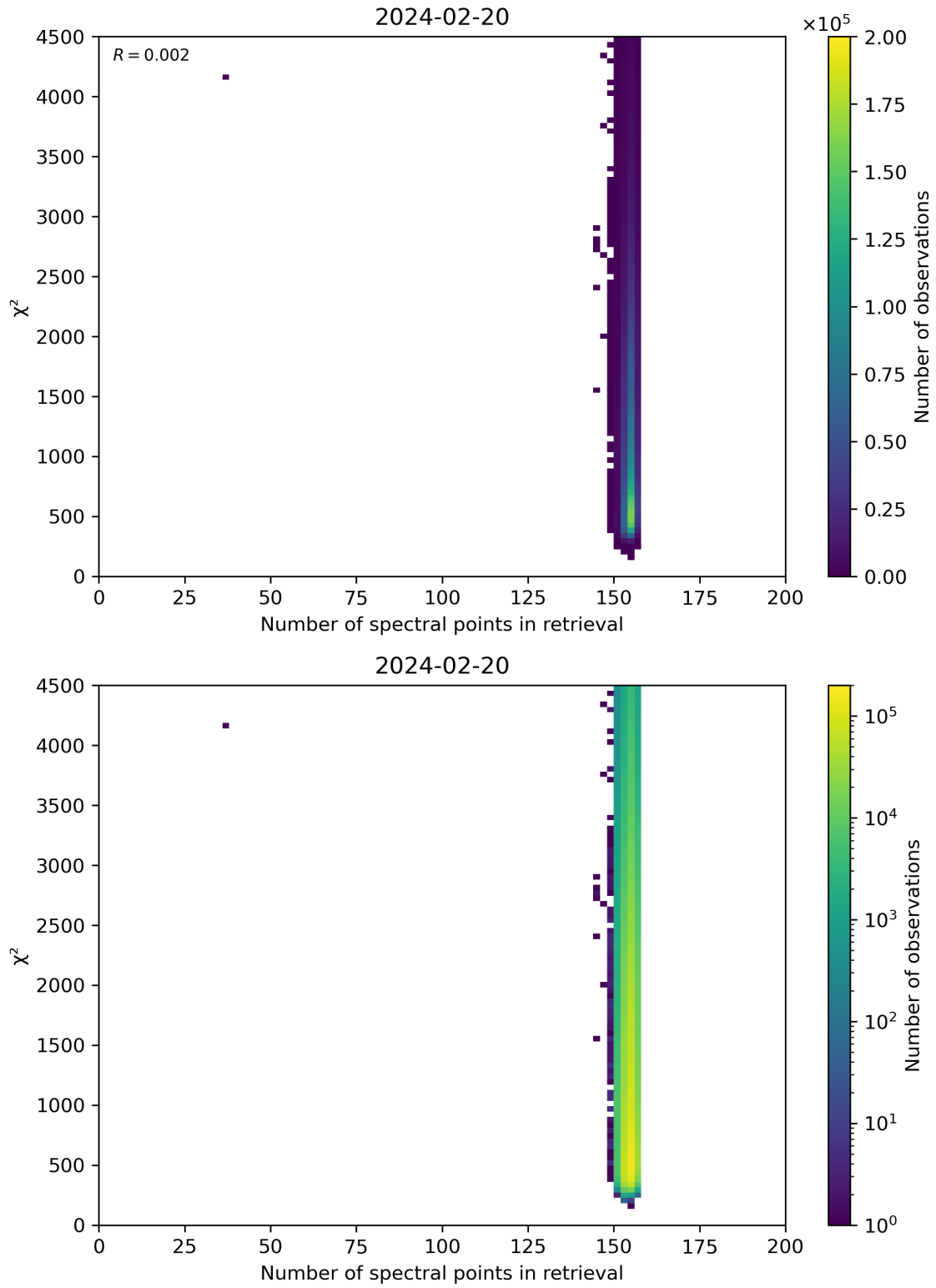
Figure 58: Scatter density plot of “Number of spectral points in retrieval” against “ \chi^2 ” for 2024-02-19 to 2024-02-21.
