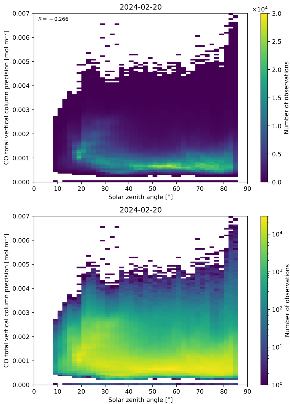
Figure 63: Scatter density plot of “Solar zenith angle” against “CO total vertical column precision” for 2024-02-19 to 2024-02-21.
