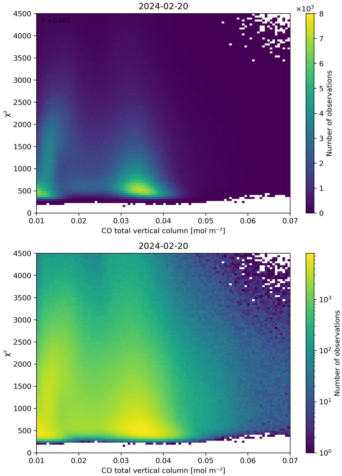
Figure 35: Scatter density plot of “CO total vertical column” against “ \chi^2 ” for 2024-02-19 to 2024-02-21.
