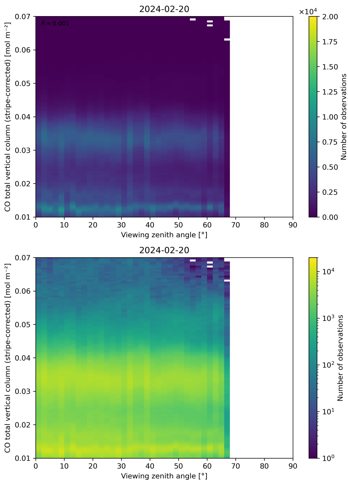
Figure 70: Scatter density plot of “Viewing zenith angle” against “CO total vertical column (stripe-corrected)” for 2024-02-19 to 2024-02-21.
