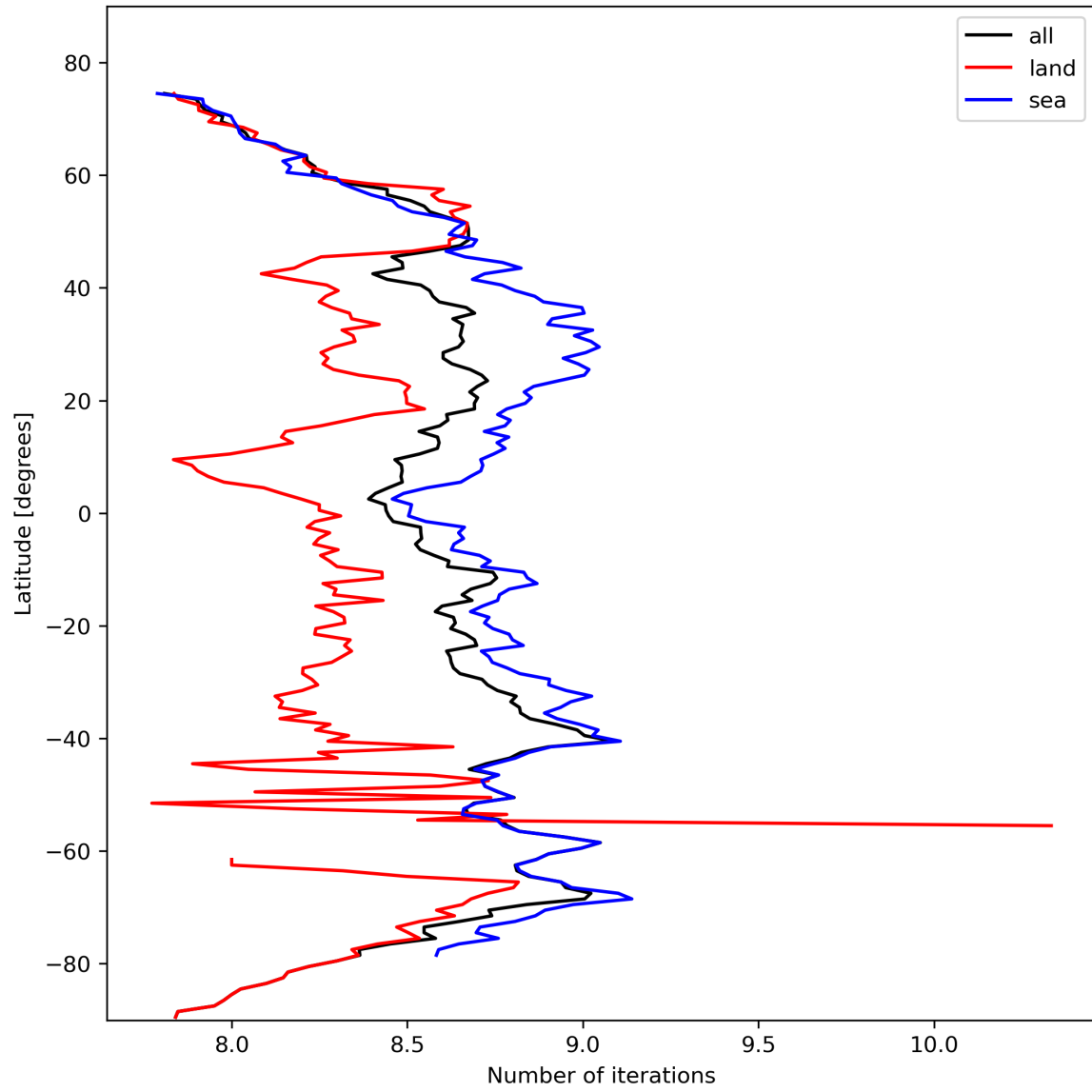
Figure 16: Zonal average of “Number of iterations” for 2024-02-19 to 2024-02-21.
