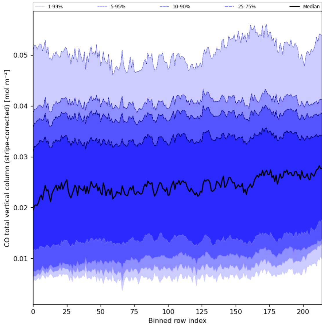
Figure 27: Along track statistics of “CO total vertical column (stripe-corrected)” for 2024-02-19 to 2024-02-21
