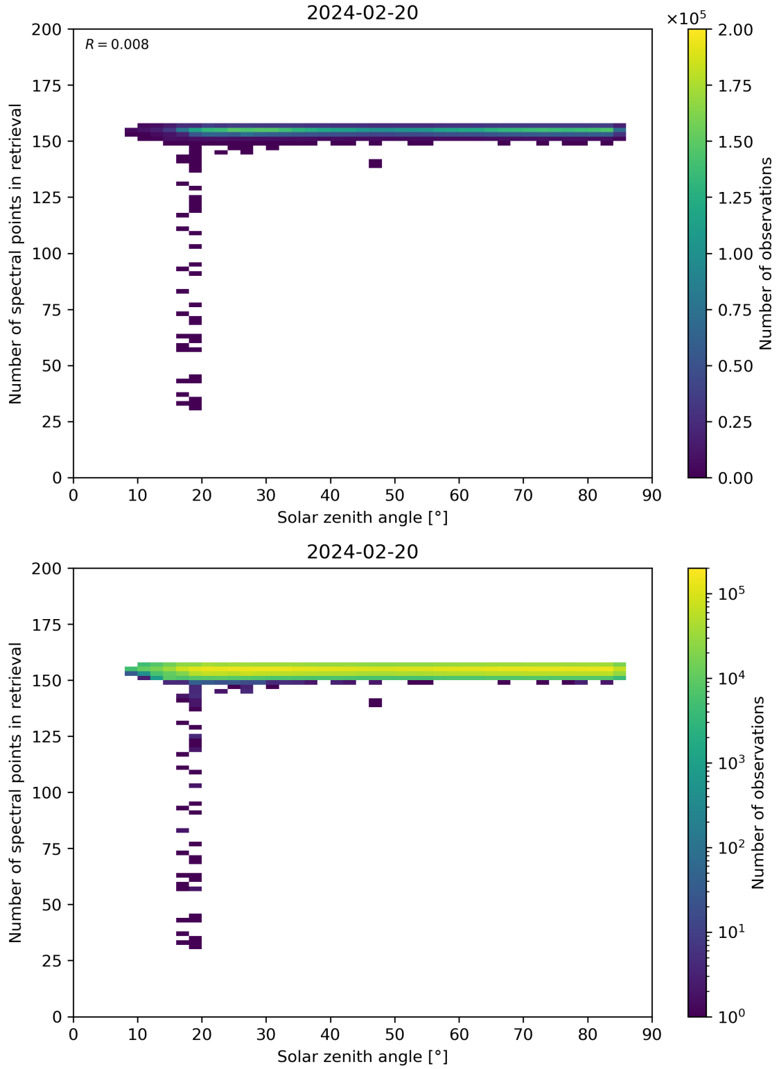
Figure 68: Scatter density plot of “Solar zenith angle” against “Number of spectral points in retrieval” for 2024-02-19 to 2024-02-21.
