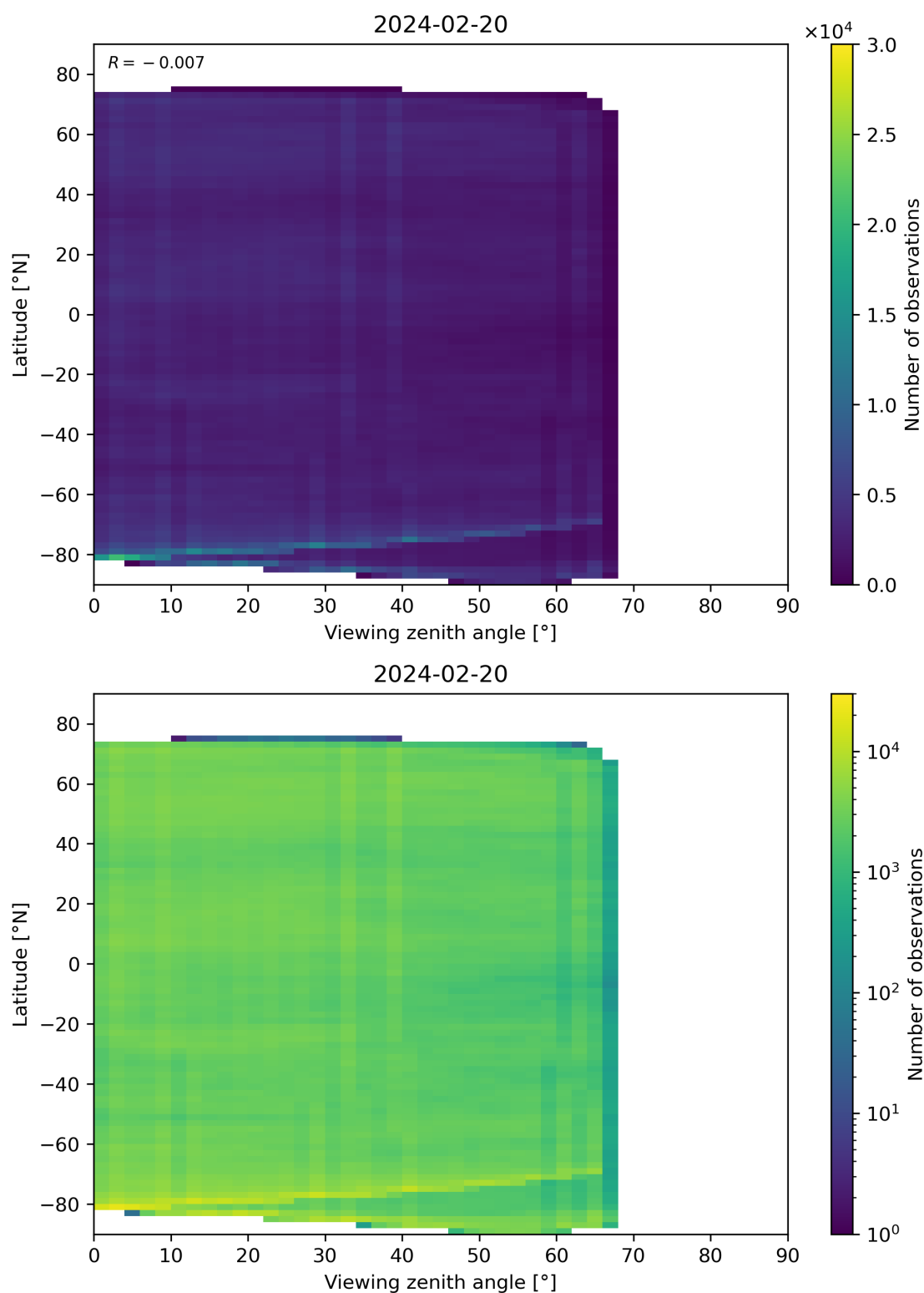
Figure 74: Scatter density plot of “Viewing zenith angle” against “Latitude” for 2024-02-19 to 2024-02-21.
