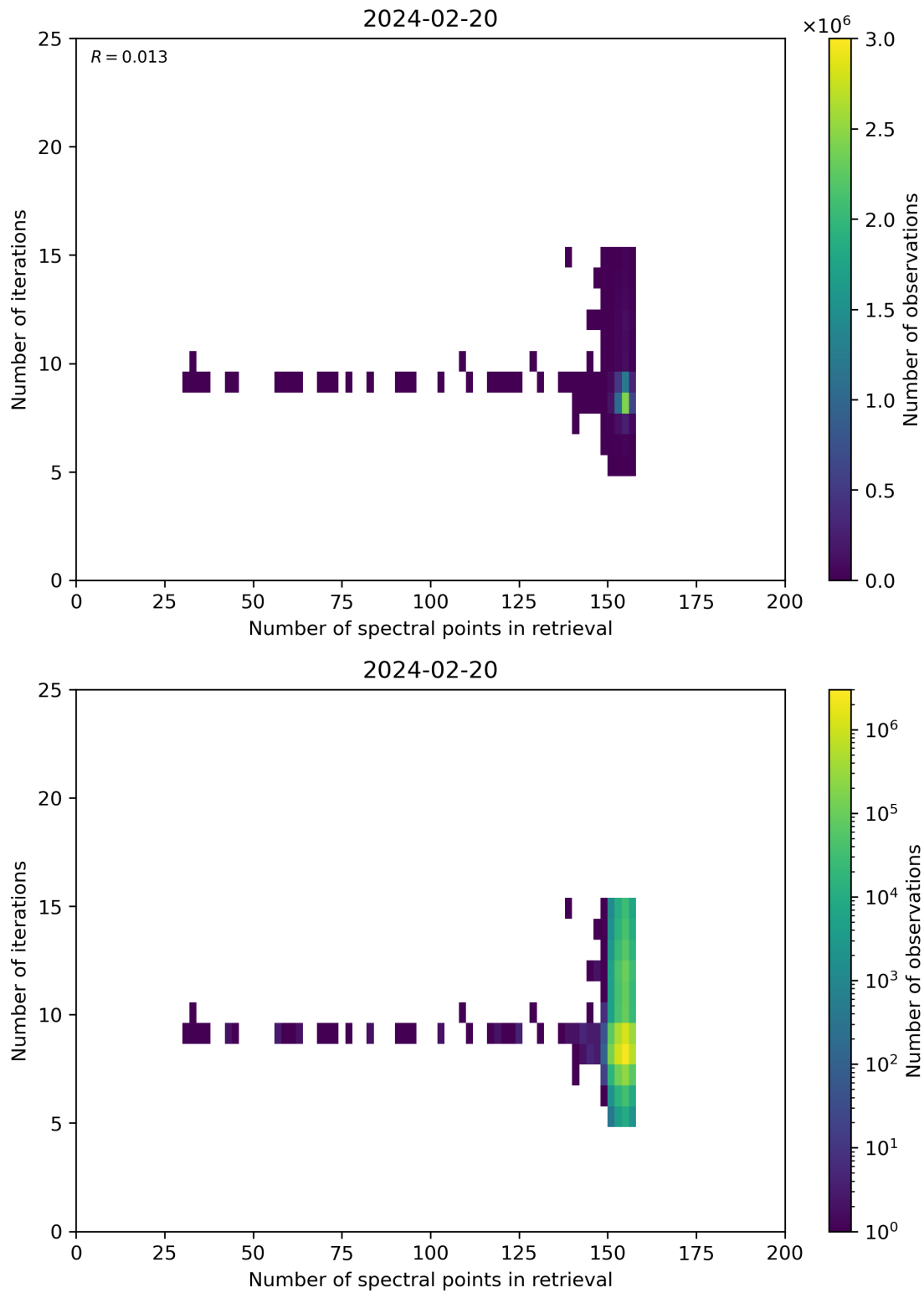
Figure 60: Scatter density plot of “Number of spectral points in retrieval” against “Number of iterations” for 2024-02-19 to 2024-02-21.
