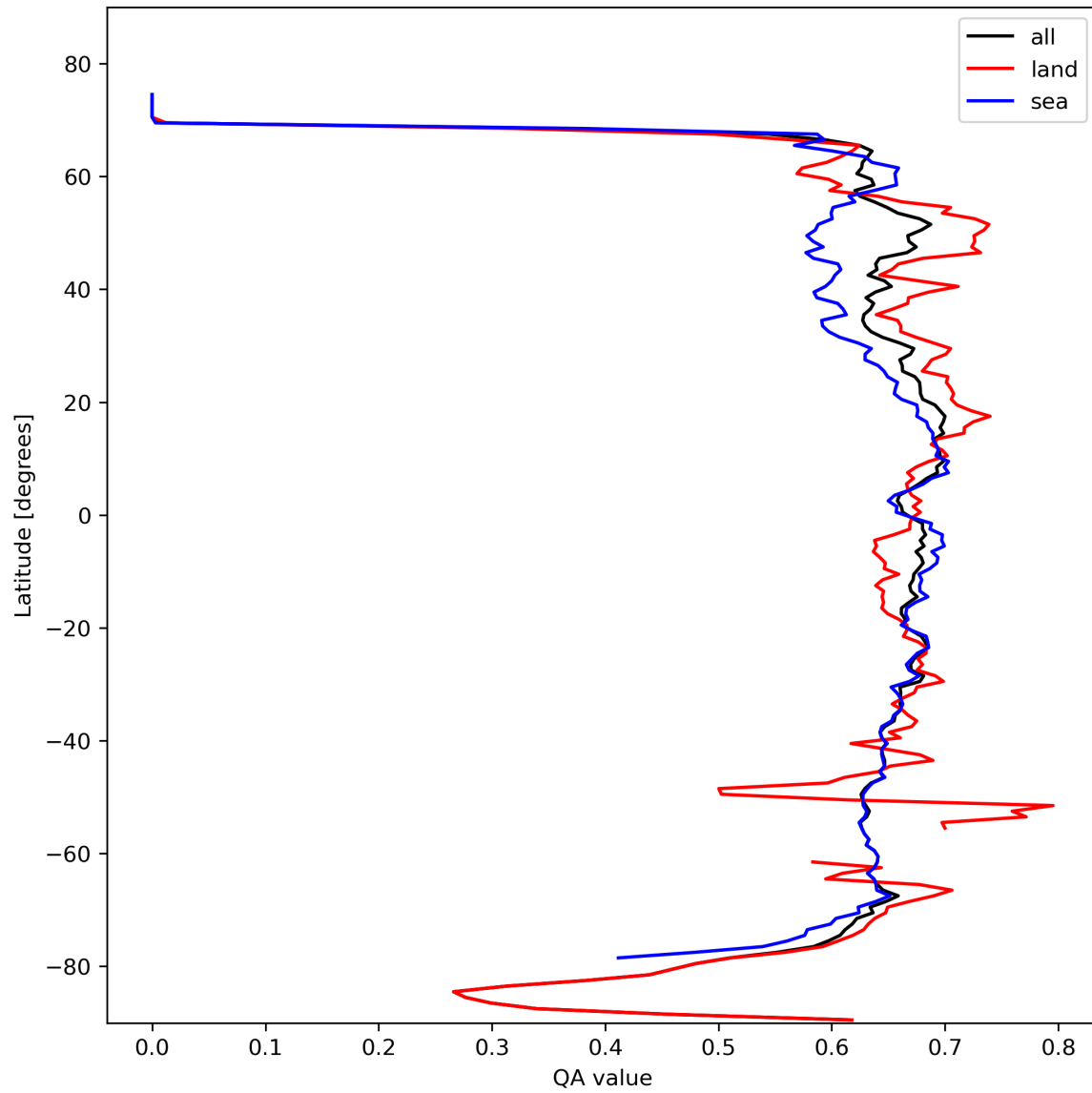
Figure 9: Zonal average of “QA value” for 2024-02-19 to 2024-02-21.
