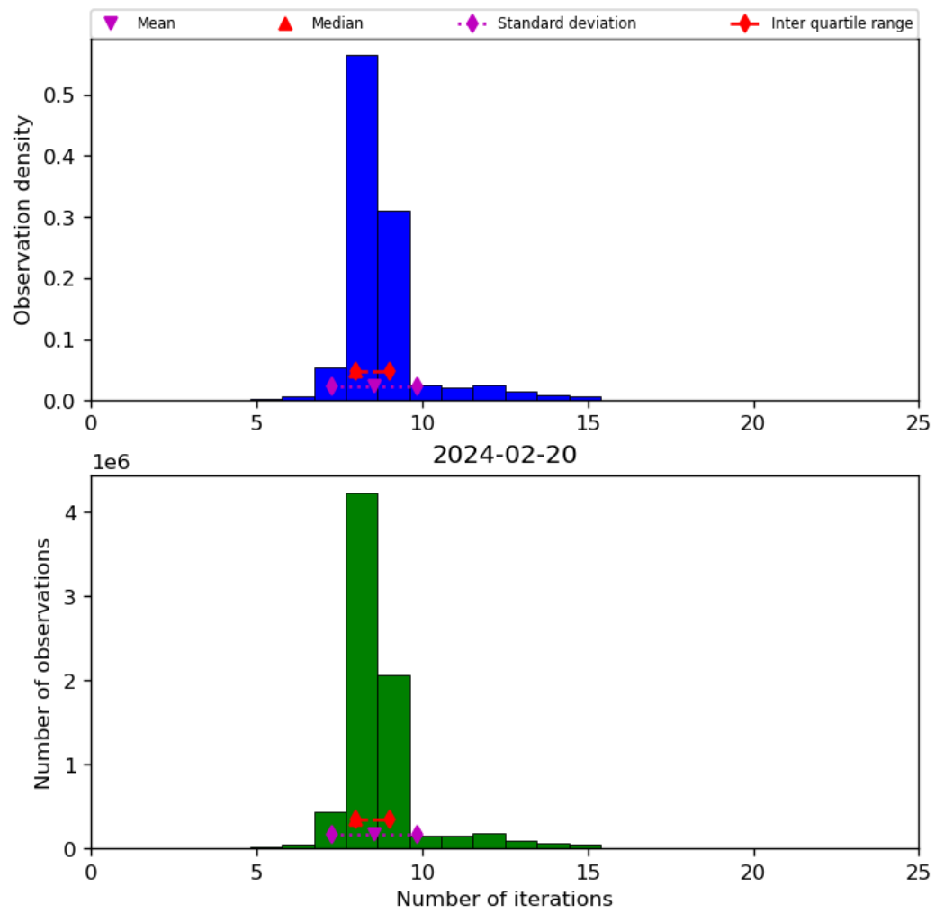
Figure 24: Histogram of “Number of iterations” for 2024-02-19 to 2024-02-21
