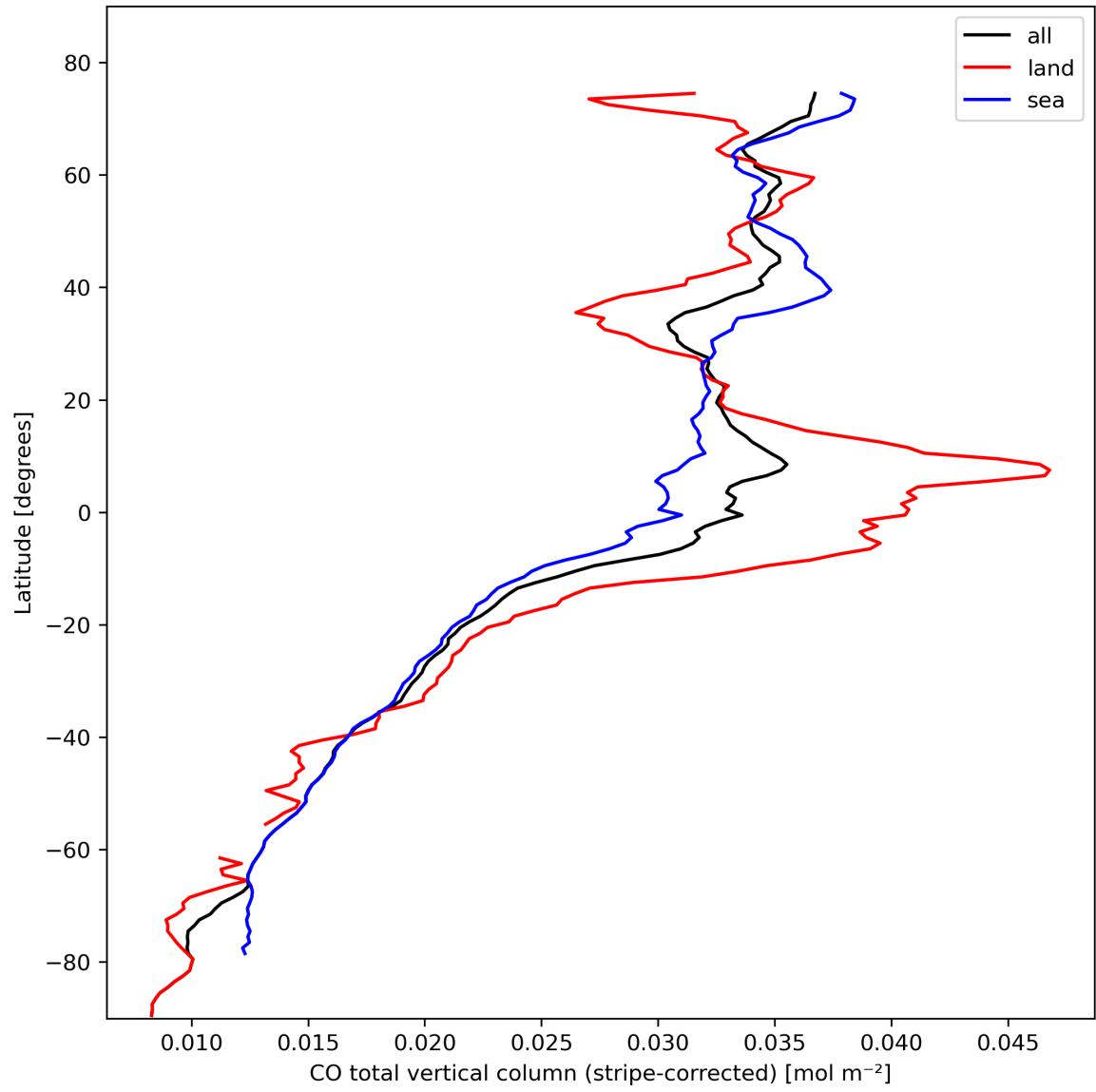
Figure 11: Zonal average of “CO total vertical column (stripe-corrected)” for 2024-02-19 to 2024-02-21.
