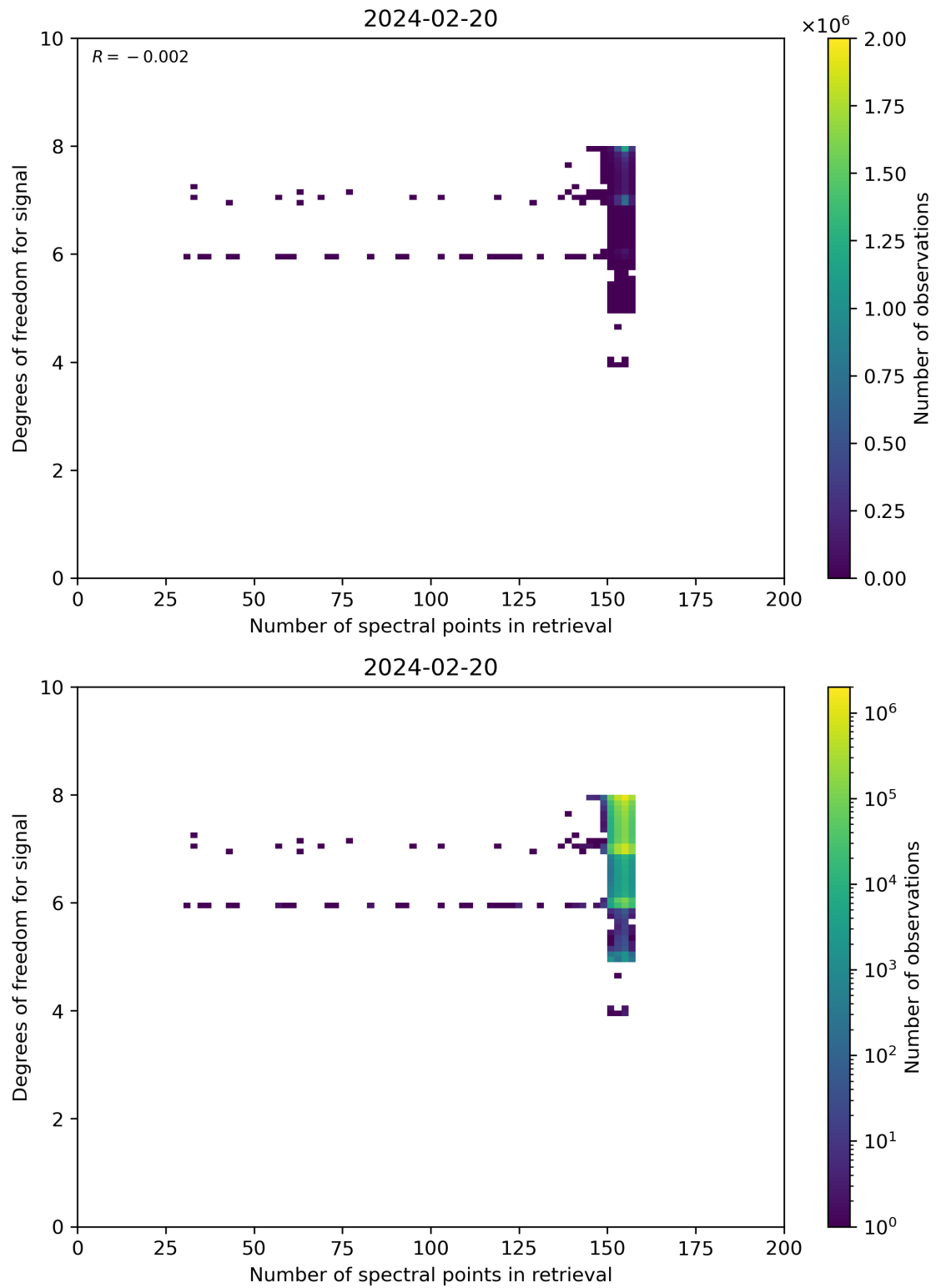
Figure 59: Scatter density plot of “Number of spectral points in retrieval” against “Degrees of freedom for signal” for 2024-02-19 to 2024-02-21.
