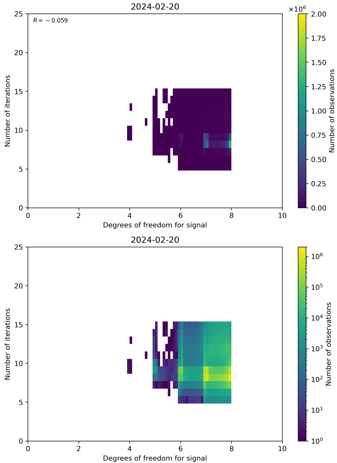
Figure 50: Scatter density plot of “Degrees of freedom for signal” against “Number of iterations” for 2024-02-19 to 2024-02-21.
