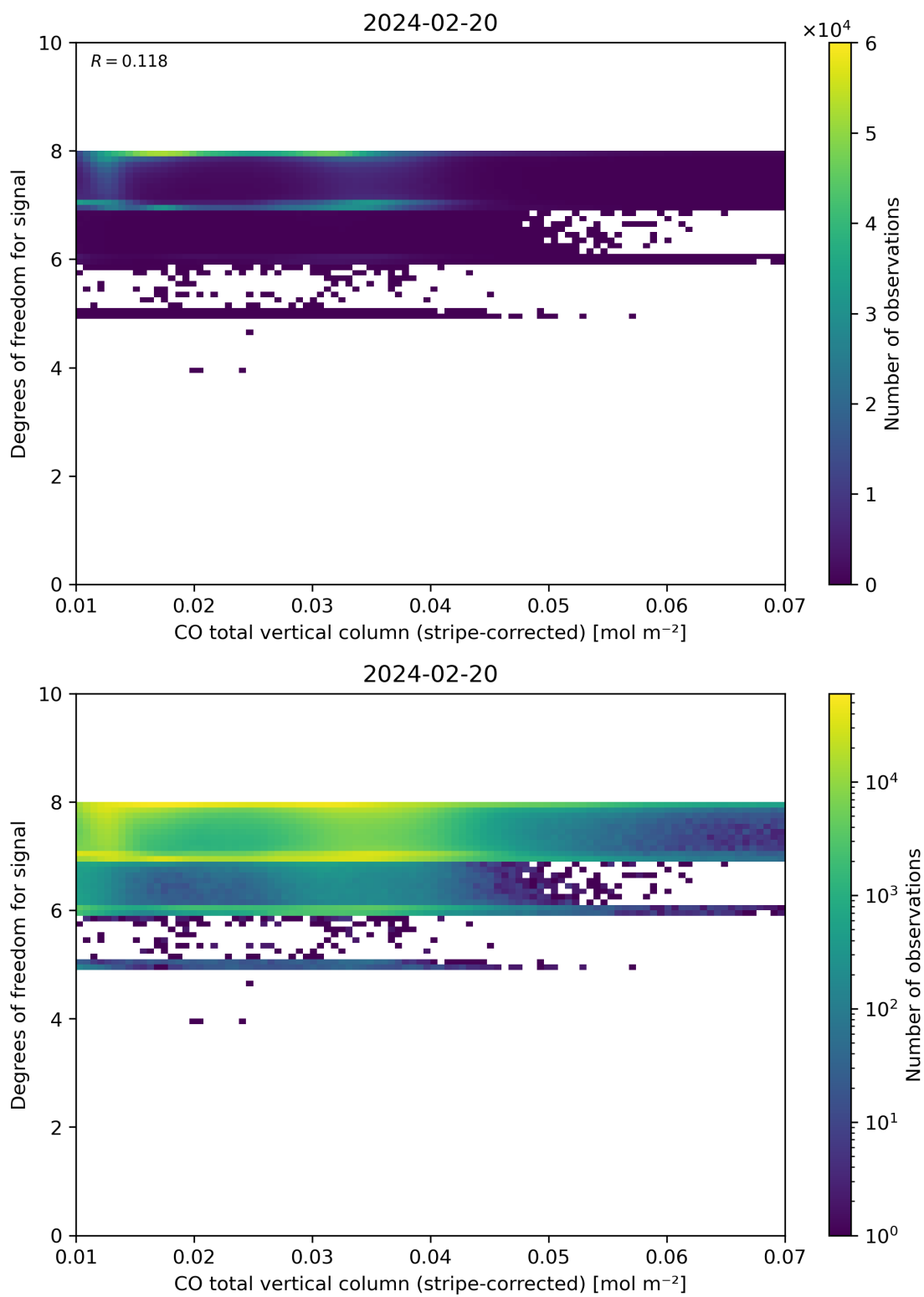
Figure 38: Scatter density plot of “CO total vertical column (stripe-corrected)” against “Degrees of freedom for signal” for 2024-02-19 to 2024-02-21.
