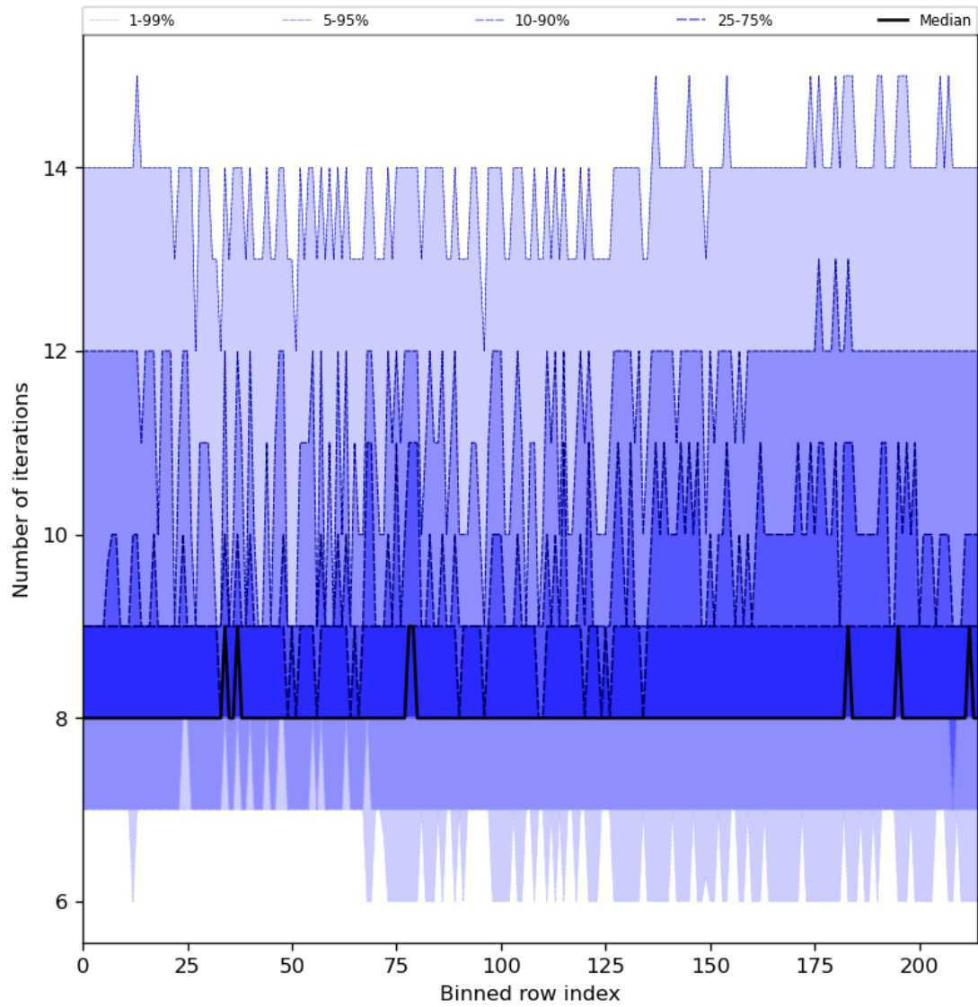
Figure 32: Along track statistics of “Number of iterations” for 2024-02-19 to 2024-02-21
