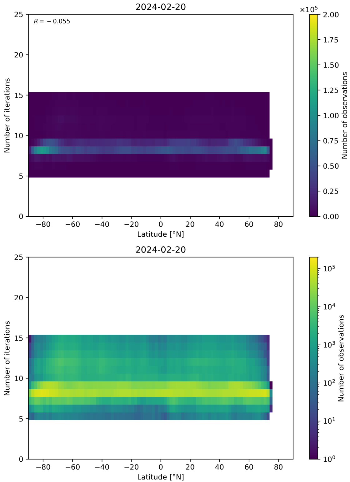
Figure 56: Scatter density plot of “Latitude” against “Number of iterations” for 2024-02-19 to 2024-02-21.
