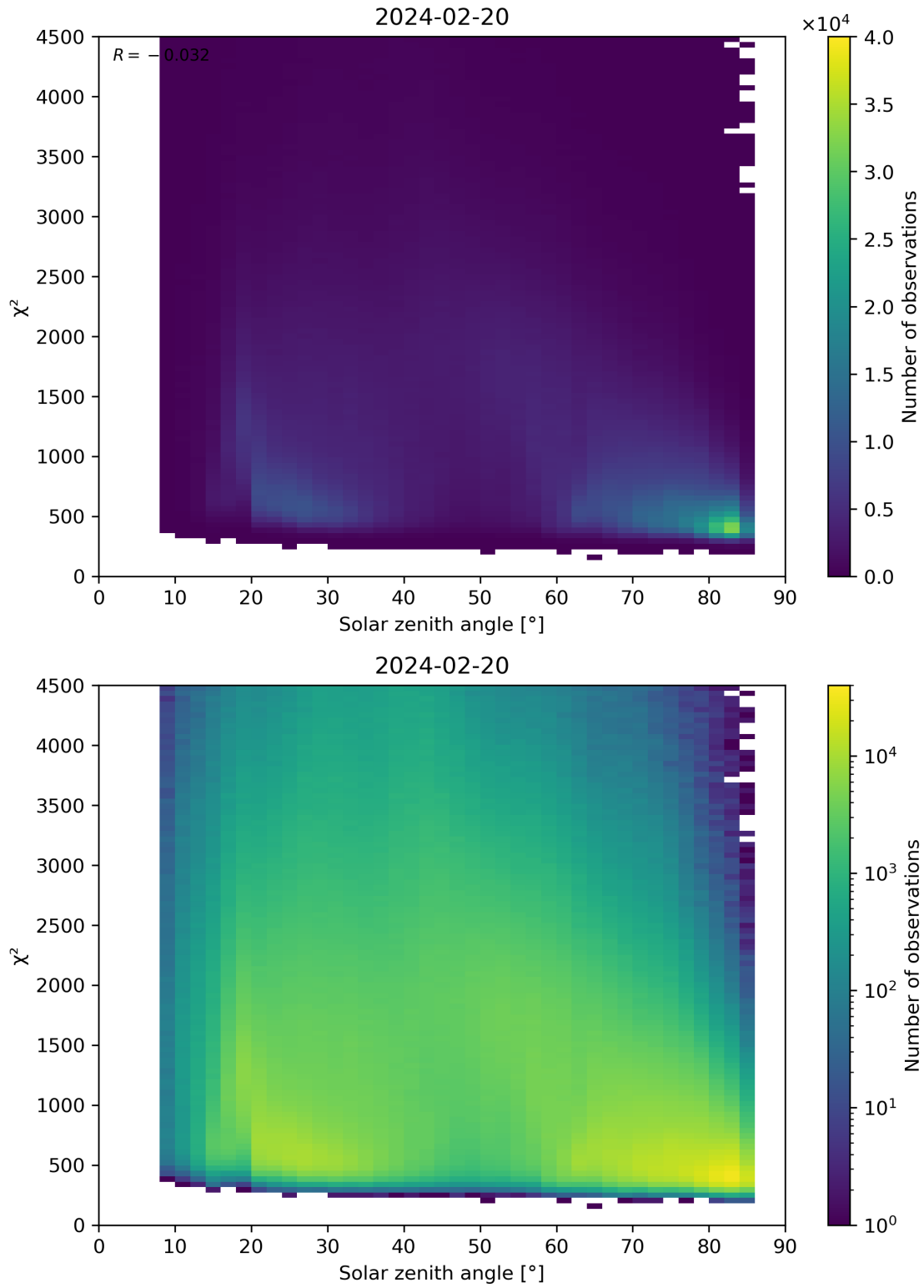
Figure 64: Scatter density plot of “Solar zenith angle” against “ \chi^2 ” for 2024-02-19 to 2024-02-21.
