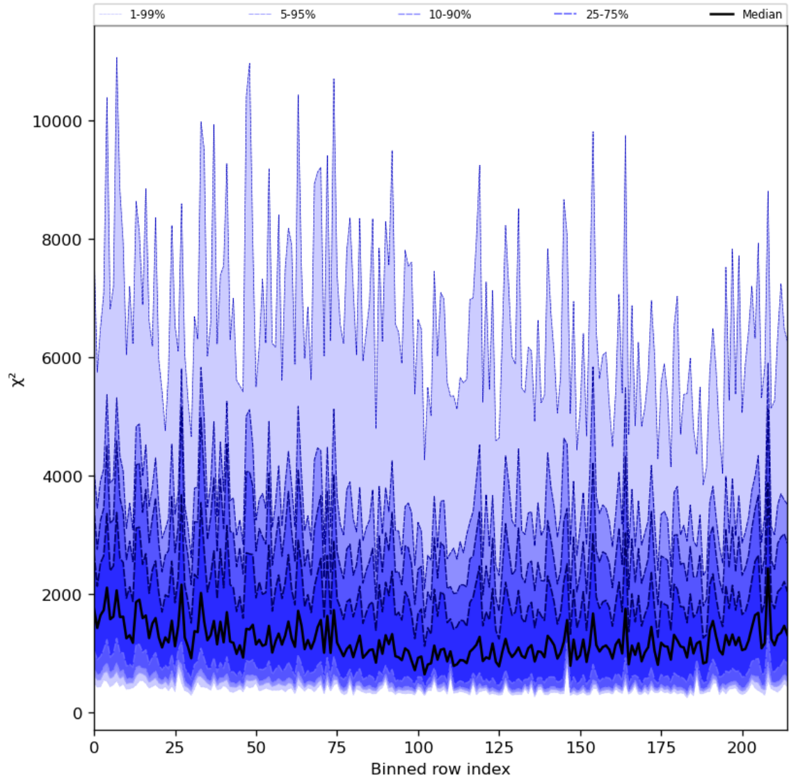
Figure 30: Along track statistics of “ \chi^2 ” for 2024-02-19 to 2024-02-21
