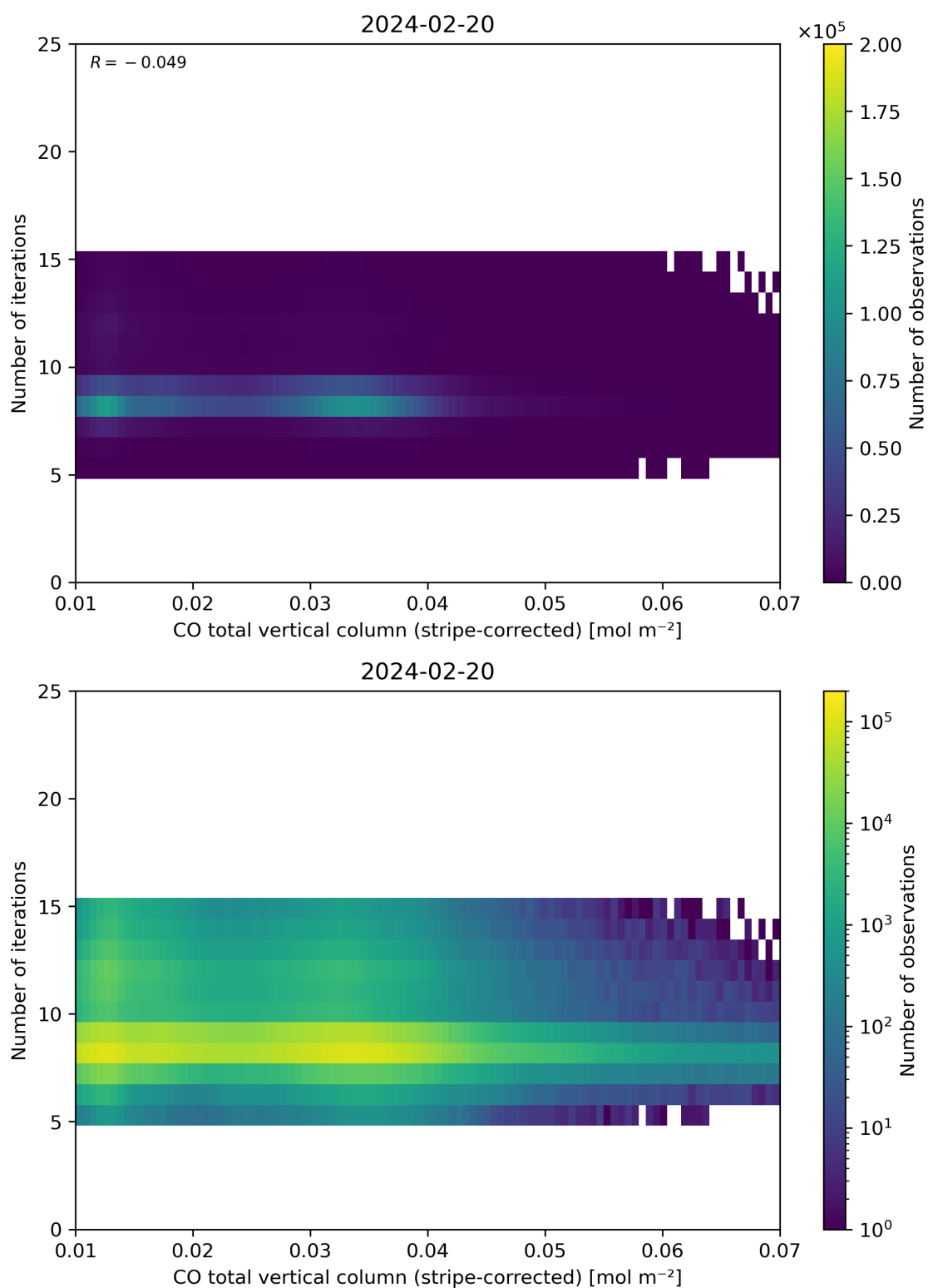
Figure 39: Scatter density plot of “CO total vertical column (stripe-corrected)” against “Number of iterations” for 2024-02-19 to 2024-02-21.
