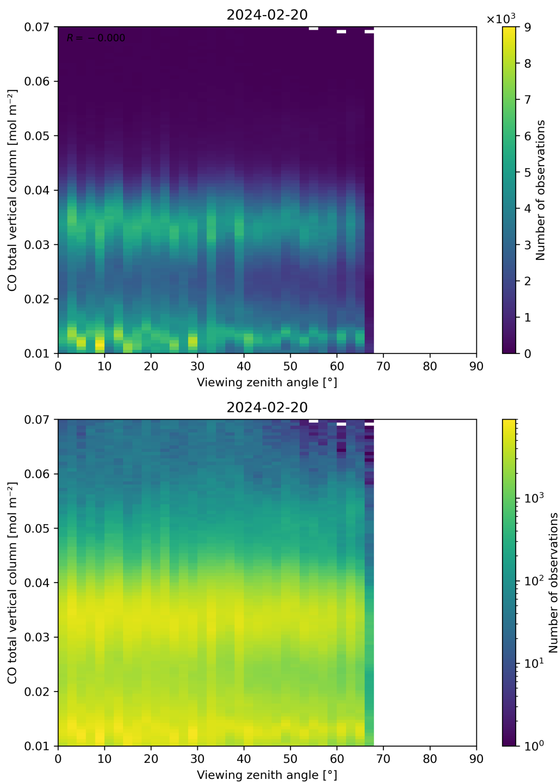
Figure 69: Scatter density plot of “Viewing zenith angle” against “CO total vertical column” for 2024-02-19 to 2024-02-21.
