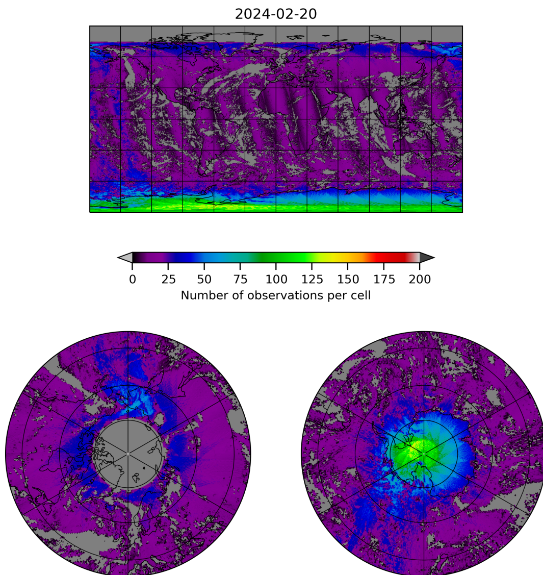
Figure 8: Map of the number of observations for 2024-02-19 to 2024-02-21
