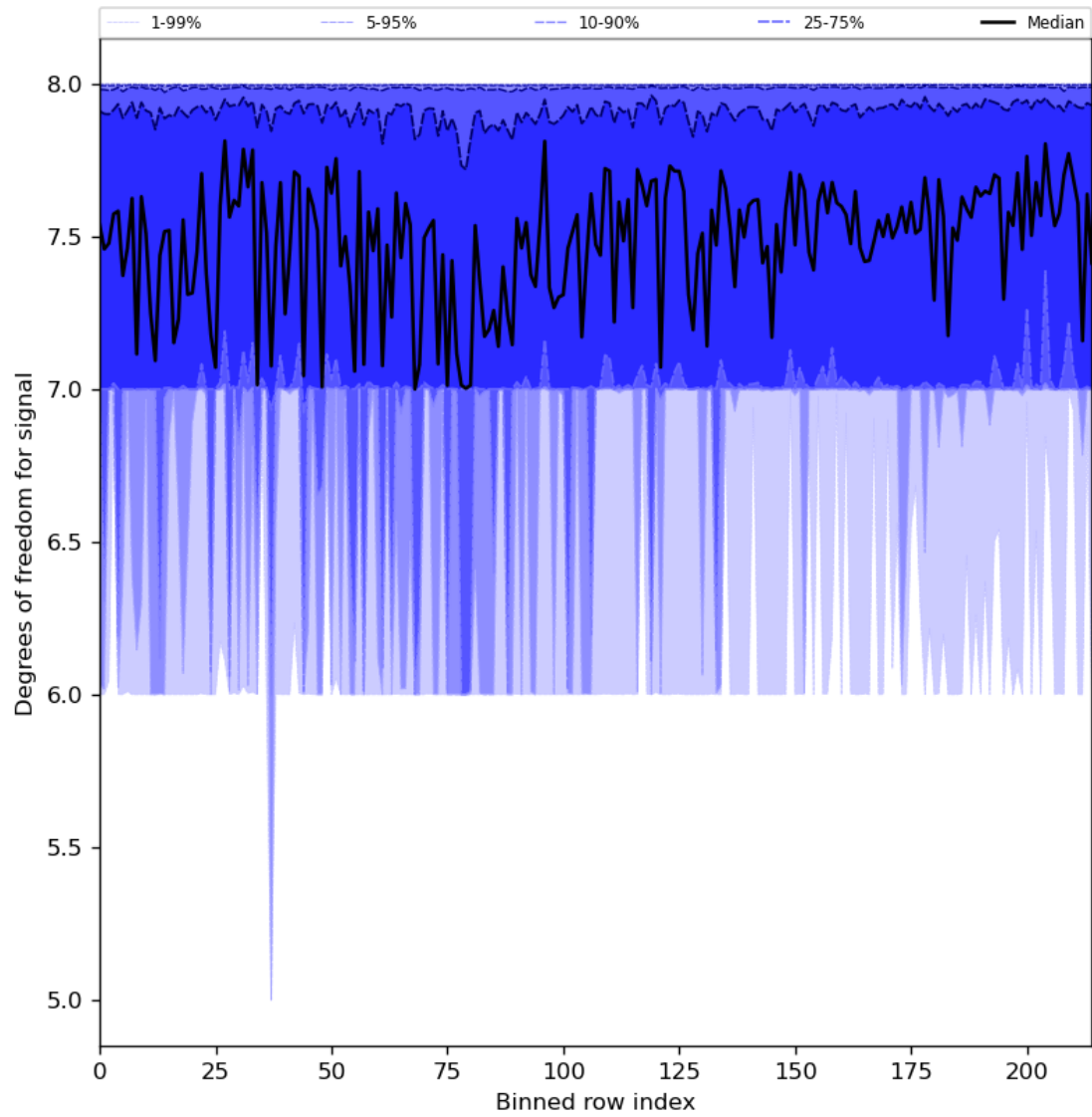
Figure 31: Along track statistics of “Degrees of freedom for signal” for 2024-02-19 to 2024-02-21
