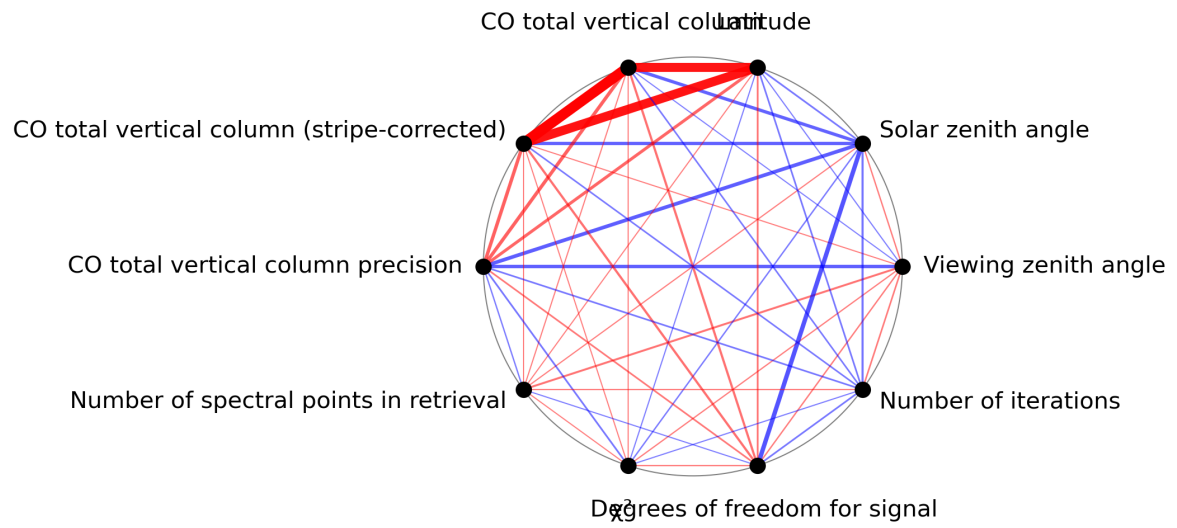
Figure 1: Map of correlation graph for 2024-02-19 to 2024-02-21.
