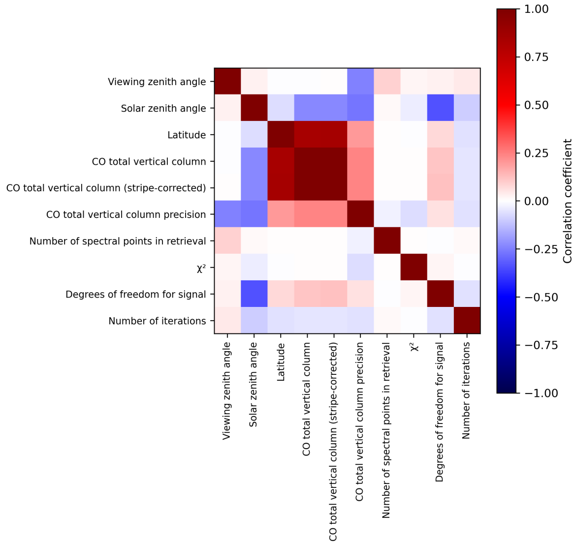
Figure 2: Map of correlation matrix for 2024-02-19 to 2024-02-21.
