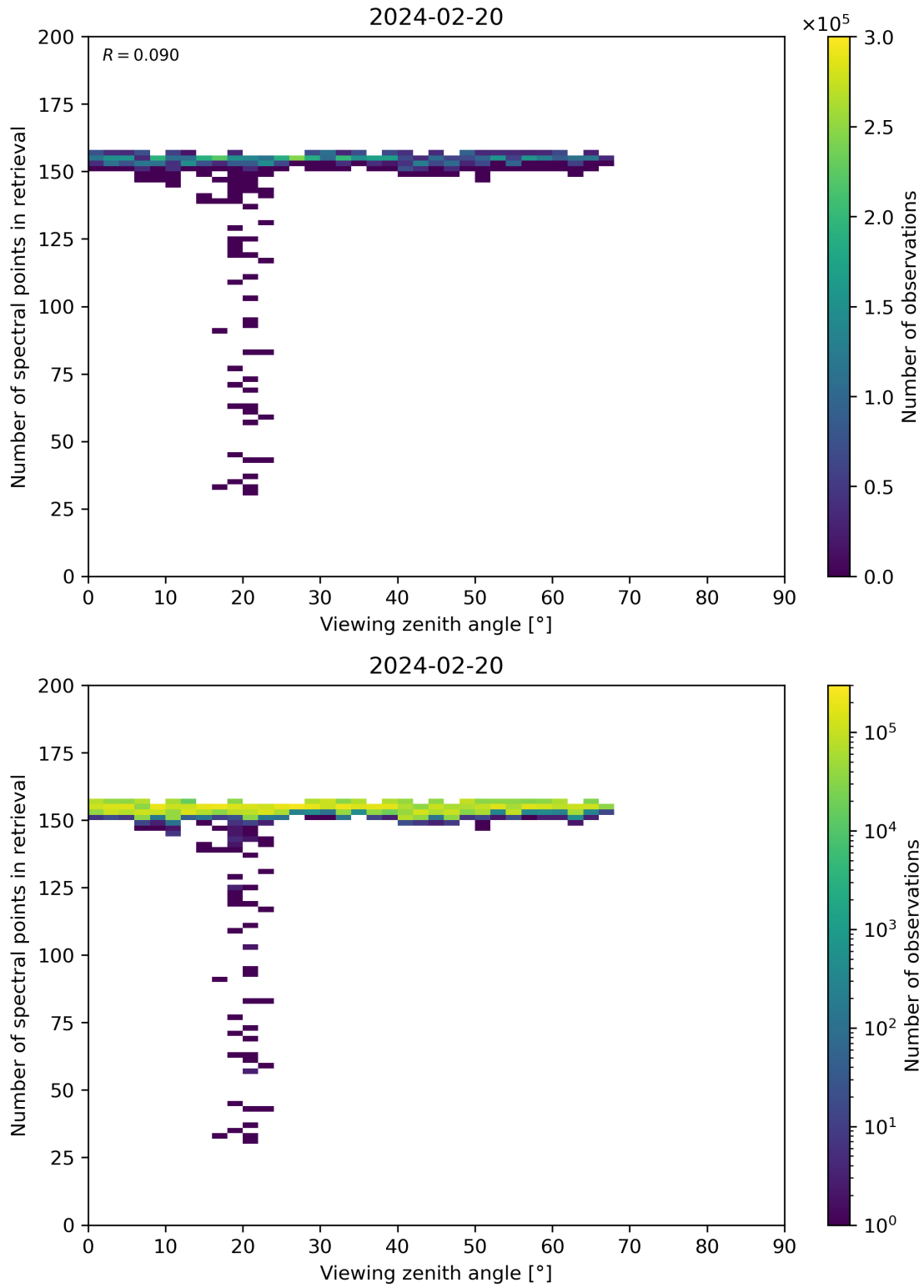
Figure 76: Scatter density plot of “Viewing zenith angle” against “Number of spectral points in retrieval” for 2024-02-19 to 2024-02-21.
