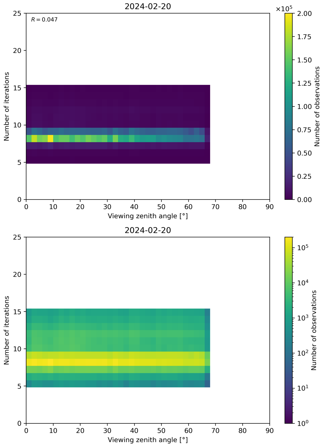
Figure 75: Scatter density plot of “Viewing zenith angle” against “Number of iterations” for 2024-02-19 to 2024-02-21.
