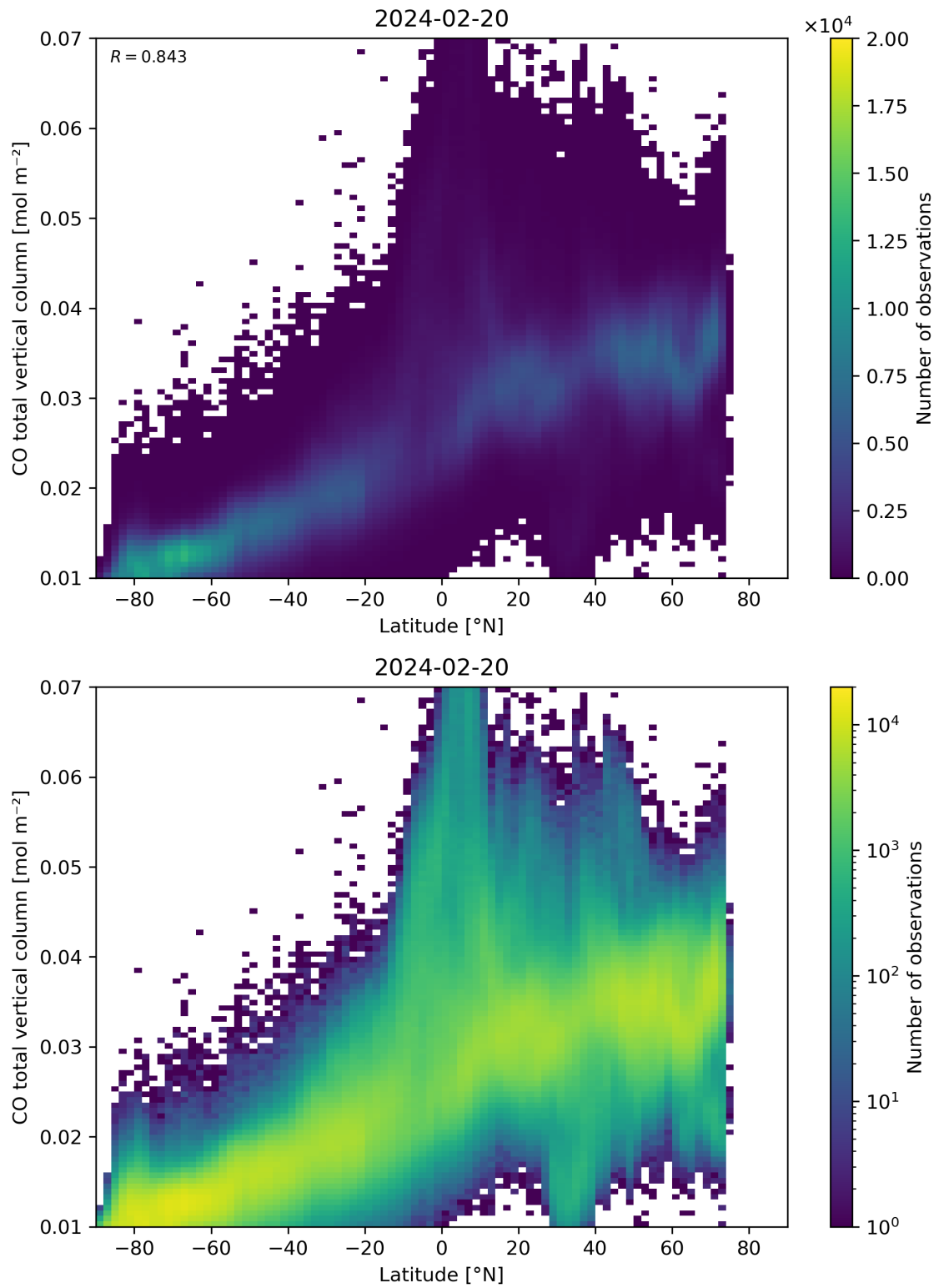
Figure 51: Scatter density plot of “Latitude” against “CO total vertical column” for 2024-02-19 to 2024-02-21.
