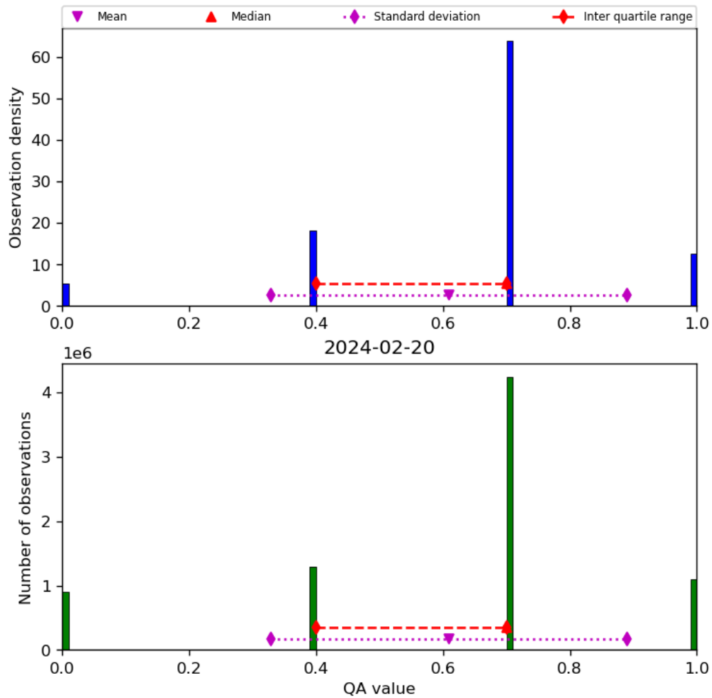
Figure 17: Histogram of “QA value” for 2024-02-19 to 2024-02-21
