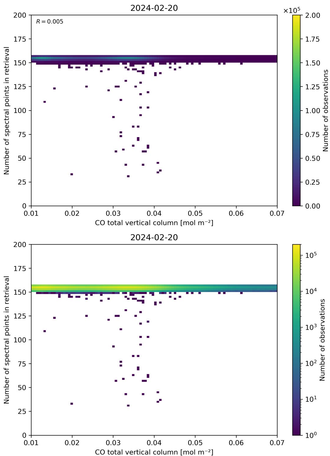
Figure 43: Scatter density plot of “CO total vertical column” against “Number of spectral points in retrieval” for 2024-02-19 to 2024-02-21.
