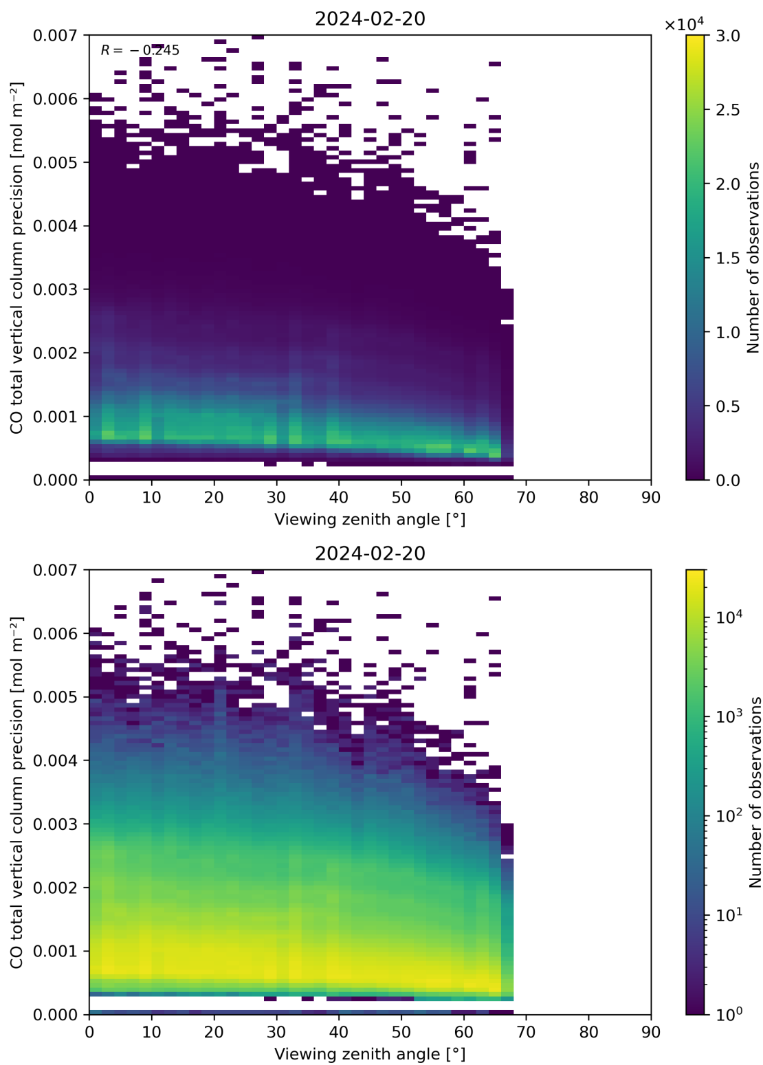
Figure 71: Scatter density plot of “Viewing zenith angle” against “CO total vertical column precision” for 2024-02-19 to 2024-02-21.
