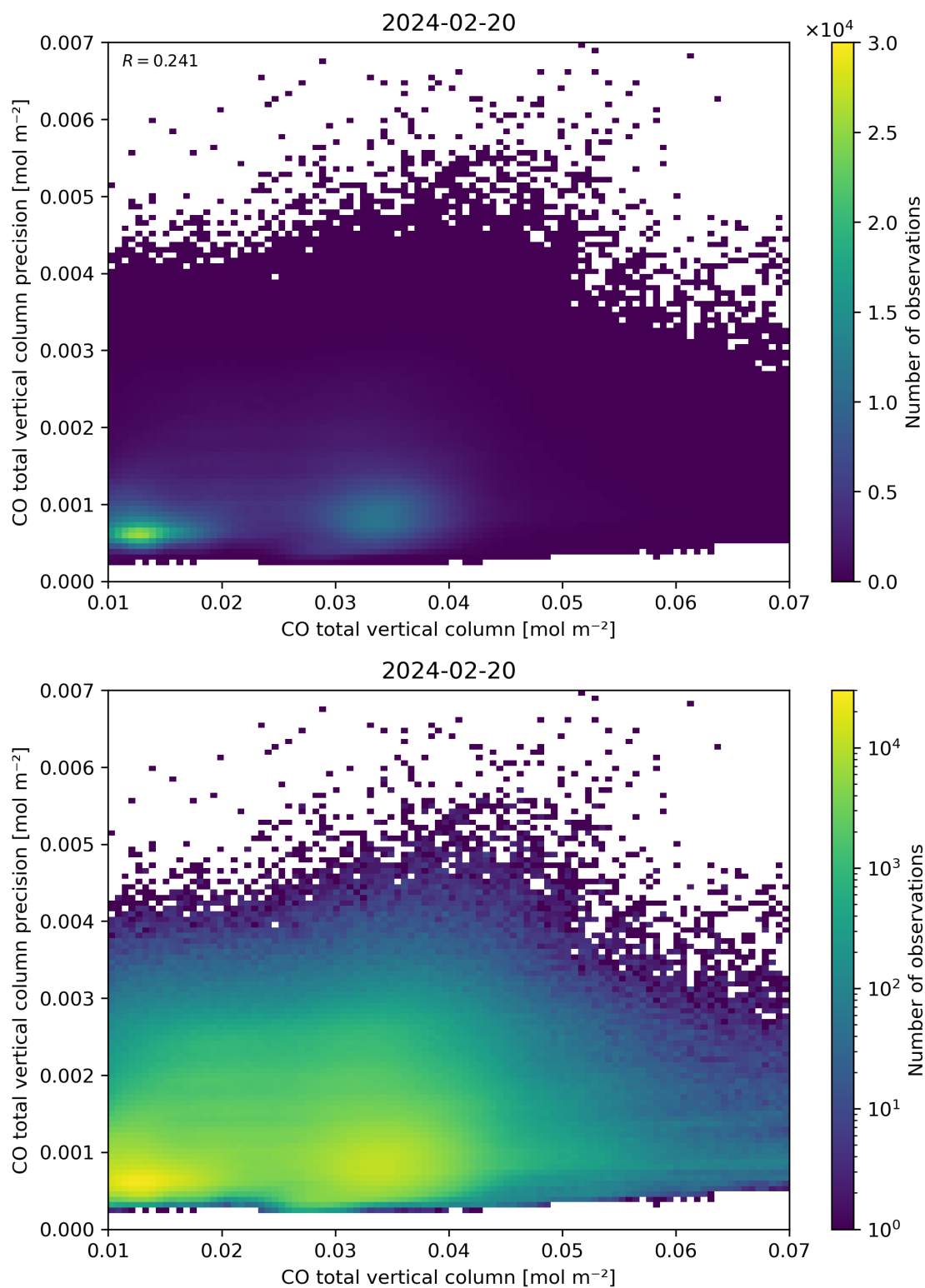
Figure 34: Scatter density plot of “CO total vertical column” against “CO total vertical column precision” for 2024-02-19 to 2024-02-21.
