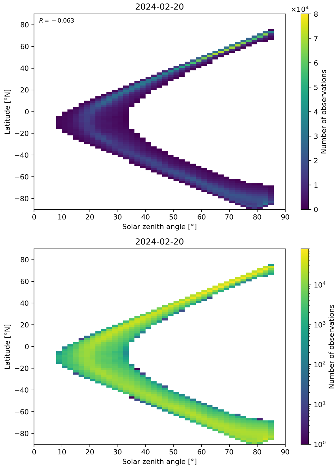
Figure 66: Scatter density plot of “Solar zenith angle” against “Latitude” for 2024-02-19 to 2024-02-21.
