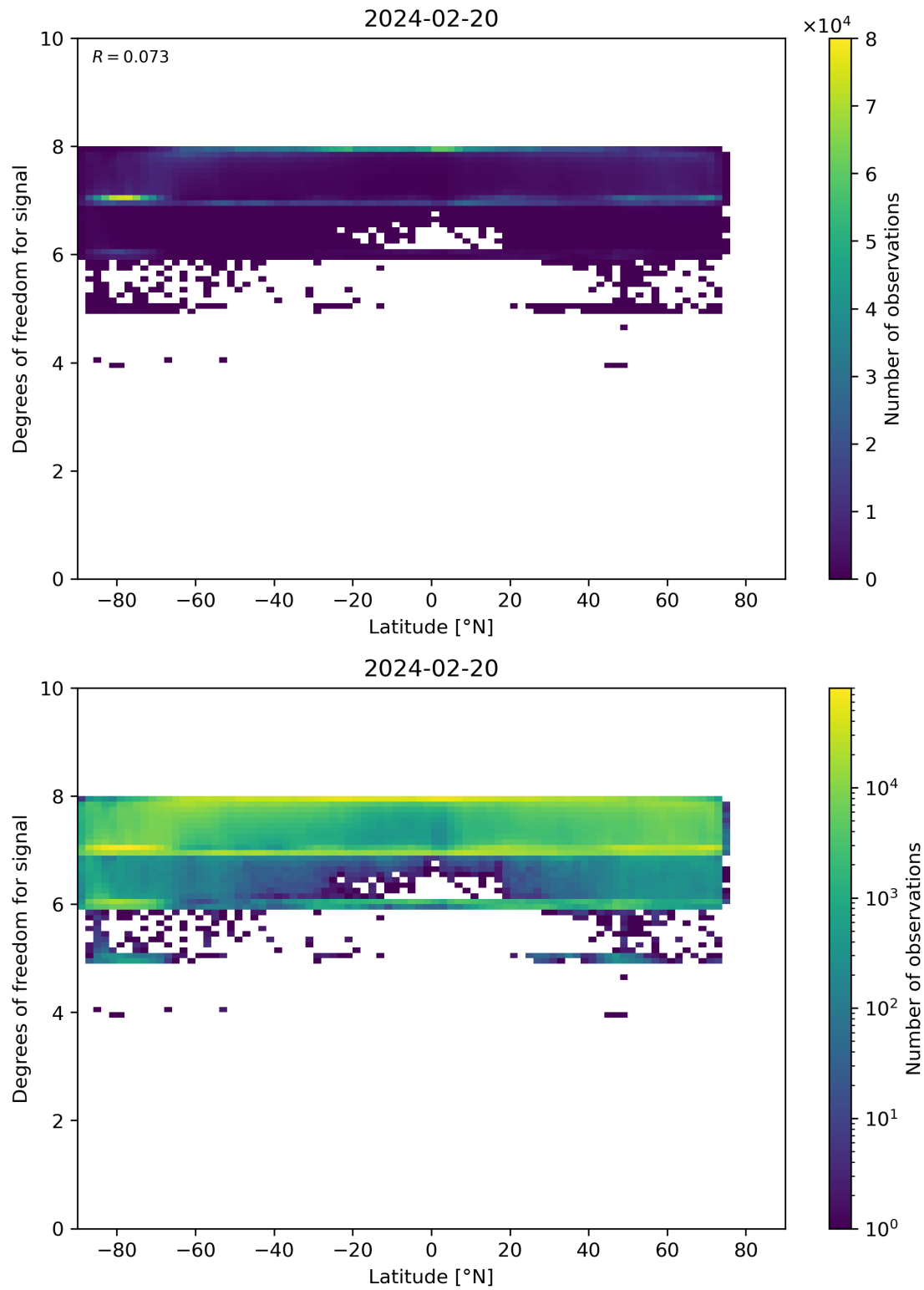
Figure 55: Scatter density plot of “Latitude” against “Degrees of freedom for signal” for 2024-02-19 to 2024-02-21.
