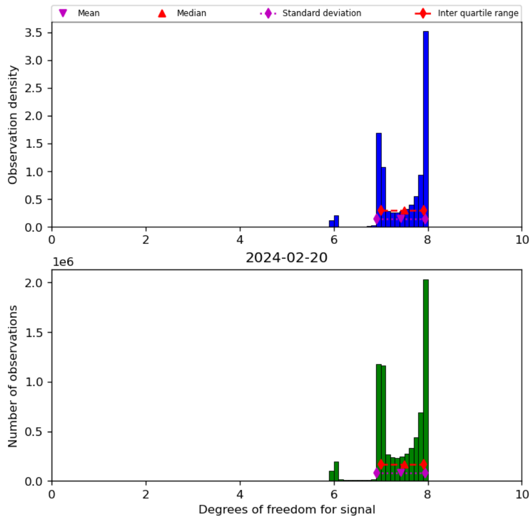
Figure 23: Histogram of “Degrees of freedom for signal” for 2024-02-19 to 2024-02-21
