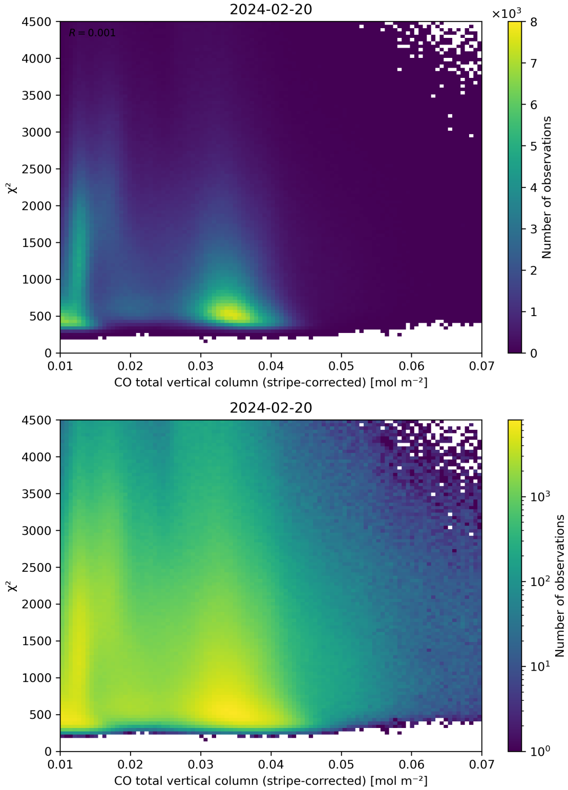
Figure 37: Scatter density plot of “CO total vertical column (stripe-corrected)” against “ \chi^2 ” for 2024-02-19 to 2024-02-21.
