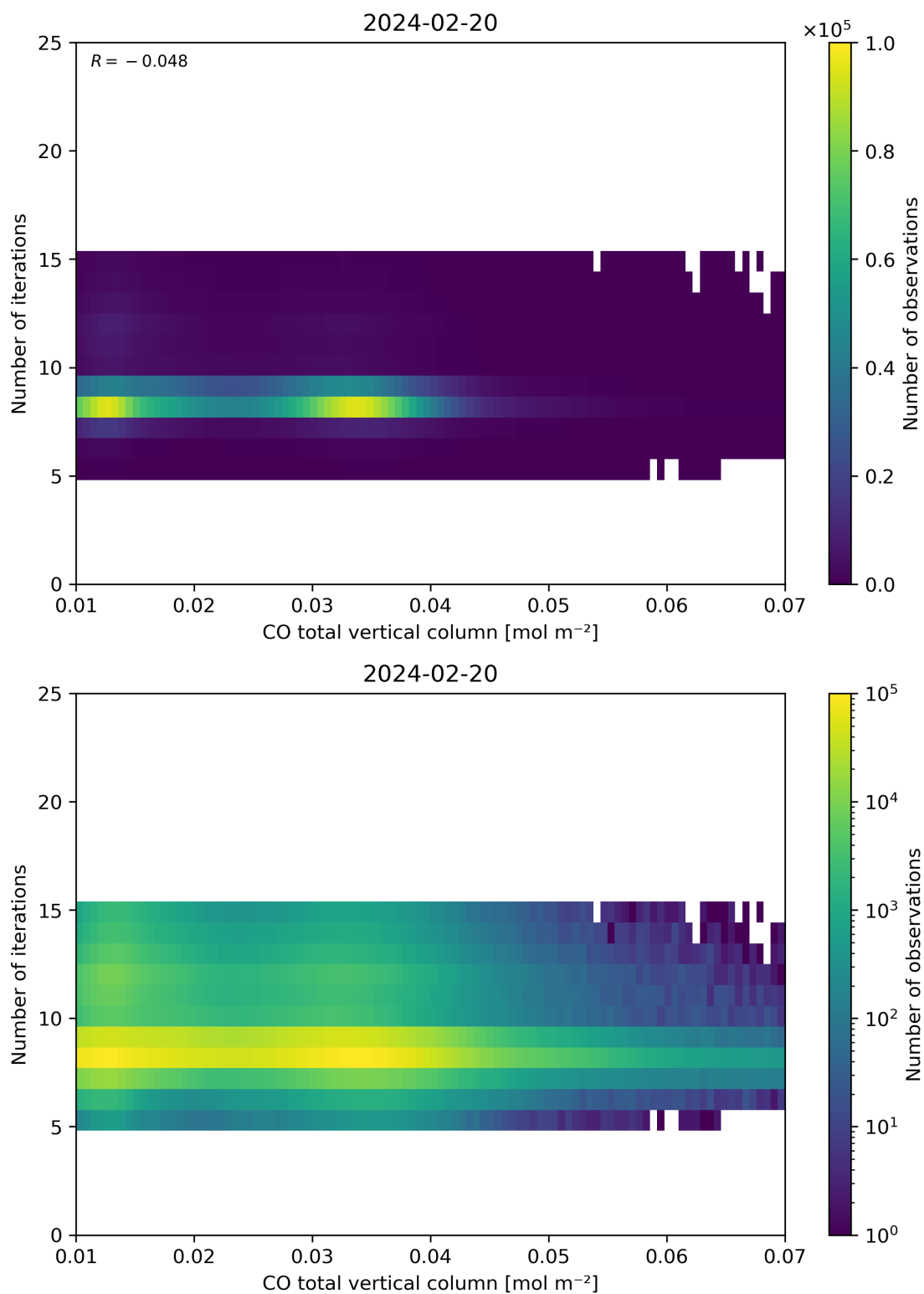
Figure 42: Scatter density plot of “CO total vertical column” against “Number of iterations” for 2024-02-19 to 2024-02-21.
