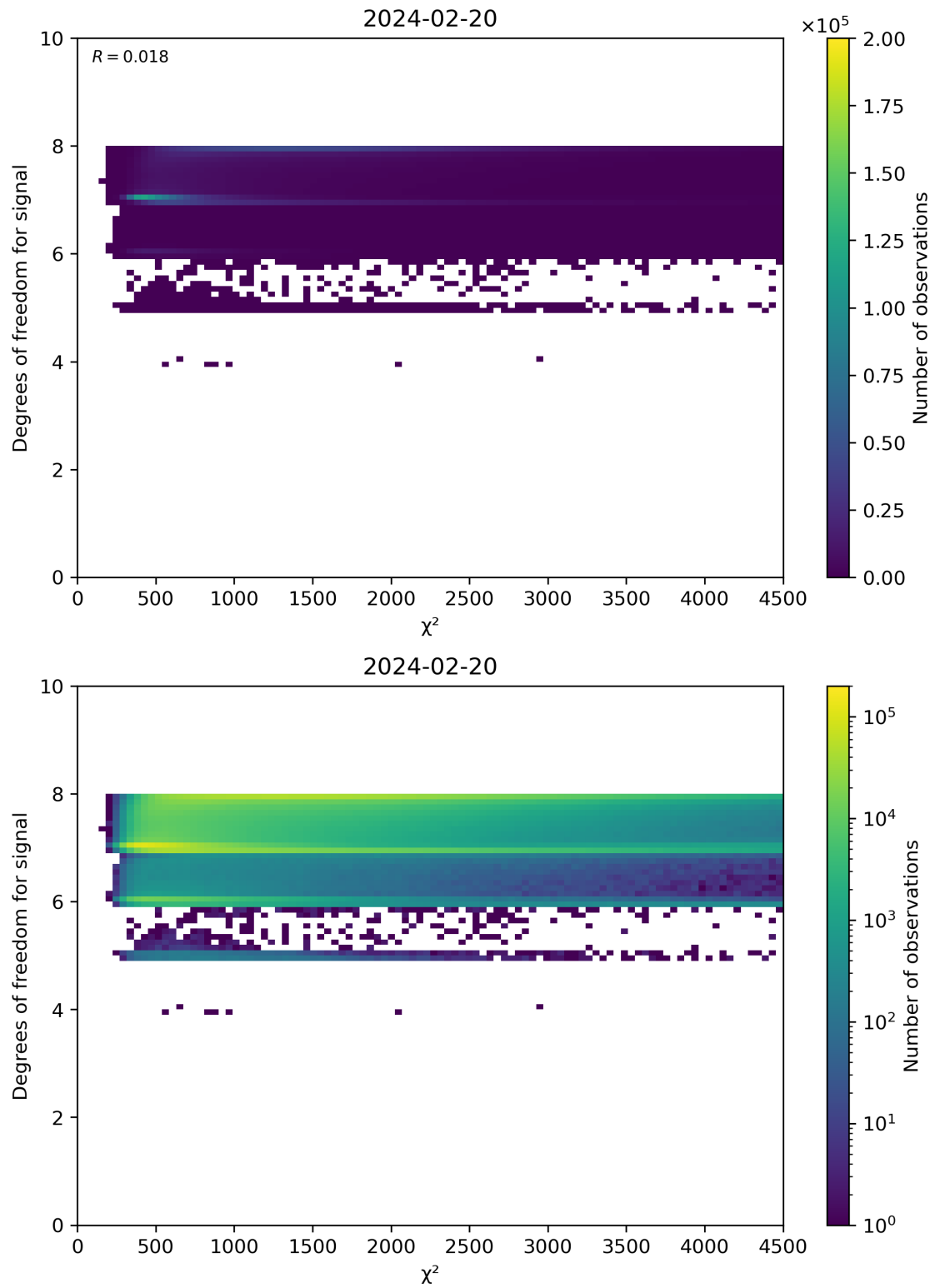
Figure 48: Scatter density plot of “ \chi^2 ” against “Degrees of freedom for signal” for 2024-02-19 to 2024-02-21.
