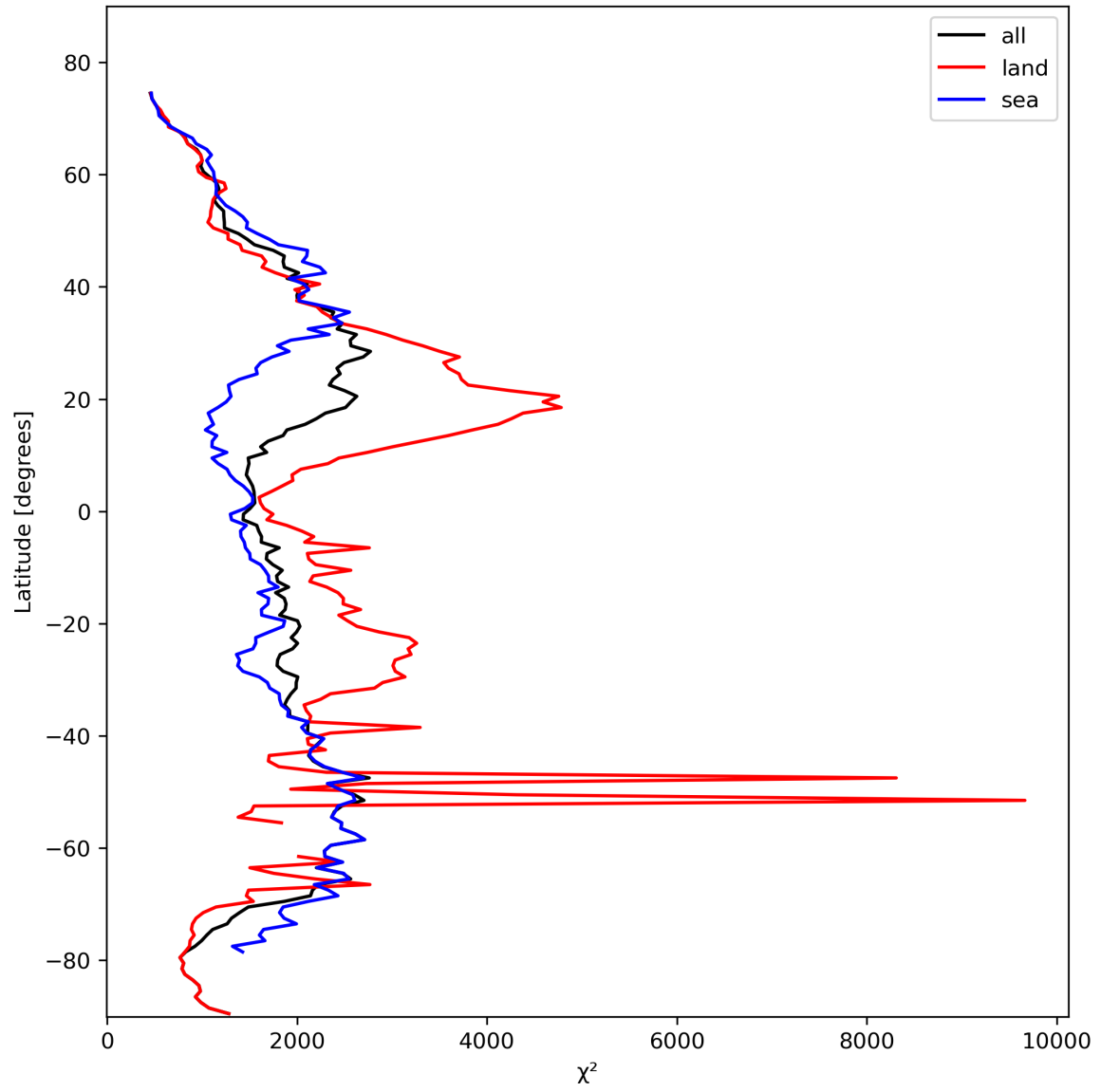
Figure 14: Zonal average of “ \chi^2 ” for 2024-02-19 to 2024-02-21.
