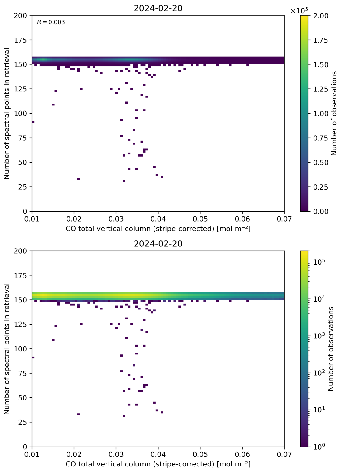
Figure 40: Scatter density plot of “CO total vertical column (stripe-corrected)” against “Number of spectral points in retrieval” for 2024-02-19 to 2024-02-21.
