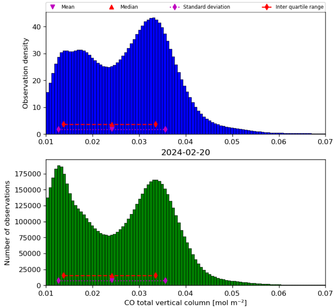
Figure 18: Histogram of “CO total vertical column” for 2024-02-19 to 2024-02-21
