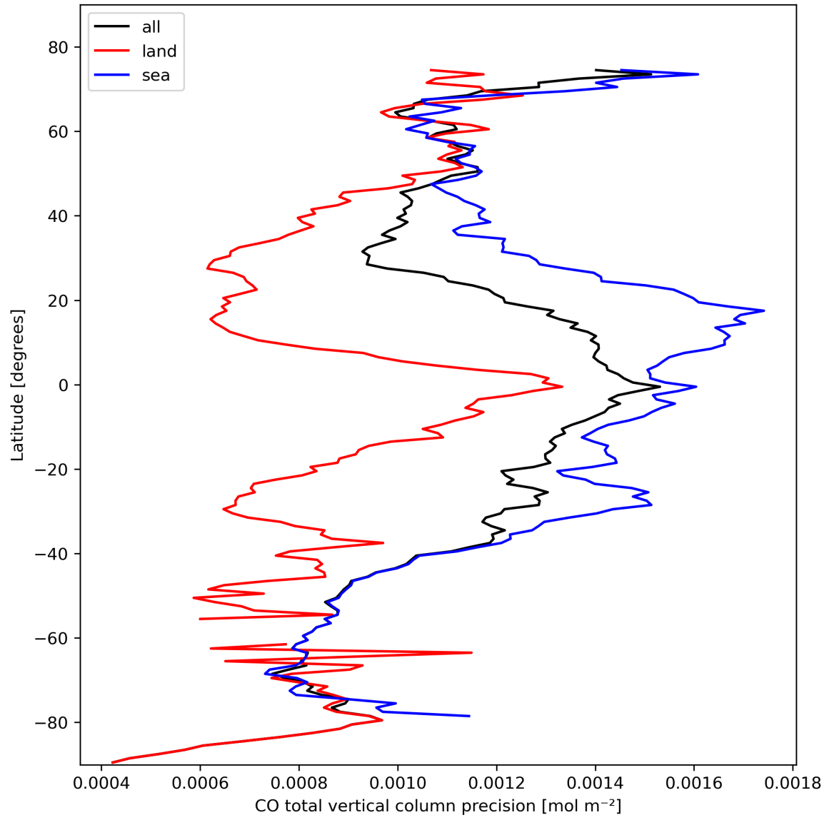
Figure 12: Zonal average of “CO total vertical column precision” for 2024-02-19 to 2024-02-21.
