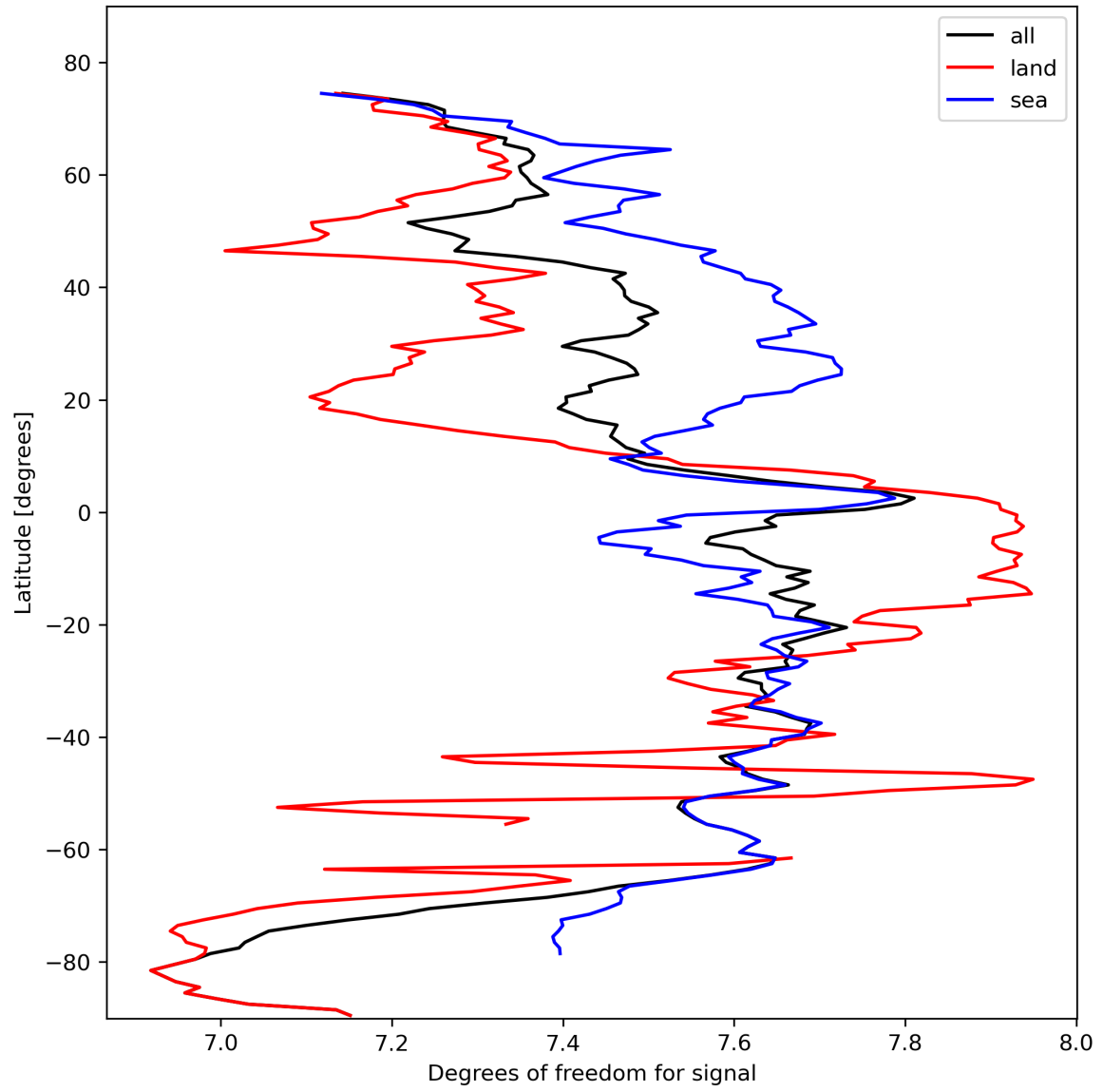
Figure 15: Zonal average of “Degrees of freedom for signal” for 2024-02-19 to 2024-02-21.
