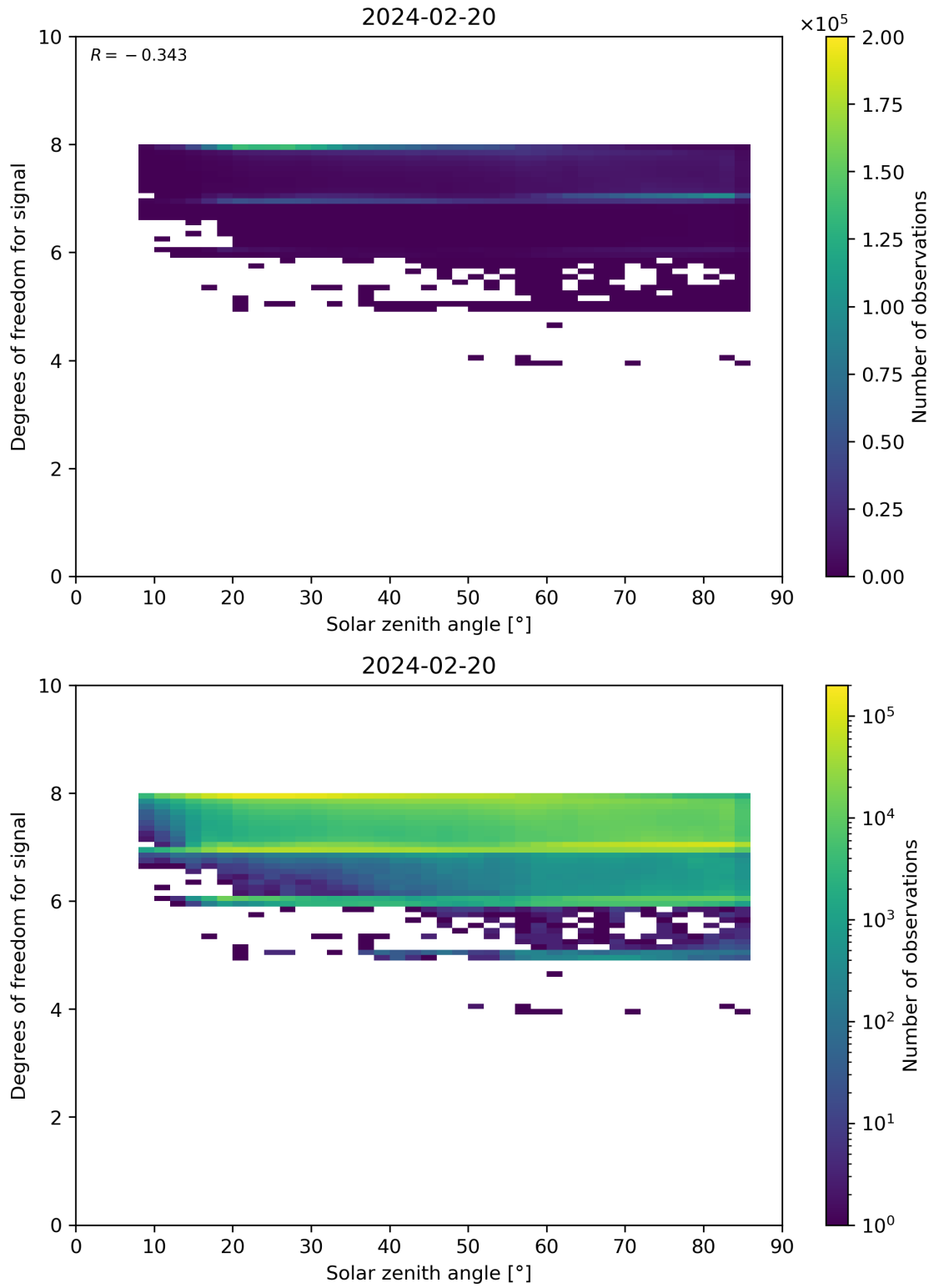
Figure 65: Scatter density plot of “Solar zenith angle” against “Degrees of freedom for signal” for 2024-02-19 to 2024-02-21.
