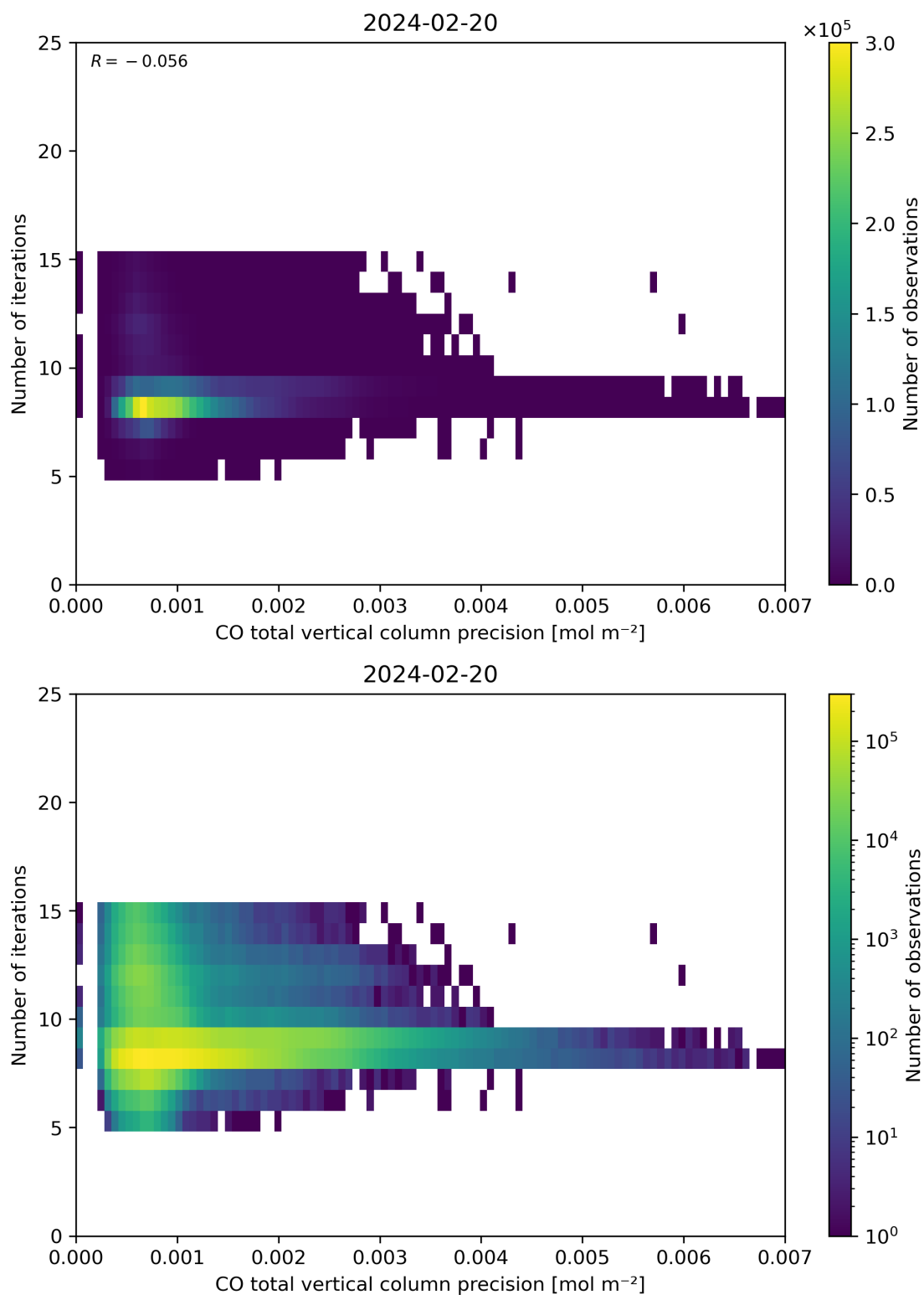
Figure 46: Scatter density plot of “CO total vertical column precision” against “Number of iterations” for 2024-02-19 to 2024-02-21.
