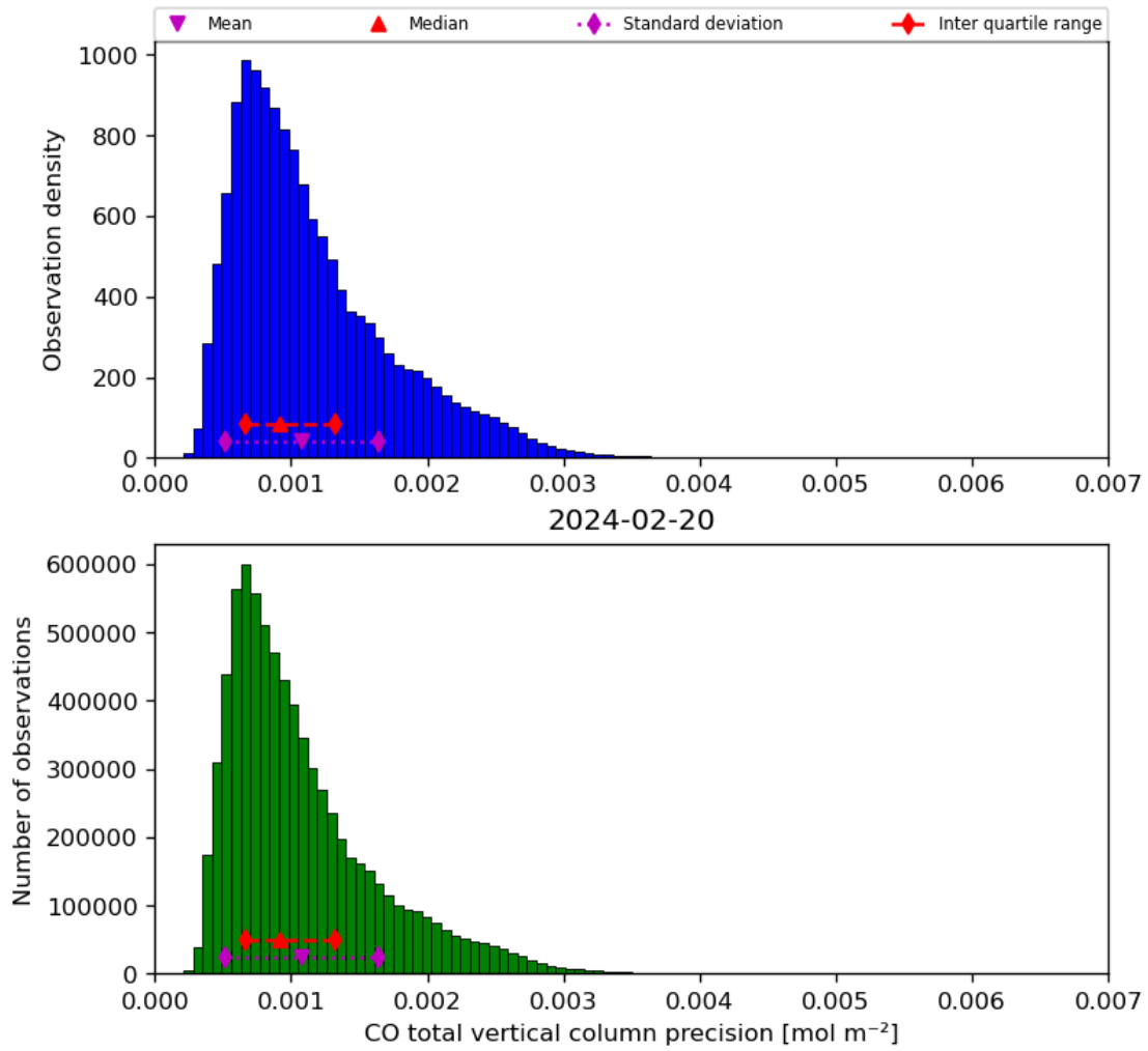
Figure 20: Histogram of “CO total vertical column precision” for 2024-02-19 to 2024-02-21
