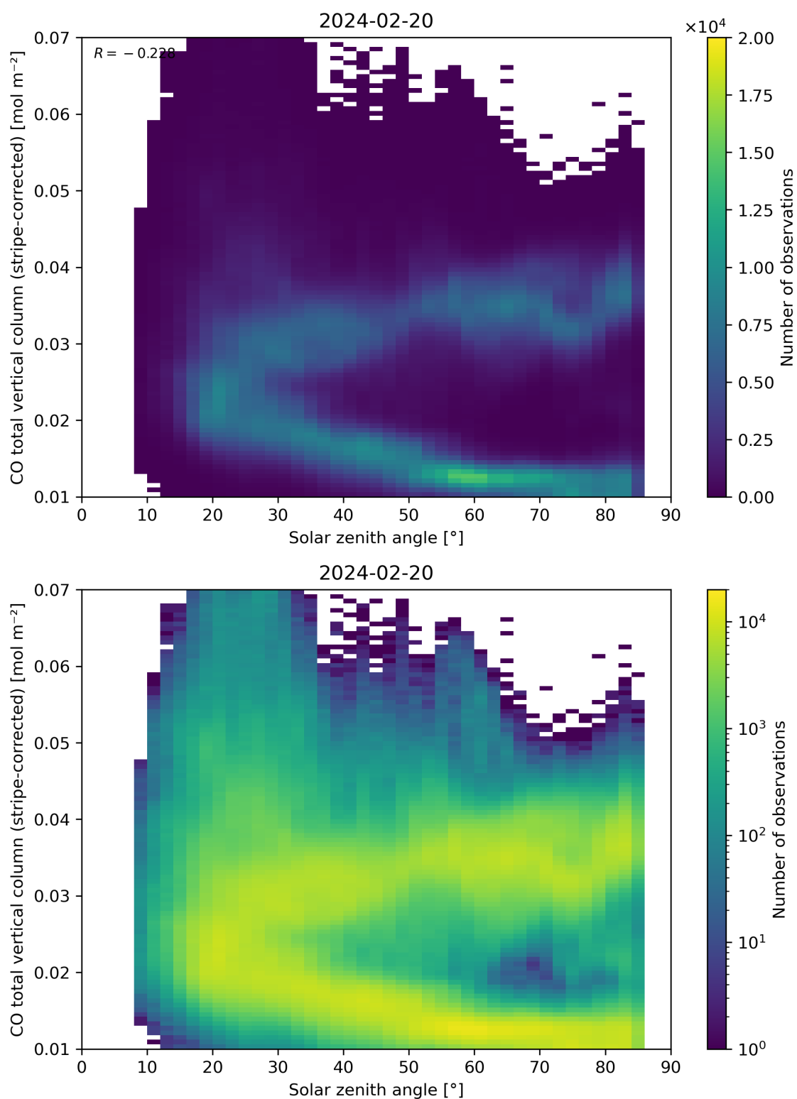
Figure 62: Scatter density plot of “Solar zenith angle” against “CO total vertical column (stripe-corrected)” for 2024-02-19 to 2024-02-21.
