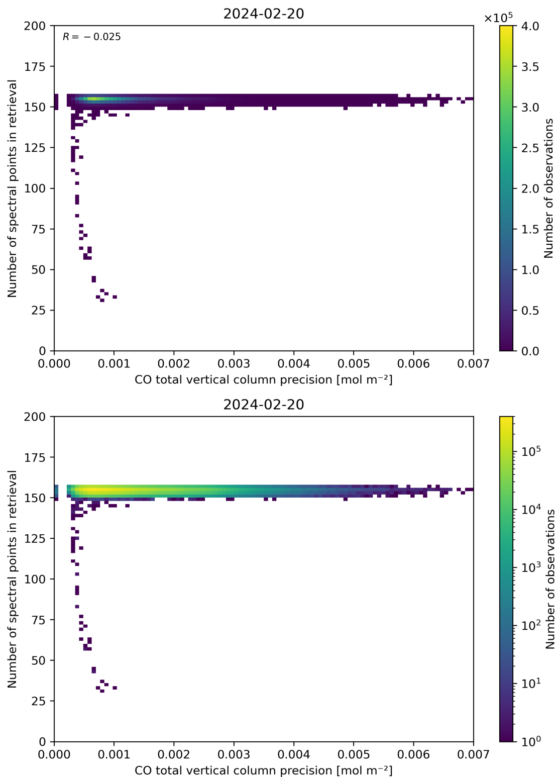
Figure 47: Scatter density plot of “CO total vertical column precision” against “Number of spectral points in retrieval” for 2024-02-19 to 2024-02-21.
