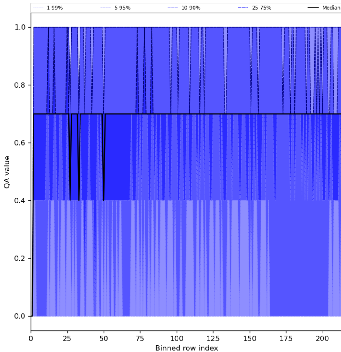
Figure 25: Along track statistics of “QA value” for 2024-02-19 to 2024-02-21
