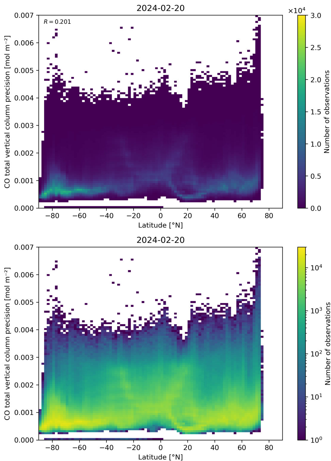
Figure 53: Scatter density plot of “Latitude” against “CO total vertical column precision” for 2024-02-19 to 2024-02-21.
