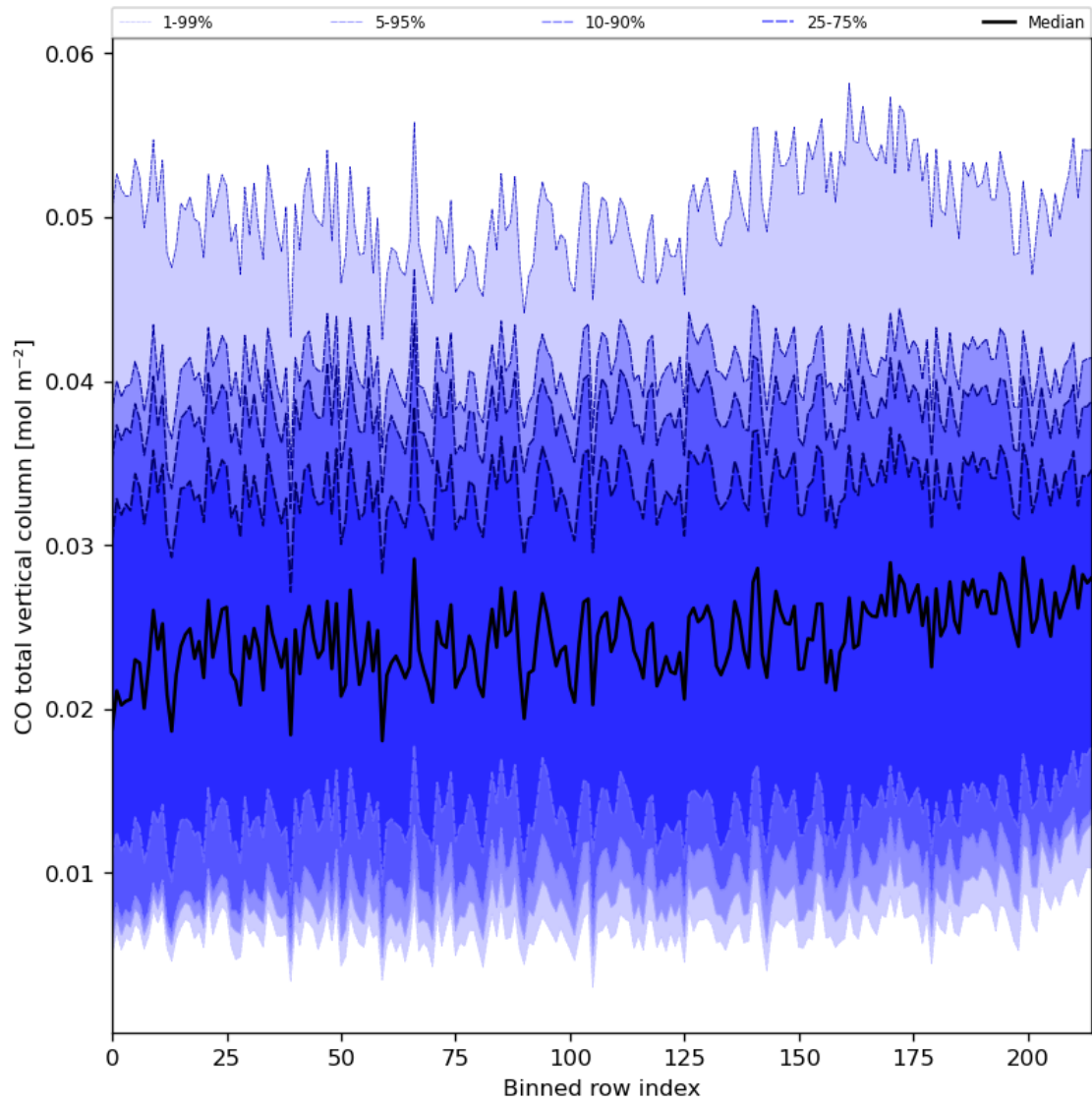
Figure 26: Along track statistics of “CO total vertical column” for 2024-02-19 to 2024-02-21
