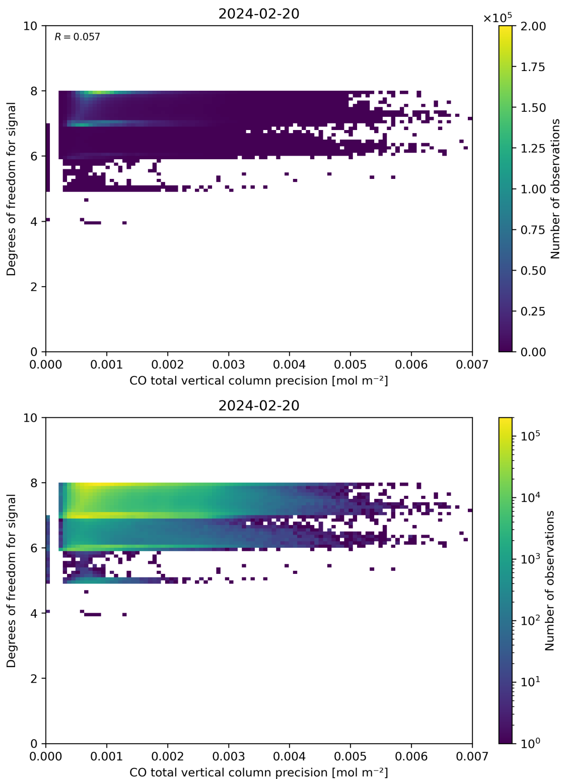
Figure 45: Scatter density plot of “CO total vertical column precision” against “Degrees of freedom for signal” for 2024-02-19 to 2024-02-21.
