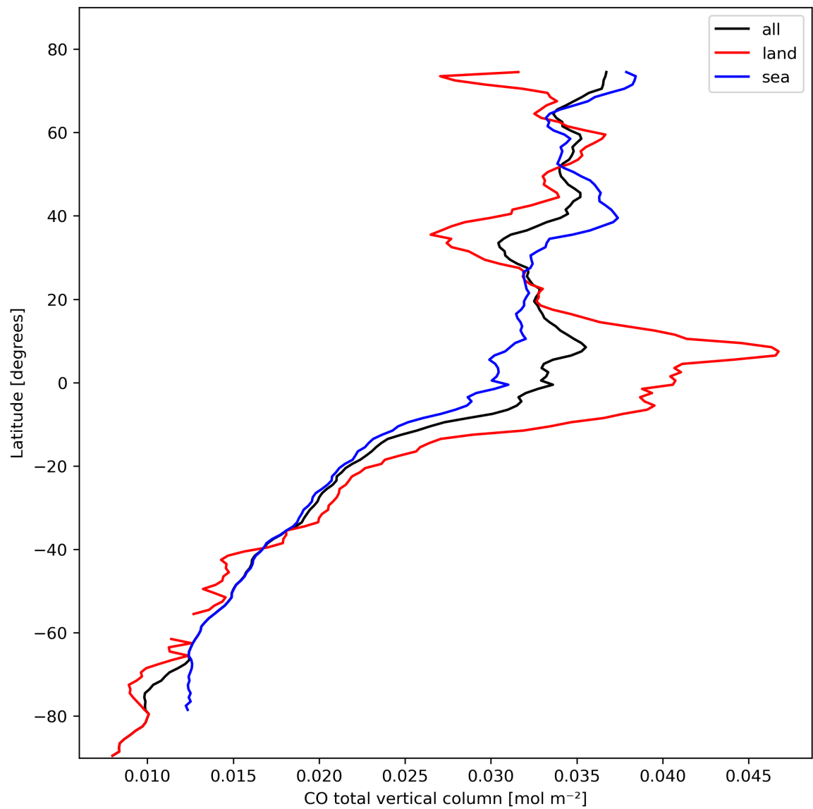
Figure 10: Zonal average of “CO total vertical column” for 2024-02-19 to 2024-02-21.
