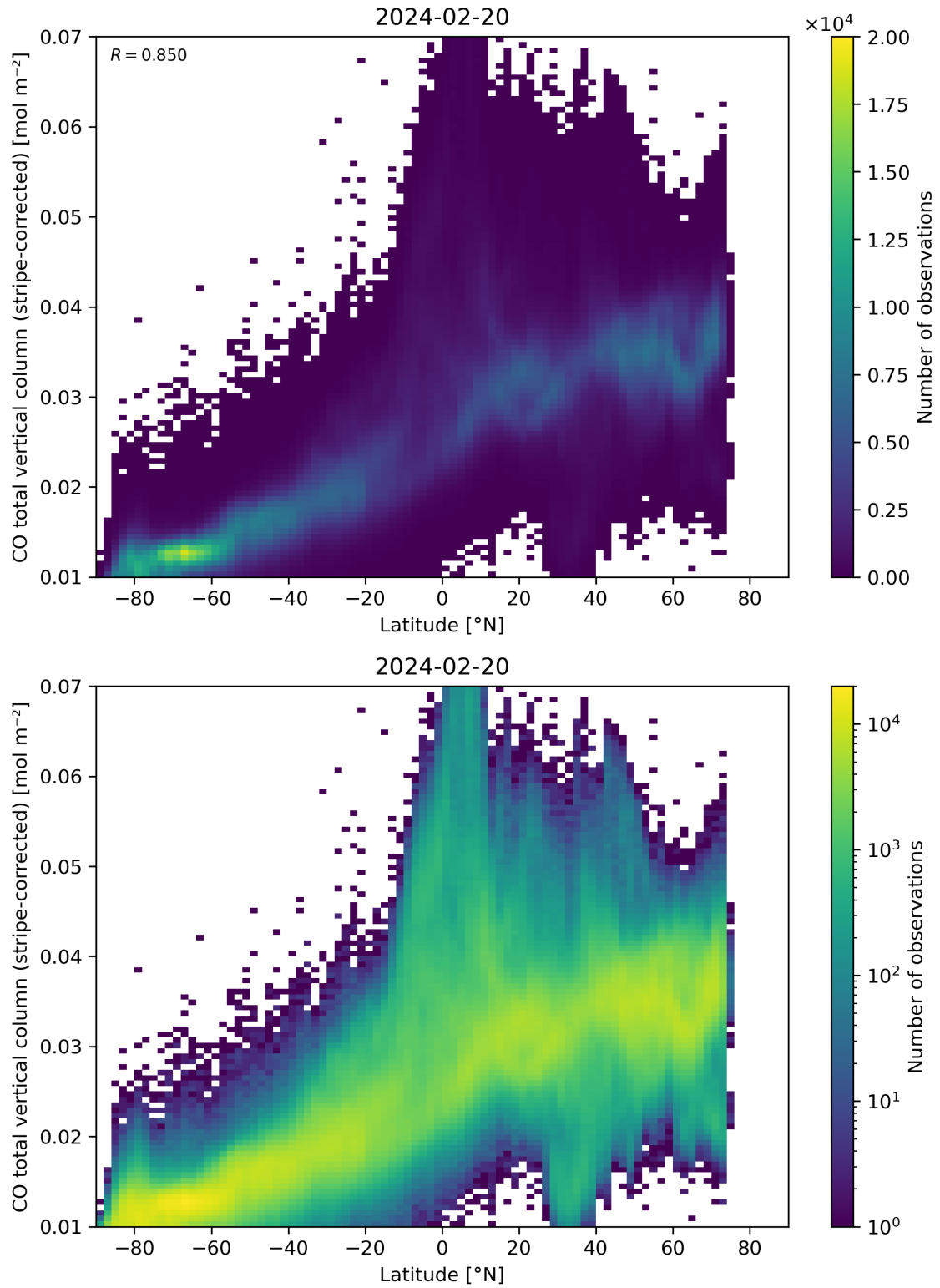
Figure 52: Scatter density plot of “Latitude” against “CO total vertical column (stripe-corrected)” for 2024-02-19 to 2024-02-21.
