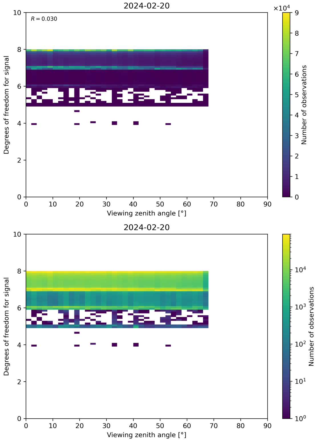
Figure 73: Scatter density plot of “Viewing zenith angle” against “Degrees of freedom for signal” for 2024-02-19 to 2024-02-21.
