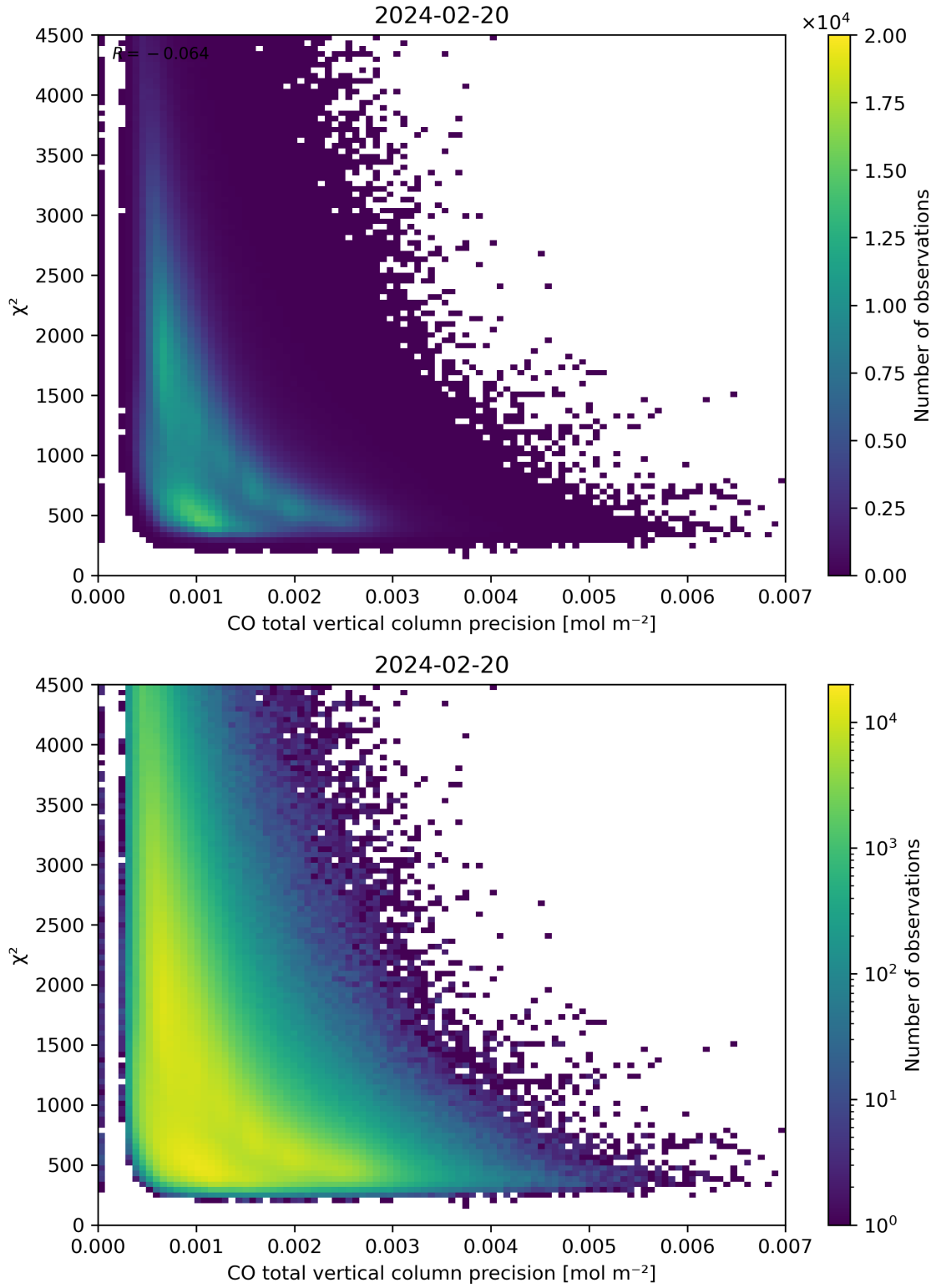
Figure 44: Scatter density plot of “CO total vertical column precision” against “ \chi^2 ” for 2024-02-19 to 2024-02-21.
