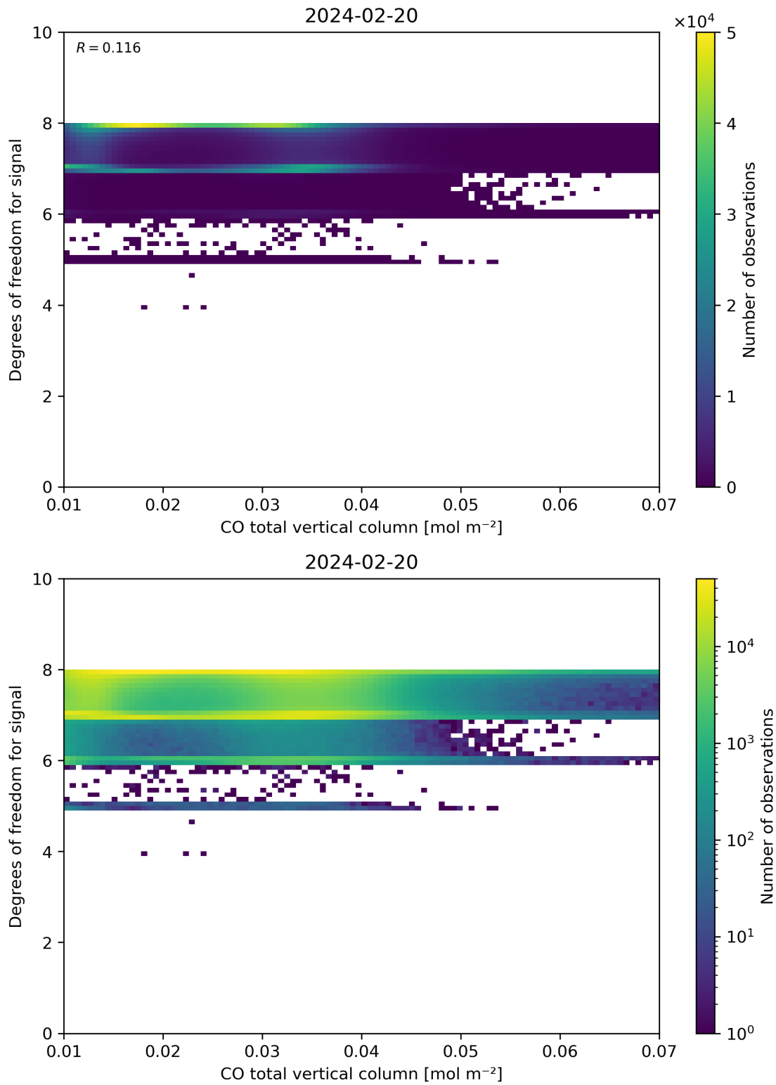
Figure 41: Scatter density plot of “CO total vertical column” against “Degrees of freedom for signal” for 2024-02-19 to 2024-02-21.
