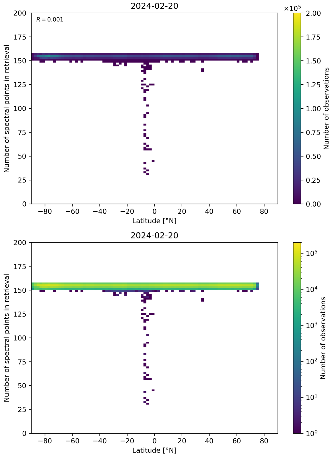
Figure 57: Scatter density plot of “Latitude” against “Number of spectral points in retrieval” for 2024-02-19 to 2024-02-21.
