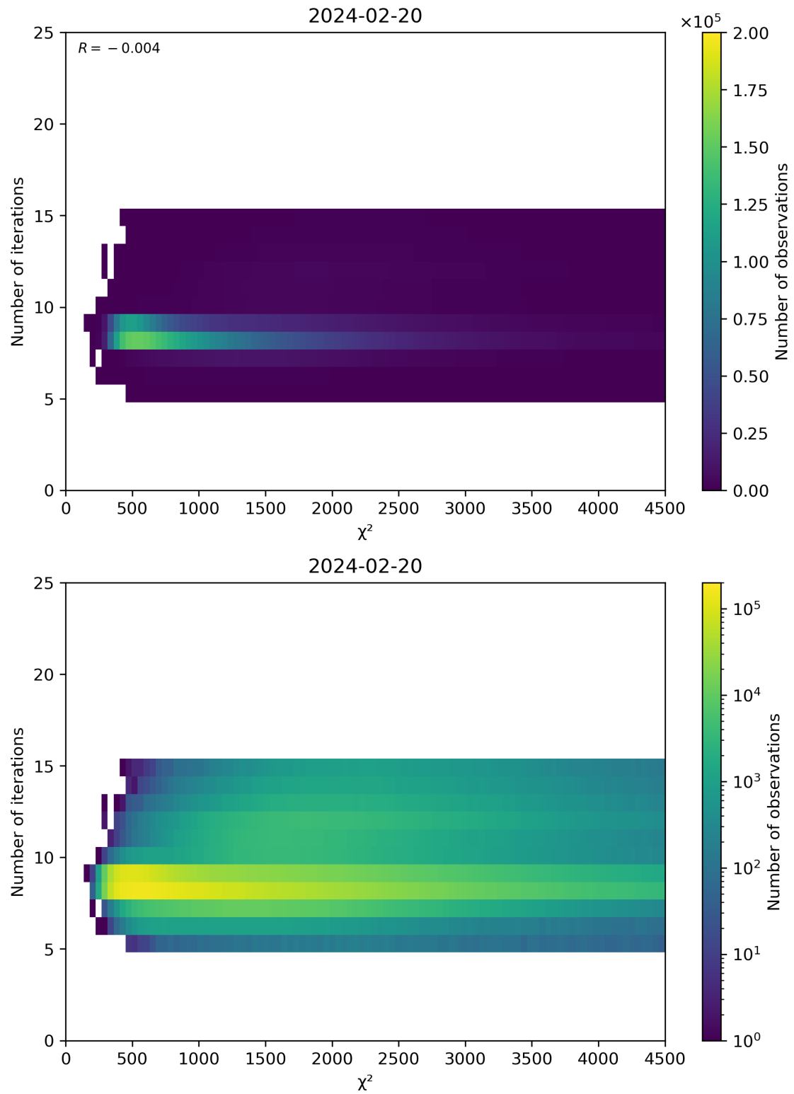
Figure 49: Scatter density plot of “ \chi^2 ” against “Number of iterations” for 2024-02-19 to 2024-02-21.
