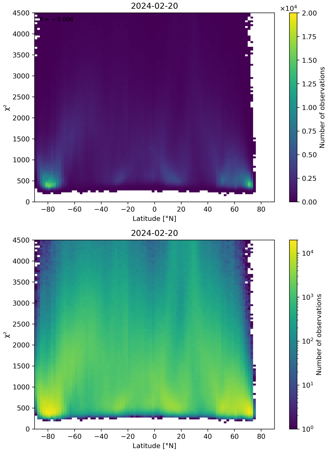
Figure 54: Scatter density plot of “Latitude” against “ \chi^2 ” for 2024-02-19 to 2024-02-21.
