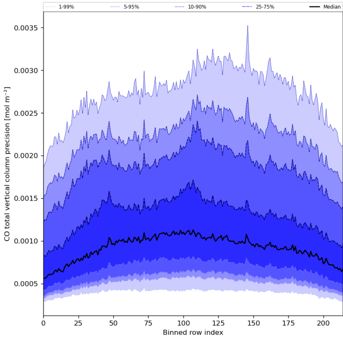
Figure 28: Along track statistics of “CO total vertical column precision” for 2024-02-19 to 2024-02-21
