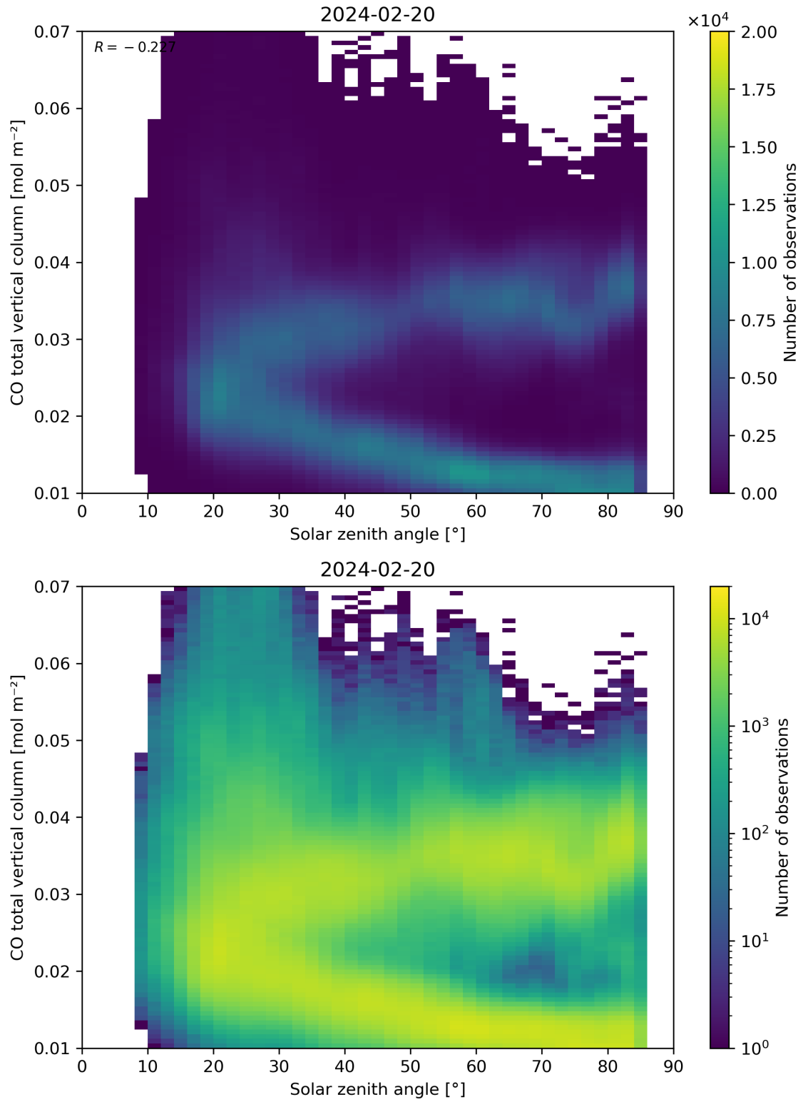
Figure 61: Scatter density plot of “Solar zenith angle” against “CO total vertical column” for 2024-02-19 to 2024-02-21.
