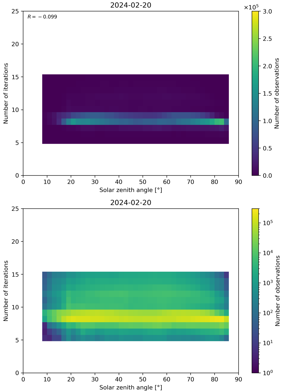
Figure 67: Scatter density plot of “Solar zenith angle” against “Number of iterations” for 2024-02-19 to 2024-02-21.
