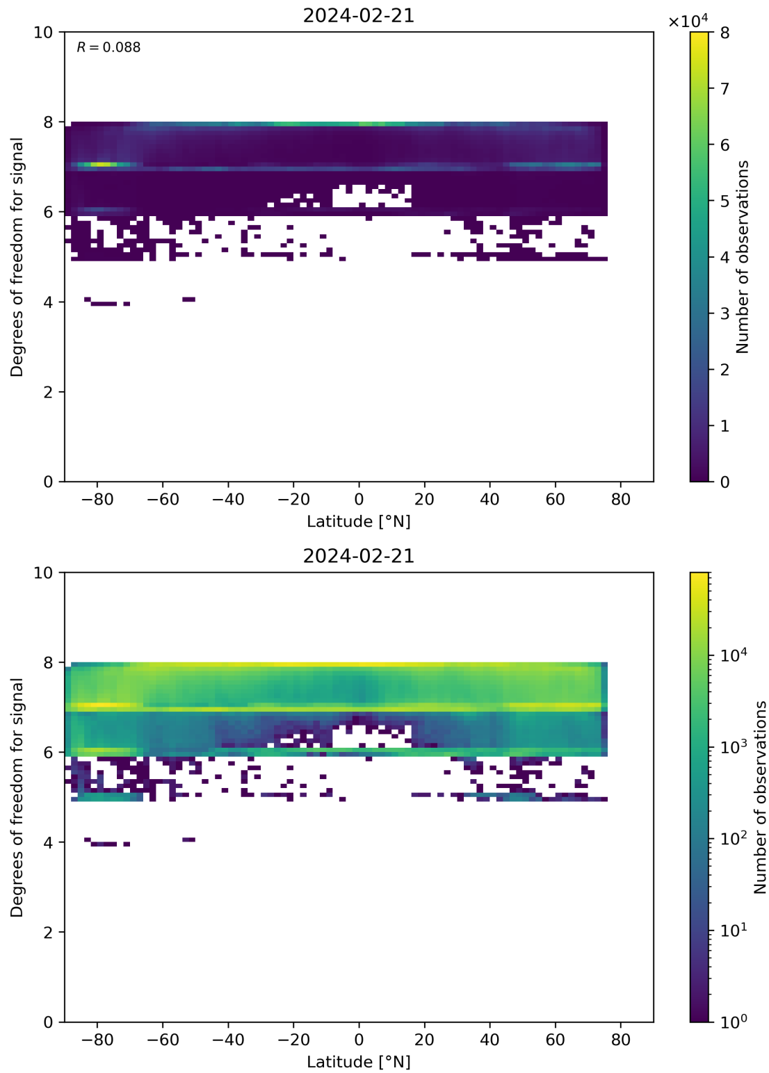
Figure 55: Scatter density plot of “Latitude” against “Degrees of freedom for signal” for 2024-02-20 to 2024-02-22.
