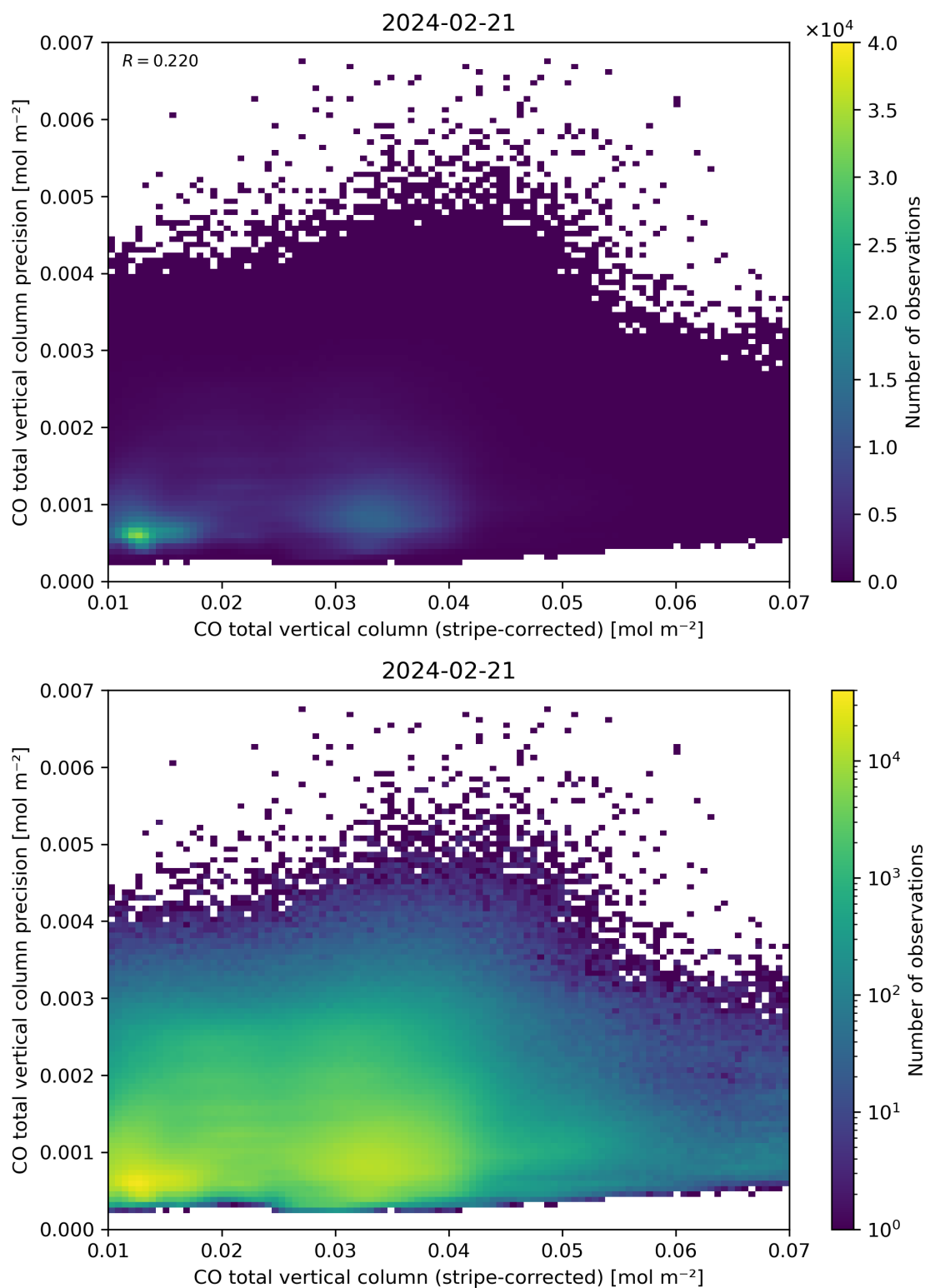
Figure 36: Scatter density plot of “CO total vertical column (stripe-corrected)” against “CO total vertical column precision” for 2024-02-20 to 2024-02-22.
