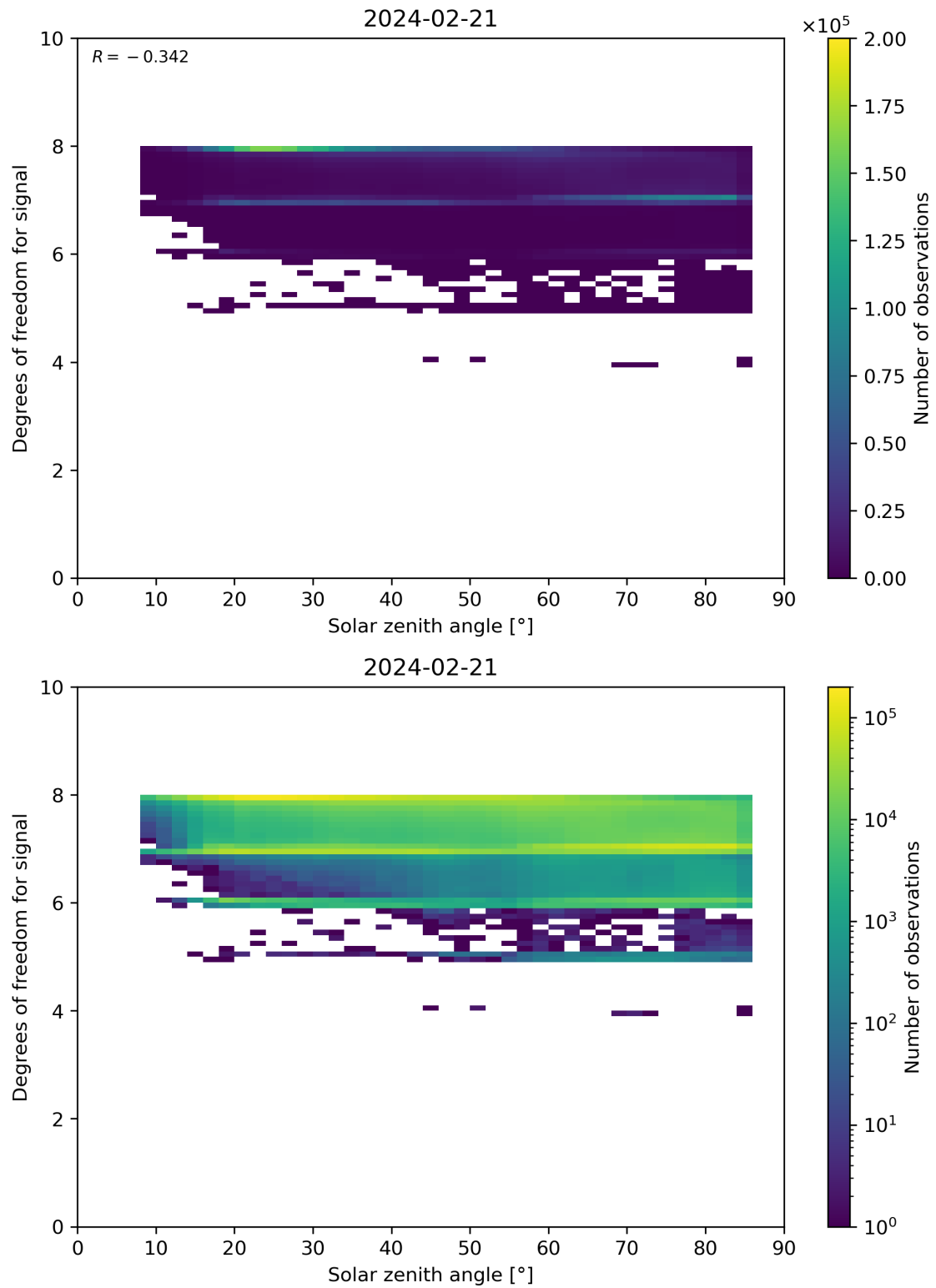
Figure 65: Scatter density plot of “Solar zenith angle” against “Degrees of freedom for signal” for 2024-02-20 to 2024-02-22.
