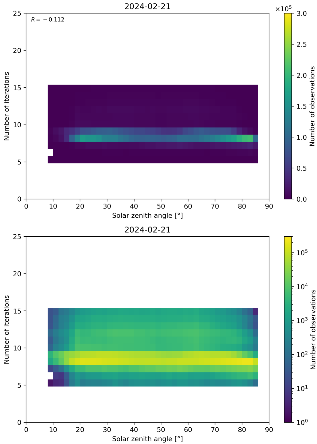
Figure 67: Scatter density plot of “Solar zenith angle” against “Number of iterations” for 2024-02-20 to 2024-02-22.
