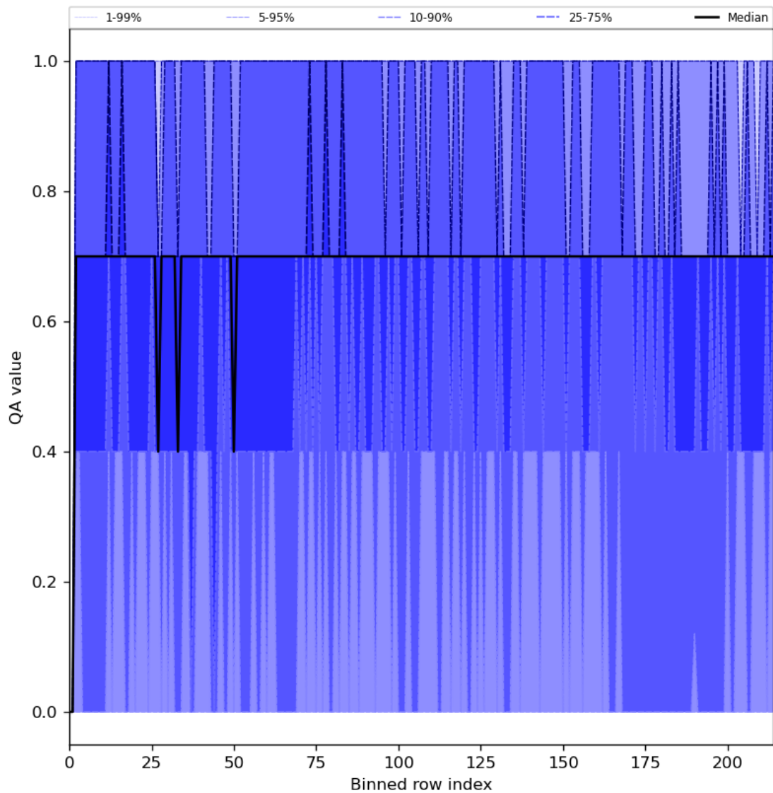
Figure 25: Along track statistics of “QA value” for 2024-02-20 to 2024-02-22
