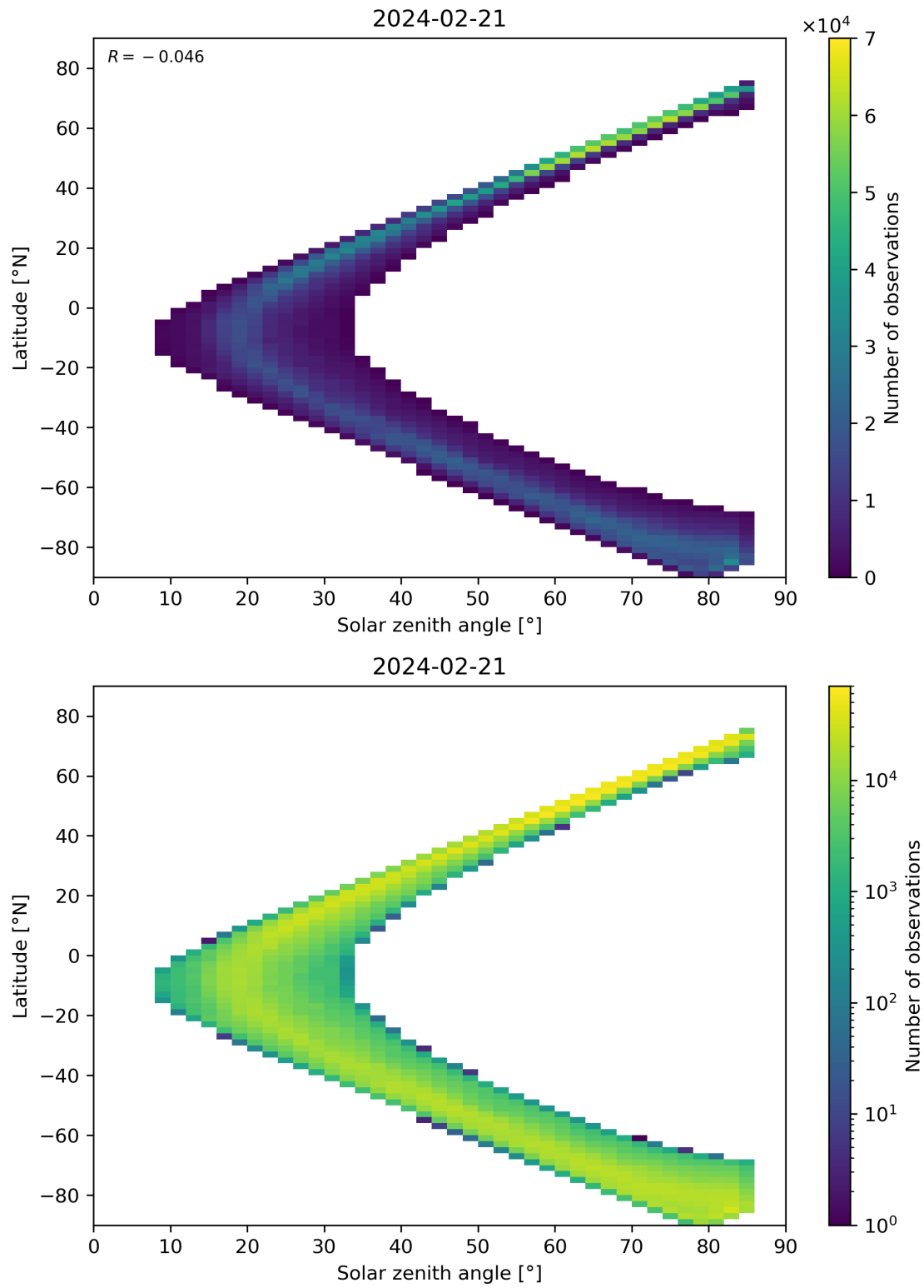
Figure 66: Scatter density plot of “Solar zenith angle” against “Latitude” for 2024-02-20 to 2024-02-22.
