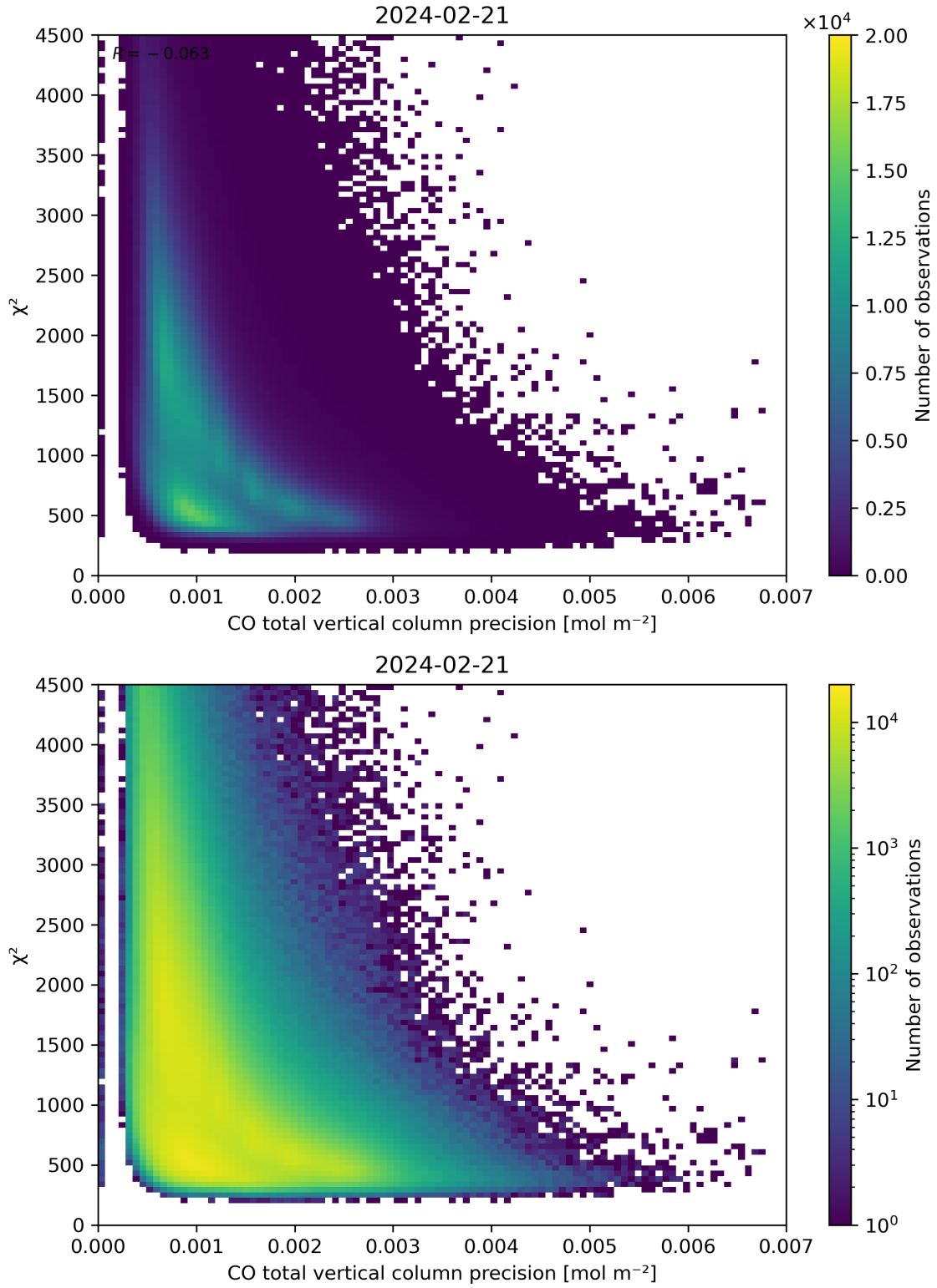
Figure 44: Scatter density plot of “CO total vertical column precision” against “ \chi^2 ” for 2024-02-20 to 2024-02-22.
