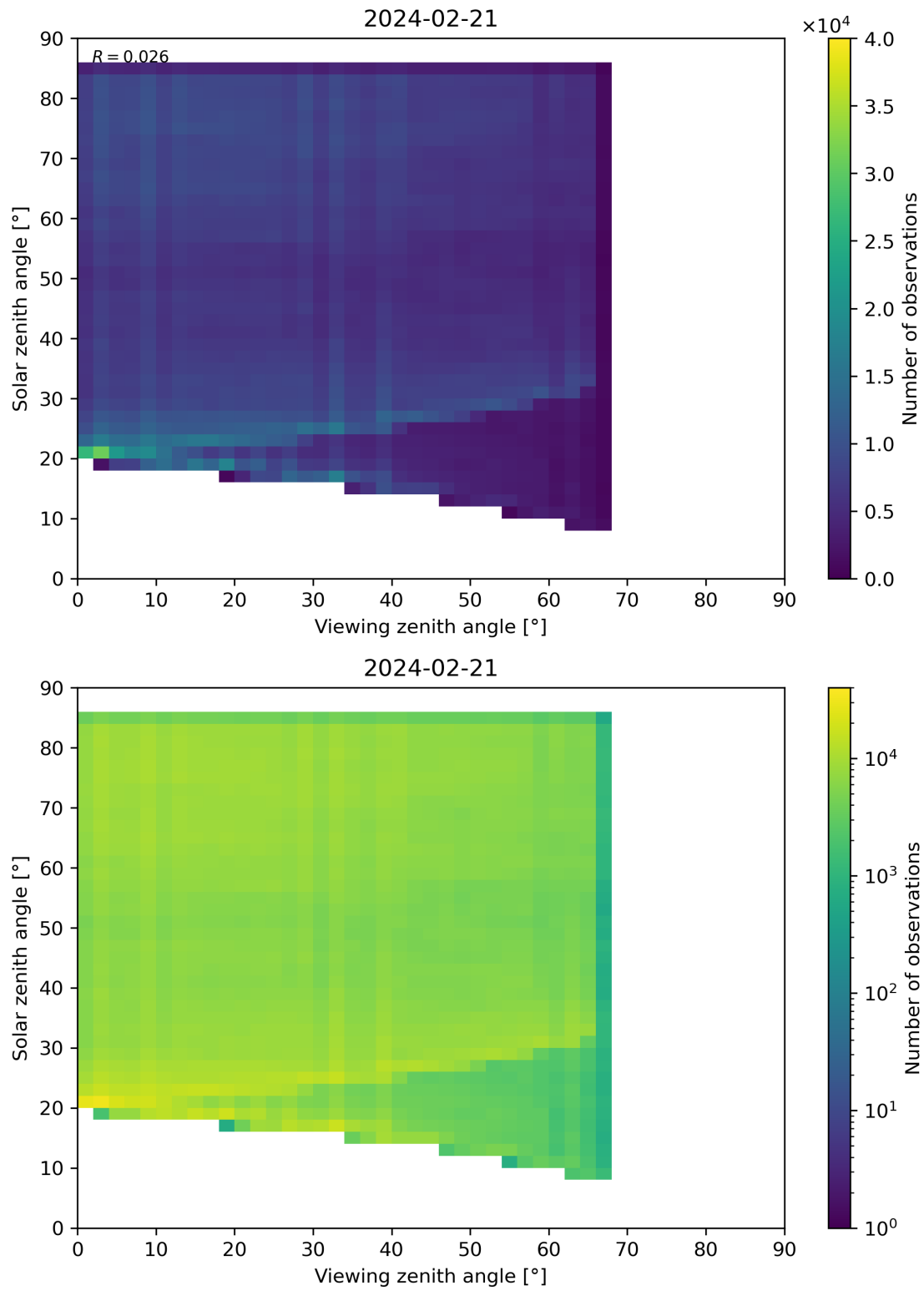
Figure 77: Scatter density plot of “Viewing zenith angle” against “Solar zenith angle” for 2024-02-20 to 2024-02-22.
