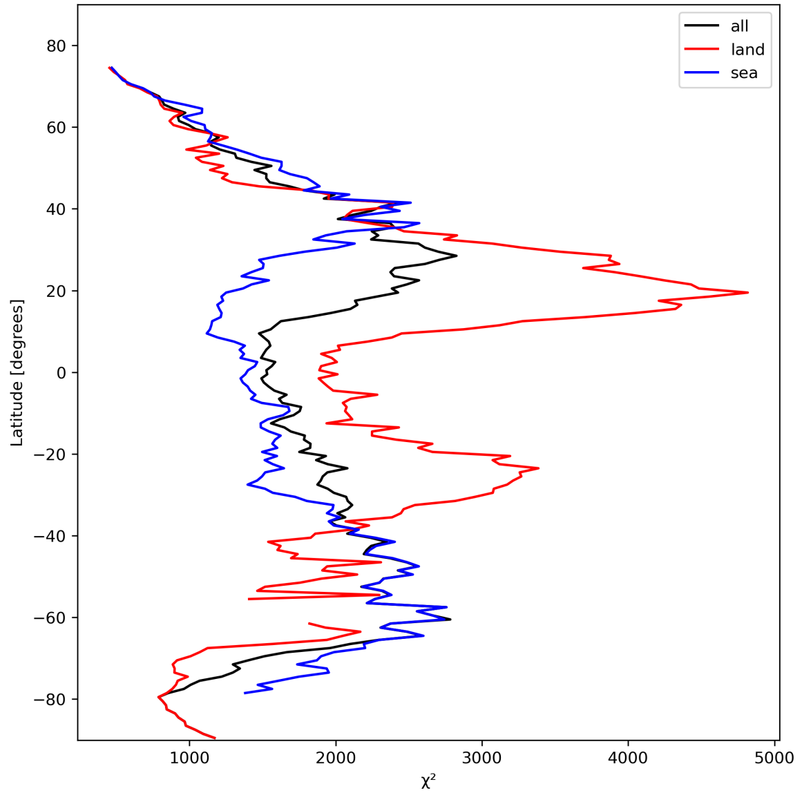
Figure 14: Zonal average of “ \chi^2 ” for 2024-02-20 to 2024-02-22.
