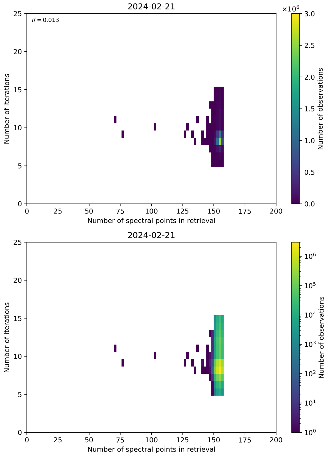
Figure 60: Scatter density plot of “Number of spectral points in retrieval” against “Number of iterations” for 2024-02-20 to 2024-02-22.
