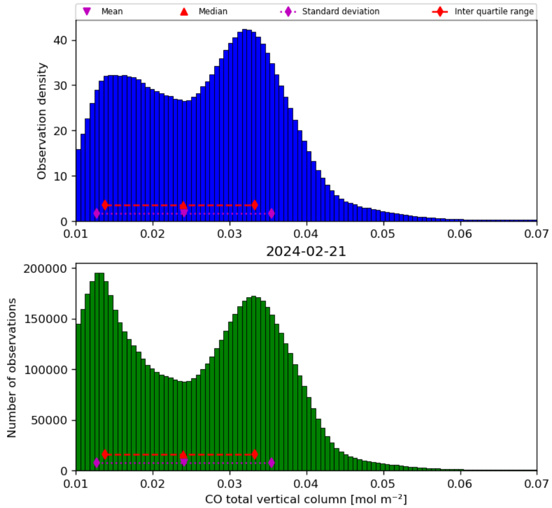
Figure 18: Histogram of “CO total vertical column” for 2024-02-20 to 2024-02-22
