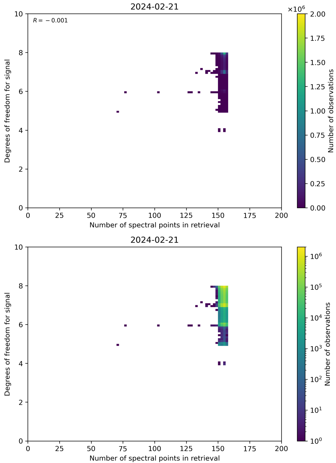
Figure 59: Scatter density plot of “Number of spectral points in retrieval” against “Degrees of freedom for signal” for 2024-02-20 to 2024-02-22.
