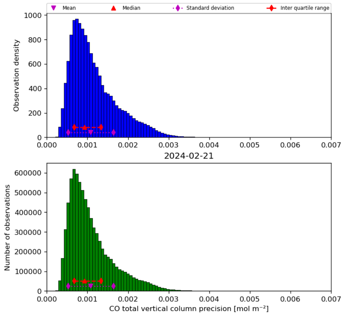
Figure 20: Histogram of “CO total vertical column precision” for 2024-02-20 to 2024-02-22
