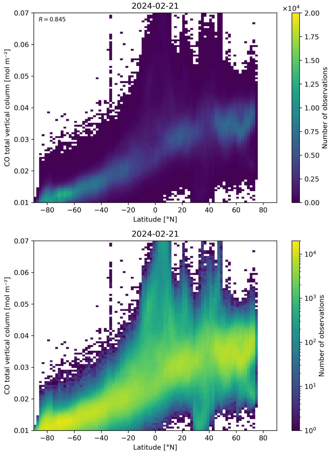
Figure 51: Scatter density plot of “Latitude” against “CO total vertical column” for 2024-02-20 to 2024-02-22.
