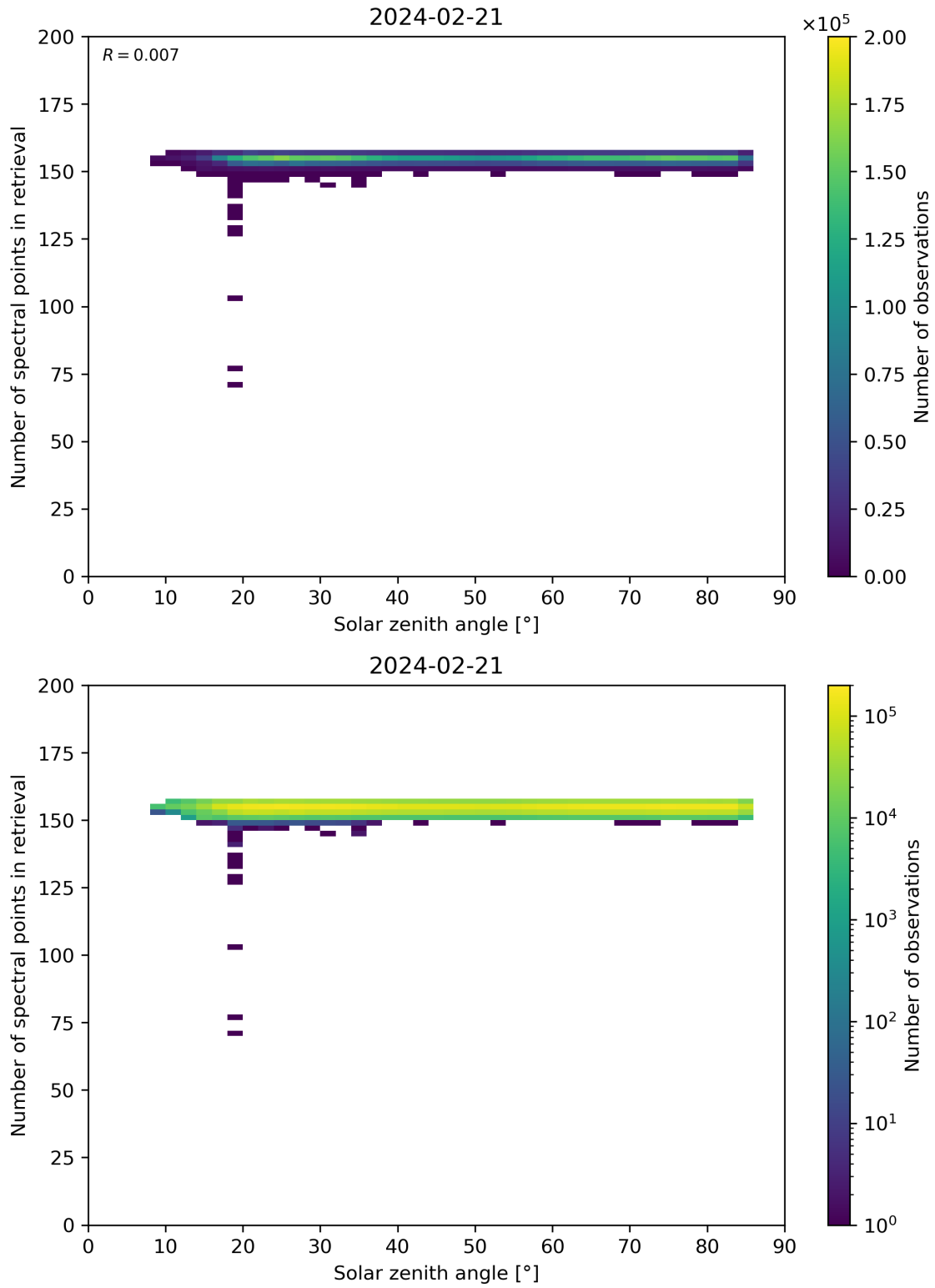
Figure 68: Scatter density plot of “Solar zenith angle” against “Number of spectral points in retrieval” for 2024-02-20 to 2024-02-22.
