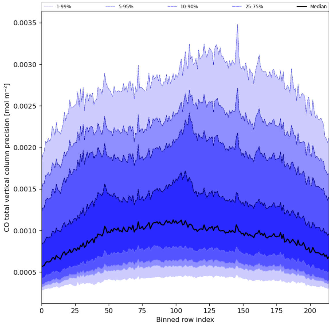
Figure 28: Along track statistics of “CO total vertical column precision” for 2024-02-20 to 2024-02-22
