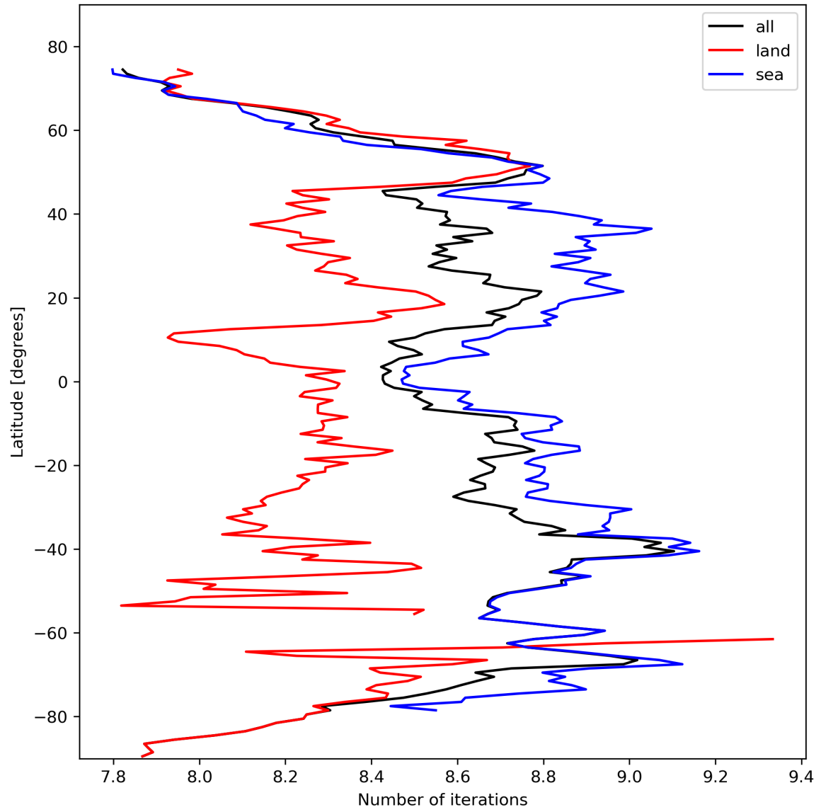
Figure 16: Zonal average of “Number of iterations” for 2024-02-20 to 2024-02-22.
