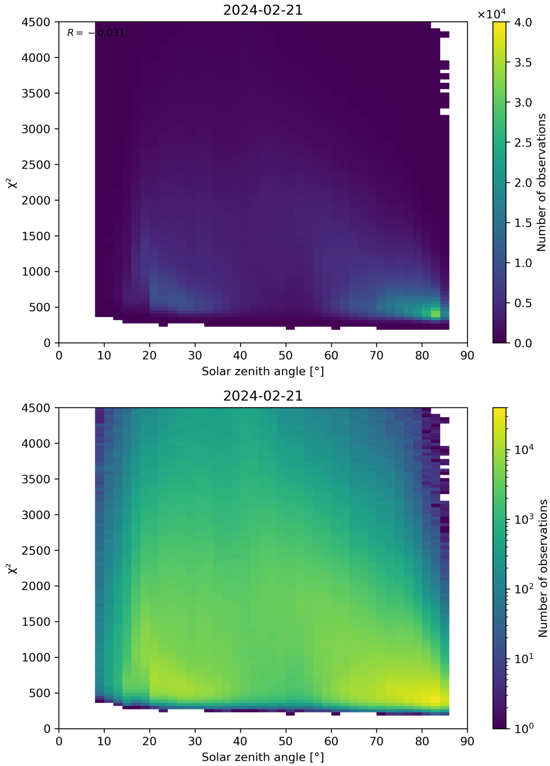
Figure 64: Scatter density plot of “Solar zenith angle” against “ \chi^2 ” for 2024-02-20 to 2024-02-22.
