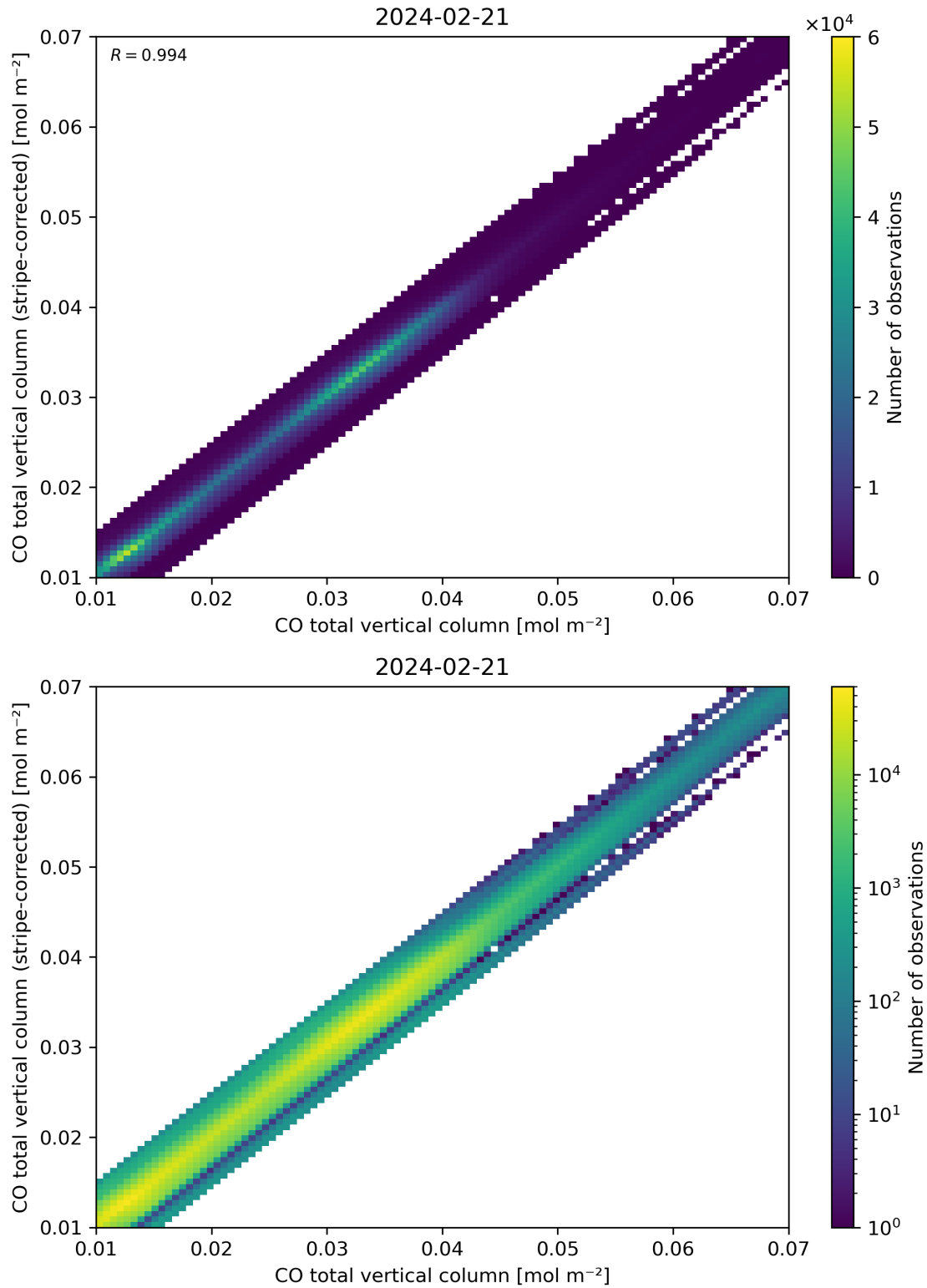
Figure 33: Scatter density plot of “CO total vertical column” against “CO total vertical column (stripe-corrected)” for 2024-02-20 to 2024-02-22.
