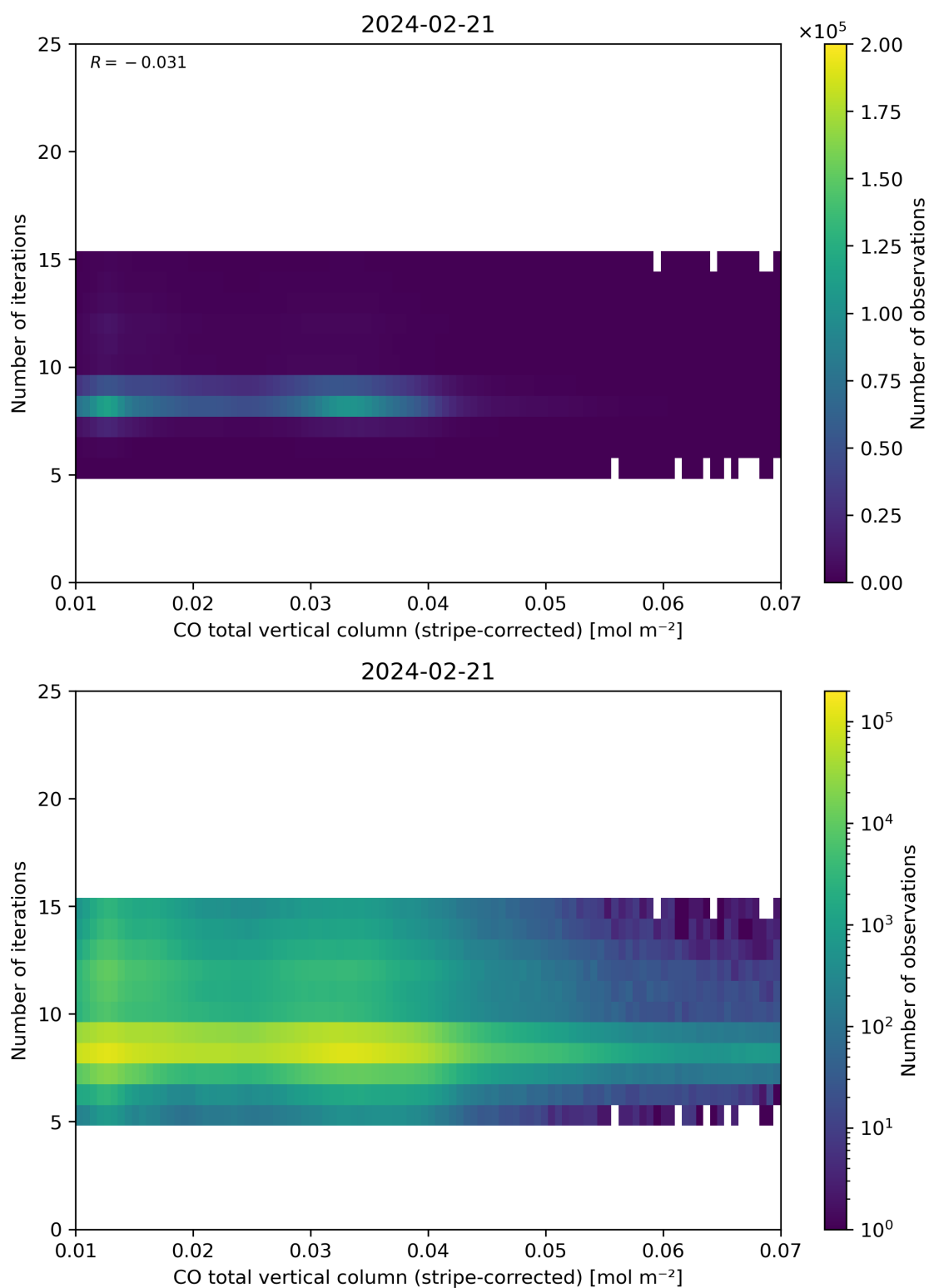
Figure 39: Scatter density plot of “CO total vertical column (stripe-corrected)” against “Number of iterations” for 2024-02-20 to 2024-02-22.
