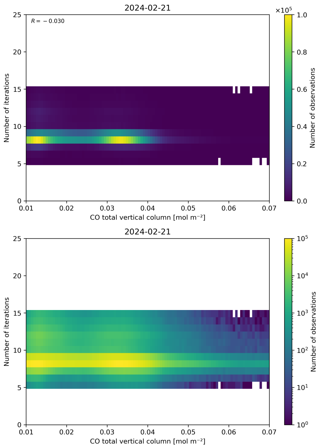
Figure 42: Scatter density plot of “CO total vertical column” against “Number of iterations” for 2024-02-20 to 2024-02-22.
