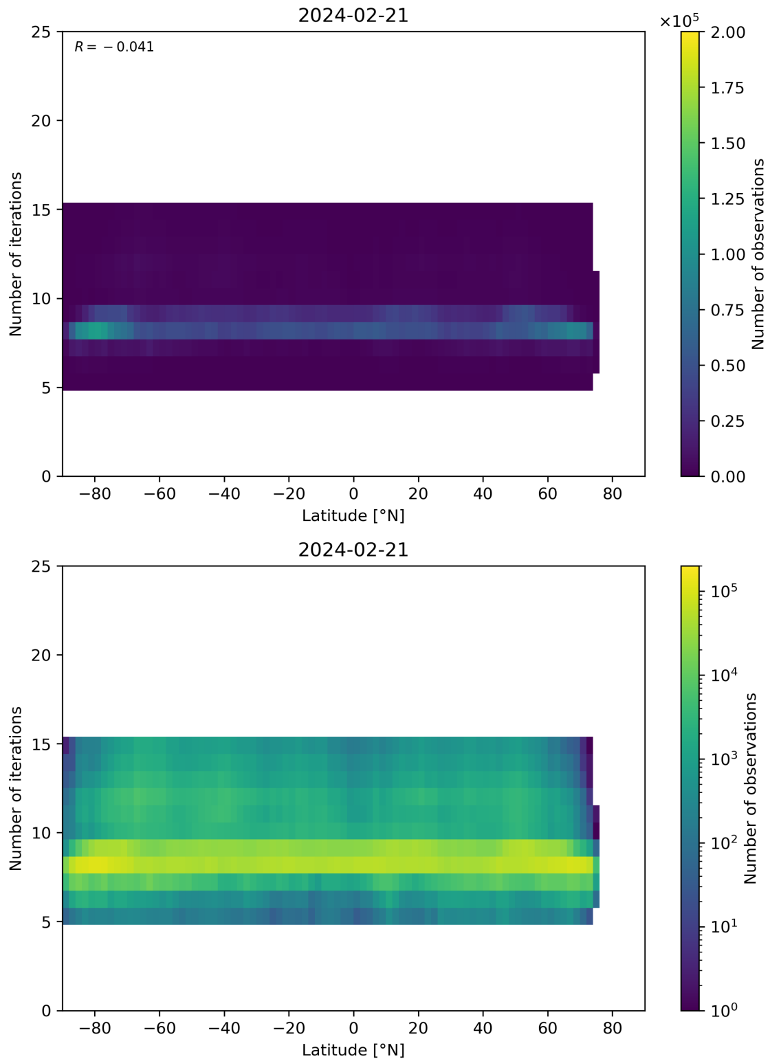
Figure 56: Scatter density plot of “Latitude” against “Number of iterations” for 2024-02-20 to 2024-02-22.
