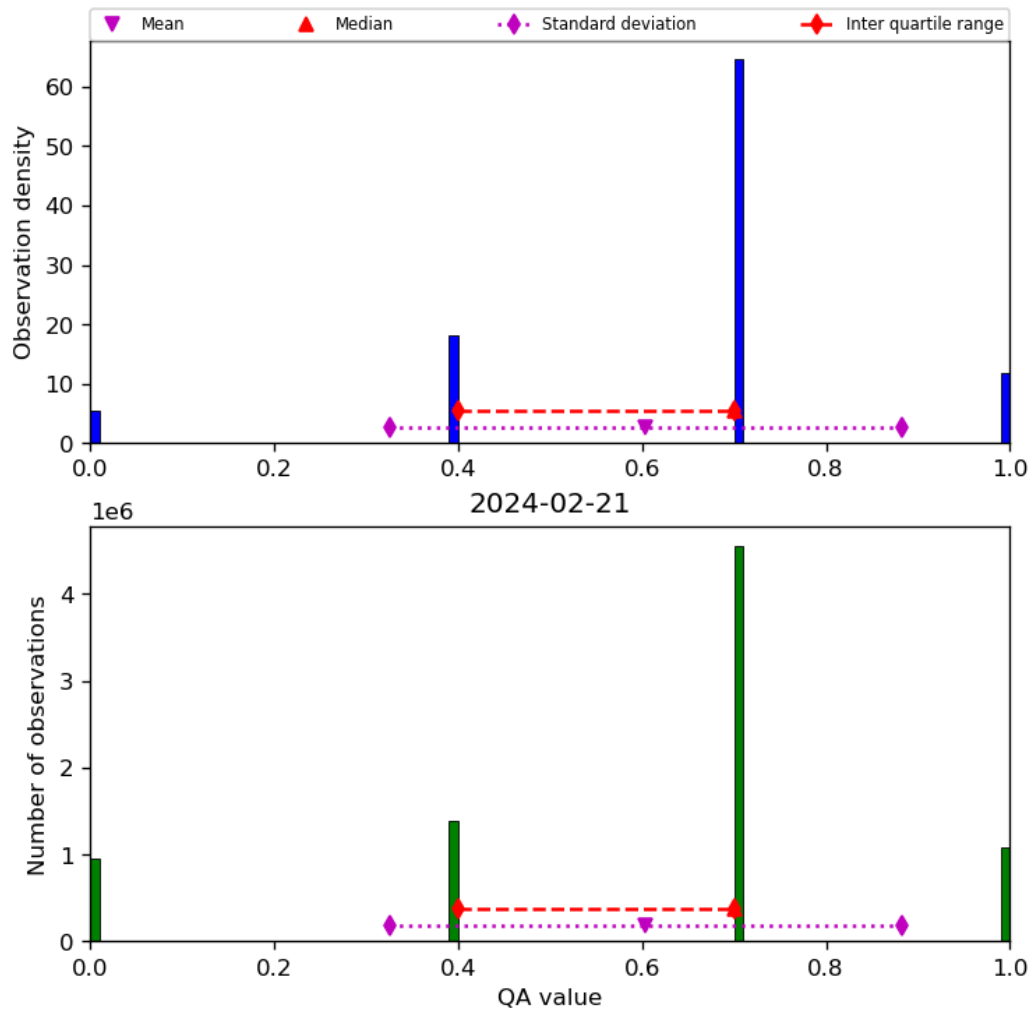
Figure 17: Histogram of “QA value” for 2024-02-20 to 2024-02-22
