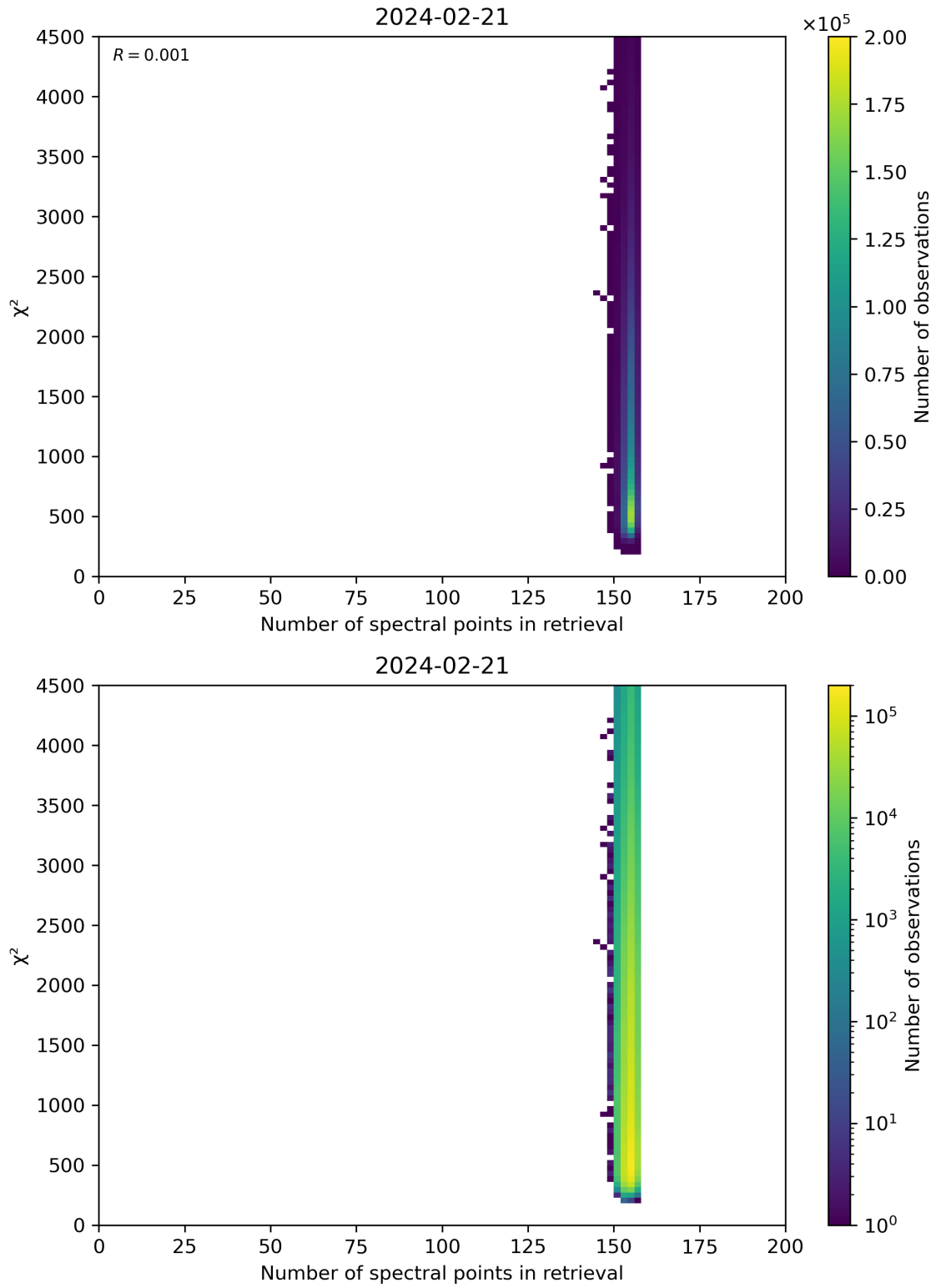
Figure 58: Scatter density plot of “Number of spectral points in retrieval” against “ \chi^2 ” for 2024-02-20 to 2024-02-22.
