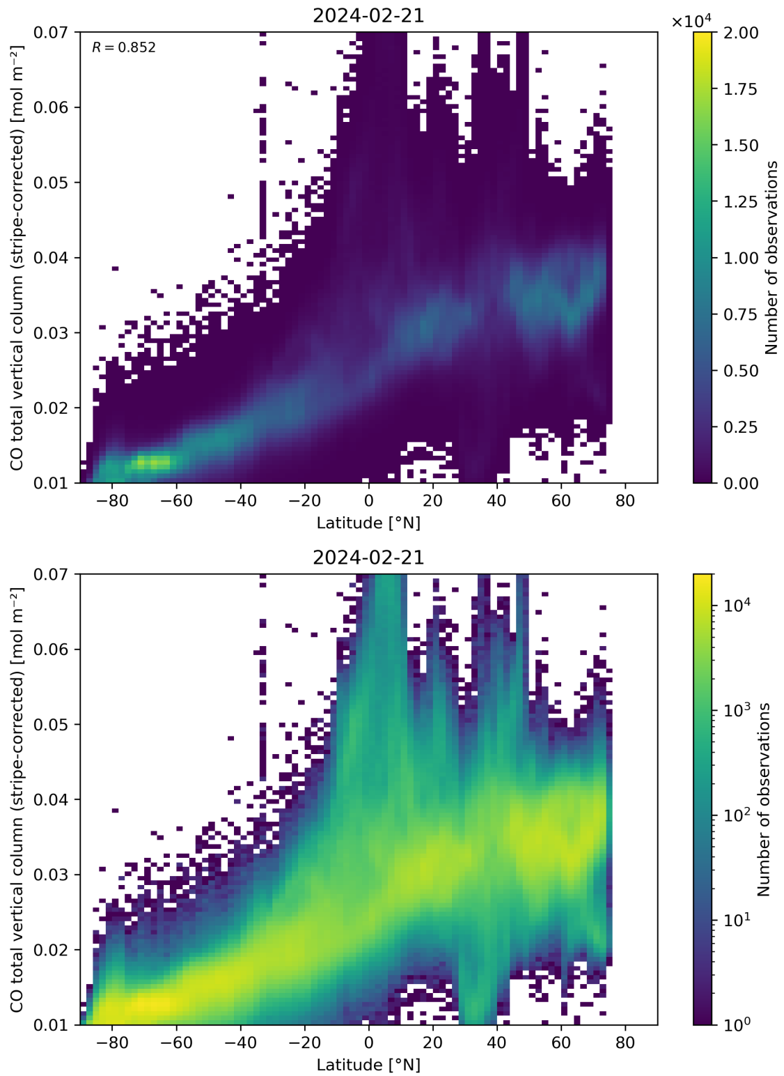
Figure 52: Scatter density plot of “Latitude” against “CO total vertical column (stripe-corrected)” for 2024-02-20 to 2024-02-22.
