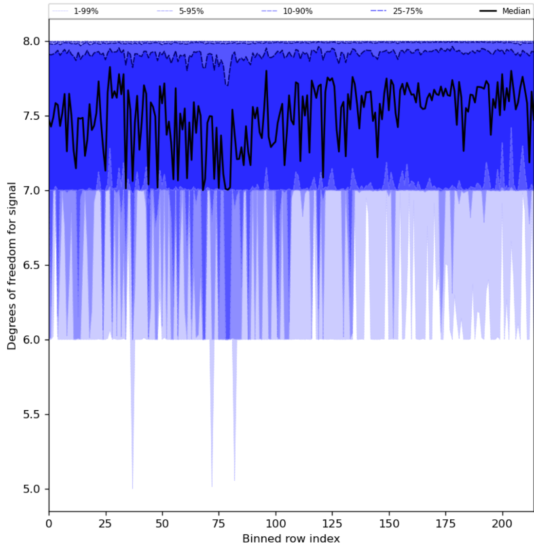
Figure 31: Along track statistics of “Degrees of freedom for signal” for 2024-02-20 to 2024-02-22
