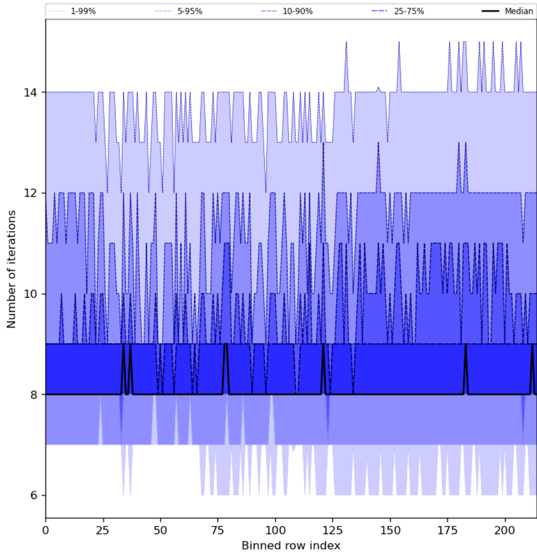
Figure 32: Along track statistics of “Number of iterations” for 2024-02-20 to 2024-02-22
