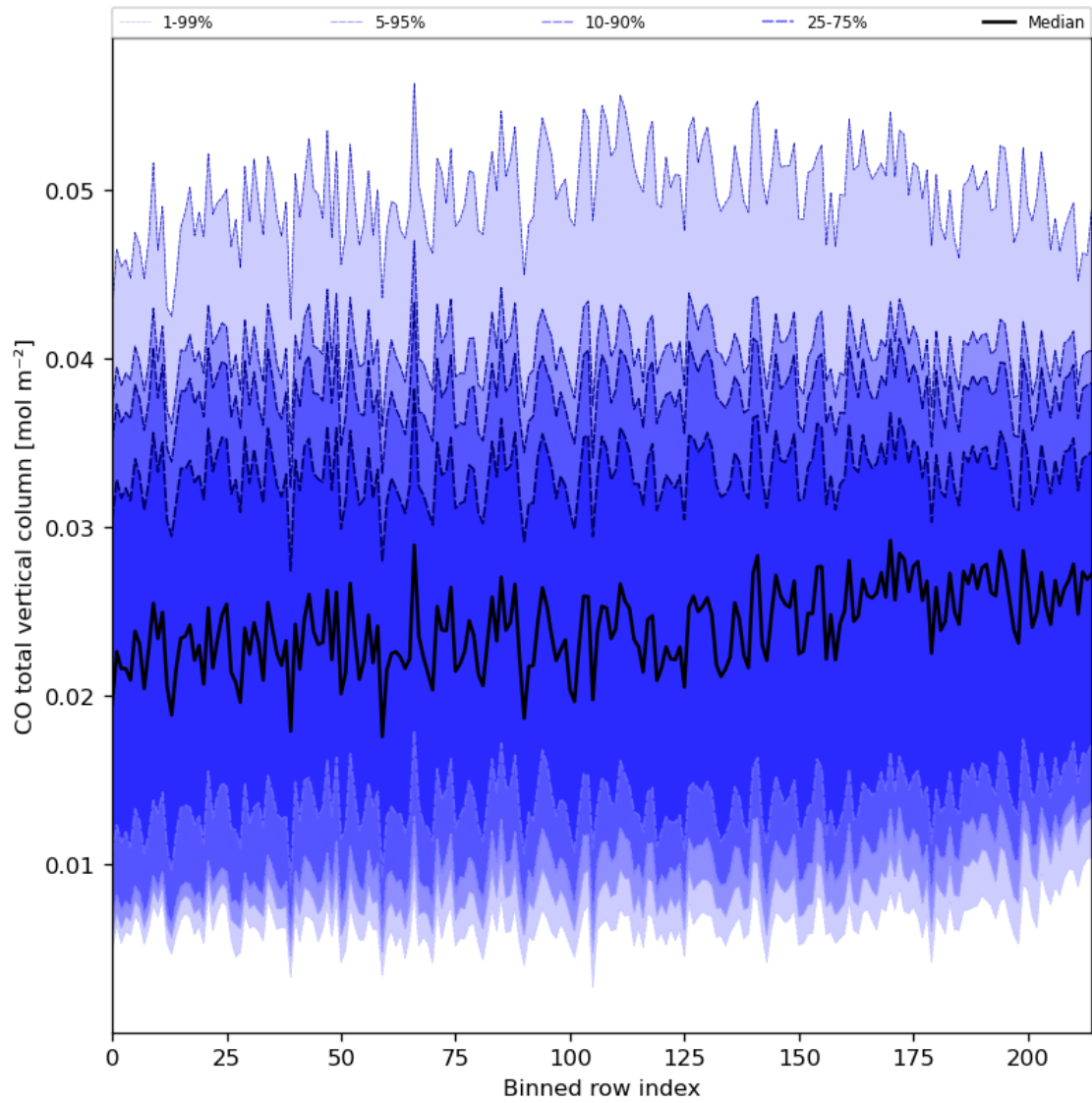
Figure 26: Along track statistics of “CO total vertical column” for 2024-02-20 to 2024-02-22
