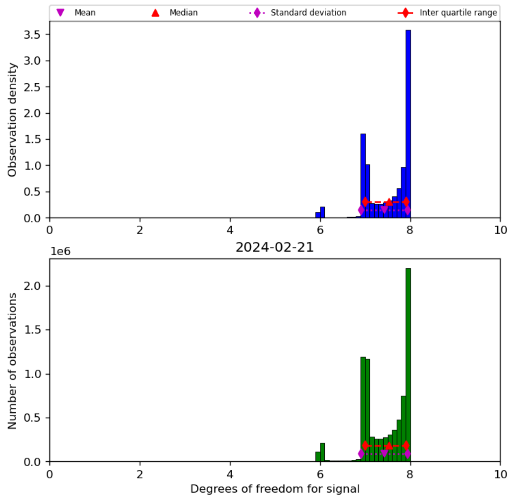
Figure 23: Histogram of “Degrees of freedom for signal” for 2024-02-20 to 2024-02-22
