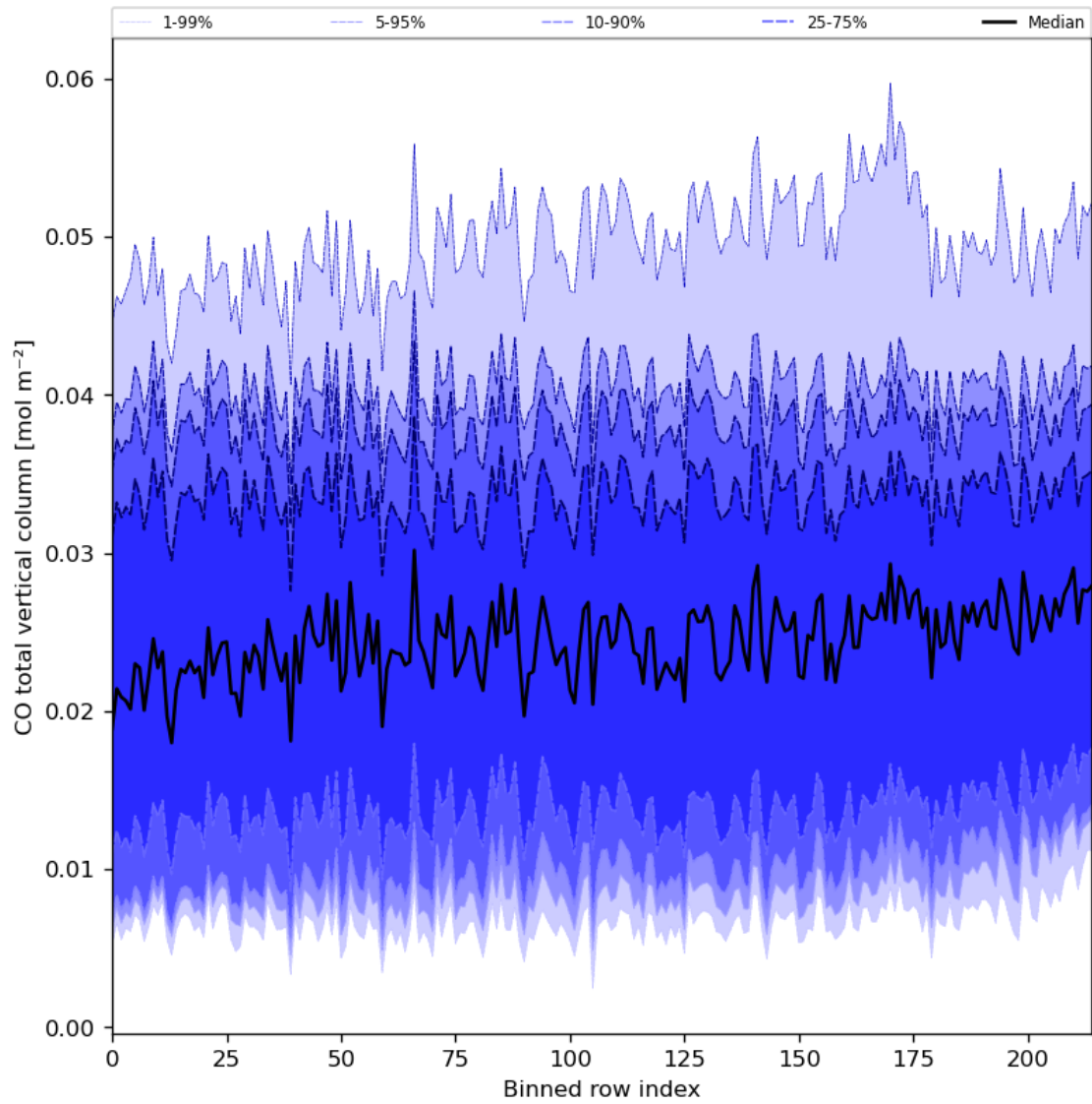
Figure 26: Along track statistics of “CO total vertical column” for 2024-02-22 to 2024-02-23
