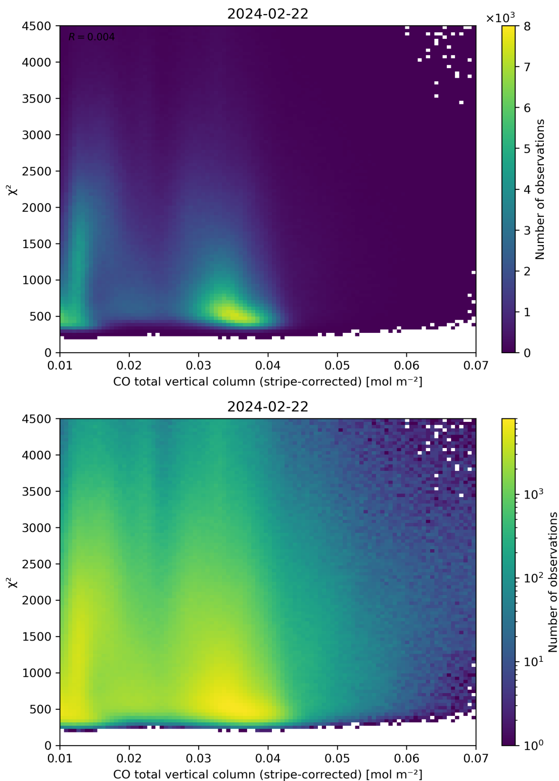
Figure 37: Scatter density plot of “CO total vertical column (stripe-corrected)” against “ \chi^2 ” for 2024-02-22 to 2024-02-23.
