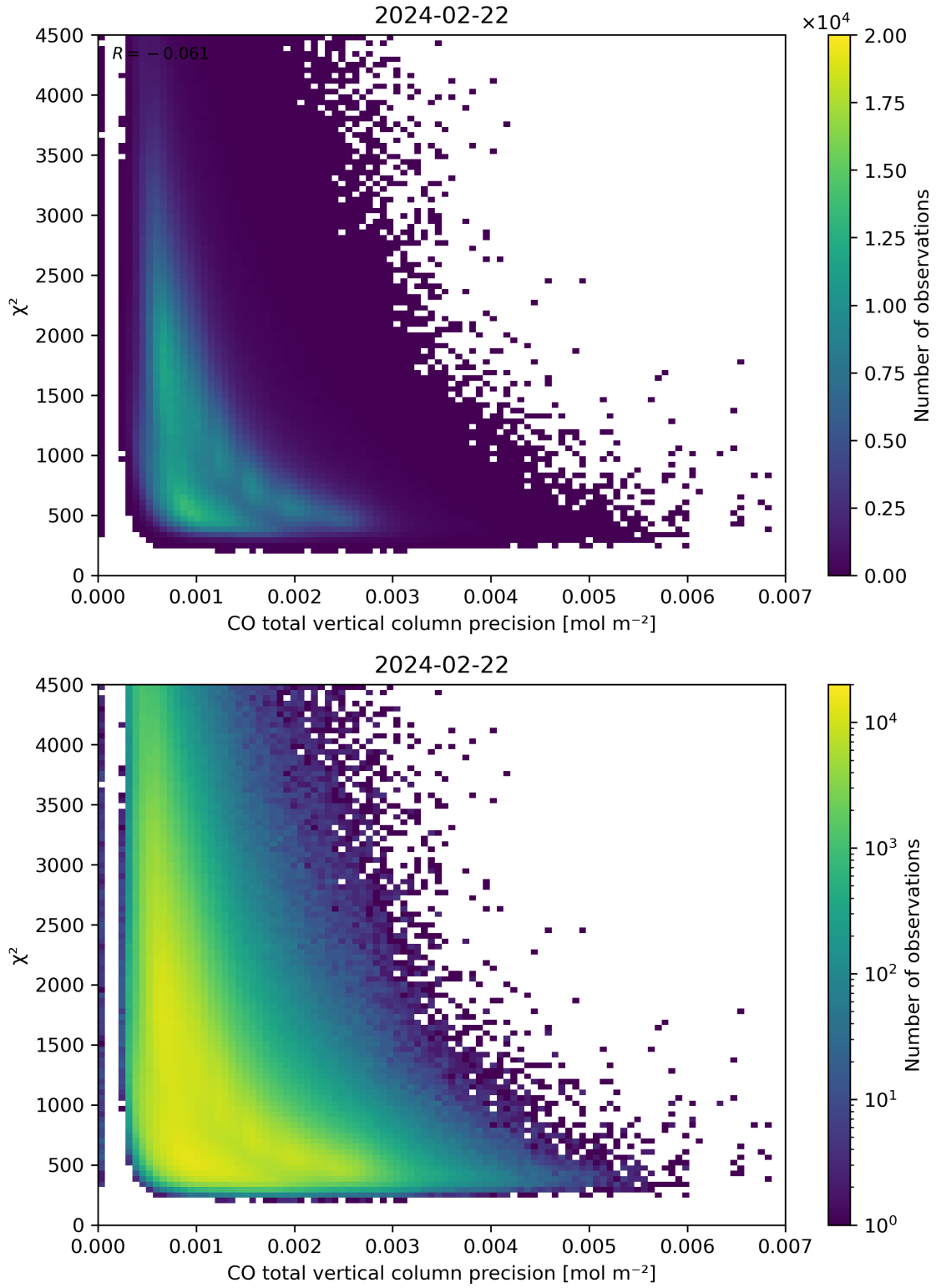
Figure 44: Scatter density plot of “CO total vertical column precision” against “ \chi^2 ” for 2024-02-22 to 2024-02-23.
