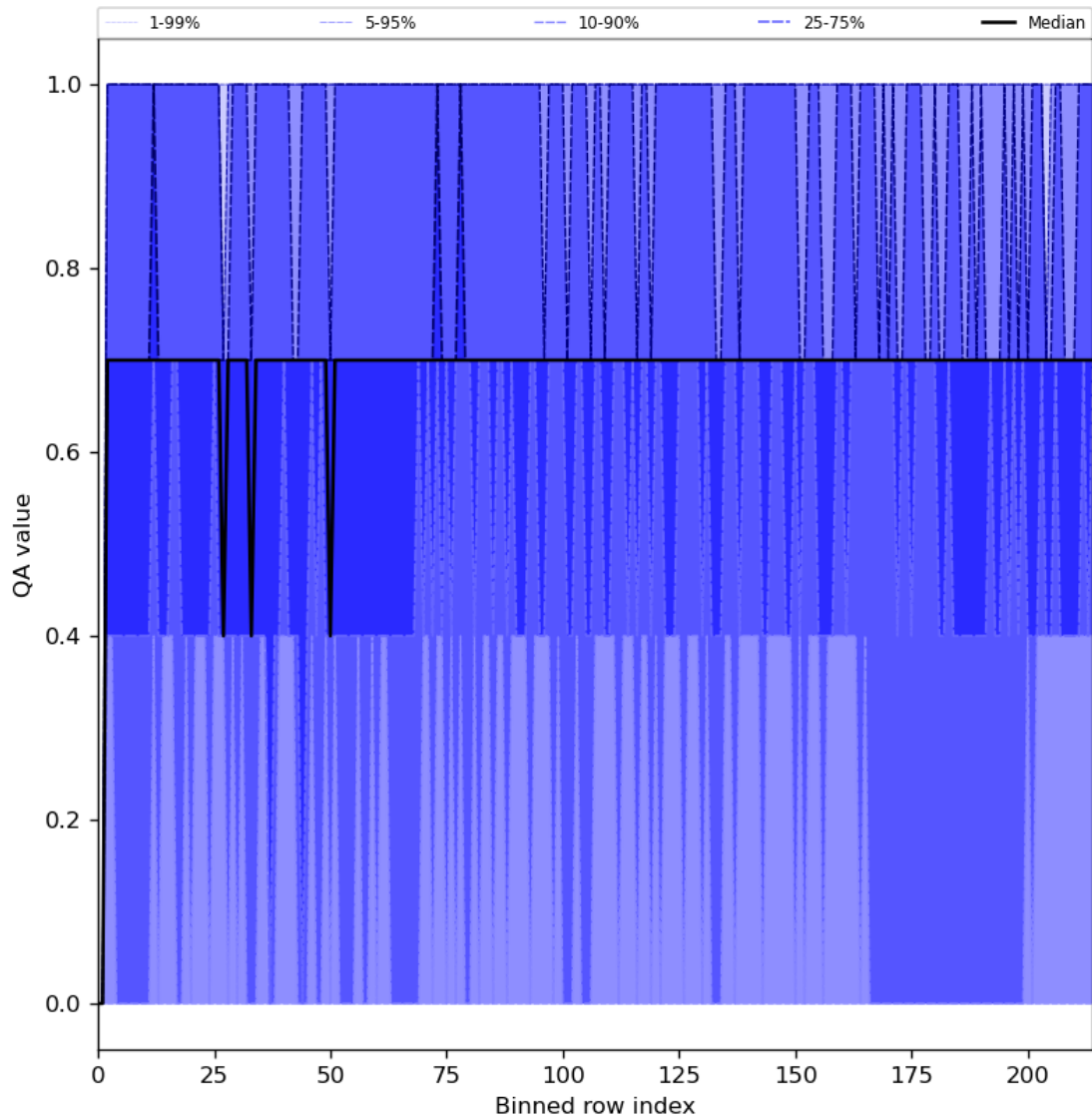
Figure 25: Along track statistics of “QA value” for 2024-02-22 to 2024-02-23
