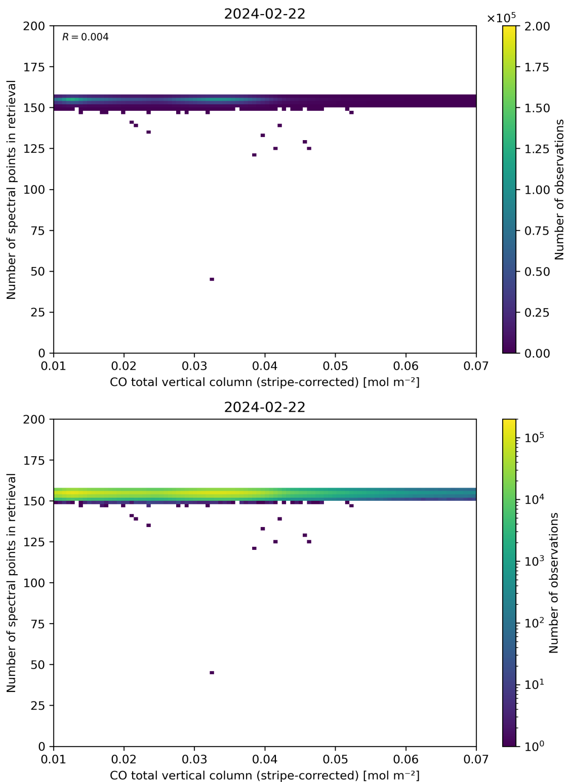
Figure 40: Scatter density plot of “CO total vertical column (stripe-corrected)” against “Number of spectral points in retrieval” for 2024-02-22 to 2024-02-23.
