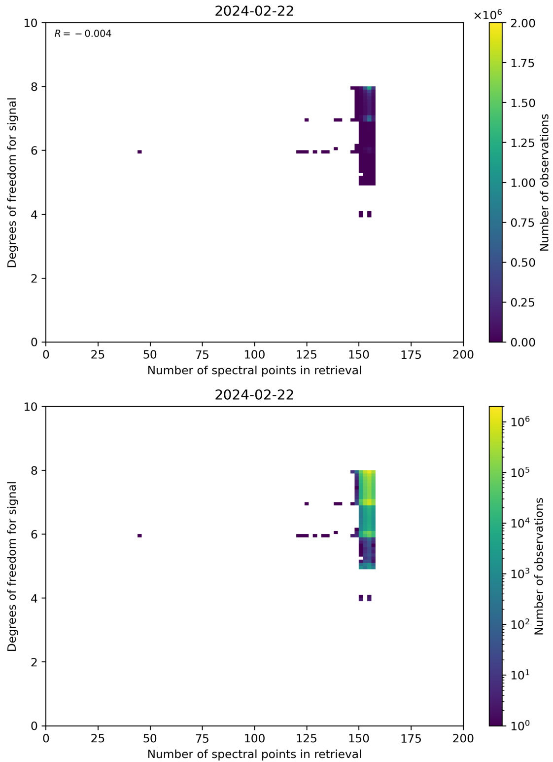
Figure 59: Scatter density plot of “Number of spectral points in retrieval” against “Degrees of freedom for signal” for 2024-02-22 to 2024-02-23.
