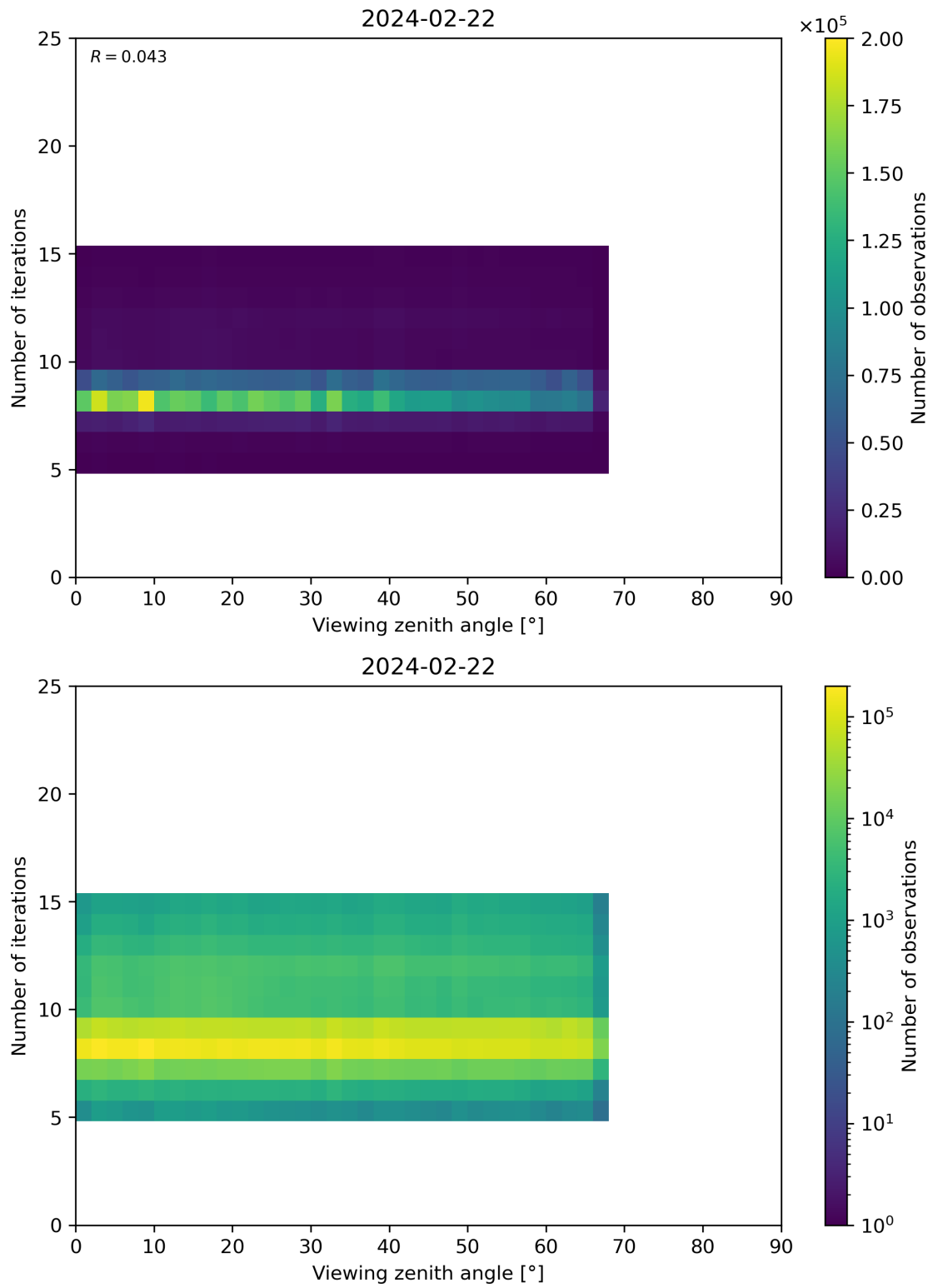
Figure 75: Scatter density plot of “Viewing zenith angle” against “Number of iterations” for 2024-02-22 to 2024-02-23.
