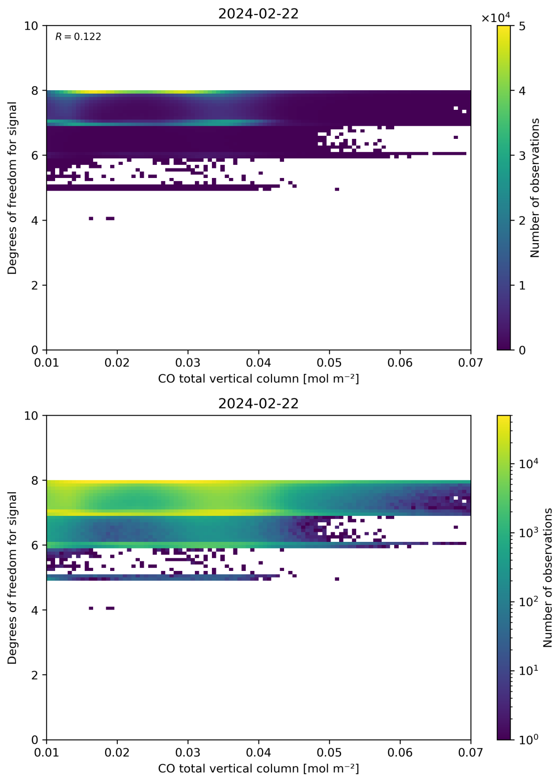
Figure 41: Scatter density plot of “CO total vertical column” against “Degrees of freedom for signal” for 2024-02-22 to 2024-02-23.
