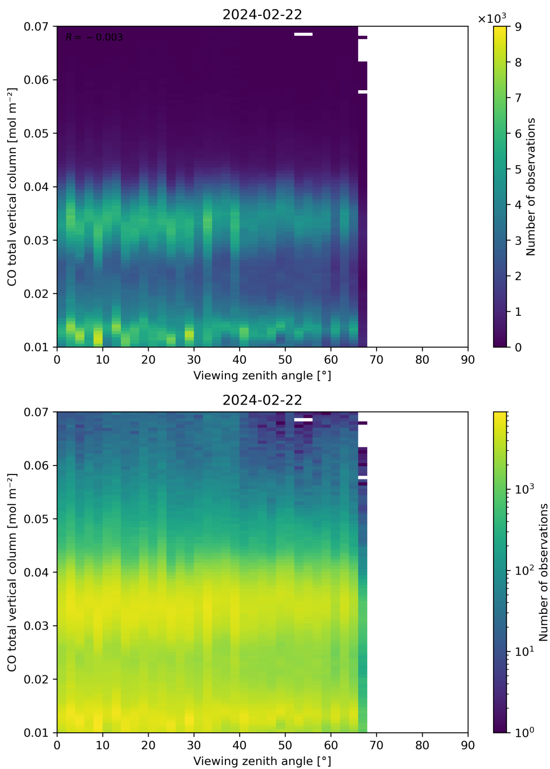
Figure 69: Scatter density plot of “Viewing zenith angle” against “CO total vertical column” for 2024-02-22 to 2024-02-23.
