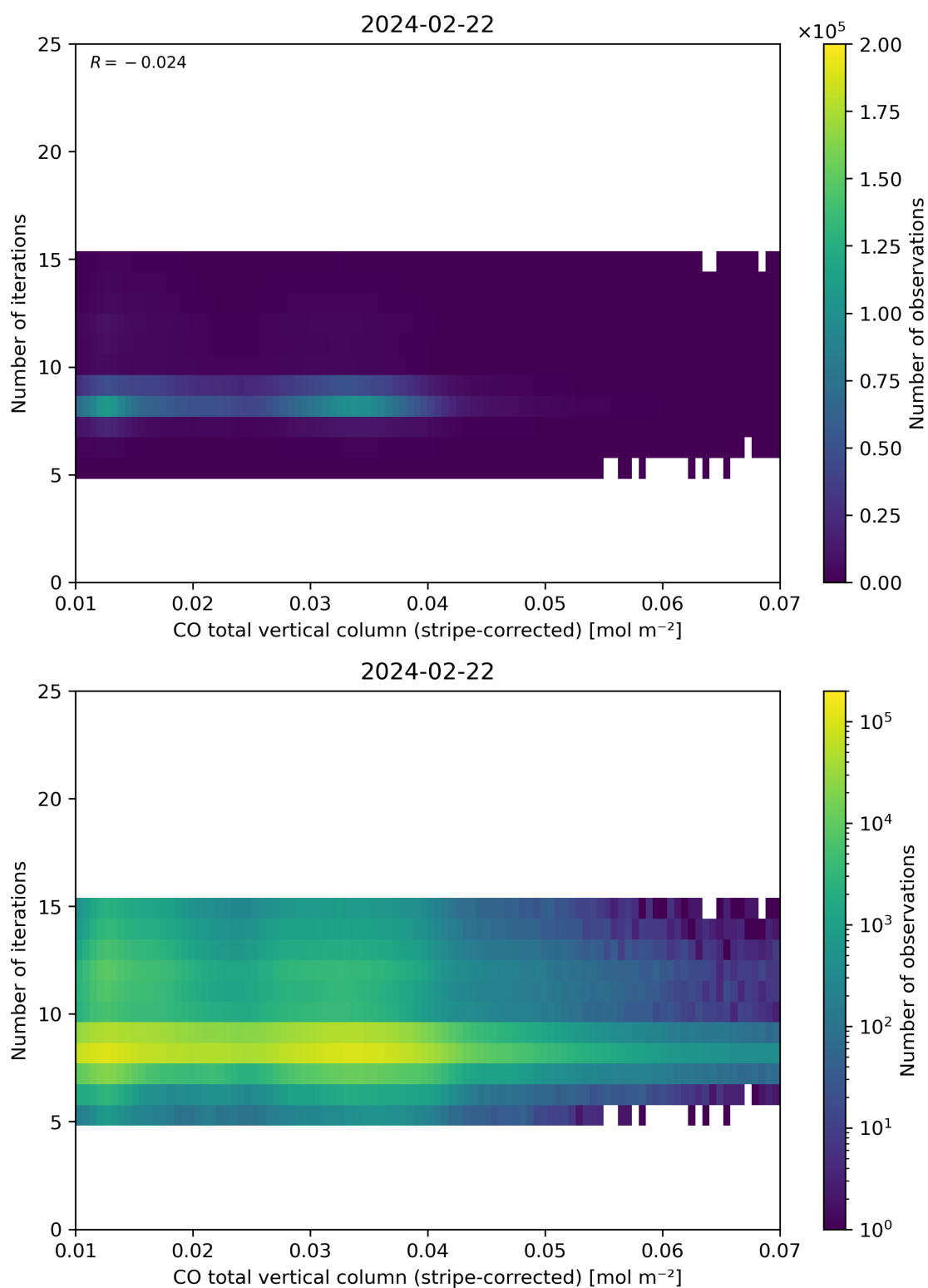
Figure 39: Scatter density plot of “CO total vertical column (stripe-corrected)” against “Number of iterations” for 2024-02-22 to 2024-02-23.
