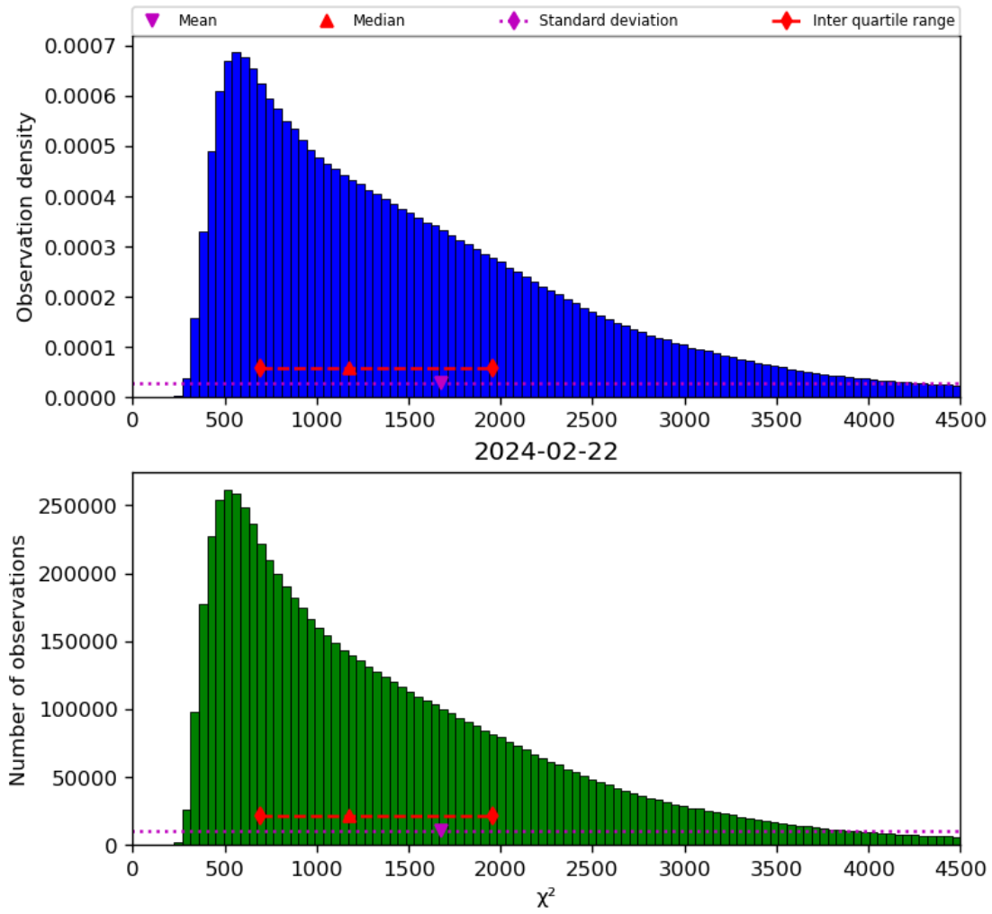
Figure 22: Histogram of “ \chi^2 ” for 2024-02-22 to 2024-02-23
