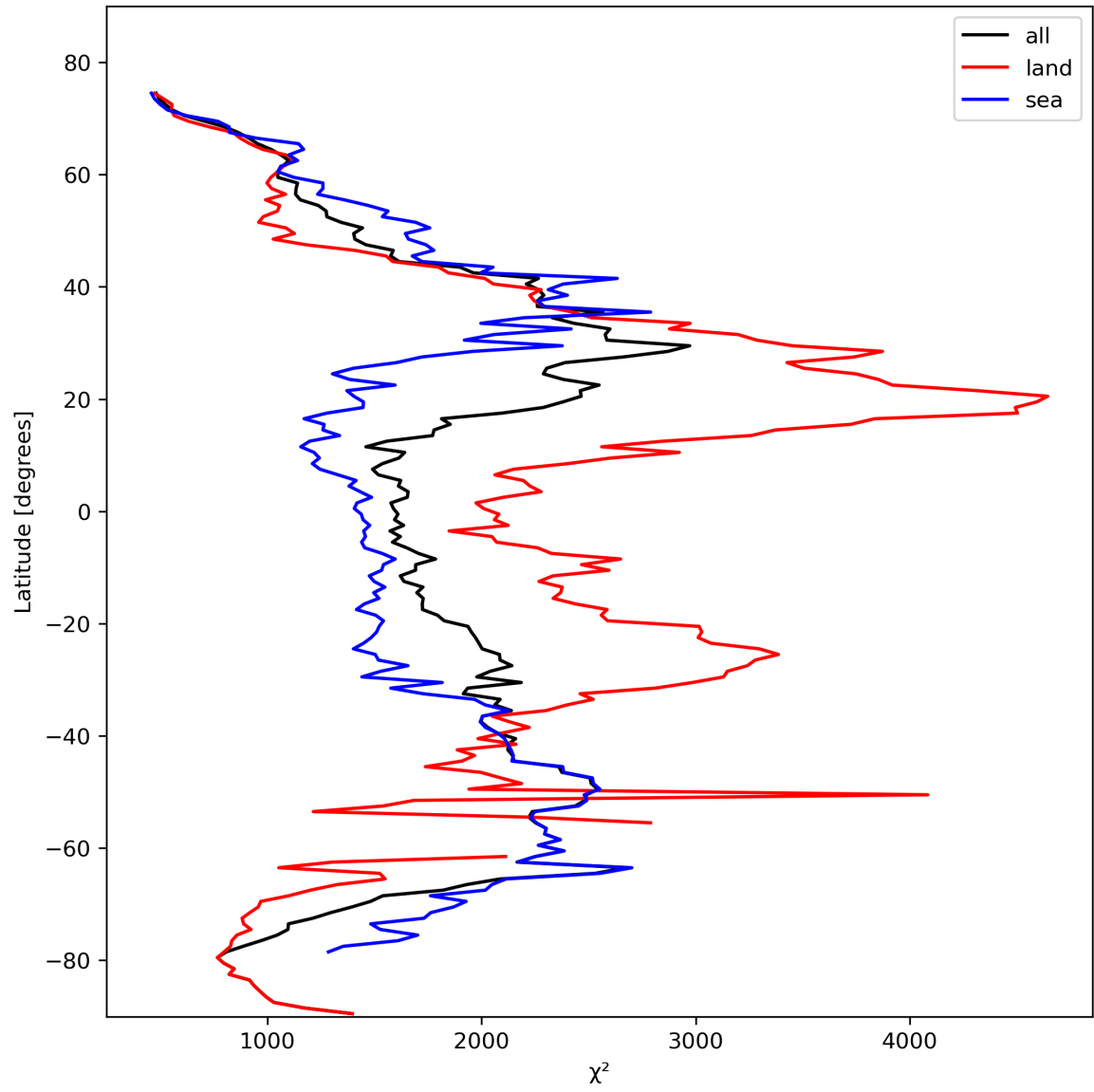
Figure 14: Zonal average of “ \chi^2 ” for 2024-02-22 to 2024-02-23.
