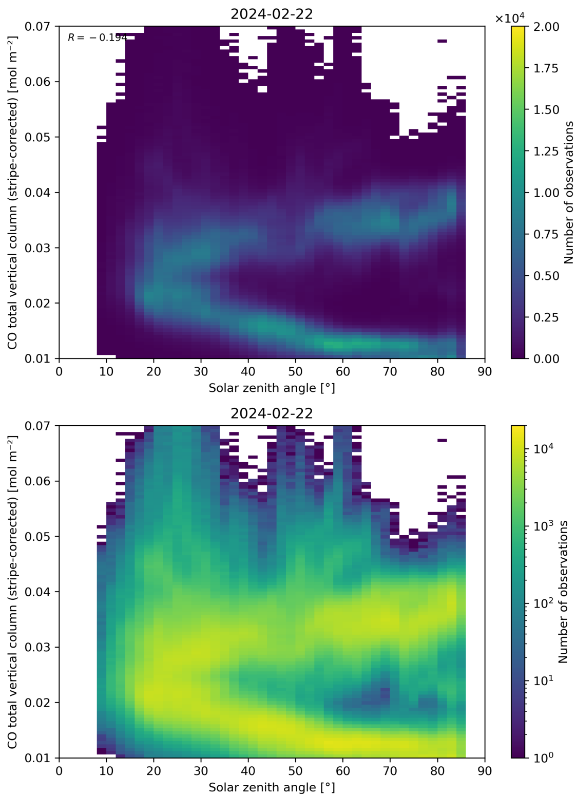
Figure 62: Scatter density plot of “Solar zenith angle” against “CO total vertical column (stripe-corrected)” for 2024-02-22 to 2024-02-23.
