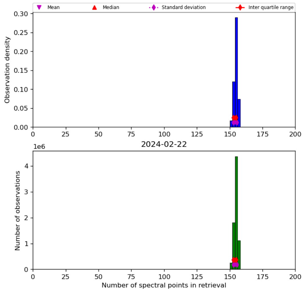
Figure 21: Histogram of “Number of spectral points in retrieval” for 2024-02-22 to 2024-02-23
