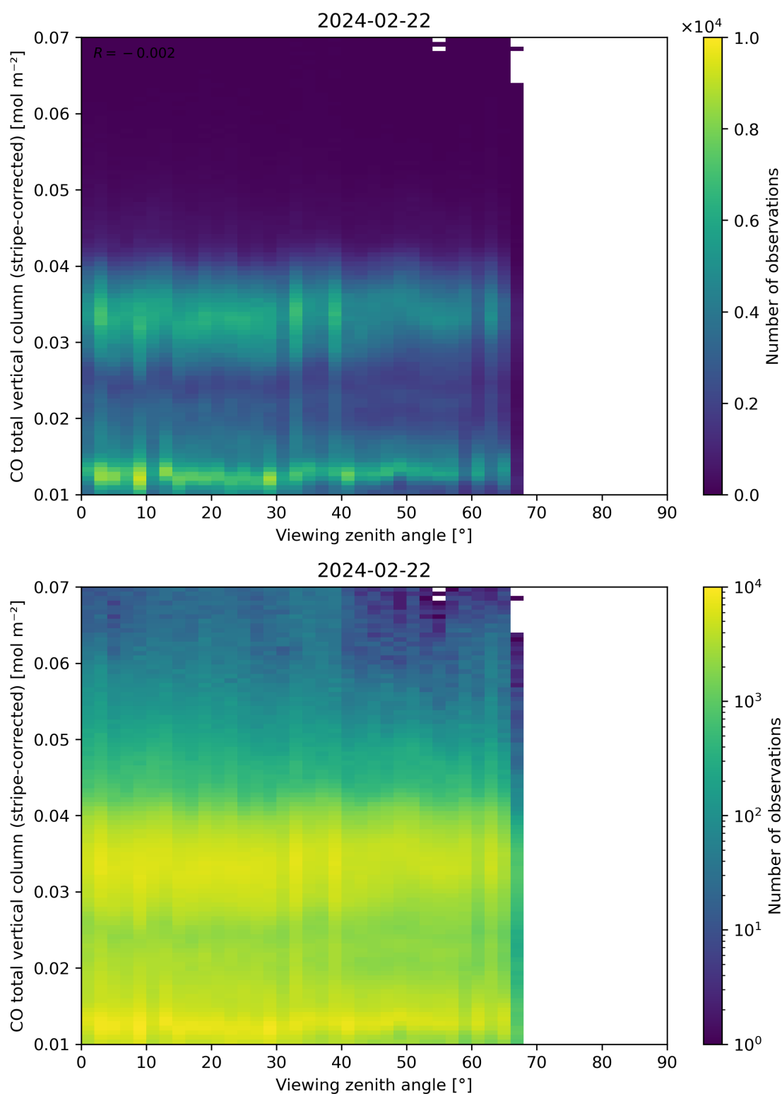
Figure 70: Scatter density plot of “Viewing zenith angle” against “CO total vertical column (stripe-corrected)” for 2024-02-22 to 2024-02-23.
