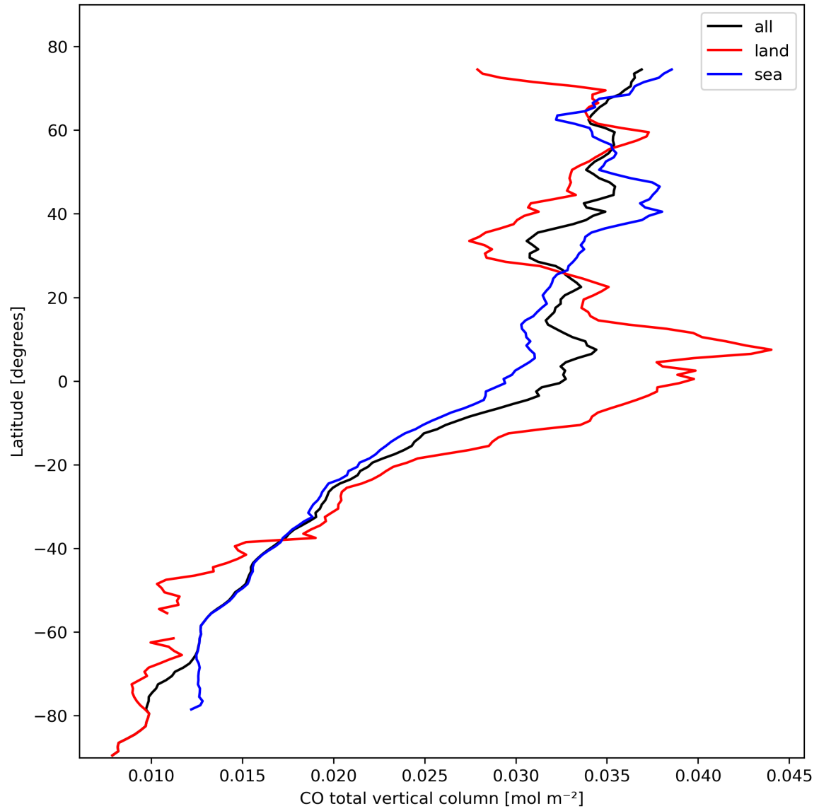
Figure 10: Zonal average of “CO total vertical column” for 2024-02-22 to 2024-02-23.
