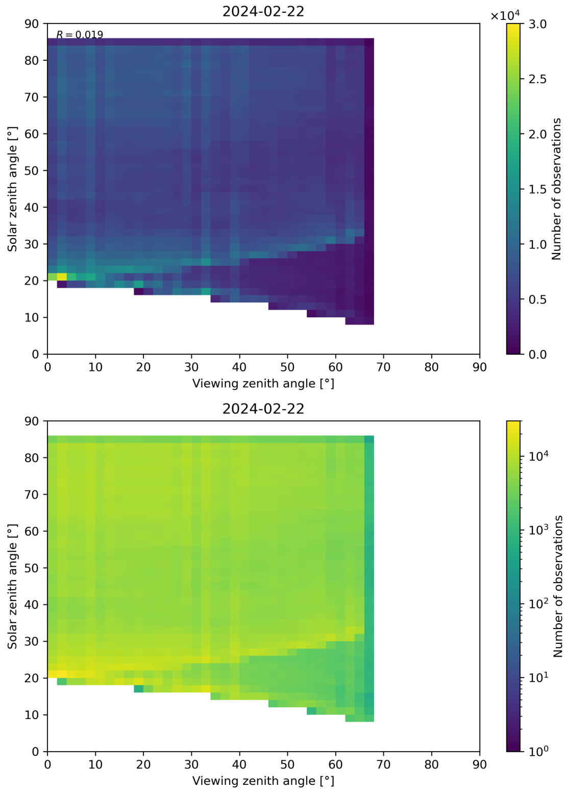
Figure 77: Scatter density plot of “Viewing zenith angle” against “Solar zenith angle” for 2024-02-22 to 2024-02-23.
