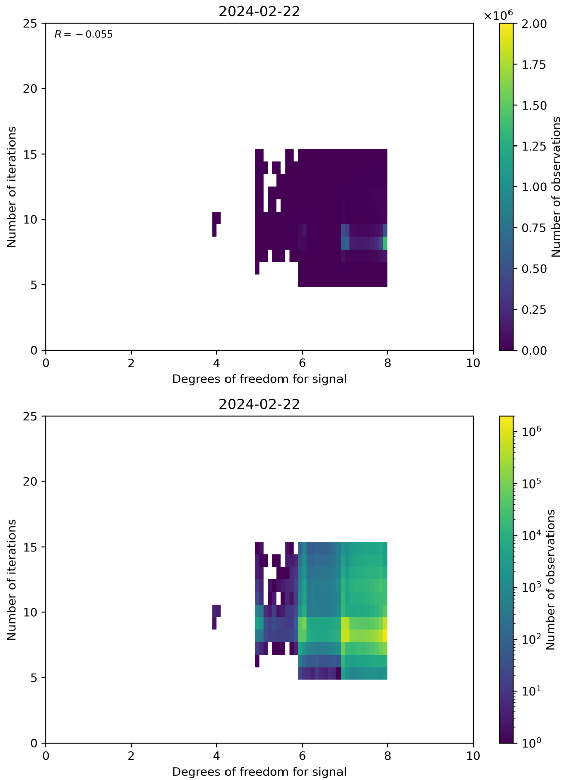
Figure 50: Scatter density plot of “Degrees of freedom for signal” against “Number of iterations” for 2024-02-22 to 2024-02-23.
