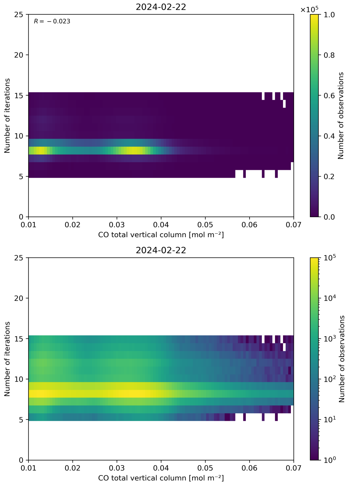
Figure 42: Scatter density plot of “CO total vertical column” against “Number of iterations” for 2024-02-22 to 2024-02-23.
