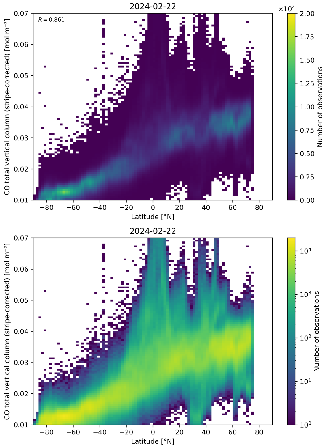
Figure 52: Scatter density plot of “Latitude” against “CO total vertical column (stripe-corrected)” for 2024-02-22 to 2024-02-23.
