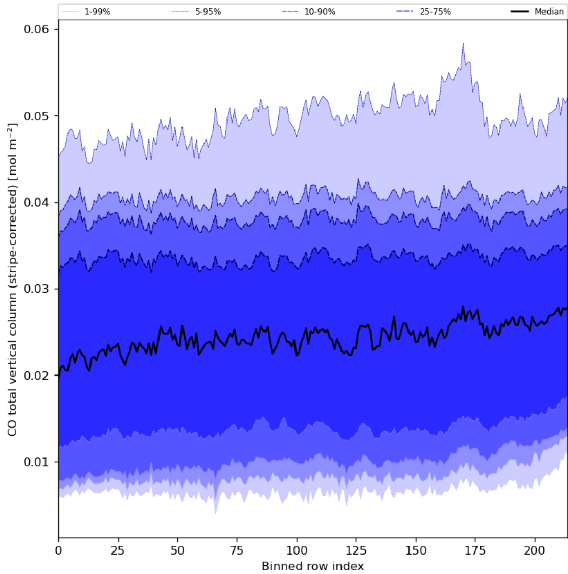
Figure 27: Along track statistics of “CO total vertical column (stripe-corrected)” for 2024-02-22 to 2024-02-23
