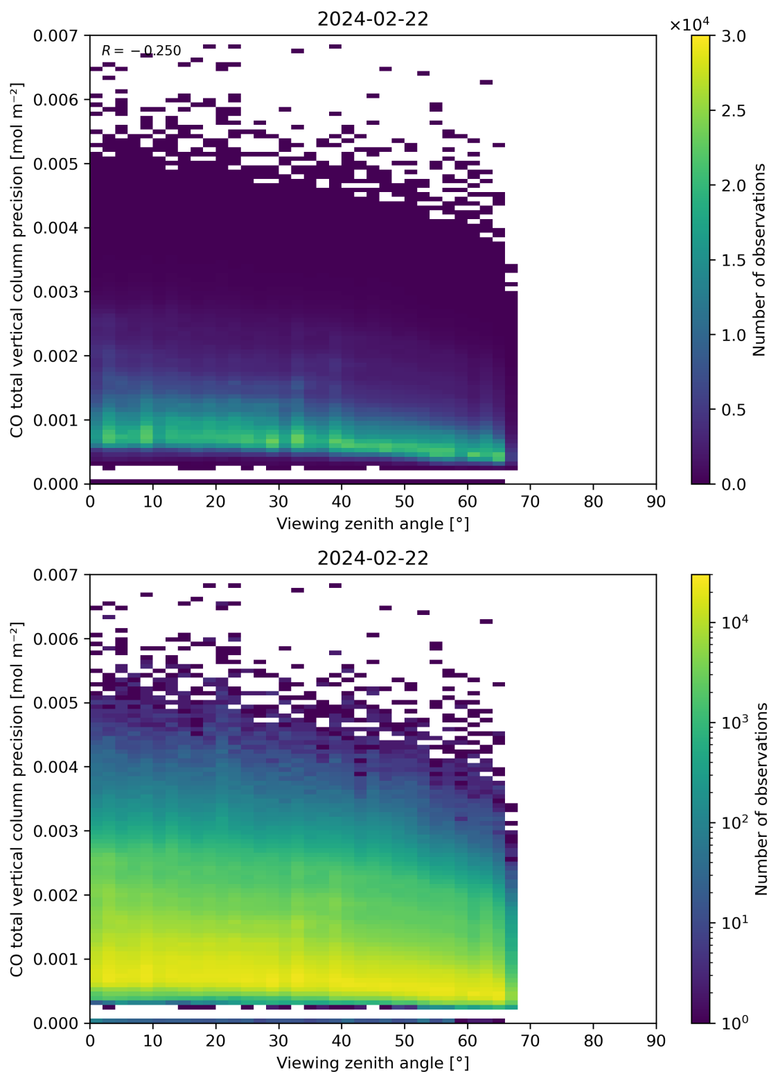
Figure 71: Scatter density plot of “Viewing zenith angle” against “CO total vertical column precision” for 2024-02-22 to 2024-02-23.
