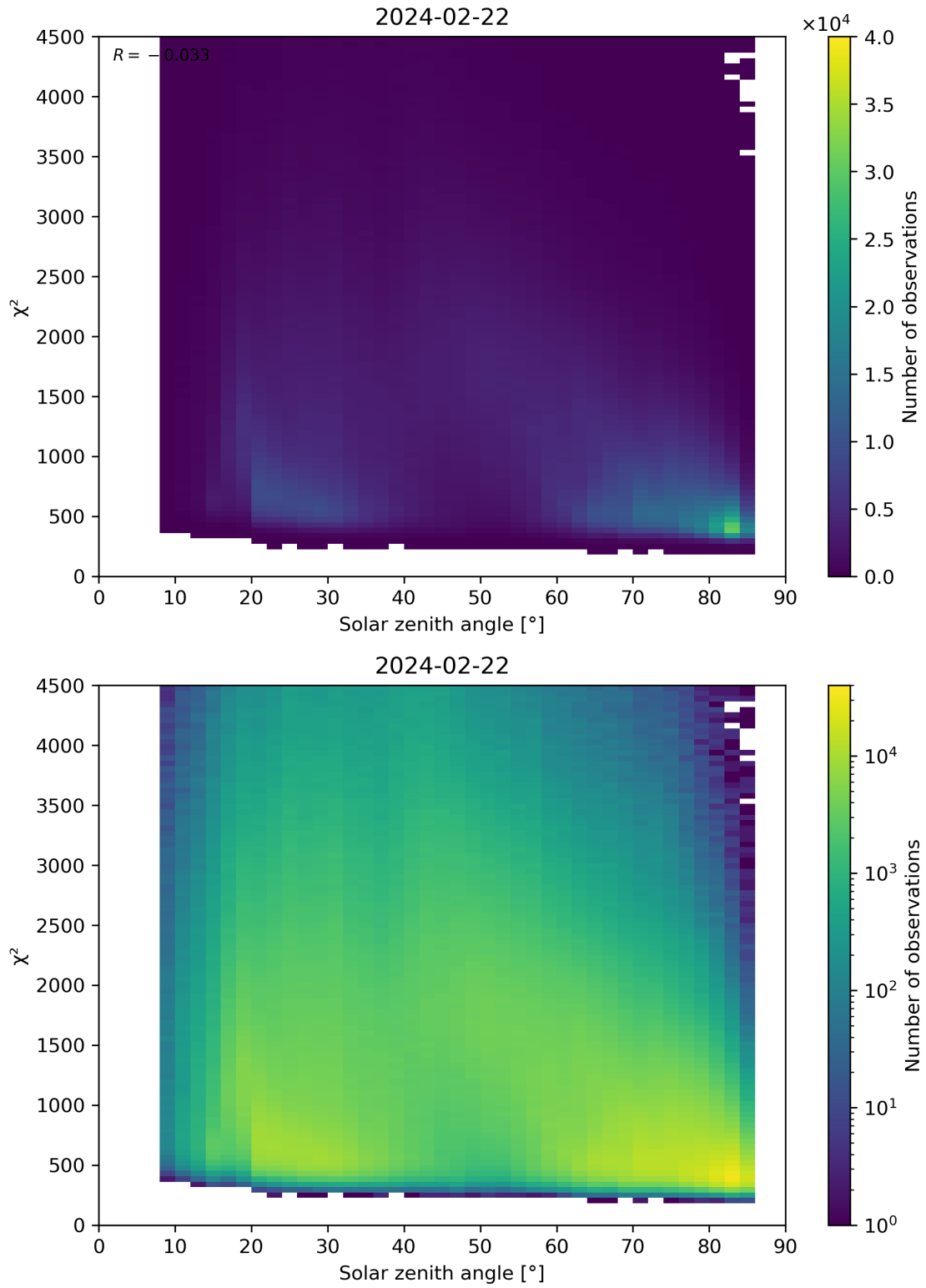
Figure 64: Scatter density plot of “Solar zenith angle” against “ \chi^2 ” for 2024-02-22 to 2024-02-23.
