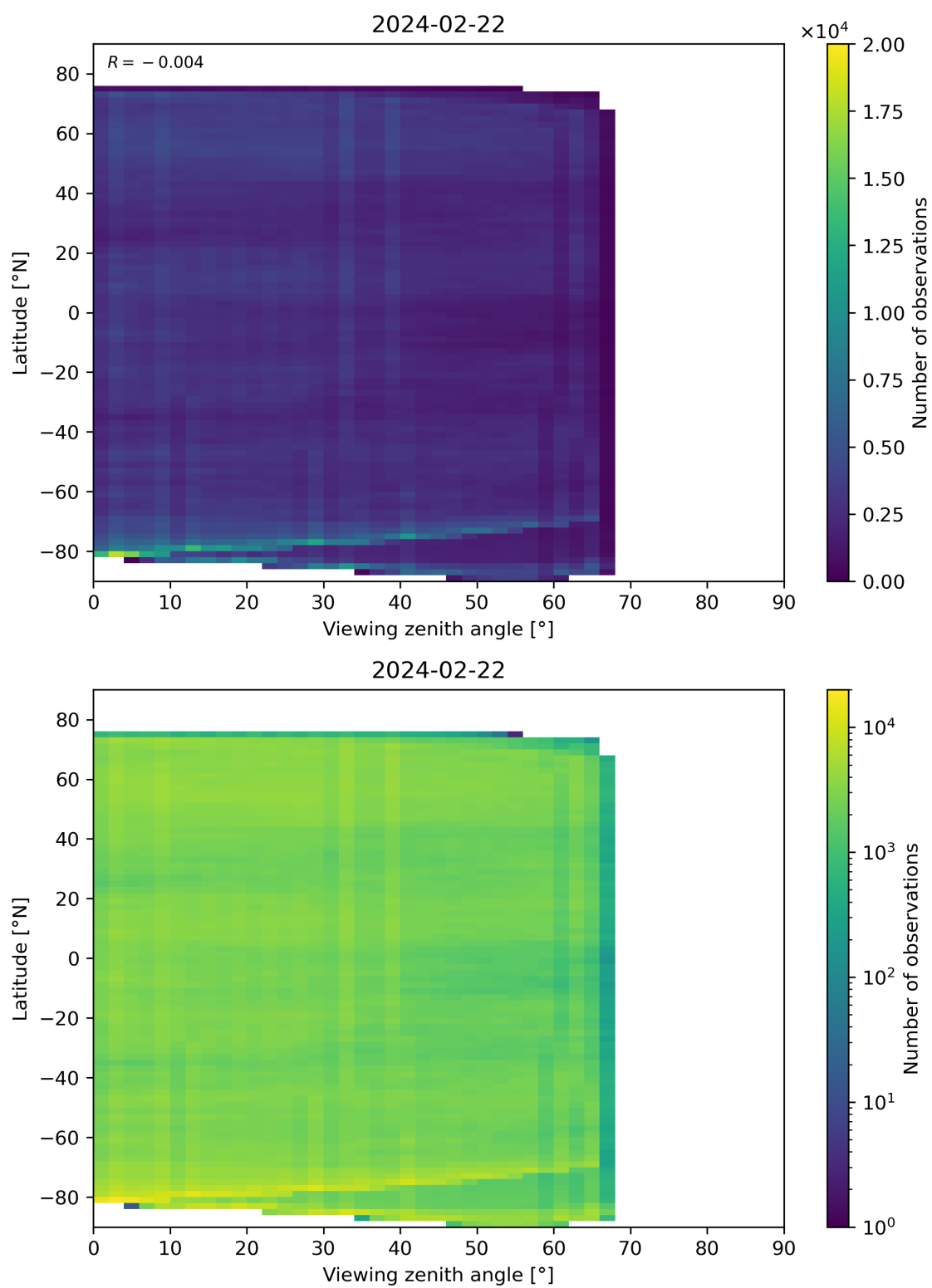
Figure 74: Scatter density plot of “Viewing zenith angle” against “Latitude” for 2024-02-22 to 2024-02-23.
