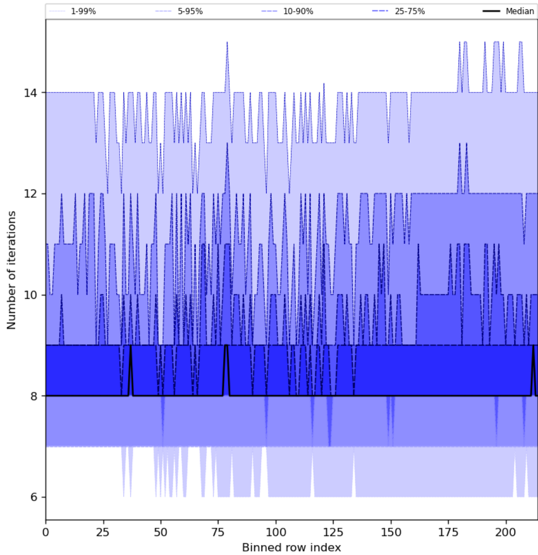
Figure 32: Along track statistics of “Number of iterations” for 2024-02-22 to 2024-02-23
