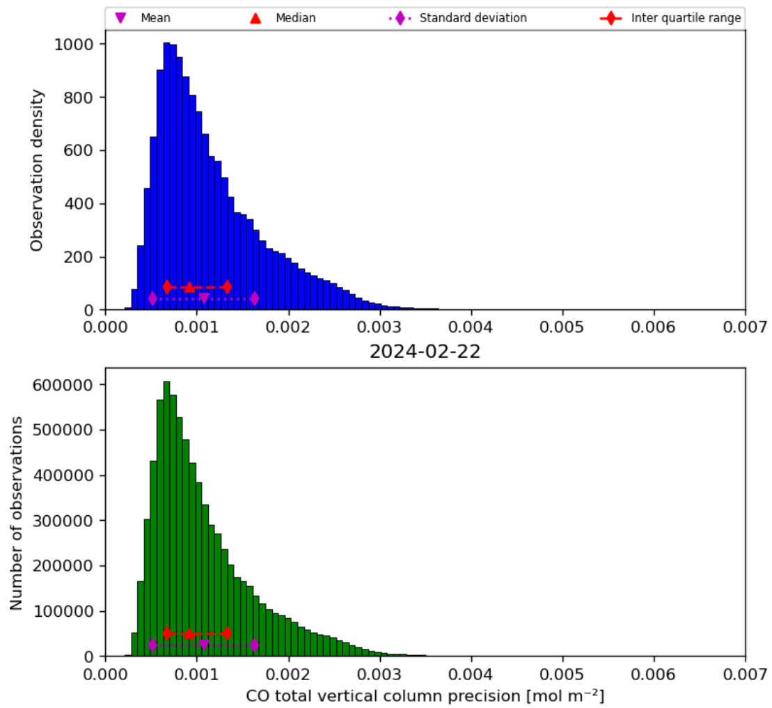
Figure 20: Histogram of “CO total vertical column precision” for 2024-02-22 to 2024-02-23
