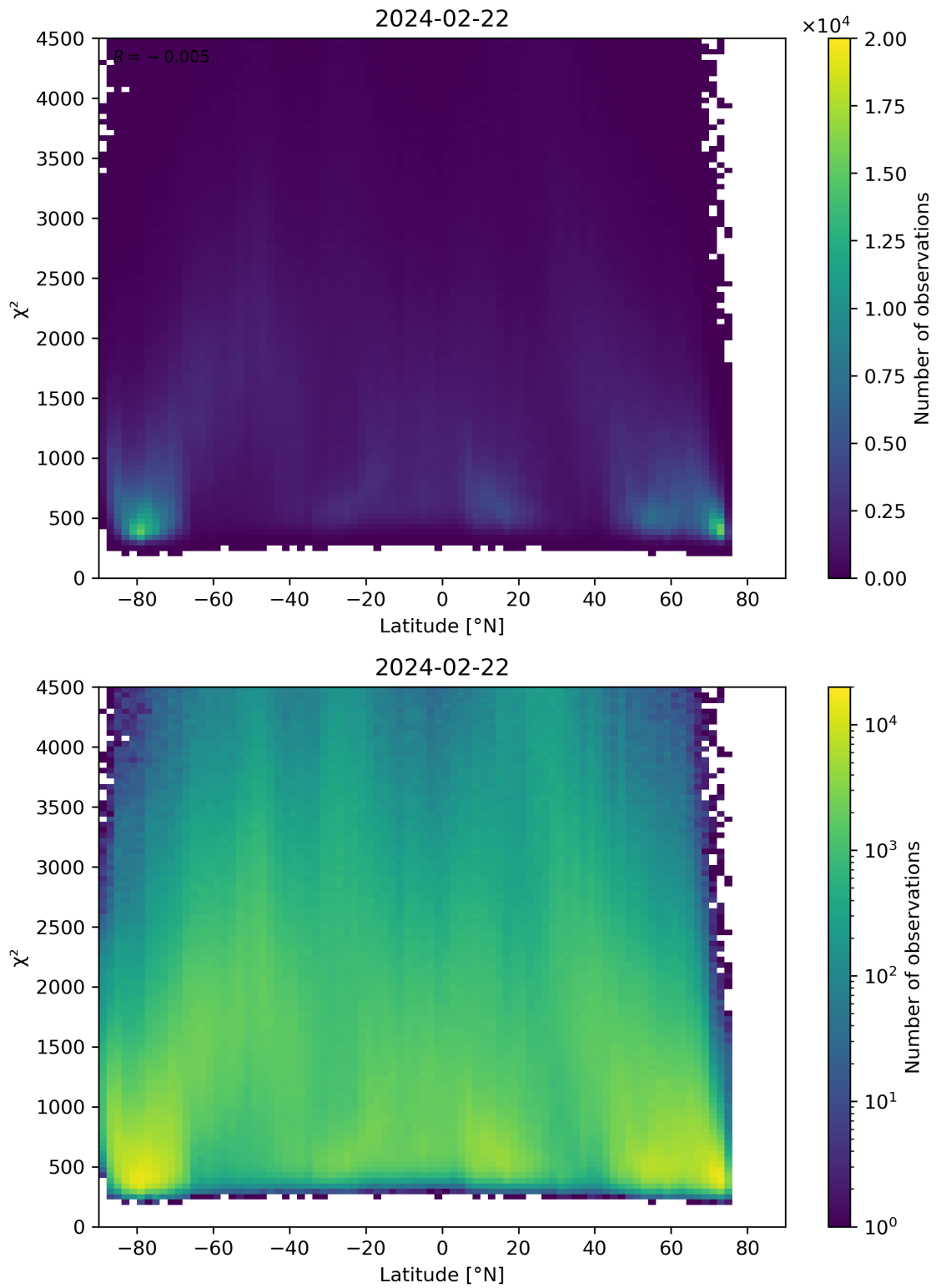
Figure 54: Scatter density plot of “Latitude” against “ \chi^2 ” for 2024-02-22 to 2024-02-23.
