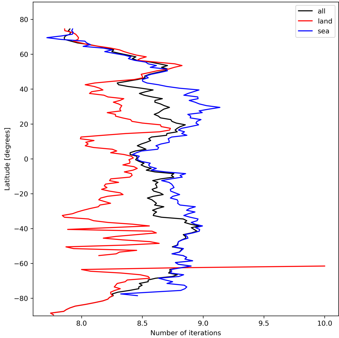
Figure 16: Zonal average of “Number of iterations” for 2024-02-22 to 2024-02-23.
