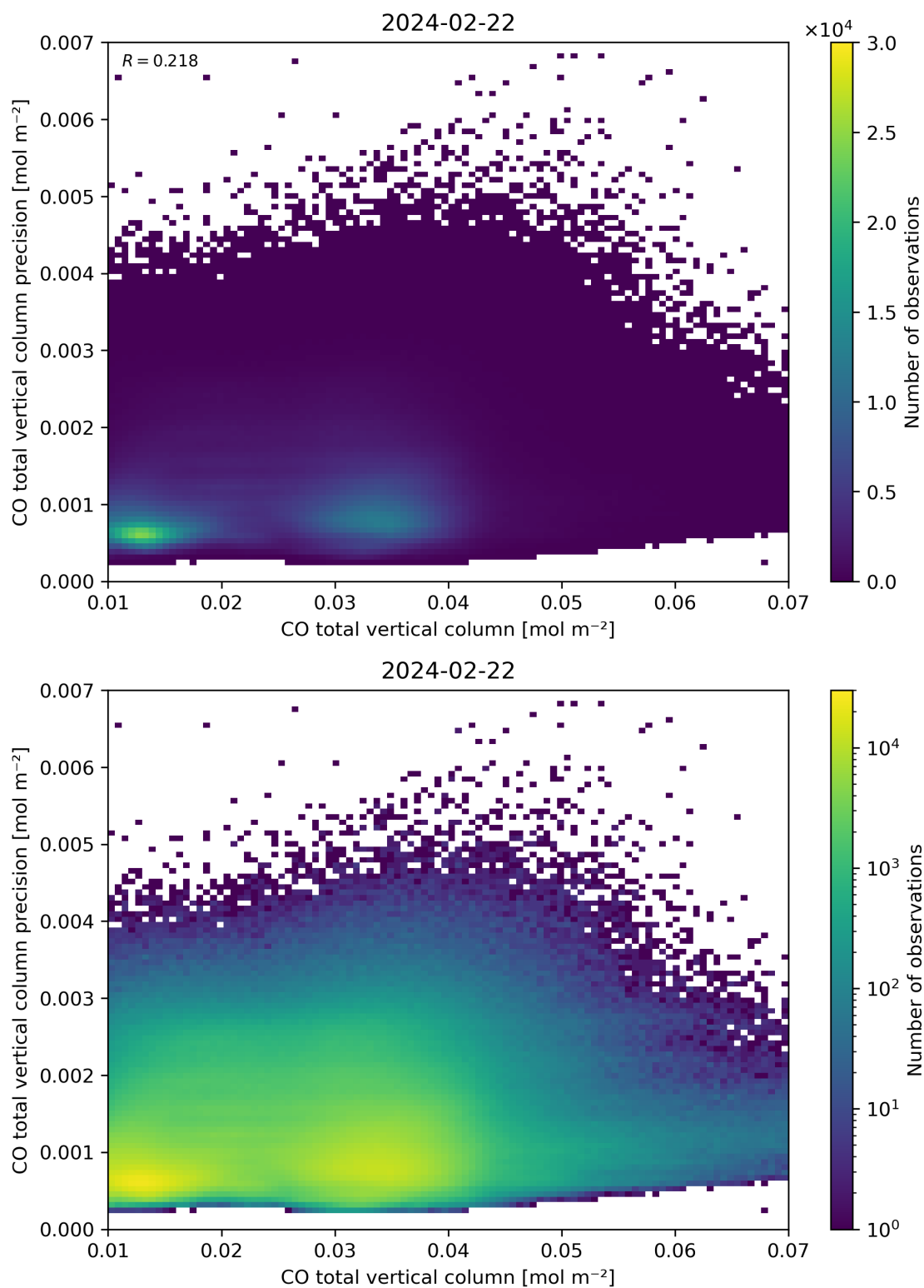
Figure 34: Scatter density plot of “CO total vertical column” against “CO total vertical column precision” for 2024-02-22 to 2024-02-23.
