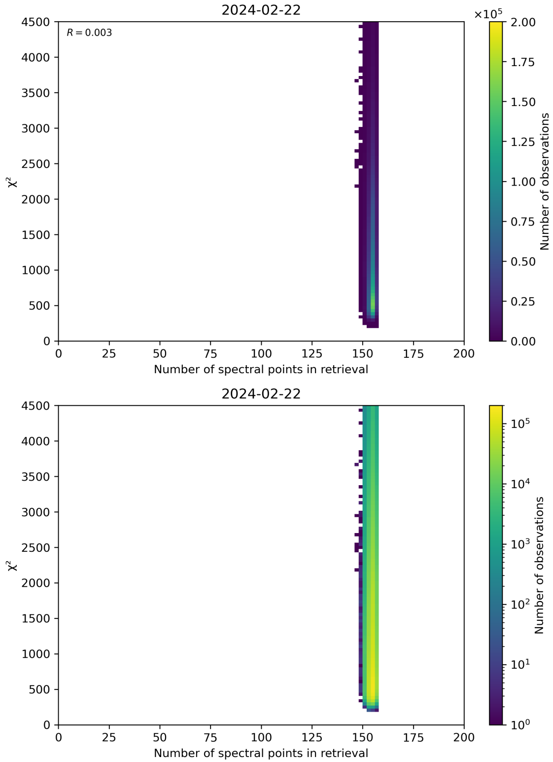
Figure 58: Scatter density plot of “Number of spectral points in retrieval” against “ \chi^2 ” for 2024-02-22 to 2024-02-23.
