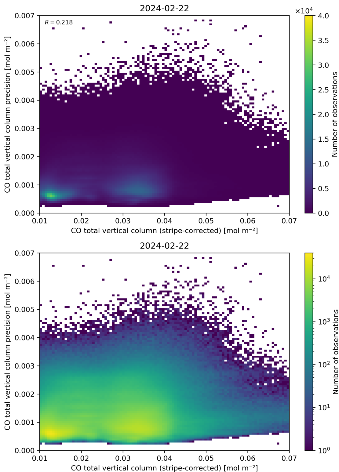
Figure 36: Scatter density plot of “CO total vertical column (stripe-corrected)” against “CO total vertical column precision” for 2024-02-22 to 2024-02-23.
