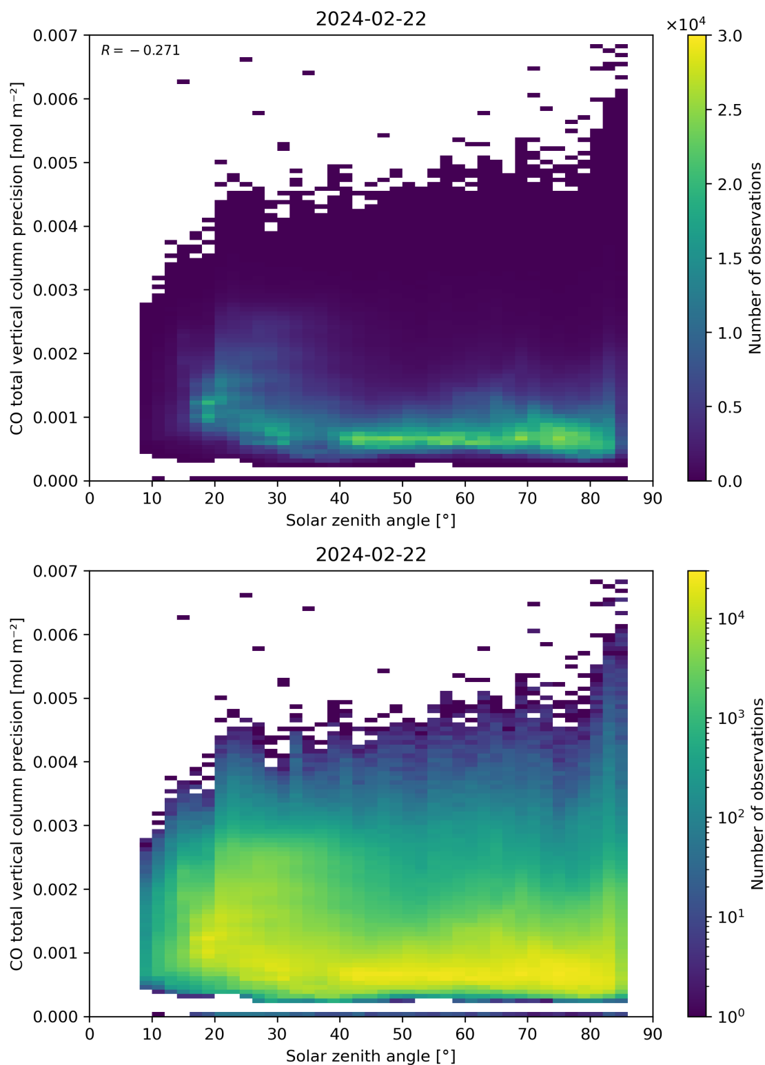
Figure 63: Scatter density plot of “Solar zenith angle” against “CO total vertical column precision” for 2024-02-22 to 2024-02-23.
