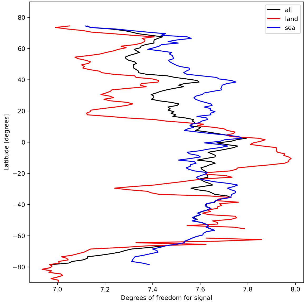
Figure 15: Zonal average of “Degrees of freedom for signal” for 2024-02-22 to 2024-02-23.
