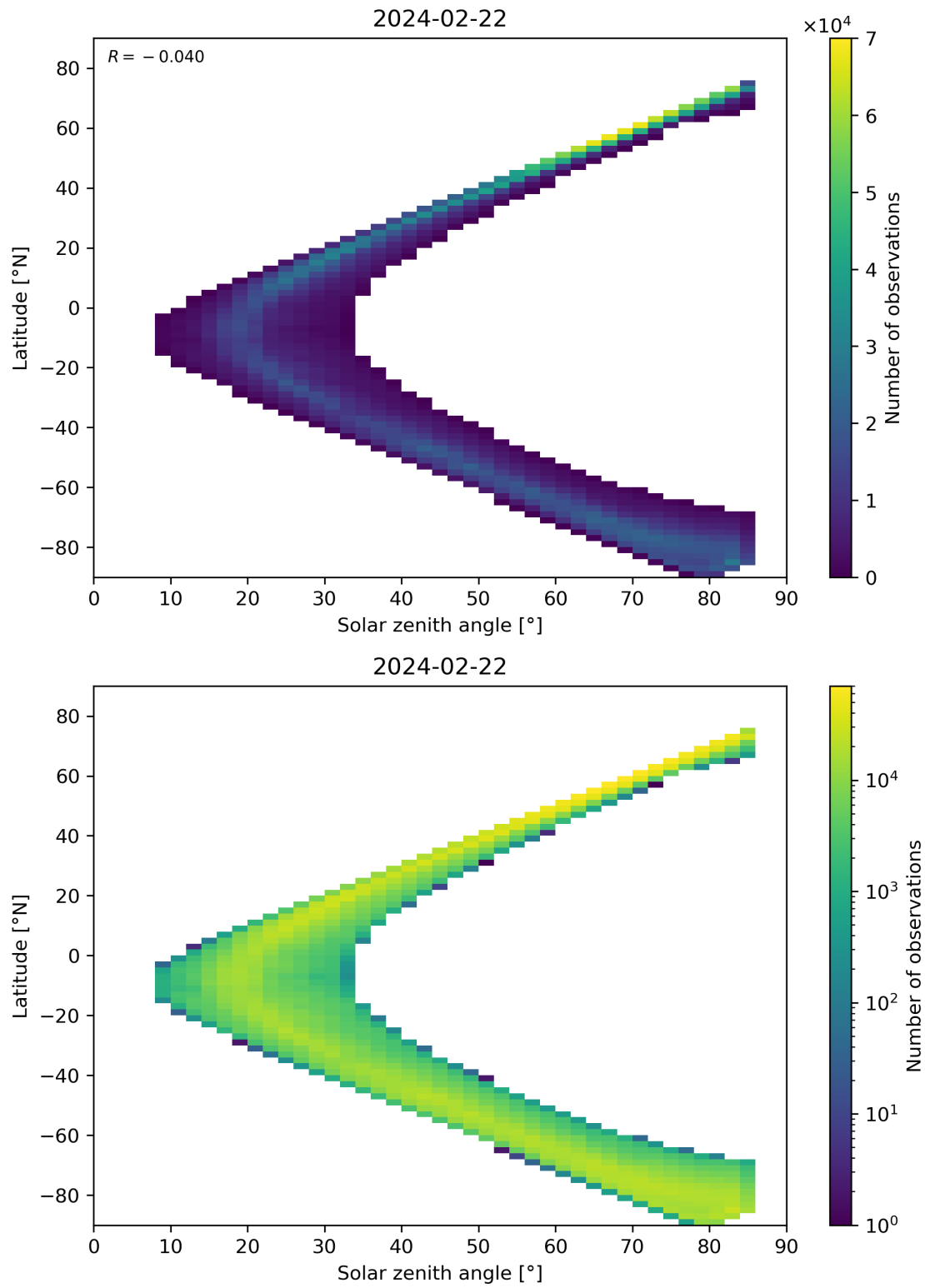
Figure 66: Scatter density plot of “Solar zenith angle” against “Latitude” for 2024-02-22 to 2024-02-23.
