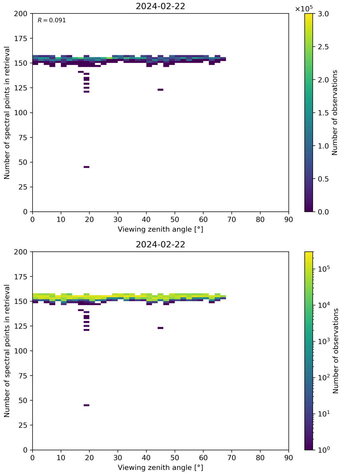
Figure 76: Scatter density plot of “Viewing zenith angle” against “Number of spectral points in retrieval” for 2024-02-22 to 2024-02-23.
