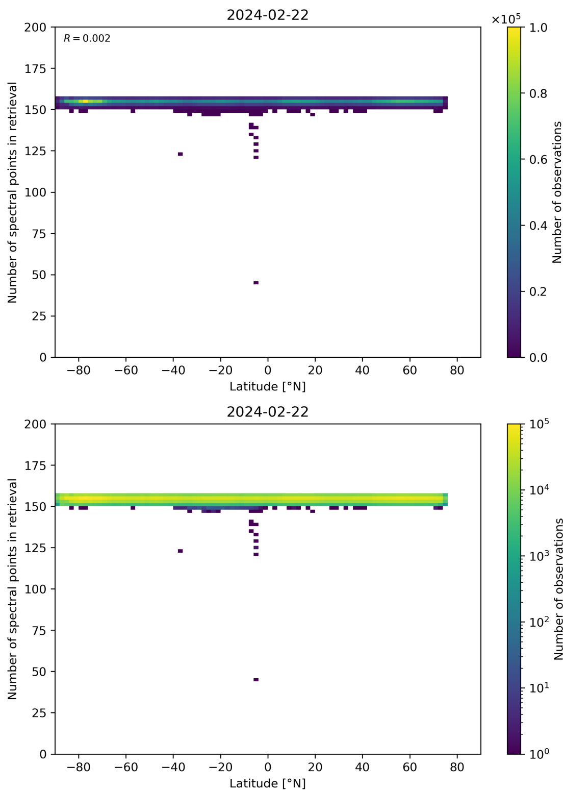
Figure 57: Scatter density plot of “Latitude” against “Number of spectral points in retrieval” for 2024-02-22 to 2024-02-23.
