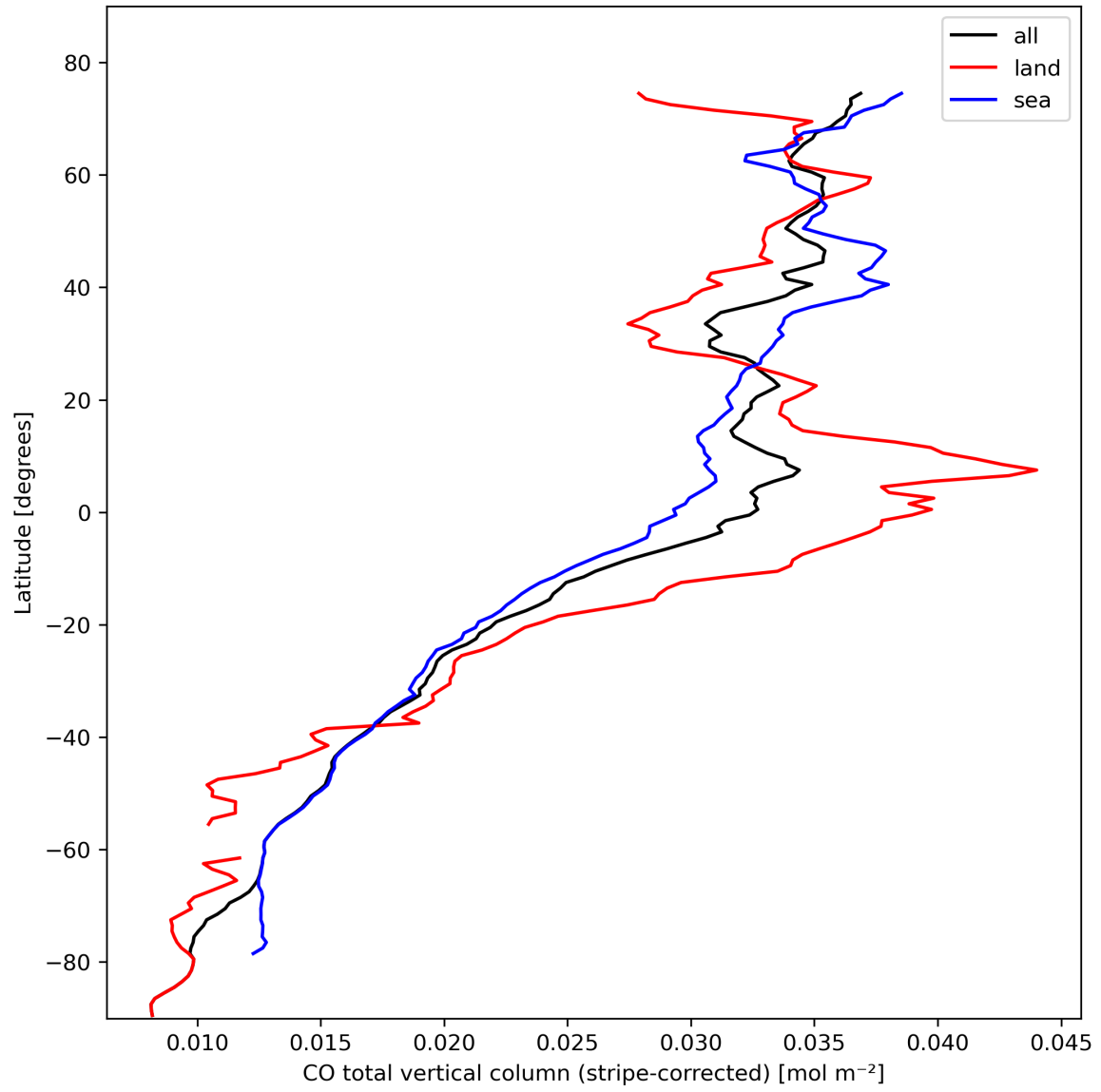
Figure 11: Zonal average of “CO total vertical column (stripe-corrected)” for 2024-02-22 to 2024-02-23.
