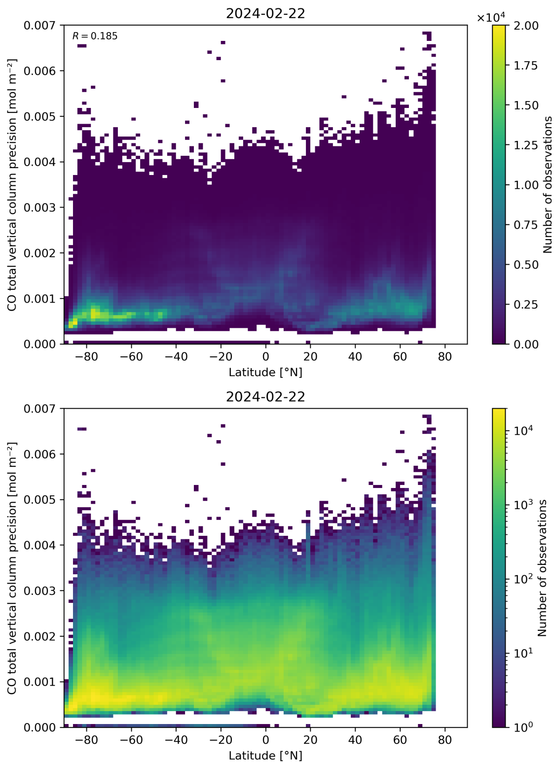
Figure 53: Scatter density plot of “Latitude” against “CO total vertical column precision” for 2024-02-22 to 2024-02-23.
