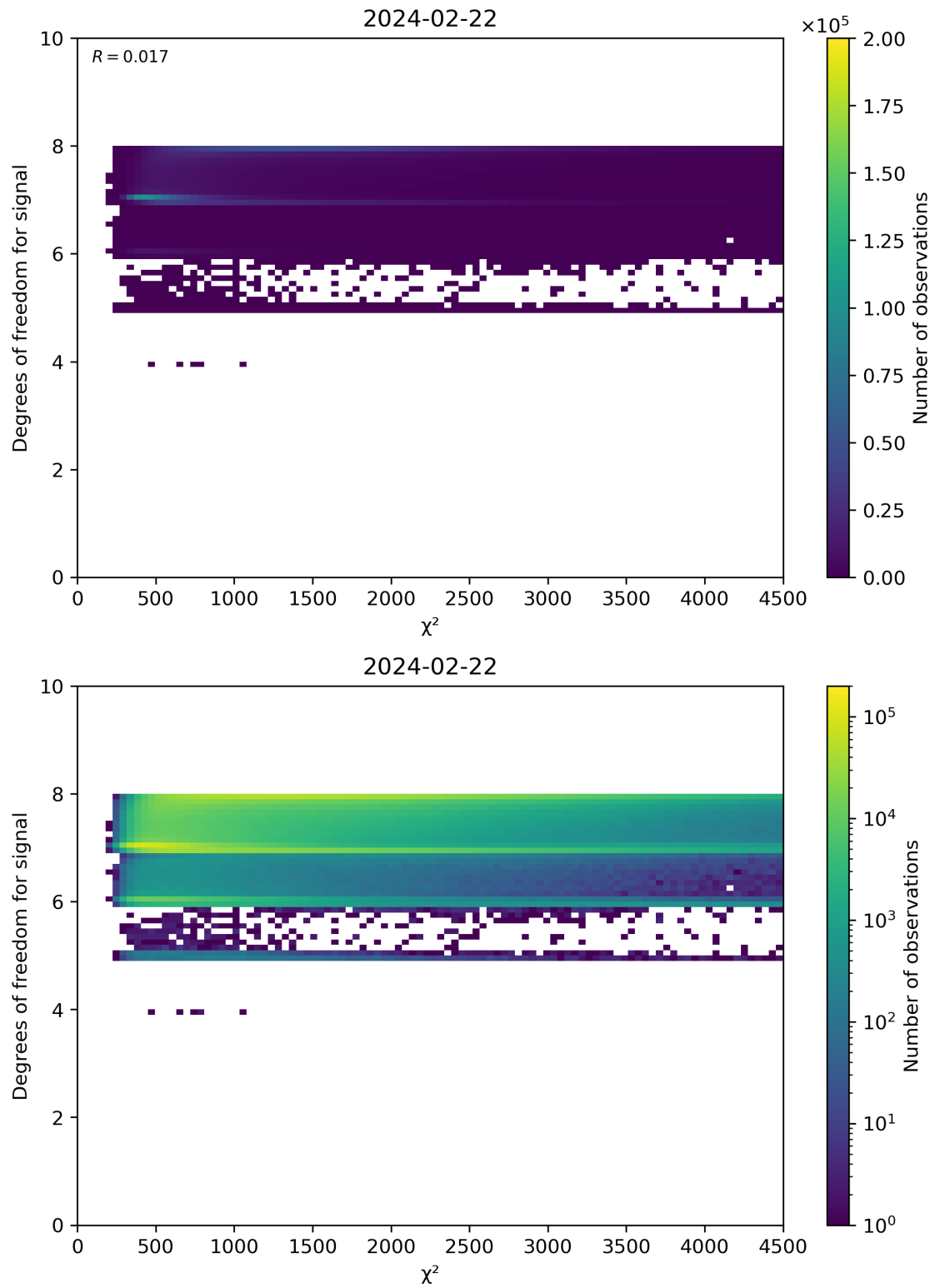
Figure 48: Scatter density plot of “ \chi^2 ” against “Degrees of freedom for signal” for 2024-02-22 to 2024-02-23.
