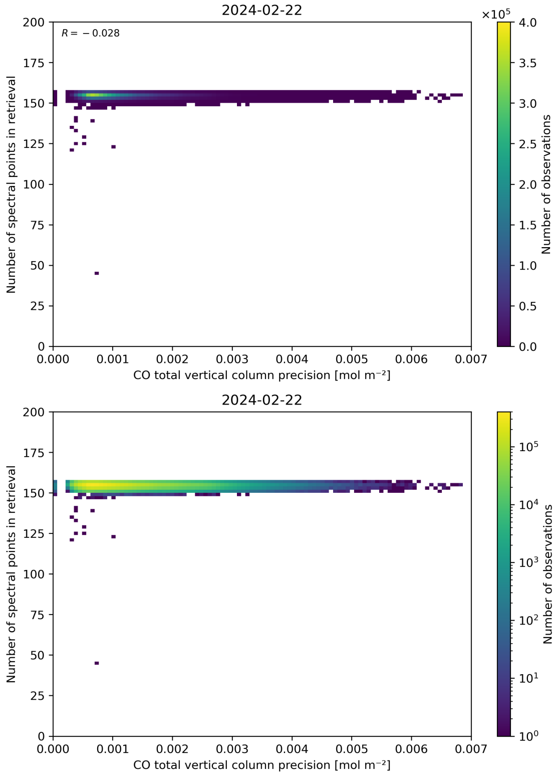
Figure 47: Scatter density plot of “CO total vertical column precision” against “Number of spectral points in retrieval” for 2024-02-22 to 2024-02-23.
