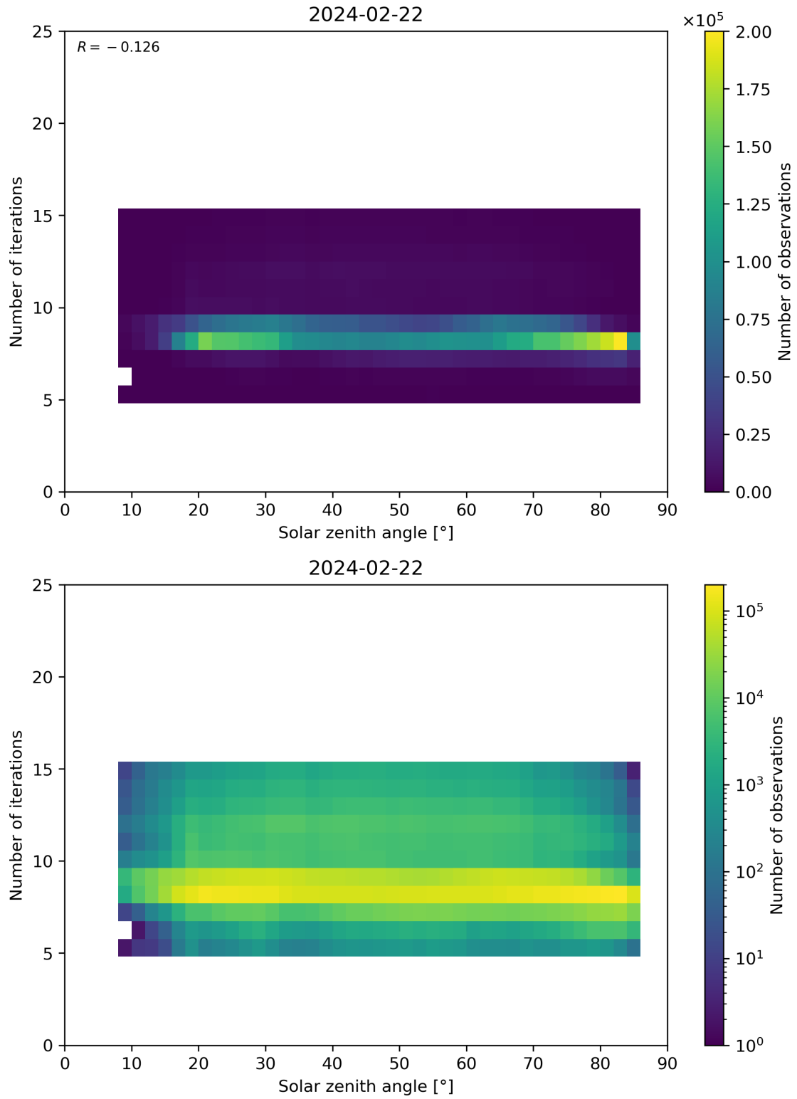
Figure 67: Scatter density plot of “Solar zenith angle” against “Number of iterations” for 2024-02-22 to 2024-02-23.
