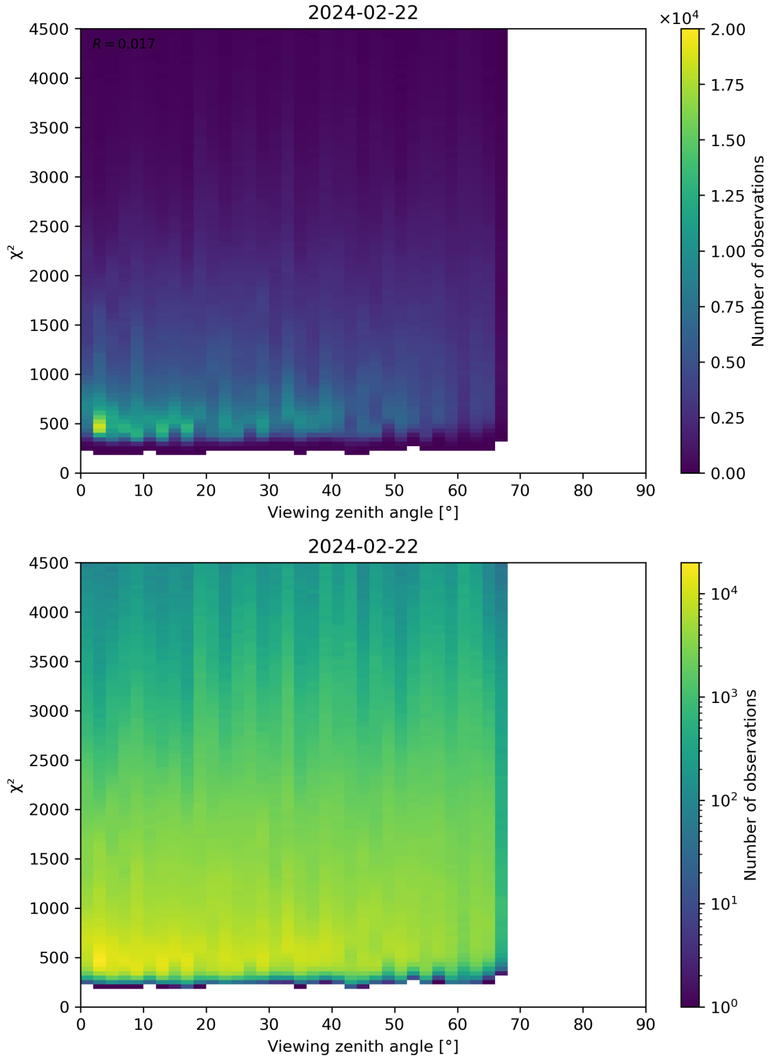
Figure 72: Scatter density plot of “Viewing zenith angle” against “ \chi^2 ” for 2024-02-22 to 2024-02-23.
