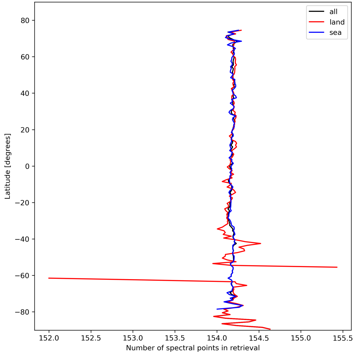
Figure 13: Zonal average of “Number of spectral points in retrieval” for 2024-02-22 to 2024-02-23.
