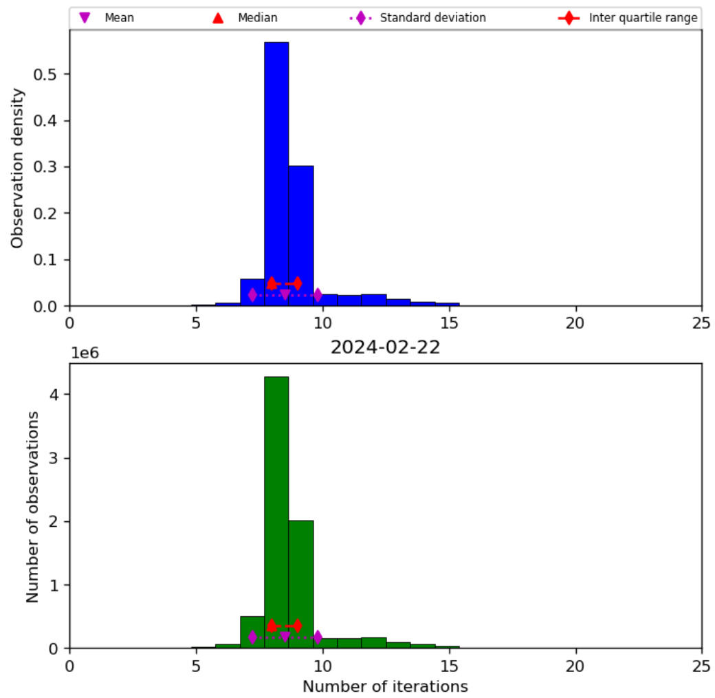
Figure 24: Histogram of “Number of iterations” for 2024-02-22 to 2024-02-23
