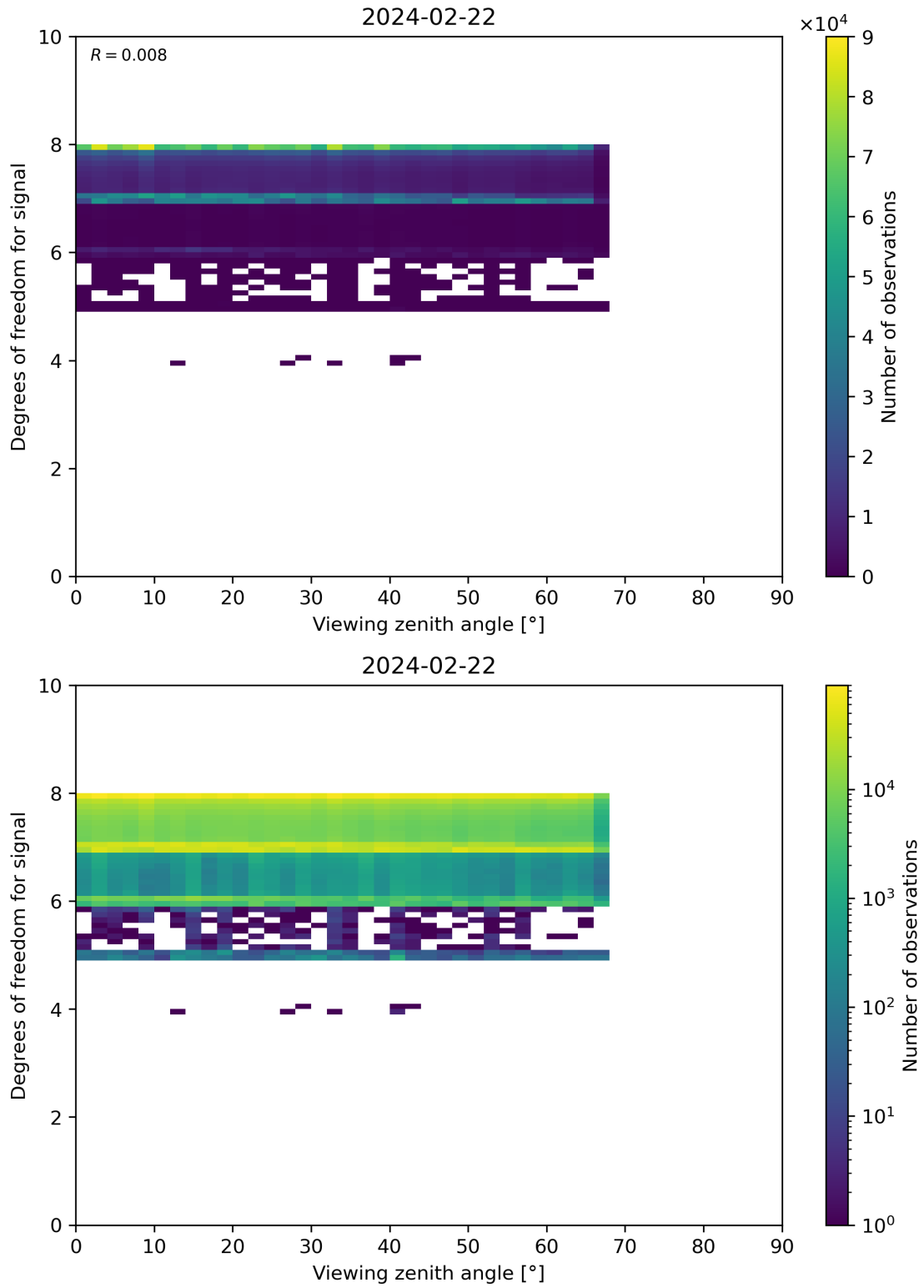
Figure 73: Scatter density plot of “Viewing zenith angle” against “Degrees of freedom for signal” for 2024-02-22 to 2024-02-23.
