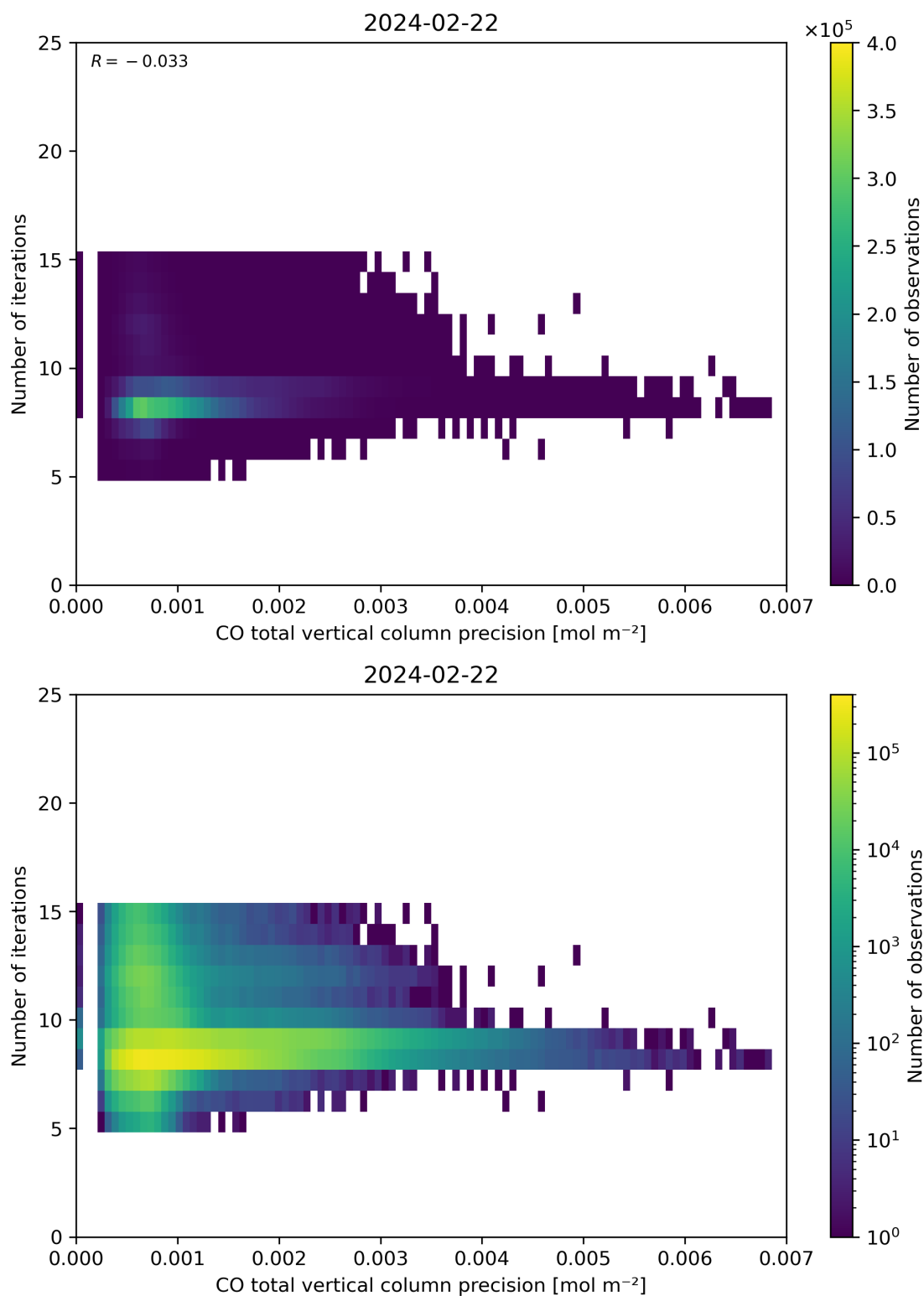
Figure 46: Scatter density plot of “CO total vertical column precision” against “Number of iterations” for 2024-02-22 to 2024-02-23.
