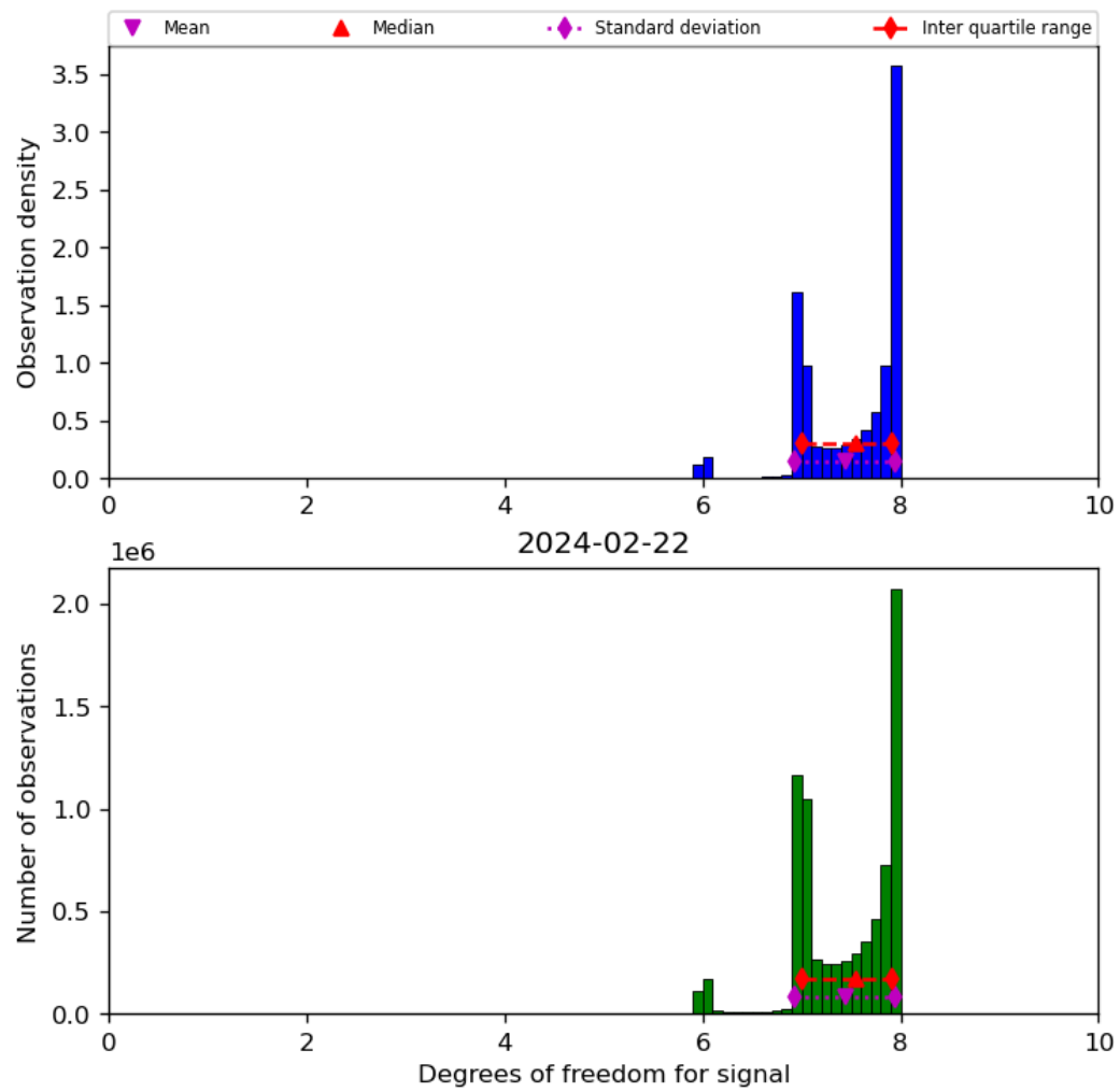
Figure 23: Histogram of “Degrees of freedom for signal” for 2024-02-22 to 2024-02-23
