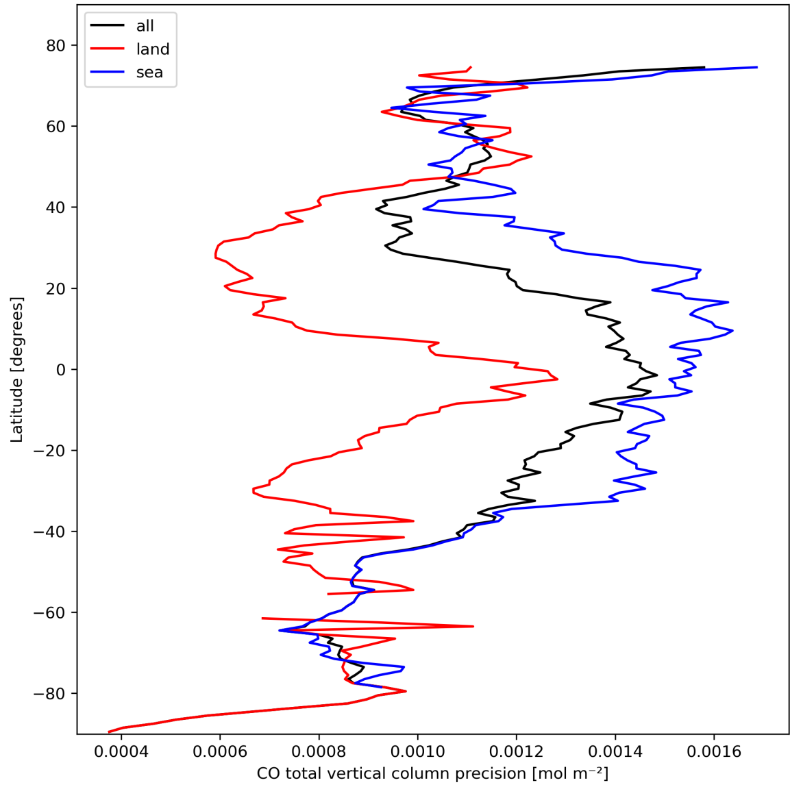
Figure 12: Zonal average of “CO total vertical column precision” for 2024-02-22 to 2024-02-23.
