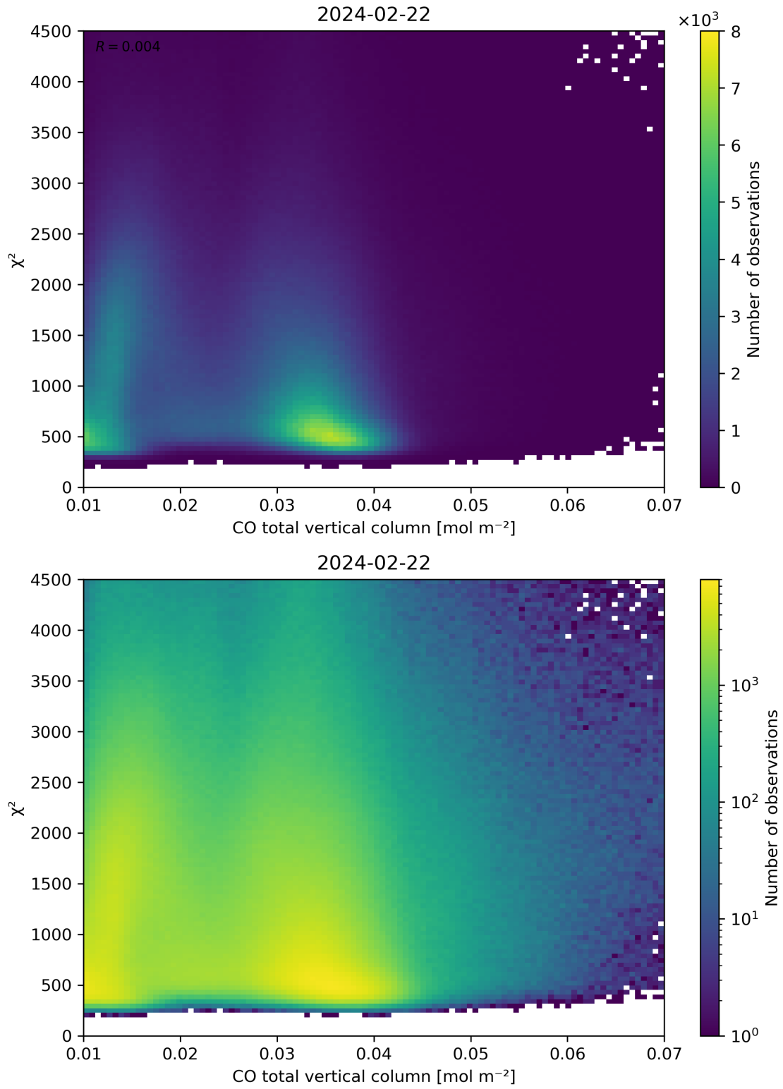
Figure 35: Scatter density plot of “CO total vertical column” against “ \chi^2 ” for 2024-02-22 to 2024-02-23.
