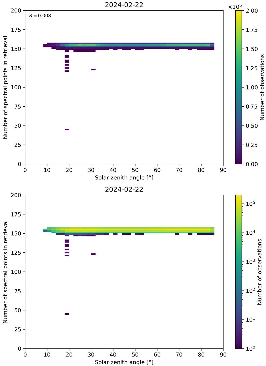
Figure 68: Scatter density plot of “Solar zenith angle” against “Number of spectral points in retrieval” for 2024-02-22 to 2024-02-23.
