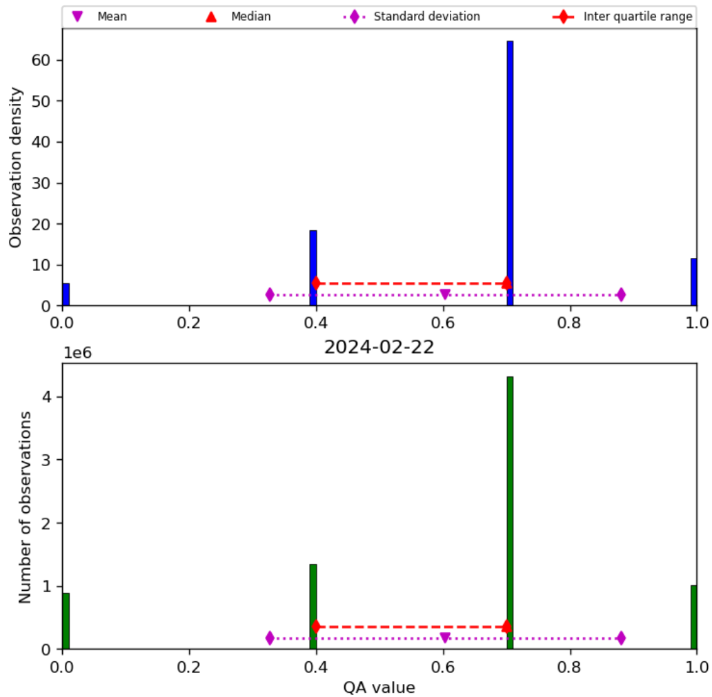
Figure 17: Histogram of “QA value” for 2024-02-22 to 2024-02-23
