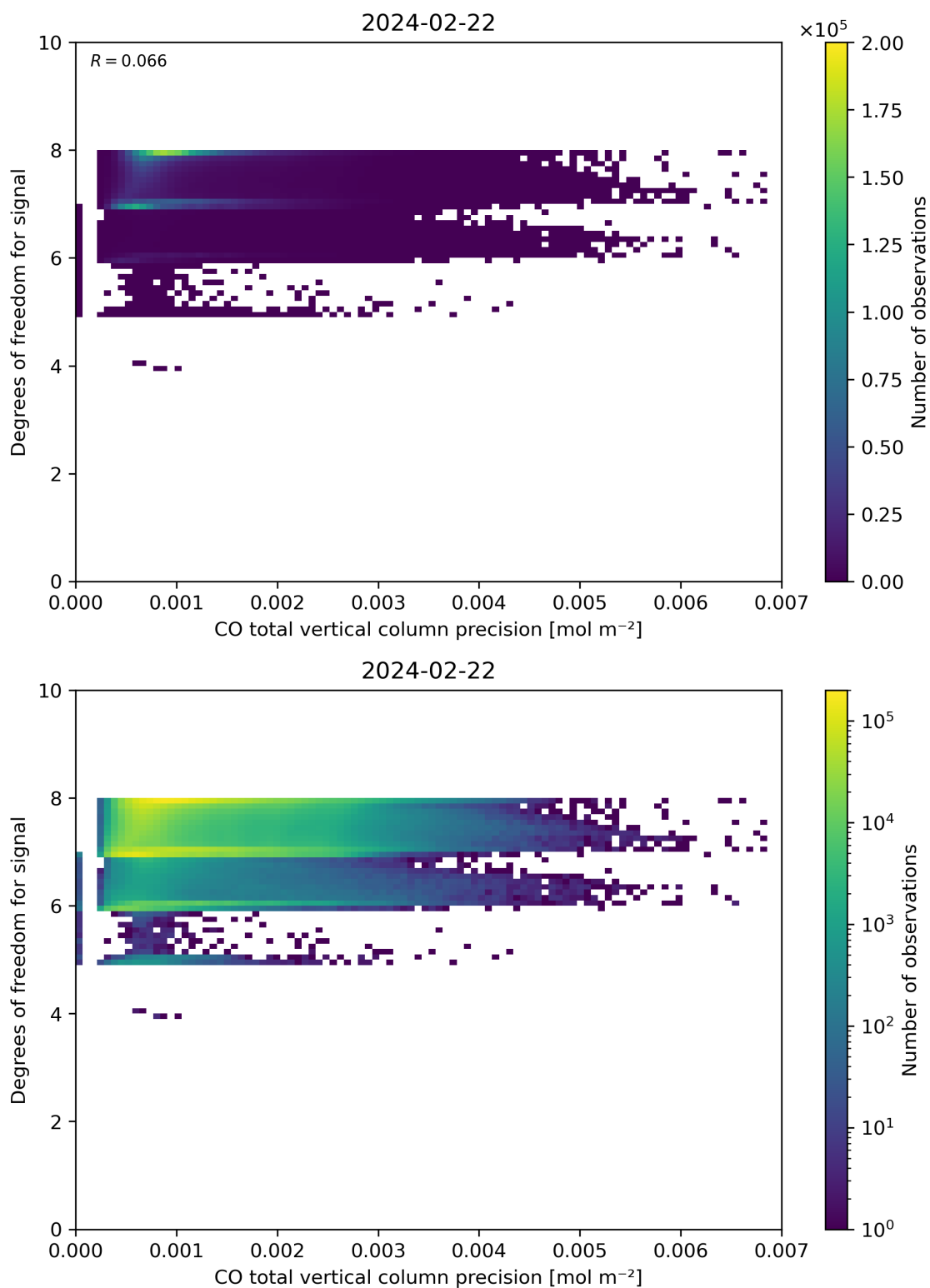
Figure 45: Scatter density plot of “CO total vertical column precision” against “Degrees of freedom for signal” for 2024-02-22 to 2024-02-23.
