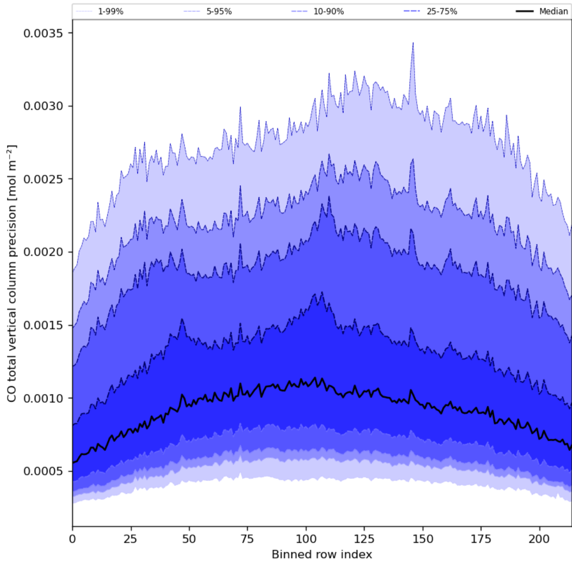
Figure 28: Along track statistics of “CO total vertical column precision” for 2024-02-22 to 2024-02-23
