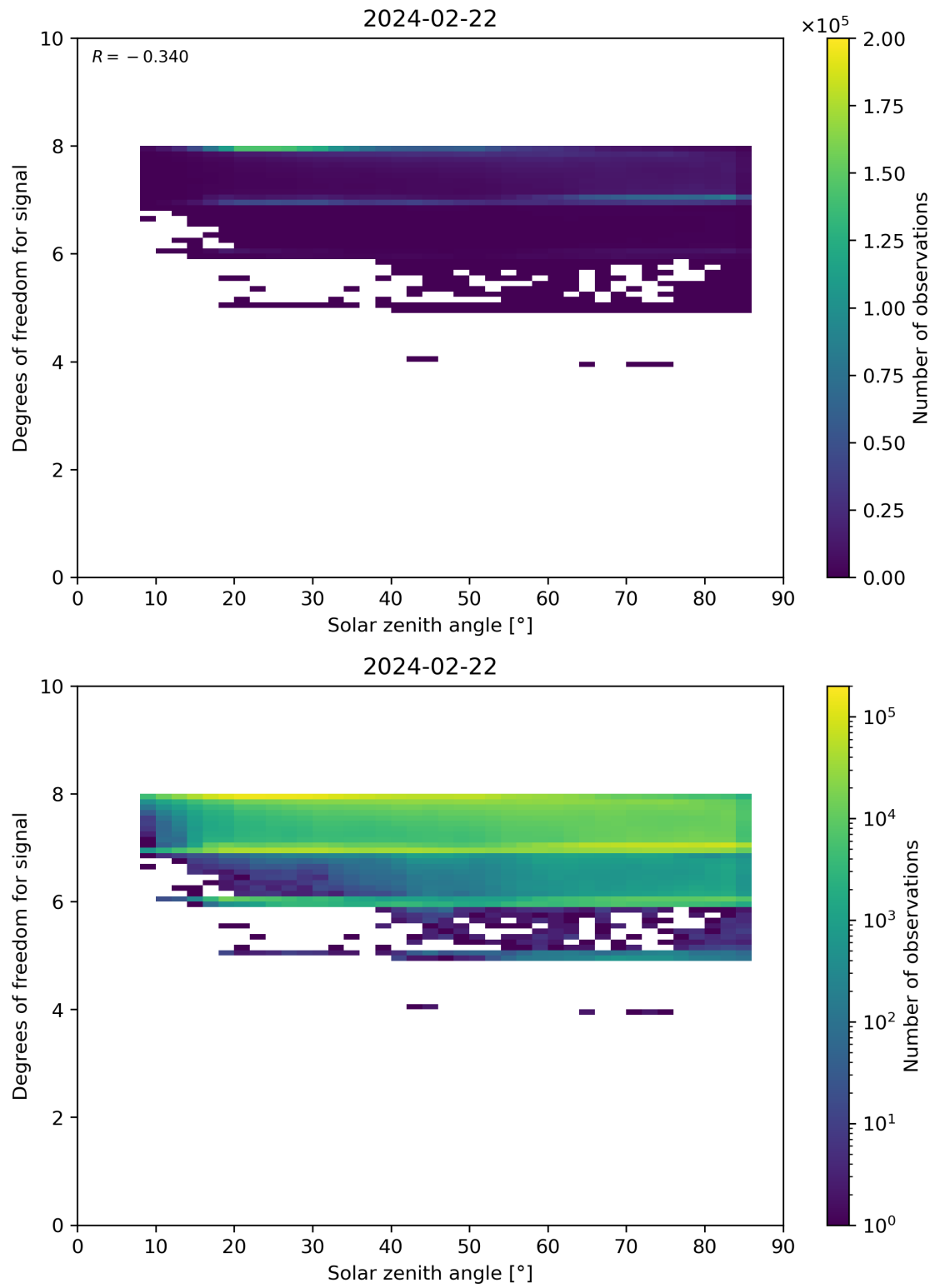
Figure 65: Scatter density plot of “Solar zenith angle” against “Degrees of freedom for signal” for 2024-02-22 to 2024-02-23.
