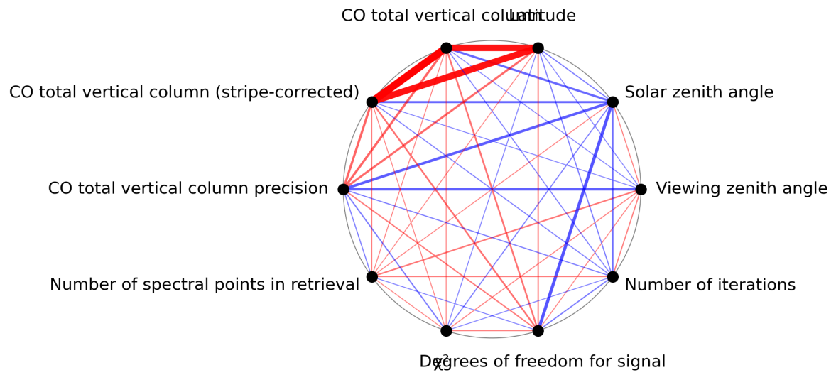
Figure 1: Map of correlation graph for 2024-02-22 to 2024-02-23.
