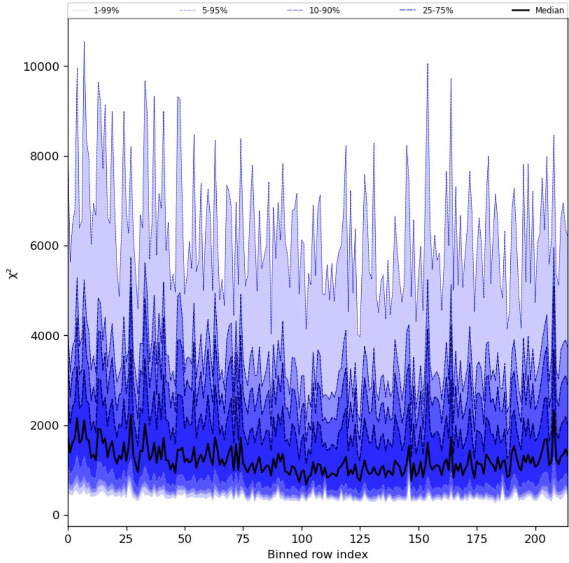
Figure 30: Along track statistics of “ \chi^2 ” for 2024-02-22 to 2024-02-23
