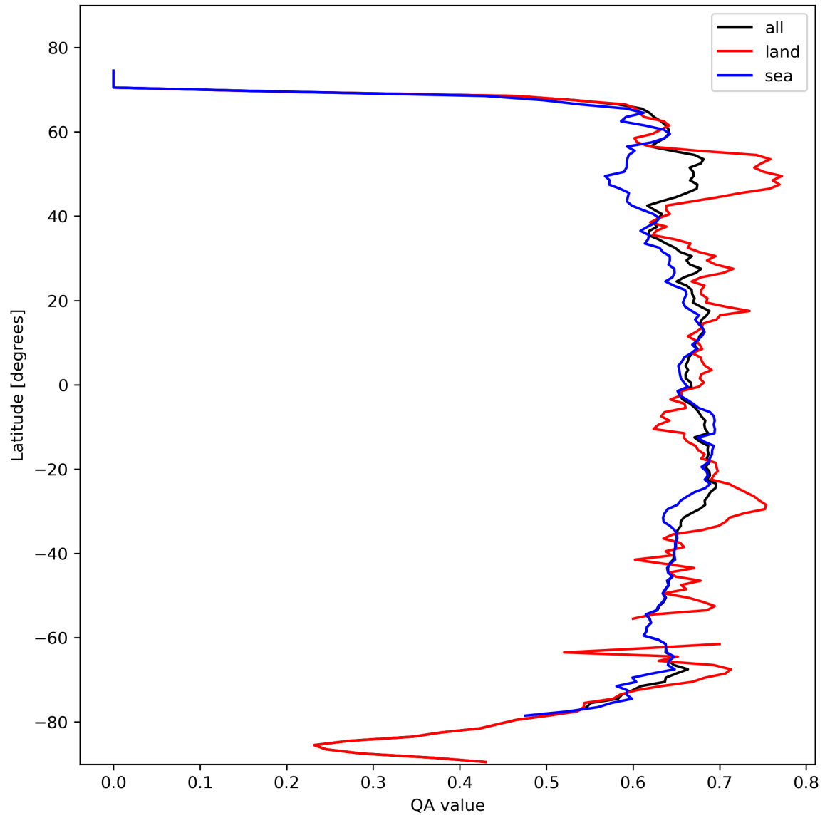
Figure 9: Zonal average of “QA value” for 2024-02-22 to 2024-02-23.
