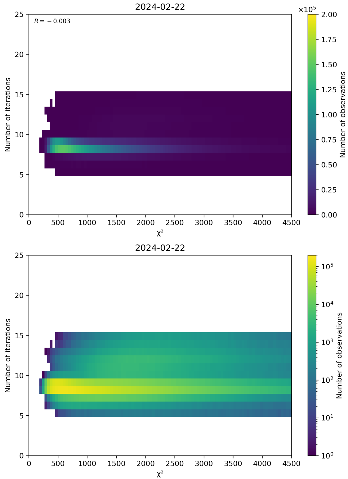
Figure 49: Scatter density plot of “ \chi^2 ” against “Number of iterations” for 2024-02-22 to 2024-02-23.
