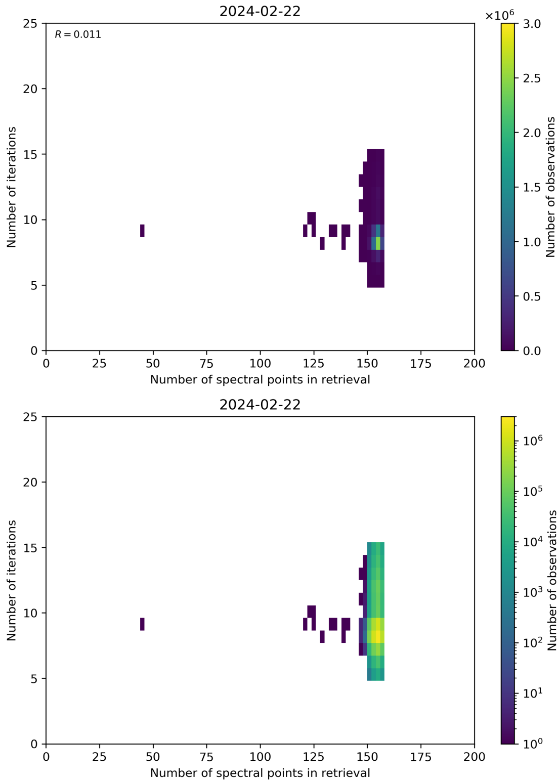
Figure 60: Scatter density plot of “Number of spectral points in retrieval” against “Number of iterations” for 2024-02-22 to 2024-02-23.
