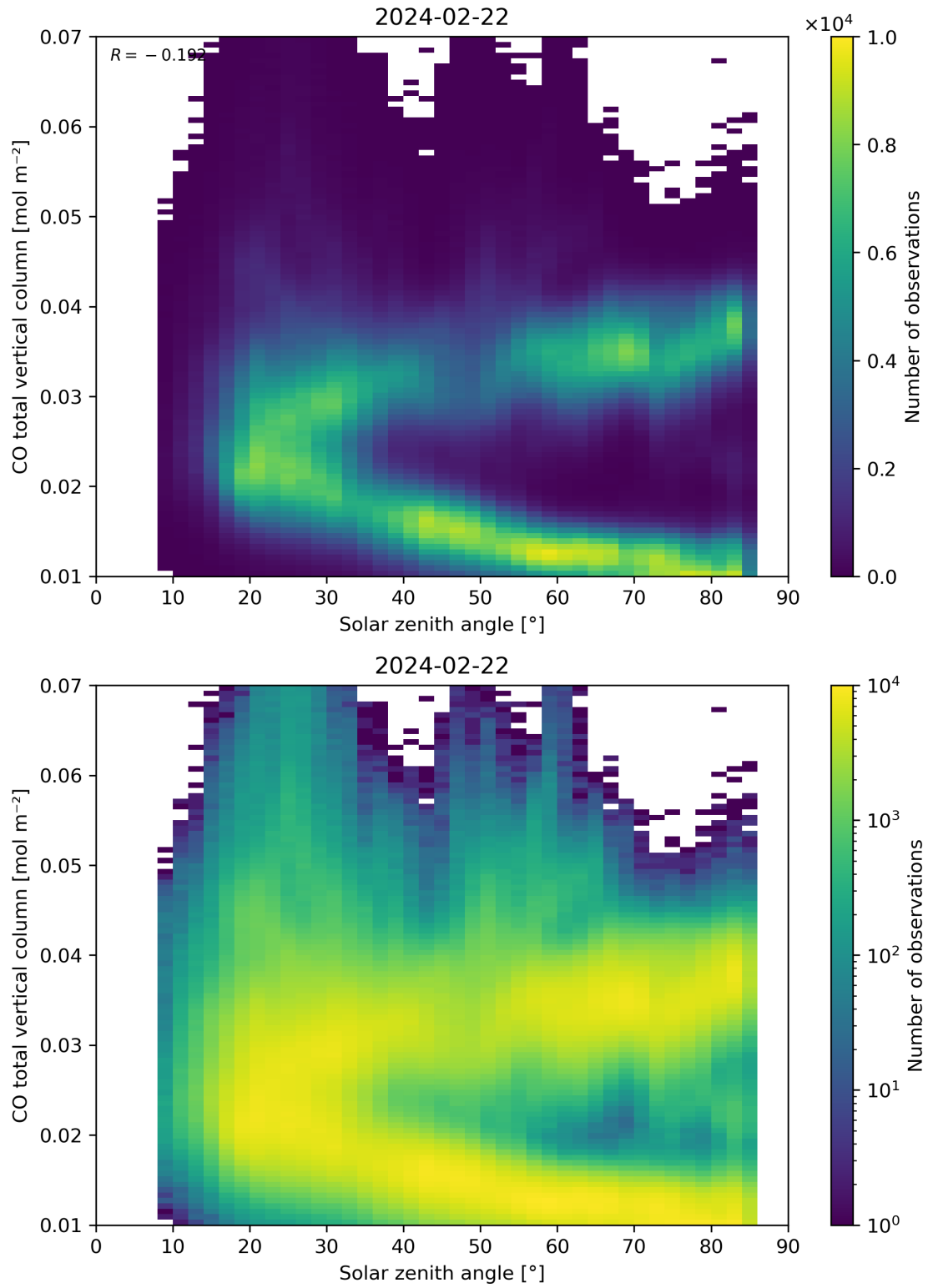
Figure 61: Scatter density plot of “Solar zenith angle” against “CO total vertical column” for 2024-02-22 to 2024-02-23.
