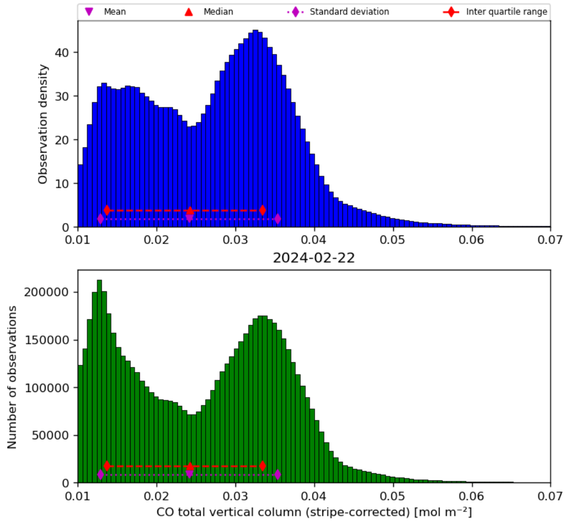
Figure 19: Histogram of “CO total vertical column (stripe-corrected)” for 2024-02-22 to 2024-02-23
