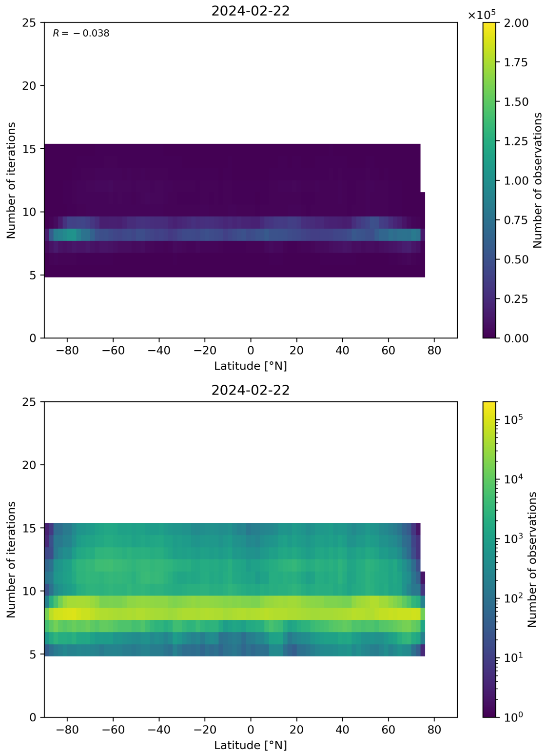
Figure 56: Scatter density plot of “Latitude” against “Number of iterations” for 2024-02-22 to 2024-02-23.
