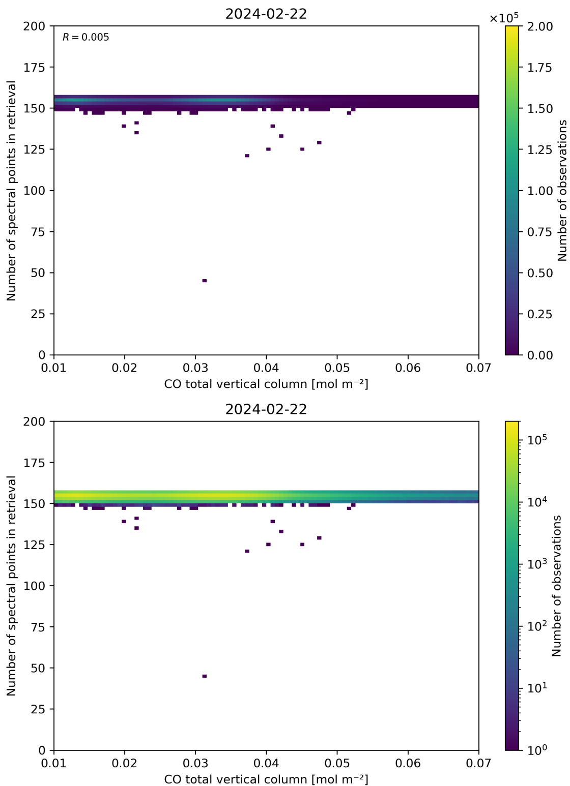
Figure 43: Scatter density plot of “CO total vertical column” against “Number of spectral points in retrieval” for 2024-02-22 to 2024-02-23.
