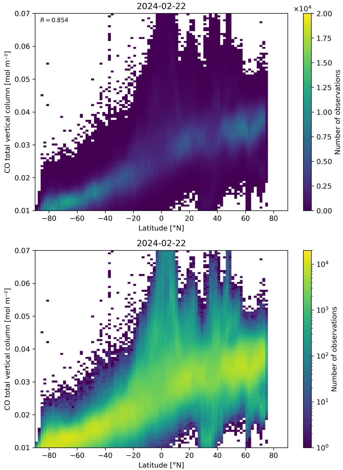
Figure 51: Scatter density plot of “Latitude” against “CO total vertical column” for 2024-02-22 to 2024-02-23.
