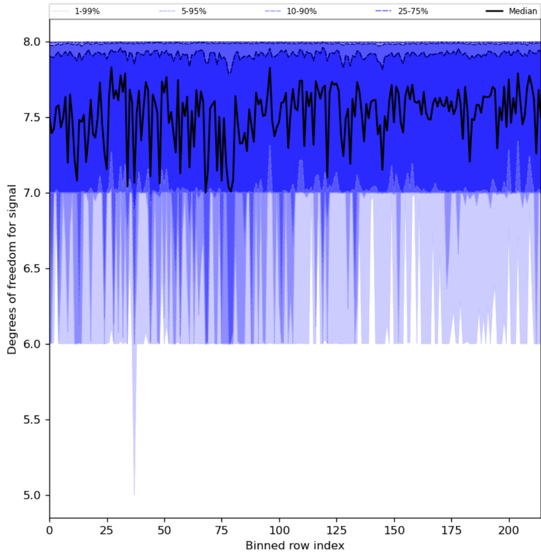
Figure 31: Along track statistics of “Degrees of freedom for signal” for 2024-02-22 to 2024-02-23
