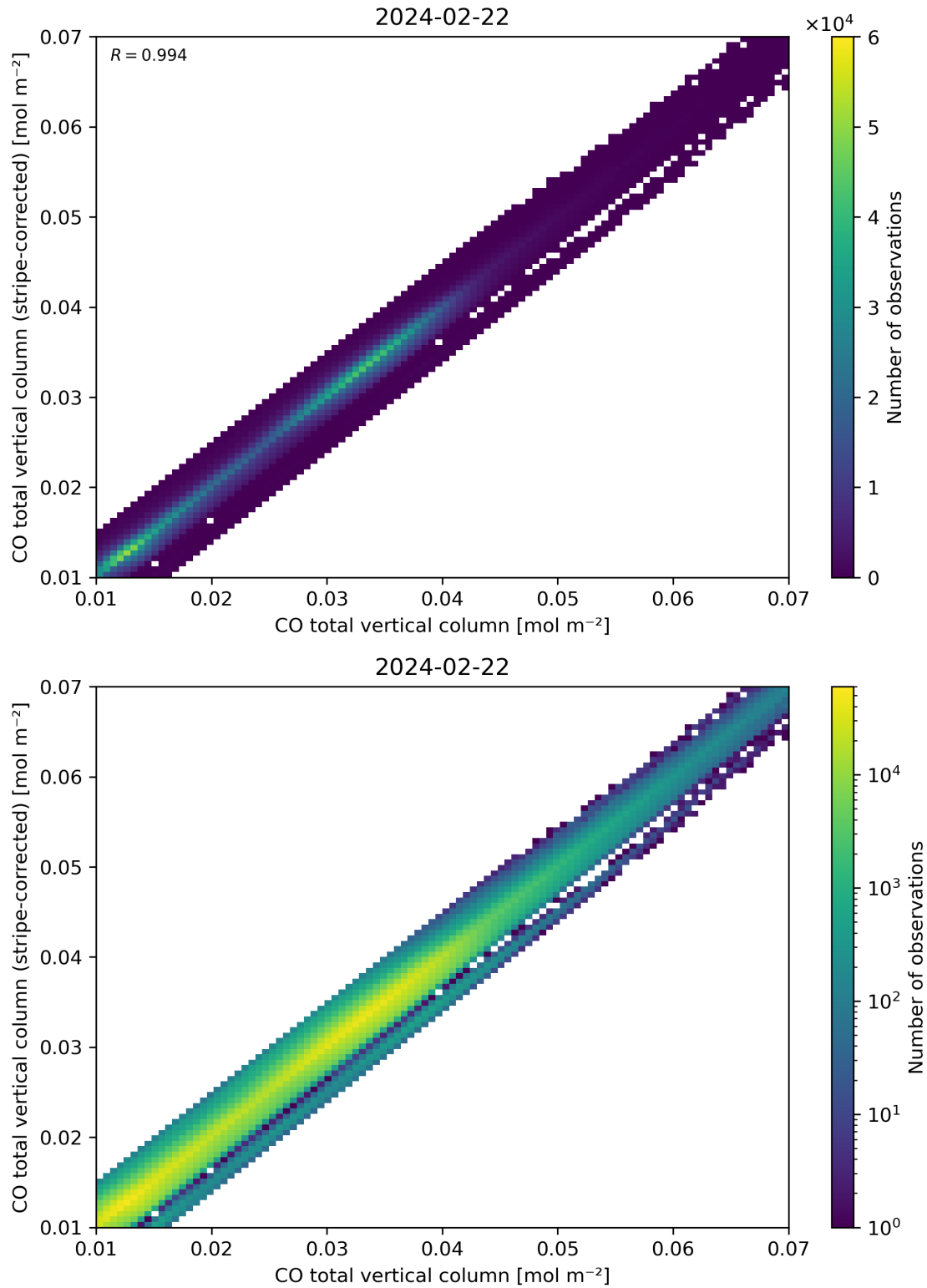
Figure 33: Scatter density plot of “CO total vertical column” against “CO total vertical column (stripe-corrected)” for 2024-02-22 to 2024-02-23.
