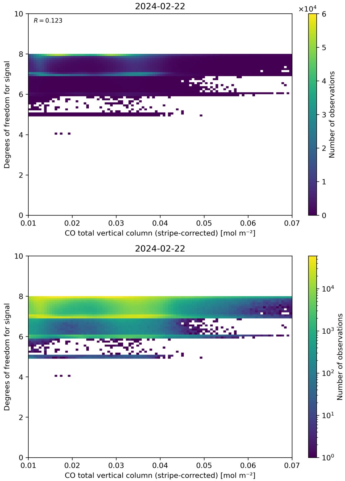
Figure 38: Scatter density plot of “CO total vertical column (stripe-corrected)” against “Degrees of freedom for signal” for 2024-02-22 to 2024-02-23.
