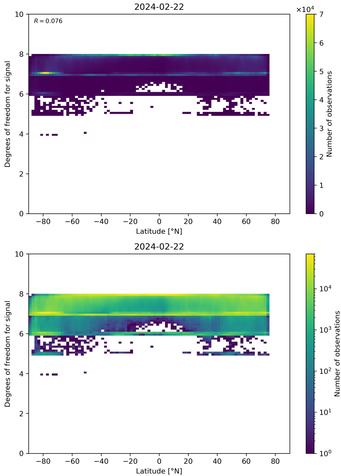
Figure 55: Scatter density plot of “Latitude” against “Degrees of freedom for signal” for 2024-02-22 to 2024-02-23.
