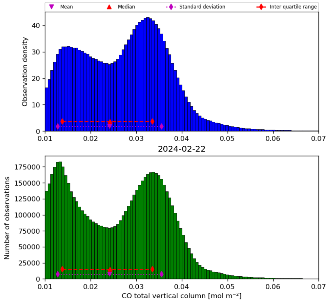
Figure 18: Histogram of “CO total vertical column” for 2024-02-22 to 2024-02-23
