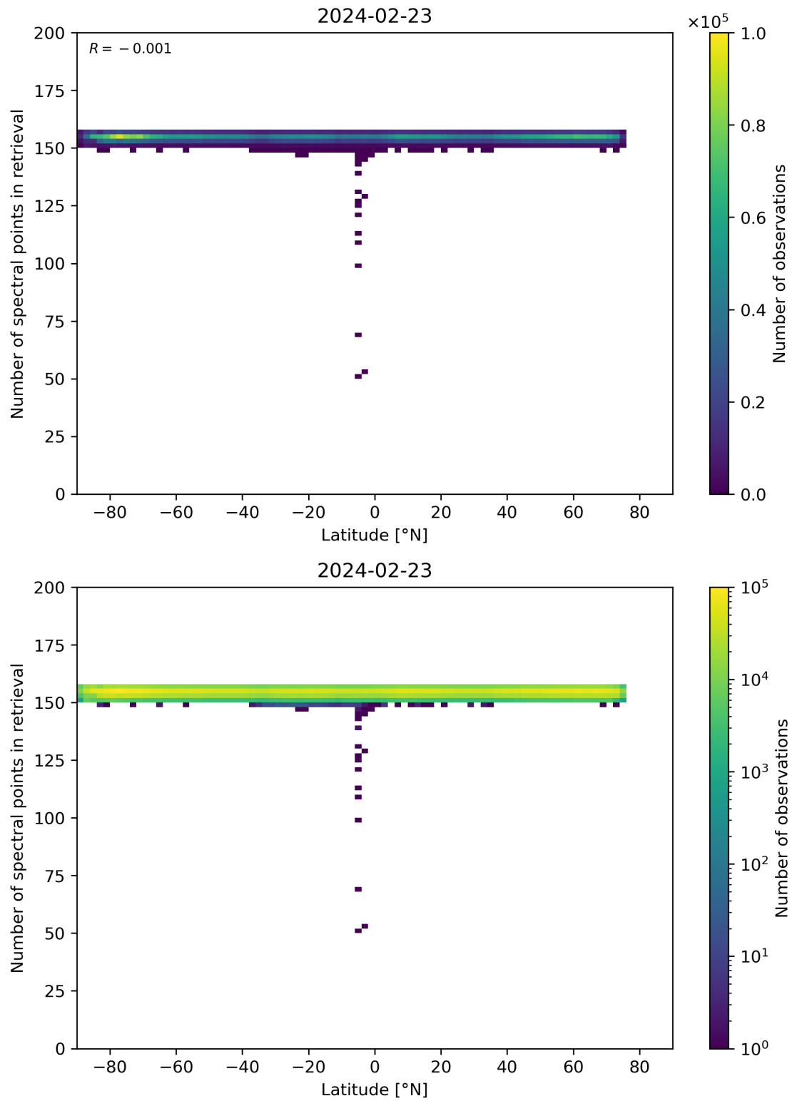
Figure 57: Scatter density plot of “Latitude” against “Number of spectral points in retrieval” for 2024-02-22 to 2024-02-24.
