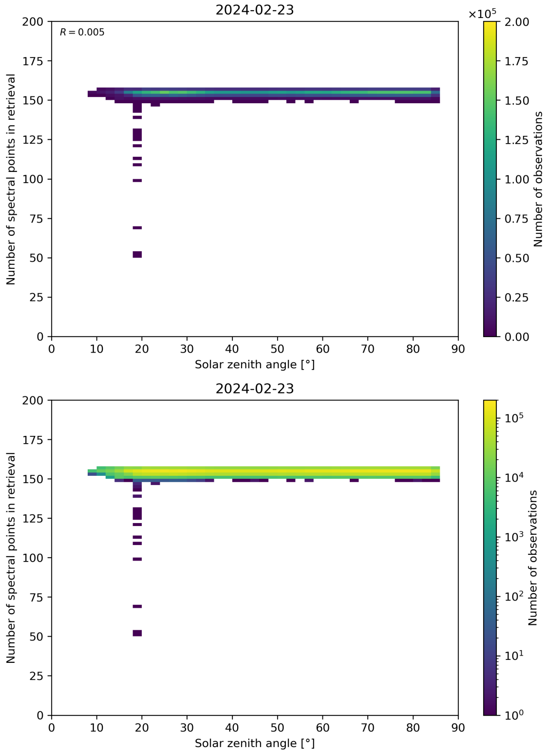
Figure 68: Scatter density plot of “Solar zenith angle” against “Number of spectral points in retrieval” for 2024-02-22 to 2024-02-24.
