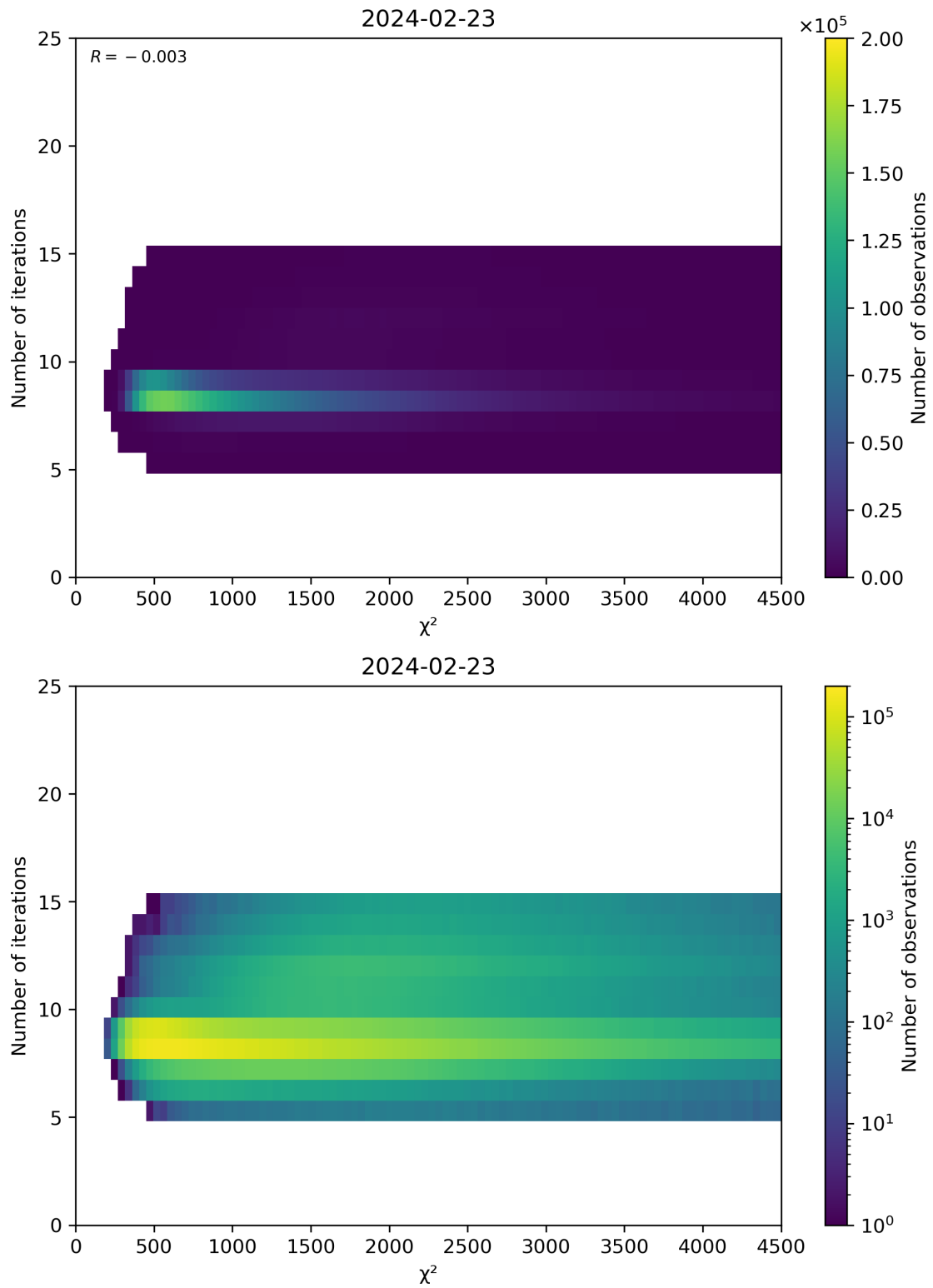
Figure 49: Scatter density plot of “ \chi^2 ” against “Number of iterations” for 2024-02-22 to 2024-02-24.
