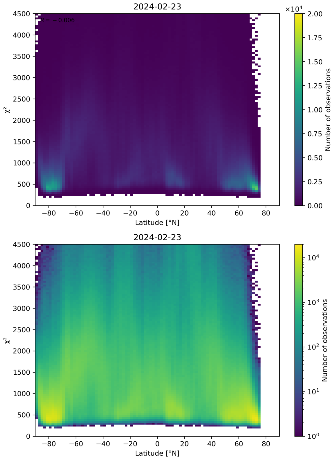
Figure 54: Scatter density plot of “Latitude” against “ \chi^2 ” for 2024-02-22 to 2024-02-24.
