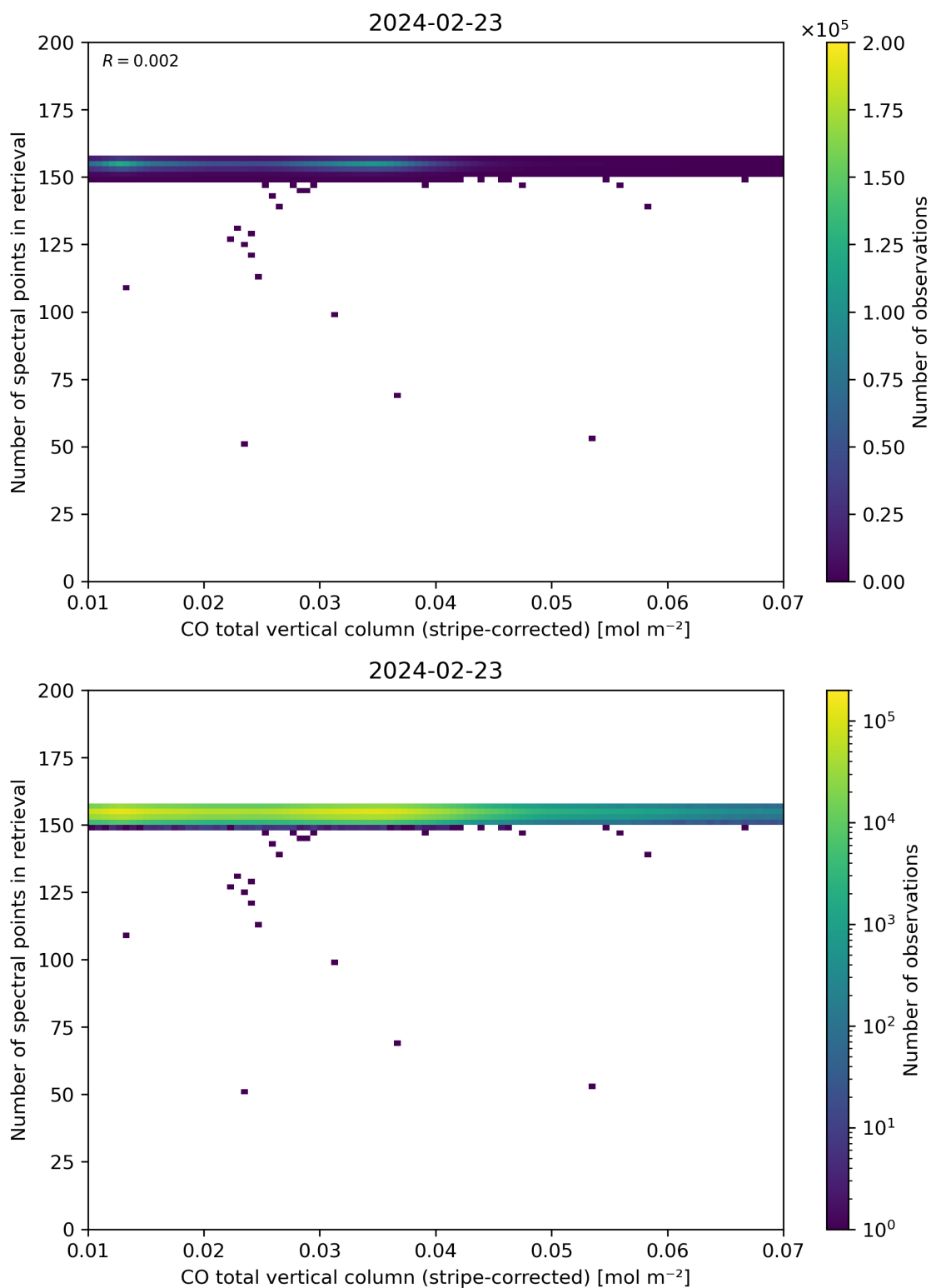
Figure 40: Scatter density plot of “CO total vertical column (stripe-corrected)” against “Number of spectral points in retrieval” for 2024-02-22 to 2024-02-24.
