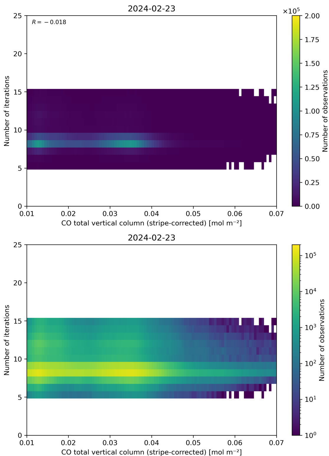
Figure 39: Scatter density plot of “CO total vertical column (stripe-corrected)” against “Number of iterations” for 2024-02-22 to 2024-02-24.
