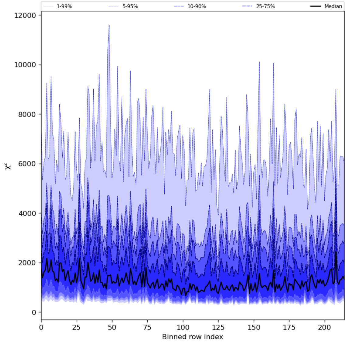
Figure 30: Along track statistics of “ \chi^2 ” for 2024-02-22 to 2024-02-24
