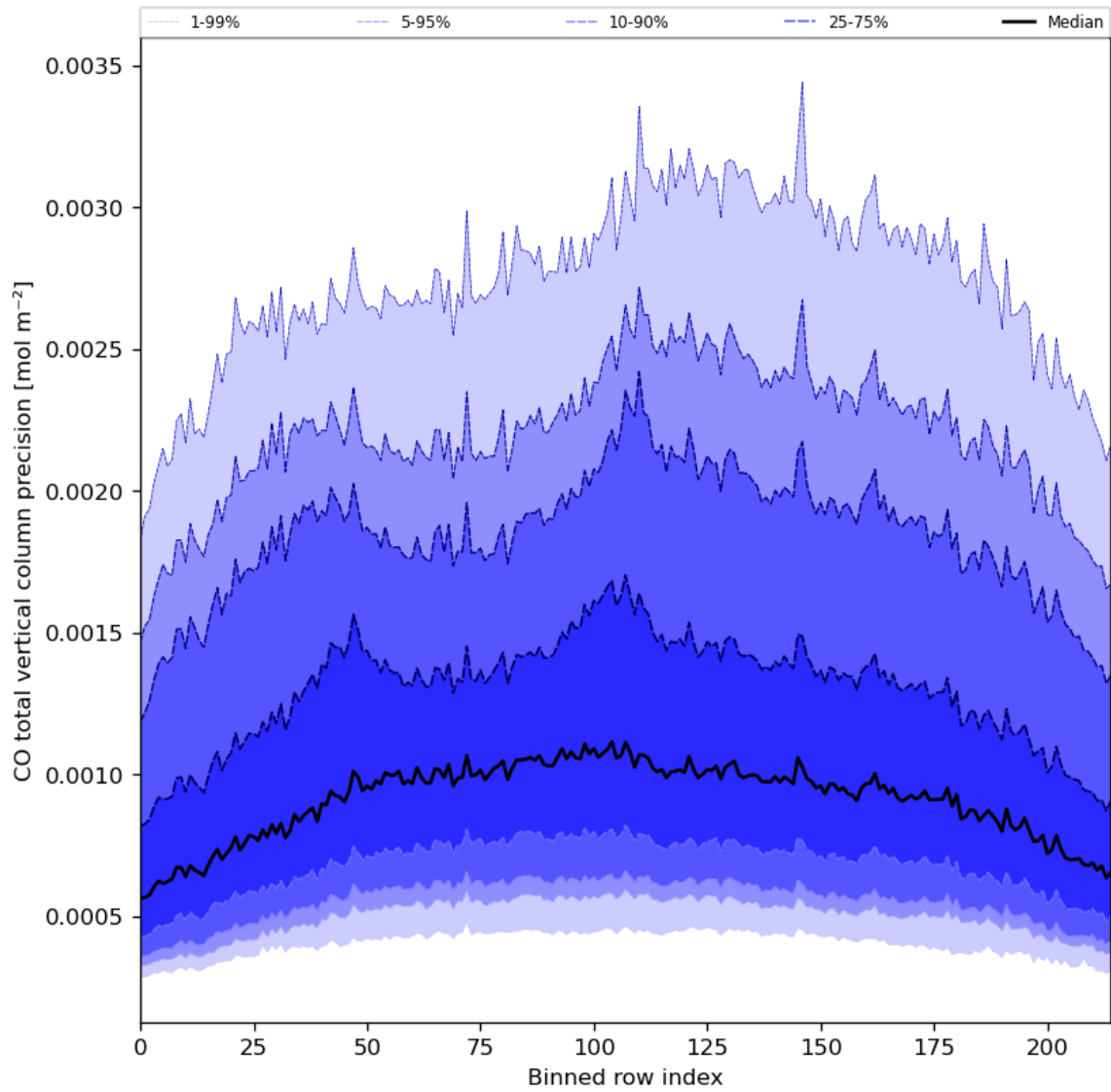
Figure 28: Along track statistics of “CO total vertical column precision” for 2024-02-22 to 2024-02-24
