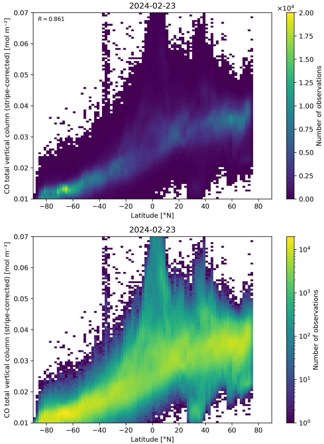
Figure 52: Scatter density plot of “Latitude” against “CO total vertical column (stripe-corrected)” for 2024-02-22 to 2024-02-24.
