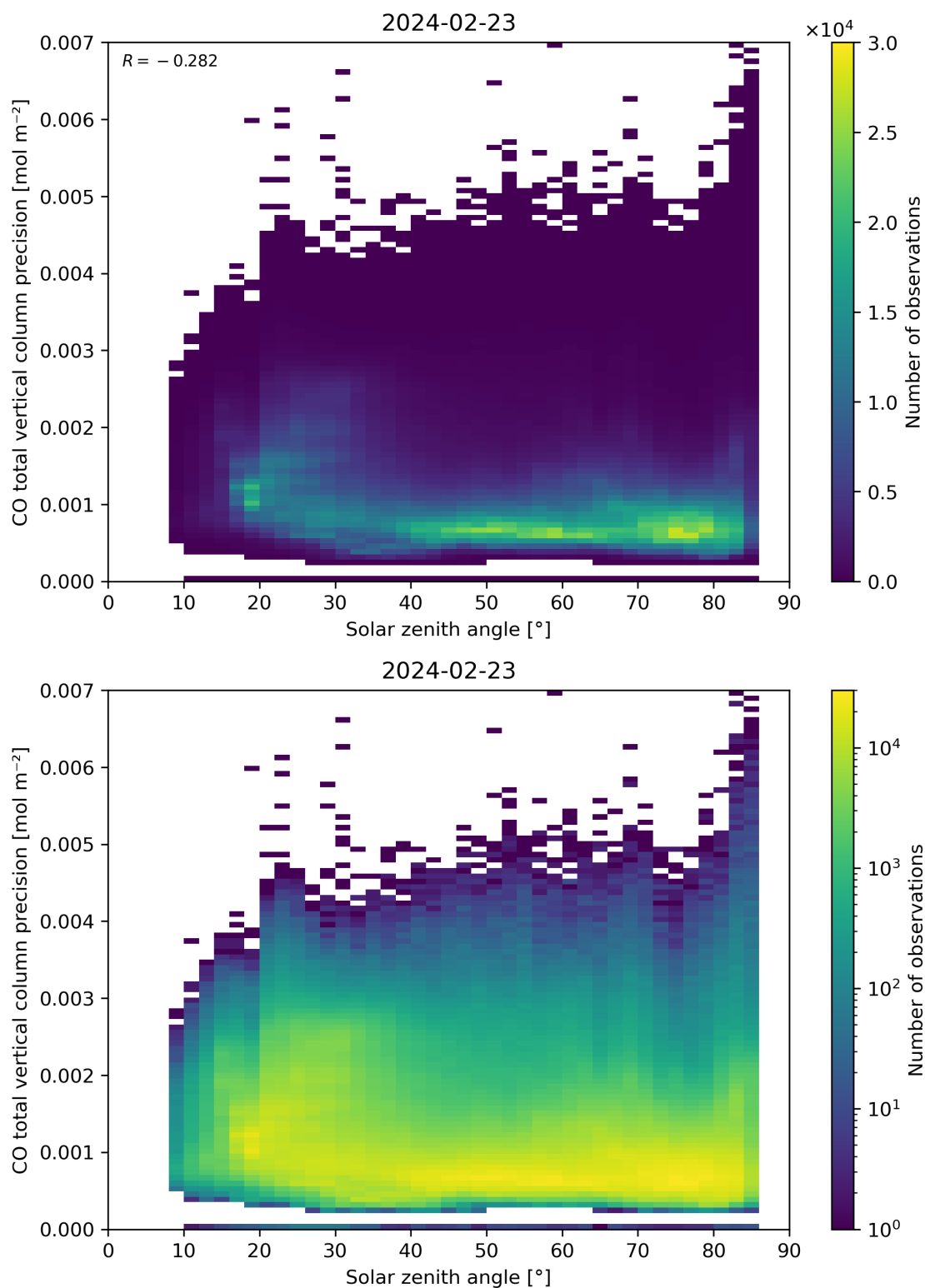
Figure 63: Scatter density plot of “Solar zenith angle” against “CO total vertical column precision” for 2024-02-22 to 2024-02-24.
