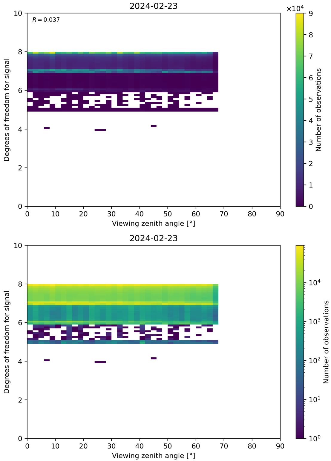
Figure 73: Scatter density plot of “Viewing zenith angle” against “Degrees of freedom for signal” for 2024-02-22 to 2024-02-24.
