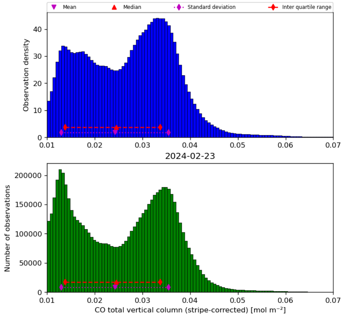
Figure 19: Histogram of “CO total vertical column (stripe-corrected)” for 2024-02-22 to 2024-02-24
