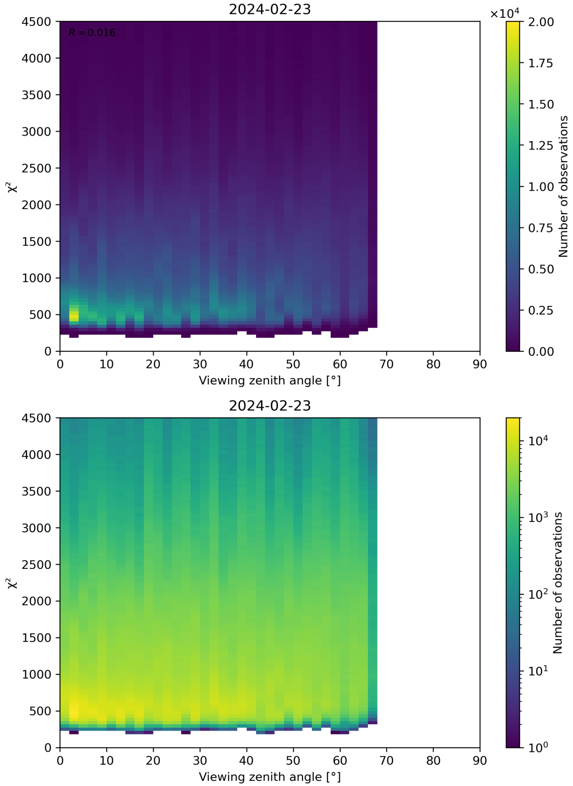
Figure 72: Scatter density plot of “Viewing zenith angle” against “ \chi^2 ” for 2024-02-22 to 2024-02-24.
