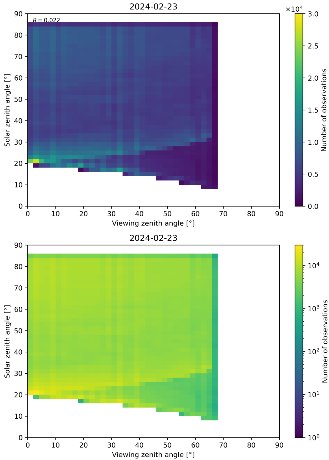
Figure 77: Scatter density plot of “Viewing zenith angle” against “Solar zenith angle” for 2024-02-22 to 2024-02-24.
