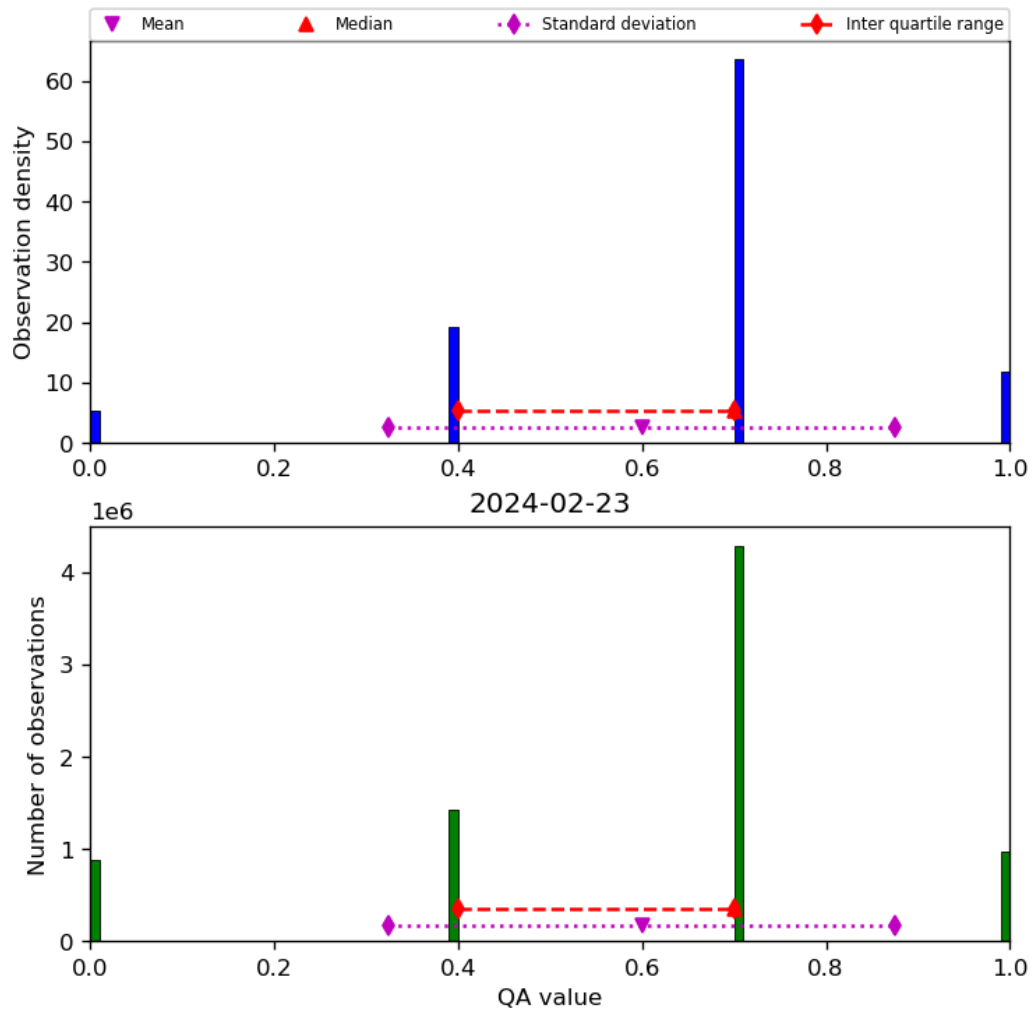
Figure 17: Histogram of “QA value” for 2024-02-22 to 2024-02-24
