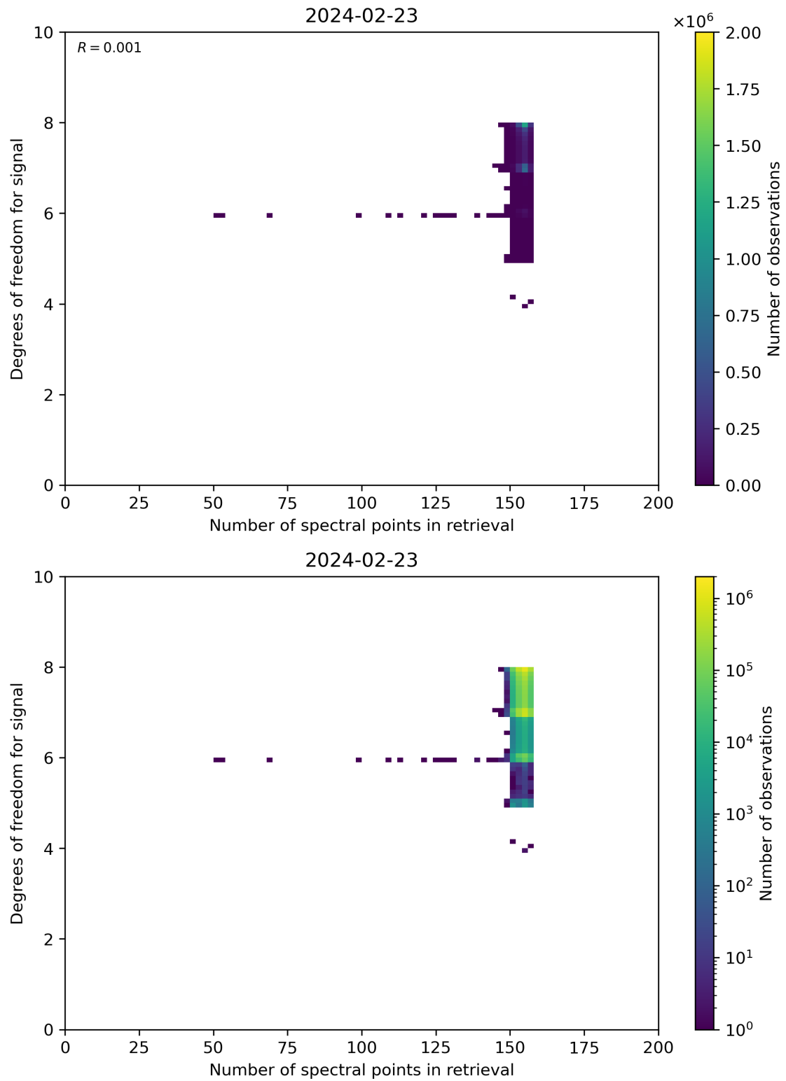
Figure 59: Scatter density plot of “Number of spectral points in retrieval” against “Degrees of freedom for signal” for 2024-02-22 to 2024-02-24.
