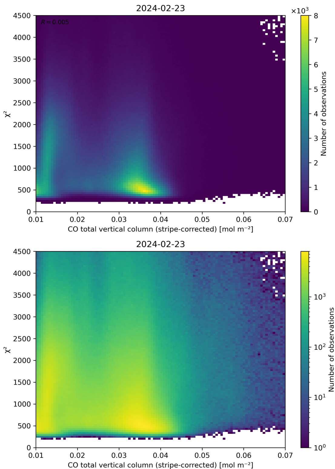
Figure 37: Scatter density plot of “CO total vertical column (stripe-corrected)” against “ \chi^2 ” for 2024-02-22 to 2024-02-24.
