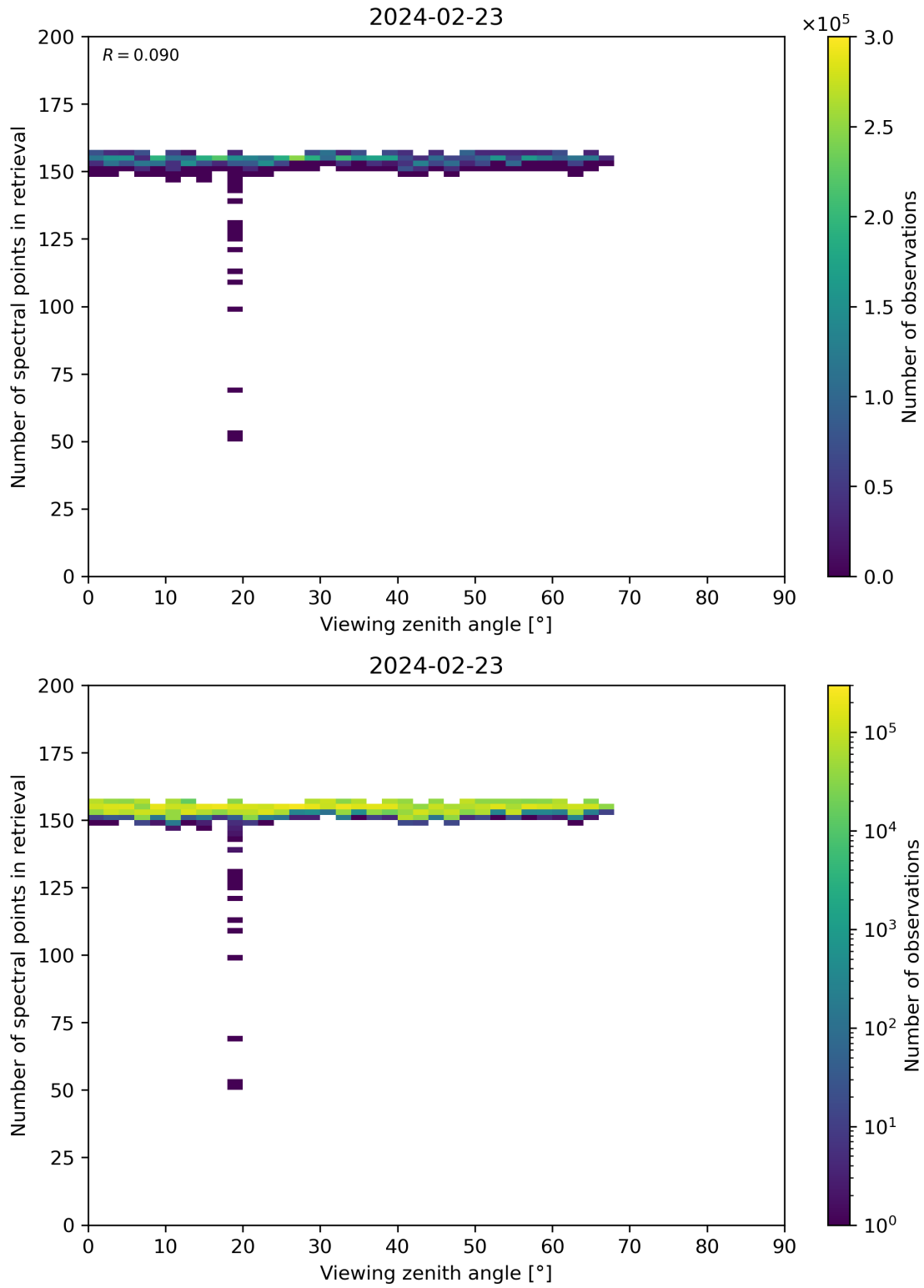
Figure 76: Scatter density plot of “Viewing zenith angle” against “Number of spectral points in retrieval” for 2024-02-22 to 2024-02-24.
