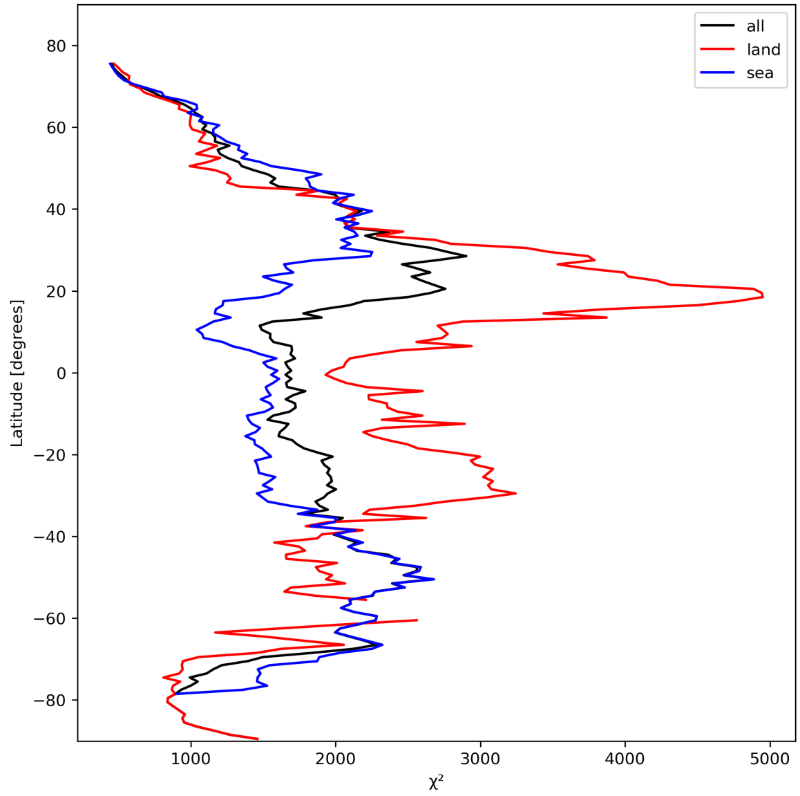
Figure 14: Zonal average of “ \chi^2 ” for 2024-02-22 to 2024-02-24.
