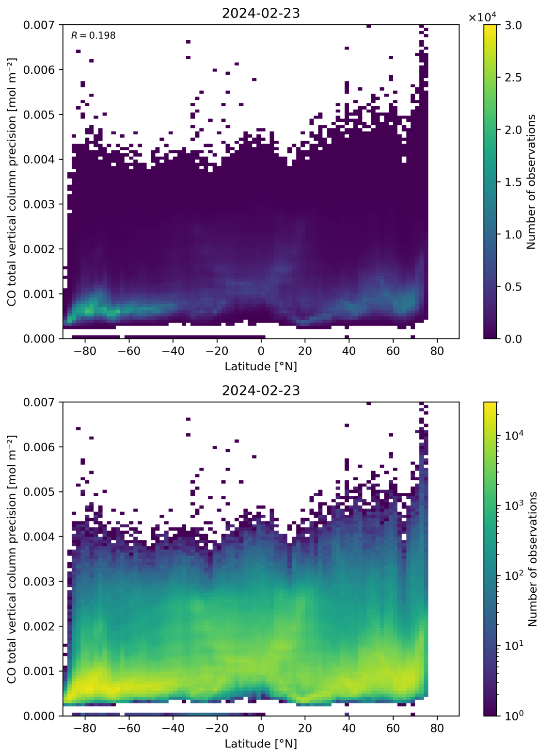
Figure 53: Scatter density plot of “Latitude” against “CO total vertical column precision” for 2024-02-22 to 2024-02-24.
