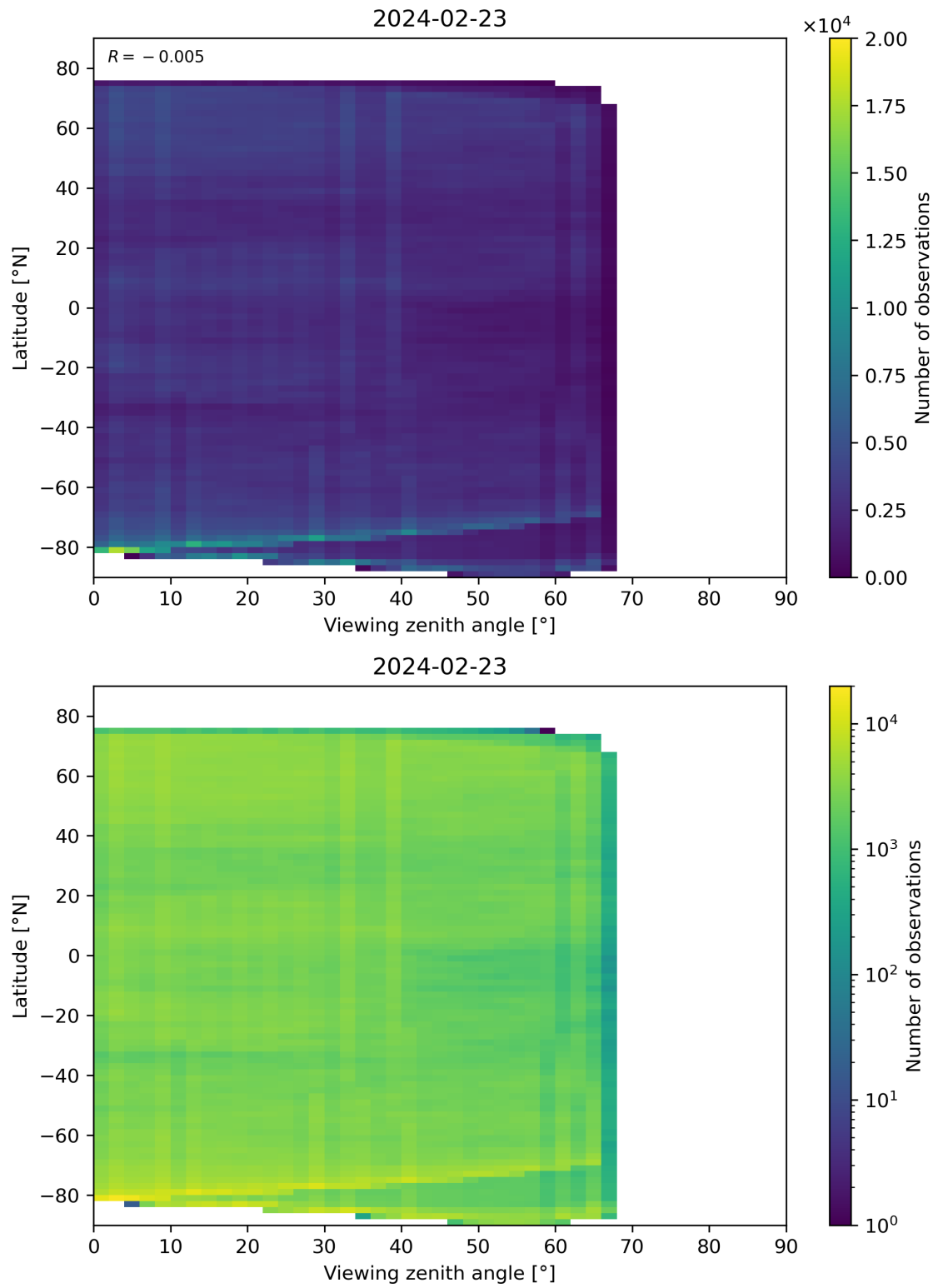
Figure 74: Scatter density plot of “Viewing zenith angle” against “Latitude” for 2024-02-22 to 2024-02-24.
