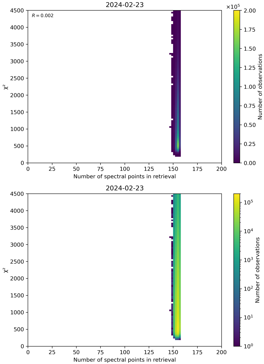
Figure 58: Scatter density plot of “Number of spectral points in retrieval” against “ \chi^2 ” for 2024-02-22 to 2024-02-24.
