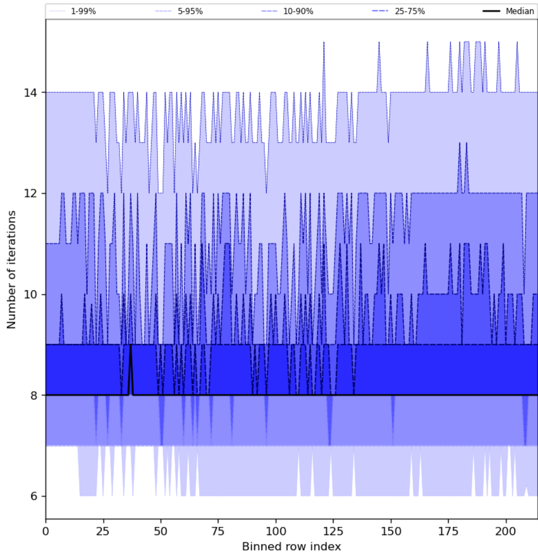
Figure 32: Along track statistics of “Number of iterations” for 2024-02-22 to 2024-02-24
