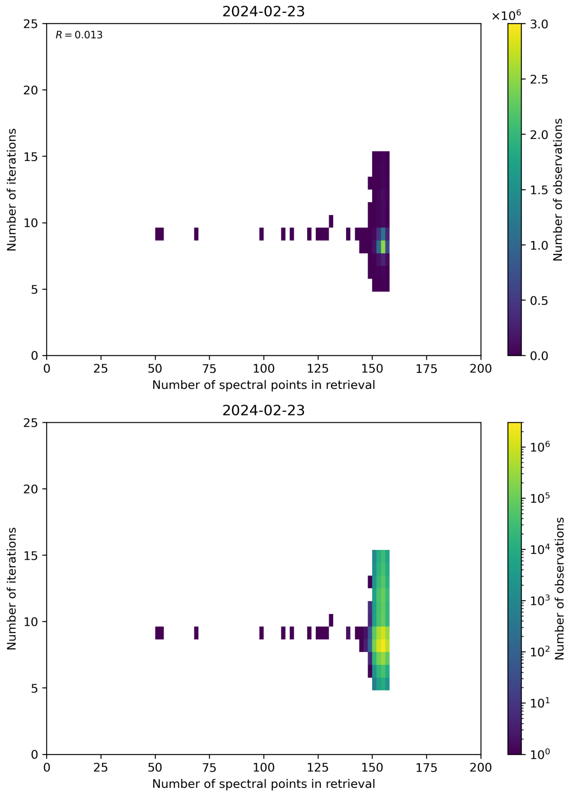
Figure 60: Scatter density plot of “Number of spectral points in retrieval” against “Number of iterations” for 2024-02-22 to 2024-02-24.
