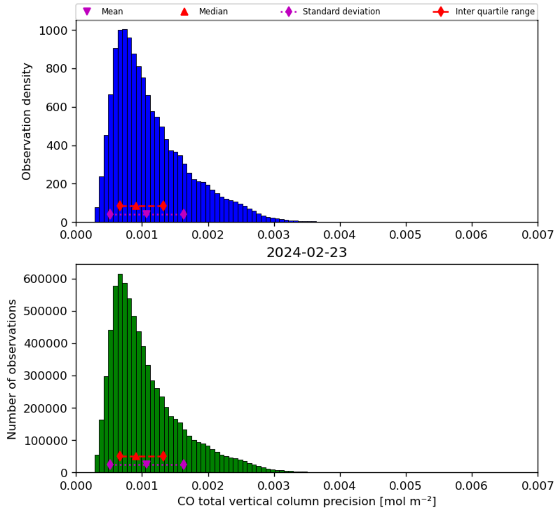
Figure 20: Histogram of “CO total vertical column precision” for 2024-02-22 to 2024-02-24
