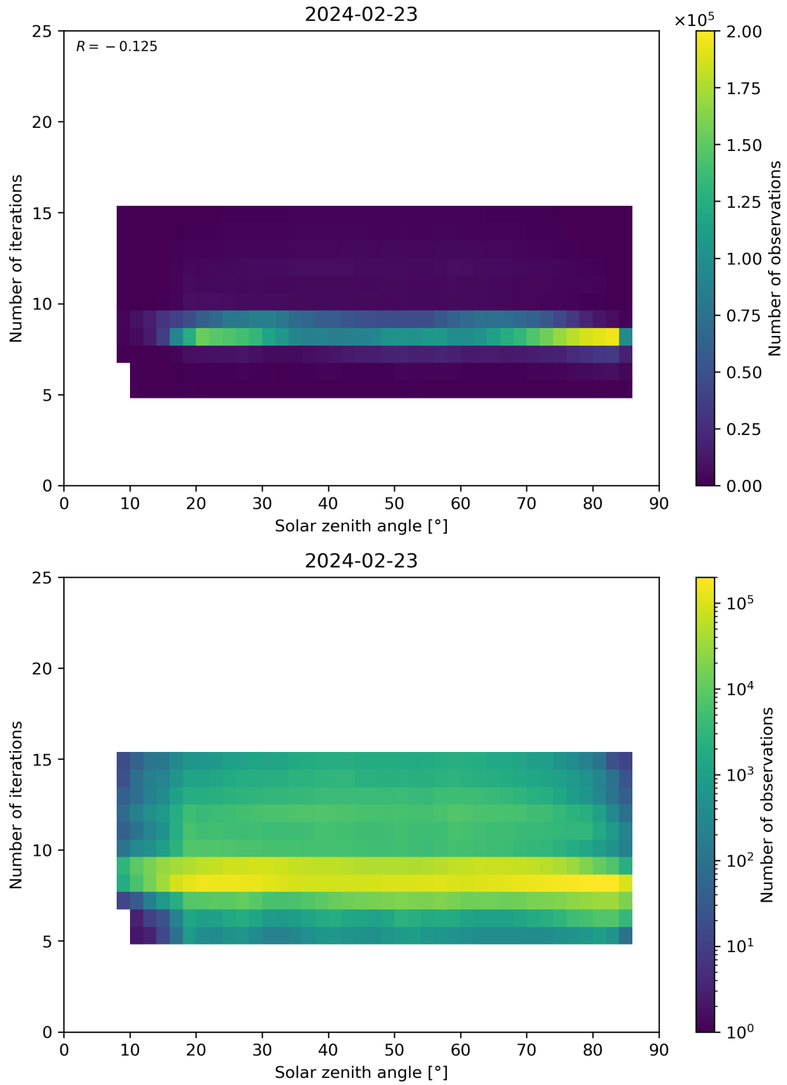
Figure 67: Scatter density plot of “Solar zenith angle” against “Number of iterations” for 2024-02-22 to 2024-02-24.
