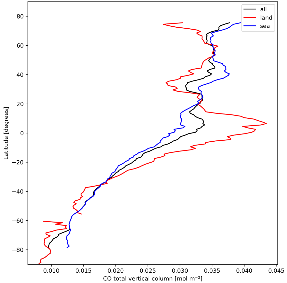
Figure 10: Zonal average of “CO total vertical column” for 2024-02-22 to 2024-02-24.
