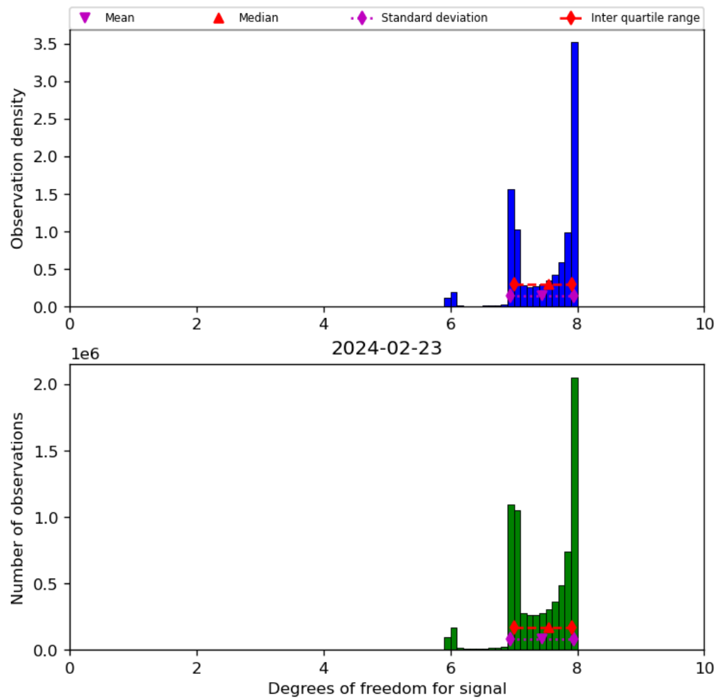
Figure 23: Histogram of “Degrees of freedom for signal” for 2024-02-22 to 2024-02-24
