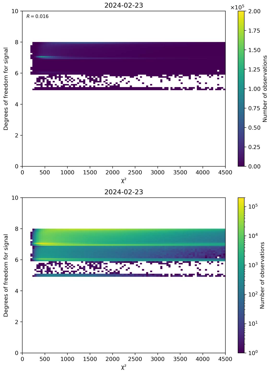
Figure 48: Scatter density plot of “ \chi^2 ” against “Degrees of freedom for signal” for 2024-02-22 to 2024-02-24.
