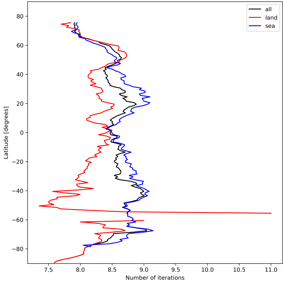
Figure 16: Zonal average of “Number of iterations” for 2024-02-22 to 2024-02-24.
