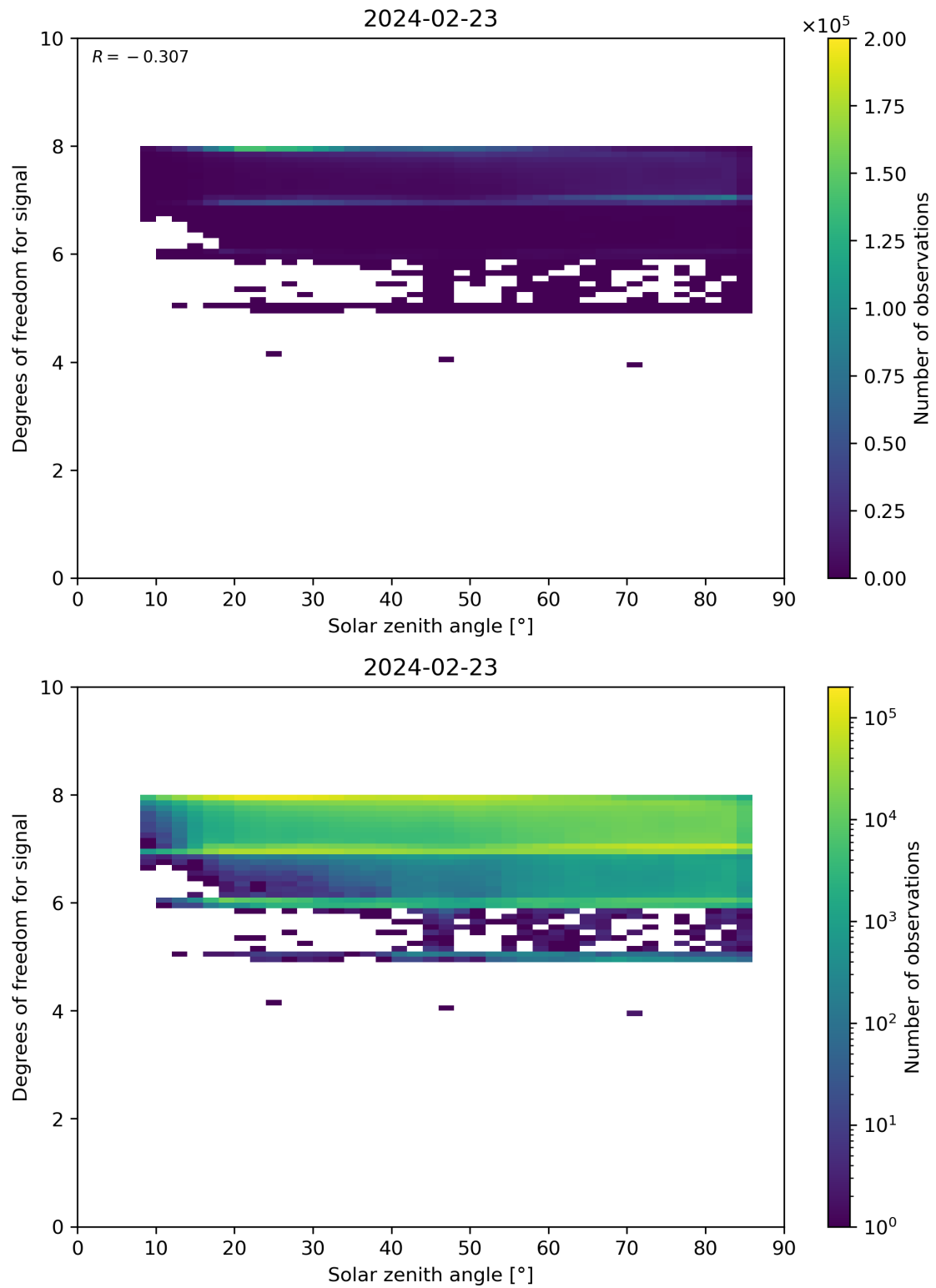
Figure 65: Scatter density plot of “Solar zenith angle” against “Degrees of freedom for signal” for 2024-02-22 to 2024-02-24.
