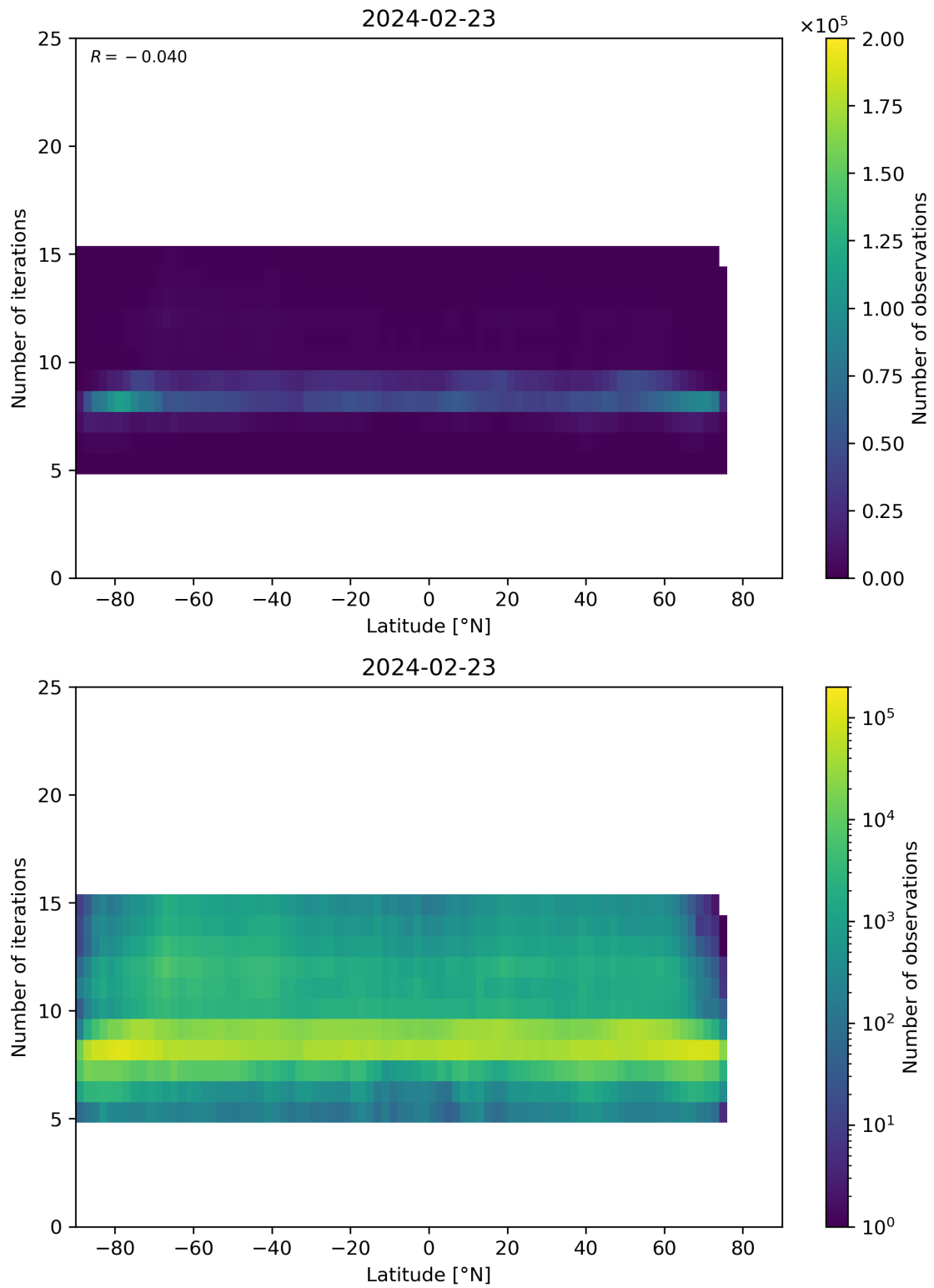
Figure 56: Scatter density plot of “Latitude” against “Number of iterations” for 2024-02-22 to 2024-02-24.
