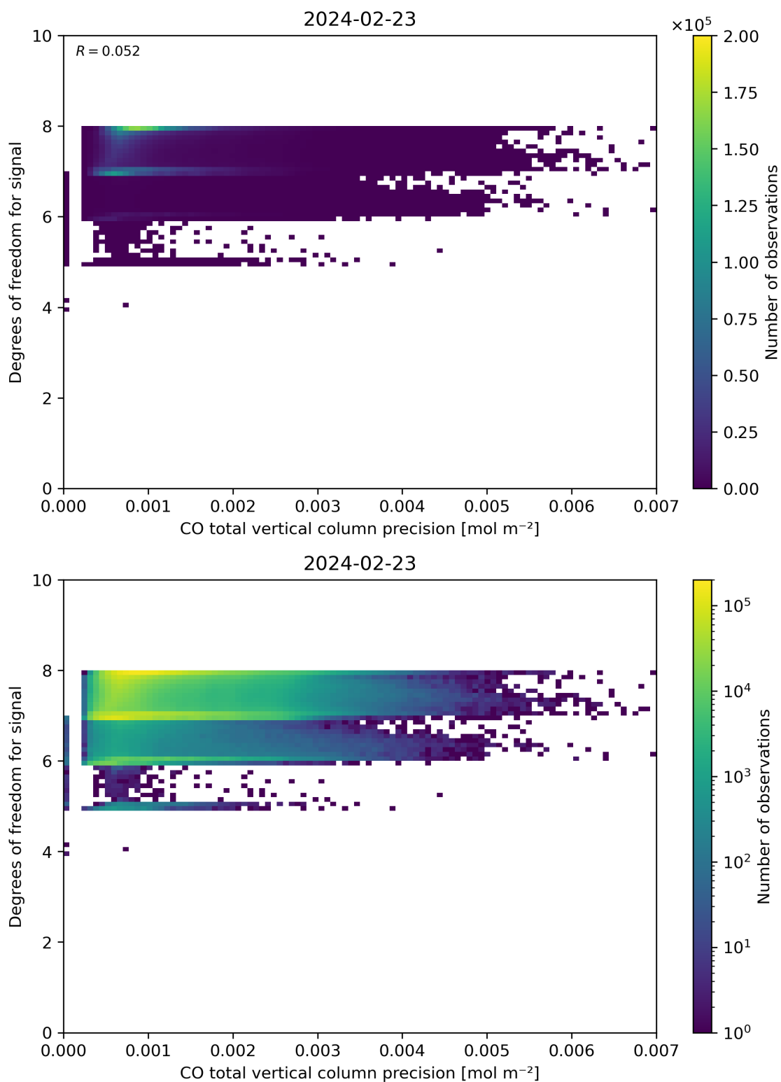
Figure 45: Scatter density plot of “CO total vertical column precision” against “Degrees of freedom for signal” for 2024-02-22 to 2024-02-24.
