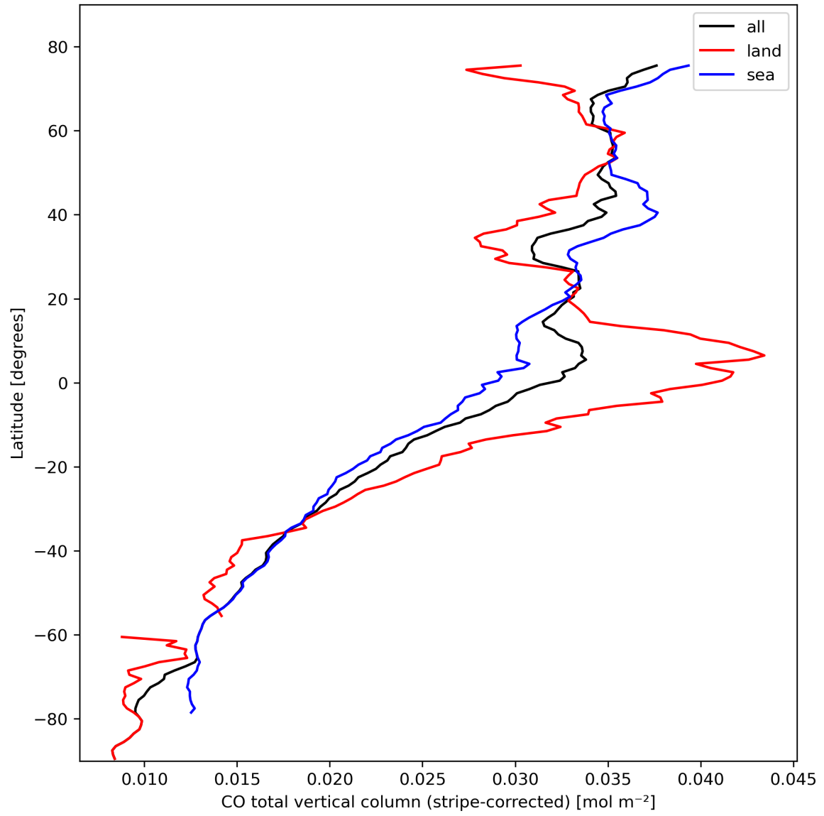
Figure 11: Zonal average of “CO total vertical column (stripe-corrected)” for 2024-02-22 to 2024-02-24.
