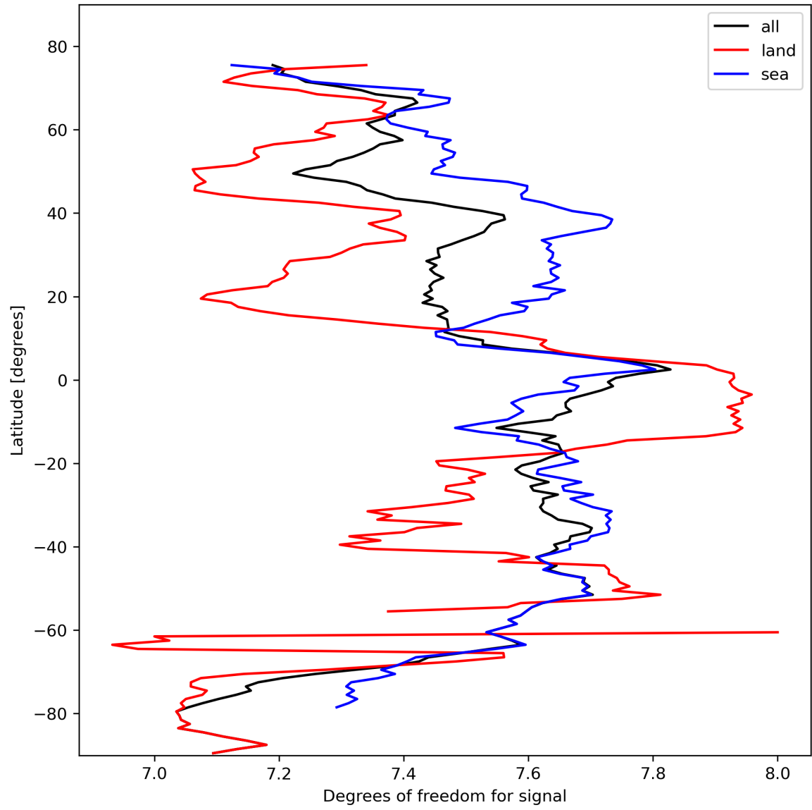
Figure 15: Zonal average of “Degrees of freedom for signal” for 2024-02-22 to 2024-02-24.
