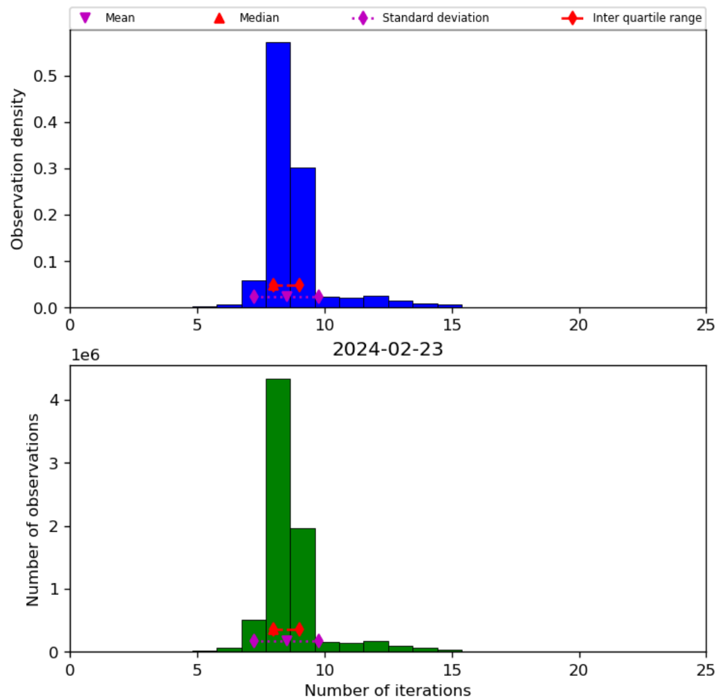
Figure 24: Histogram of “Number of iterations” for 2024-02-22 to 2024-02-24
