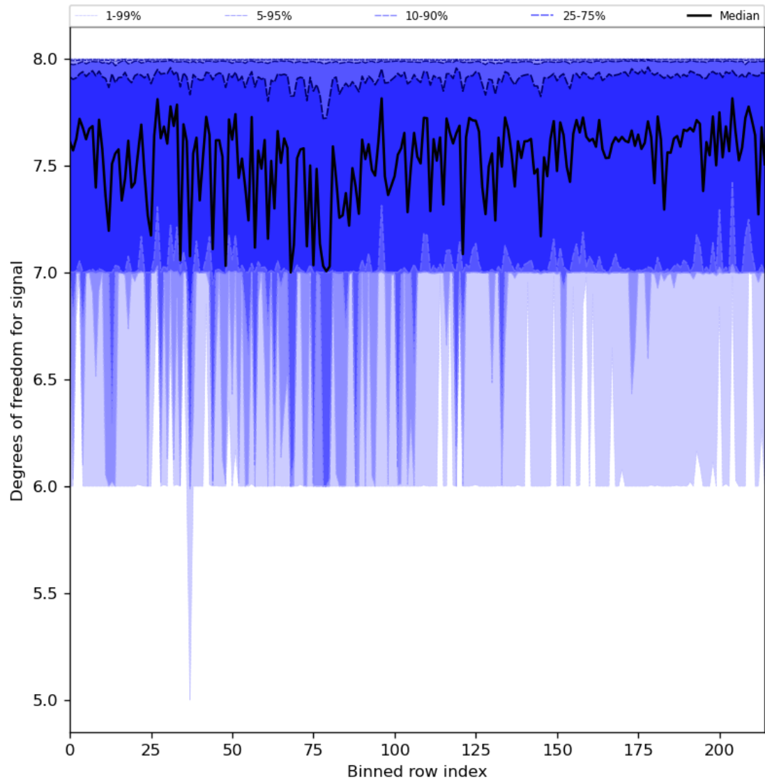
Figure 31: Along track statistics of “Degrees of freedom for signal” for 2024-02-22 to 2024-02-24
