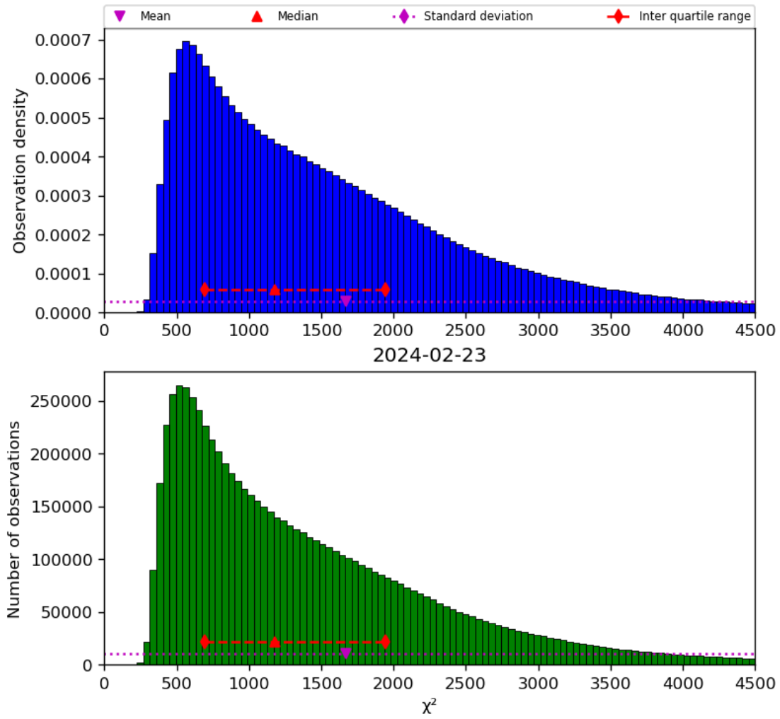
Figure 22: Histogram of “ \chi^2 ” for 2024-02-22 to 2024-02-24
