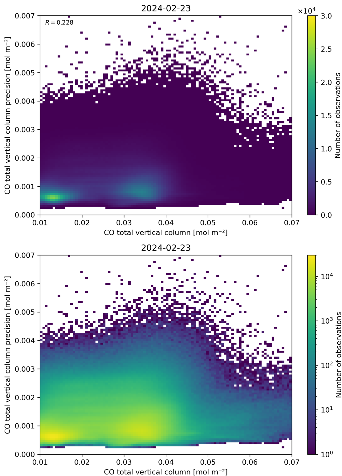
Figure 34: Scatter density plot of “CO total vertical column” against “CO total vertical column precision” for 2024-02-22 to 2024-02-24.
