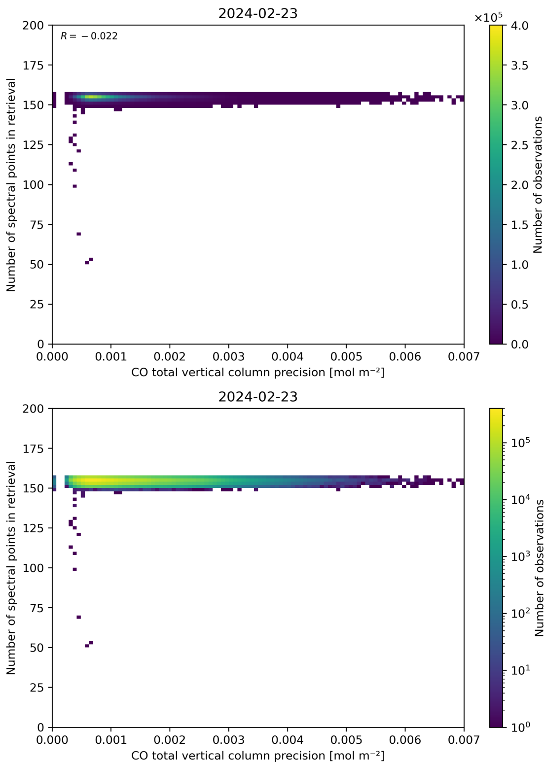
Figure 47: Scatter density plot of “CO total vertical column precision” against “Number of spectral points in retrieval” for 2024-02-22 to 2024-02-24.
