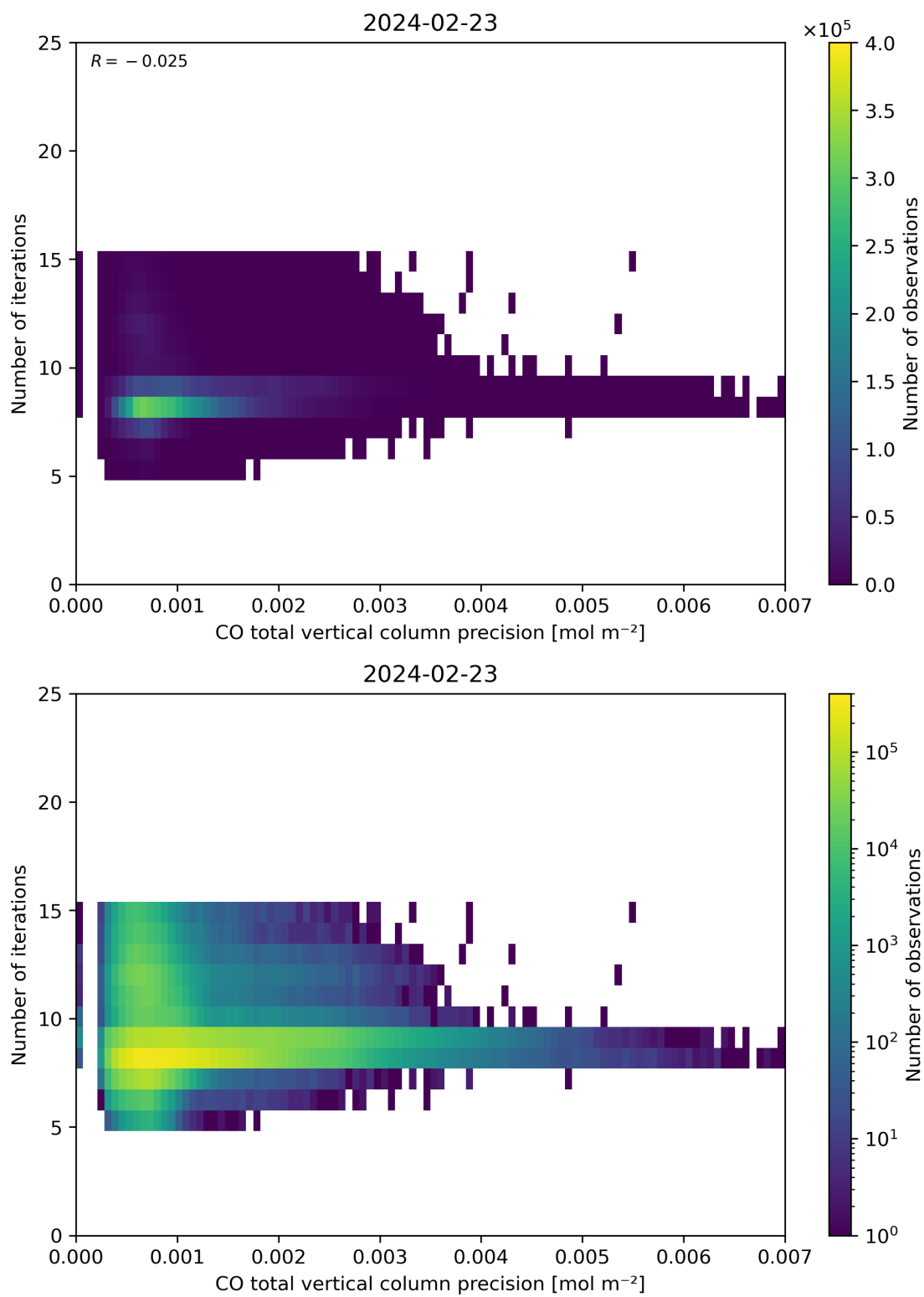
Figure 46: Scatter density plot of “CO total vertical column precision” against “Number of iterations” for 2024-02-22 to 2024-02-24.
