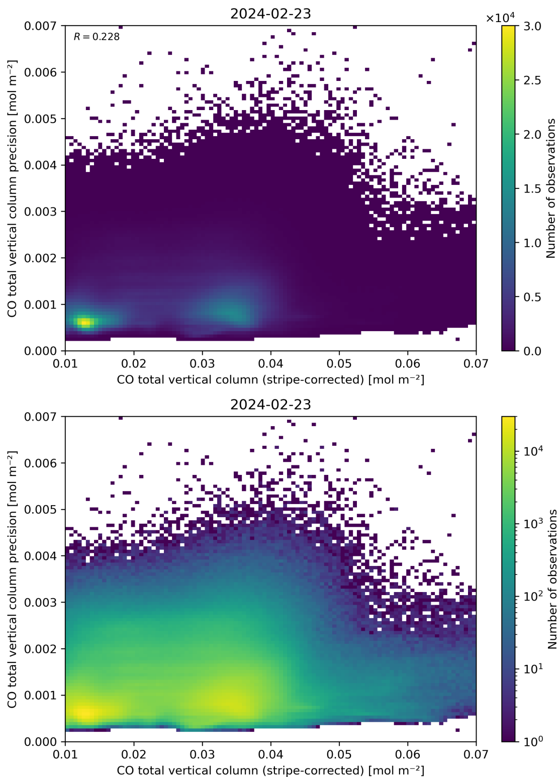
Figure 36: Scatter density plot of “CO total vertical column (stripe-corrected)” against “CO total vertical column precision” for 2024-02-22 to 2024-02-24.
