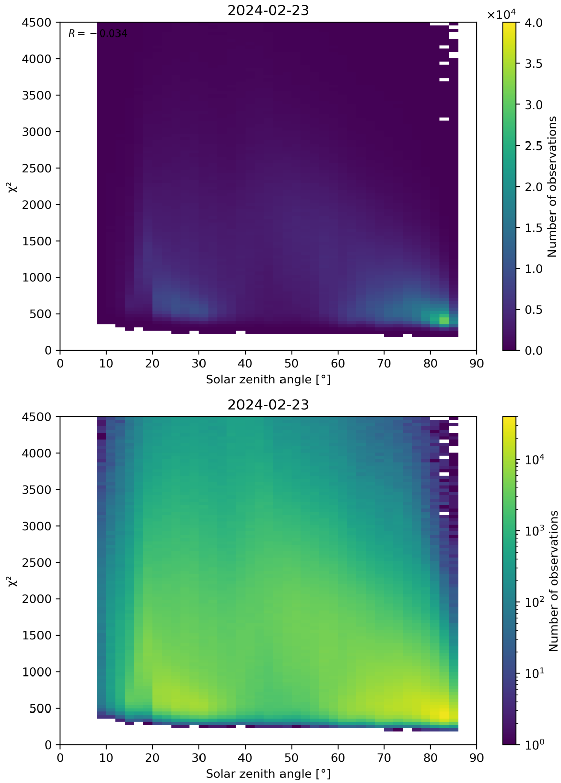
Figure 64: Scatter density plot of “Solar zenith angle” against “ \chi^2 ” for 2024-02-22 to 2024-02-24.
