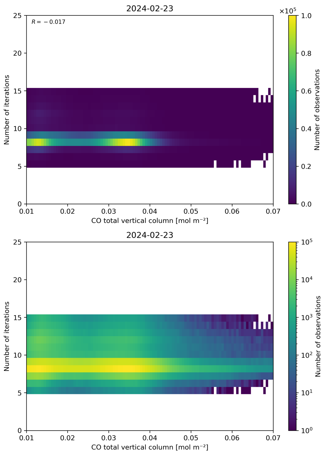
Figure 42: Scatter density plot of “CO total vertical column” against “Number of iterations” for 2024-02-22 to 2024-02-24.
