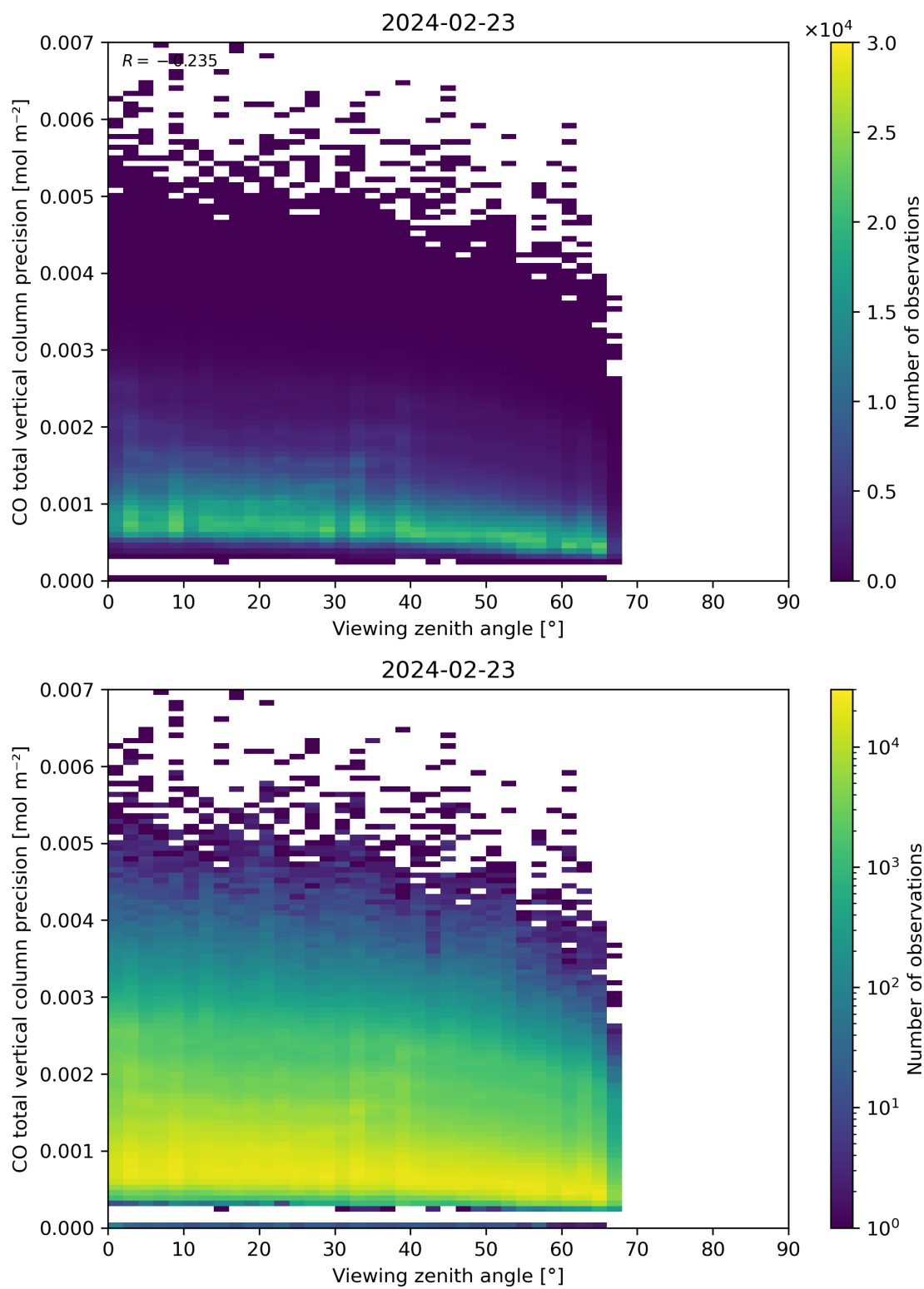
Figure 71: Scatter density plot of “Viewing zenith angle” against “CO total vertical column precision” for 2024-02-22 to 2024-02-24.
