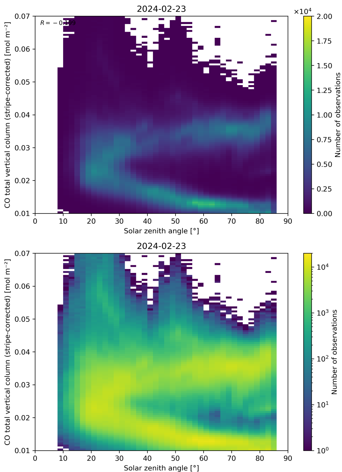
Figure 62: Scatter density plot of “Solar zenith angle” against “CO total vertical column (stripe-corrected)” for 2024-02-22 to 2024-02-24.
