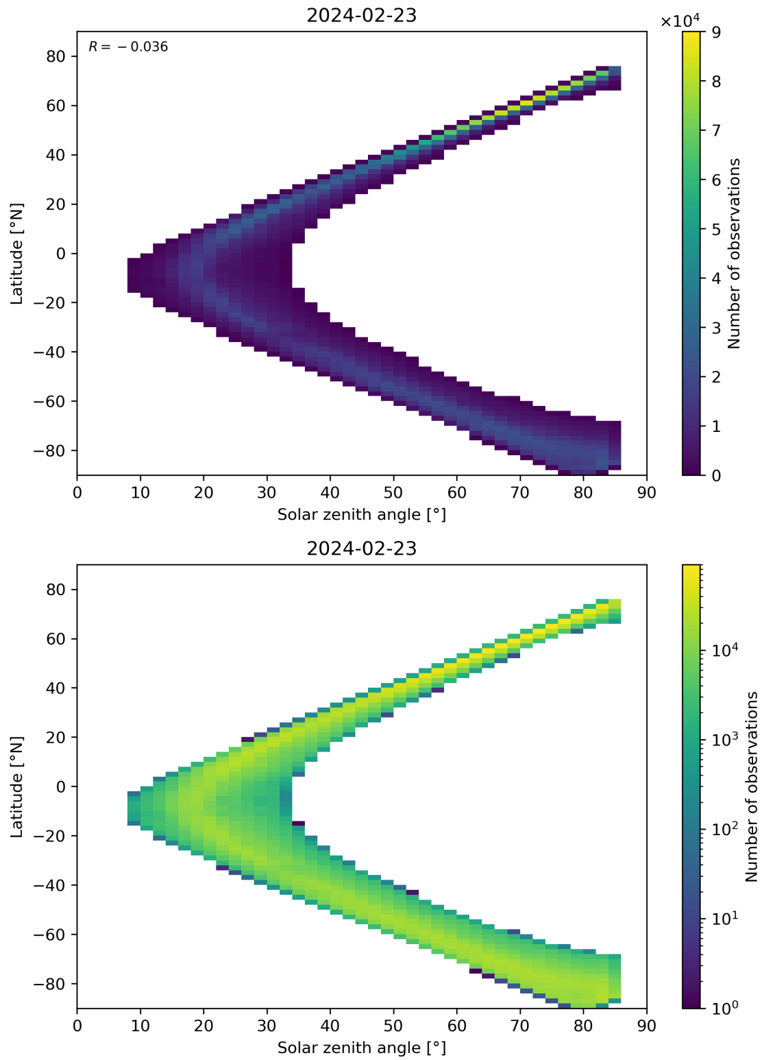
Figure 66: Scatter density plot of “Solar zenith angle” against “Latitude” for 2024-02-22 to 2024-02-24.
