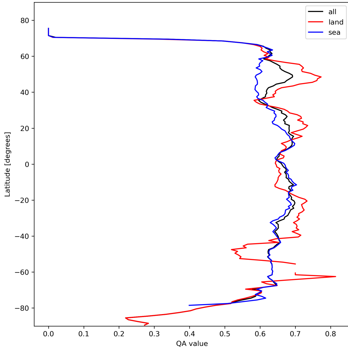
Figure 9: Zonal average of “QA value” for 2024-02-22 to 2024-02-24.
