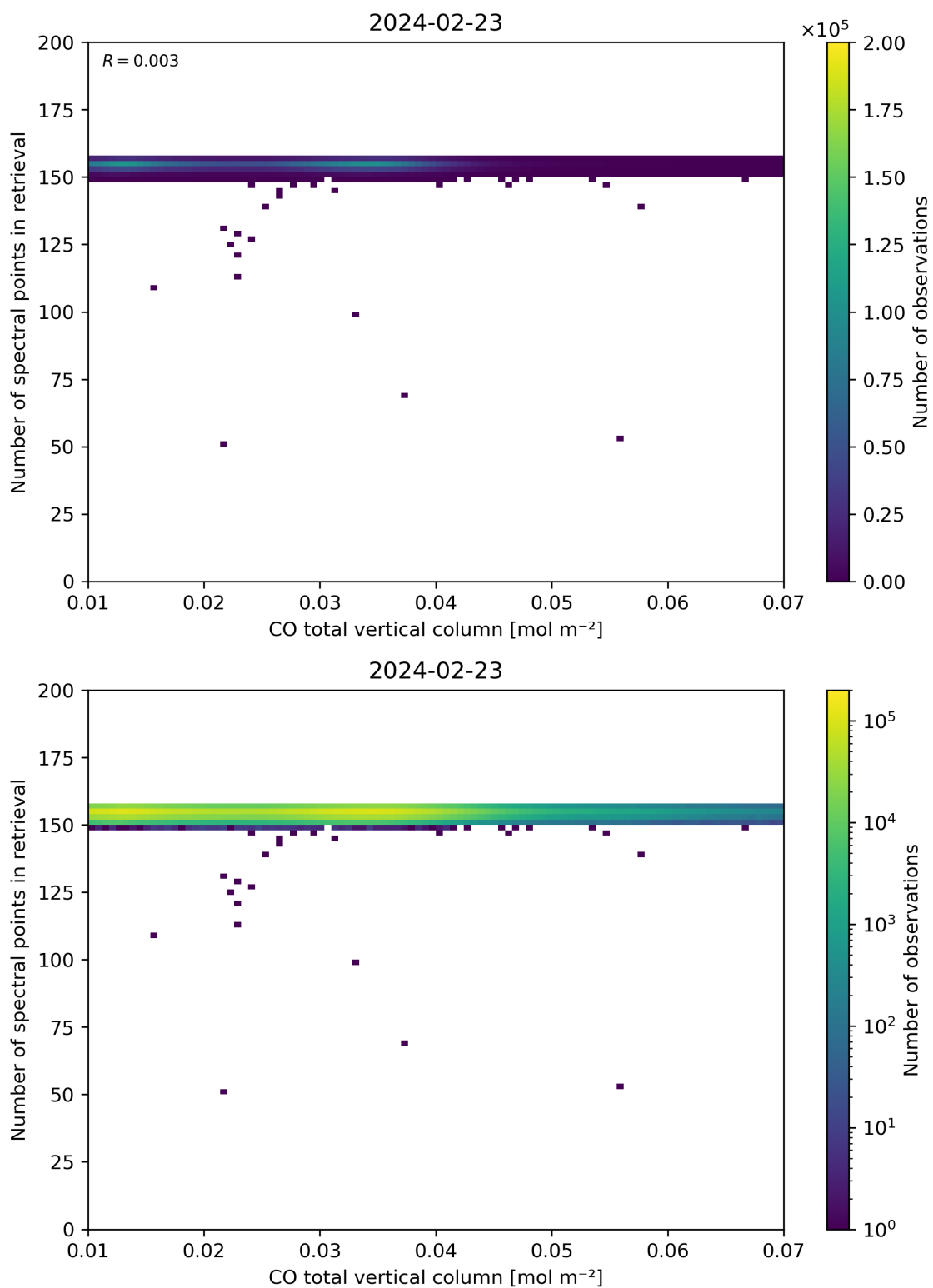
Figure 43: Scatter density plot of “CO total vertical column” against “Number of spectral points in retrieval” for 2024-02-22 to 2024-02-24.
