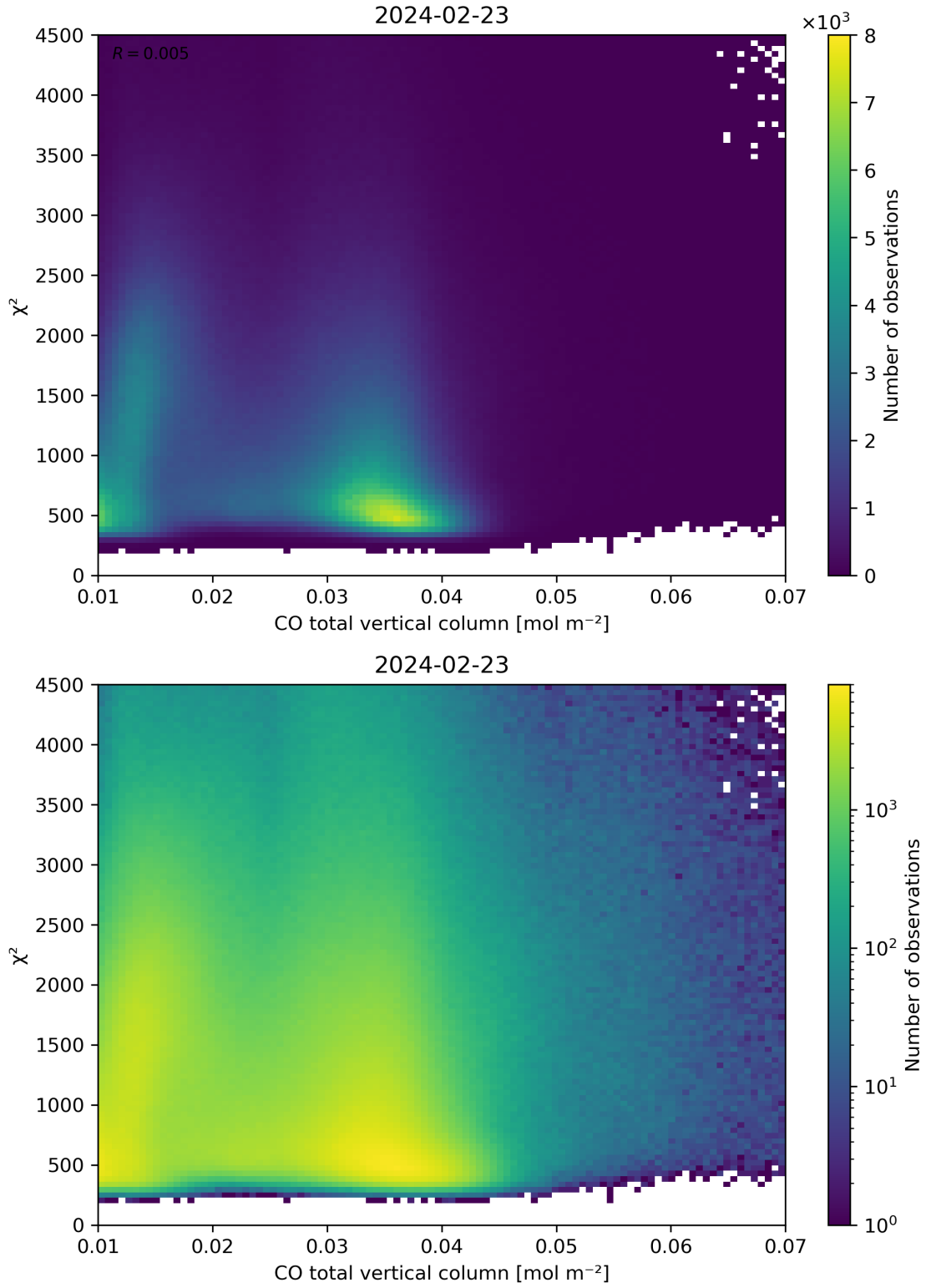
Figure 35: Scatter density plot of “CO total vertical column” against “ \chi^2 ” for 2024-02-22 to 2024-02-24.
