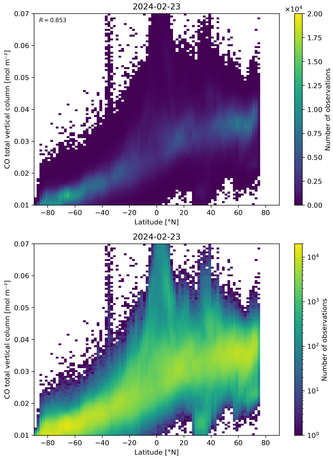
Figure 51: Scatter density plot of “Latitude” against “CO total vertical column” for 2024-02-22 to 2024-02-24.
