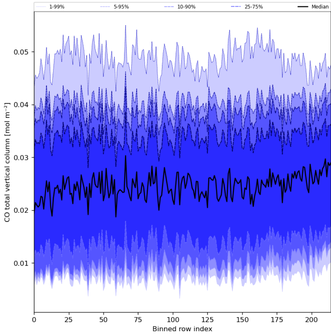
Figure 26: Along track statistics of “CO total vertical column” for 2024-02-22 to 2024-02-24
