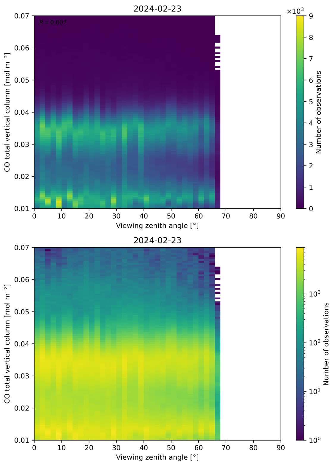
Figure 69: Scatter density plot of “Viewing zenith angle” against “CO total vertical column” for 2024-02-22 to 2024-02-24.
