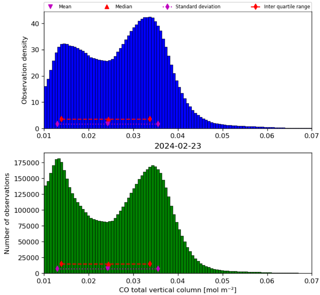
Figure 18: Histogram of “CO total vertical column” for 2024-02-22 to 2024-02-24
