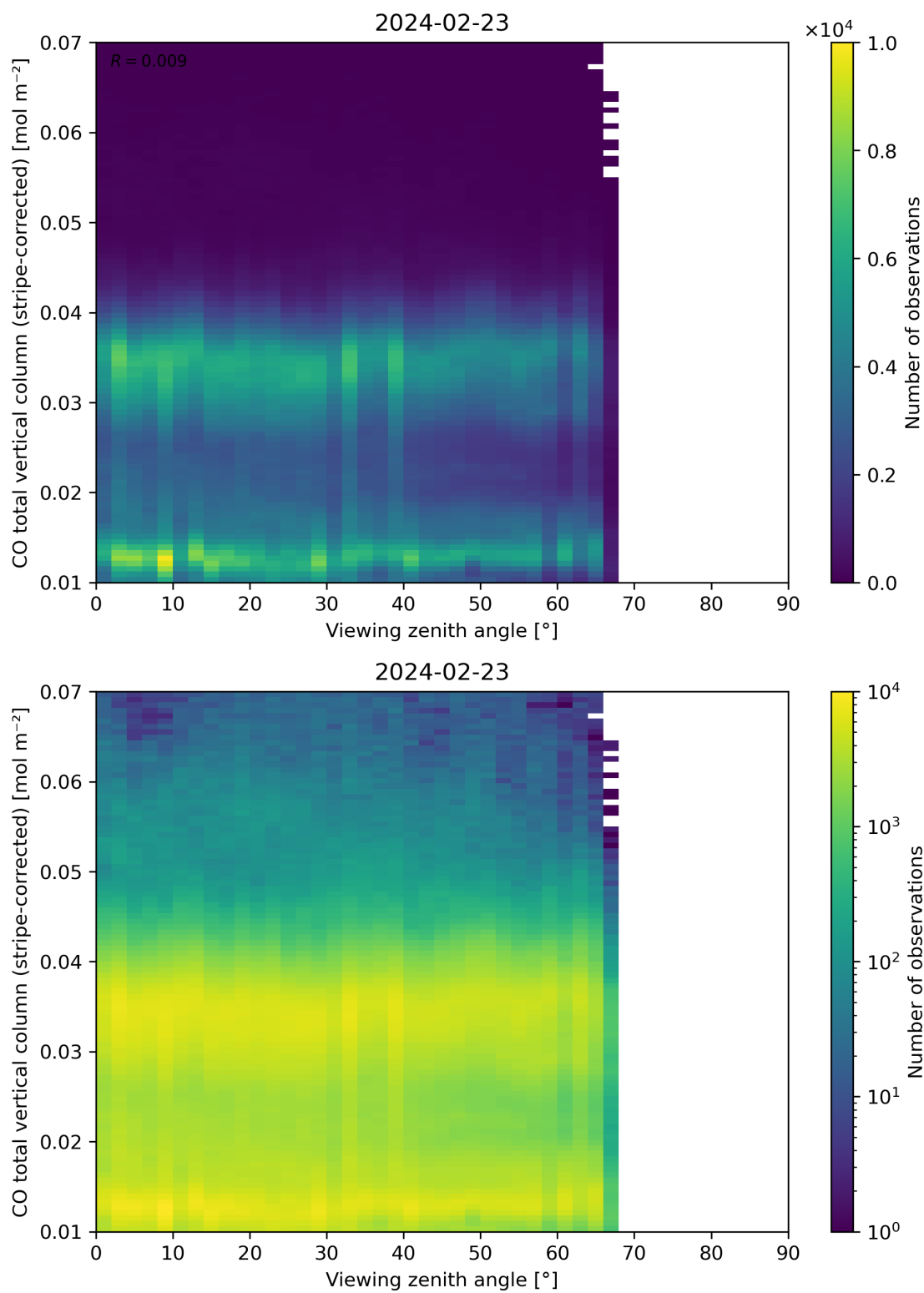
Figure 70: Scatter density plot of “Viewing zenith angle” against “CO total vertical column (stripe-corrected)” for 2024-02-22 to 2024-02-24.
