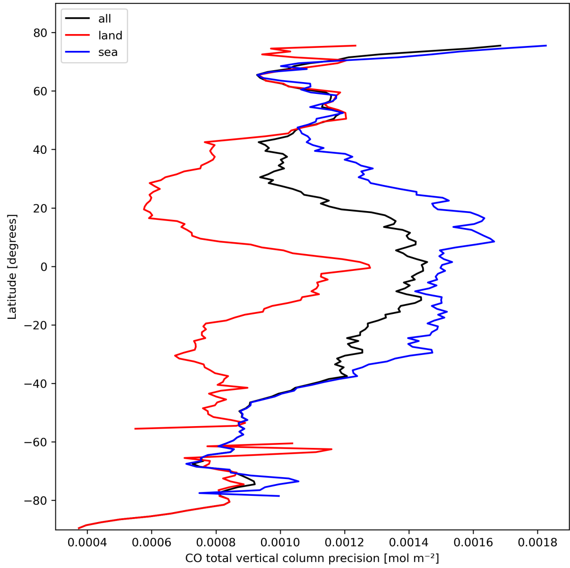
Figure 12: Zonal average of “CO total vertical column precision” for 2024-02-22 to 2024-02-24.
