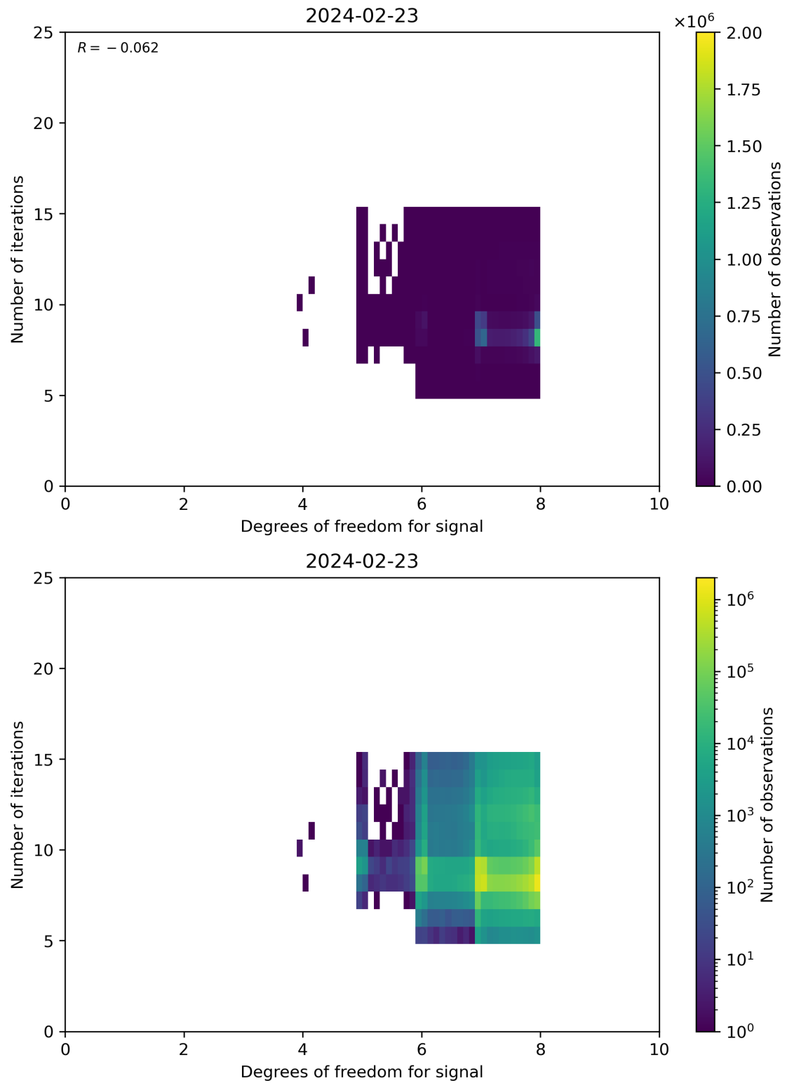
Figure 50: Scatter density plot of “Degrees of freedom for signal” against “Number of iterations” for 2024-02-22 to 2024-02-24.
