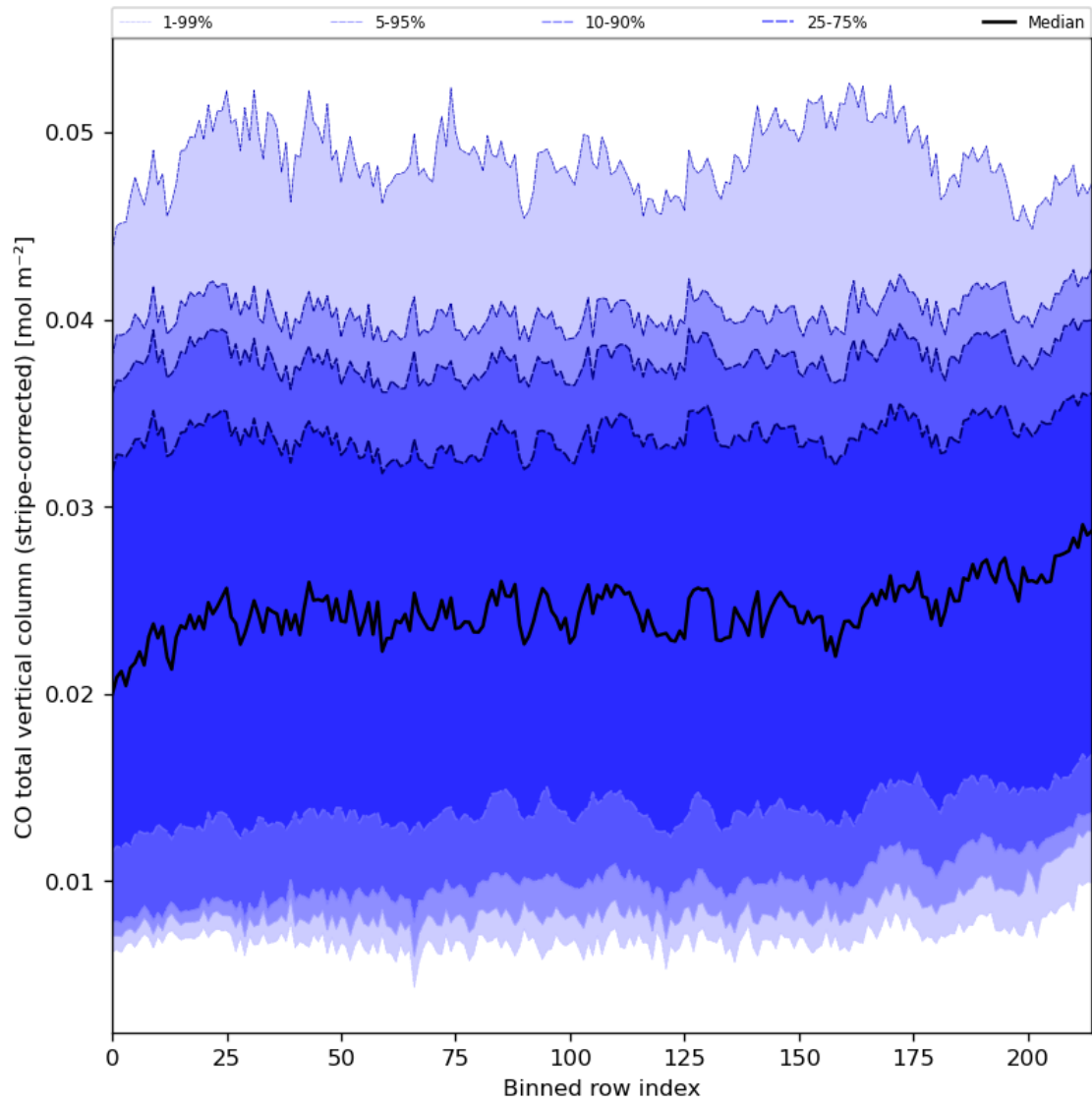
Figure 27: Along track statistics of “CO total vertical column (stripe-corrected)” for 2024-02-22 to 2024-02-24
