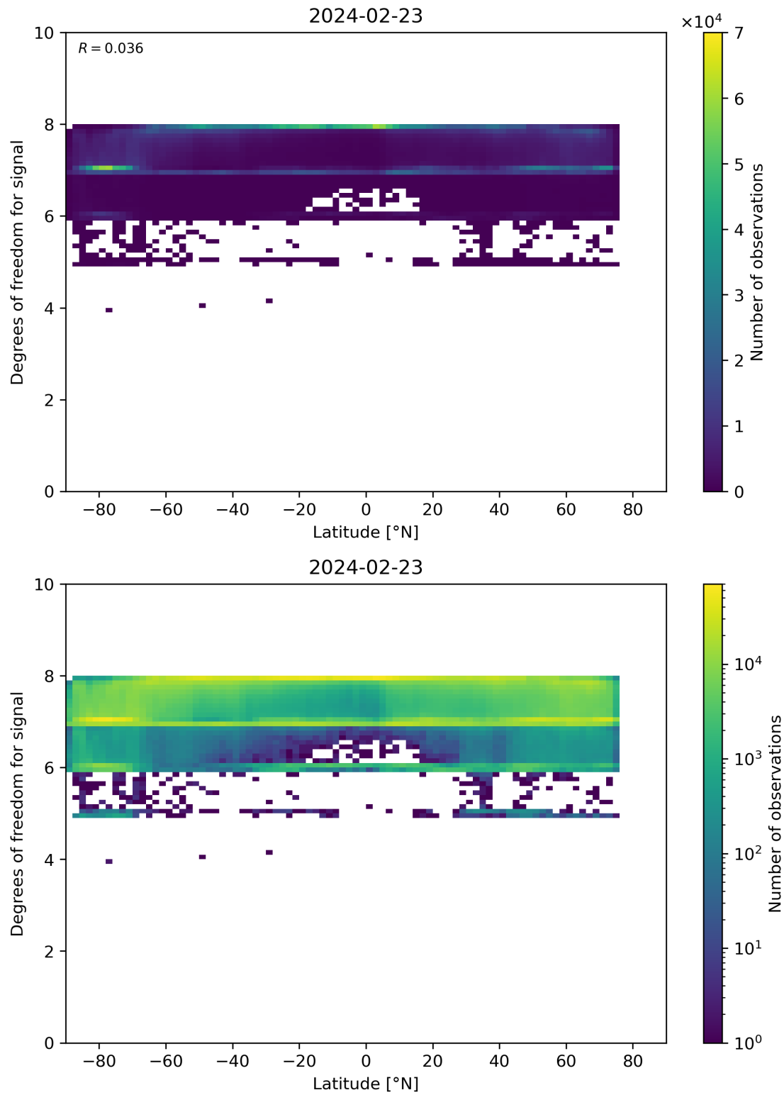
Figure 55: Scatter density plot of “Latitude” against “Degrees of freedom for signal” for 2024-02-22 to 2024-02-24.
