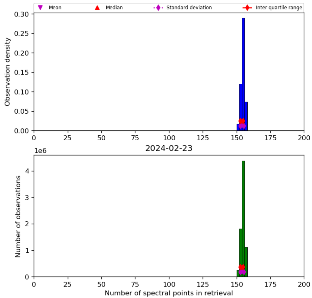
Figure 21: Histogram of “Number of spectral points in retrieval” for 2024-02-22 to 2024-02-24
