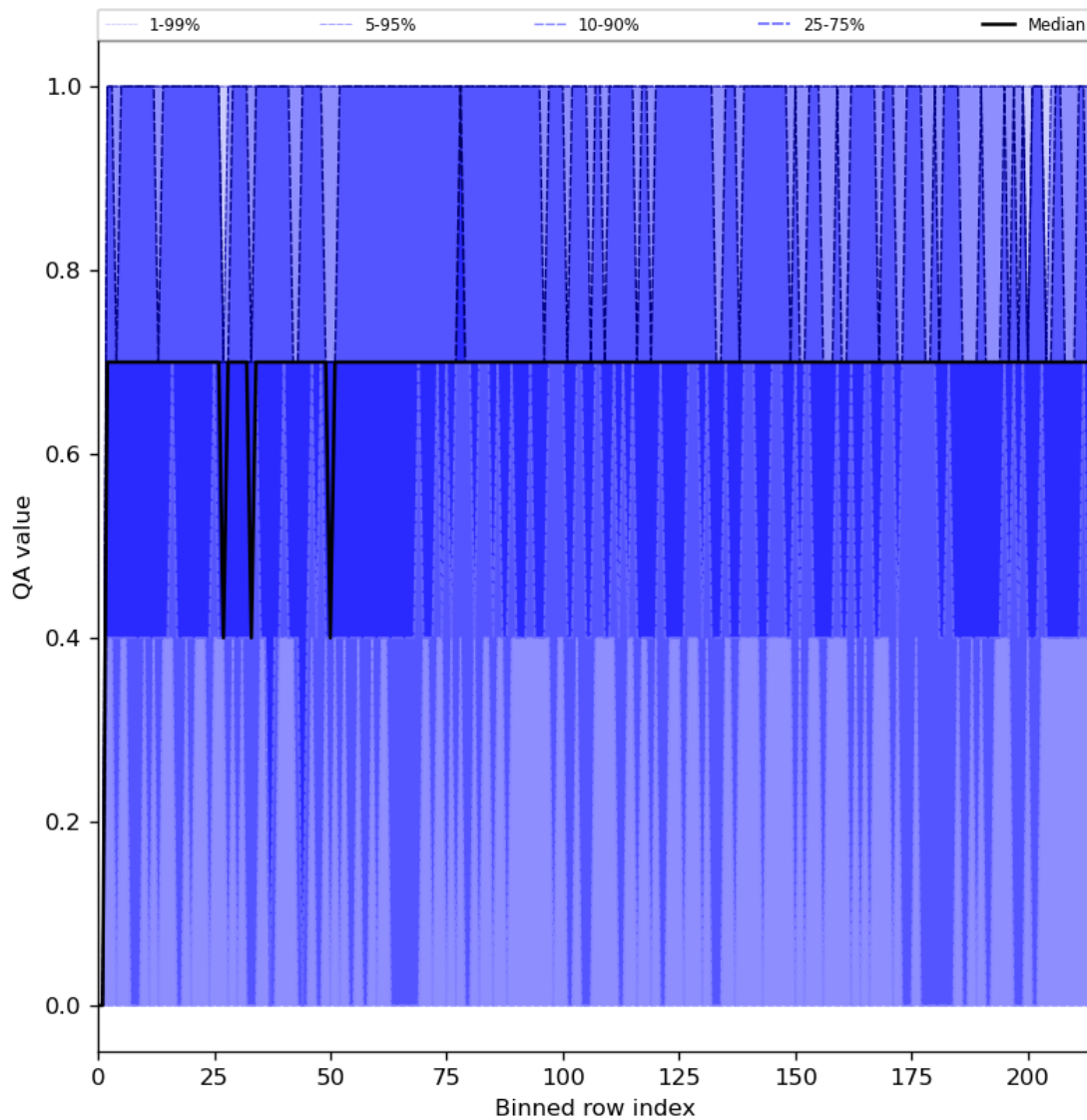
Figure 25: Along track statistics of “QA value” for 2024-02-22 to 2024-02-24
