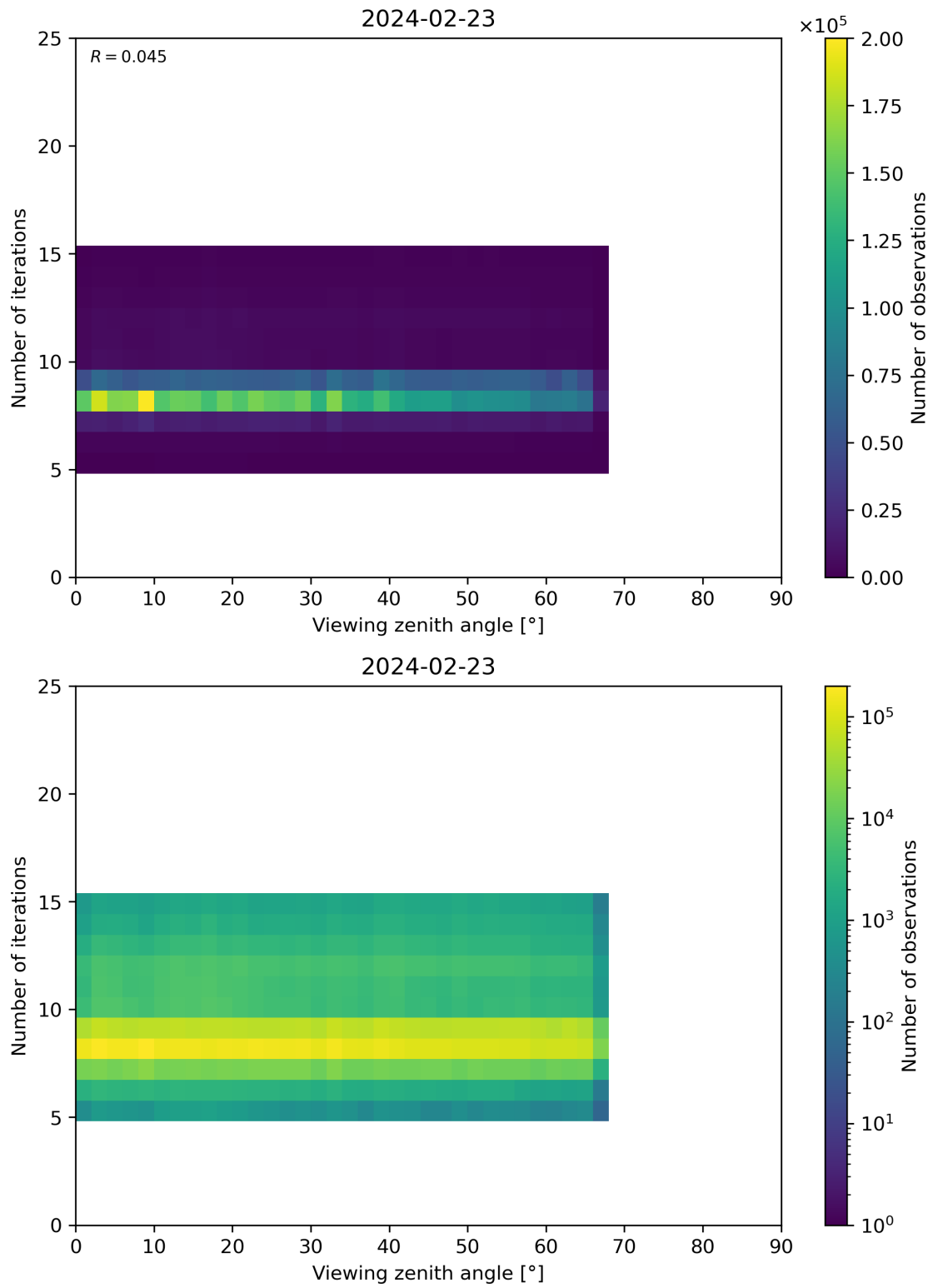
Figure 75: Scatter density plot of “Viewing zenith angle” against “Number of iterations” for 2024-02-22 to 2024-02-24.
