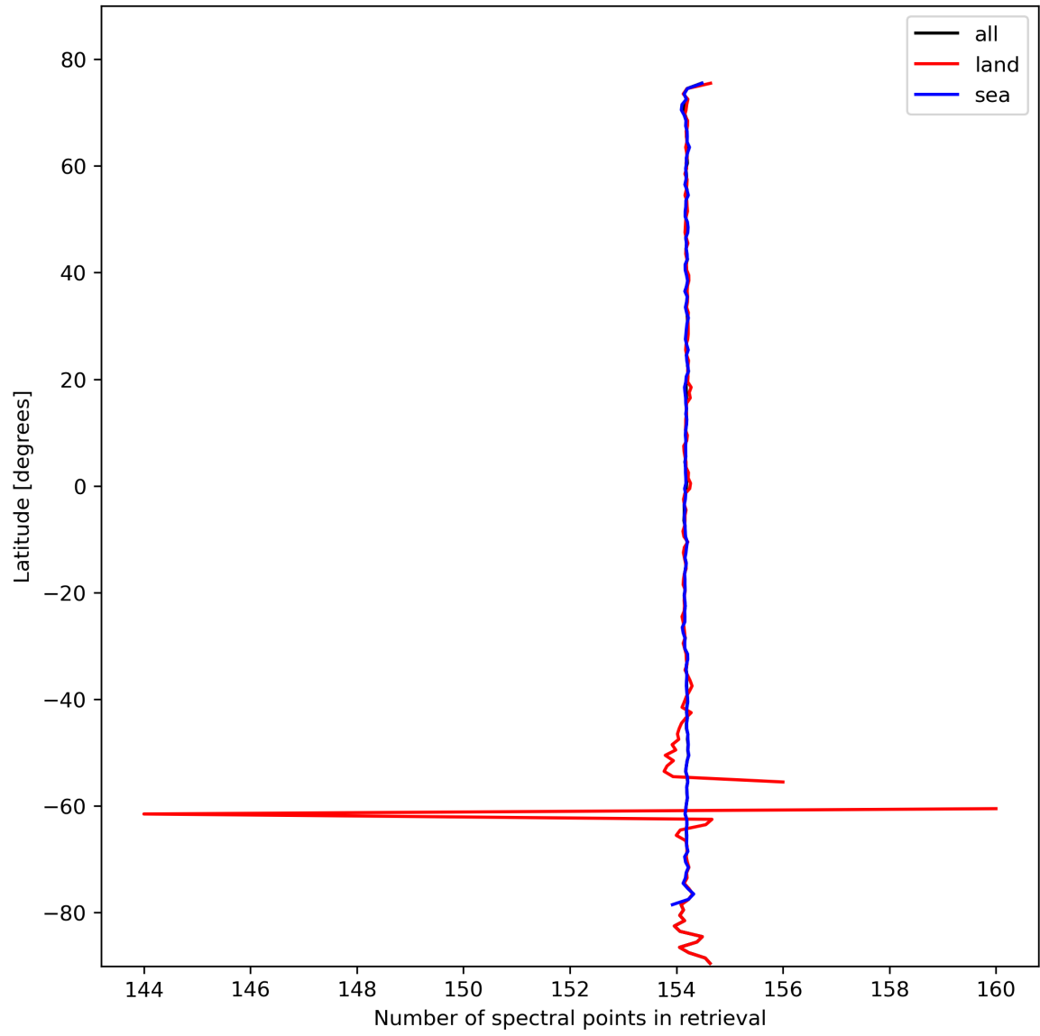
Figure 13: Zonal average of “Number of spectral points in retrieval” for 2024-02-22 to 2024-02-24.
