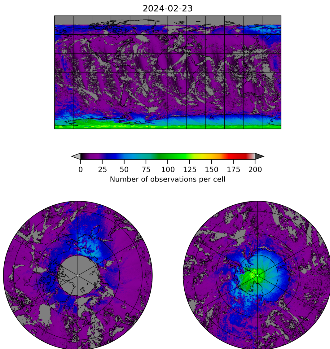
Figure 8: Map of the number of observations for 2024-02-22 to 2024-02-24
