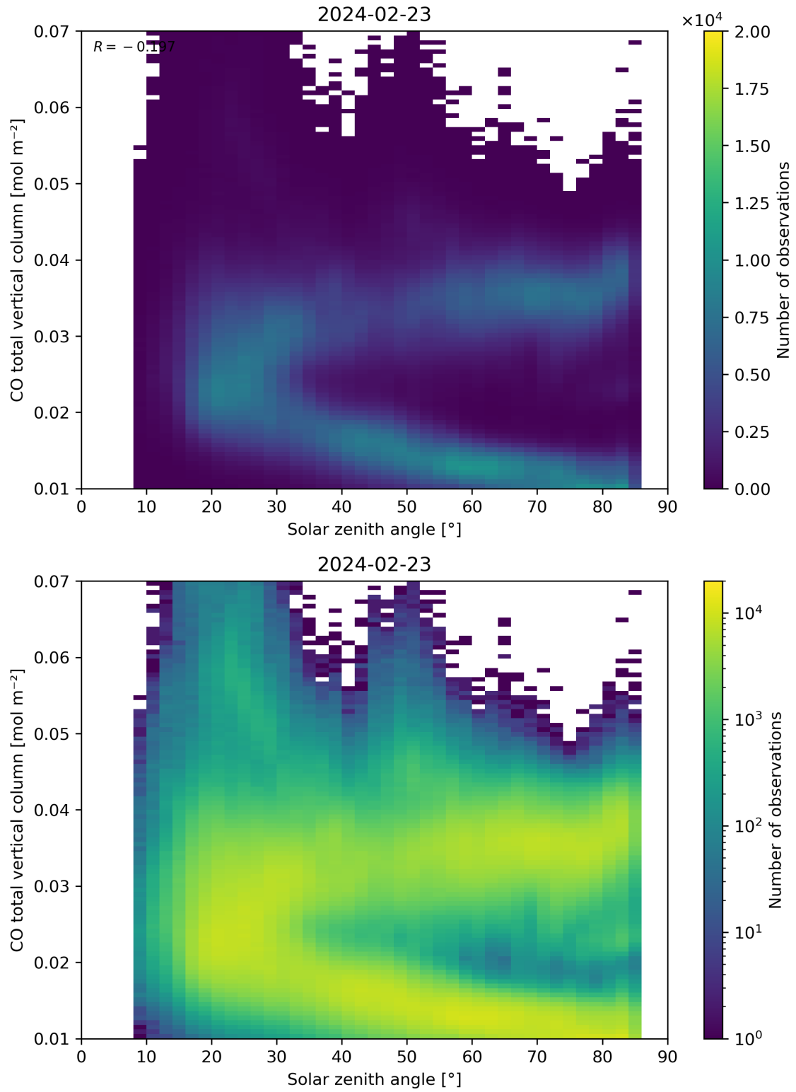
Figure 61: Scatter density plot of “Solar zenith angle” against “CO total vertical column” for 2024-02-22 to 2024-02-24.
