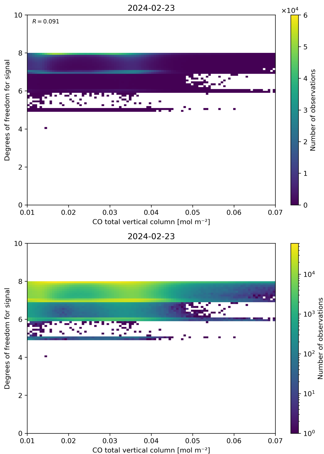
Figure 41: Scatter density plot of “CO total vertical column” against “Degrees of freedom for signal” for 2024-02-22 to 2024-02-24.
