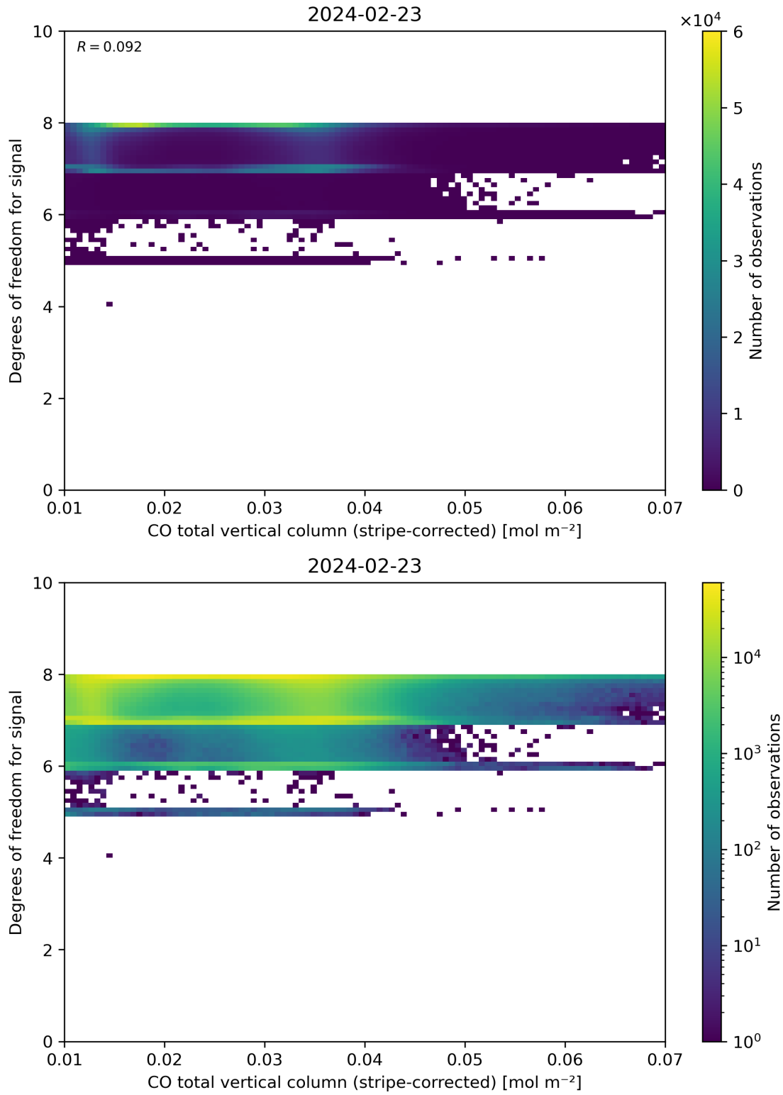
Figure 38: Scatter density plot of “CO total vertical column (stripe-corrected)” against “Degrees of freedom for signal” for 2024-02-22 to 2024-02-24.
