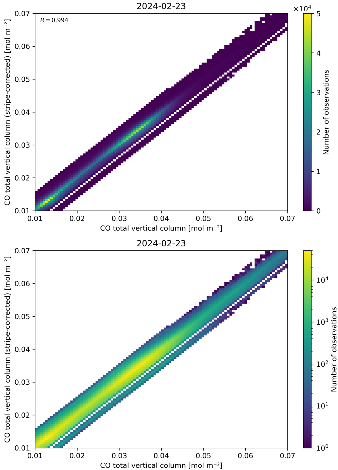
Figure 33: Scatter density plot of “CO total vertical column” against “CO total vertical column (stripe-corrected)” for 2024-02-22 to 2024-02-24.
