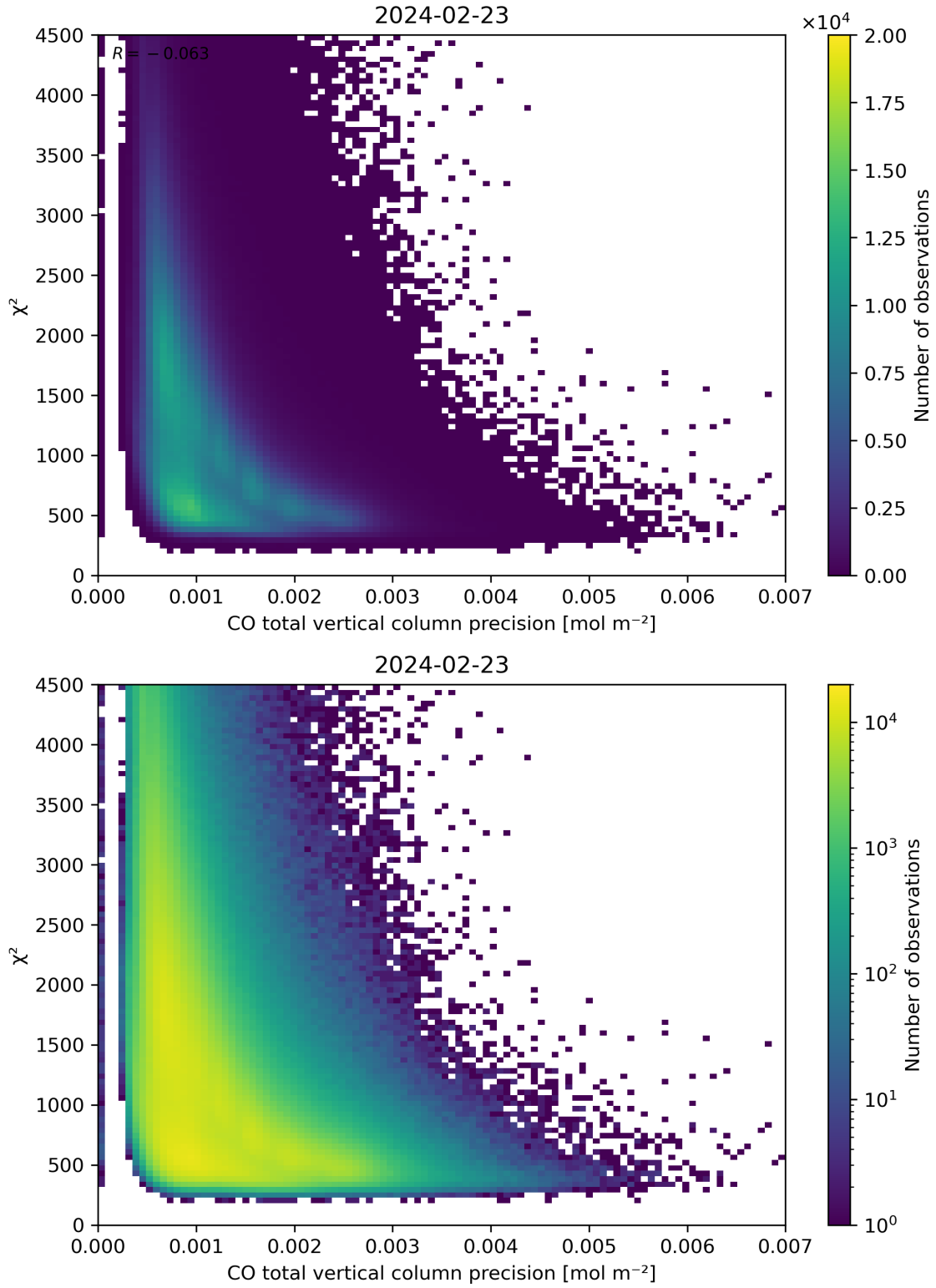
Figure 44: Scatter density plot of “CO total vertical column precision” against “ \chi^2 ” for 2024-02-22 to 2024-02-24.
