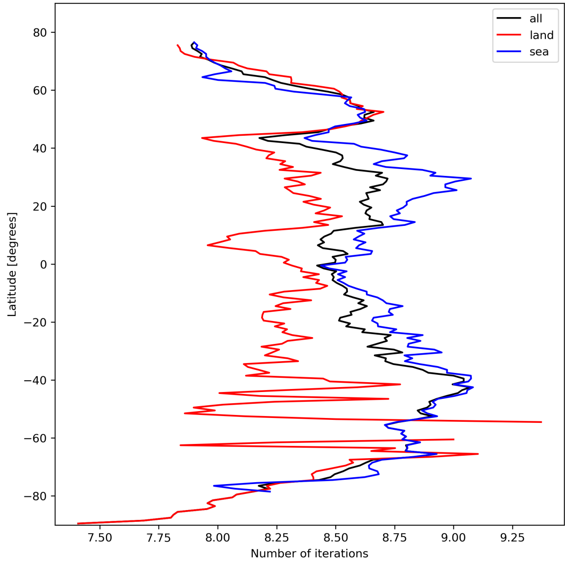
Figure 16: Zonal average of “Number of iterations” for 2024-02-24 to 2024-02-26.
