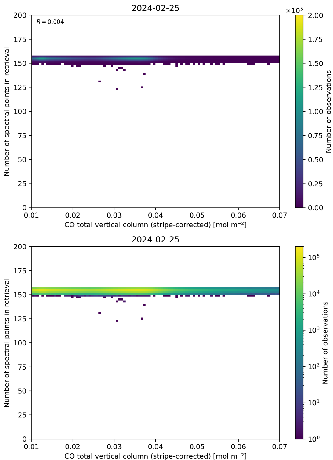
Figure 40: Scatter density plot of “CO total vertical column (stripe-corrected)” against “Number of spectral points in retrieval” for 2024-02-24 to 2024-02-26.
