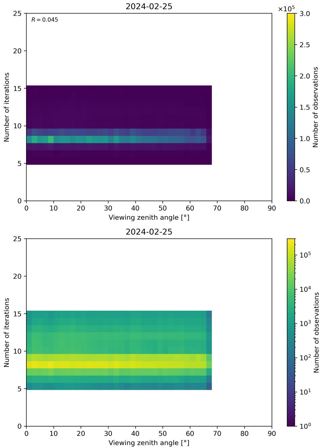
Figure 75: Scatter density plot of “Viewing zenith angle” against “Number of iterations” for 2024-02-24 to 2024-02-26.
