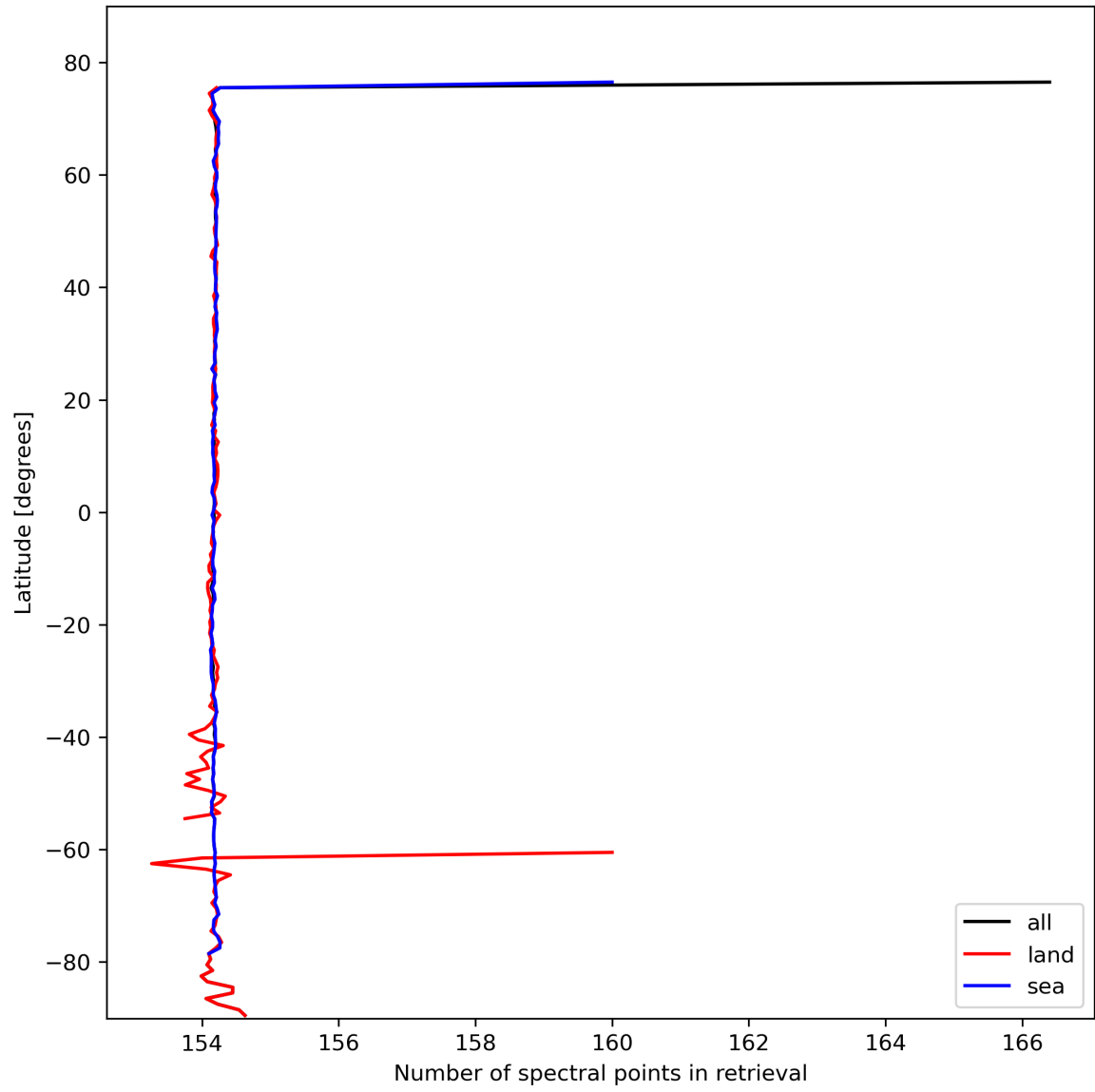
Figure 13: Zonal average of “Number of spectral points in retrieval” for 2024-02-24 to 2024-02-26.
