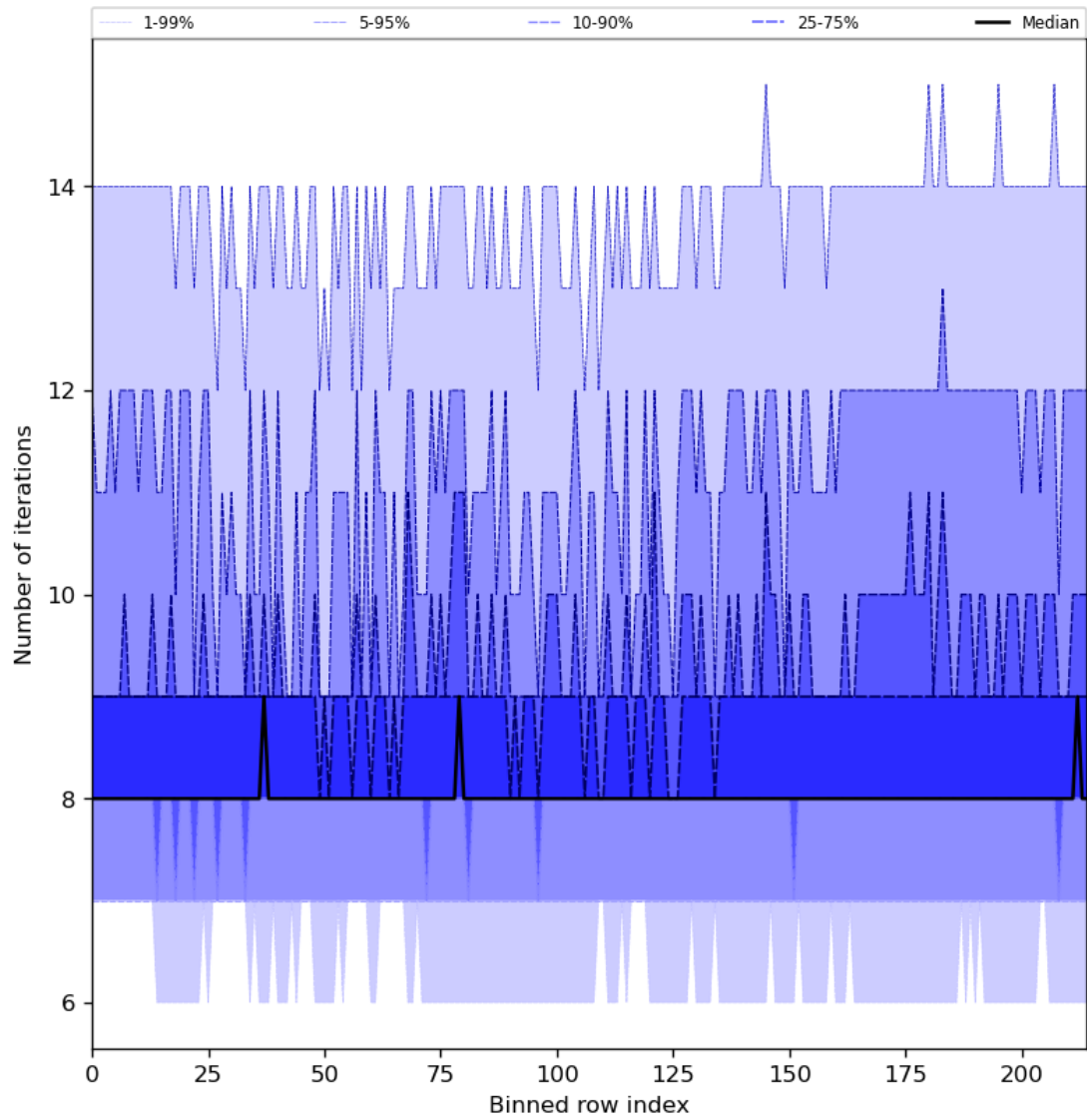
Figure 32: Along track statistics of “Number of iterations” for 2024-02-24 to 2024-02-26
