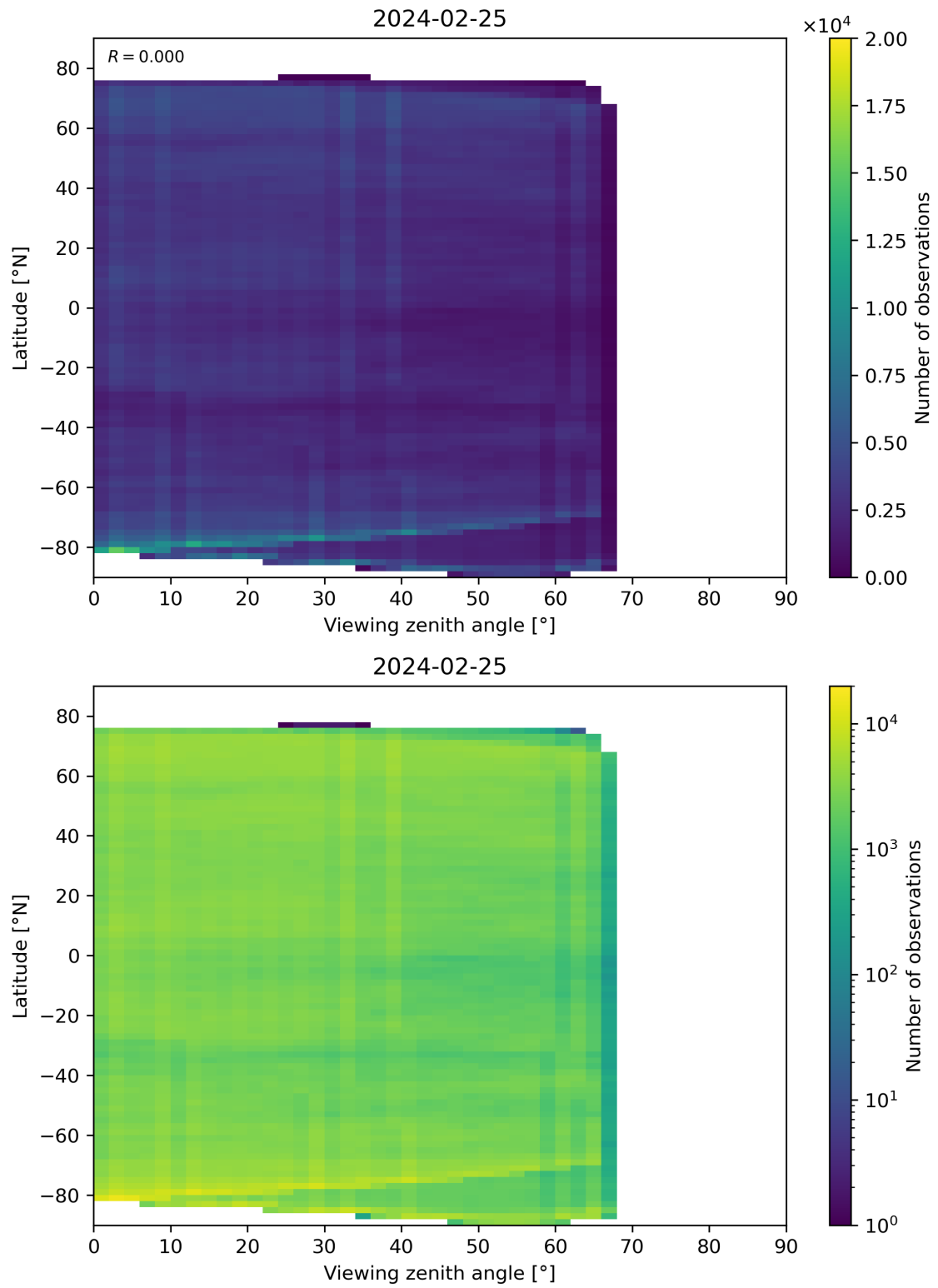
Figure 74: Scatter density plot of “Viewing zenith angle” against “Latitude” for 2024-02-24 to 2024-02-26.
