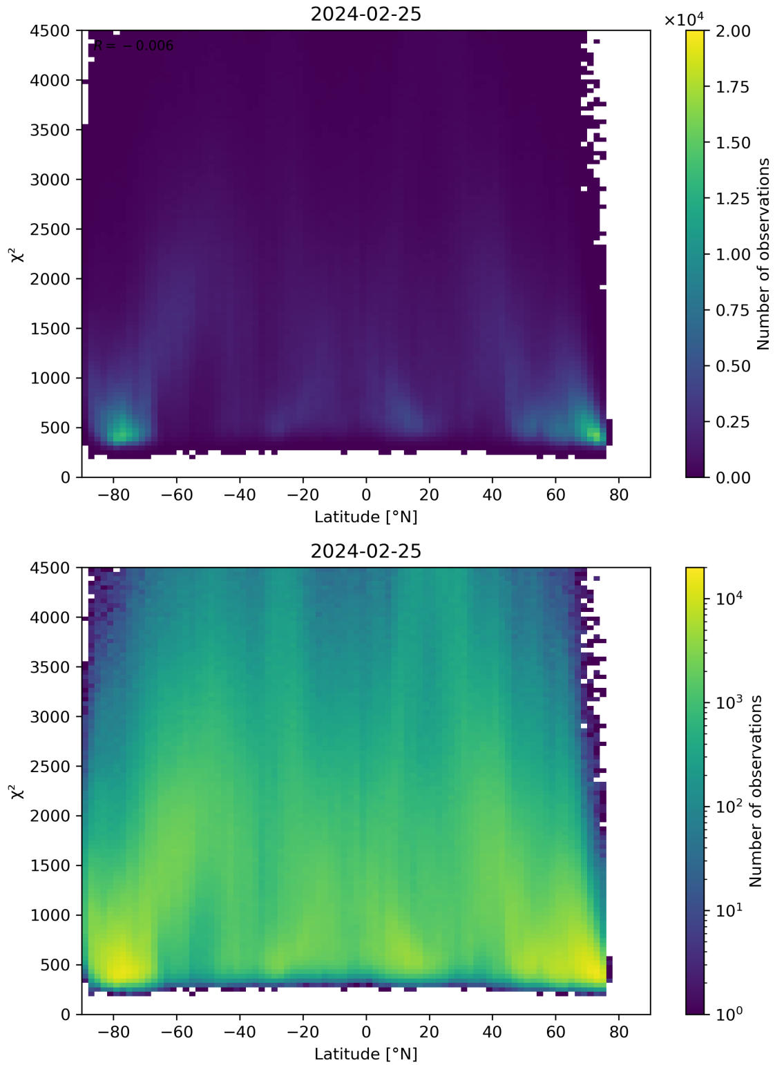
Figure 54: Scatter density plot of “Latitude” against “ \chi^2 ” for 2024-02-24 to 2024-02-26.
