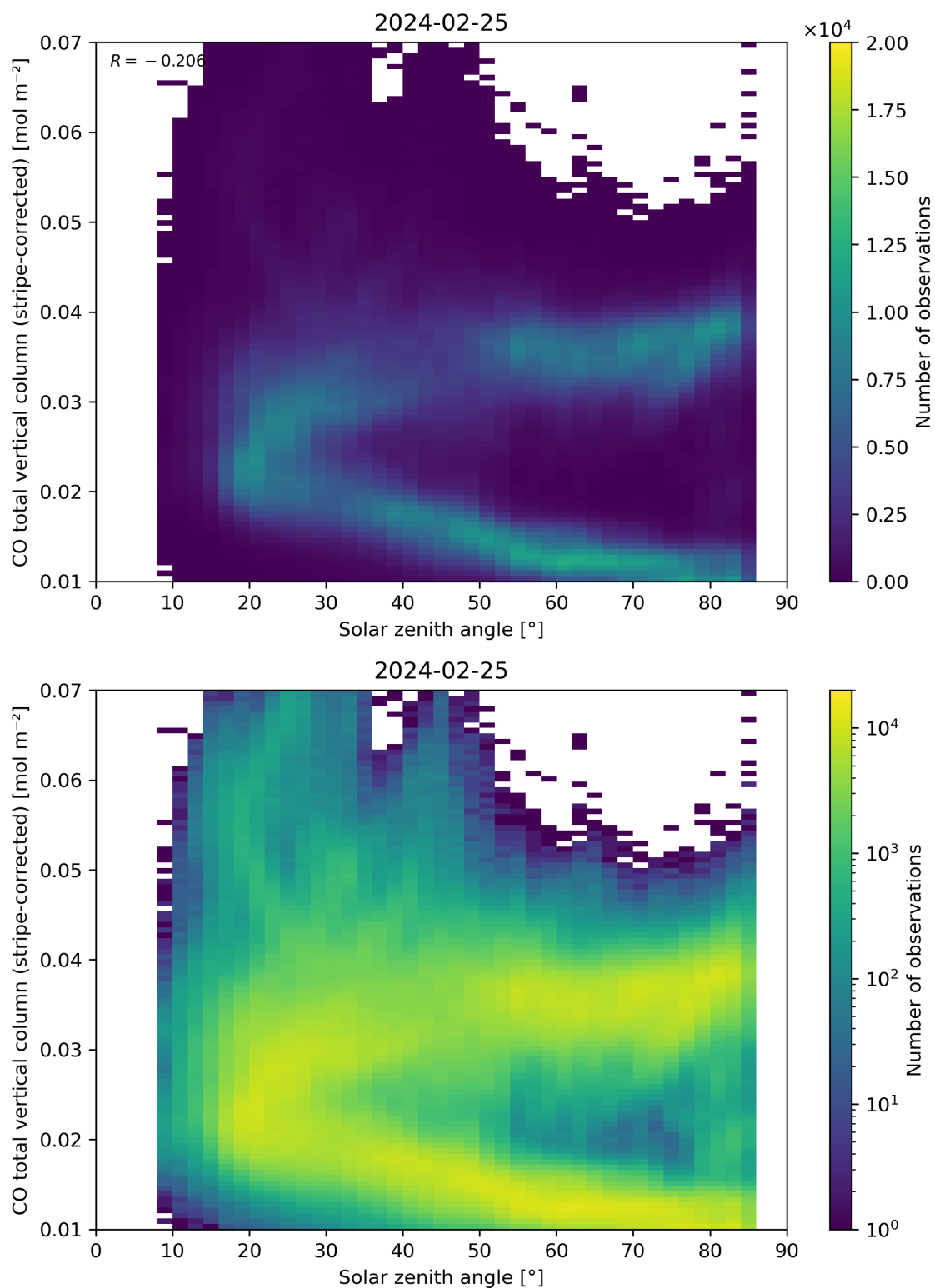
Figure 62: Scatter density plot of “Solar zenith angle” against “CO total vertical column (stripe-corrected)” for 2024-02-24 to 2024-02-26.
