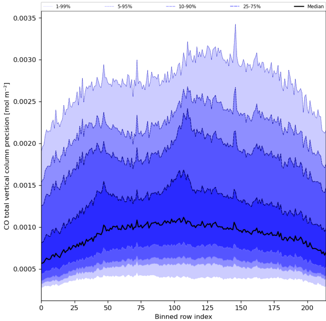
Figure 28: Along track statistics of “CO total vertical column precision” for 2024-02-24 to 2024-02-26
