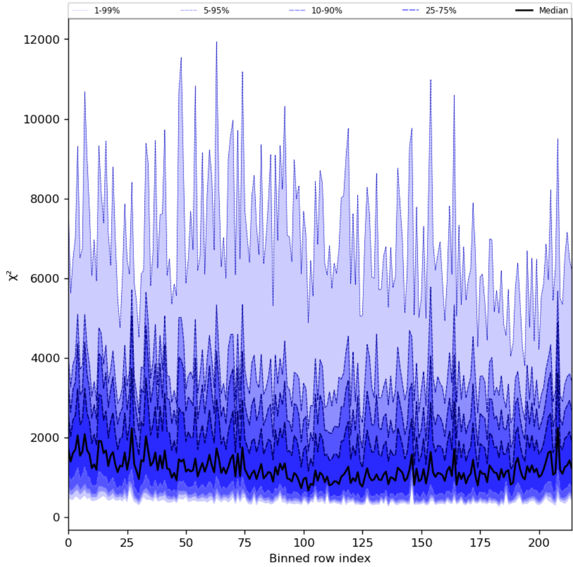
Figure 30: Along track statistics of “ \chi^2 ” for 2024-02-24 to 2024-02-26
