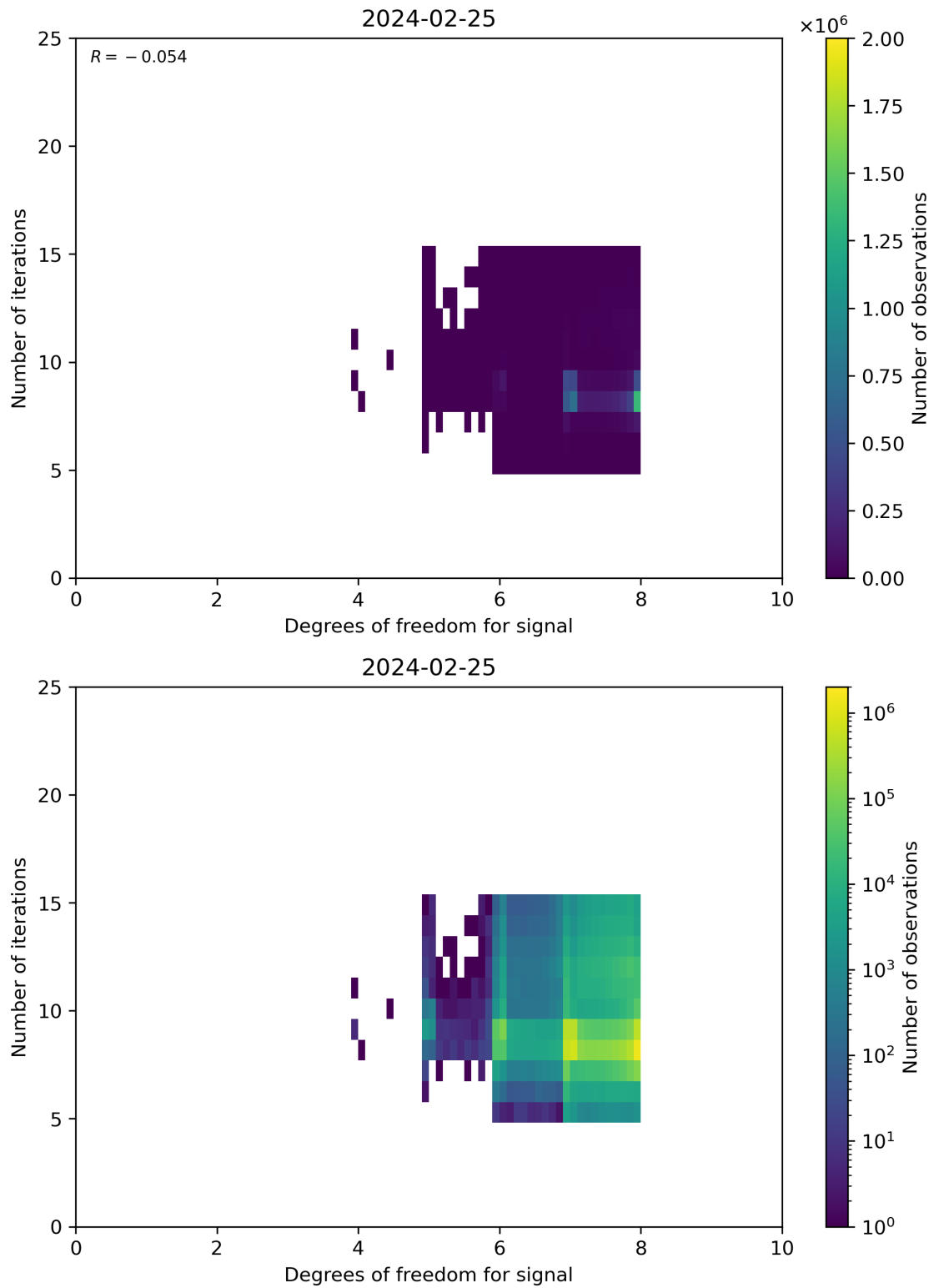
Figure 50: Scatter density plot of “Degrees of freedom for signal” against “Number of iterations” for 2024-02-24 to 2024-02-26.
