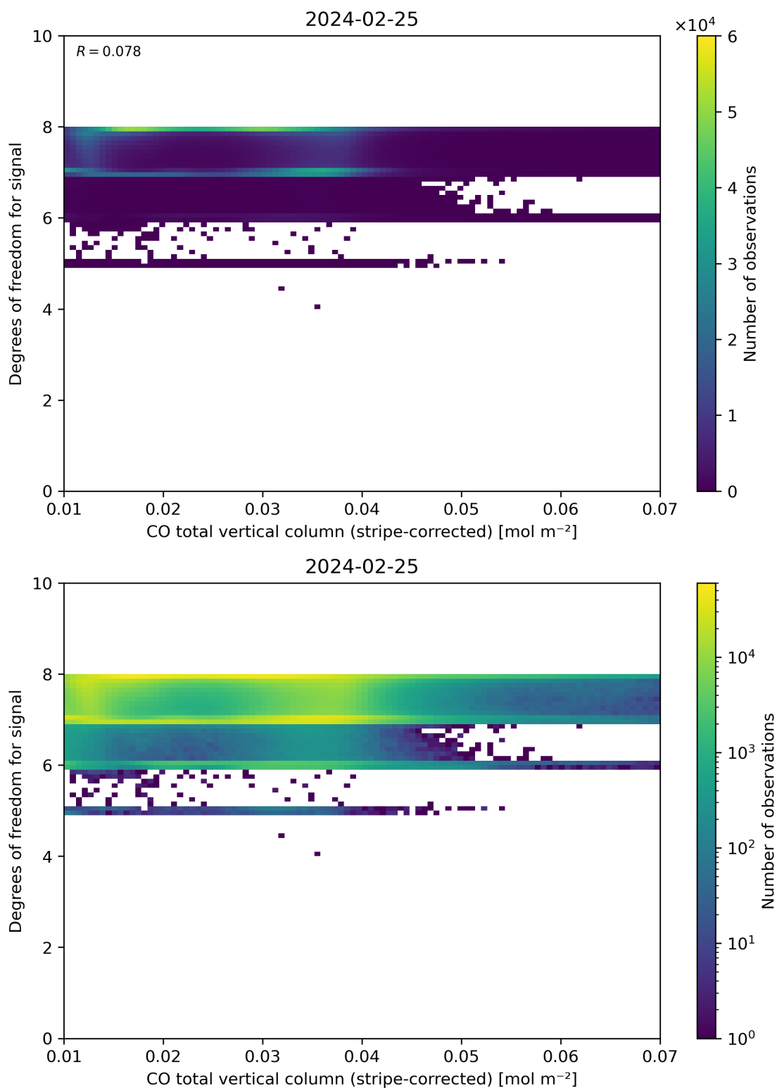
Figure 38: Scatter density plot of “CO total vertical column (stripe-corrected)” against “Degrees of freedom for signal” for 2024-02-24 to 2024-02-26.
