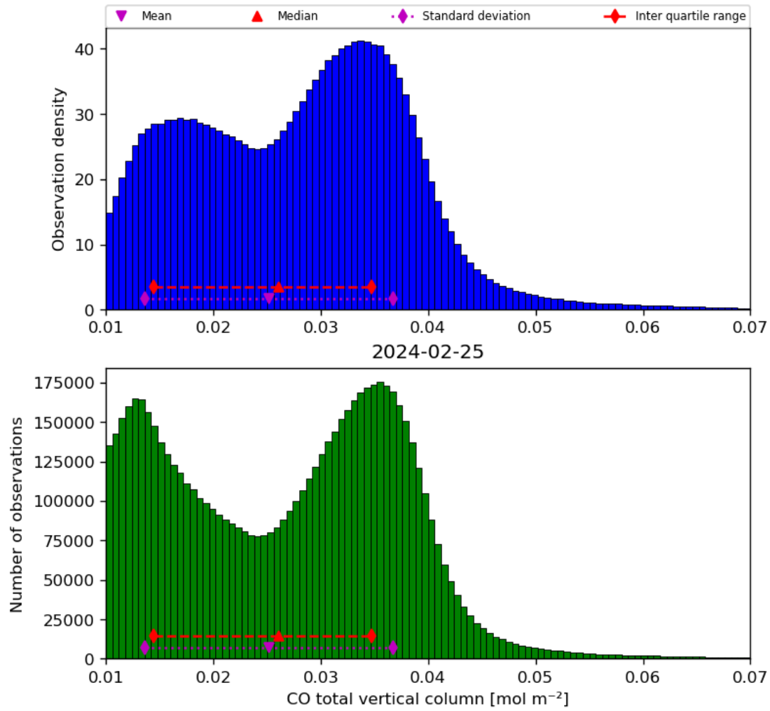
Figure 18: Histogram of “CO total vertical column” for 2024-02-24 to 2024-02-26
