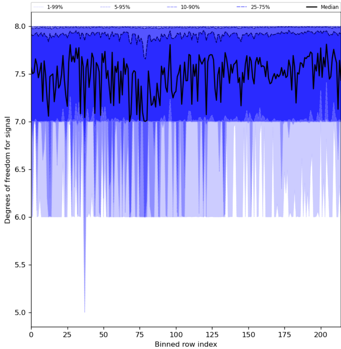
Figure 31: Along track statistics of “Degrees of freedom for signal” for 2024-02-24 to 2024-02-26
