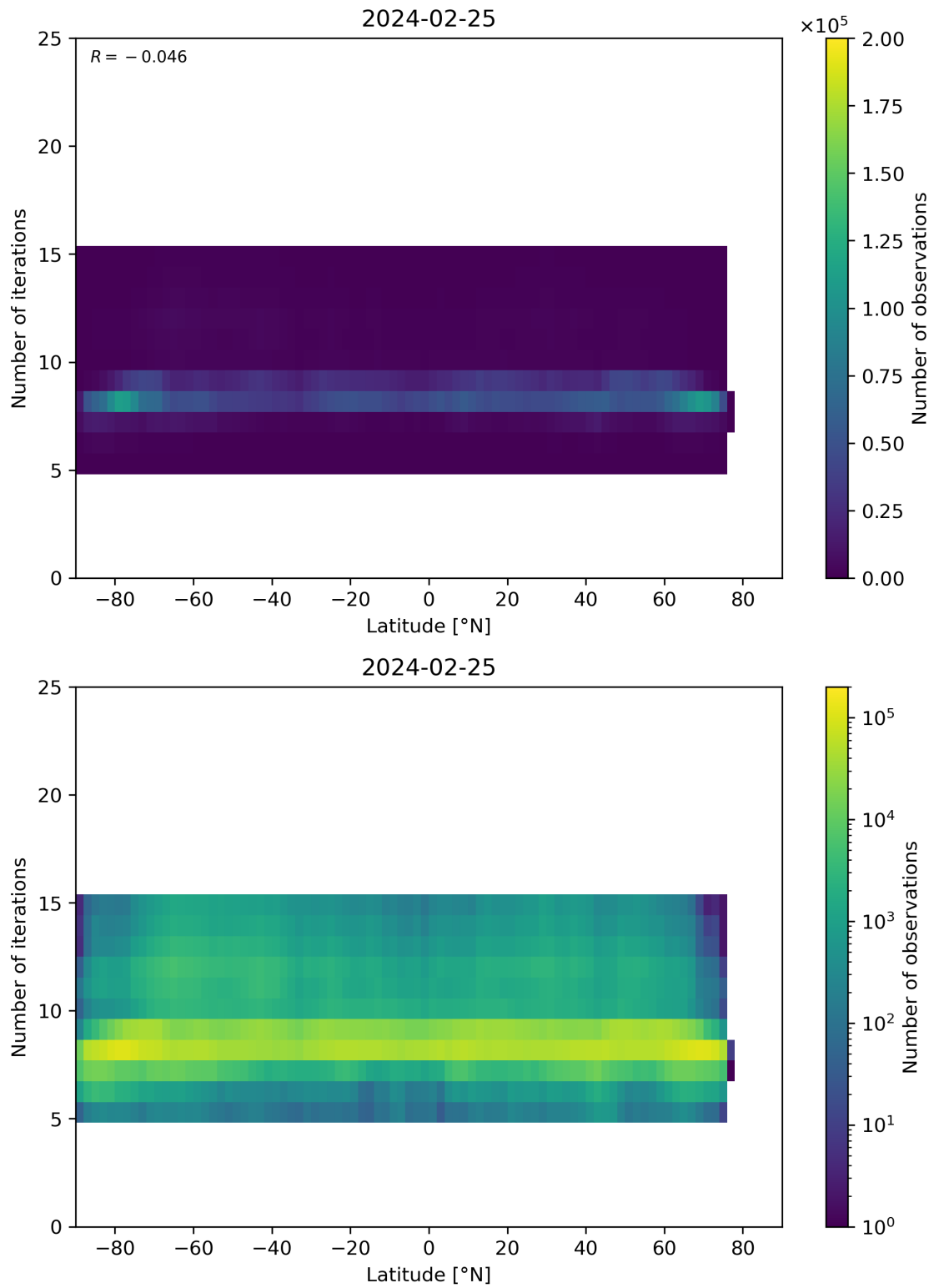
Figure 56: Scatter density plot of “Latitude” against “Number of iterations” for 2024-02-24 to 2024-02-26.
