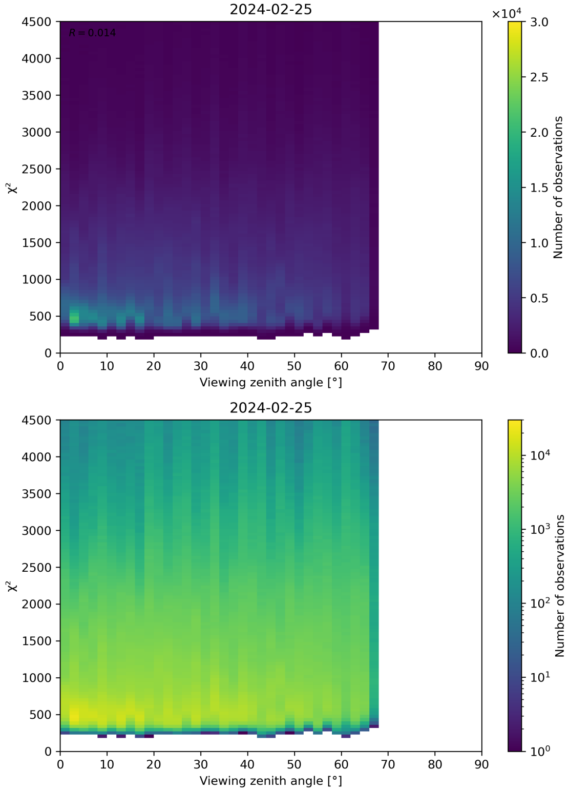
Figure 72: Scatter density plot of “Viewing zenith angle” against “ \chi^2 ” for 2024-02-24 to 2024-02-26.
