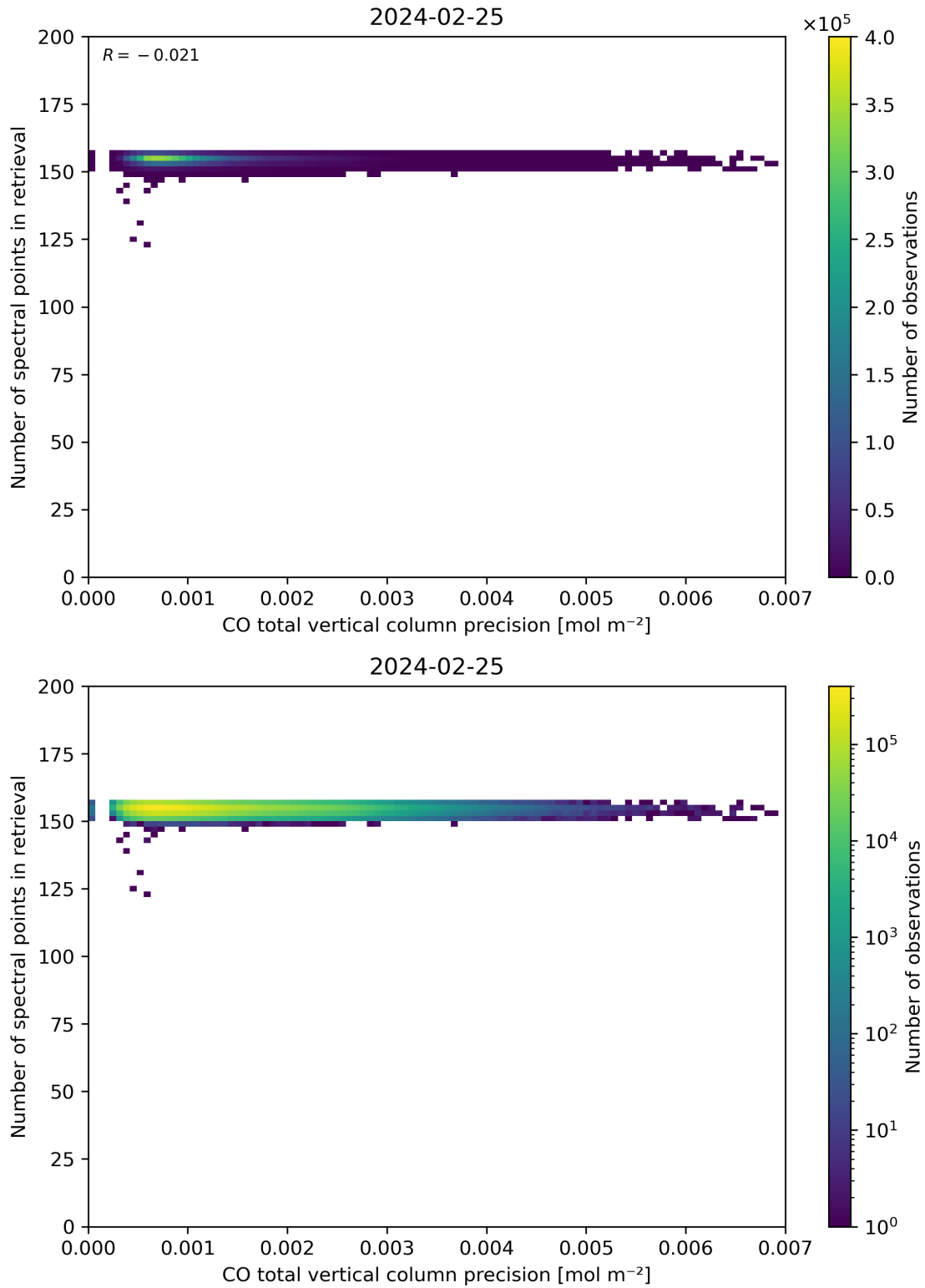
Figure 47: Scatter density plot of “CO total vertical column precision” against “Number of spectral points in retrieval” for 2024-02-24 to 2024-02-26.
