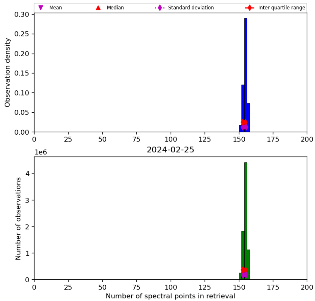
Figure 21: Histogram of “Number of spectral points in retrieval” for 2024-02-24 to 2024-02-26
