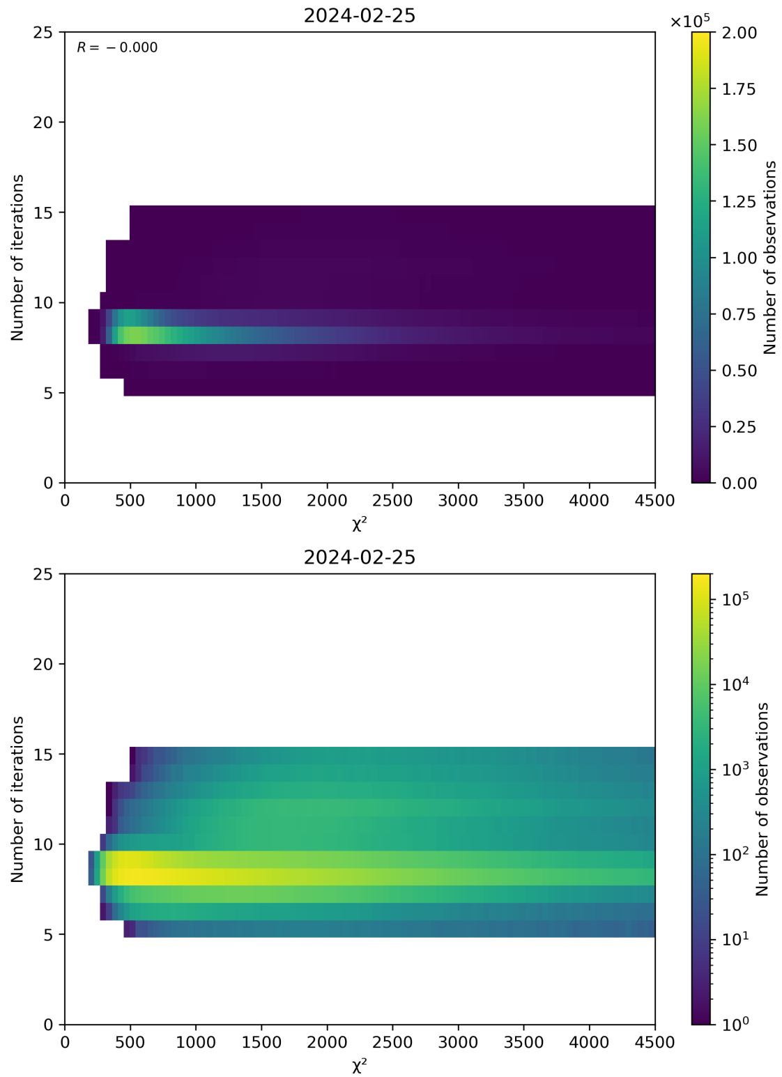
Figure 49: Scatter density plot of “ \chi^2 ” against “Number of iterations” for 2024-02-24 to 2024-02-26.
