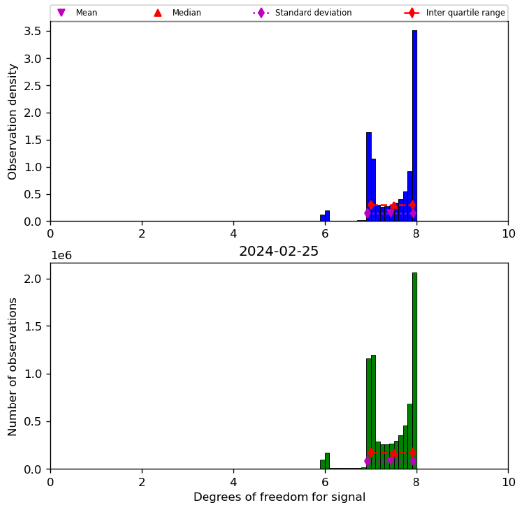
Figure 23: Histogram of “Degrees of freedom for signal” for 2024-02-24 to 2024-02-26
