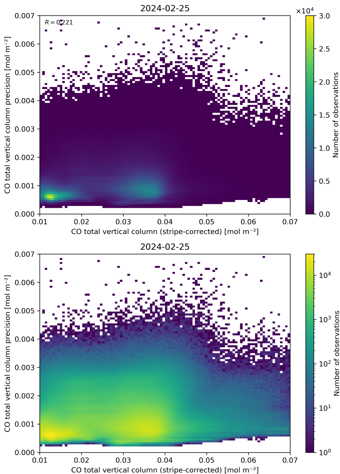
Figure 36: Scatter density plot of “CO total vertical column (stripe-corrected)” against “CO total vertical column precision” for 2024-02-24 to 2024-02-26.
