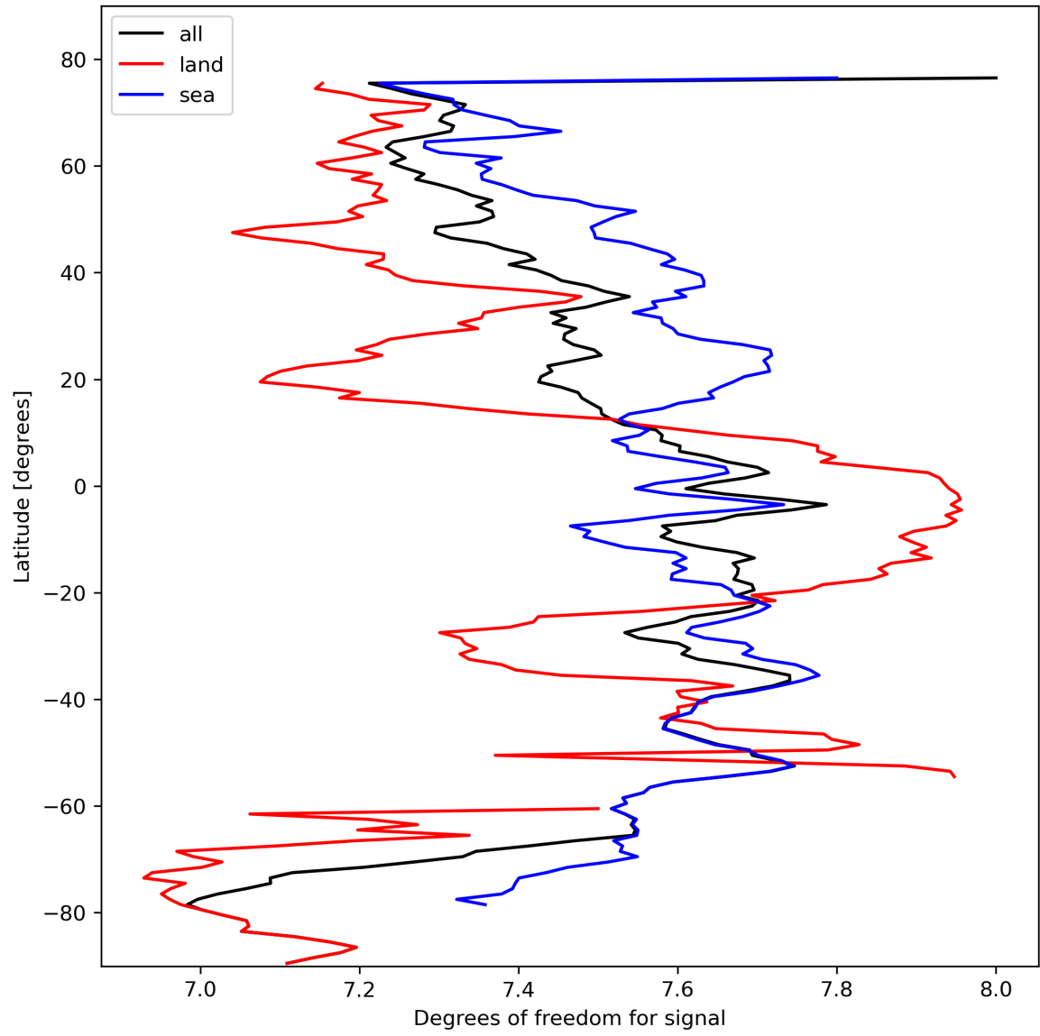
Figure 15: Zonal average of “Degrees of freedom for signal” for 2024-02-24 to 2024-02-26.
