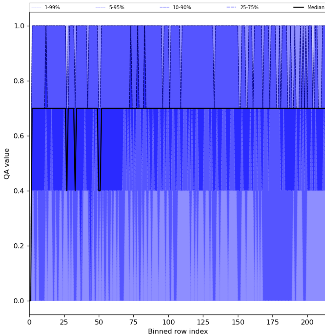
Figure 25: Along track statistics of “QA value” for 2024-02-24 to 2024-02-26
