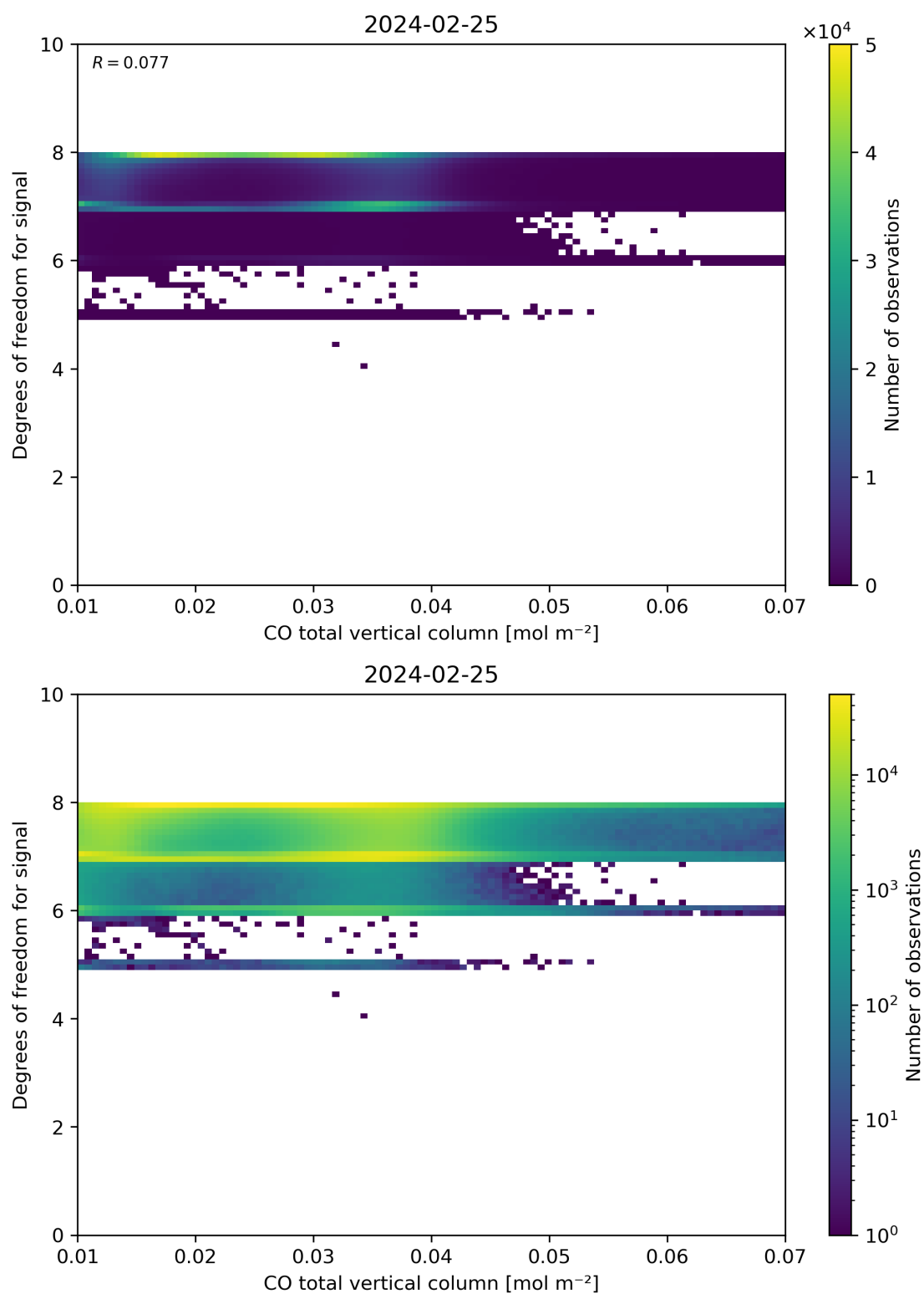
Figure 41: Scatter density plot of “CO total vertical column” against “Degrees of freedom for signal” for 2024-02-24 to 2024-02-26.
