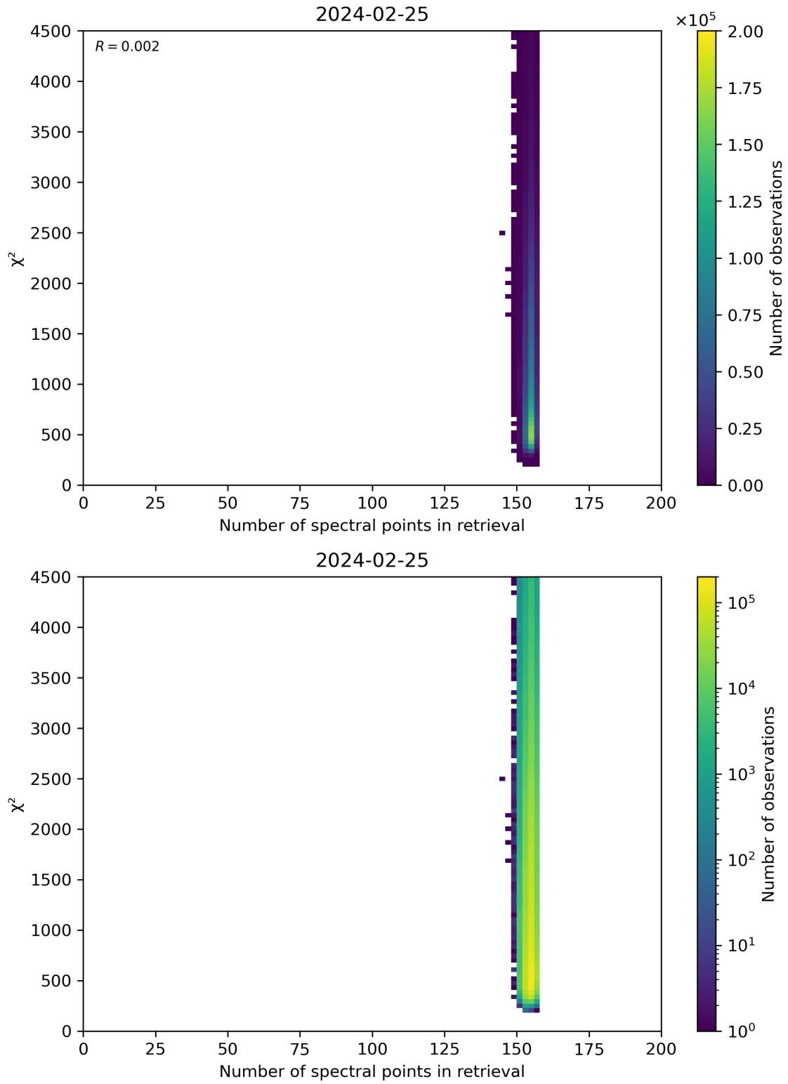
Figure 58: Scatter density plot of “Number of spectral points in retrieval” against “ \chi^2 ” for 2024-02-24 to 2024-02-26.
