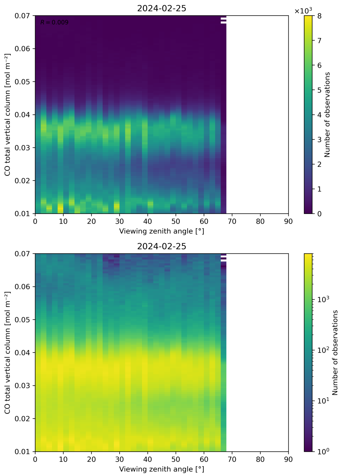
Figure 69: Scatter density plot of “Viewing zenith angle” against “CO total vertical column” for 2024-02-24 to 2024-02-26.
