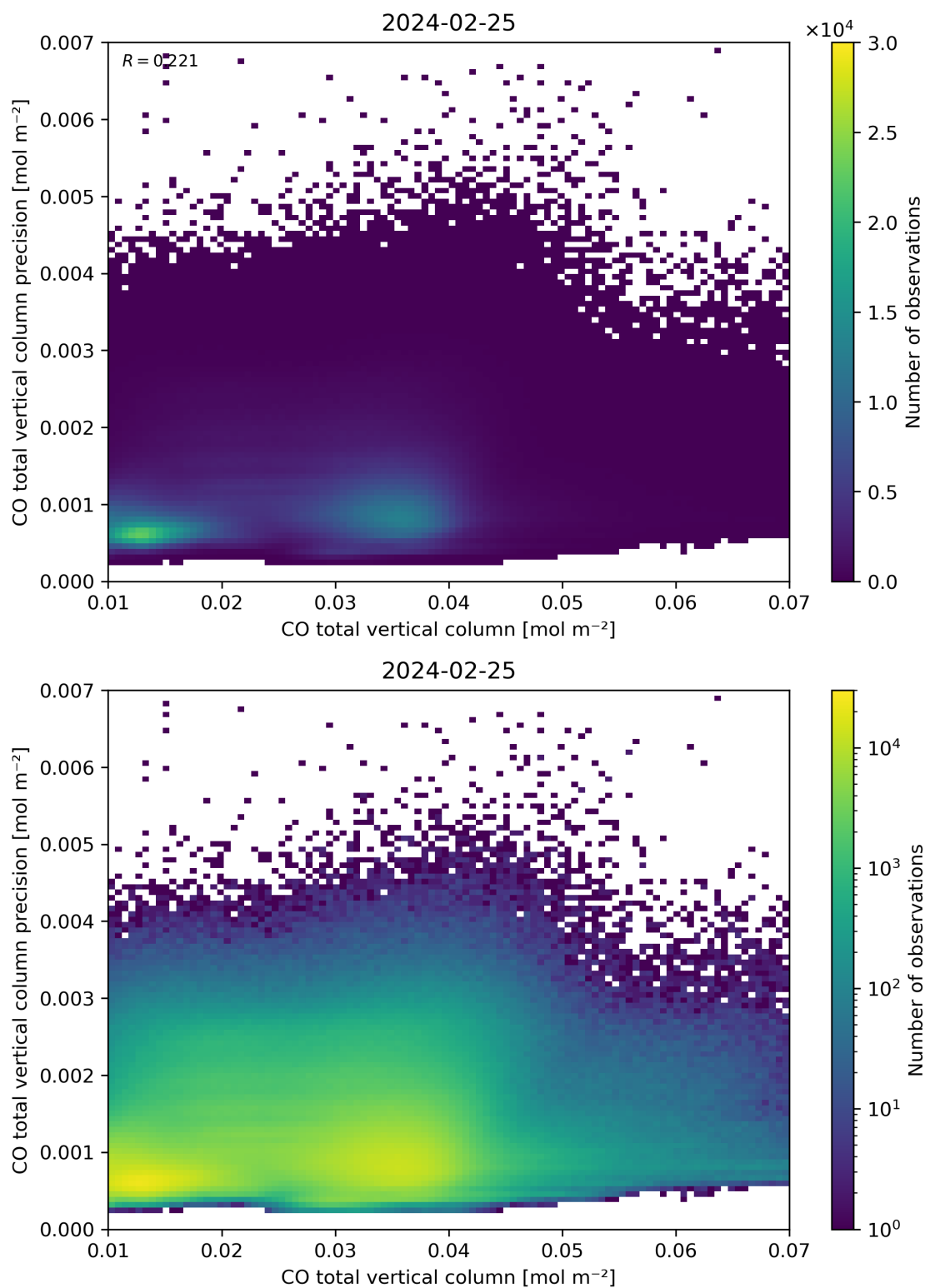
Figure 34: Scatter density plot of “CO total vertical column” against “CO total vertical column precision” for 2024-02-24 to 2024-02-26.
