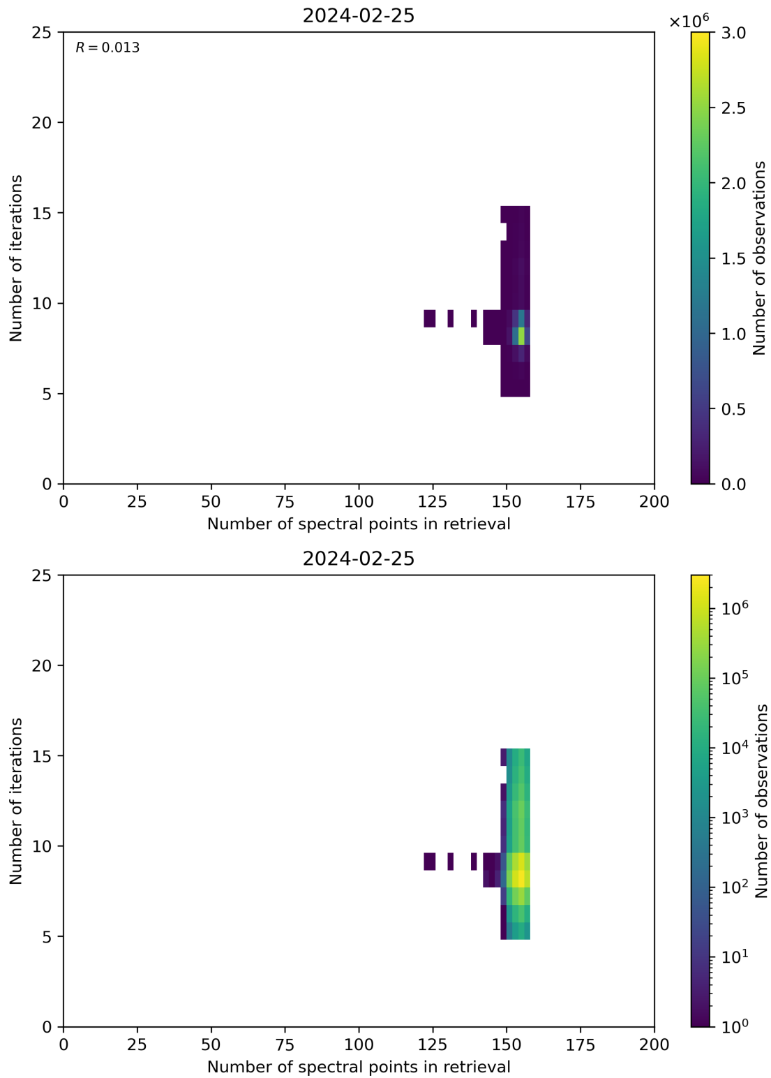
Figure 60: Scatter density plot of “Number of spectral points in retrieval” against “Number of iterations” for 2024-02-24 to 2024-02-26.
