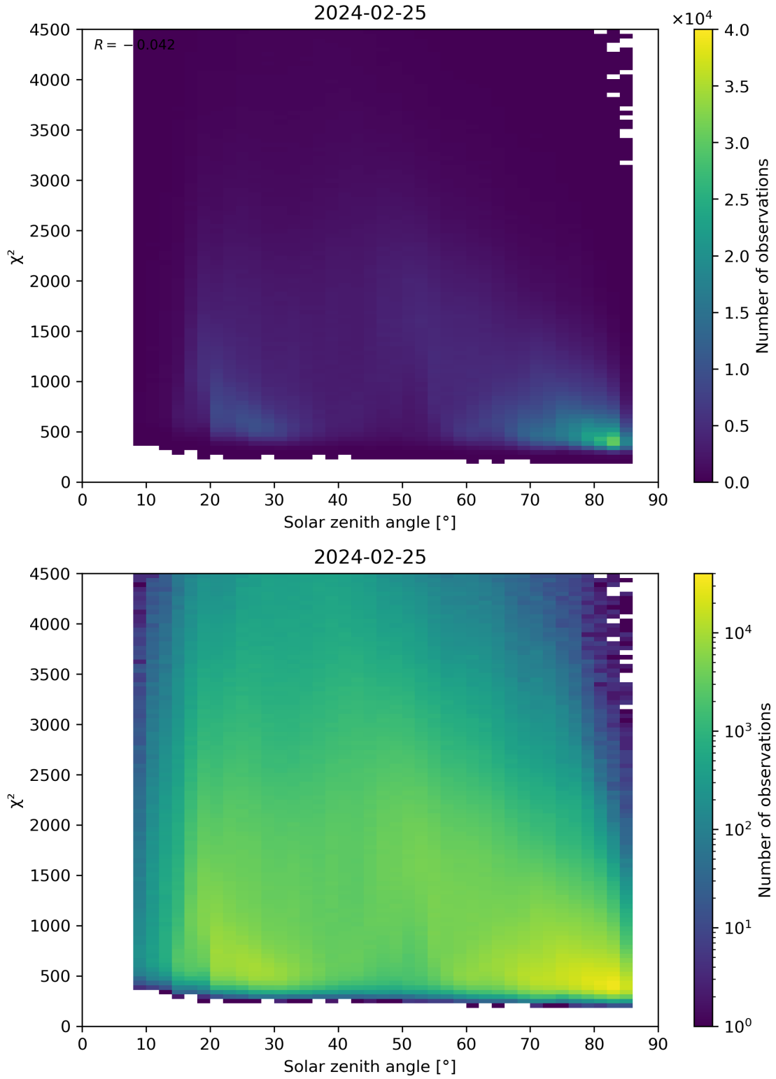
Figure 64: Scatter density plot of “Solar zenith angle” against “ \chi^2 ” for 2024-02-24 to 2024-02-26.
