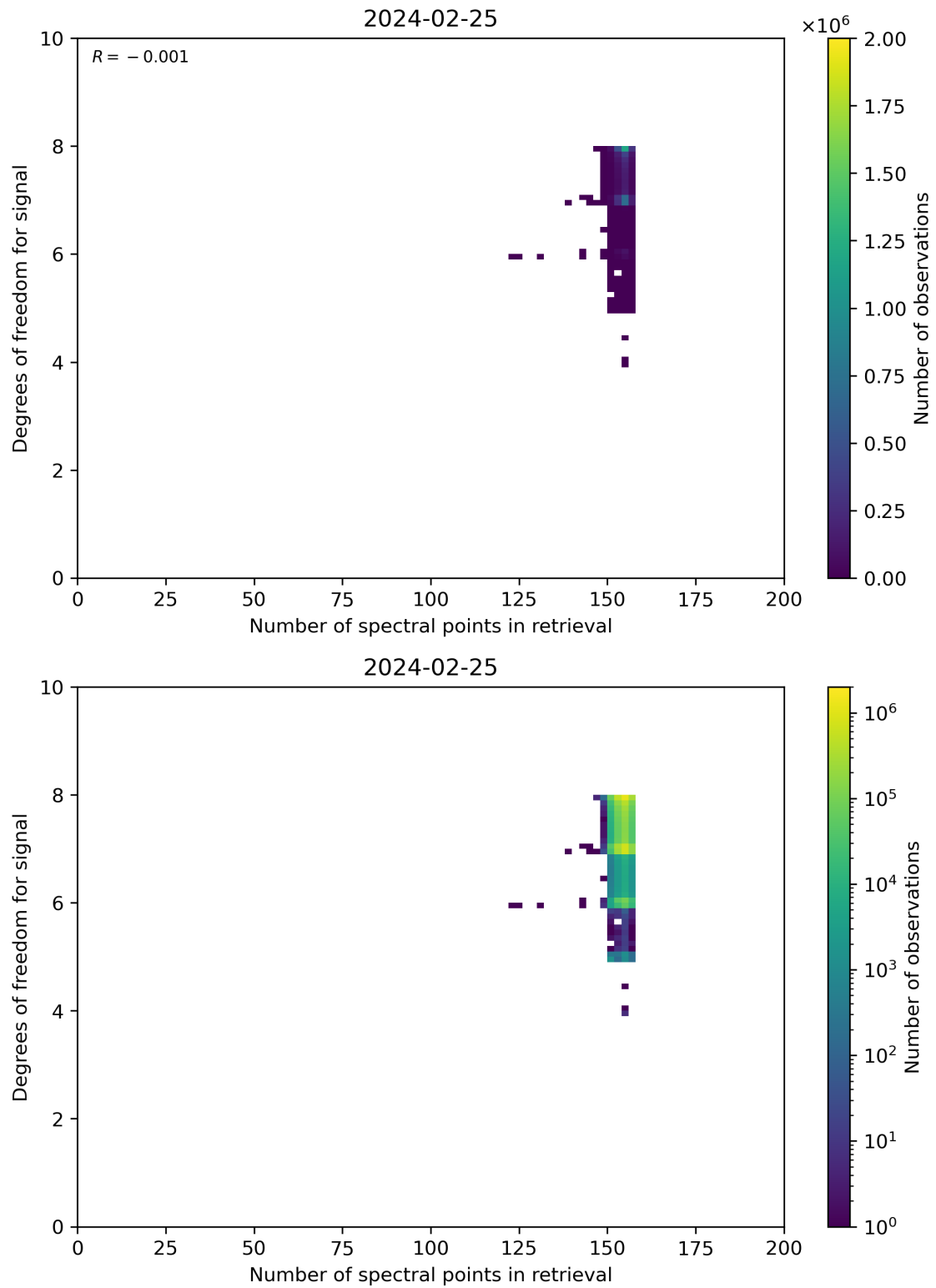
Figure 59: Scatter density plot of “Number of spectral points in retrieval” against “Degrees of freedom for signal” for 2024-02-24 to 2024-02-26.
