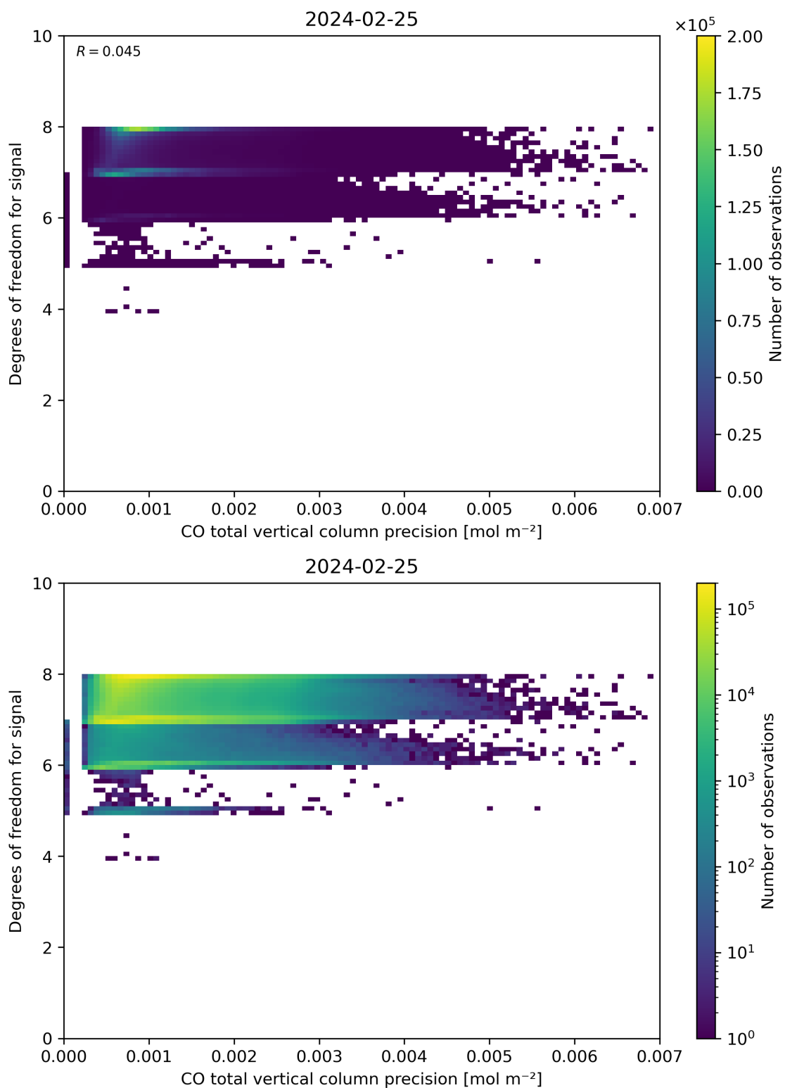
Figure 45: Scatter density plot of “CO total vertical column precision” against “Degrees of freedom for signal” for 2024-02-24 to 2024-02-26.
