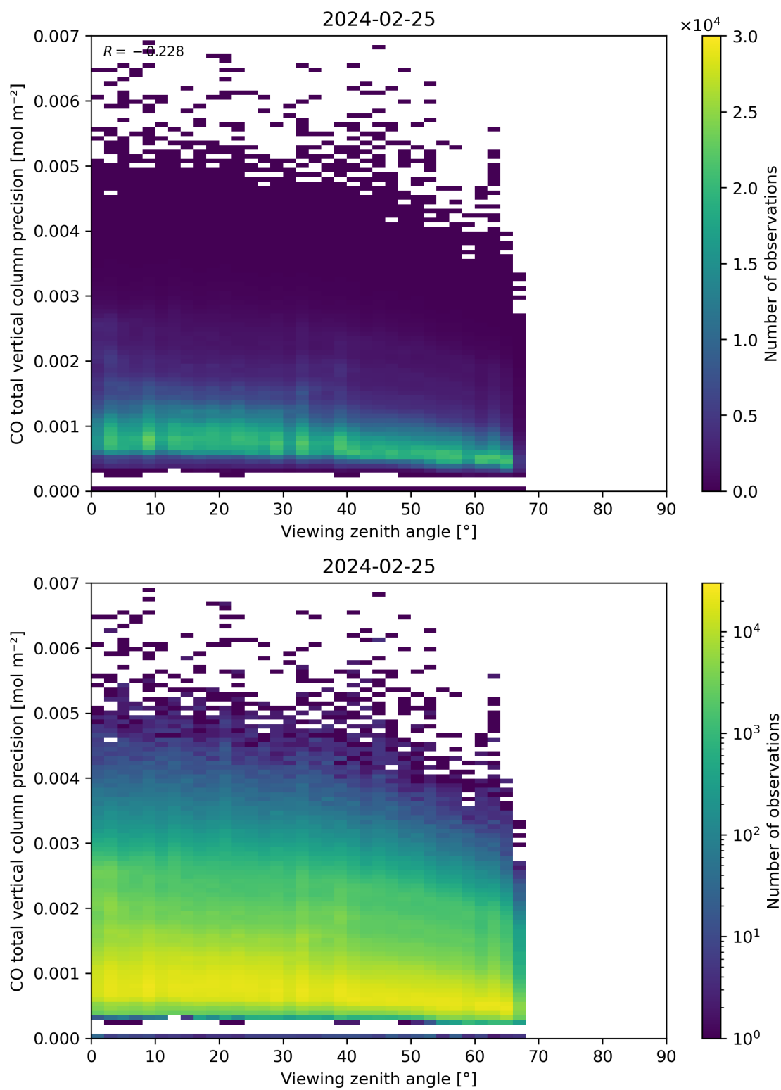
Figure 71: Scatter density plot of “Viewing zenith angle” against “CO total vertical column precision” for 2024-02-24 to 2024-02-26.
