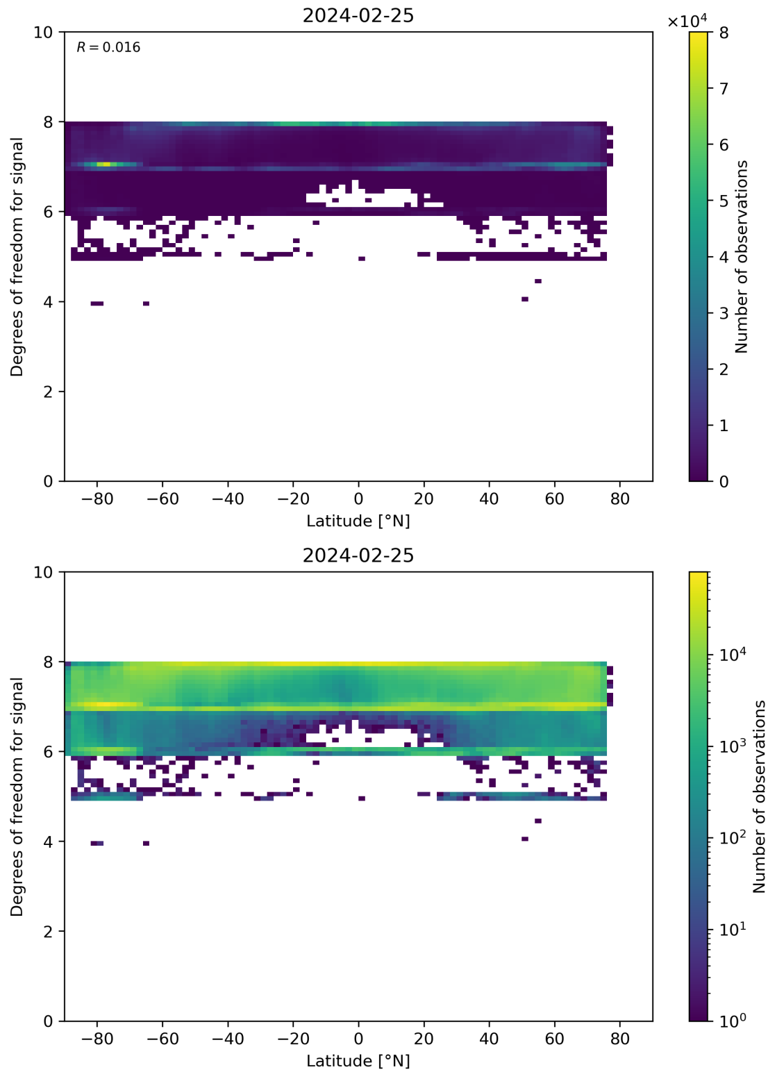
Figure 55: Scatter density plot of “Latitude” against “Degrees of freedom for signal” for 2024-02-24 to 2024-02-26.
