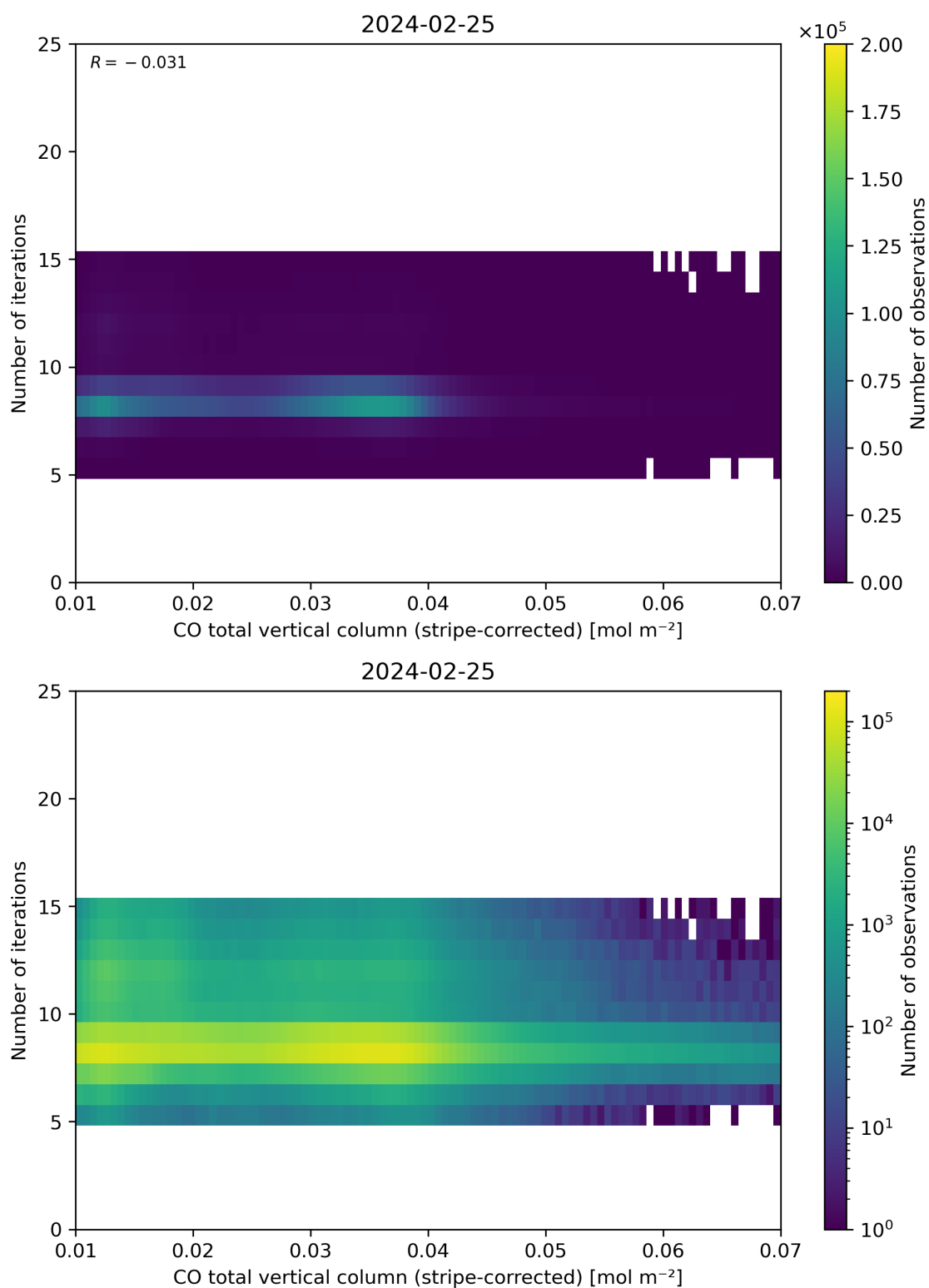
Figure 39: Scatter density plot of “CO total vertical column (stripe-corrected)” against “Number of iterations” for 2024-02-24 to 2024-02-26.
