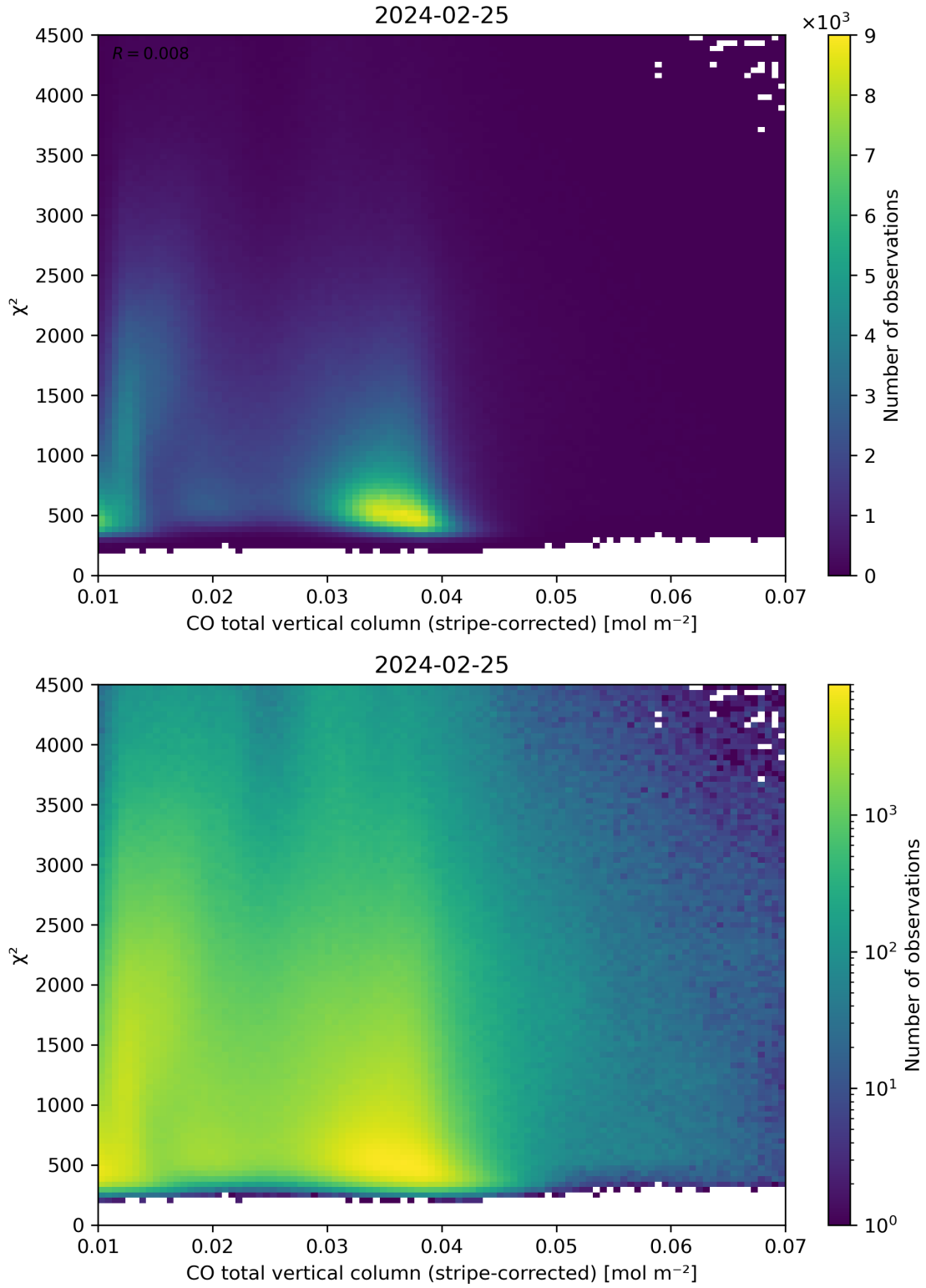
Figure 37: Scatter density plot of “CO total vertical column (stripe-corrected)” against “ \chi^2 ” for 2024-02-24 to 2024-02-26.
