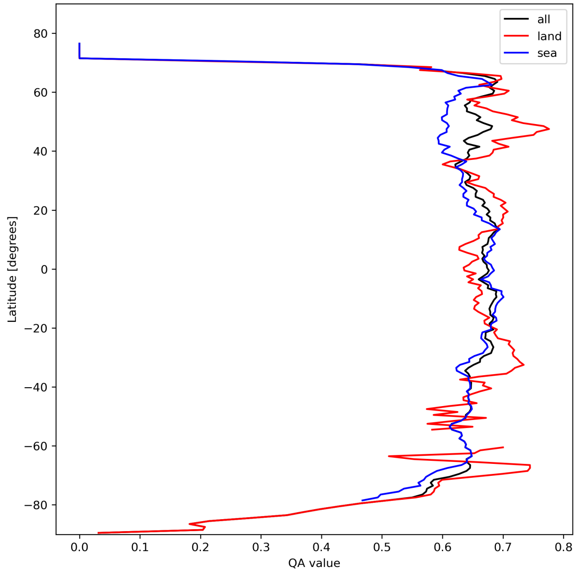
Figure 9: Zonal average of “QA value” for 2024-02-24 to 2024-02-26.
