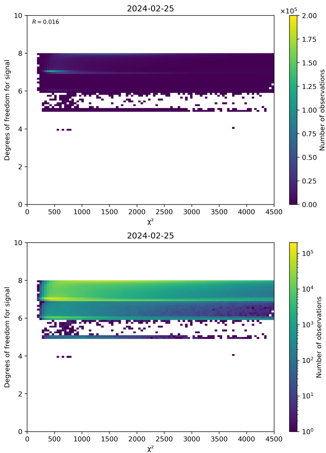
Figure 48: Scatter density plot of “ \chi^2 ” against “Degrees of freedom for signal” for 2024-02-24 to 2024-02-26.
