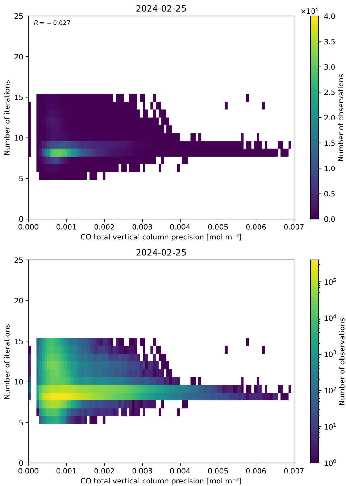
Figure 46: Scatter density plot of “CO total vertical column precision” against “Number of iterations” for 2024-02-24 to 2024-02-26.
