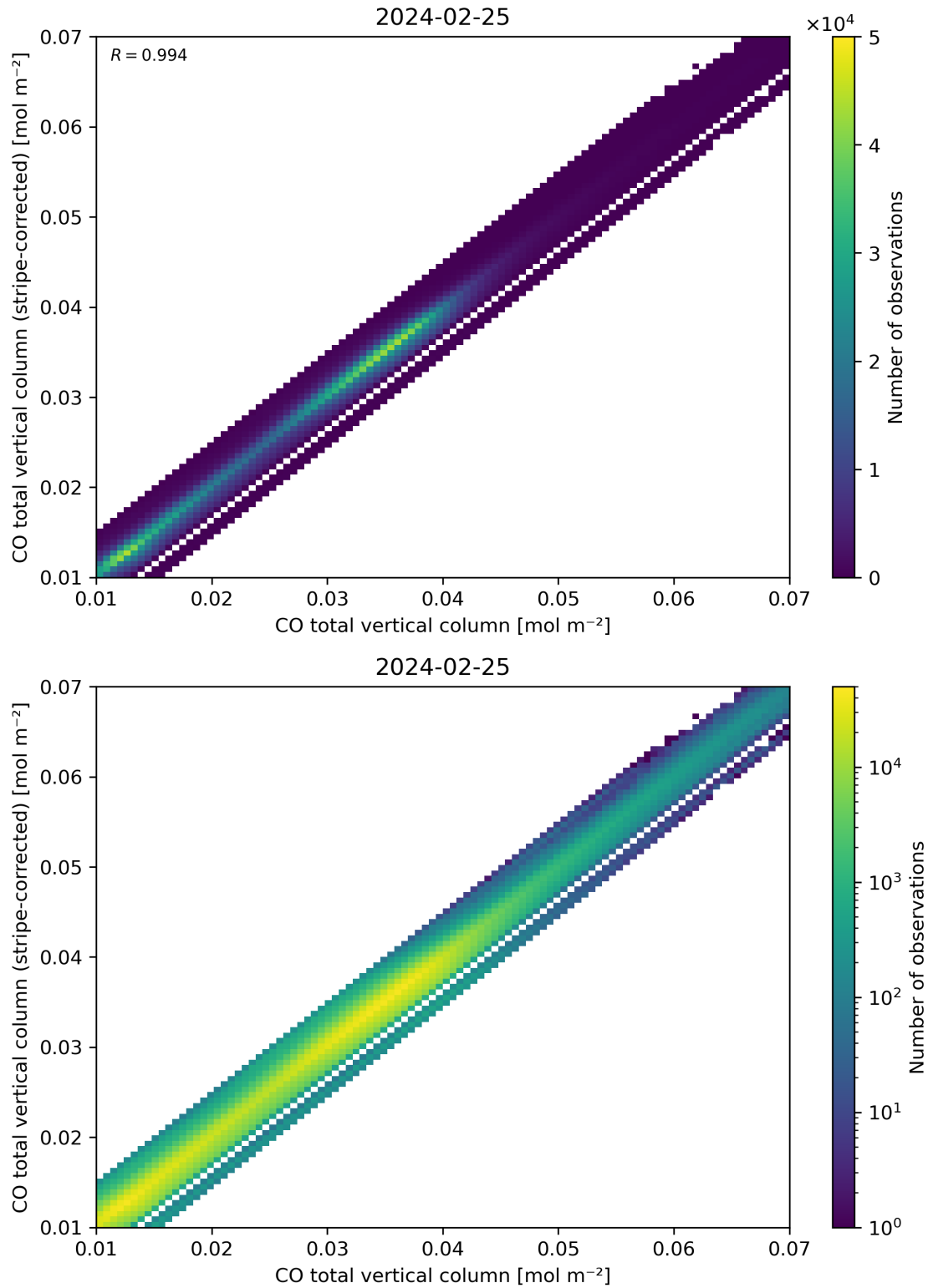
Figure 33: Scatter density plot of “CO total vertical column” against “CO total vertical column (stripe-corrected)” for 2024-02-24 to 2024-02-26.
