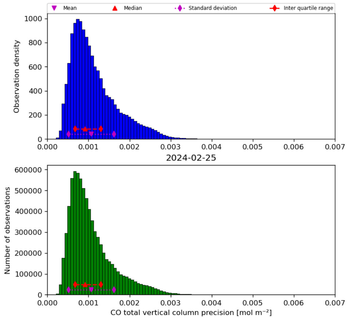
Figure 20: Histogram of “CO total vertical column precision” for 2024-02-24 to 2024-02-26
