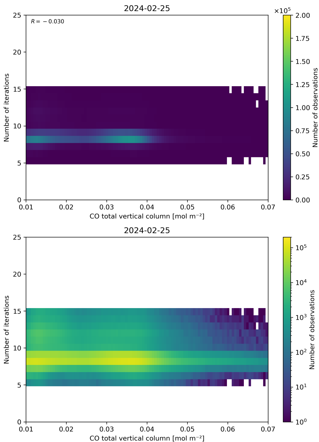
Figure 42: Scatter density plot of “CO total vertical column” against “Number of iterations” for 2024-02-24 to 2024-02-26.
