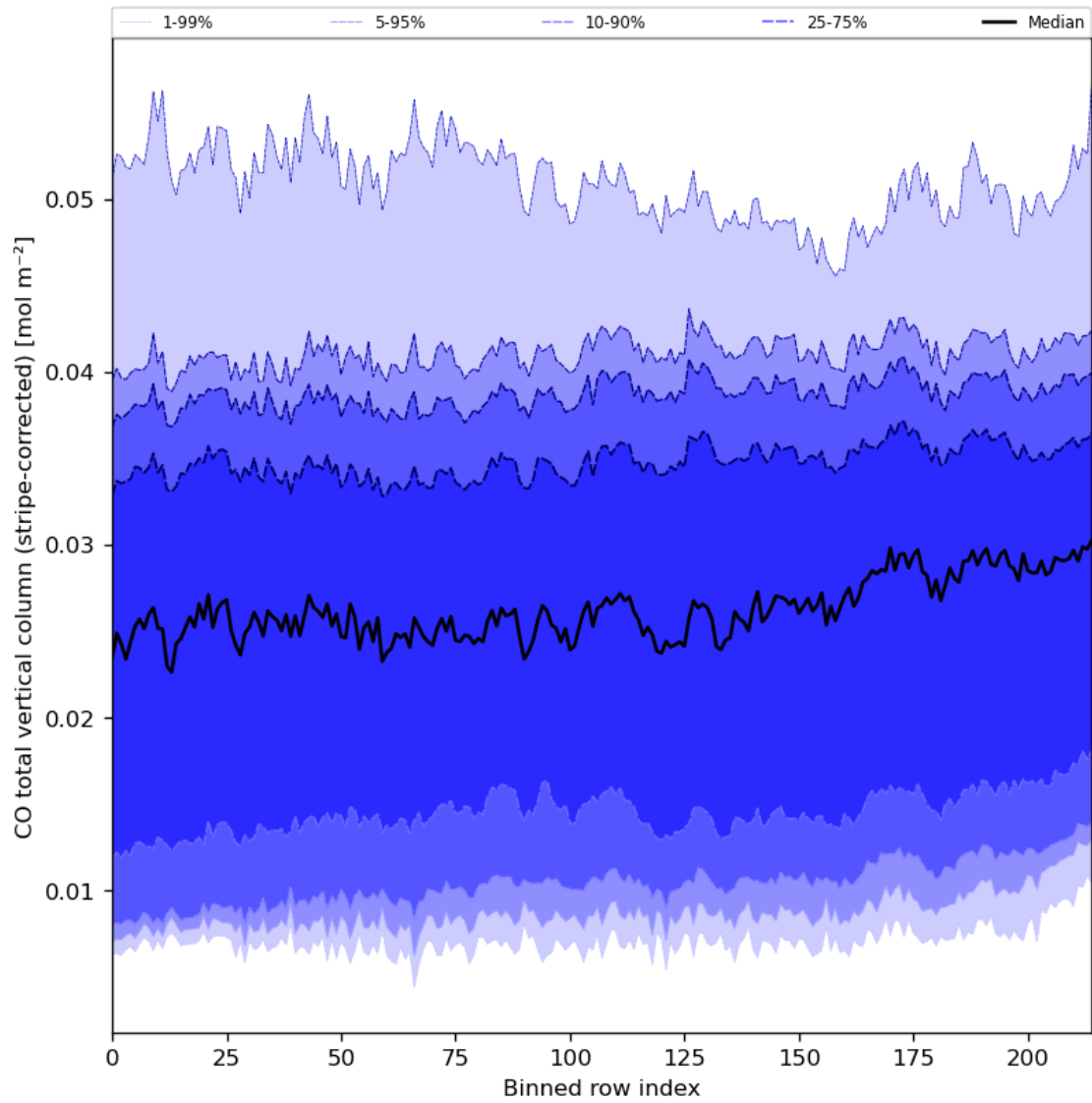
Figure 27: Along track statistics of "CO total vertical column (stripe-corrected)" for 2024-02-24 to 2024-02-26
