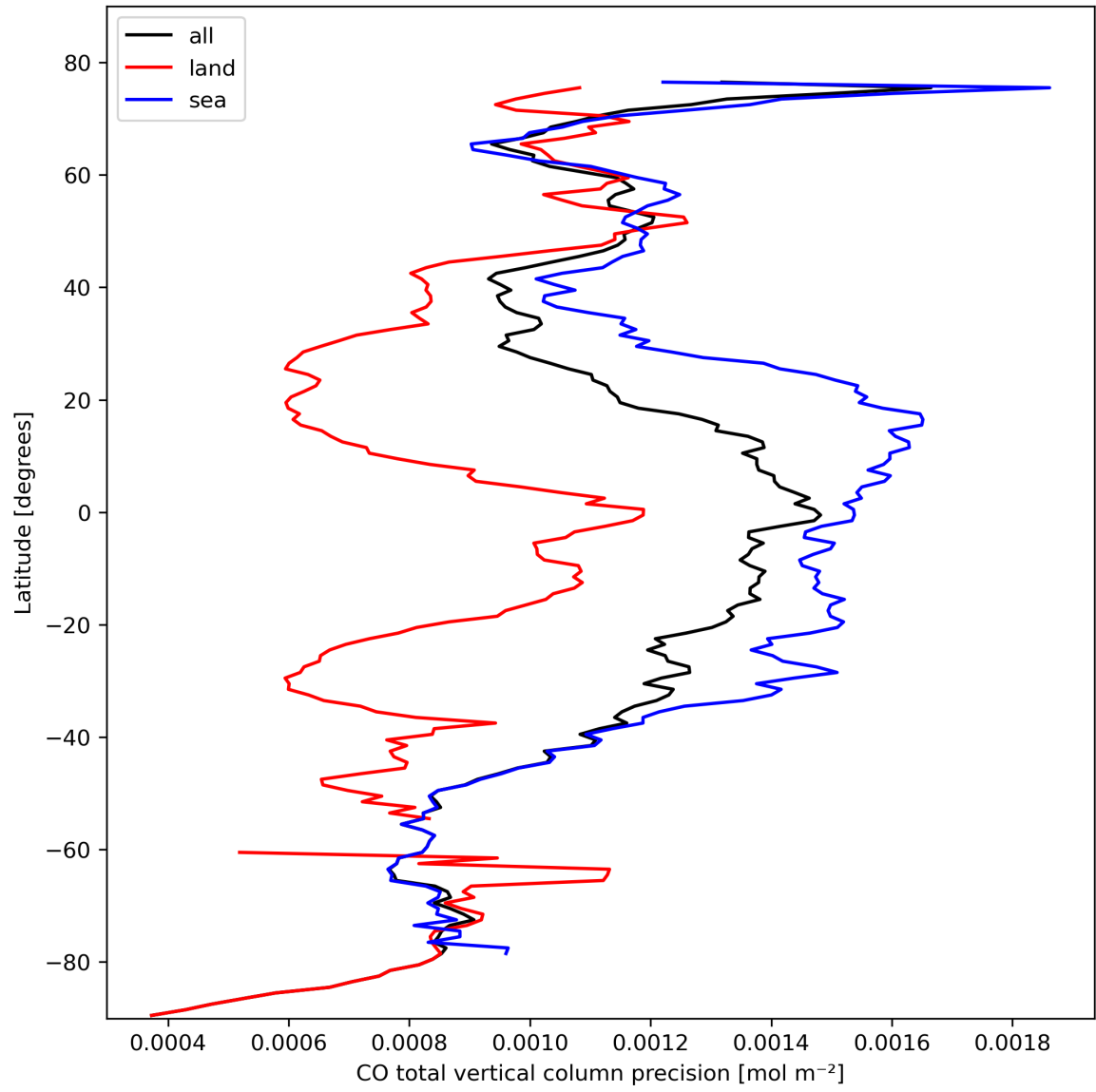
Figure 12: Zonal average of “CO total vertical column precision” for 2024-02-24 to 2024-02-26.
