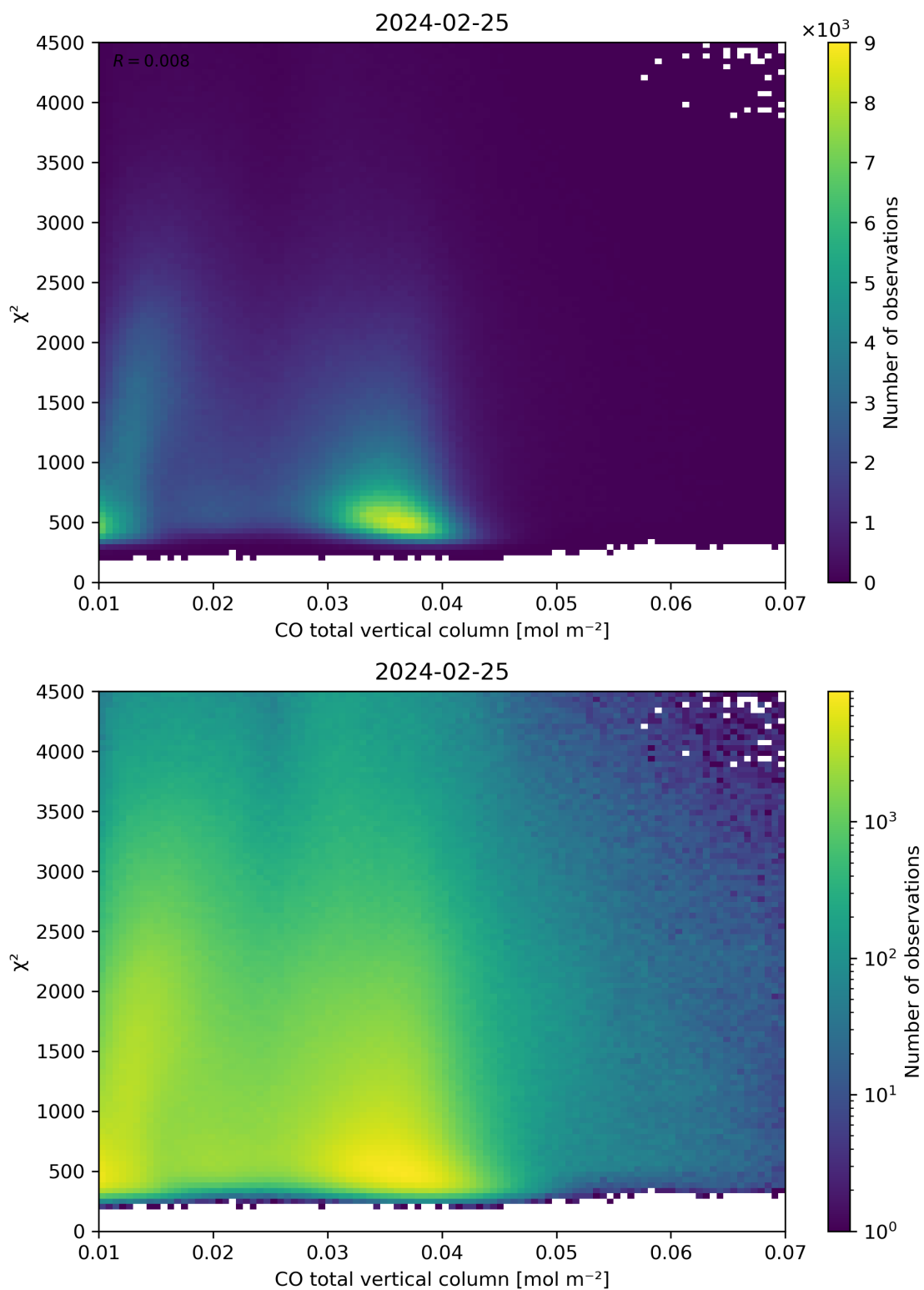
Figure 35: Scatter density plot of “CO total vertical column” against “ \chi^2 ” for 2024-02-24 to 2024-02-26.
