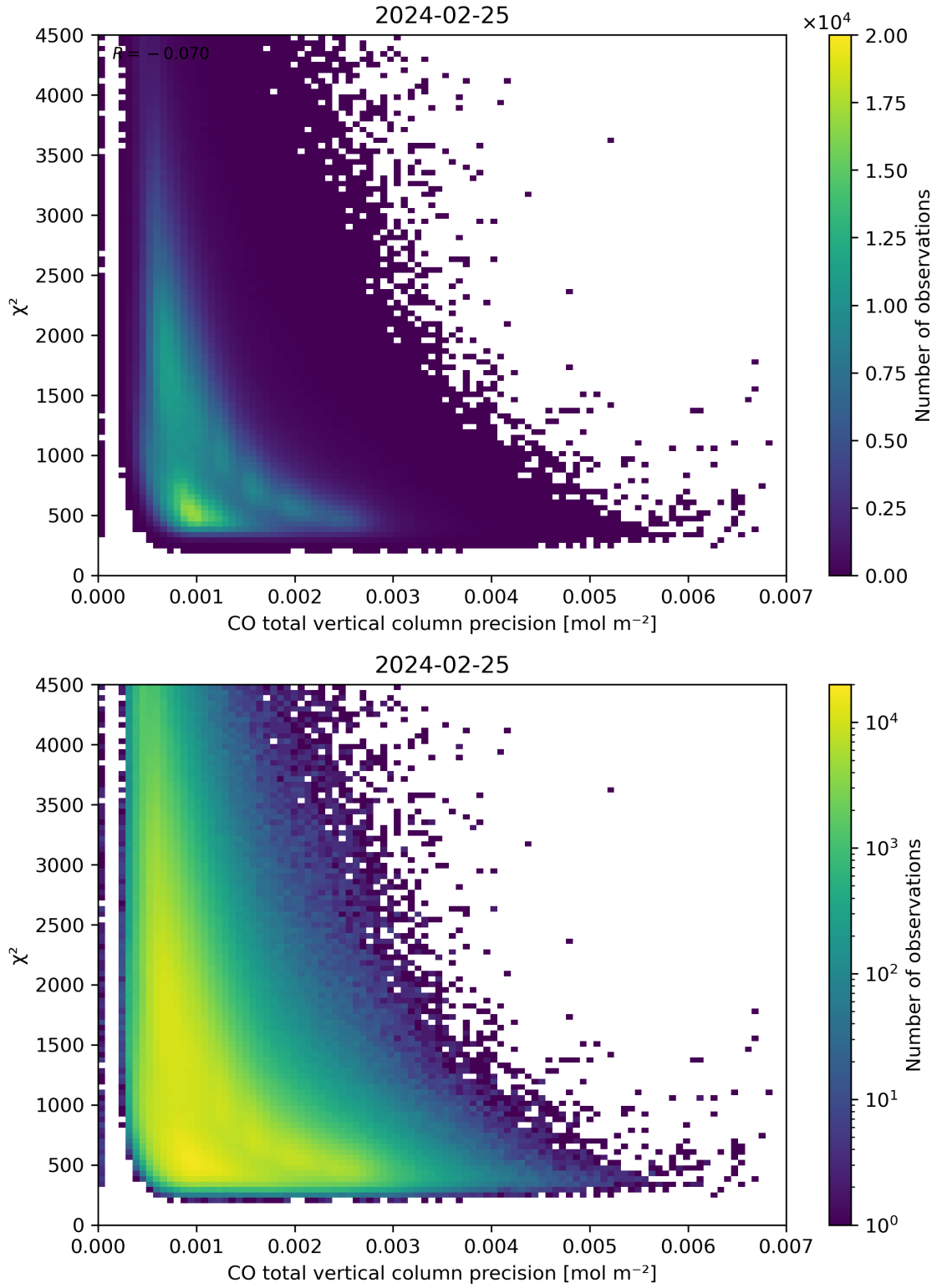
Figure 44: Scatter density plot of “CO total vertical column precision” against “ \chi^2 ” for 2024-02-24 to 2024-02-26.
