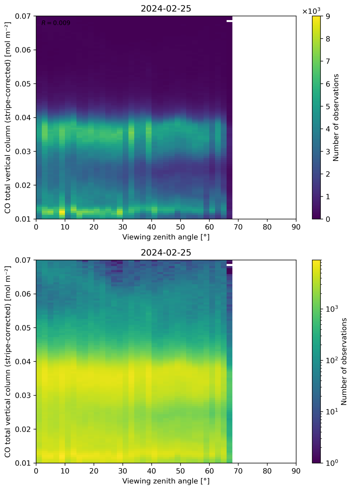
Figure 70: Scatter density plot of “Viewing zenith angle” against “CO total vertical column (stripe-corrected)” for 2024-02-24 to 2024-02-26.
