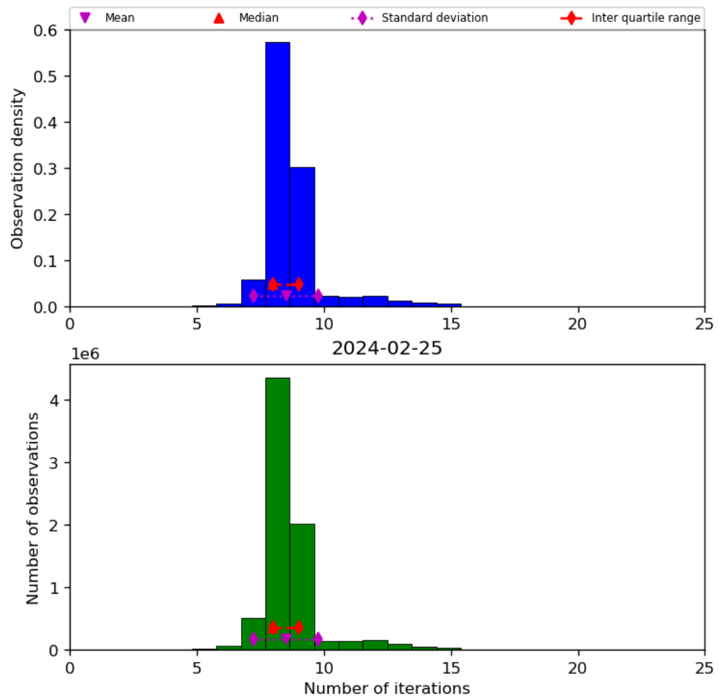
Figure 24: Histogram of “Number of iterations” for 2024-02-24 to 2024-02-26
