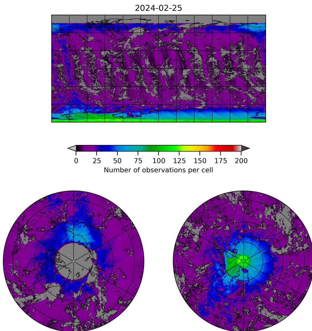
Figure 8: Map of the number of observations for 2024-02-24 to 2024-02-26
