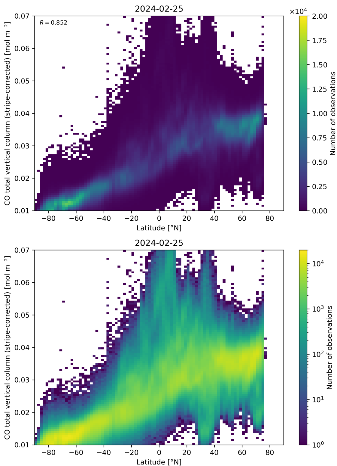
Figure 52: Scatter density plot of “Latitude” against “CO total vertical column (stripe-corrected)” for 2024-02-24 to 2024-02-26.
