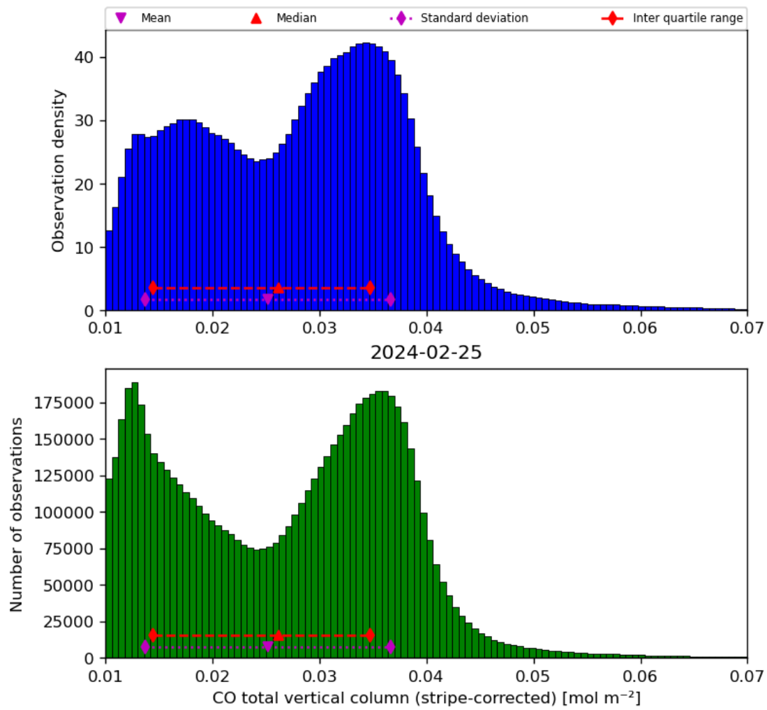
Figure 19: Histogram of “CO total vertical column (stripe-corrected)” for 2024-02-24 to 2024-02-26
