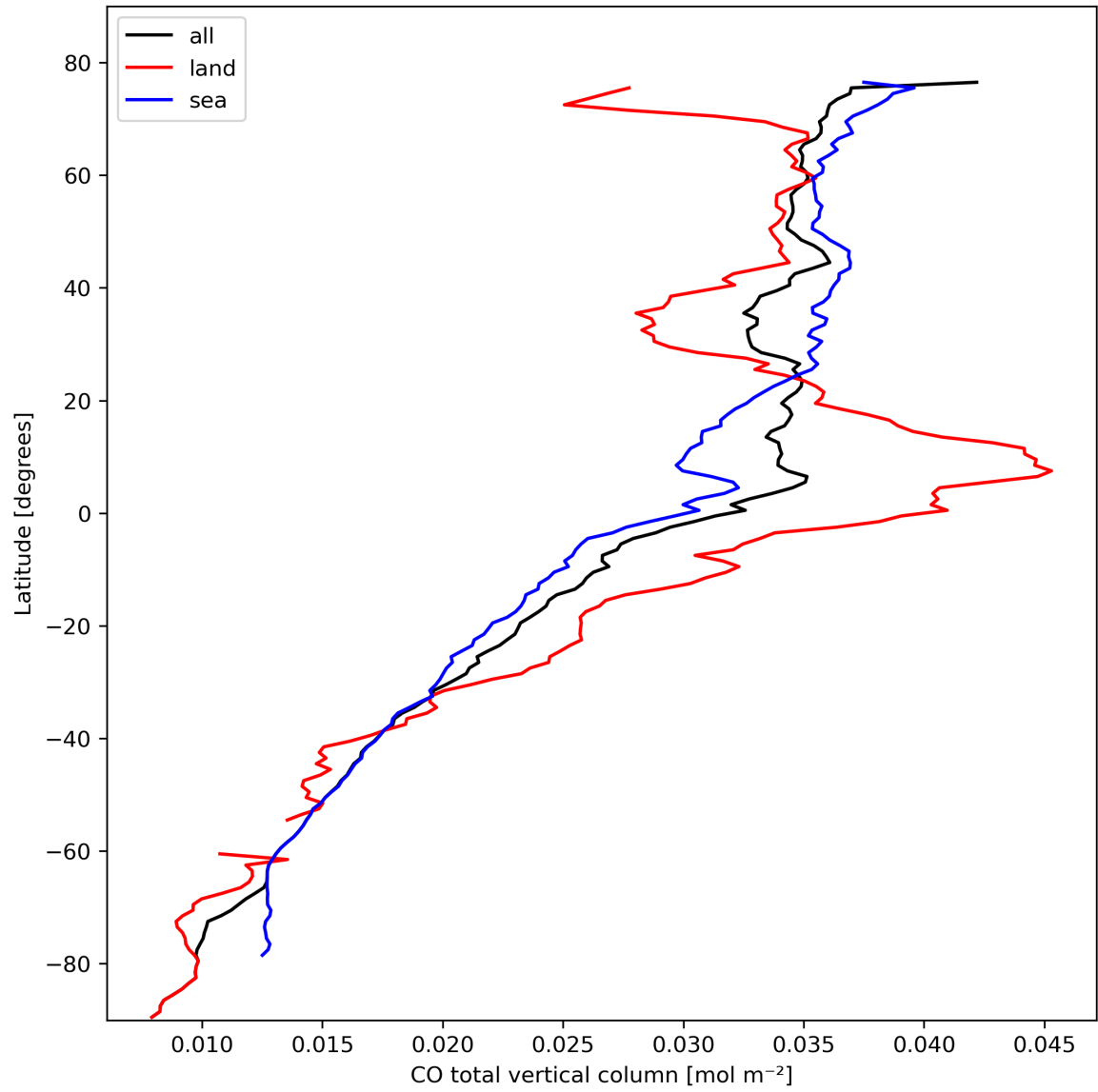
Figure 10: Zonal average of “CO total vertical column” for 2024-02-24 to 2024-02-26.
