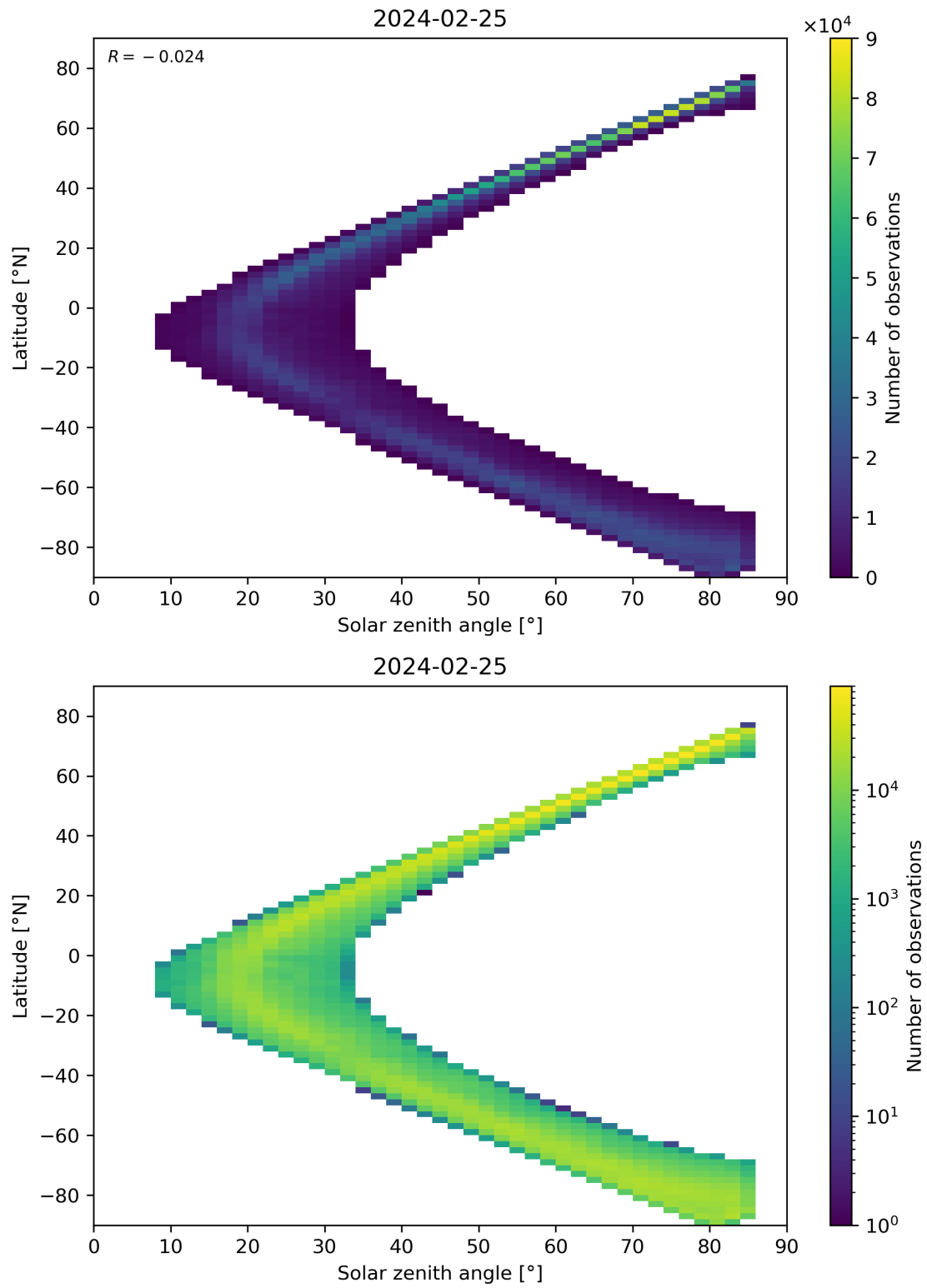
Figure 66: Scatter density plot of “Solar zenith angle” against “Latitude” for 2024-02-24 to 2024-02-26.
