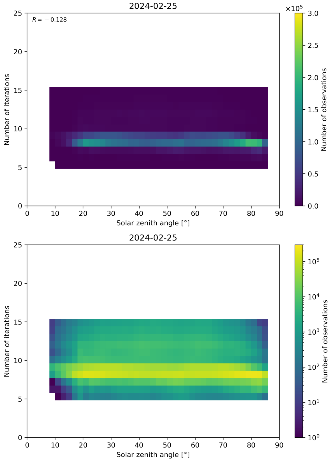
Figure 67: Scatter density plot of “Solar zenith angle” against “Number of iterations” for 2024-02-24 to 2024-02-26.
