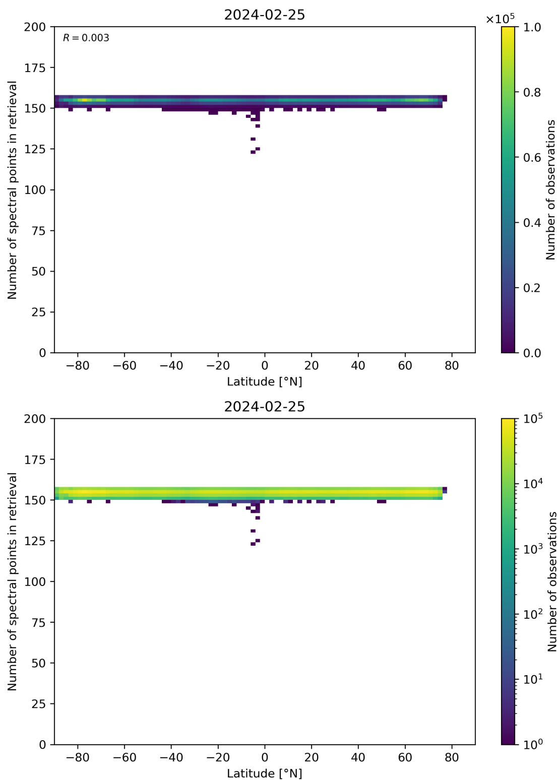
Figure 57: Scatter density plot of “Latitude” against “Number of spectral points in retrieval” for 2024-02-24 to 2024-02-26.
