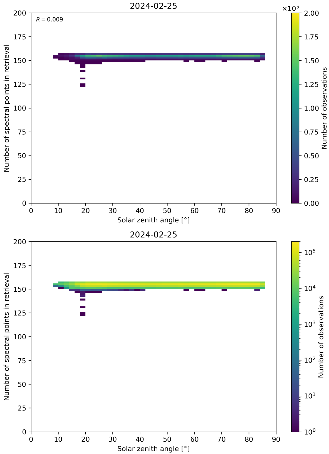
Figure 68: Scatter density plot of “Solar zenith angle” against “Number of spectral points in retrieval” for 2024-02-24 to 2024-02-26.
