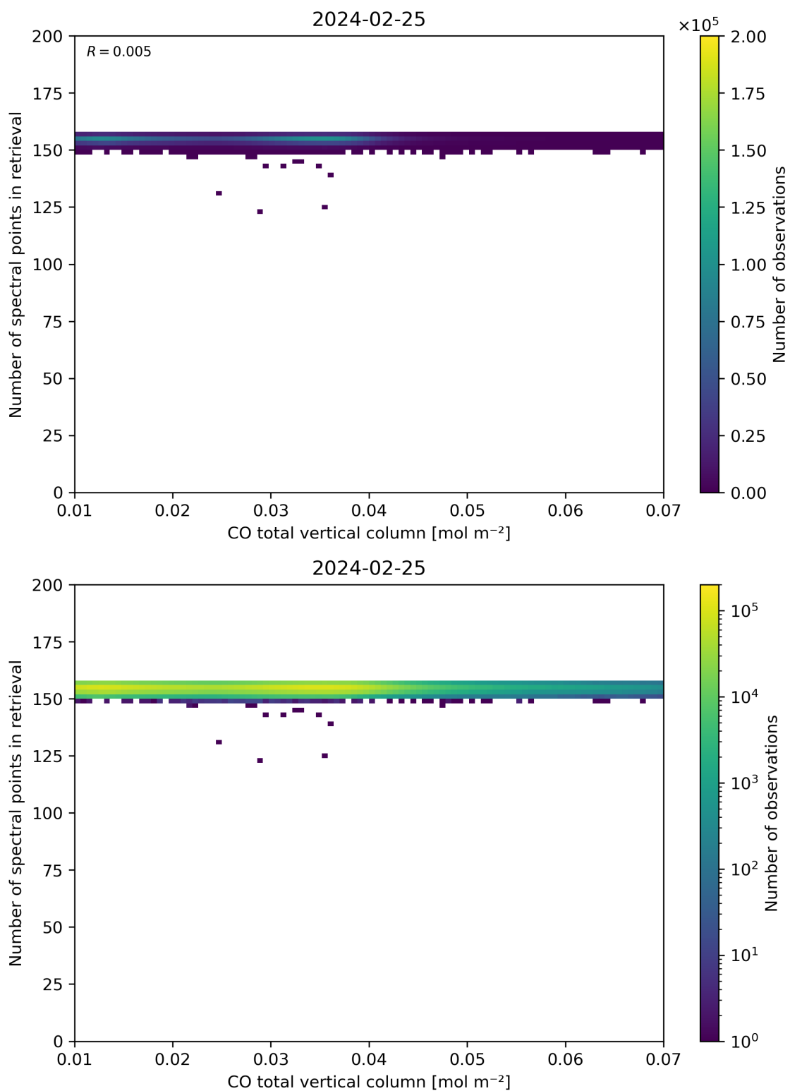
Figure 43: Scatter density plot of “CO total vertical column” against “Number of spectral points in retrieval” for 2024-02-24 to 2024-02-26.
