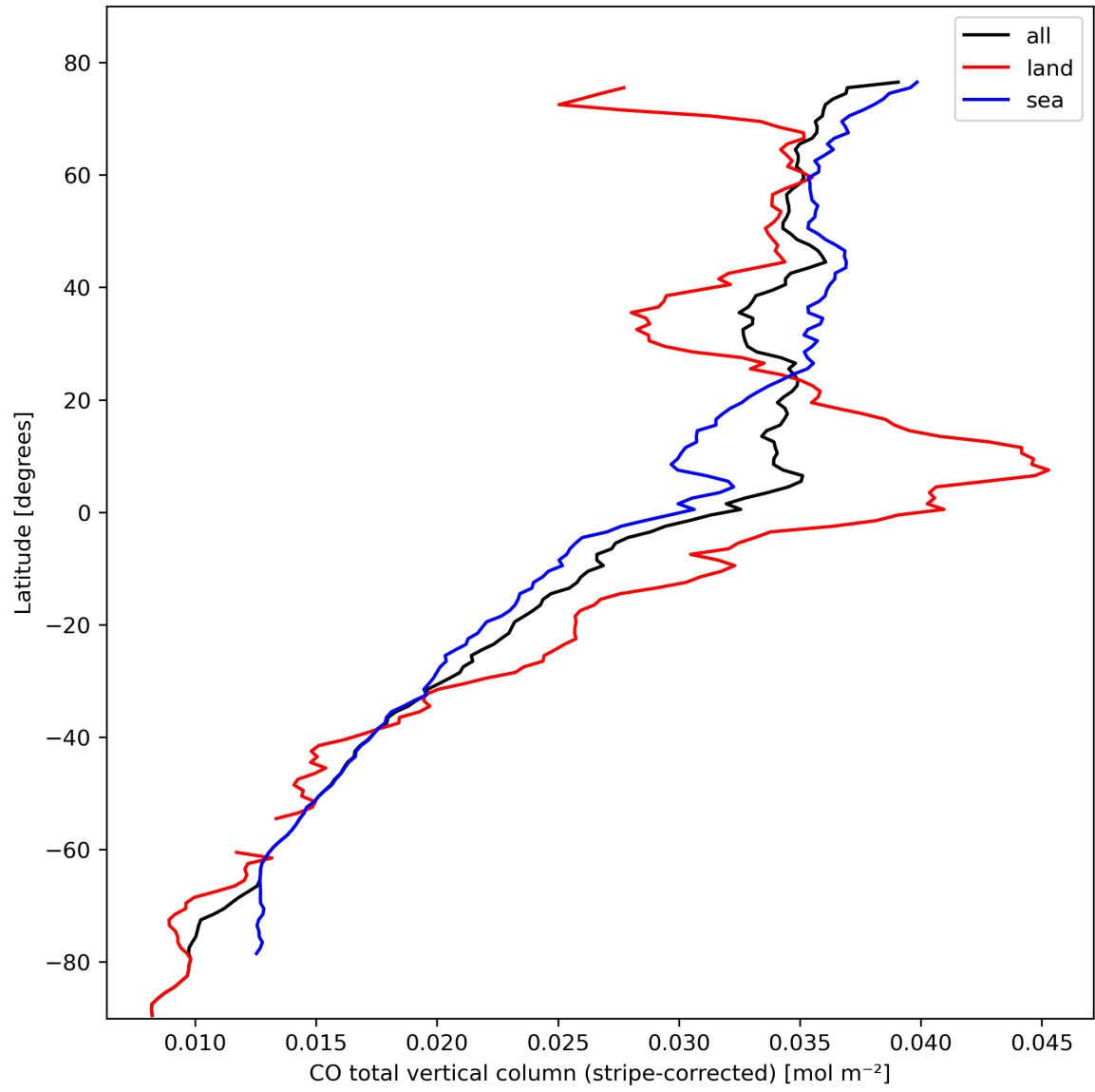
Figure 11: Zonal average of “CO total vertical column (stripe-corrected)” for 2024-02-24 to 2024-02-26.
