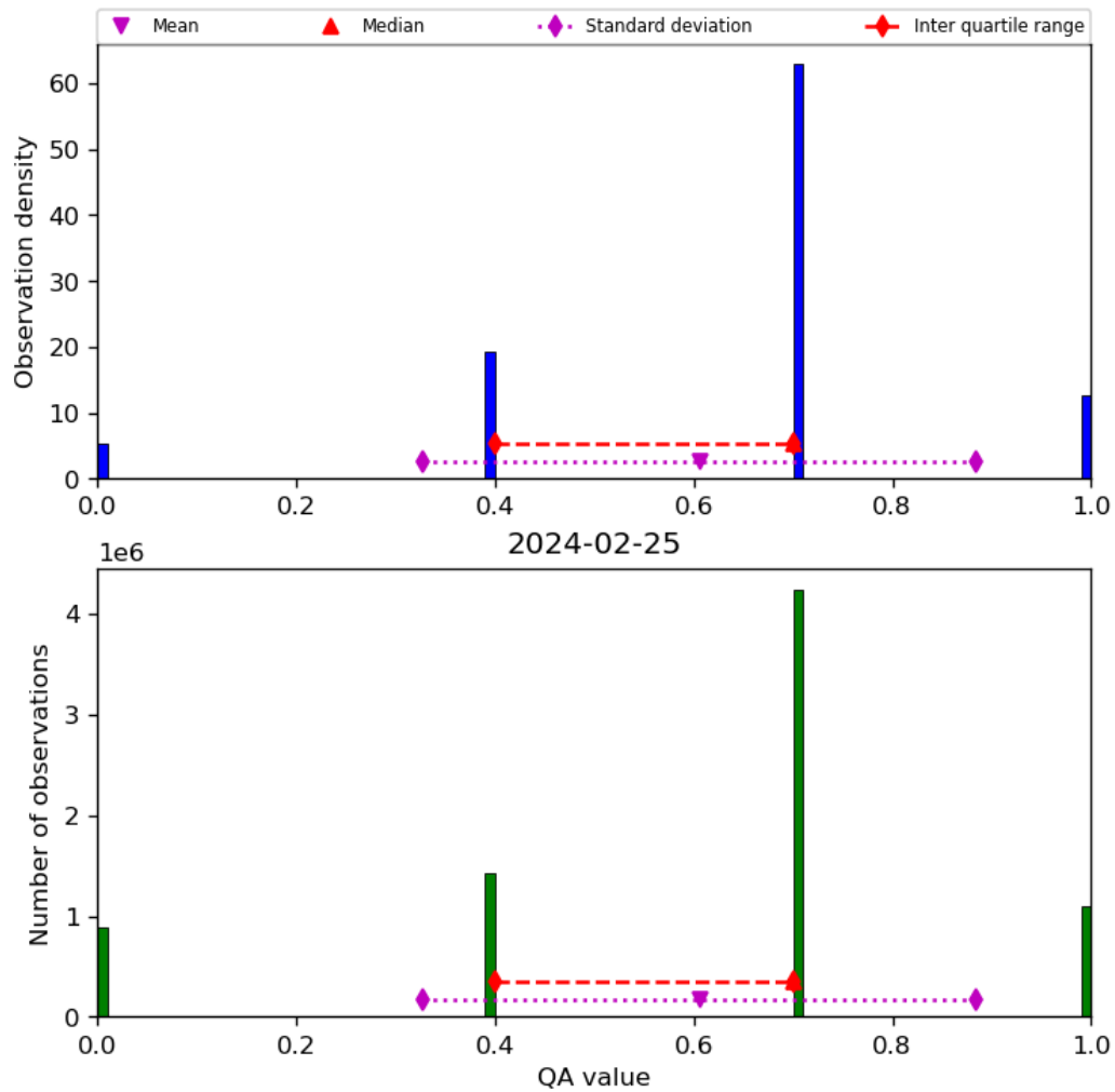
Figure 17: Histogram of “QA value” for 2024-02-24 to 2024-02-26
