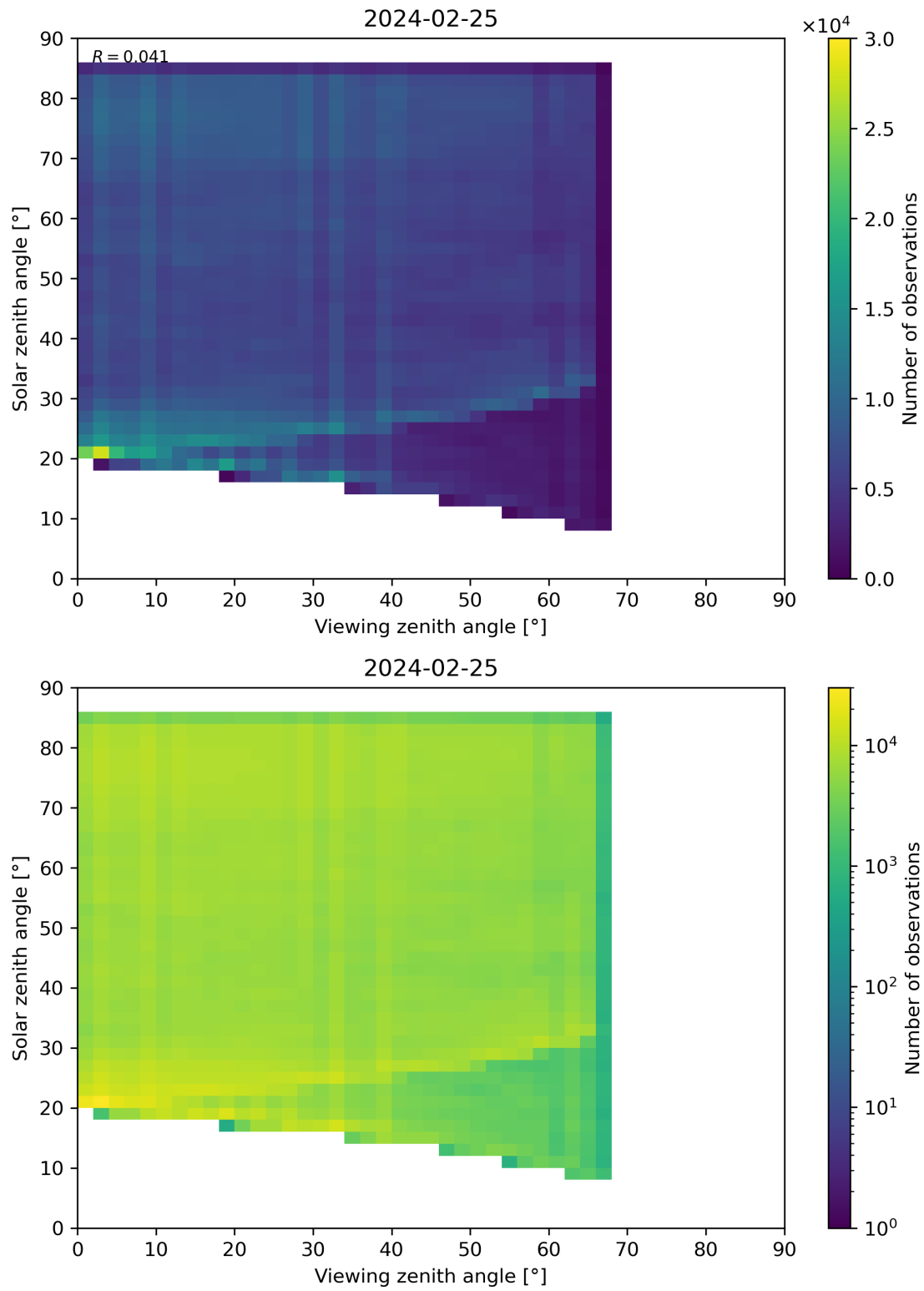
Figure 77: Scatter density plot of “Viewing zenith angle” against “Solar zenith angle” for 2024-02-24 to 2024-02-26.
