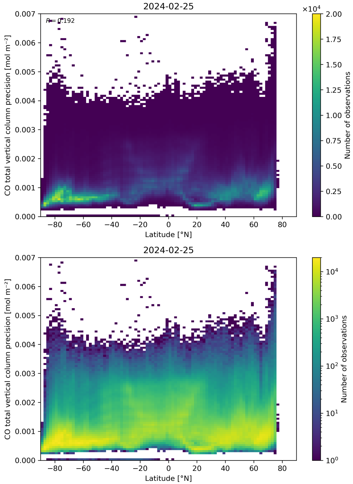
Figure 53: Scatter density plot of “Latitude” against “CO total vertical column precision” for 2024-02-24 to 2024-02-26.
