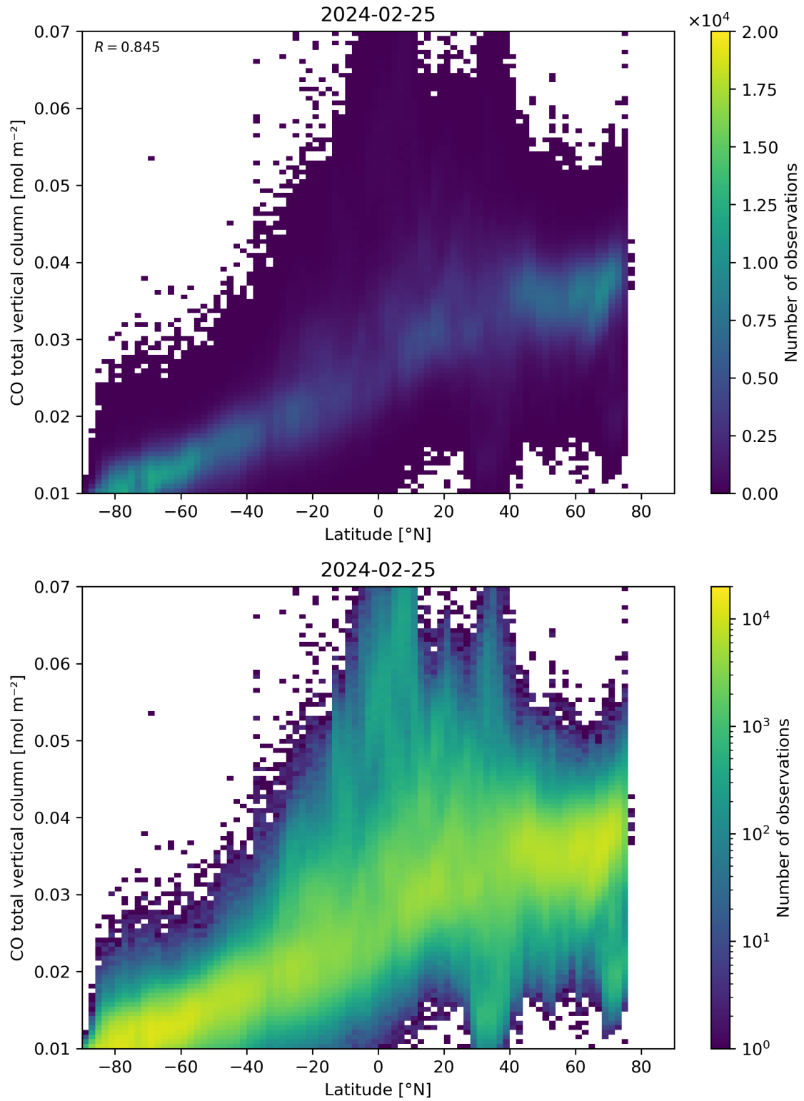
Figure 51: Scatter density plot of “Latitude” against “CO total vertical column” for 2024-02-24 to 2024-02-26.
