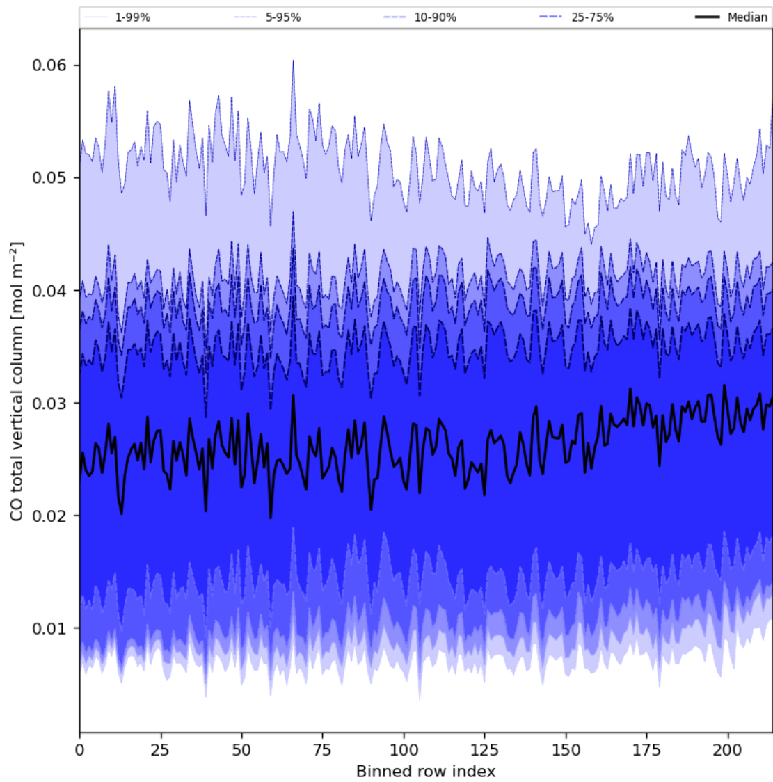
Figure 26: Along track statistics of “CO total vertical column” for 2024-02-24 to 2024-02-26
