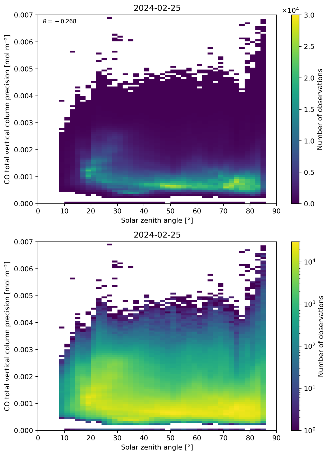
Figure 63: Scatter density plot of “Solar zenith angle” against “CO total vertical column precision” for 2024-02-24 to 2024-02-26.
