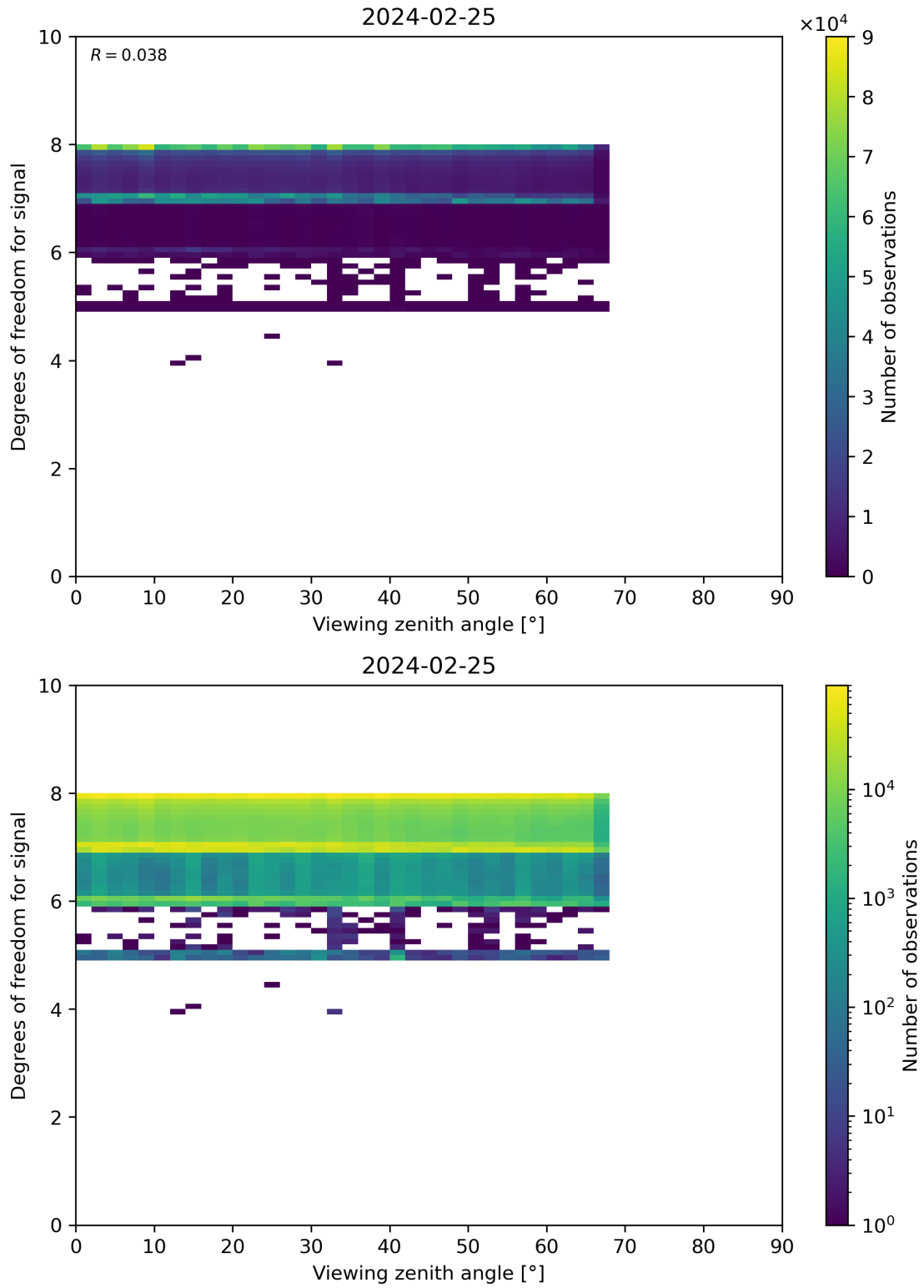
Figure 73: Scatter density plot of “Viewing zenith angle” against “Degrees of freedom for signal” for 2024-02-24 to 2024-02-26.
