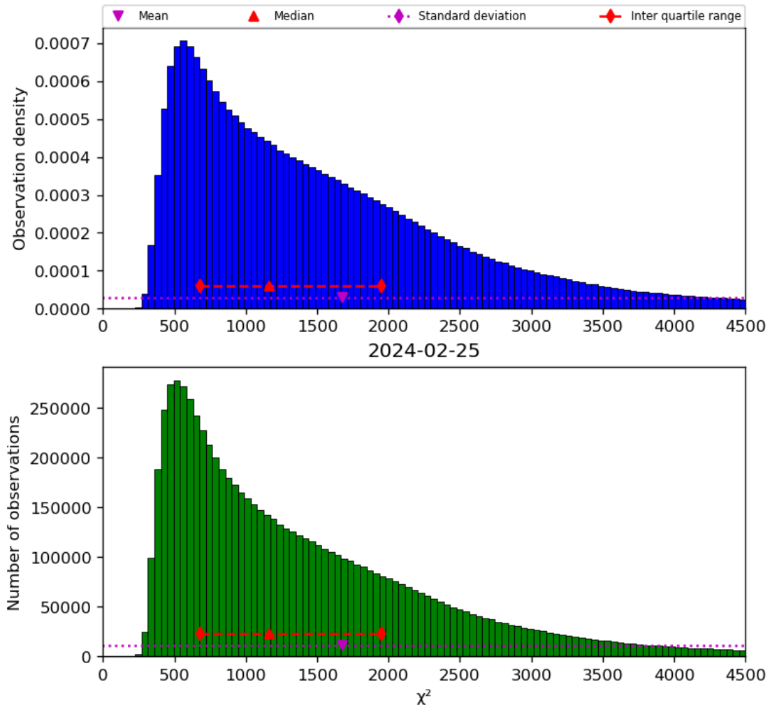
Figure 22: Histogram of “ \chi^2 ” for 2024-02-24 to 2024-02-26
