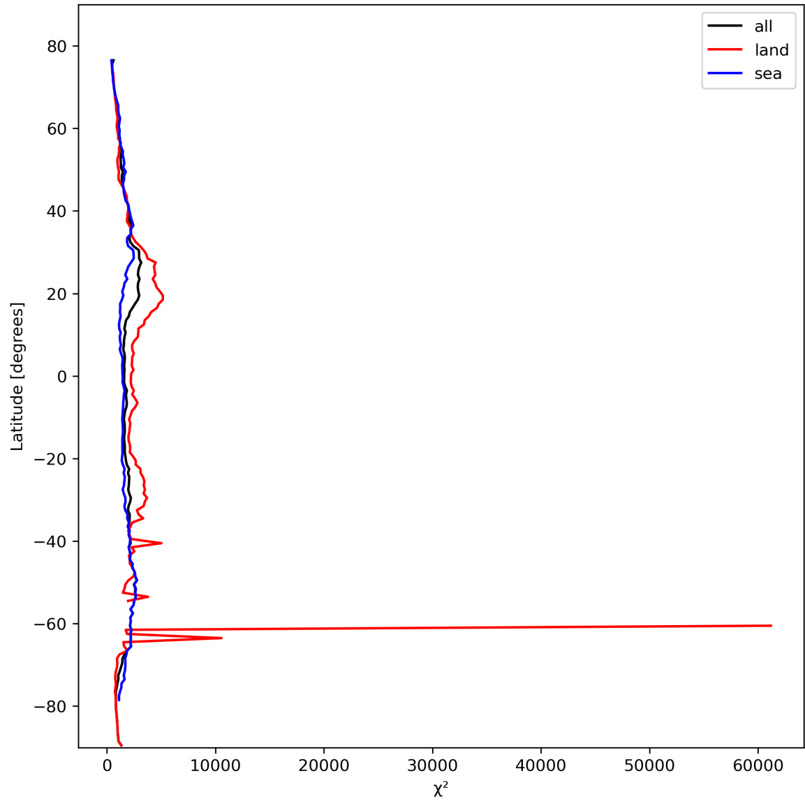
Figure 14: Zonal average of “ \chi^2 ” for 2024-02-24 to 2024-02-26.
