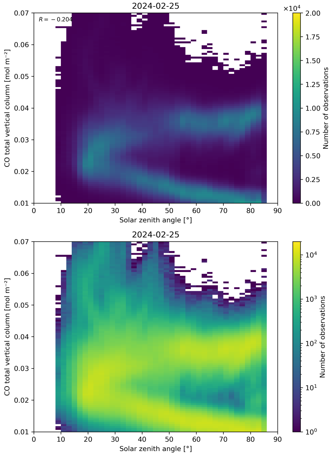
Figure 61: Scatter density plot of “Solar zenith angle” against “CO total vertical column” for 2024-02-24 to 2024-02-26.
