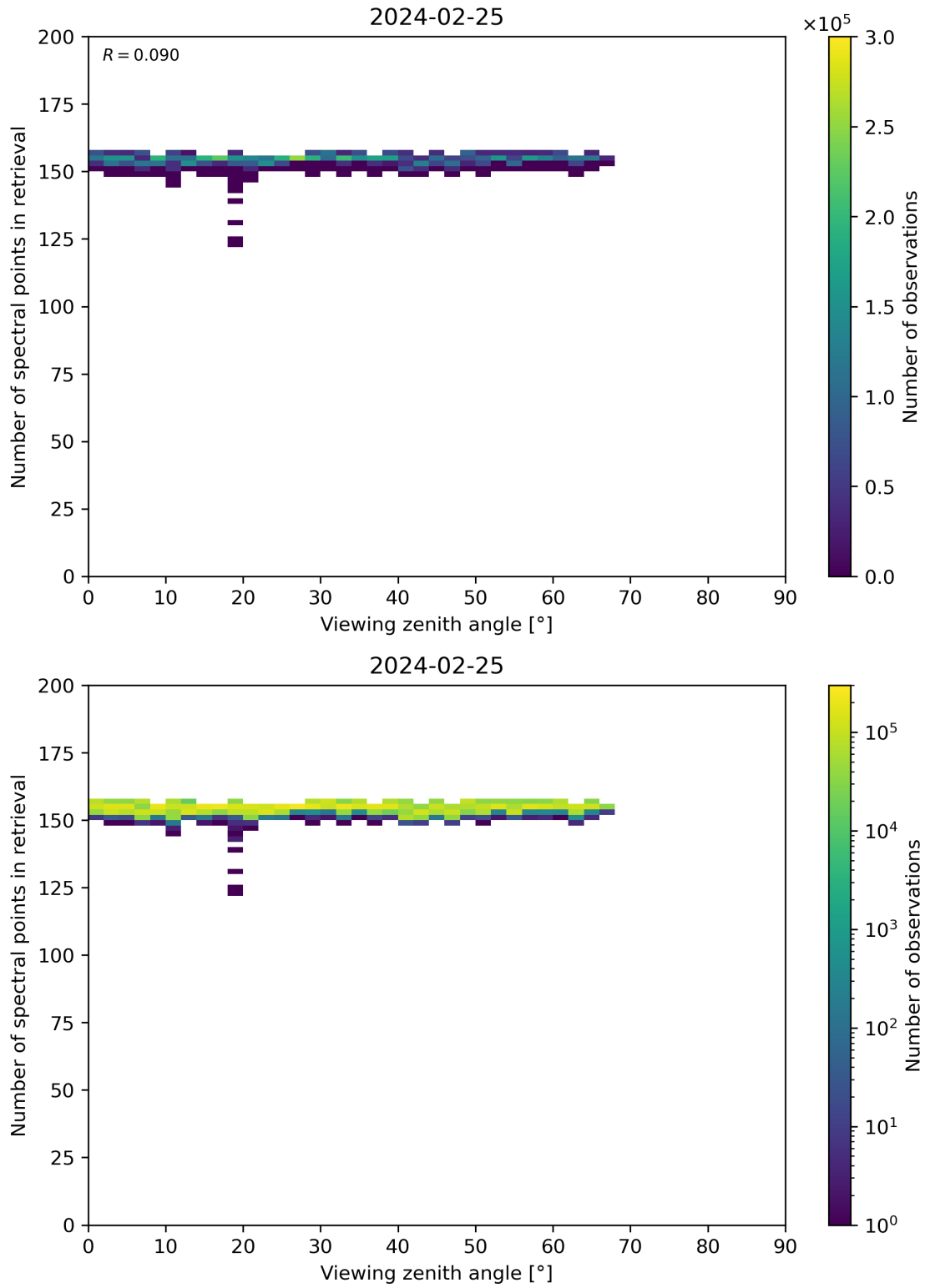
Figure 76: Scatter density plot of “Viewing zenith angle” against “Number of spectral points in retrieval” for 2024-02-24 to 2024-02-26.
