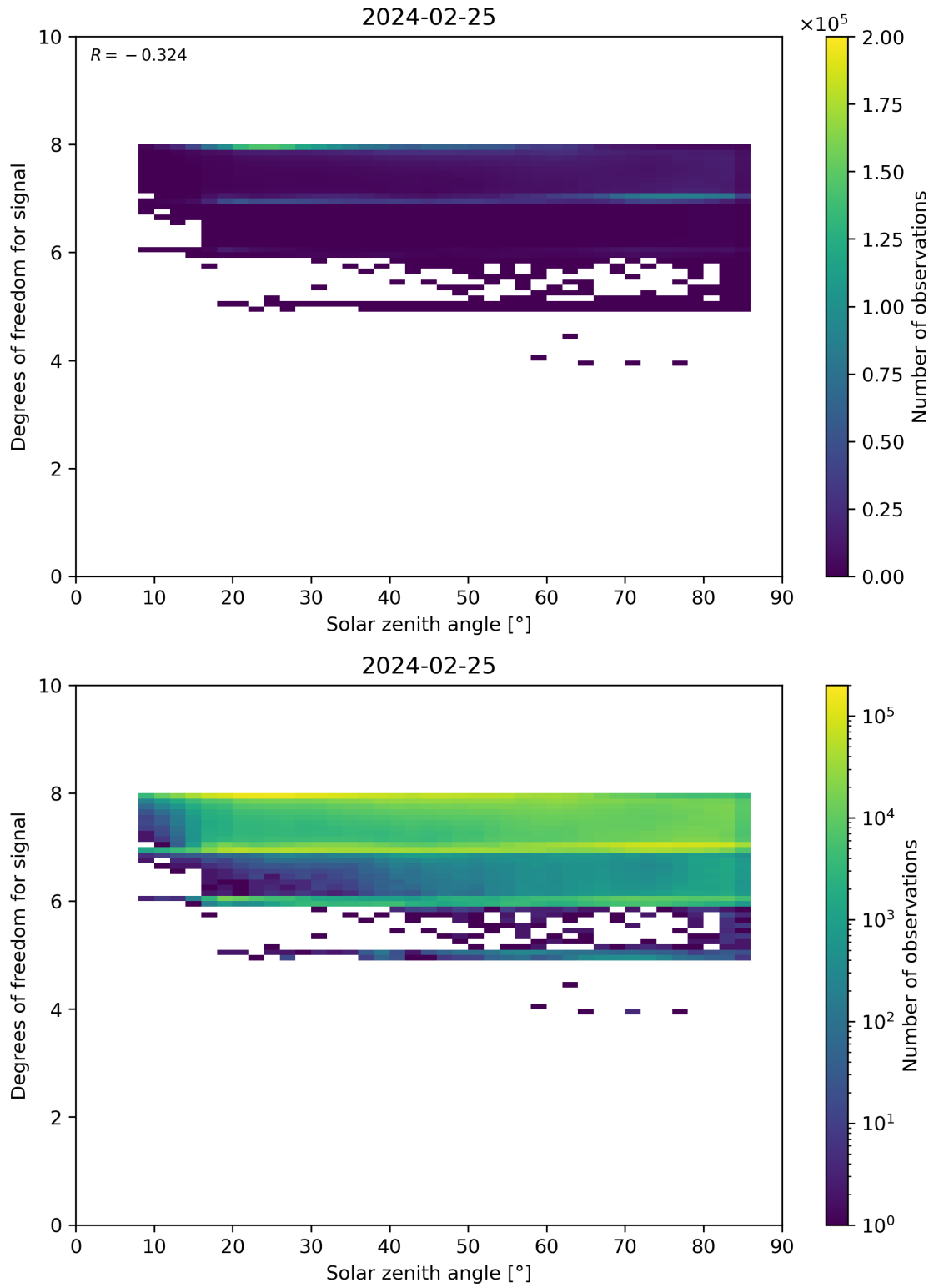
Figure 65: Scatter density plot of “Solar zenith angle” against “Degrees of freedom for signal” for 2024-02-24 to 2024-02-26.
