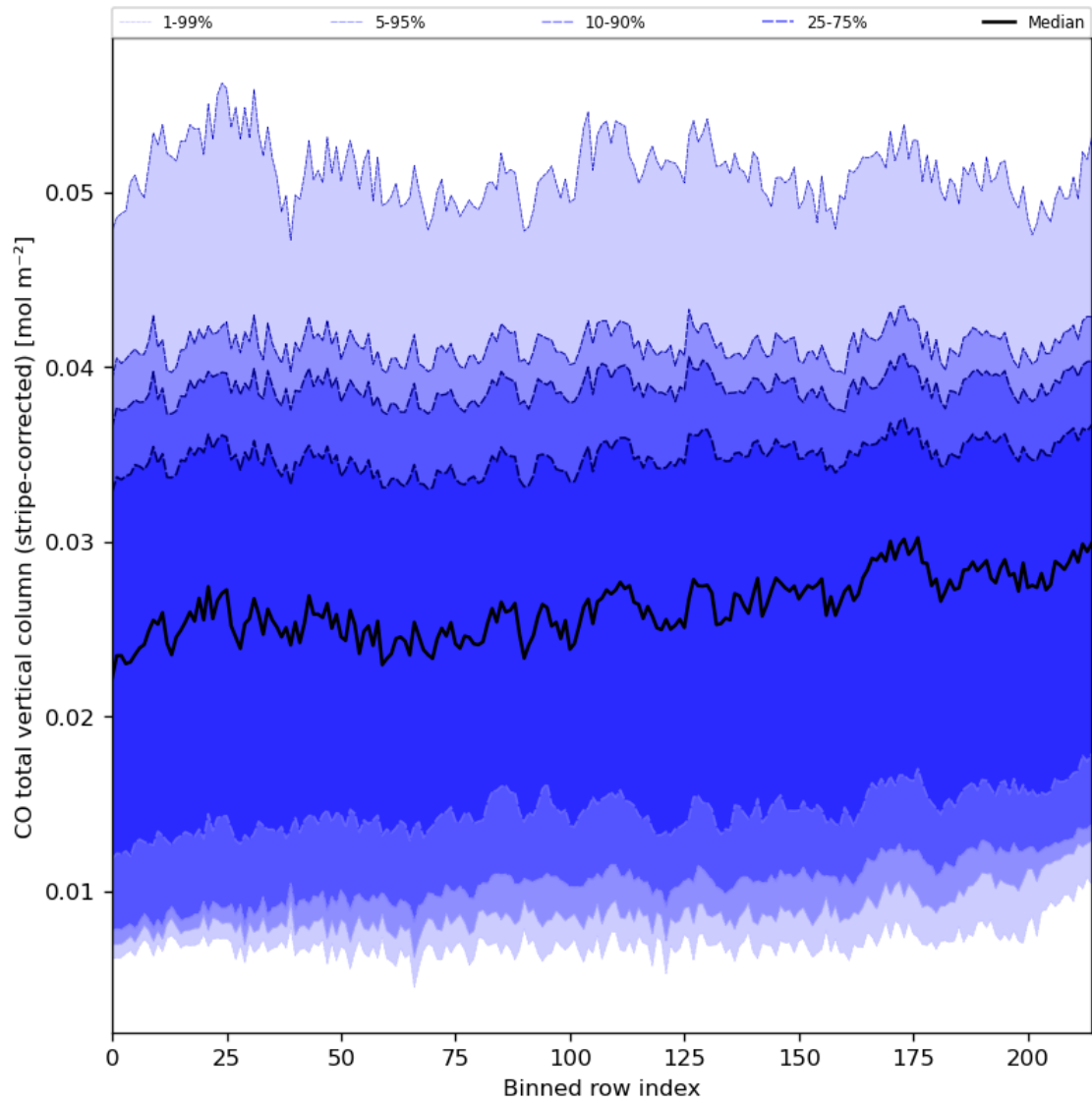
Figure 27: Along track statistics of “CO total vertical column (stripe-corrected)” for 2024-02-25 to 2024-02-27
