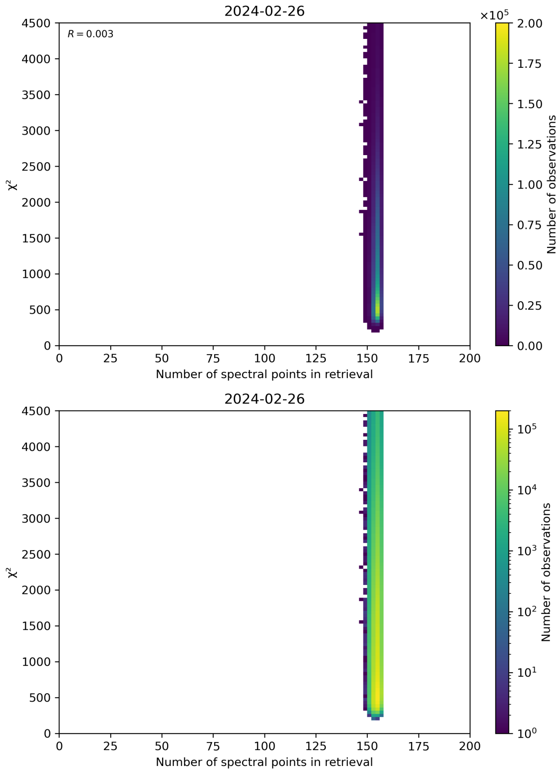
Figure 58: Scatter density plot of “Number of spectral points in retrieval” against “ \chi^2 ” for 2024-02-25 to 2024-02-27.
