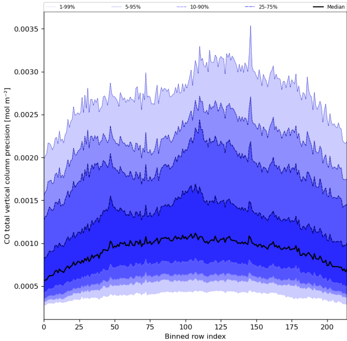
Figure 28: Along track statistics of “CO total vertical column precision” for 2024-02-25 to 2024-02-27
