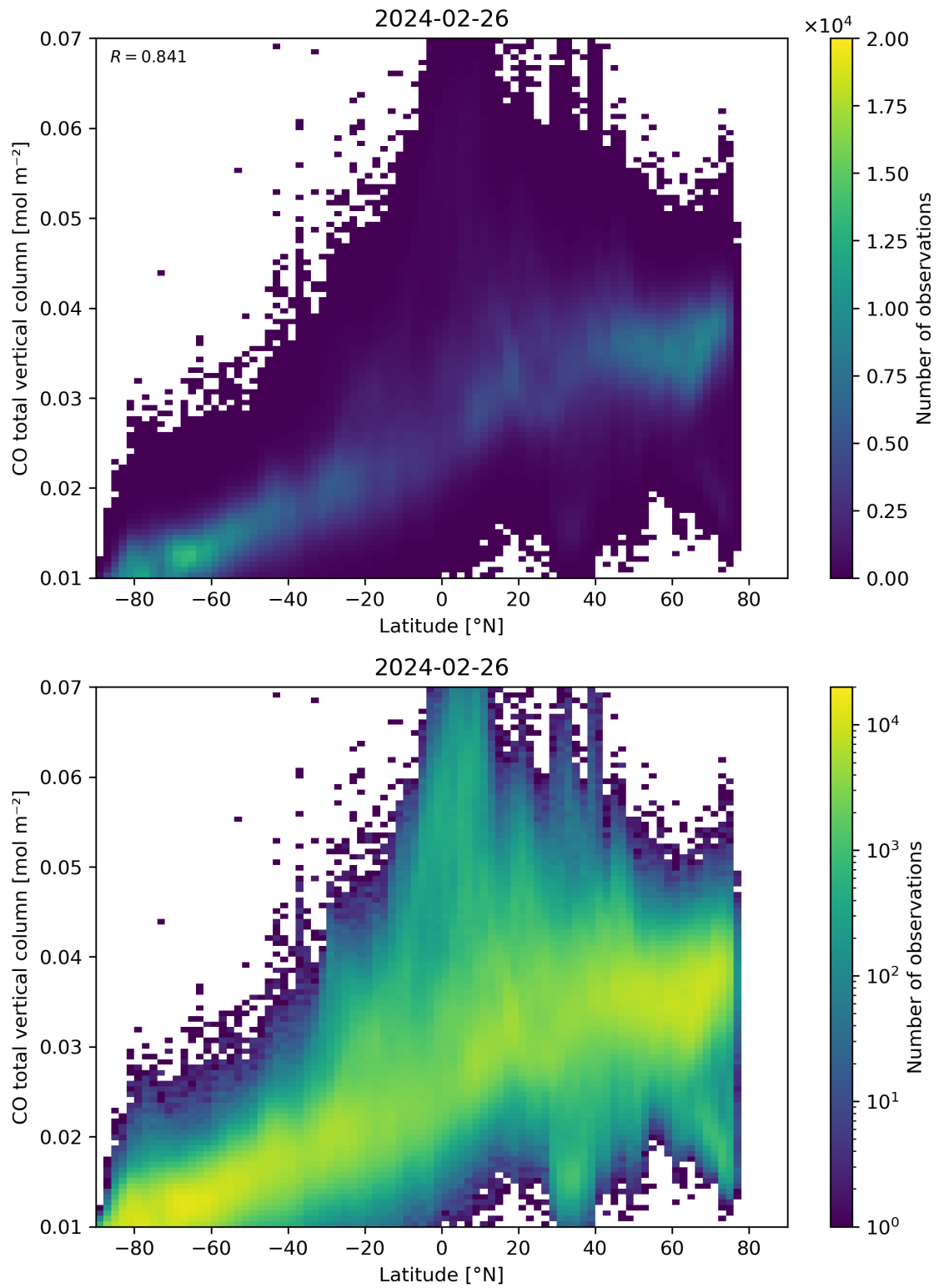
Figure 51: Scatter density plot of “Latitude” against “CO total vertical column” for 2024-02-25 to 2024-02-27.
