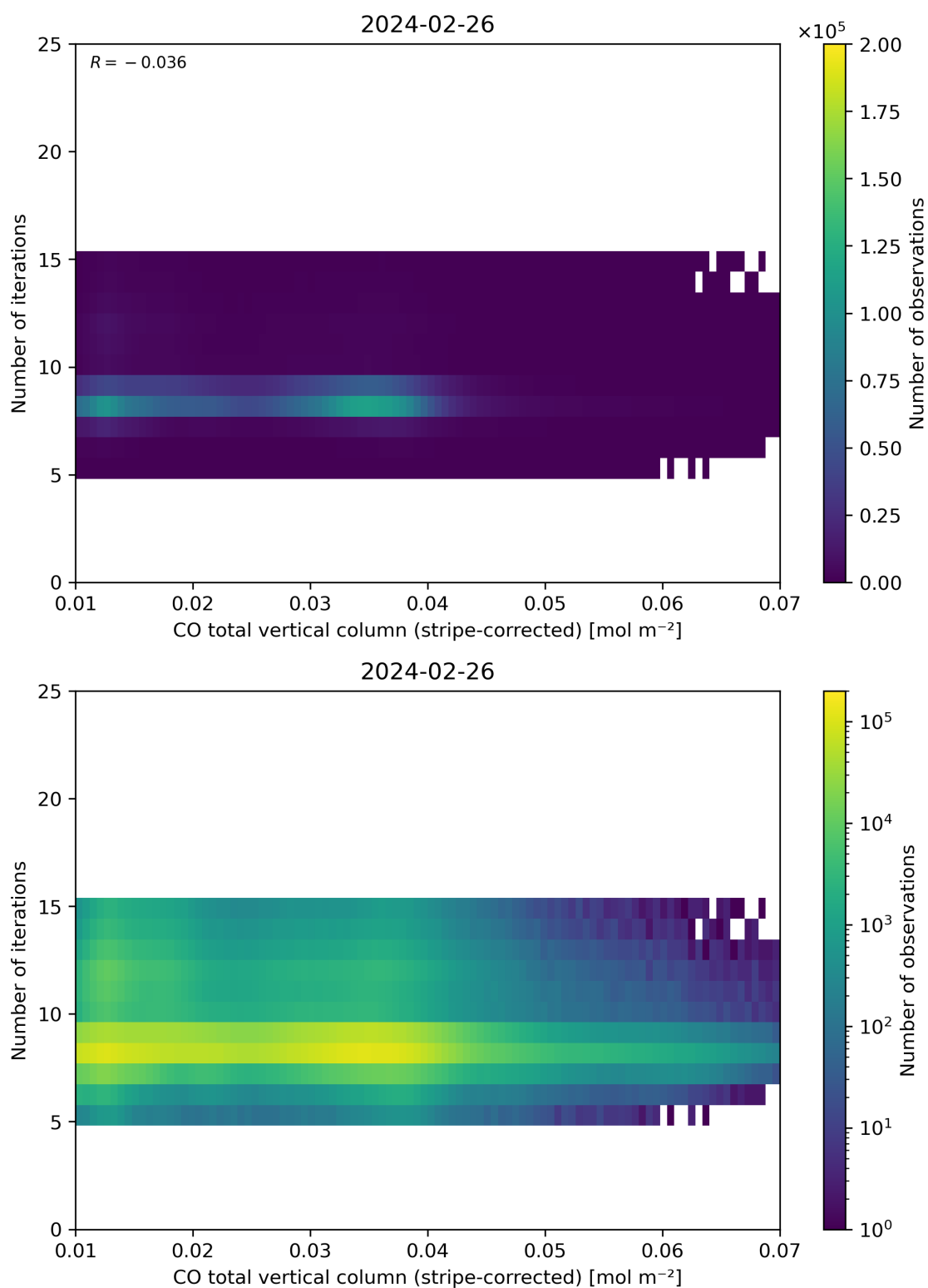
Figure 39: Scatter density plot of “CO total vertical column (stripe-corrected)” against “Number of iterations” for 2024-02-25 to 2024-02-27.
