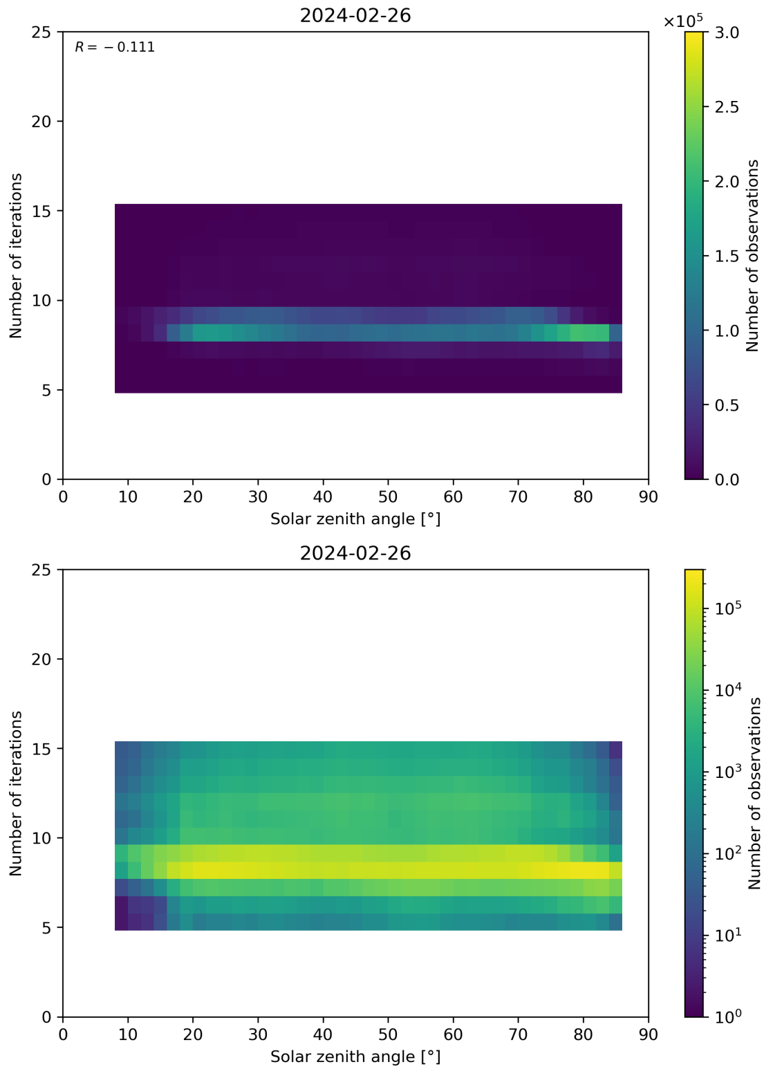
Figure 67: Scatter density plot of “Solar zenith angle” against “Number of iterations” for 2024-02-25 to 2024-02-27.
