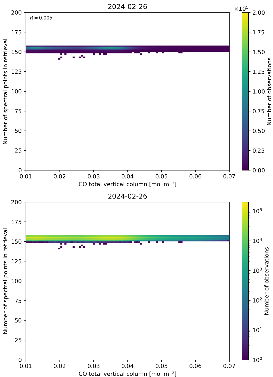
Figure 43: Scatter density plot of “CO total vertical column” against “Number of spectral points in retrieval” for 2024-02-25 to 2024-02-27.
