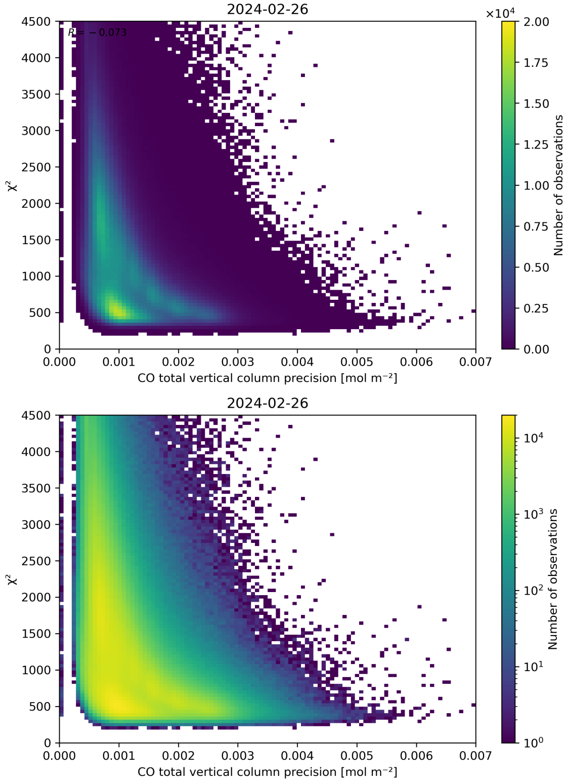
Figure 44: Scatter density plot of “CO total vertical column precision” against “ \chi^2 ” for 2024-02-25 to 2024-02-27.
