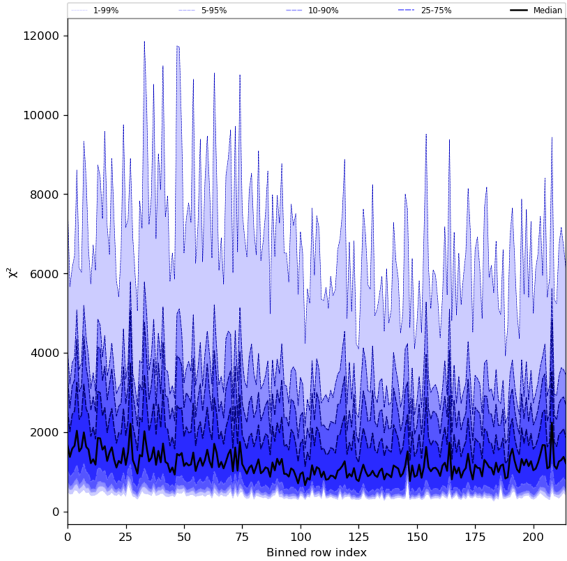
Figure 30: Along track statistics of “ \chi^2 ” for 2024-02-25 to 2024-02-27
