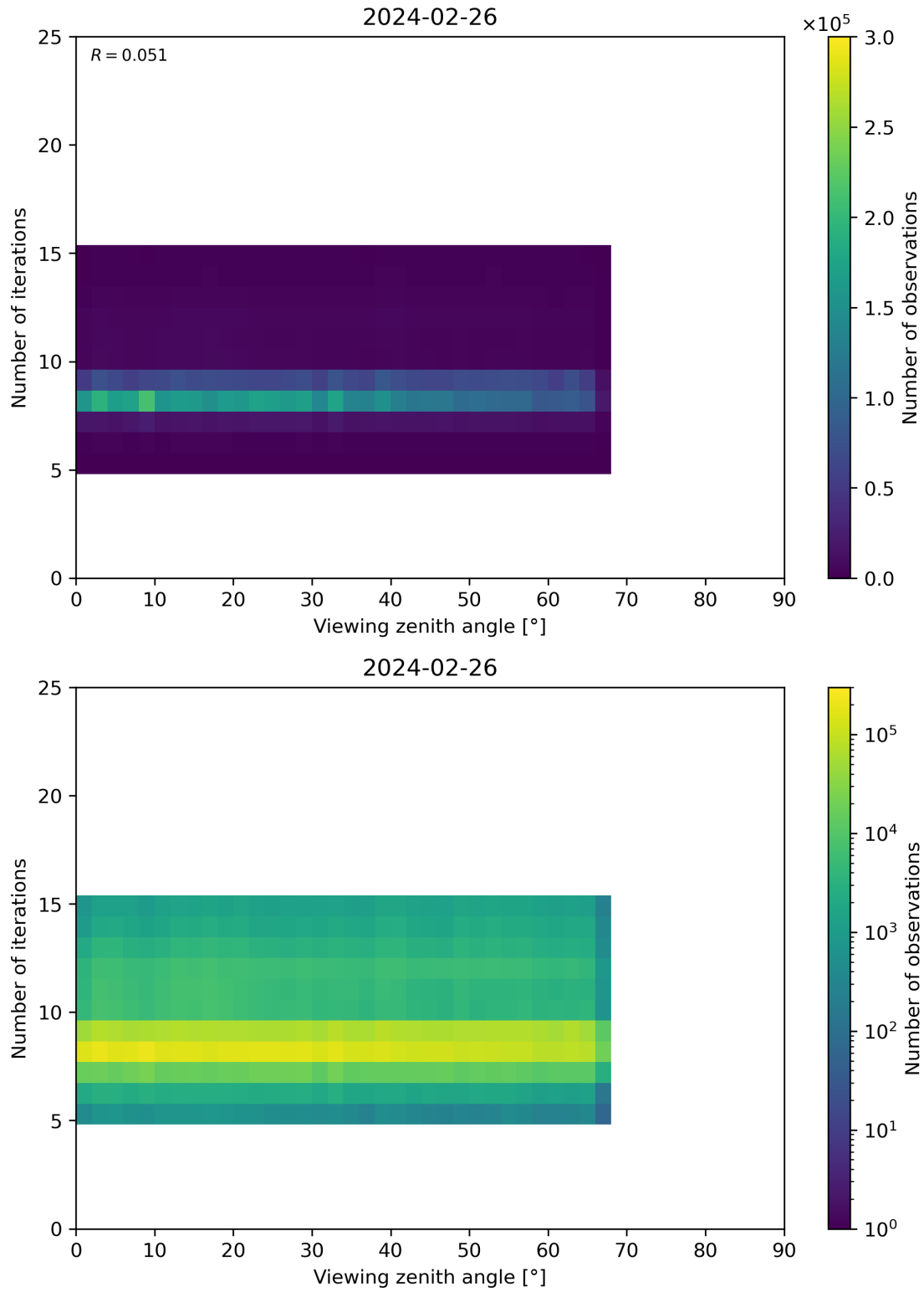
Figure 75: Scatter density plot of “Viewing zenith angle” against “Number of iterations” for 2024-02-25 to 2024-02-27.
