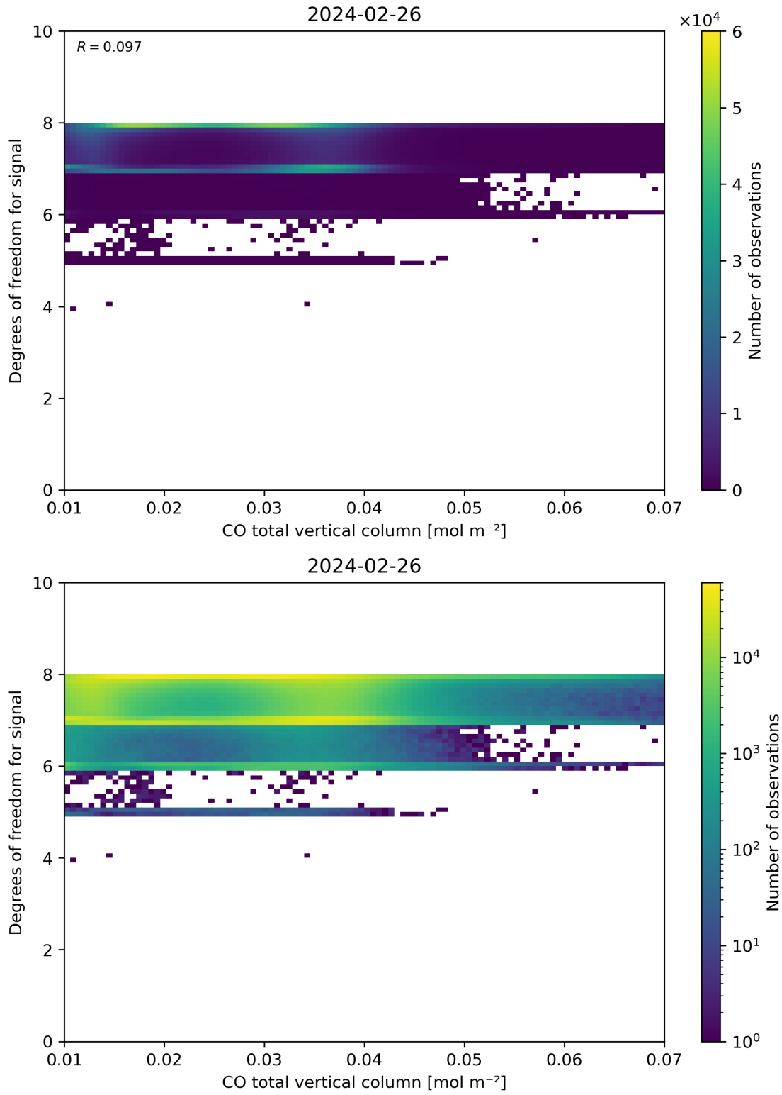
Figure 41: Scatter density plot of “CO total vertical column” against “Degrees of freedom for signal” for 2024-02-25 to 2024-02-27.
