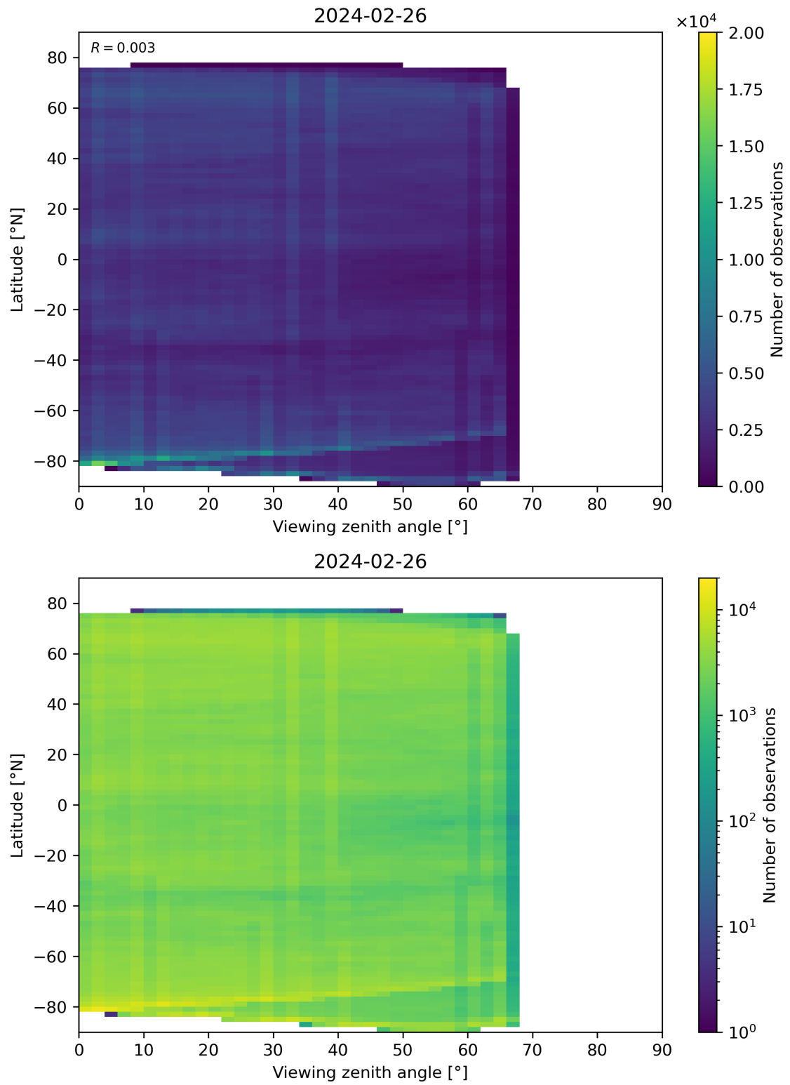
Figure 74: Scatter density plot of “Viewing zenith angle” against “Latitude” for 2024-02-25 to 2024-02-27.
