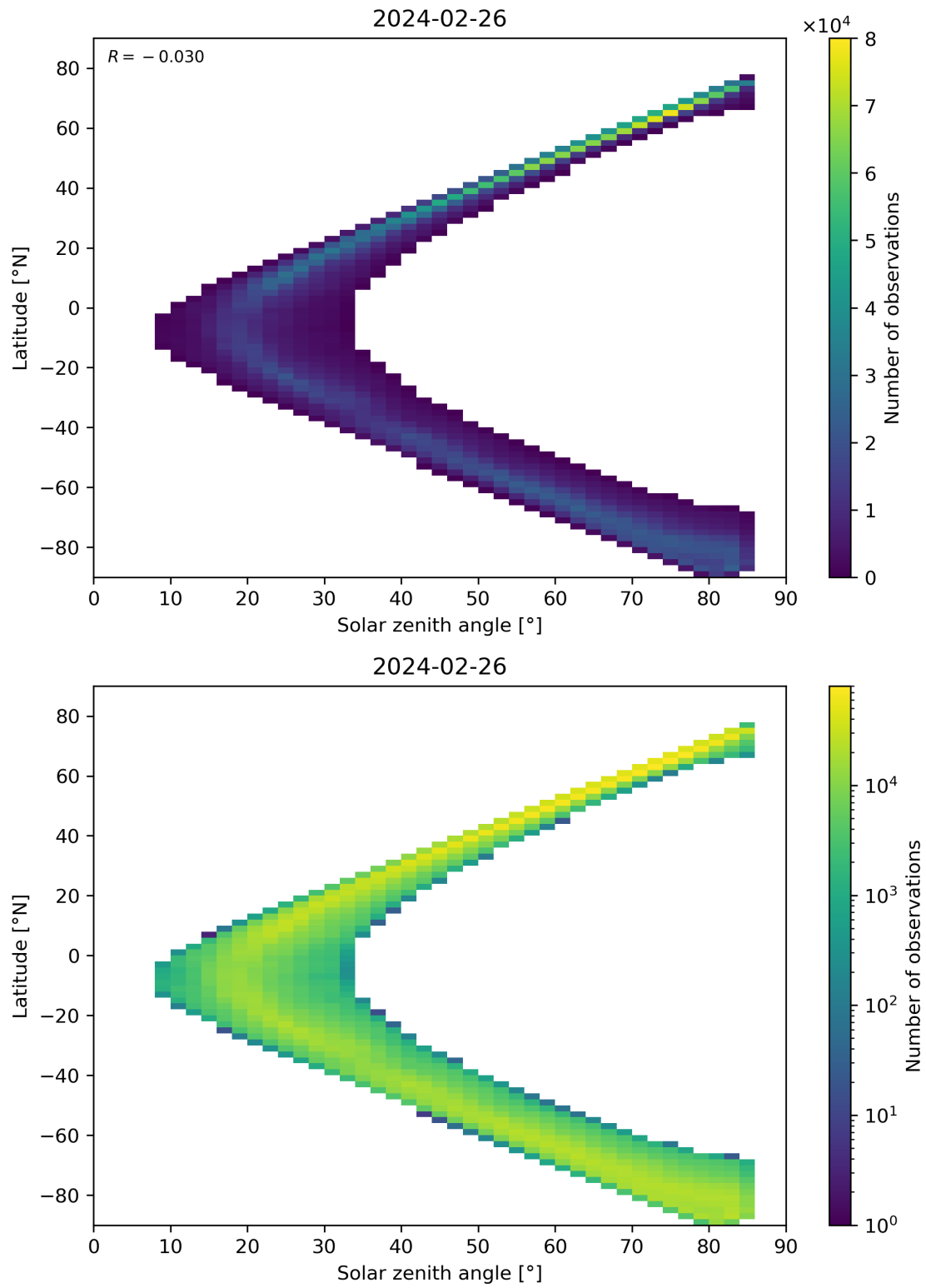
Figure 66: Scatter density plot of “Solar zenith angle” against “Latitude” for 2024-02-25 to 2024-02-27.
