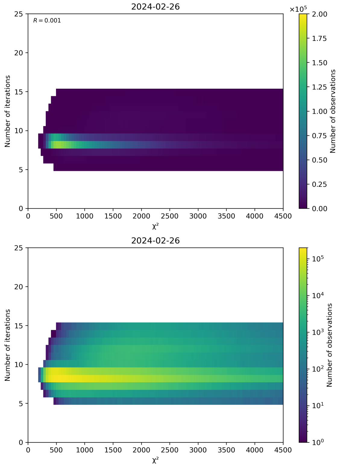
Figure 49: Scatter density plot of “ \chi^2 ” against “Number of iterations” for 2024-02-25 to 2024-02-27.
