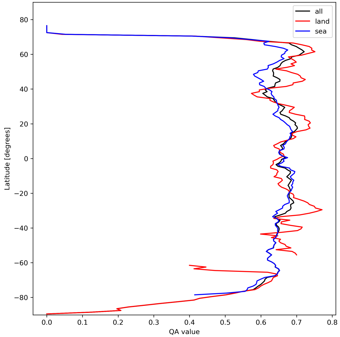
Figure 9: Zonal average of “QA value” for 2024-02-25 to 2024-02-27.
