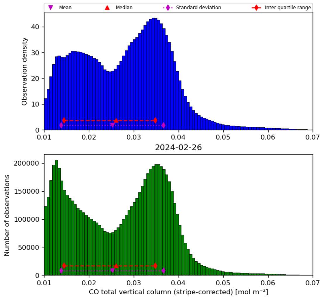
Figure 19: Histogram of “CO total vertical column (stripe-corrected)” for 2024-02-25 to 2024-02-27
