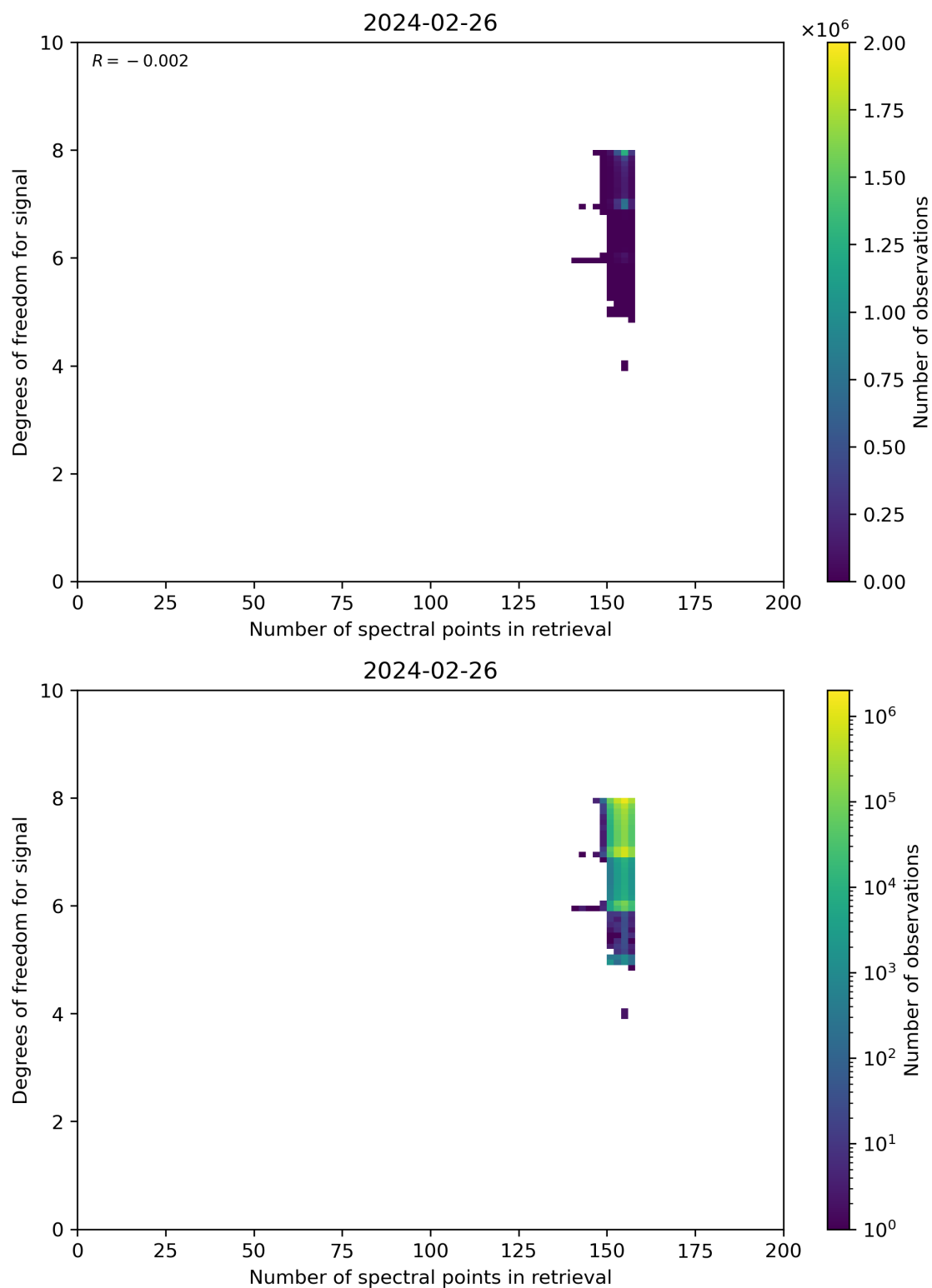
Figure 59: Scatter density plot of “Number of spectral points in retrieval” against “Degrees of freedom for signal” for 2024-02-25 to 2024-02-27.
