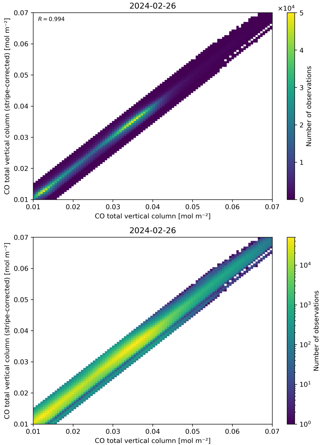
Figure 33: Scatter density plot of “CO total vertical column” against “CO total vertical column (stripe-corrected)” for 2024-02-25 to 2024-02-27.
