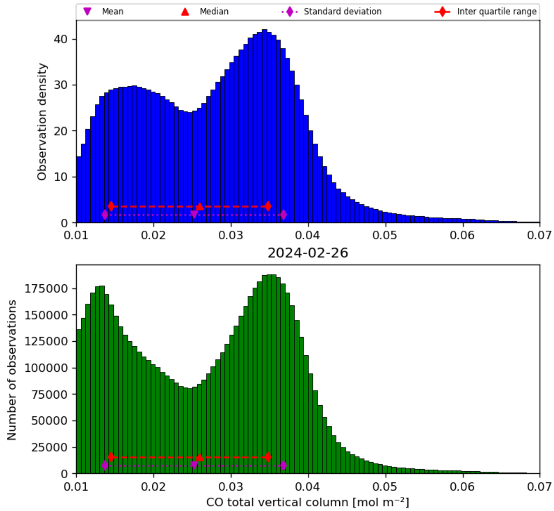
Figure 18: Histogram of “CO total vertical column” for 2024-02-25 to 2024-02-27
