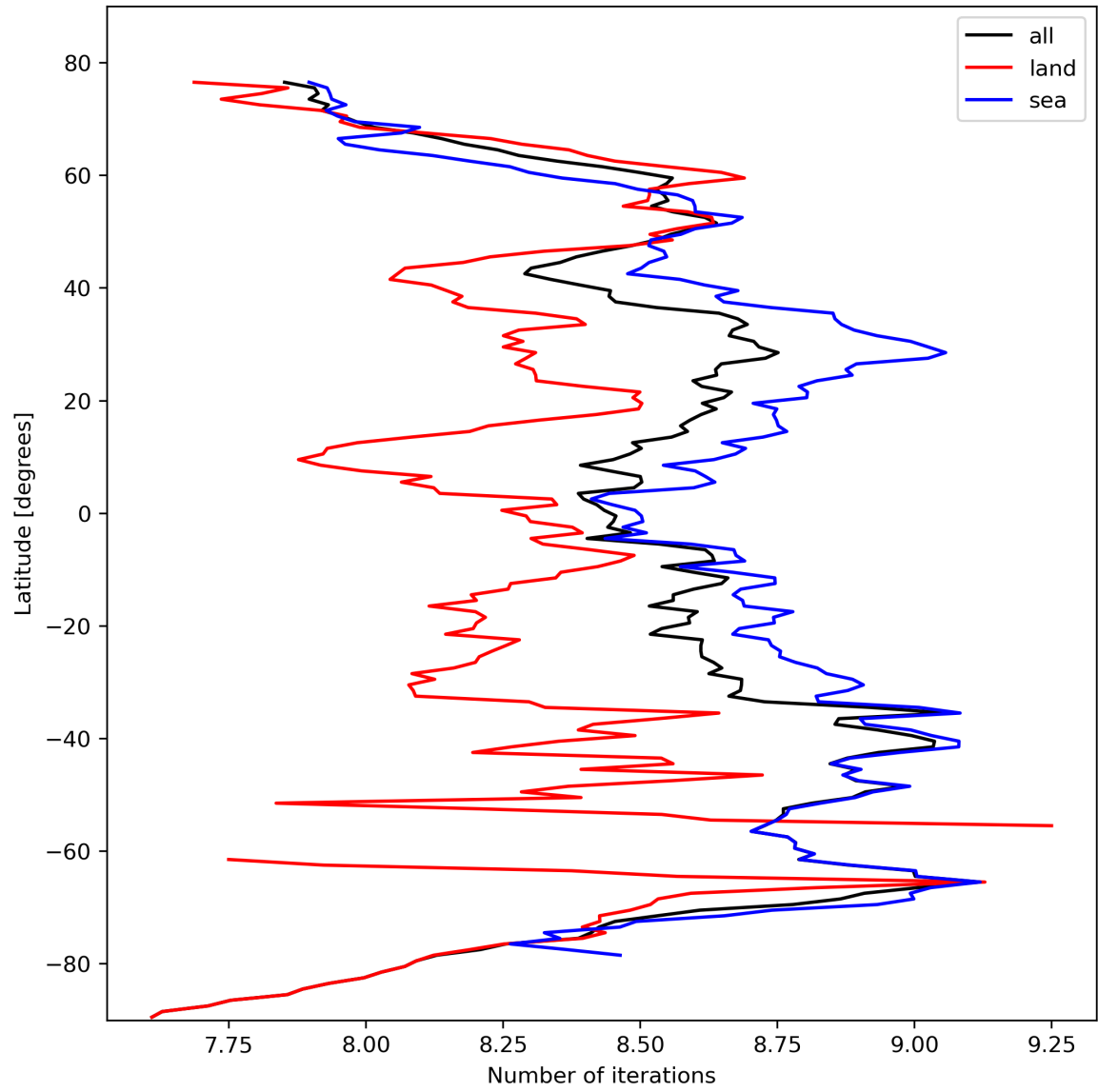
Figure 16: Zonal average of “Number of iterations” for 2024-02-25 to 2024-02-27.
