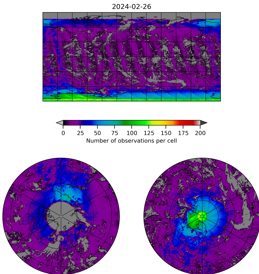
Figure 8: Map of the number of observations for 2024-02-25 to 2024-02-27
