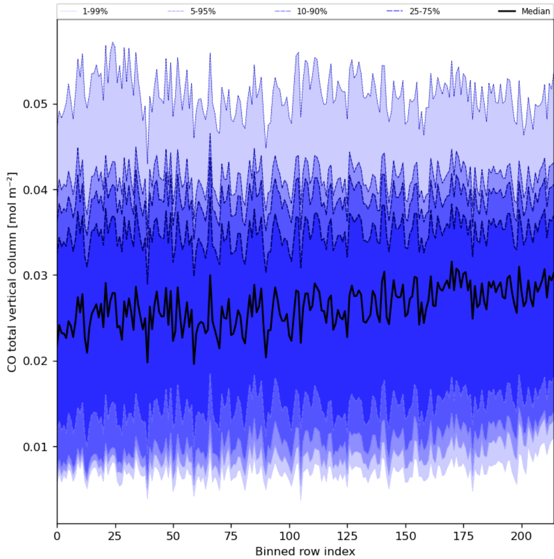
Figure 26: Along track statistics of "CO total vertical column" for 2024-02-25 to 2024-02-27
