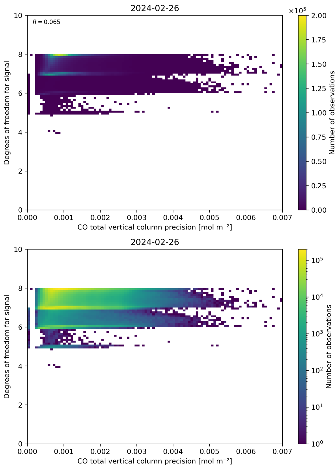
Figure 45: Scatter density plot of “CO total vertical column precision” against “Degrees of freedom for signal” for 2024-02-25 to 2024-02-27.
