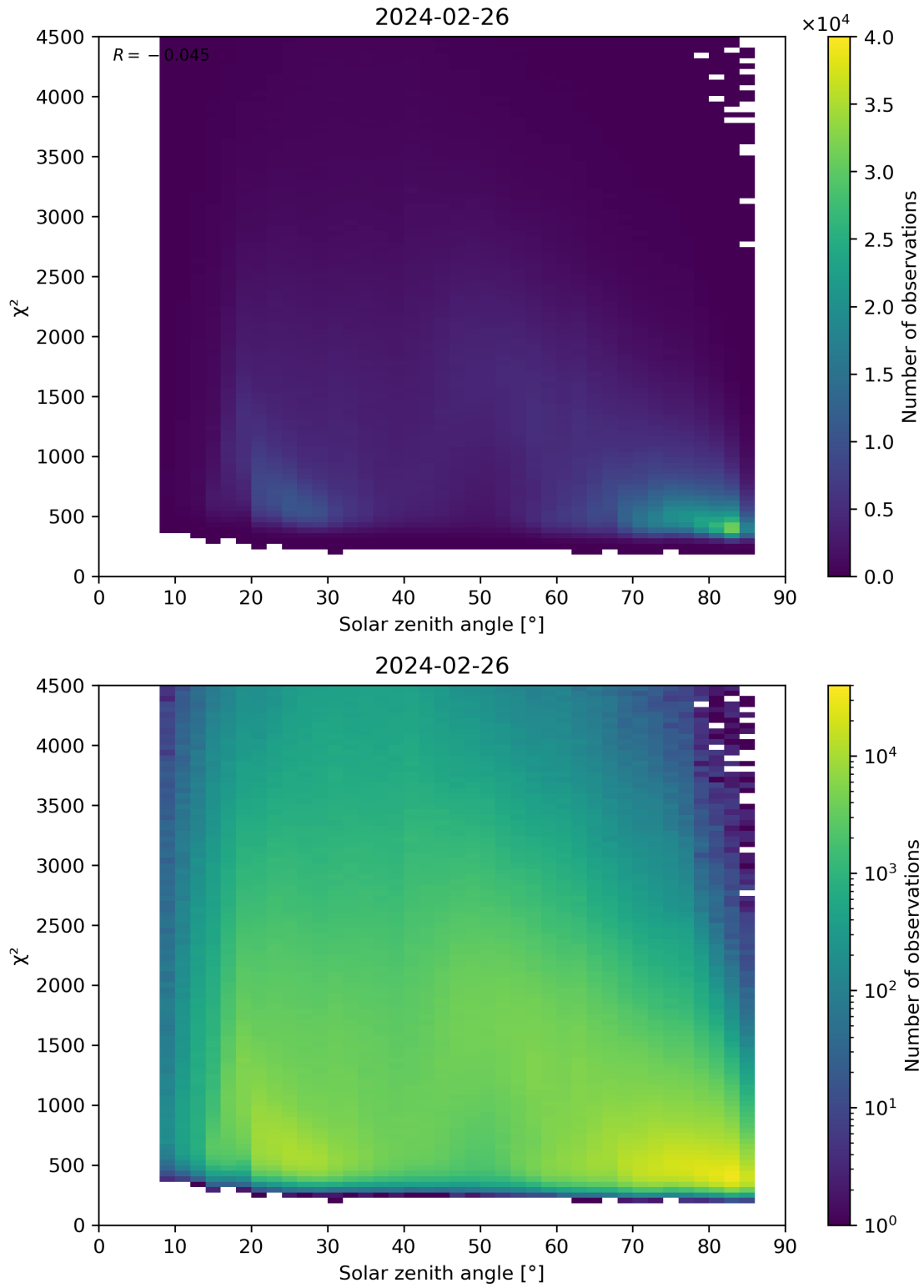
Figure 64: Scatter density plot of “Solar zenith angle” against “ \chi^2 ” for 2024-02-25 to 2024-02-27.
