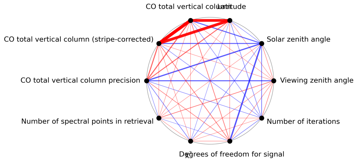
Figure 1: Map of correlation graph for 2024-02-25 to 2024-02-27.
