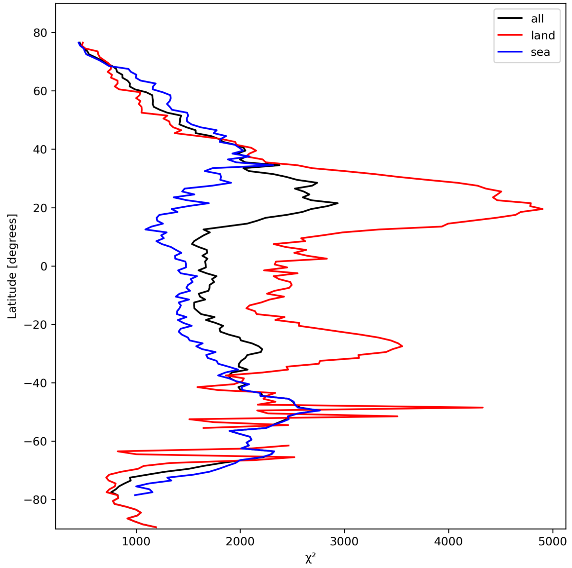
Figure 14: Zonal average of “ \chi^2 ” for 2024-02-25 to 2024-02-27.
