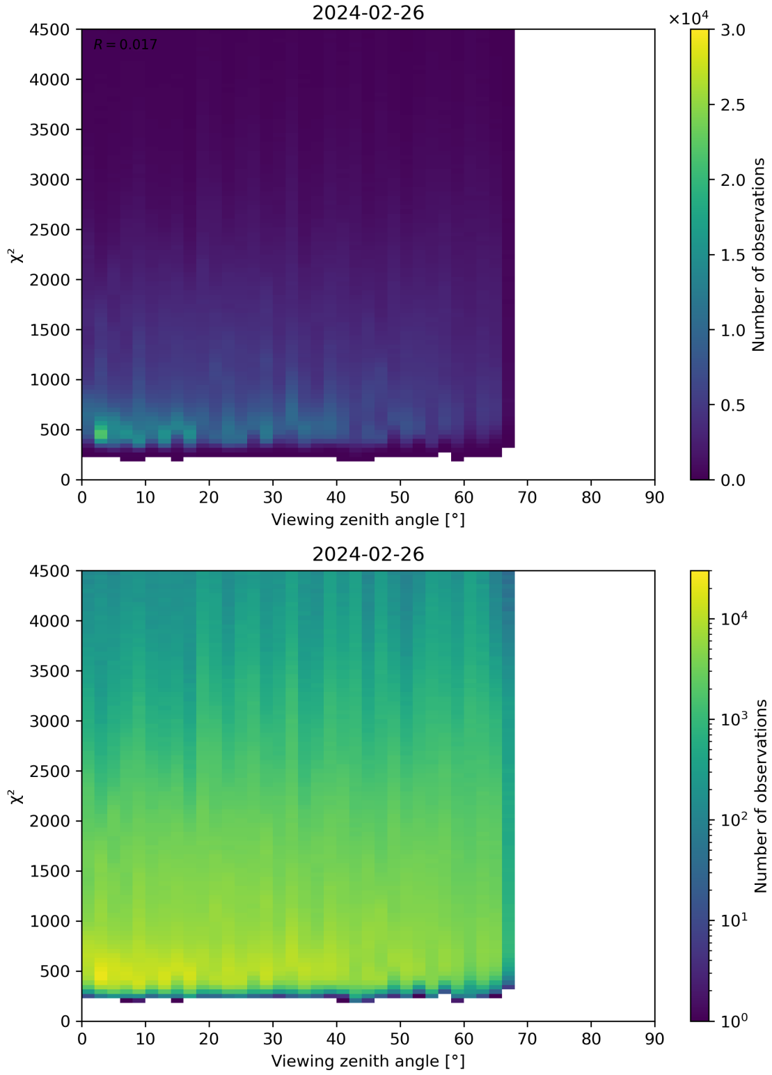
Figure 72: Scatter density plot of “Viewing zenith angle” against “ \chi^2 ” for 2024-02-25 to 2024-02-27.
