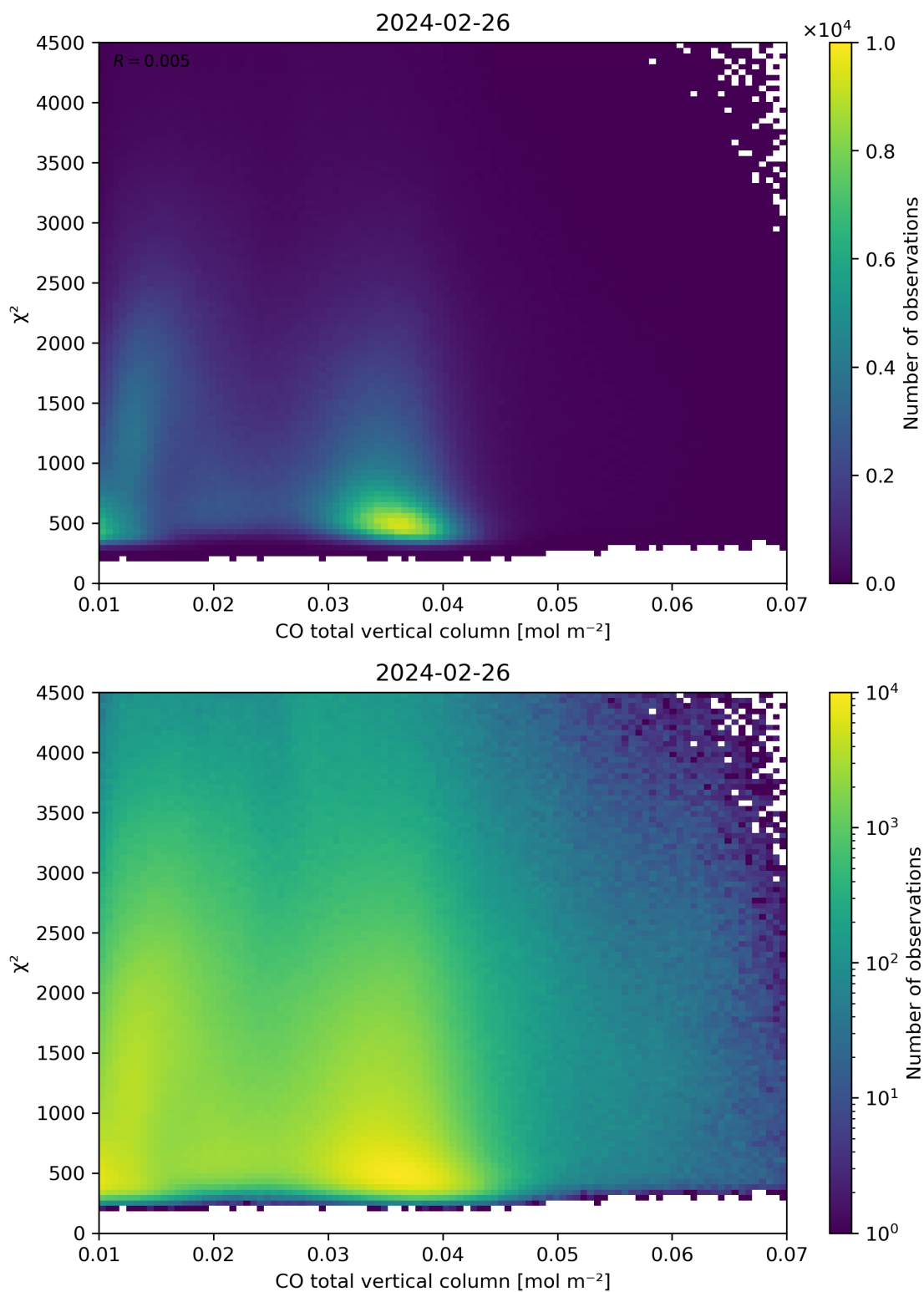
Figure 35: Scatter density plot of “CO total vertical column” against “ \chi^2 ” for 2024-02-25 to 2024-02-27.
