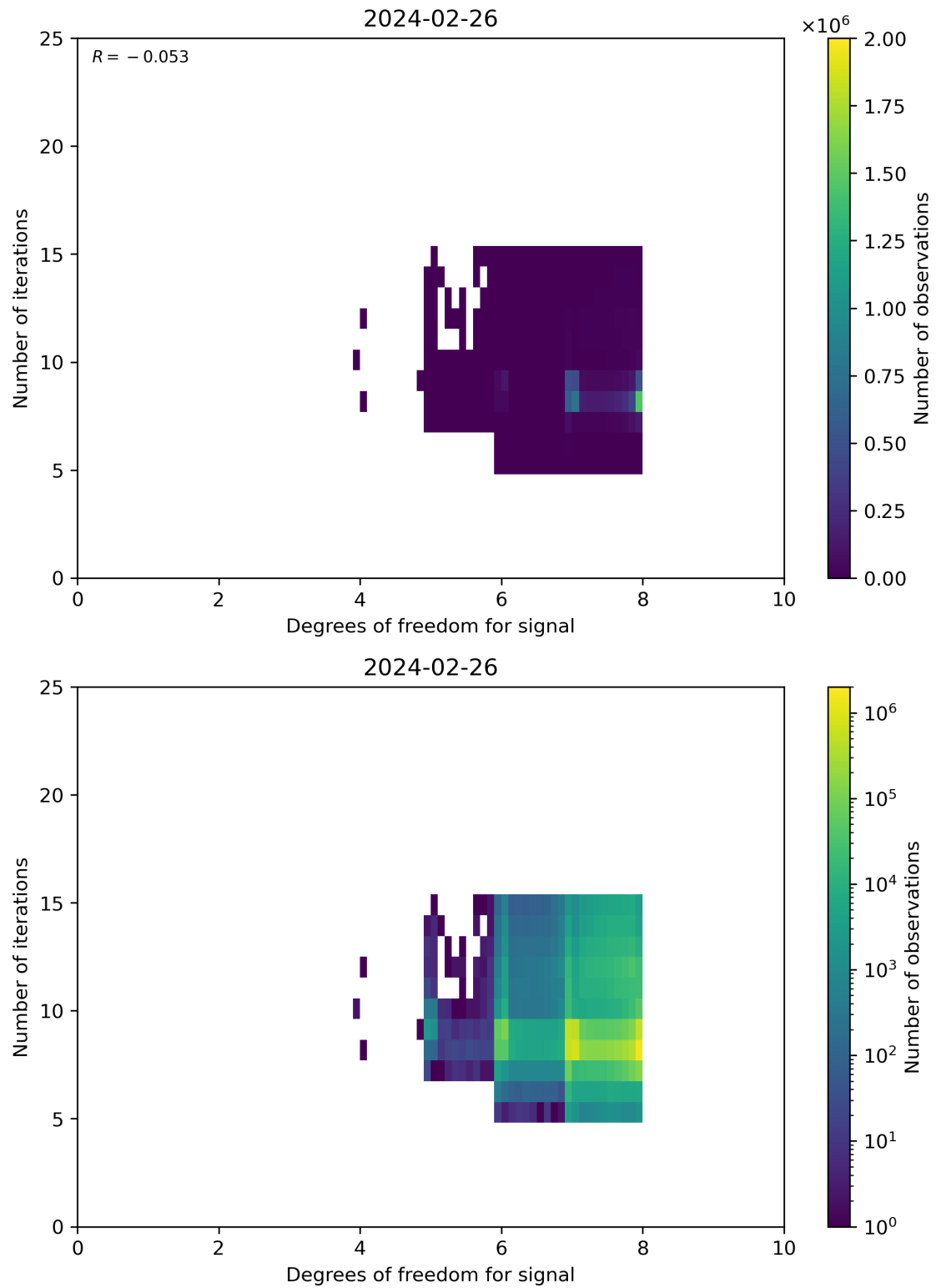
Figure 50: Scatter density plot of “Degrees of freedom for signal” against “Number of iterations” for 2024-02-25 to 2024-02-27.
