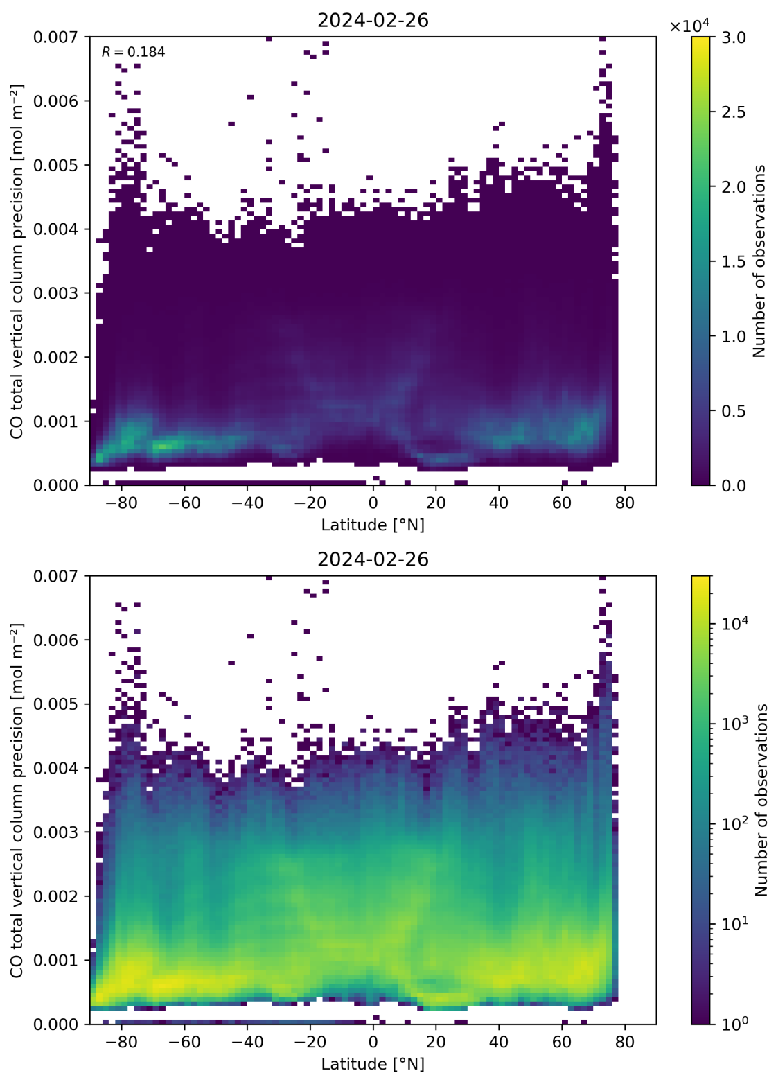
Figure 53: Scatter density plot of “Latitude” against “CO total vertical column precision” for 2024-02-25 to 2024-02-27.
