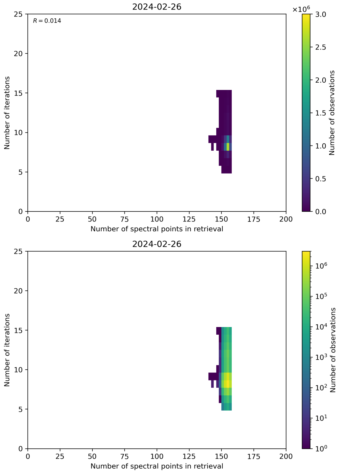
Figure 60: Scatter density plot of “Number of spectral points in retrieval” against “Number of iterations” for 2024-02-25 to 2024-02-27.
