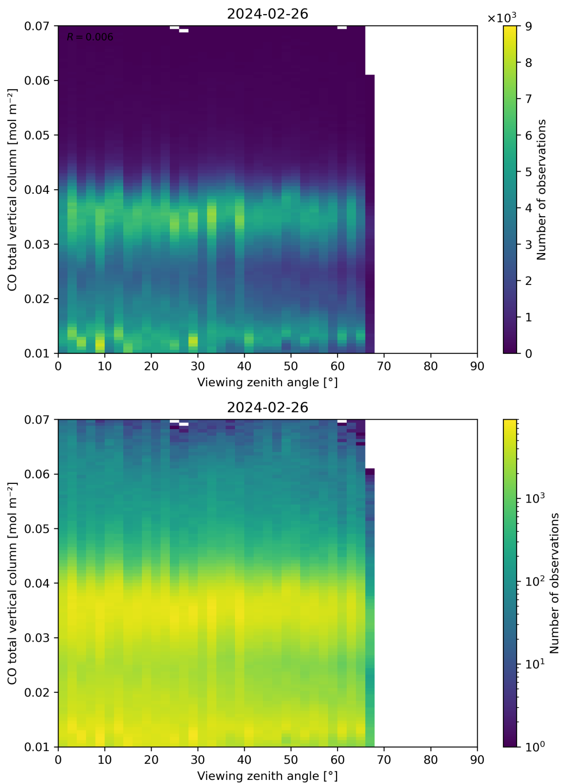
Figure 69: Scatter density plot of “Viewing zenith angle” against “CO total vertical column” for 2024-02-25 to 2024-02-27.
