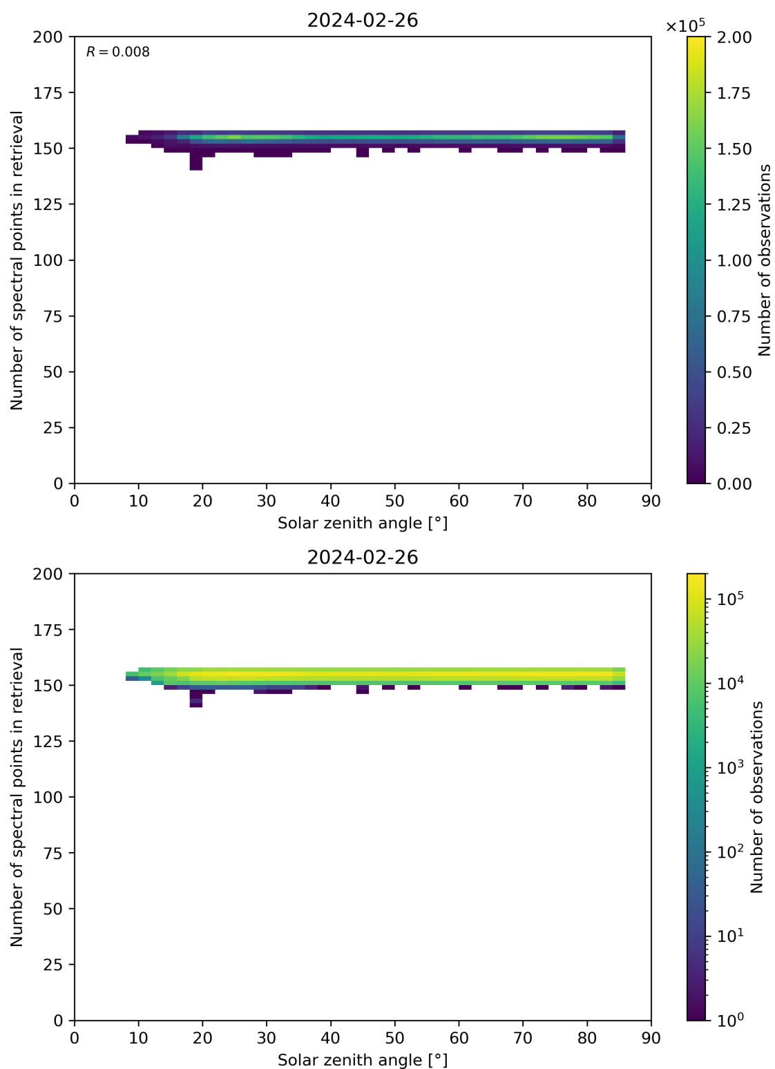
Figure 68: Scatter density plot of “Solar zenith angle” against “Number of spectral points in retrieval” for 2024-02-25 to 2024-02-27.
