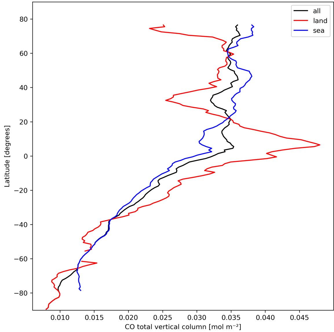
Figure 10: Zonal average of “CO total vertical column” for 2024-02-25 to 2024-02-27.
