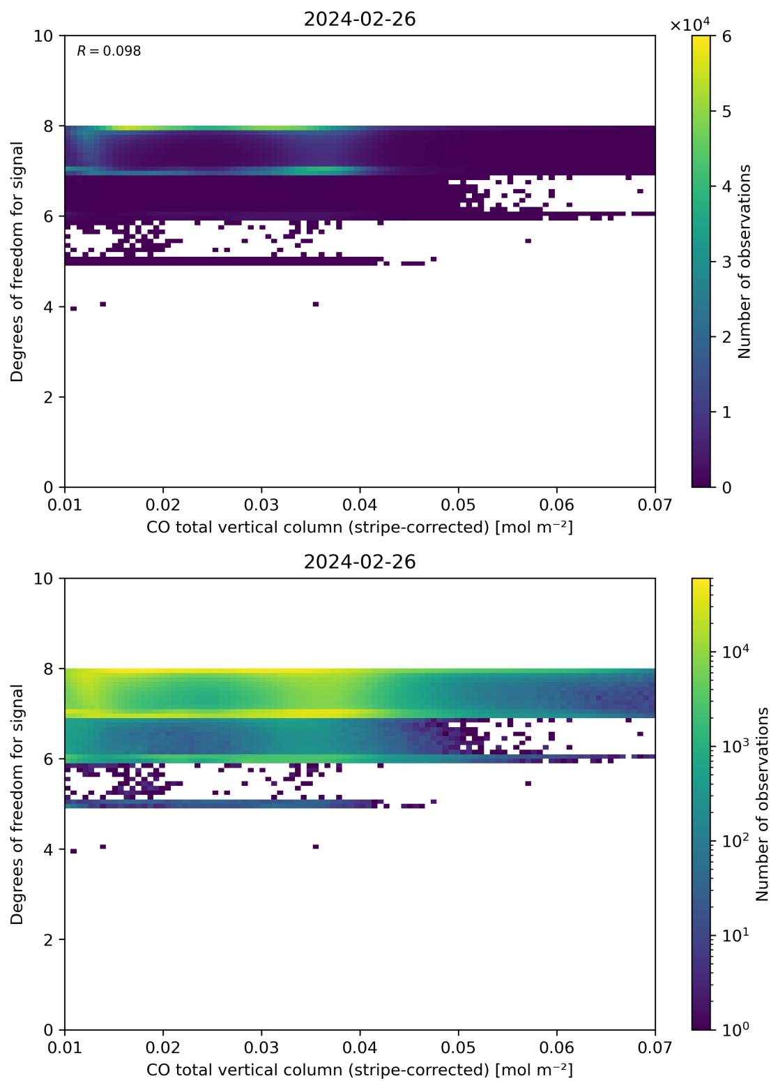
Figure 38: Scatter density plot of “CO total vertical column (stripe-corrected)” against “Degrees of freedom for signal” for 2024-02-25 to 2024-02-27.
