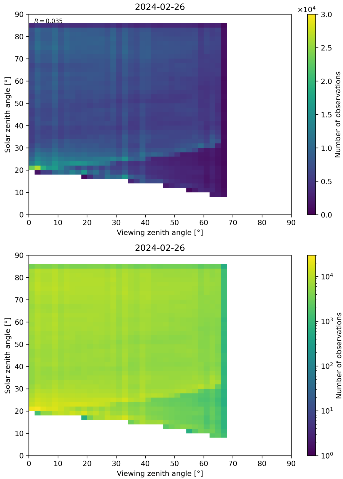
Figure 77: Scatter density plot of “Viewing zenith angle” against “Solar zenith angle” for 2024-02-25 to 2024-02-27.
