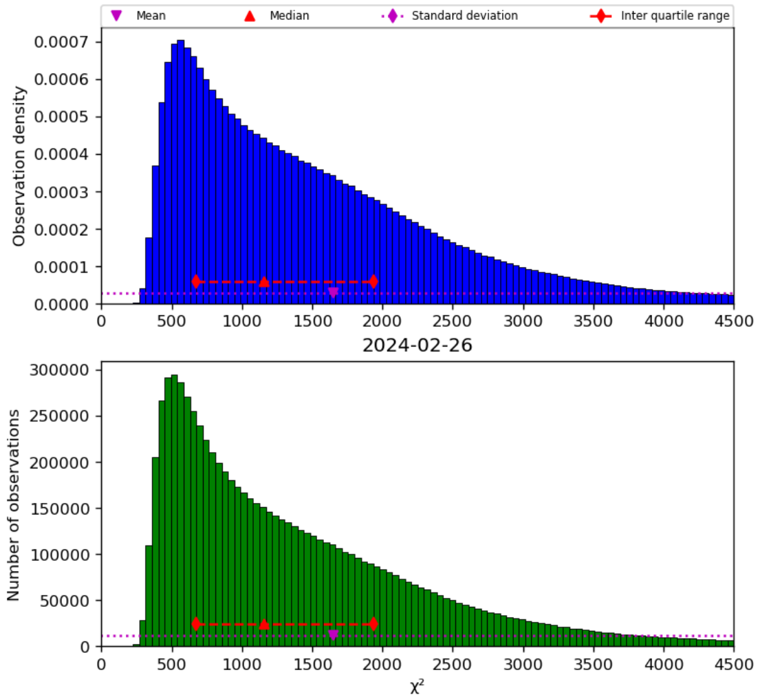
Figure 22: Histogram of “ \chi^2 ” for 2024-02-25 to 2024-02-27
