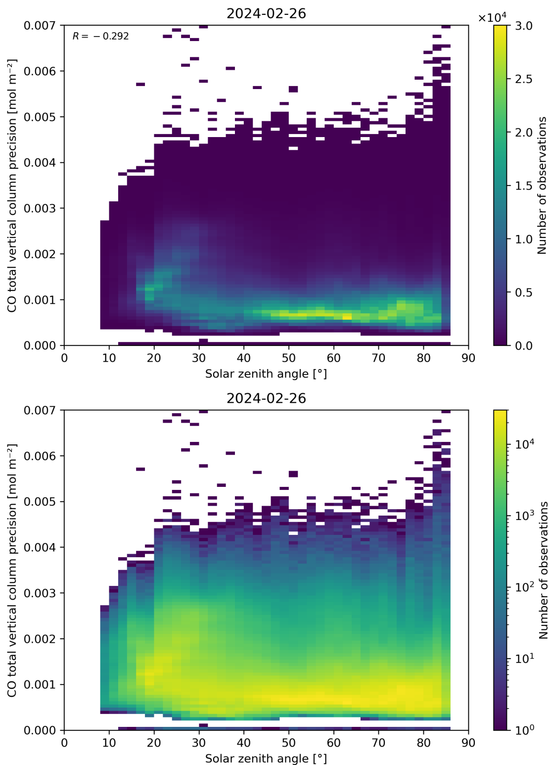
Figure 63: Scatter density plot of “Solar zenith angle” against “CO total vertical column precision” for 2024-02-25 to 2024-02-27.
