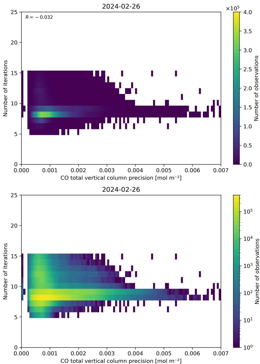
Figure 46: Scatter density plot of “CO total vertical column precision” against “Number of iterations” for 2024-02-25 to 2024-02-27.
