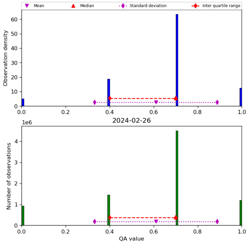
Figure 17: Histogram of “QA value” for 2024-02-25 to 2024-02-27
