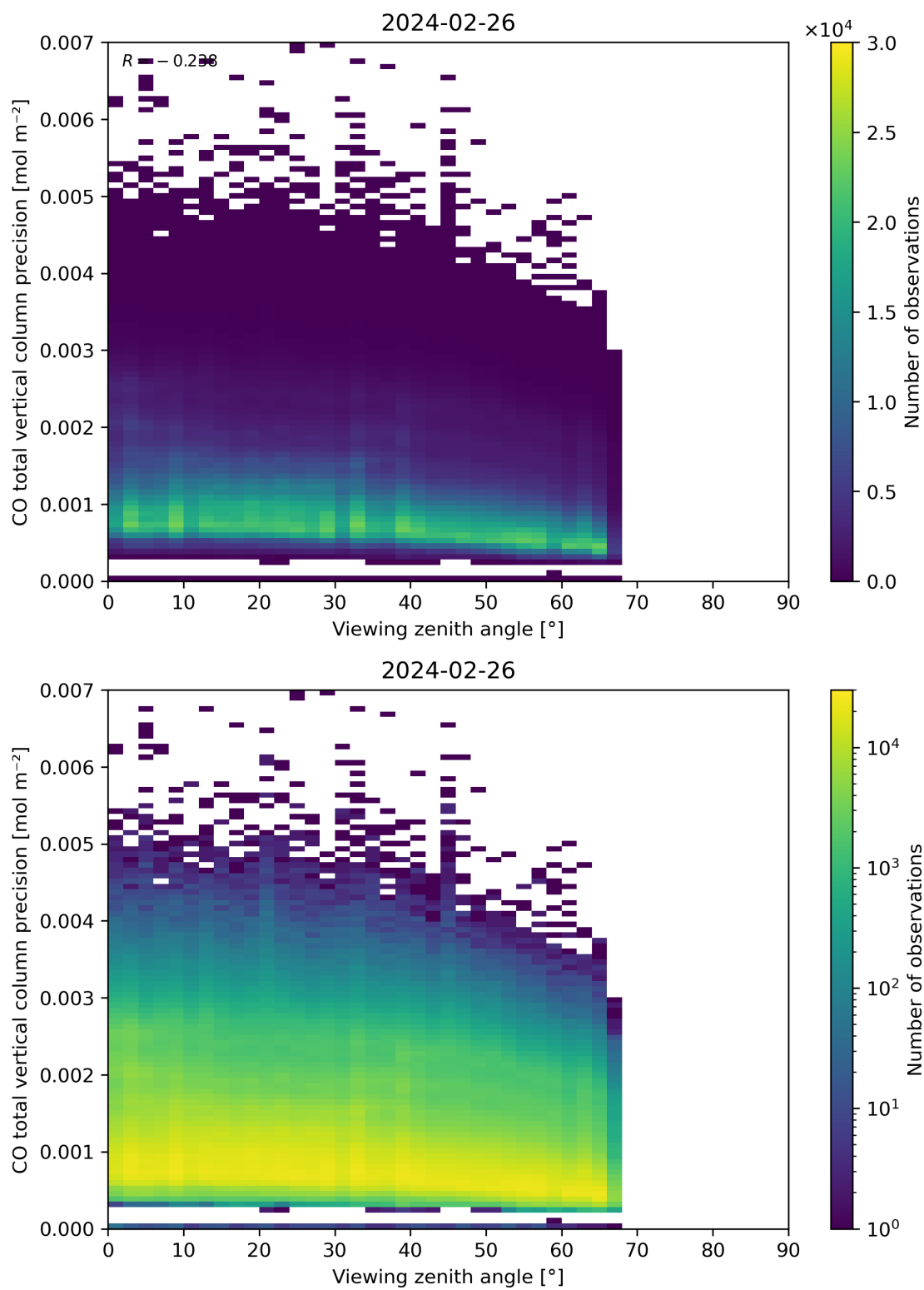
Figure 71: Scatter density plot of “Viewing zenith angle” against “CO total vertical column precision” for 2024-02-25 to 2024-02-27.
