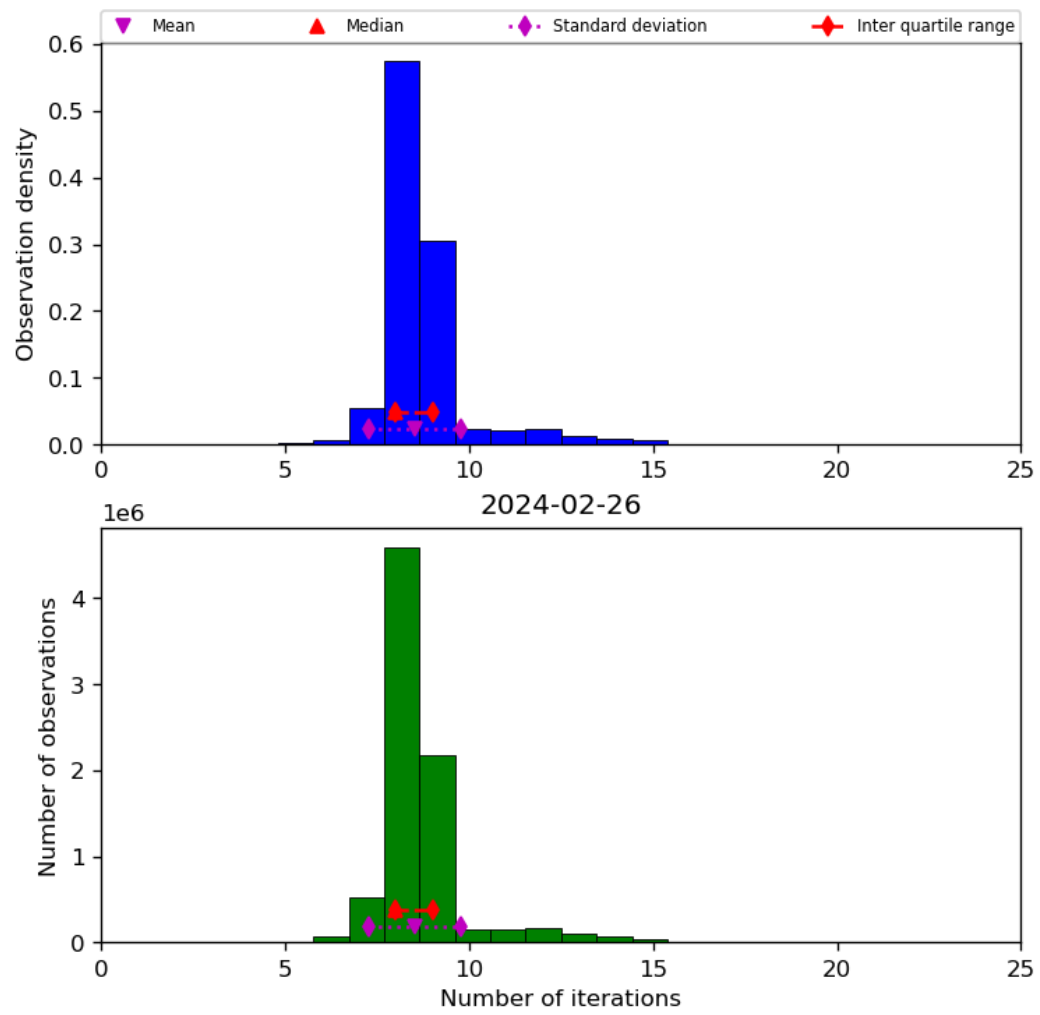
Figure 24: Histogram of “Number of iterations” for 2024-02-25 to 2024-02-27
