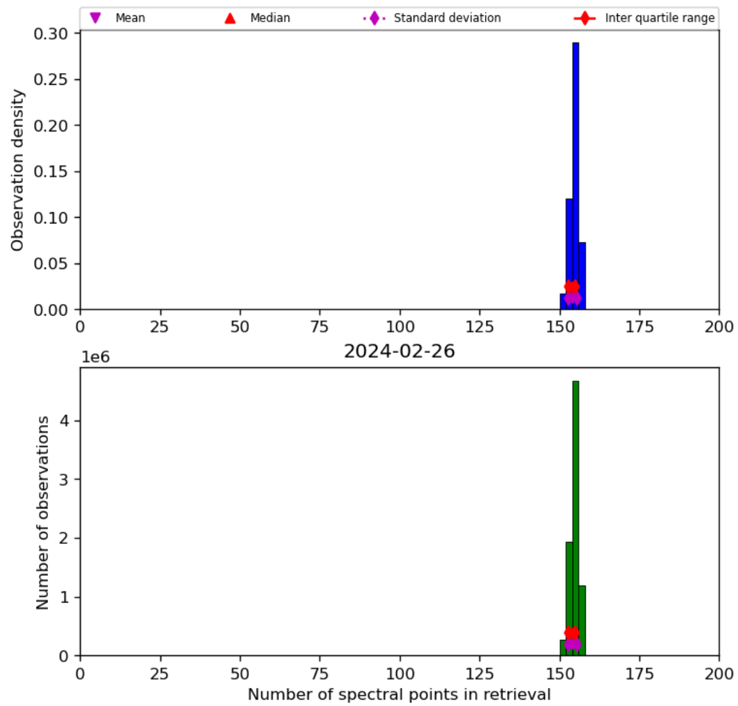
Figure 21: Histogram of “Number of spectral points in retrieval” for 2024-02-25 to 2024-02-27
