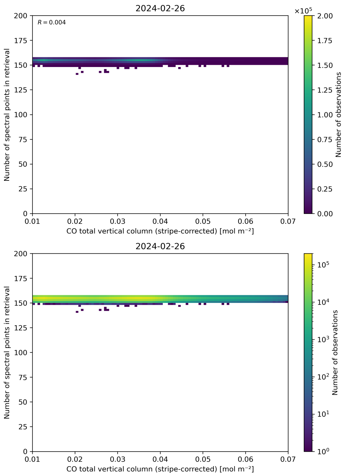
Figure 40: Scatter density plot of “CO total vertical column (stripe-corrected)” against “Number of spectral points in retrieval” for 2024-02-25 to 2024-02-27.
