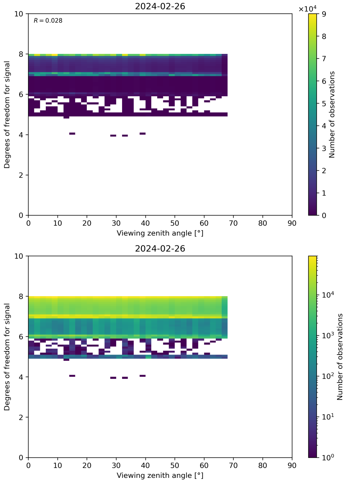
Figure 73: Scatter density plot of “Viewing zenith angle” against “Degrees of freedom for signal” for 2024-02-25 to 2024-02-27.
