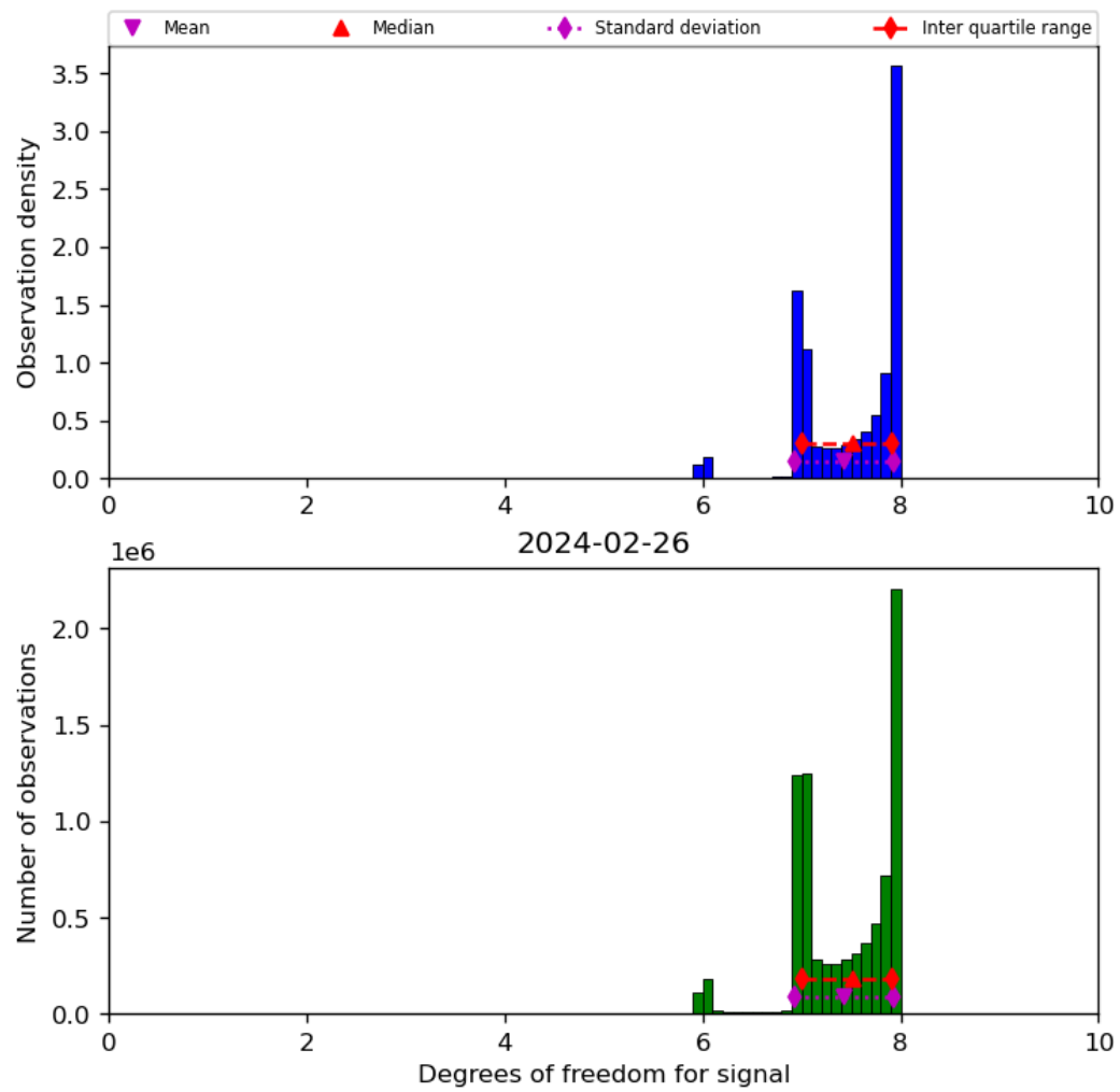
Figure 23: Histogram of “Degrees of freedom for signal” for 2024-02-25 to 2024-02-27
