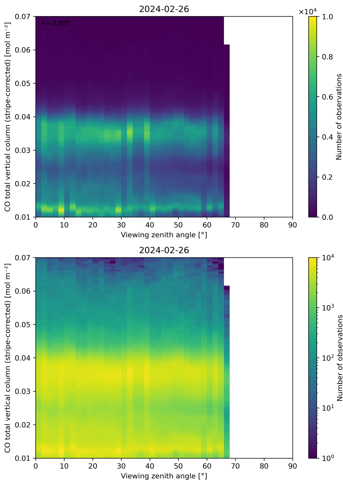
Figure 70: Scatter density plot of “Viewing zenith angle” against “CO total vertical column (stripe-corrected)” for 2024-02-25 to 2024-02-27.
