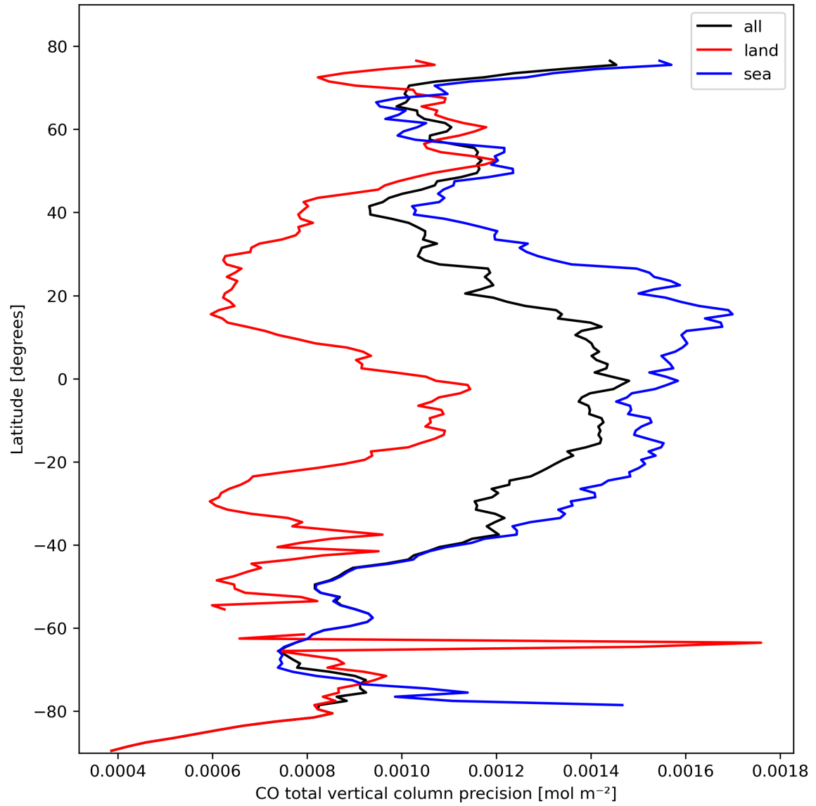
Figure 12: Zonal average of "CO total vertical column precision" for 2024-02-25 to 2024-02-27.
