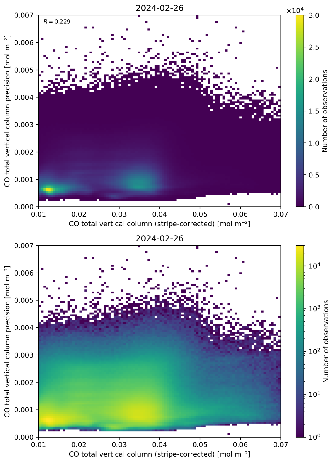
Figure 36: Scatter density plot of “CO total vertical column (stripe-corrected)” against “CO total vertical column precision” for 2024-02-25 to 2024-02-27.
