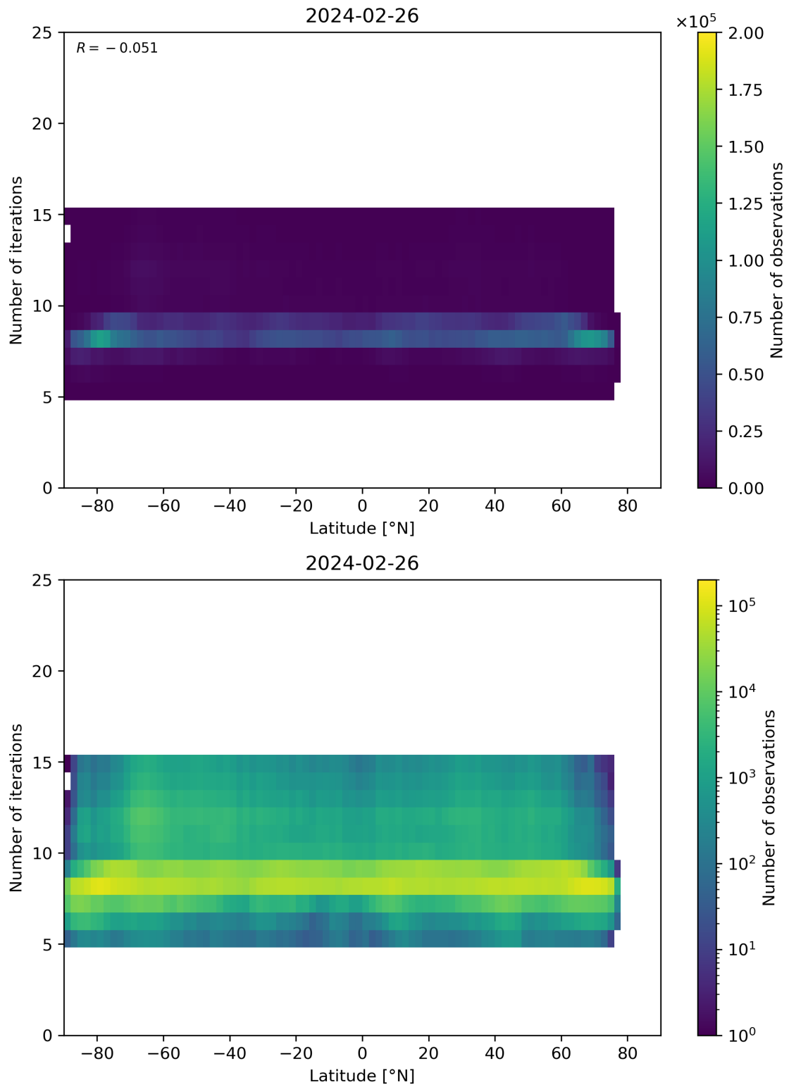
Figure 56: Scatter density plot of “Latitude” against “Number of iterations” for 2024-02-25 to 2024-02-27.
