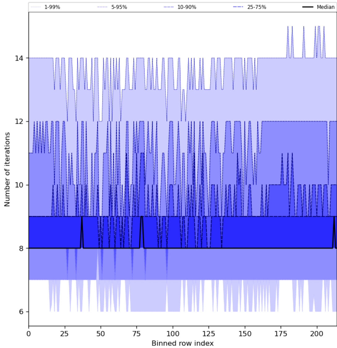
Figure 32: Along track statistics of “Number of iterations” for 2024-02-25 to 2024-02-27
