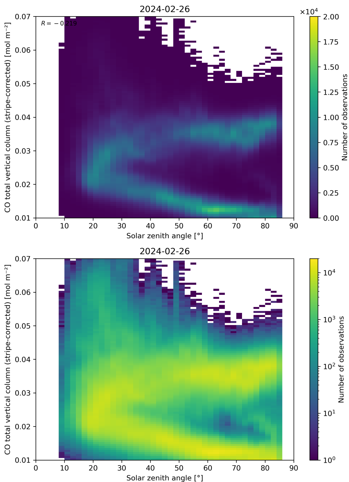
Figure 62: Scatter density plot of “Solar zenith angle” against “CO total vertical column (stripe-corrected)” for 2024-02-25 to 2024-02-27.
