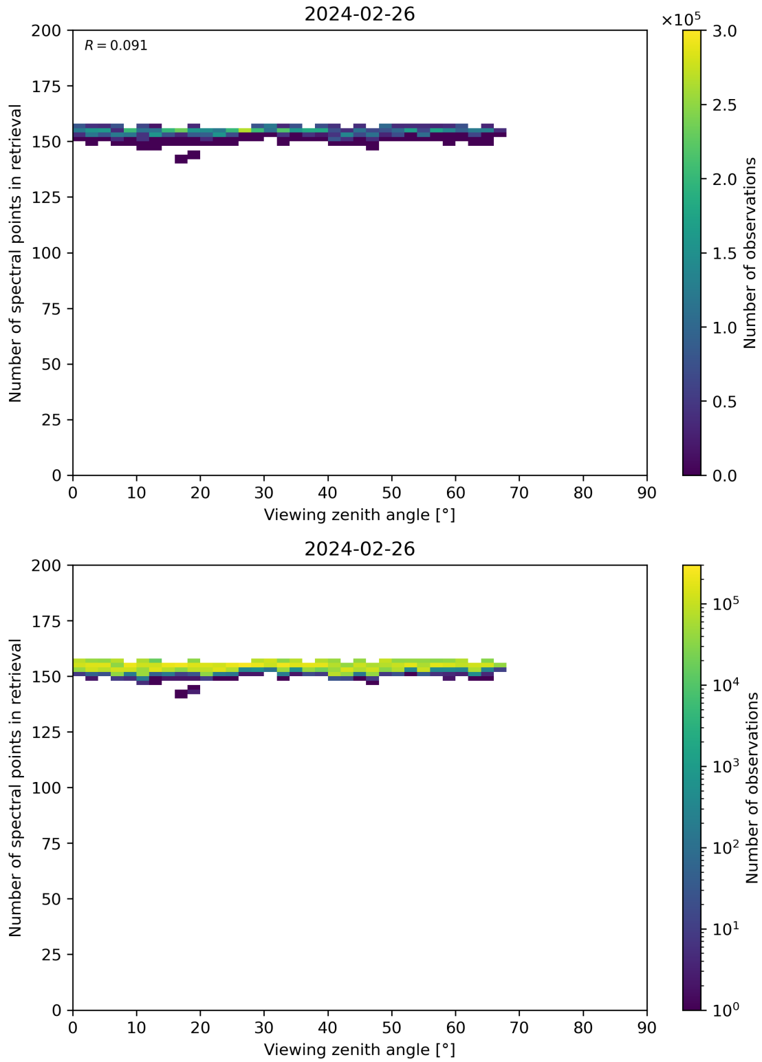
Figure 76: Scatter density plot of “Viewing zenith angle” against “Number of spectral points in retrieval” for 2024-02-25 to 2024-02-27.
