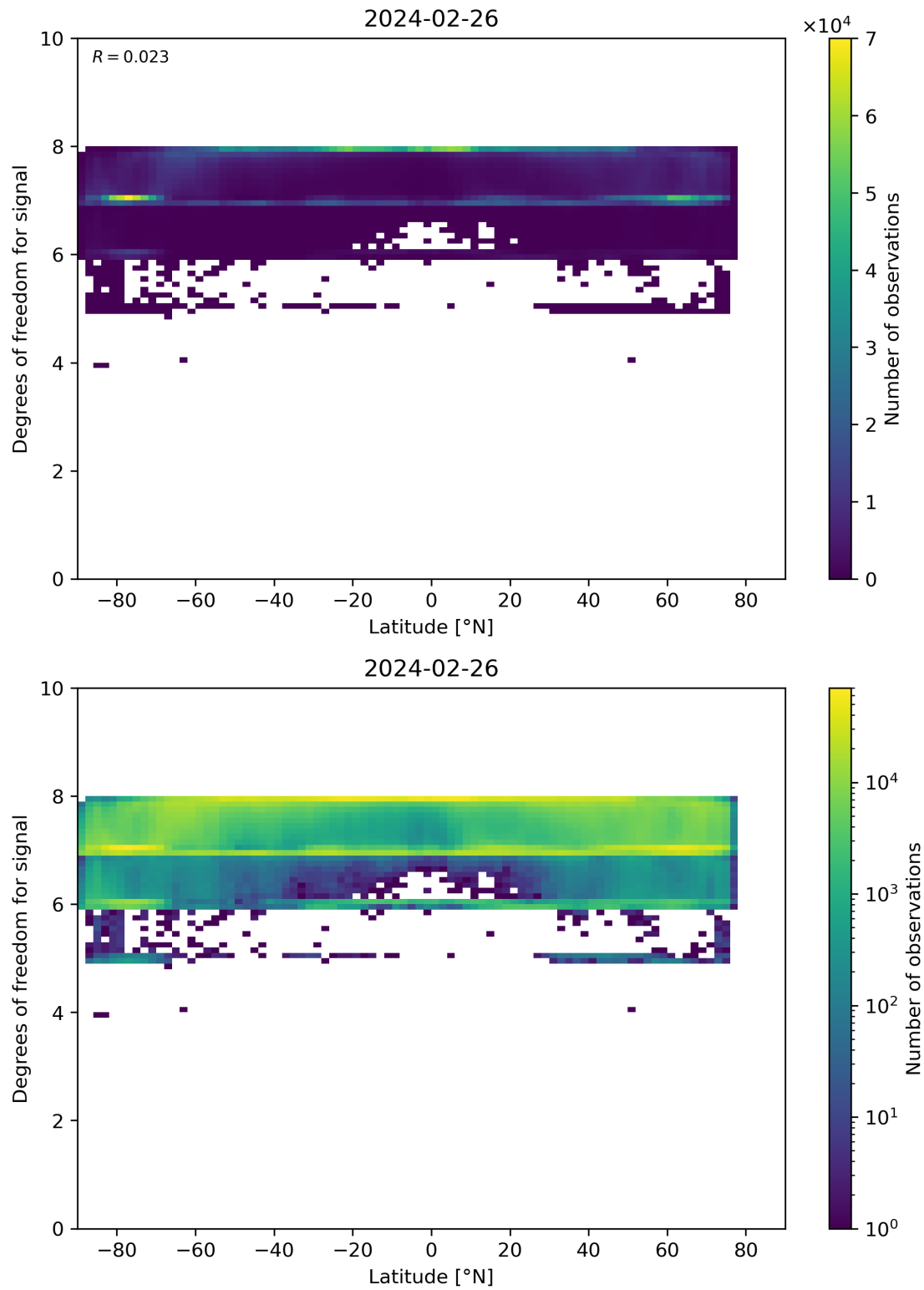
Figure 55: Scatter density plot of “Latitude” against “Degrees of freedom for signal” for 2024-02-25 to 2024-02-27.
