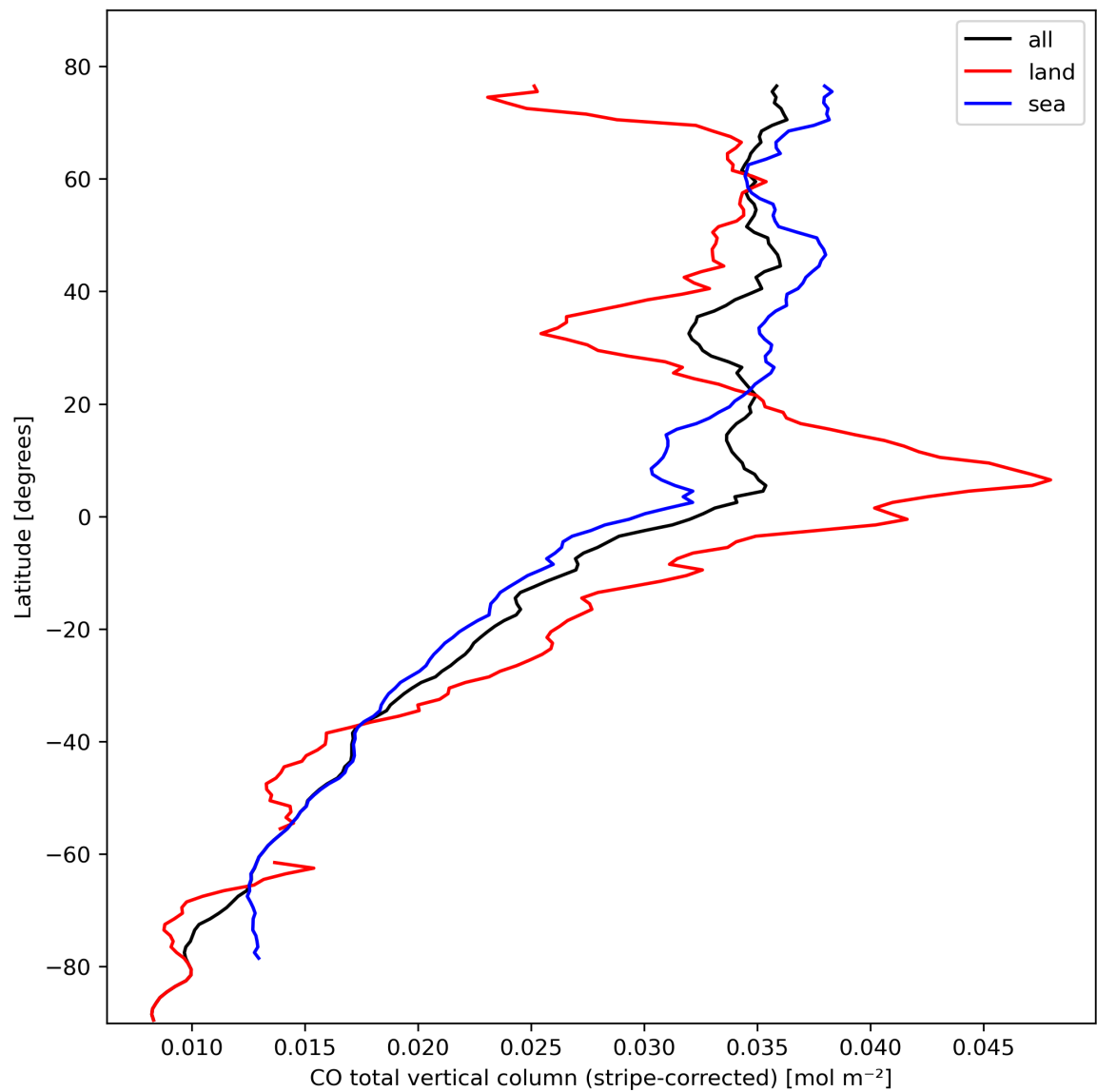
Figure 11: Zonal average of “CO total vertical column (stripe-corrected)” for 2024-02-25 to 2024-02-27.
