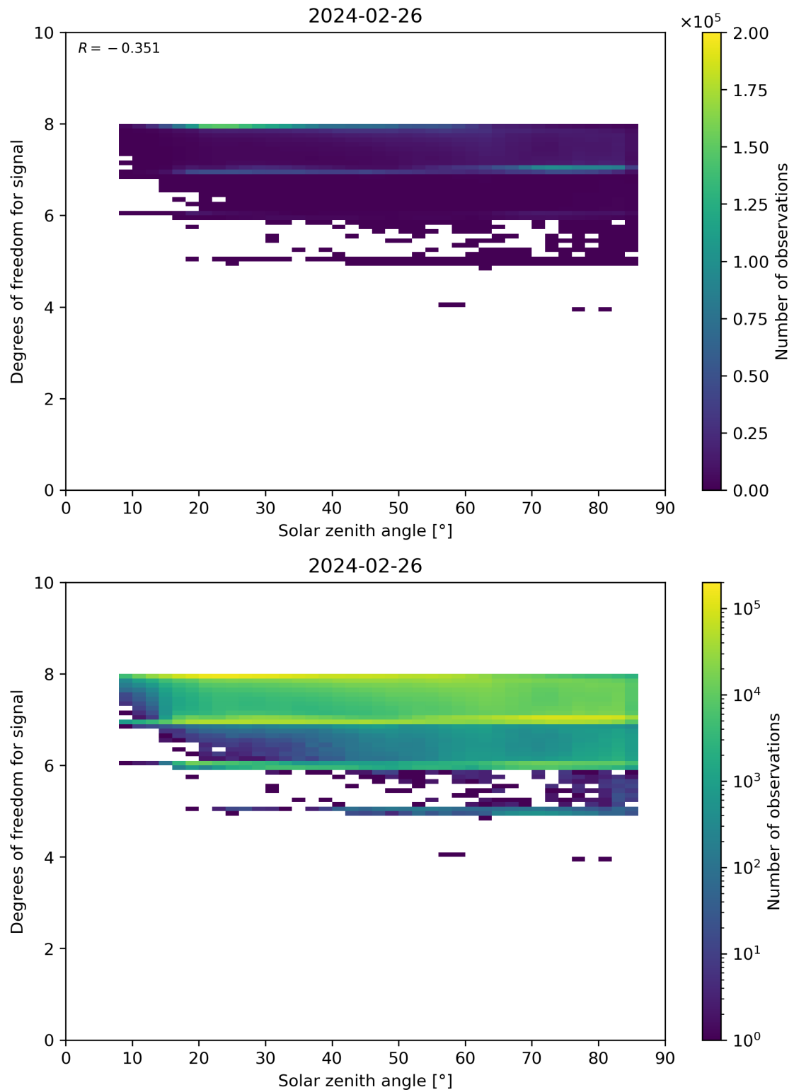
Figure 65: Scatter density plot of “Solar zenith angle” against “Degrees of freedom for signal” for 2024-02-25 to 2024-02-27.
