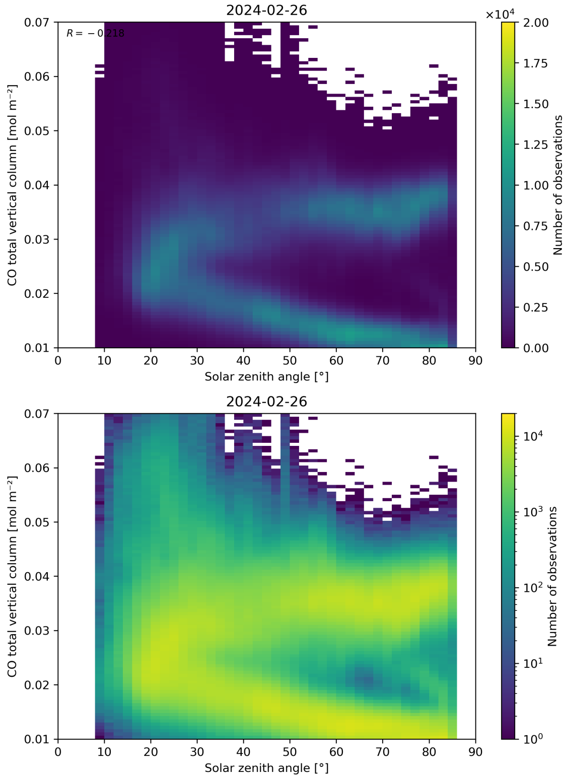
Figure 61: Scatter density plot of “Solar zenith angle” against “CO total vertical column” for 2024-02-25 to 2024-02-27.
