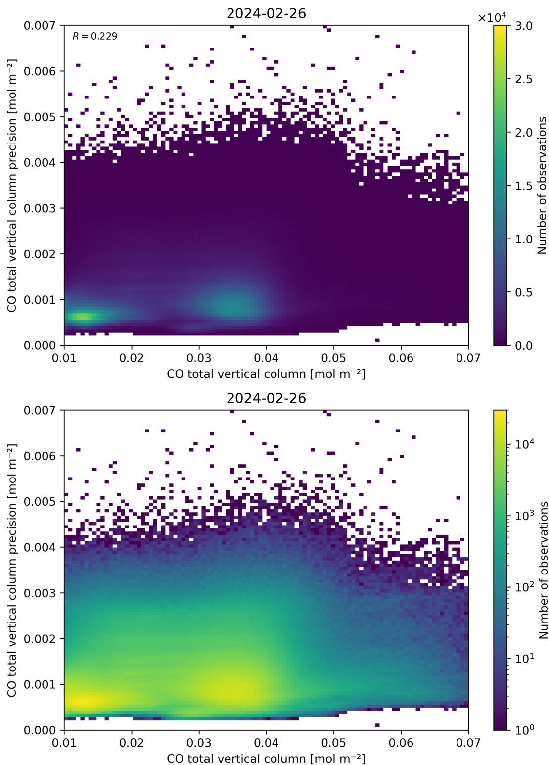
Figure 34: Scatter density plot of “CO total vertical column” against “CO total vertical column precision” for 2024-02-25 to 2024-02-27.
