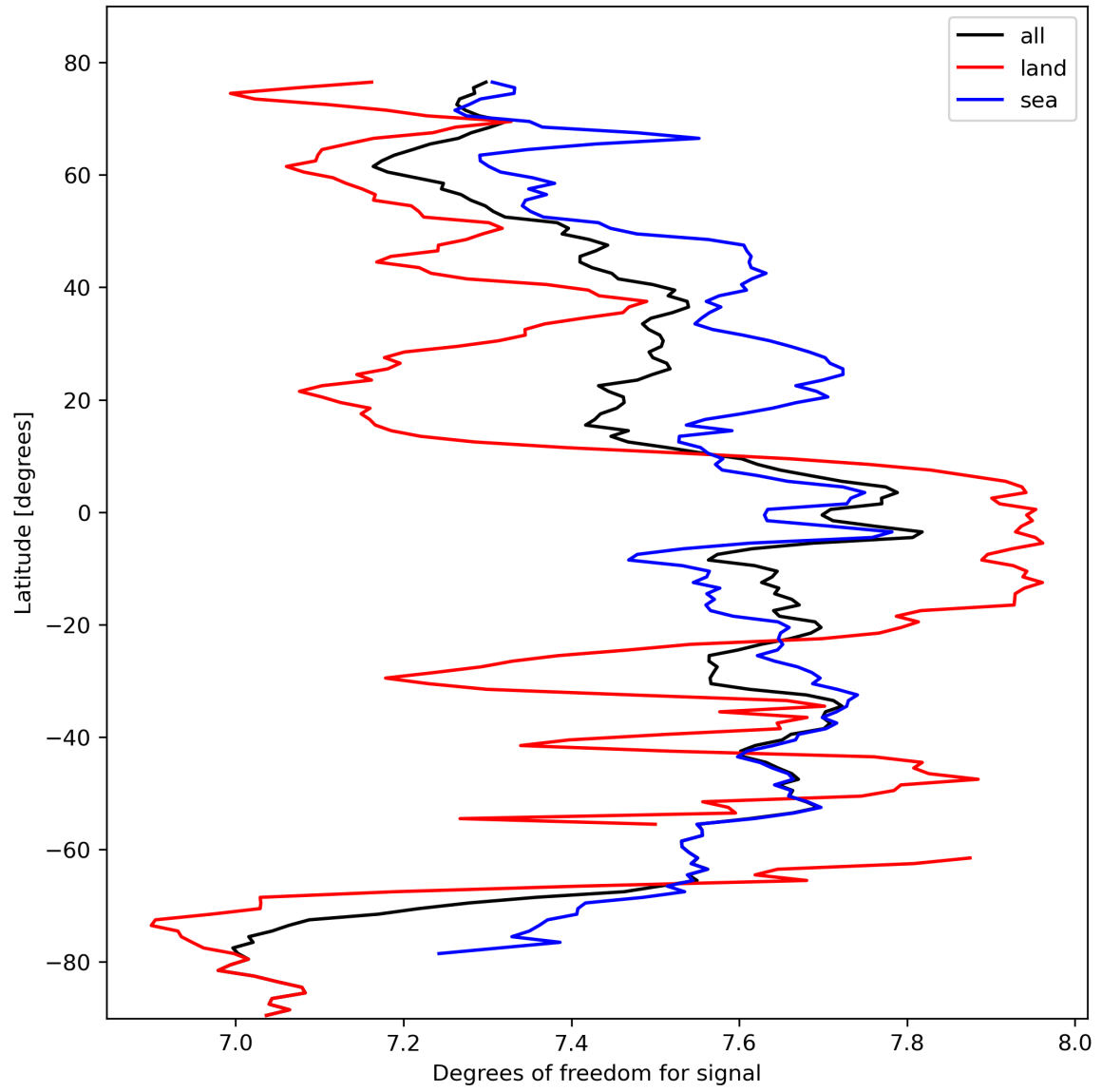
Figure 15: Zonal average of “Degrees of freedom for signal” for 2024-02-25 to 2024-02-27.
