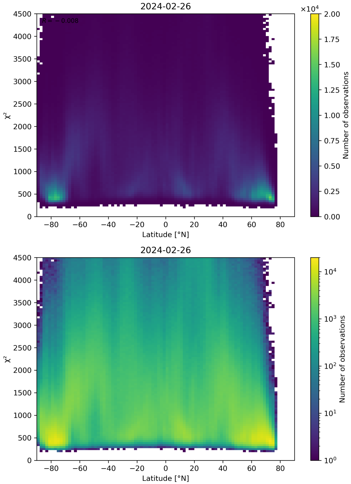
Figure 54: Scatter density plot of “Latitude” against “ \chi^2 ” for 2024-02-25 to 2024-02-27.
