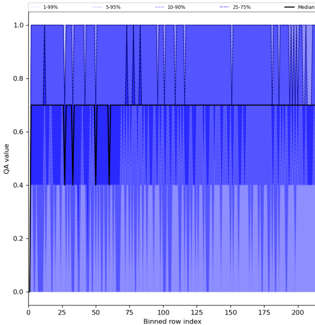
Figure 25: Along track statistics of “QA value” for 2024-02-25 to 2024-02-27
