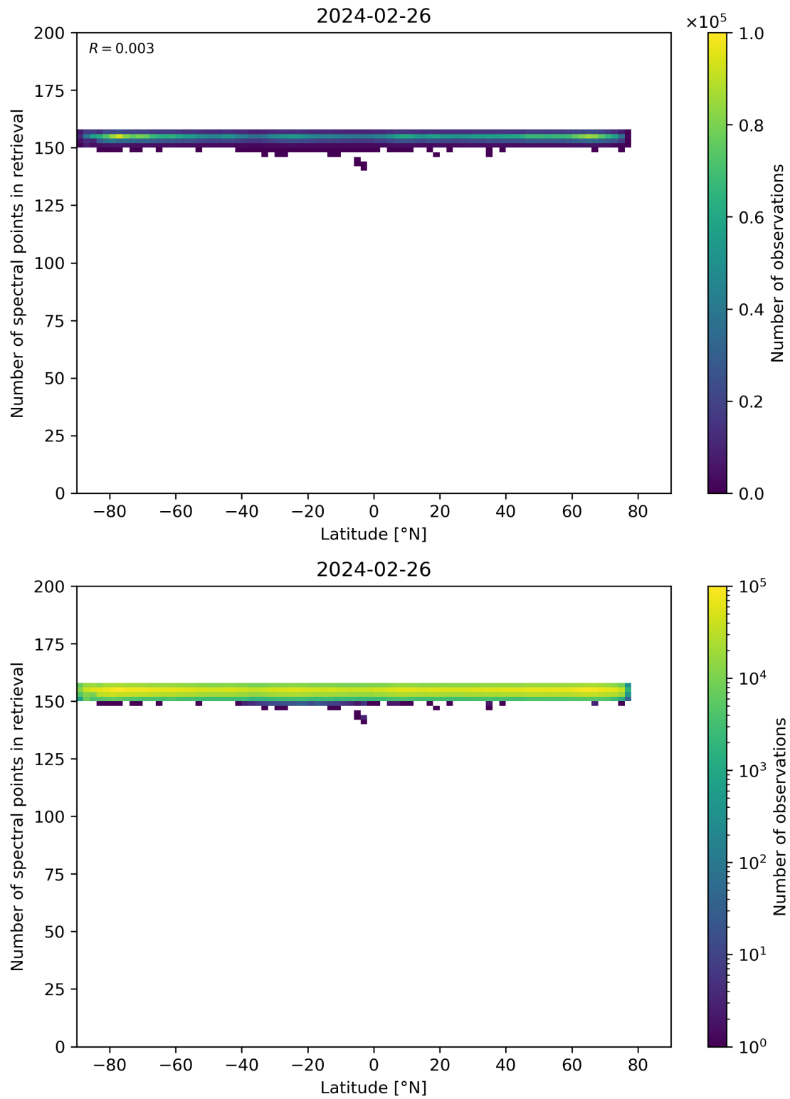
Figure 57: Scatter density plot of “Latitude” against “Number of spectral points in retrieval” for 2024-02-25 to 2024-02-27.
