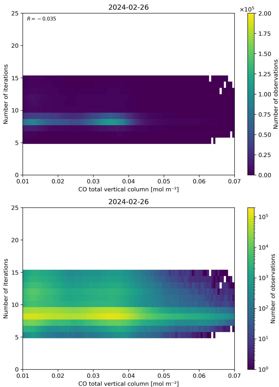
Figure 42: Scatter density plot of “CO total vertical column” against “Number of iterations” for 2024-02-25 to 2024-02-27.
