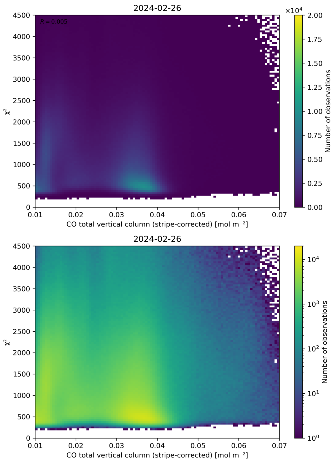
Figure 37: Scatter density plot of “CO total vertical column (stripe-corrected)” against “ \chi^2 ” for 2024-02-25 to 2024-02-27.
