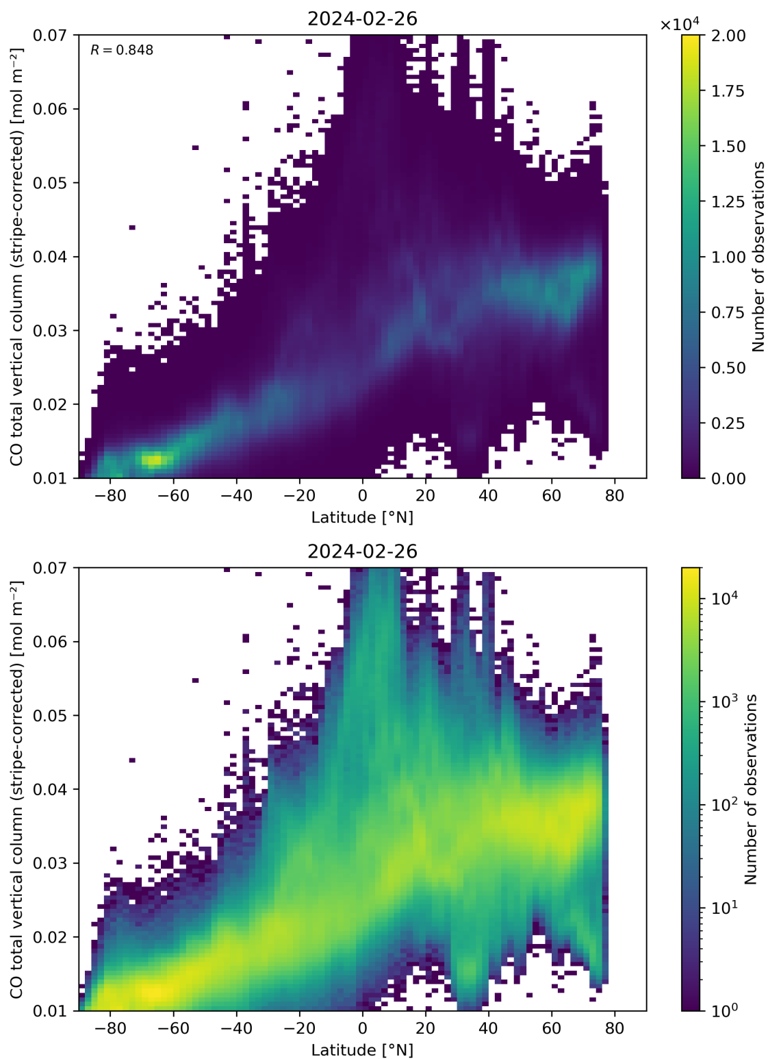
Figure 52: Scatter density plot of “Latitude” against “CO total vertical column (stripe-corrected)” for 2024-02-25 to 2024-02-27.
