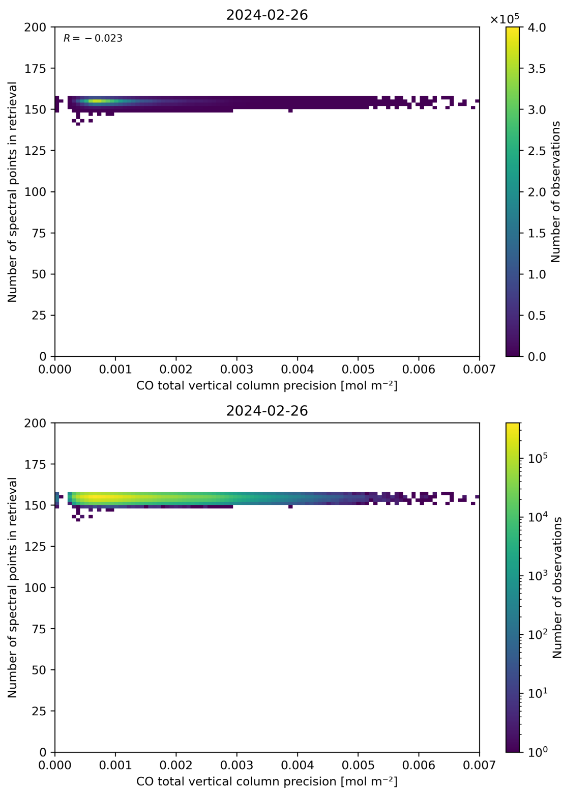
Figure 47: Scatter density plot of “CO total vertical column precision” against “Number of spectral points in retrieval” for 2024-02-25 to 2024-02-27.
