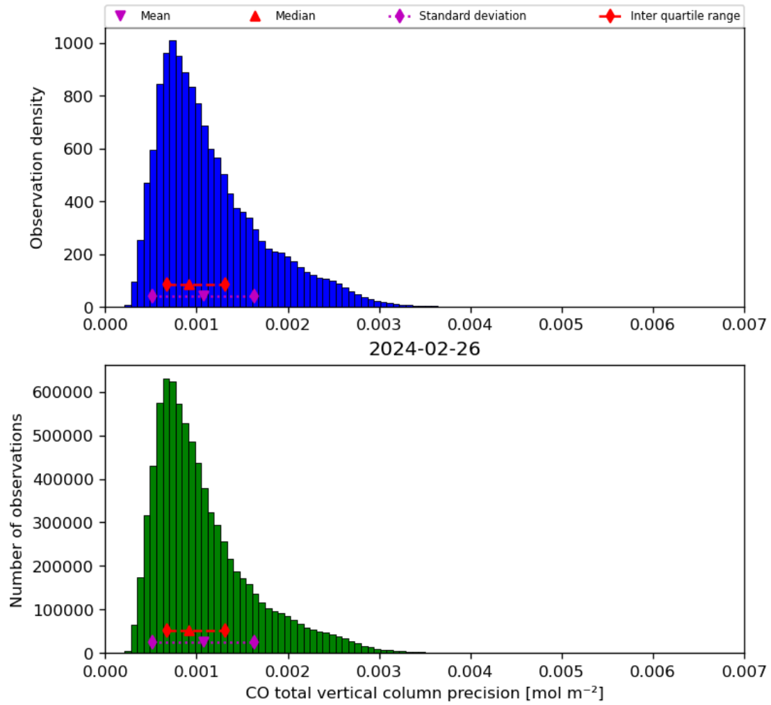
Figure 20: Histogram of “CO total vertical column precision” for 2024-02-25 to 2024-02-27
