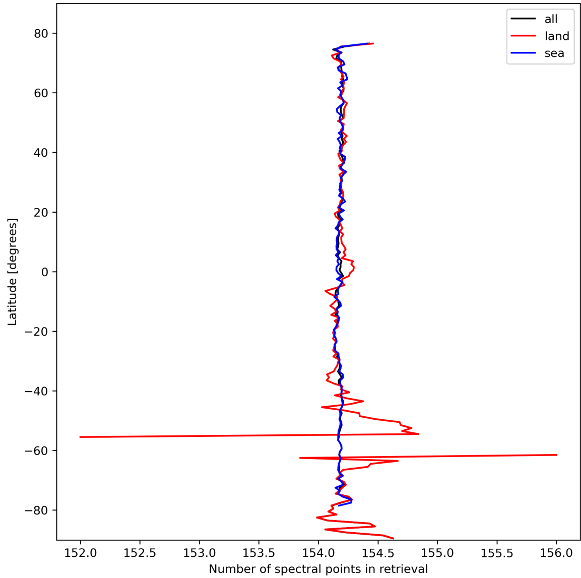
Figure 13: Zonal average of “Number of spectral points in retrieval” for 2024-02-25 to 2024-02-27.
