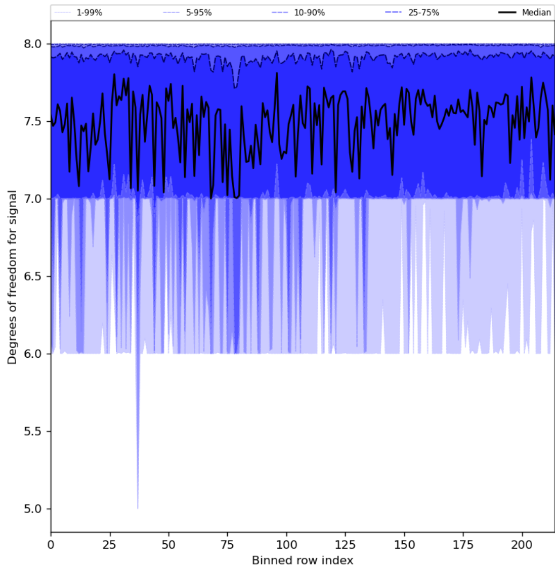
Figure 31: Along track statistics of “Degrees of freedom for signal” for 2024-02-25 to 2024-02-27
