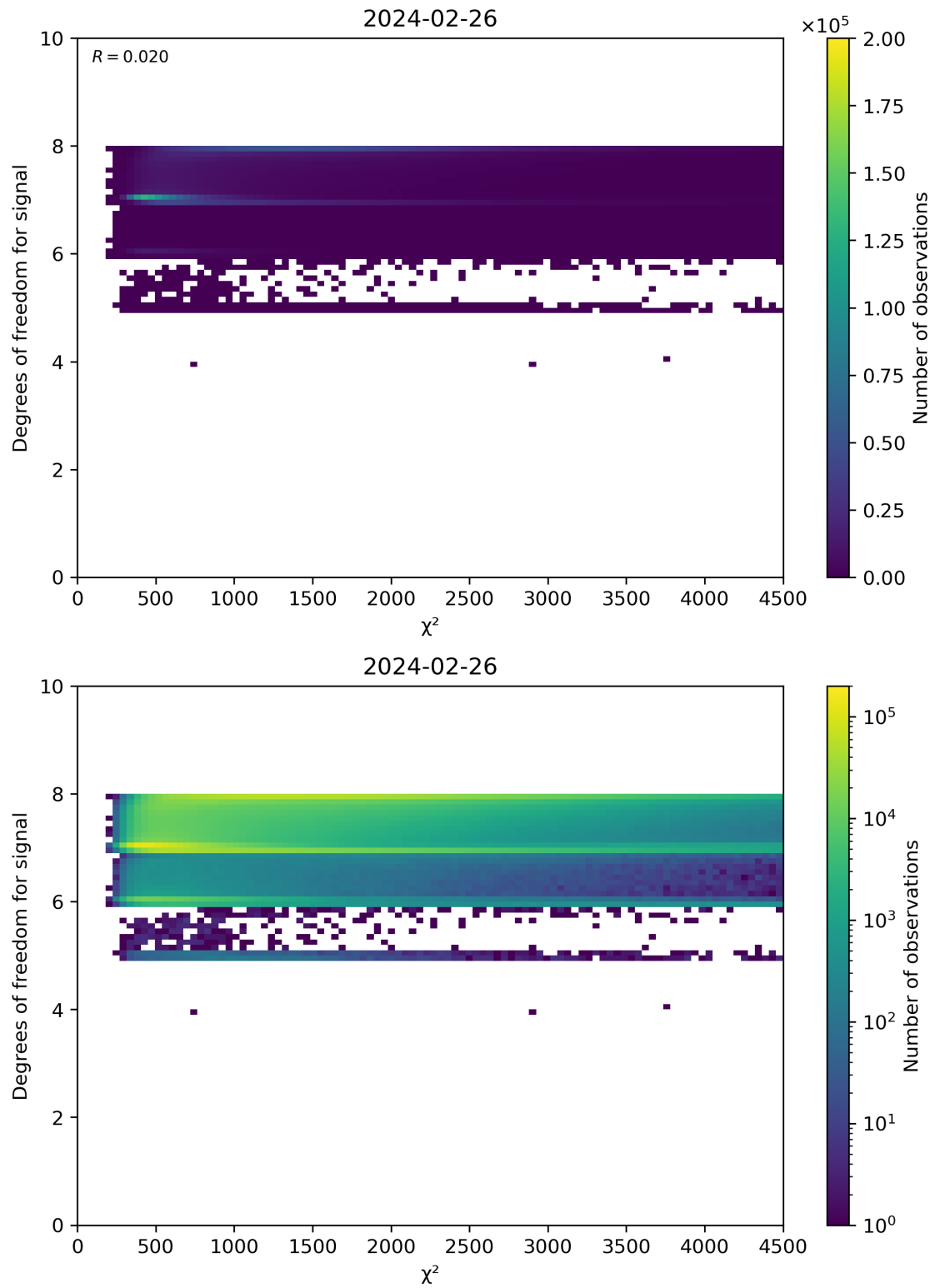
Figure 48: Scatter density plot of “ \chi^2 ” against “Degrees of freedom for signal” for 2024-02-25 to 2024-02-27.
