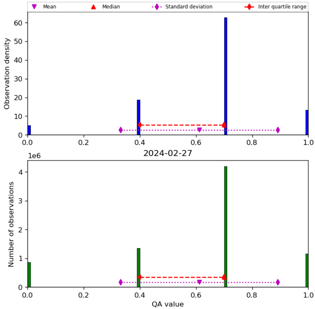
Figure 17: Histogram of “QA value” for 2024-02-27 to 2024-02-28
