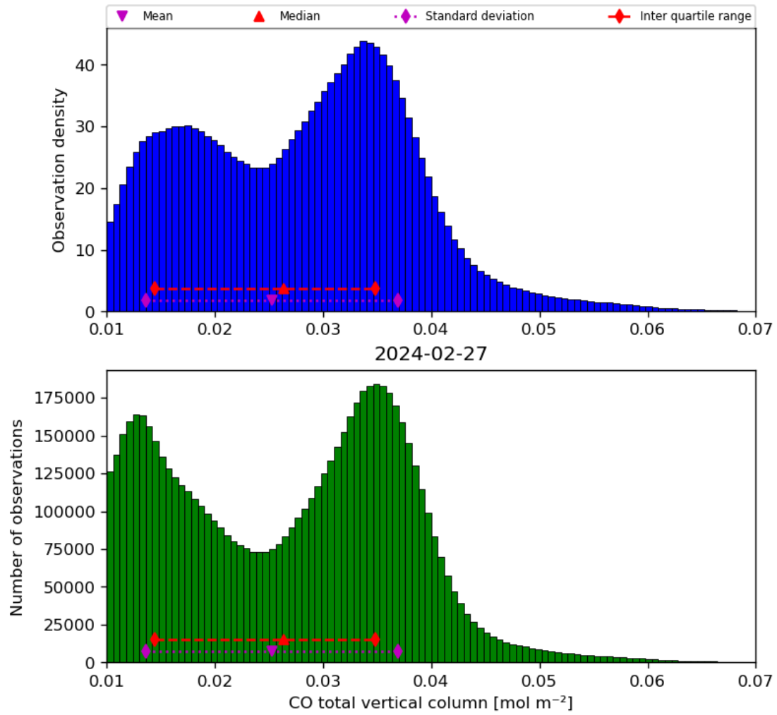
Figure 18: Histogram of “CO total vertical column” for 2024-02-27 to 2024-02-28
