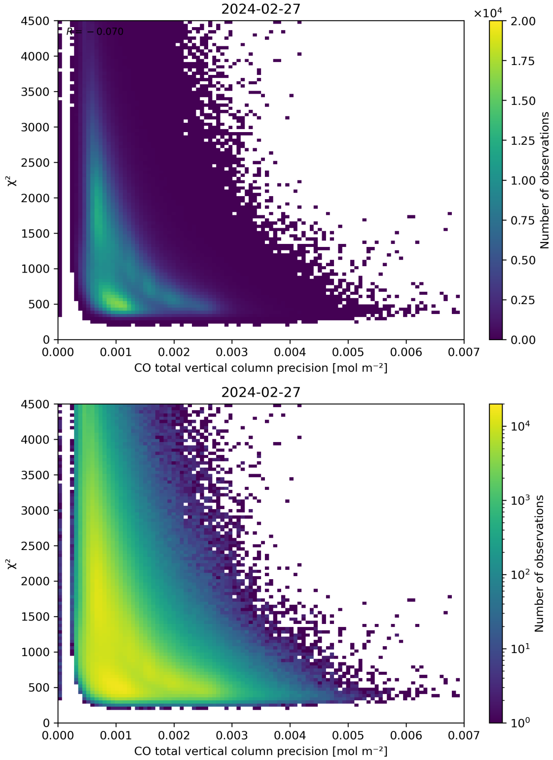
Figure 44: Scatter density plot of “CO total vertical column precision” against “ \chi^2 ” for 2024-02-27 to 2024-02-28.
