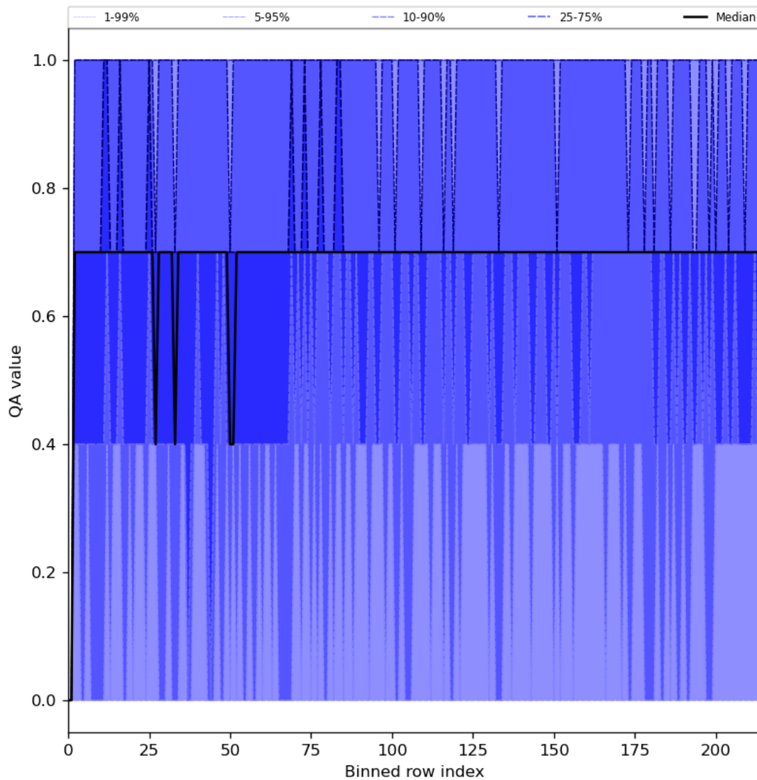
Figure 25: Along track statistics of “QA value” for 2024-02-27 to 2024-02-28
