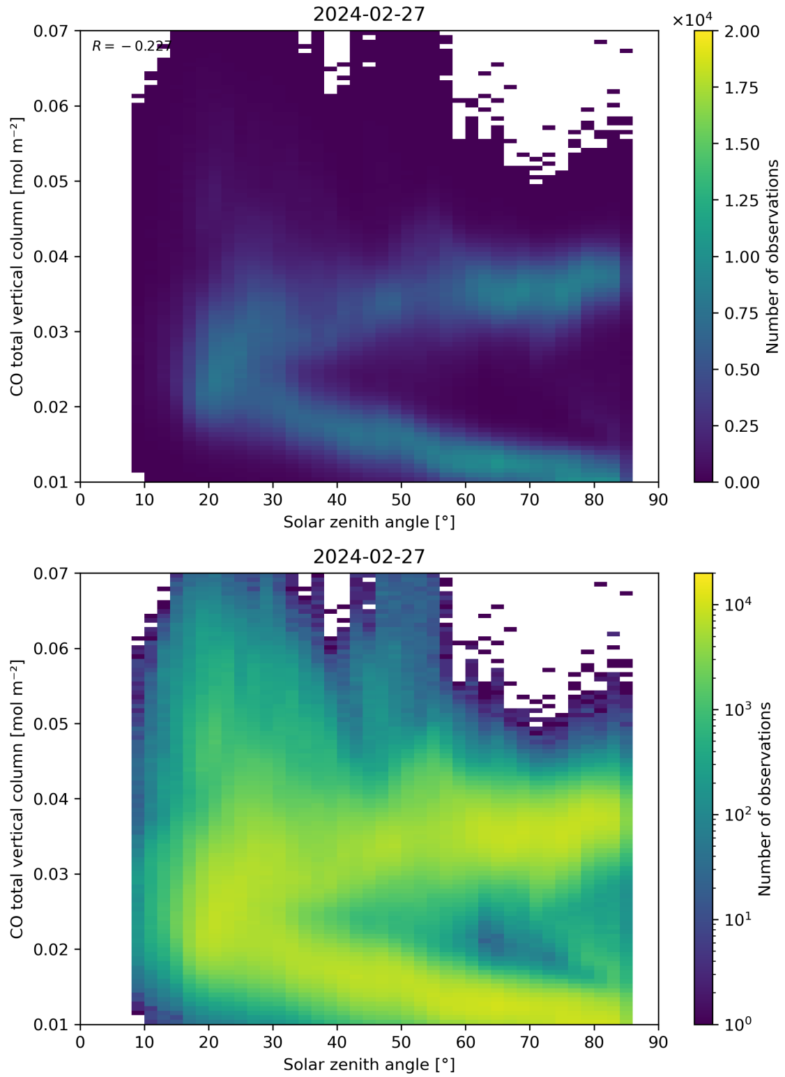
Figure 61: Scatter density plot of “Solar zenith angle” against “CO total vertical column” for 2024-02-27 to 2024-02-28.
