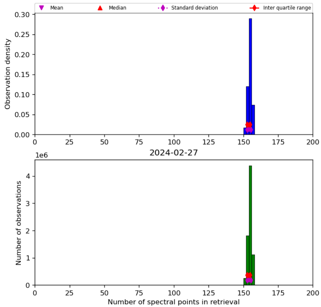
Figure 21: Histogram of “Number of spectral points in retrieval” for 2024-02-27 to 2024-02-28
