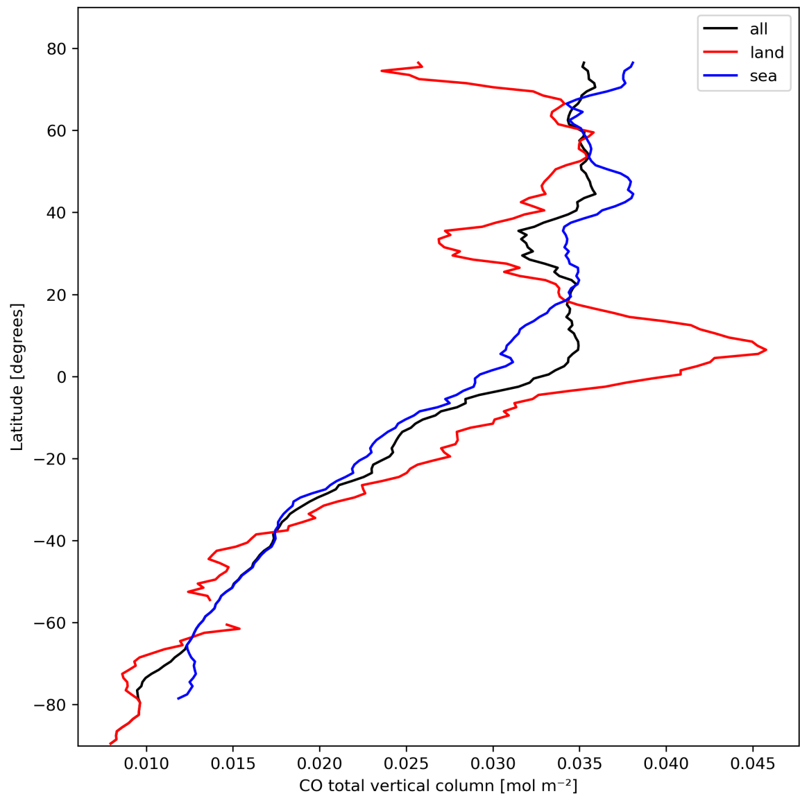
Figure 10: Zonal average of “CO total vertical column” for 2024-02-27 to 2024-02-28.
