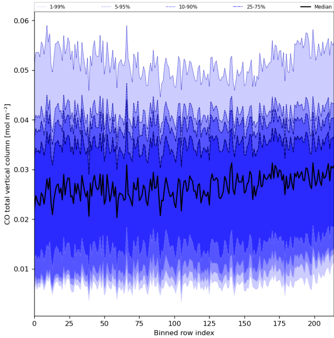
Figure 26: Along track statistics of “CO total vertical column” for 2024-02-27 to 2024-02-28
