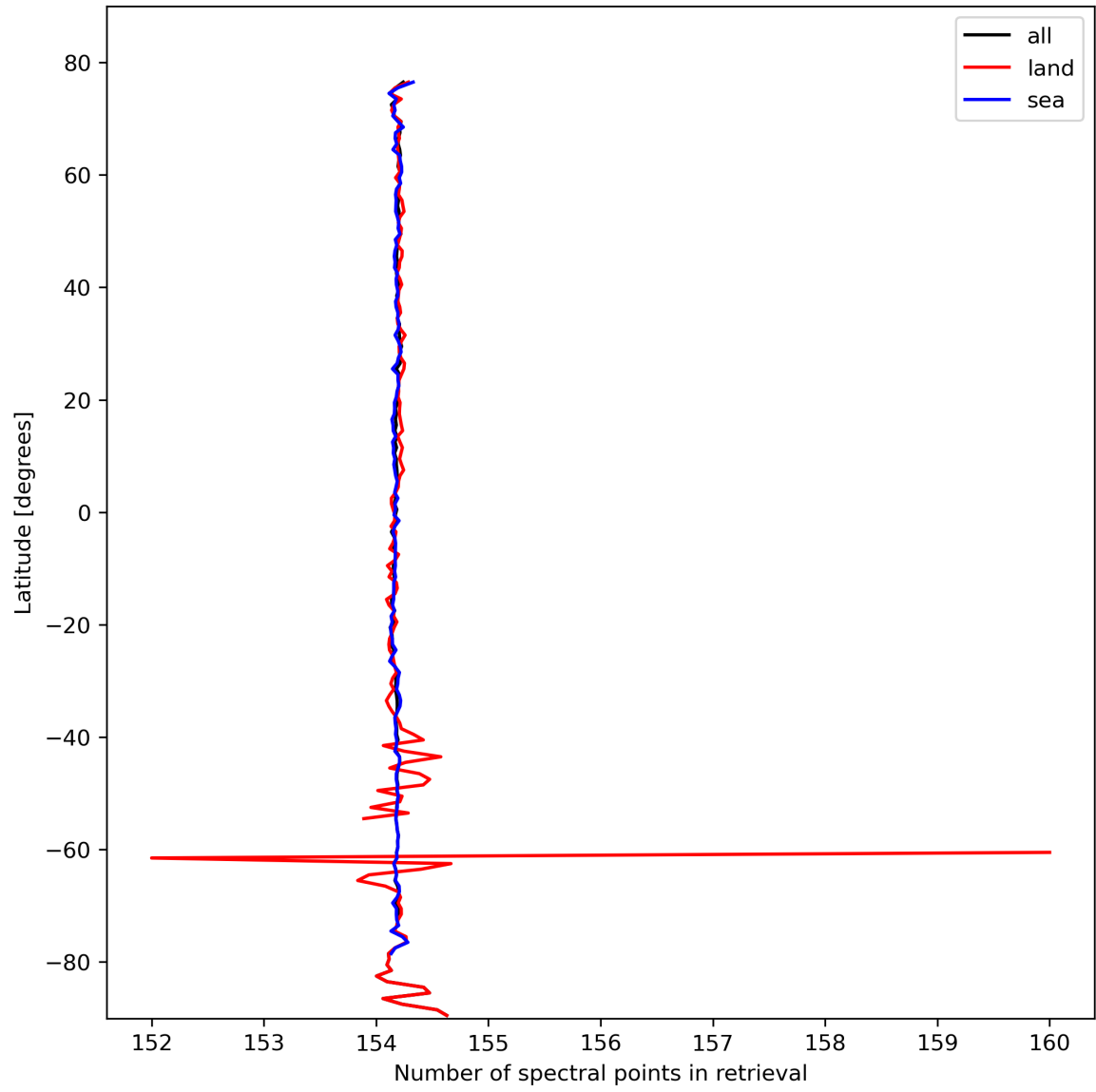
Figure 13: Zonal average of “Number of spectral points in retrieval” for 2024-02-27 to 2024-02-28.
