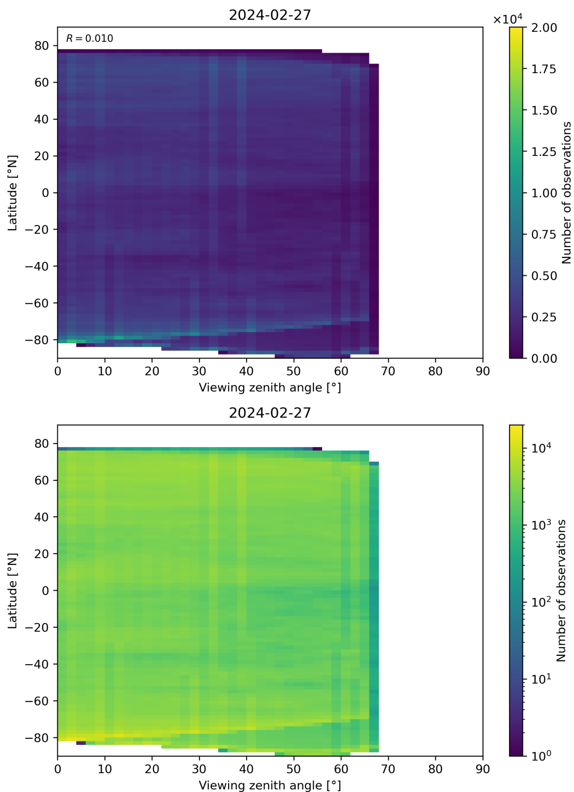
Figure 74: Scatter density plot of “Viewing zenith angle” against “Latitude” for 2024-02-27 to 2024-02-28.
