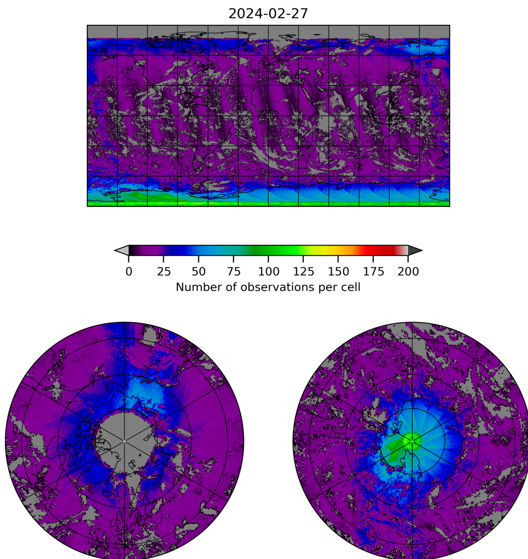
Figure 8: Map of the number of observations for 2024-02-27 to 2024-02-28
