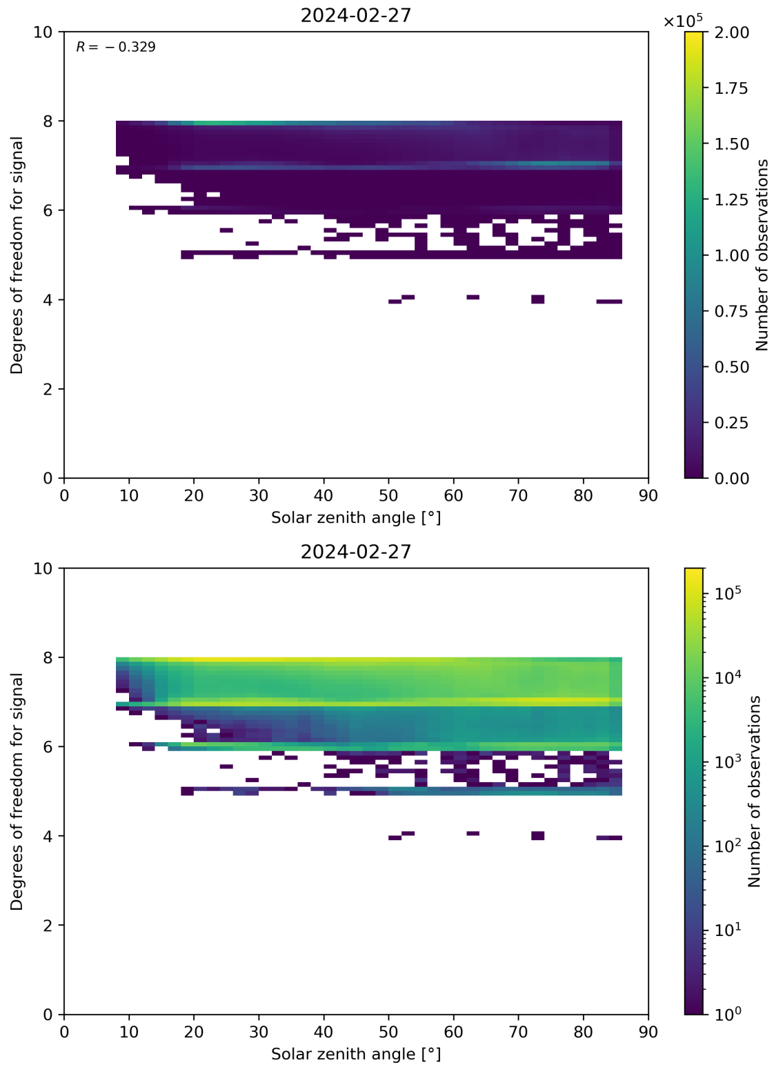
Figure 65: Scatter density plot of “Solar zenith angle” against “Degrees of freedom for signal” for 2024-02-27 to 2024-02-28.
