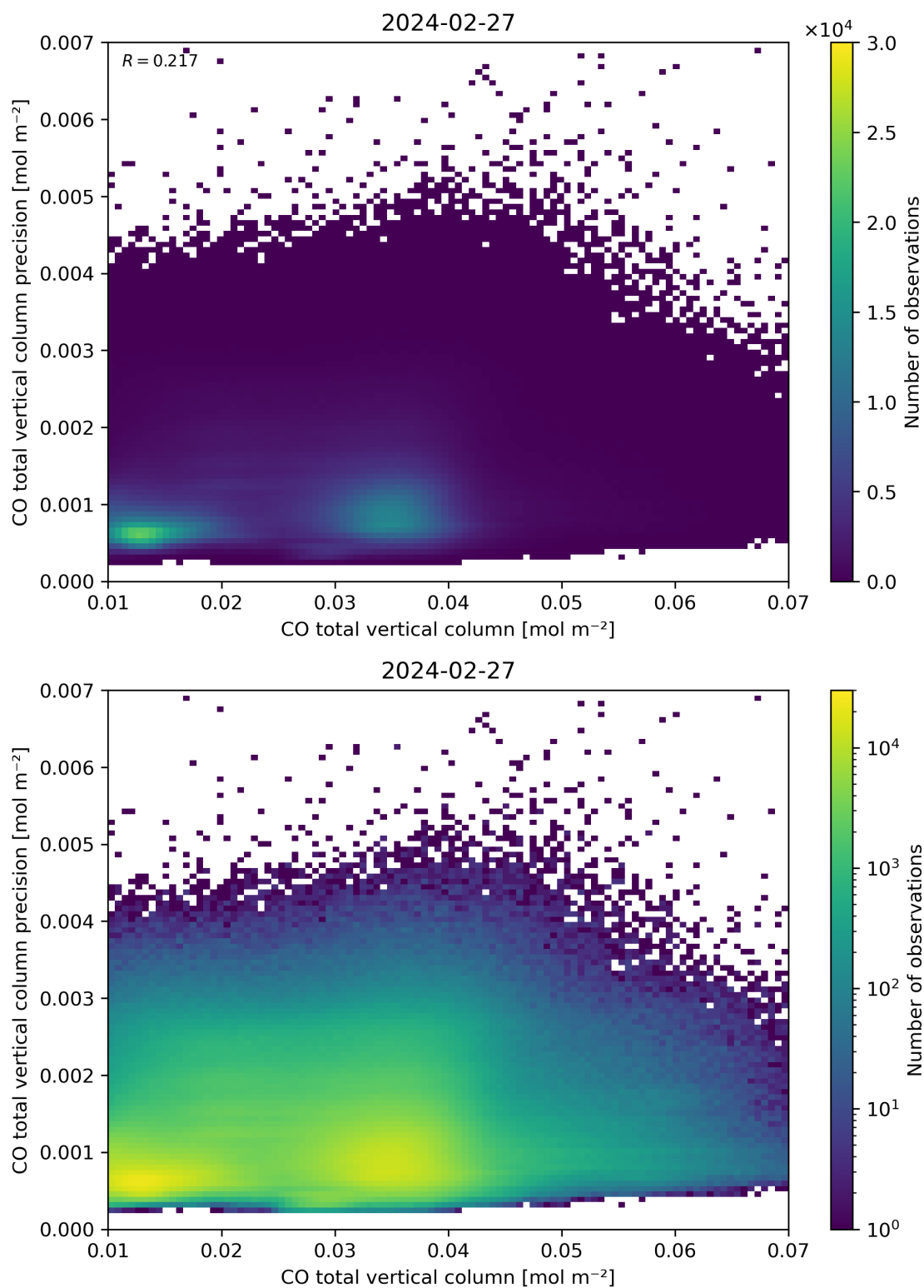
Figure 34: Scatter density plot of “CO total vertical column” against “CO total vertical column precision” for 2024-02-27 to 2024-02-28.
