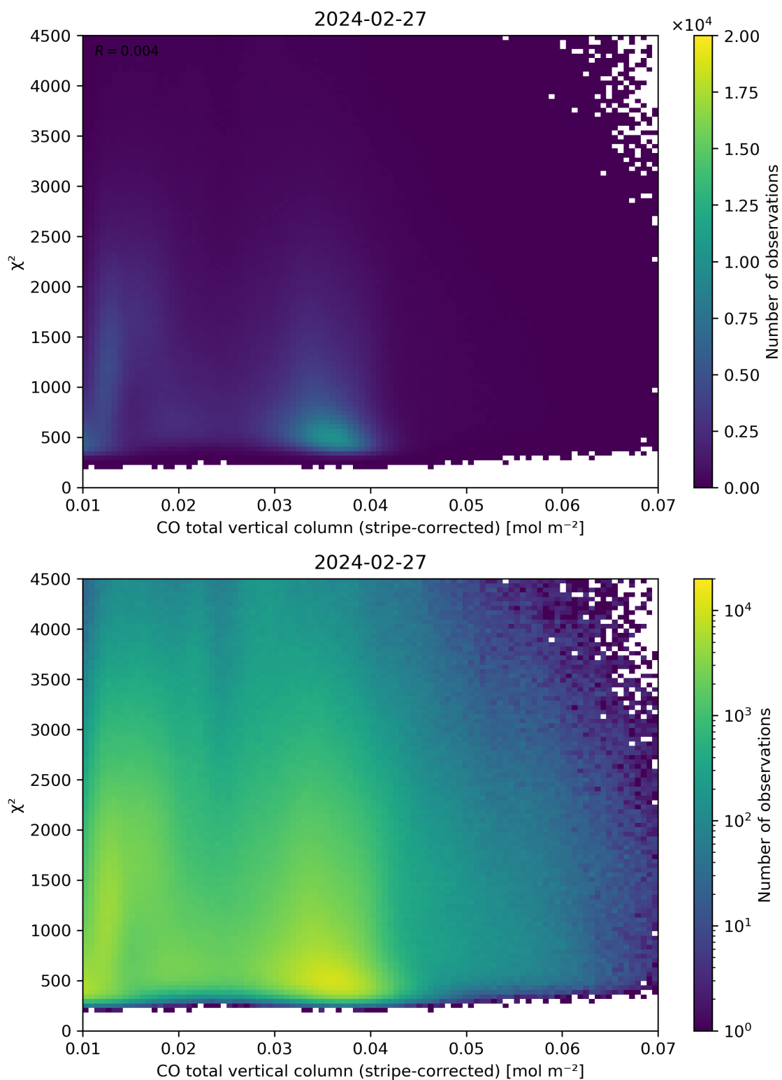
Figure 37: Scatter density plot of “CO total vertical column (stripe-corrected)” against “ \chi^2 ” for 2024-02-27 to 2024-02-28.
