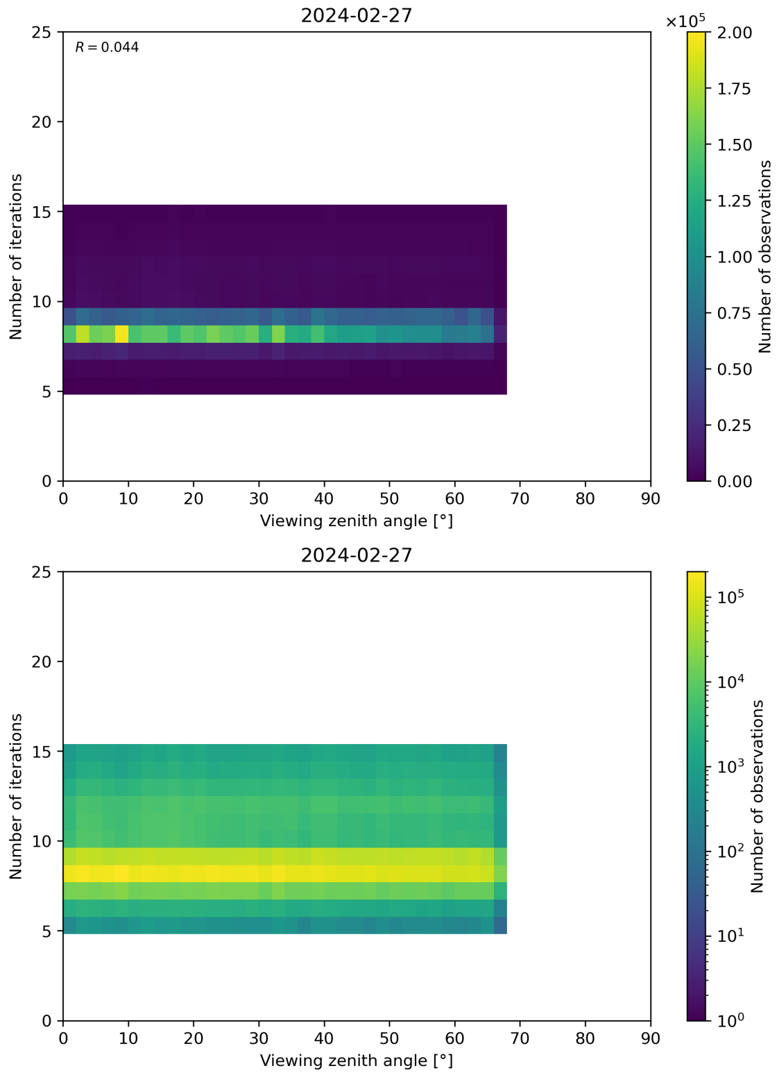
Figure 75: Scatter density plot of “Viewing zenith angle” against “Number of iterations” for 2024-02-27 to 2024-02-28.
