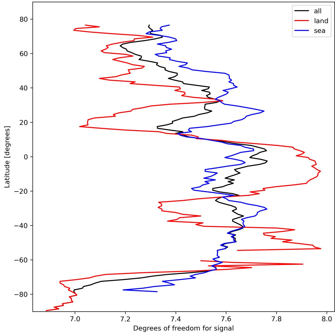
Figure 15: Zonal average of “Degrees of freedom for signal” for 2024-02-27 to 2024-02-28.
