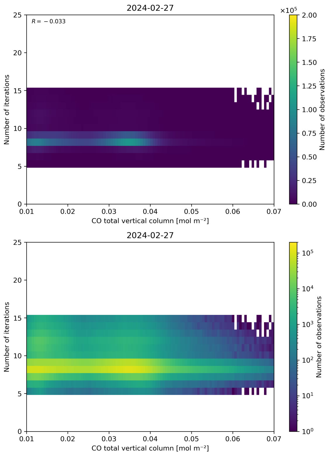
Figure 42: Scatter density plot of “CO total vertical column” against “Number of iterations” for 2024-02-27 to 2024-02-28.
