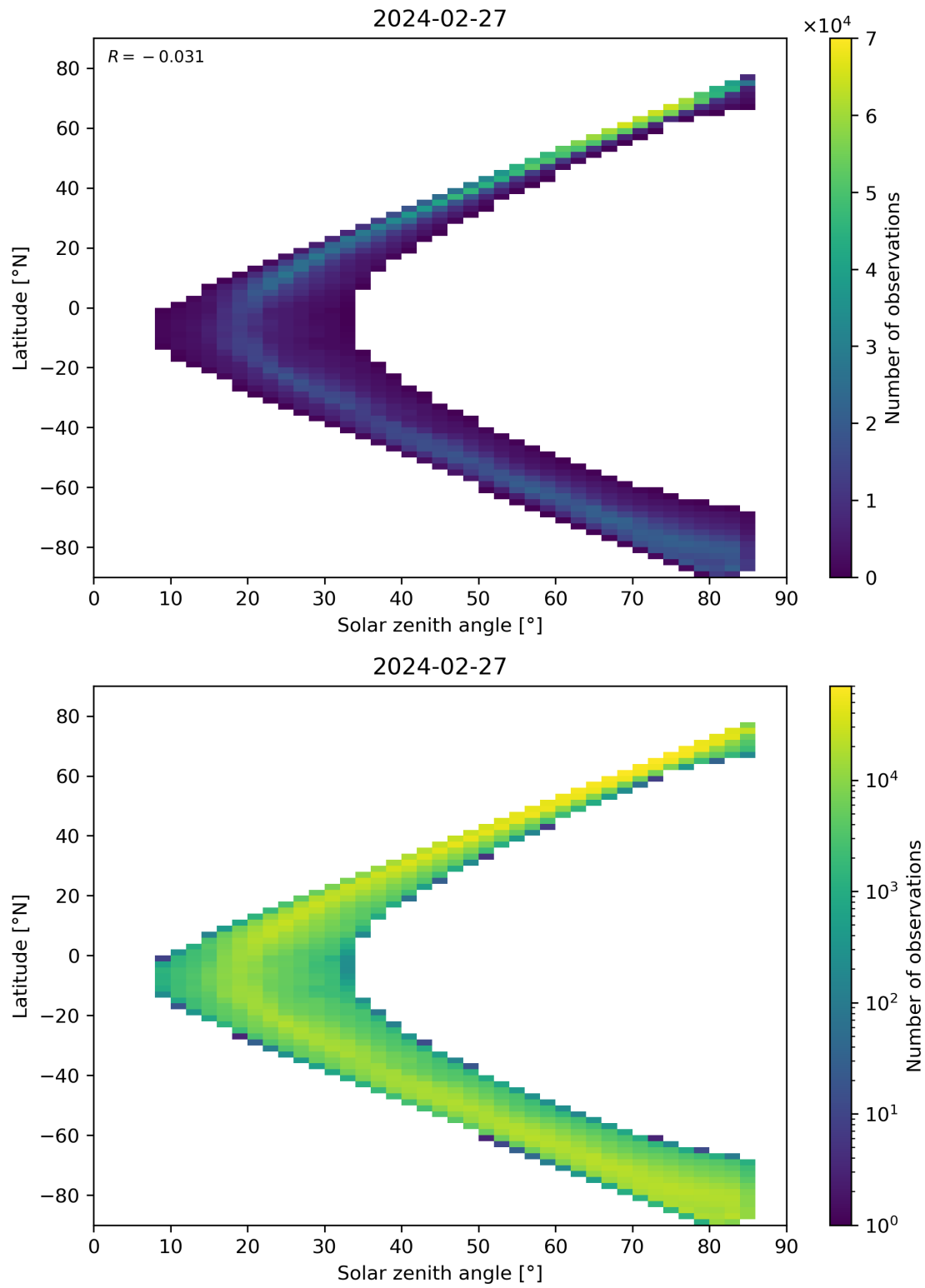
Figure 66: Scatter density plot of “Solar zenith angle” against “Latitude” for 2024-02-27 to 2024-02-28.
