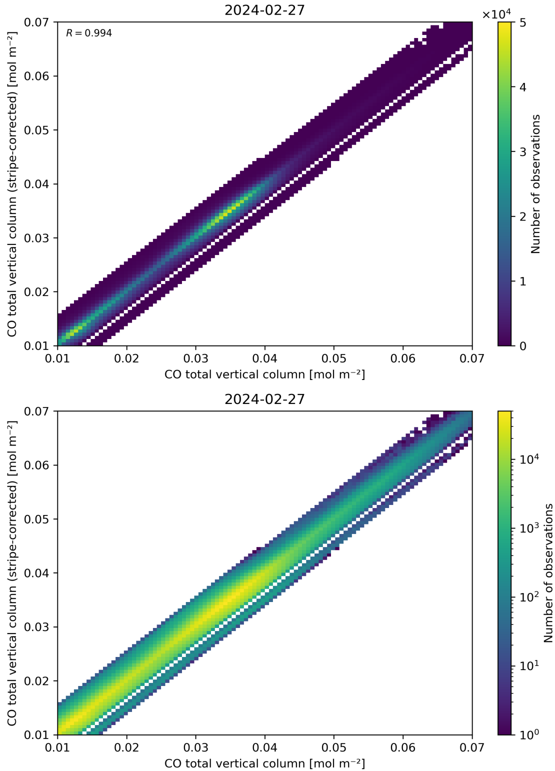
Figure 33: Scatter density plot of “CO total vertical column” against “CO total vertical column (stripe-corrected)” for 2024-02-27 to 2024-02-28.
