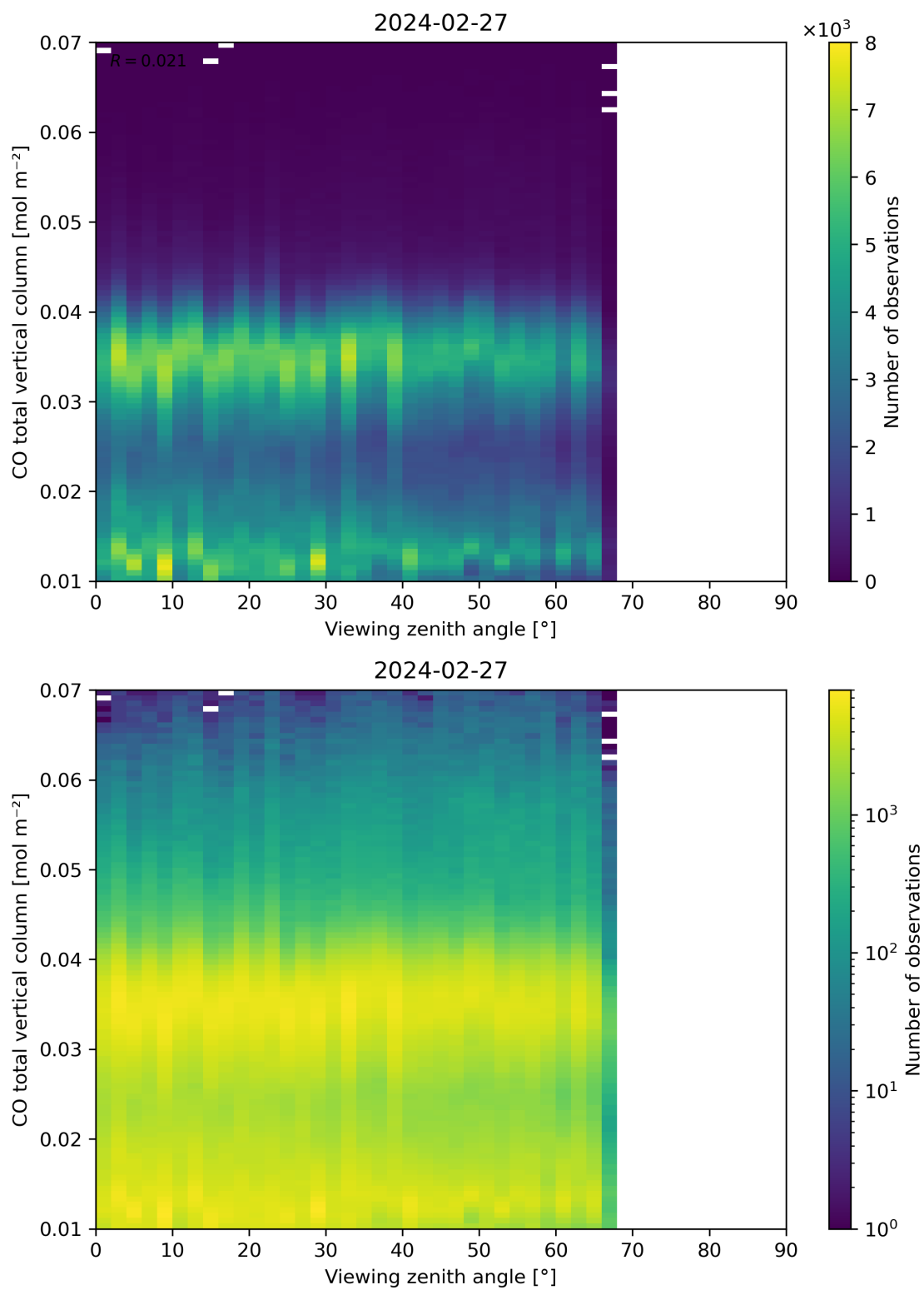
Figure 69: Scatter density plot of “Viewing zenith angle” against “CO total vertical column” for 2024-02-27 to 2024-02-28.
