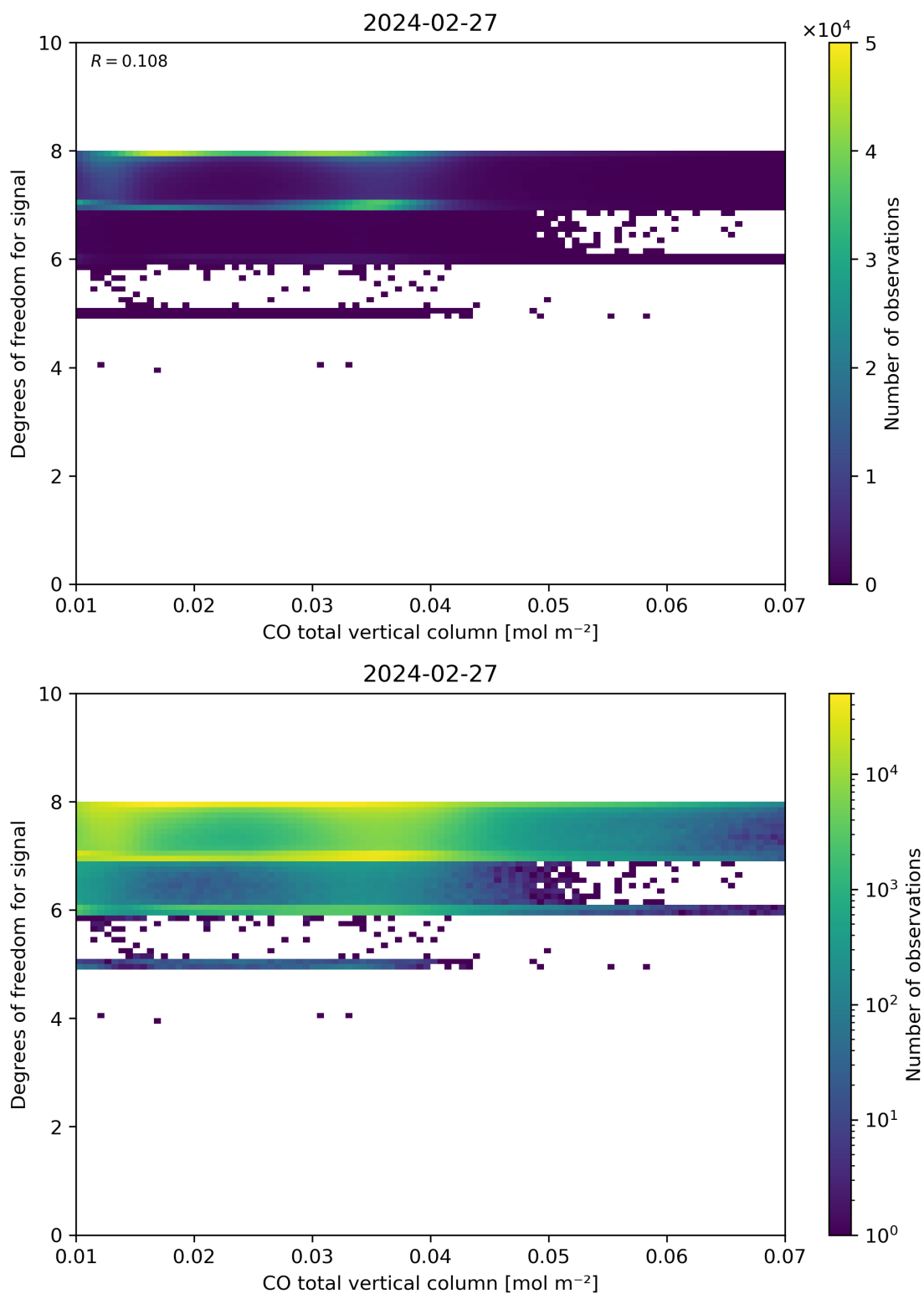
Figure 41: Scatter density plot of “CO total vertical column” against “Degrees of freedom for signal” for 2024-02-27 to 2024-02-28.
