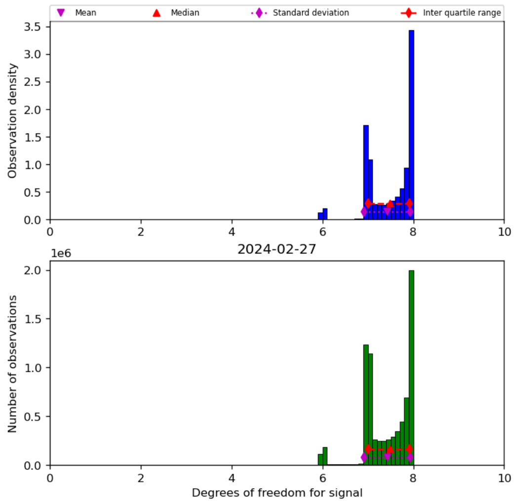
Figure 23: Histogram of “Degrees of freedom for signal” for 2024-02-27 to 2024-02-28
