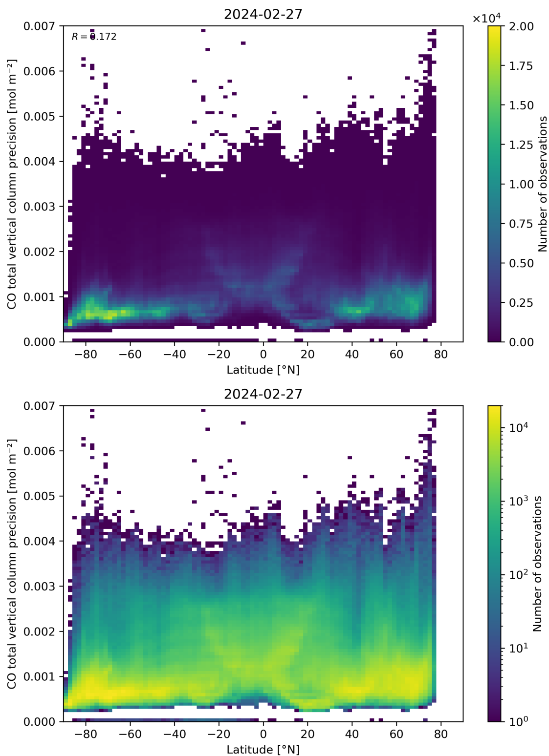
Figure 53: Scatter density plot of “Latitude” against “CO total vertical column precision” for 2024-02-27 to 2024-02-28.
