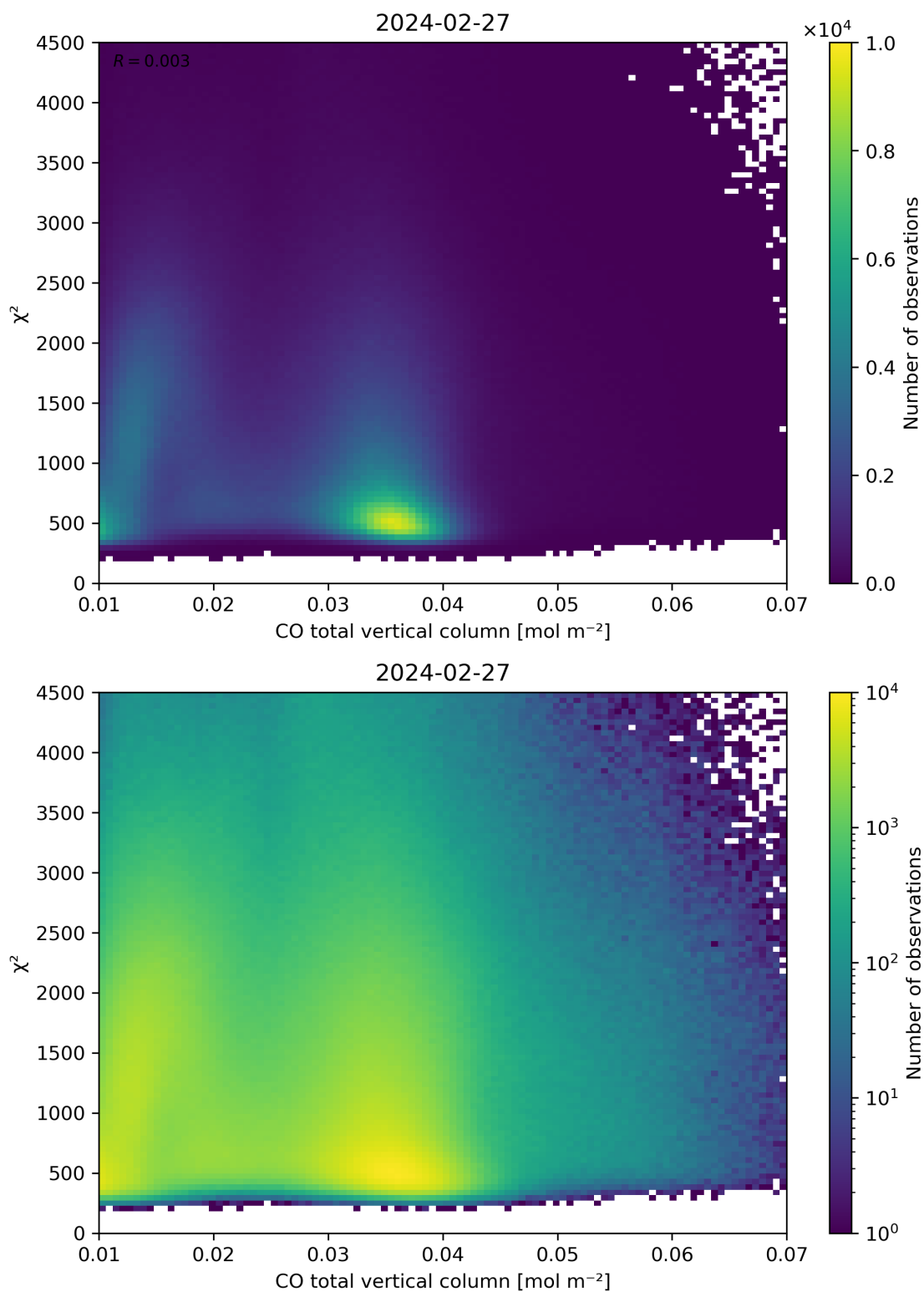
Figure 35: Scatter density plot of “CO total vertical column” against “ \chi^2 ” for 2024-02-27 to 2024-02-28.
