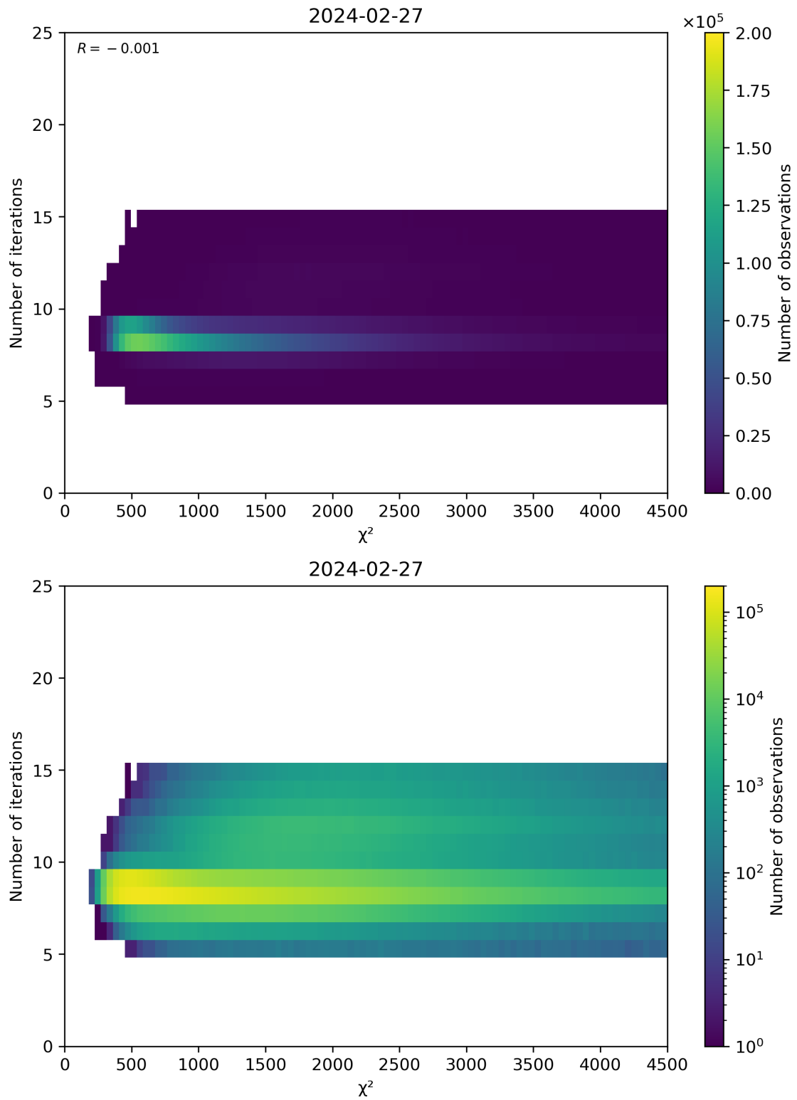
Figure 49: Scatter density plot of “ \chi^2 ” against “Number of iterations” for 2024-02-27 to 2024-02-28.
