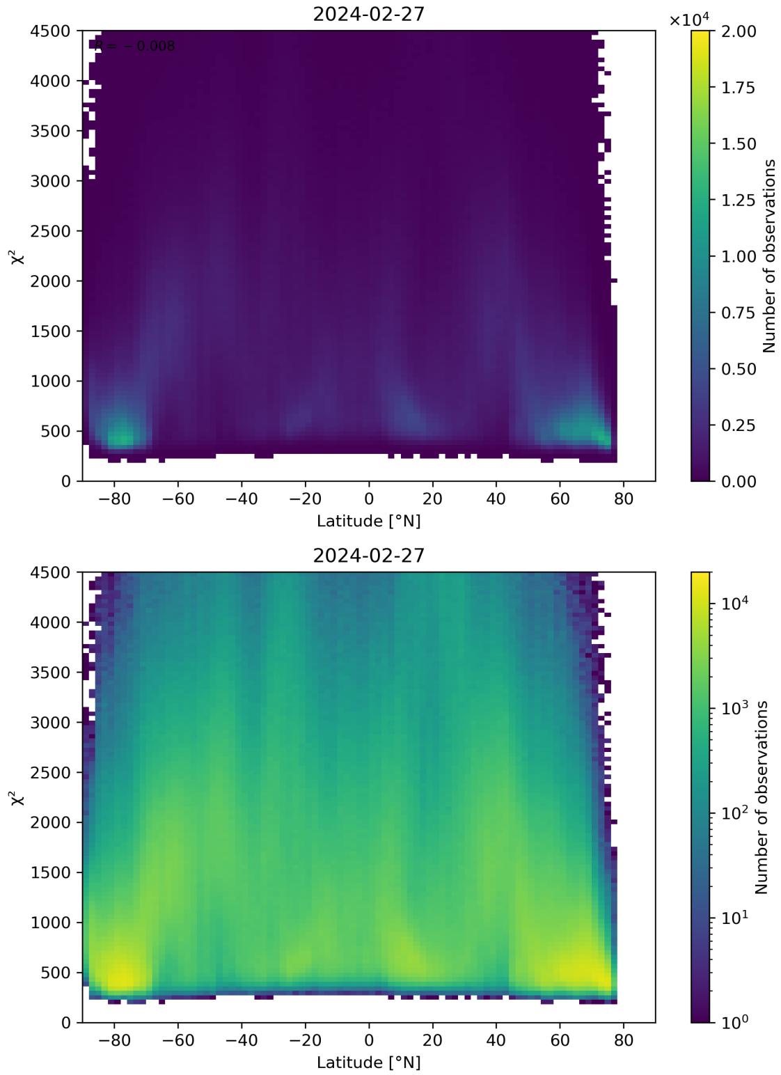
Figure 54: Scatter density plot of “Latitude” against “ \chi^2 ” for 2024-02-27 to 2024-02-28.
