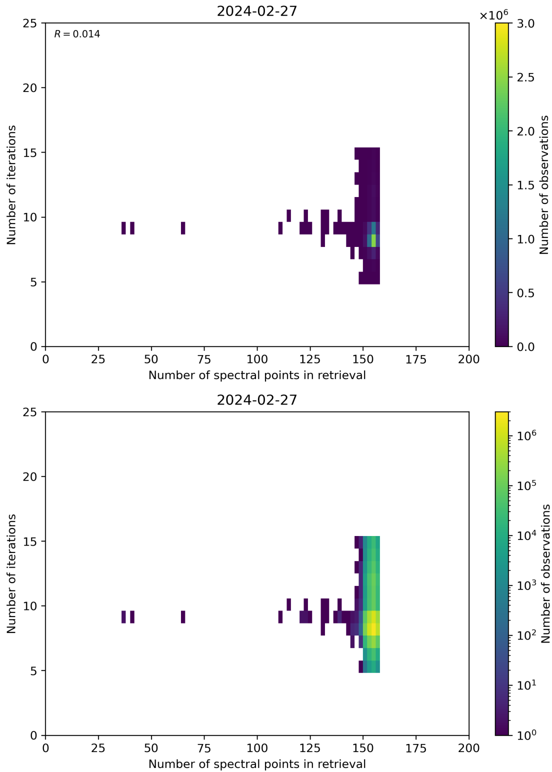
Figure 60: Scatter density plot of “Number of spectral points in retrieval” against “Number of iterations” for 2024-02-27 to 2024-02-28.
