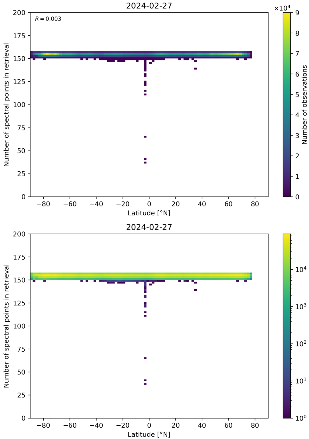
Figure 57: Scatter density plot of “Latitude” against “Number of spectral points in retrieval” for 2024-02-27 to 2024-02-28.
