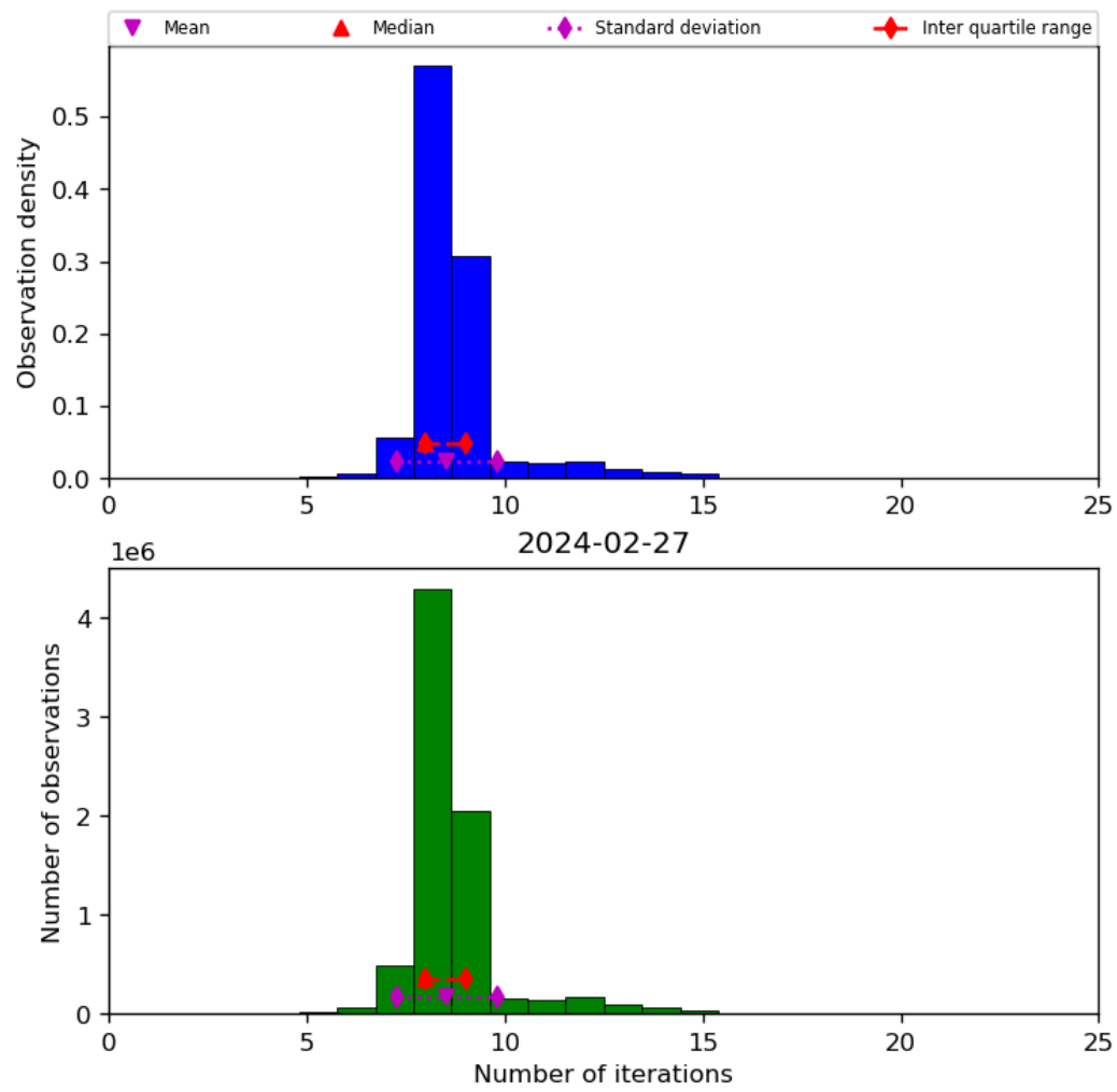
Figure 24: Histogram of “Number of iterations” for 2024-02-27 to 2024-02-28
