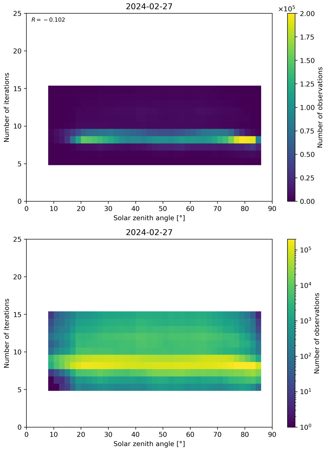
Figure 67: Scatter density plot of “Solar zenith angle” against “Number of iterations” for 2024-02-27 to 2024-02-28.
