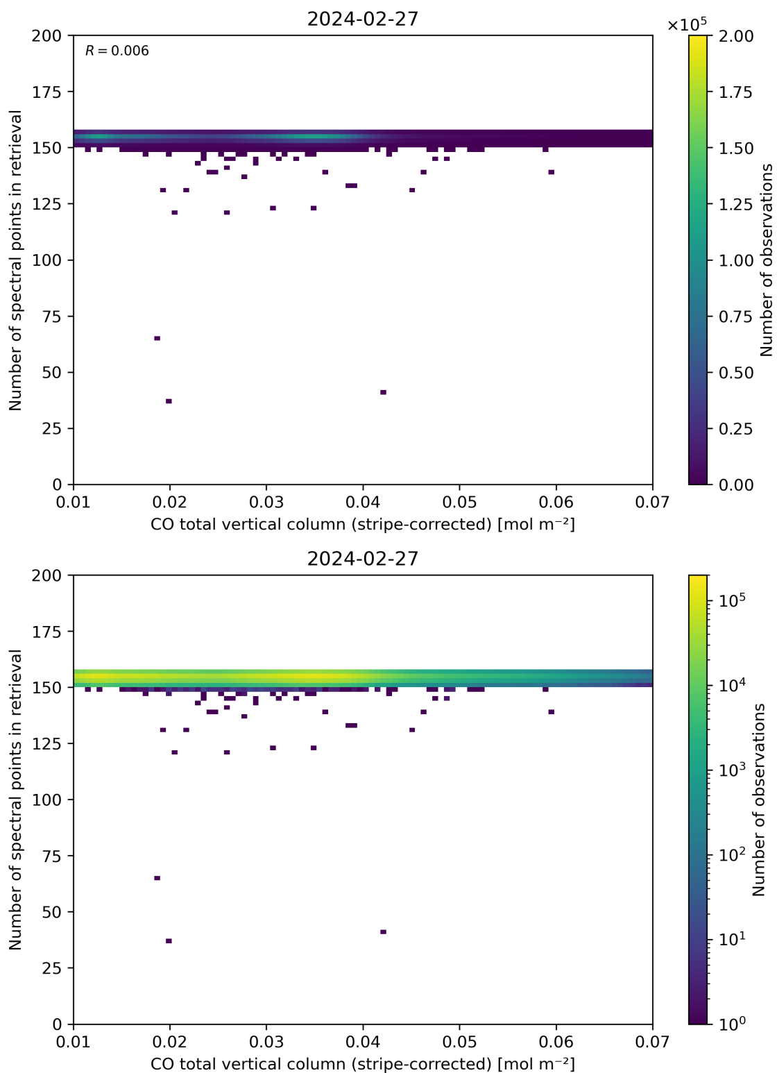
Figure 40: Scatter density plot of “CO total vertical column (stripe-corrected)” against “Number of spectral points in retrieval” for 2024-02-27 to 2024-02-28.
