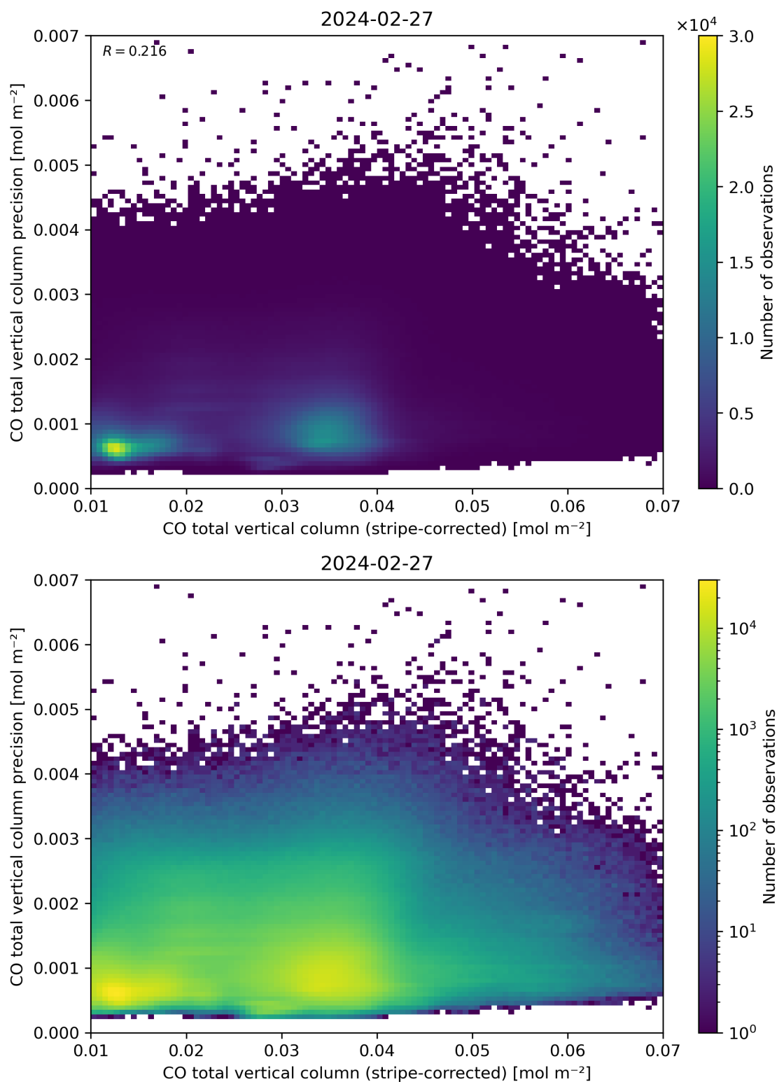
Figure 36: Scatter density plot of “CO total vertical column (stripe-corrected)” against “CO total vertical column precision” for 2024-02-27 to 2024-02-28.
