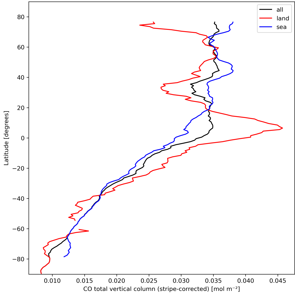
Figure 11: Zonal average of “CO total vertical column (stripe-corrected)” for 2024-02-27 to 2024-02-28.
