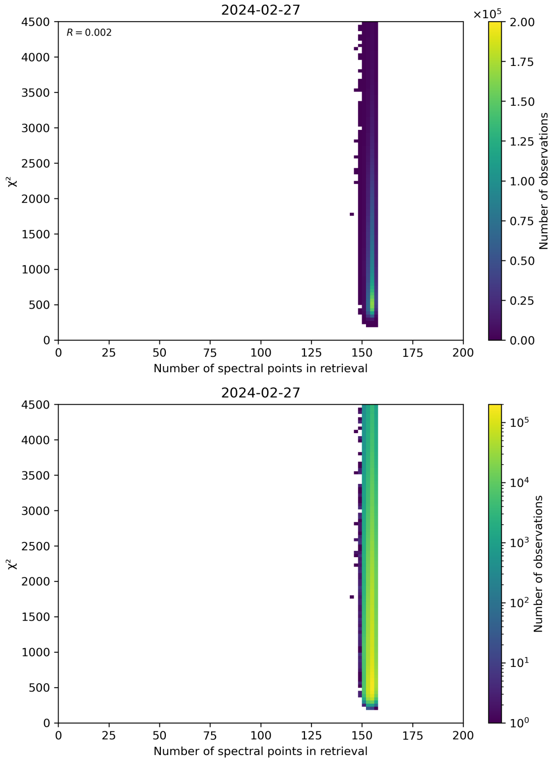
Figure 58: Scatter density plot of “Number of spectral points in retrieval” against “ \chi^2 ” for 2024-02-27 to 2024-02-28.
