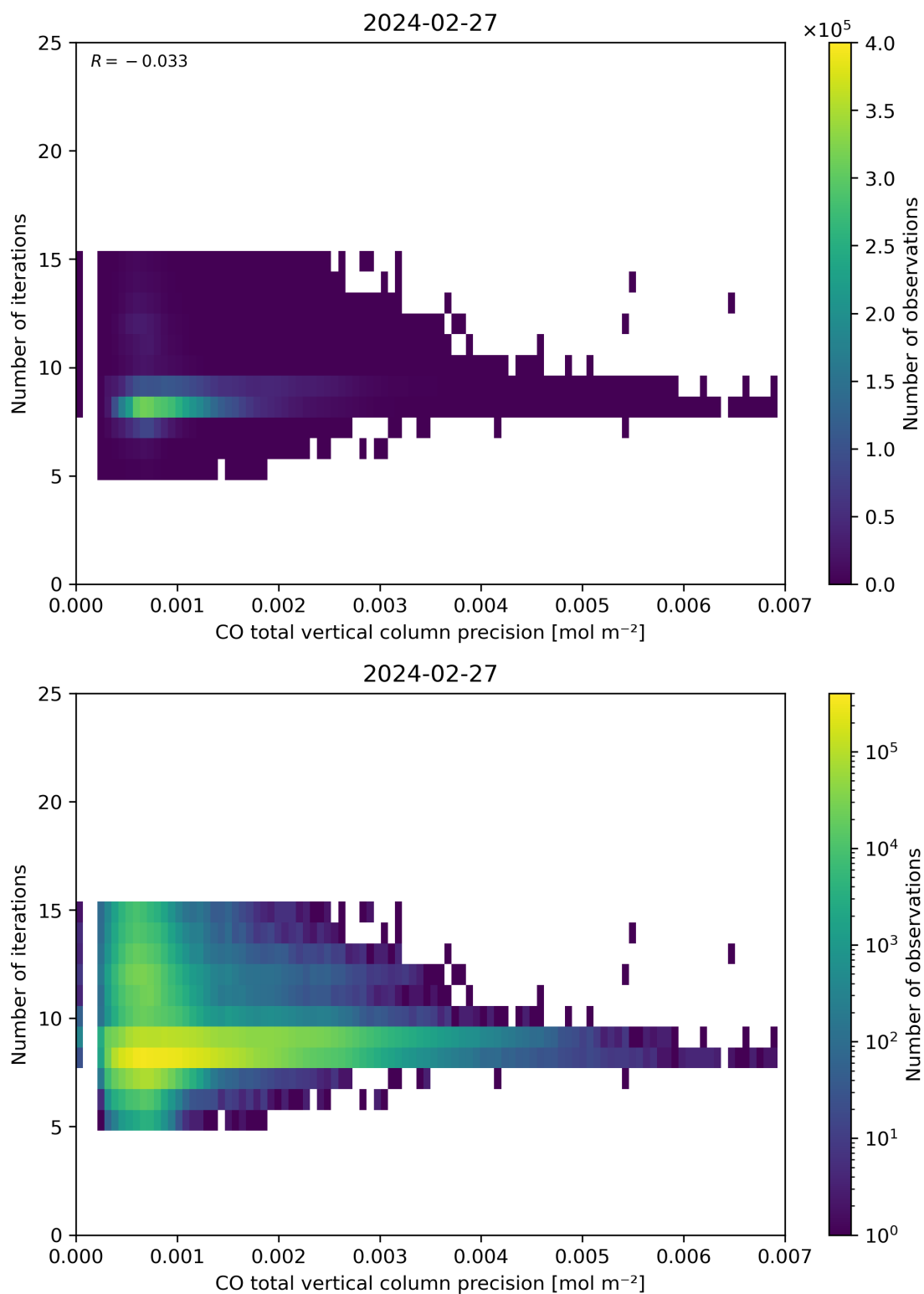
Figure 46: Scatter density plot of “CO total vertical column precision” against “Number of iterations” for 2024-02-27 to 2024-02-28.
