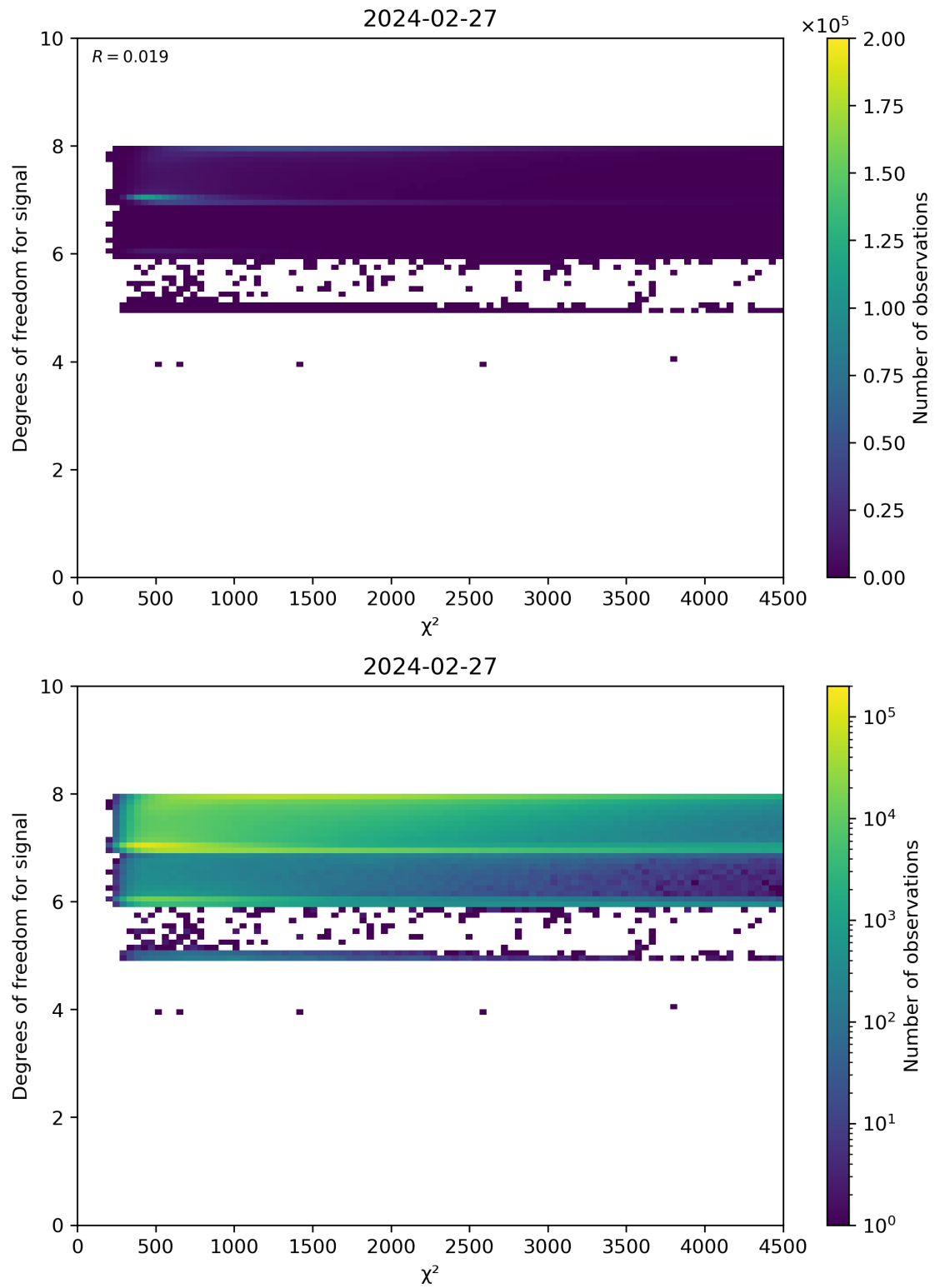
Figure 48: Scatter density plot of “ \chi^2 ” against “Degrees of freedom for signal” for 2024-02-27 to 2024-02-28.
