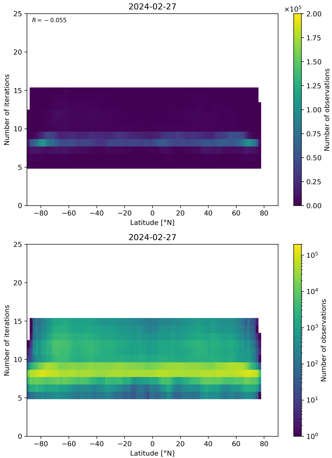
Figure 56: Scatter density plot of “Latitude” against “Number of iterations” for 2024-02-27 to 2024-02-28.
