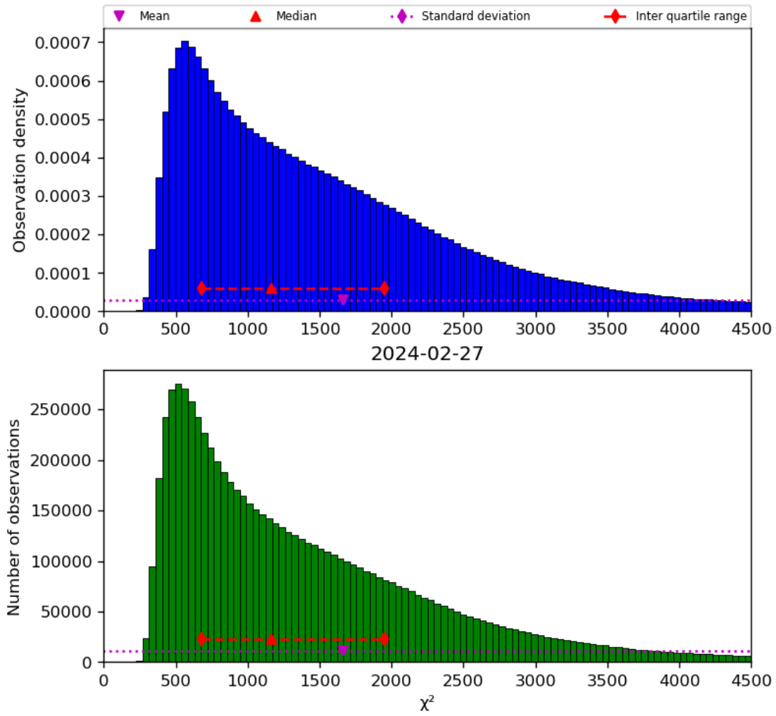
Figure 22: Histogram of “ \chi^2 ” for 2024-02-27 to 2024-02-28
