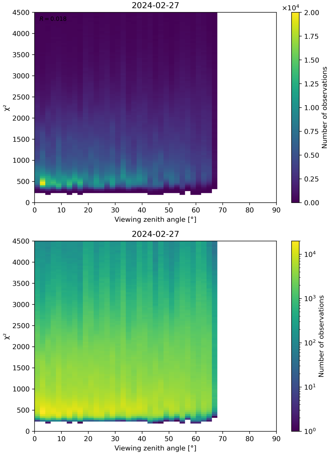
Figure 72: Scatter density plot of “Viewing zenith angle” against “ \chi^2 ” for 2024-02-27 to 2024-02-28.
