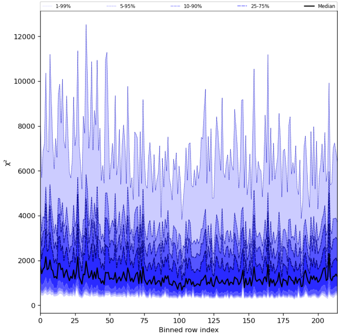
Figure 30: Along track statistics of “ \chi^2 ” for 2024-02-27 to 2024-02-28
