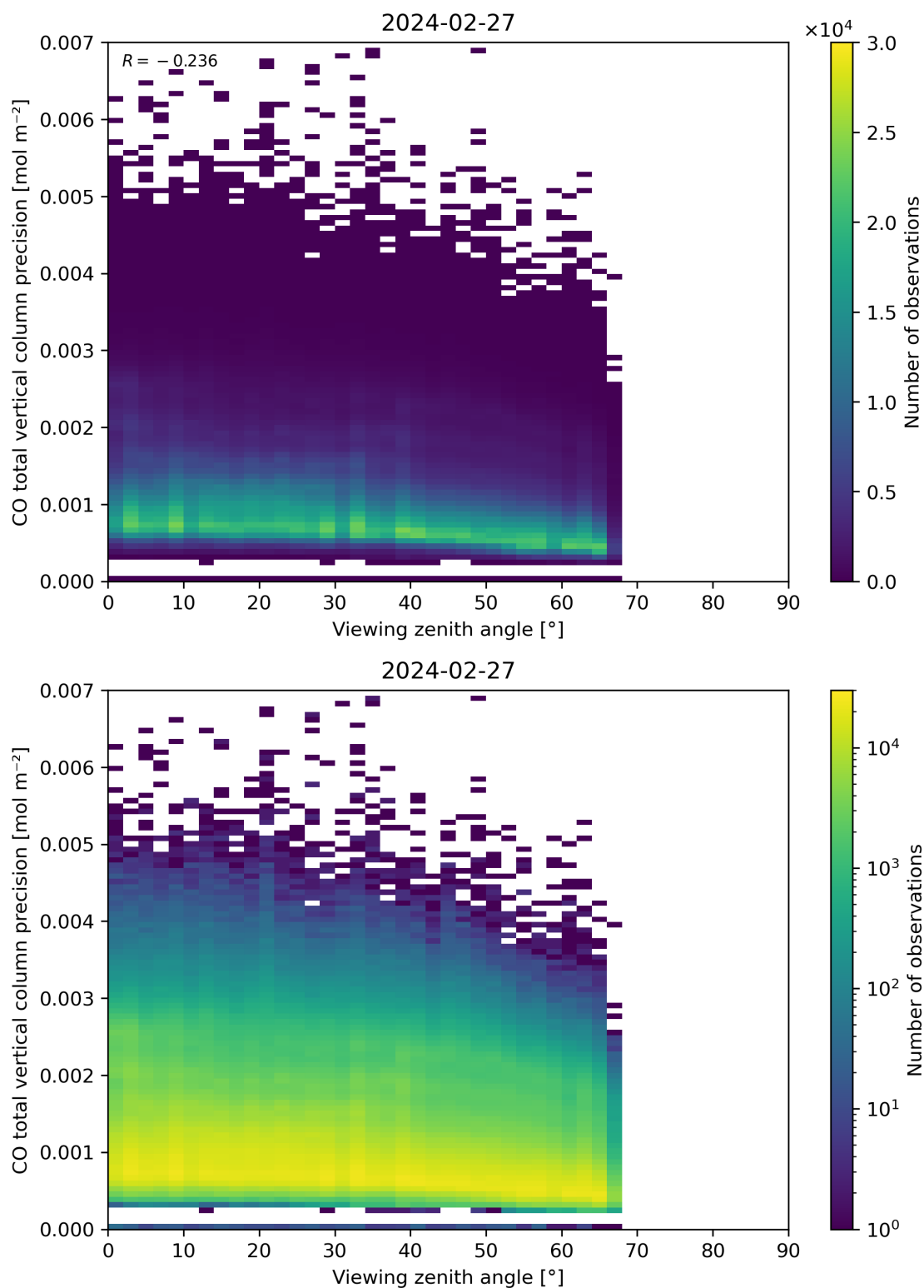
Figure 71: Scatter density plot of “Viewing zenith angle” against “CO total vertical column precision” for 2024-02-27 to 2024-02-28.
