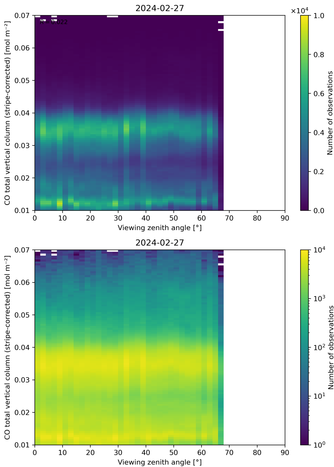
Figure 70: Scatter density plot of “Viewing zenith angle” against “CO total vertical column (stripe-corrected)” for 2024-02-27 to 2024-02-28.
