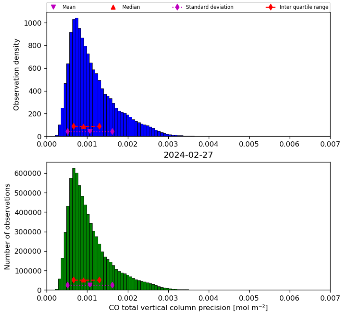
Figure 20: Histogram of “CO total vertical column precision” for 2024-02-27 to 2024-02-28
