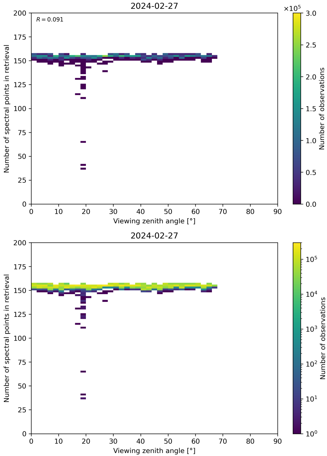
Figure 76: Scatter density plot of “Viewing zenith angle” against “Number of spectral points in retrieval” for 2024-02-27 to 2024-02-28.
