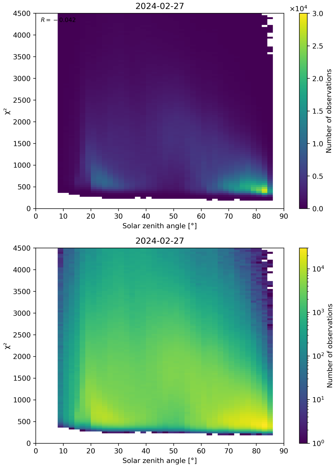
Figure 64: Scatter density plot of “Solar zenith angle” against “ \chi^2 ” for 2024-02-27 to 2024-02-28.
