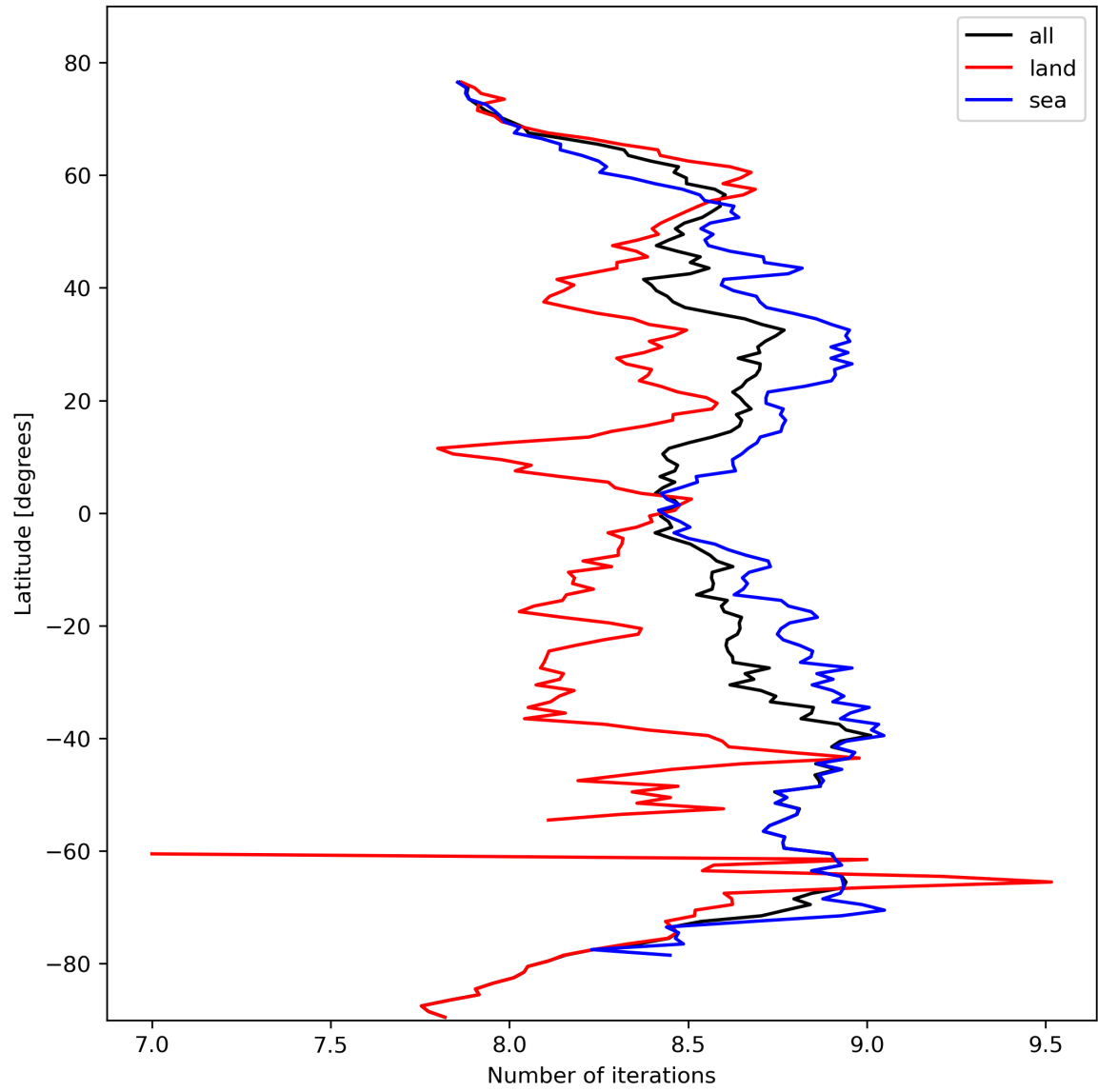
Figure 16: Zonal average of “Number of iterations” for 2024-02-27 to 2024-02-28.
