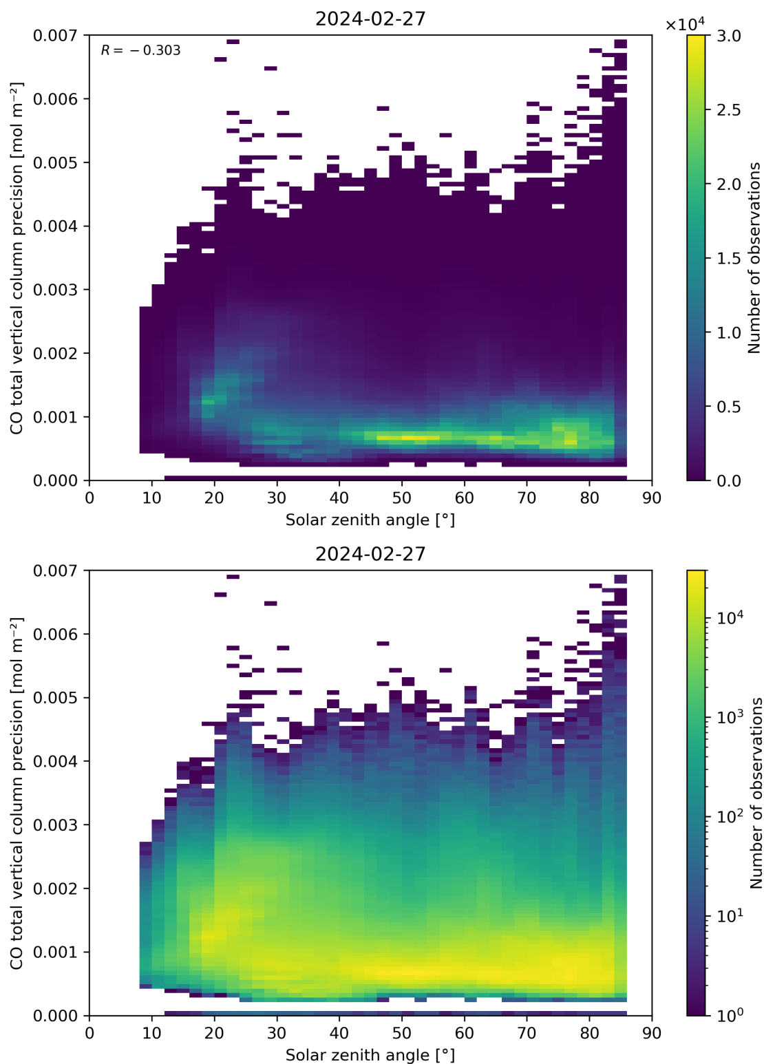
Figure 63: Scatter density plot of “Solar zenith angle” against “CO total vertical column precision” for 2024-02-27 to 2024-02-28.
