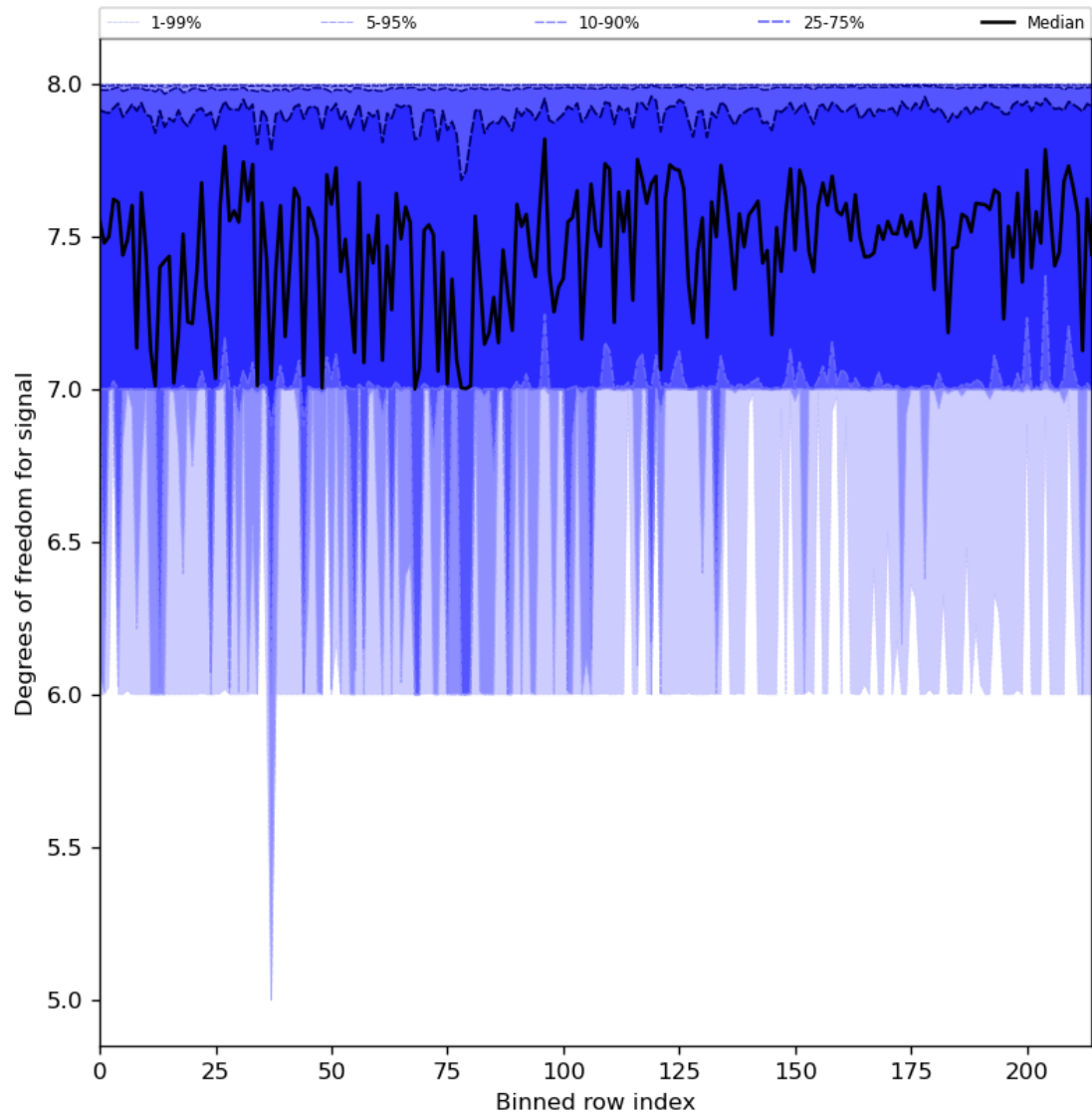
Figure 31: Along track statistics of “Degrees of freedom for signal” for 2024-02-27 to 2024-02-28
