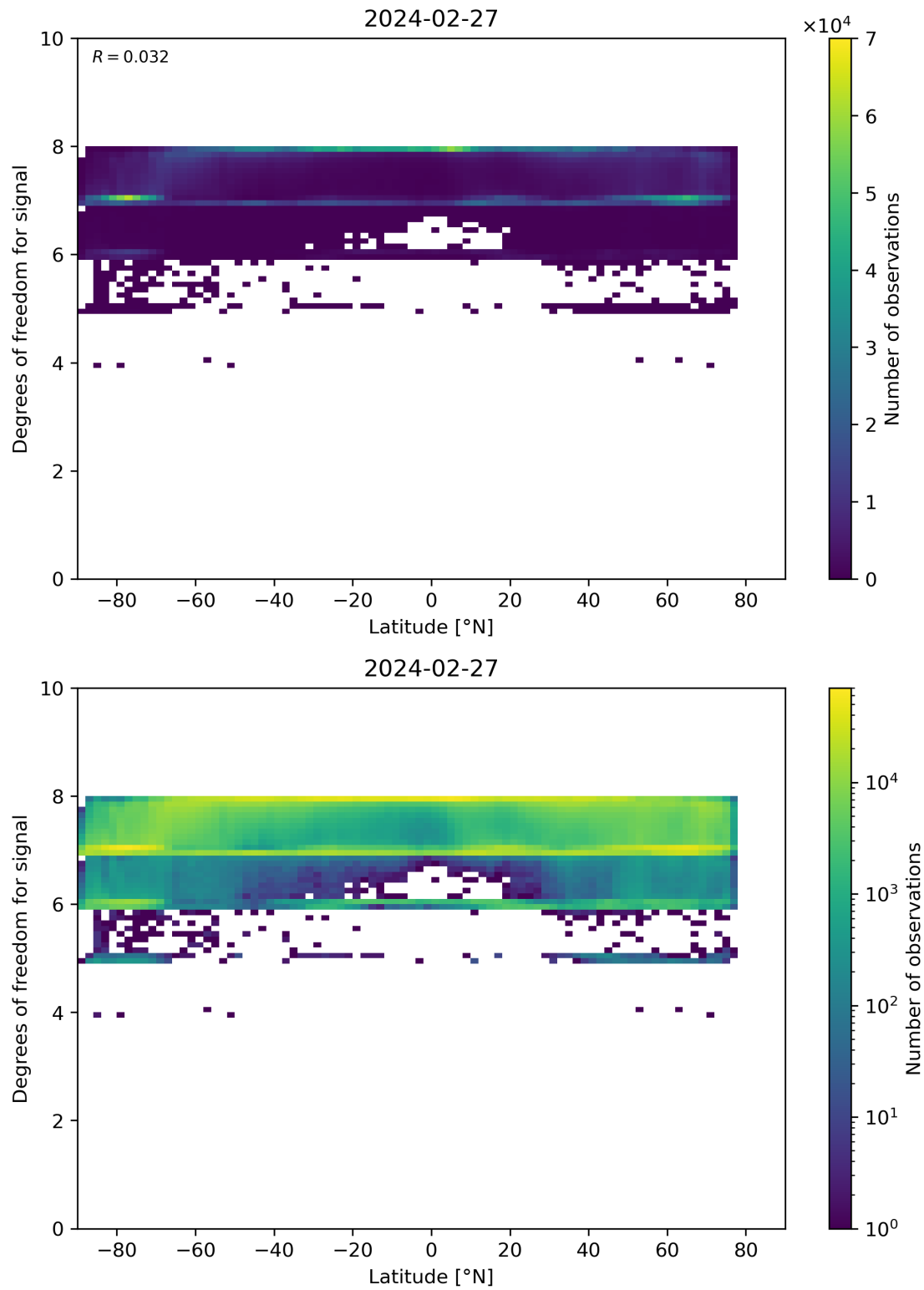
Figure 55: Scatter density plot of “Latitude” against “Degrees of freedom for signal” for 2024-02-27 to 2024-02-28.
