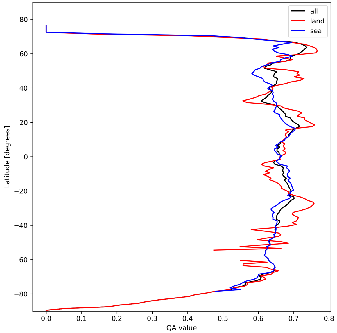
Figure 9: Zonal average of “QA value” for 2024-02-27 to 2024-02-28.
