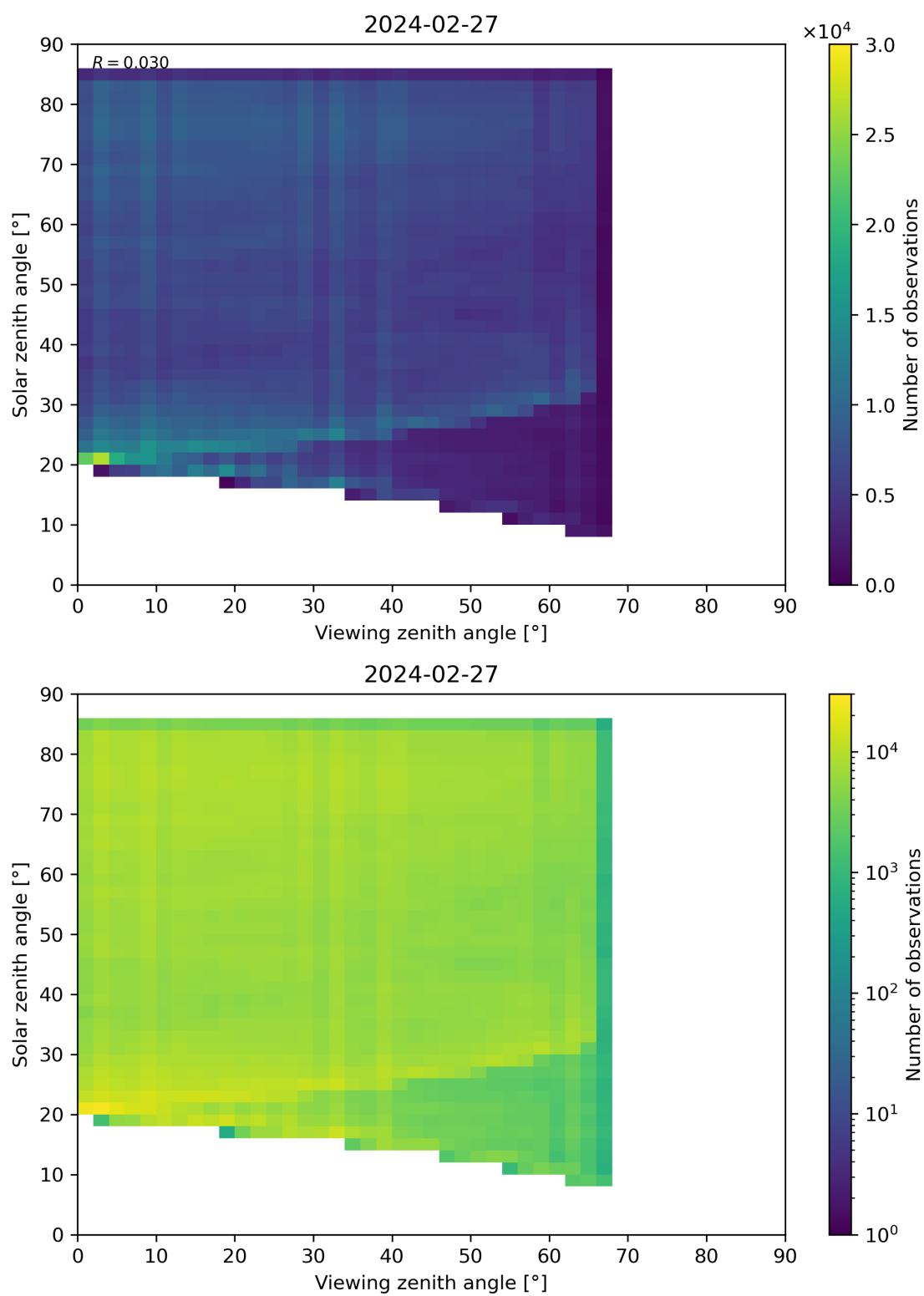
Figure 77: Scatter density plot of “Viewing zenith angle” against “Solar zenith angle” for 2024-02-27 to 2024-02-28.
