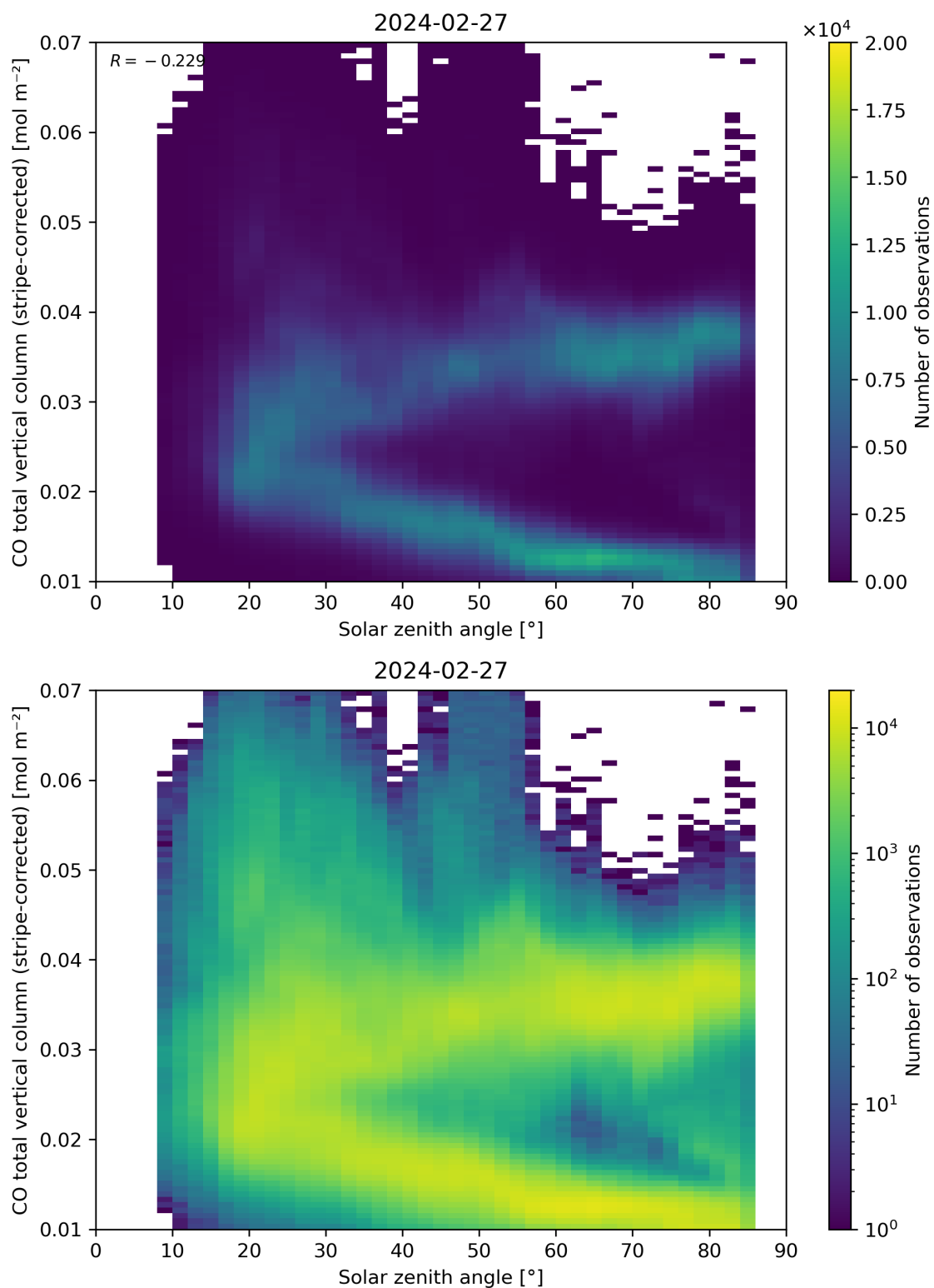
Figure 62: Scatter density plot of “Solar zenith angle” against “CO total vertical column (stripe-corrected)” for 2024-02-27 to 2024-02-28.
