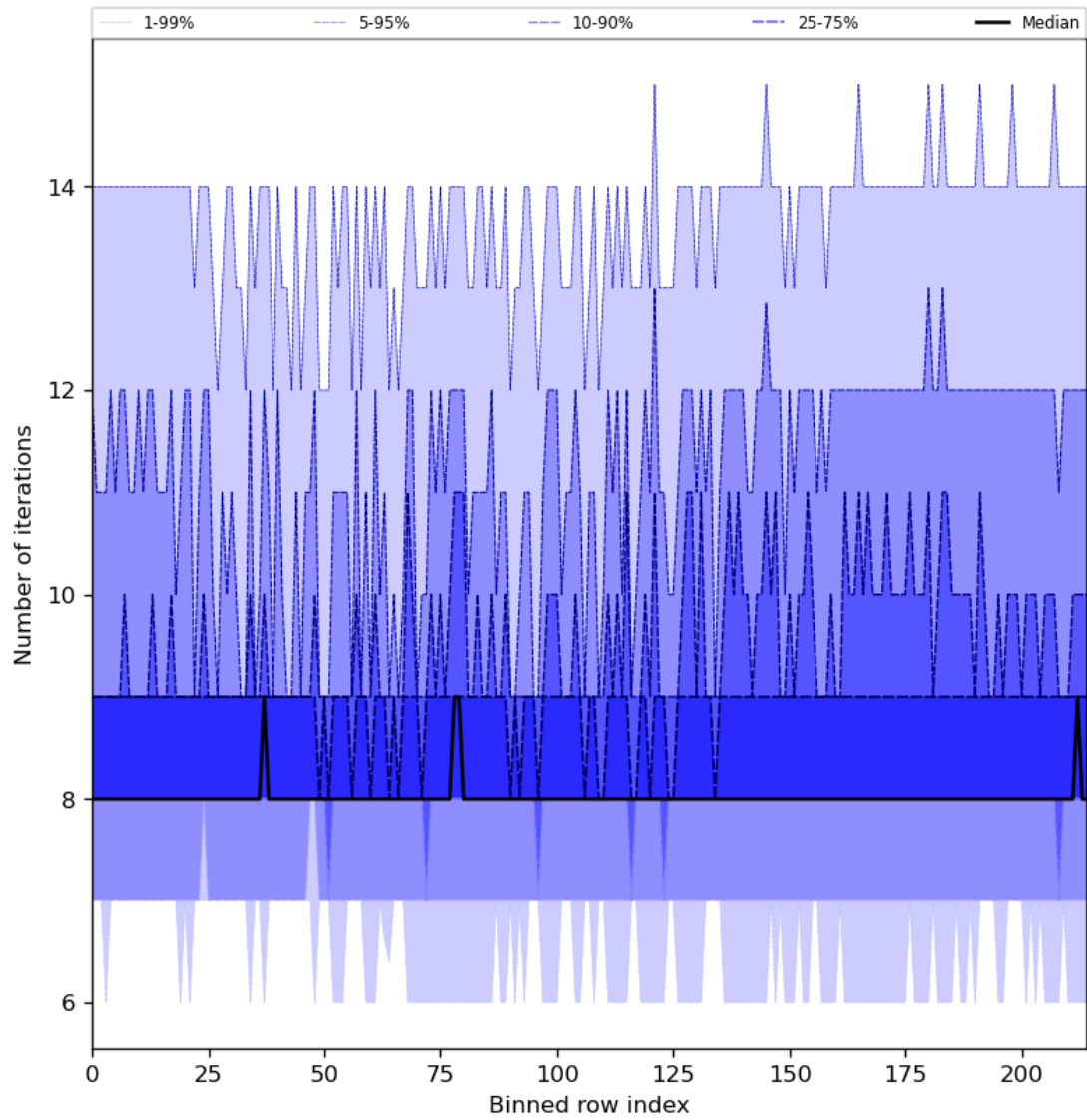
Figure 32: Along track statistics of “Number of iterations” for 2024-02-27 to 2024-02-28
