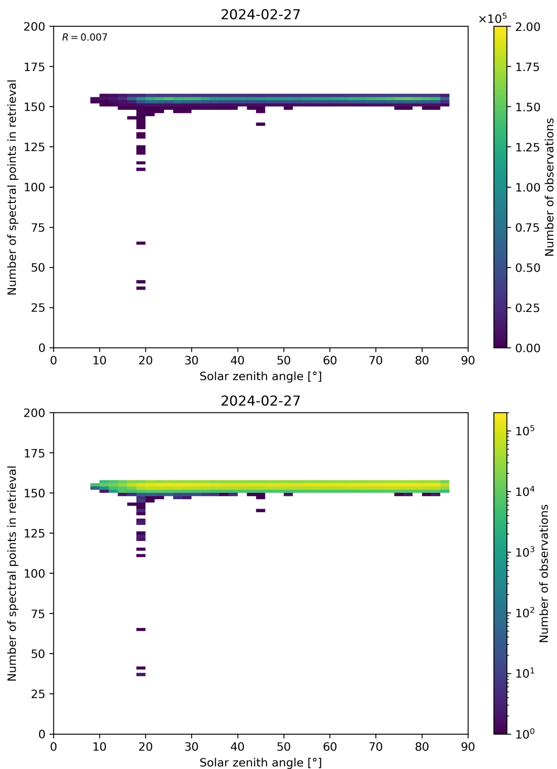
Figure 68: Scatter density plot of “Solar zenith angle” against “Number of spectral points in retrieval” for 2024-02-27 to 2024-02-28.
