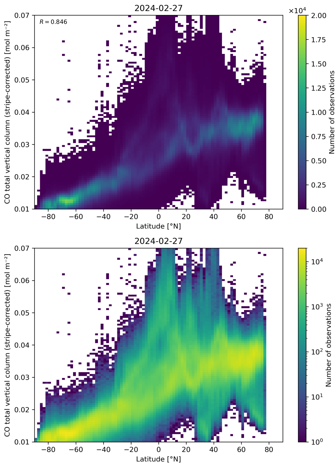
Figure 52: Scatter density plot of “Latitude” against “CO total vertical column (stripe-corrected)” for 2024-02-27 to 2024-02-28.
