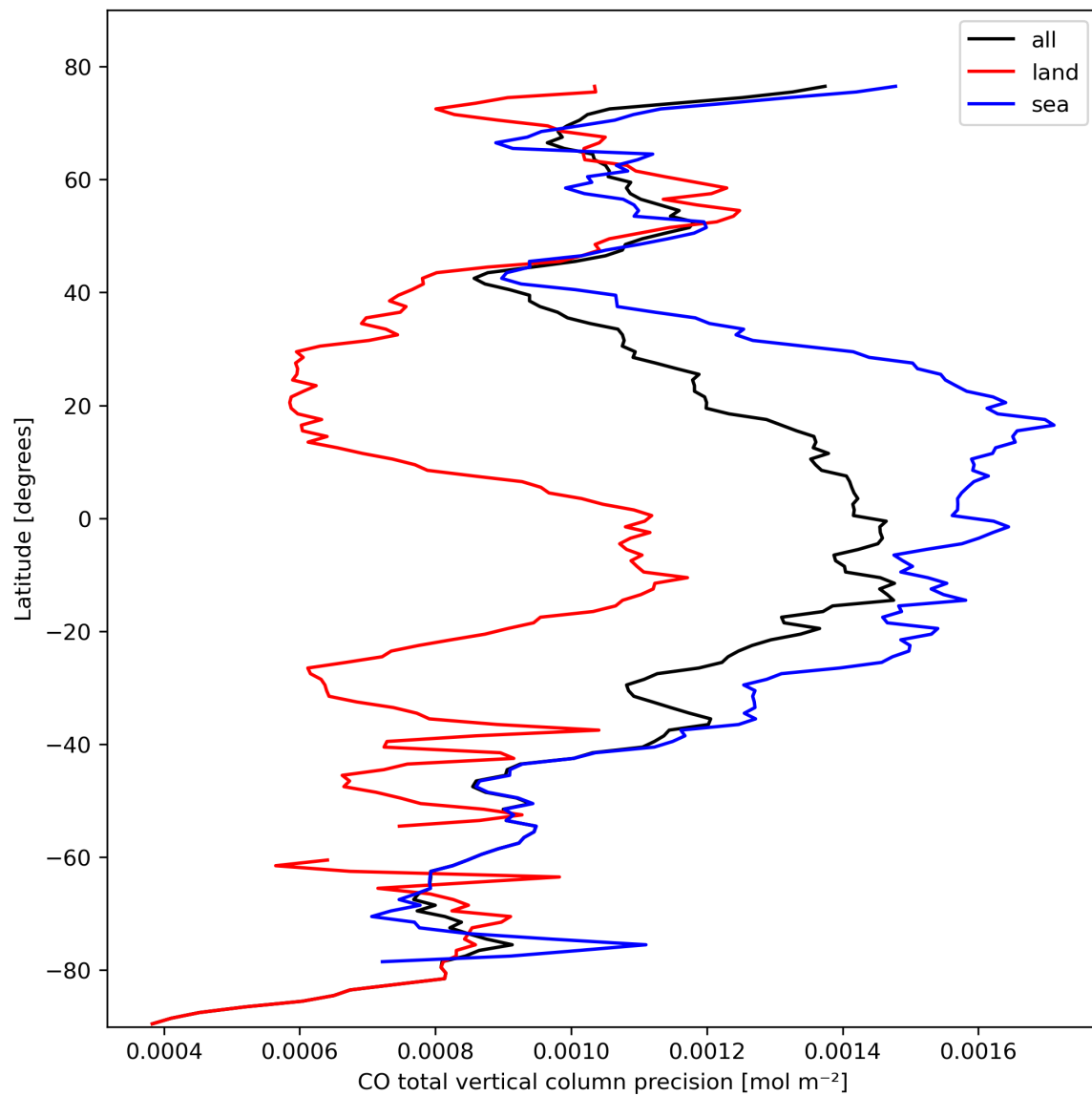
Figure 12: Zonal average of “CO total vertical column precision” for 2024-02-27 to 2024-02-28.
