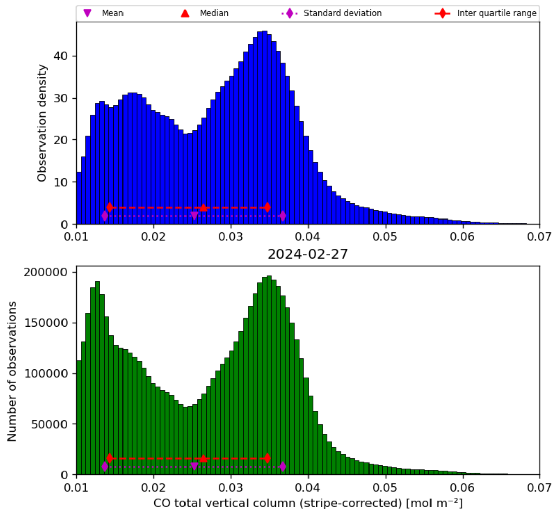
Figure 19: Histogram of “CO total vertical column (stripe-corrected)” for 2024-02-27 to 2024-02-28
