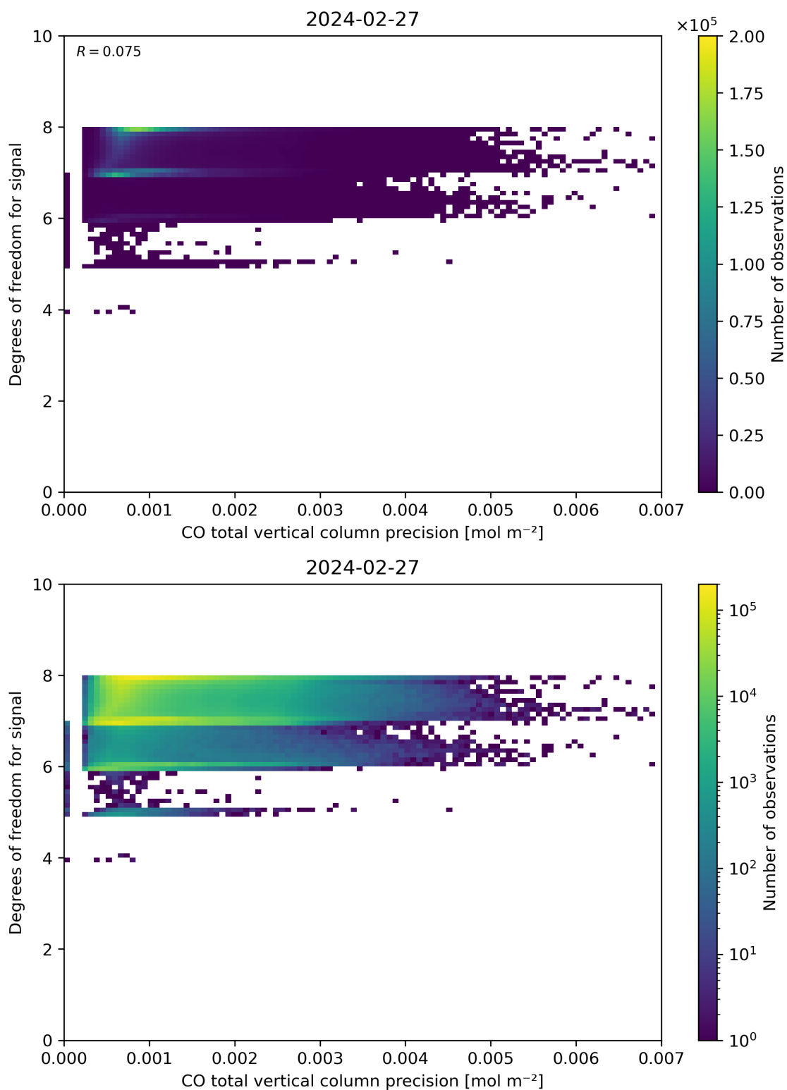
Figure 45: Scatter density plot of “CO total vertical column precision” against “Degrees of freedom for signal” for 2024-02-27 to 2024-02-28.
