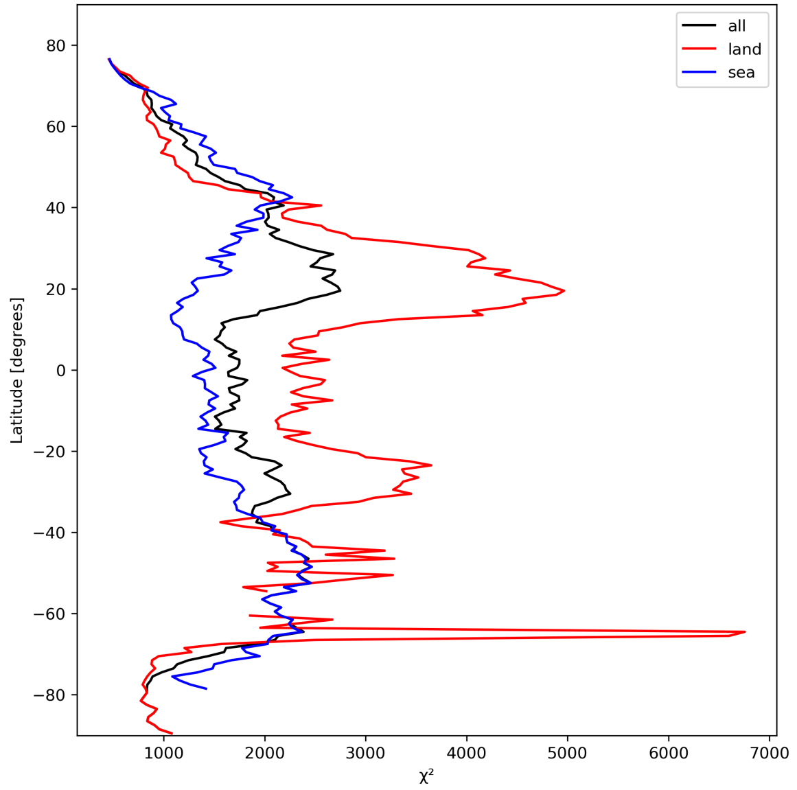
Figure 14: Zonal average of “ \chi^2 ” for 2024-02-27 to 2024-02-28.
