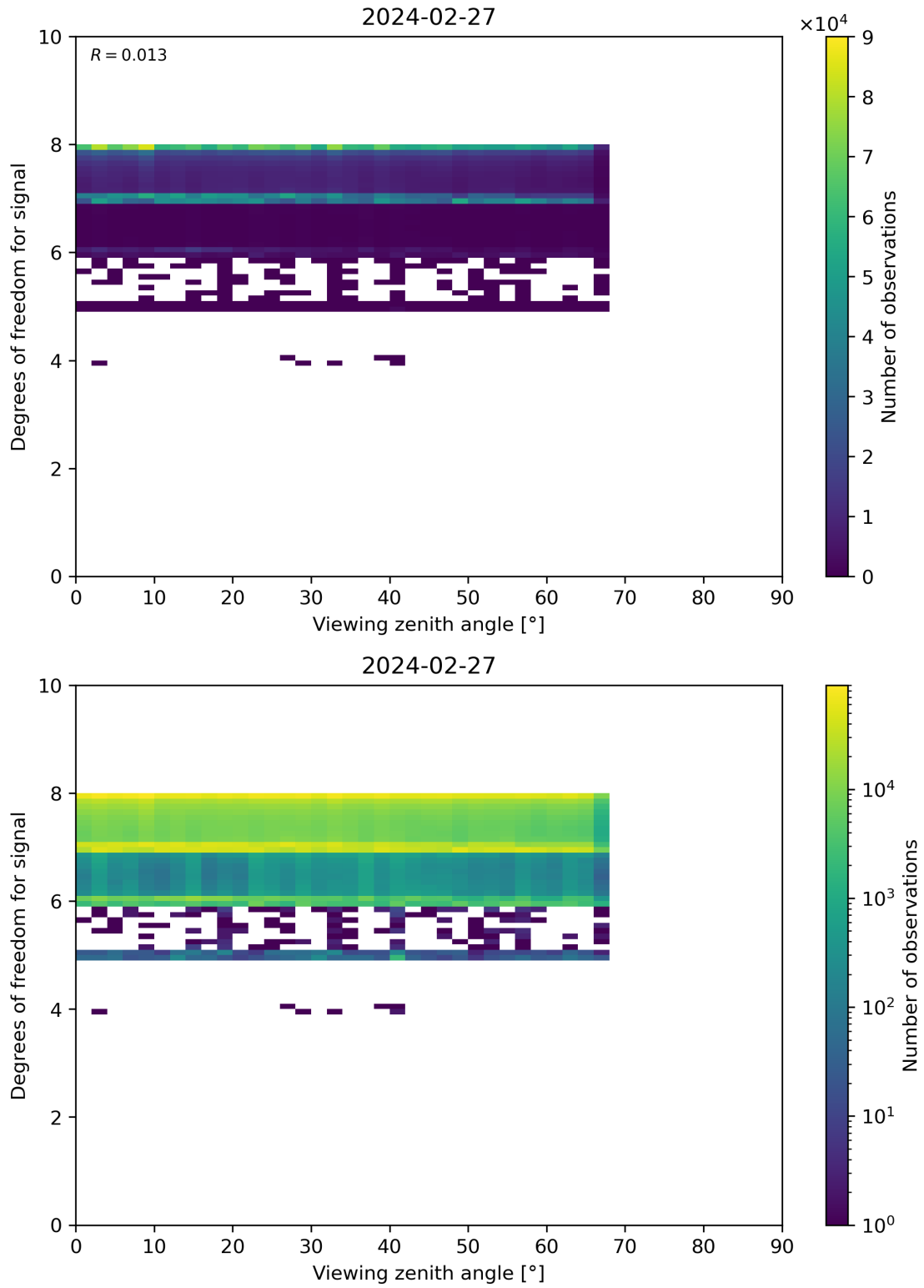
Figure 73: Scatter density plot of “Viewing zenith angle” against “Degrees of freedom for signal” for 2024-02-27 to 2024-02-28.
