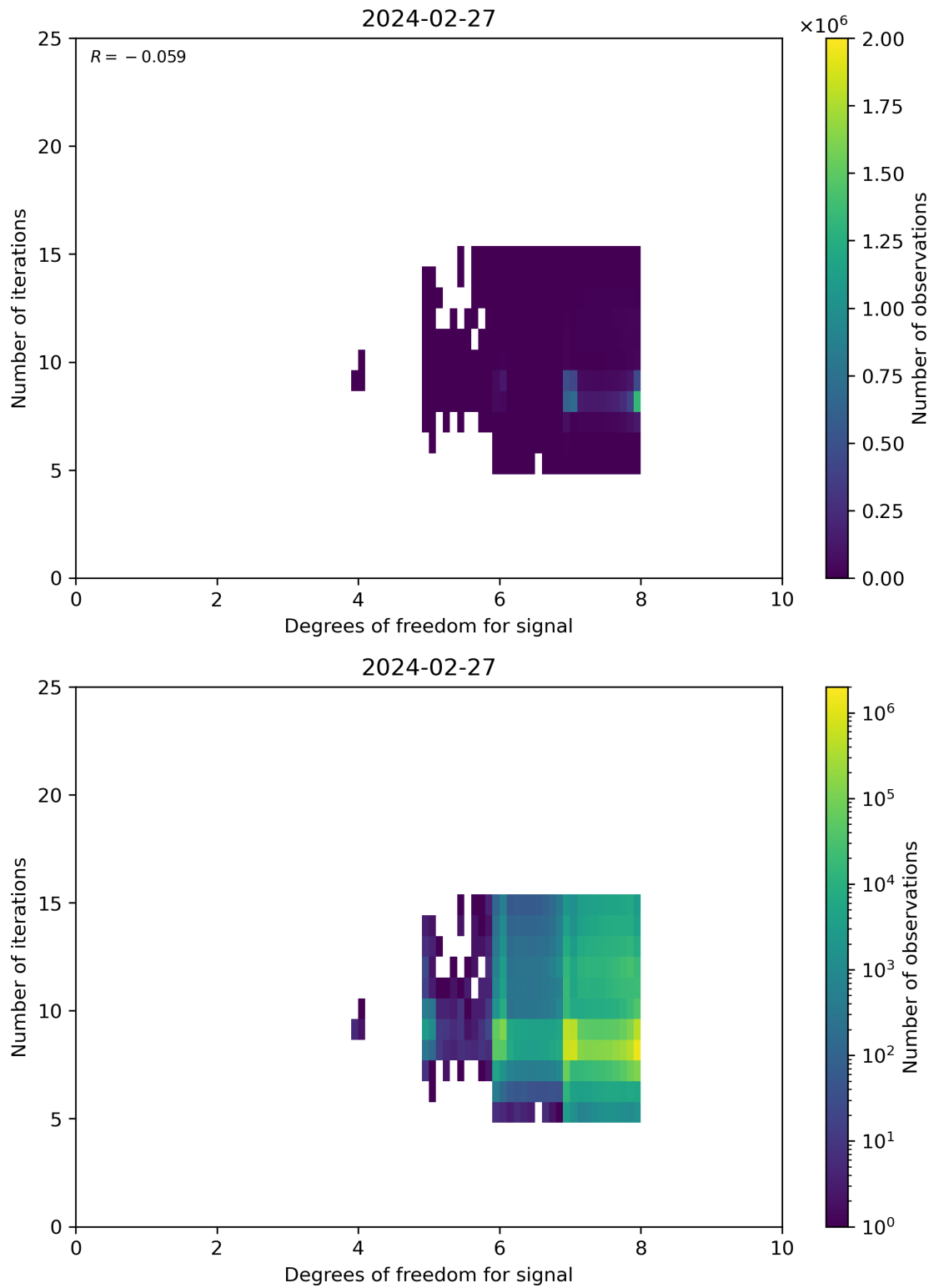
Figure 50: Scatter density plot of “Degrees of freedom for signal” against “Number of iterations” for 2024-02-27 to 2024-02-28.
