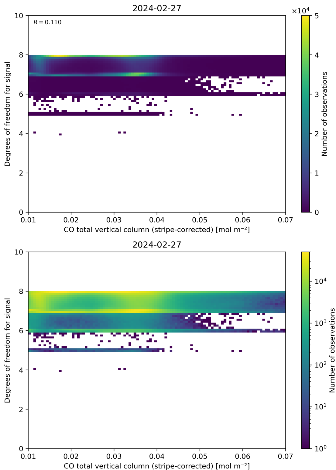
Figure 38: Scatter density plot of “CO total vertical column (stripe-corrected)” against “Degrees of freedom for signal” for 2024-02-27 to 2024-02-28.
