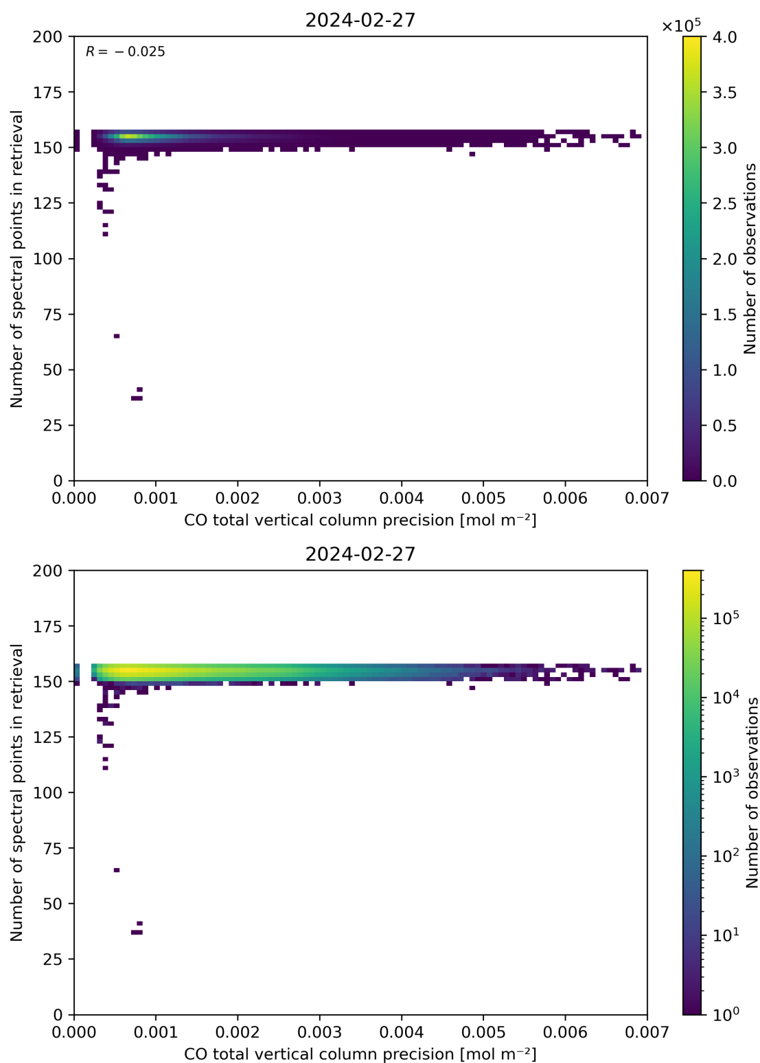
Figure 47: Scatter density plot of “CO total vertical column precision” against “Number of spectral points in retrieval” for 2024-02-27 to 2024-02-28.
