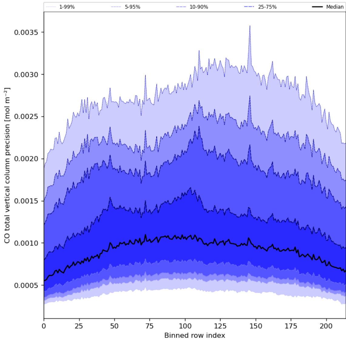
Figure 28: Along track statistics of “CO total vertical column precision” for 2024-02-27 to 2024-02-28
