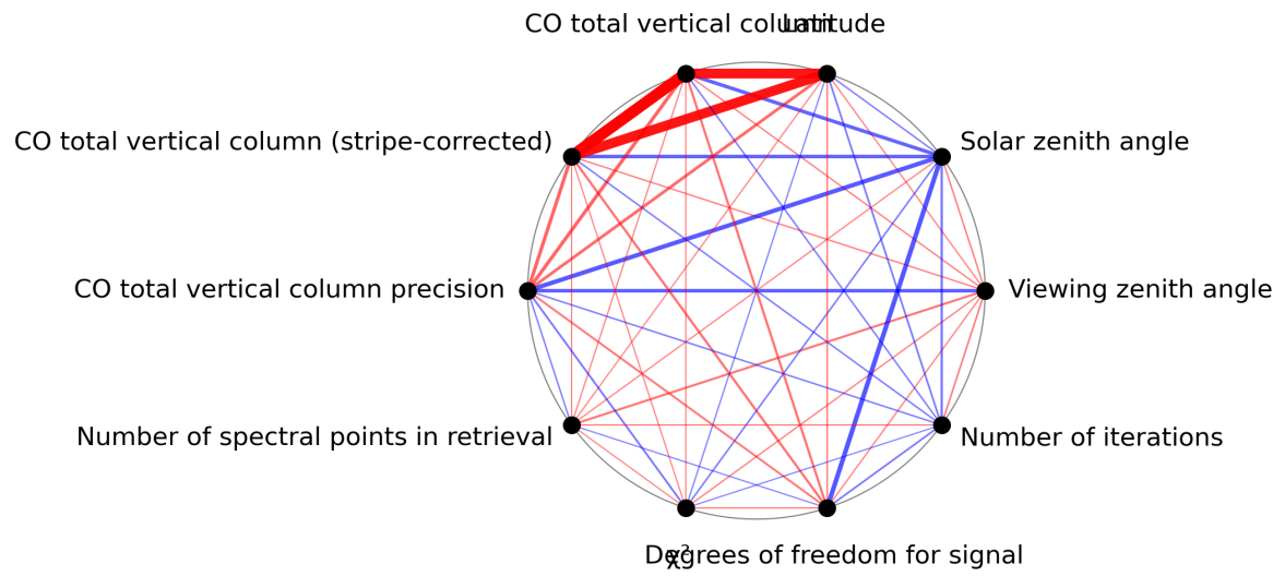
Figure 1: Map of correlation graph for 2024-02-27 to 2024-02-28.
