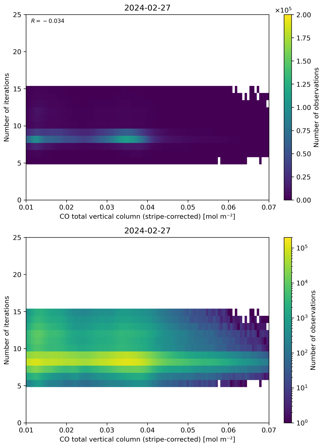
Figure 39: Scatter density plot of “CO total vertical column (stripe-corrected)” against “Number of iterations” for 2024-02-27 to 2024-02-28.
