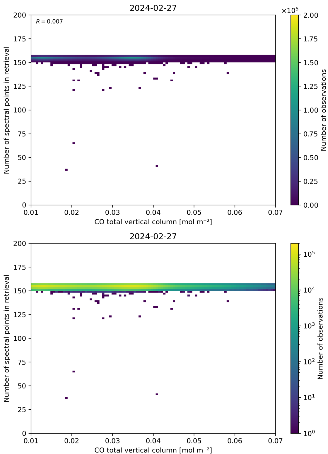
Figure 43: Scatter density plot of “CO total vertical column” against “Number of spectral points in retrieval” for 2024-02-27 to 2024-02-28.
