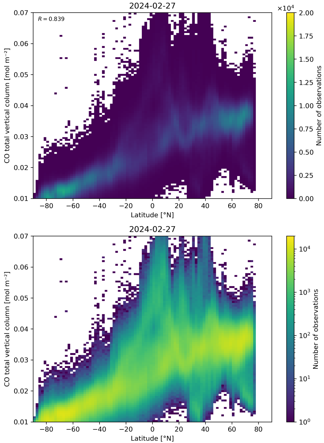
Figure 51: Scatter density plot of “Latitude” against “CO total vertical column” for 2024-02-27 to 2024-02-28.
