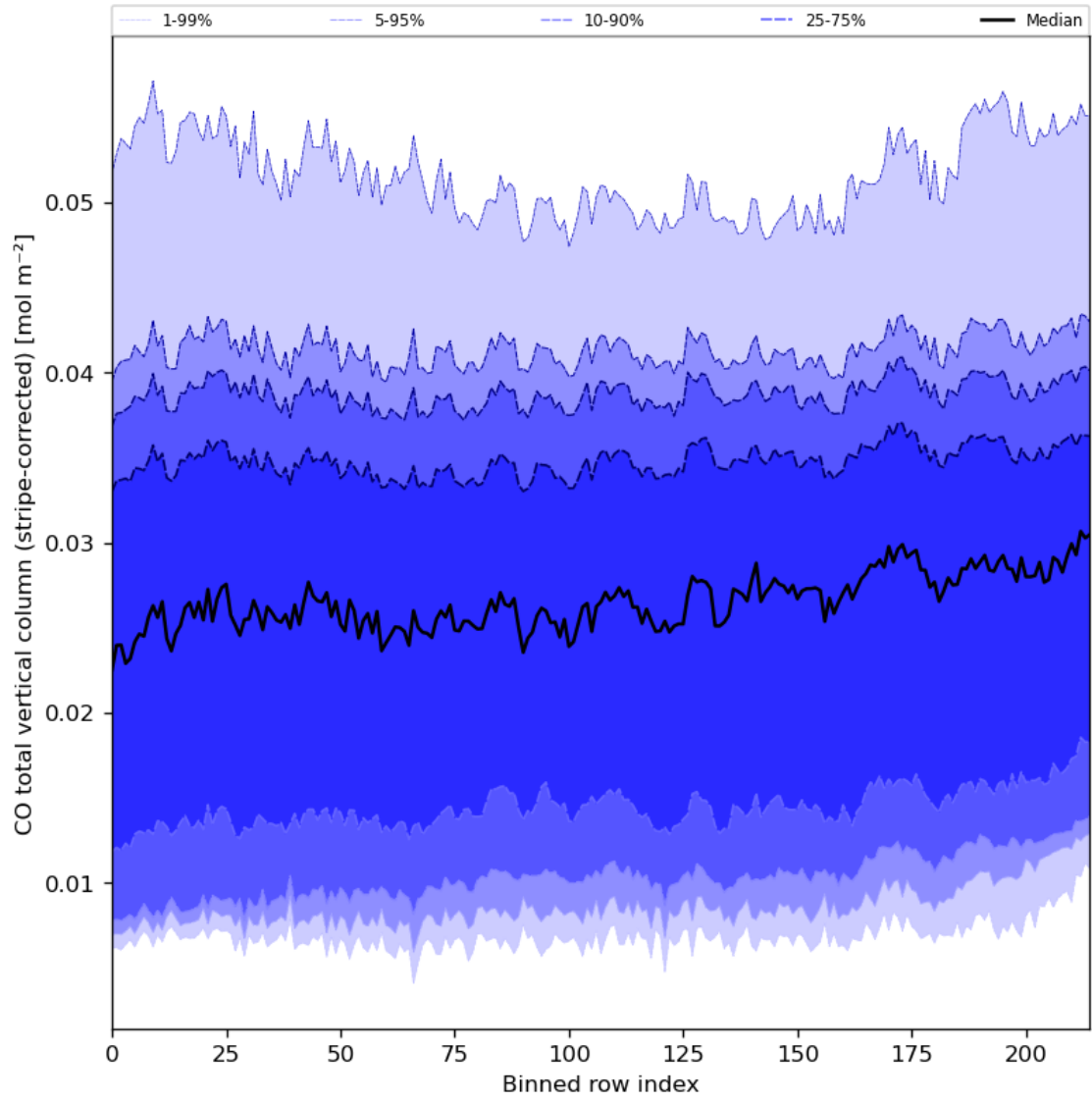
Figure 27: Along track statistics of “CO total vertical column (stripe-corrected)” for 2024-02-27 to 2024-02-28
