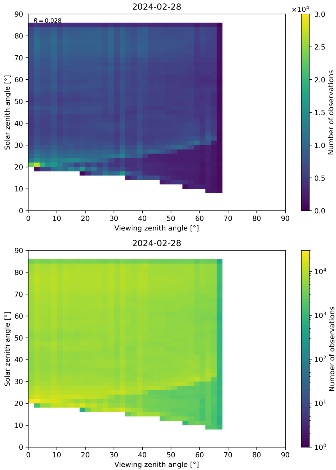
Figure 77: Scatter density plot of “Viewing zenith angle” against “Solar zenith angle” for 2024-02-27 to 2024-02-29.
