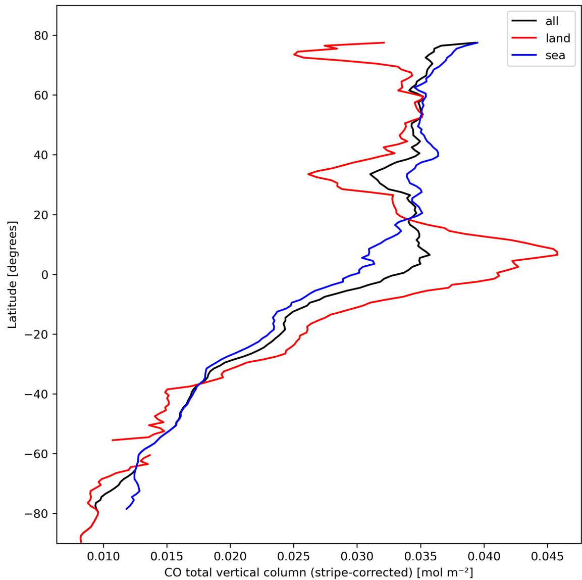
Figure 11: Zonal average of “CO total vertical column (stripe-corrected)” for 2024-02-27 to 2024-02-29.
