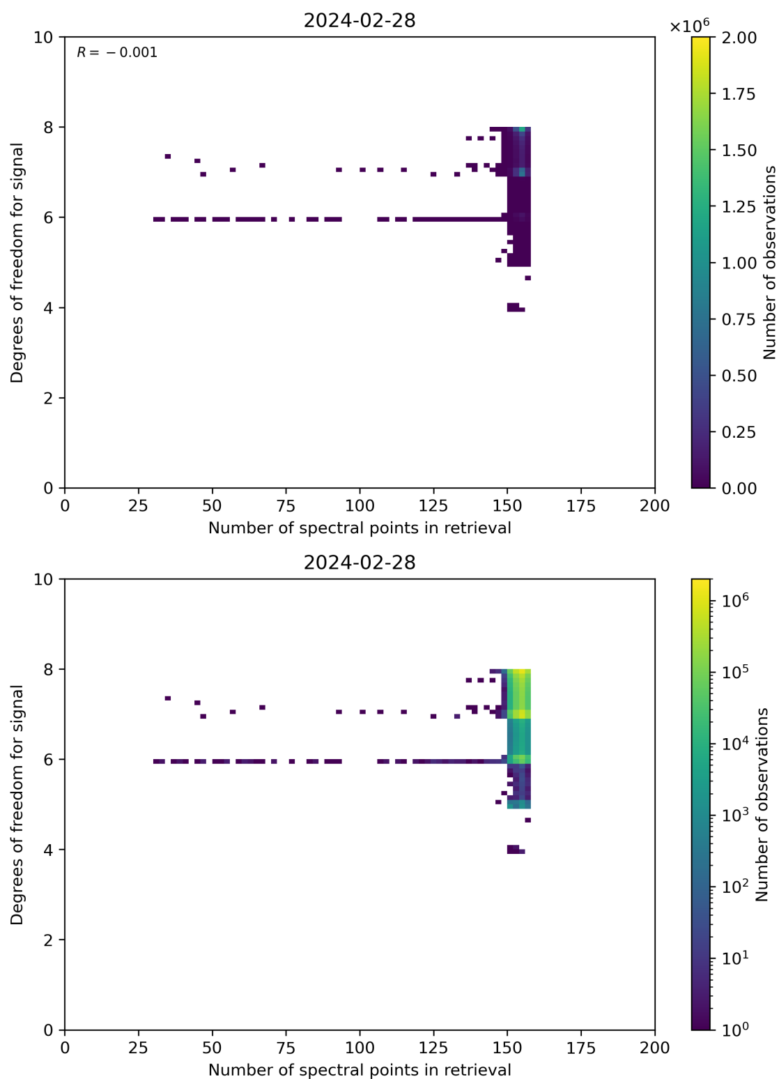
Figure 59: Scatter density plot of “Number of spectral points in retrieval” against “Degrees of freedom for signal” for 2024-02-27 to 2024-02-29.
