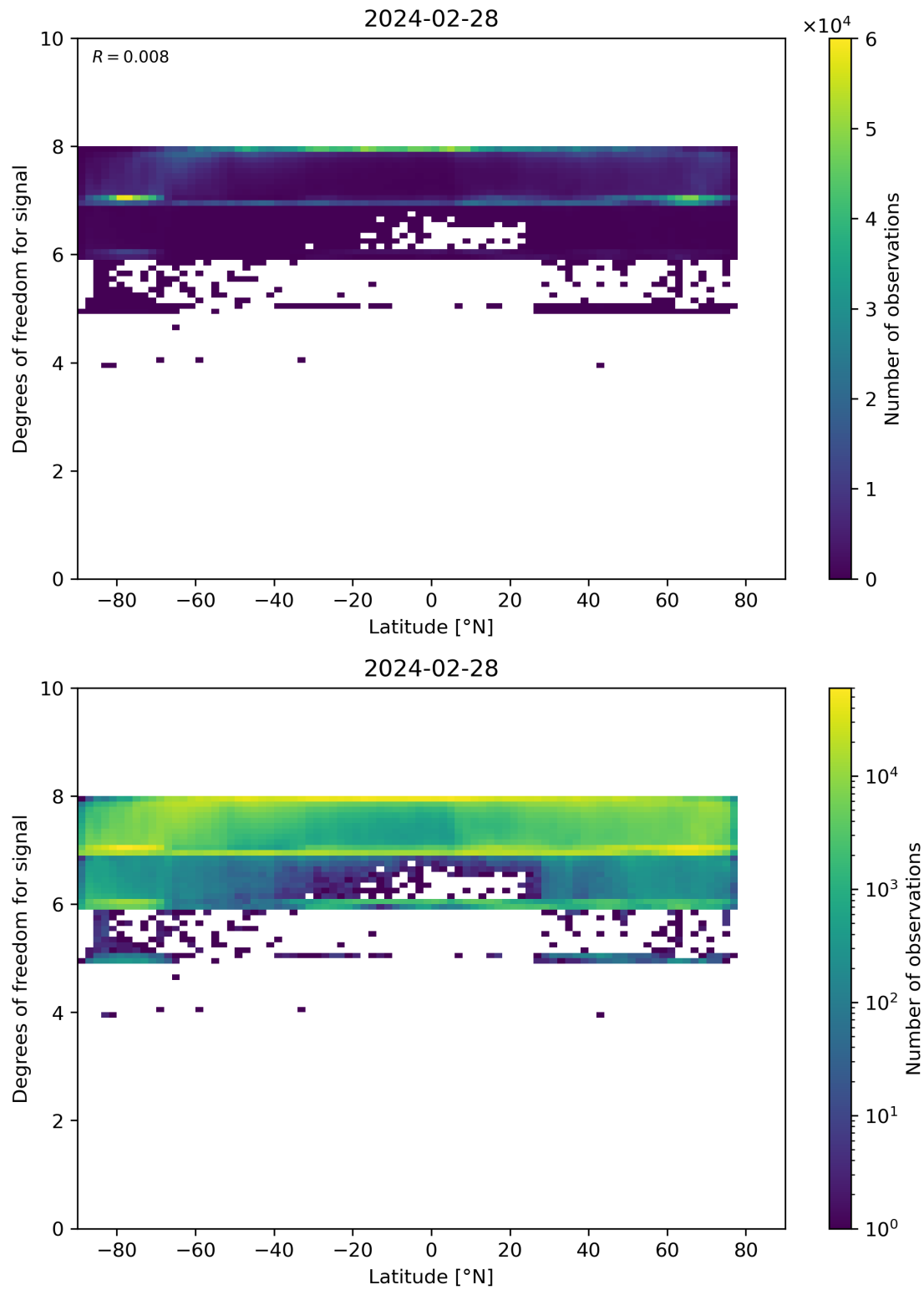
Figure 55: Scatter density plot of “Latitude” against “Degrees of freedom for signal” for 2024-02-27 to 2024-02-29.
