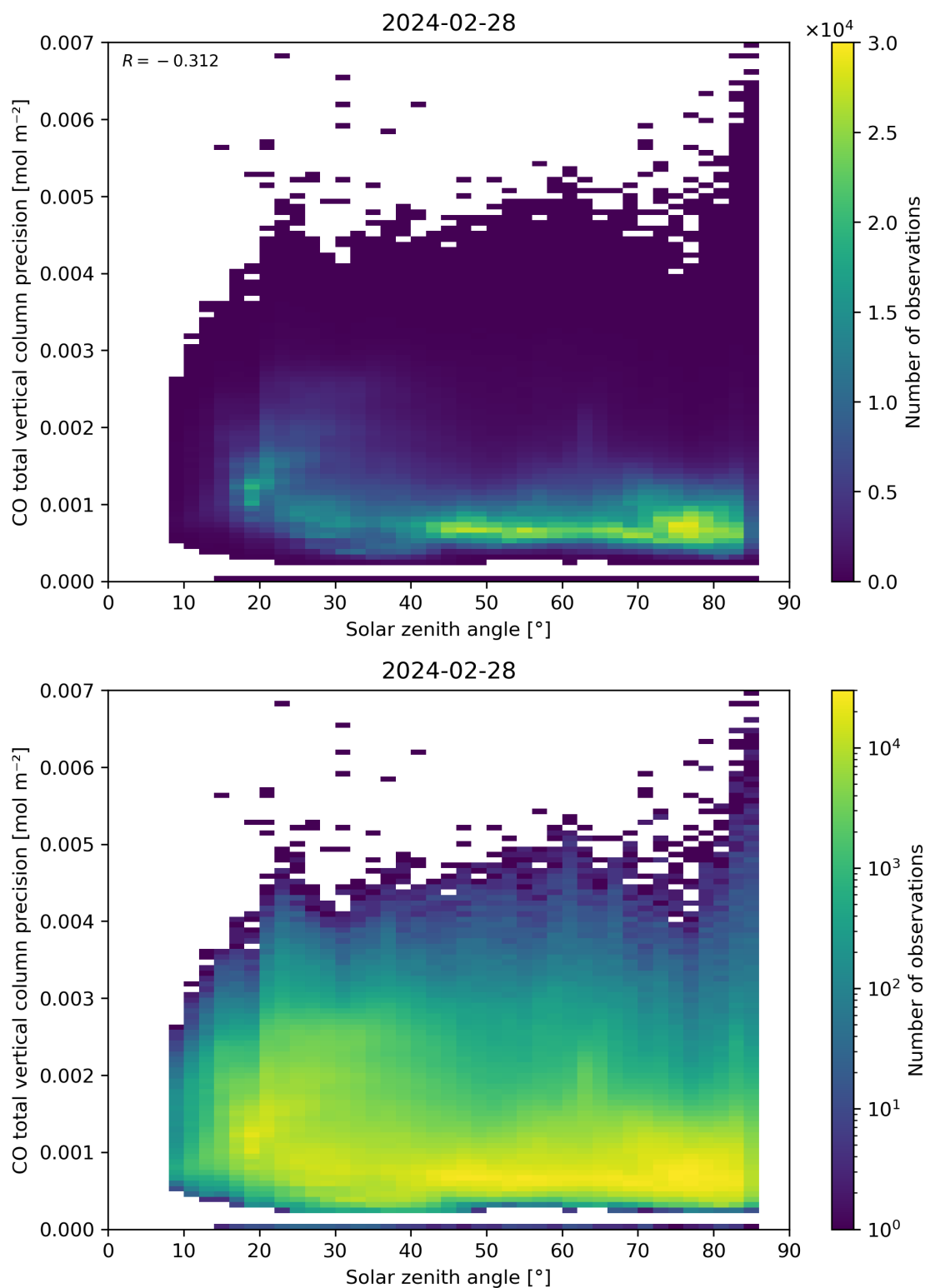
Figure 63: Scatter density plot of “Solar zenith angle” against “CO total vertical column precision” for 2024-02-27 to 2024-02-29.
