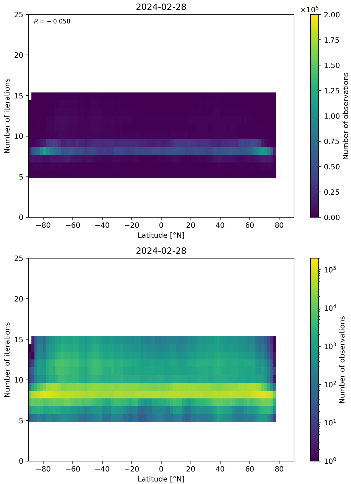
Figure 56: Scatter density plot of “Latitude” against “Number of iterations” for 2024-02-27 to 2024-02-29.
