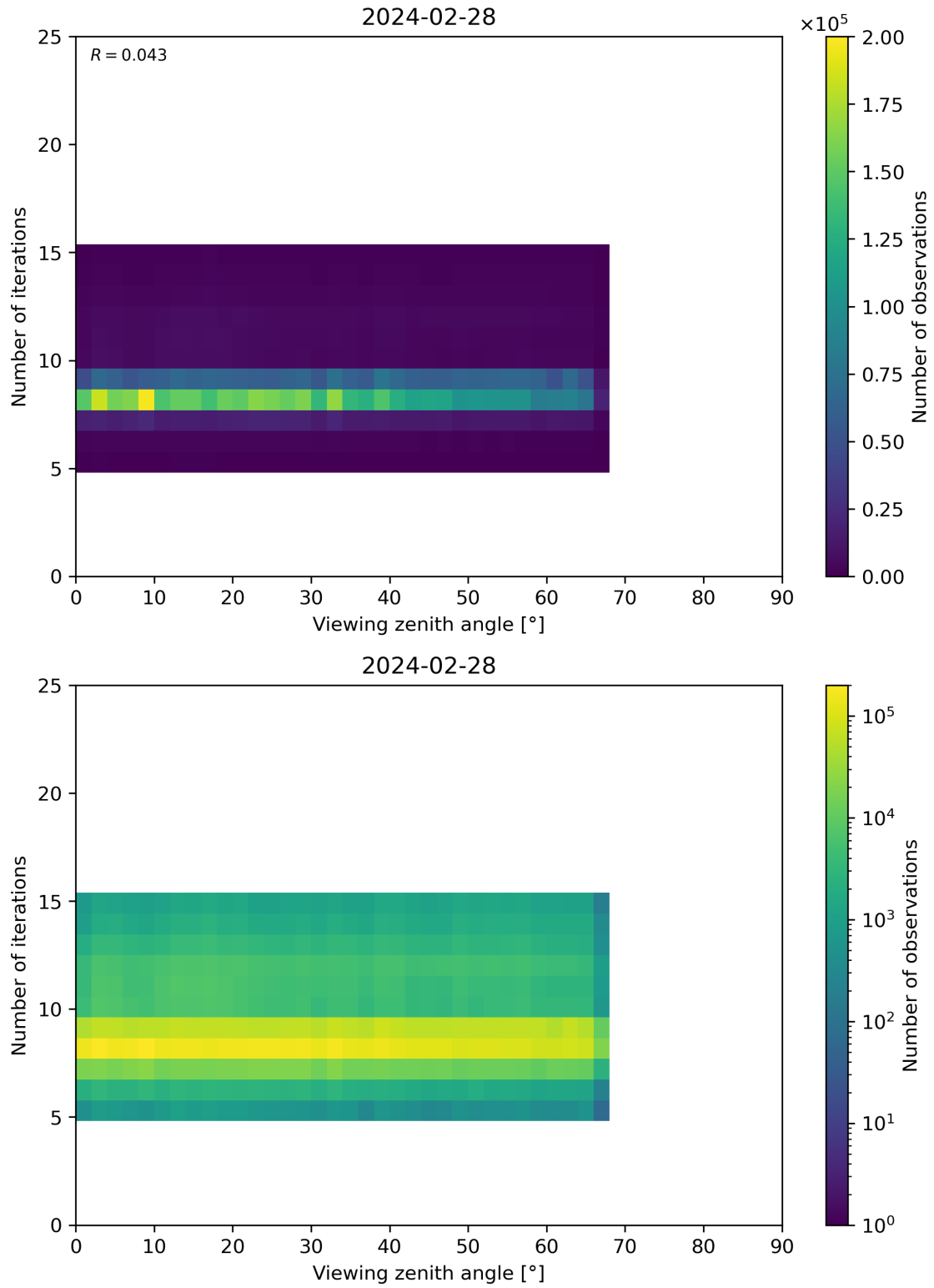
Figure 75: Scatter density plot of “Viewing zenith angle” against “Number of iterations” for 2024-02-27 to 2024-02-29.
