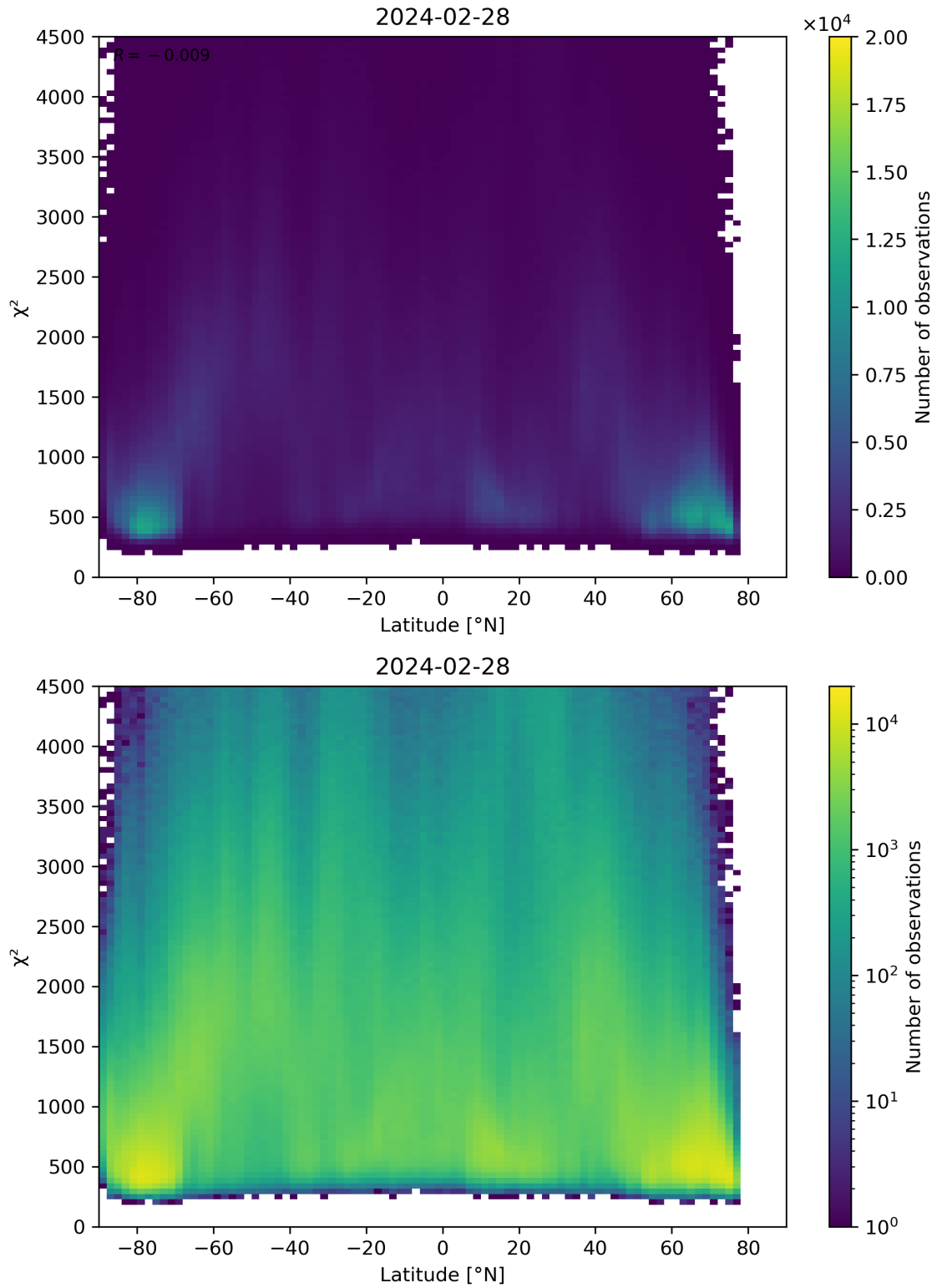
Figure 54: Scatter density plot of “Latitude” against “ \chi^2 ” for 2024-02-27 to 2024-02-29.
