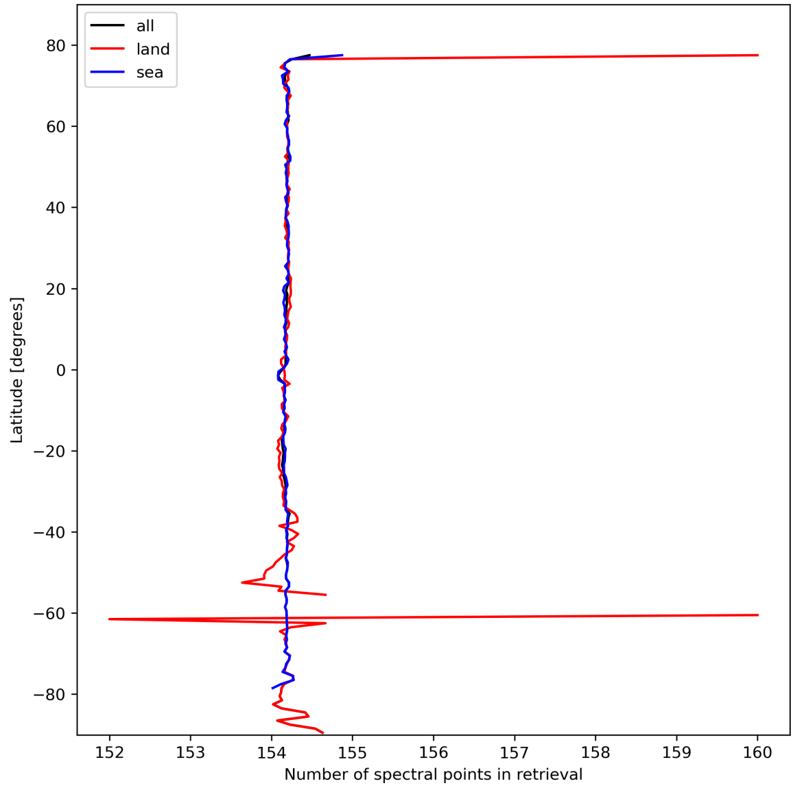
Figure 13: Zonal average of “Number of spectral points in retrieval” for 2024-02-27 to 2024-02-29.
