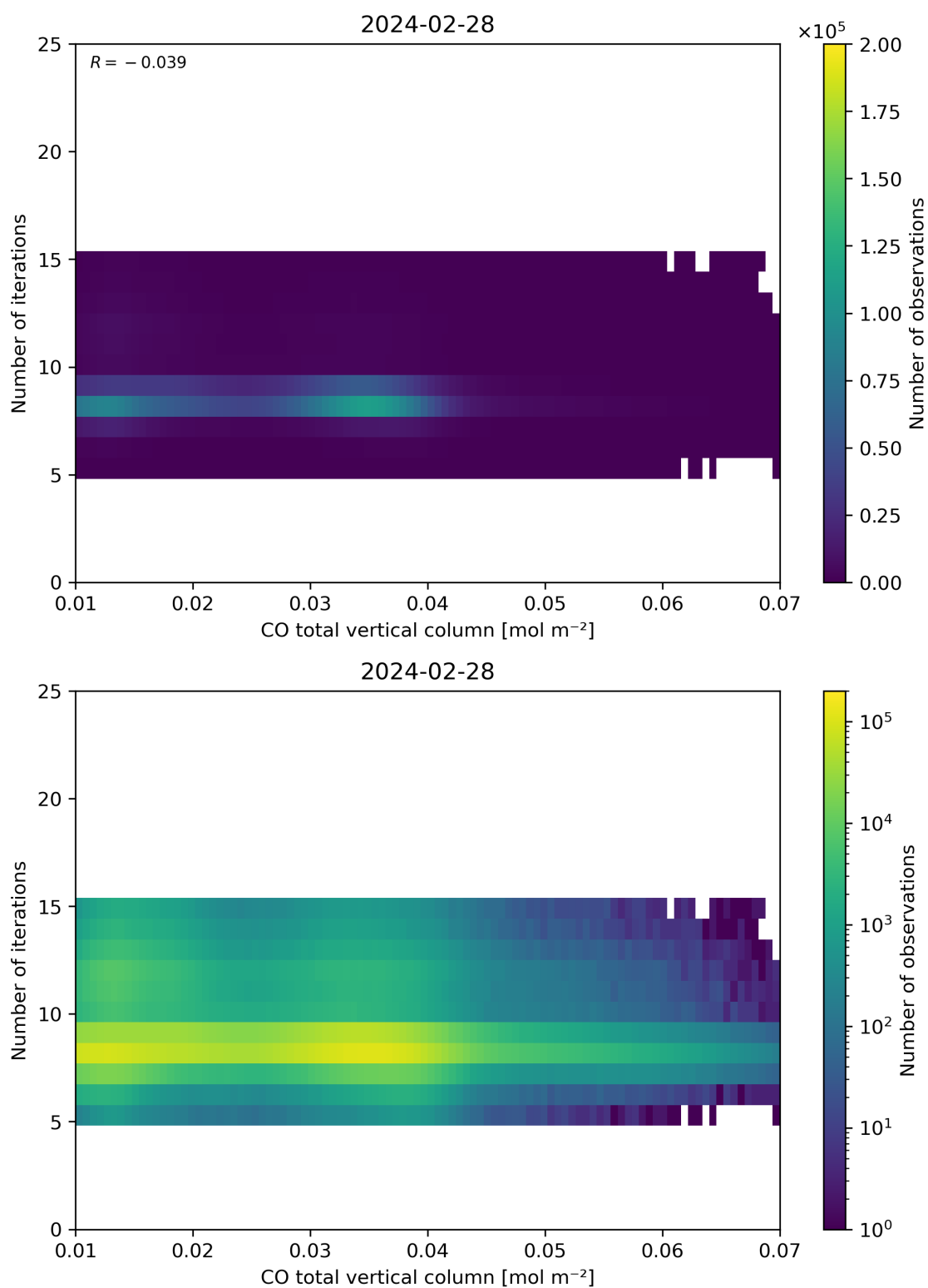
Figure 42: Scatter density plot of “CO total vertical column” against “Number of iterations” for 2024-02-27 to 2024-02-29.
