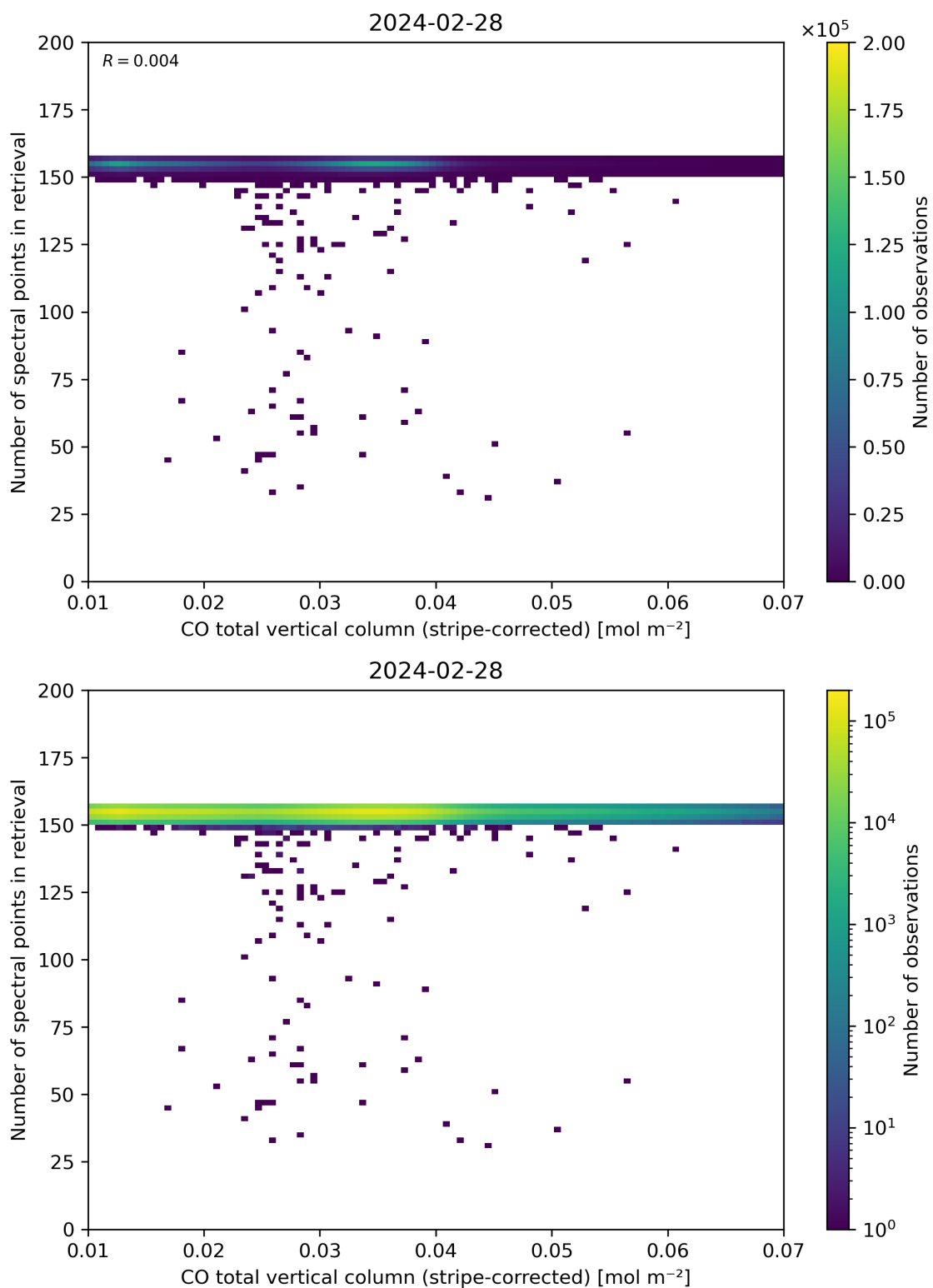
Figure 40: Scatter density plot of “CO total vertical column (stripe-corrected)” against “Number of spectral points in retrieval” for 2024-02-27 to 2024-02-29.
