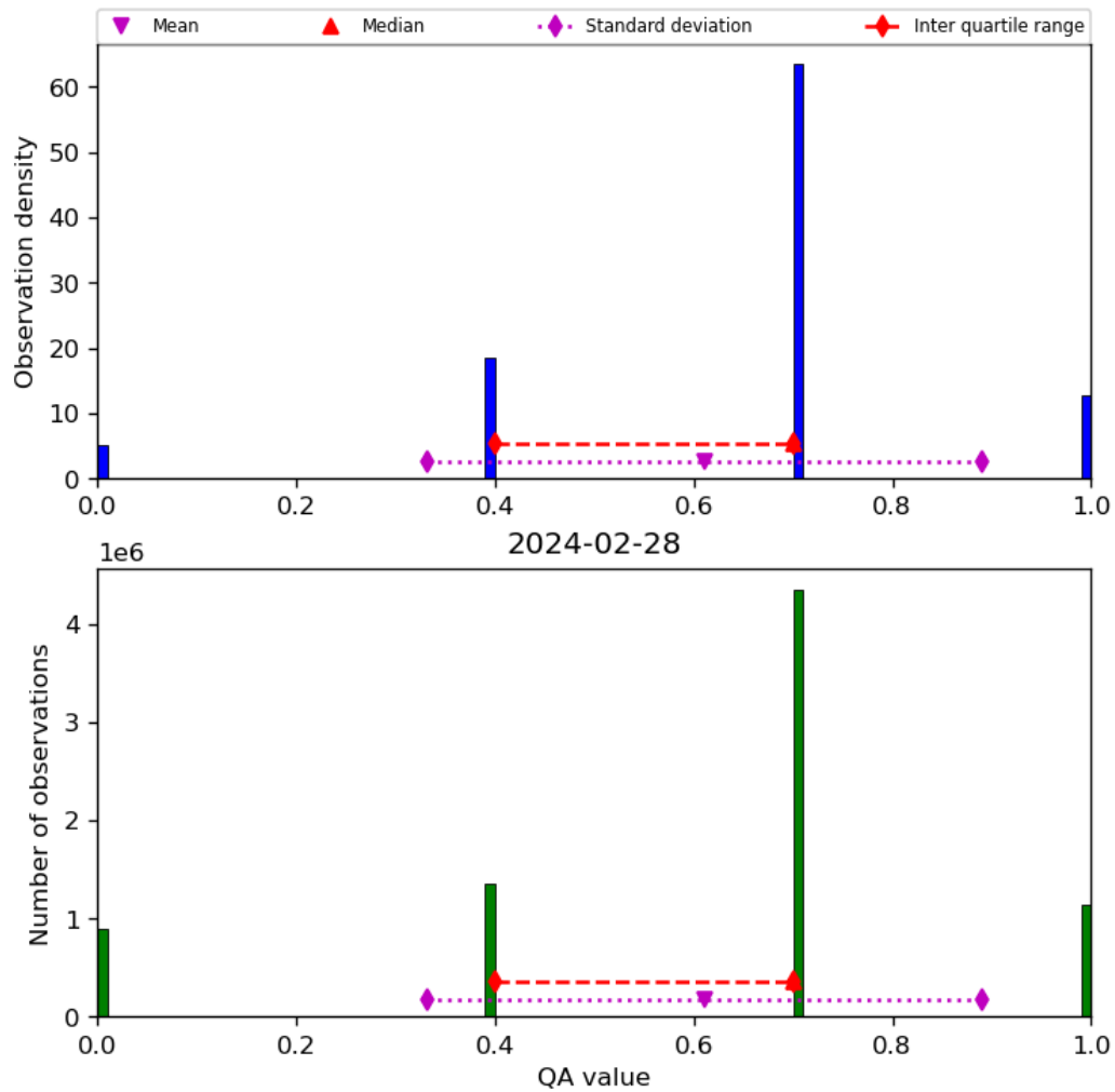
Figure 17: Histogram of “QA value” for 2024-02-27 to 2024-02-29
