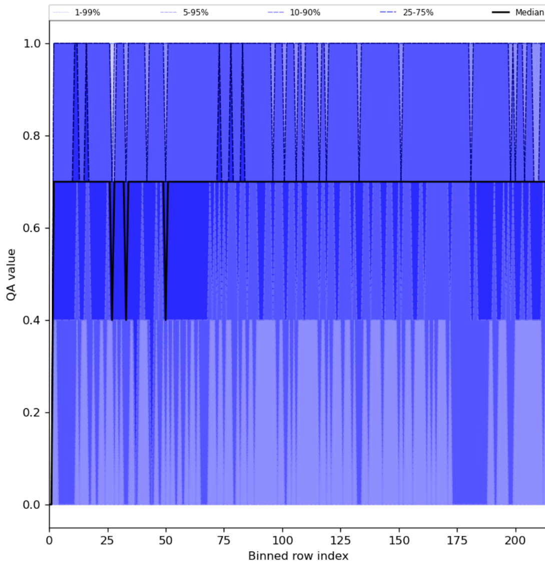
Figure 25: Along track statistics of “QA value” for 2024-02-27 to 2024-02-29
