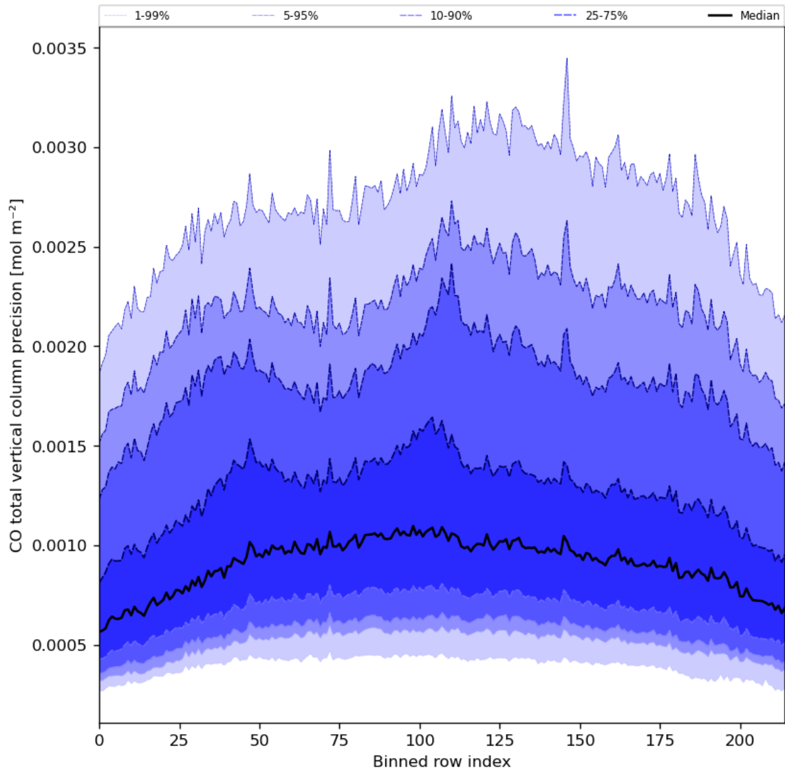
Figure 28: Along track statistics of “CO total vertical column precision” for 2024-02-27 to 2024-02-29
