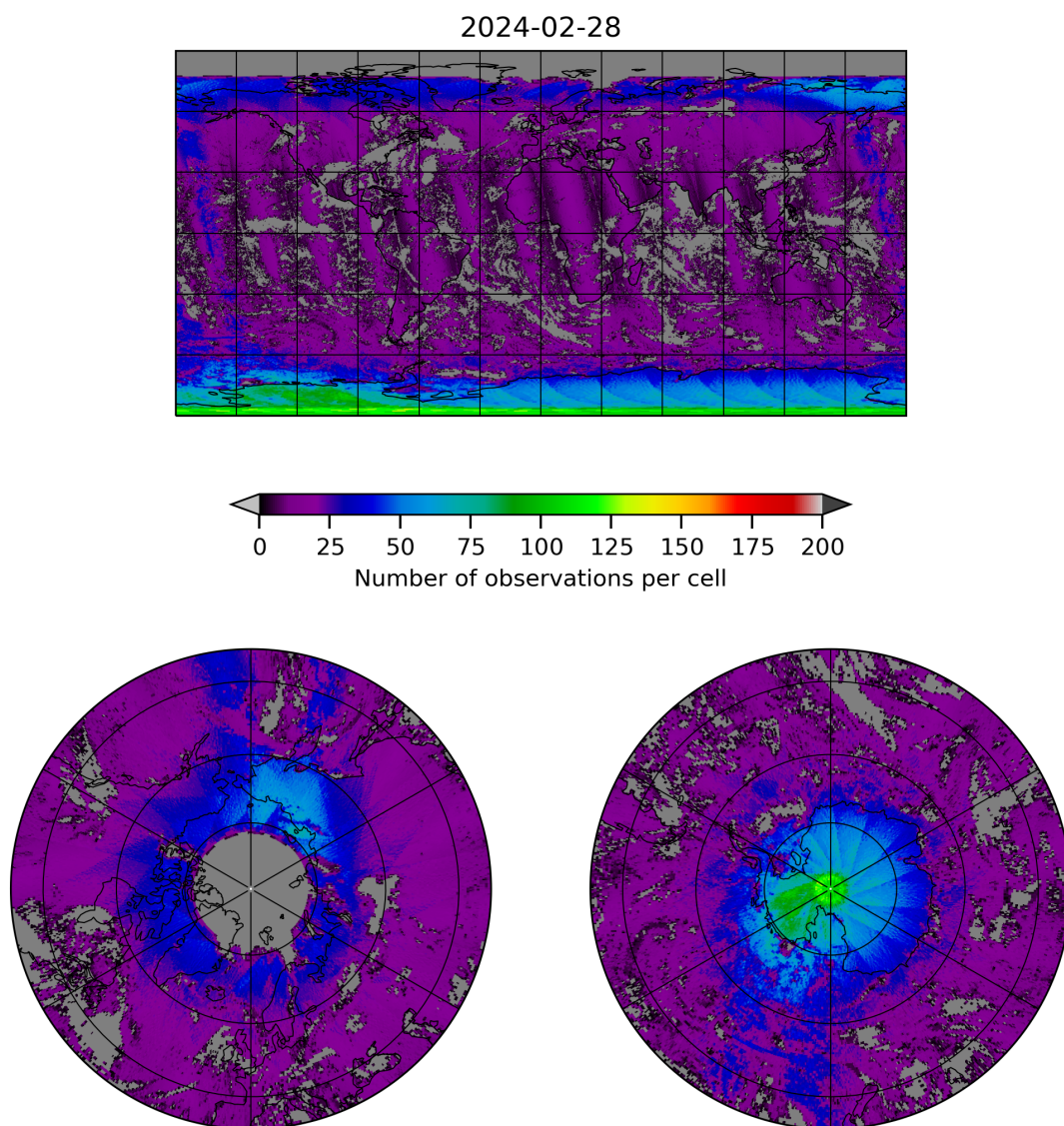
Figure 8: Map of the number of observations for 2024-02-27 to 2024-02-29
