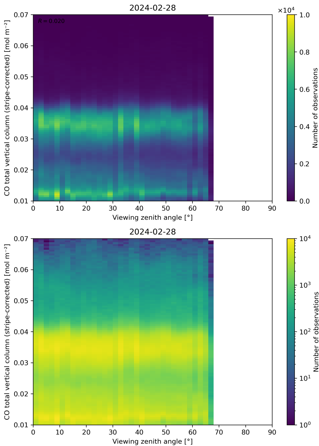
Figure 70: Scatter density plot of “Viewing zenith angle” against “CO total vertical column (stripe-corrected)” for 2024-02-27 to 2024-02-29.
