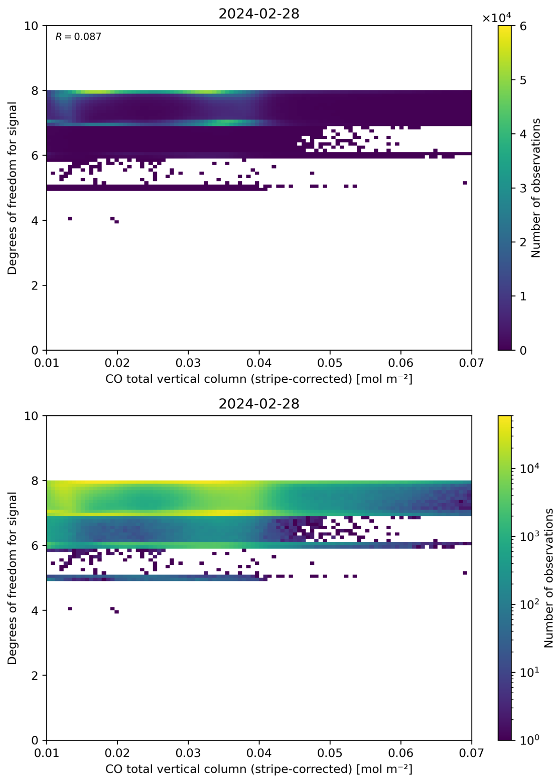
Figure 38: Scatter density plot of “CO total vertical column (stripe-corrected)” against “Degrees of freedom for signal” for 2024-02-27 to 2024-02-29.
