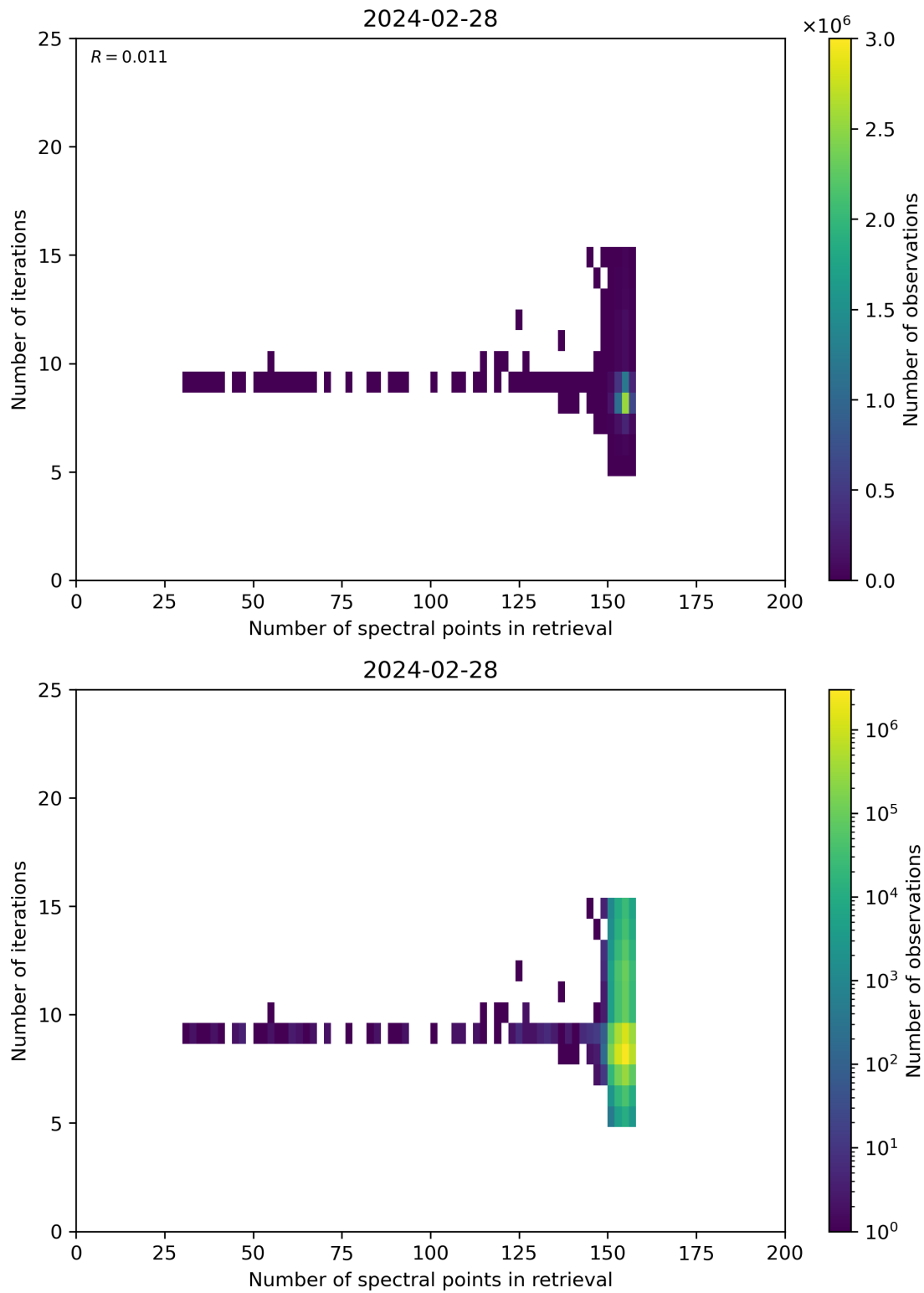
Figure 60: Scatter density plot of “Number of spectral points in retrieval” against “Number of iterations” for 2024-02-27 to 2024-02-29.
