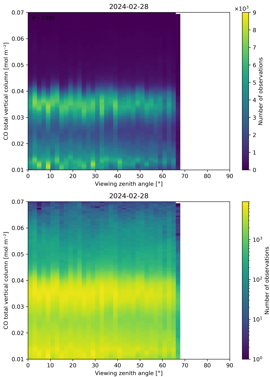
Figure 69: Scatter density plot of “Viewing zenith angle” against “CO total vertical column” for 2024-02-27 to 2024-02-29.
