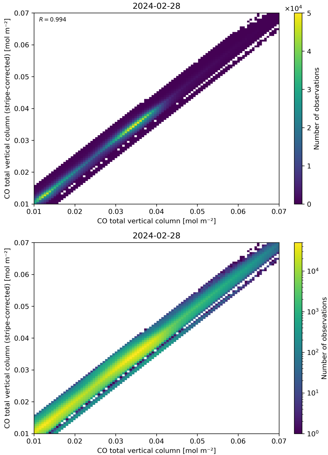
Figure 33: Scatter density plot of “CO total vertical column” against “CO total vertical column (stripe-corrected)” for 2024-02-27 to 2024-02-29.
