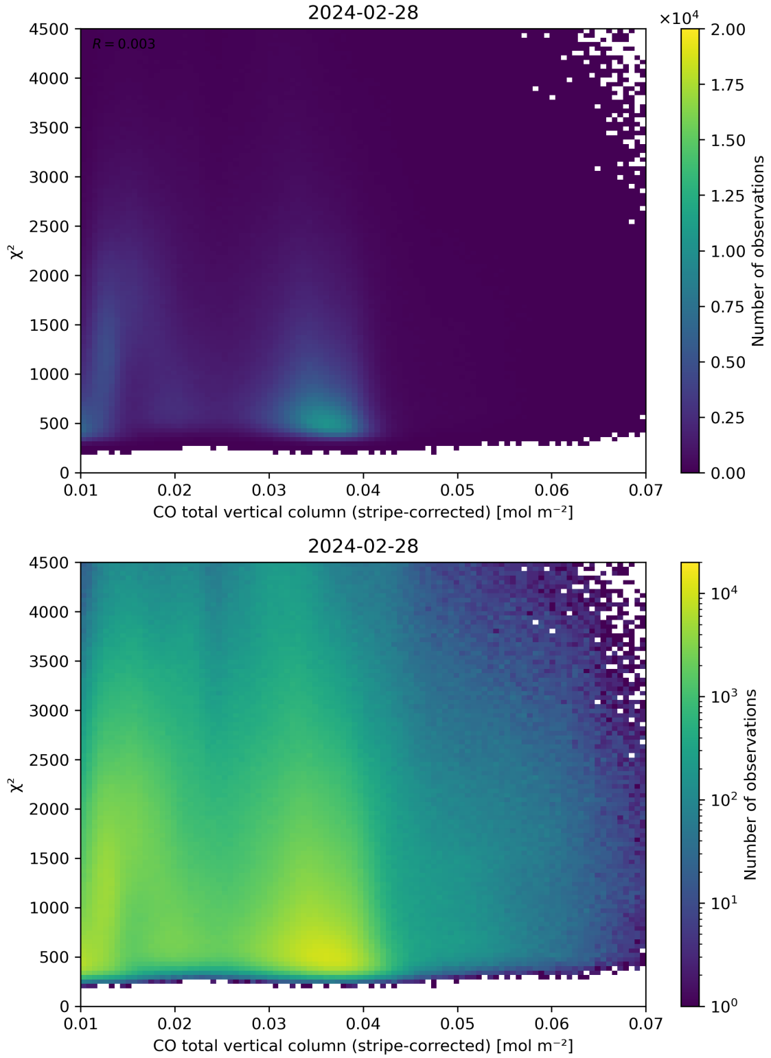
Figure 37: Scatter density plot of “CO total vertical column (stripe-corrected)” against “ \chi^2 ” for 2024-02-27 to 2024-02-29.
