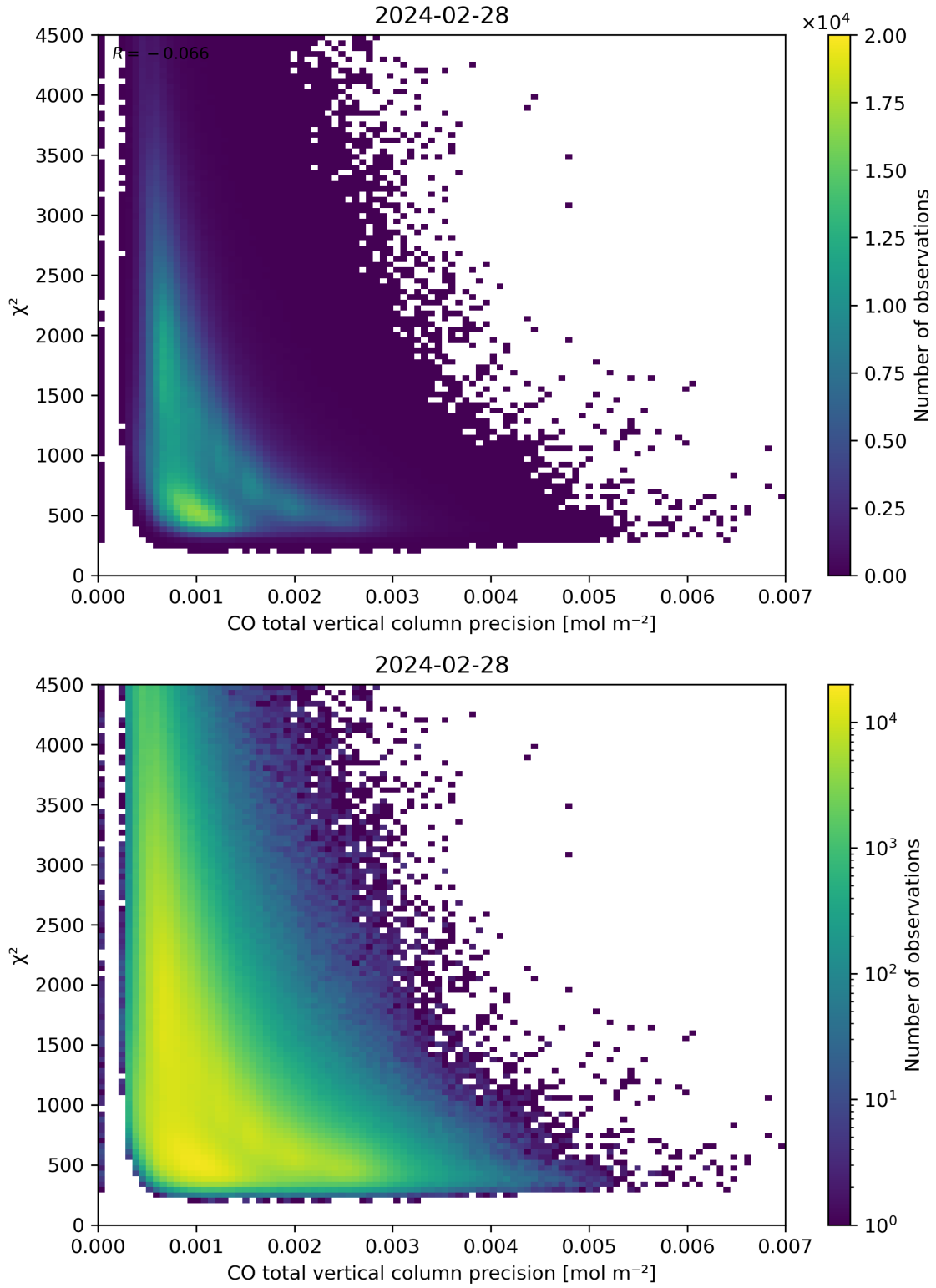
Figure 44: Scatter density plot of “CO total vertical column precision” against “ \chi^2 ” for 2024-02-27 to 2024-02-29.
