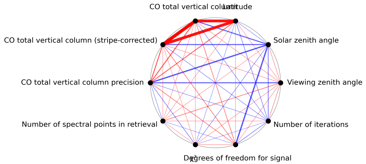
Figure 1: Map of correlation graph for 2024-02-27 to 2024-02-29.
