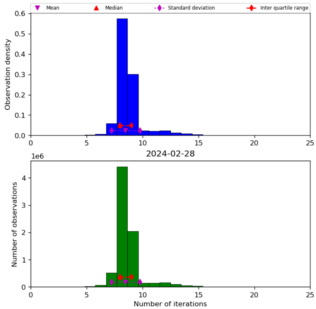
Figure 24: Histogram of “Number of iterations” for 2024-02-27 to 2024-02-29
