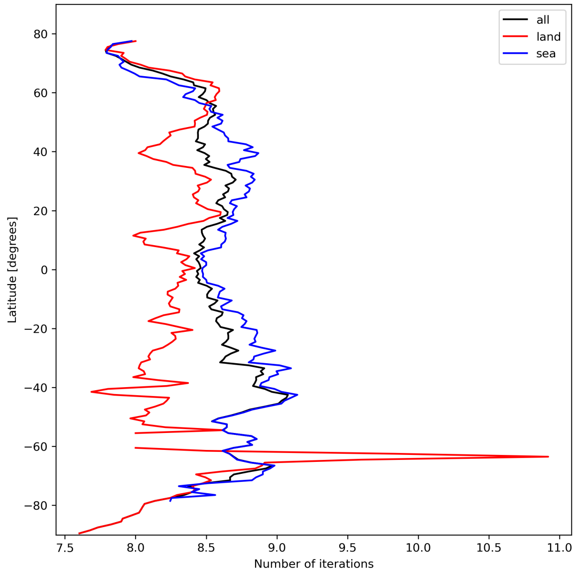
Figure 16: Zonal average of “Number of iterations” for 2024-02-27 to 2024-02-29.
