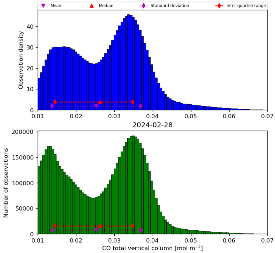
Figure 18: Histogram of “CO total vertical column” for 2024-02-27 to 2024-02-29
