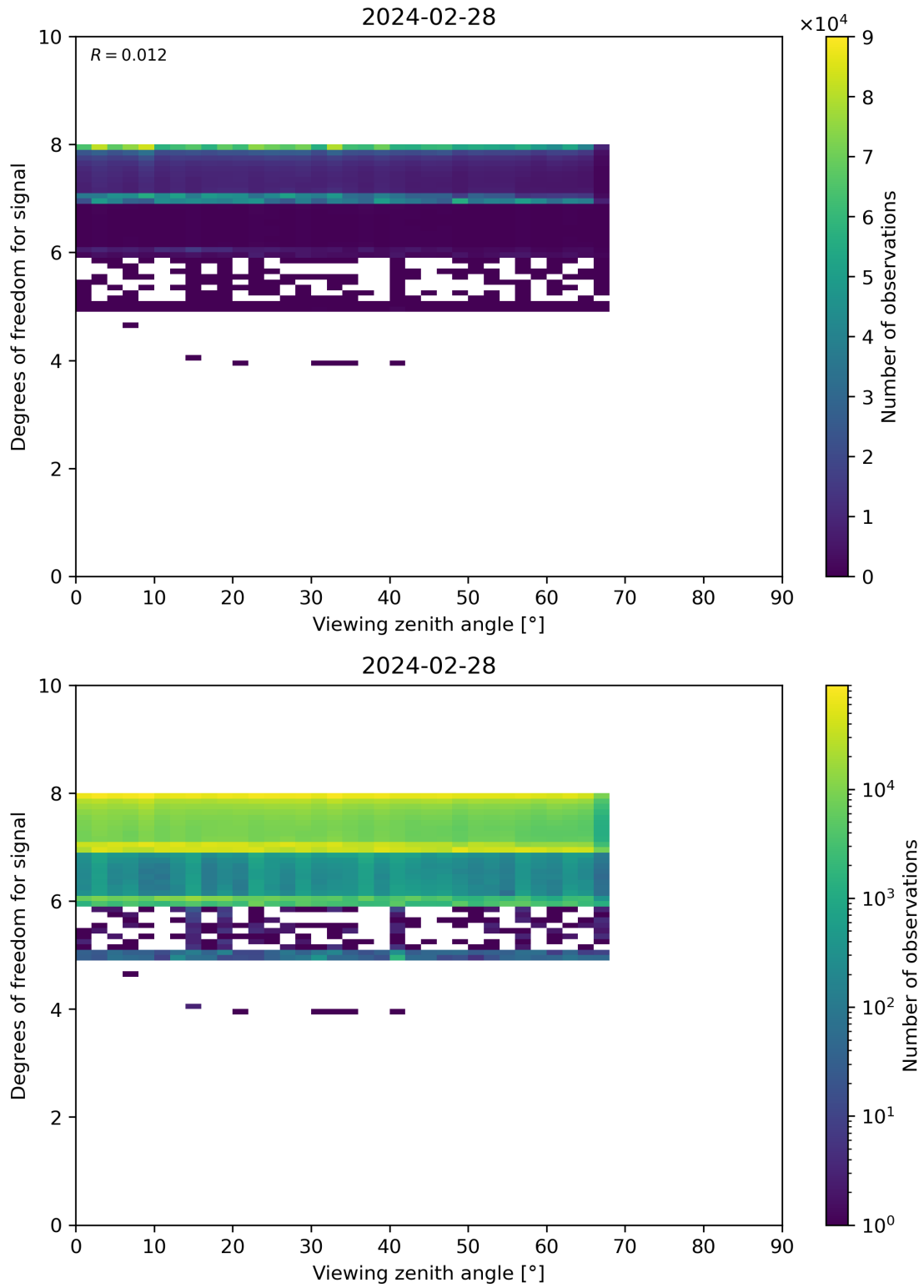
Figure 73: Scatter density plot of “Viewing zenith angle” against “Degrees of freedom for signal” for 2024-02-27 to 2024-02-29.
