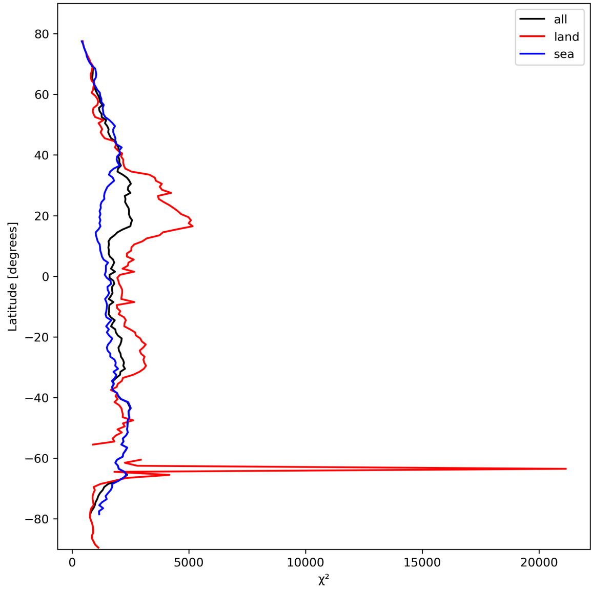
Figure 14: Zonal average of “ \chi^2 ” for 2024-02-27 to 2024-02-29.
