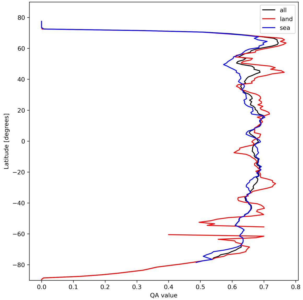
Figure 9: Zonal average of “QA value” for 2024-02-27 to 2024-02-29.
