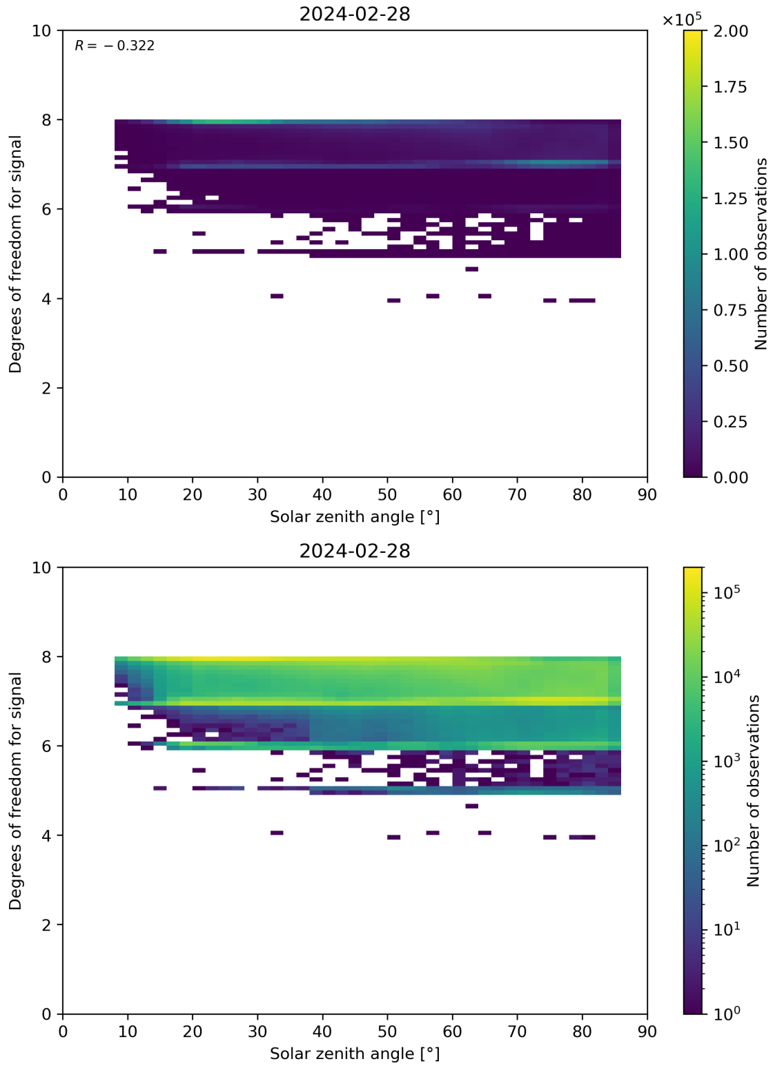
Figure 65: Scatter density plot of “Solar zenith angle” against “Degrees of freedom for signal” for 2024-02-27 to 2024-02-29.
