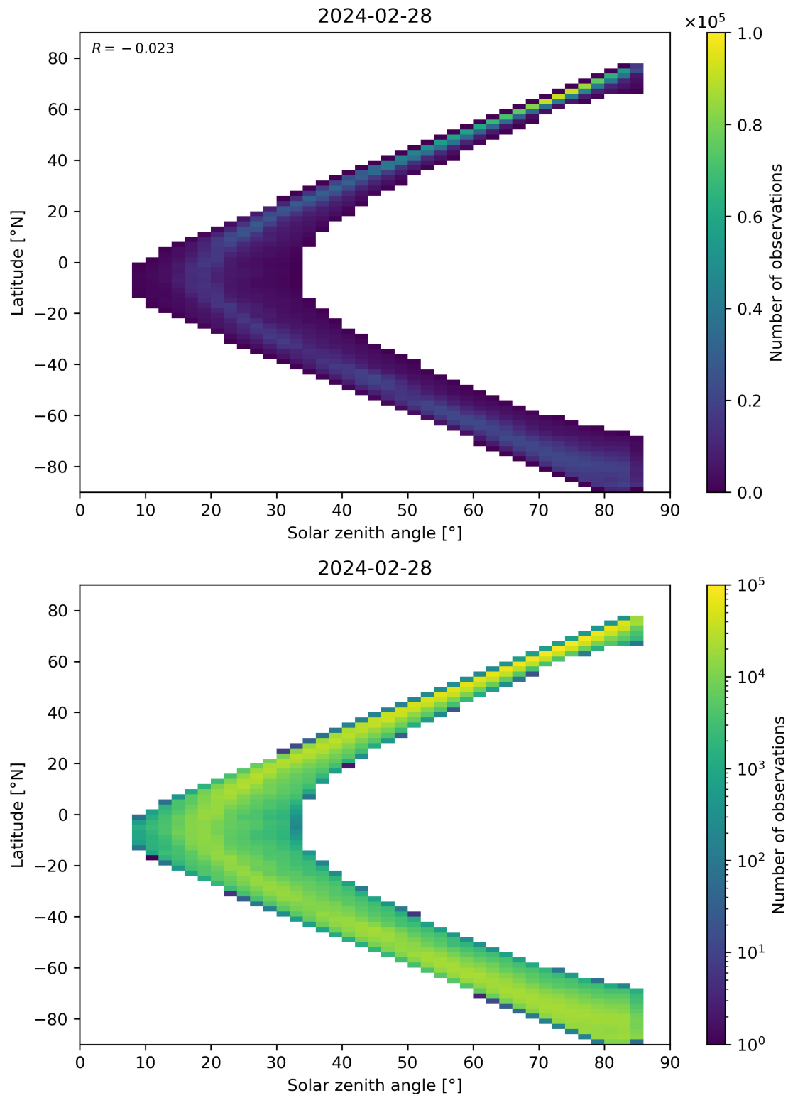
Figure 66: Scatter density plot of “Solar zenith angle” against “Latitude” for 2024-02-27 to 2024-02-29.
