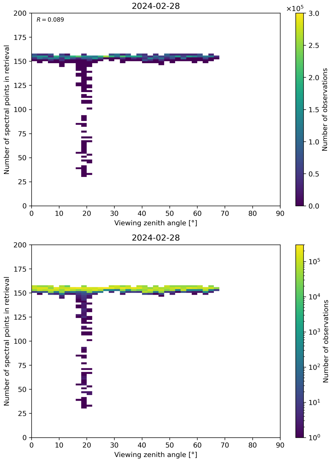
Figure 76: Scatter density plot of “Viewing zenith angle” against “Number of spectral points in retrieval” for 2024-02-27 to 2024-02-29.
