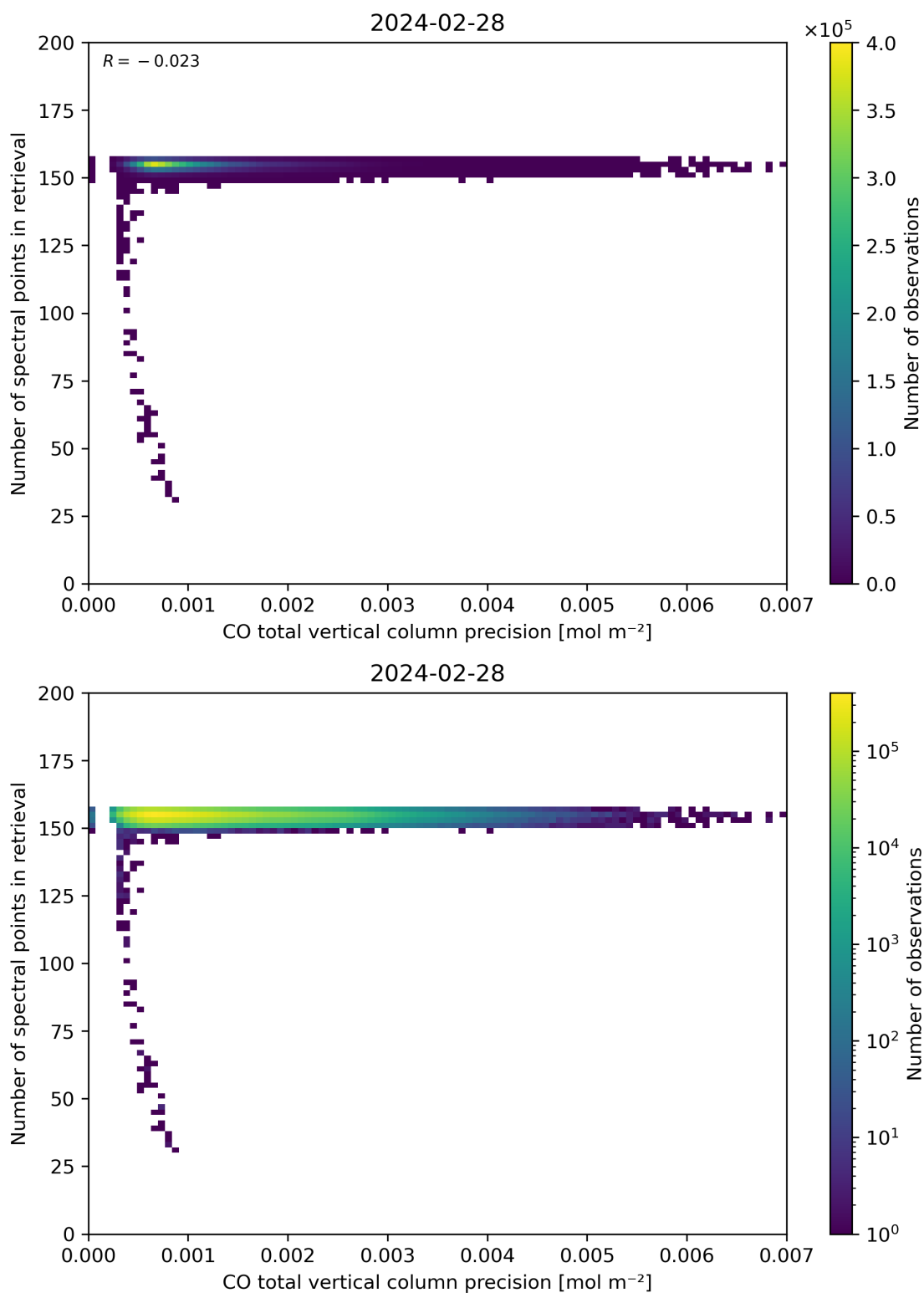
Figure 47: Scatter density plot of “CO total vertical column precision” against “Number of spectral points in retrieval” for 2024-02-27 to 2024-02-29.
