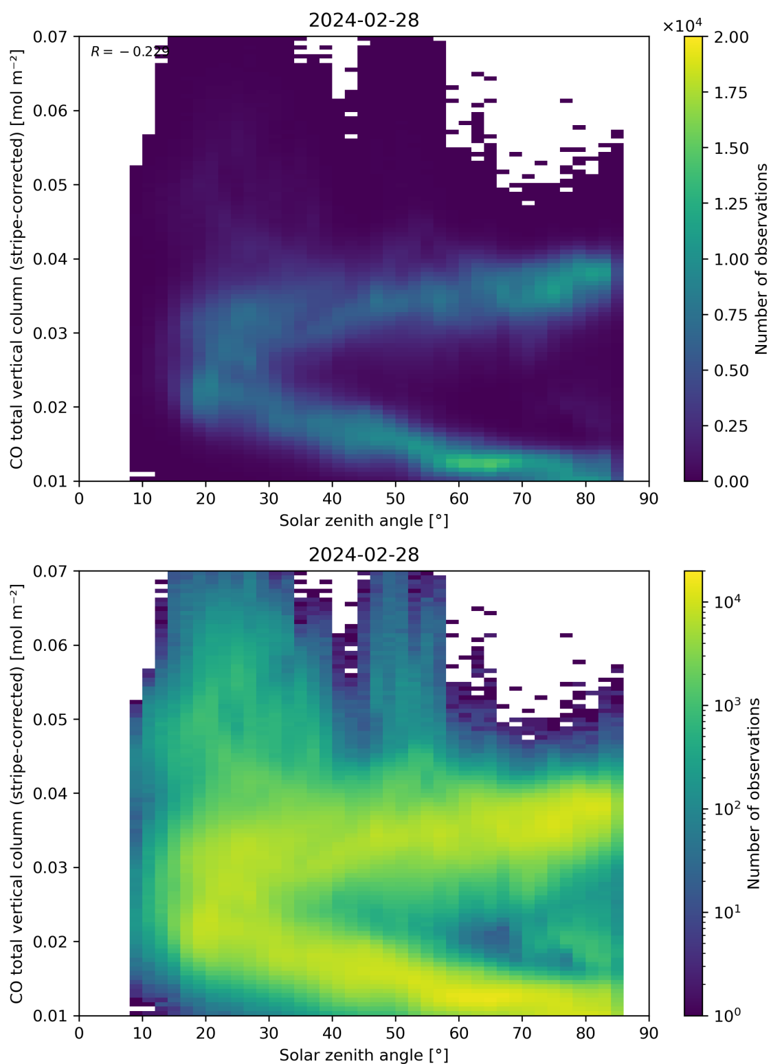
Figure 62: Scatter density plot of “Solar zenith angle” against “CO total vertical column (stripe-corrected)” for 2024-02-27 to 2024-02-29.
