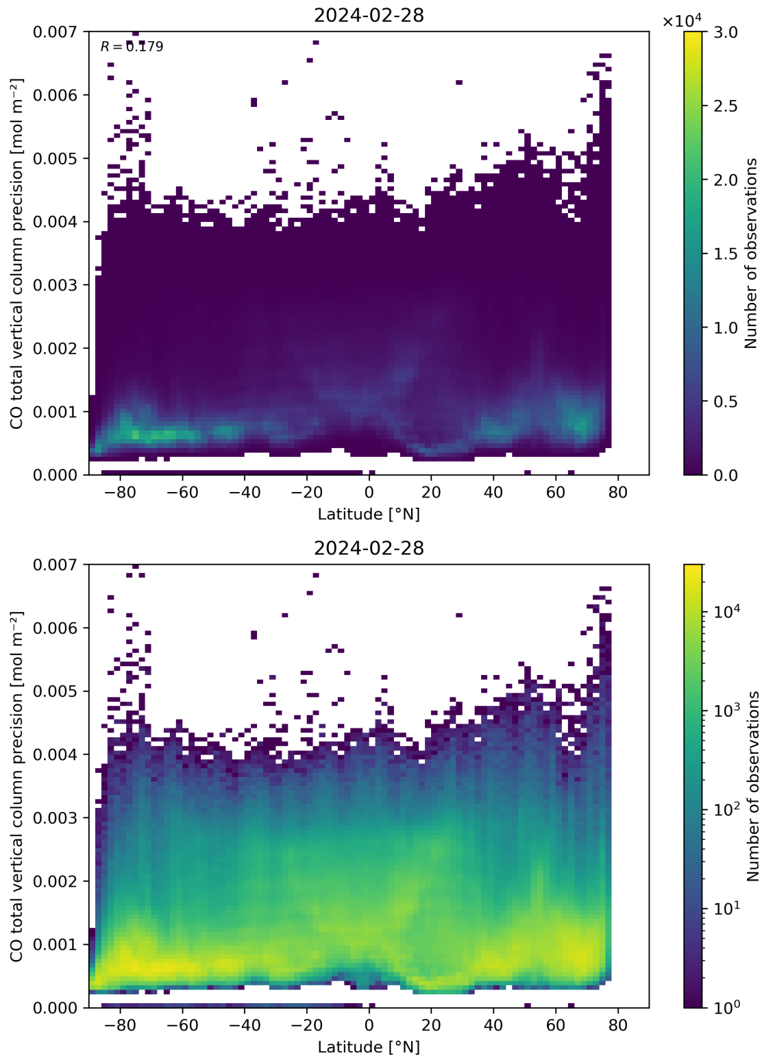
Figure 53: Scatter density plot of “Latitude” against “CO total vertical column precision” for 2024-02-27 to 2024-02-29.
