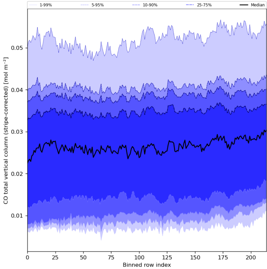
Figure 27: Along track statistics of “CO total vertical column (stripe-corrected)” for 2024-02-27 to 2024-02-29
