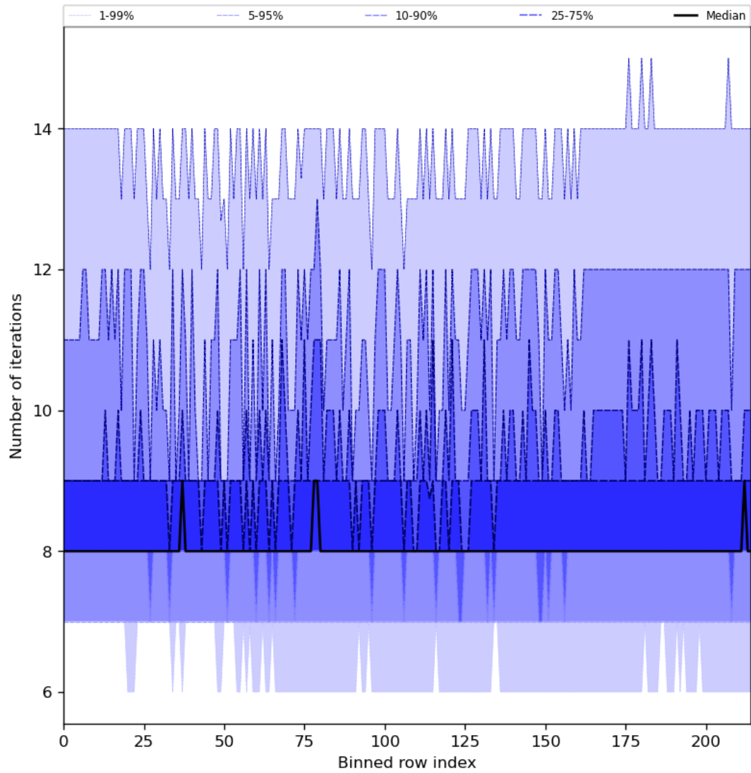
Figure 32: Along track statistics of “Number of iterations” for 2024-02-27 to 2024-02-29
