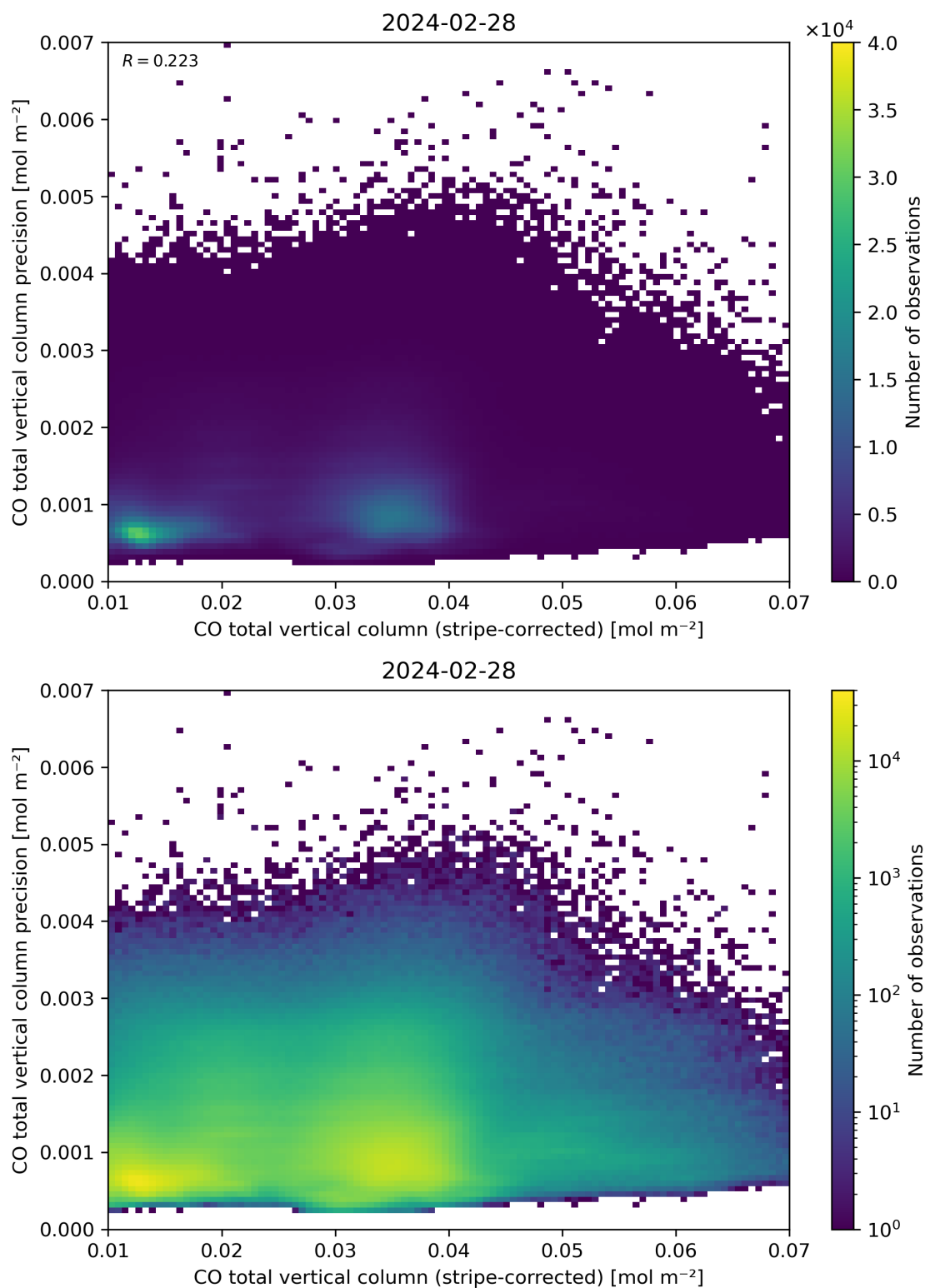
Figure 36: Scatter density plot of “CO total vertical column (stripe-corrected)” against “CO total vertical column precision” for 2024-02-27 to 2024-02-29.
