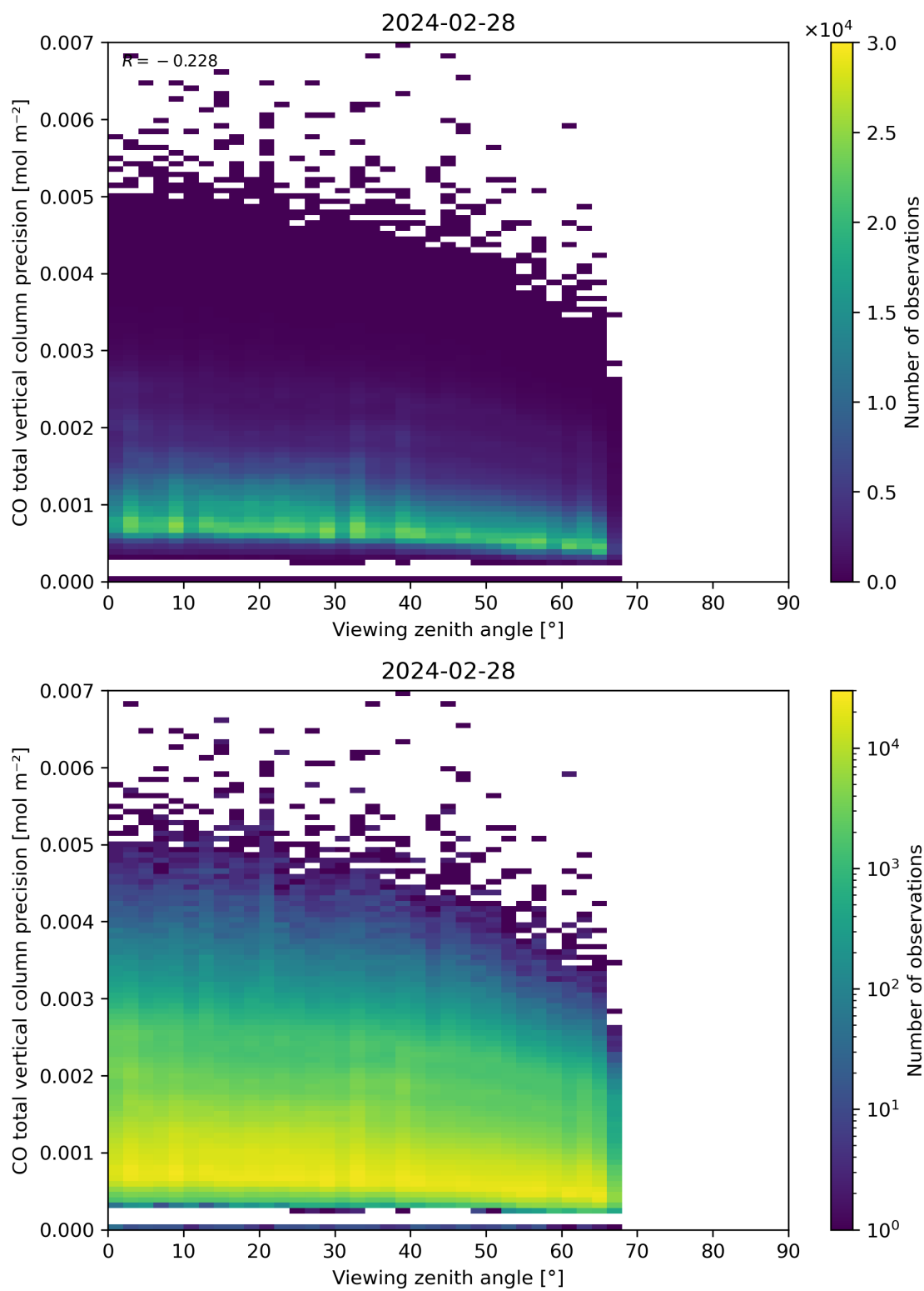
Figure 71: Scatter density plot of “Viewing zenith angle” against “CO total vertical column precision” for 2024-02-27 to 2024-02-29.
