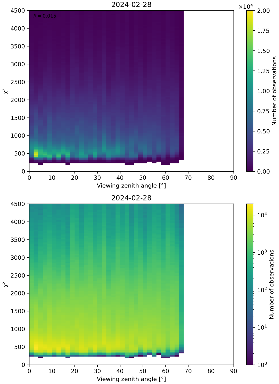
Figure 72: Scatter density plot of “Viewing zenith angle” against “ \chi^2 ” for 2024-02-27 to 2024-02-29.
