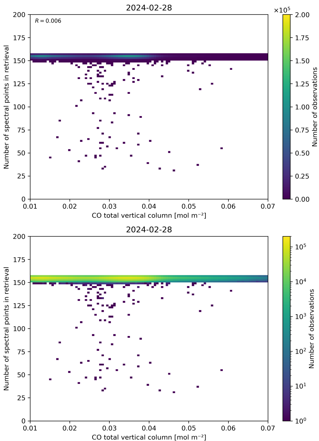
Figure 43: Scatter density plot of “CO total vertical column” against “Number of spectral points in retrieval” for 2024-02-27 to 2024-02-29.
