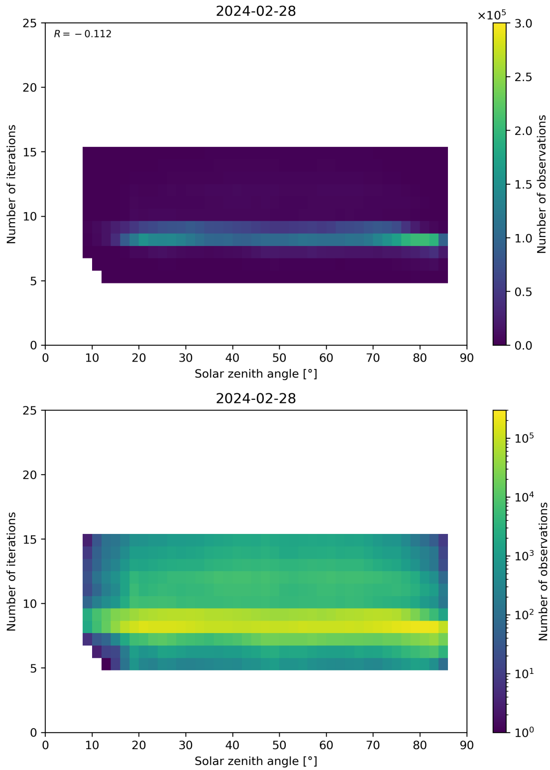
Figure 67: Scatter density plot of “Solar zenith angle” against “Number of iterations” for 2024-02-27 to 2024-02-29.
