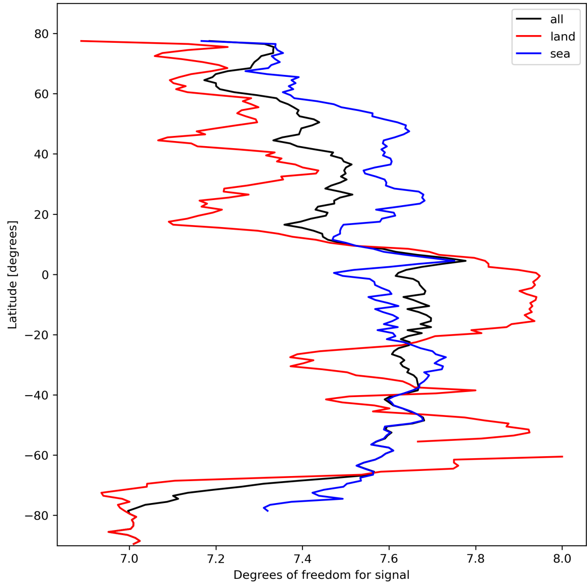
Figure 15: Zonal average of “Degrees of freedom for signal” for 2024-02-27 to 2024-02-29.
