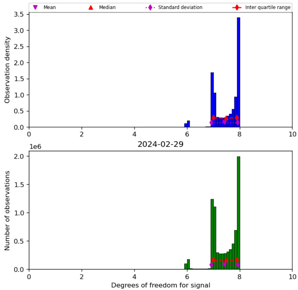
Figure 23: Histogram of “Degrees of freedom for signal” for 2024-02-28 to 2024-03-01
