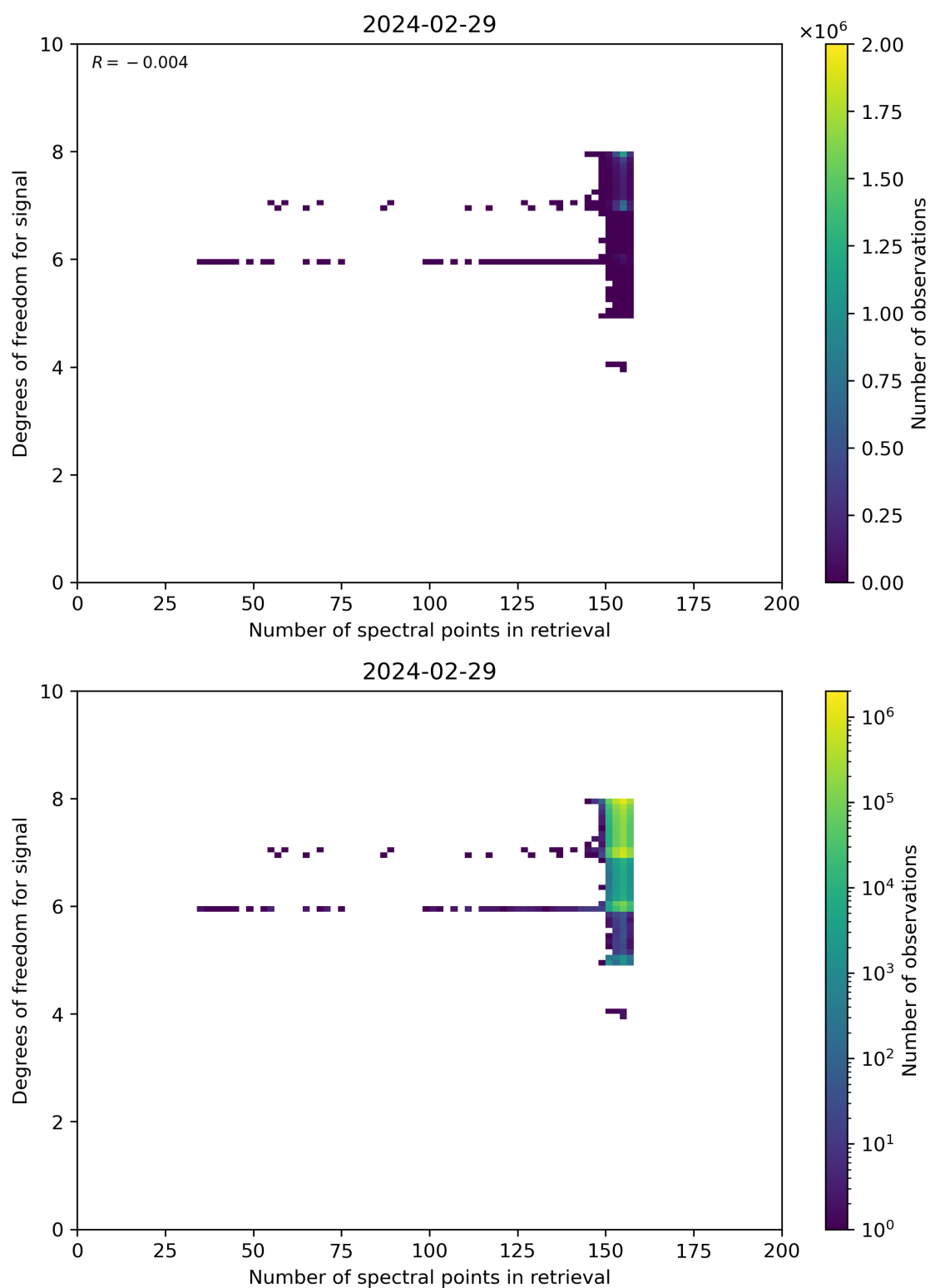
Figure 59: Scatter density plot of “Number of spectral points in retrieval” against “Degrees of freedom for signal” for 2024-02-28 to 2024-03-01.
