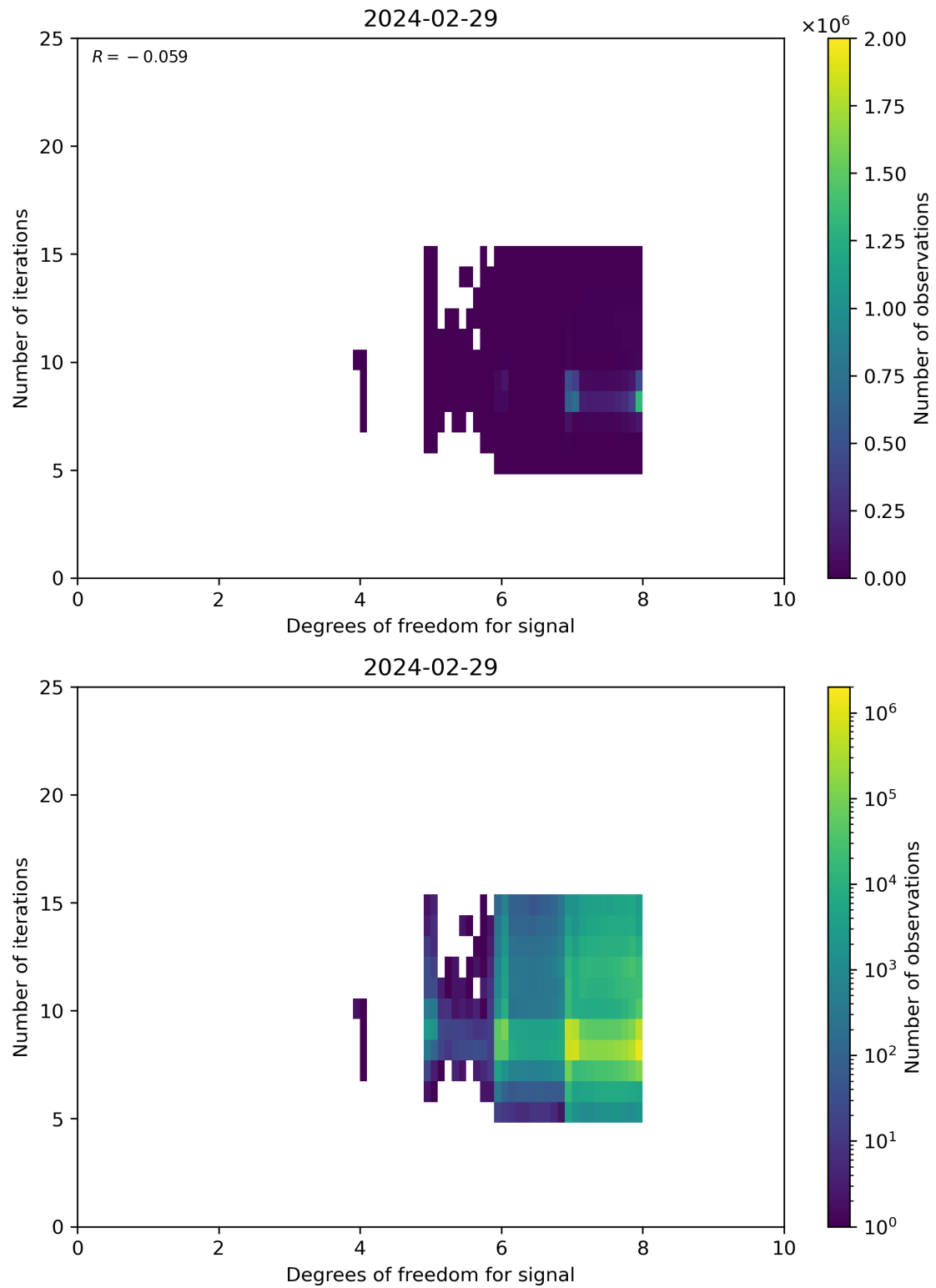
Figure 50: Scatter density plot of “Degrees of freedom for signal” against “Number of iterations” for 2024-02-28 to 2024-03-01.
