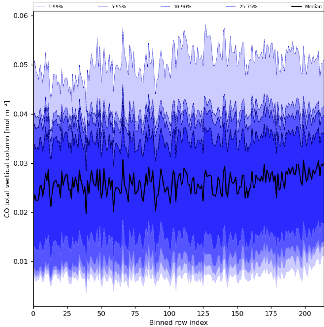
Figure 26: Along track statistics of “CO total vertical column” for 2024-02-28 to 2024-03-01
