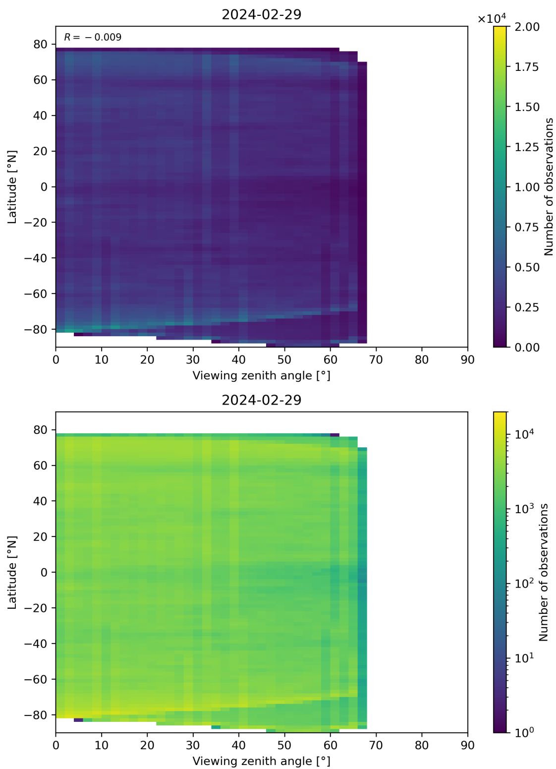
Figure 74: Scatter density plot of “Viewing zenith angle” against “Latitude” for 2024-02-28 to 2024-03-01.
