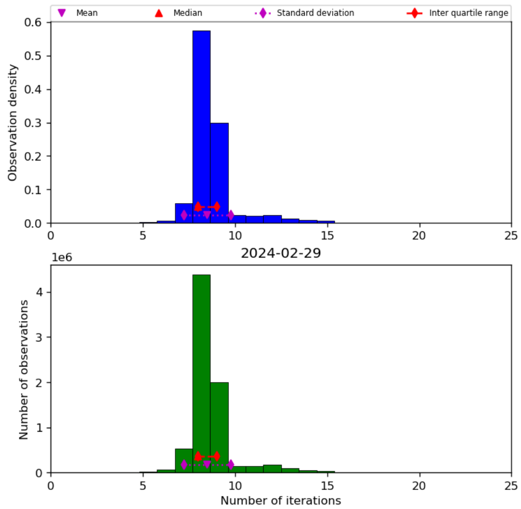
Figure 24: Histogram of “Number of iterations” for 2024-02-28 to 2024-03-01
