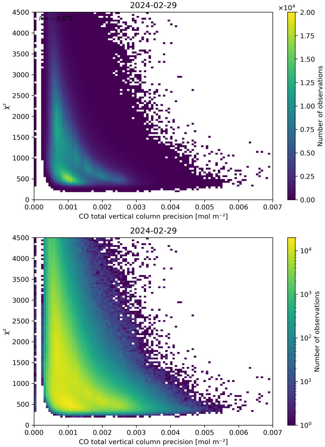
Figure 44: Scatter density plot of “CO total vertical column precision” against “ \chi^2 ” for 2024-02-28 to 2024-03-01.
