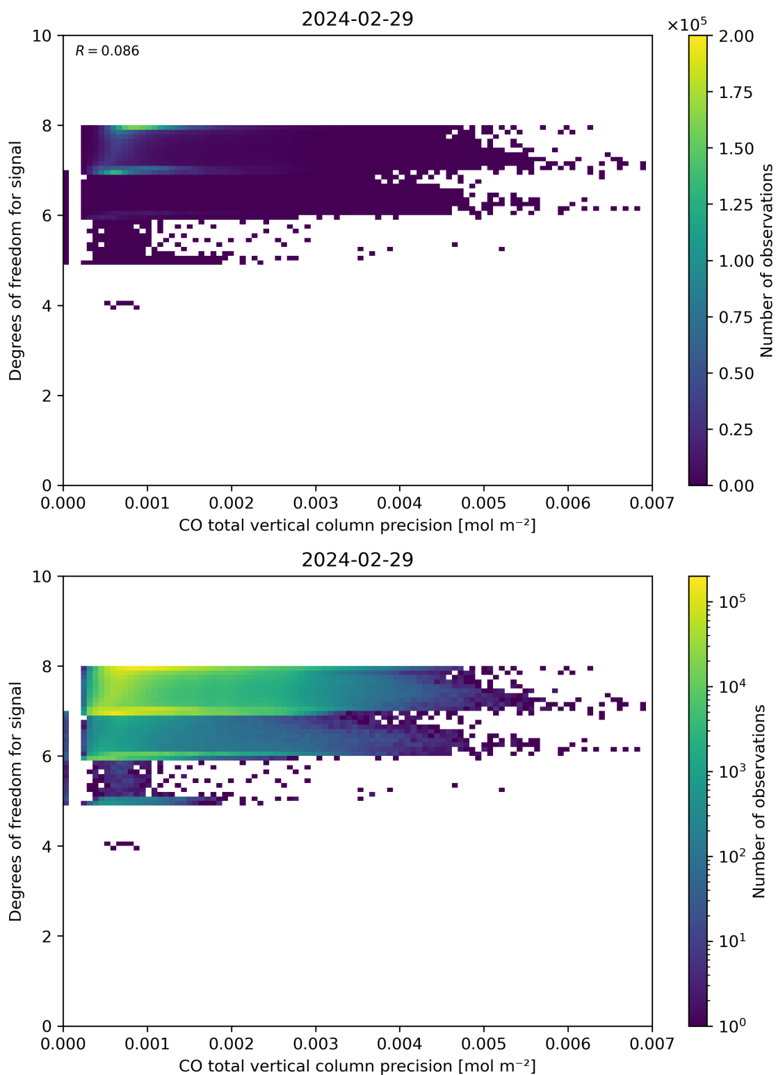
Figure 45: Scatter density plot of “CO total vertical column precision” against “Degrees of freedom for signal” for 2024-02-28 to 2024-03-01.
