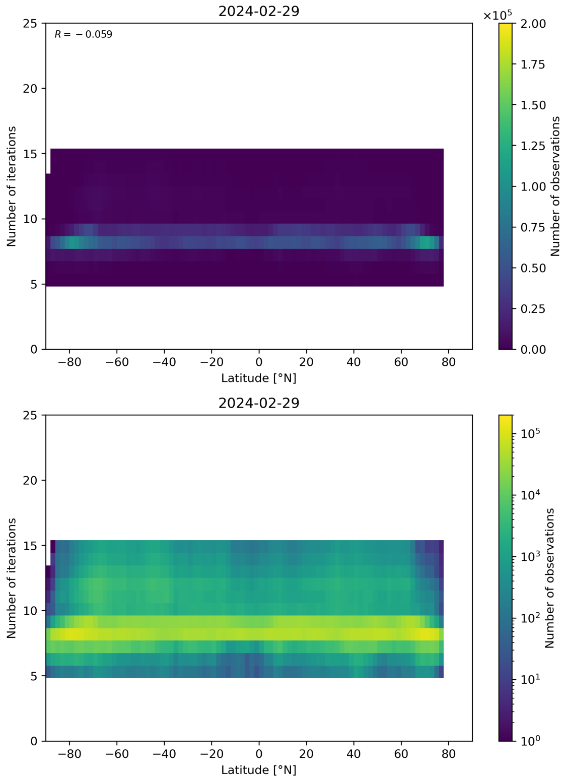
Figure 56: Scatter density plot of “Latitude” against “Number of iterations” for 2024-02-28 to 2024-03-01.
