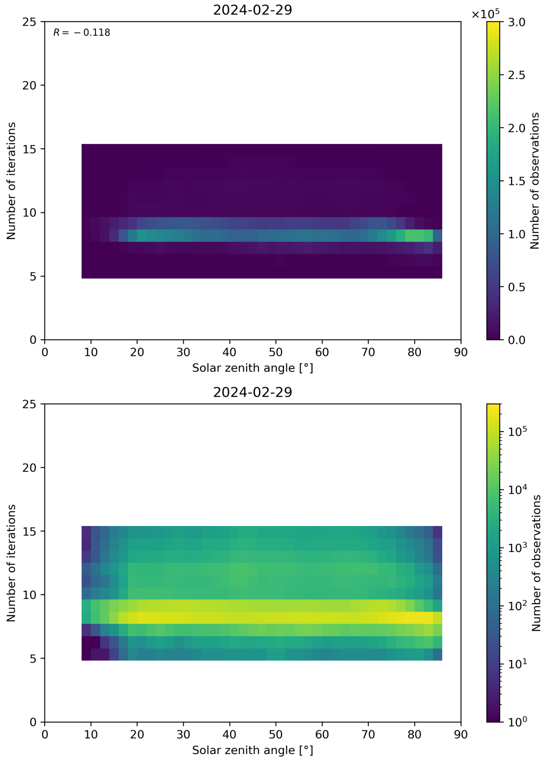
Figure 67: Scatter density plot of “Solar zenith angle” against “Number of iterations” for 2024-02-28 to 2024-03-01.
