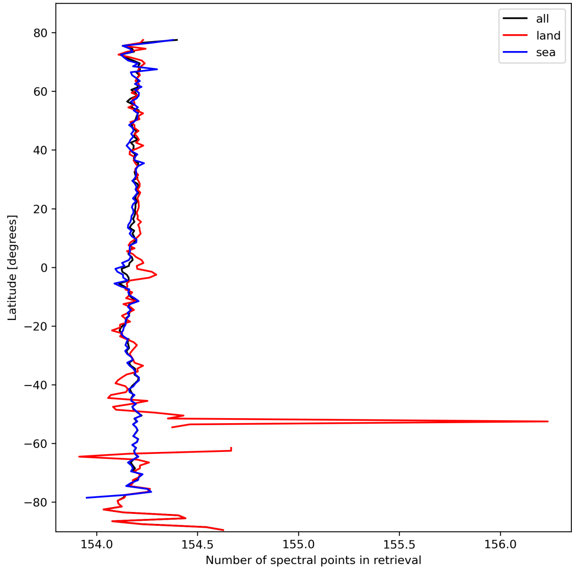
Figure 13: Zonal average of “Number of spectral points in retrieval” for 2024-02-28 to 2024-03-01.
