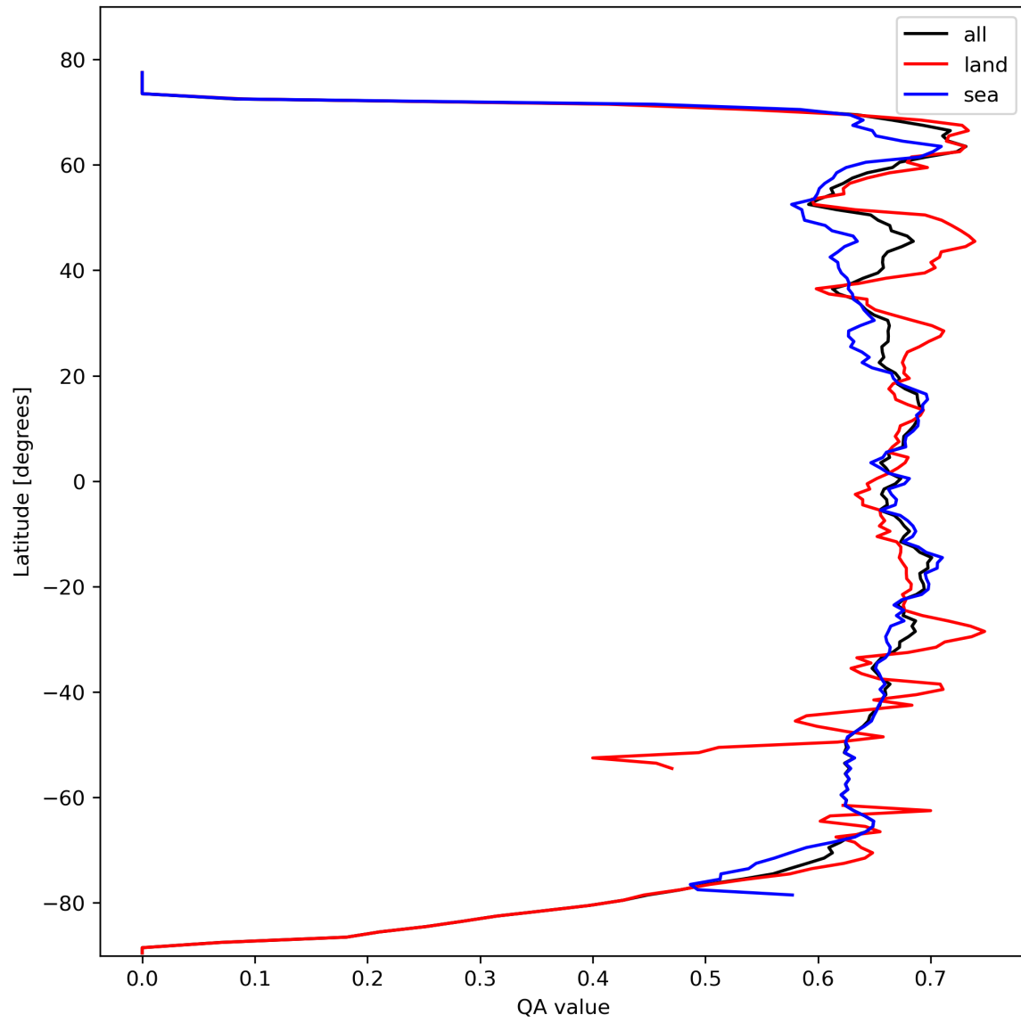
Figure 9: Zonal average of “QA value” for 2024-02-28 to 2024-03-01.
