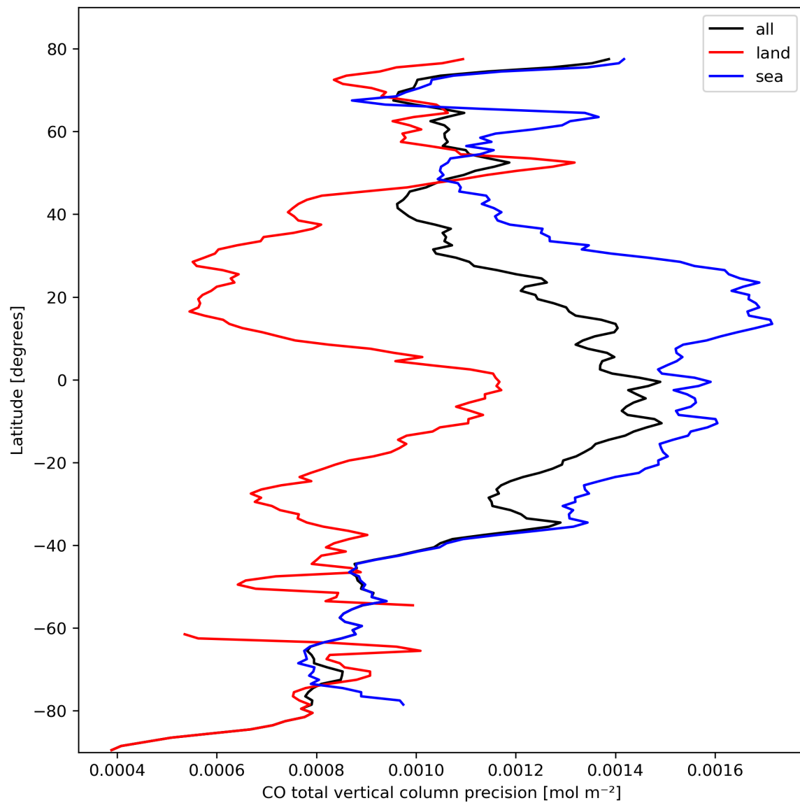
Figure 12: Zonal average of “CO total vertical column precision” for 2024-02-28 to 2024-03-01.
