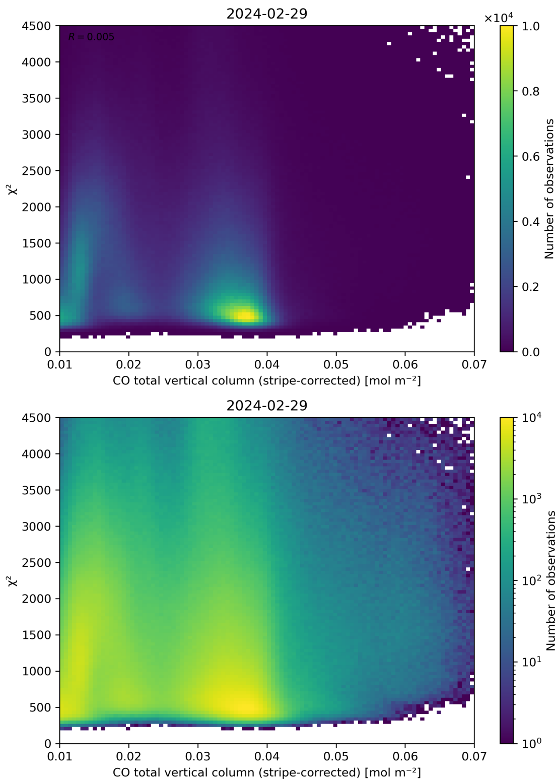
Figure 37: Scatter density plot of “CO total vertical column (stripe-corrected)” against “ \chi^2 ” for 2024-02-28 to 2024-03-01.
