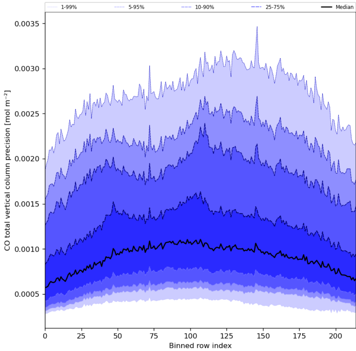
Figure 28: Along track statistics of “CO total vertical column precision” for 2024-02-28 to 2024-03-01
