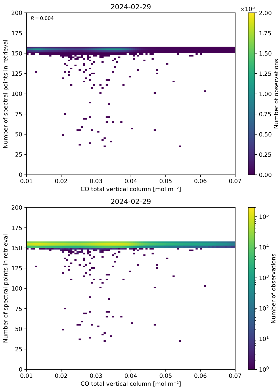
Figure 43: Scatter density plot of “CO total vertical column” against “Number of spectral points in retrieval” for 2024-02-28 to 2024-03-01.
