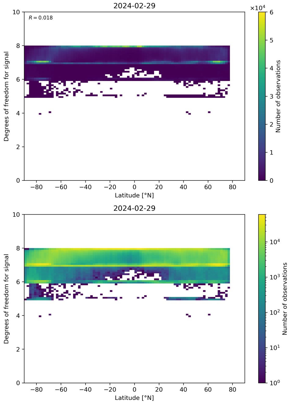
Figure 55: Scatter density plot of “Latitude” against “Degrees of freedom for signal” for 2024-02-28 to 2024-03-01.
