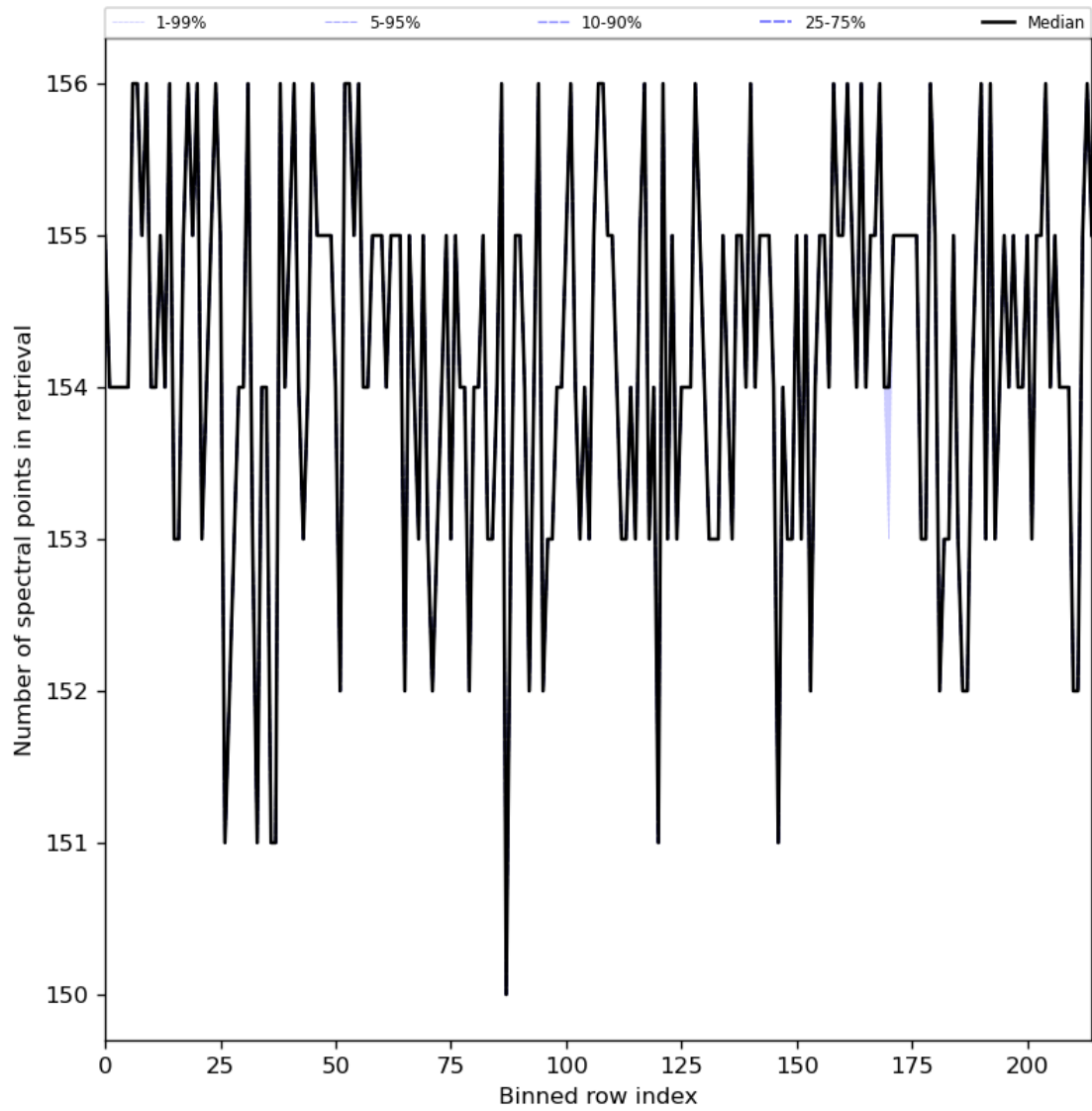
Figure 29: Along track statistics of “Number of spectral points in retrieval” for 2024-02-28 to 2024-03-01
