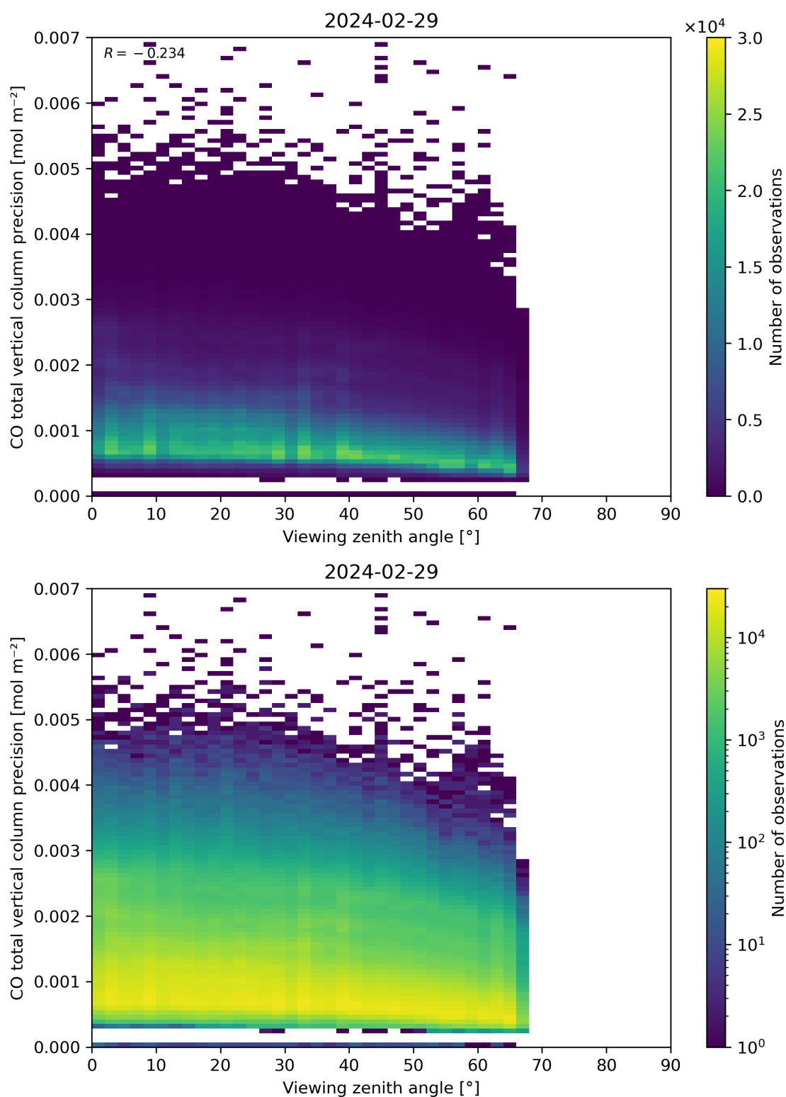
Figure 71: Scatter density plot of “Viewing zenith angle” against “CO total vertical column precision” for 2024-02-28 to 2024-03-01.
