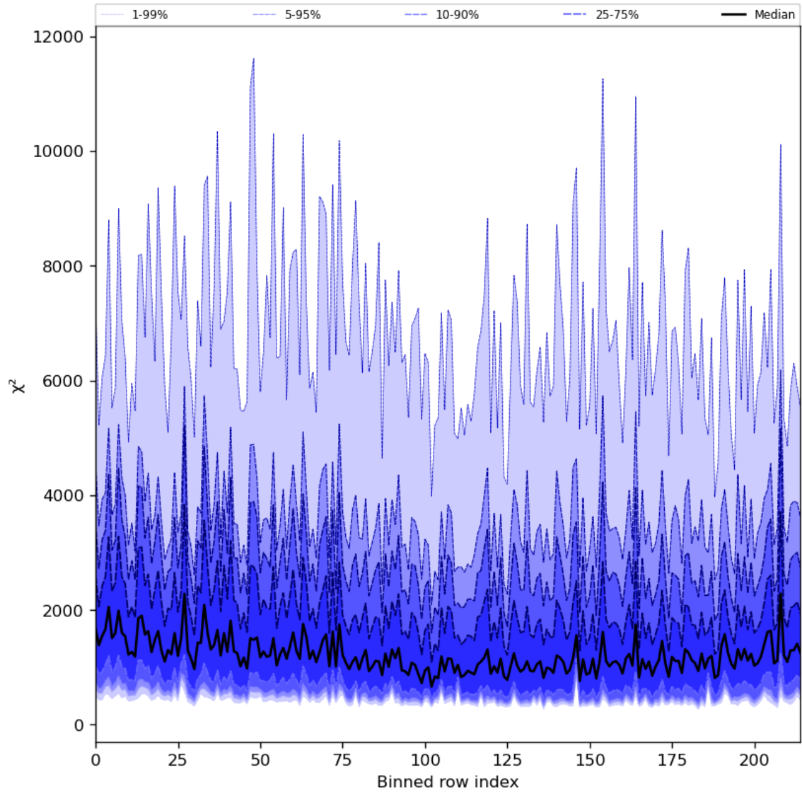
Figure 30: Along track statistics of “ \chi^2 ” for 2024-02-28 to 2024-03-01
