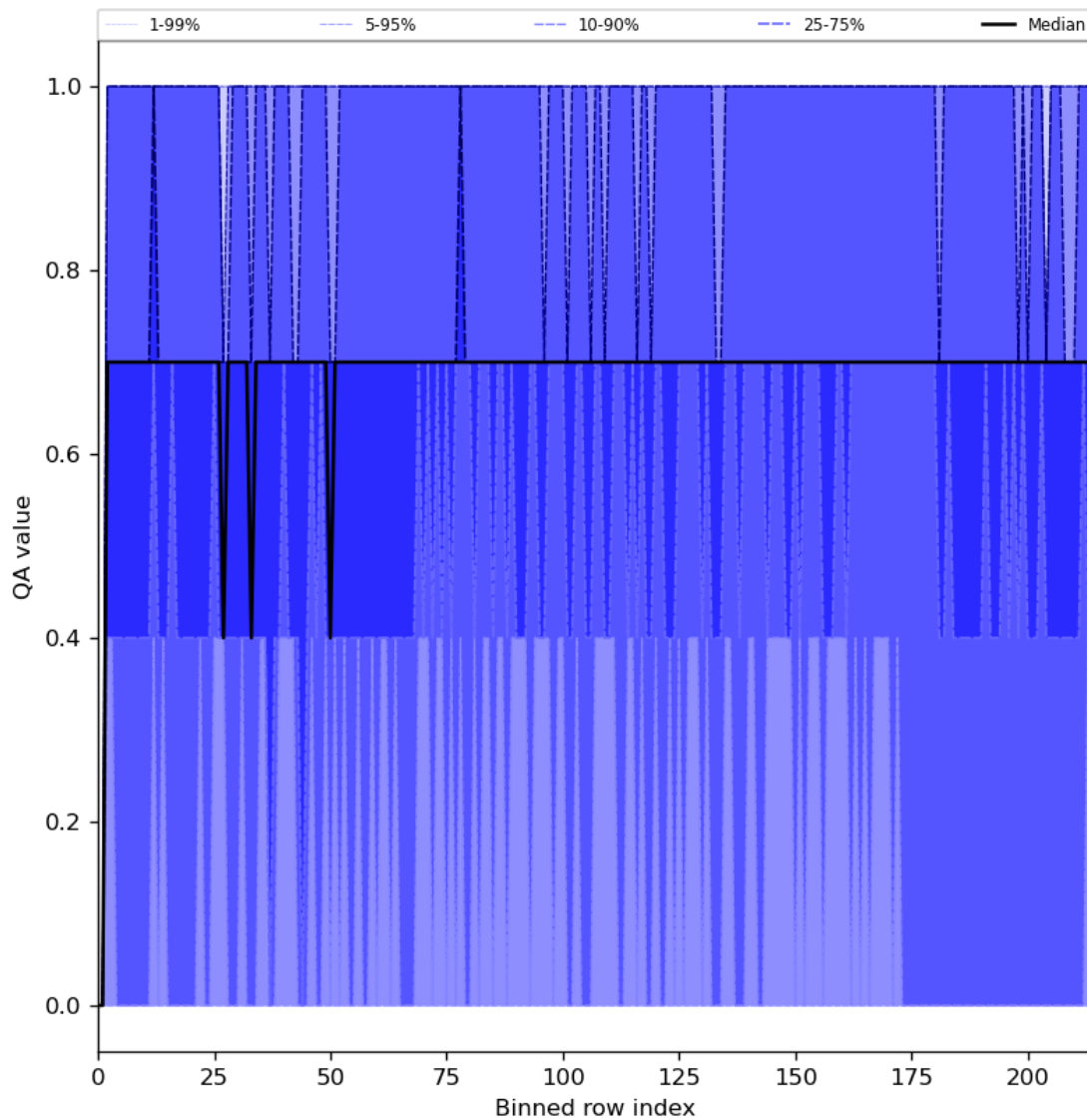
Figure 25: Along track statistics of “QA value” for 2024-02-28 to 2024-03-01
