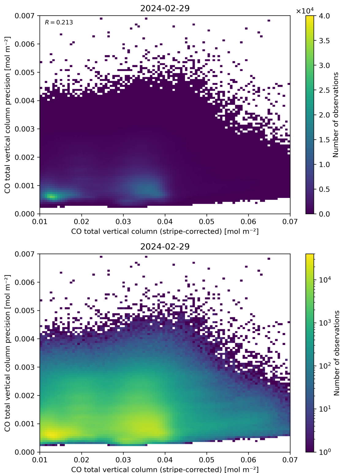
Figure 36: Scatter density plot of “CO total vertical column (stripe-corrected)” against “CO total vertical column precision” for 2024-02-28 to 2024-03-01.
