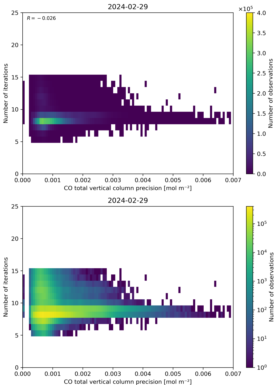
Figure 46: Scatter density plot of “CO total vertical column precision” against “Number of iterations” for 2024-02-28 to 2024-03-01.
