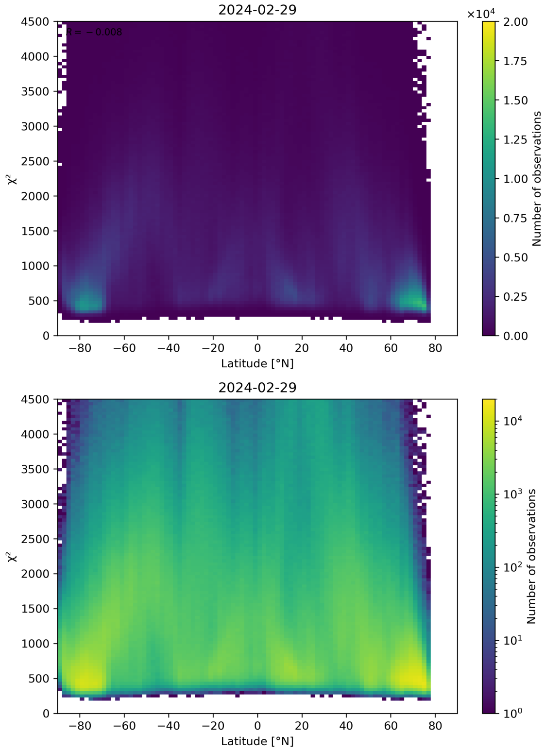
Figure 54: Scatter density plot of “Latitude” against “ \chi^2 ” for 2024-02-28 to 2024-03-01.
