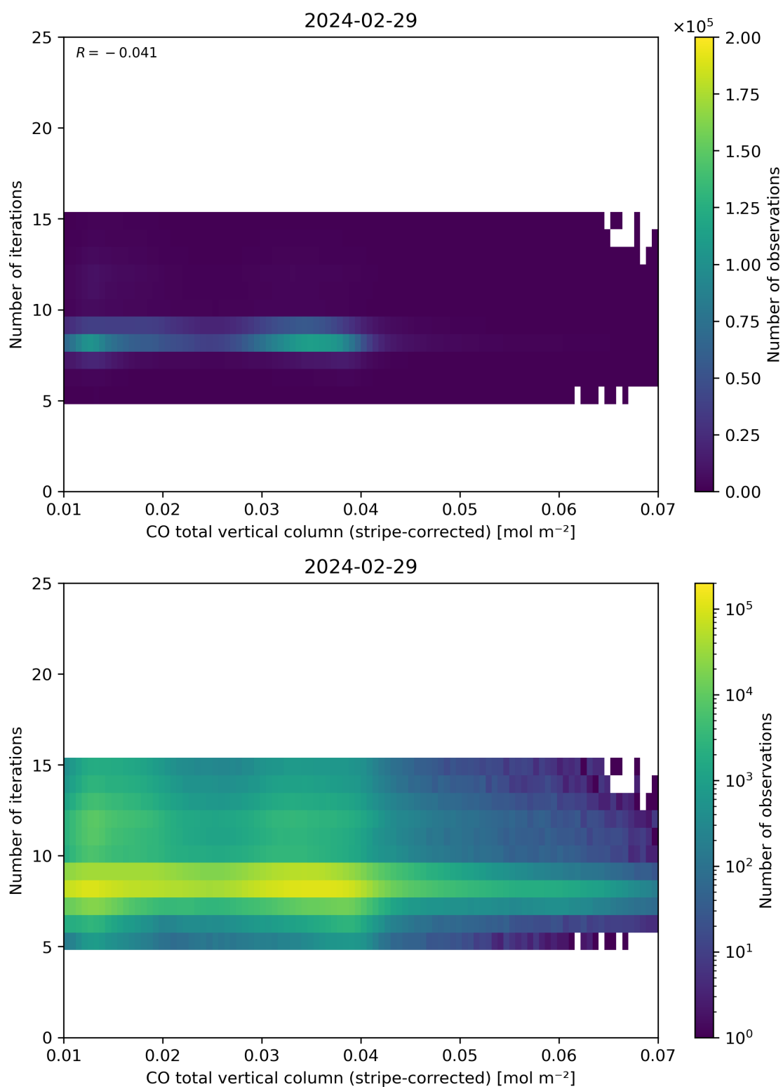
Figure 39: Scatter density plot of “CO total vertical column (stripe-corrected)” against “Number of iterations” for 2024-02-28 to 2024-03-01.
