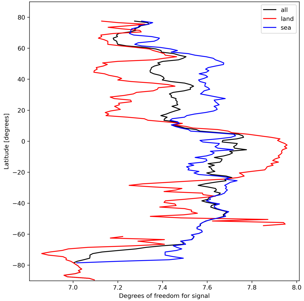
Figure 15: Zonal average of “Degrees of freedom for signal” for 2024-02-28 to 2024-03-01.
