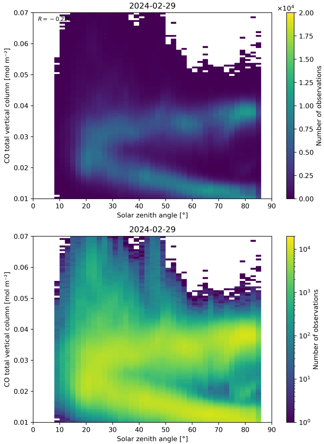
Figure 61: Scatter density plot of “Solar zenith angle” against “CO total vertical column” for 2024-02-28 to 2024-03-01.
