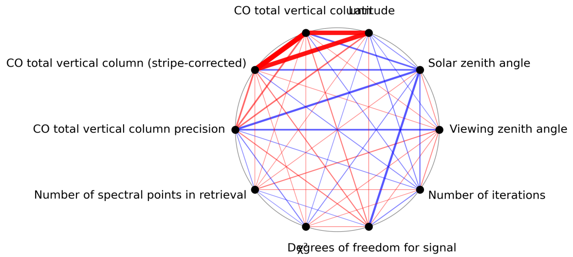
Figure 1: Map of correlation graph for 2024-02-28 to 2024-03-01.
