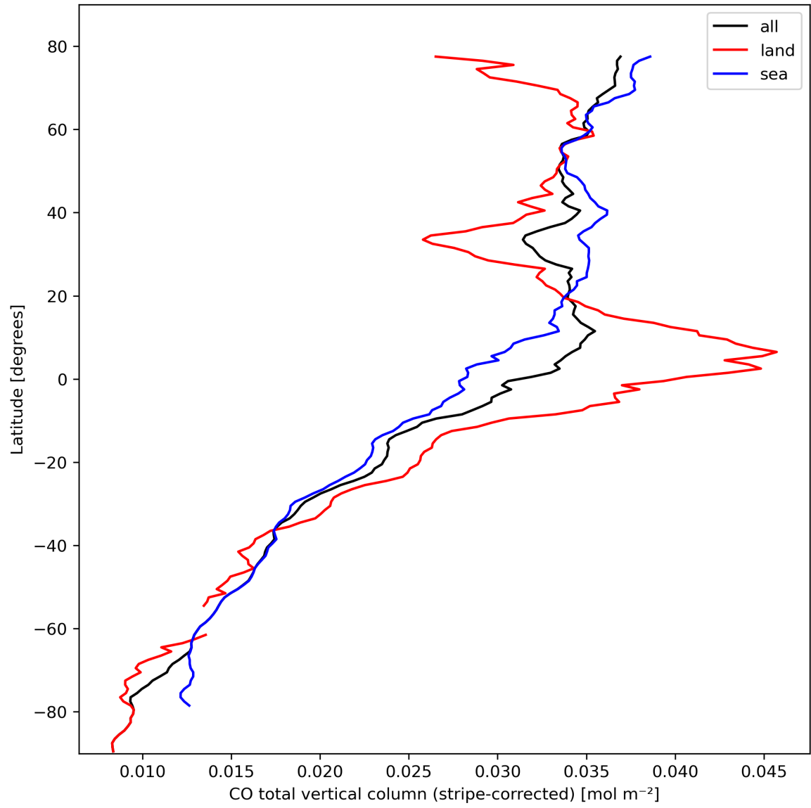
Figure 11: Zonal average of “CO total vertical column (stripe-corrected)” for 2024-02-28 to 2024-03-01.
