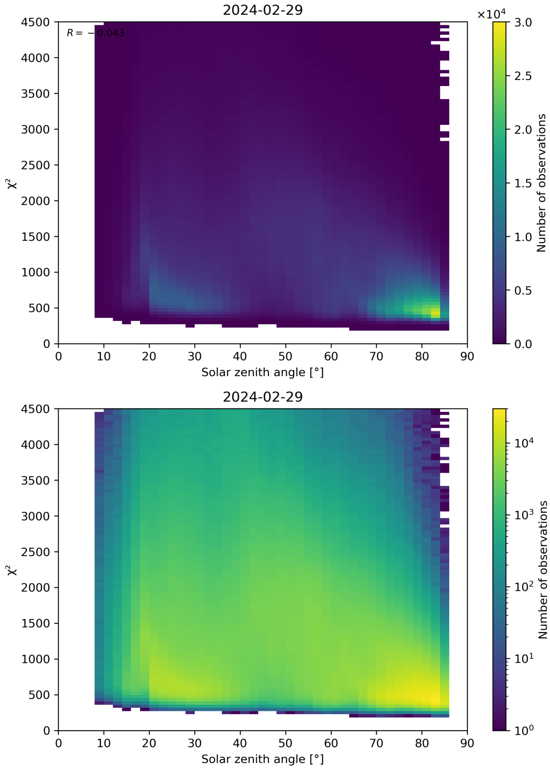
Figure 64: Scatter density plot of “Solar zenith angle” against “ \chi^2 ” for 2024-02-28 to 2024-03-01.
