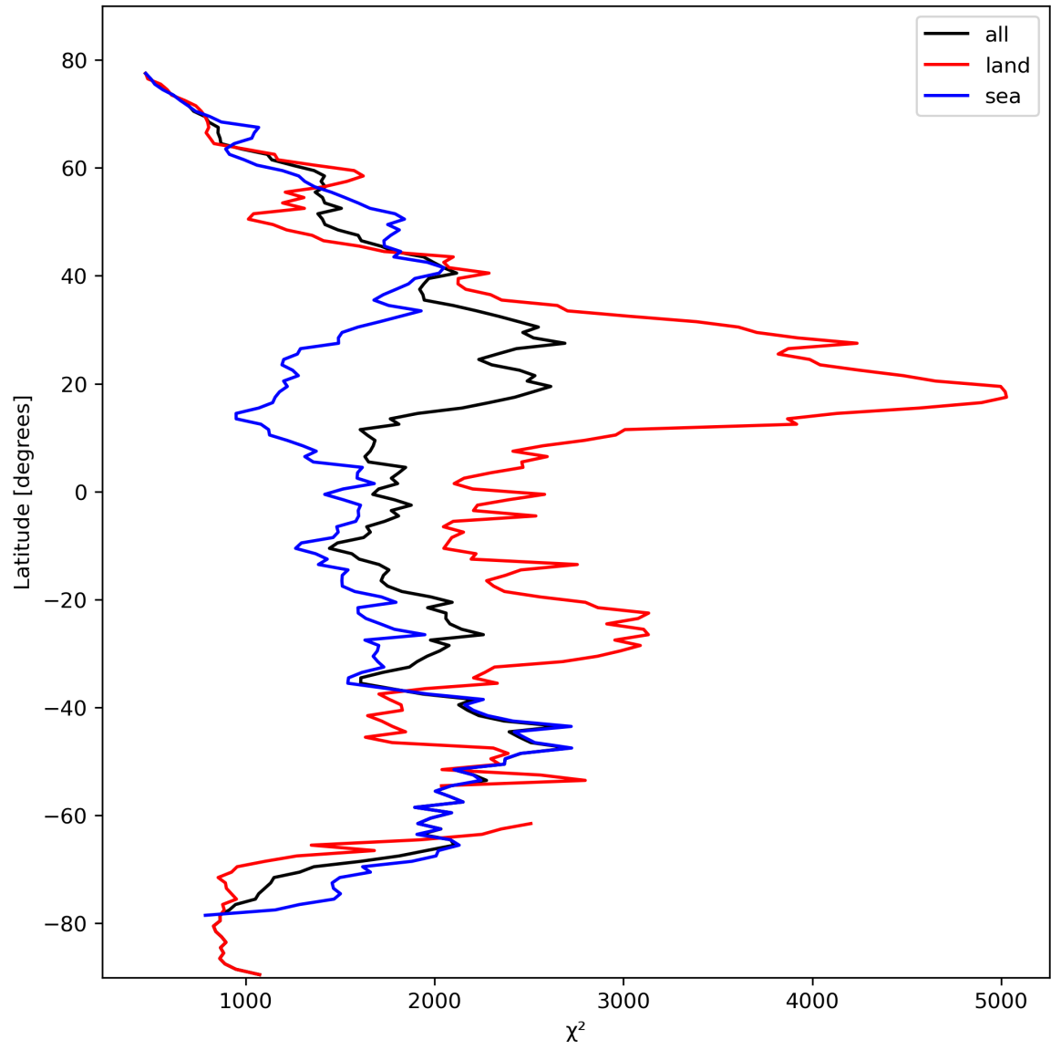
Figure 14: Zonal average of “ \chi^2 ” for 2024-02-28 to 2024-03-01.
