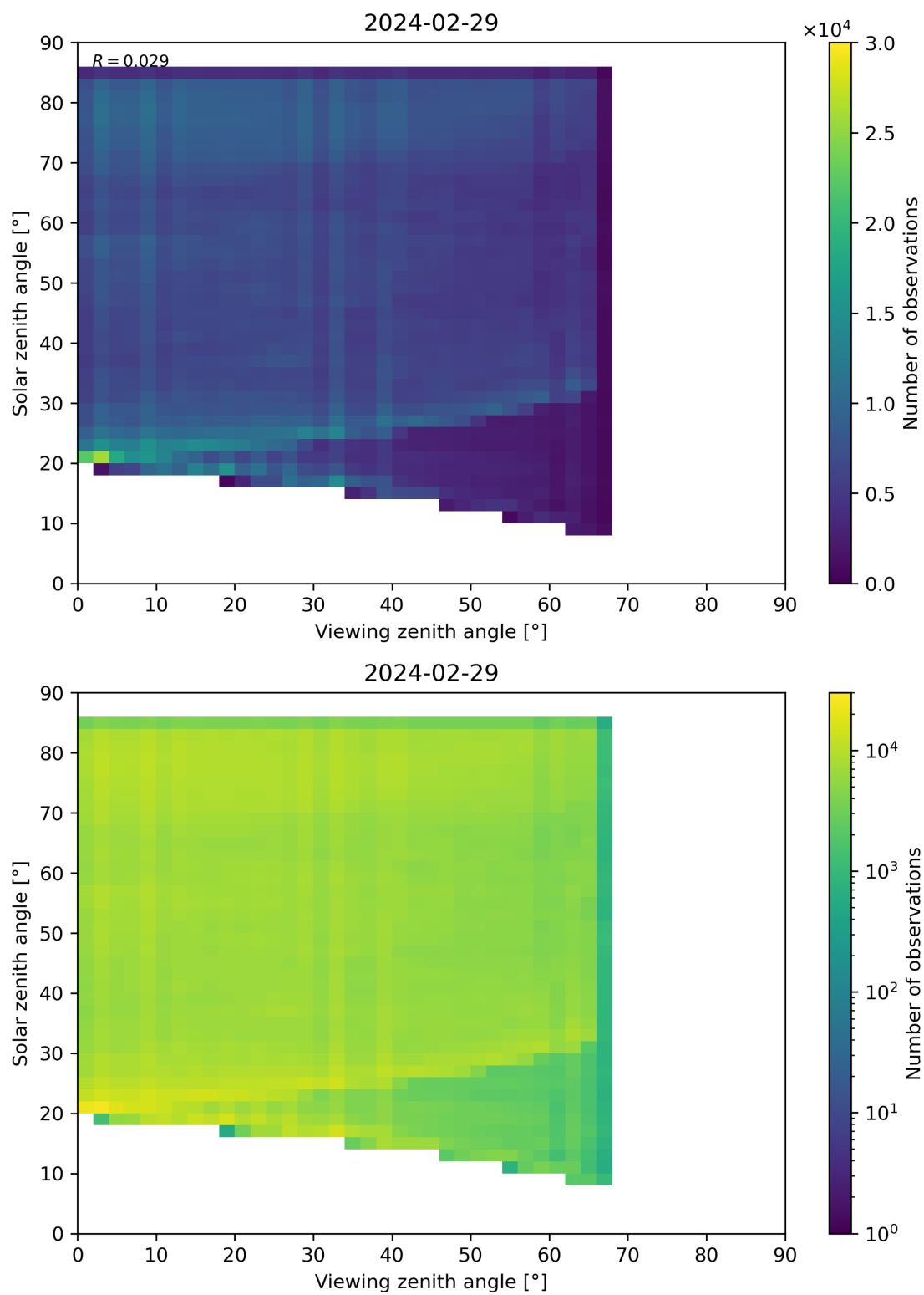
Figure 77: Scatter density plot of “Viewing zenith angle” against “Solar zenith angle” for 2024-02-28 to 2024-03-01.
