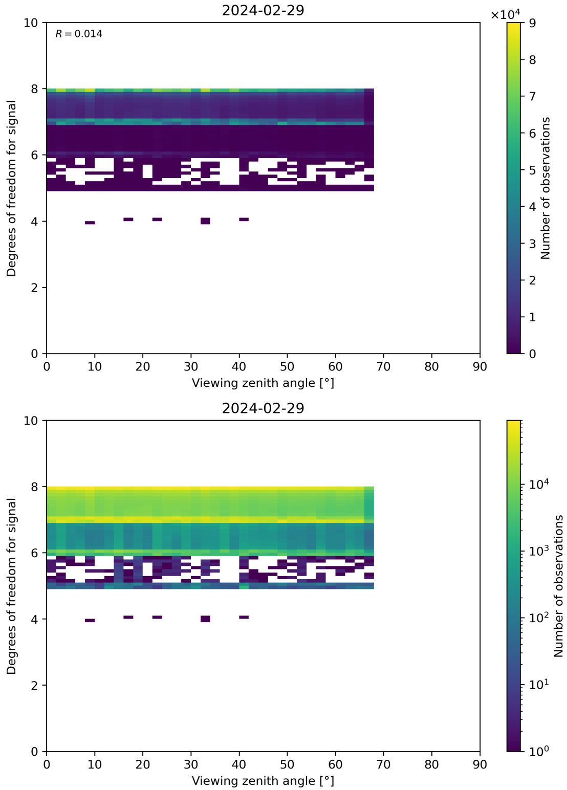
Figure 73: Scatter density plot of “Viewing zenith angle” against “Degrees of freedom for signal” for 2024-02-28 to 2024-03-01.
