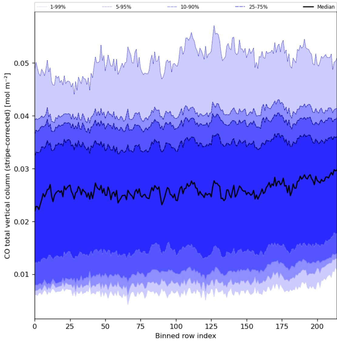
Figure 27: Along track statistics of “CO total vertical column (stripe-corrected)” for 2024-02-28 to 2024-03-01
