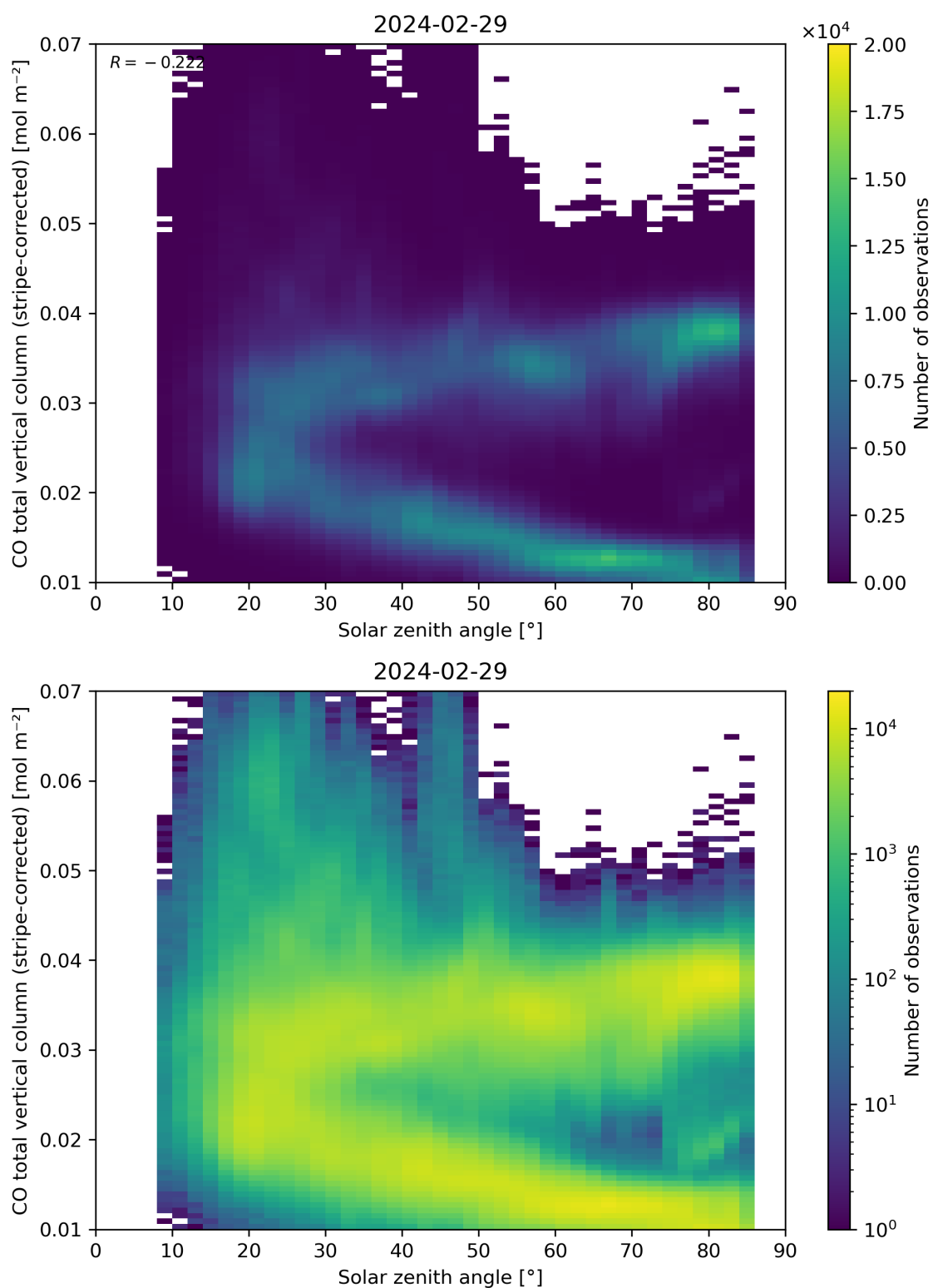
Figure 62: Scatter density plot of “Solar zenith angle” against “CO total vertical column (stripe-corrected)” for 2024-02-28 to 2024-03-01.
