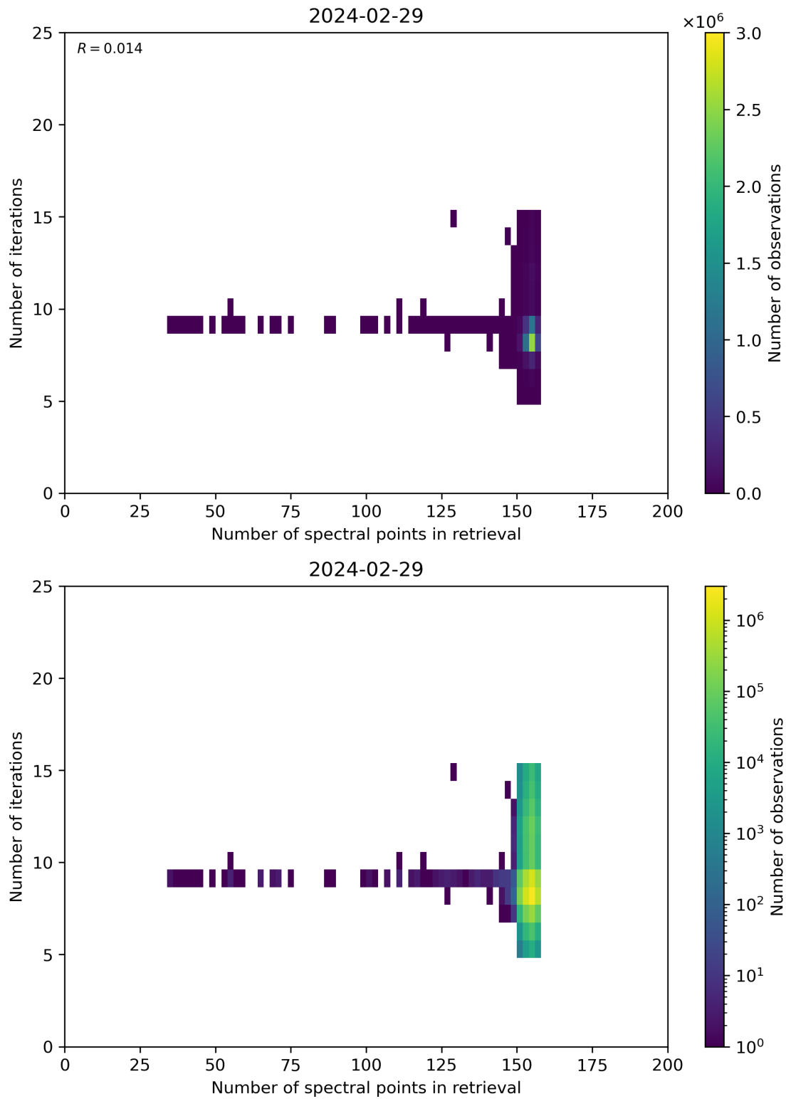
Figure 60: Scatter density plot of “Number of spectral points in retrieval” against “Number of iterations” for 2024-02-28 to 2024-03-01.
