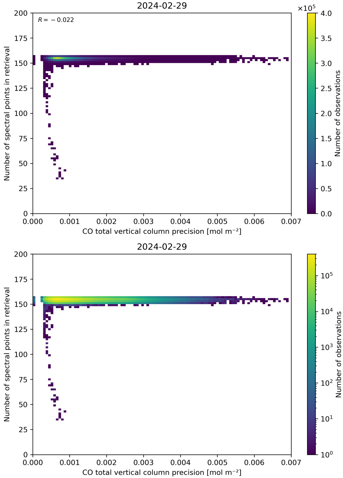
Figure 47: Scatter density plot of “CO total vertical column precision” against “Number of spectral points in retrieval” for 2024-02-28 to 2024-03-01.
