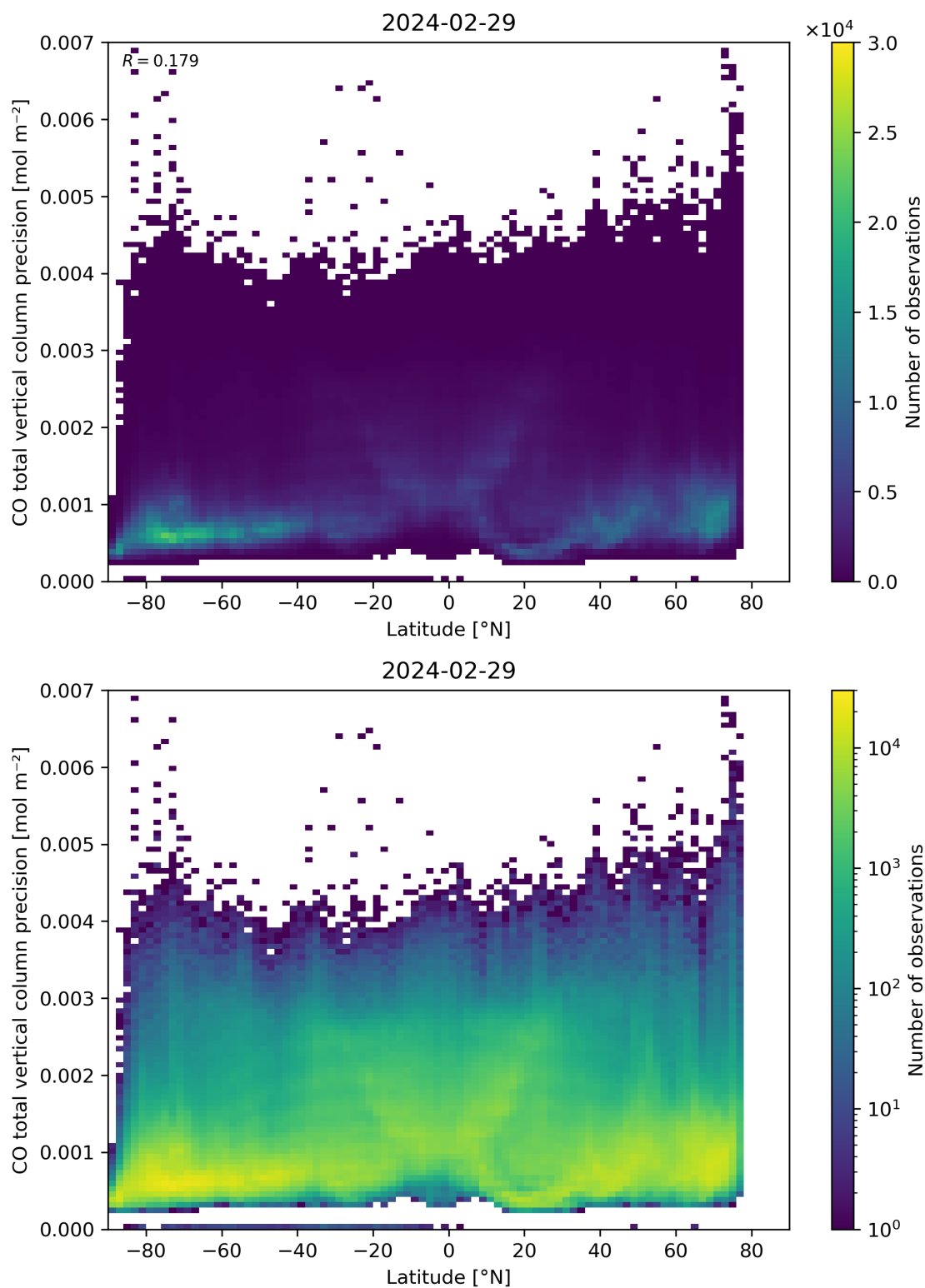
Figure 53: Scatter density plot of “Latitude” against “CO total vertical column precision” for 2024-02-28 to 2024-03-01.
