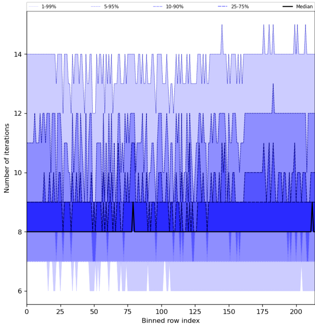
Figure 32: Along track statistics of “Number of iterations” for 2024-02-28 to 2024-03-01
