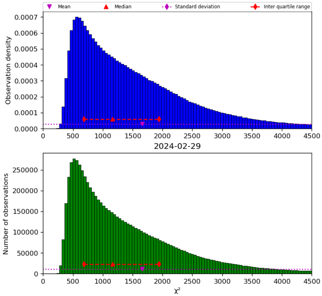
Figure 22: Histogram of “ \chi^2 ” for 2024-02-28 to 2024-03-01
