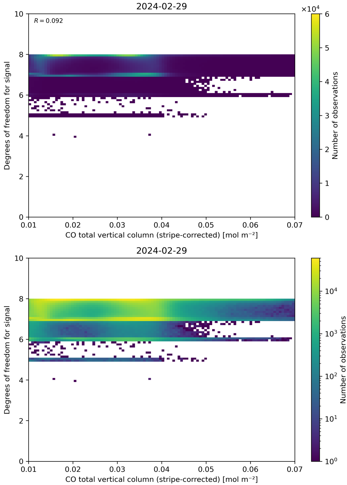
Figure 38: Scatter density plot of “CO total vertical column (stripe-corrected)” against “Degrees of freedom for signal” for 2024-02-28 to 2024-03-01.
