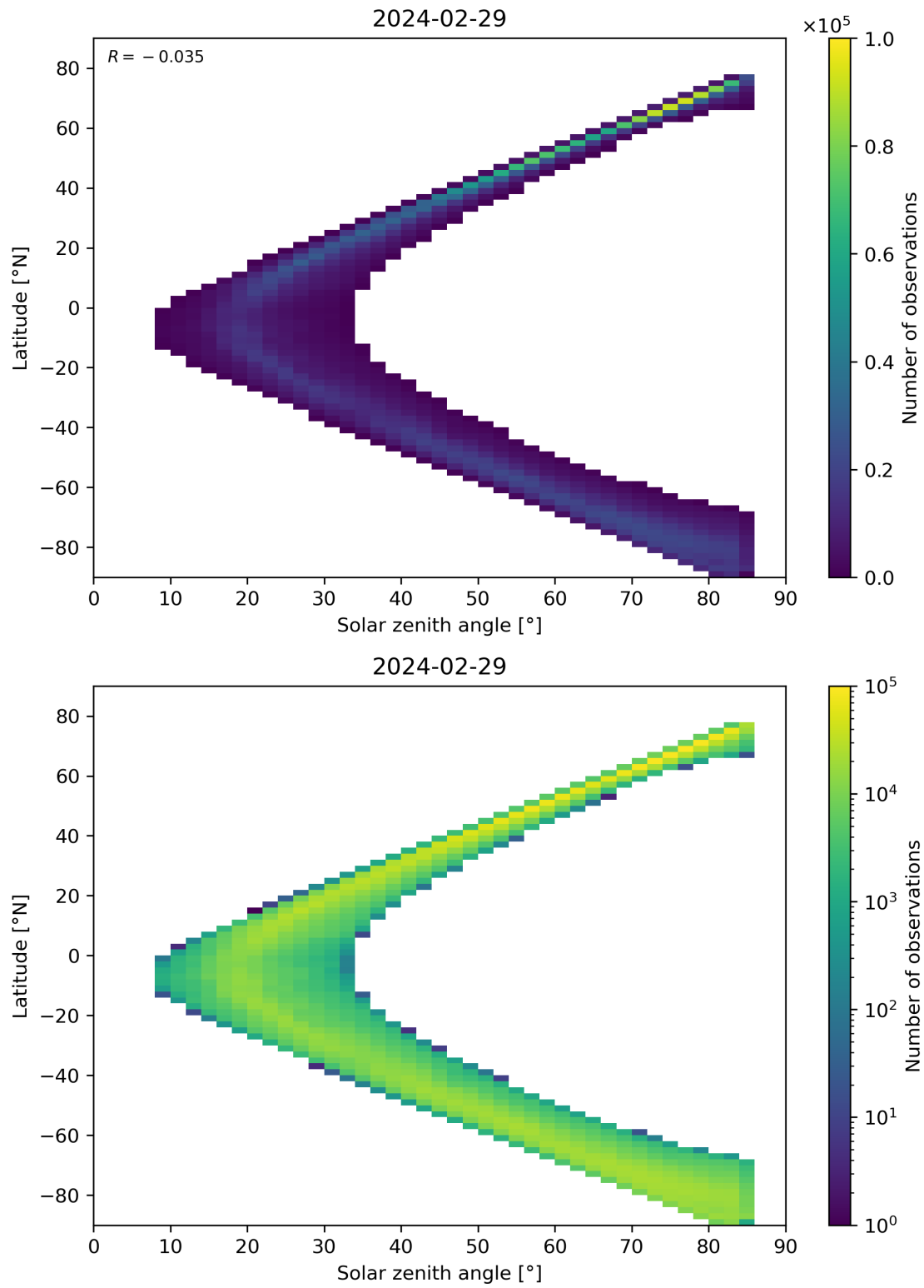
Figure 66: Scatter density plot of “Solar zenith angle” against “Latitude” for 2024-02-28 to 2024-03-01.
