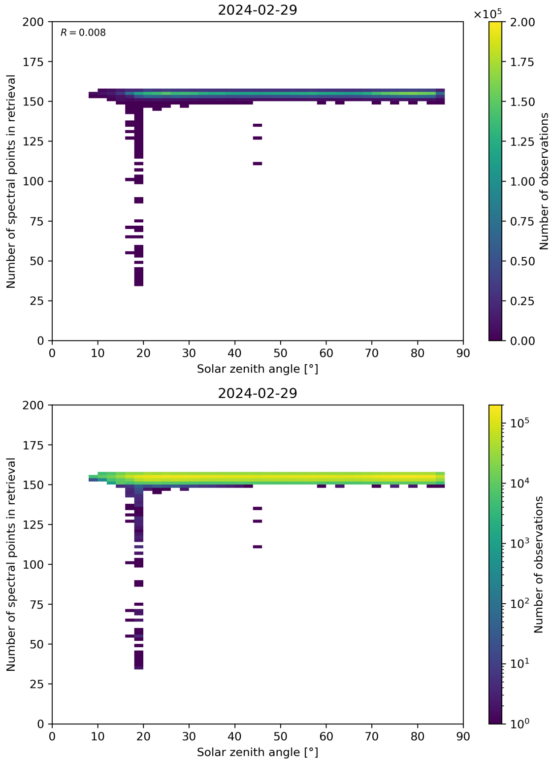
Figure 68: Scatter density plot of “Solar zenith angle” against “Number of spectral points in retrieval” for 2024-02-28 to 2024-03-01.
