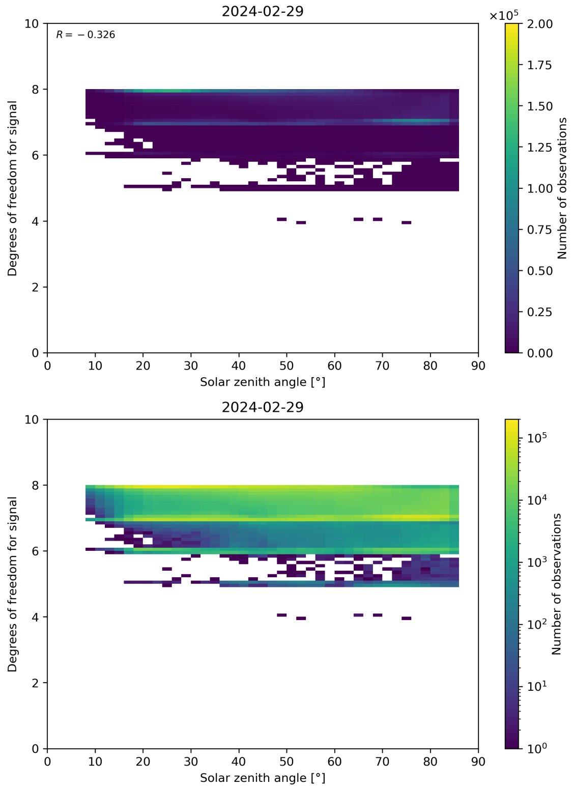
Figure 65: Scatter density plot of “Solar zenith angle” against “Degrees of freedom for signal” for 2024-02-28 to 2024-03-01.
