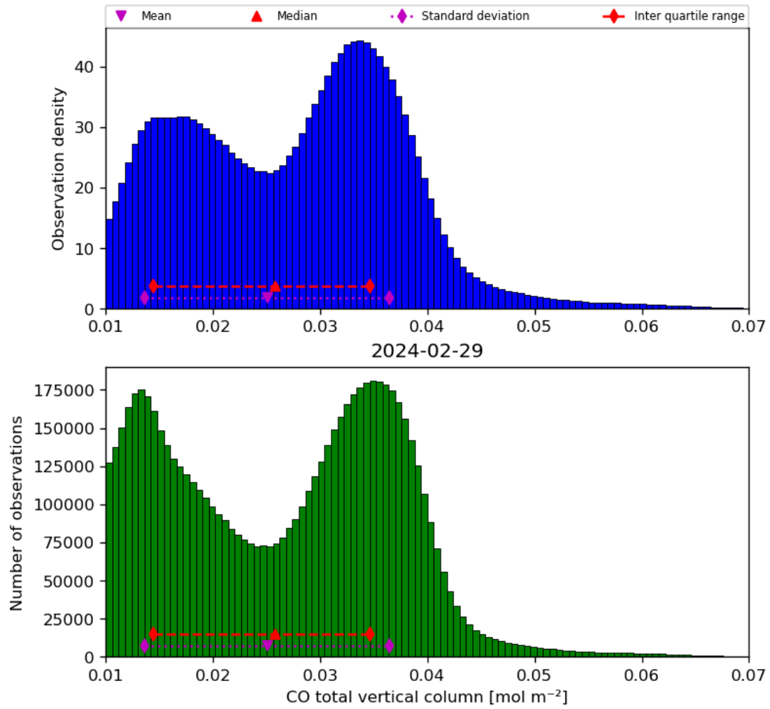
Figure 18: Histogram of “CO total vertical column” for 2024-02-28 to 2024-03-01
