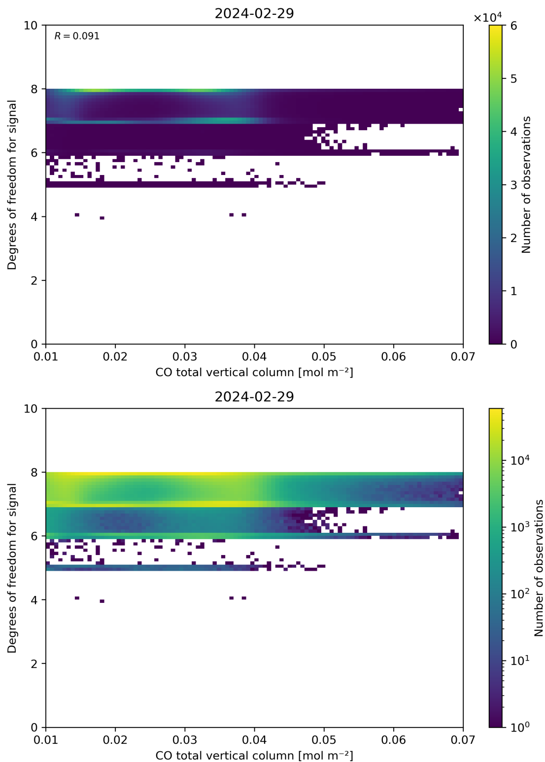
Figure 41: Scatter density plot of “CO total vertical column” against “Degrees of freedom for signal” for 2024-02-28 to 2024-03-01.
