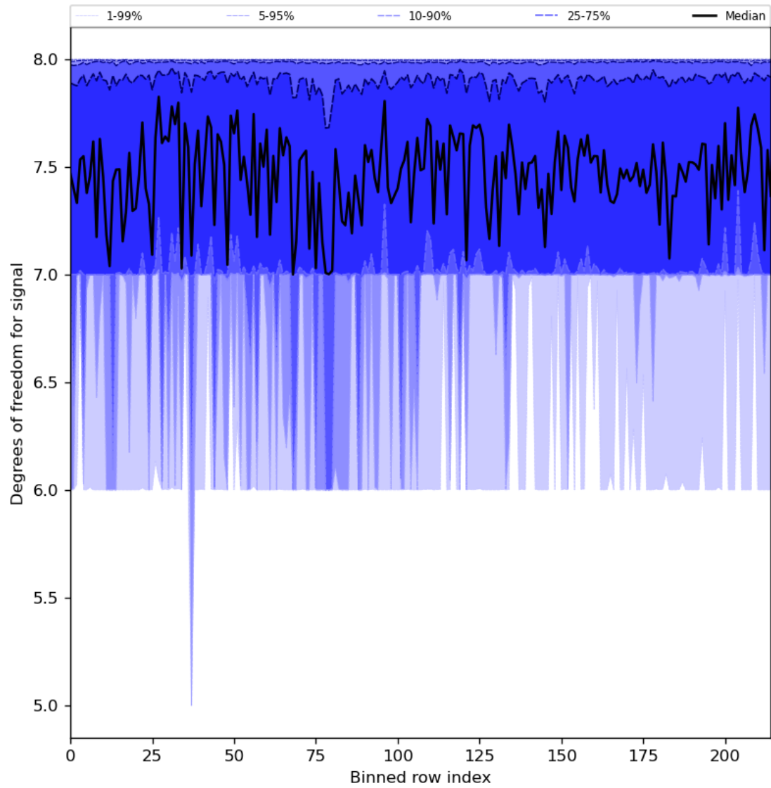
Figure 31: Along track statistics of “Degrees of freedom for signal” for 2024-02-28 to 2024-03-01
