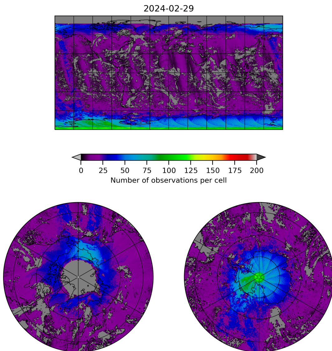
Figure 8: Map of the number of observations for 2024-02-28 to 2024-03-01
