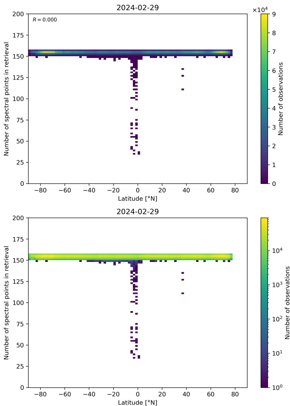
Figure 57: Scatter density plot of “Latitude” against “Number of spectral points in retrieval” for 2024-02-28 to 2024-03-01.
