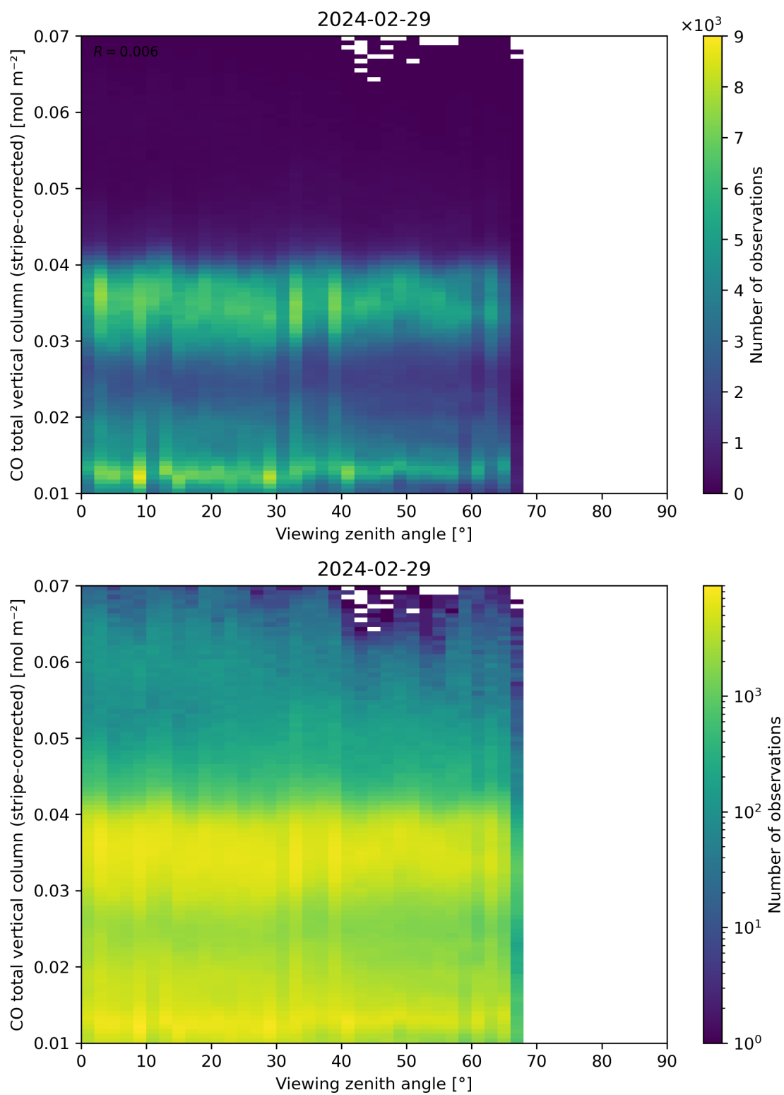
Figure 70: Scatter density plot of “Viewing zenith angle” against “CO total vertical column (stripe-corrected)” for 2024-02-28 to 2024-03-01.
