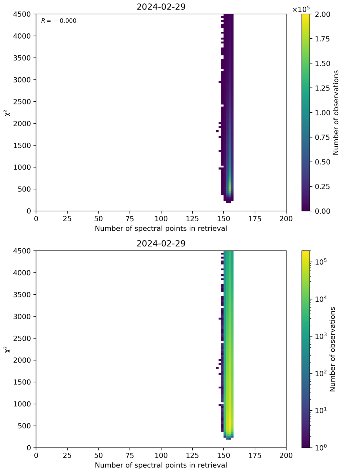
Figure 58: Scatter density plot of “Number of spectral points in retrieval” against “ \chi^2 ” for 2024-02-28 to 2024-03-01.
