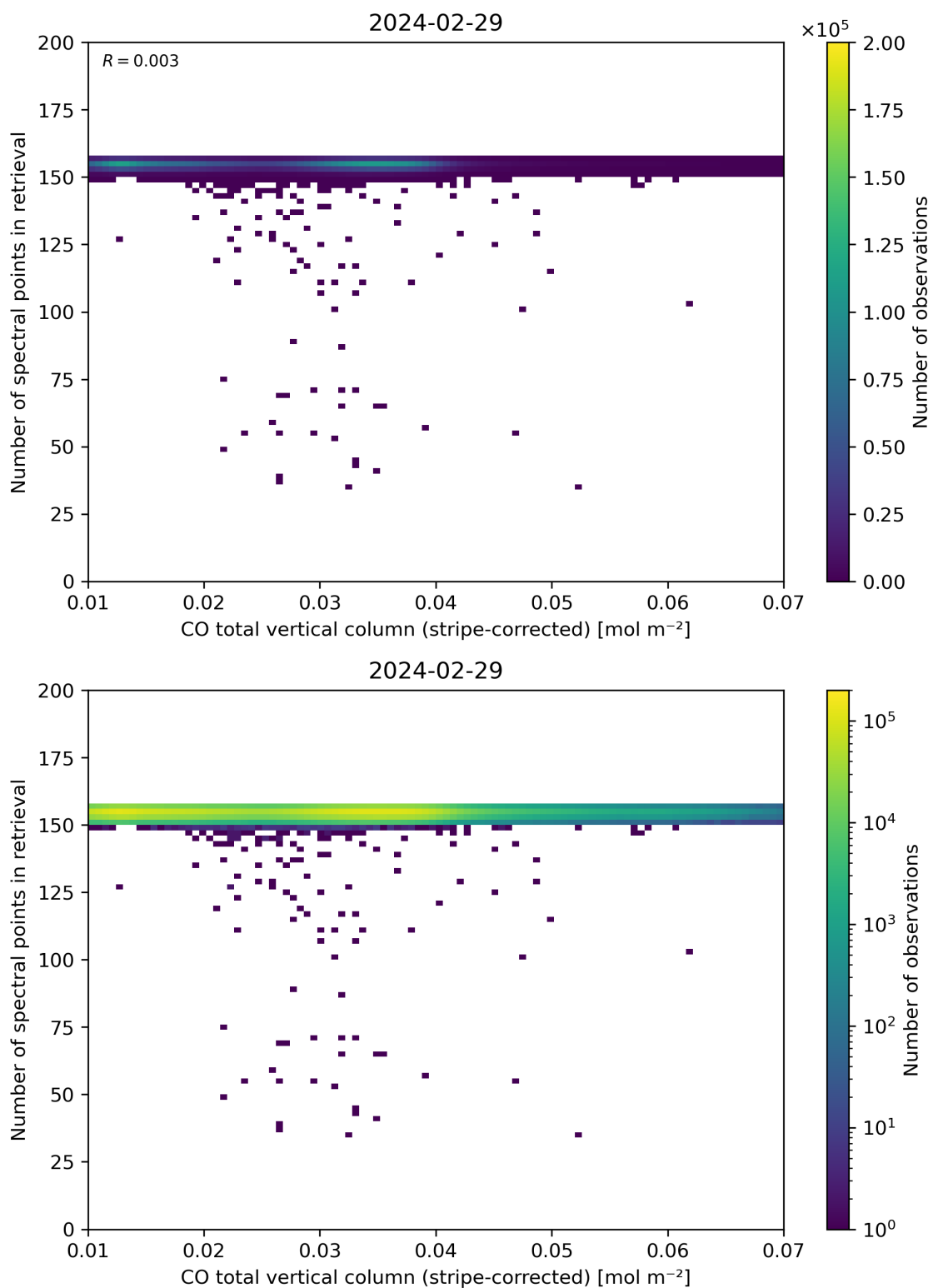
Figure 40: Scatter density plot of “CO total vertical column (stripe-corrected)” against “Number of spectral points in retrieval” for 2024-02-28 to 2024-03-01.
