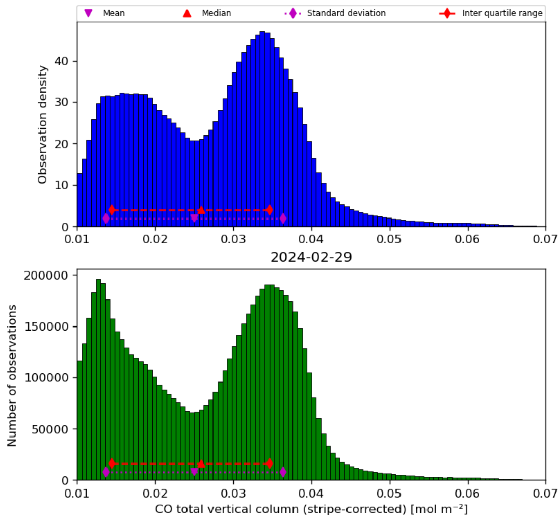
Figure 19: Histogram of “CO total vertical column (stripe-corrected)” for 2024-02-28 to 2024-03-01
