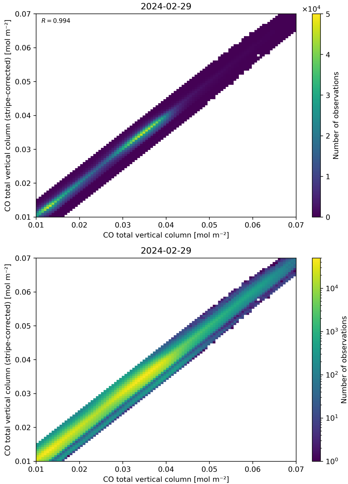
Figure 33: Scatter density plot of “CO total vertical column” against “CO total vertical column (stripe-corrected)” for 2024-02-28 to 2024-03-01.
