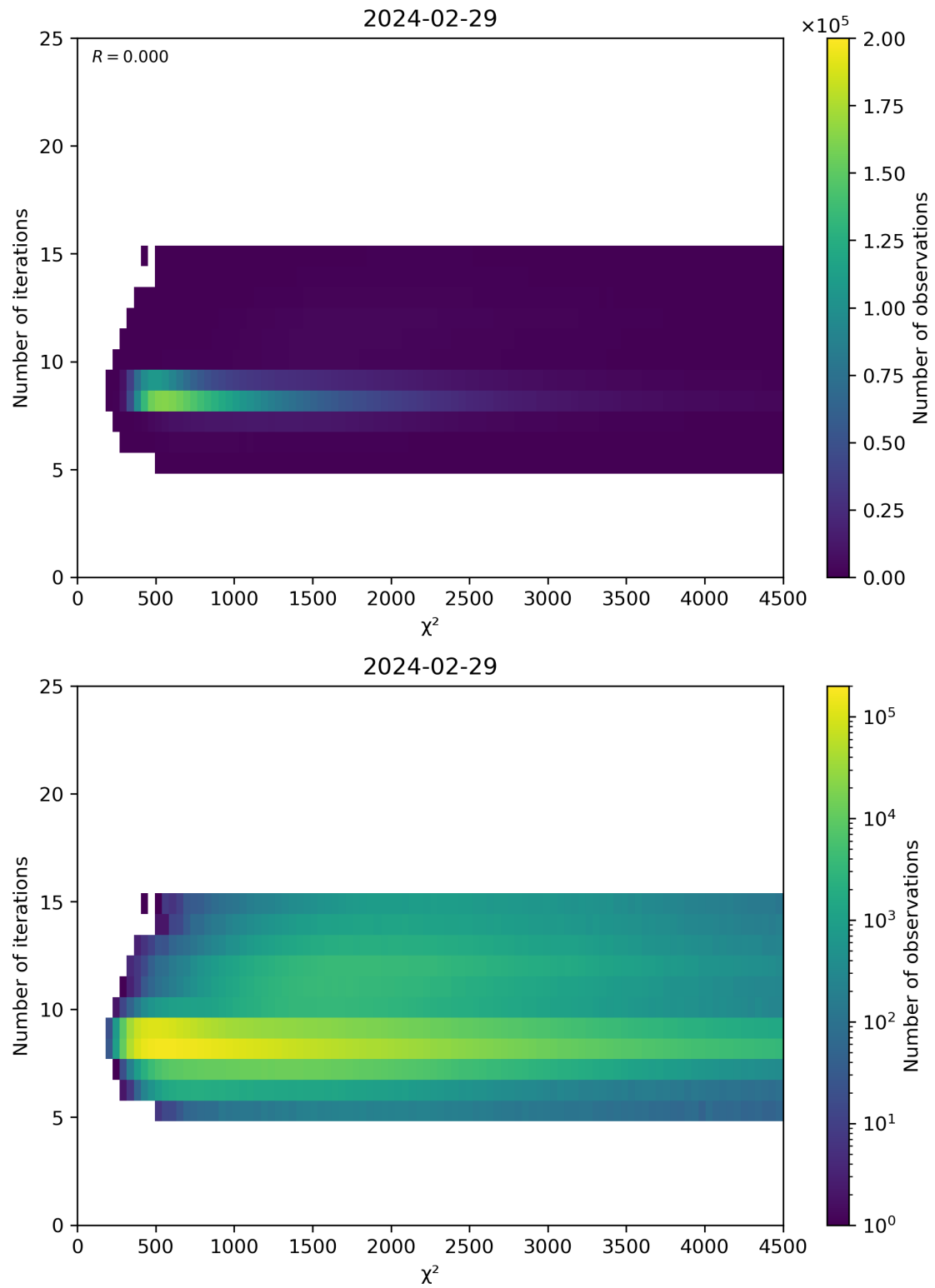
Figure 49: Scatter density plot of “ \chi^2 ” against “Number of iterations” for 2024-02-28 to 2024-03-01.
