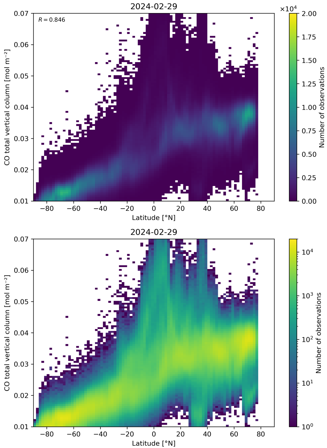
Figure 51: Scatter density plot of “Latitude” against “CO total vertical column” for 2024-02-28 to 2024-03-01.
