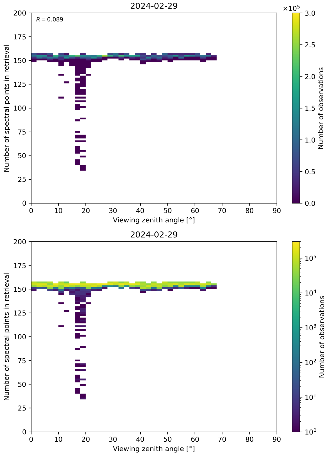
Figure 76: Scatter density plot of “Viewing zenith angle” against “Number of spectral points in retrieval” for 2024-02-28 to 2024-03-01.
