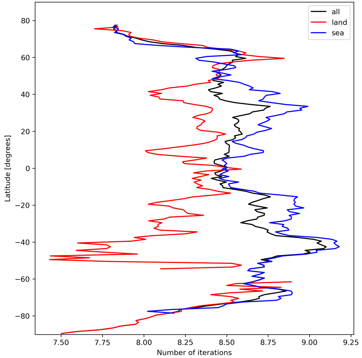
Figure 16: Zonal average of “Number of iterations” for 2024-02-28 to 2024-03-01.
