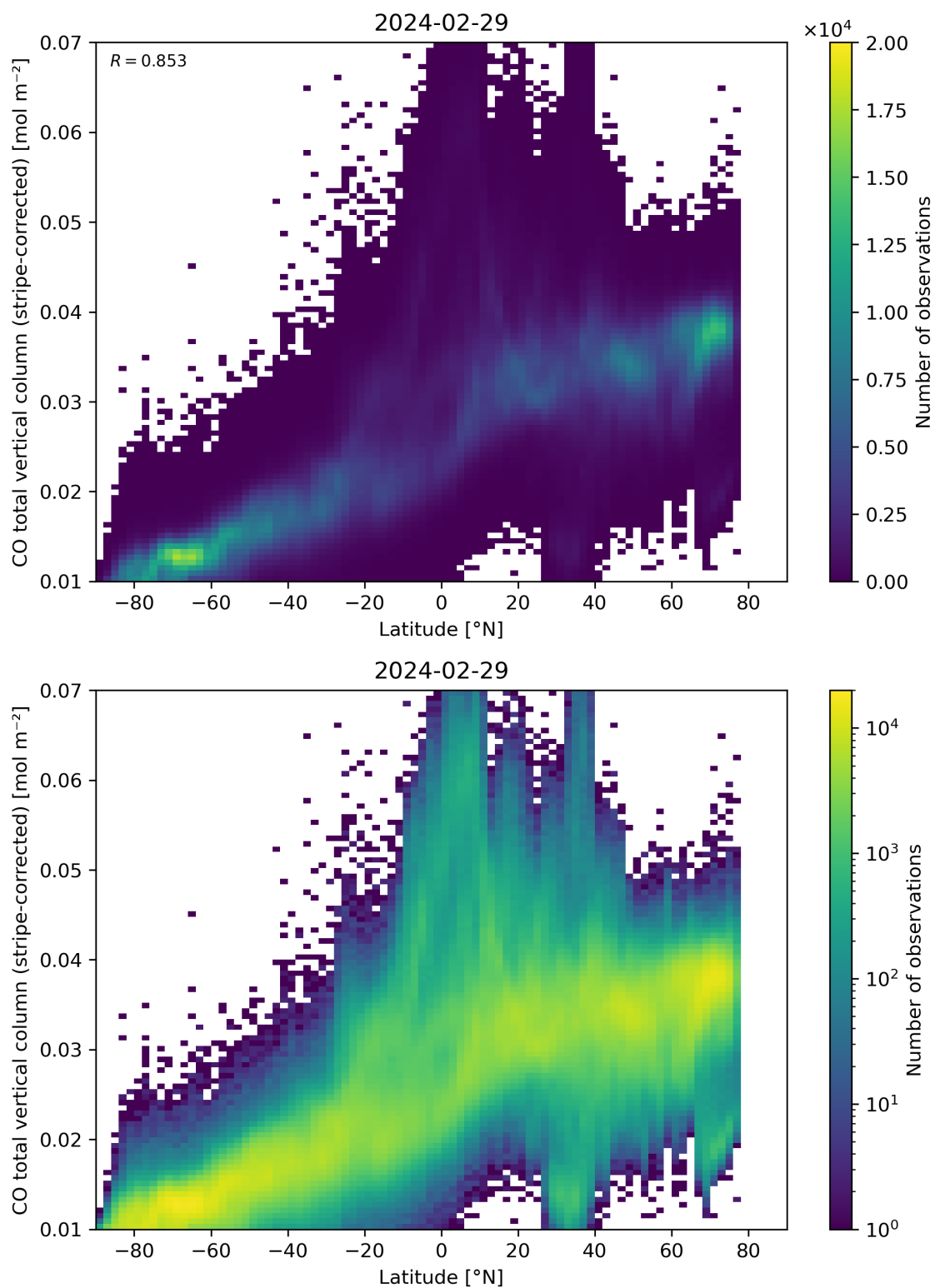
Figure 52: Scatter density plot of “Latitude” against “CO total vertical column (stripe-corrected)” for 2024-02-28 to 2024-03-01.
