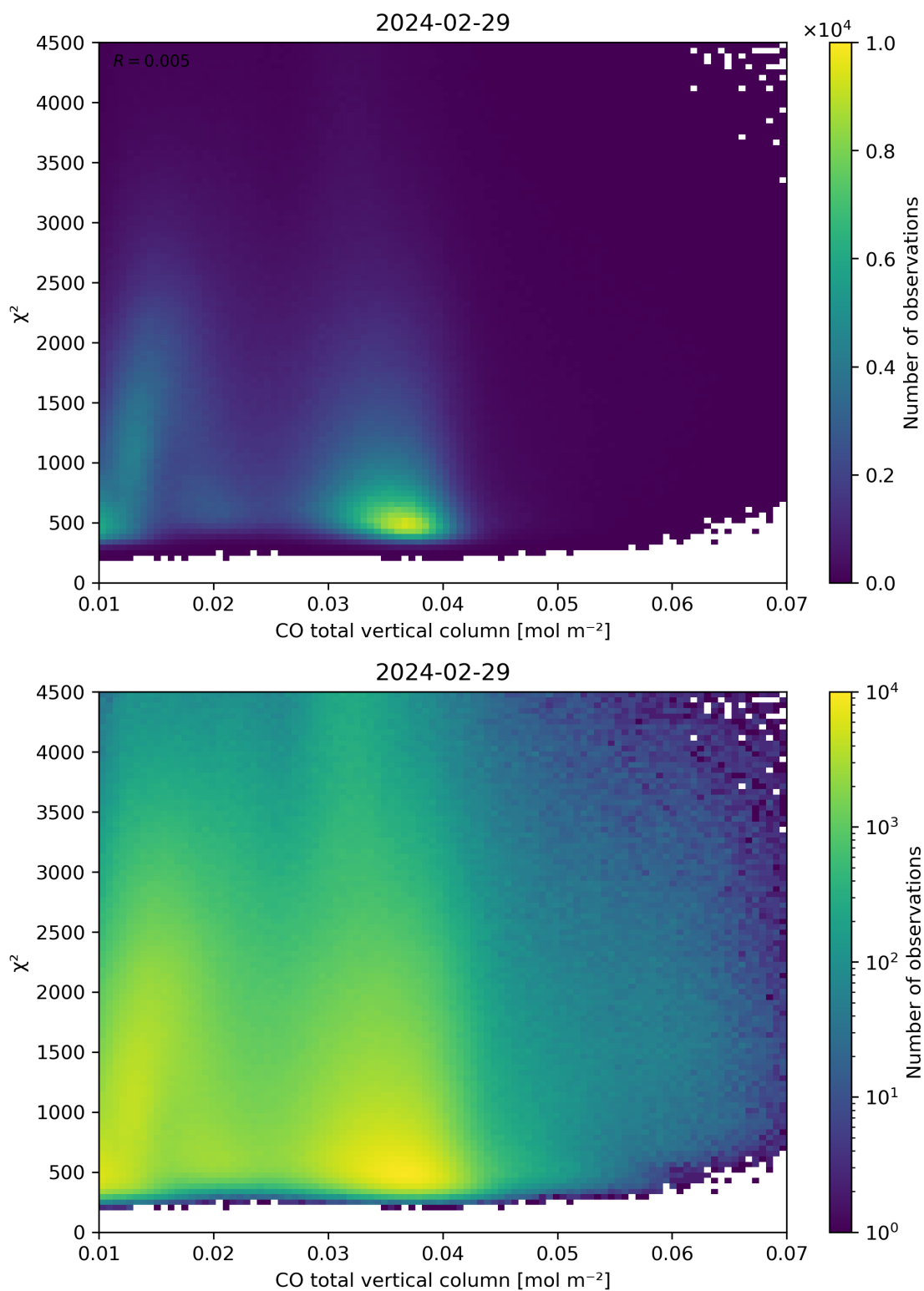
Figure 35: Scatter density plot of “CO total vertical column” against “ \chi^2 ” for 2024-02-28 to 2024-03-01.
