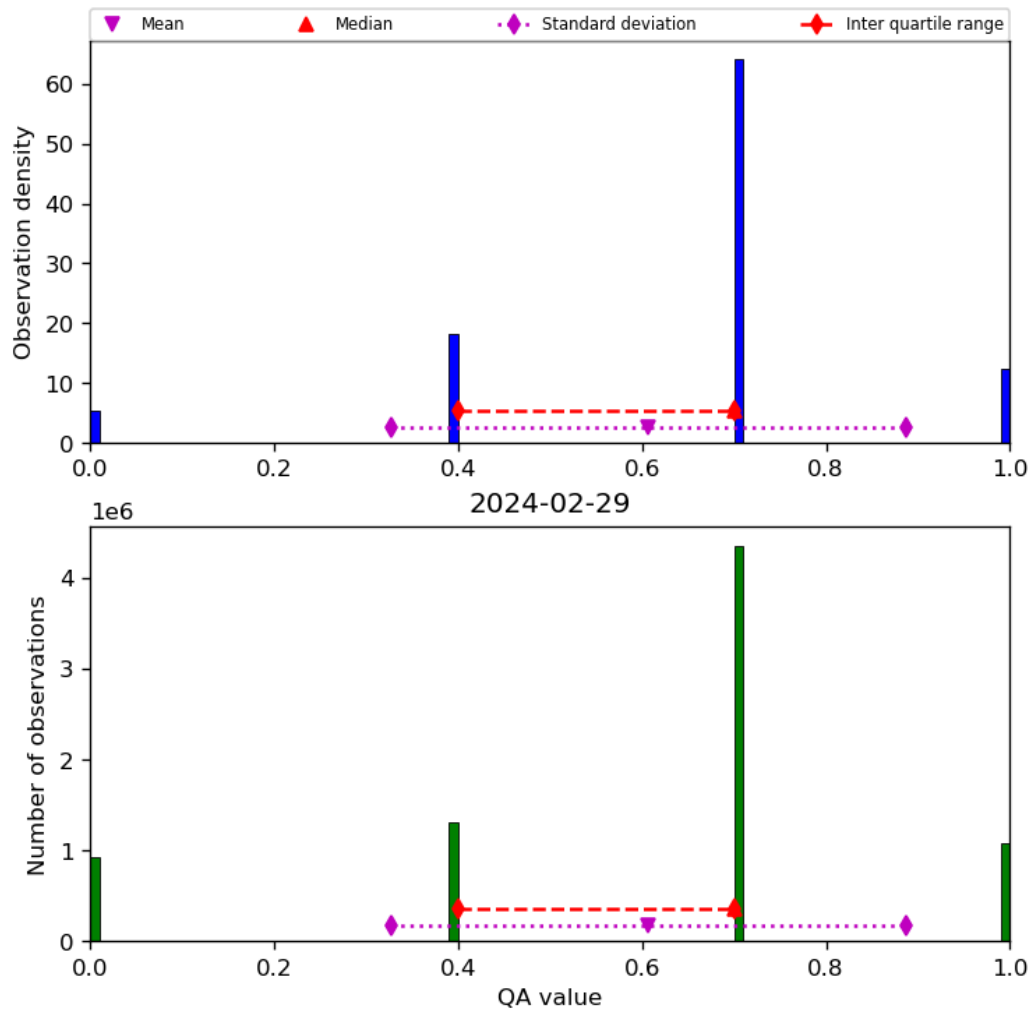
Figure 17: Histogram of “QA value” for 2024-02-28 to 2024-03-01
