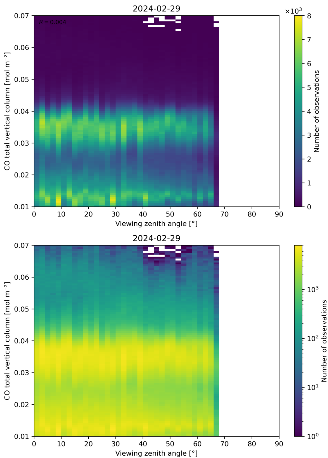
Figure 69: Scatter density plot of “Viewing zenith angle” against “CO total vertical column” for 2024-02-28 to 2024-03-01.
