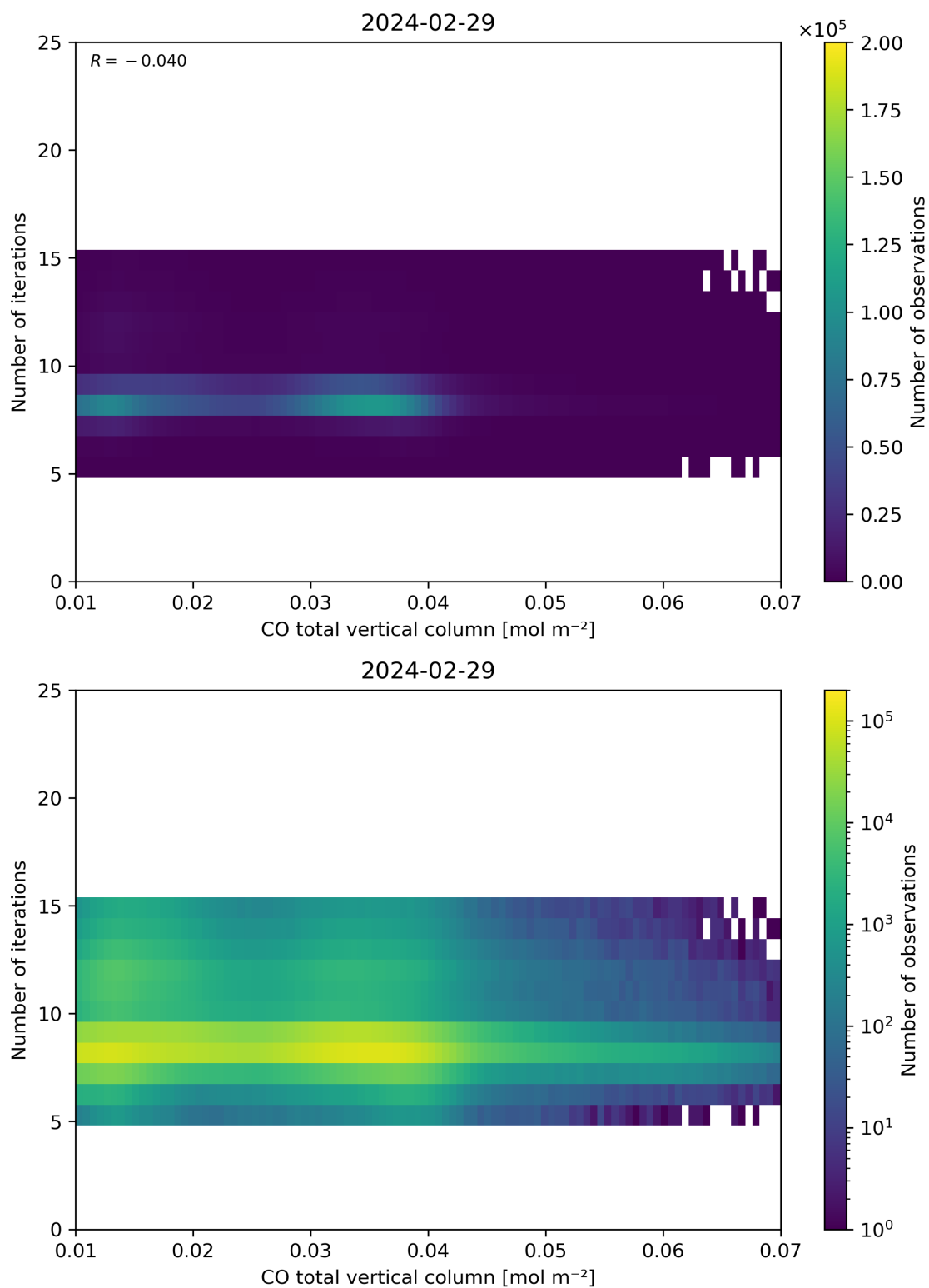
Figure 42: Scatter density plot of “CO total vertical column” against “Number of iterations” for 2024-02-28 to 2024-03-01.
