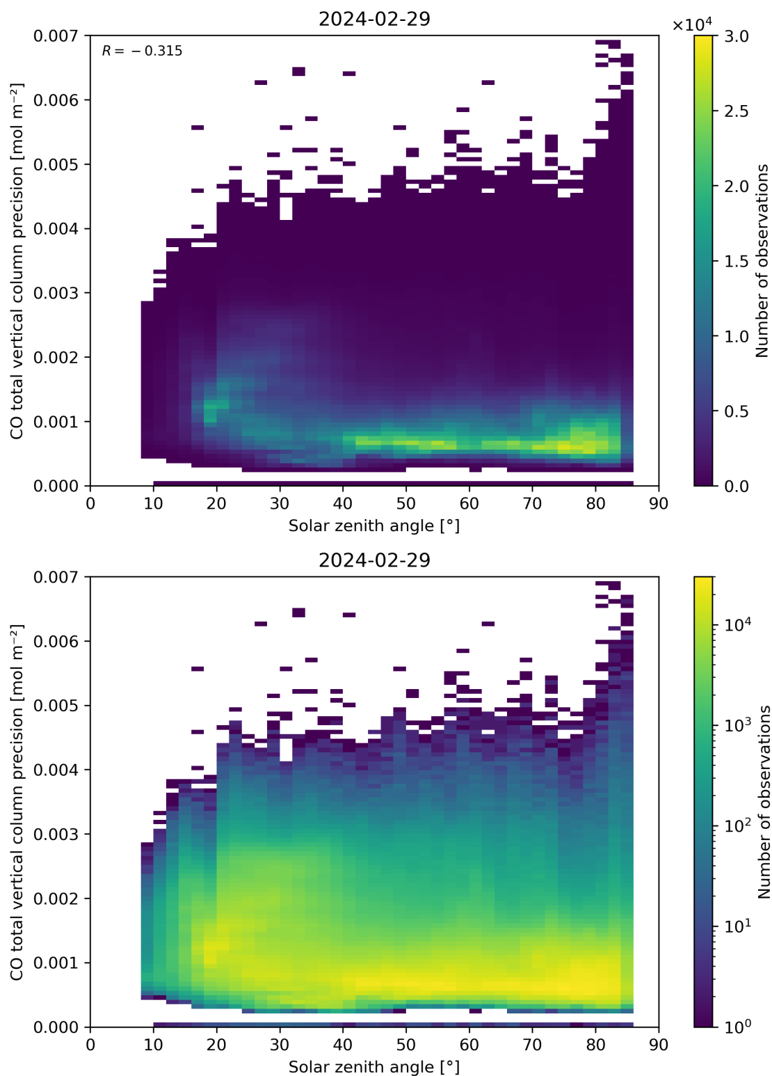
Figure 63: Scatter density plot of “Solar zenith angle” against “CO total vertical column precision” for 2024-02-28 to 2024-03-01.
