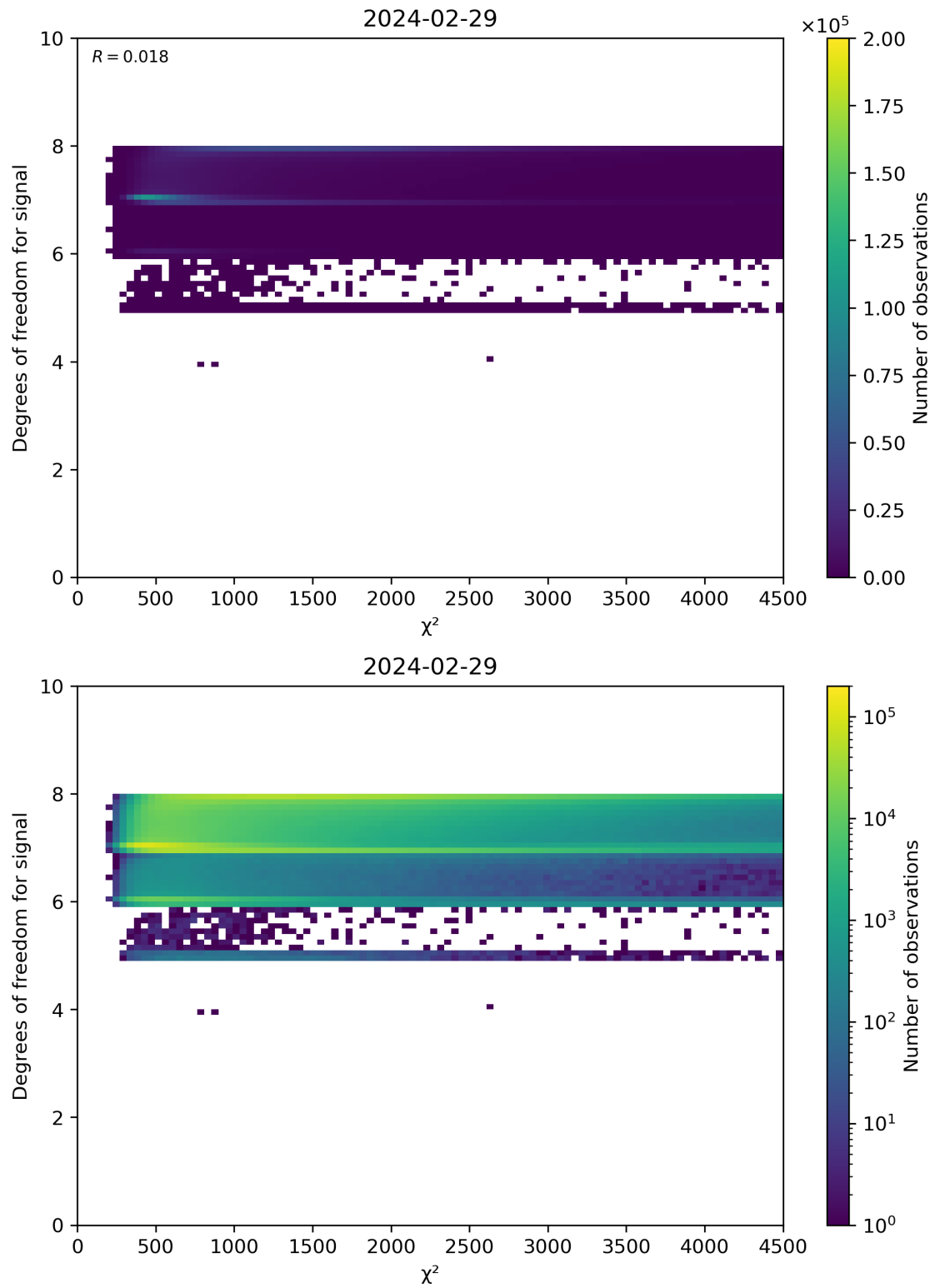
Figure 48: Scatter density plot of " \chi^2 " against "Degrees of freedom for signal" for 2024-02-28 to 2024-03-01.
