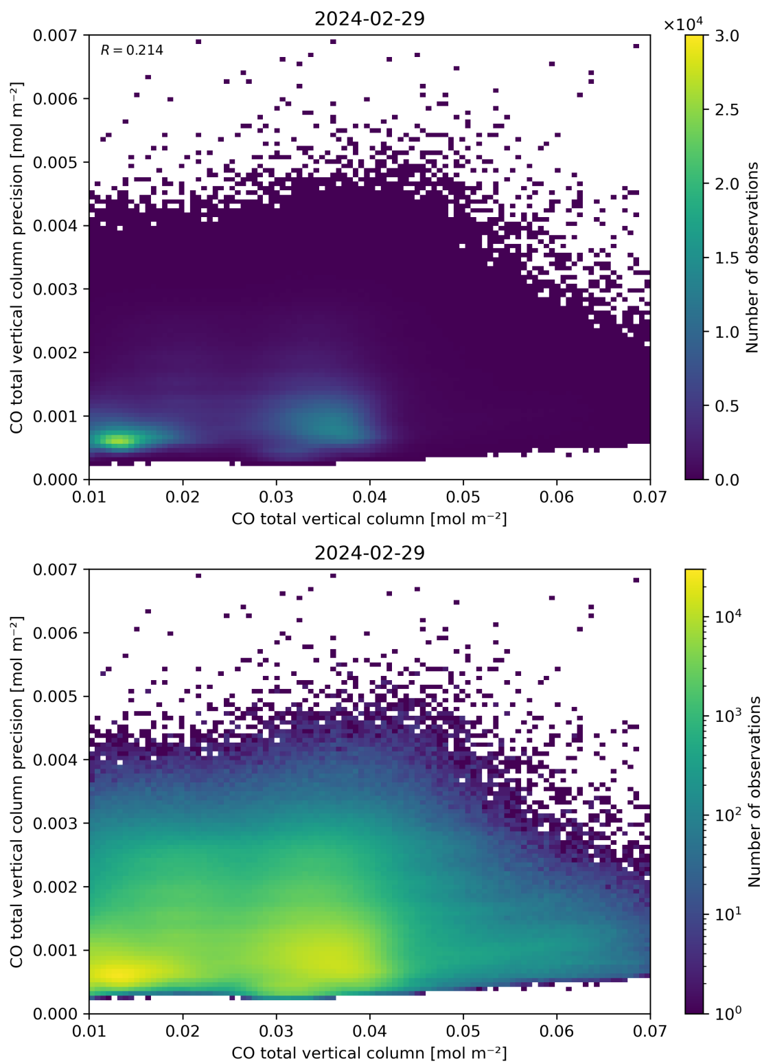
Figure 34: Scatter density plot of “CO total vertical column” against “CO total vertical column precision” for 2024-02-28 to 2024-03-01.
