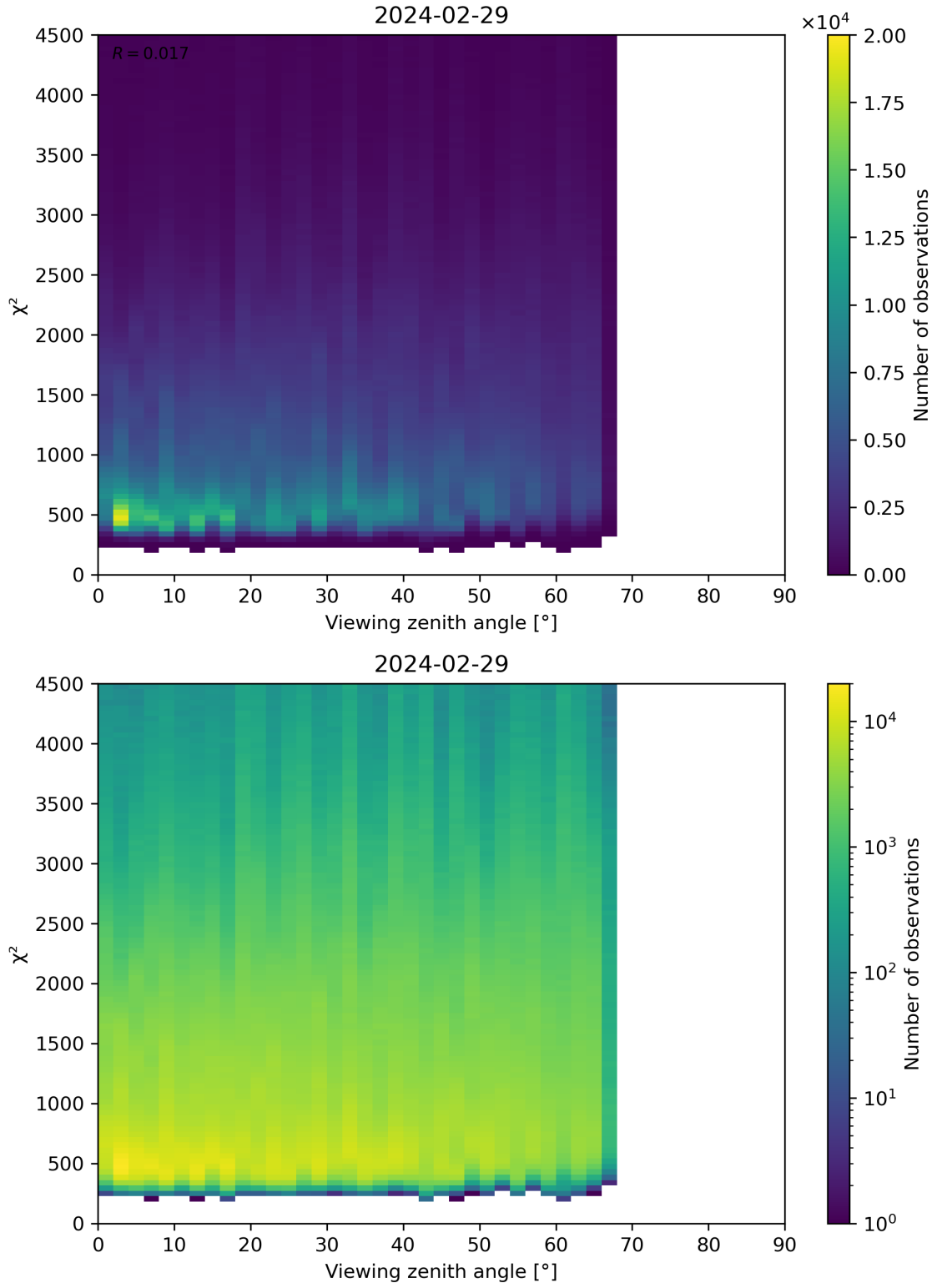
Figure 72: Scatter density plot of “Viewing zenith angle” against “ \chi^2 ” for 2024-02-28 to 2024-03-01.
