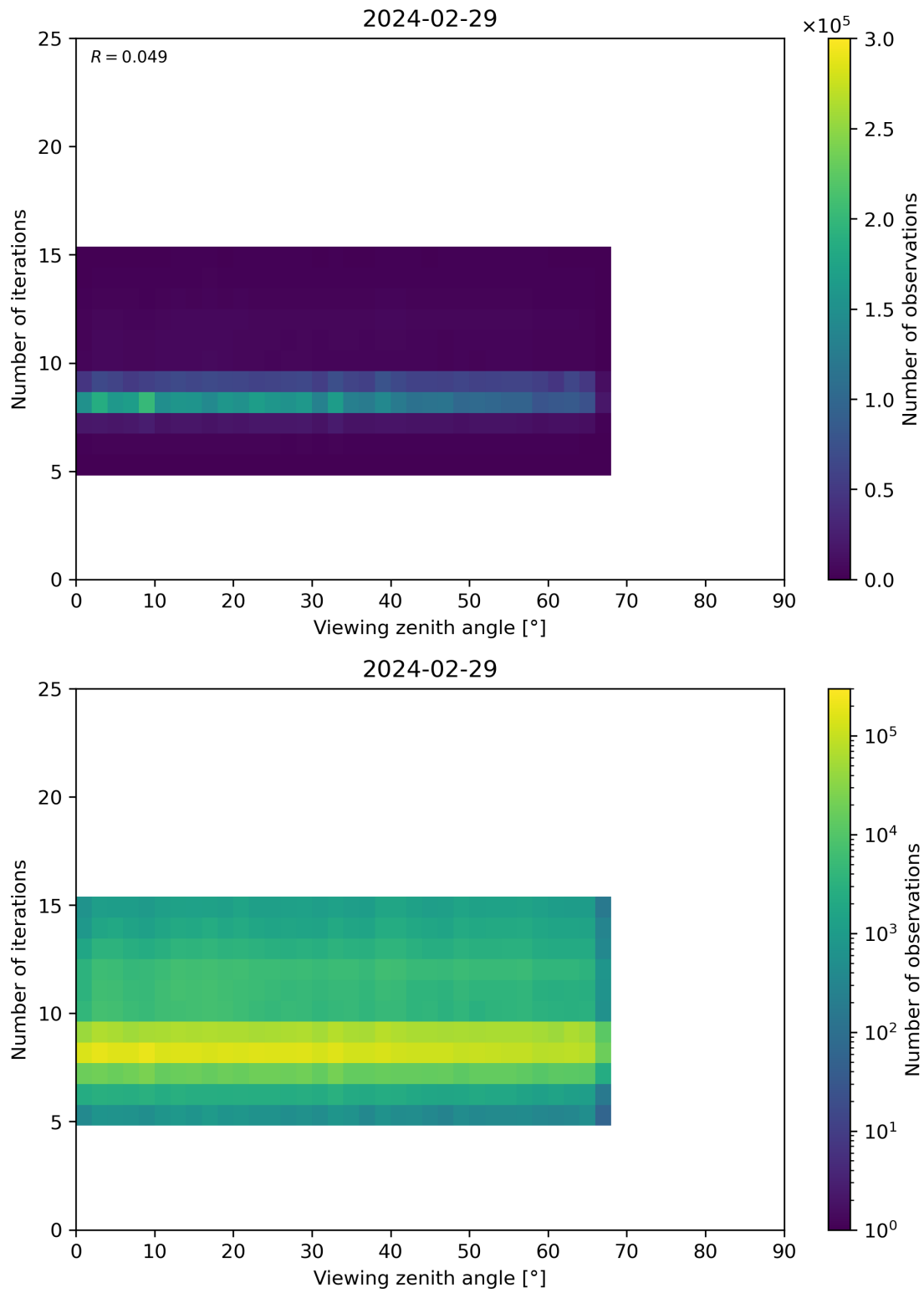
Figure 75: Scatter density plot of “Viewing zenith angle” against “Number of iterations” for 2024-02-28 to 2024-03-01.
