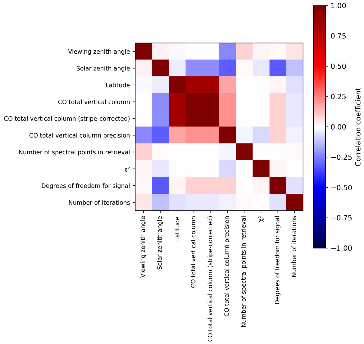
Figure 2: Map of correlation matrix for 2024-02-28 to 2024-03-01.
