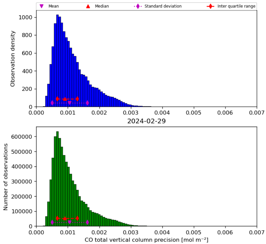
Figure 20: Histogram of “CO total vertical column precision” for 2024-02-28 to 2024-03-01
