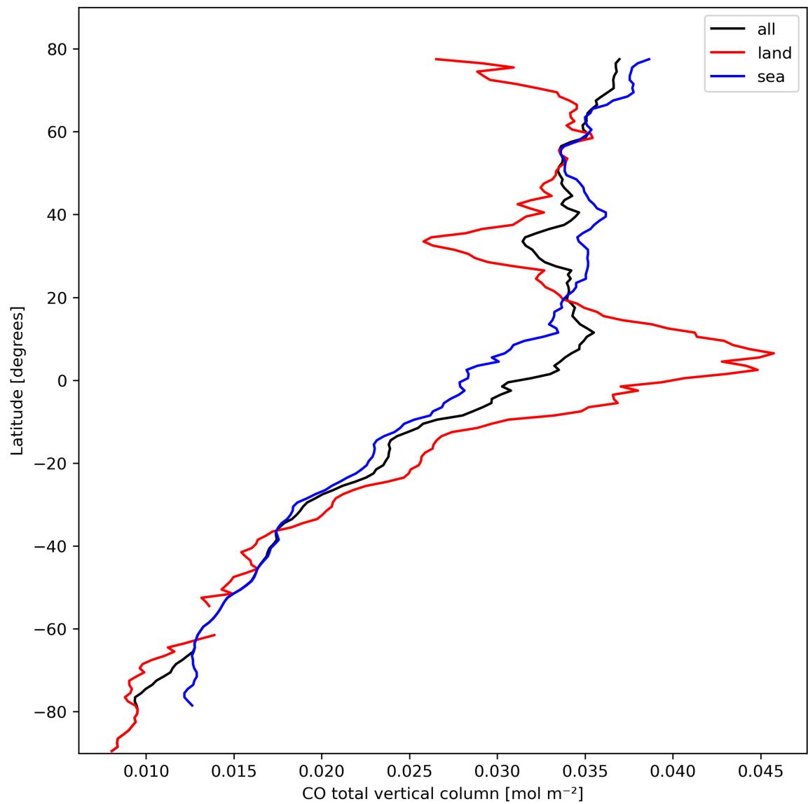
Figure 10: Zonal average of “CO total vertical column” for 2024-02-28 to 2024-03-01.
