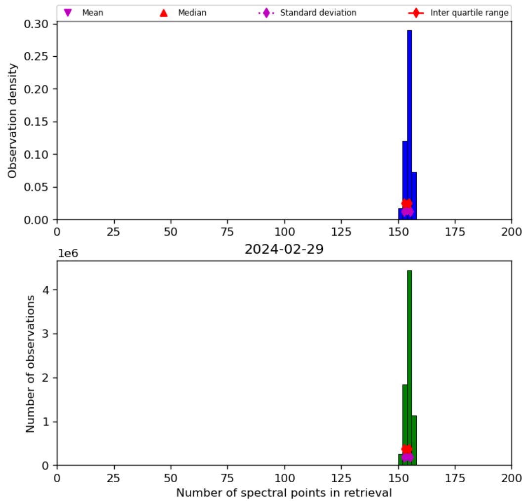
Figure 21: Histogram of “Number of spectral points in retrieval” for 2024-02-28 to 2024-03-01
