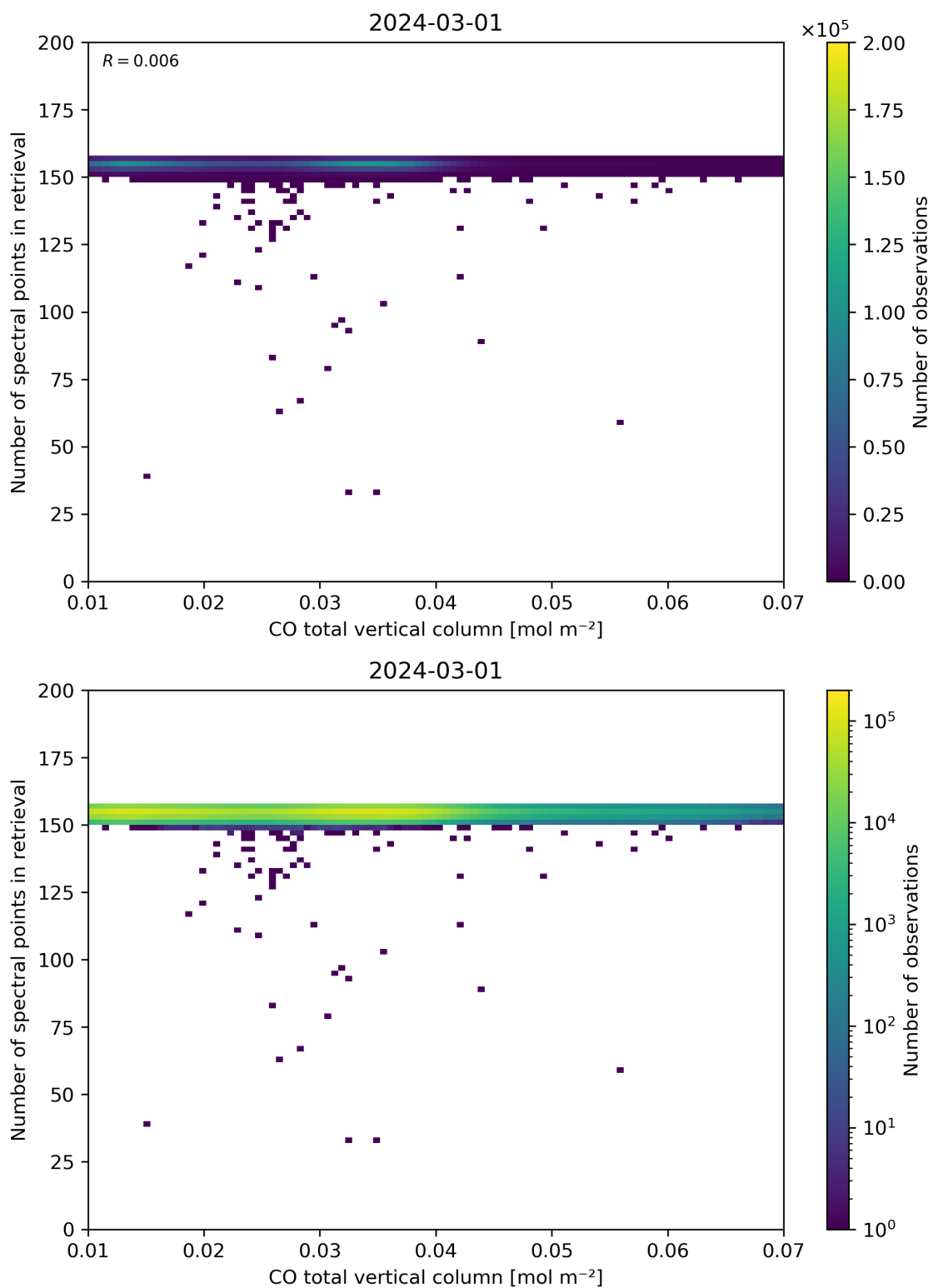
Figure 43: Scatter density plot of “CO total vertical column” against “Number of spectral points in retrieval” for 2024-02-29 to 2024-03-02.
