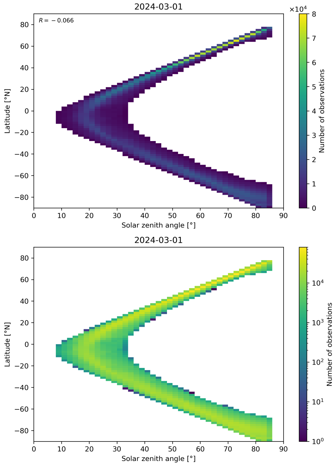
Figure 66: Scatter density plot of “Solar zenith angle” against “Latitude” for 2024-02-29 to 2024-03-02.
