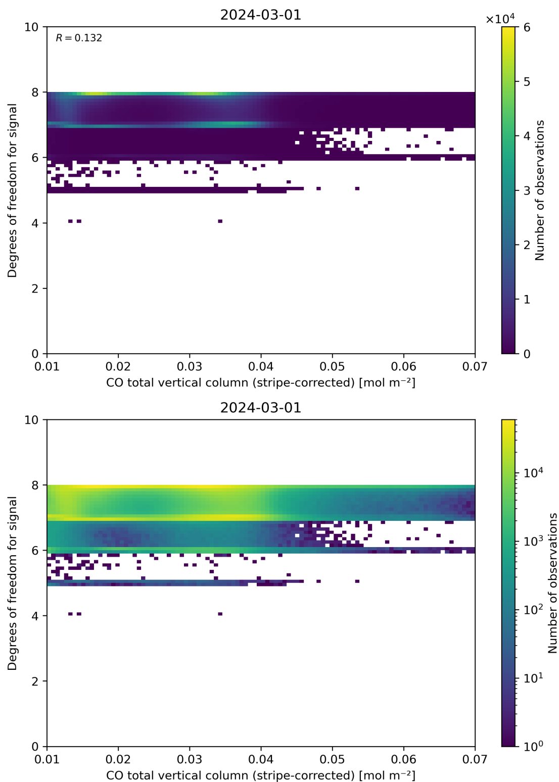
Figure 38: Scatter density plot of “CO total vertical column (stripe-corrected)” against “Degrees of freedom for signal” for 2024-02-29 to 2024-03-02.
