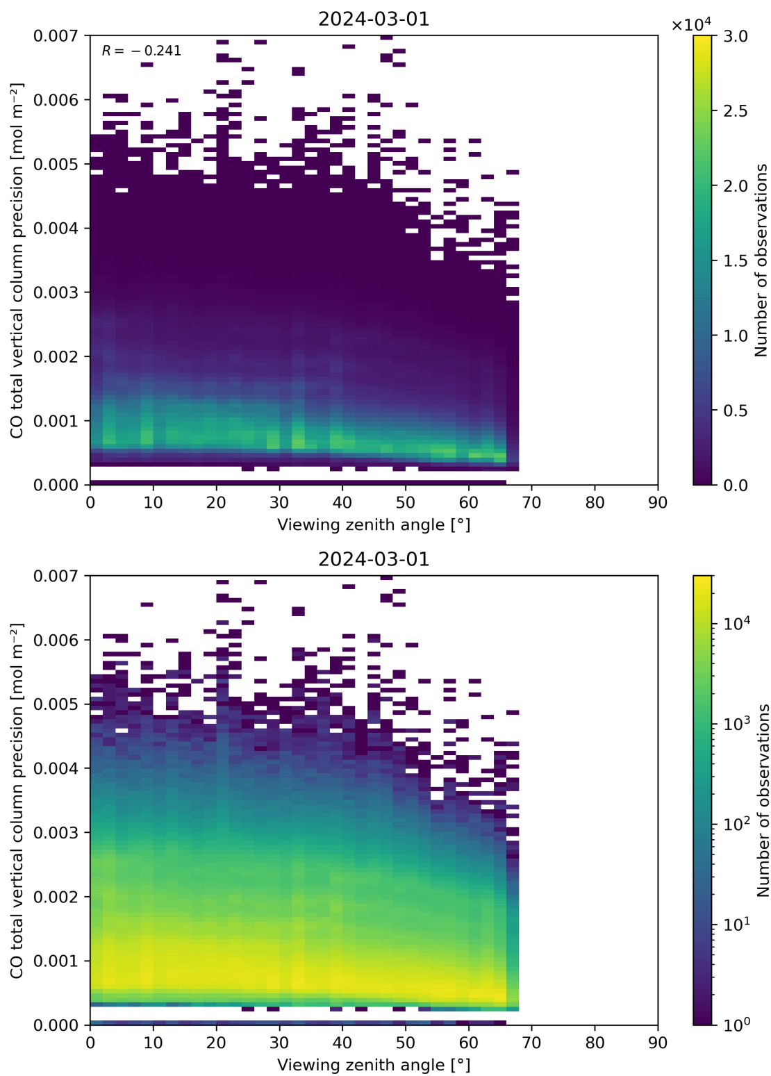
Figure 71: Scatter density plot of “Viewing zenith angle” against “CO total vertical column precision” for 2024-02-29 to 2024-03-02.
