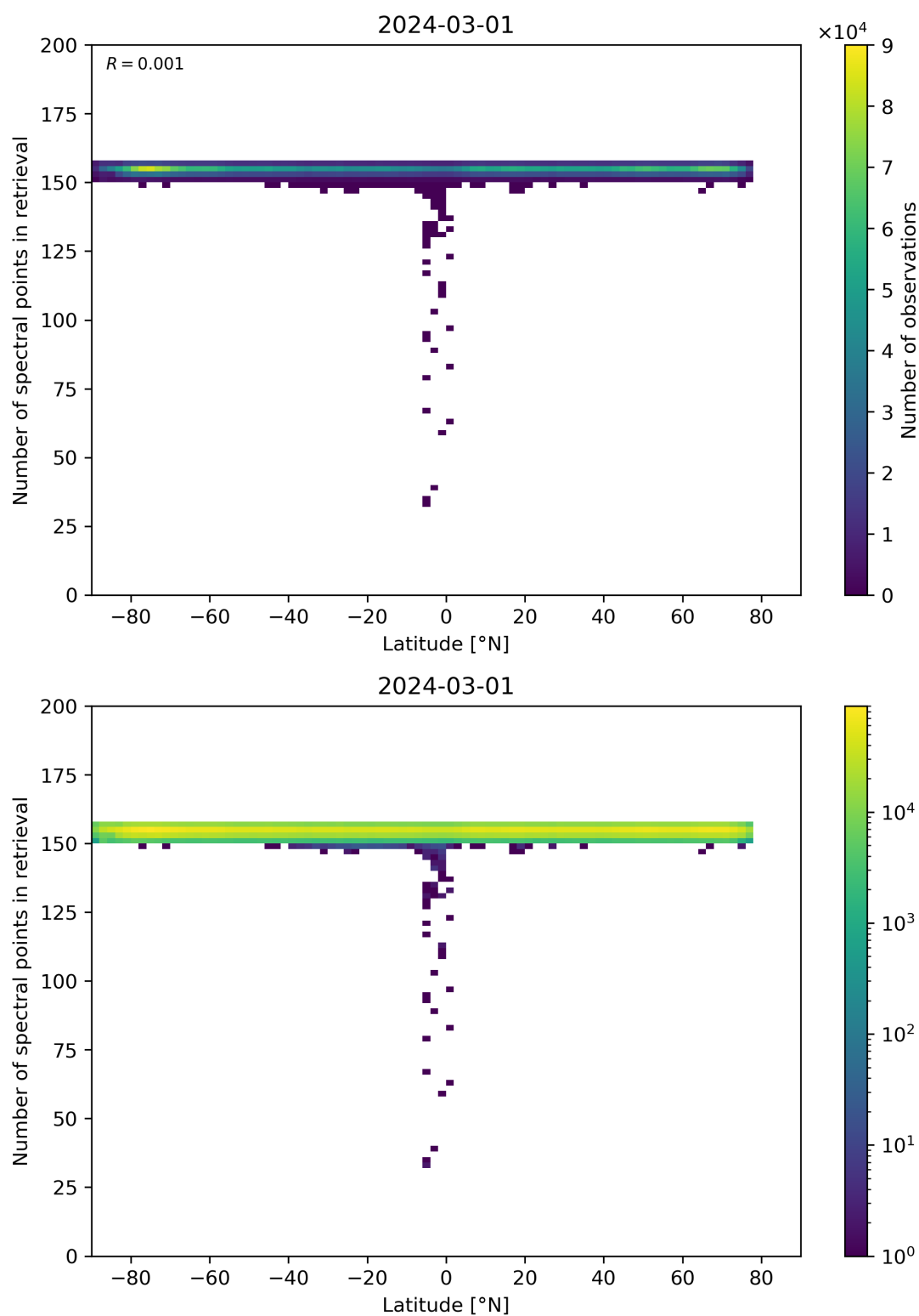
Figure 57: Scatter density plot of “Latitude” against “Number of spectral points in retrieval” for 2024-02-29 to 2024-03-02.
