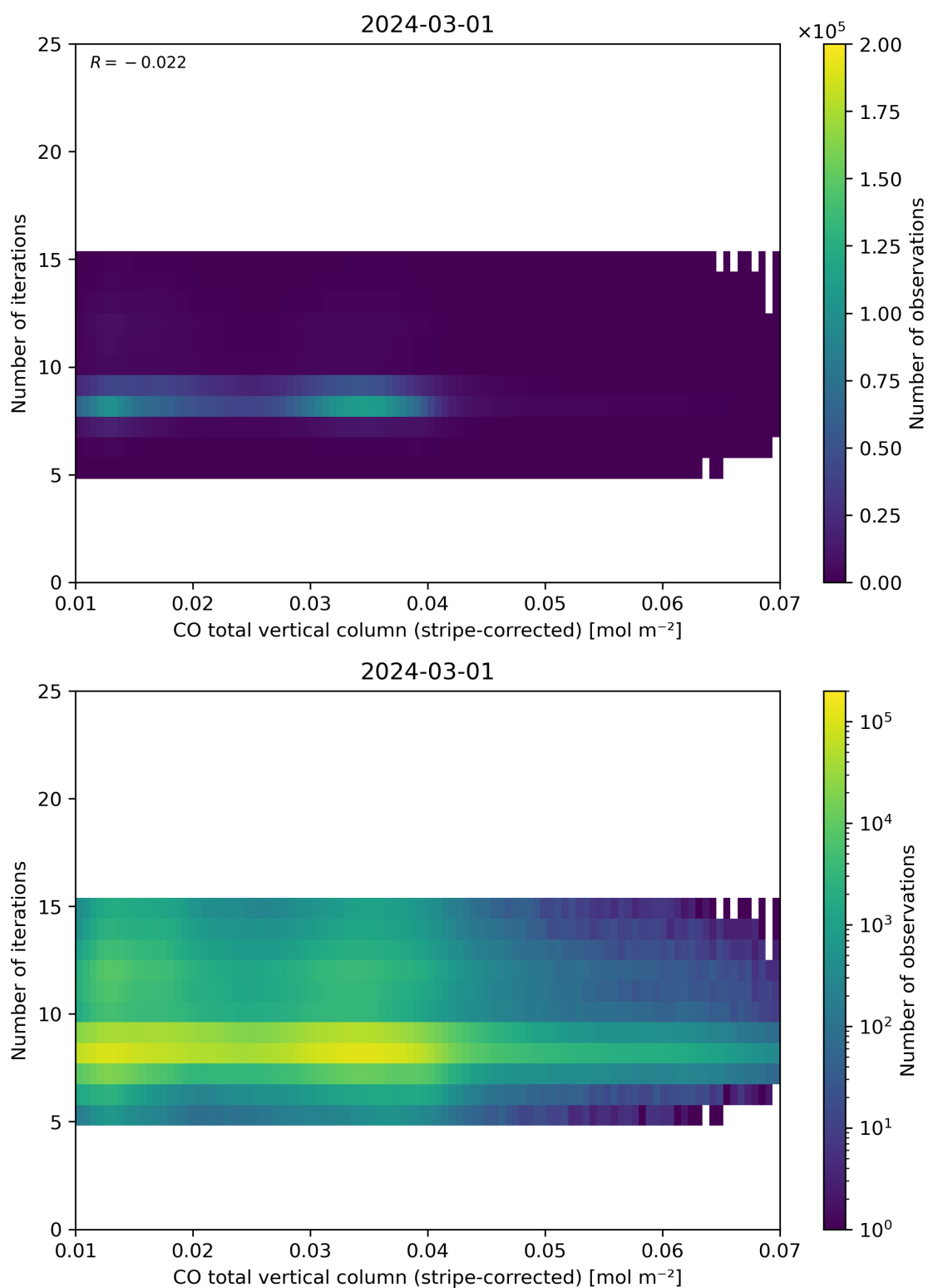
Figure 39: Scatter density plot of “CO total vertical column (stripe-corrected)” against “Number of iterations” for 2024-02-29 to 2024-03-02.
