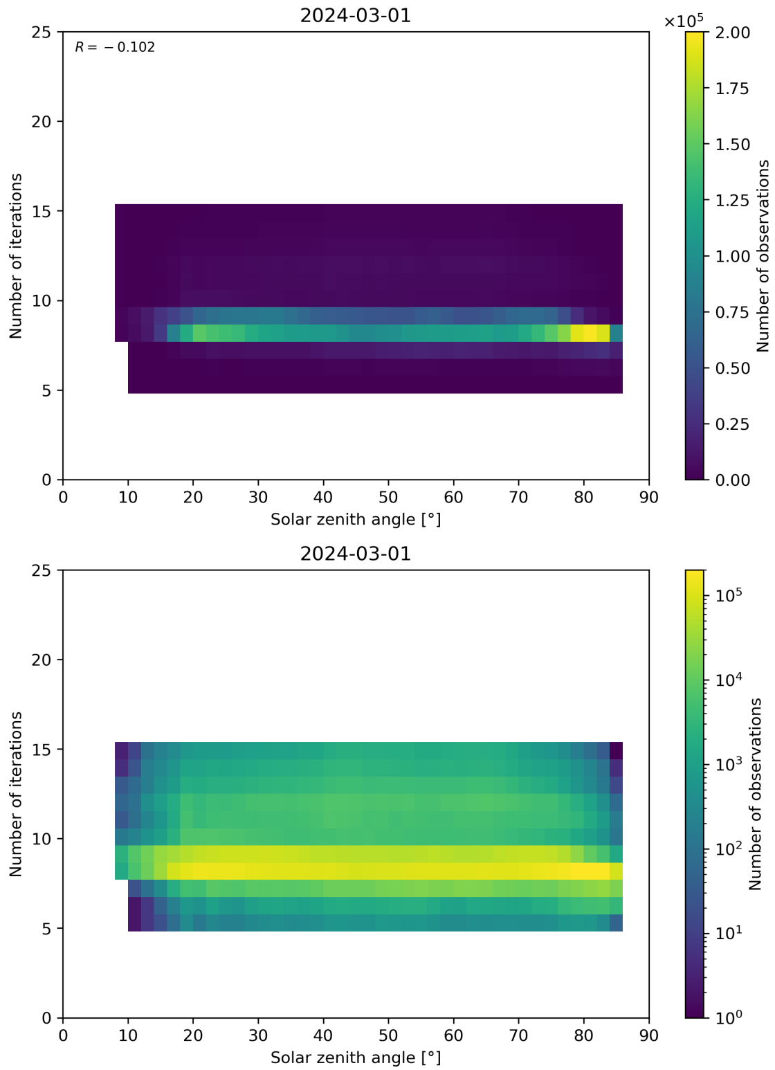
Figure 67: Scatter density plot of “Solar zenith angle” against “Number of iterations” for 2024-02-29 to 2024-03-02.
