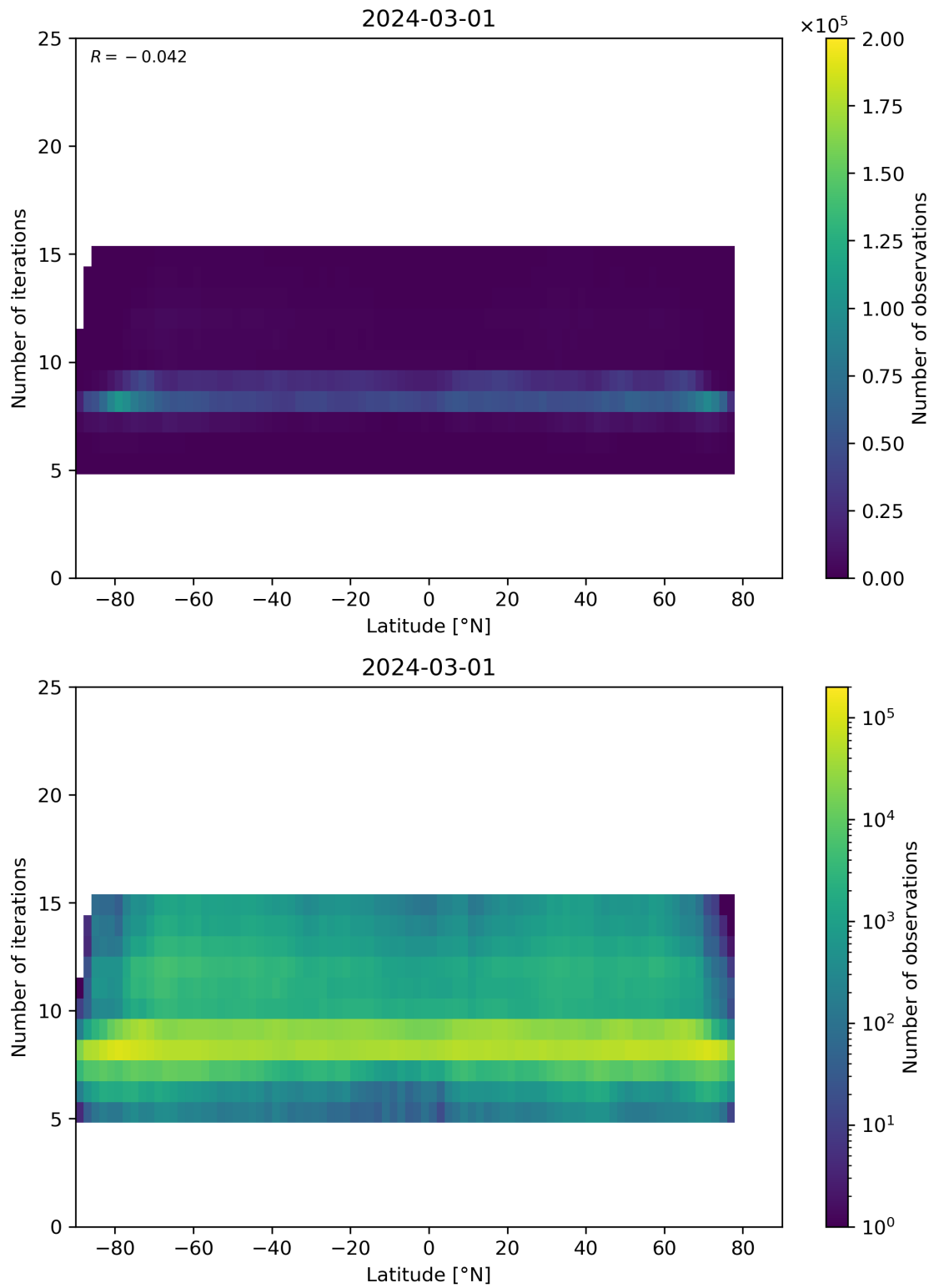
Figure 56: Scatter density plot of “Latitude” against “Number of iterations” for 2024-02-29 to 2024-03-02.
