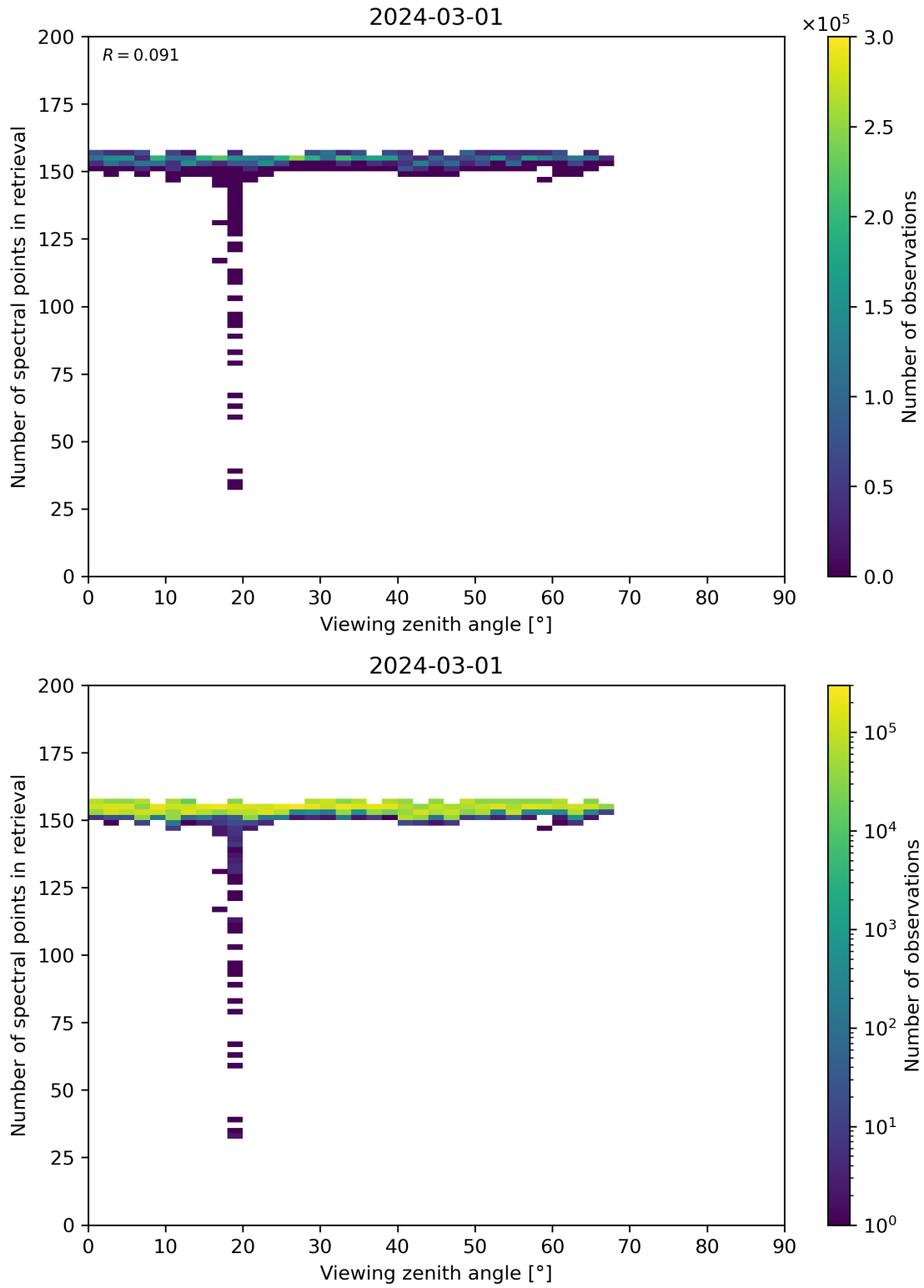
Figure 76: Scatter density plot of “Viewing zenith angle” against “Number of spectral points in retrieval” for 2024-02-29 to 2024-03-02.
