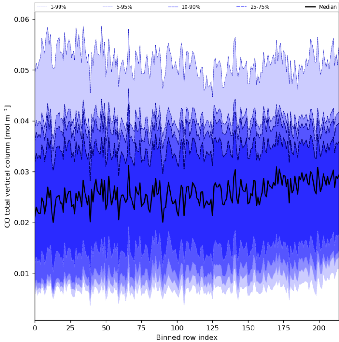
Figure 26: Along track statistics of “CO total vertical column” for 2024-02-29 to 2024-03-02
