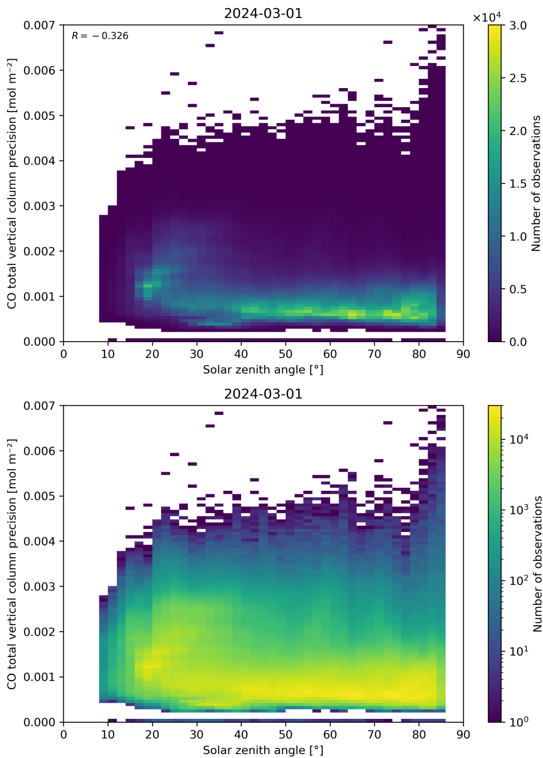
Figure 63: Scatter density plot of “Solar zenith angle” against “CO total vertical column precision” for 2024-02-29 to 2024-03-02.
