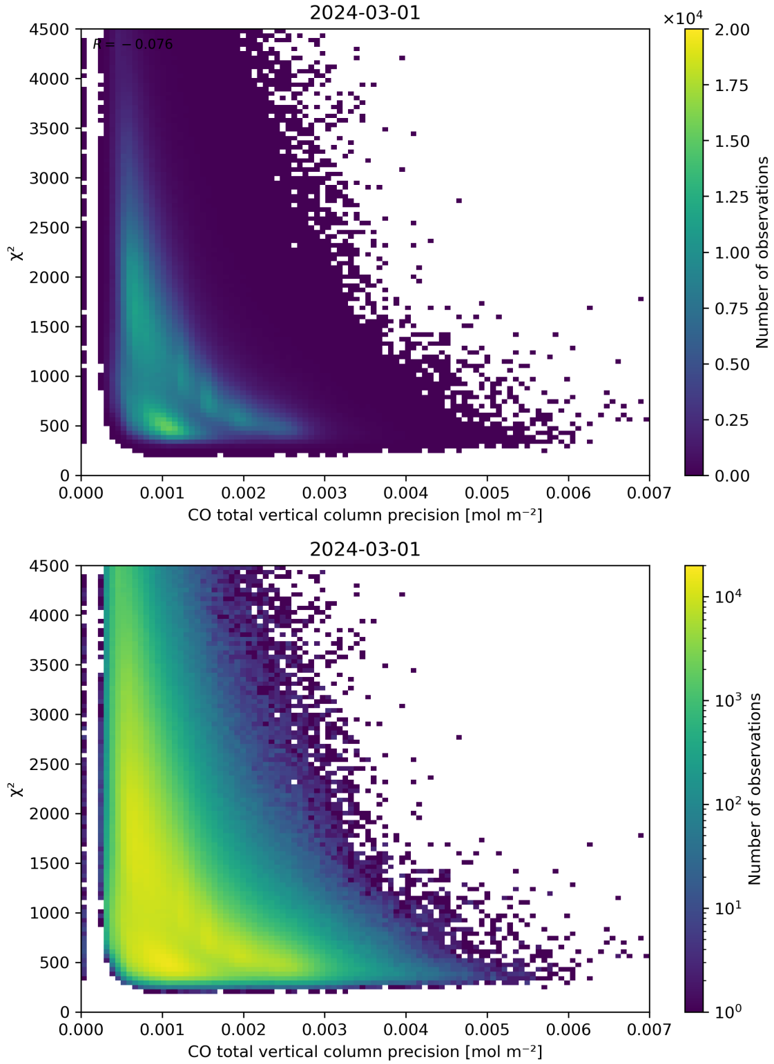
Figure 44: Scatter density plot of “CO total vertical column precision” against “ \chi^2 ” for 2024-02-29 to 2024-03-02.
