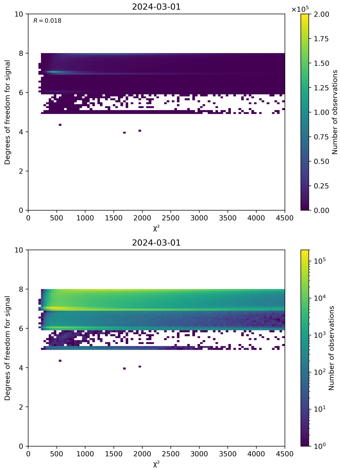
Figure 48: Scatter density plot of “ \chi^2 ” against “Degrees of freedom for signal” for 2024-02-29 to 2024-03-02.
