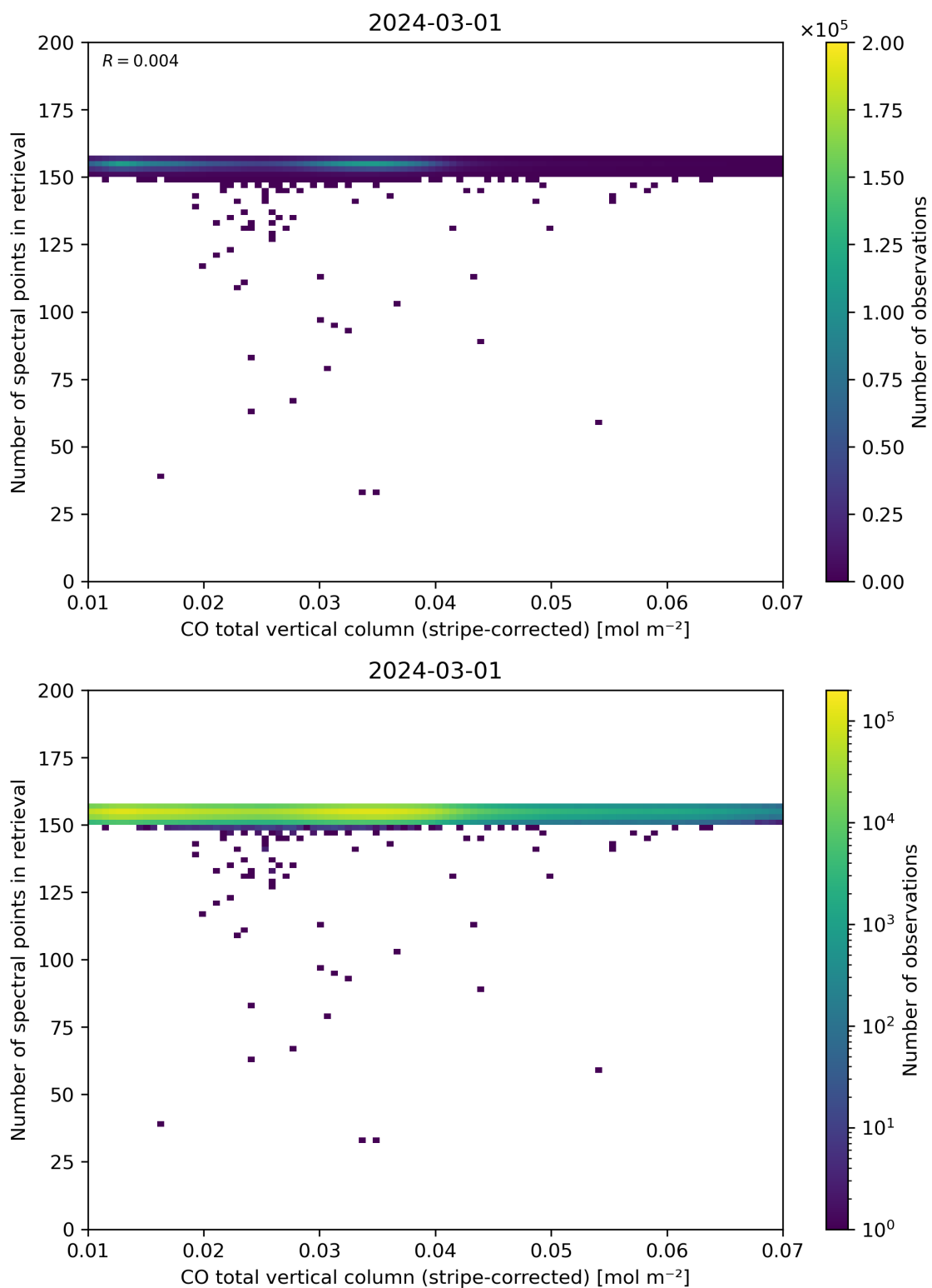
Figure 40: Scatter density plot of “CO total vertical column (stripe-corrected)” against “Number of spectral points in retrieval” for 2024-02-29 to 2024-03-02.
