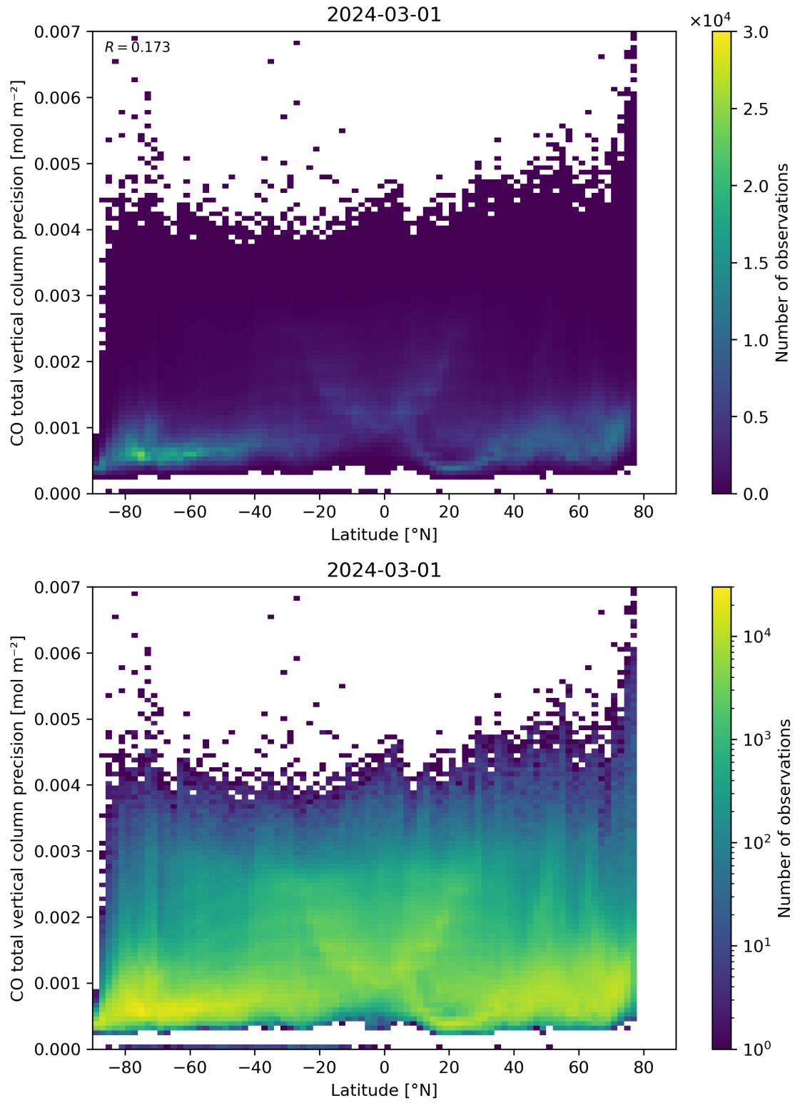
Figure 53: Scatter density plot of “Latitude” against “CO total vertical column precision” for 2024-02-29 to 2024-03-02.
