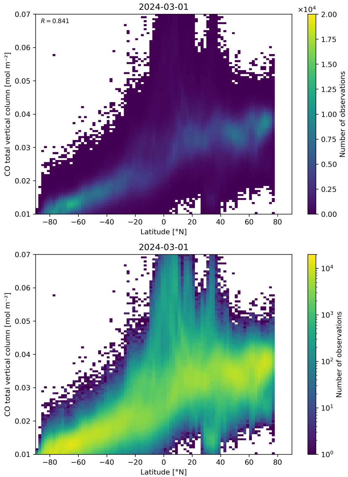
Figure 51: Scatter density plot of “Latitude” against “CO total vertical column” for 2024-02-29 to 2024-03-02.
