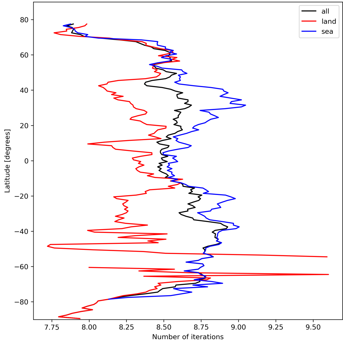
Figure 16: Zonal average of “Number of iterations” for 2024-02-29 to 2024-03-02.
