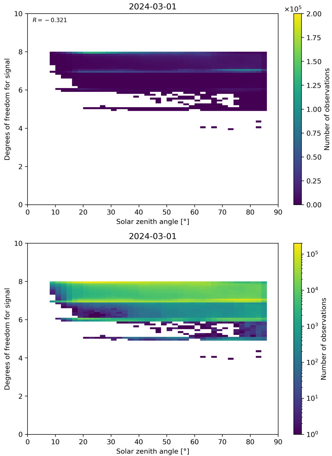
Figure 65: Scatter density plot of “Solar zenith angle” against “Degrees of freedom for signal” for 2024-02-29 to 2024-03-02.
