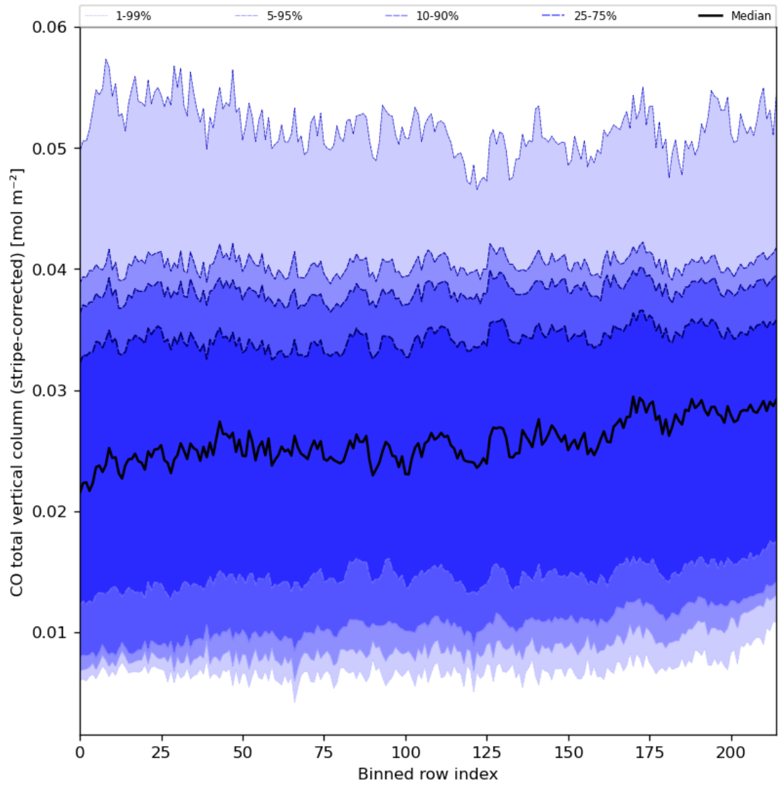
Figure 27: Along track statistics of “CO total vertical column (stripe-corrected)” for 2024-02-29 to 2024-03-02
