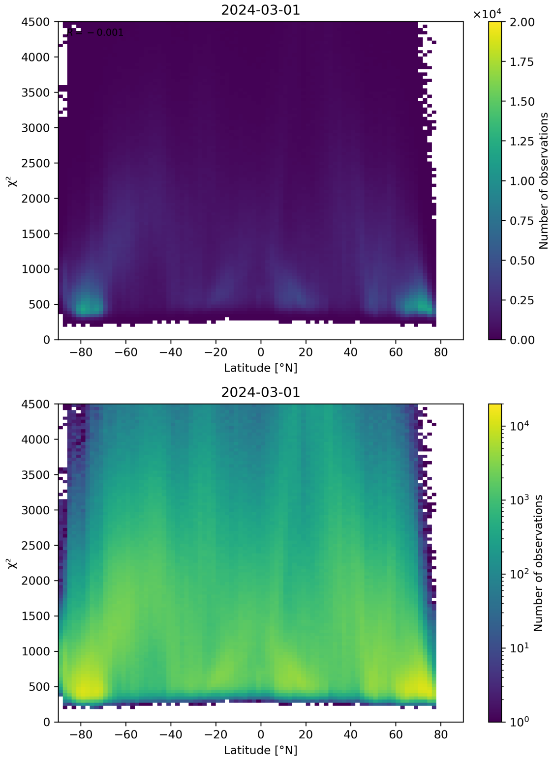
Figure 54: Scatter density plot of “Latitude” against “ \chi^2 ” for 2024-02-29 to 2024-03-02.
