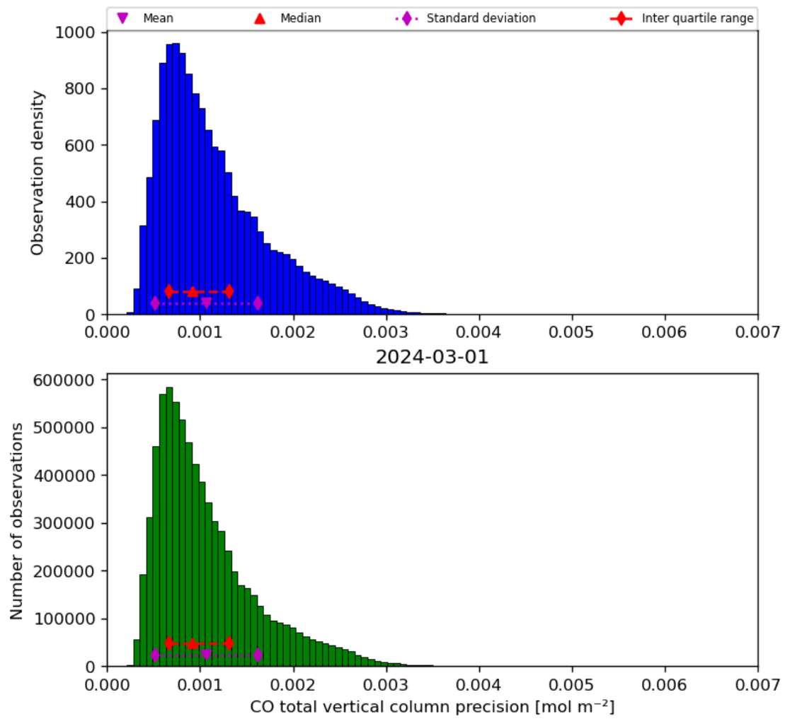
Figure 20: Histogram of “CO total vertical column precision” for 2024-02-29 to 2024-03-02
