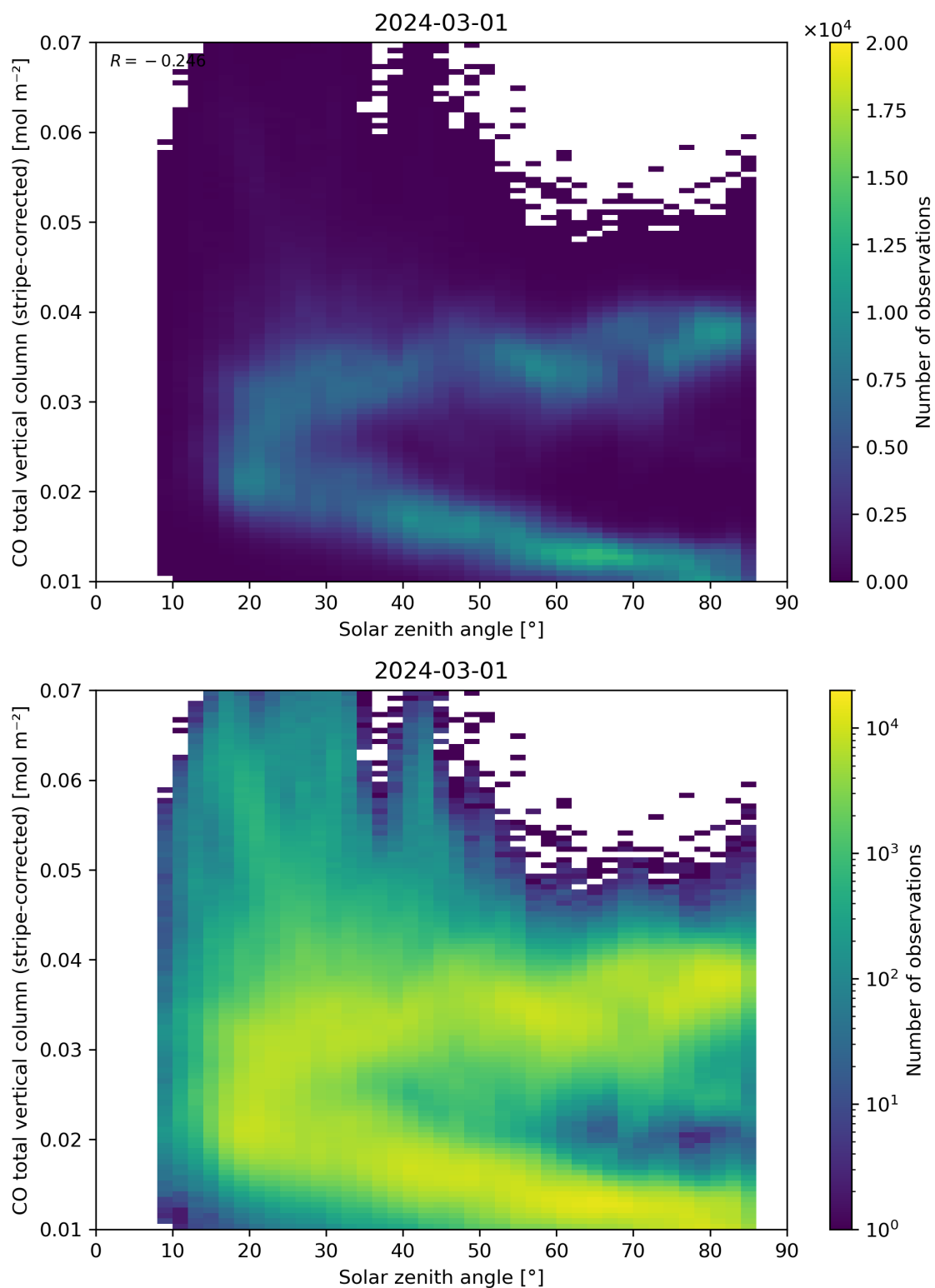
Figure 62: Scatter density plot of “Solar zenith angle” against “CO total vertical column (stripe-corrected)” for 2024-02-29 to 2024-03-02.
