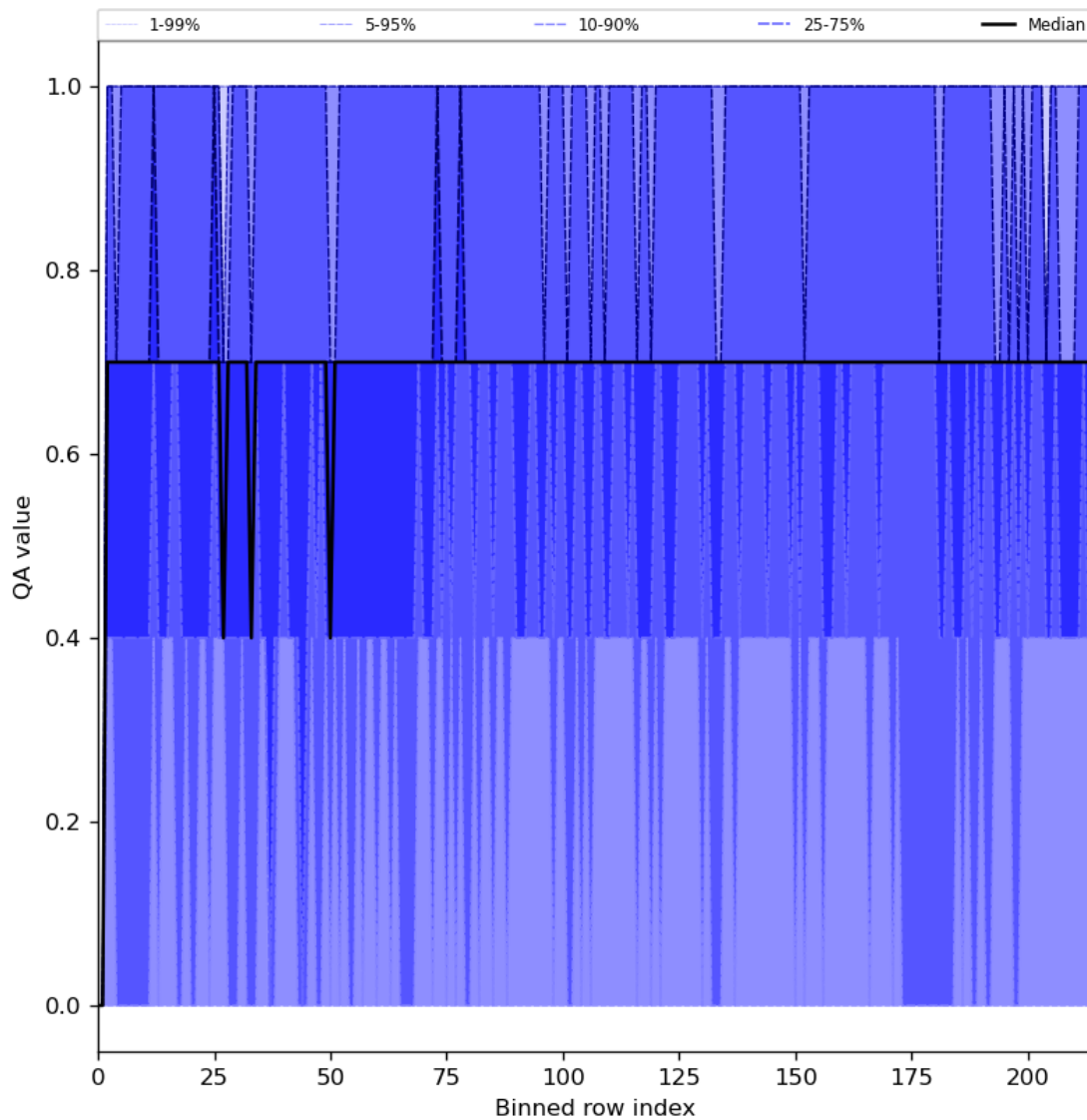
Figure 25: Along track statistics of “QA value” for 2024-02-29 to 2024-03-02
