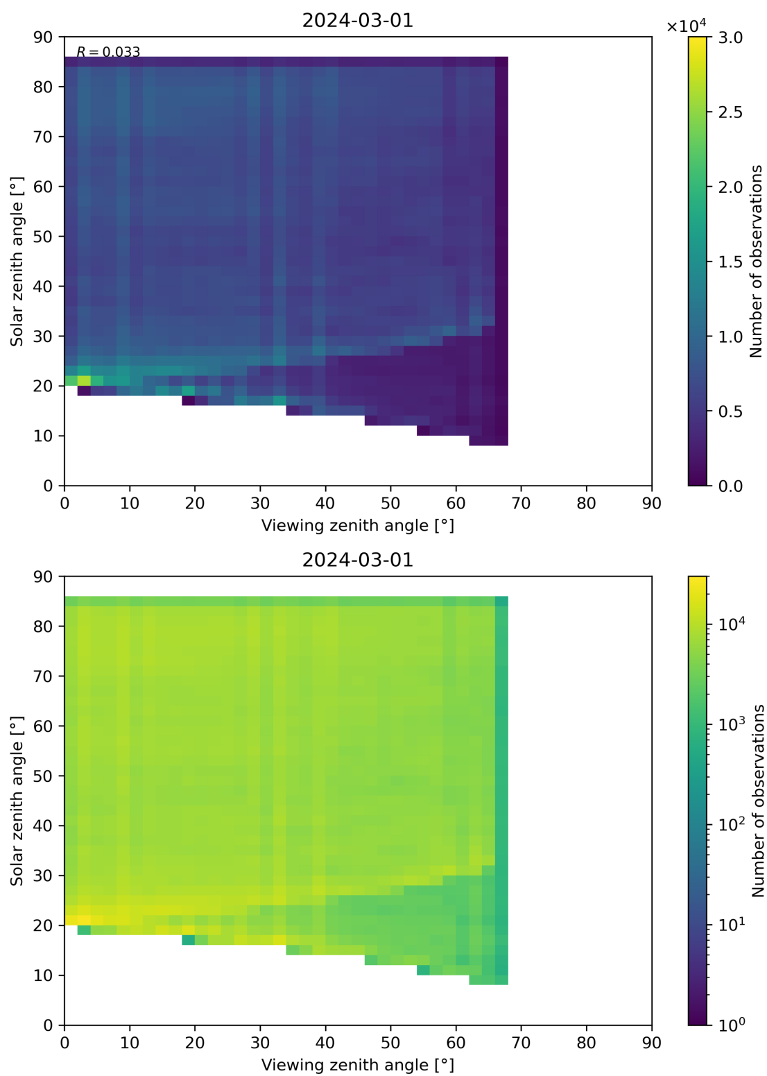
Figure 77: Scatter density plot of “Viewing zenith angle” against “Solar zenith angle” for 2024-02-29 to 2024-03-02.
