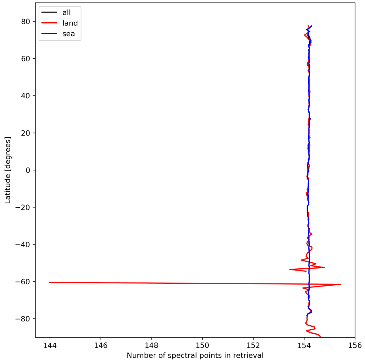
Figure 13: Zonal average of “Number of spectral points in retrieval” for 2024-02-29 to 2024-03-02.
