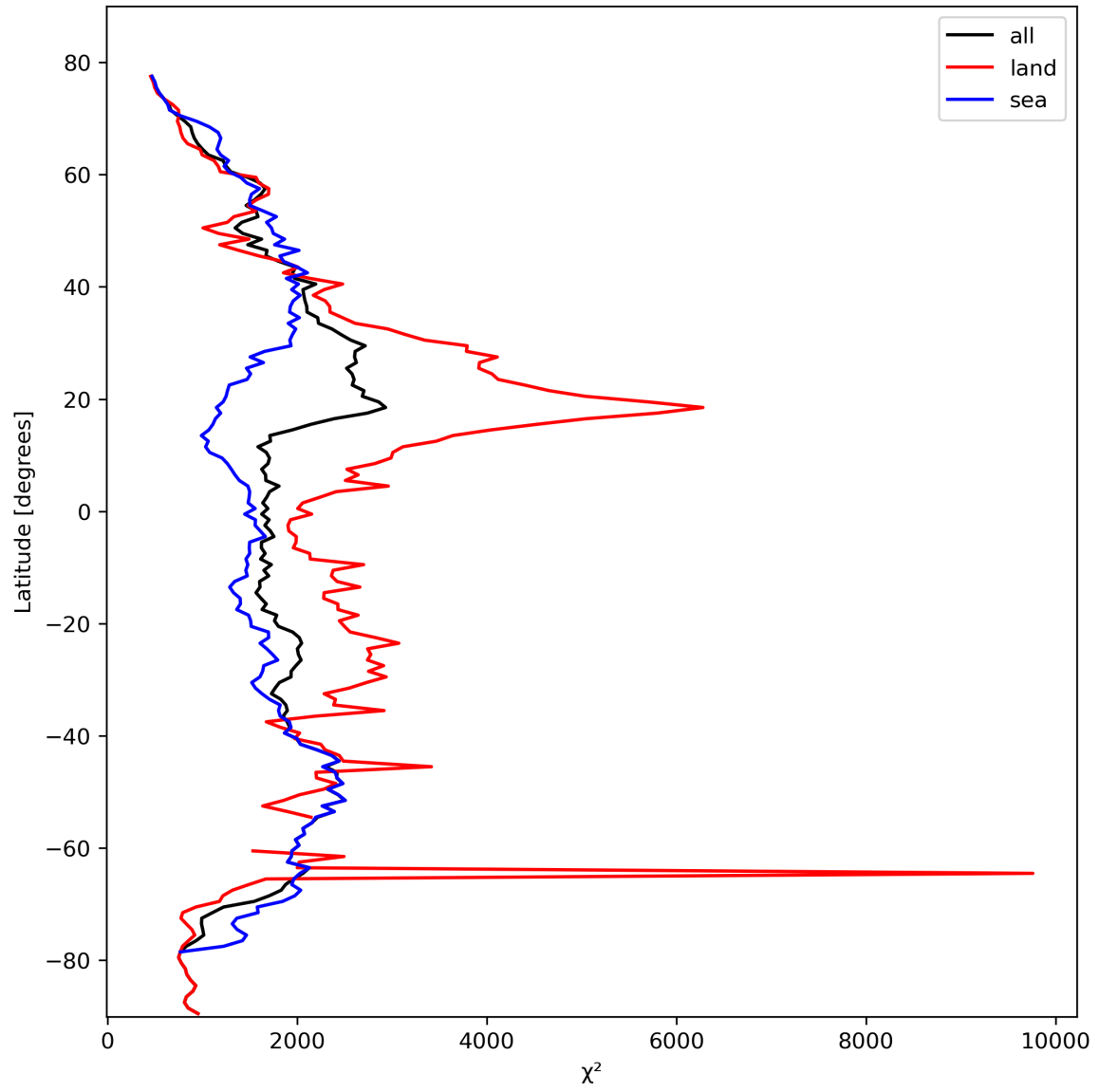
Figure 14: Zonal average of “ \chi^2 ” for 2024-02-29 to 2024-03-02.
