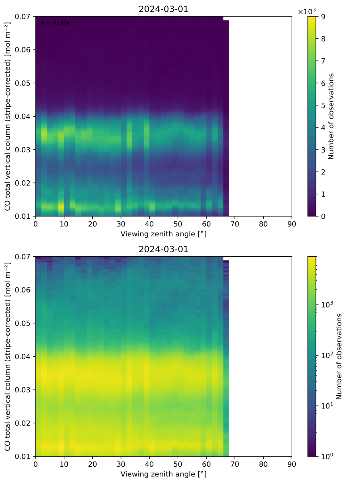
Figure 70: Scatter density plot of “Viewing zenith angle” against “CO total vertical column (stripe-corrected)” for 2024-02-29 to 2024-03-02.
