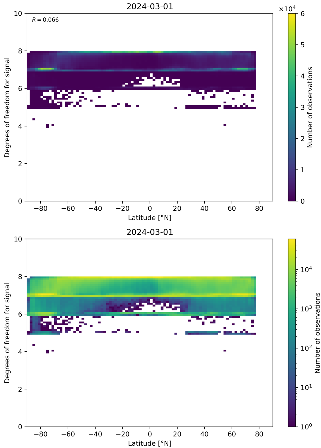
Figure 55: Scatter density plot of “Latitude” against “Degrees of freedom for signal” for 2024-02-29 to 2024-03-02.
