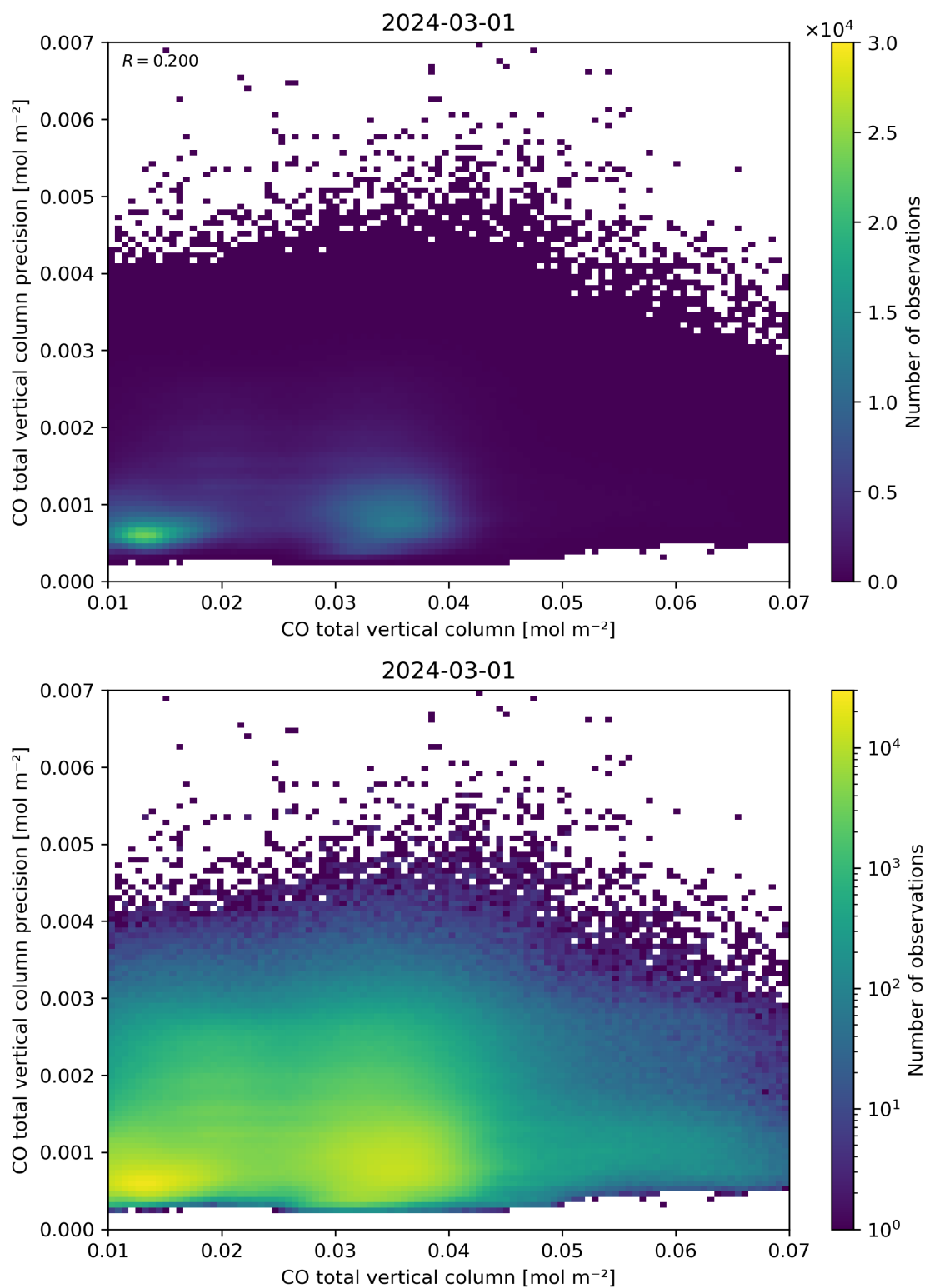
Figure 34: Scatter density plot of “CO total vertical column” against “CO total vertical column precision” for 2024-02-29 to 2024-03-02.
