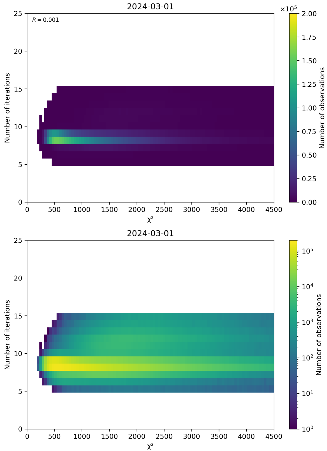
Figure 49: Scatter density plot of “ \chi^2 ” against “Number of iterations” for 2024-02-29 to 2024-03-02.
