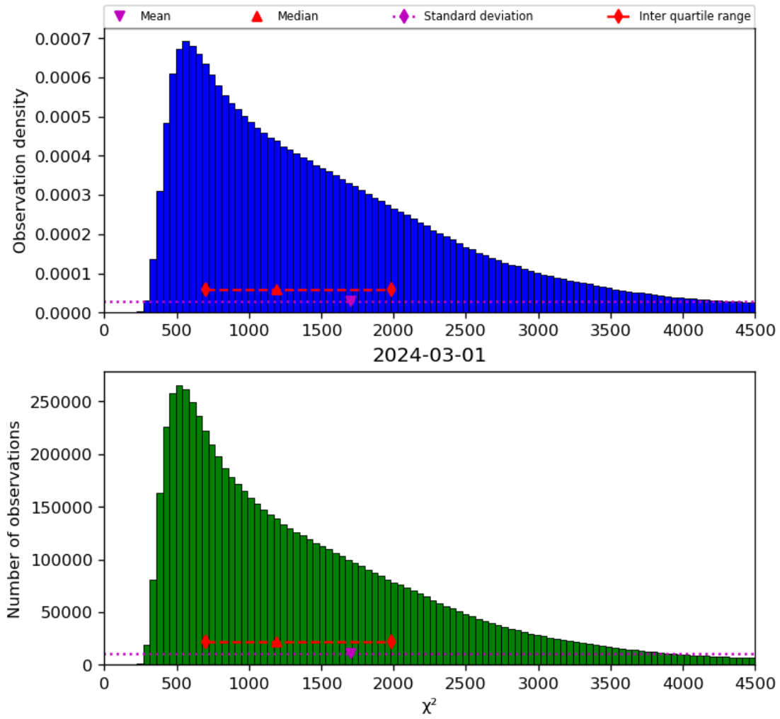
Figure 22: Histogram of “ \chi^2 ” for 2024-02-29 to 2024-03-02
