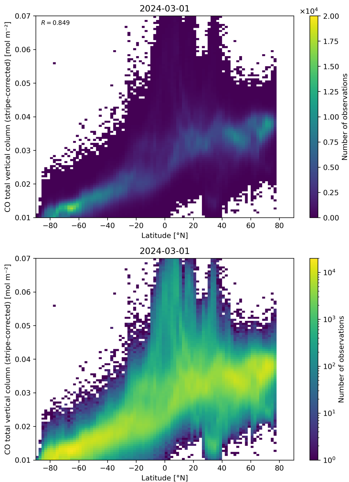
Figure 52: Scatter density plot of “Latitude” against “CO total vertical column (stripe-corrected)” for 2024-02-29 to 2024-03-02.
