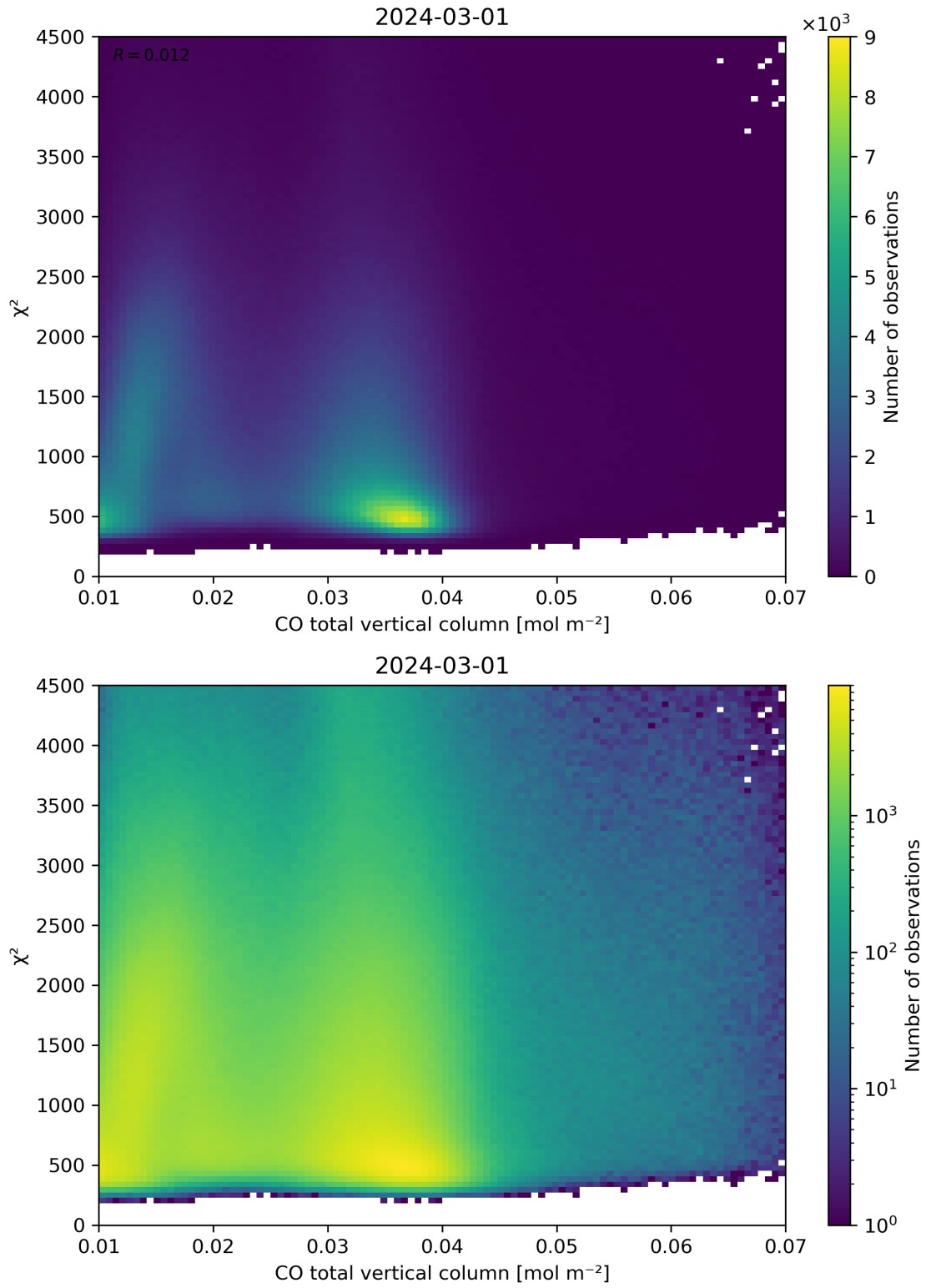
Figure 35: Scatter density plot of “CO total vertical column” against “ \chi^2 ” for 2024-02-29 to 2024-03-02.
