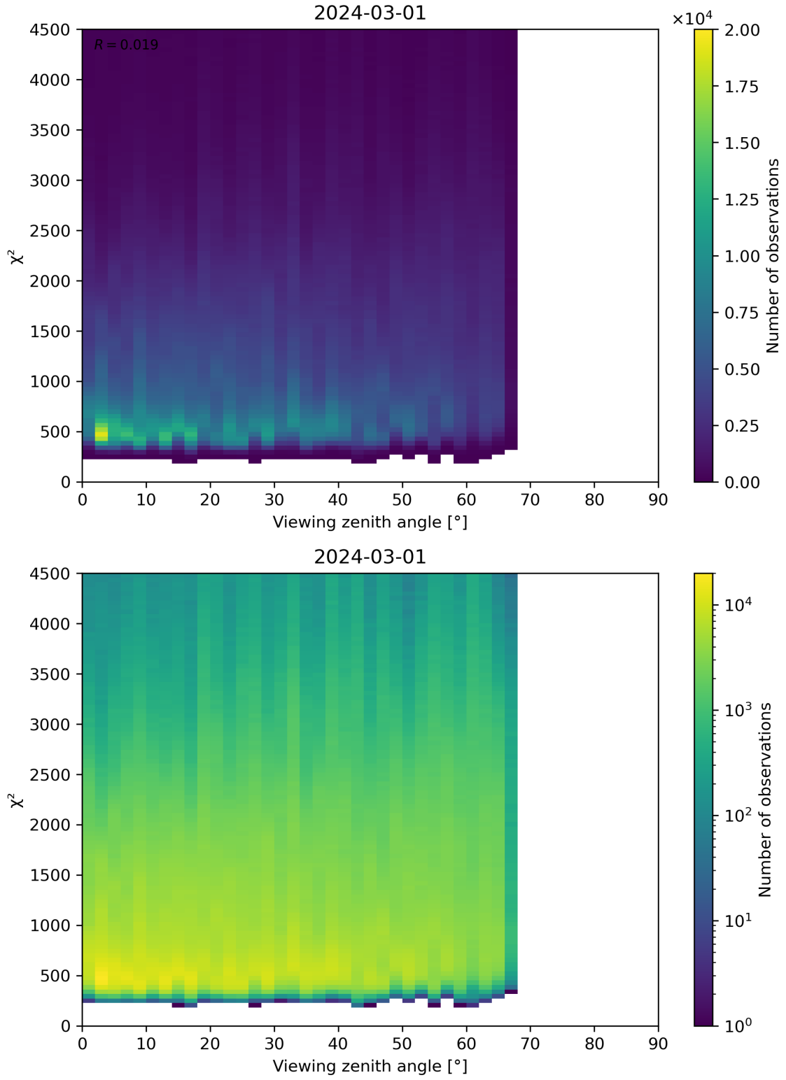
Figure 72: Scatter density plot of “Viewing zenith angle” against “ \chi^2 ” for 2024-02-29 to 2024-03-02.
