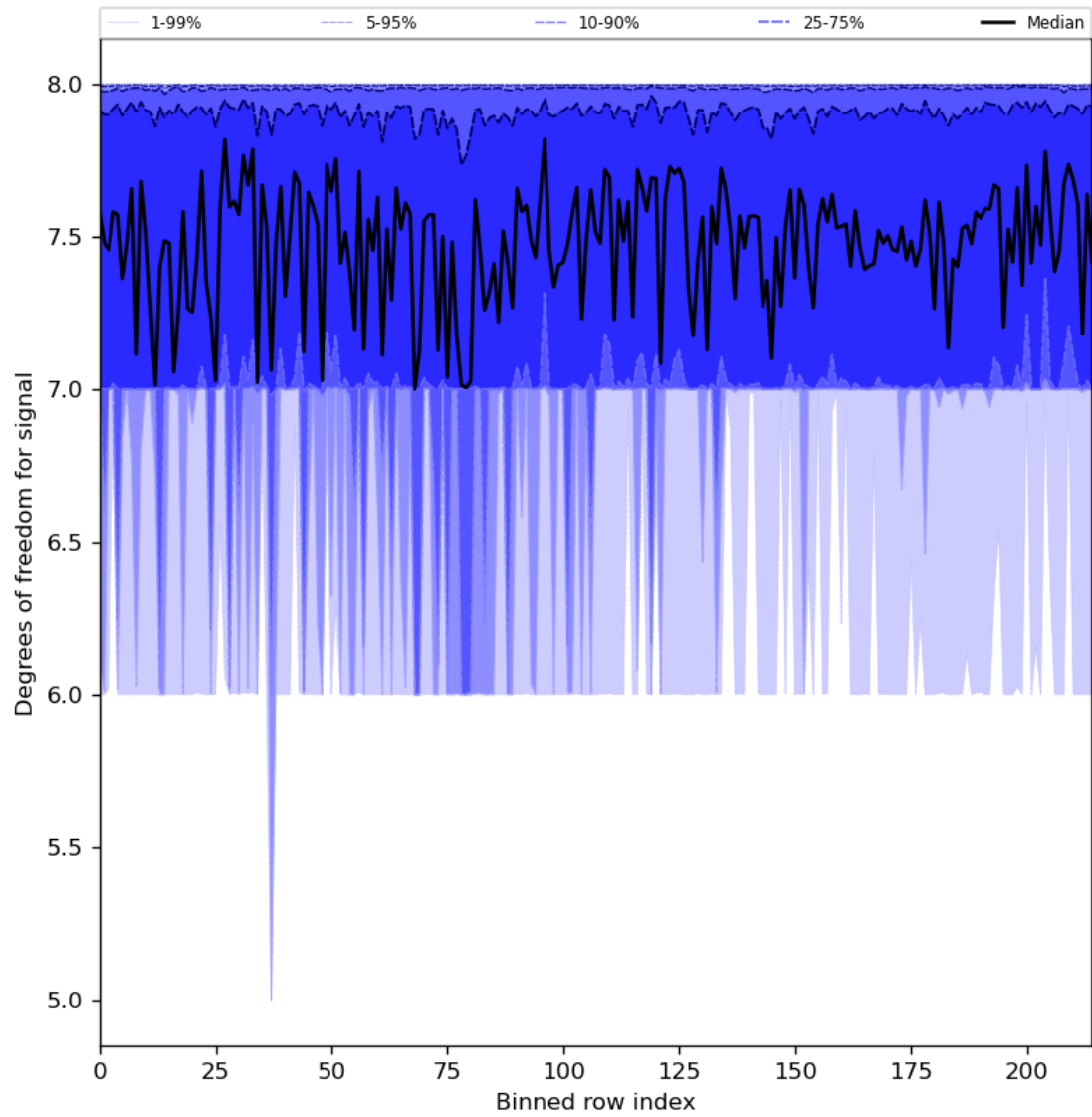
Figure 31: Along track statistics of “Degrees of freedom for signal” for 2024-02-29 to 2024-03-02
