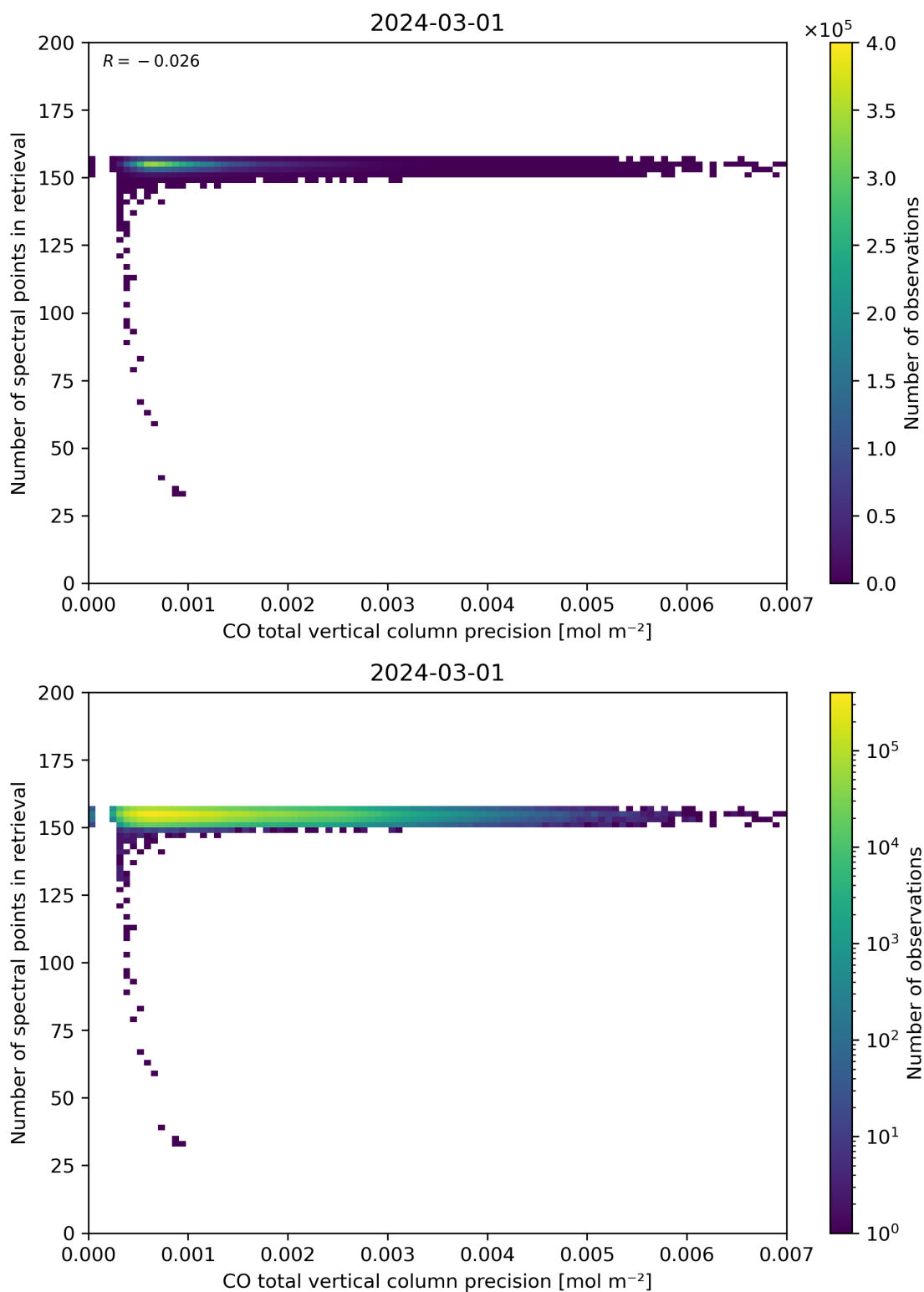
Figure 47: Scatter density plot of “CO total vertical column precision” against “Number of spectral points in retrieval” for 2024-02-29 to 2024-03-02.
