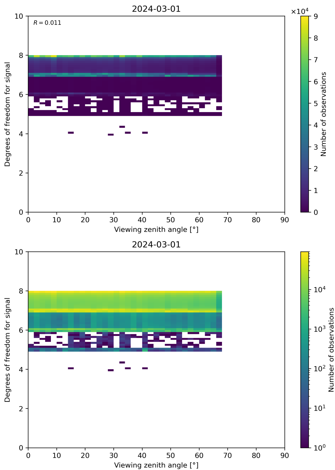
Figure 73: Scatter density plot of “Viewing zenith angle” against “Degrees of freedom for signal” for 2024-02-29 to 2024-03-02.
