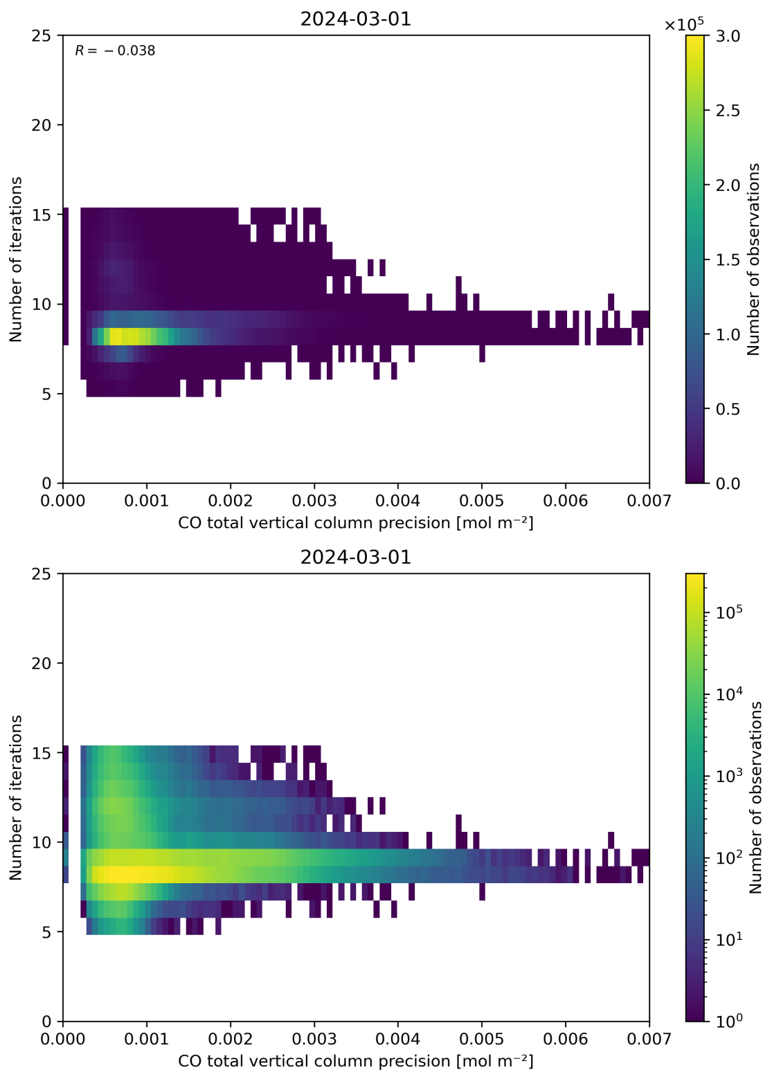
Figure 46: Scatter density plot of “CO total vertical column precision” against “Number of iterations” for 2024-02-29 to 2024-03-02.
