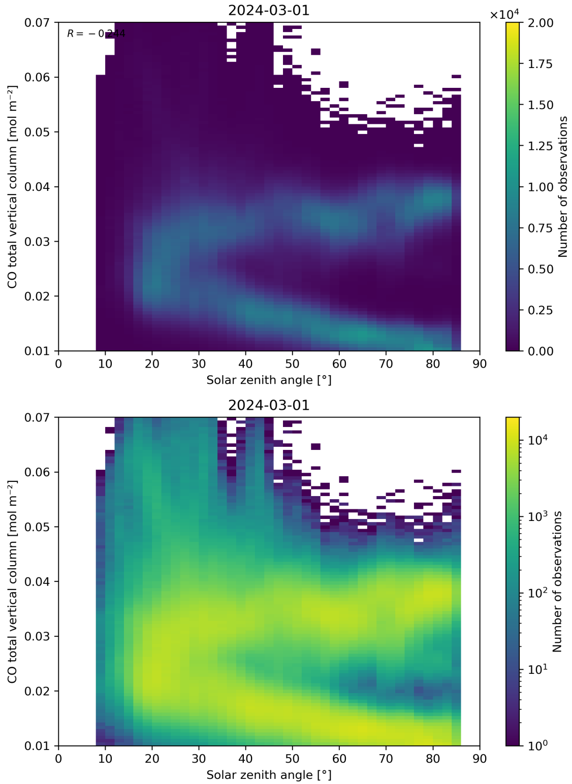
Figure 61: Scatter density plot of “Solar zenith angle” against “CO total vertical column” for 2024-02-29 to 2024-03-02.
