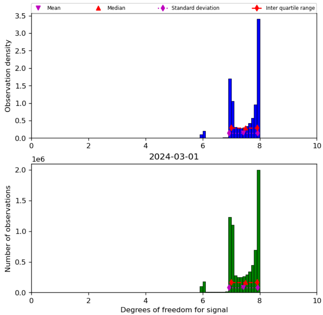
Figure 23: Histogram of “Degrees of freedom for signal” for 2024-02-29 to 2024-03-02
