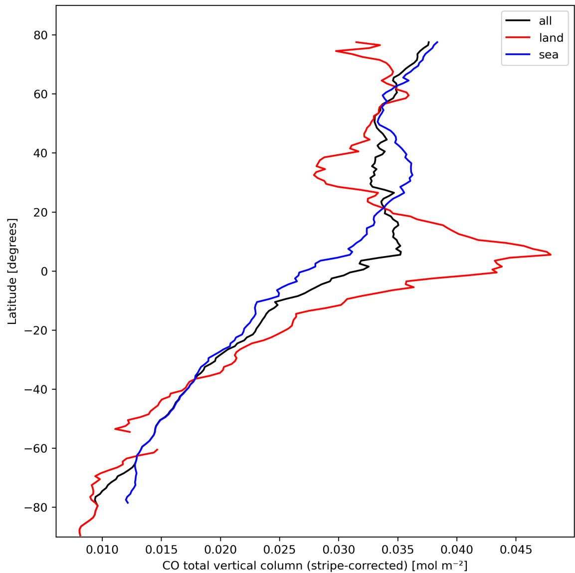
Figure 11: Zonal average of “CO total vertical column (stripe-corrected)” for 2024-02-29 to 2024-03-02.
