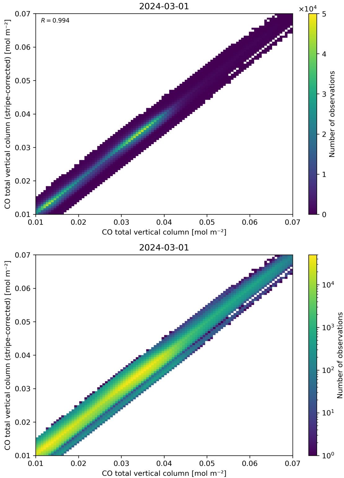
Figure 33: Scatter density plot of “CO total vertical column” against “CO total vertical column (stripe-corrected)” for 2024-02-29 to 2024-03-02.
