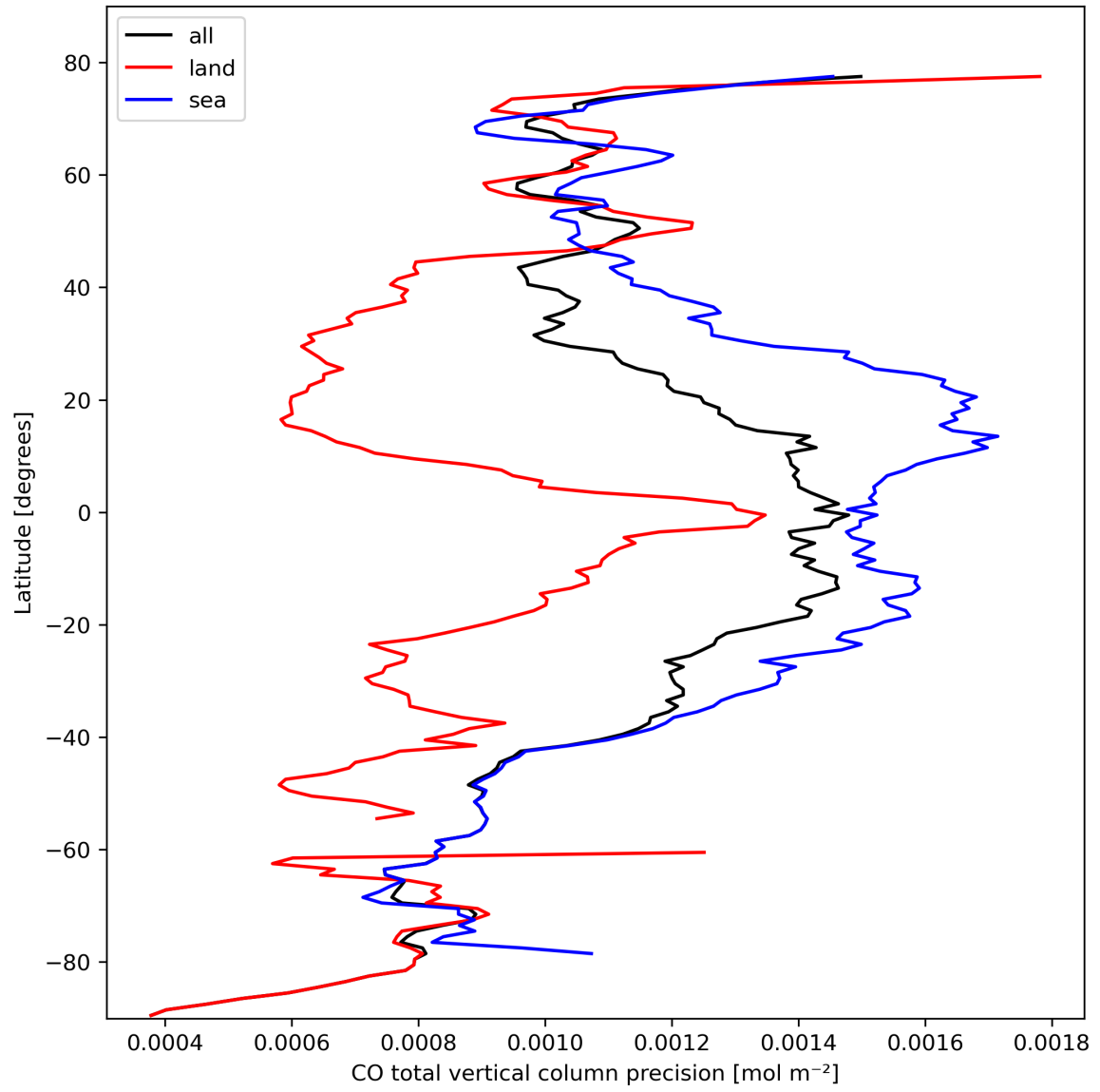
Figure 12: Zonal average of “CO total vertical column precision” for 2024-02-29 to 2024-03-02.
