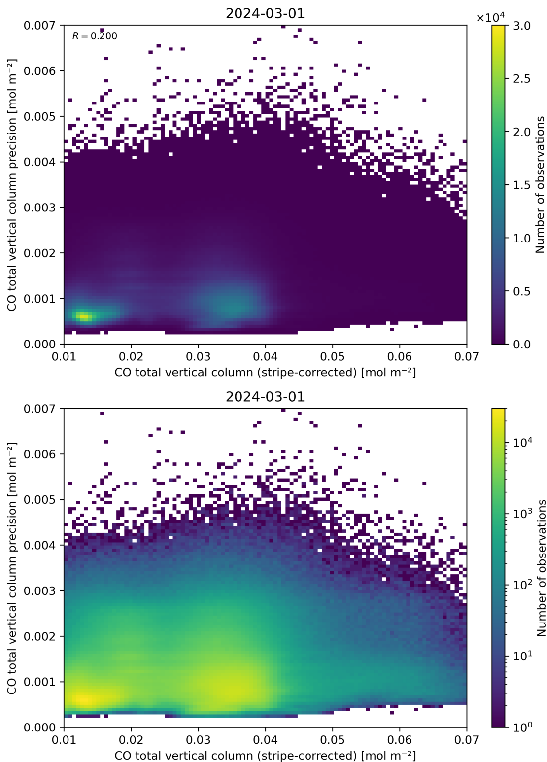
Figure 36: Scatter density plot of “CO total vertical column (stripe-corrected)” against “CO total vertical column precision” for 2024-02-29 to 2024-03-02.
