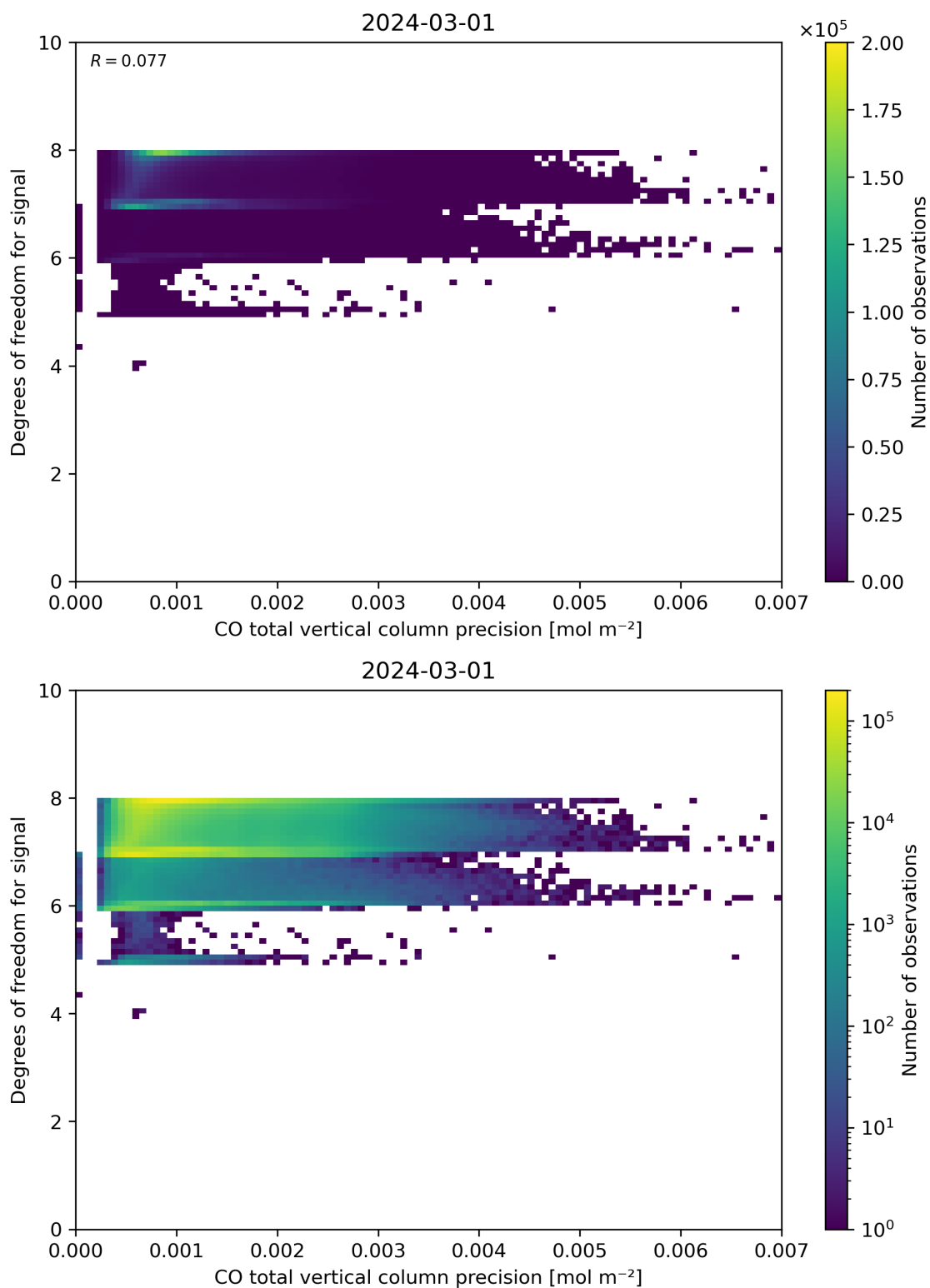
Figure 45: Scatter density plot of “CO total vertical column precision” against “Degrees of freedom for signal” for 2024-02-29 to 2024-03-02.
