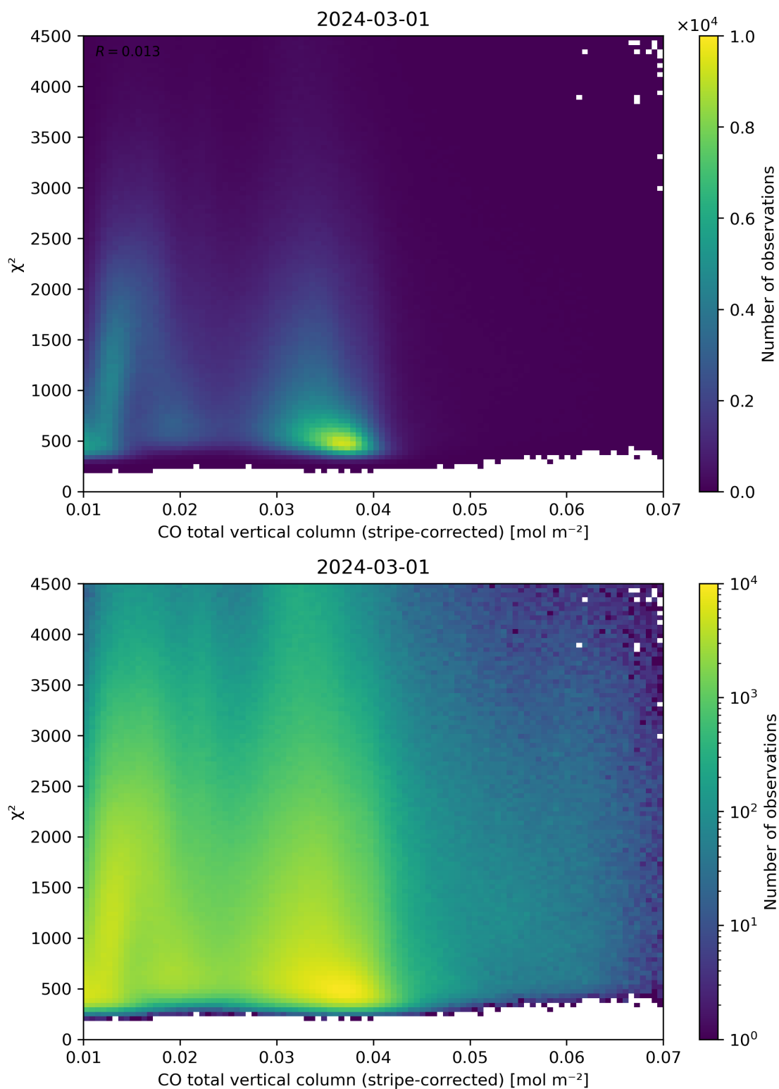
Figure 37: Scatter density plot of “CO total vertical column (stripe-corrected)” against “ \chi^2 ” for 2024-02-29 to 2024-03-02.
