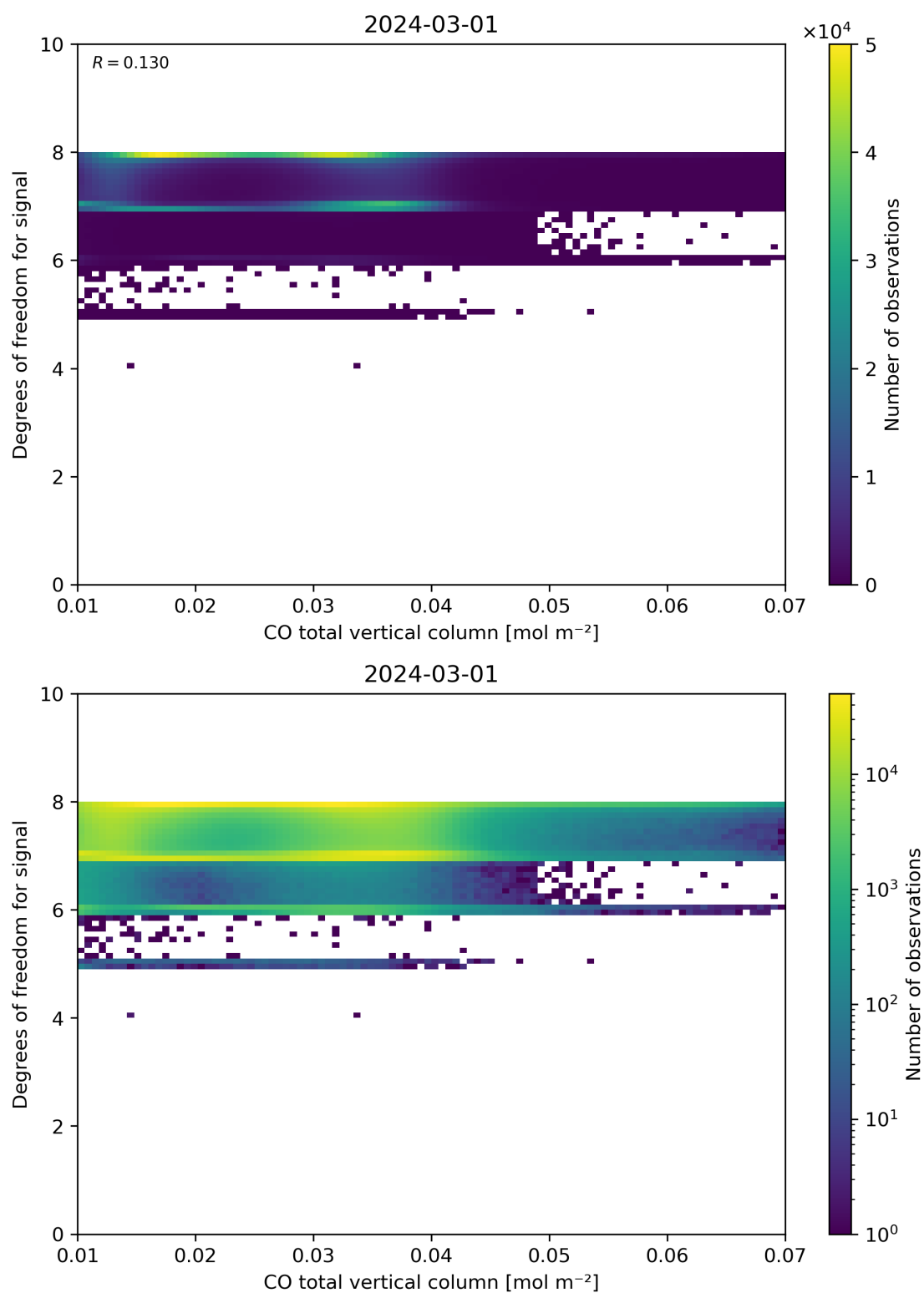
Figure 41: Scatter density plot of “CO total vertical column” against “Degrees of freedom for signal” for 2024-02-29 to 2024-03-02.
