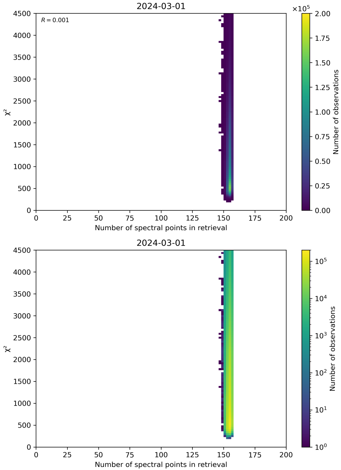
Figure 58: Scatter density plot of “Number of spectral points in retrieval” against “ \chi^2 ” for 2024-02-29 to 2024-03-02.
