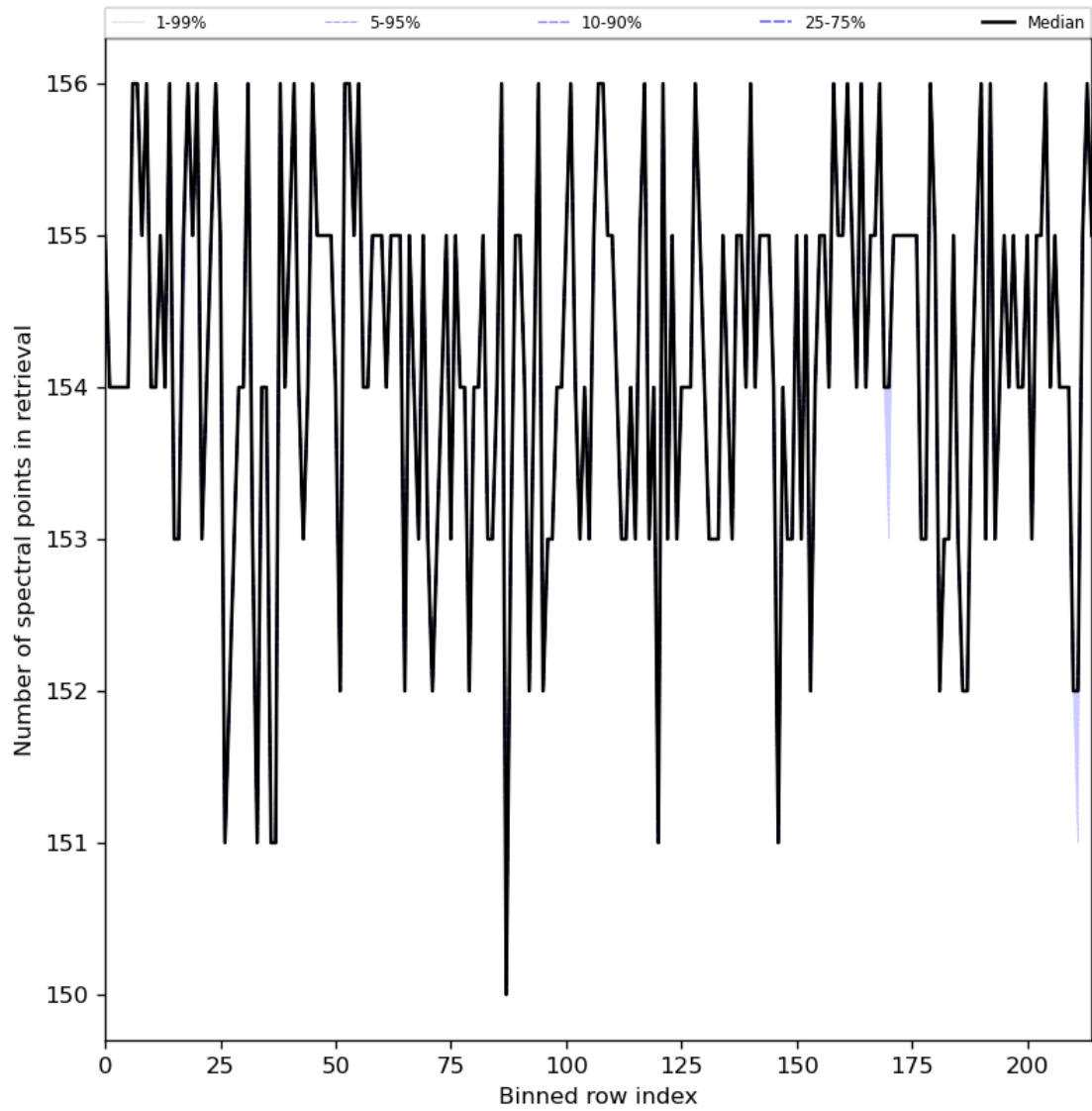
Figure 29: Along track statistics of “Number of spectral points in retrieval” for 2024-02-29 to 2024-03-02
