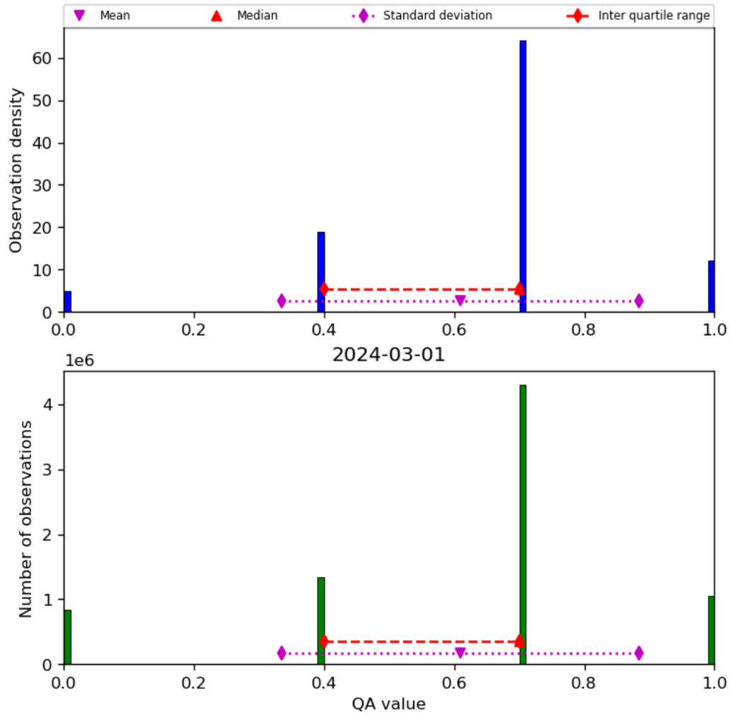
Figure 17: Histogram of “QA value” for 2024-02-29 to 2024-03-02
