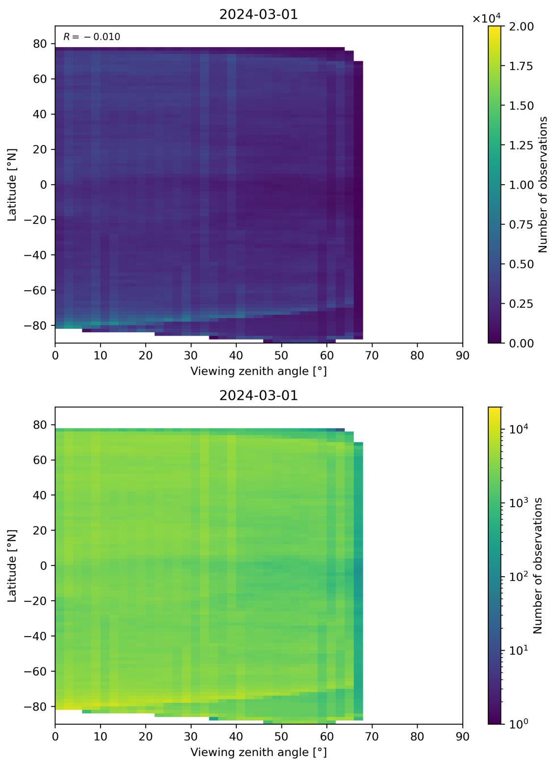
Figure 74: Scatter density plot of “Viewing zenith angle” against “Latitude” for 2024-02-29 to 2024-03-02.
