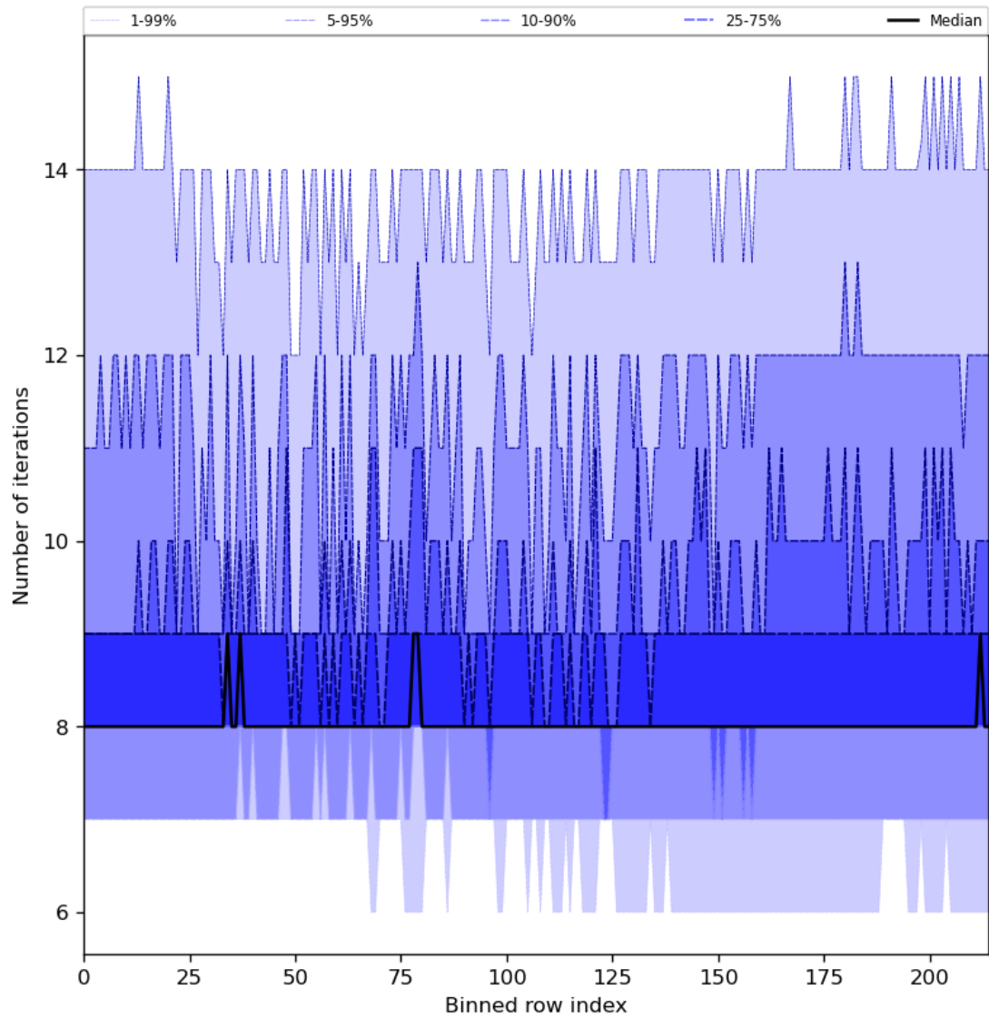
Figure 32: Along track statistics of “Number of iterations” for 2024-02-29 to 2024-03-02
