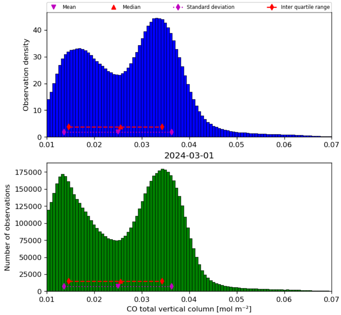
Figure 18: Histogram of “CO total vertical column” for 2024-02-29 to 2024-03-02
