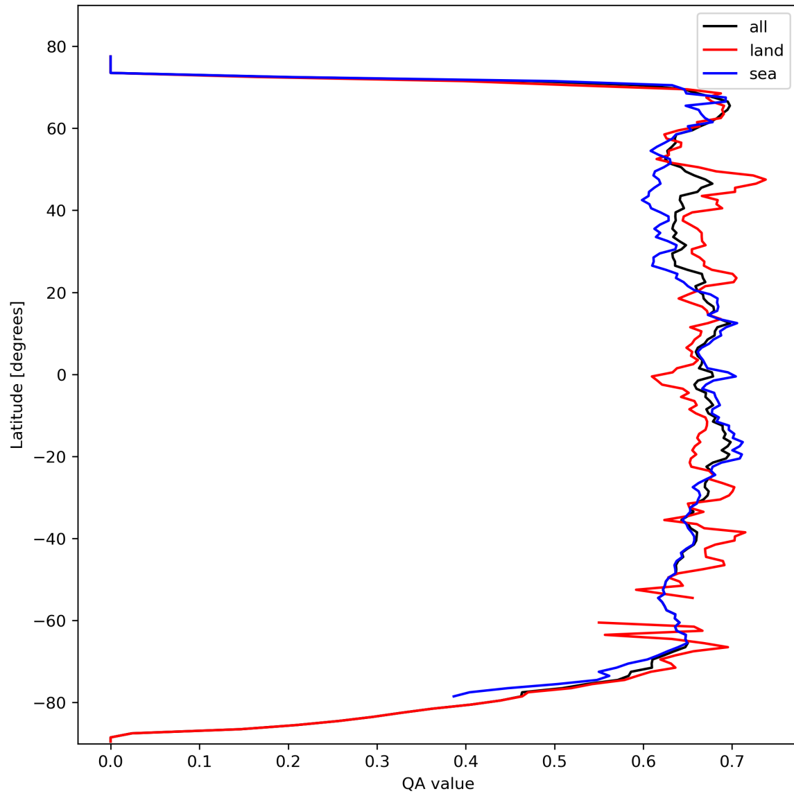
Figure 9: Zonal average of “QA value” for 2024-02-29 to 2024-03-02.
