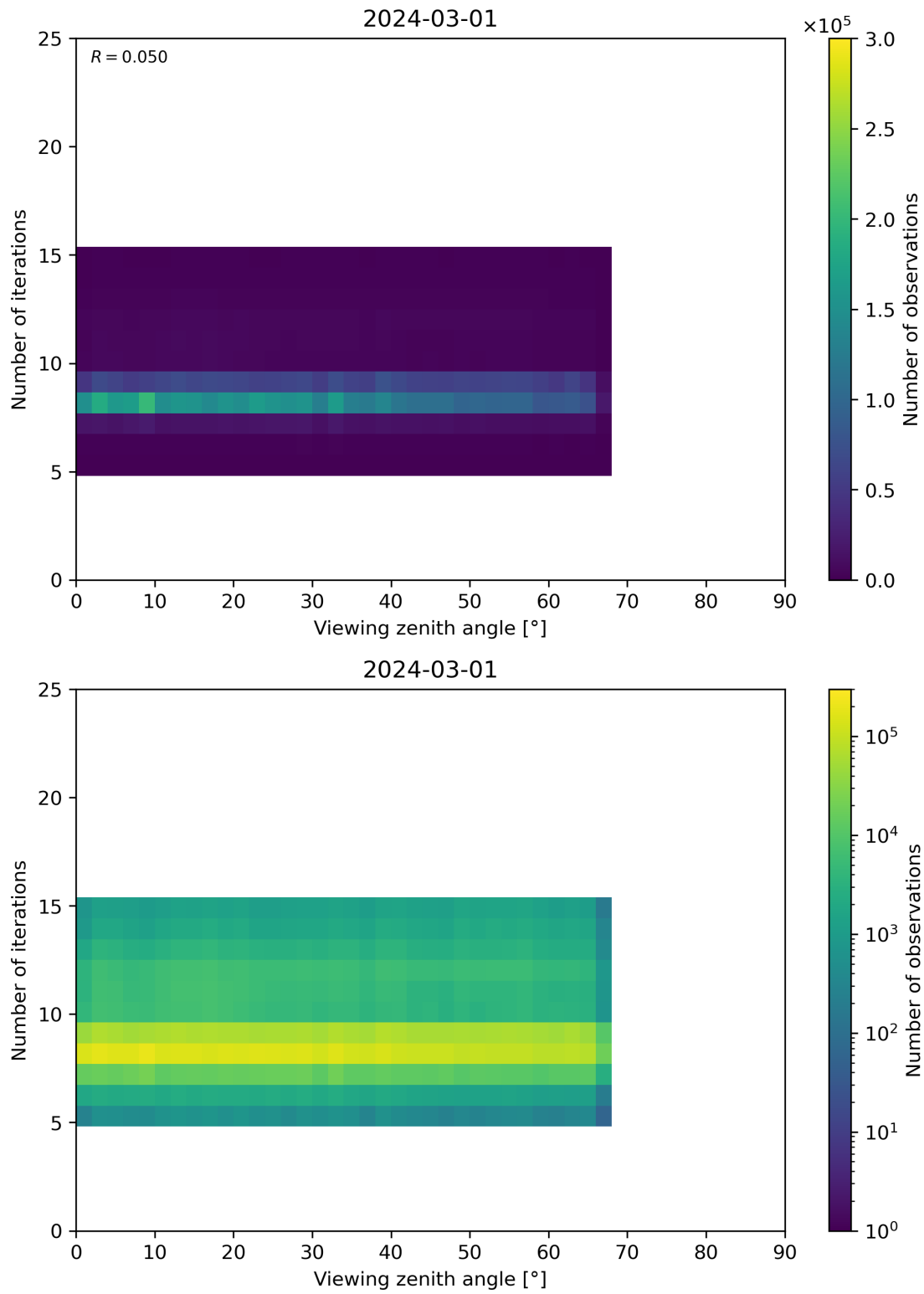
Figure 75: Scatter density plot of “Viewing zenith angle” against “Number of iterations” for 2024-02-29 to 2024-03-02.
