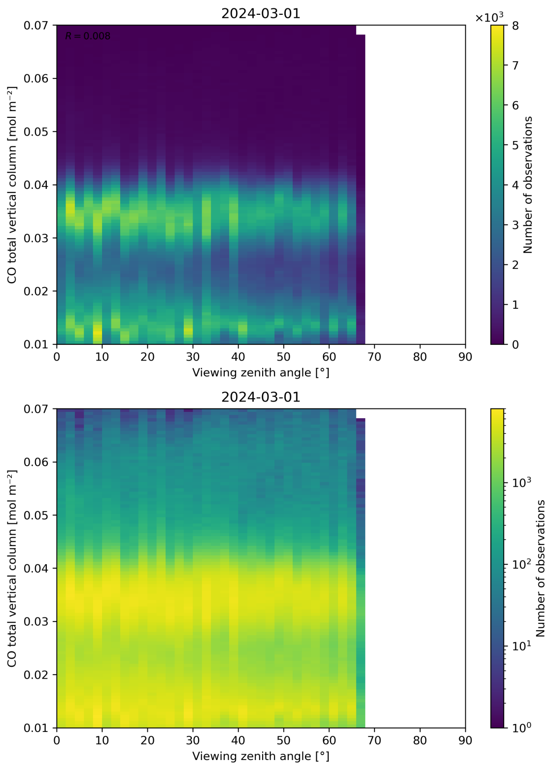
Figure 69: Scatter density plot of “Viewing zenith angle” against “CO total vertical column” for 2024-02-29 to 2024-03-02.
