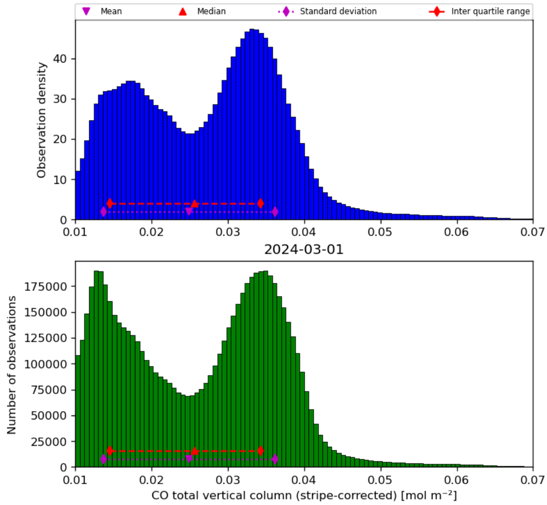
Figure 19: Histogram of “CO total vertical column (stripe-corrected)” for 2024-02-29 to 2024-03-02
