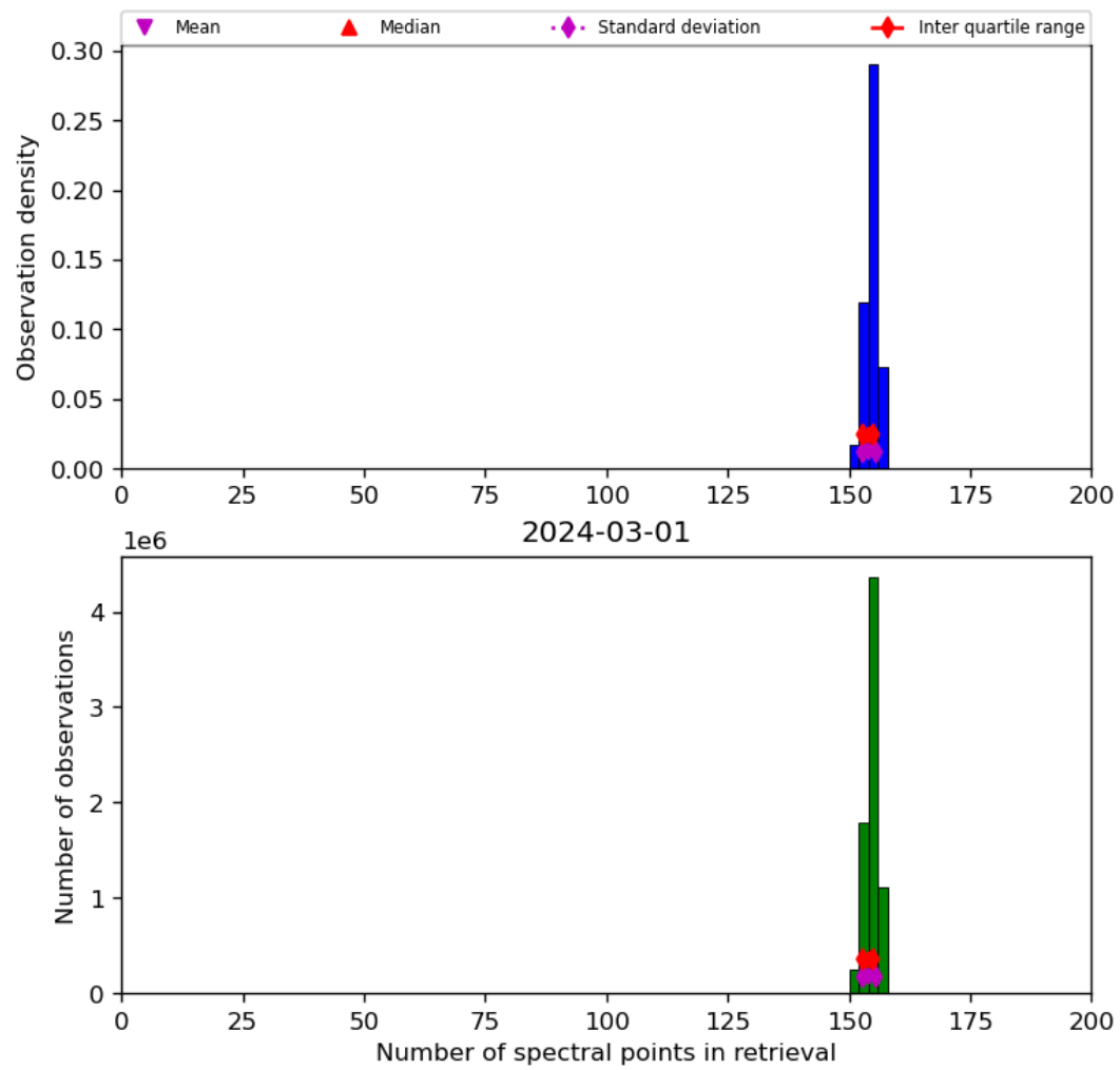
Figure 21: Histogram of “Number of spectral points in retrieval” for 2024-02-29 to 2024-03-02
