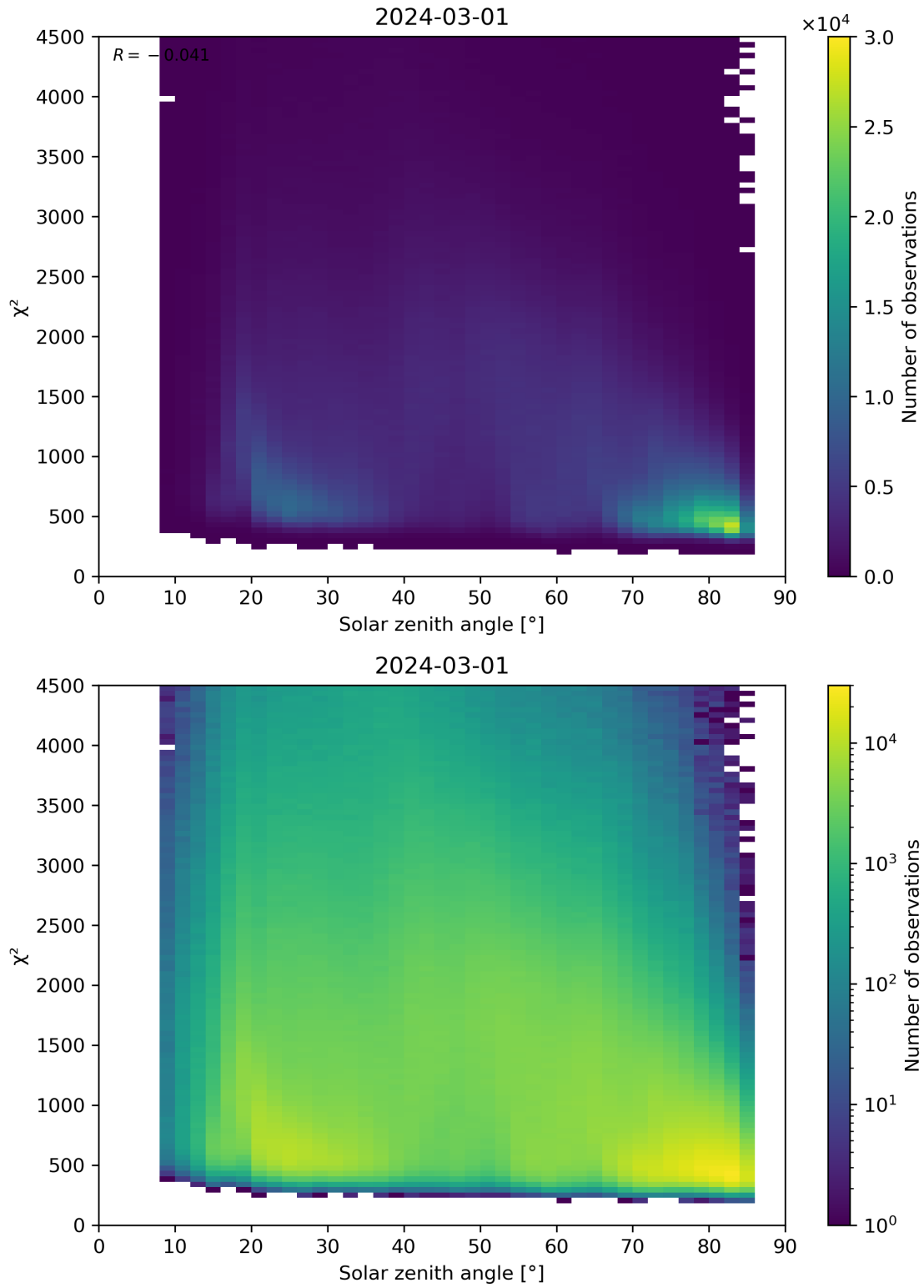
Figure 64: Scatter density plot of “Solar zenith angle” against “ \chi^2 ” for 2024-02-29 to 2024-03-02.
