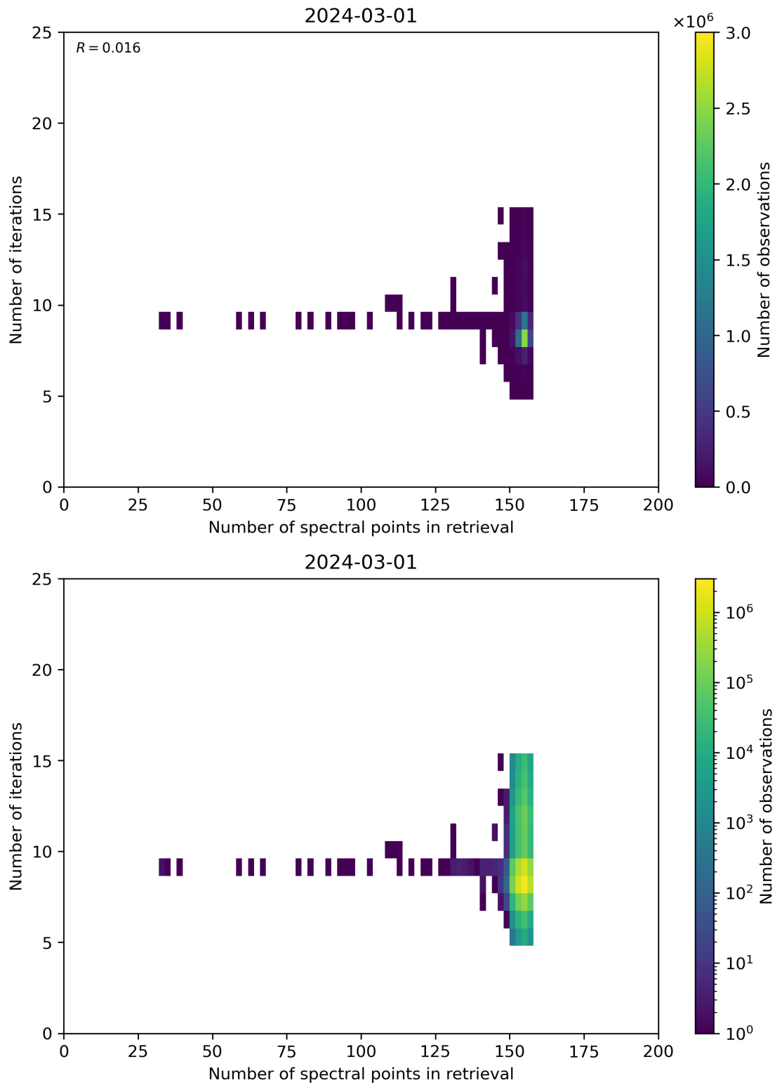
Figure 60: Scatter density plot of “Number of spectral points in retrieval” against “Number of iterations” for 2024-02-29 to 2024-03-02.
