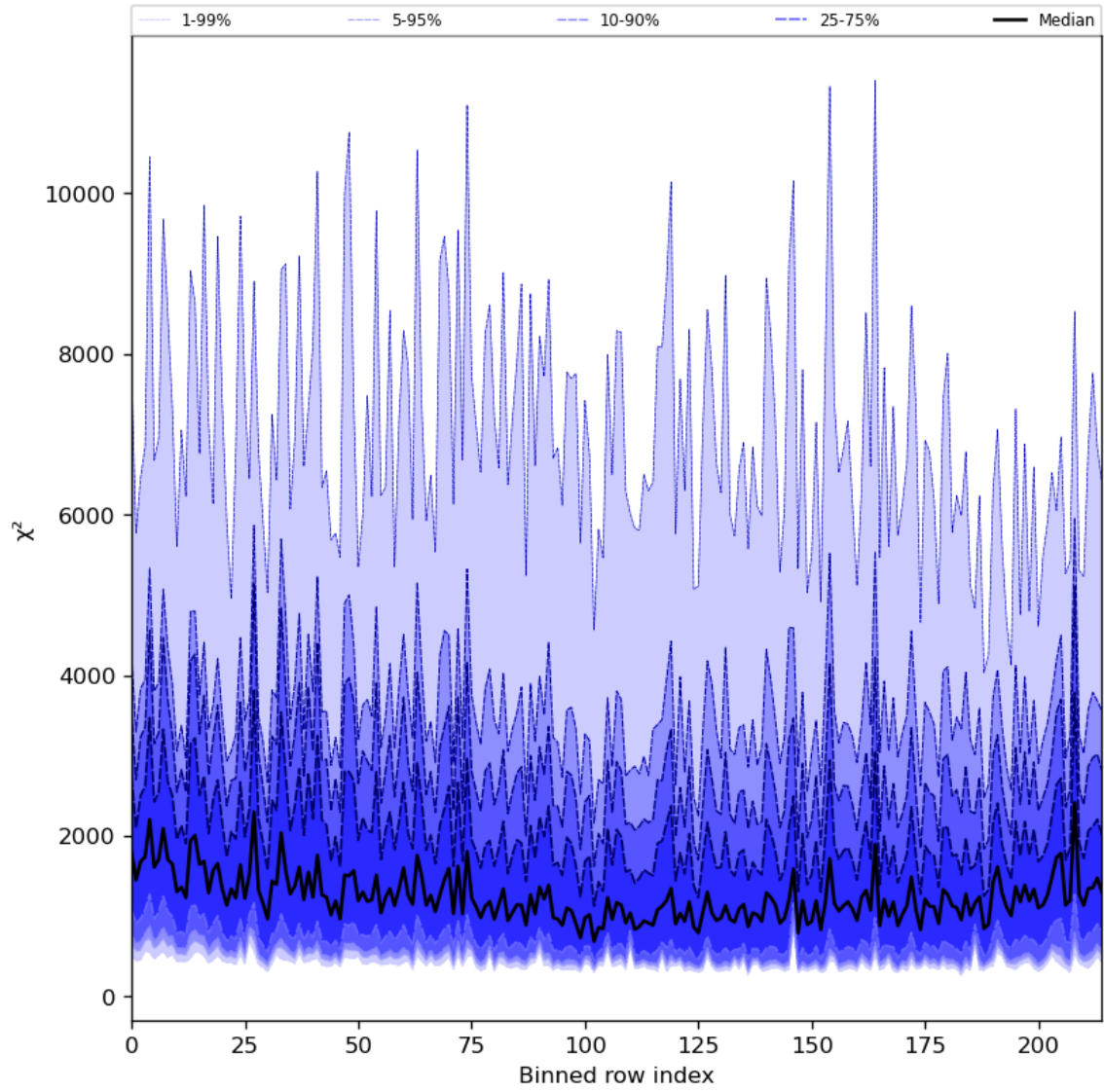
Figure 30: Along track statistics of “ \chi^2 ” for 2024-02-29 to 2024-03-02
