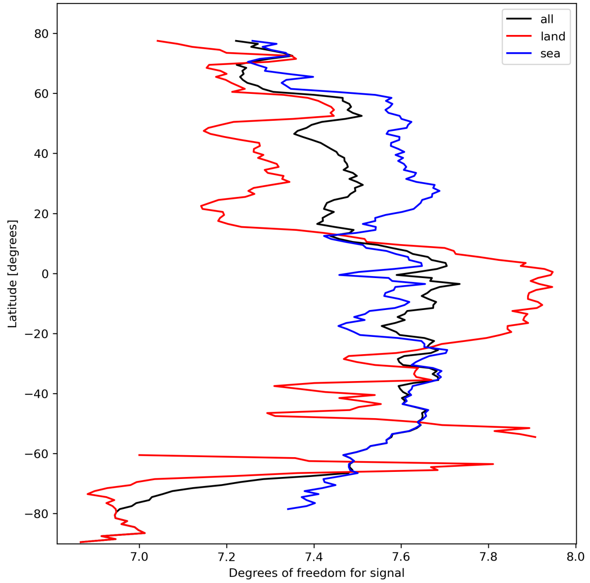
Figure 15: Zonal average of “Degrees of freedom for signal” for 2024-02-29 to 2024-03-02.
