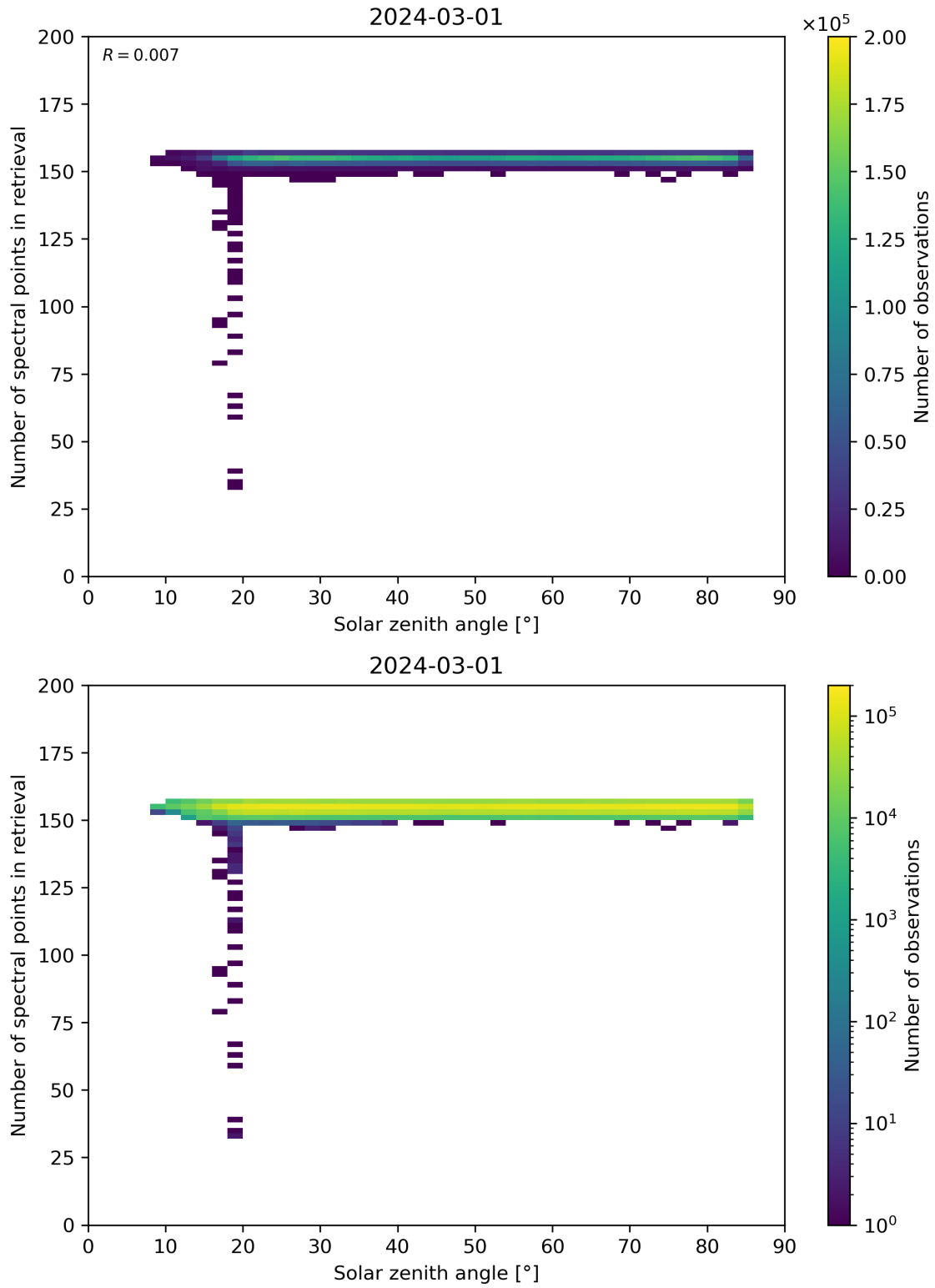
Figure 68: Scatter density plot of “Solar zenith angle” against “Number of spectral points in retrieval” for 2024-02-29 to 2024-03-02.
