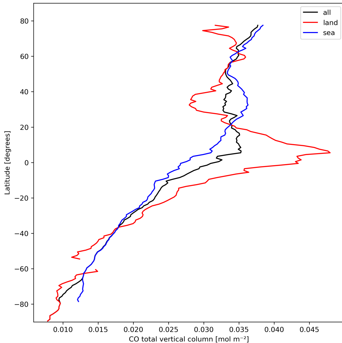
Figure 10: Zonal average of “CO total vertical column” for 2024-02-29 to 2024-03-02.
