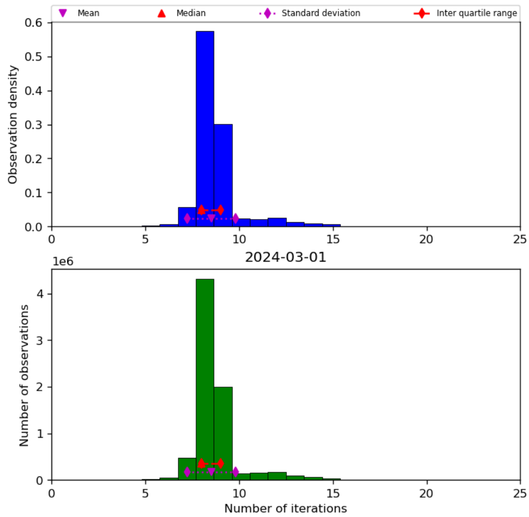
Figure 24: Histogram of “Number of iterations” for 2024-02-29 to 2024-03-02
