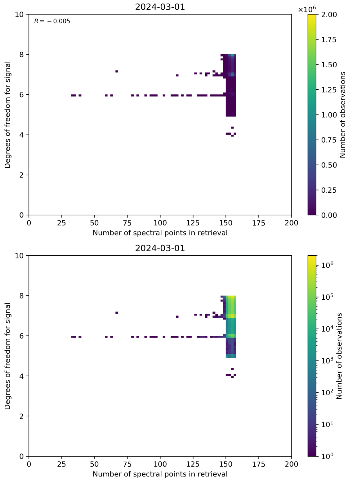
Figure 59: Scatter density plot of “Number of spectral points in retrieval” against “Degrees of freedom for signal” for 2024-02-29 to 2024-03-02.
