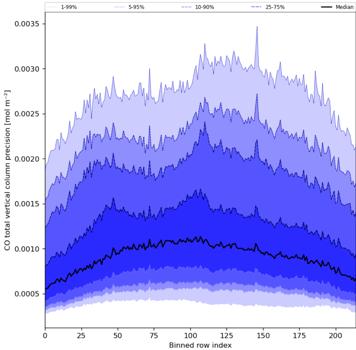
Figure 28: Along track statistics of “CO total vertical column precision” for 2024-02-29 to 2024-03-02
