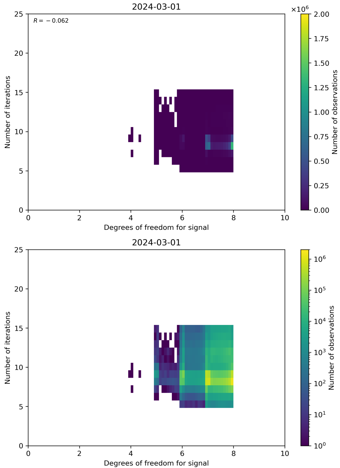
Figure 50: Scatter density plot of “Degrees of freedom for signal” against “Number of iterations” for 2024-02-29 to 2024-03-02.
