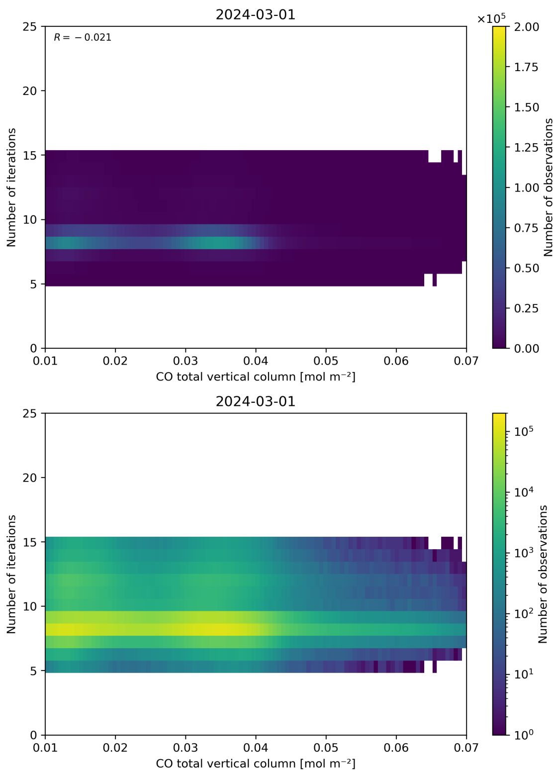
Figure 42: Scatter density plot of “CO total vertical column” against “Number of iterations” for 2024-02-29 to 2024-03-02.
