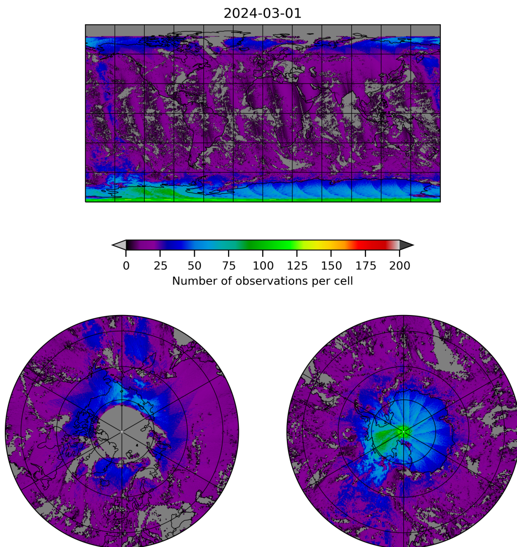
Figure 8: Map of the number of observations for 2024-02-29 to 2024-03-02
