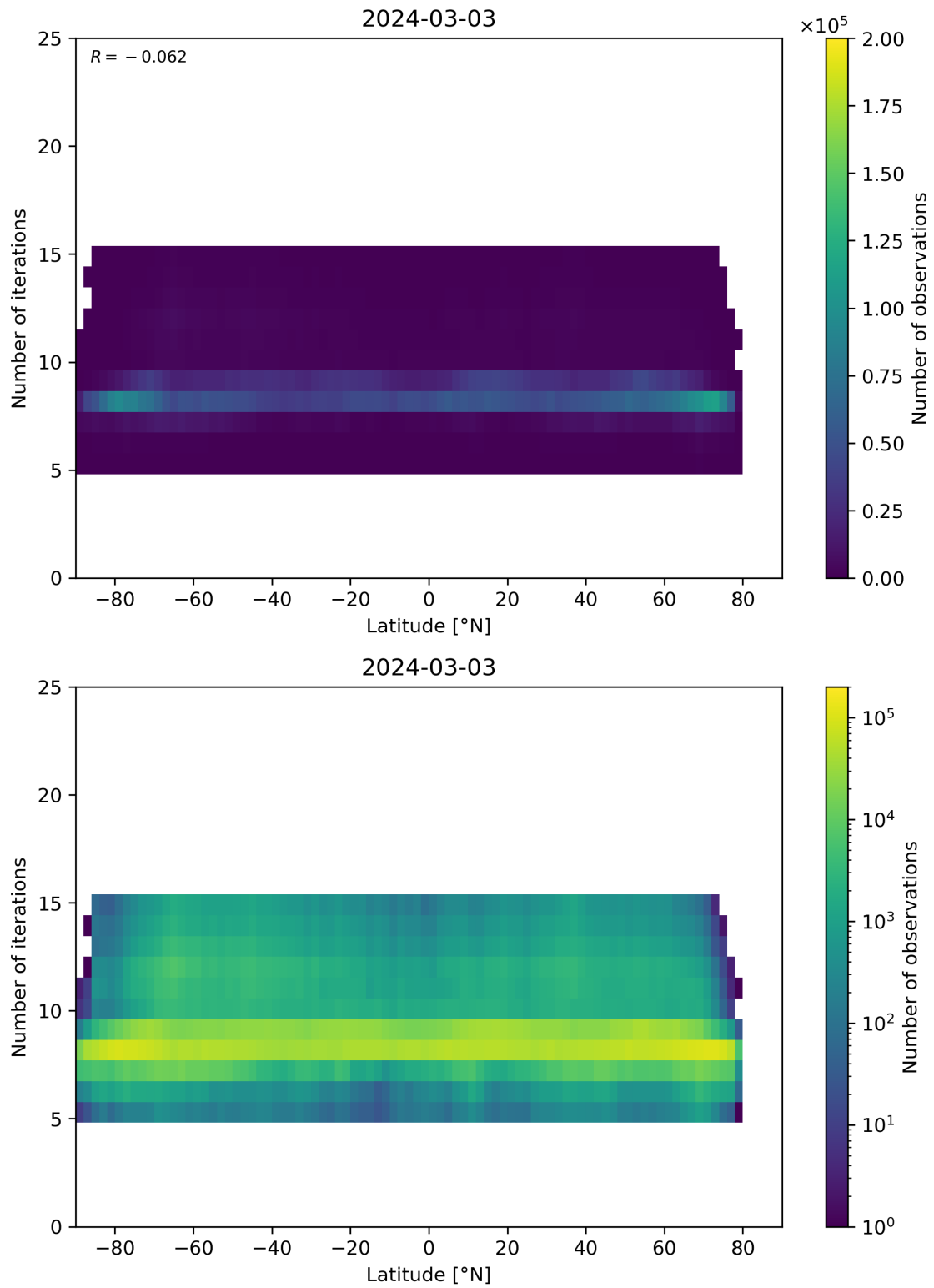
Figure 56: Scatter density plot of “Latitude” against “Number of iterations” for 2024-03-02 to 2024-03-04.
