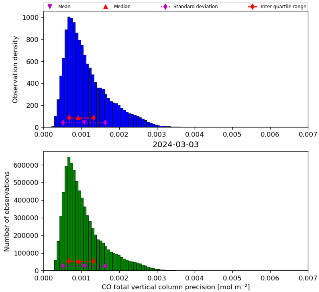
Figure 20: Histogram of “CO total vertical column precision” for 2024-03-02 to 2024-03-04
