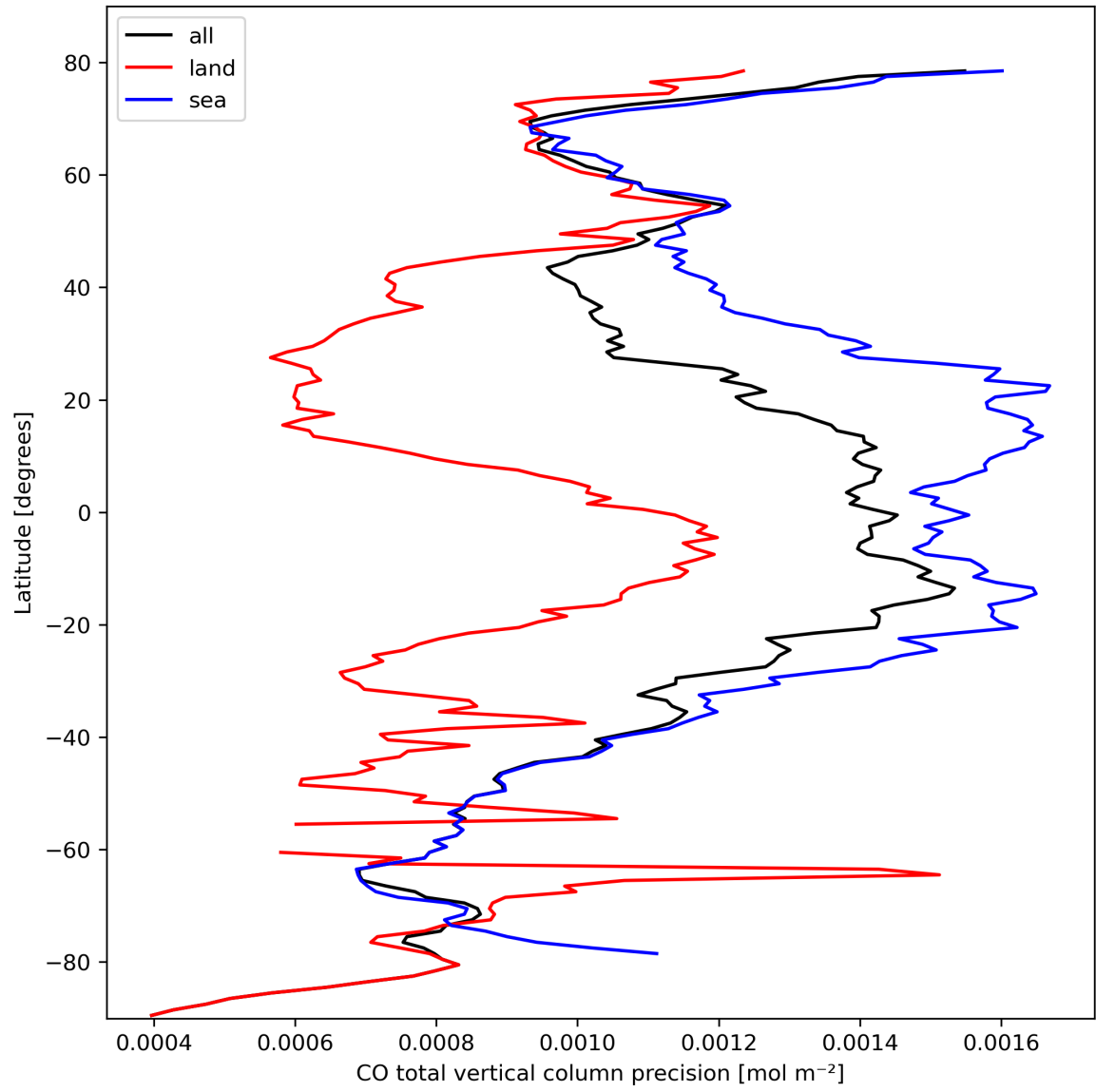
Figure 12: Zonal average of “CO total vertical column precision” for 2024-03-02 to 2024-03-04.
