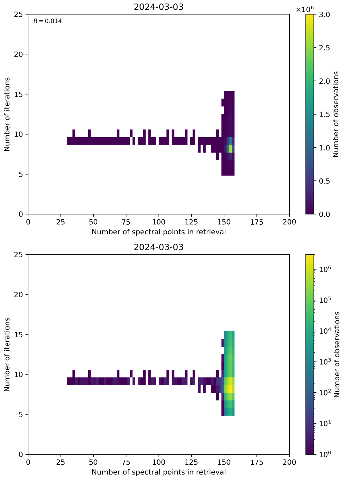
Figure 60: Scatter density plot of “Number of spectral points in retrieval” against “Number of iterations” for 2024-03-02 to 2024-03-04.
