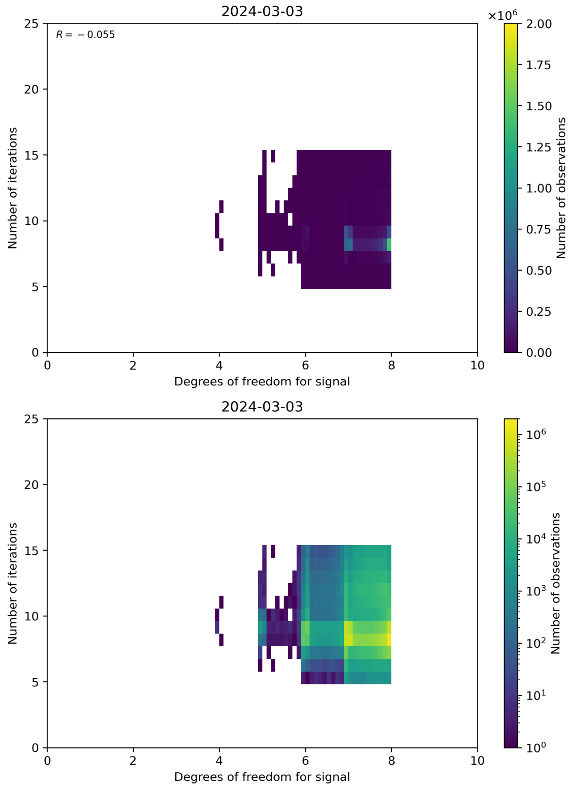
Figure 50: Scatter density plot of “Degrees of freedom for signal” against “Number of iterations” for 2024-03-02 to 2024-03-04.
