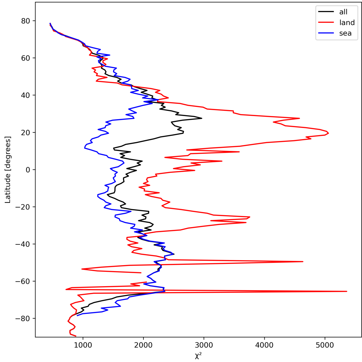
Figure 14: Zonal average of “ \chi^2 ” for 2024-03-02 to 2024-03-04.
