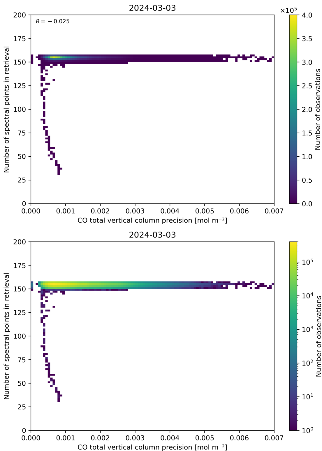
Figure 47: Scatter density plot of “CO total vertical column precision” against “Number of spectral points in retrieval” for 2024-03-02 to 2024-03-04.
