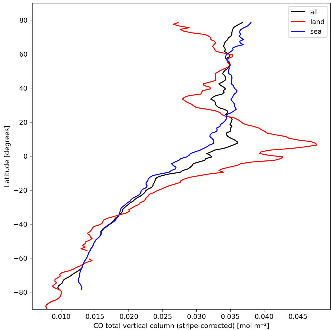
Figure 11: Zonal average of “CO total vertical column (stripe-corrected)” for 2024-03-02 to 2024-03-04.
