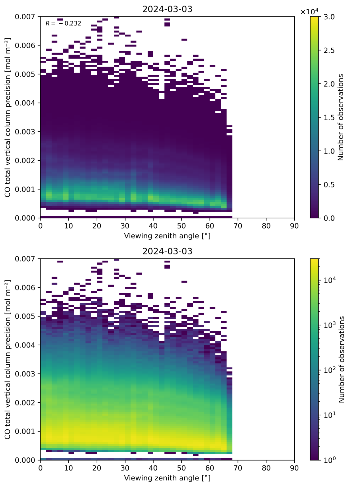
Figure 71: Scatter density plot of “Viewing zenith angle” against “CO total vertical column precision” for 2024-03-02 to 2024-03-04.
