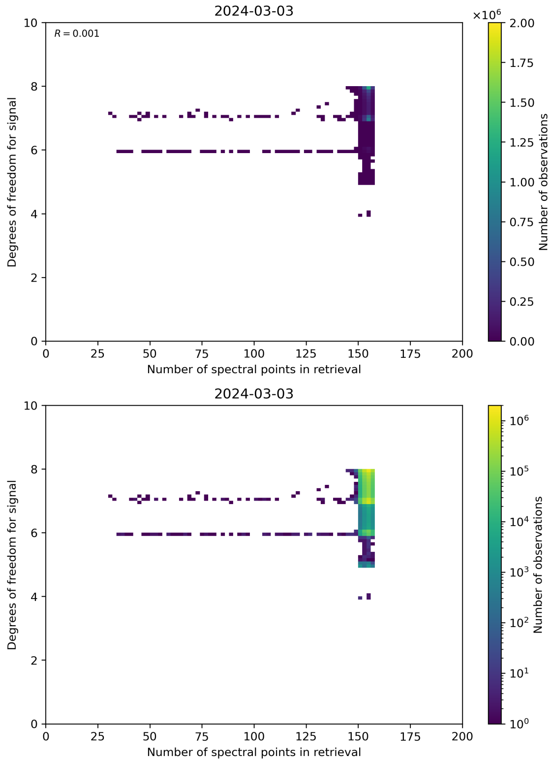
Figure 59: Scatter density plot of “Number of spectral points in retrieval” against “Degrees of freedom for signal” for 2024-03-02 to 2024-03-04.
