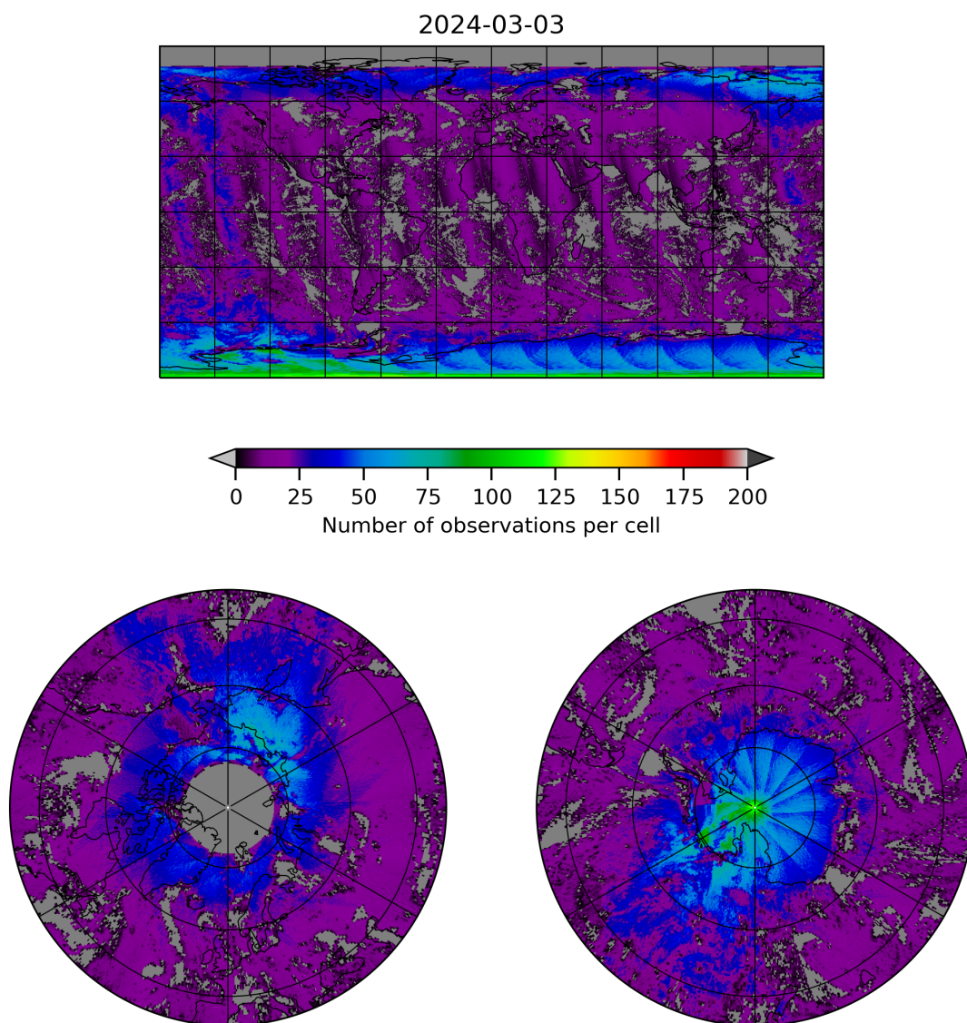
Figure 8: Map of the number of observations for 2024-03-02 to 2024-03-04
