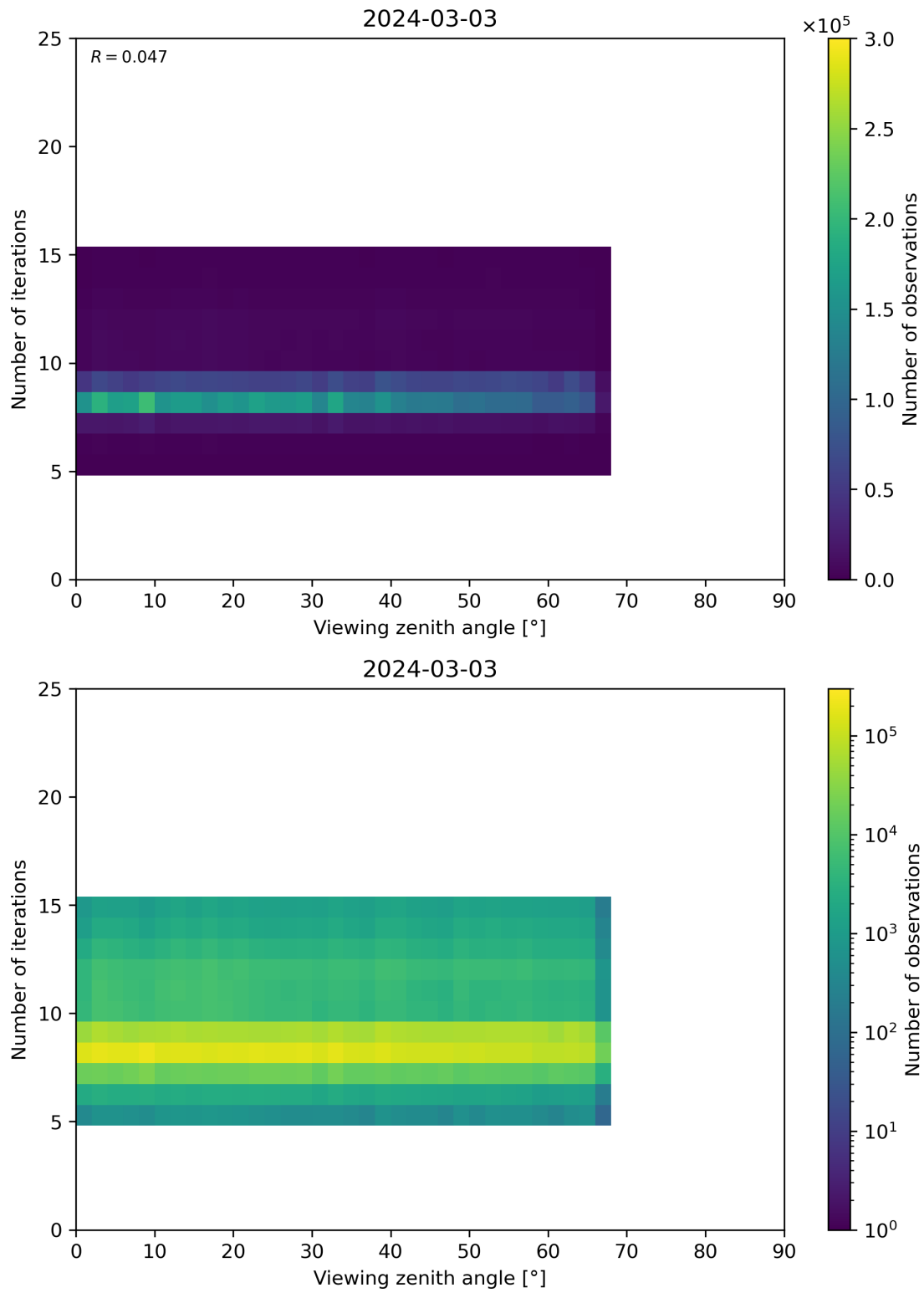
Figure 75: Scatter density plot of “Viewing zenith angle” against “Number of iterations” for 2024-03-02 to 2024-03-04.
