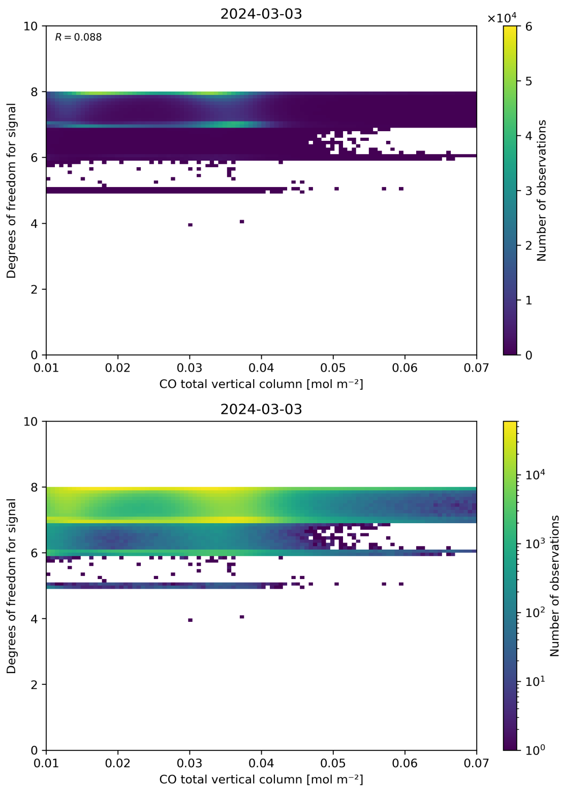
Figure 41: Scatter density plot of “CO total vertical column” against “Degrees of freedom for signal” for 2024-03-02 to 2024-03-04.
