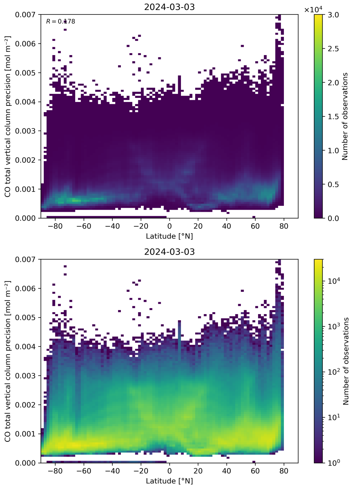
Figure 53: Scatter density plot of “Latitude” against “CO total vertical column precision” for 2024-03-02 to 2024-03-04.
