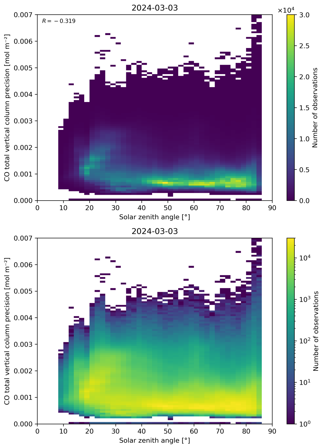
Figure 63: Scatter density plot of “Solar zenith angle” against “CO total vertical column precision” for 2024-03-02 to 2024-03-04.
