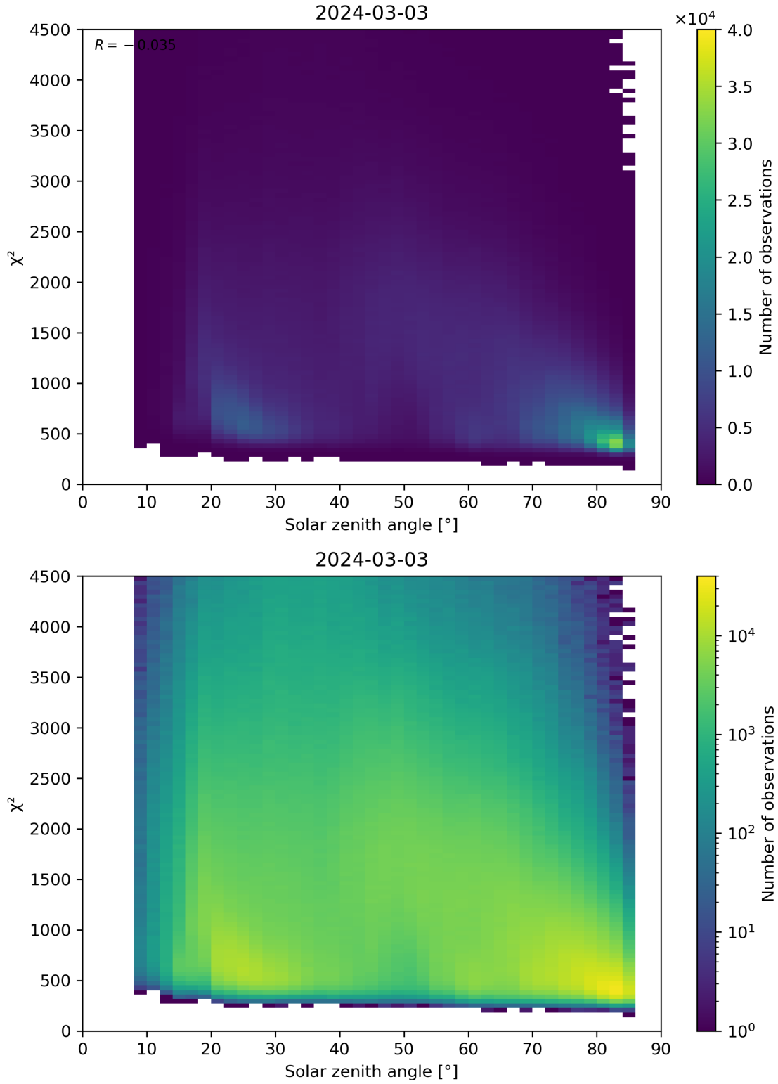
Figure 64: Scatter density plot of “Solar zenith angle” against “ \chi^2 ” for 2024-03-02 to 2024-03-04.
