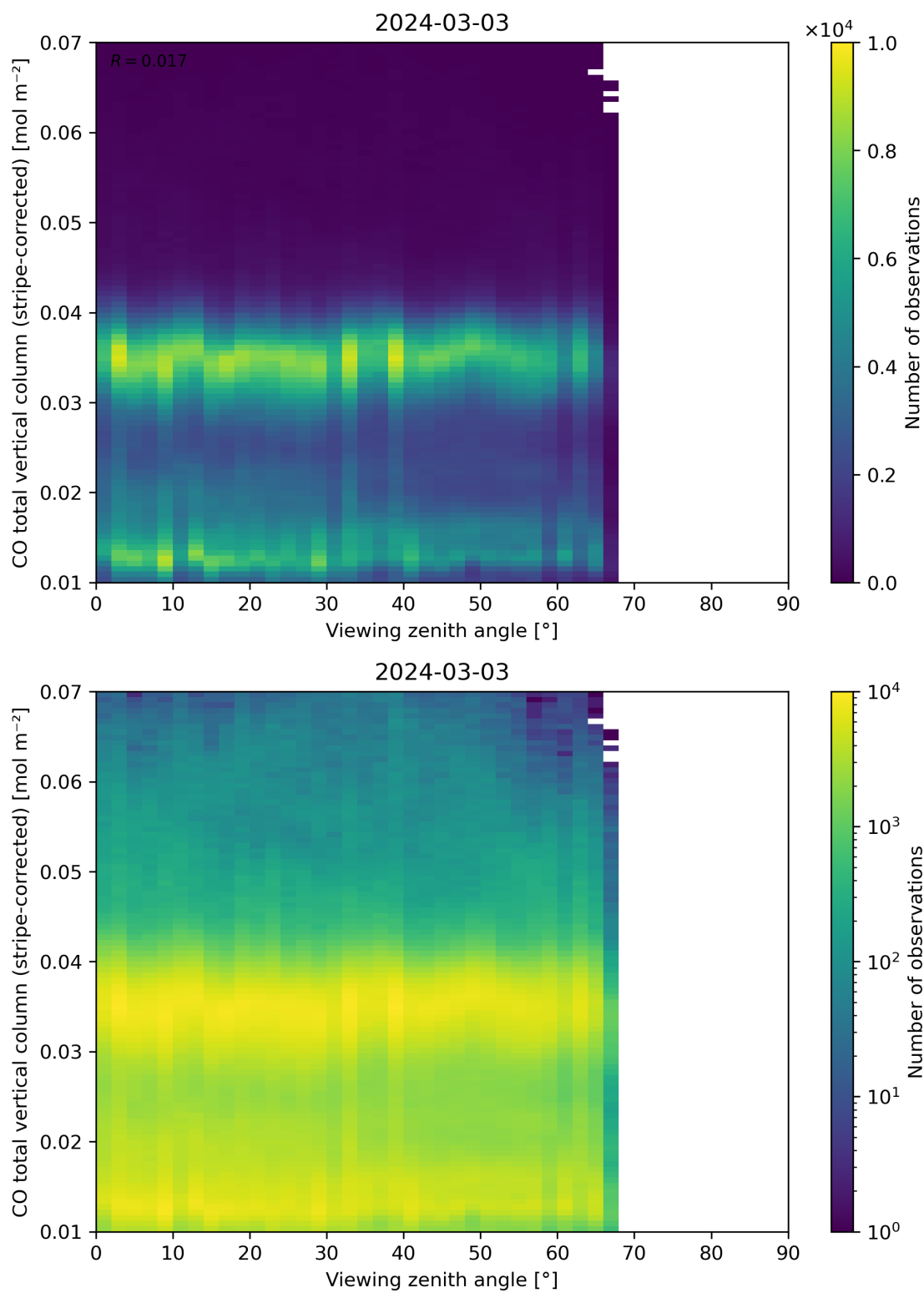
Figure 70: Scatter density plot of “Viewing zenith angle” against “CO total vertical column (stripe-corrected)” for 2024-03-02 to 2024-03-04.
