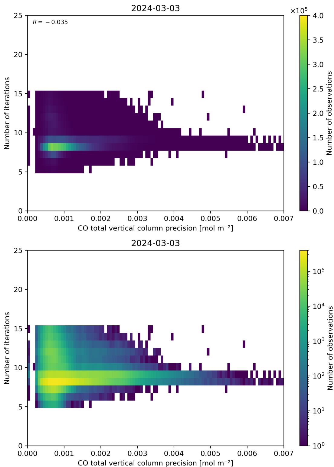
Figure 46: Scatter density plot of “CO total vertical column precision” against “Number of iterations” for 2024-03-02 to 2024-03-04.
