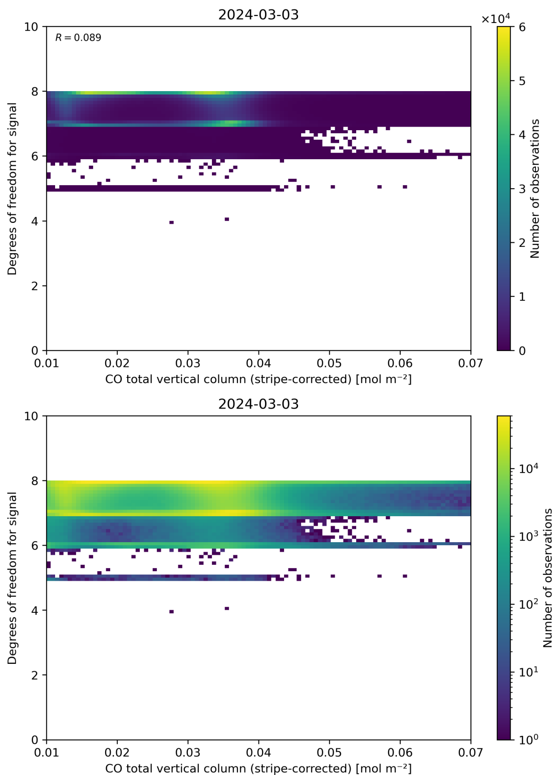
Figure 38: Scatter density plot of “CO total vertical column (stripe-corrected)” against “Degrees of freedom for signal” for 2024-03-02 to 2024-03-04.
