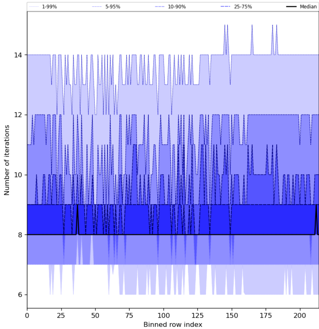
Figure 32: Along track statistics of “Number of iterations” for 2024-03-02 to 2024-03-04
