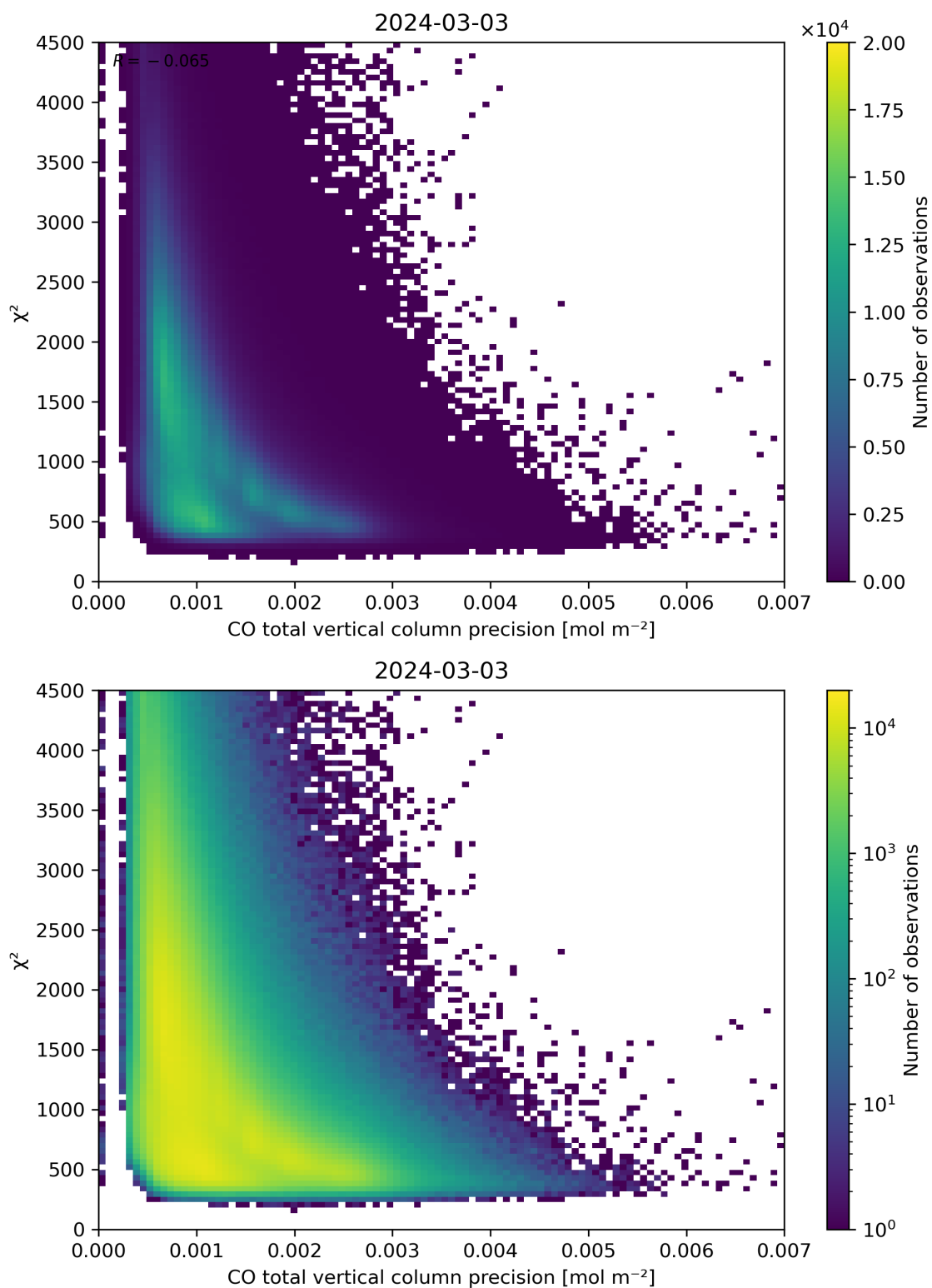
Figure 44: Scatter density plot of “CO total vertical column precision” against “ \chi^2 ” for 2024-03-02 to 2024-03-04.
