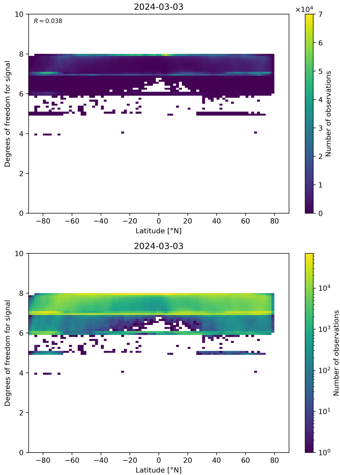
Figure 55: Scatter density plot of “Latitude” against “Degrees of freedom for signal” for 2024-03-02 to 2024-03-04.
