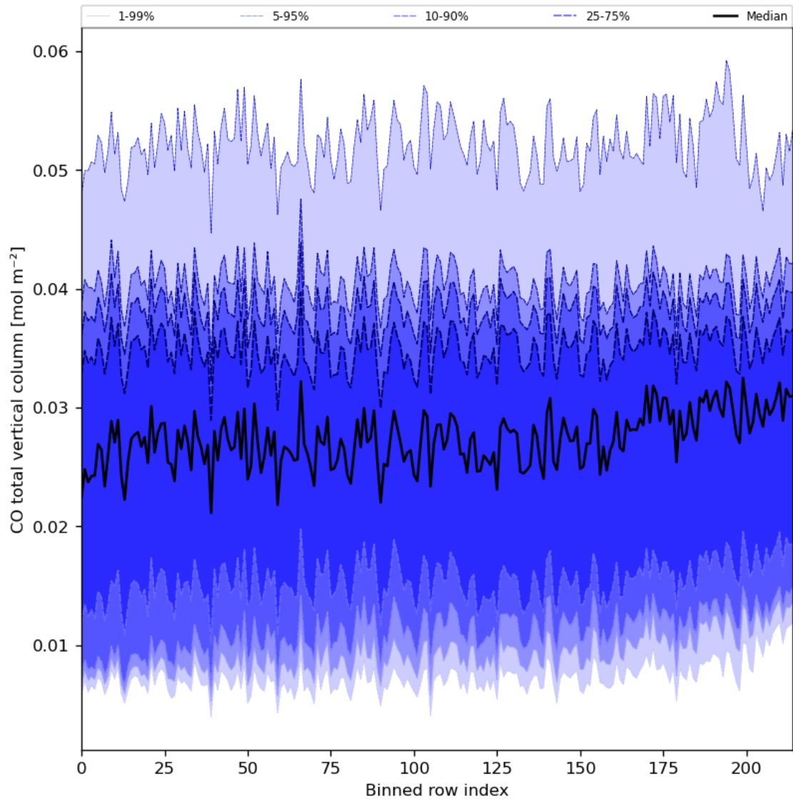
Figure 26: Along track statistics of “CO total vertical column” for 2024-03-02 to 2024-03-04
