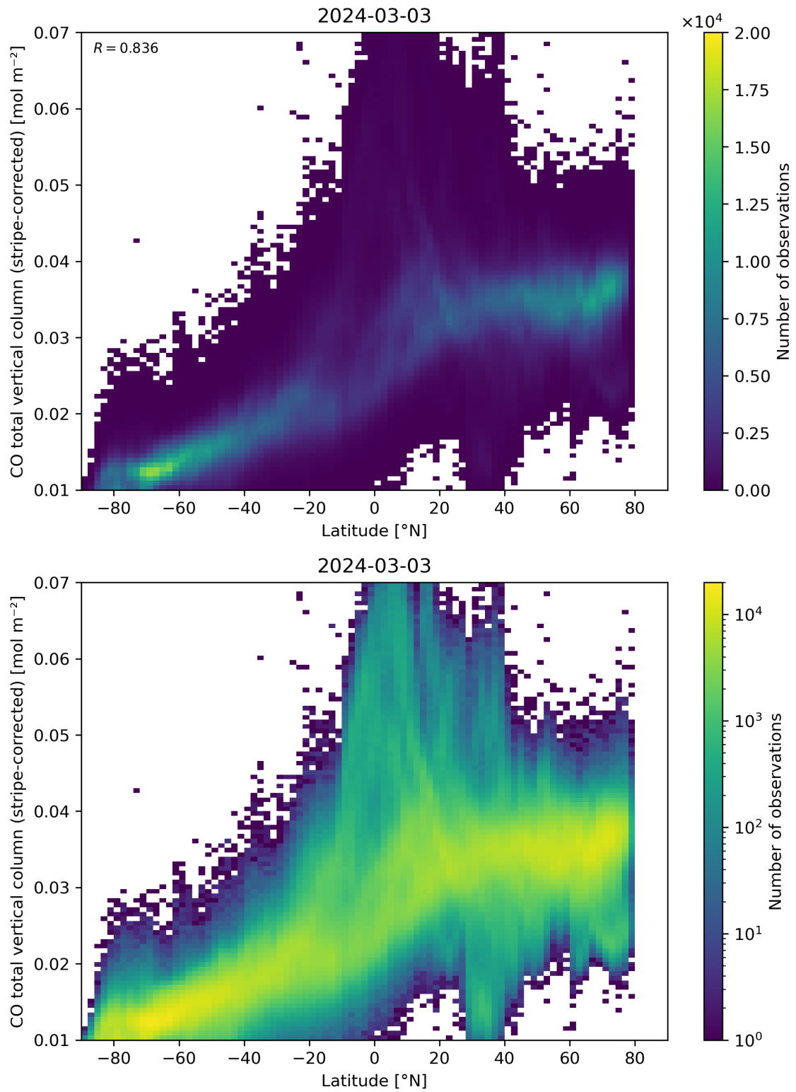
Figure 52: Scatter density plot of “Latitude” against “CO total vertical column (stripe-corrected)” for 2024-03-02 to 2024-03-04.
