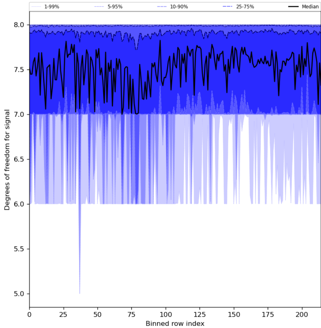
Figure 31: Along track statistics of “Degrees of freedom for signal” for 2024-03-02 to 2024-03-04
