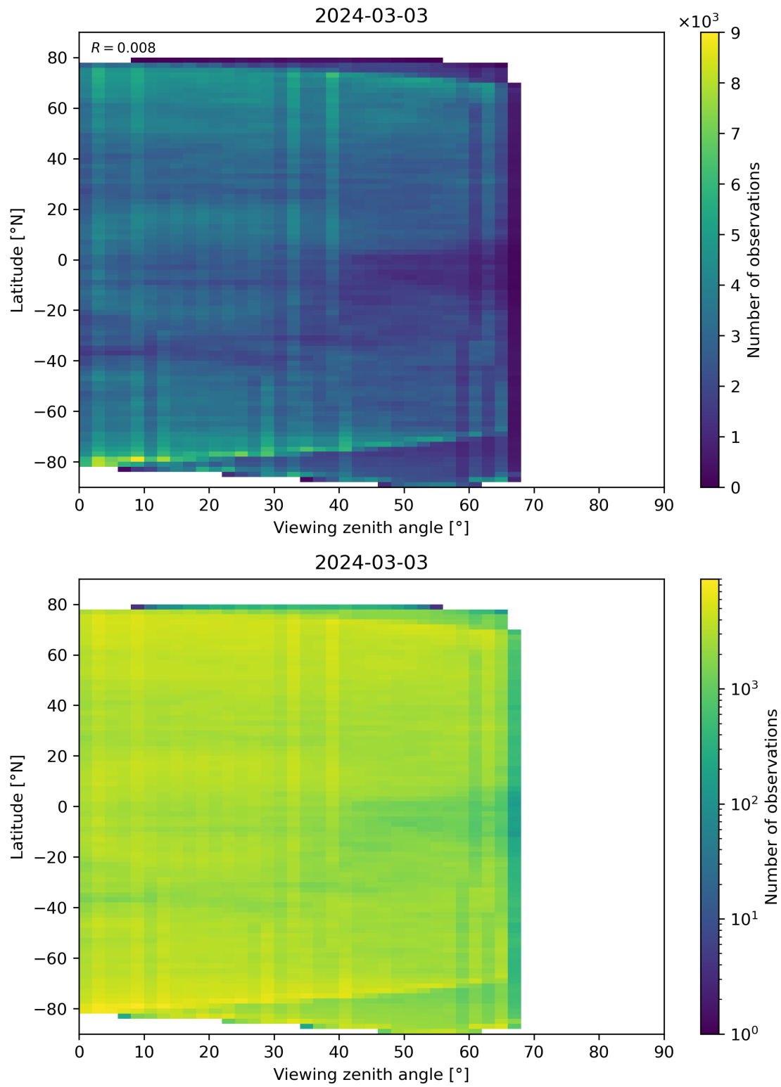
Figure 74: Scatter density plot of “Viewing zenith angle” against “Latitude” for 2024-03-02 to 2024-03-04.
