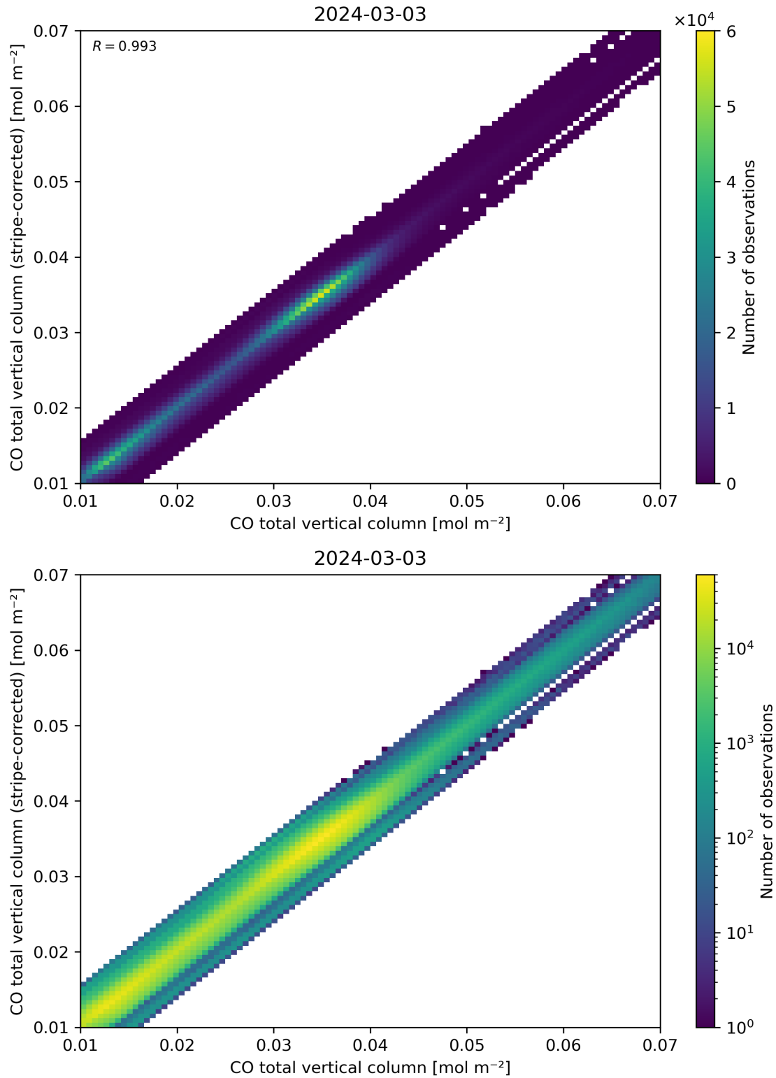
Figure 33: Scatter density plot of “CO total vertical column” against “CO total vertical column (stripe-corrected)” for 2024-03-02 to 2024-03-04.
