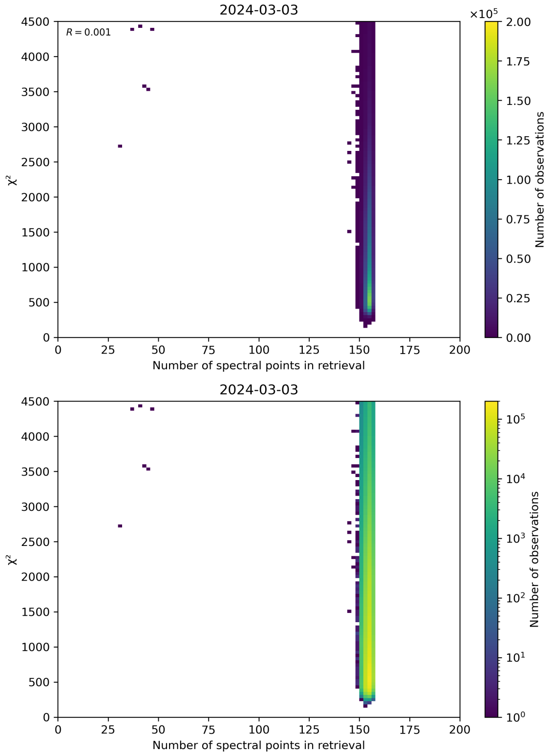
Figure 58: Scatter density plot of “Number of spectral points in retrieval” against “ \chi^2 ” for 2024-03-02 to 2024-03-04.
