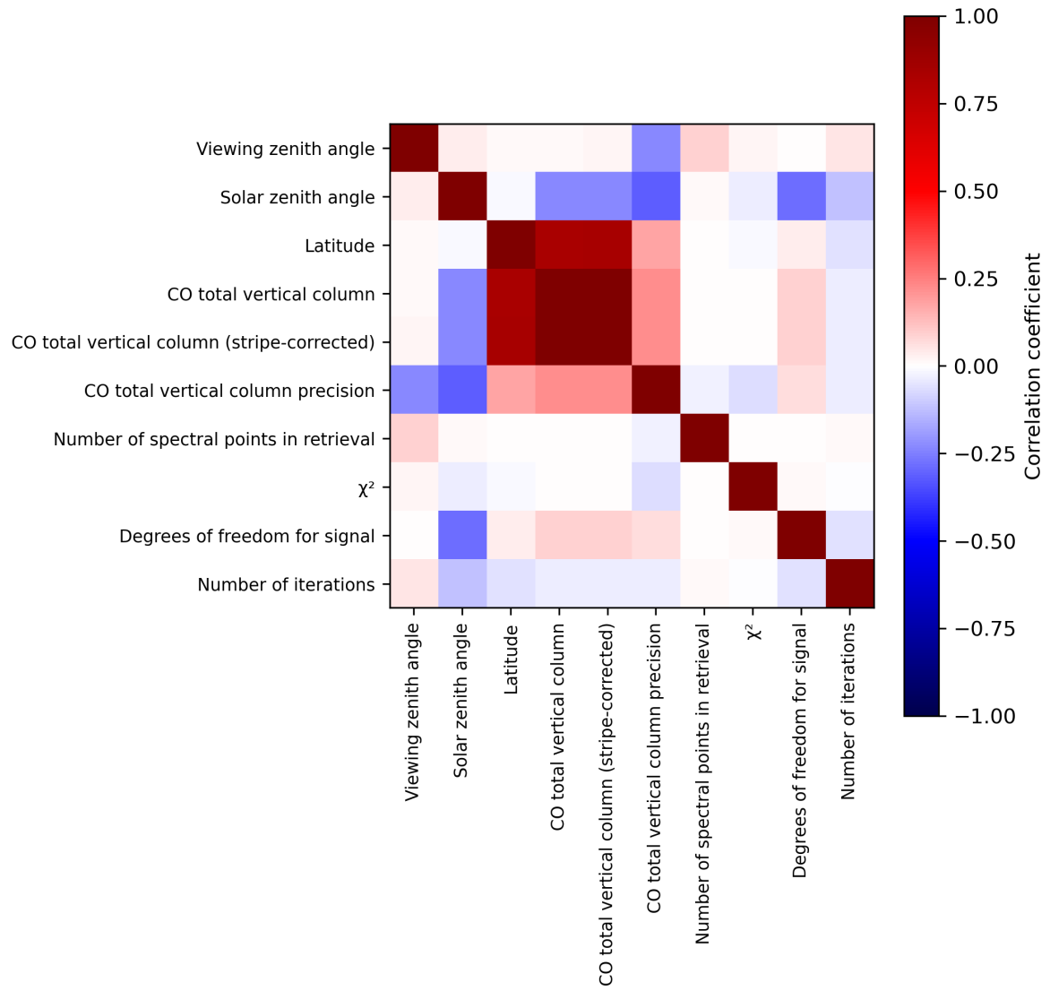
Figure 2: Map of correlation matrix for 2024-03-02 to 2024-03-04.
