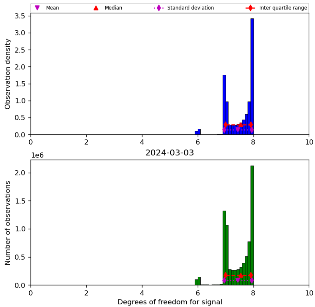
Figure 23: Histogram of “Degrees of freedom for signal” for 2024-03-02 to 2024-03-04
