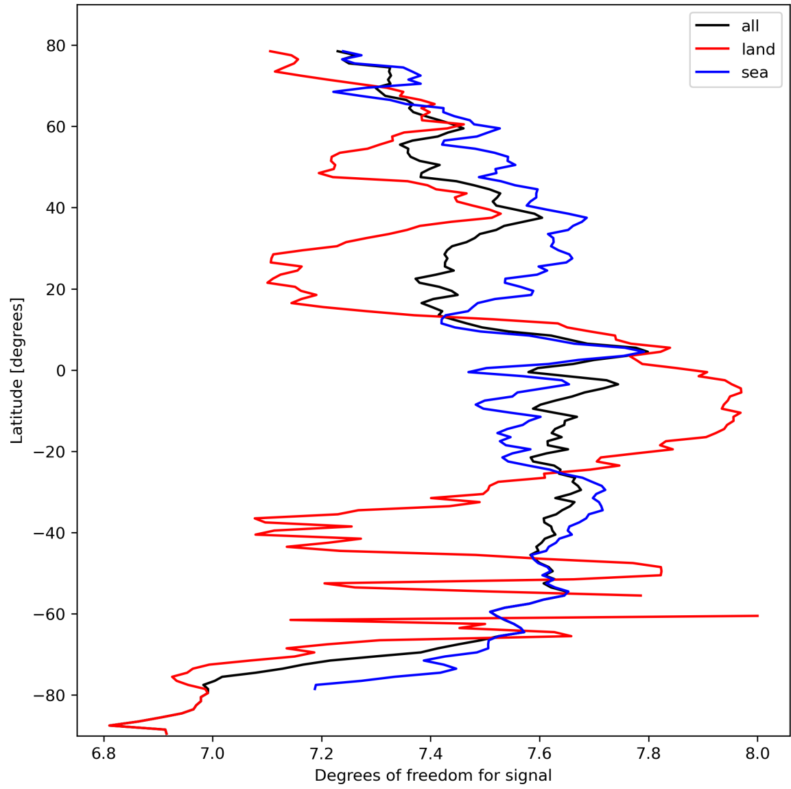
Figure 15: Zonal average of “Degrees of freedom for signal” for 2024-03-02 to 2024-03-04.
