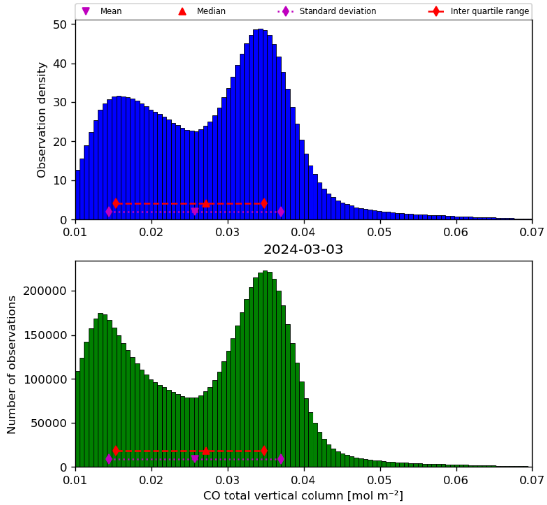
Figure 18: Histogram of “CO total vertical column” for 2024-03-02 to 2024-03-04
