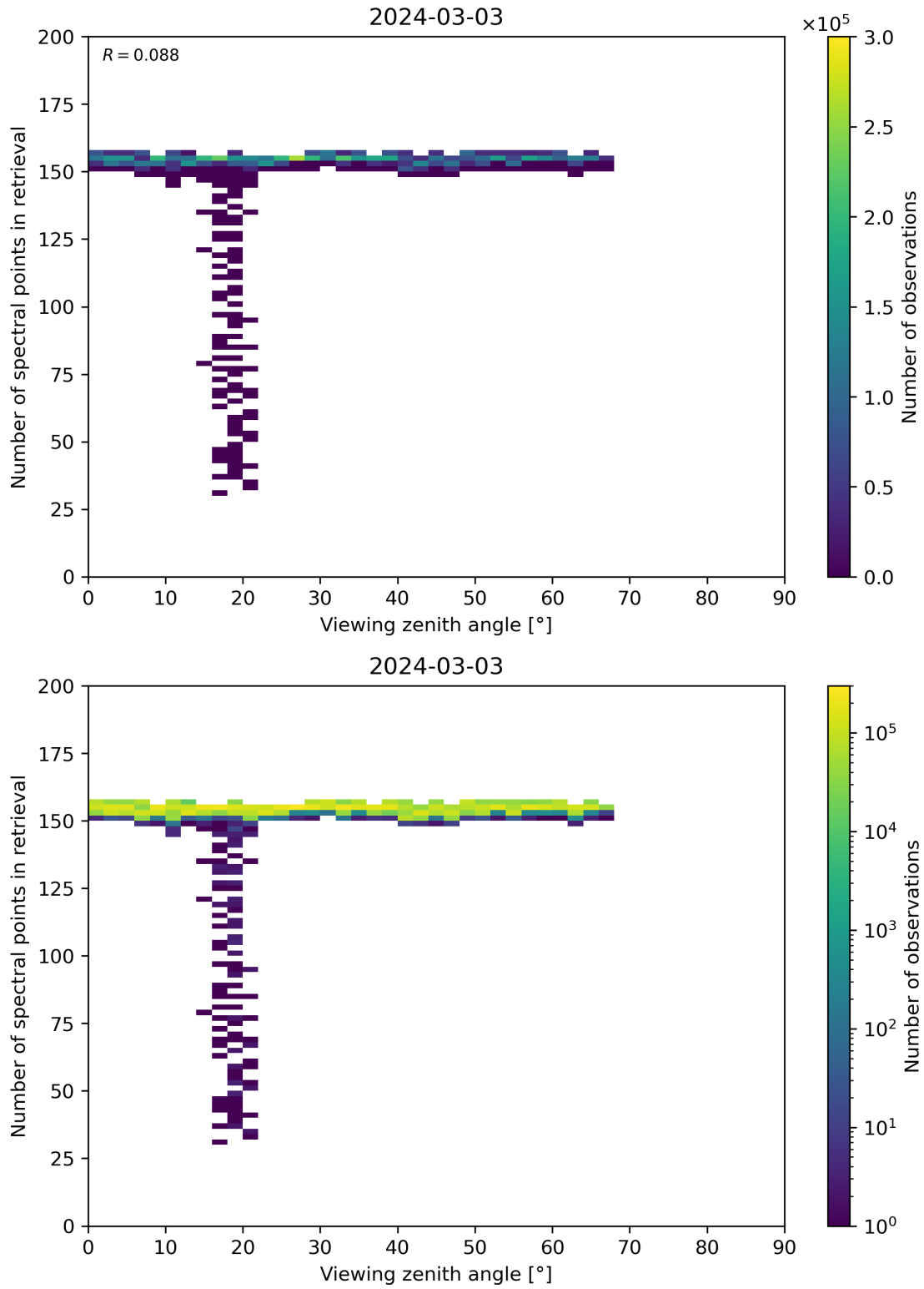
Figure 76: Scatter density plot of “Viewing zenith angle” against “Number of spectral points in retrieval” for 2024-03-02 to 2024-03-04.
