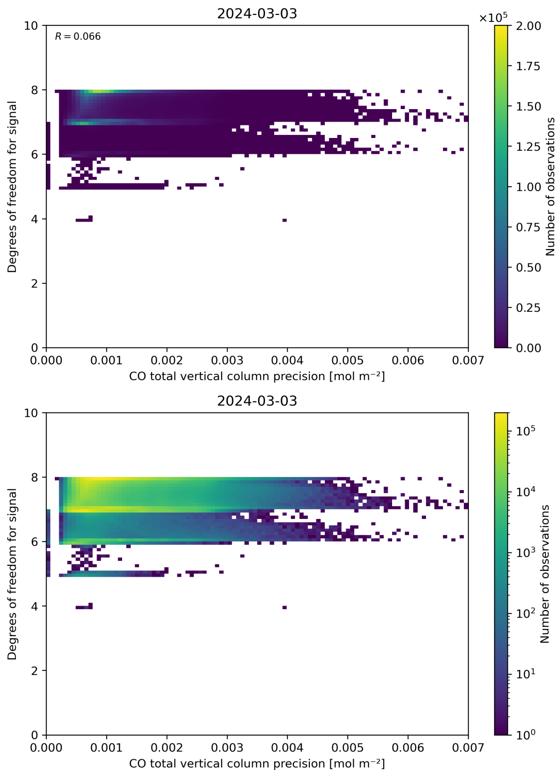
Figure 45: Scatter density plot of “CO total vertical column precision” against “Degrees of freedom for signal” for 2024-03-02 to 2024-03-04.
