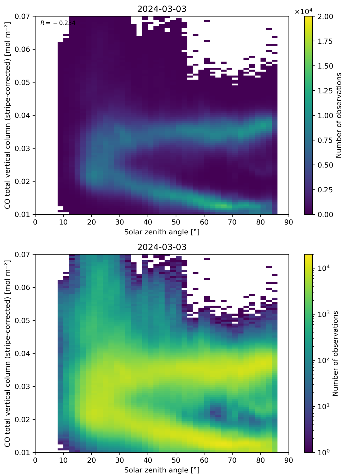
Figure 62: Scatter density plot of “Solar zenith angle” against “CO total vertical column (stripe-corrected)” for 2024-03-02 to 2024-03-04.
