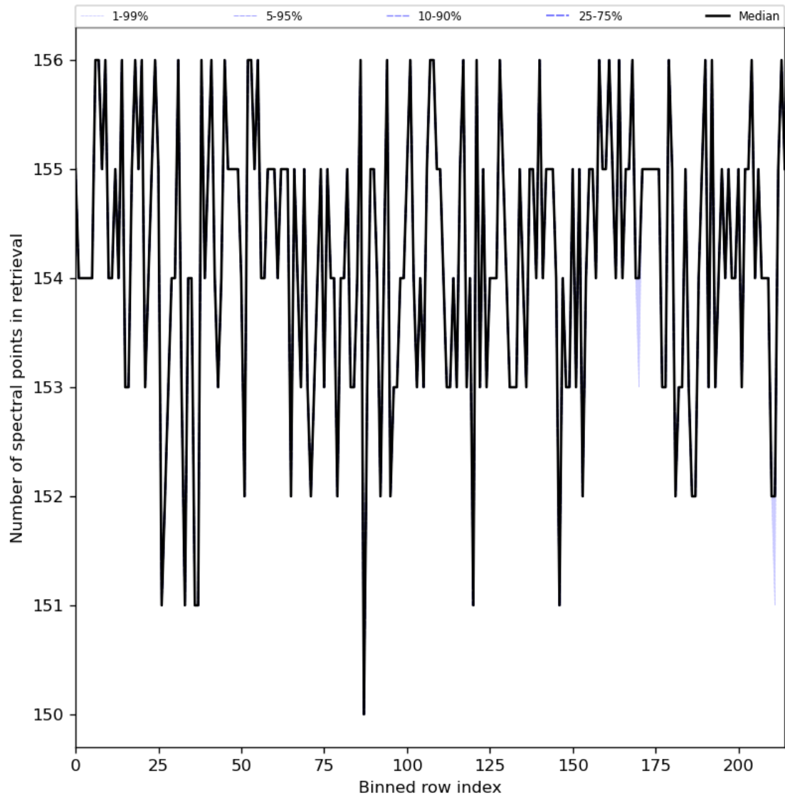
Figure 29: Along track statistics of “Number of spectral points in retrieval” for 2024-03-02 to 2024-03-04
