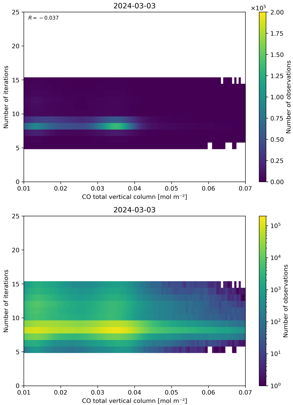
Figure 42: Scatter density plot of “CO total vertical column” against “Number of iterations” for 2024-03-02 to 2024-03-04.
