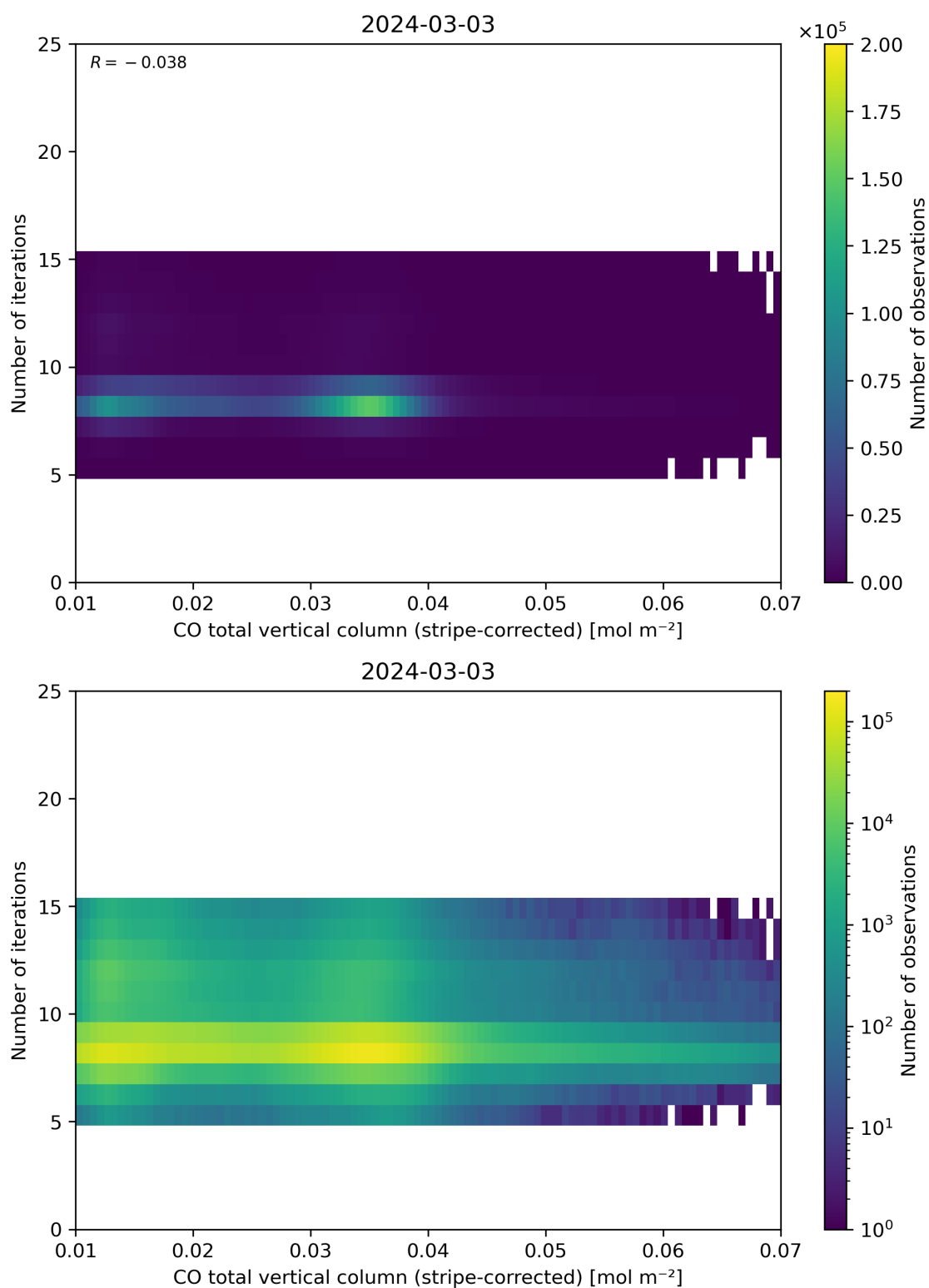
Figure 39: Scatter density plot of “CO total vertical column (stripe-corrected)” against “Number of iterations” for 2024-03-02 to 2024-03-04.
