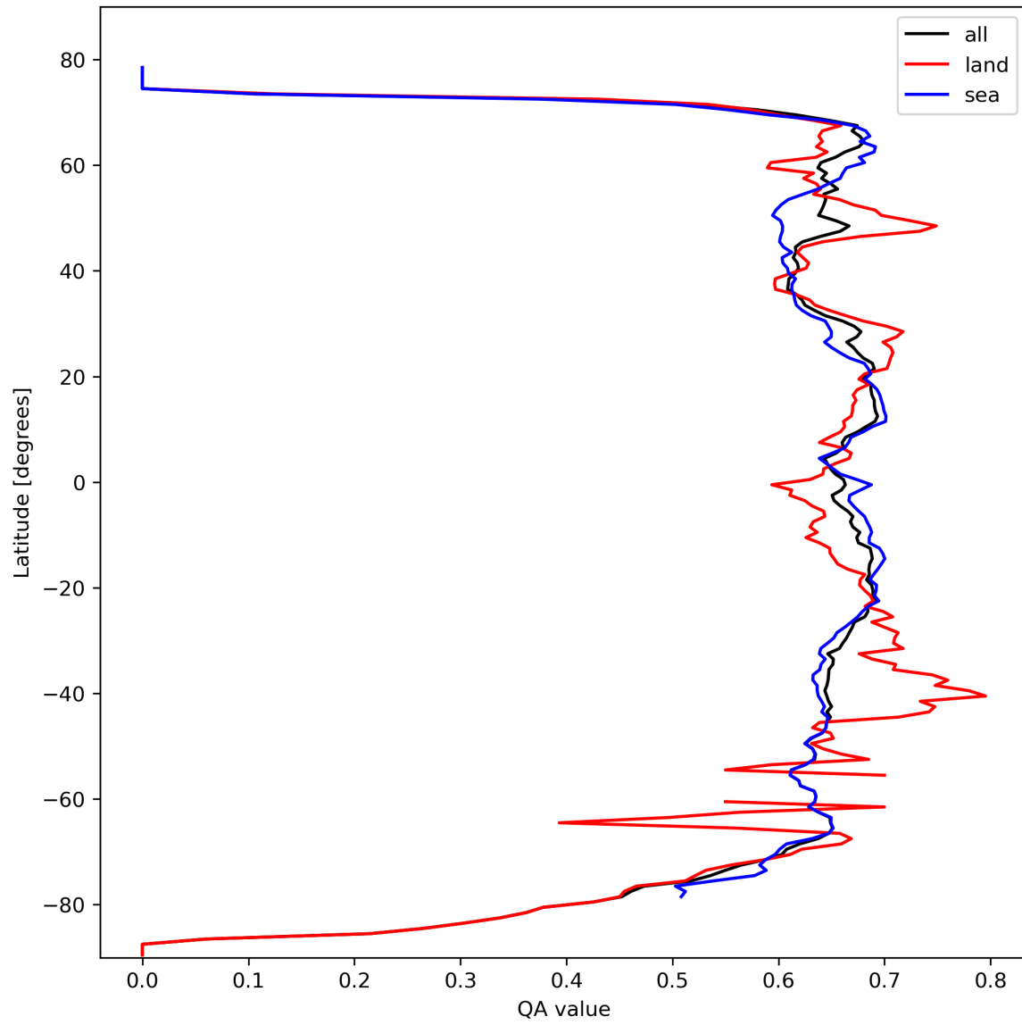
Figure 9: Zonal average of “QA value” for 2024-03-02 to 2024-03-04.
