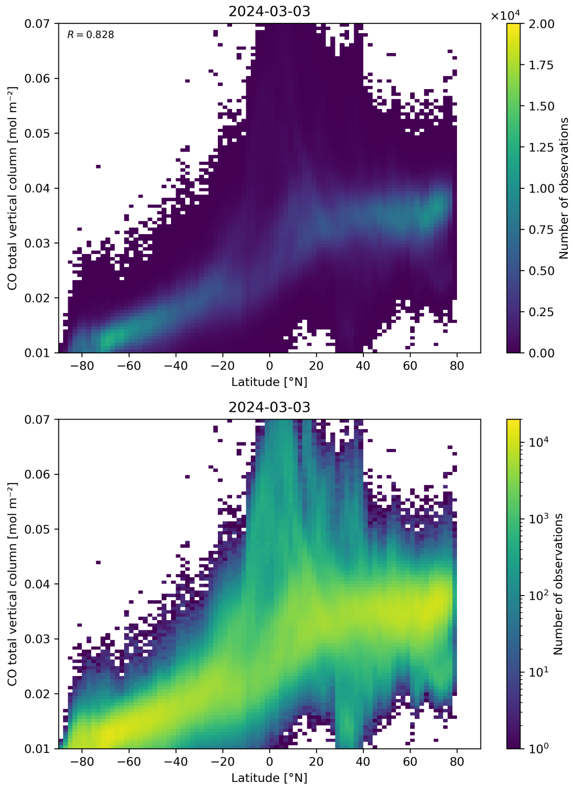
Figure 51: Scatter density plot of “Latitude” against “CO total vertical column” for 2024-03-02 to 2024-03-04.
