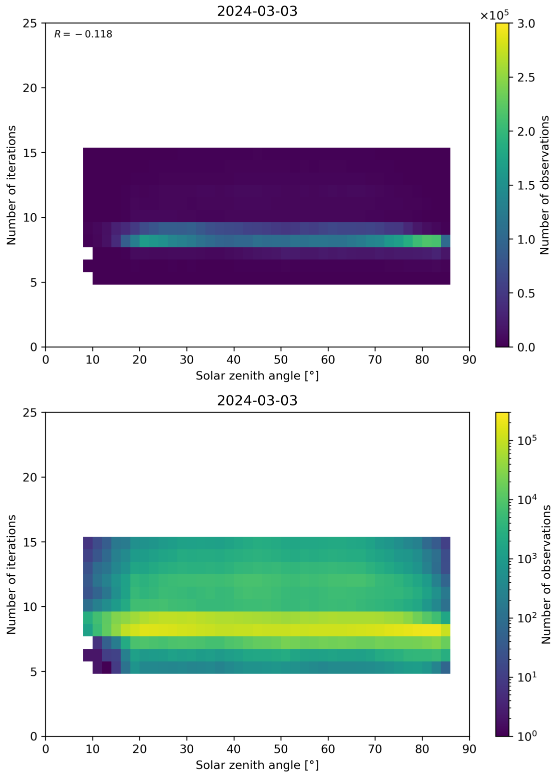
Figure 67: Scatter density plot of “Solar zenith angle” against “Number of iterations” for 2024-03-02 to 2024-03-04.
