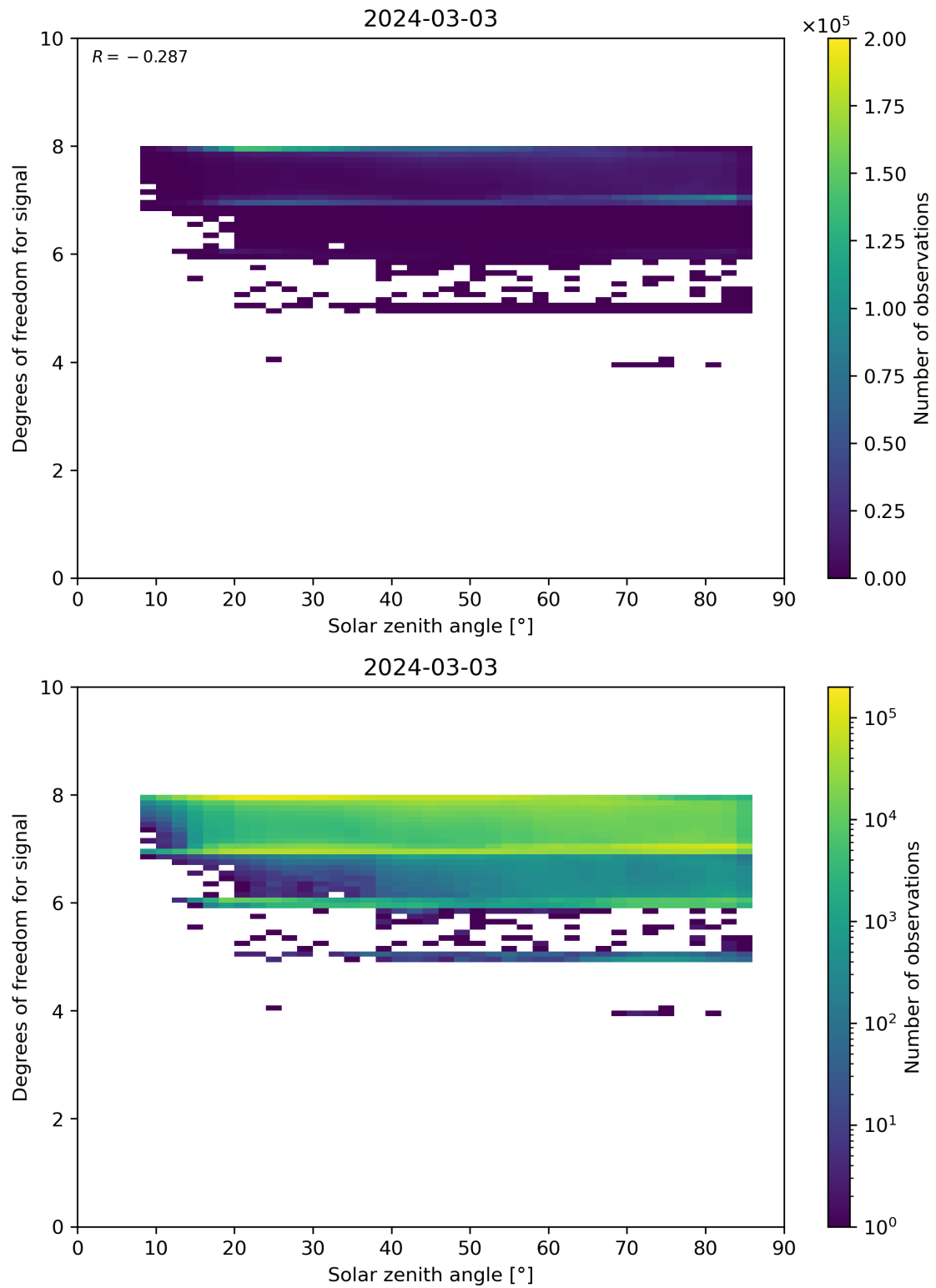
Figure 65: Scatter density plot of “Solar zenith angle” against “Degrees of freedom for signal” for 2024-03-02 to 2024-03-04.
