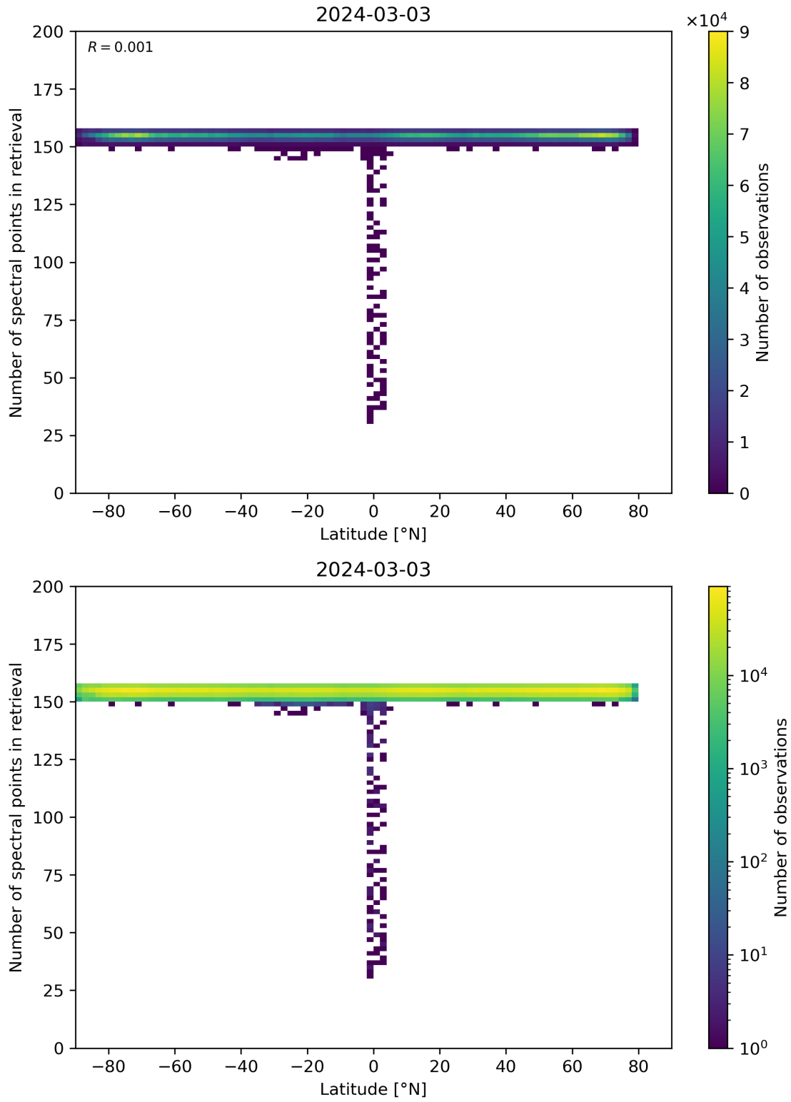
Figure 57: Scatter density plot of “Latitude” against “Number of spectral points in retrieval” for 2024-03-02 to 2024-03-04.
