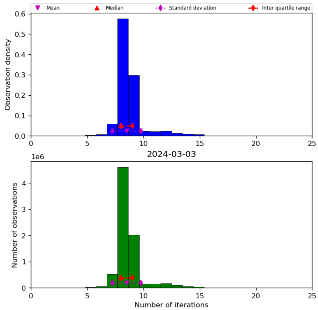
Figure 24: Histogram of “Number of iterations” for 2024-03-02 to 2024-03-04
