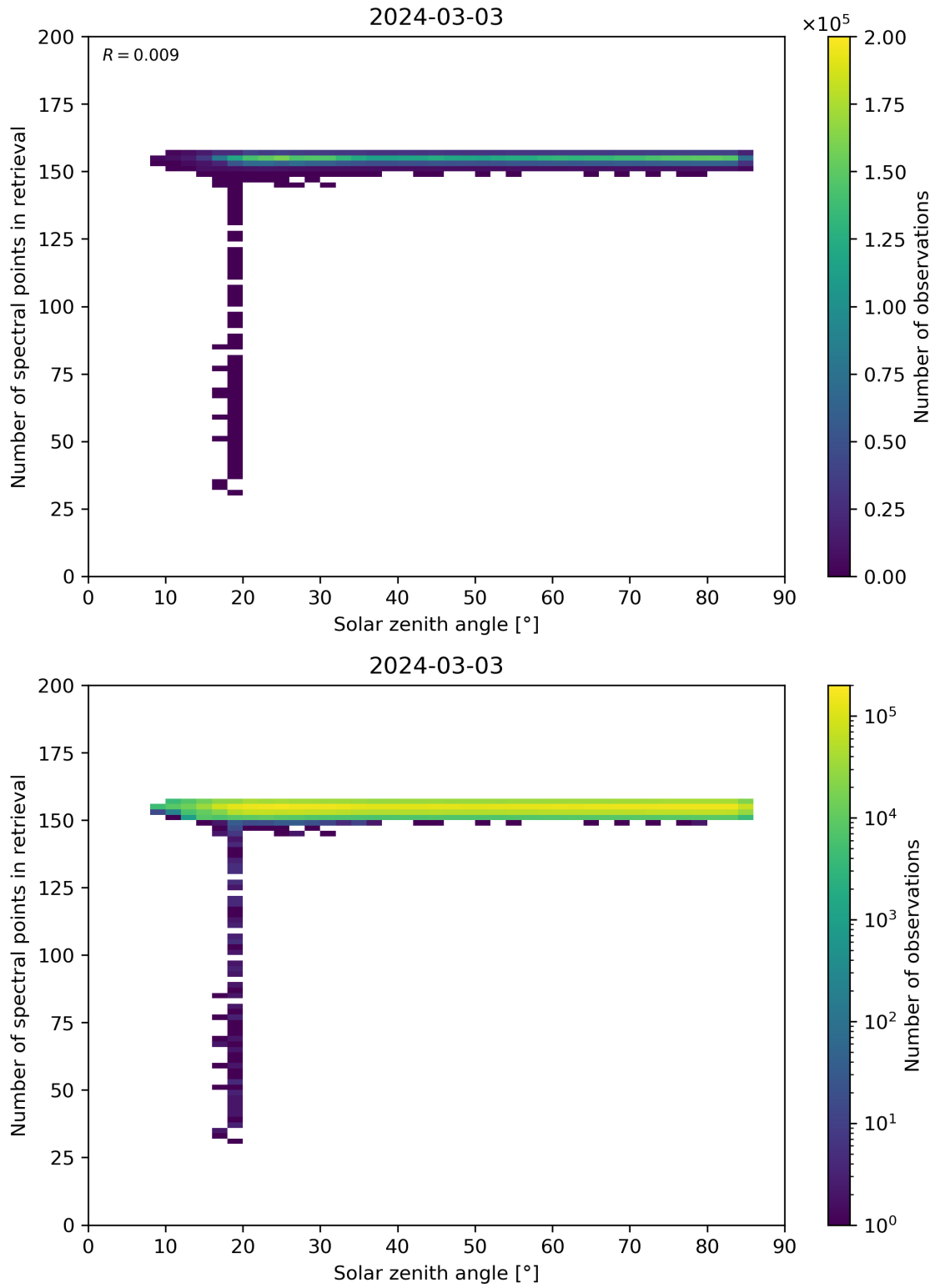
Figure 68: Scatter density plot of “Solar zenith angle” against “Number of spectral points in retrieval” for 2024-03-02 to 2024-03-04.
