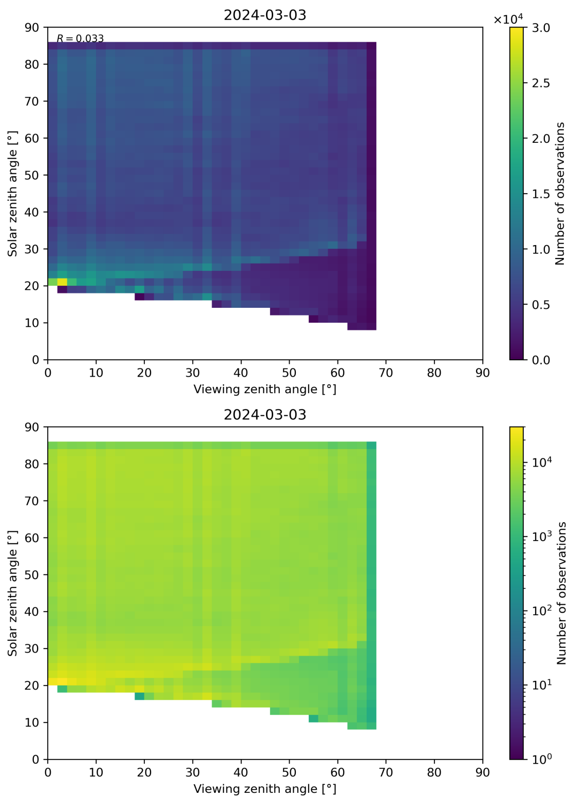
Figure 77: Scatter density plot of “Viewing zenith angle” against “Solar zenith angle” for 2024-03-02 to 2024-03-04.
