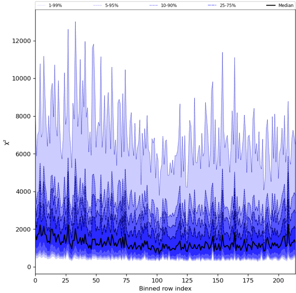
Figure 30: Along track statistics of “ \chi^2 ” for 2024-03-02 to 2024-03-04
