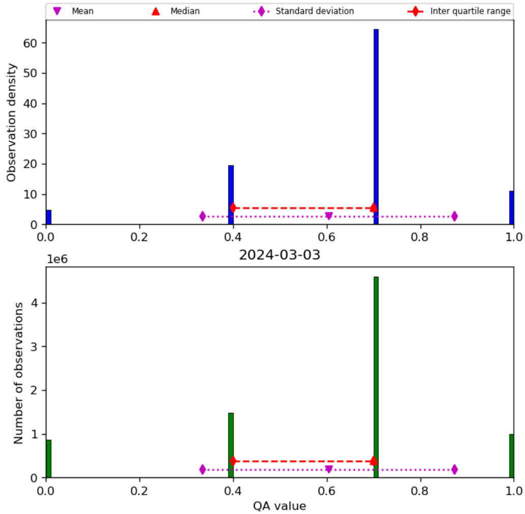
Figure 17: Histogram of “QA value” for 2024-03-02 to 2024-03-04
