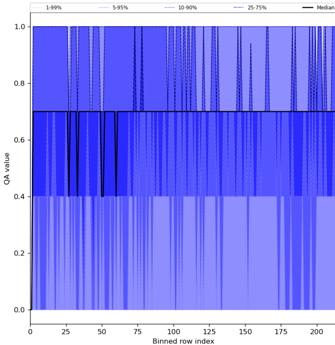
Figure 25: Along track statistics of “QA value” for 2024-03-02 to 2024-03-04
