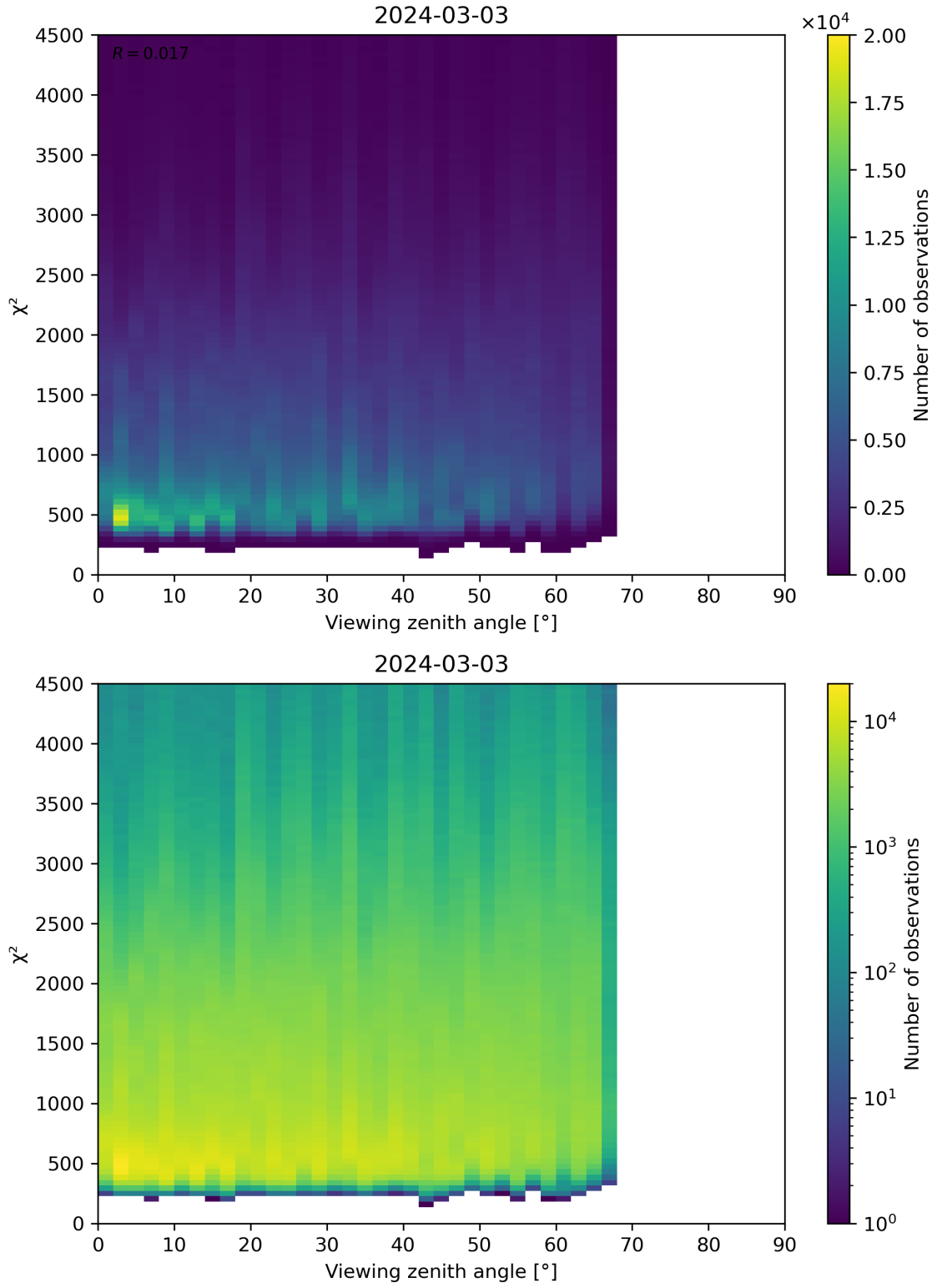
Figure 72: Scatter density plot of “Viewing zenith angle” against “ \chi^2 ” for 2024-03-02 to 2024-03-04.
