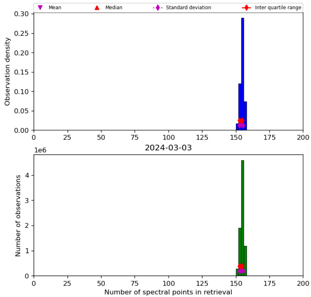
Figure 21: Histogram of “Number of spectral points in retrieval” for 2024-03-02 to 2024-03-04
