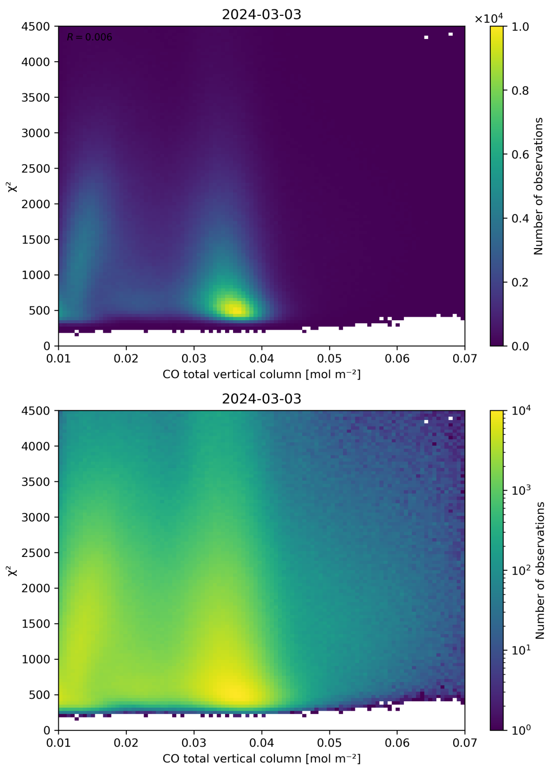
Figure 35: Scatter density plot of “CO total vertical column” against “ \chi^2 ” for 2024-03-02 to 2024-03-04.
