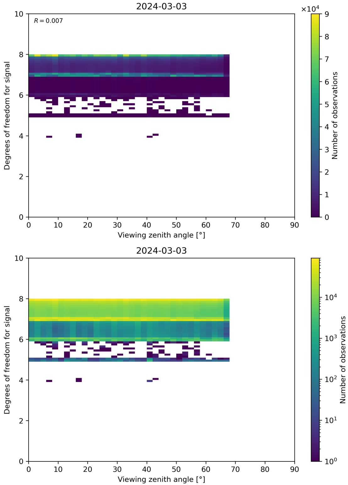
Figure 73: Scatter density plot of “Viewing zenith angle” against “Degrees of freedom for signal” for 2024-03-02 to 2024-03-04.
