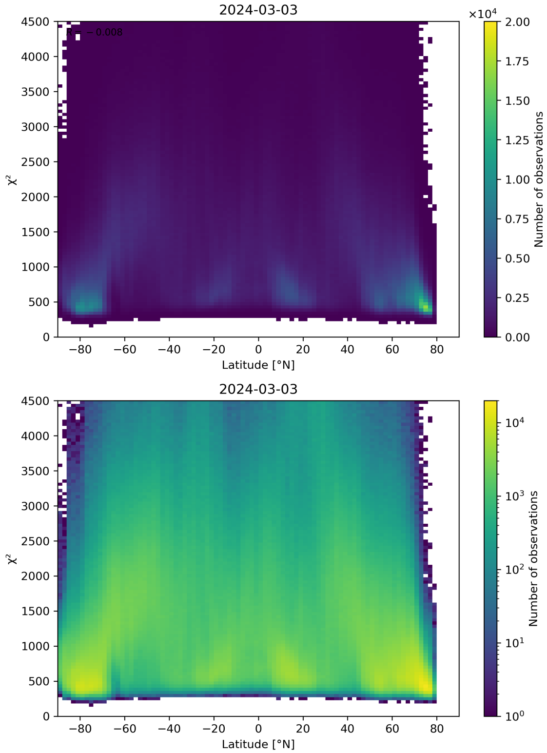
Figure 54: Scatter density plot of “Latitude” against “ \chi^2 ” for 2024-03-02 to 2024-03-04.
