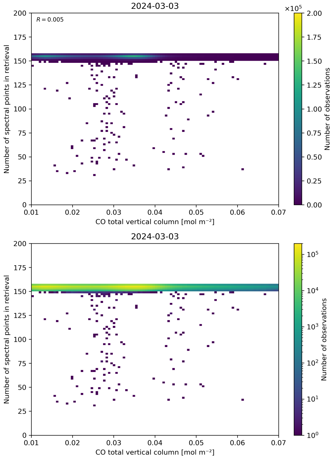
Figure 43: Scatter density plot of “CO total vertical column” against “Number of spectral points in retrieval” for 2024-03-02 to 2024-03-04.
