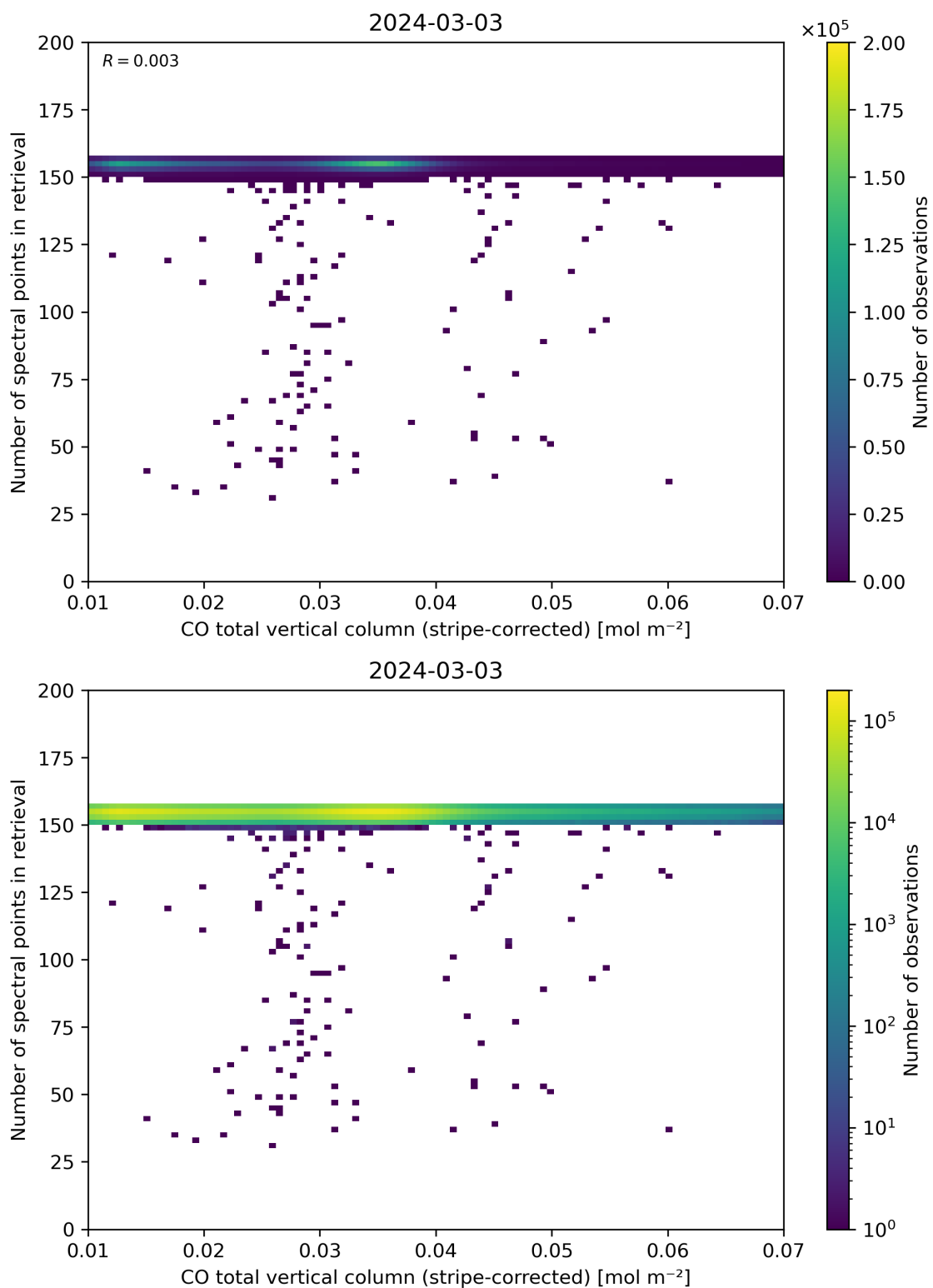
Figure 40: Scatter density plot of “CO total vertical column (stripe-corrected)” against “Number of spectral points in retrieval” for 2024-03-02 to 2024-03-04.
