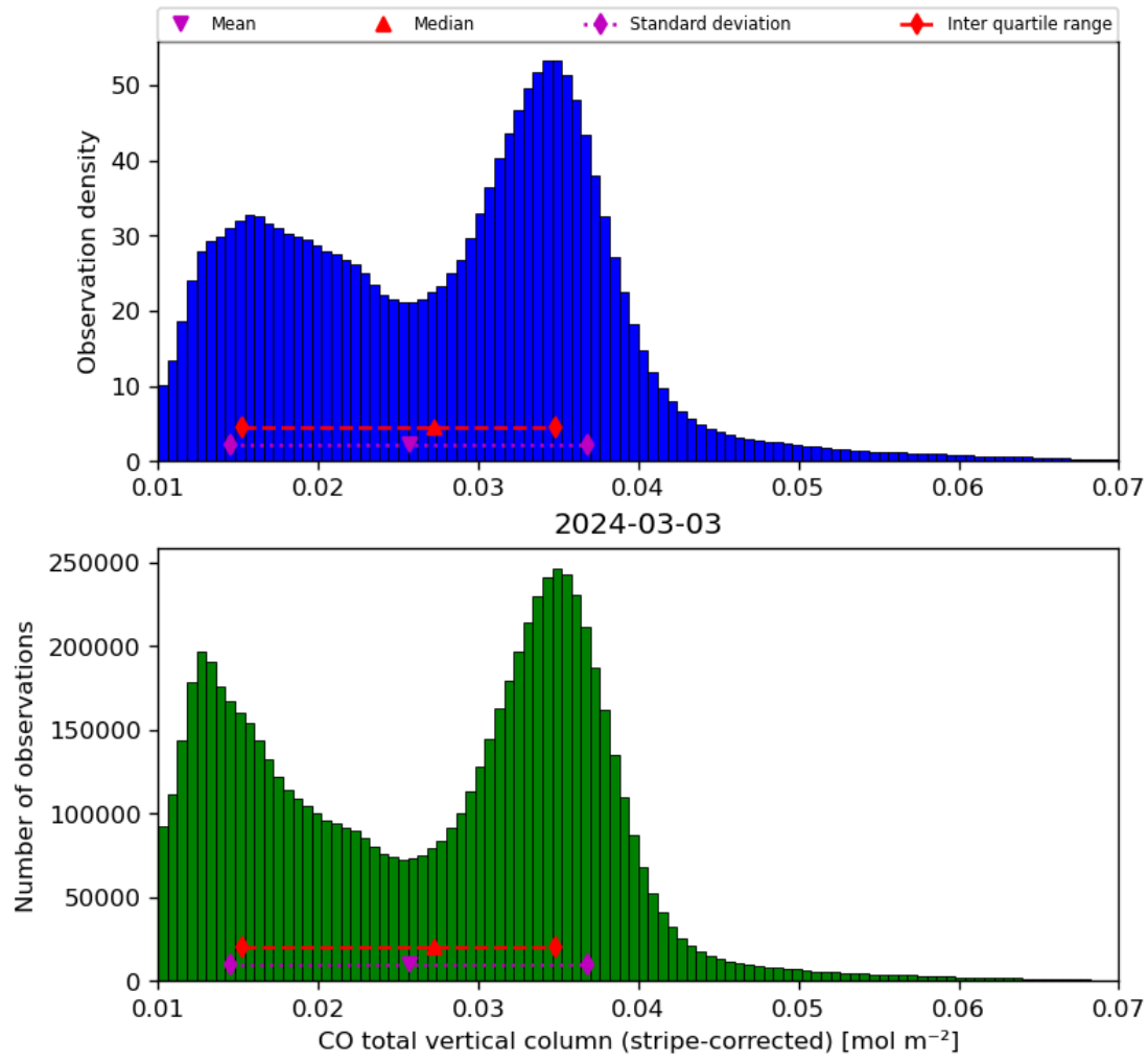
Figure 19: Histogram of “CO total vertical column (stripe-corrected)” for 2024-03-02 to 2024-03-04
