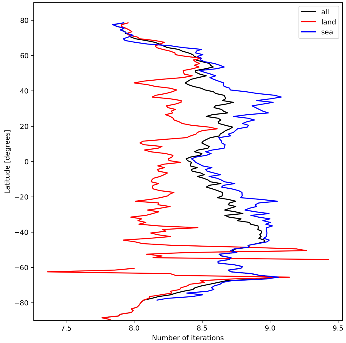
Figure 16: Zonal average of “Number of iterations” for 2024-03-02 to 2024-03-04.
