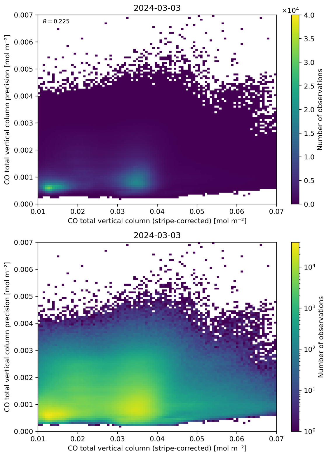
Figure 36: Scatter density plot of “CO total vertical column (stripe-corrected)” against “CO total vertical column precision” for 2024-03-02 to 2024-03-04.
