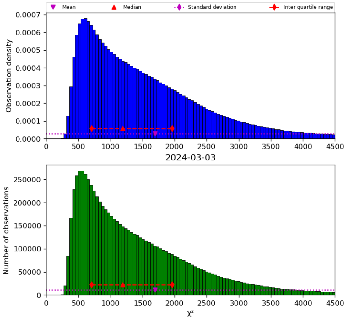
Figure 22: Histogram of “ \chi^2 ” for 2024-03-02 to 2024-03-04
