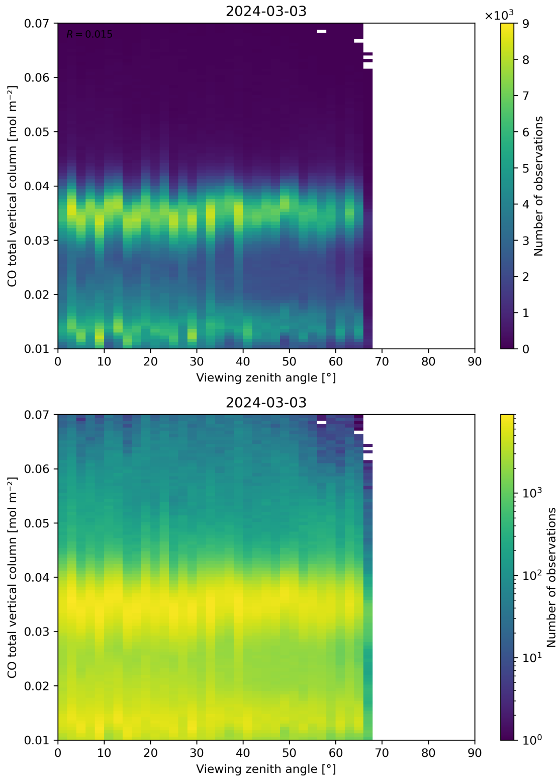
Figure 69: Scatter density plot of “Viewing zenith angle” against “CO total vertical column” for 2024-03-02 to 2024-03-04.
