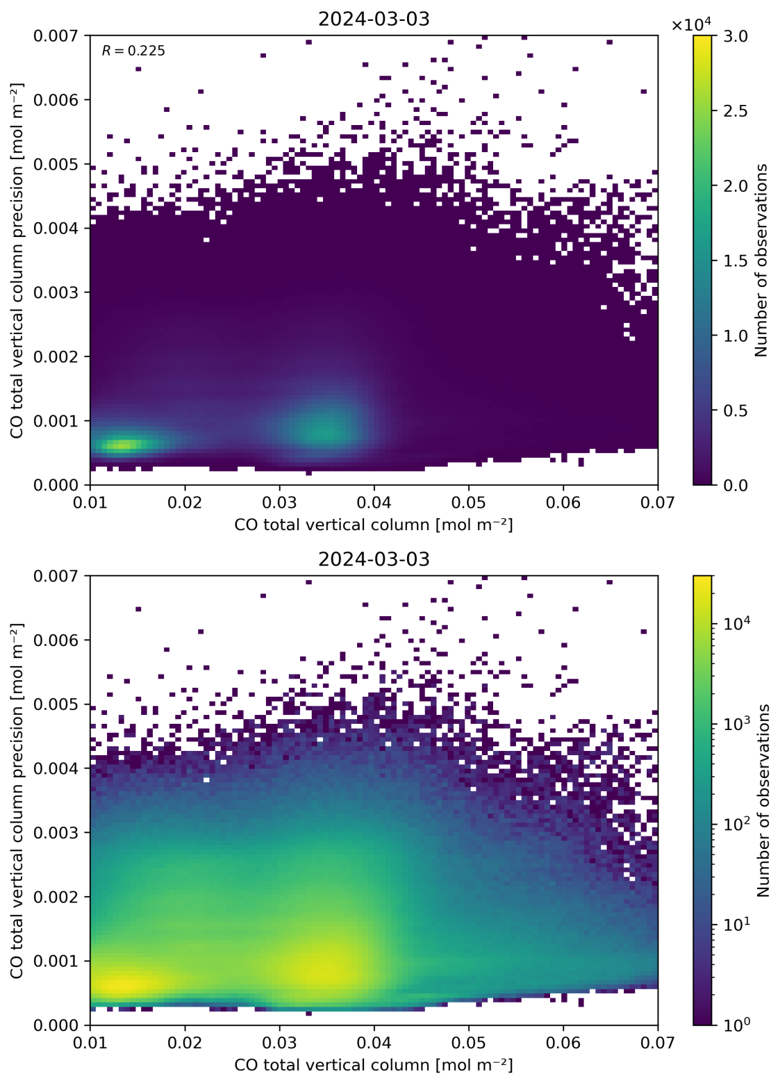
Figure 34: Scatter density plot of “CO total vertical column” against “CO total vertical column precision” for 2024-03-02 to 2024-03-04.
