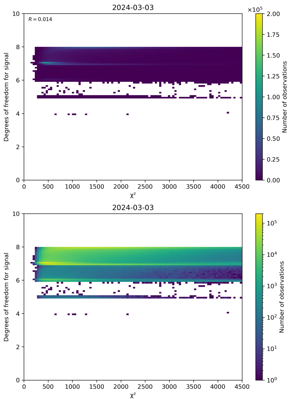
Figure 48: Scatter density plot of “ \chi^2 ” against “Degrees of freedom for signal” for 2024-03-02 to 2024-03-04.
