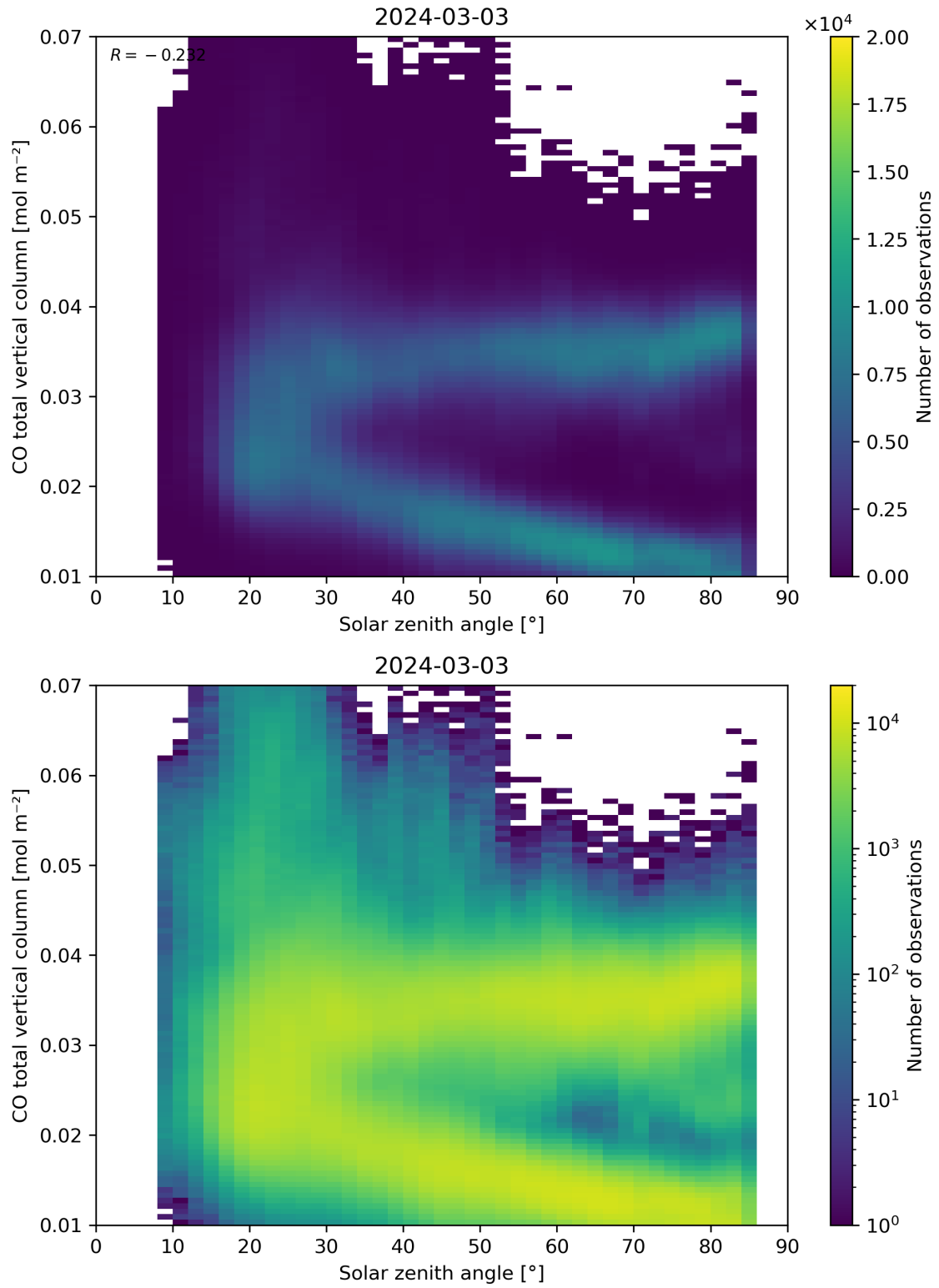
Figure 61: Scatter density plot of “Solar zenith angle” against “CO total vertical column” for 2024-03-02 to 2024-03-04.
