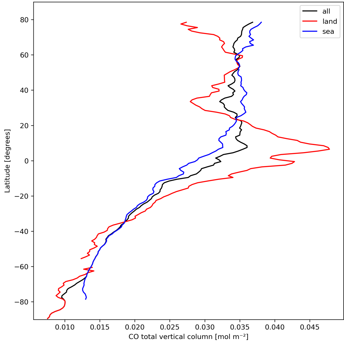
Figure 10: Zonal average of “CO total vertical column” for 2024-03-02 to 2024-03-04.
