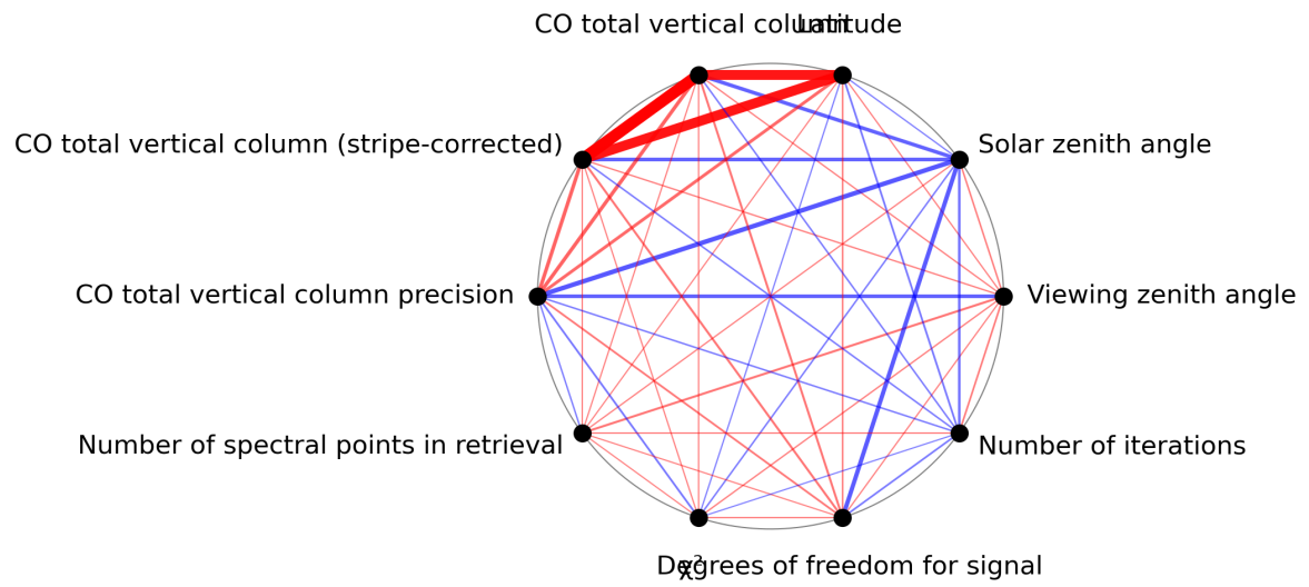
Figure 1: Map of correlation graph for 2024-03-02 to 2024-03-04.
