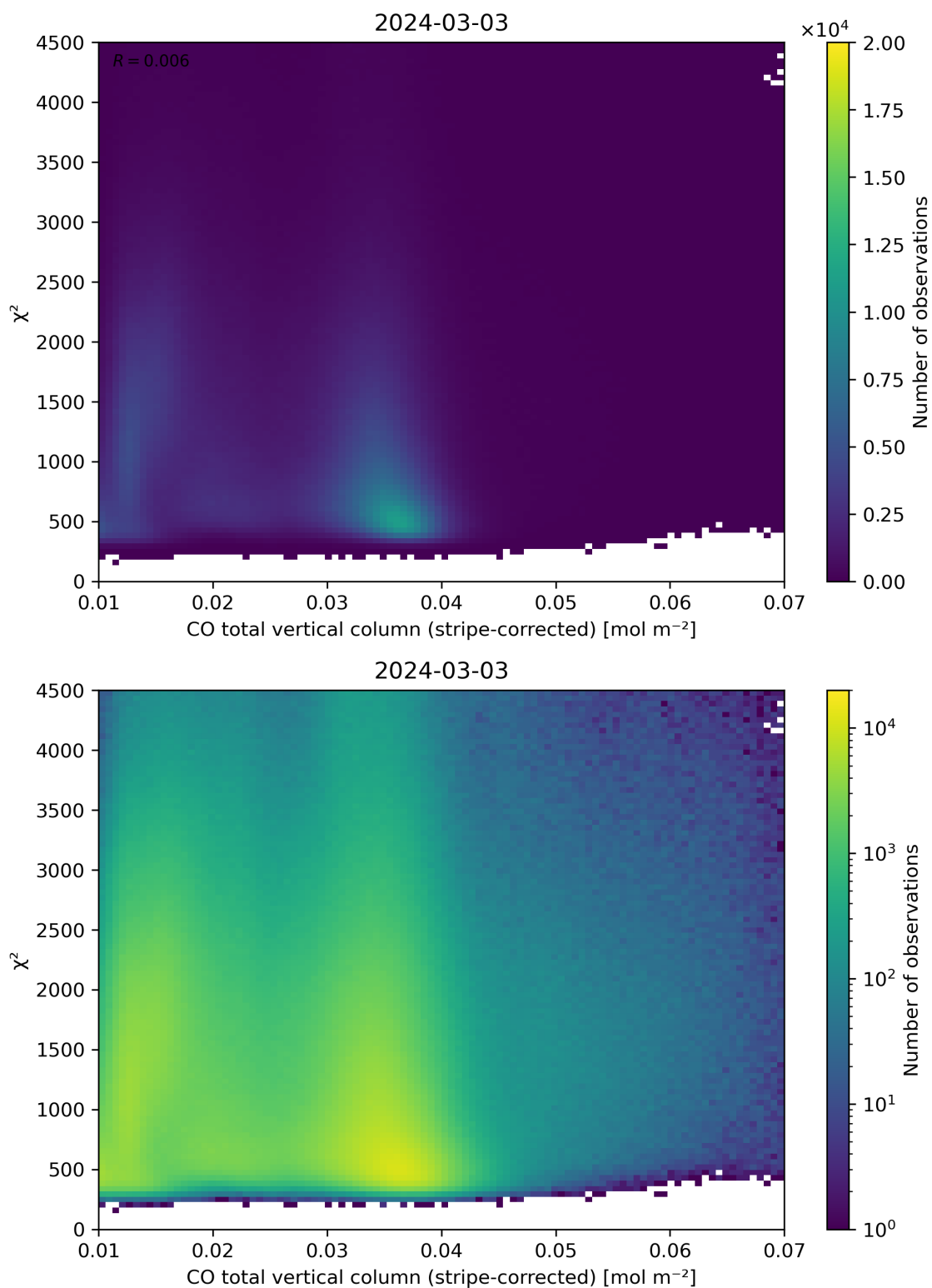
Figure 37: Scatter density plot of “CO total vertical column (stripe-corrected)” against “ \chi^2 ” for 2024-03-02 to 2024-03-04.
