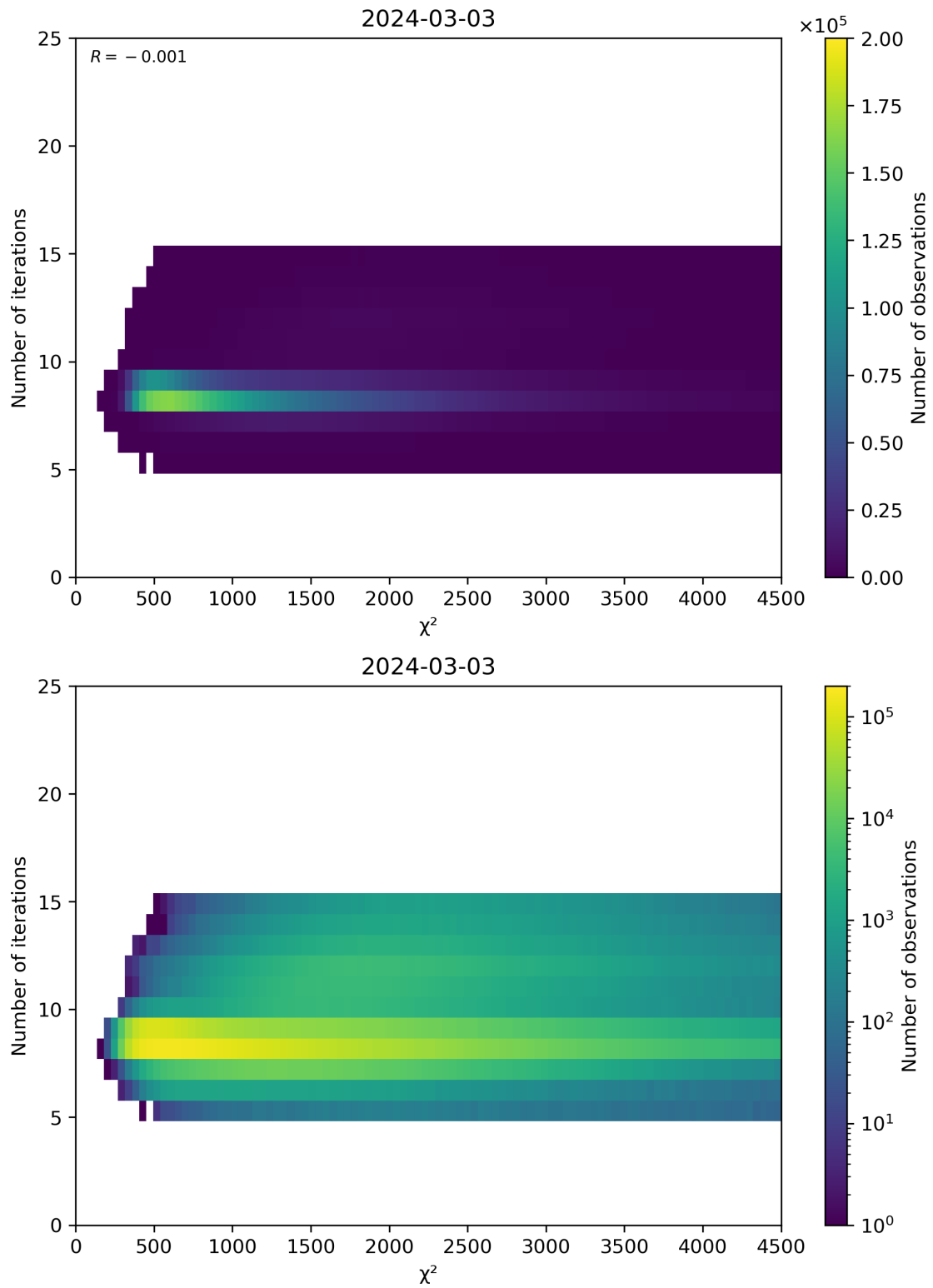
Figure 49: Scatter density plot of “ \chi^2 ” against “Number of iterations” for 2024-03-02 to 2024-03-04.
