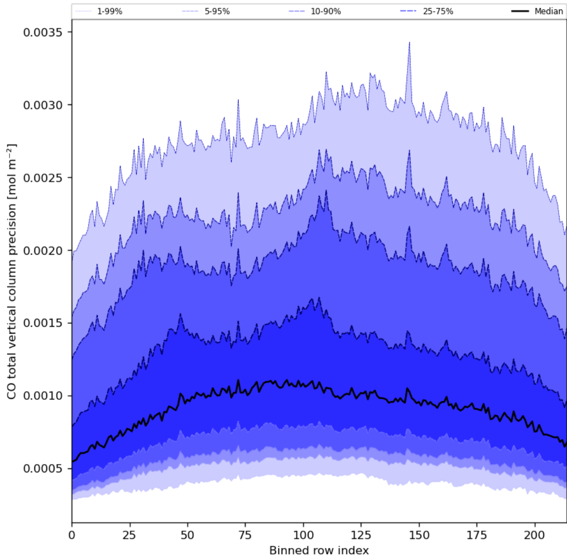
Figure 28: Along track statistics of “CO total vertical column precision” for 2024-03-02 to 2024-03-04
