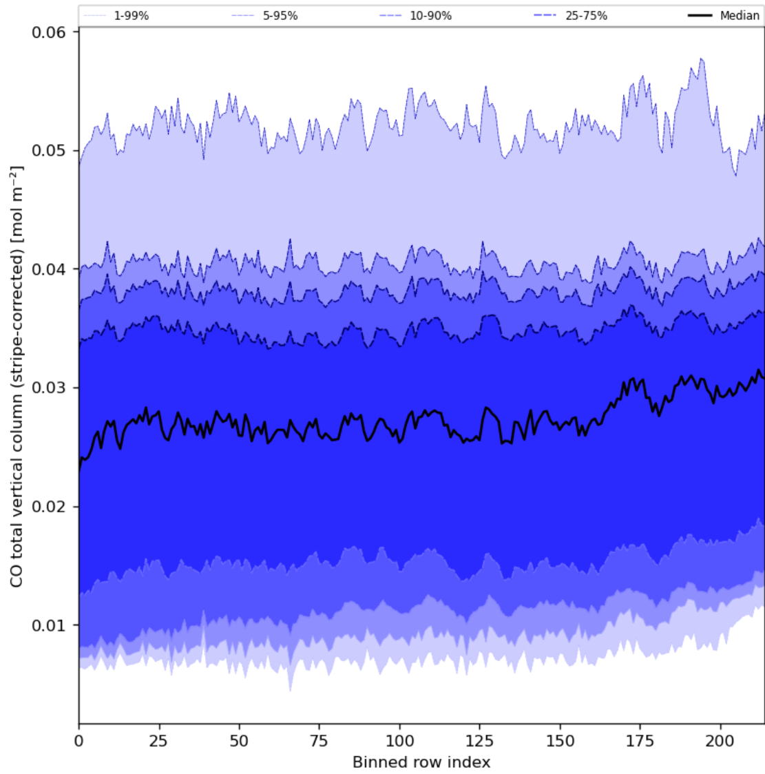
Figure 27: Along track statistics of “CO total vertical column (stripe-corrected)” for 2024-03-02 to 2024-03-04
