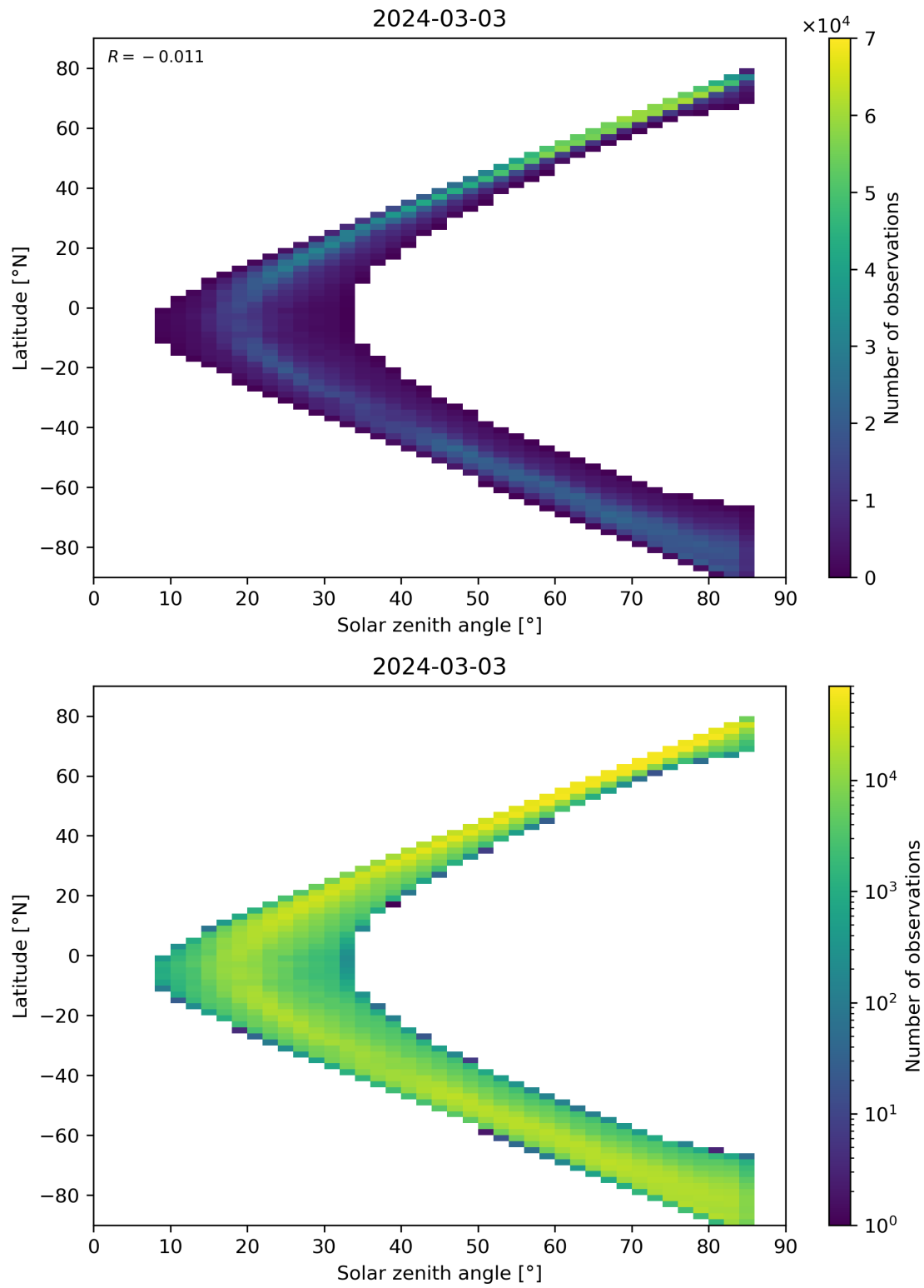
Figure 66: Scatter density plot of “Solar zenith angle” against “Latitude” for 2024-03-02 to 2024-03-04.
