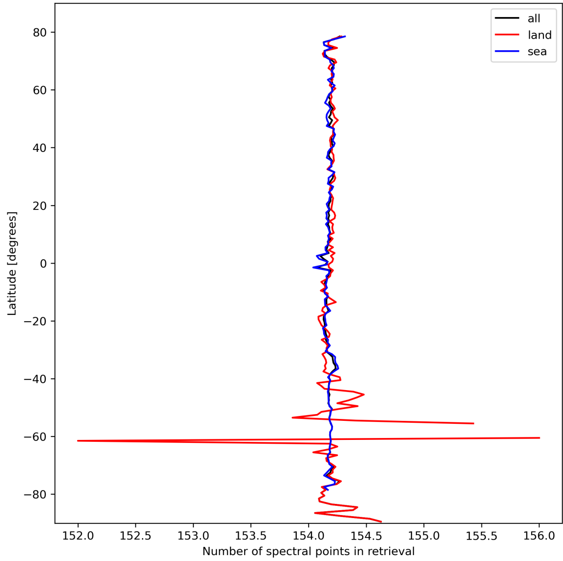
Figure 13: Zonal average of “Number of spectral points in retrieval” for 2024-03-02 to 2024-03-04.
