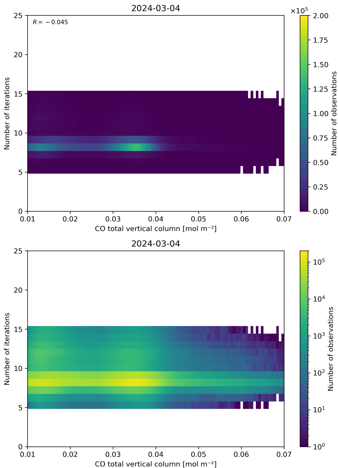
Figure 42: Scatter density plot of “CO total vertical column” against “Number of iterations” for 2024-03-04 to 2024-03-05.
