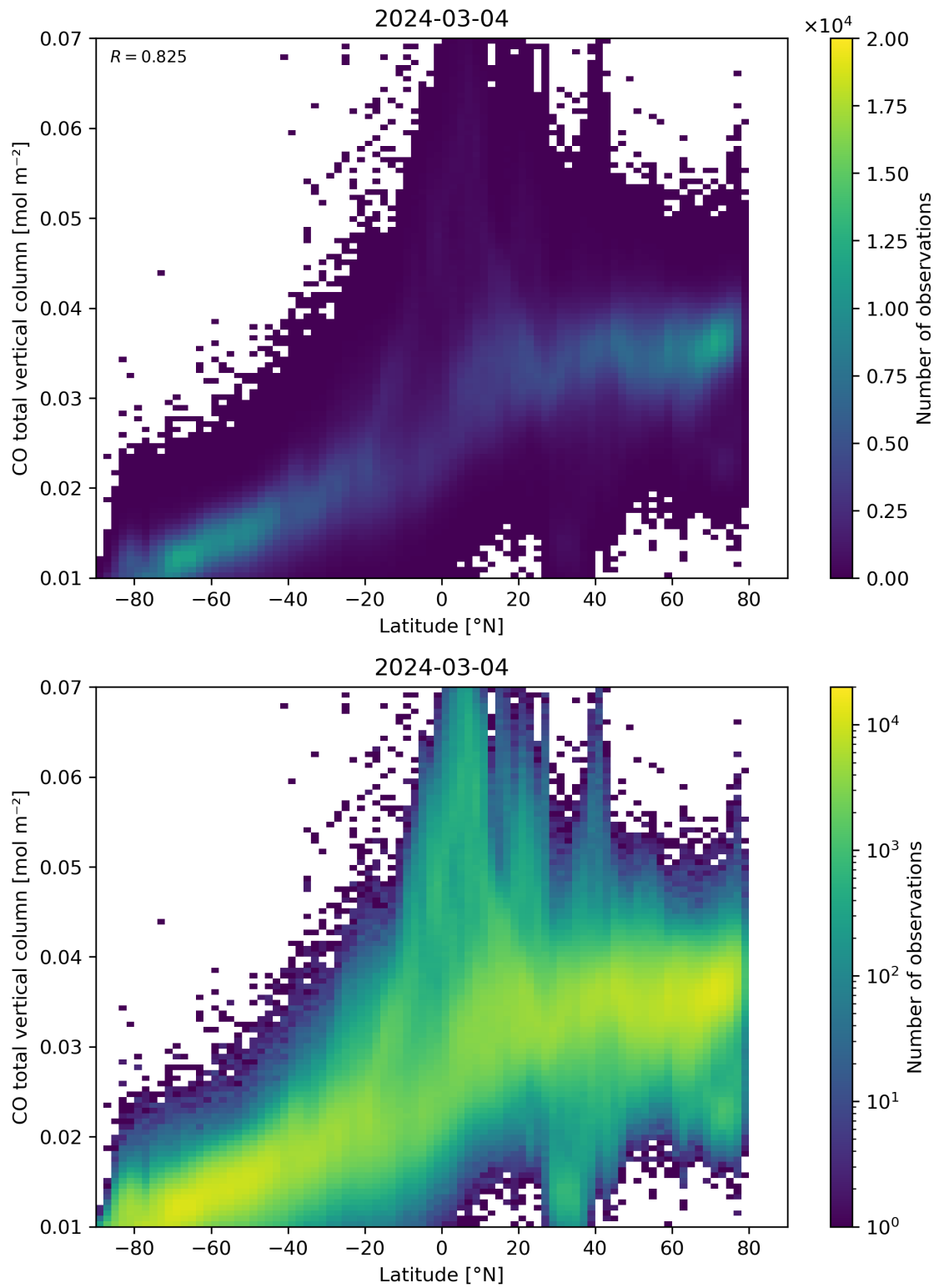
Figure 51: Scatter density plot of “Latitude” against “CO total vertical column” for 2024-03-04 to 2024-03-05.
