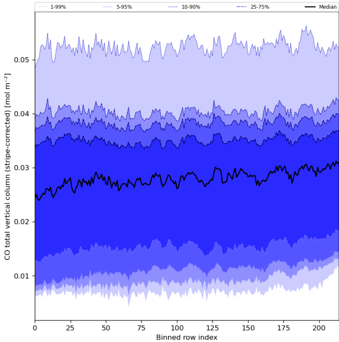
Figure 27: Along track statistics of “CO total vertical column (stripe-corrected)” for 2024-03-04 to 2024-03-05
