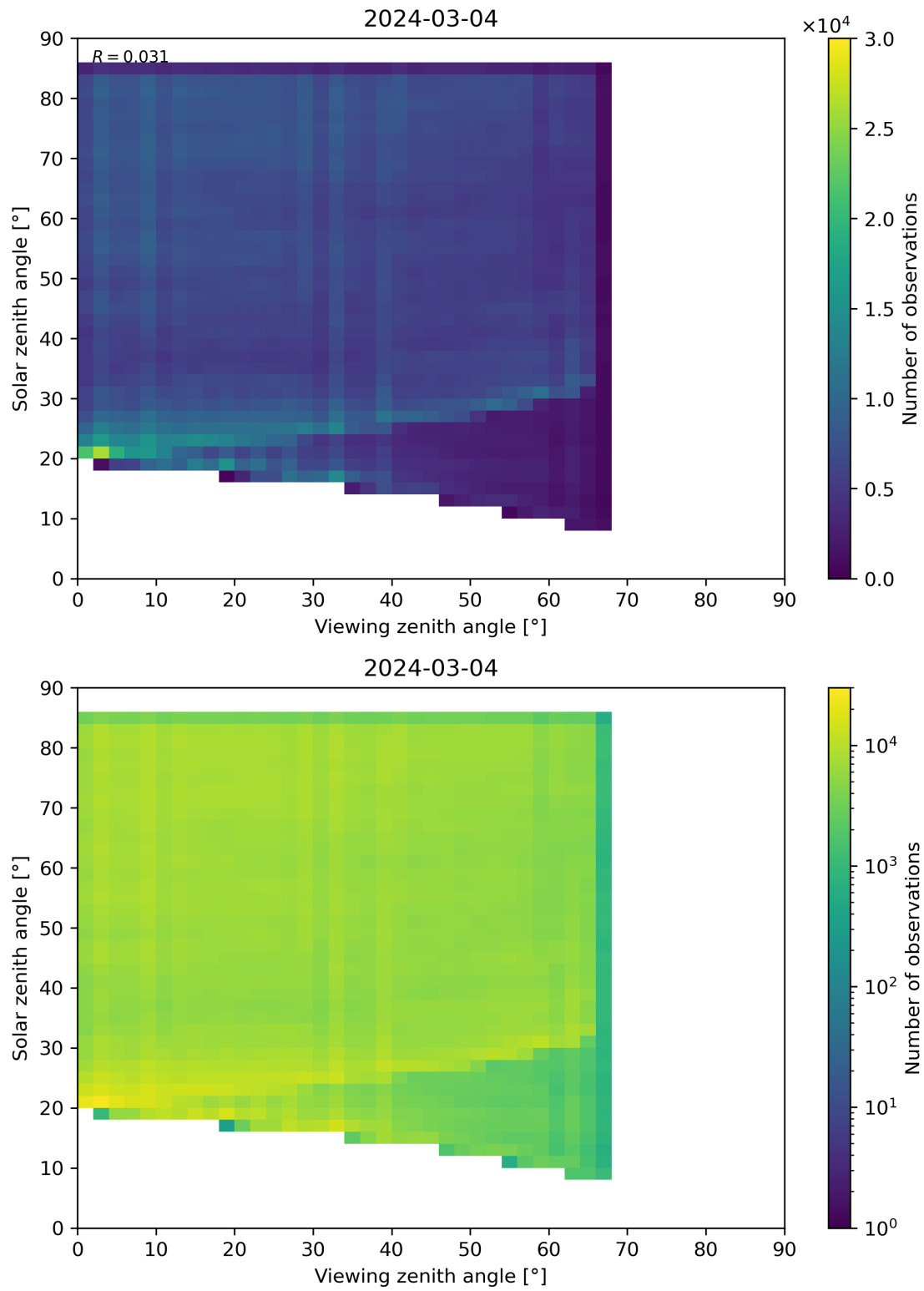
Figure 77: Scatter density plot of “Viewing zenith angle” against “Solar zenith angle” for 2024-03-04 to 2024-03-05.
