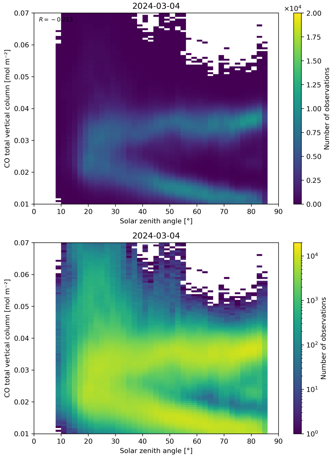
Figure 61: Scatter density plot of “Solar zenith angle” against “CO total vertical column” for 2024-03-04 to 2024-03-05.
