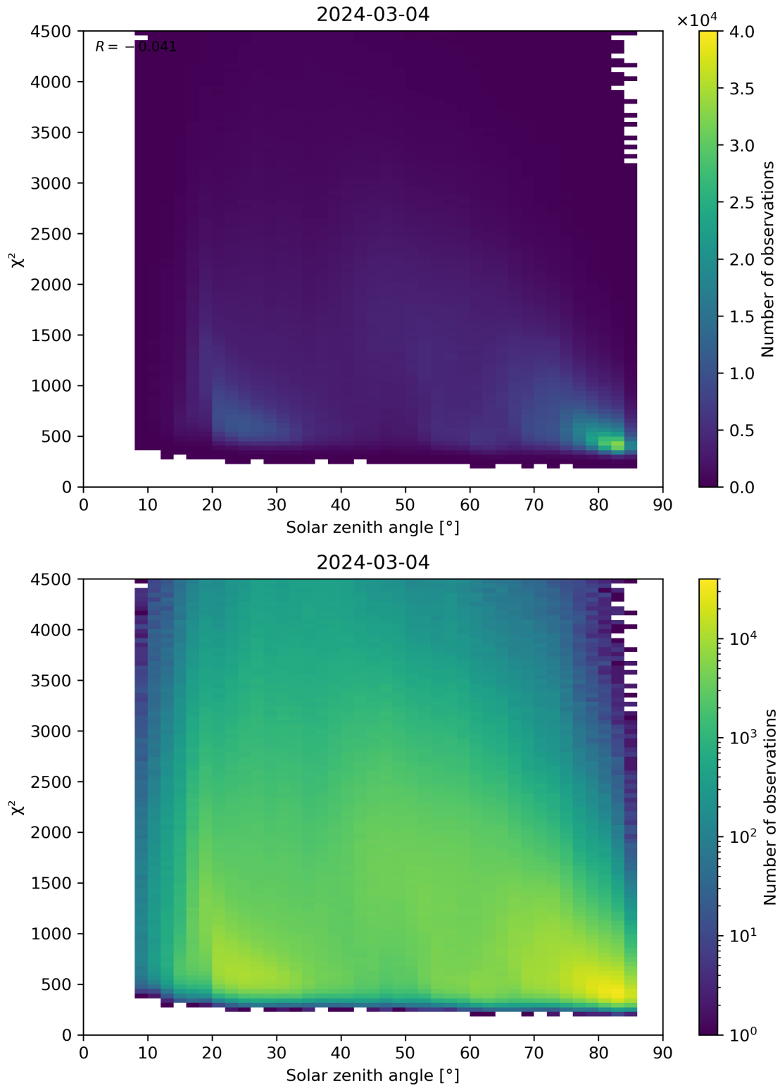
Figure 64: Scatter density plot of “Solar zenith angle” against “ \chi^2 ” for 2024-03-04 to 2024-03-05.
