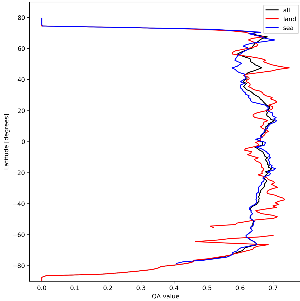
Figure 9: Zonal average of “QA value” for 2024-03-04 to 2024-03-05.
