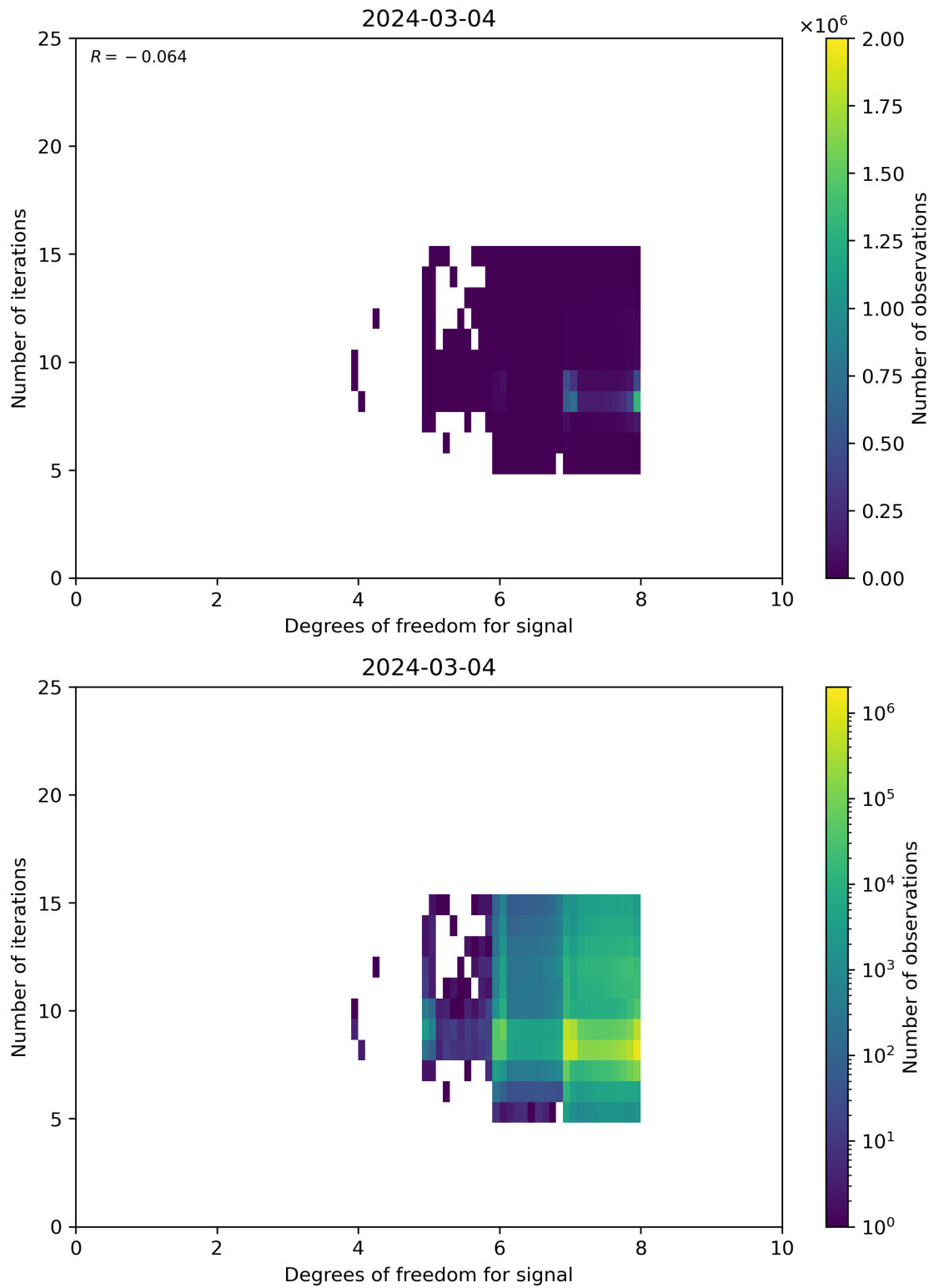
Figure 50: Scatter density plot of “Degrees of freedom for signal” against “Number of iterations” for 2024-03-04 to 2024-03-05.
