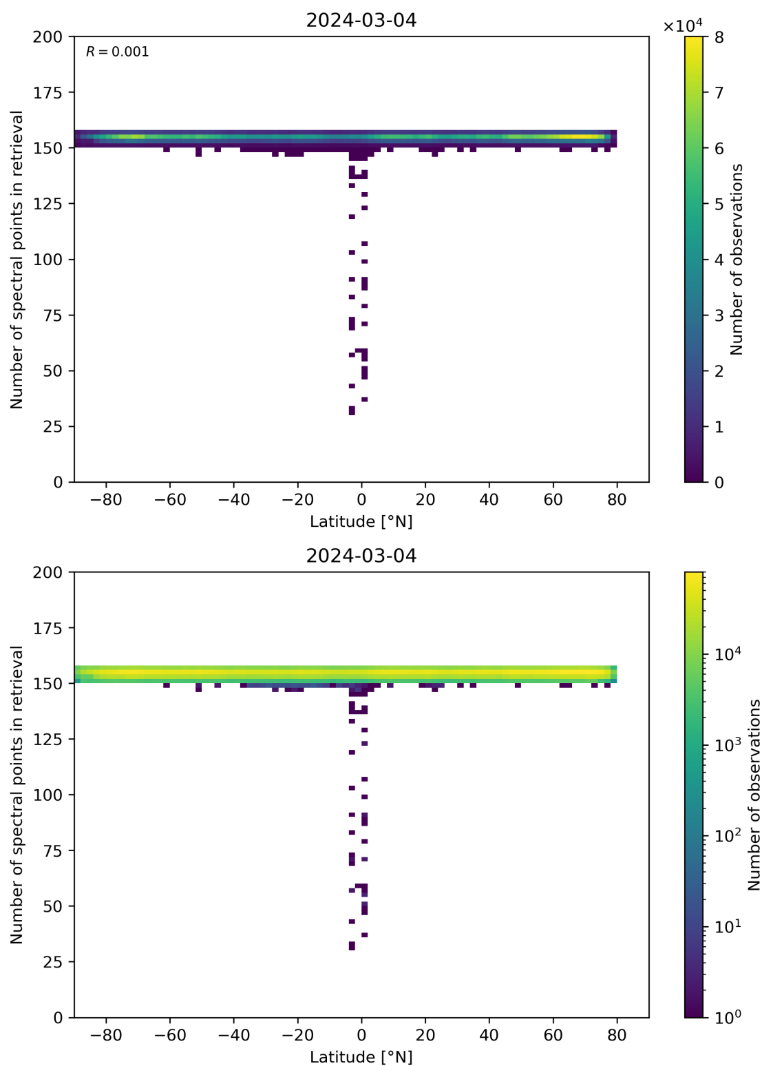
Figure 57: Scatter density plot of “Latitude” against “Number of spectral points in retrieval” for 2024-03-04 to 2024-03-05.
