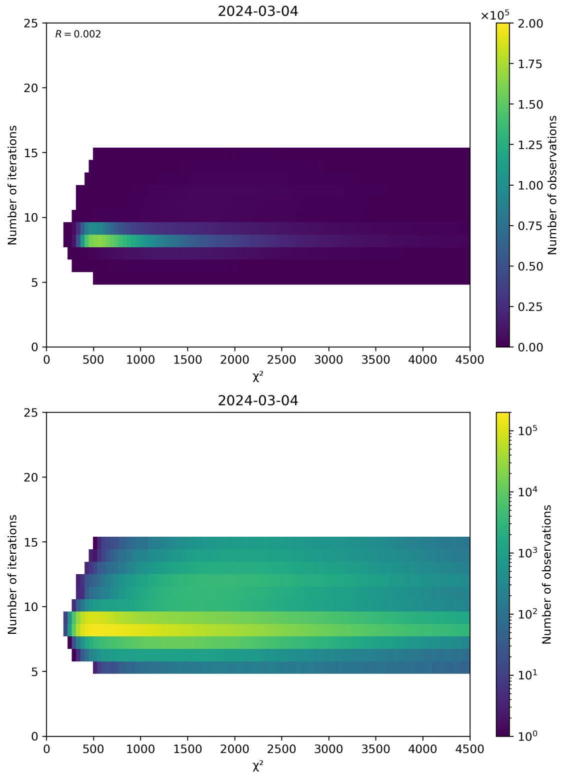
Figure 49: Scatter density plot of “ \chi^2 ” against “Number of iterations” for 2024-03-04 to 2024-03-05.
