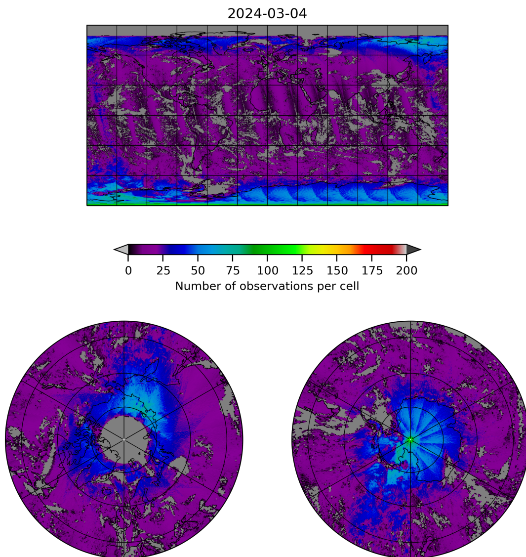
Figure 8: Map of the number of observations for 2024-03-04 to 2024-03-05
