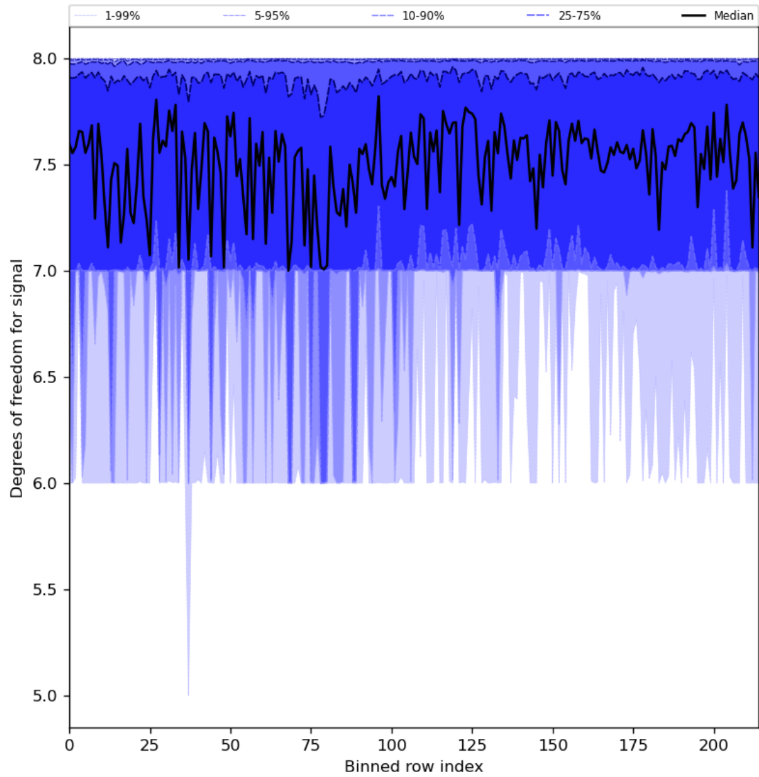
Figure 31: Along track statistics of “Degrees of freedom for signal” for 2024-03-04 to 2024-03-05
