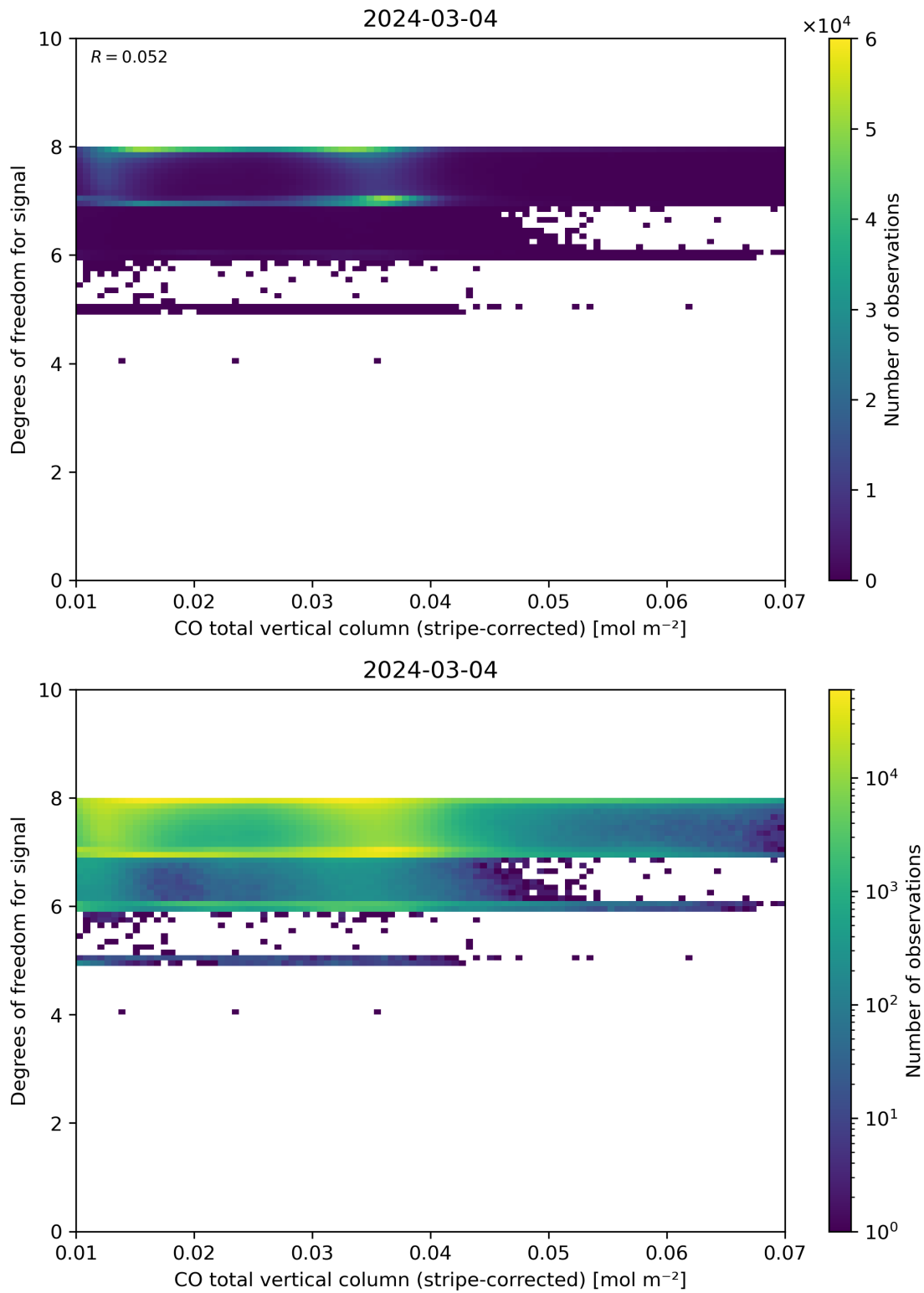
Figure 38: Scatter density plot of “CO total vertical column (stripe-corrected)” against “Degrees of freedom for signal” for 2024-03-04 to 2024-03-05.
