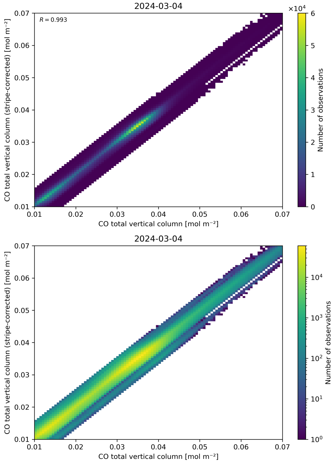
Figure 33: Scatter density plot of “CO total vertical column” against “CO total vertical column (stripe-corrected)” for 2024-03-04 to 2024-03-05.
