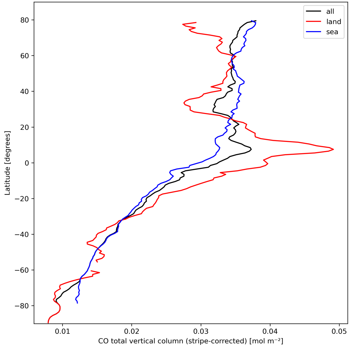
Figure 11: Zonal average of “CO total vertical column (stripe-corrected)” for 2024-03-04 to 2024-03-05.
