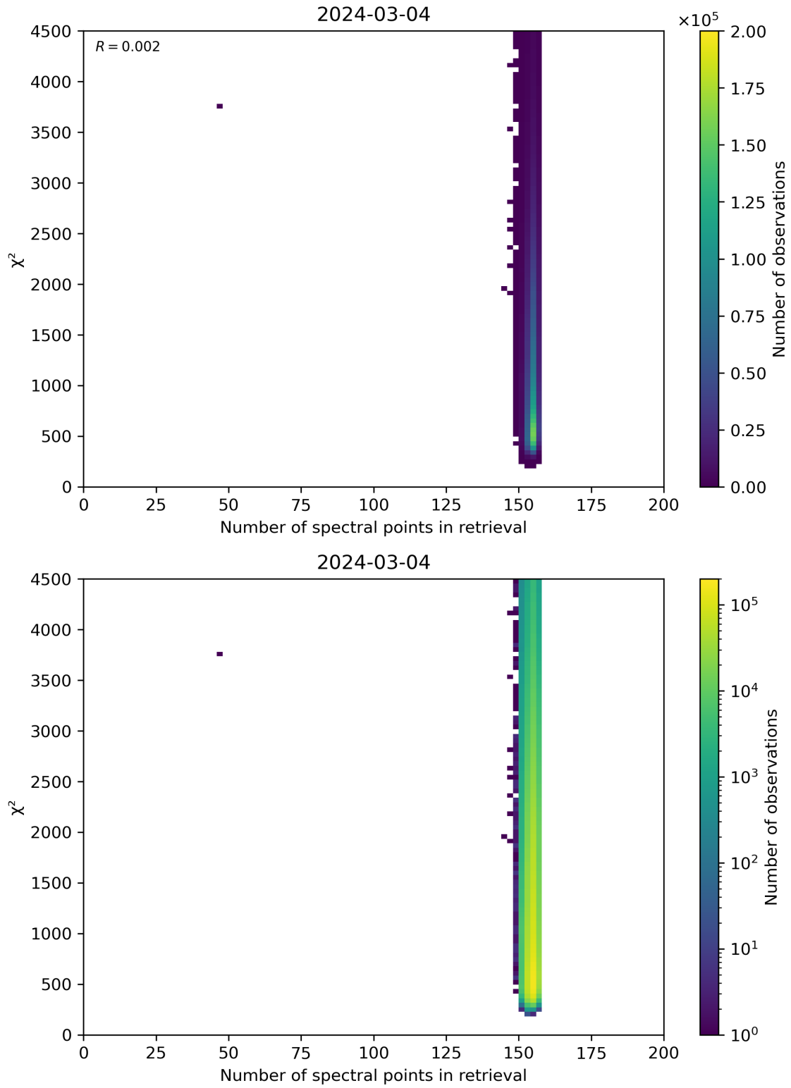
Figure 58: Scatter density plot of “Number of spectral points in retrieval” against “ \chi^2 ” for 2024-03-04 to 2024-03-05.
