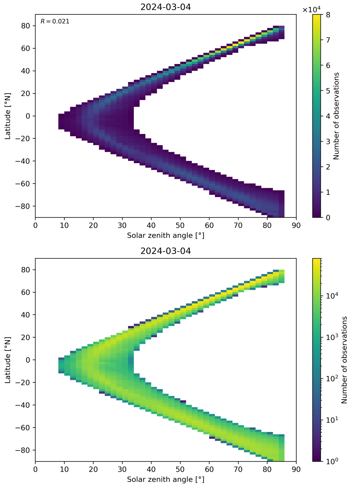
Figure 66: Scatter density plot of “Solar zenith angle” against “Latitude” for 2024-03-04 to 2024-03-05.
