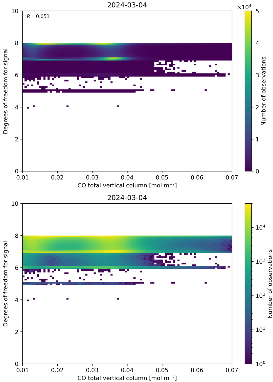
Figure 41: Scatter density plot of “CO total vertical column” against “Degrees of freedom for signal” for 2024-03-04 to 2024-03-05.
