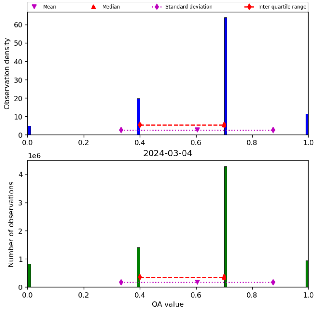
Figure 17: Histogram of “QA value” for 2024-03-04 to 2024-03-05
