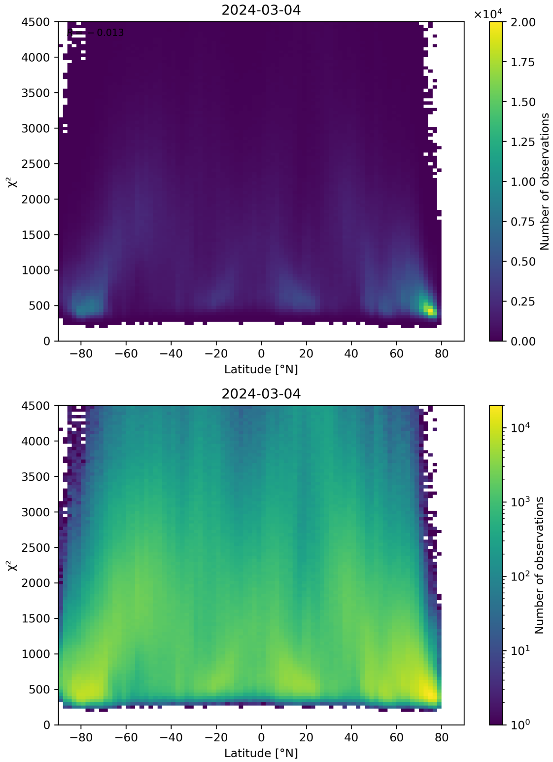
Figure 54: Scatter density plot of “Latitude” against “ \chi^2 ” for 2024-03-04 to 2024-03-05.
