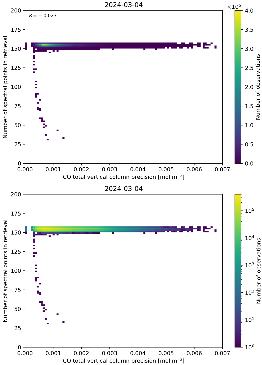
Figure 47: Scatter density plot of “CO total vertical column precision” against “Number of spectral points in retrieval” for 2024-03-04 to 2024-03-05.
