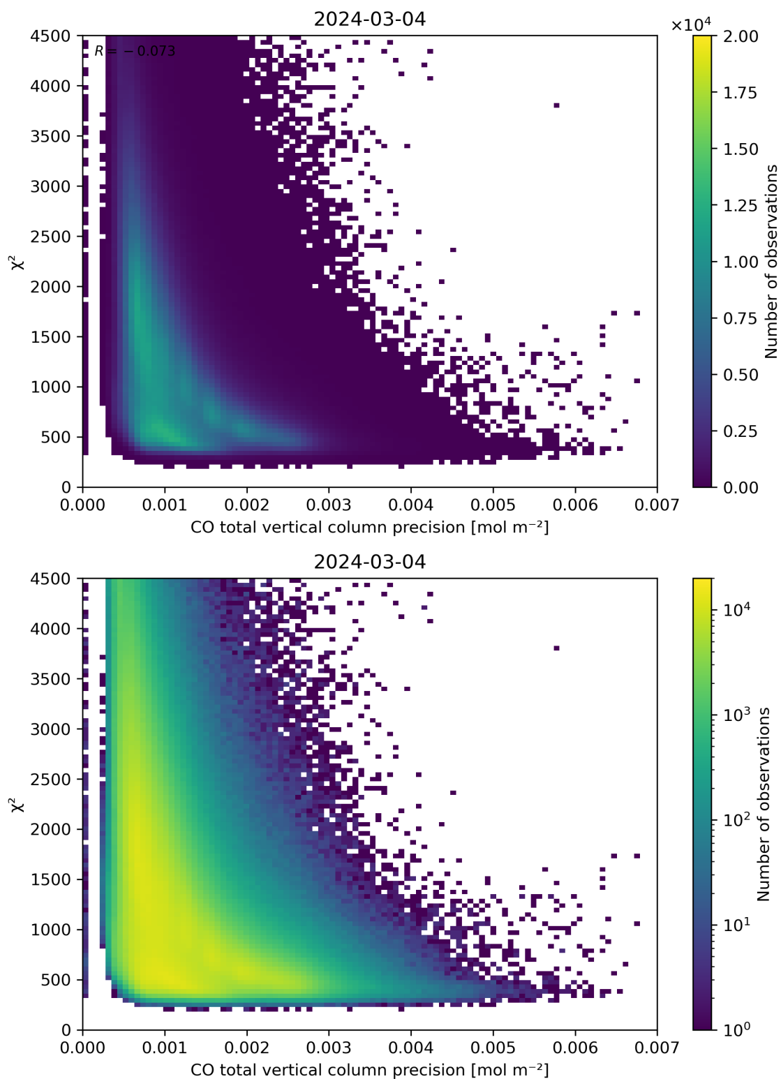
Figure 44: Scatter density plot of “CO total vertical column precision” against “ \chi^2 ” for 2024-03-04 to 2024-03-05.
