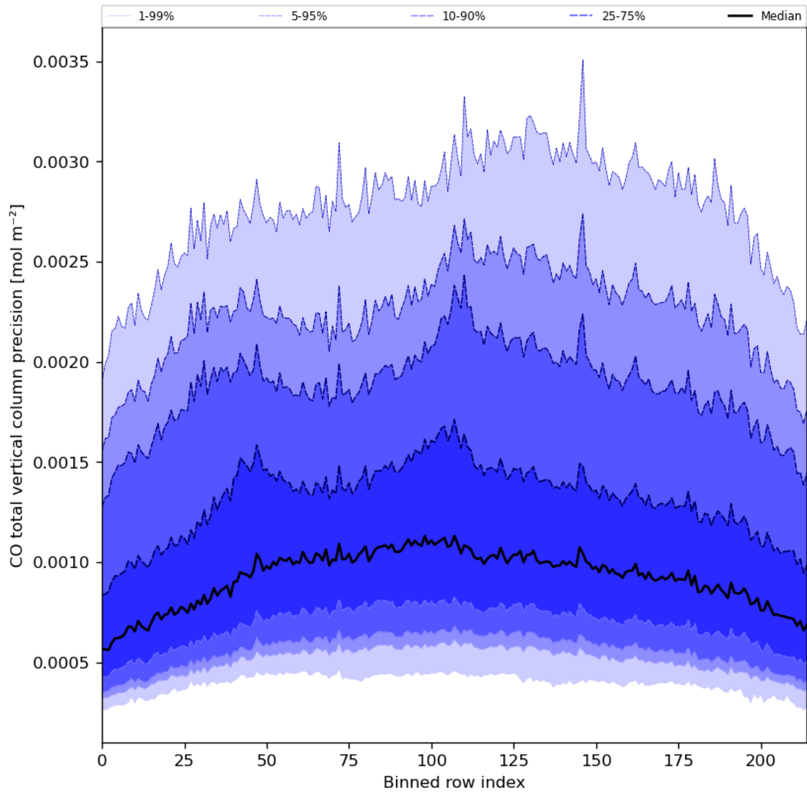
Figure 28: Along track statistics of “CO total vertical column precision” for 2024-03-04 to 2024-03-05
