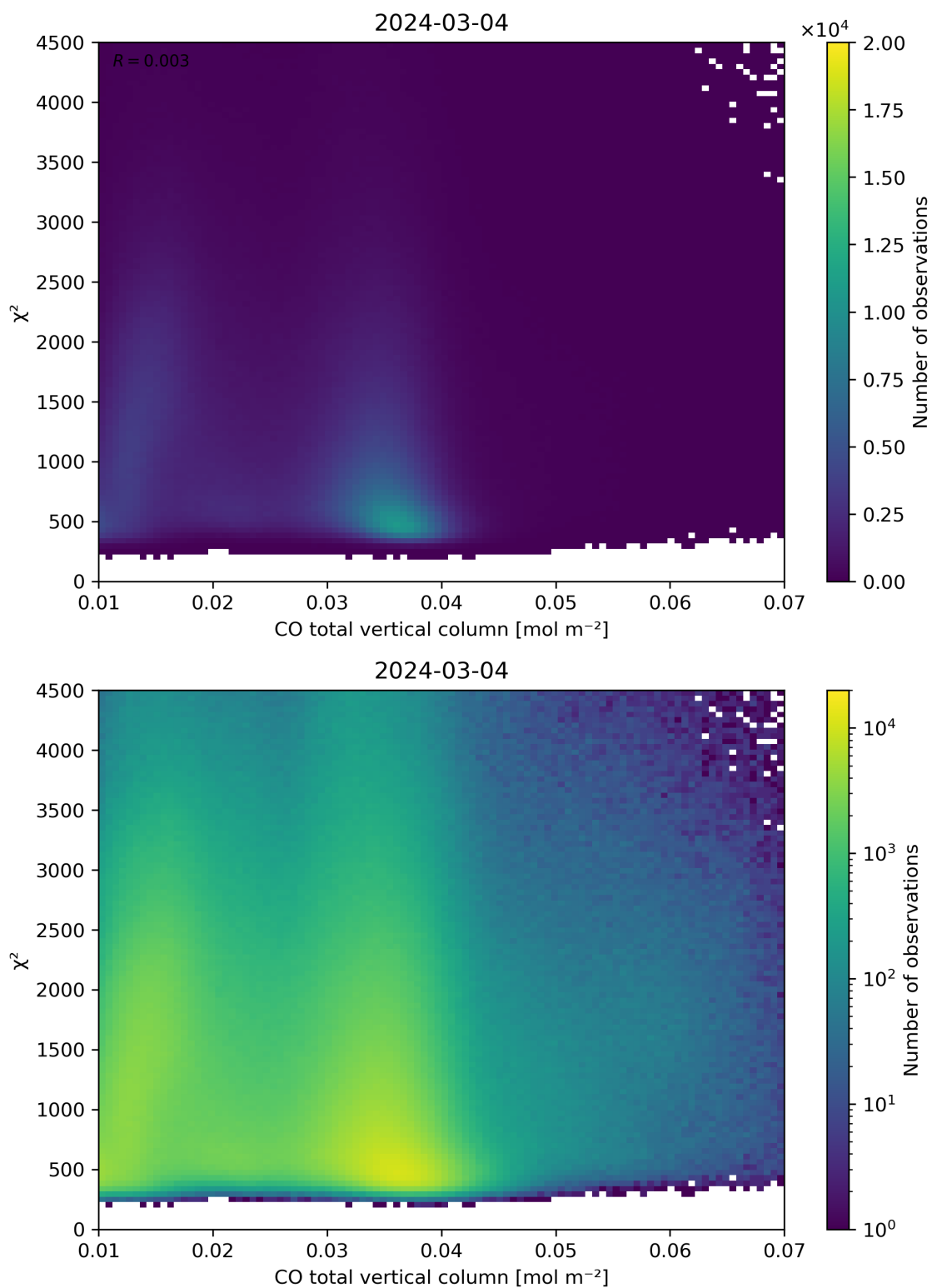
Figure 35: Scatter density plot of “CO total vertical column” against “ \chi^2 ” for 2024-03-04 to 2024-03-05.
