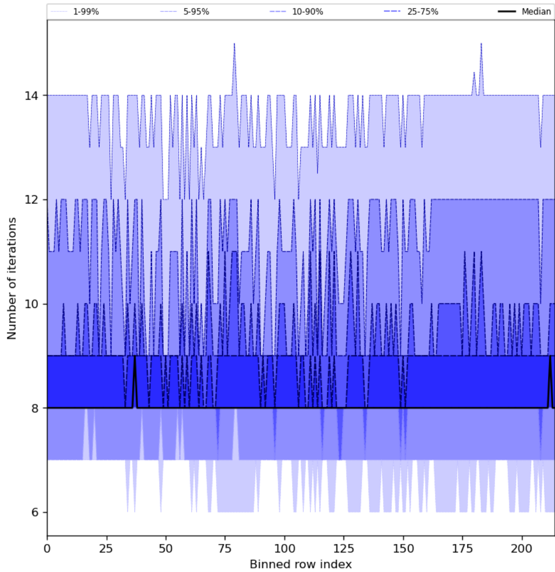
Figure 32: Along track statistics of “Number of iterations” for 2024-03-04 to 2024-03-05
