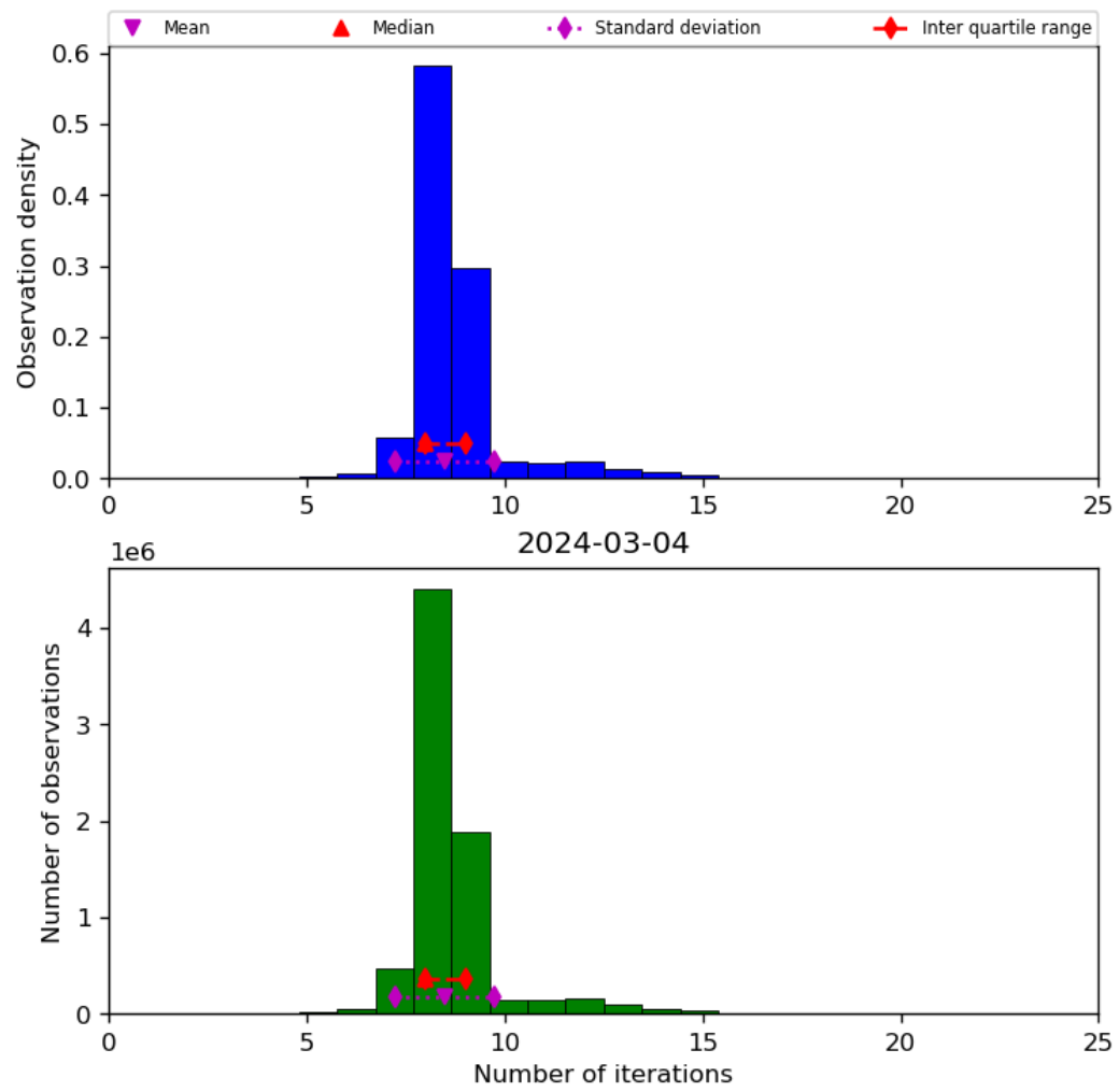
Figure 24: Histogram of “Number of iterations” for 2024-03-04 to 2024-03-05
