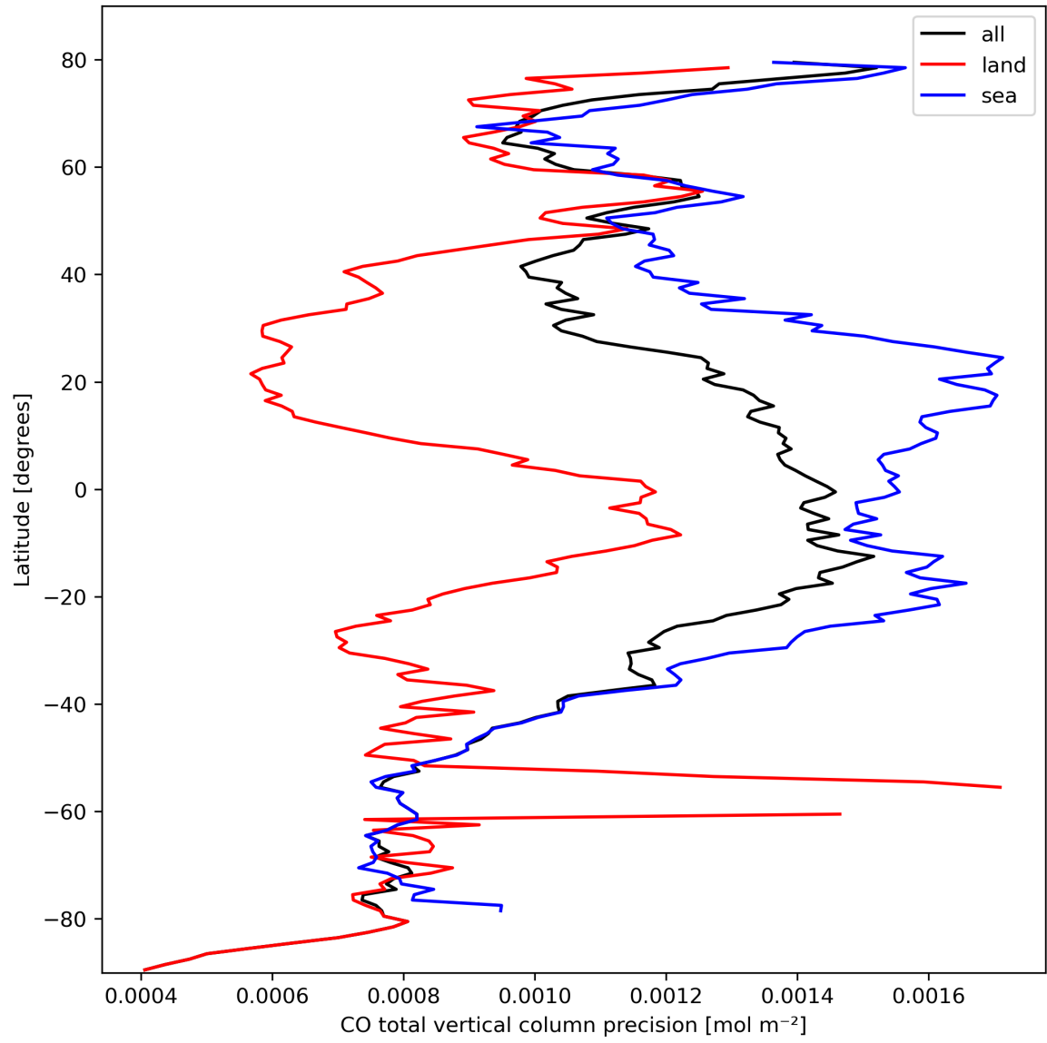
Figure 12: Zonal average of “CO total vertical column precision” for 2024-03-04 to 2024-03-05.
