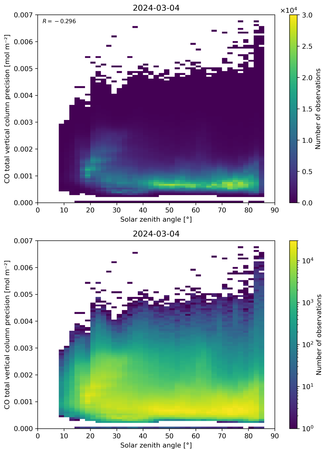
Figure 63: Scatter density plot of “Solar zenith angle” against “CO total vertical column precision” for 2024-03-04 to 2024-03-05.
