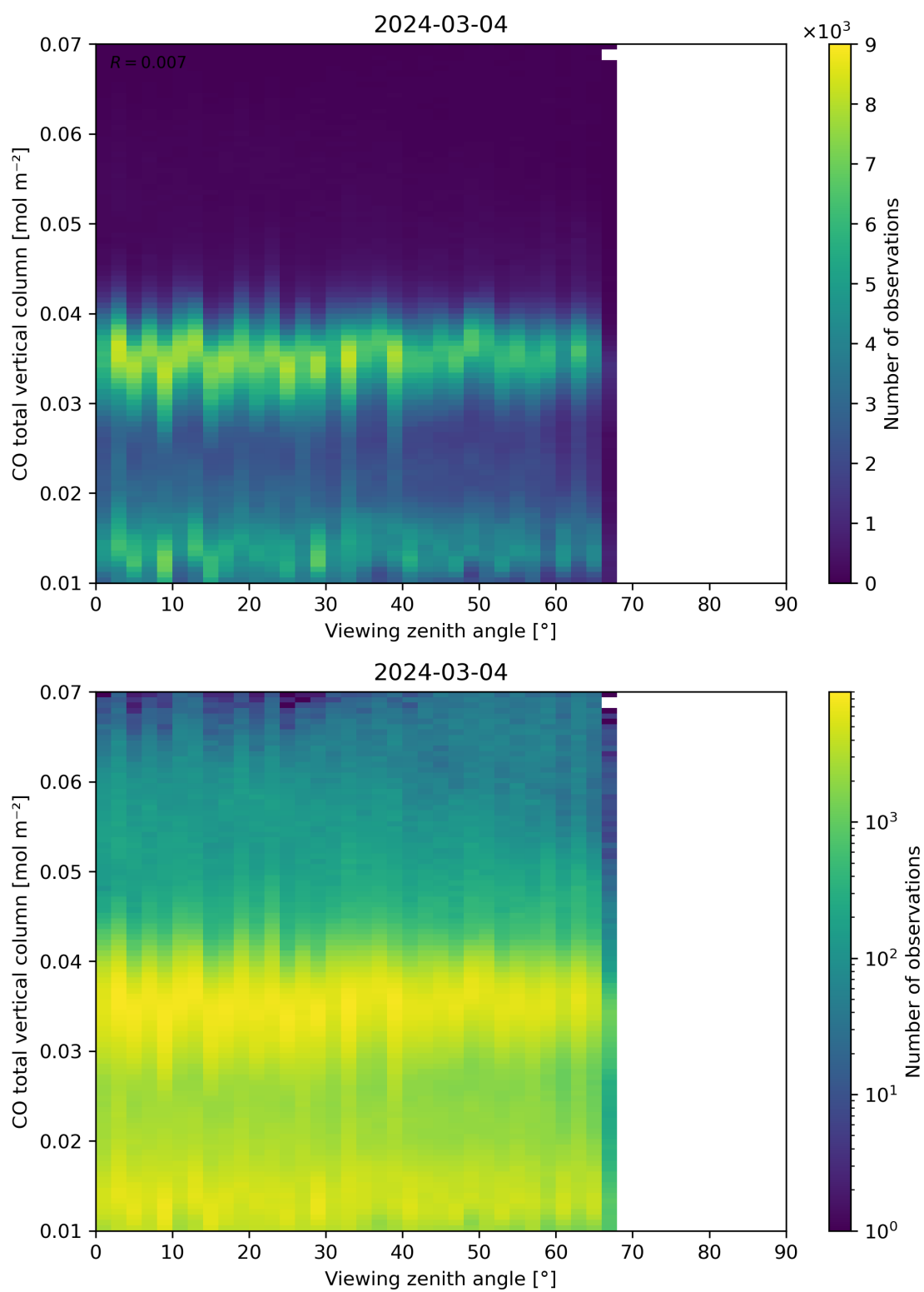
Figure 69: Scatter density plot of “Viewing zenith angle” against “CO total vertical column” for 2024-03-04 to 2024-03-05.
