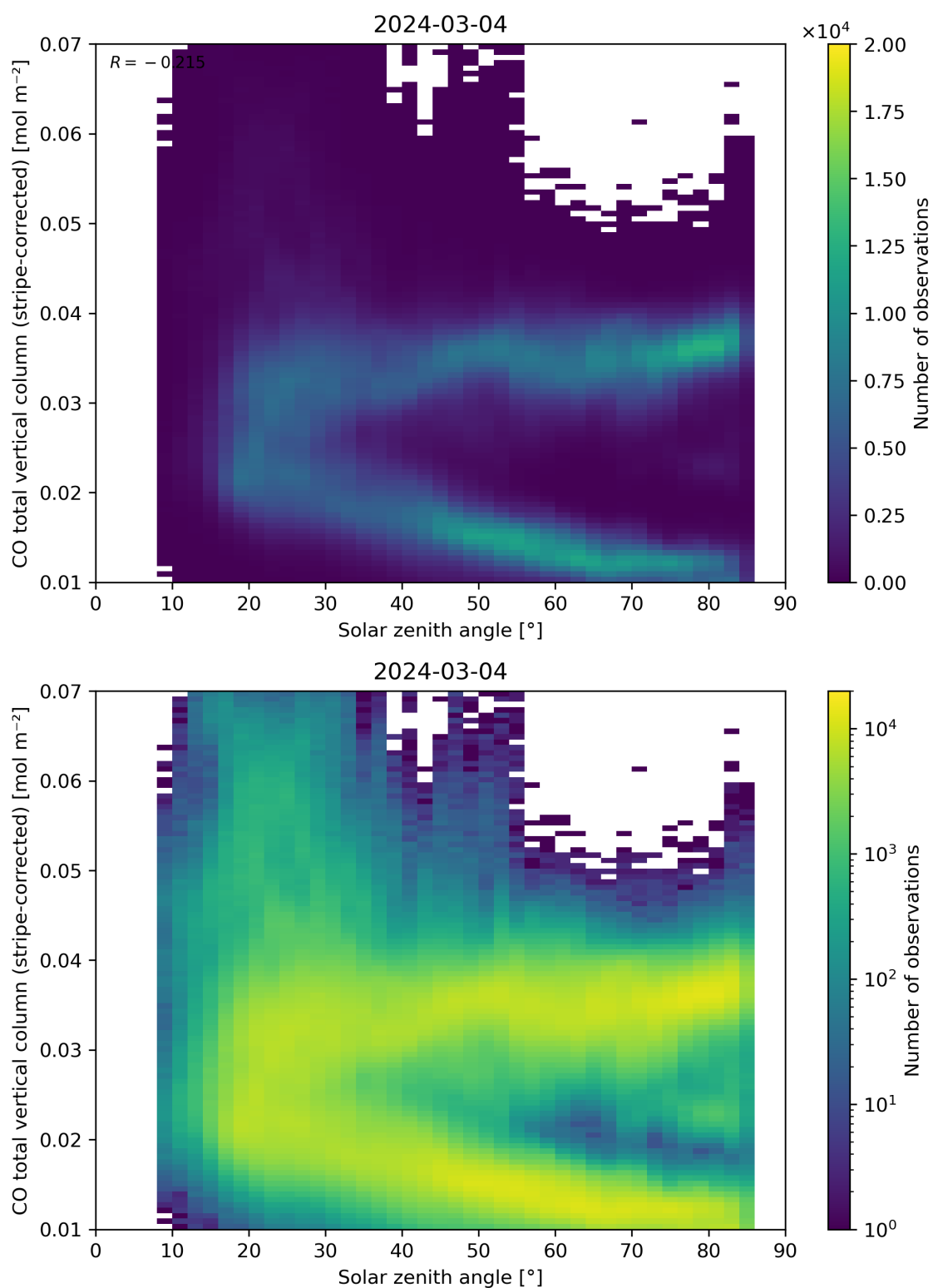
Figure 62: Scatter density plot of “Solar zenith angle” against “CO total vertical column (stripe-corrected)” for 2024-03-04 to 2024-03-05.
