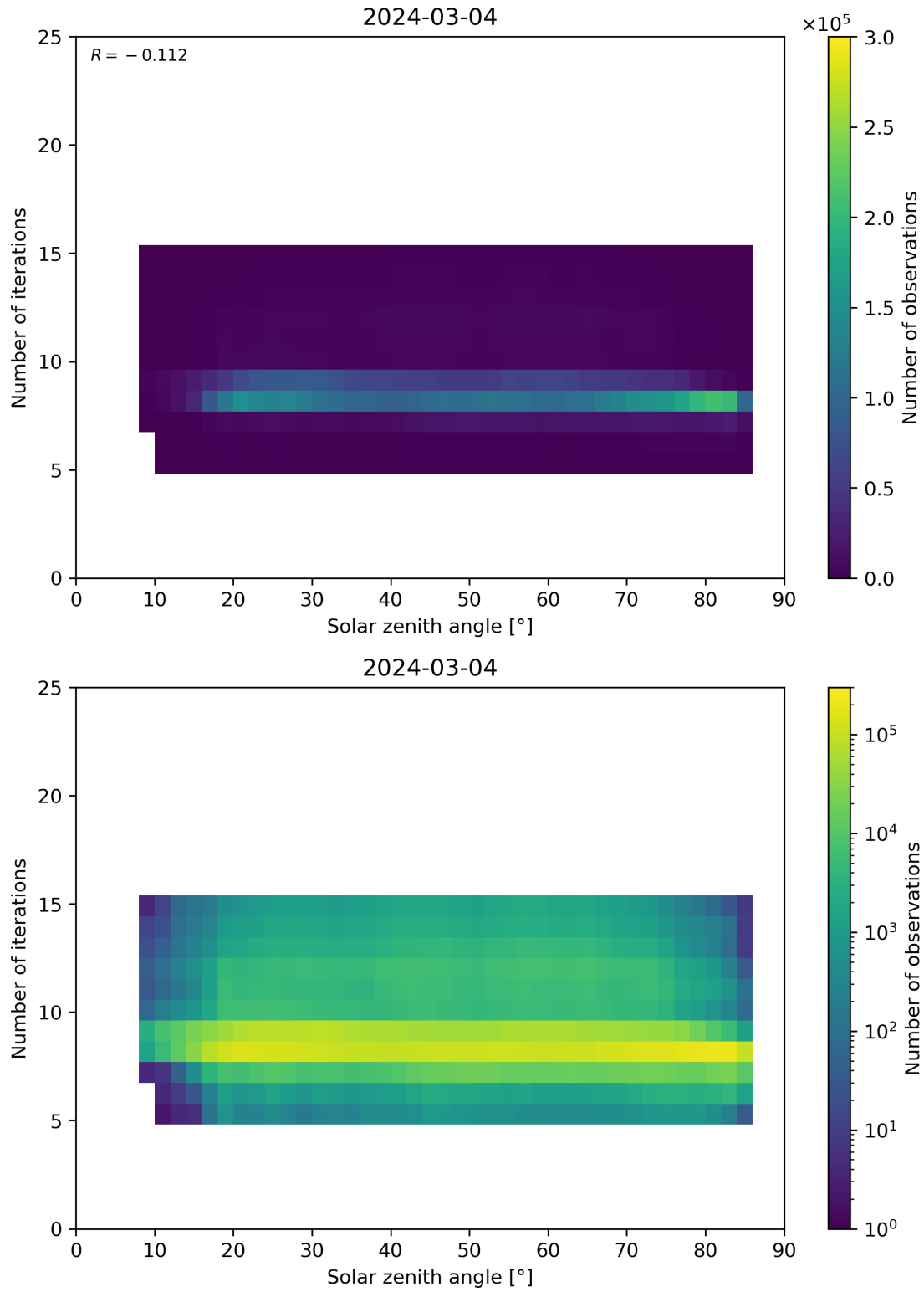
Figure 67: Scatter density plot of “Solar zenith angle” against “Number of iterations” for 2024-03-04 to 2024-03-05.
