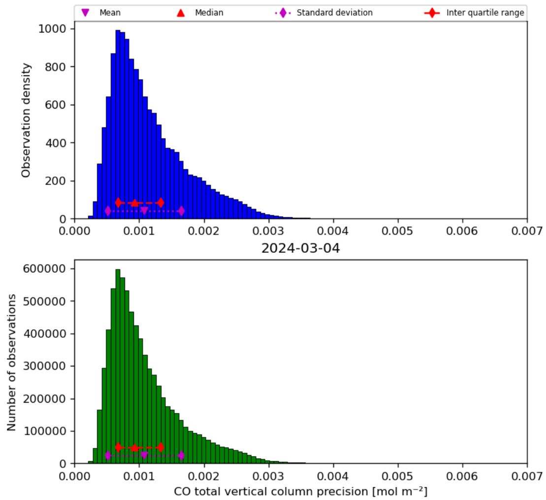
Figure 20: Histogram of “CO total vertical column precision” for 2024-03-04 to 2024-03-05
