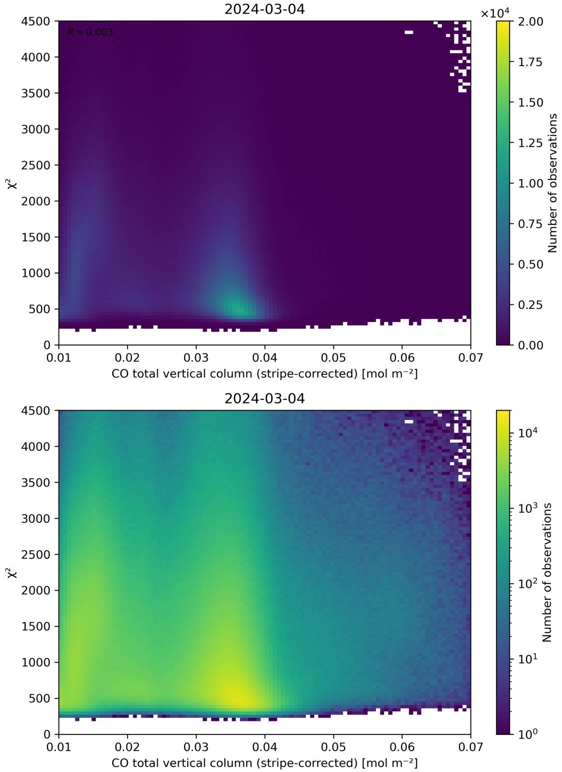
Figure 37: Scatter density plot of “CO total vertical column (stripe-corrected)” against “ \chi^2 ” for 2024-03-04 to 2024-03-05.
