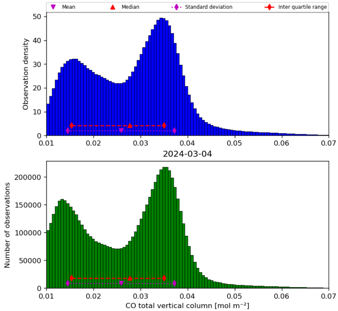
Figure 18: Histogram of “CO total vertical column” for 2024-03-04 to 2024-03-05
