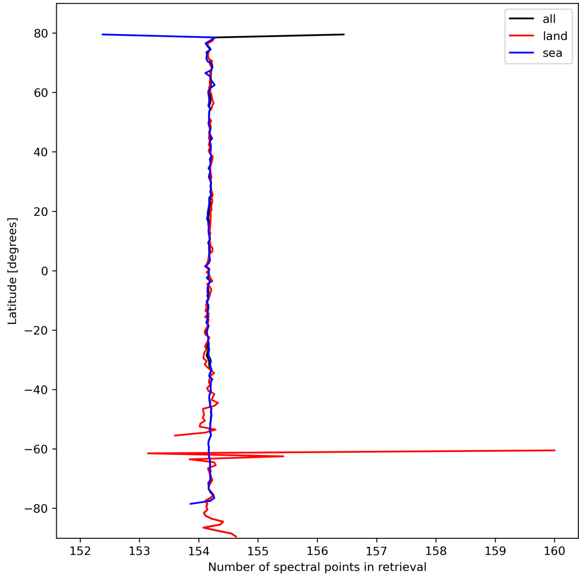
Figure 13: Zonal average of “Number of spectral points in retrieval” for 2024-03-04 to 2024-03-05.
