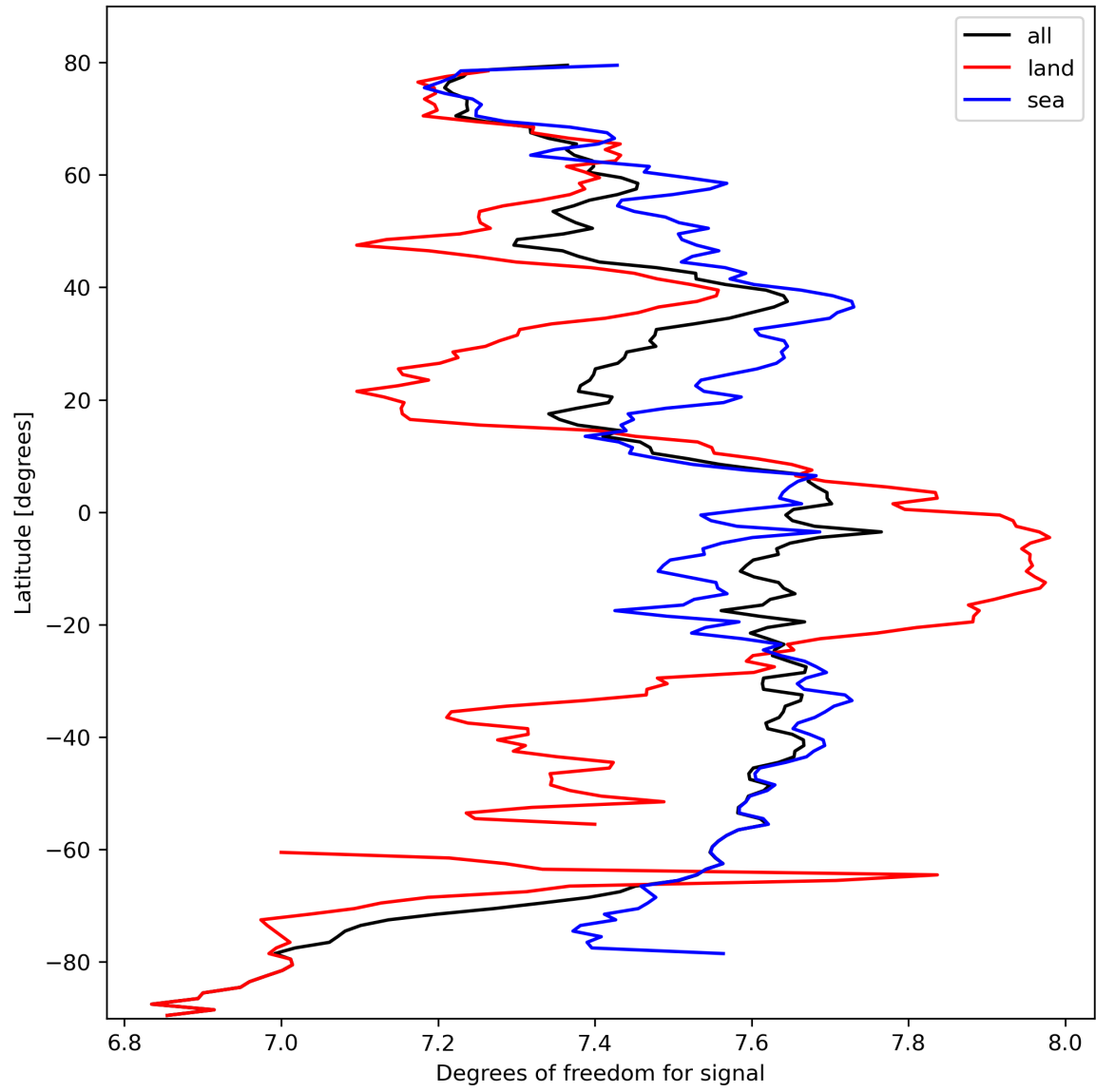
Figure 15: Zonal average of “Degrees of freedom for signal” for 2024-03-04 to 2024-03-05.
