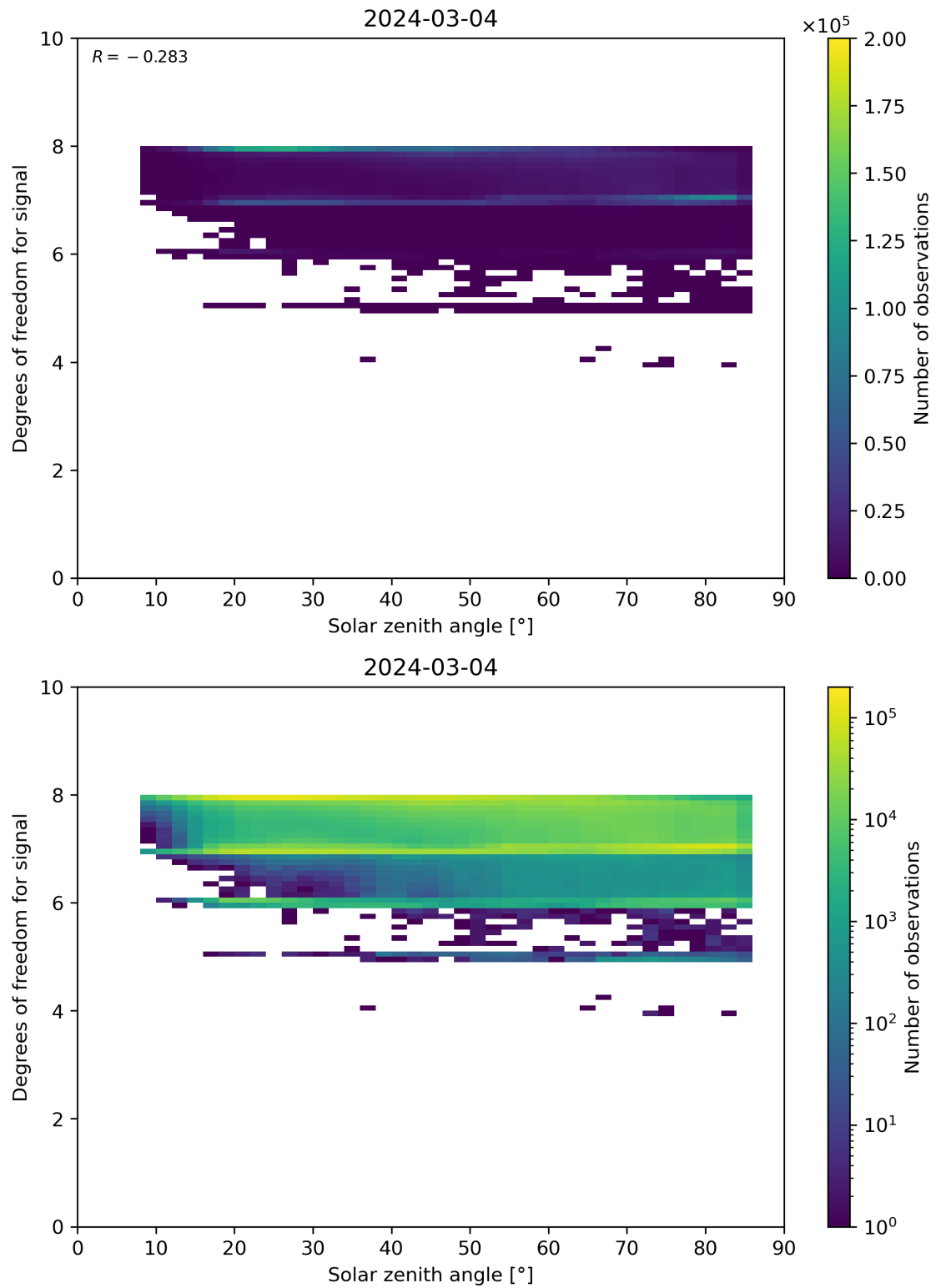
Figure 65: Scatter density plot of “Solar zenith angle” against “Degrees of freedom for signal” for 2024-03-04 to 2024-03-05.
