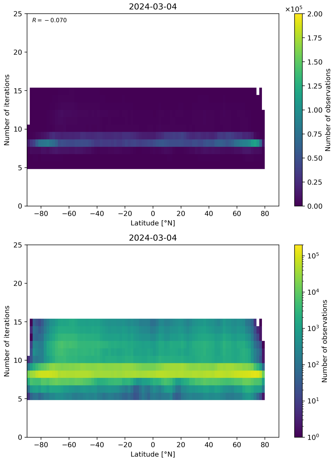
Figure 56: Scatter density plot of “Latitude” against “Number of iterations” for 2024-03-04 to 2024-03-05.
