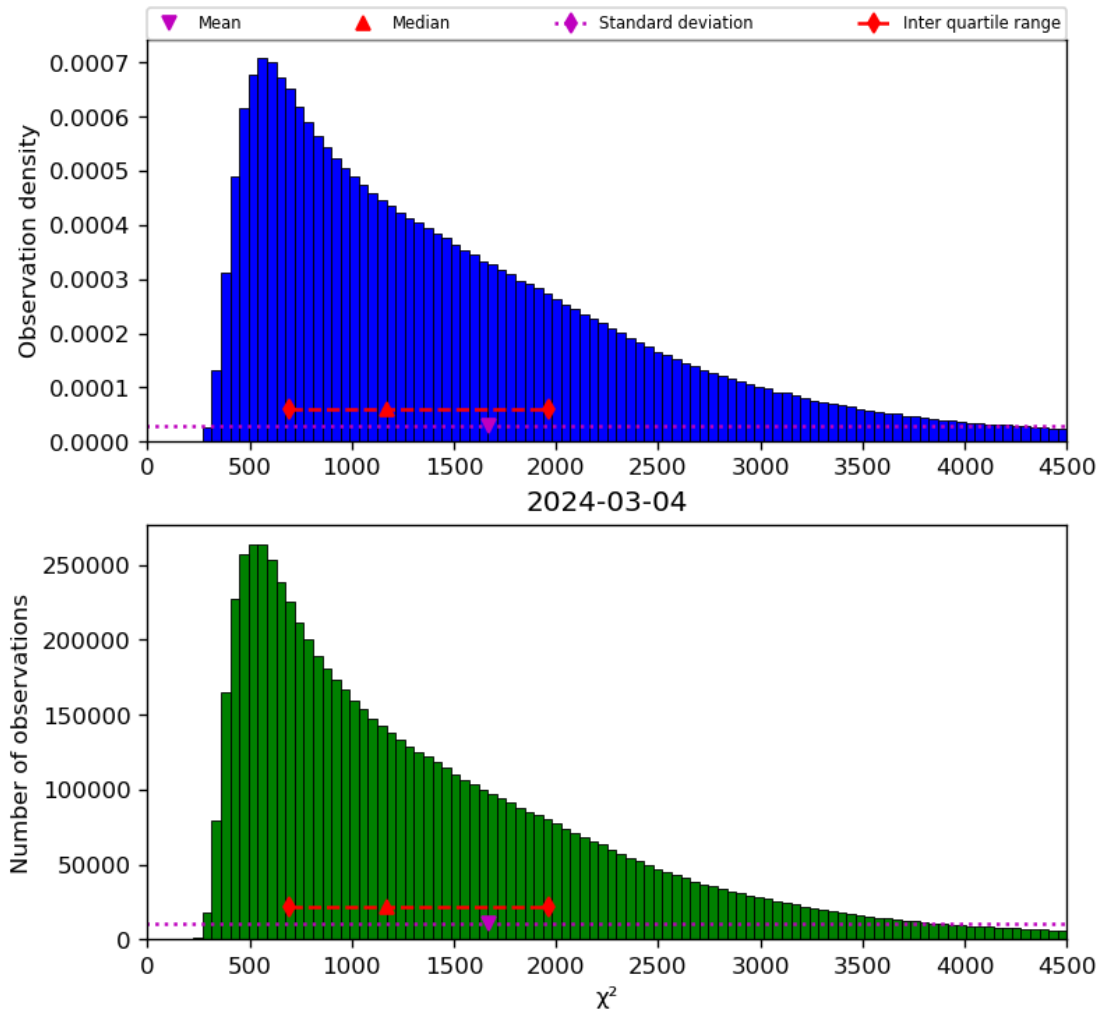
Figure 22: Histogram of “ \chi^2 ” for 2024-03-04 to 2024-03-05
