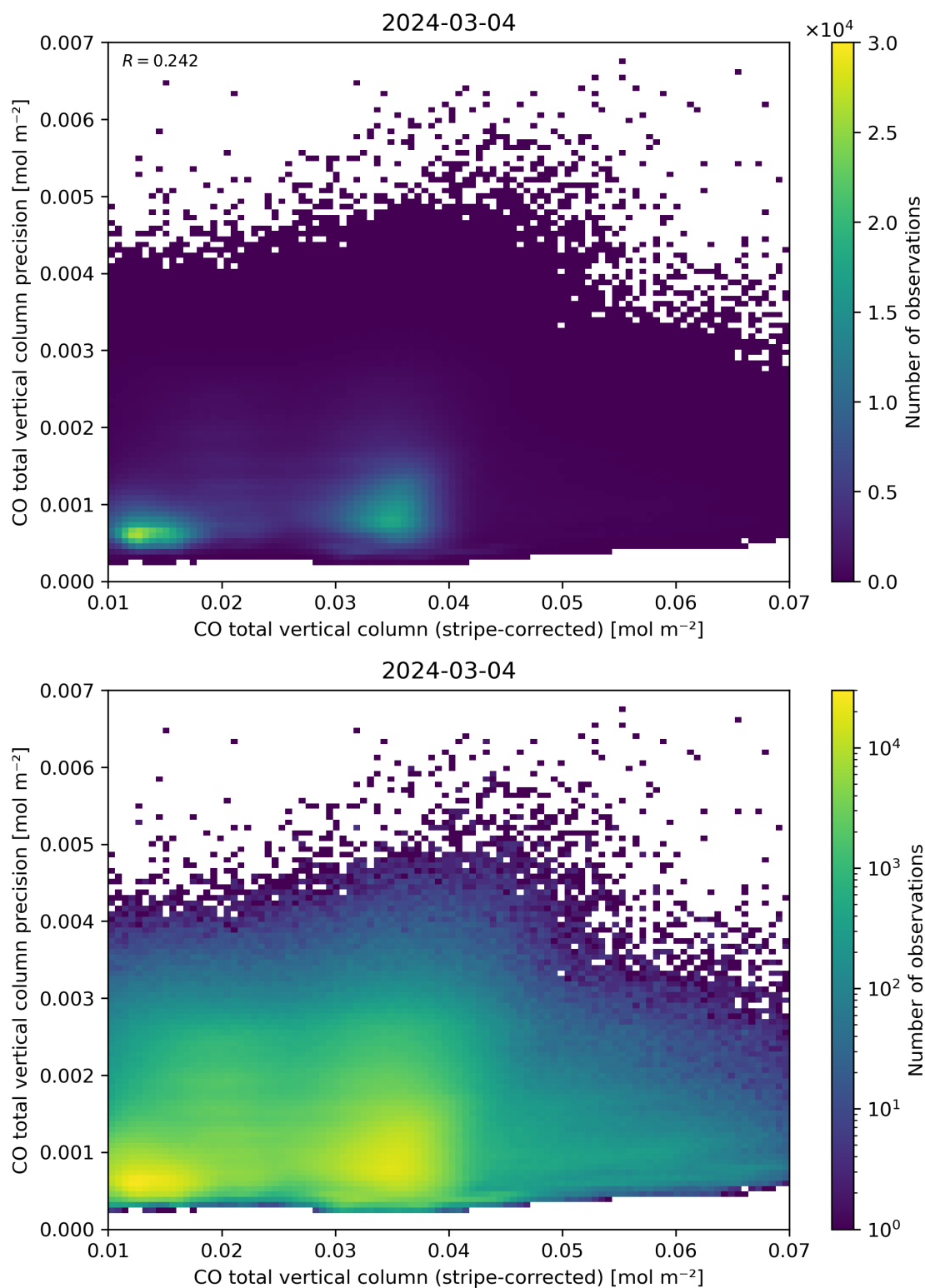
Figure 36: Scatter density plot of “CO total vertical column (stripe-corrected)” against “CO total vertical column precision” for 2024-03-04 to 2024-03-05.
