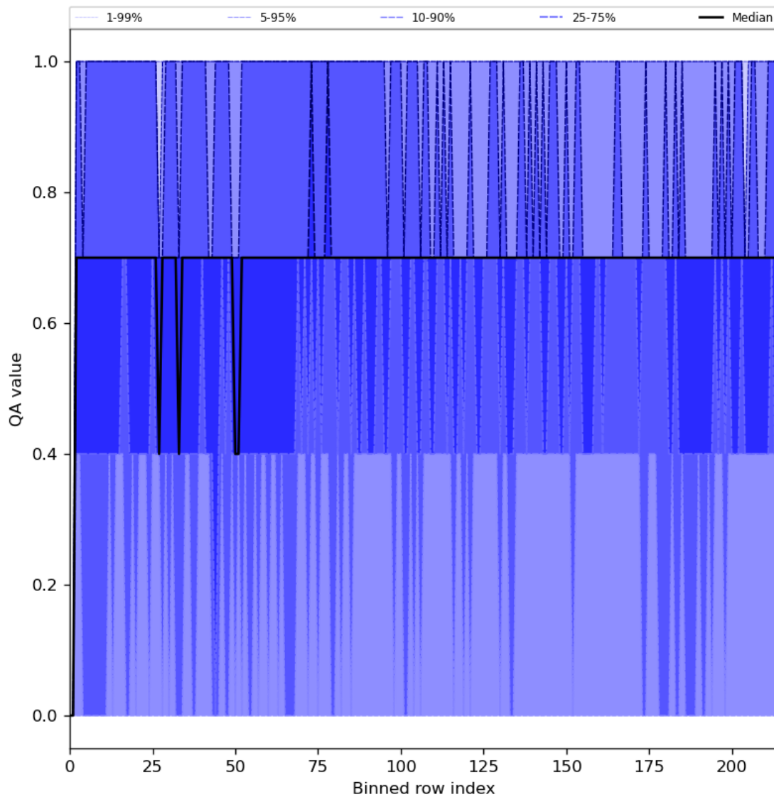
Figure 25: Along track statistics of “QA value” for 2024-03-04 to 2024-03-05
