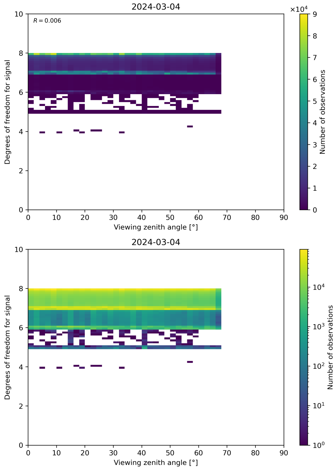
Figure 73: Scatter density plot of “Viewing zenith angle” against “Degrees of freedom for signal” for 2024-03-04 to 2024-03-05.
