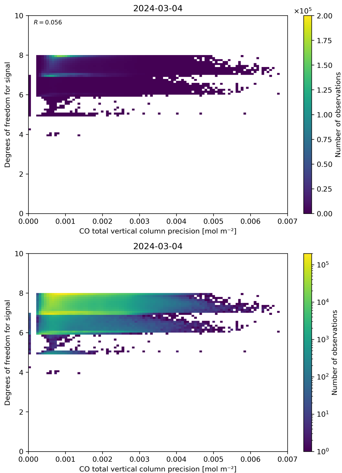
Figure 45: Scatter density plot of “CO total vertical column precision” against “Degrees of freedom for signal” for 2024-03-04 to 2024-03-05.
