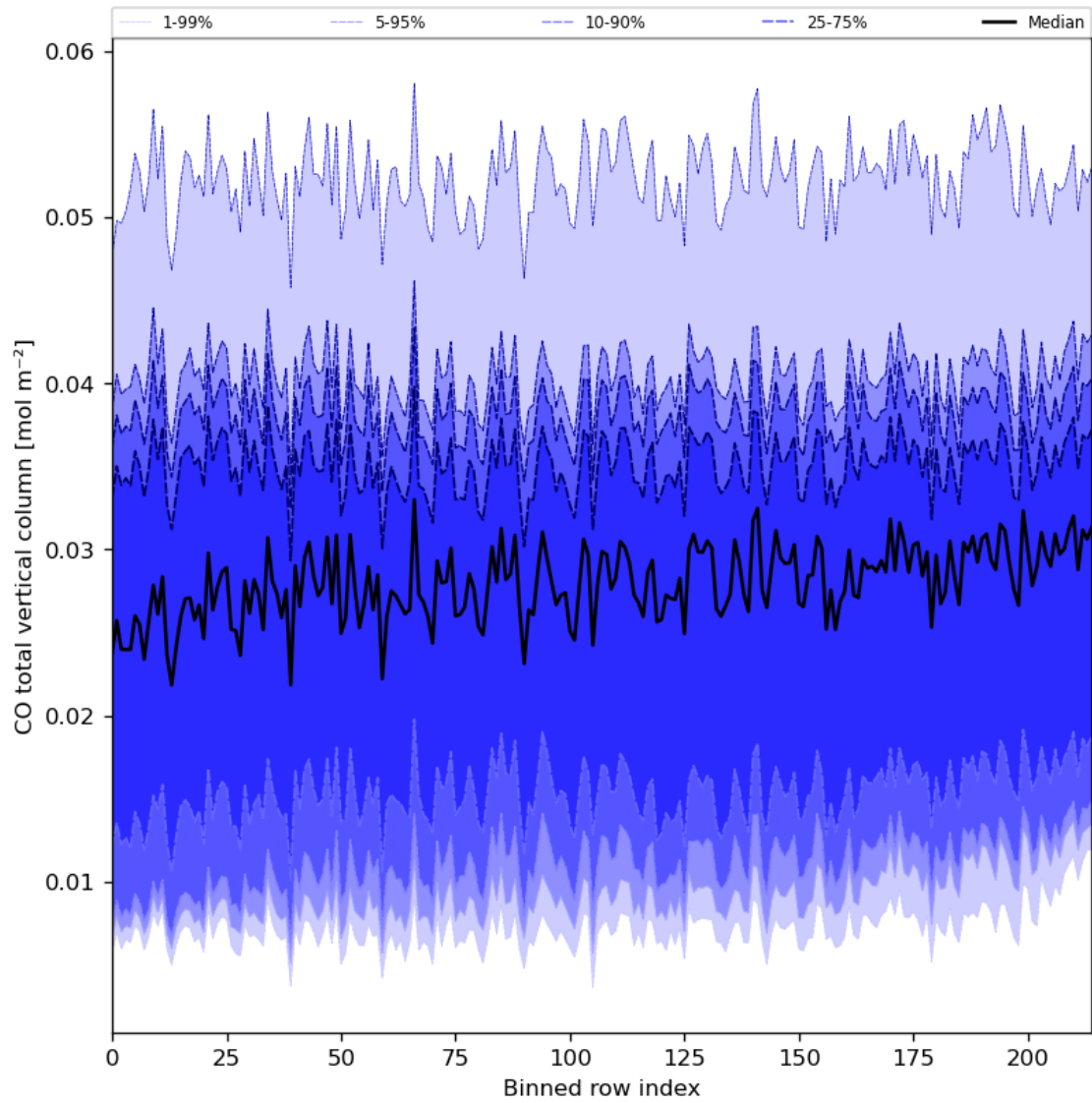
Figure 26: Along track statistics of “CO total vertical column” for 2024-03-04 to 2024-03-05
