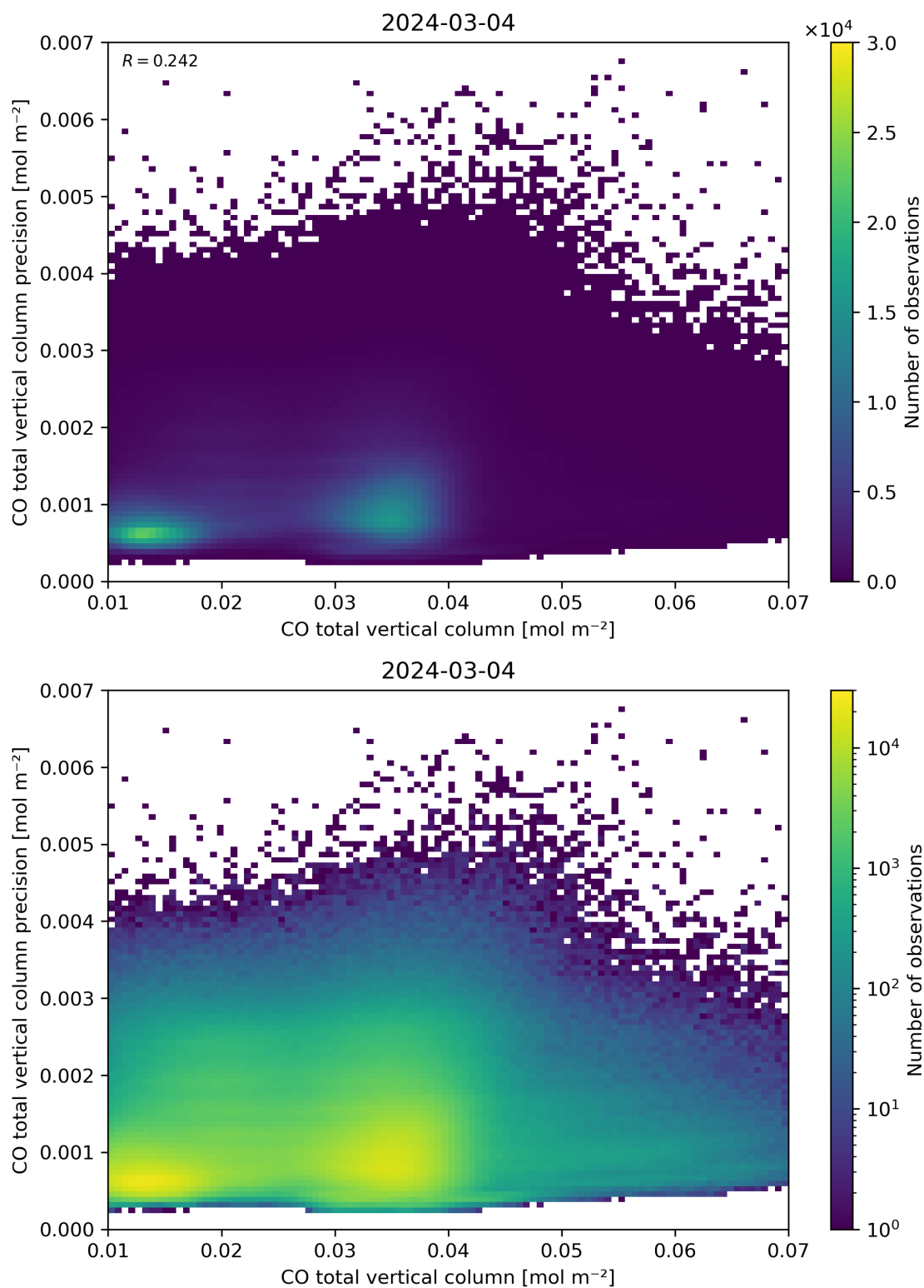
Figure 34: Scatter density plot of “CO total vertical column” against “CO total vertical column precision” for 2024-03-04 to 2024-03-05.
