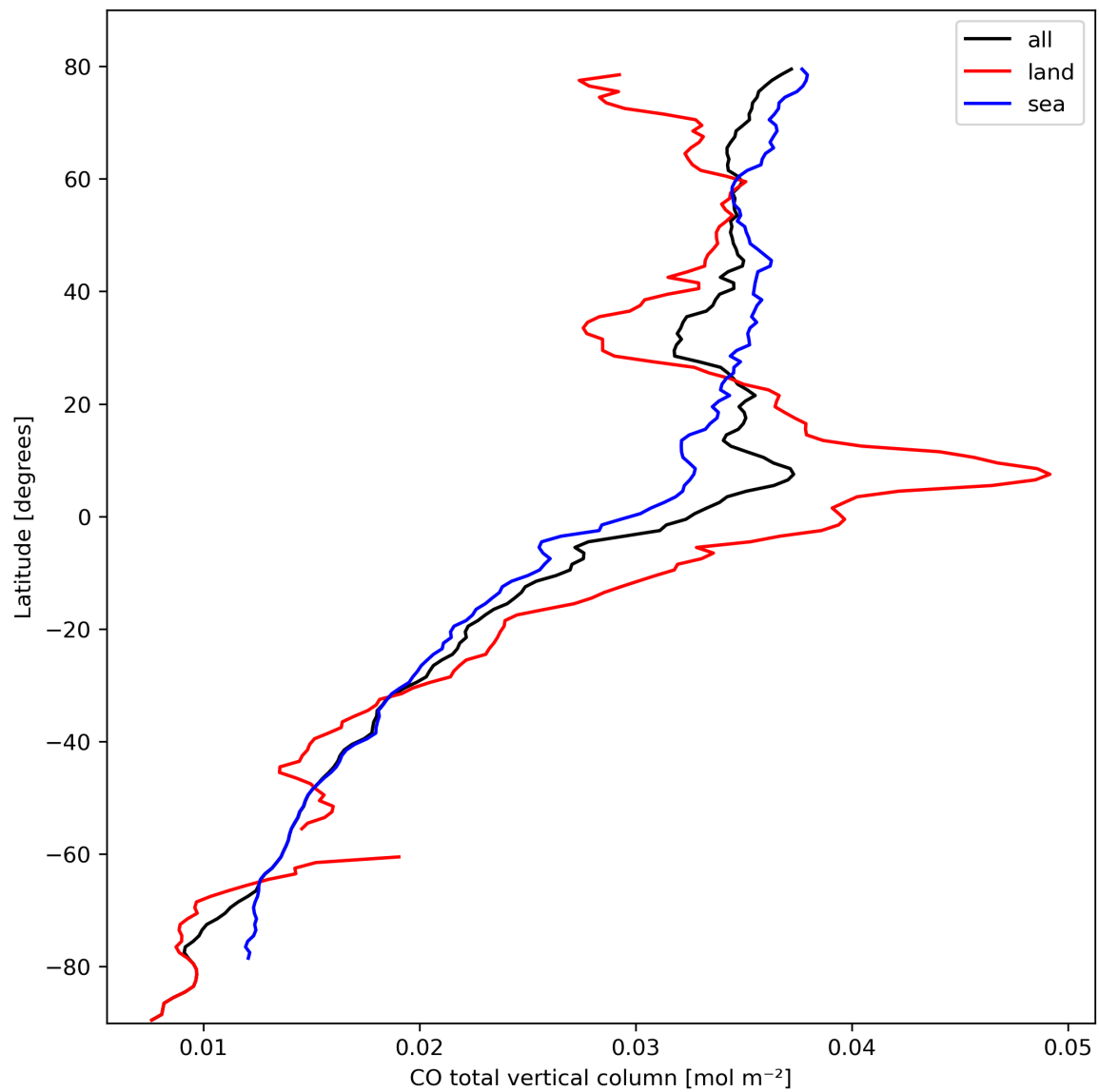
Figure 10: Zonal average of “CO total vertical column” for 2024-03-04 to 2024-03-05.
