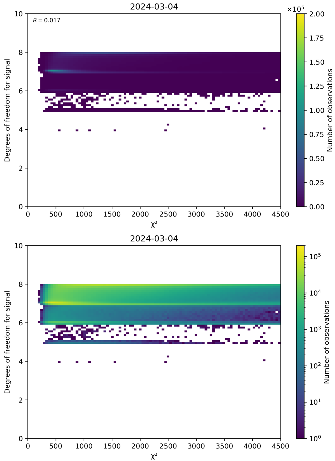
Figure 48: Scatter density plot of “ \chi^2 ” against “Degrees of freedom for signal” for 2024-03-04 to 2024-03-05.
