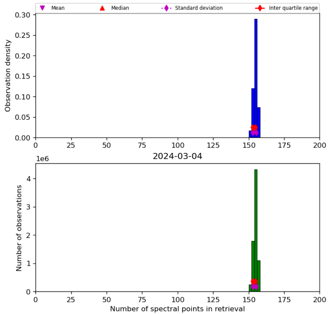
Figure 21: Histogram of “Number of spectral points in retrieval” for 2024-03-04 to 2024-03-05
