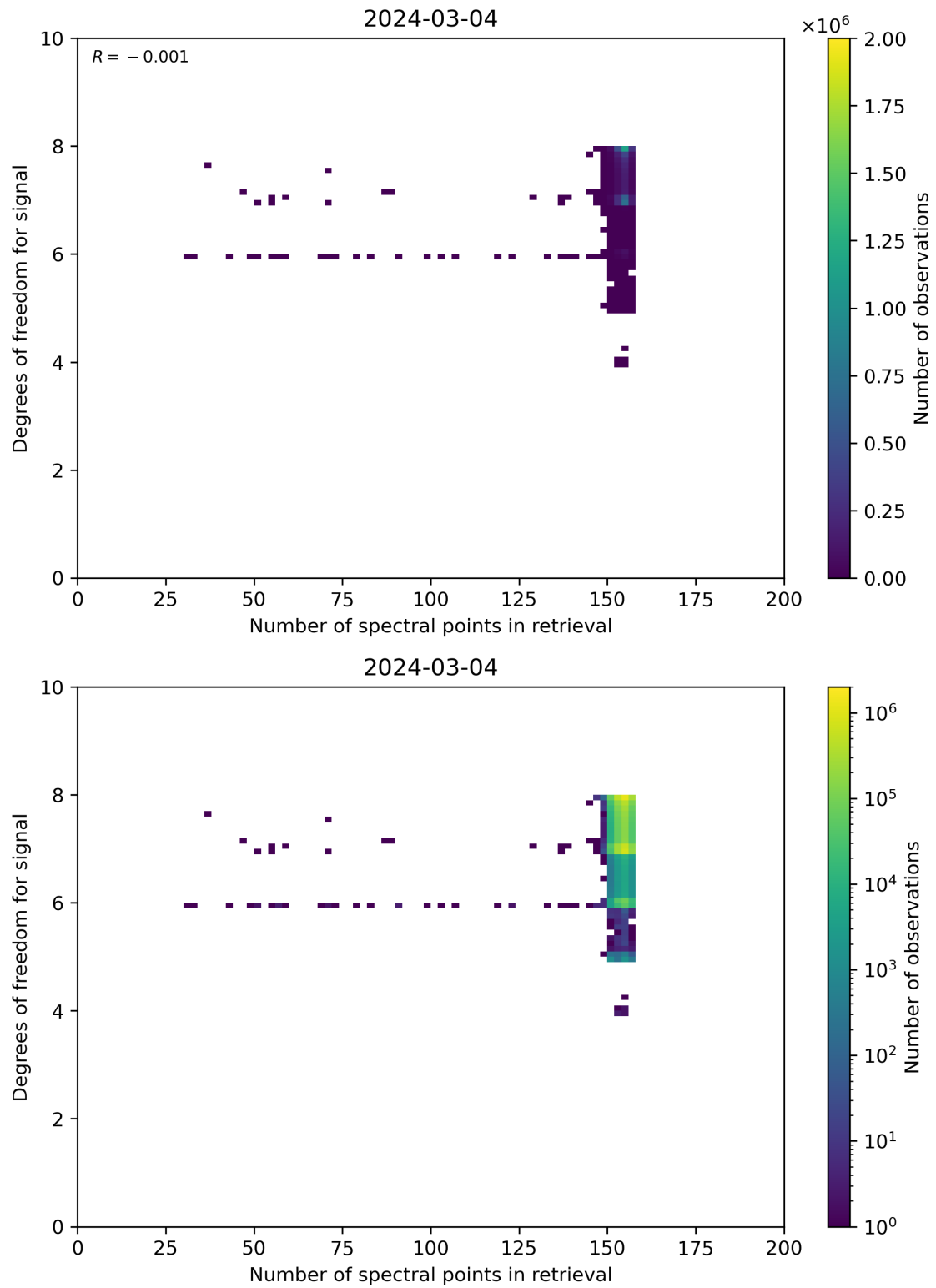
Figure 59: Scatter density plot of “Number of spectral points in retrieval” against “Degrees of freedom for signal” for 2024-03-04 to 2024-03-05.
