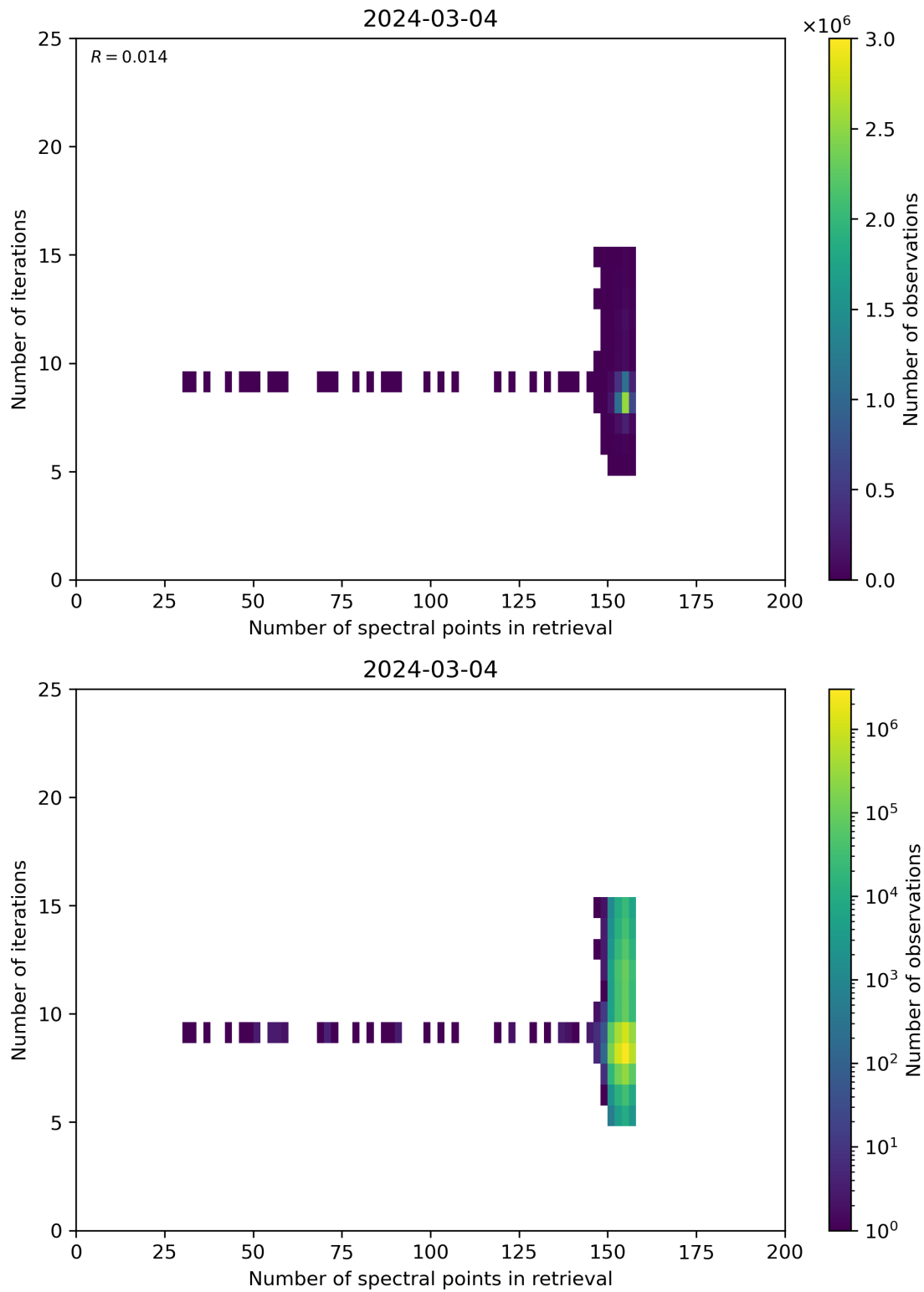
Figure 60: Scatter density plot of “Number of spectral points in retrieval” against “Number of iterations” for 2024-03-04 to 2024-03-05.
