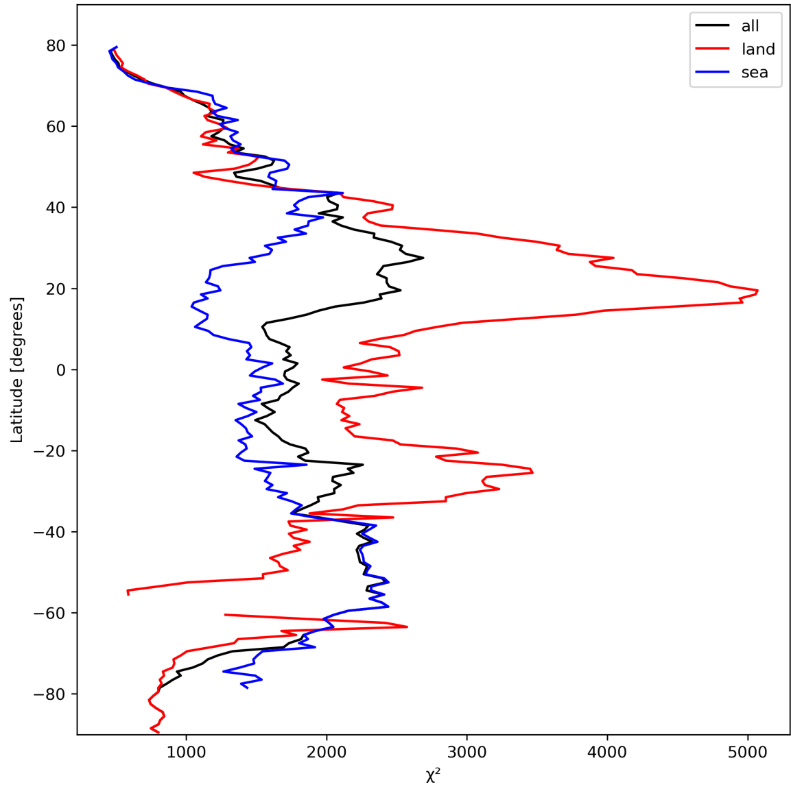
Figure 14: Zonal average of “ \chi^2 ” for 2024-03-04 to 2024-03-05.
