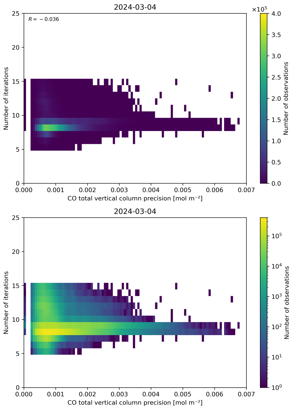
Figure 46: Scatter density plot of “CO total vertical column precision” against “Number of iterations” for 2024-03-04 to 2024-03-05.
