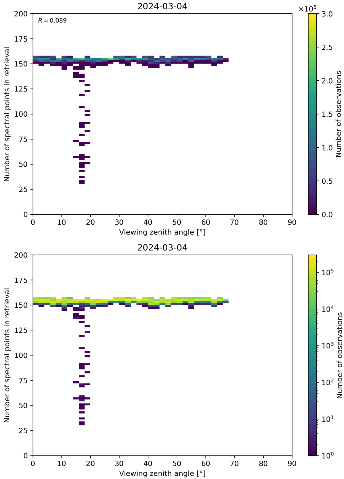
Figure 76: Scatter density plot of “Viewing zenith angle” against “Number of spectral points in retrieval” for 2024-03-04 to 2024-03-05.
