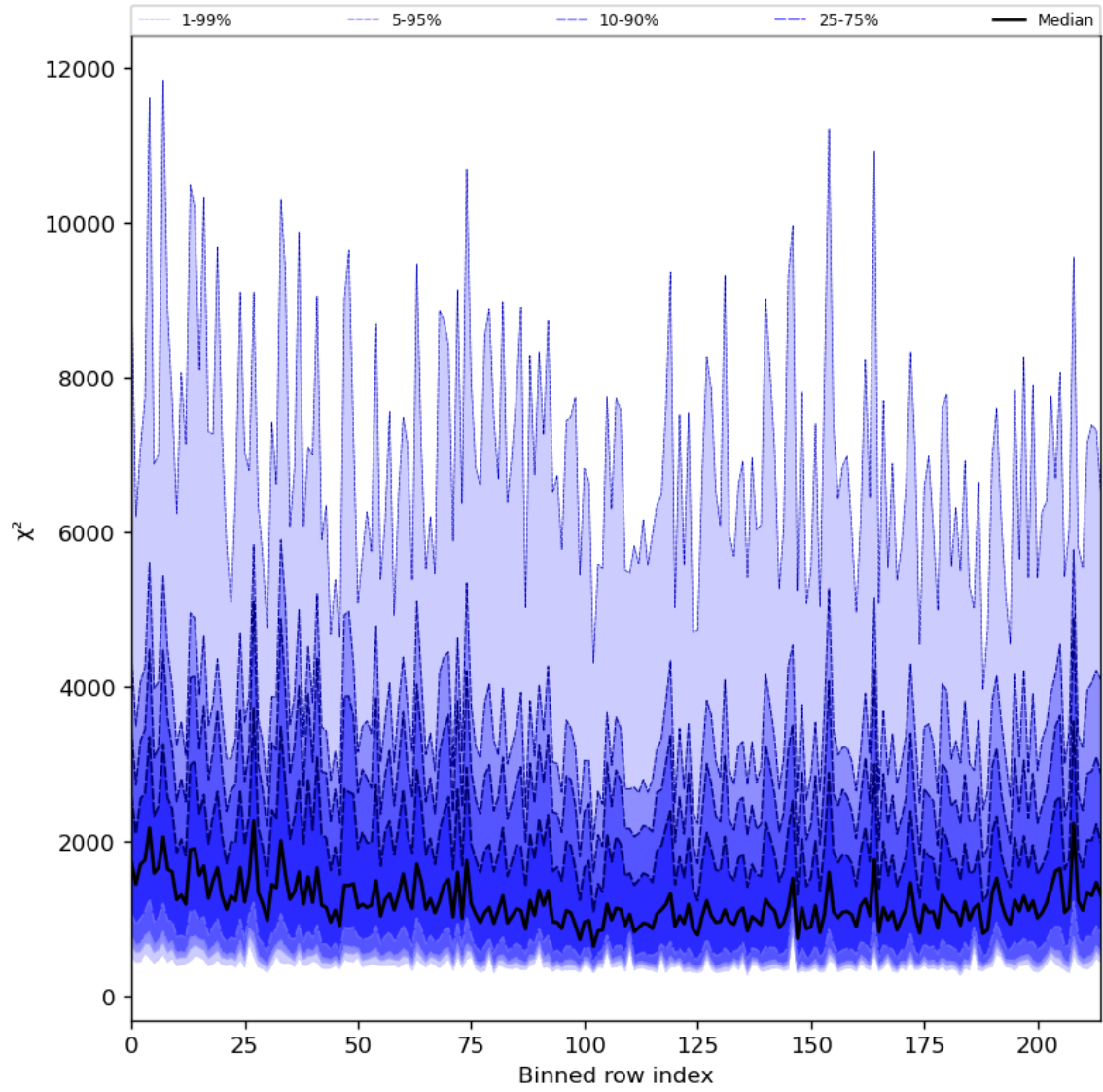
Figure 30: Along track statistics of “ \chi^2 ” for 2024-03-04 to 2024-03-05
