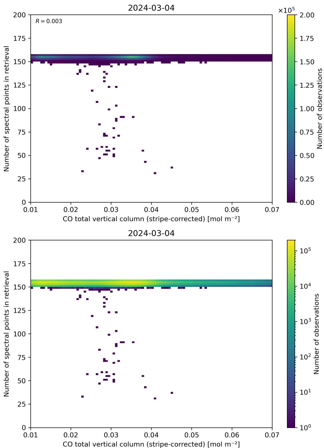
Figure 40: Scatter density plot of “CO total vertical column (stripe-corrected)” against “Number of spectral points in retrieval” for 2024-03-04 to 2024-03-05.
