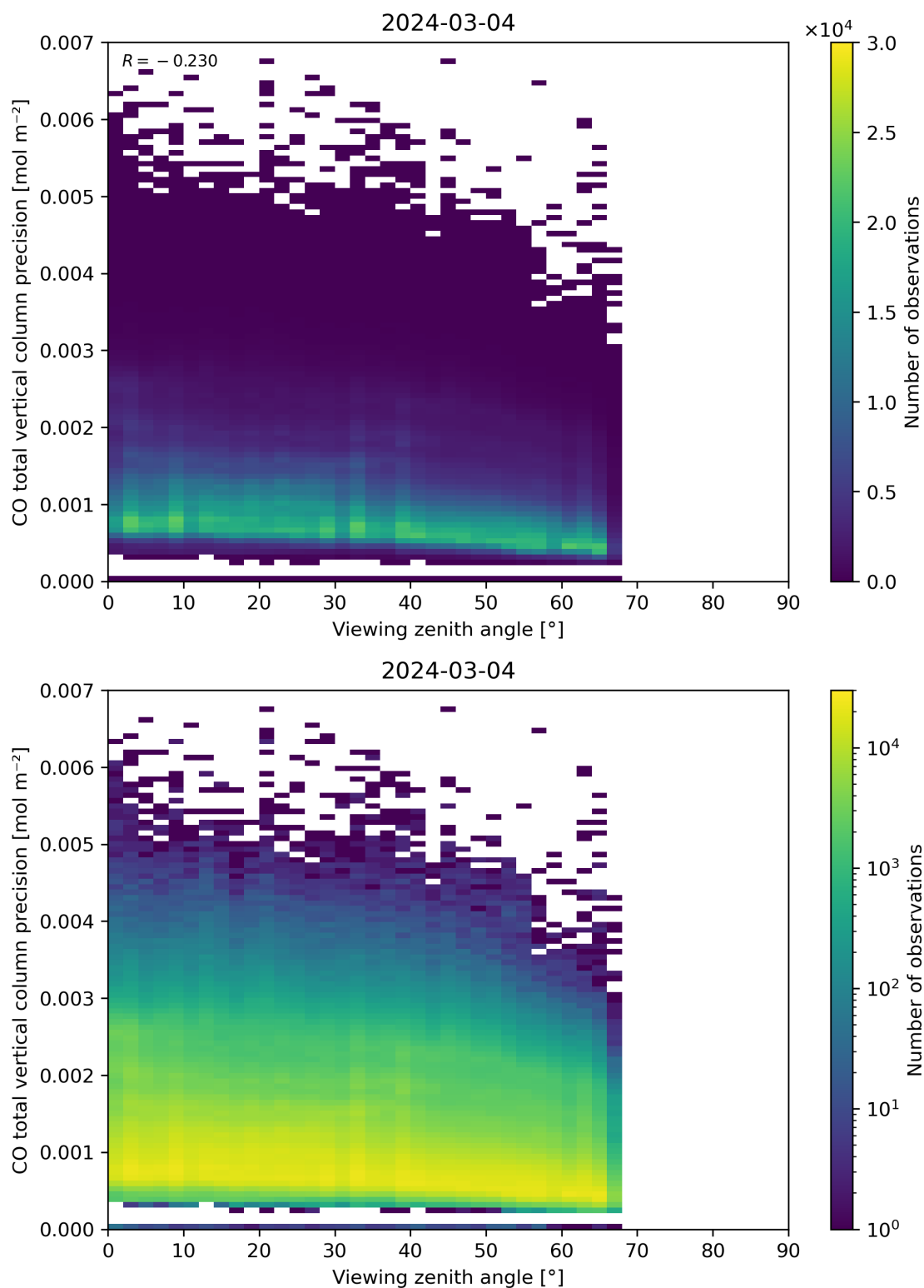
Figure 71: Scatter density plot of “Viewing zenith angle” against “CO total vertical column precision” for 2024-03-04 to 2024-03-05.
