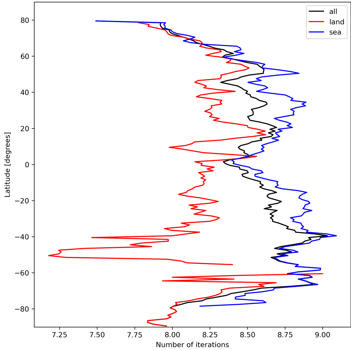
Figure 16: Zonal average of “Number of iterations” for 2024-03-04 to 2024-03-05.
