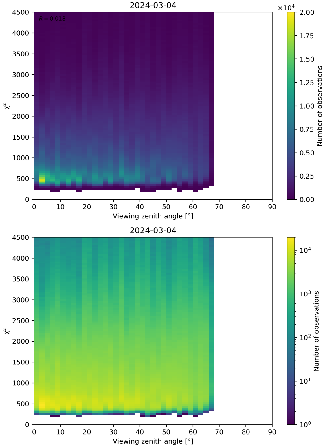
Figure 72: Scatter density plot of “Viewing zenith angle” against “ \chi^2 ” for 2024-03-04 to 2024-03-05.
