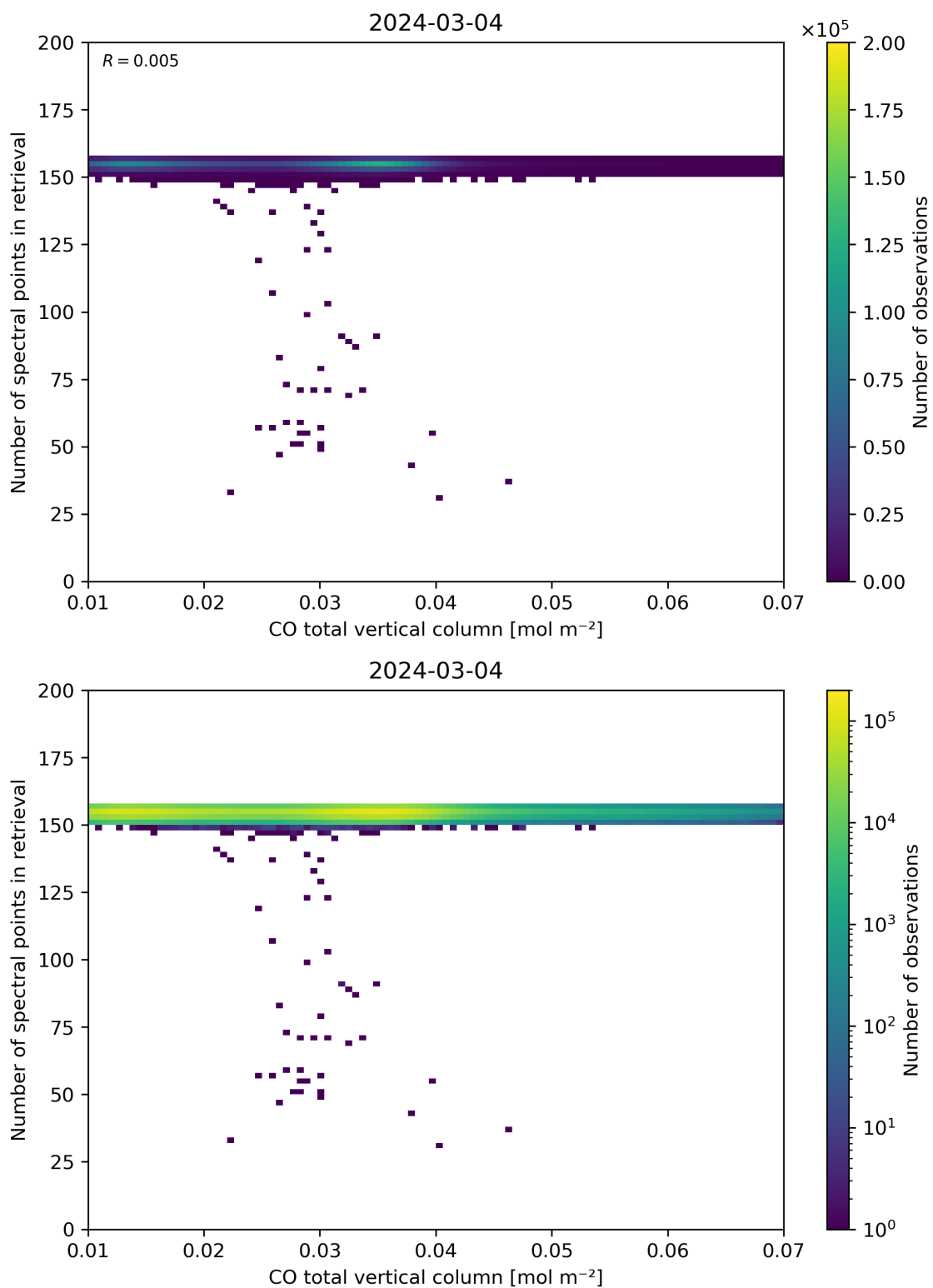
Figure 43: Scatter density plot of “CO total vertical column” against “Number of spectral points in retrieval” for 2024-03-04 to 2024-03-05.
