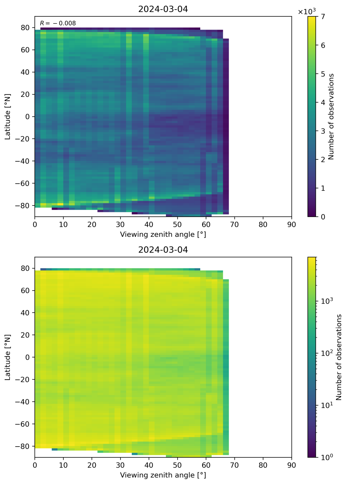
Figure 74: Scatter density plot of “Viewing zenith angle” against “Latitude” for 2024-03-04 to 2024-03-05.
