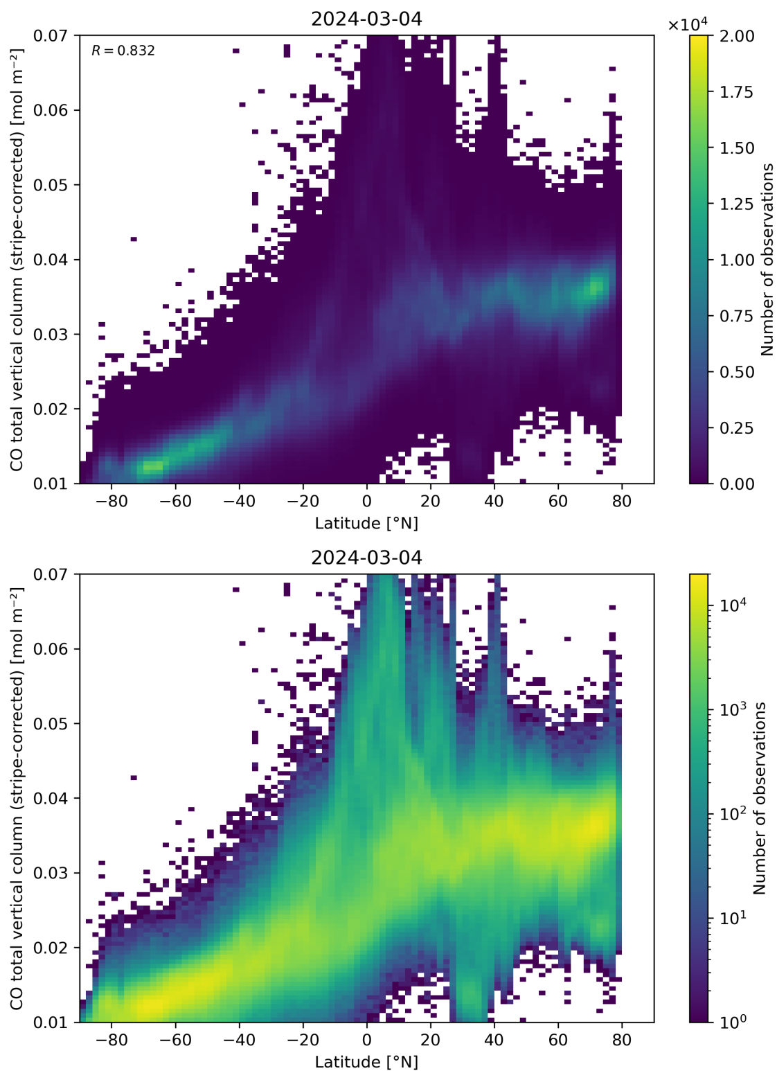
Figure 52: Scatter density plot of “Latitude” against “CO total vertical column (stripe-corrected)” for 2024-03-04 to 2024-03-05.
