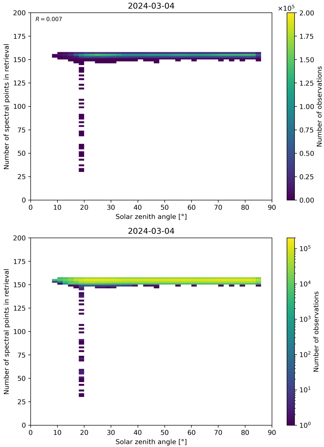
Figure 68: Scatter density plot of “Solar zenith angle” against “Number of spectral points in retrieval” for 2024-03-04 to 2024-03-05.
