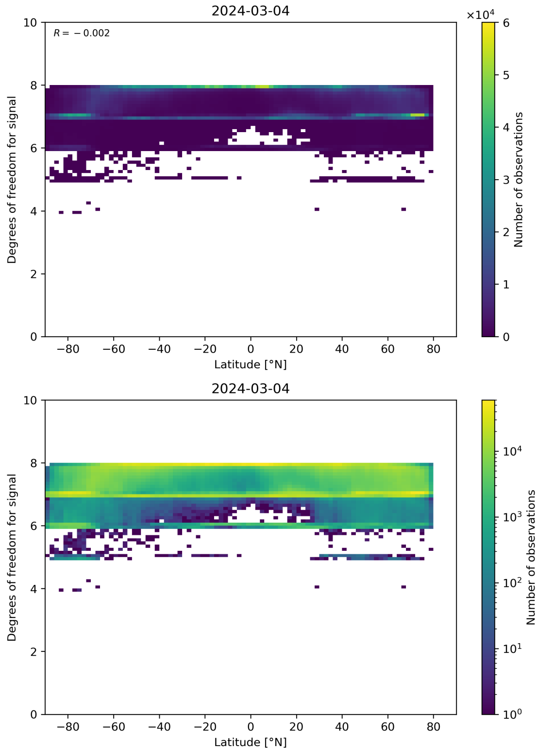
Figure 55: Scatter density plot of “Latitude” against “Degrees of freedom for signal” for 2024-03-04 to 2024-03-05.
