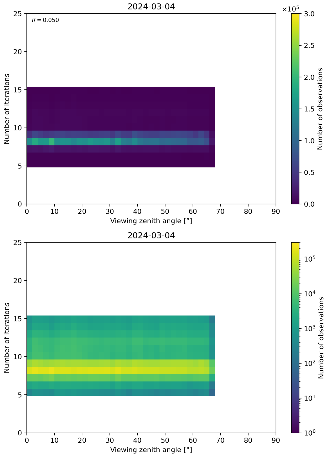
Figure 75: Scatter density plot of “Viewing zenith angle” against “Number of iterations” for 2024-03-04 to 2024-03-05.
