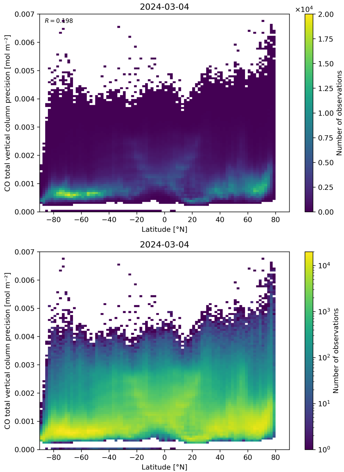
Figure 53: Scatter density plot of “Latitude” against “CO total vertical column precision” for 2024-03-04 to 2024-03-05.
