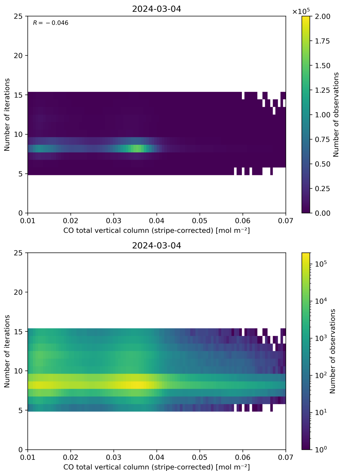
Figure 39: Scatter density plot of “CO total vertical column (stripe-corrected)” against “Number of iterations” for 2024-03-04 to 2024-03-05.
