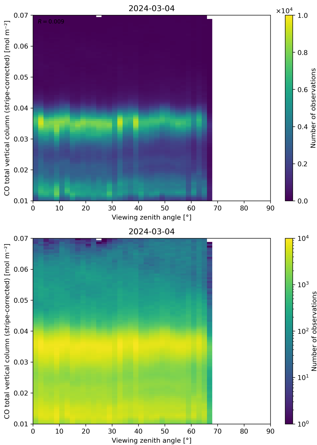
Figure 70: Scatter density plot of “Viewing zenith angle” against “CO total vertical column (stripe-corrected)” for 2024-03-04 to 2024-03-05.
