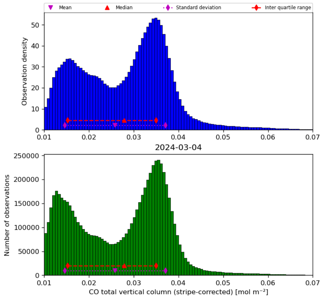
Figure 19: Histogram of “CO total vertical column (stripe-corrected)” for 2024-03-04 to 2024-03-05
