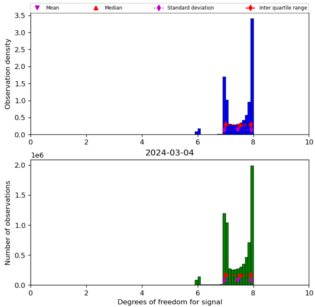
Figure 23: Histogram of “Degrees of freedom for signal” for 2024-03-04 to 2024-03-05
