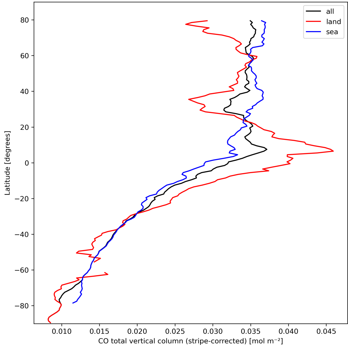
Figure 11: Zonal average of “CO total vertical column (stripe-corrected)” for 2024-03-04 to 2024-03-06.
