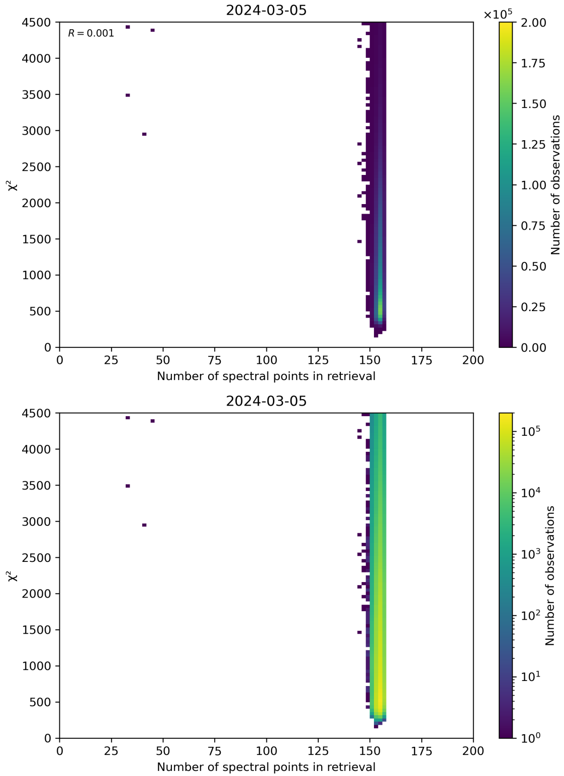
Figure 58: Scatter density plot of “Number of spectral points in retrieval” against “ \chi^2 ” for 2024-03-04 to 2024-03-06.
