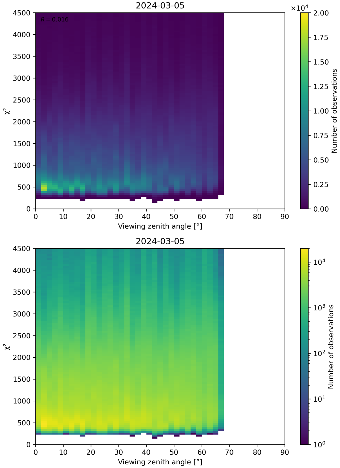
Figure 72: Scatter density plot of “Viewing zenith angle” against “ \chi^2 ” for 2024-03-04 to 2024-03-06.
