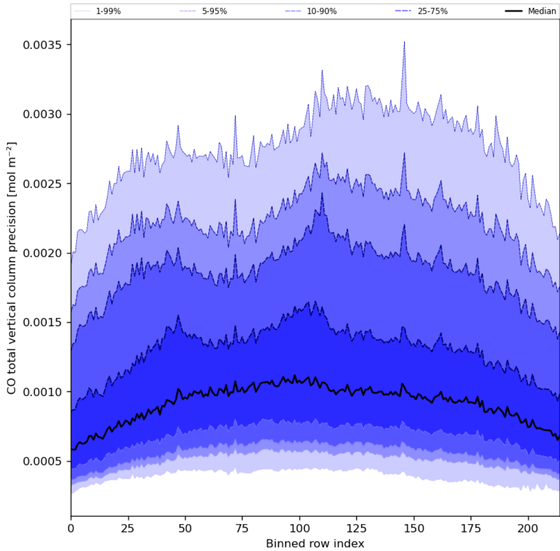
Figure 28: Along track statistics of “CO total vertical column precision” for 2024-03-04 to 2024-03-06
