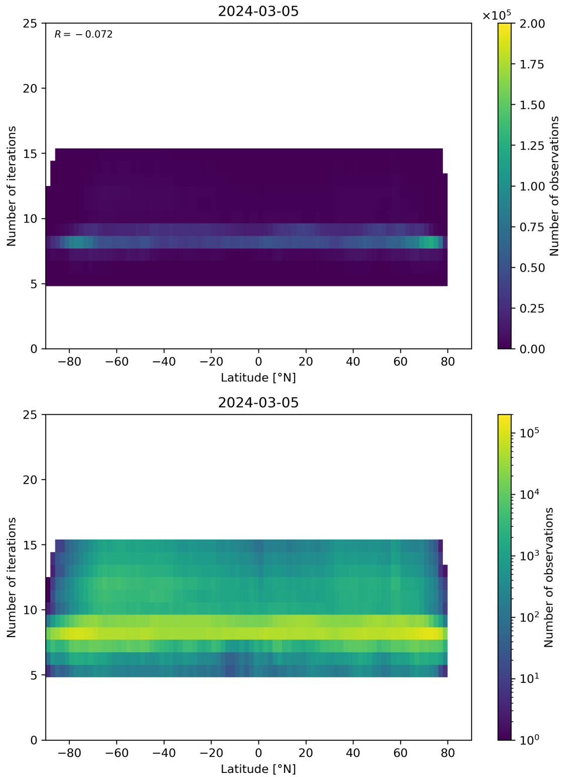
Figure 56: Scatter density plot of “Latitude” against “Number of iterations” for 2024-03-04 to 2024-03-06.
