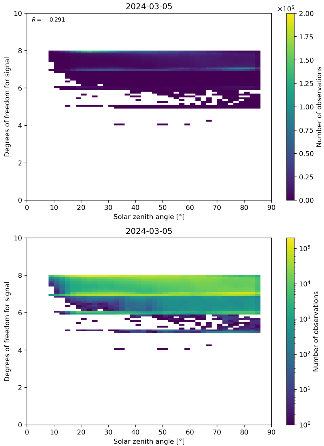
Figure 65: Scatter density plot of “Solar zenith angle” against “Degrees of freedom for signal” for 2024-03-04 to 2024-03-06.
