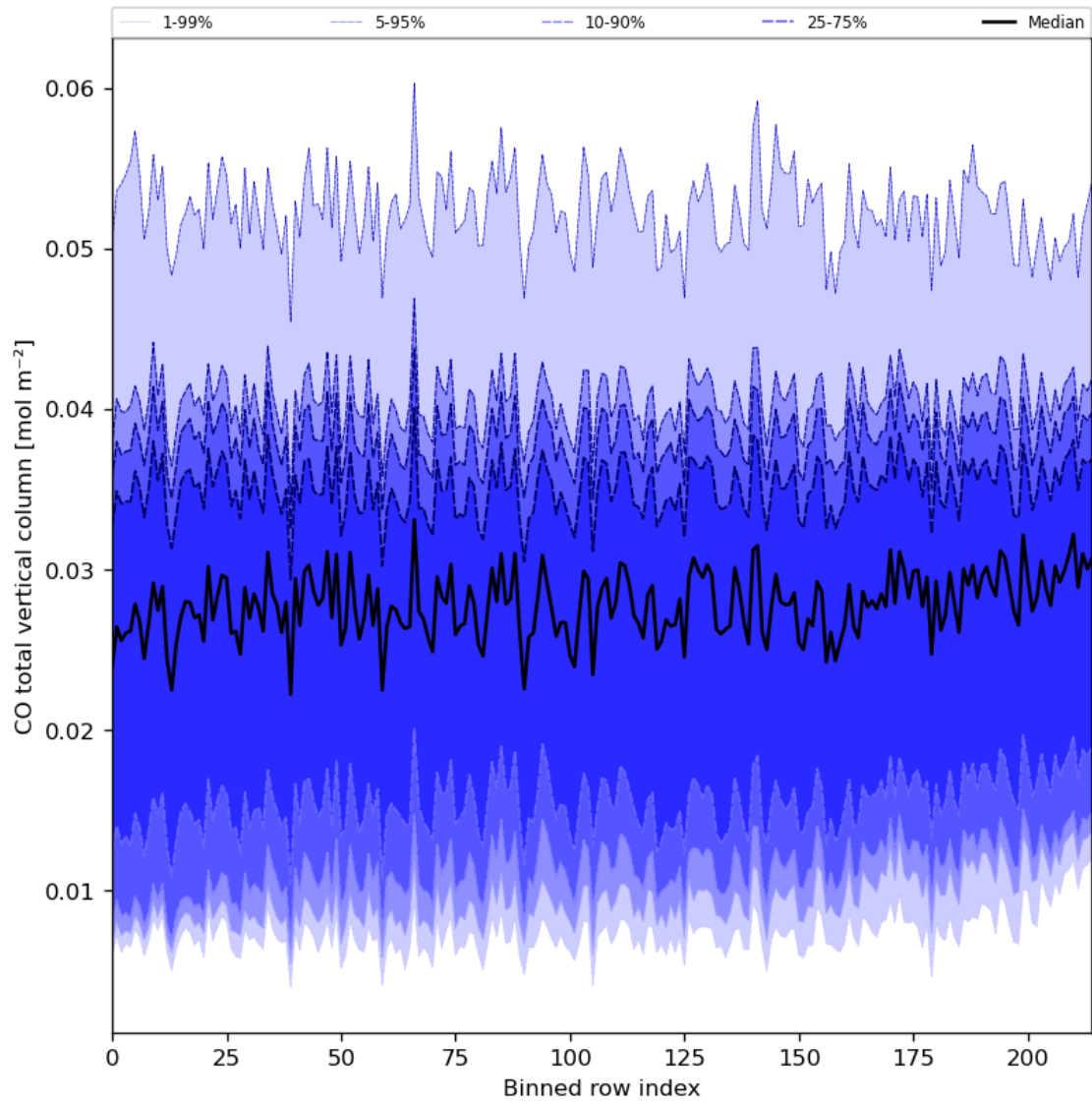
Figure 26: Along track statistics of “CO total vertical column” for 2024-03-04 to 2024-03-06
