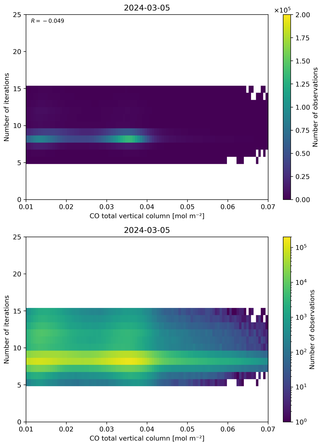
Figure 42: Scatter density plot of “CO total vertical column” against “Number of iterations” for 2024-03-04 to 2024-03-06.
