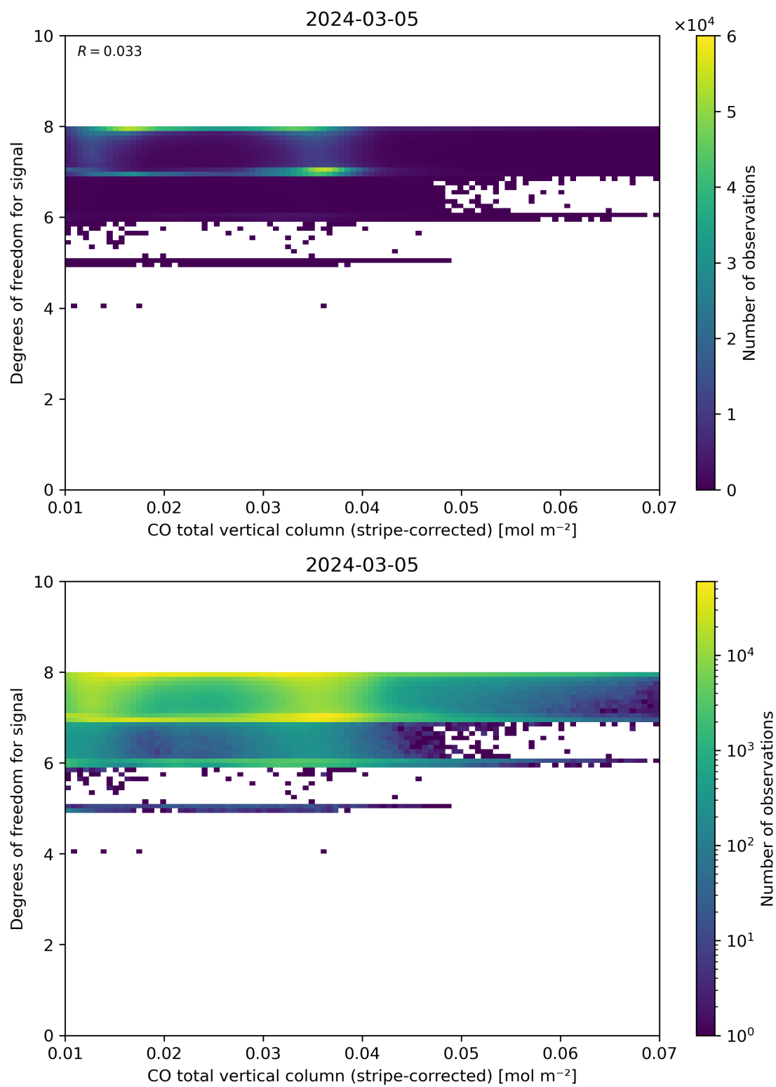
Figure 38: Scatter density plot of “CO total vertical column (stripe-corrected)” against “Degrees of freedom for signal” for 2024-03-04 to 2024-03-06.
