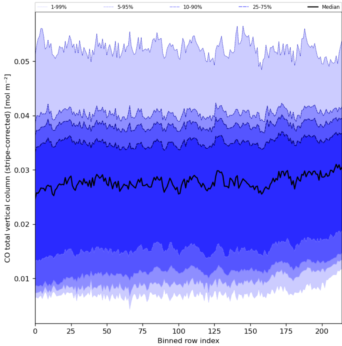
Figure 27: Along track statistics of “CO total vertical column (stripe-corrected)” for 2024-03-04 to 2024-03-06
