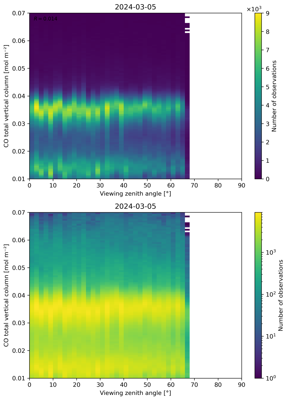
Figure 69: Scatter density plot of “Viewing zenith angle” against “CO total vertical column” for 2024-03-04 to 2024-03-06.
