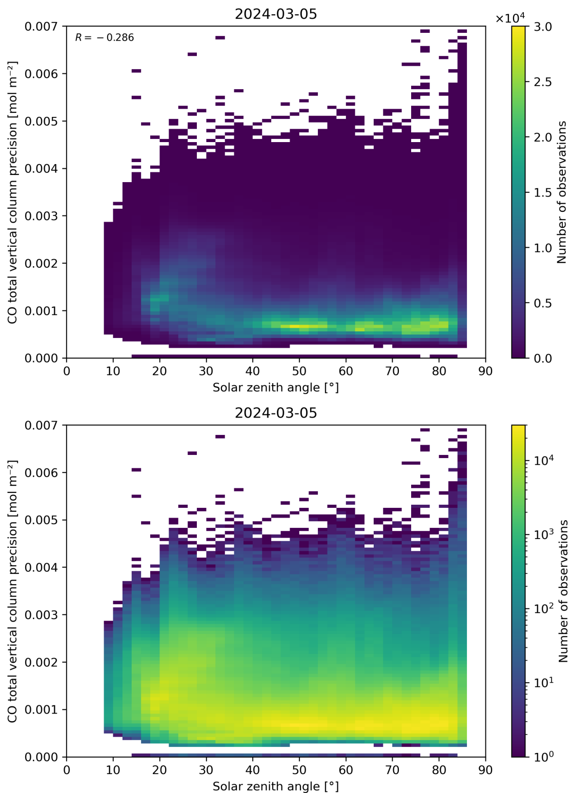
Figure 63: Scatter density plot of “Solar zenith angle” against “CO total vertical column precision” for 2024-03-04 to 2024-03-06.
