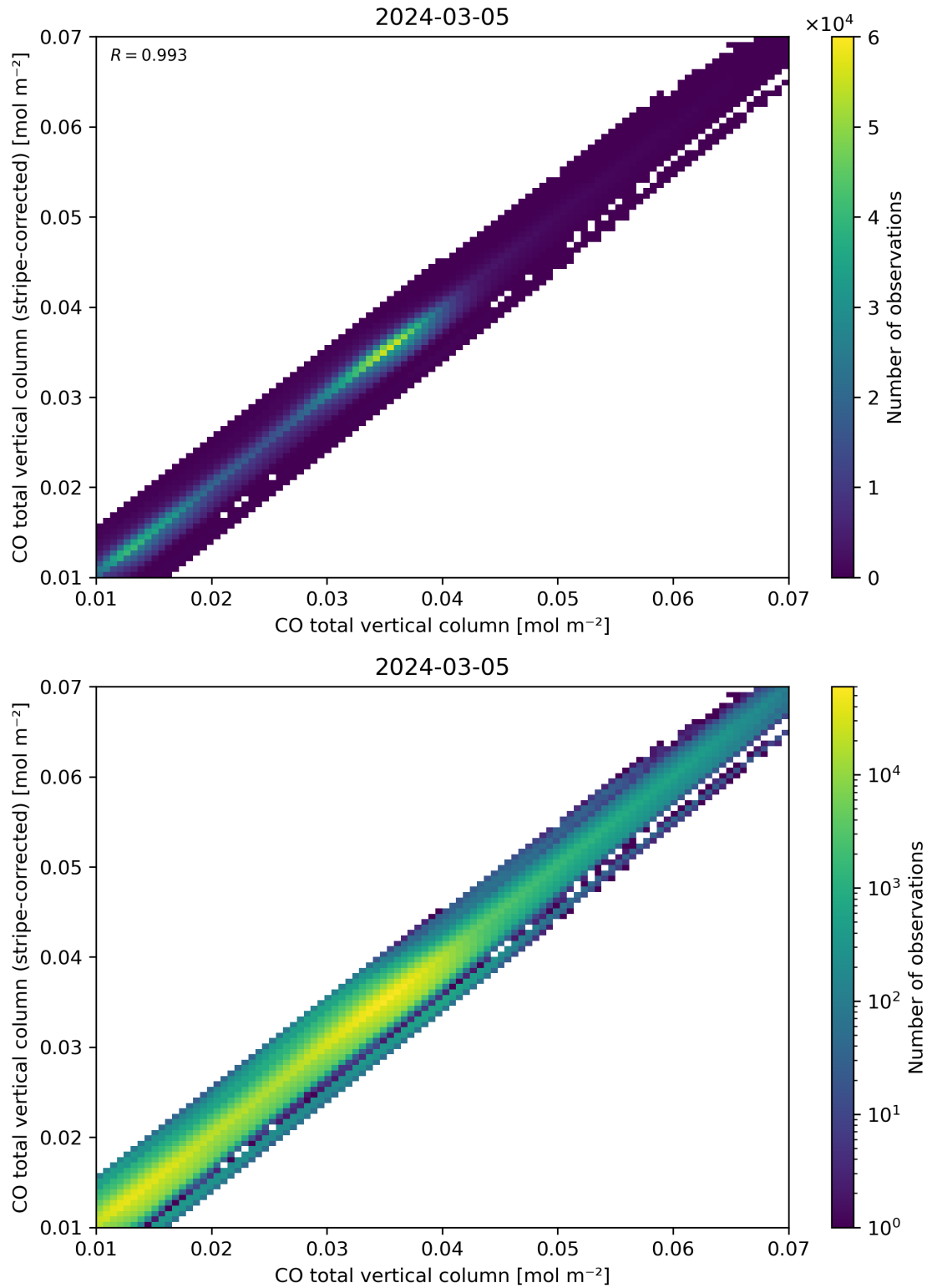
Figure 33: Scatter density plot of “CO total vertical column” against “CO total vertical column (stripe-corrected)” for 2024-03-04 to 2024-03-06.
