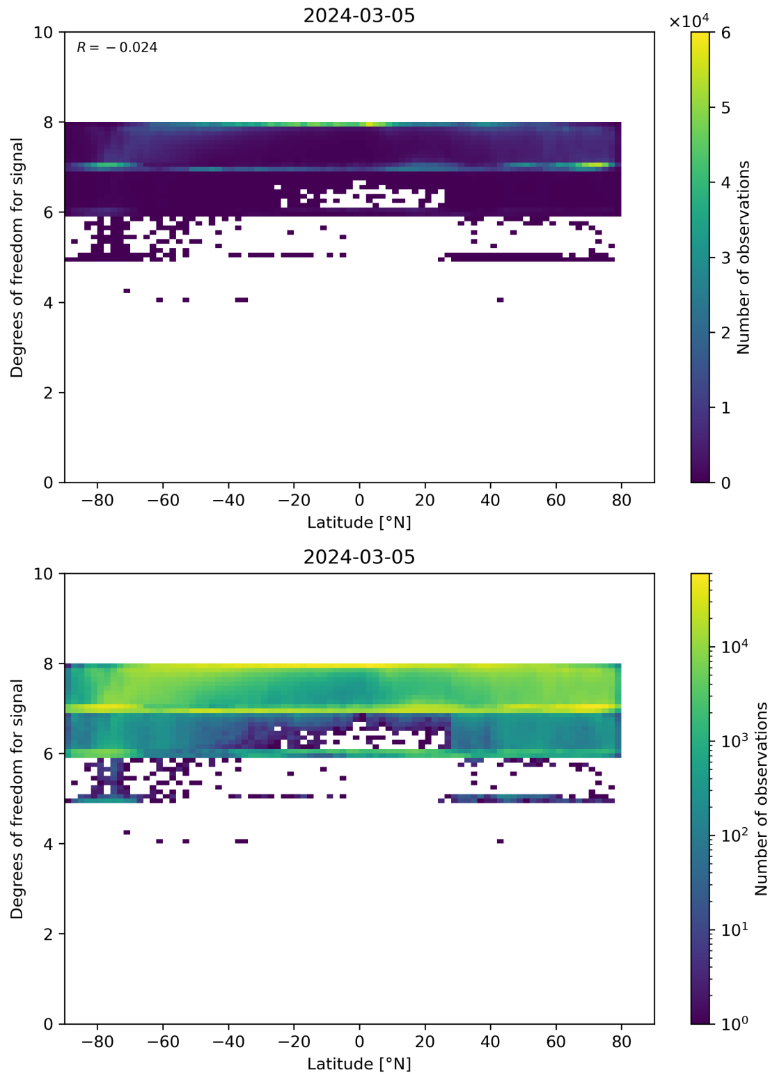
Figure 55: Scatter density plot of “Latitude” against “Degrees of freedom for signal” for 2024-03-04 to 2024-03-06.
