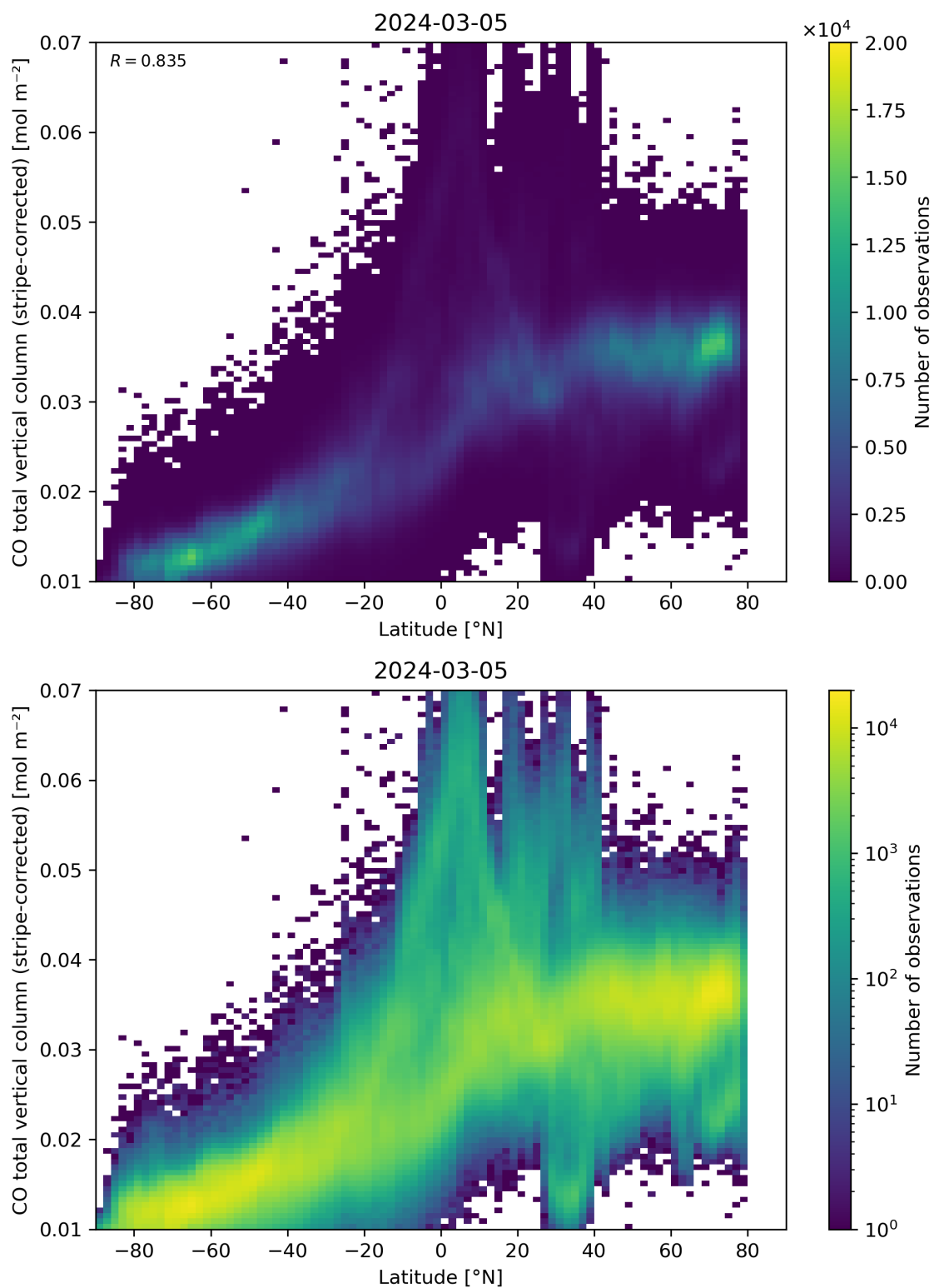
Figure 52: Scatter density plot of “Latitude” against “CO total vertical column (stripe-corrected)” for 2024-03-04 to 2024-03-06.
