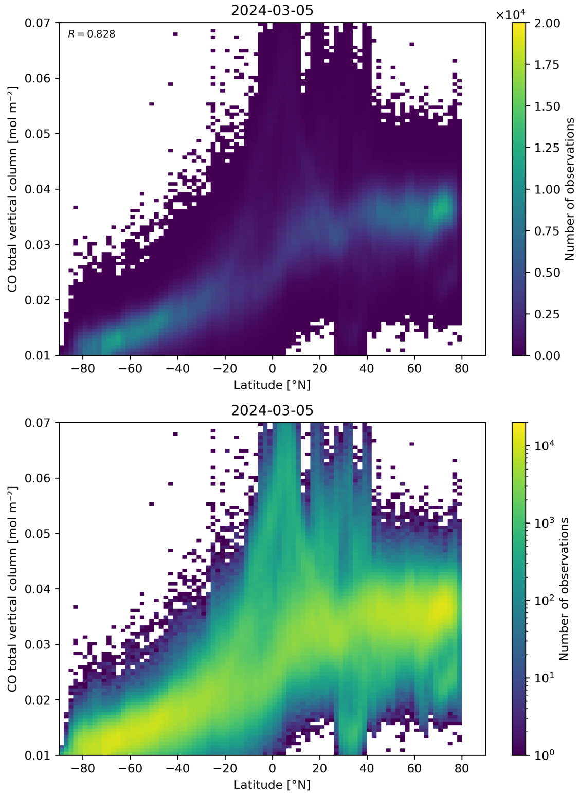
Figure 51: Scatter density plot of “Latitude” against “CO total vertical column” for 2024-03-04 to 2024-03-06.
