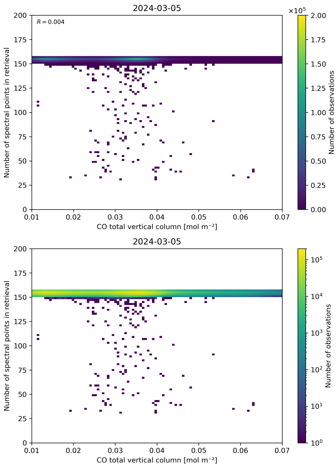
Figure 43: Scatter density plot of “CO total vertical column” against “Number of spectral points in retrieval” for 2024-03-04 to 2024-03-06.
