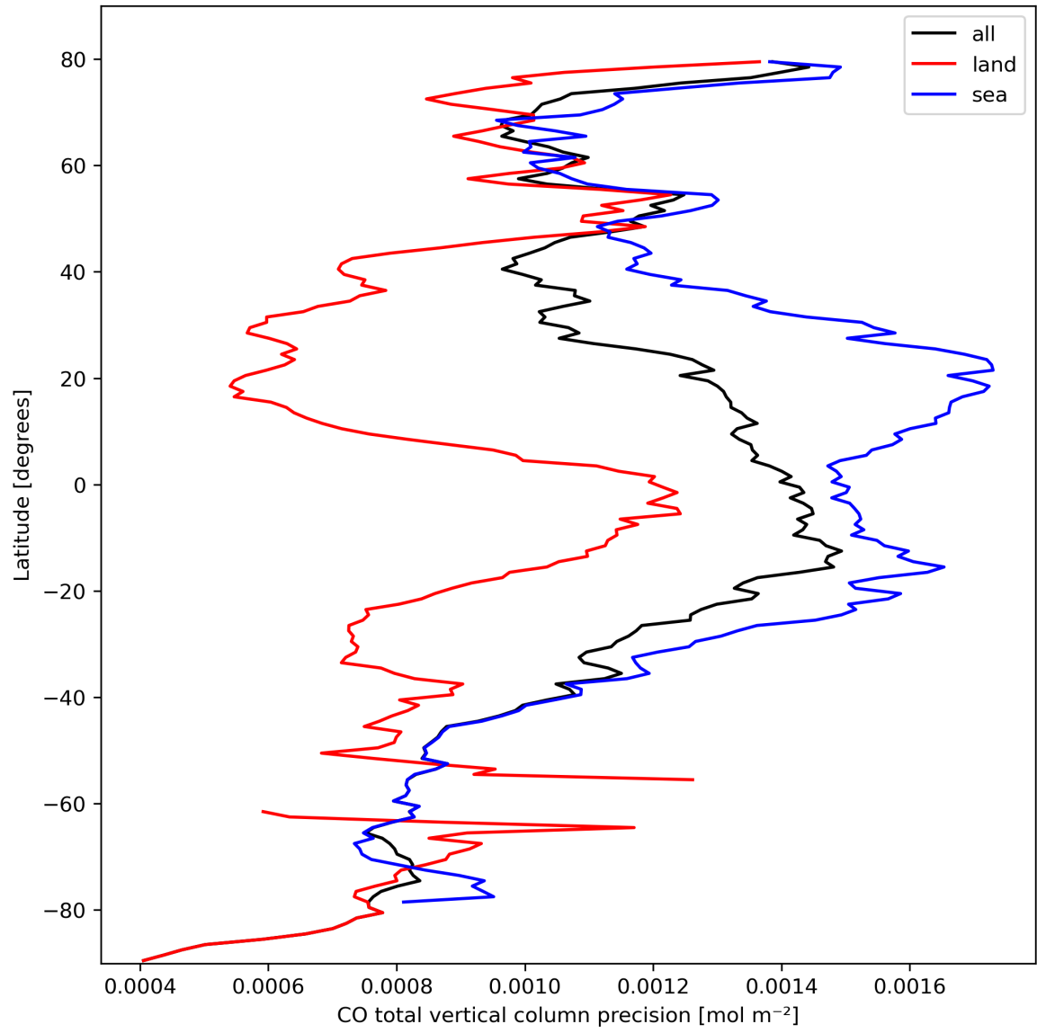
Figure 12: Zonal average of “CO total vertical column precision” for 2024-03-04 to 2024-03-06.
