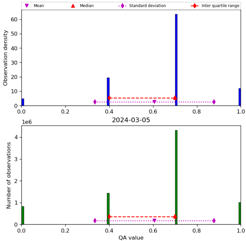
Figure 17: Histogram of “QA value” for 2024-03-04 to 2024-03-06
