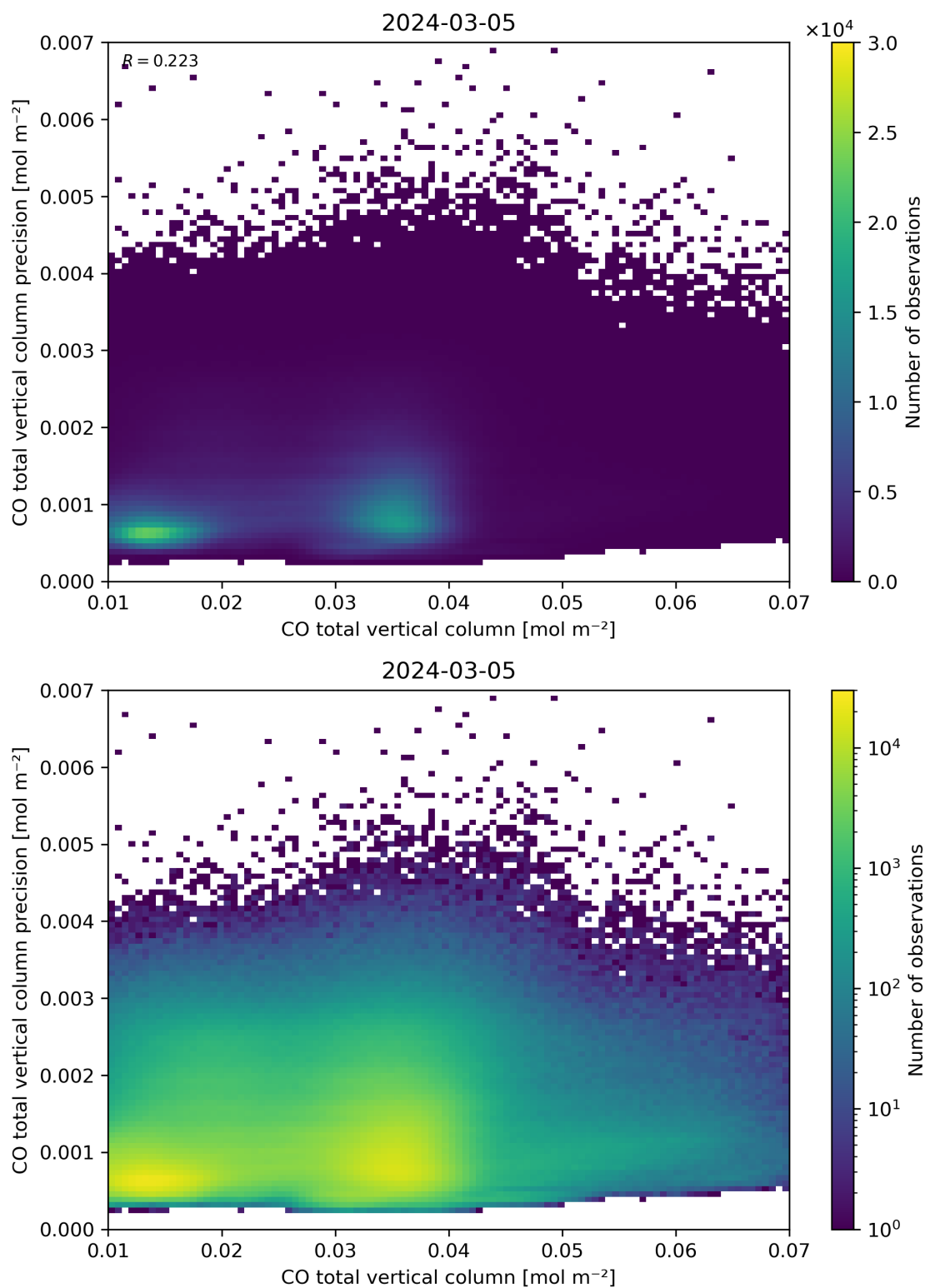
Figure 34: Scatter density plot of “CO total vertical column” against “CO total vertical column precision” for 2024-03-04 to 2024-03-06.
