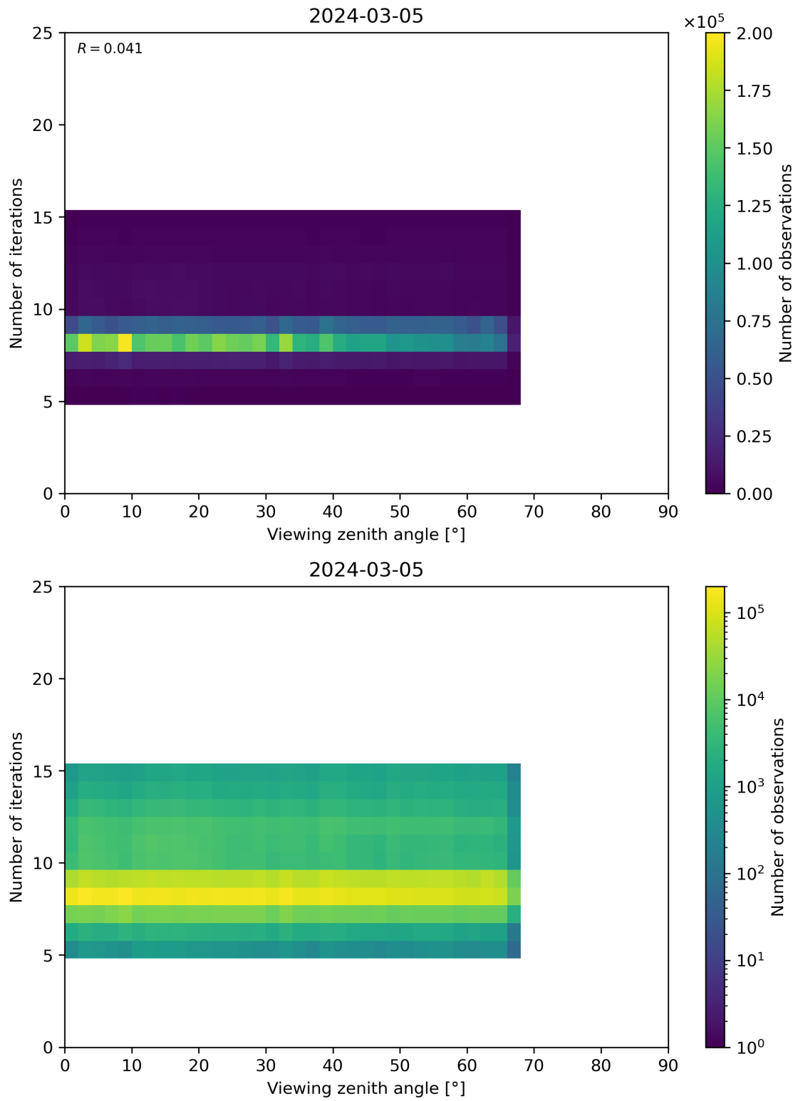
Figure 75: Scatter density plot of “Viewing zenith angle” against “Number of iterations” for 2024-03-04 to 2024-03-06.
