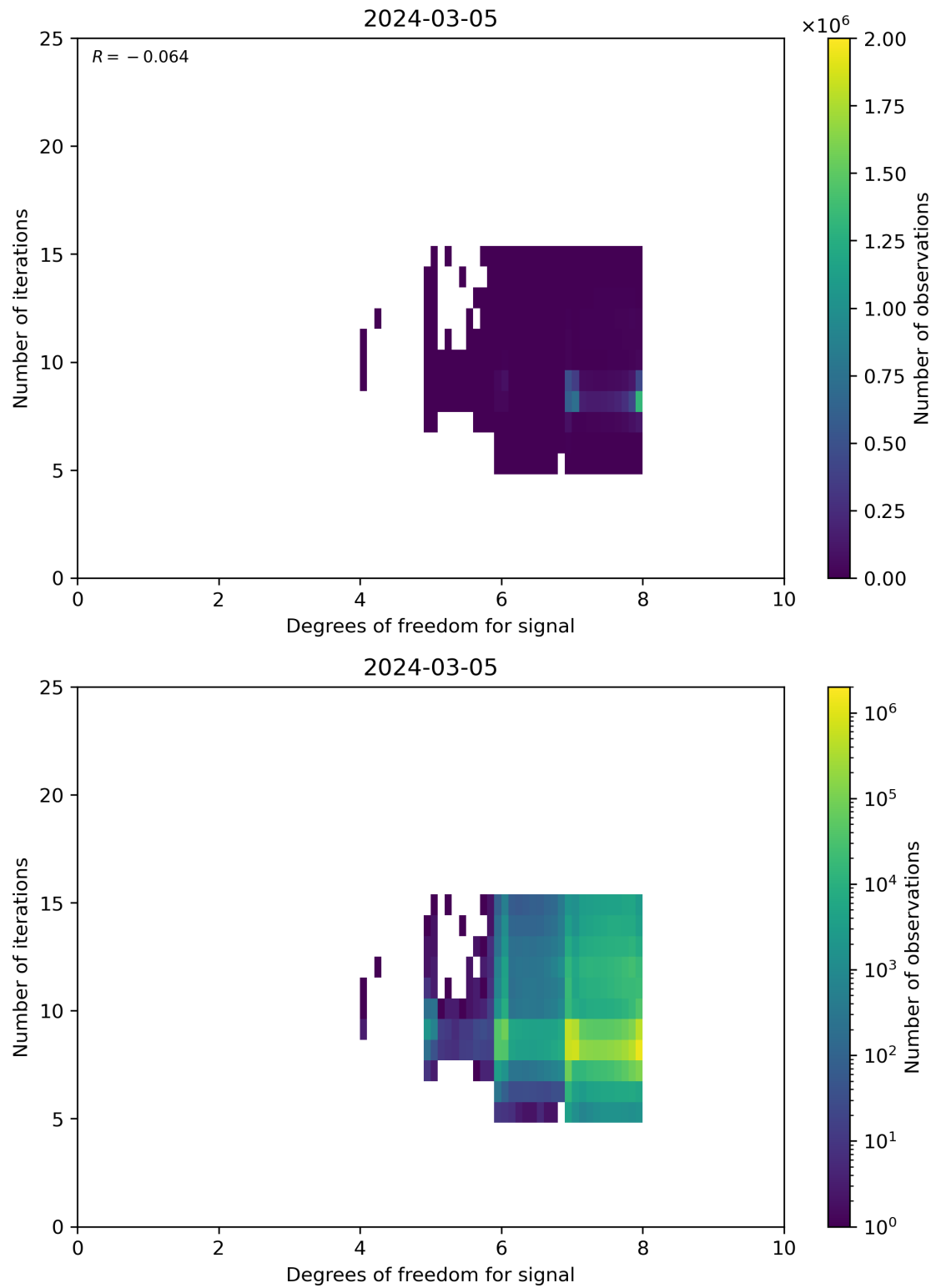
Figure 50: Scatter density plot of “Degrees of freedom for signal” against “Number of iterations” for 2024-03-04 to 2024-03-06.
