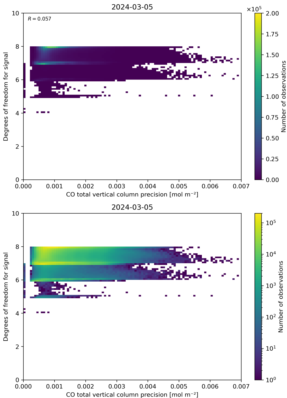
Figure 45: Scatter density plot of “CO total vertical column precision” against “Degrees of freedom for signal” for 2024-03-04 to 2024-03-06.
