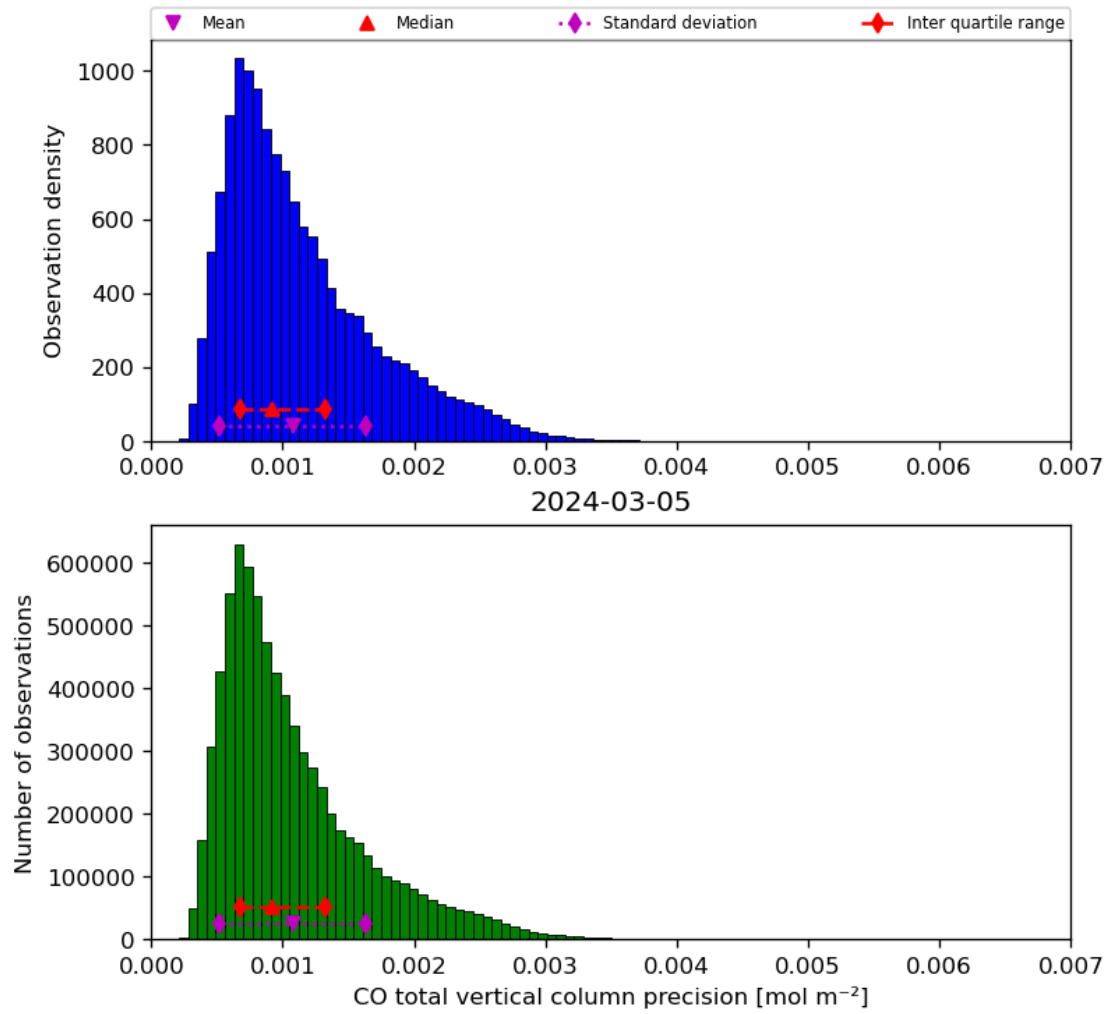
Figure 20: Histogram of “CO total vertical column precision” for 2024-03-04 to 2024-03-06
