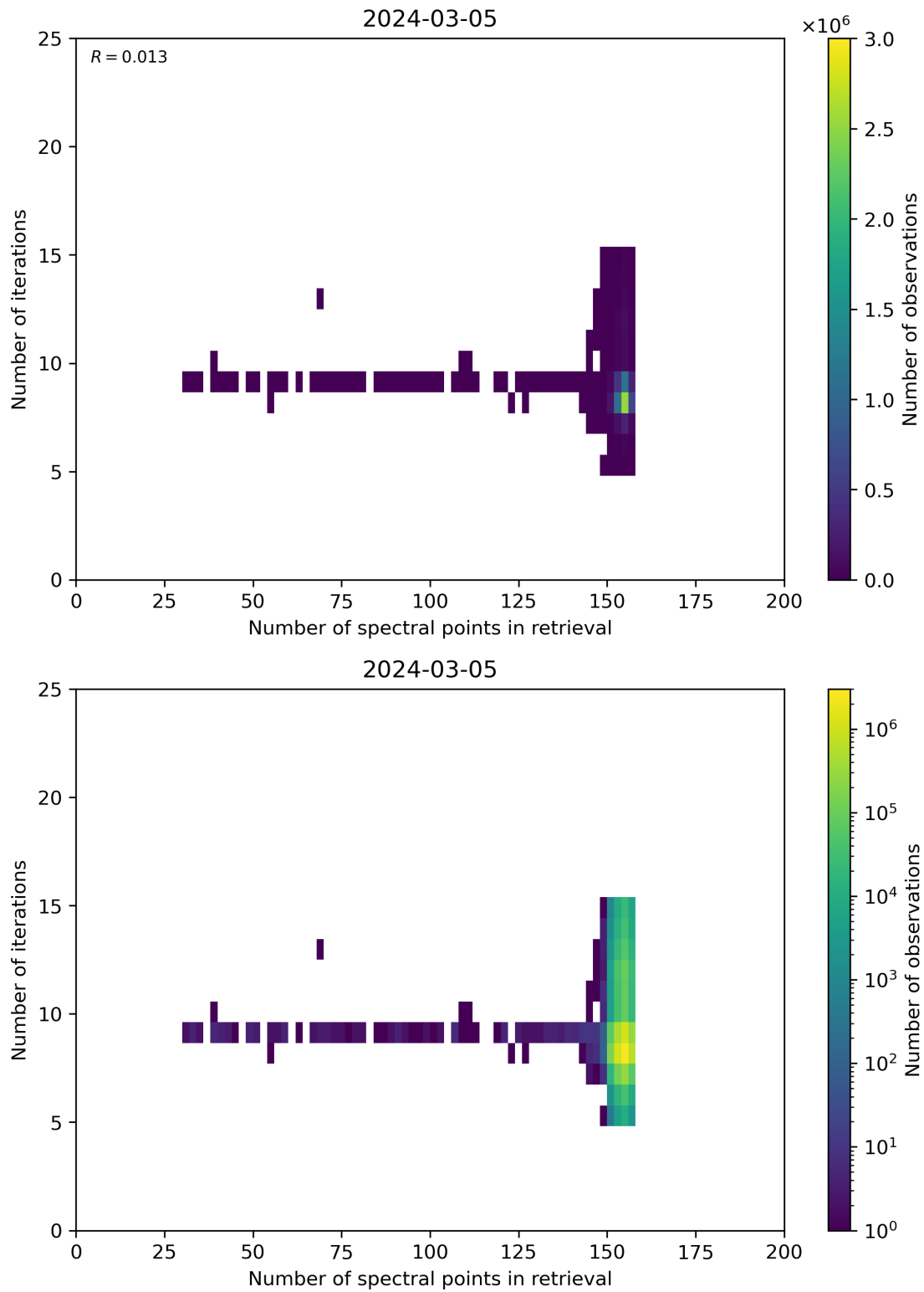
Figure 60: Scatter density plot of “Number of spectral points in retrieval” against “Number of iterations” for 2024-03-04 to 2024-03-06.
