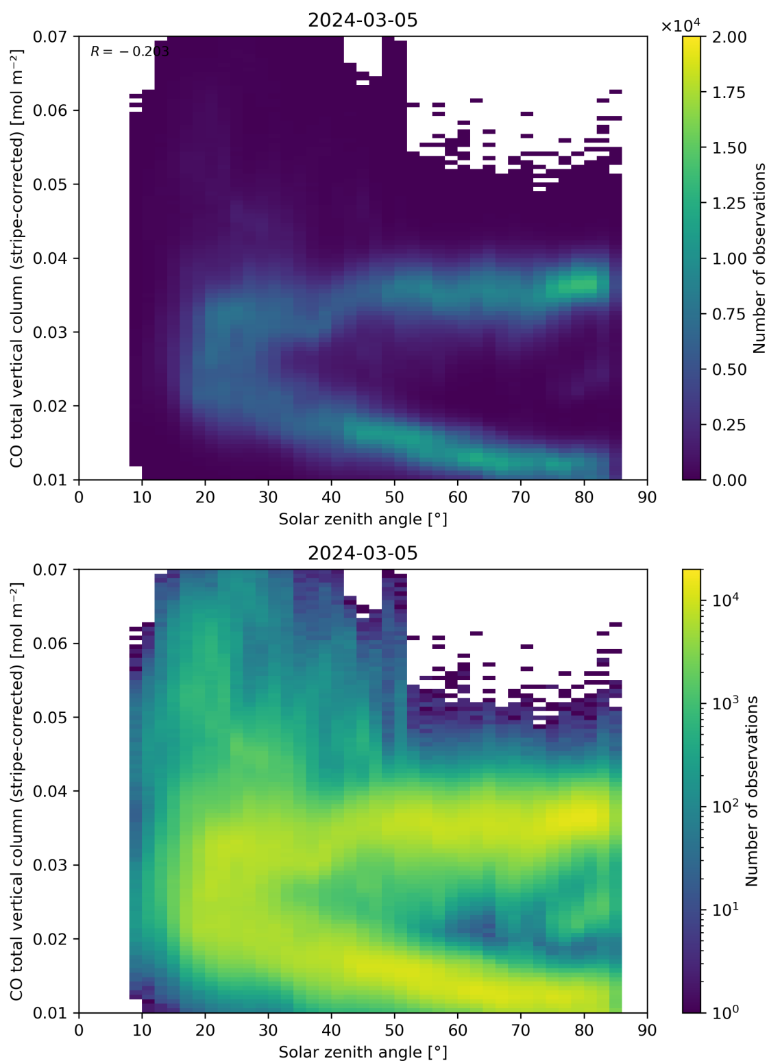
Figure 62: Scatter density plot of “Solar zenith angle” against “CO total vertical column (stripe-corrected)” for 2024-03-04 to 2024-03-06.
