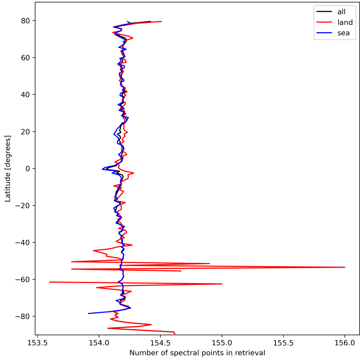
Figure 13: Zonal average of “Number of spectral points in retrieval” for 2024-03-04 to 2024-03-06.
