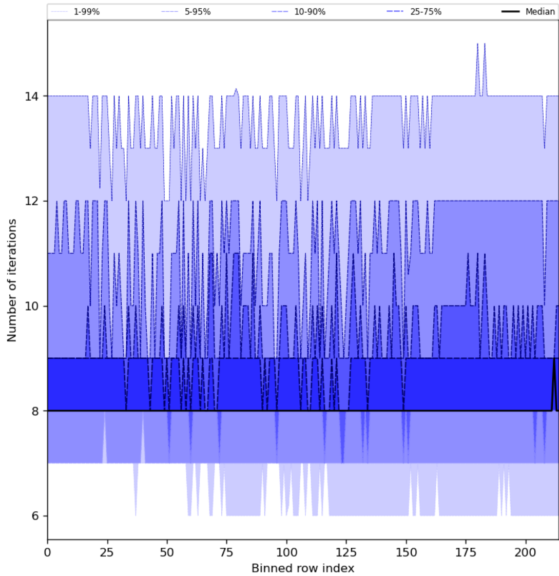
Figure 32: Along track statistics of “Number of iterations” for 2024-03-04 to 2024-03-06
