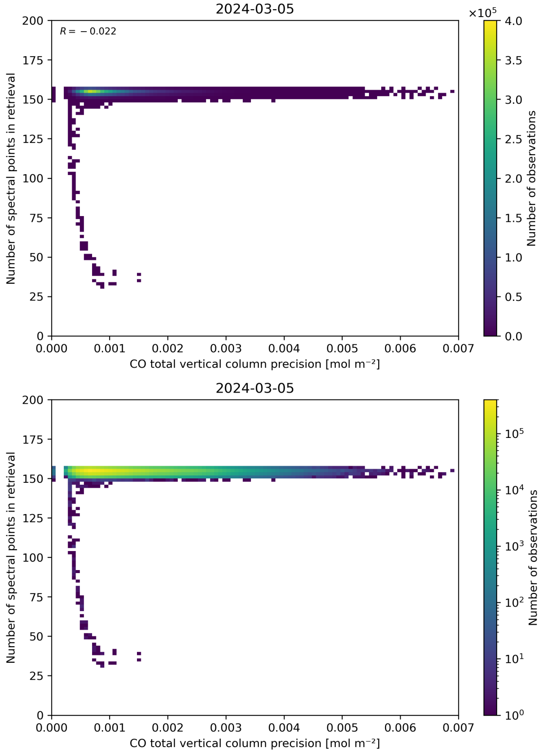
Figure 47: Scatter density plot of “CO total vertical column precision” against “Number of spectral points in retrieval” for 2024-03-04 to 2024-03-06.
