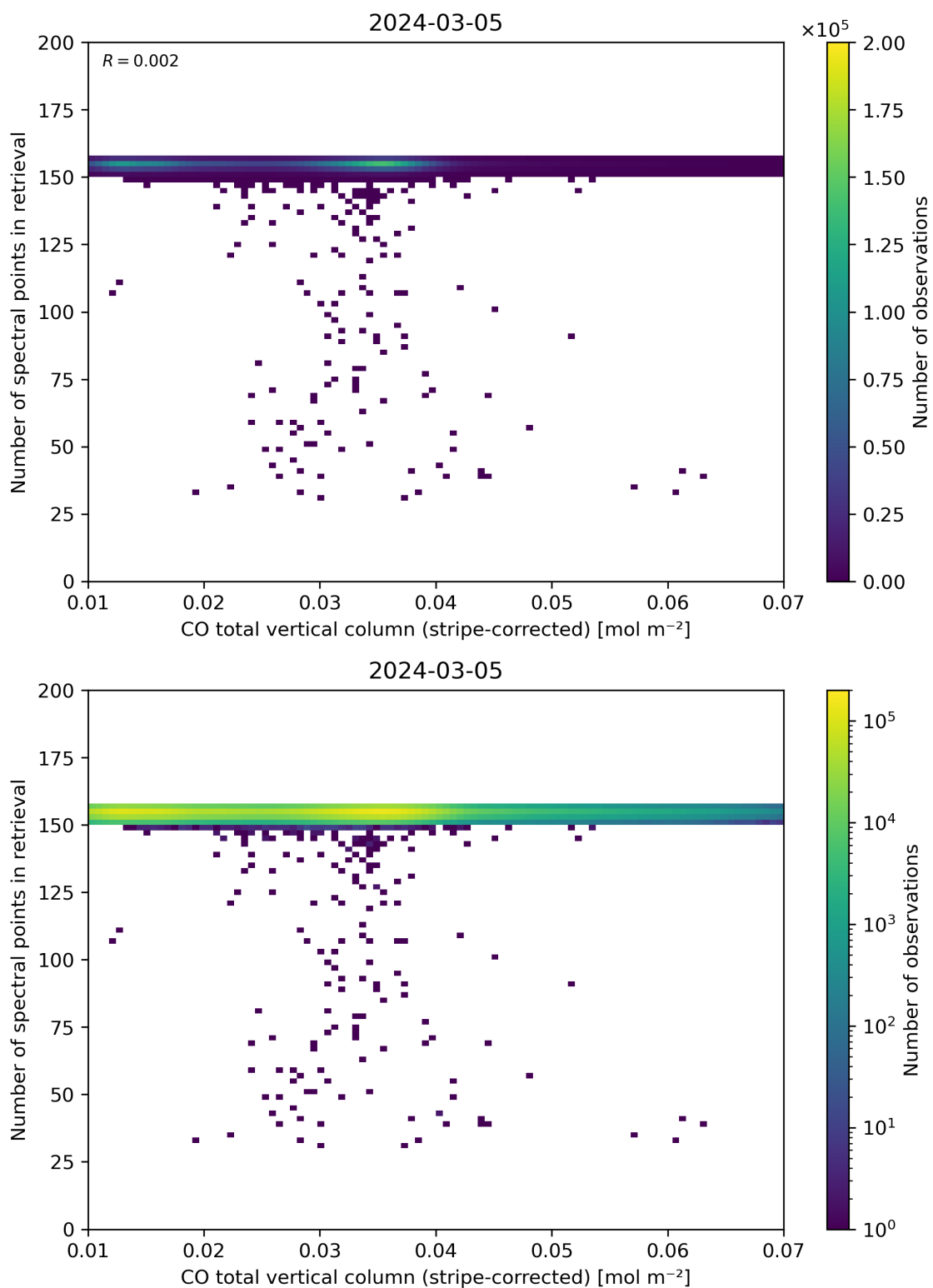
Figure 40: Scatter density plot of “CO total vertical column (stripe-corrected)” against “Number of spectral points in retrieval” for 2024-03-04 to 2024-03-06.
