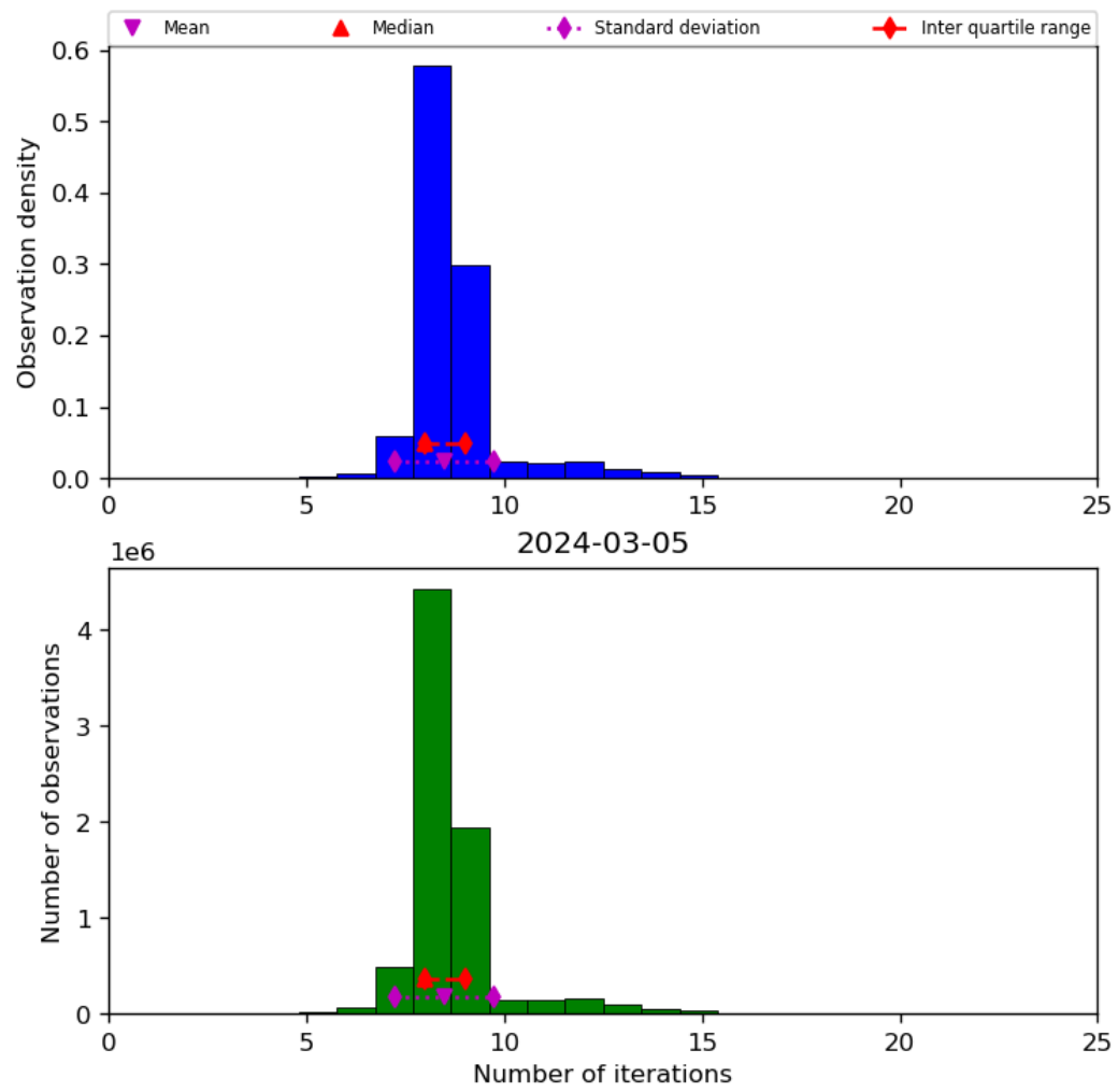
Figure 24: Histogram of “Number of iterations” for 2024-03-04 to 2024-03-06
