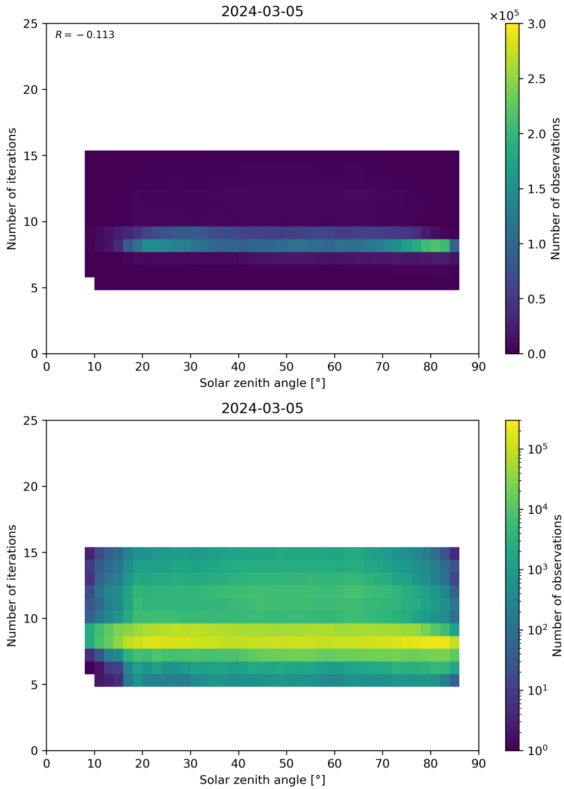
Figure 67: Scatter density plot of “Solar zenith angle” against “Number of iterations” for 2024-03-04 to 2024-03-06.
