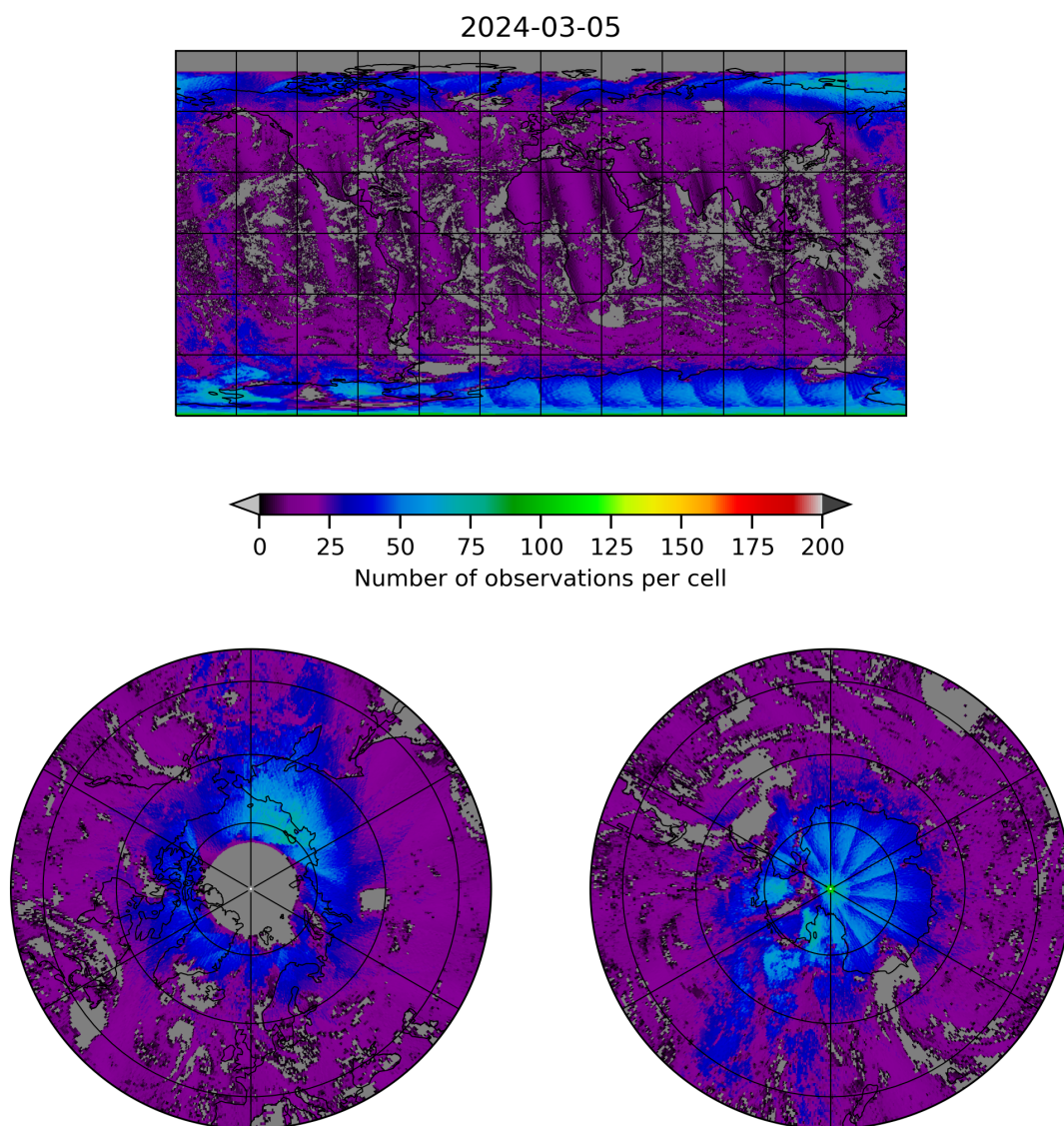
Figure 8: Map of the number of observations for 2024-03-04 to 2024-03-06
