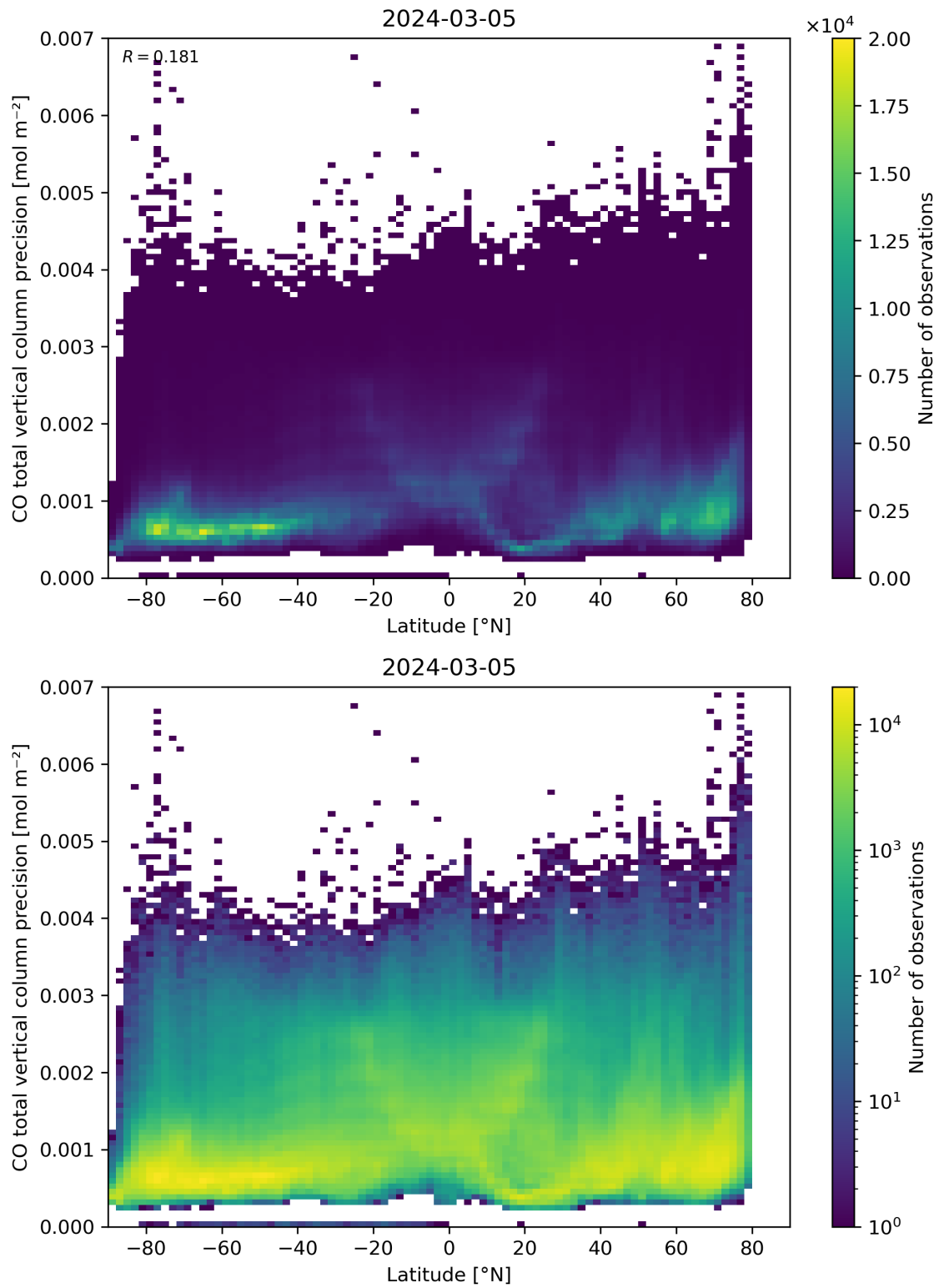
Figure 53: Scatter density plot of “Latitude” against “CO total vertical column precision” for 2024-03-04 to 2024-03-06.
