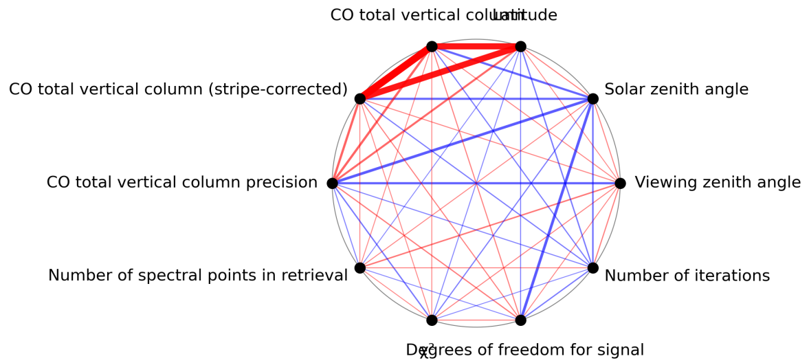
Figure 1: Map of correlation graph for 2024-03-04 to 2024-03-06.
