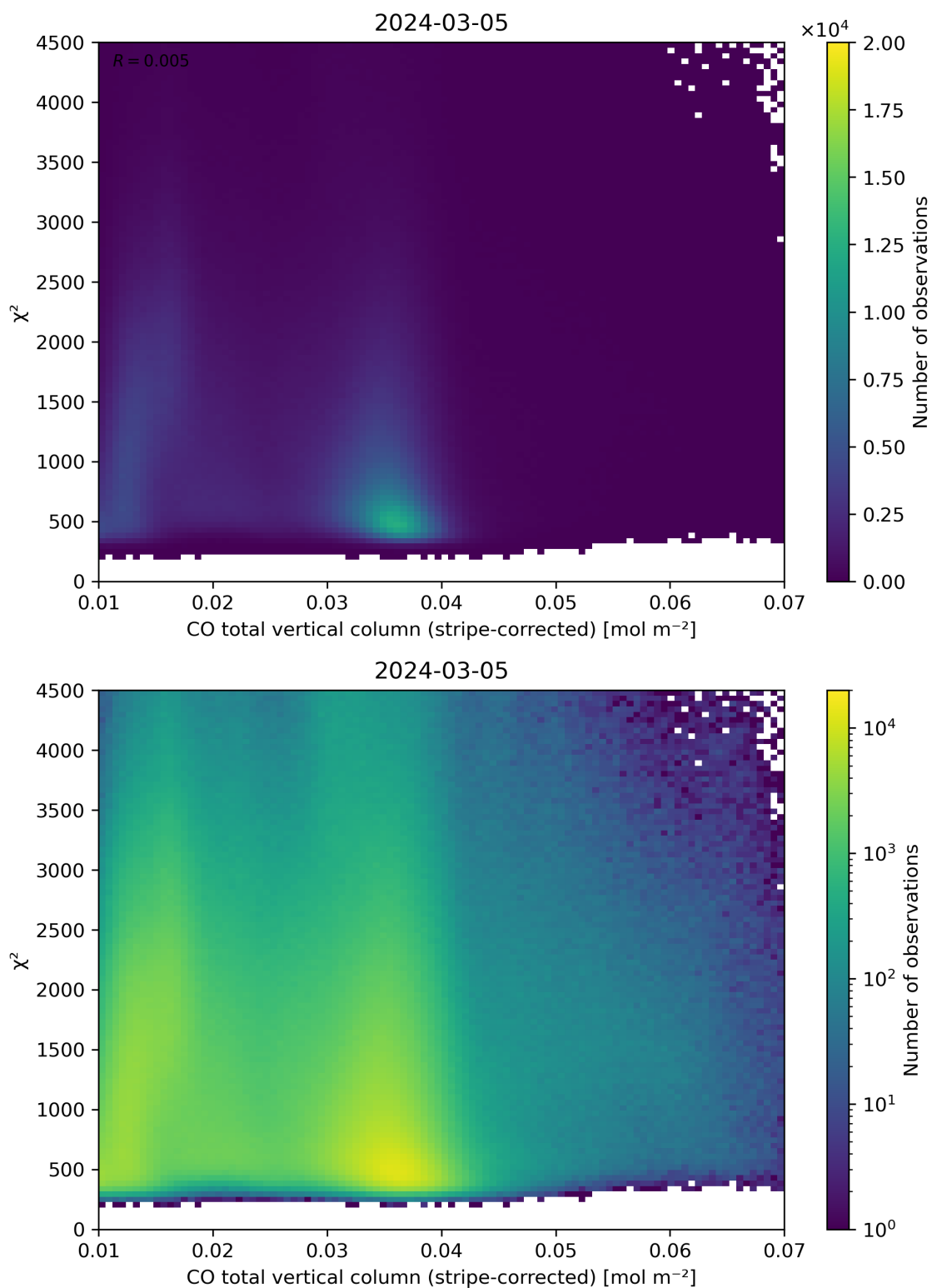
Figure 37: Scatter density plot of “CO total vertical column (stripe-corrected)” against “ \chi^2 ” for 2024-03-04 to 2024-03-06.
