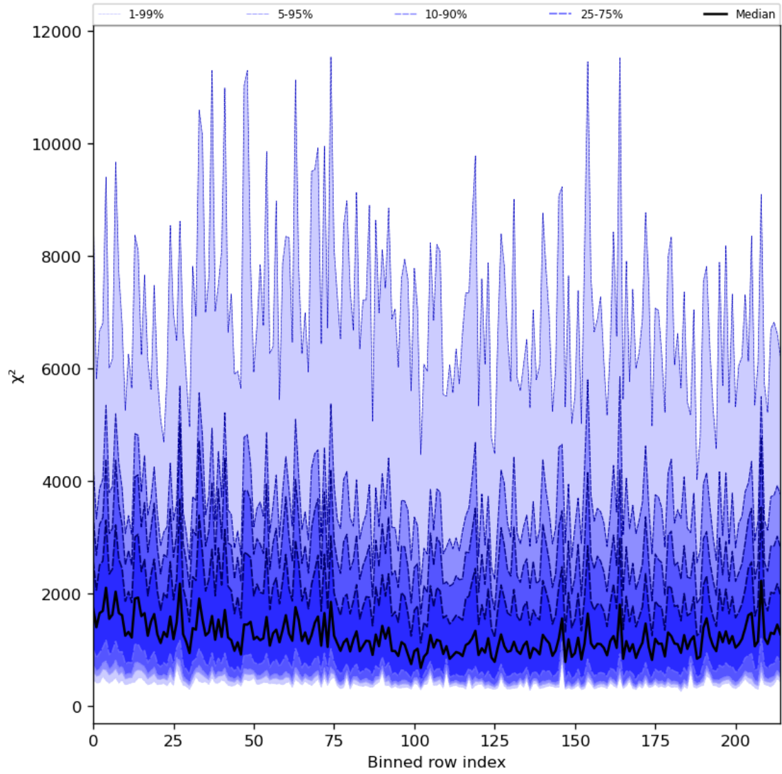
Figure 30: Along track statistics of “ \chi^2 ” for 2024-03-04 to 2024-03-06
