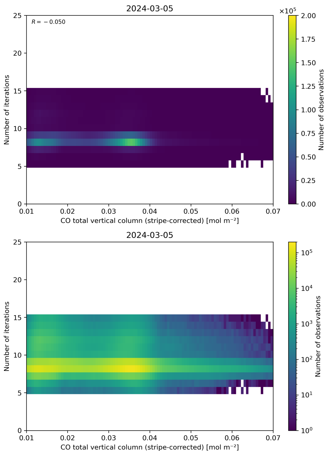
Figure 39: Scatter density plot of “CO total vertical column (stripe-corrected)” against “Number of iterations” for 2024-03-04 to 2024-03-06.
