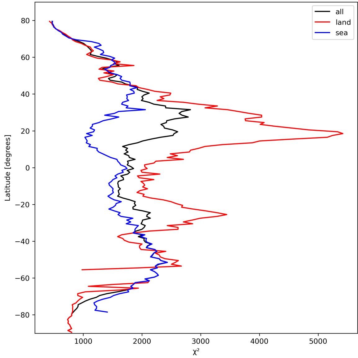
Figure 14: Zonal average of “ \chi^2 ” for 2024-03-04 to 2024-03-06.
