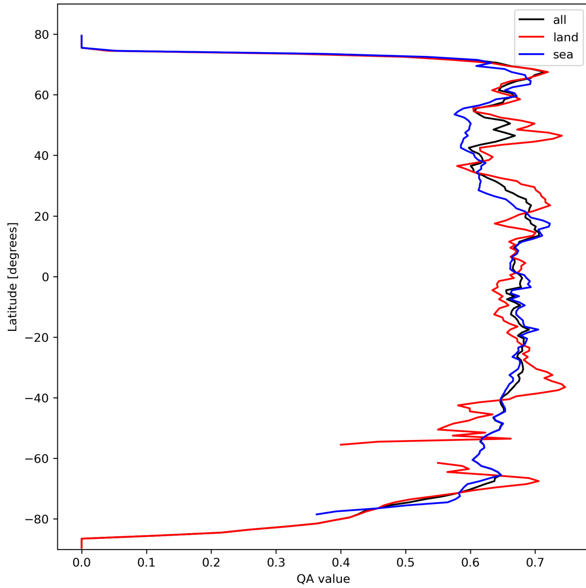
Figure 9: Zonal average of “QA value” for 2024-03-04 to 2024-03-06.
