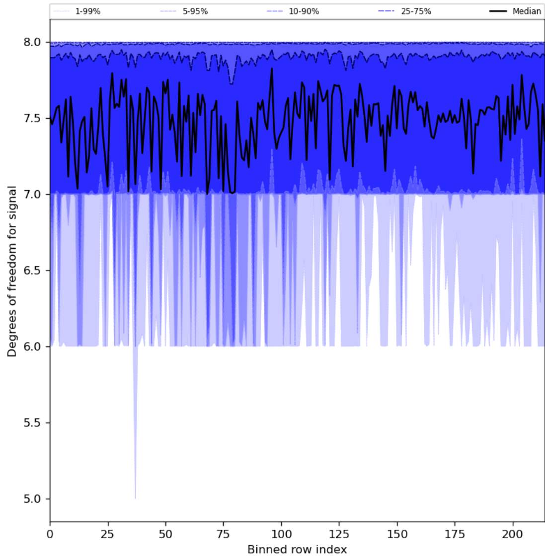
Figure 31: Along track statistics of “Degrees of freedom for signal” for 2024-03-04 to 2024-03-06
