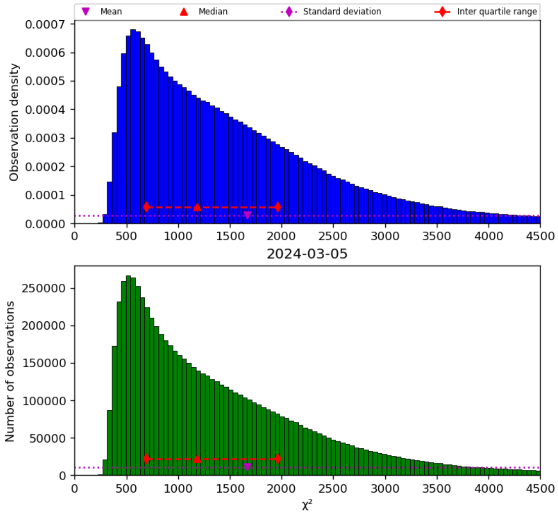
Figure 22: Histogram of “ \chi^2 ” for 2024-03-04 to 2024-03-06
