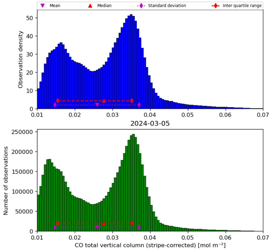
Figure 19: Histogram of “CO total vertical column (stripe-corrected)” for 2024-03-04 to 2024-03-06
