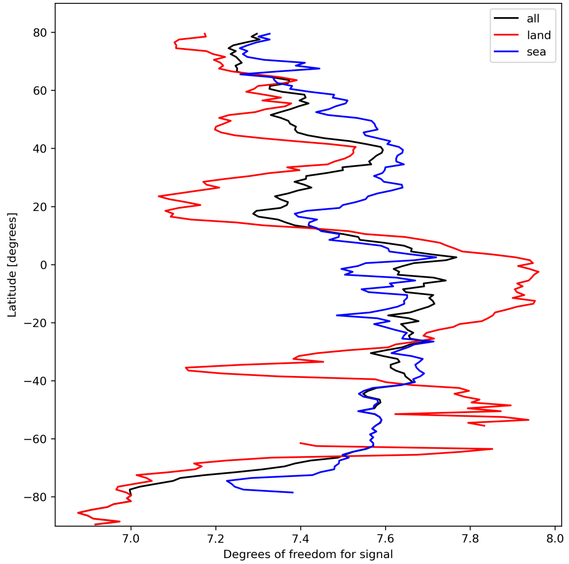
Figure 15: Zonal average of “Degrees of freedom for signal” for 2024-03-04 to 2024-03-06.
