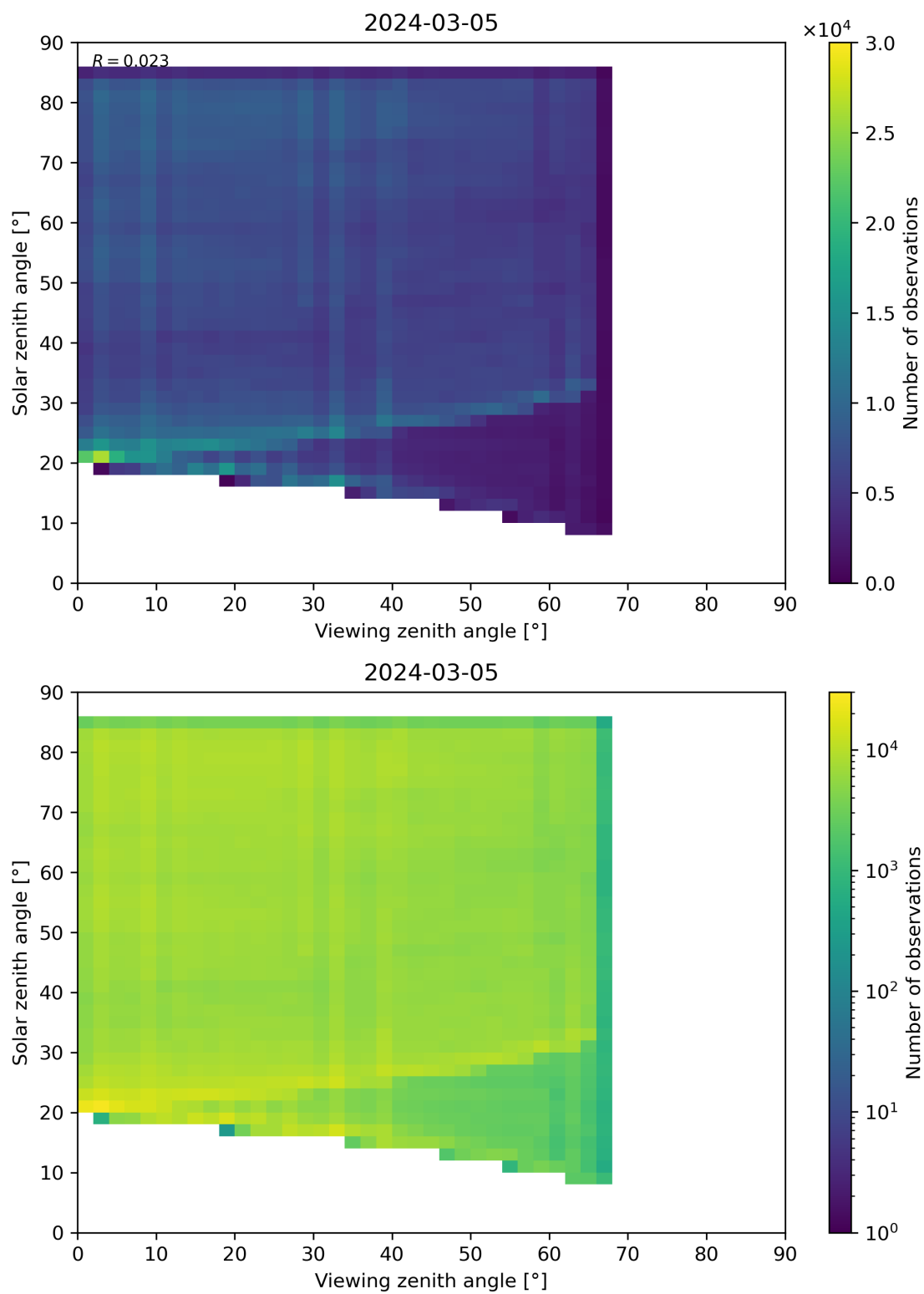
Figure 77: Scatter density plot of “Viewing zenith angle” against “Solar zenith angle” for 2024-03-04 to 2024-03-06.
