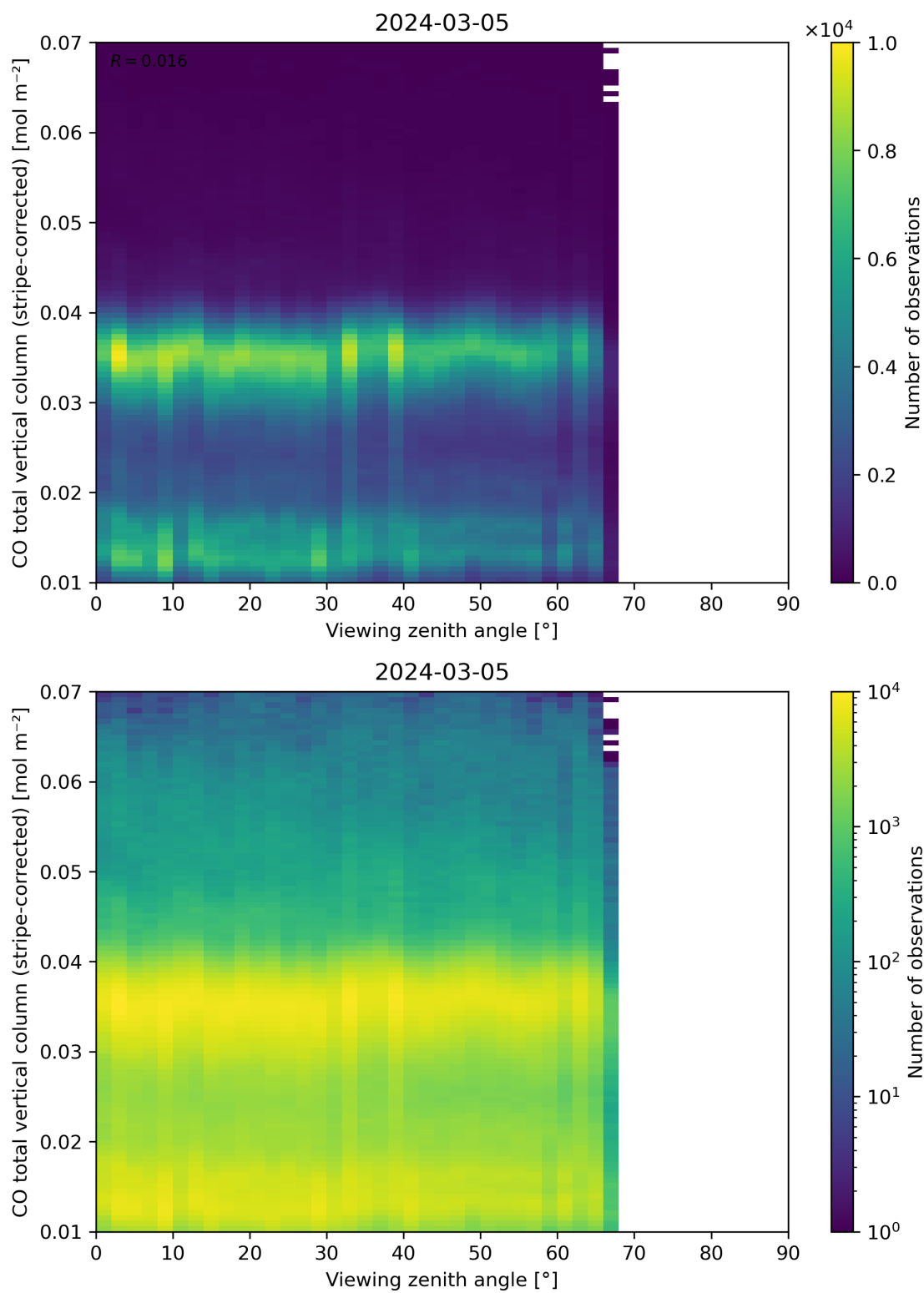
Figure 70: Scatter density plot of “Viewing zenith angle” against “CO total vertical column (stripe-corrected)” for 2024-03-04 to 2024-03-06.
