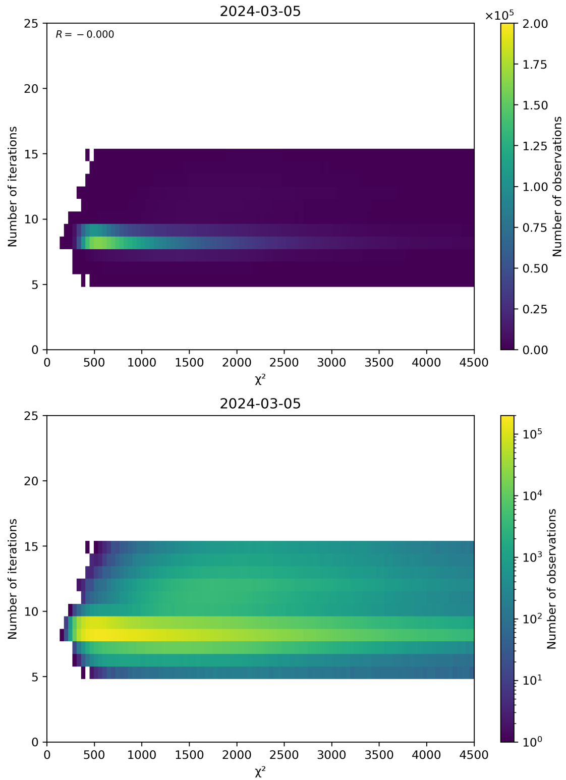
Figure 49: Scatter density plot of “ \chi^2 ” against “Number of iterations” for 2024-03-04 to 2024-03-06.
