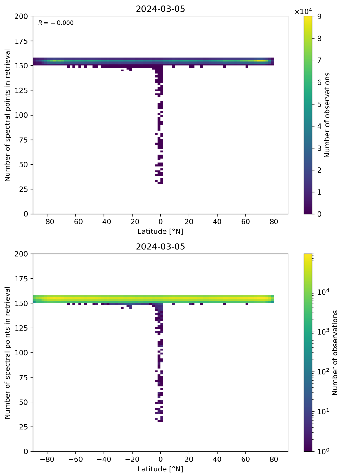
Figure 57: Scatter density plot of “Latitude” against “Number of spectral points in retrieval” for 2024-03-04 to 2024-03-06.
