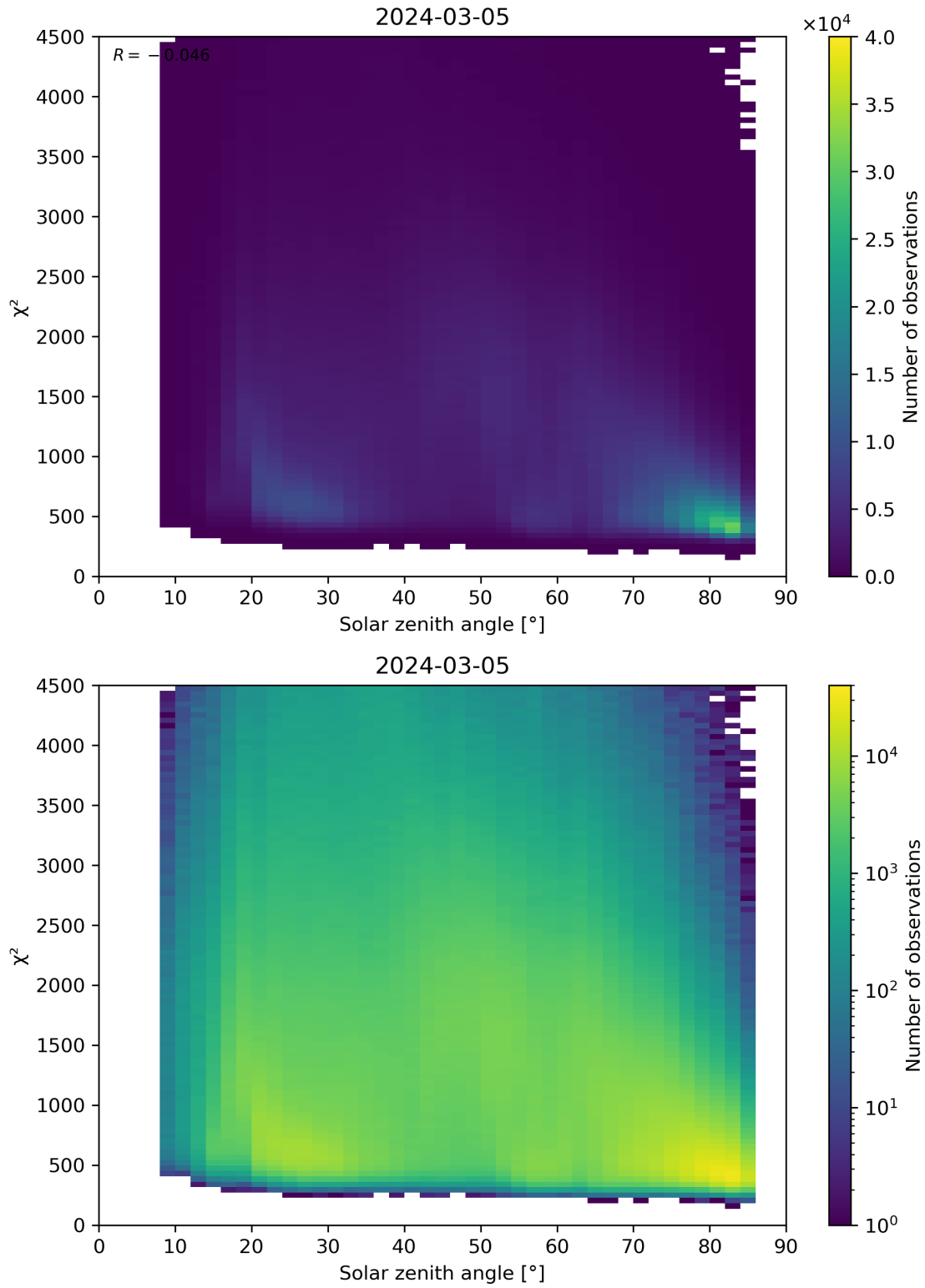
Figure 64: Scatter density plot of “Solar zenith angle” against “ \chi^2 ” for 2024-03-04 to 2024-03-06.
