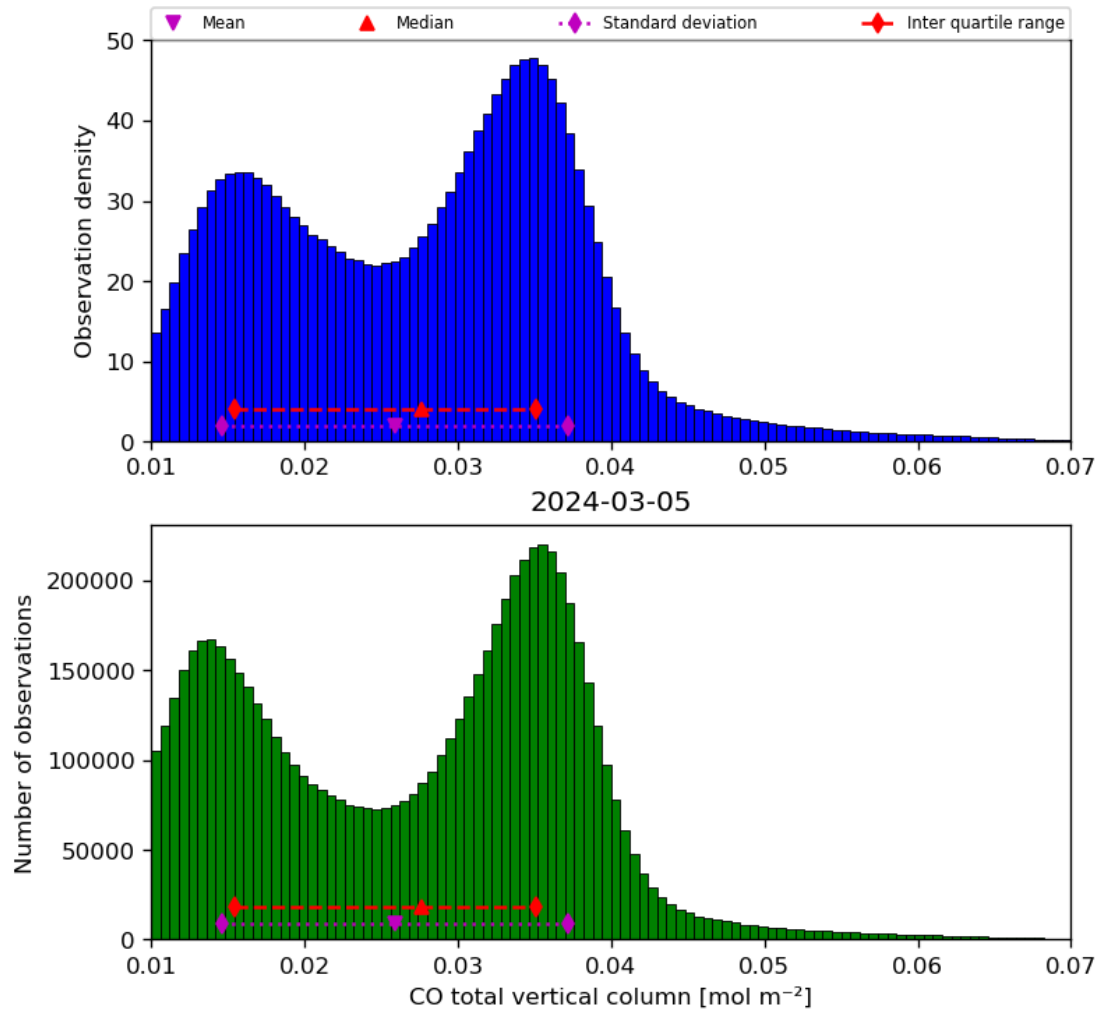
Figure 18: Histogram of “CO total vertical column” for 2024-03-04 to 2024-03-06
