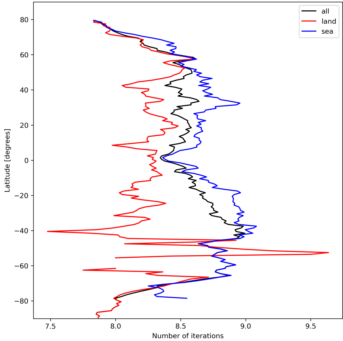
Figure 16: Zonal average of “Number of iterations” for 2024-03-04 to 2024-03-06.
