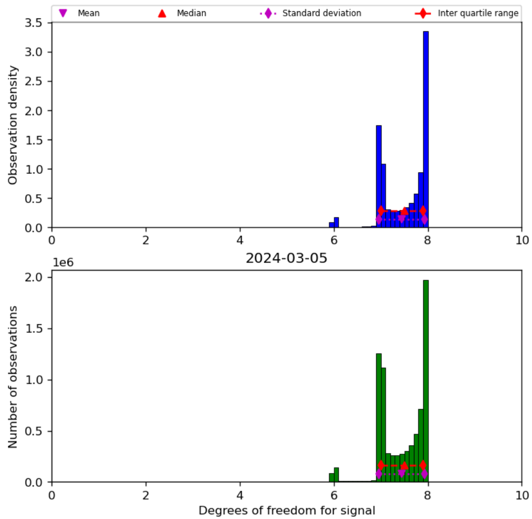
Figure 23: Histogram of “Degrees of freedom for signal” for 2024-03-04 to 2024-03-06
