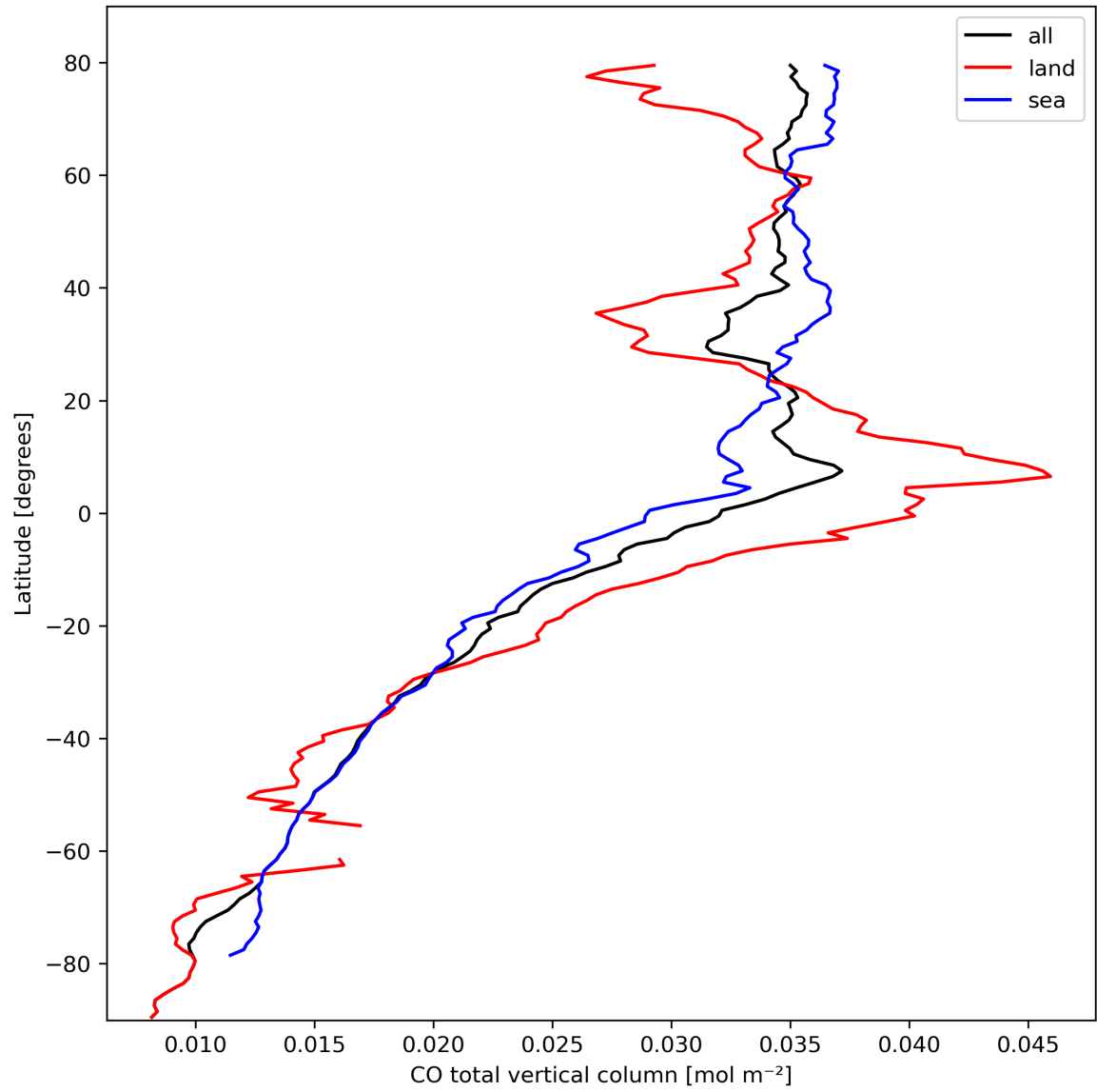
Figure 10: Zonal average of “CO total vertical column” for 2024-03-04 to 2024-03-06.
