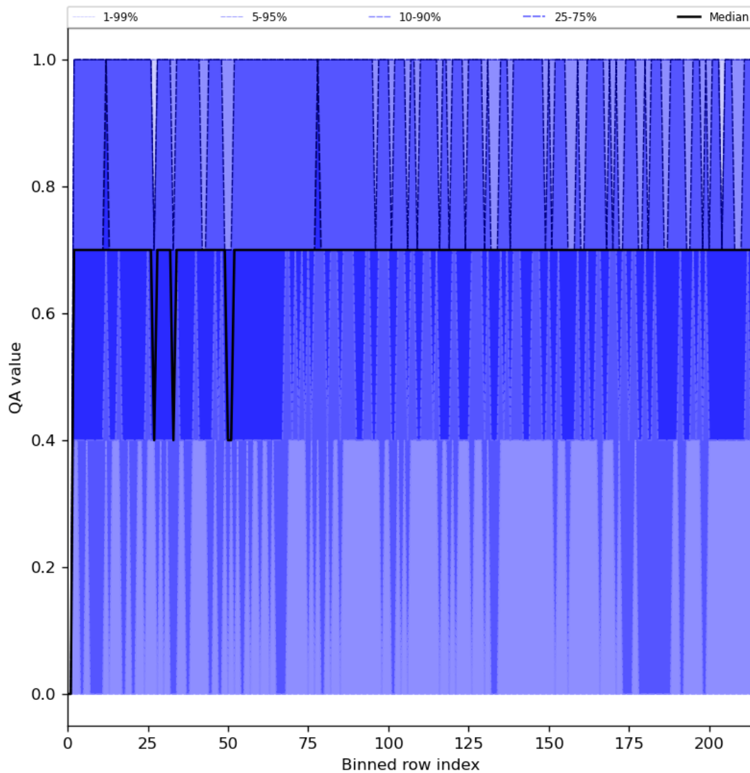
Figure 25: Along track statistics of “QA value” for 2024-03-04 to 2024-03-06
