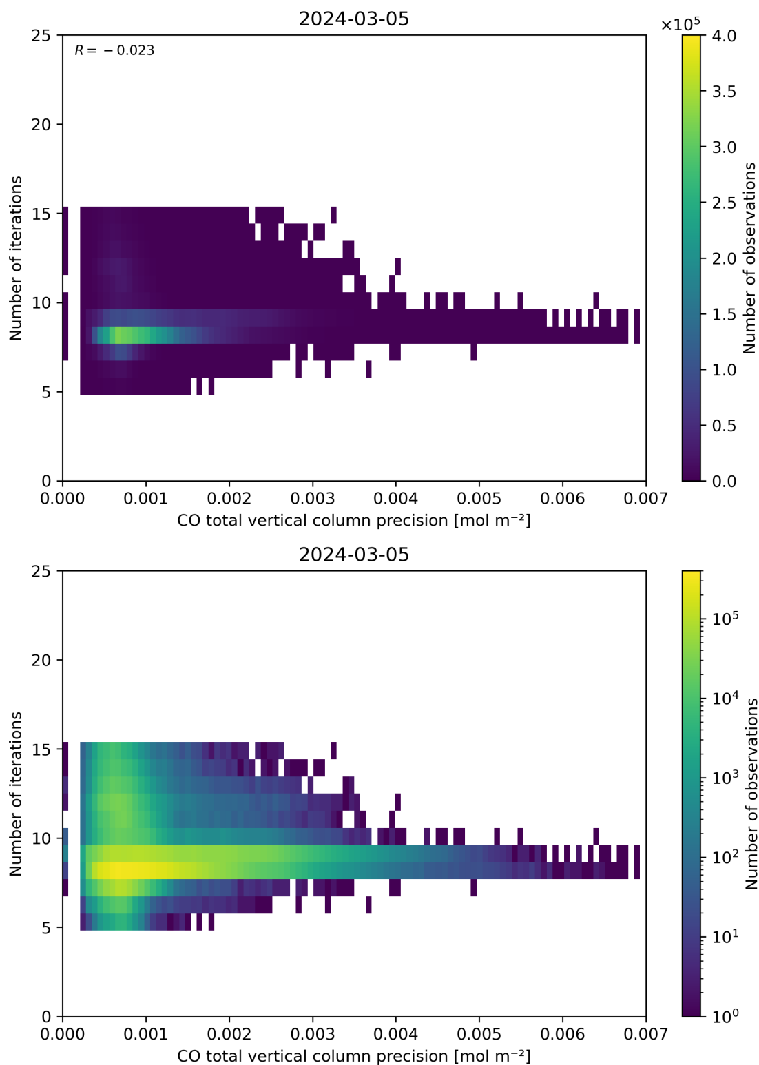
Figure 46: Scatter density plot of “CO total vertical column precision” against “Number of iterations” for 2024-03-04 to 2024-03-06.
