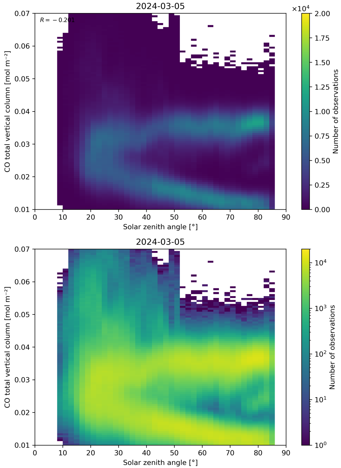
Figure 61: Scatter density plot of “Solar zenith angle” against “CO total vertical column” for 2024-03-04 to 2024-03-06.
