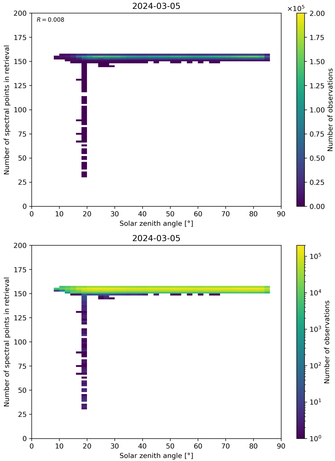
Figure 68: Scatter density plot of “Solar zenith angle” against “Number of spectral points in retrieval” for 2024-03-04 to 2024-03-06.
