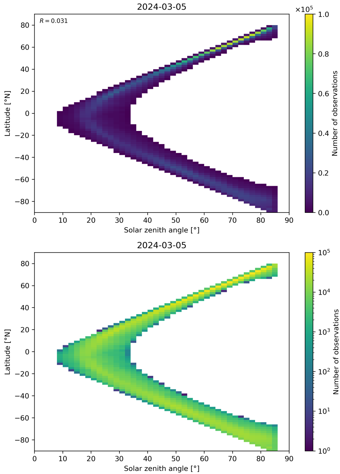
Figure 66: Scatter density plot of “Solar zenith angle” against “Latitude” for 2024-03-04 to 2024-03-06.
