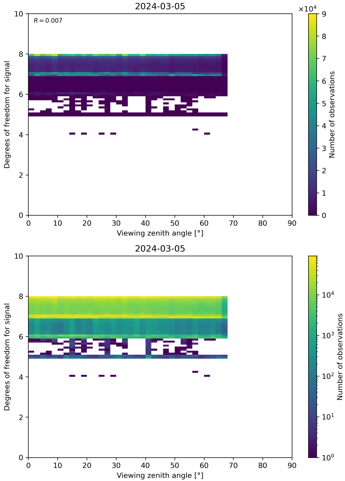
Figure 73: Scatter density plot of “Viewing zenith angle” against “Degrees of freedom for signal” for 2024-03-04 to 2024-03-06.
