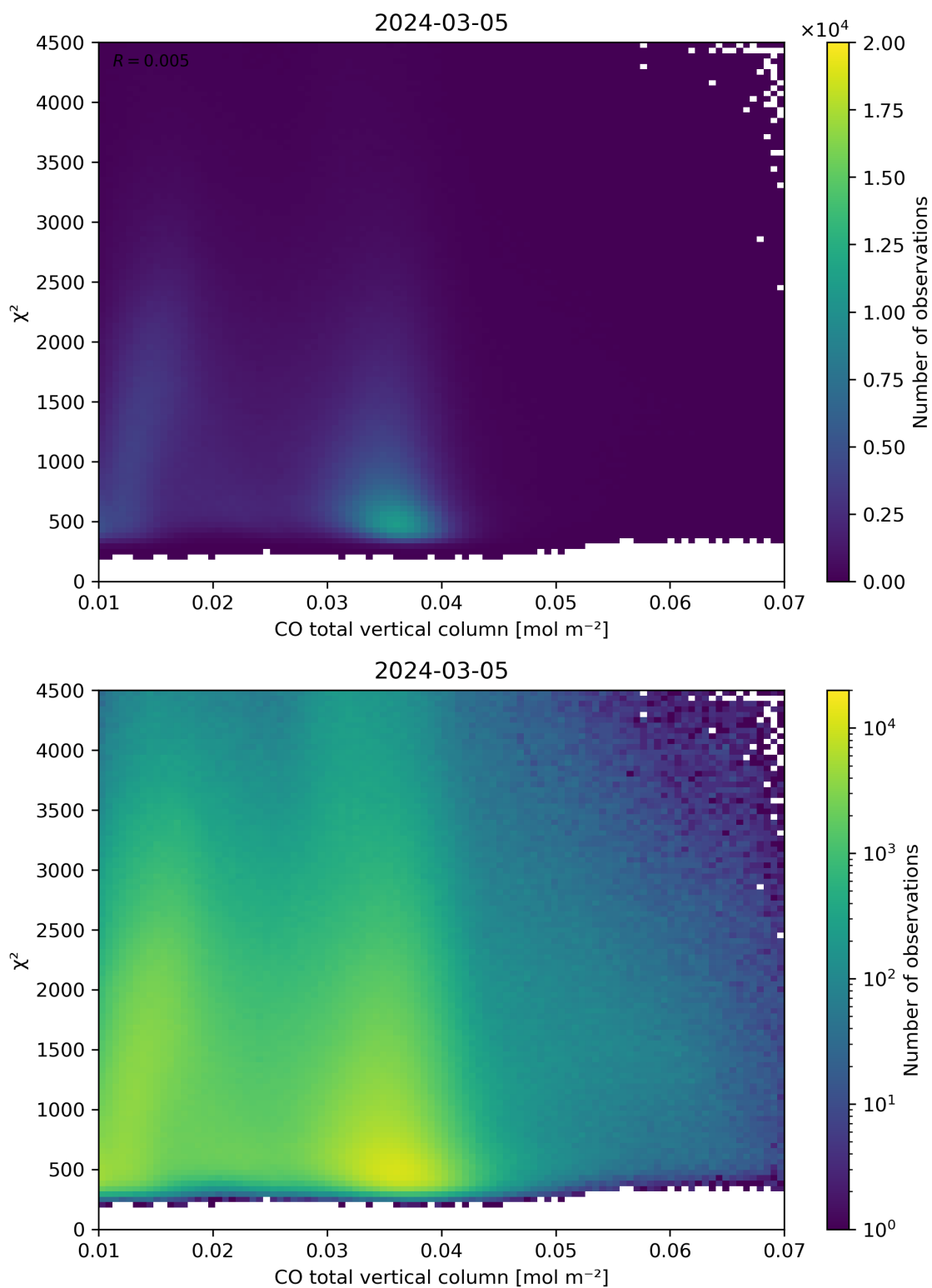
Figure 35: Scatter density plot of “CO total vertical column” against “ \chi^2 ” for 2024-03-04 to 2024-03-06.
