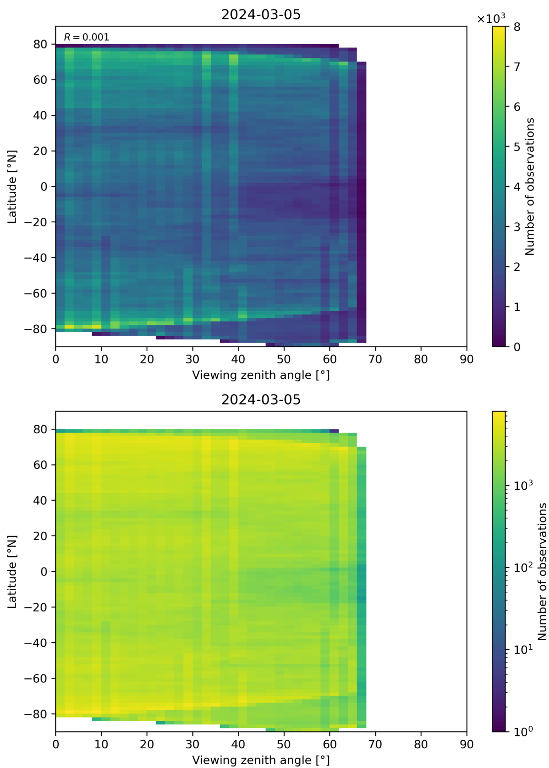
Figure 74: Scatter density plot of “Viewing zenith angle” against “Latitude” for 2024-03-04 to 2024-03-06.
