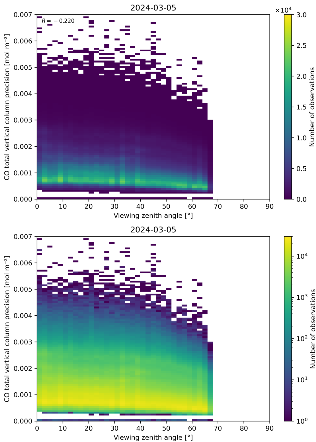
Figure 71: Scatter density plot of “Viewing zenith angle” against “CO total vertical column precision” for 2024-03-04 to 2024-03-06.
