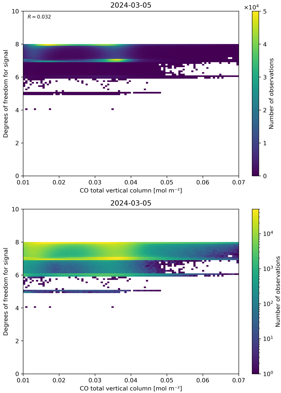
Figure 41: Scatter density plot of “CO total vertical column” against “Degrees of freedom for signal” for 2024-03-04 to 2024-03-06.
