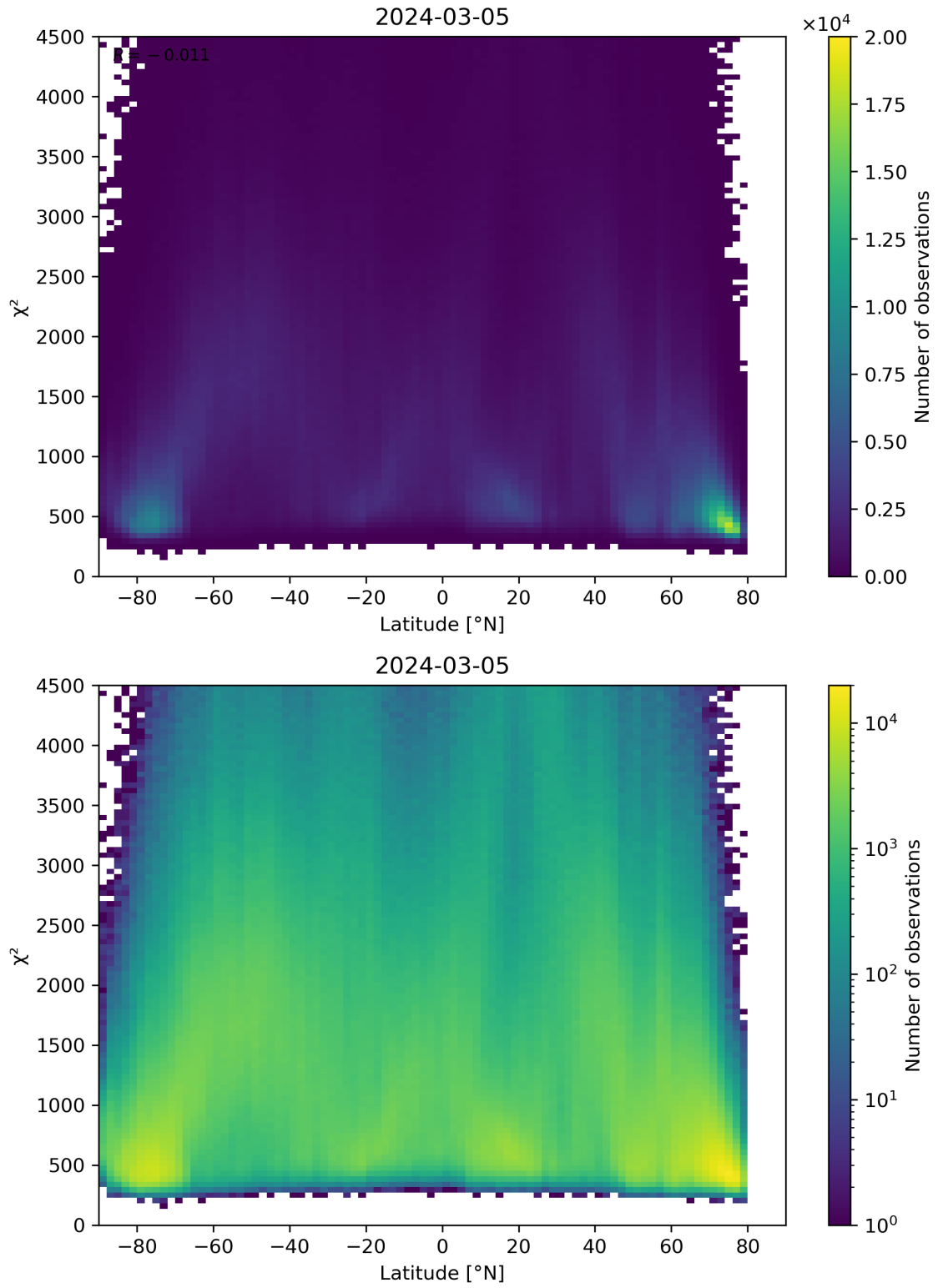
Figure 54: Scatter density plot of “Latitude” against “ \chi^2 ” for 2024-03-04 to 2024-03-06.
