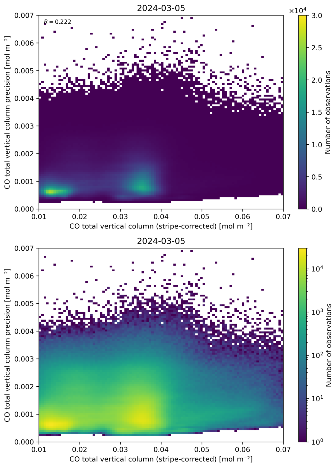
Figure 36: Scatter density plot of “CO total vertical column (stripe-corrected)” against “CO total vertical column precision” for 2024-03-04 to 2024-03-06.
