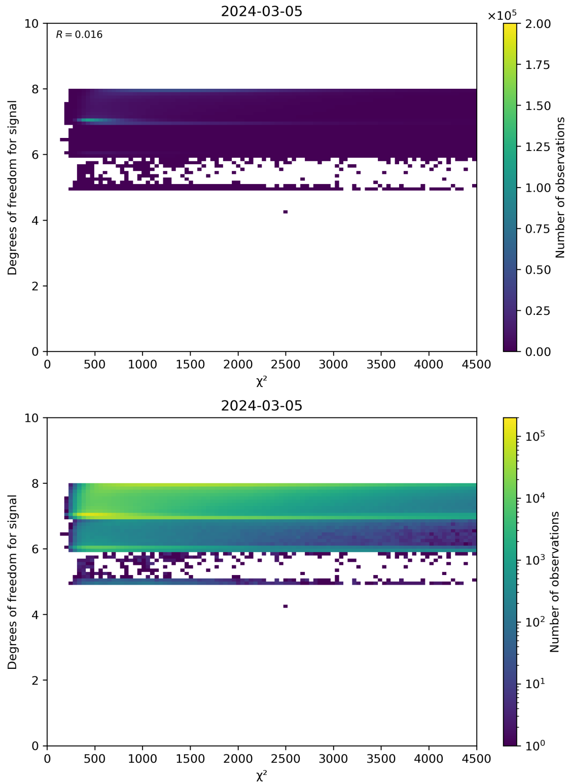
Figure 48: Scatter density plot of “ \chi^2 ” against “Degrees of freedom for signal” for 2024-03-04 to 2024-03-06.
