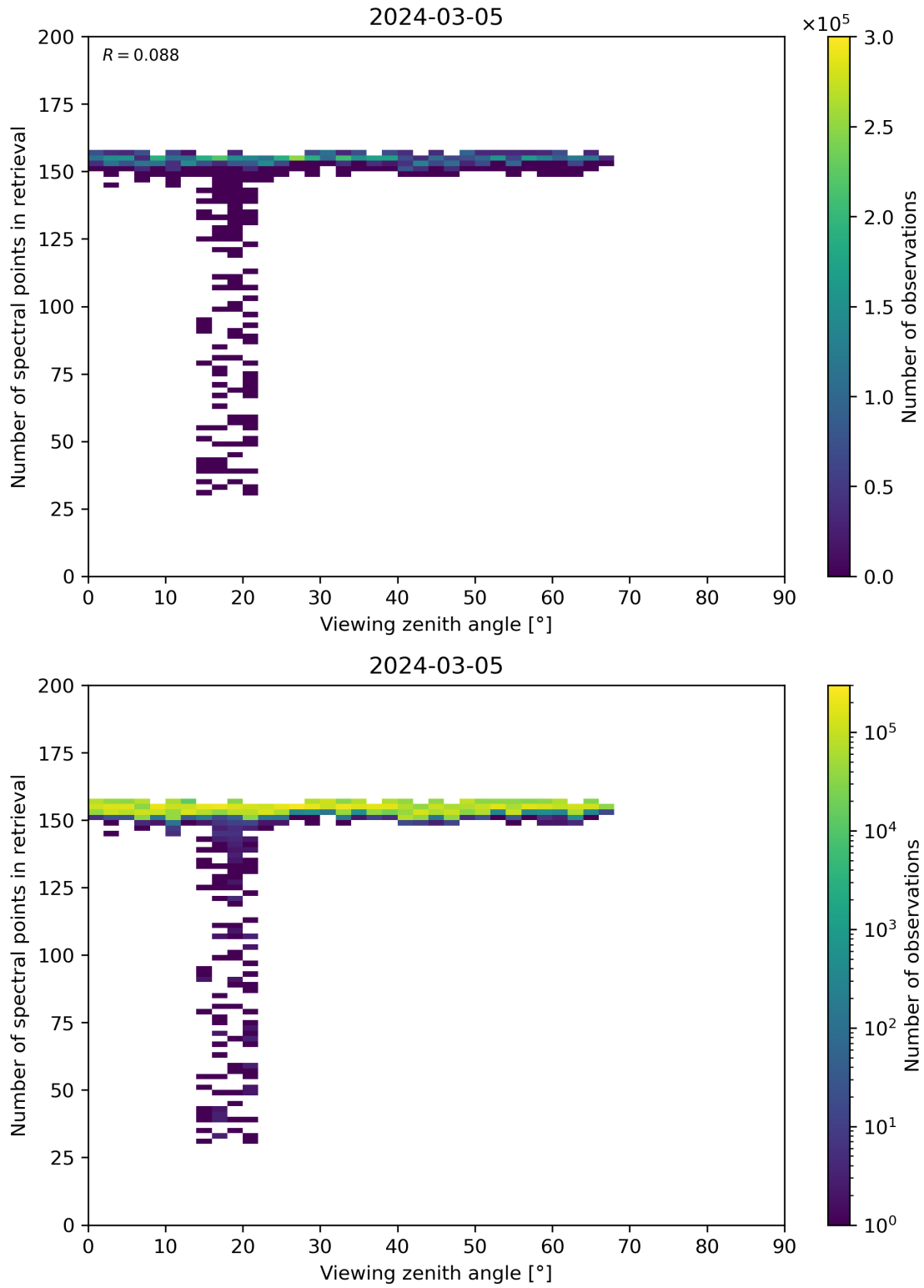
Figure 76: Scatter density plot of “Viewing zenith angle” against “Number of spectral points in retrieval” for 2024-03-04 to 2024-03-06.
