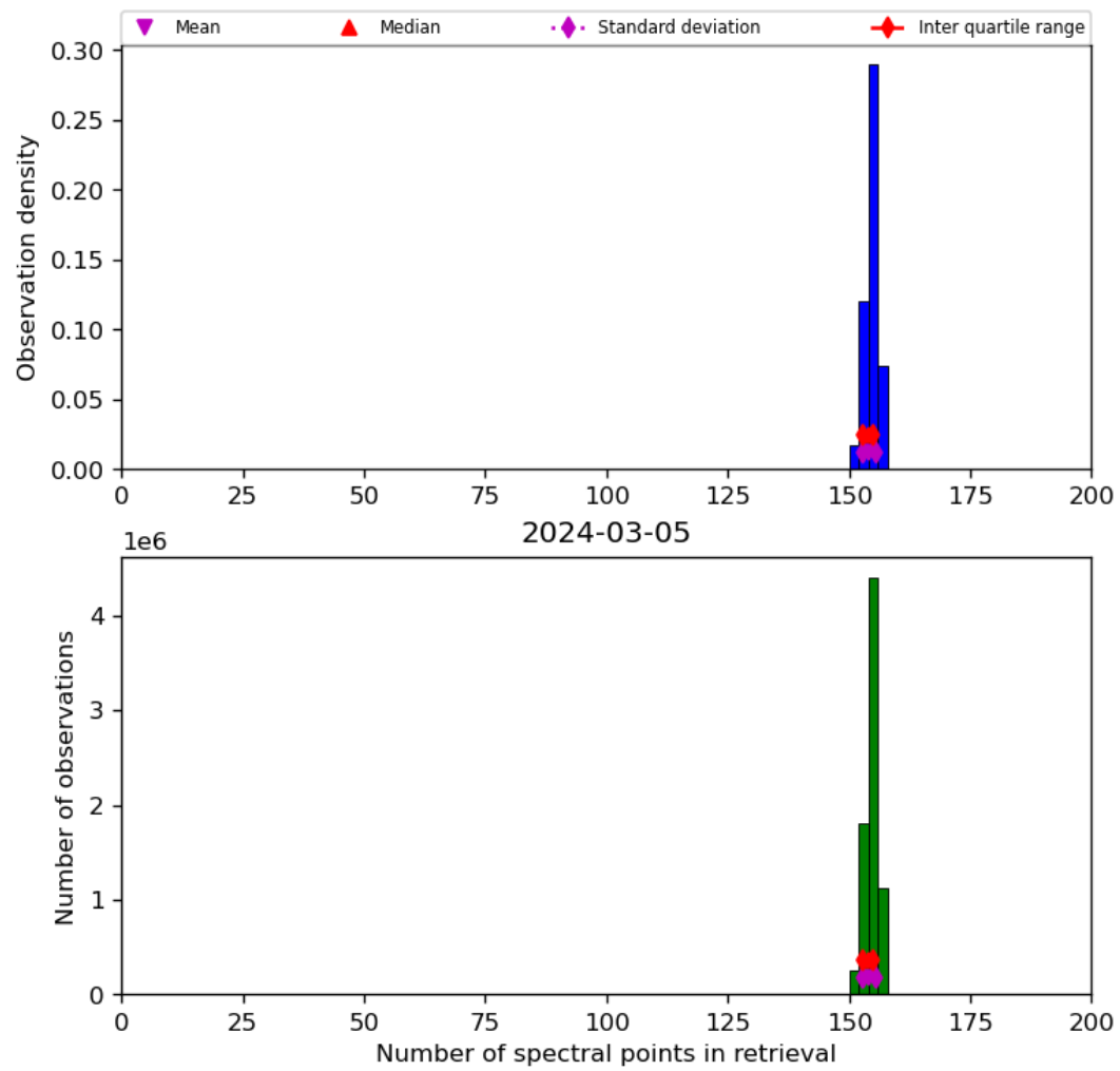
Figure 21: Histogram of “Number of spectral points in retrieval” for 2024-03-04 to 2024-03-06
