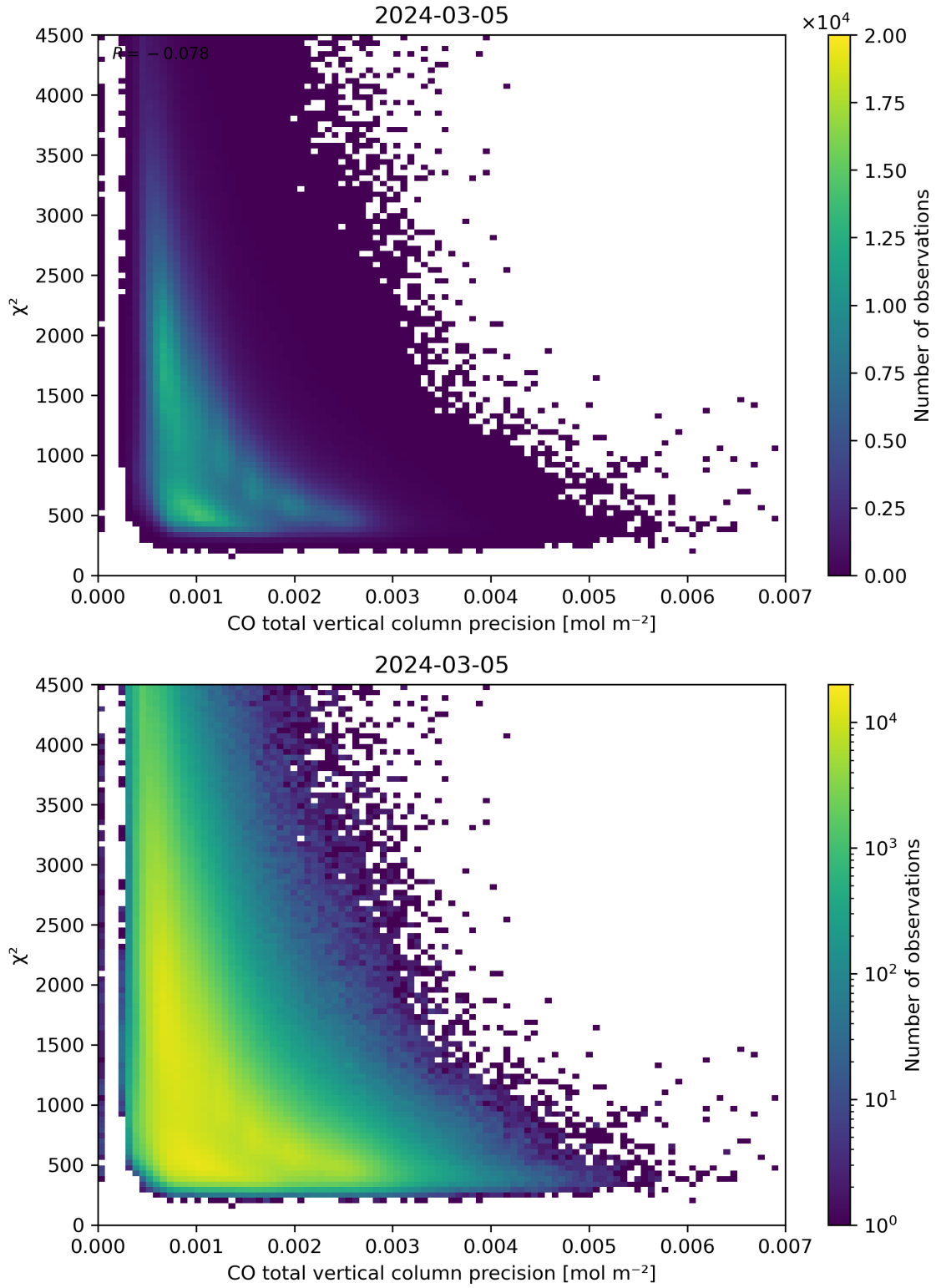
Figure 44: Scatter density plot of “CO total vertical column precision” against “ \chi^2 ” for 2024-03-04 to 2024-03-06.
