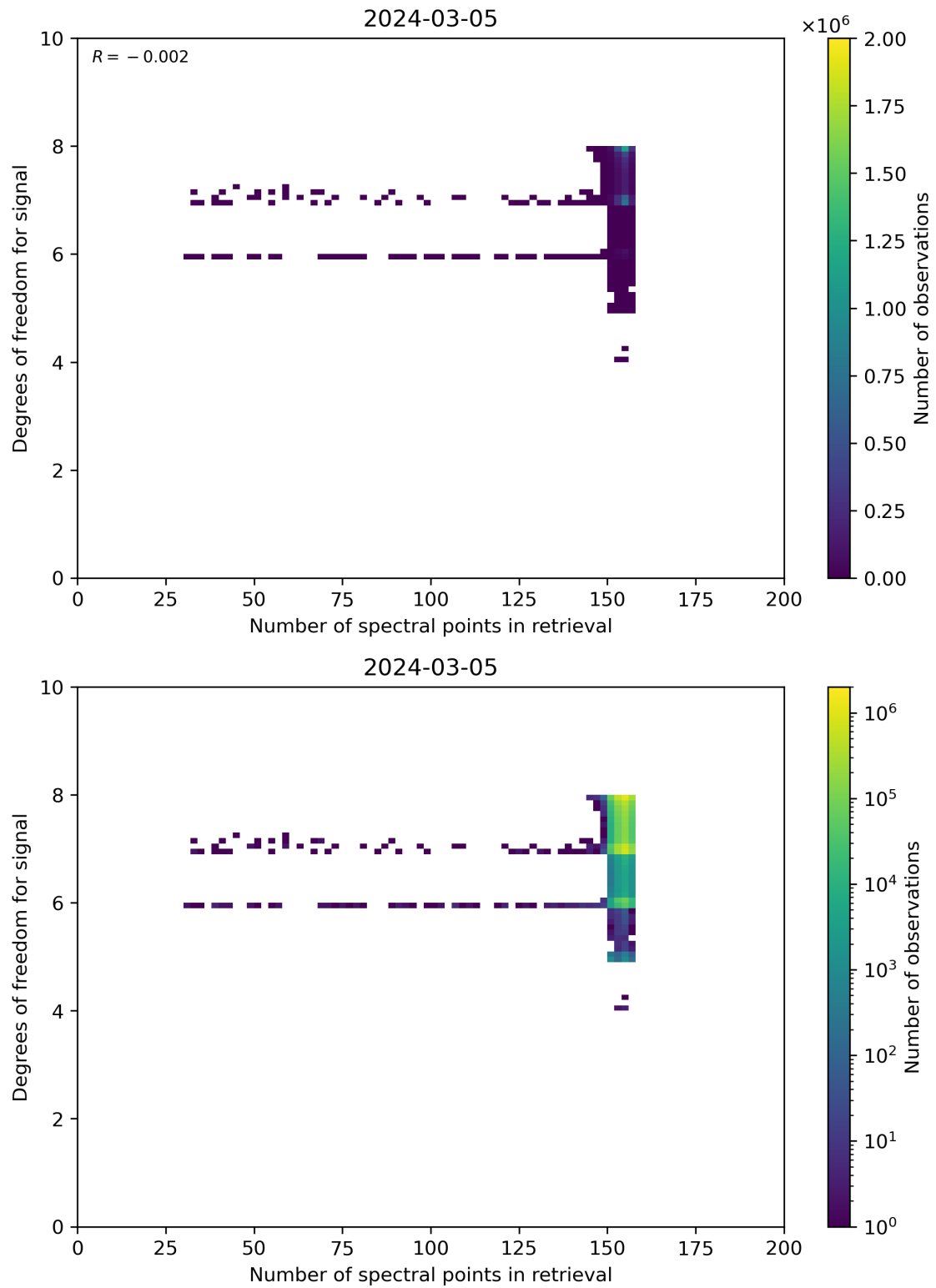
Figure 59: Scatter density plot of “Number of spectral points in retrieval” against “Degrees of freedom for signal” for 2024-03-04 to 2024-03-06.
