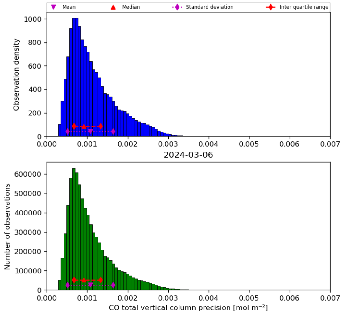
Figure 20: Histogram of “CO total vertical column precision” for 2024-03-05 to 2024-03-07
