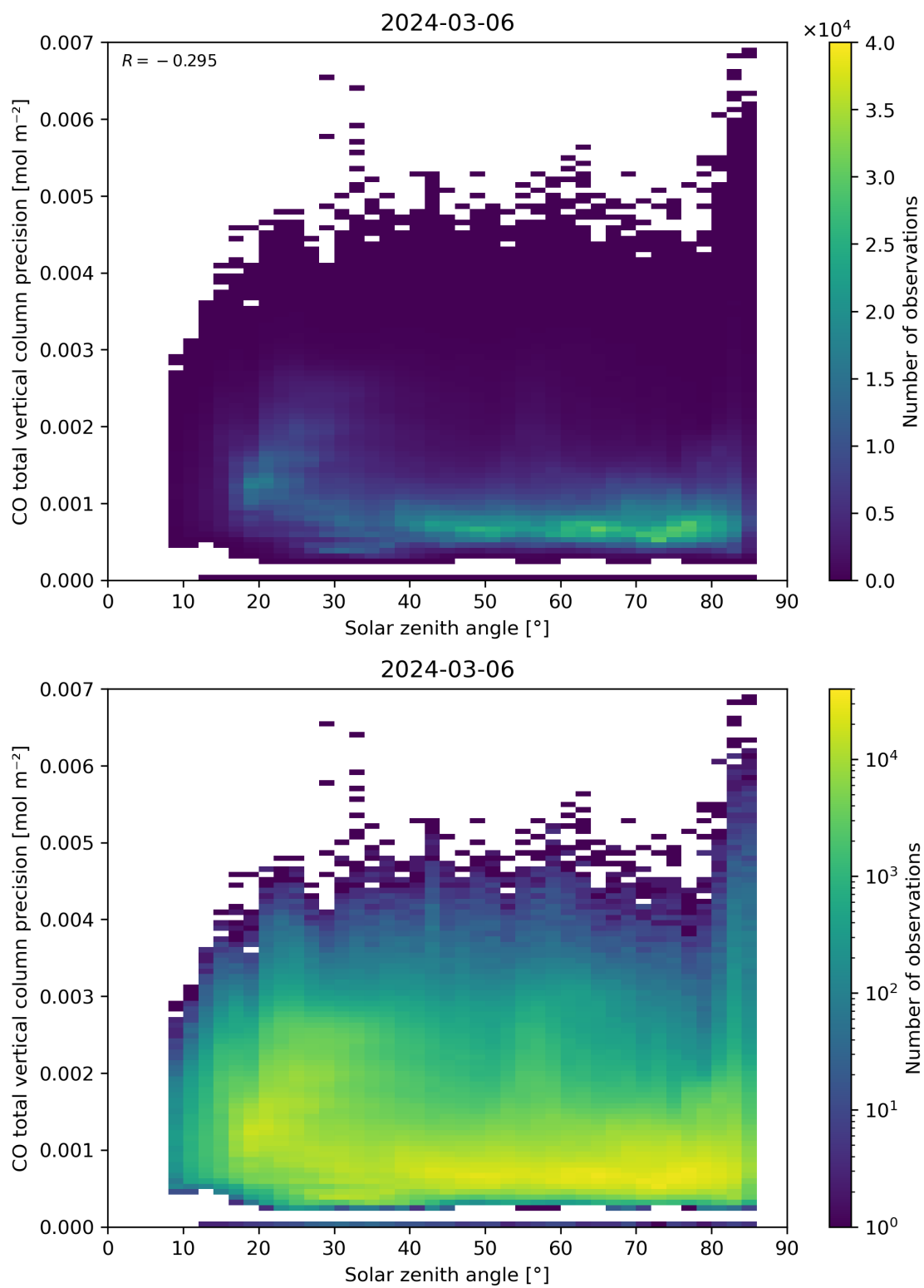
Figure 63: Scatter density plot of “Solar zenith angle” against “CO total vertical column precision” for 2024-03-05 to 2024-03-07.
