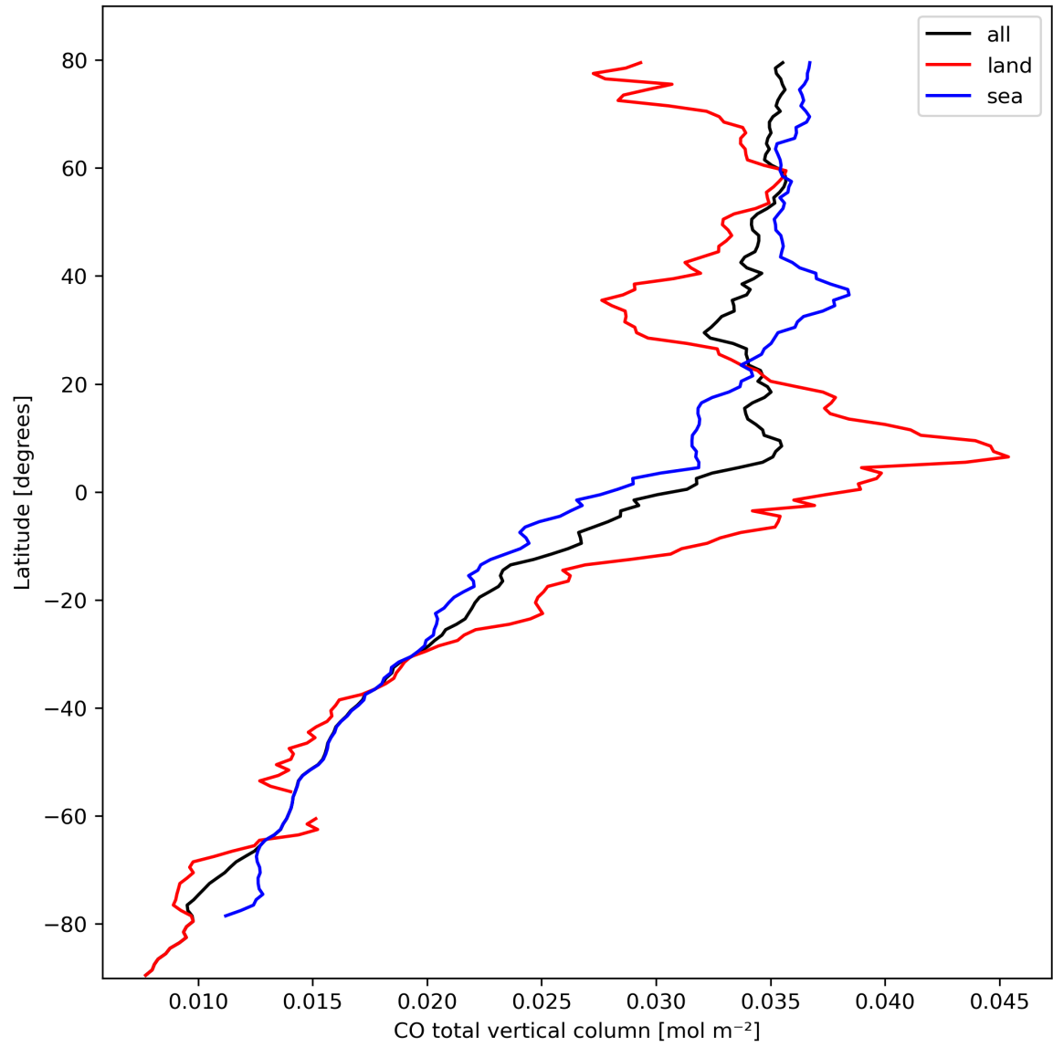
Figure 10: Zonal average of “CO total vertical column” for 2024-03-05 to 2024-03-07.
