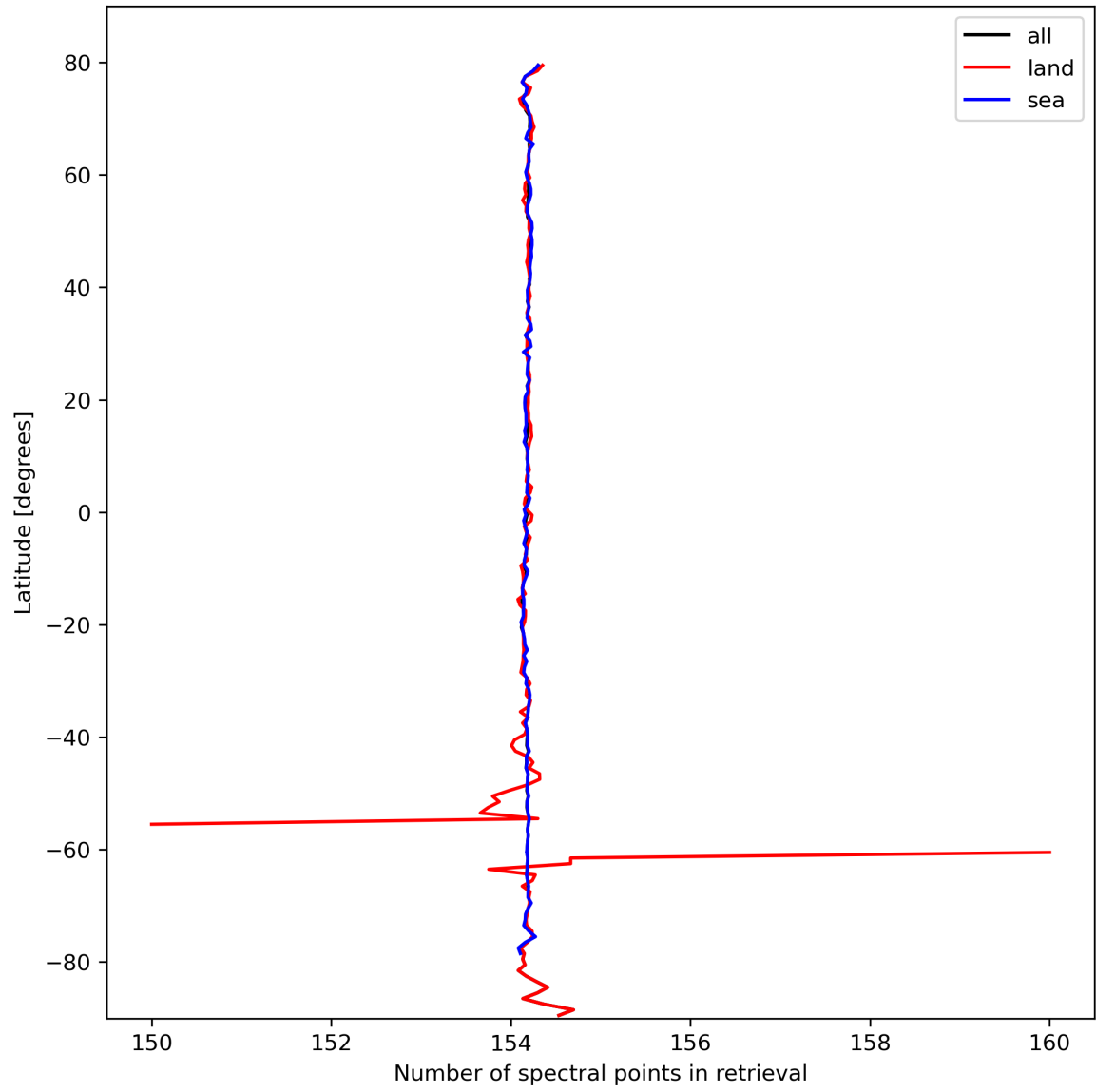
Figure 13: Zonal average of “Number of spectral points in retrieval” for 2024-03-05 to 2024-03-07.
