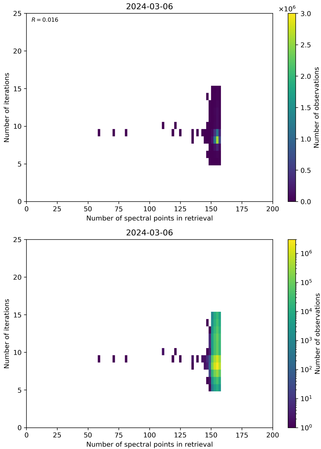
Figure 60: Scatter density plot of “Number of spectral points in retrieval” against “Number of iterations” for 2024-03-05 to 2024-03-07.
