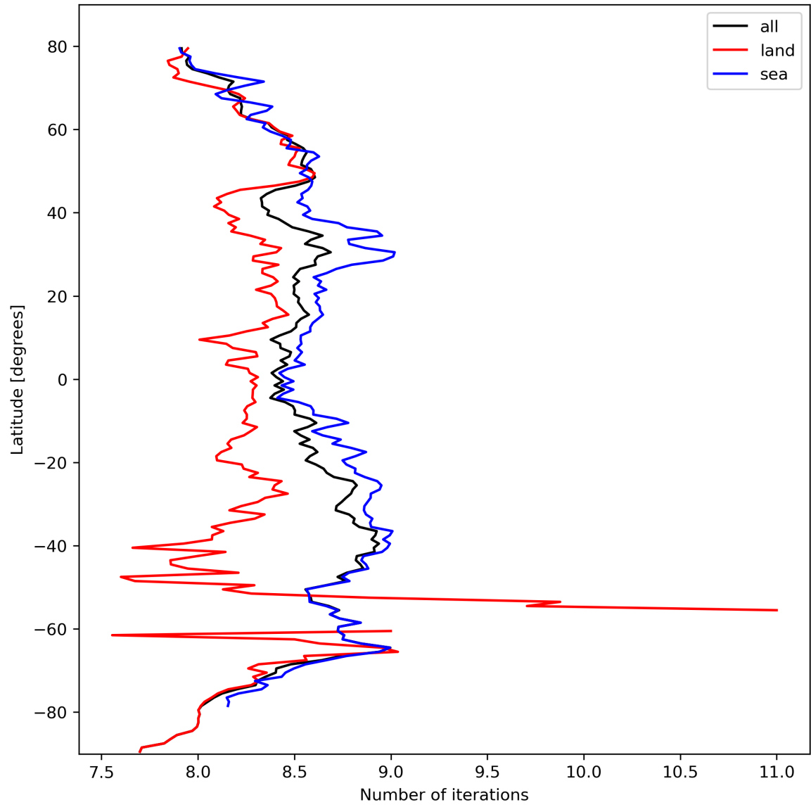
Figure 16: Zonal average of “Number of iterations” for 2024-03-05 to 2024-03-07.
