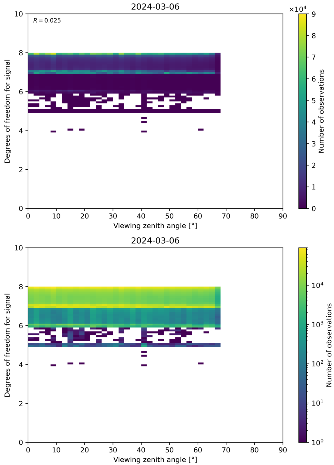
Figure 73: Scatter density plot of “Viewing zenith angle” against “Degrees of freedom for signal” for 2024-03-05 to 2024-03-07.
