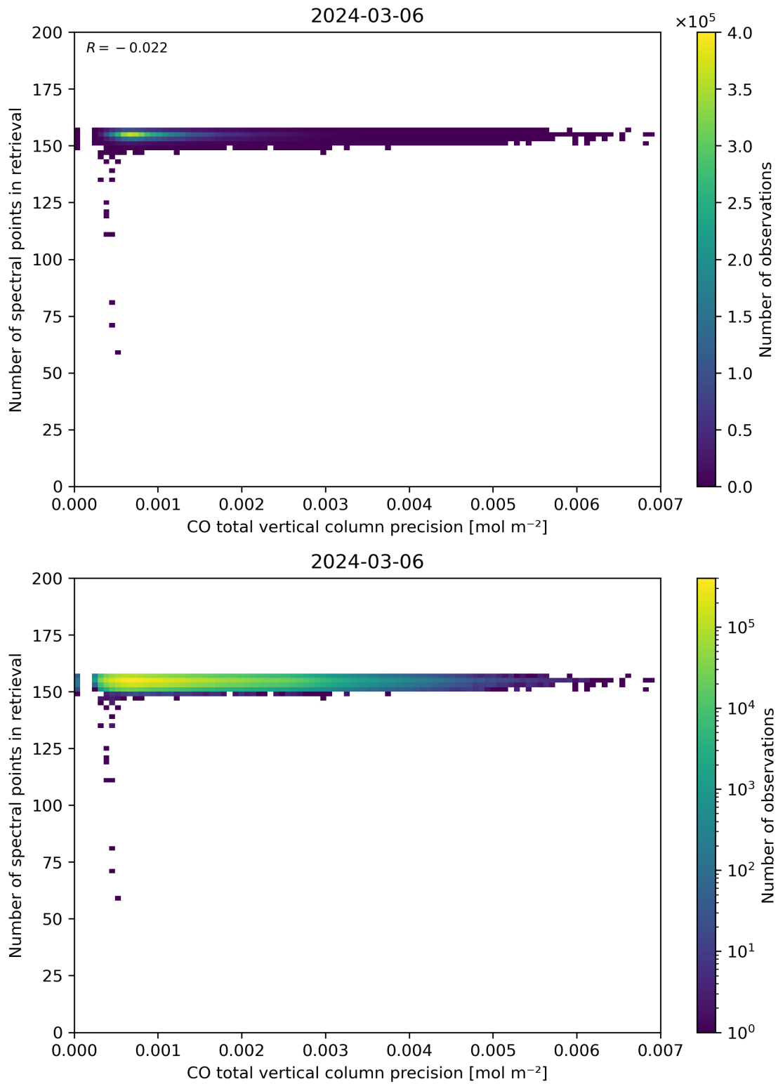
Figure 47: Scatter density plot of “CO total vertical column precision” against “Number of spectral points in retrieval” for 2024-03-05 to 2024-03-07.
