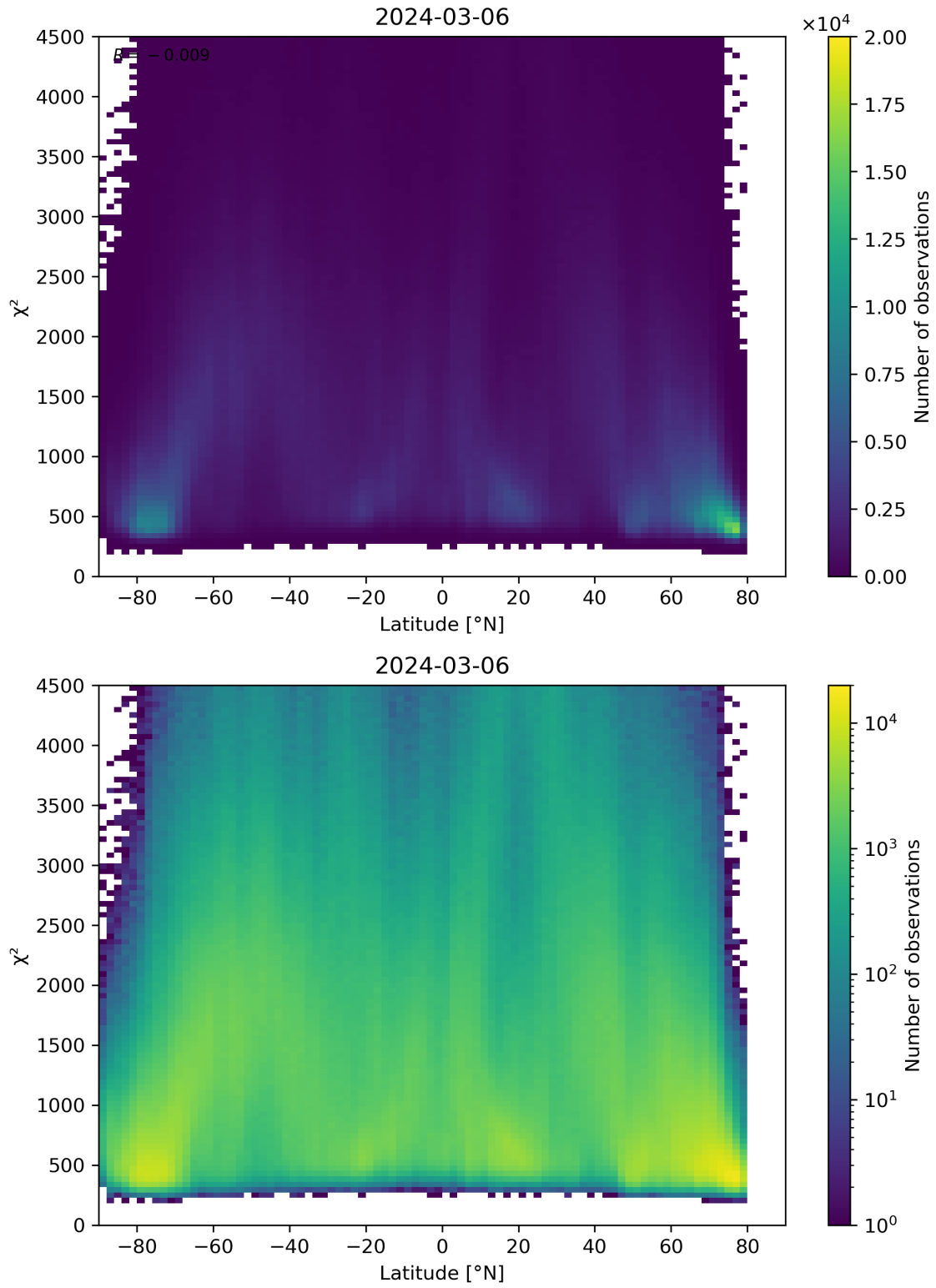
Figure 54: Scatter density plot of “Latitude” against “ \chi^2 ” for 2024-03-05 to 2024-03-07.
