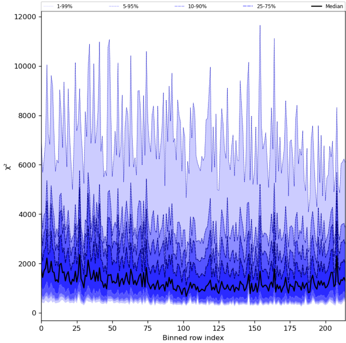
Figure 30: Along track statistics of “ \chi^2 ” for 2024-03-05 to 2024-03-07
