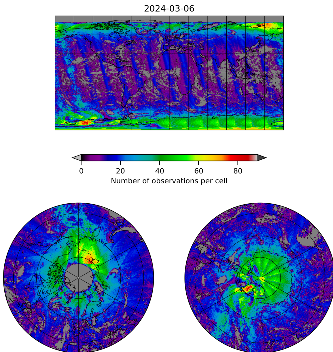
Figure 8: Map of the number of observations for 2024-03-05 to 2024-03-07
