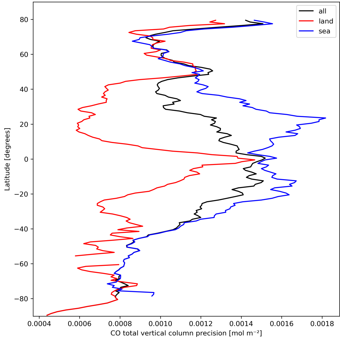
Figure 12: Zonal average of “CO total vertical column precision” for 2024-03-05 to 2024-03-07.
