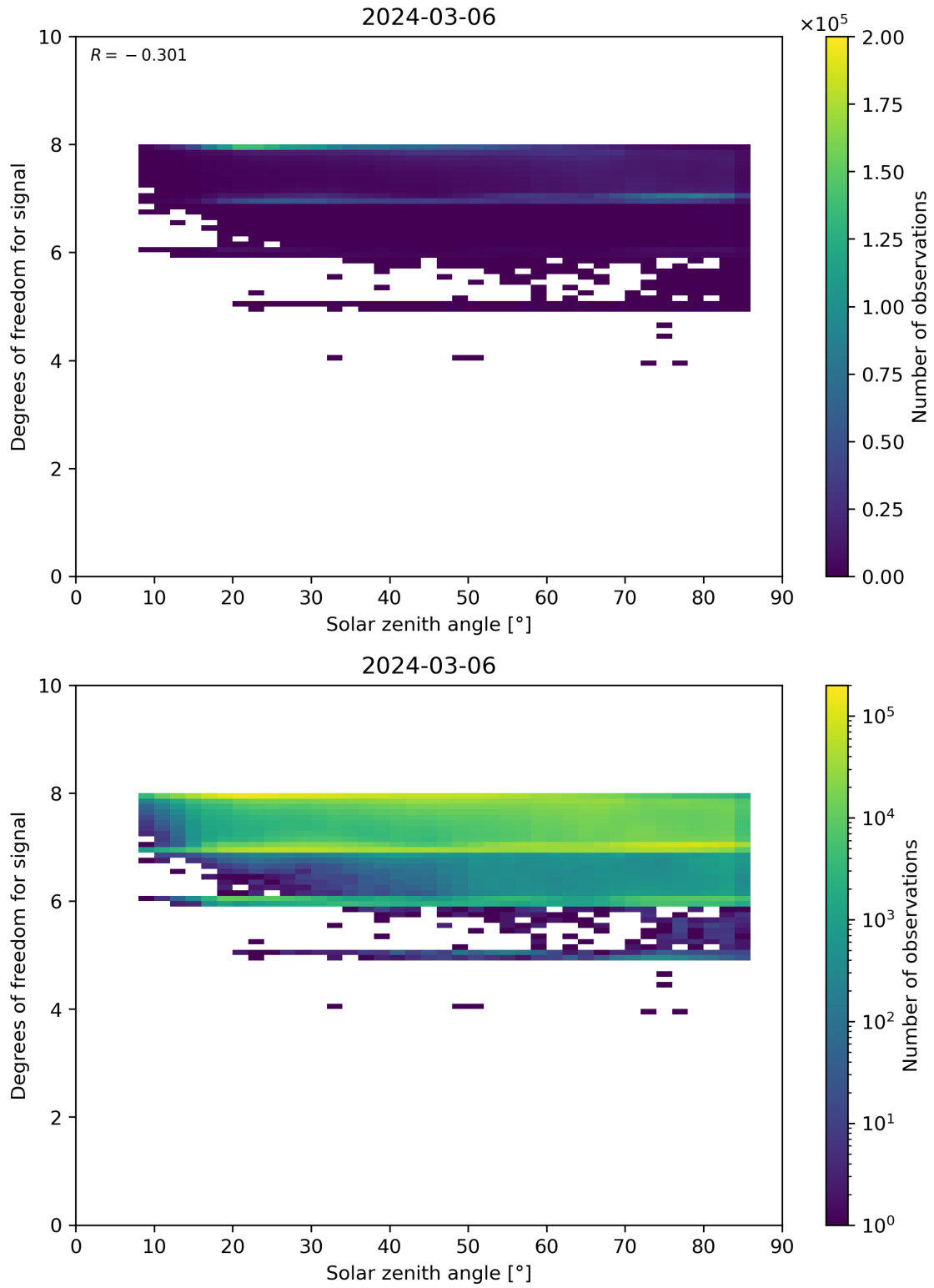
Figure 65: Scatter density plot of “Solar zenith angle” against “Degrees of freedom for signal” for 2024-03-05 to 2024-03-07.
