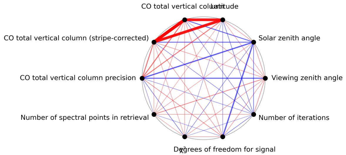
Figure 1: Map of correlation graph for 2024-03-05 to 2024-03-07.
