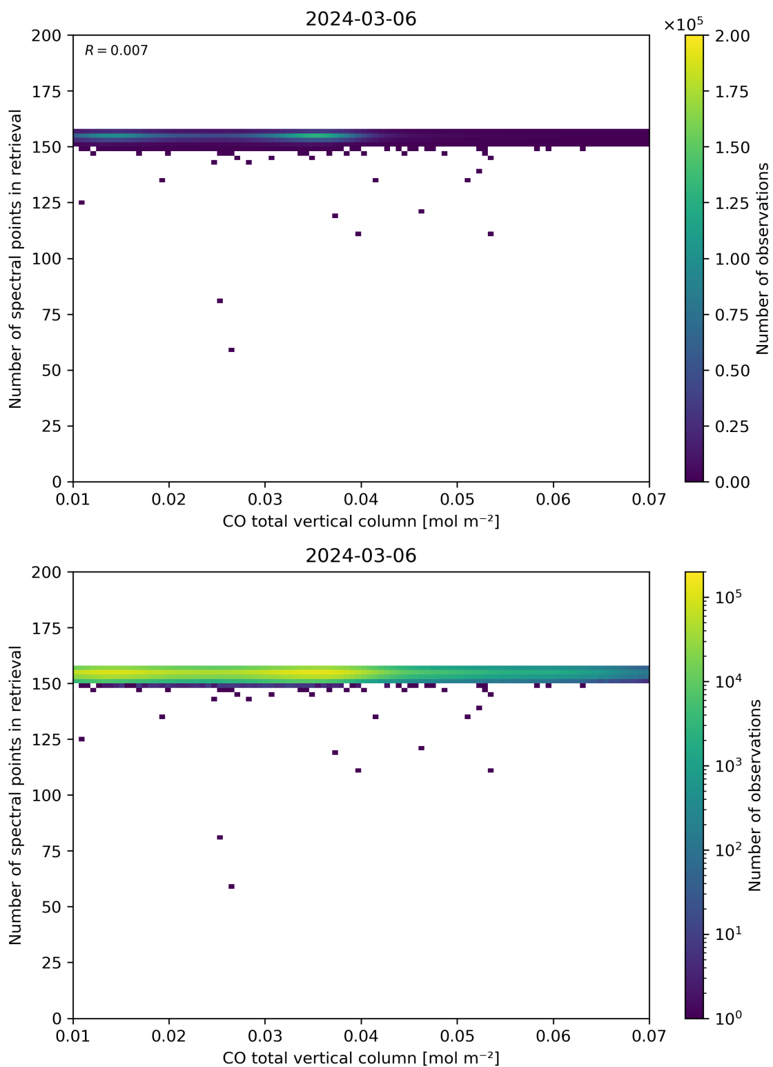
Figure 43: Scatter density plot of “CO total vertical column” against “Number of spectral points in retrieval” for 2024-03-05 to 2024-03-07.
