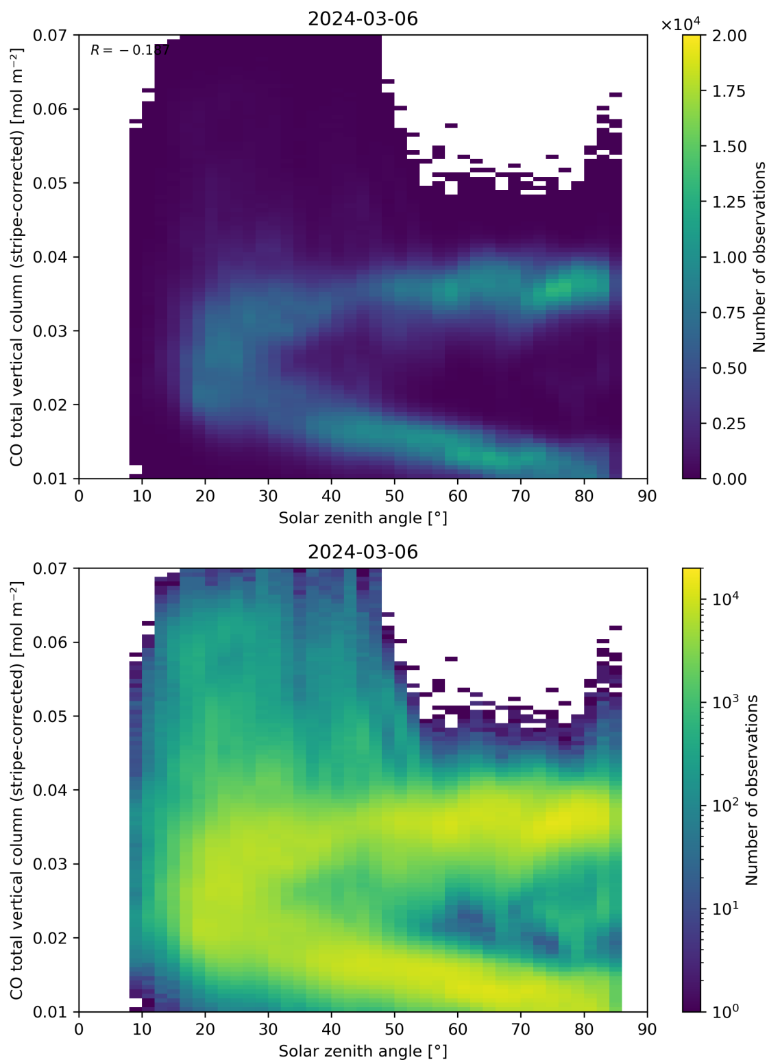
Figure 62: Scatter density plot of “Solar zenith angle” against “CO total vertical column (stripe-corrected)” for 2024-03-05 to 2024-03-07.
