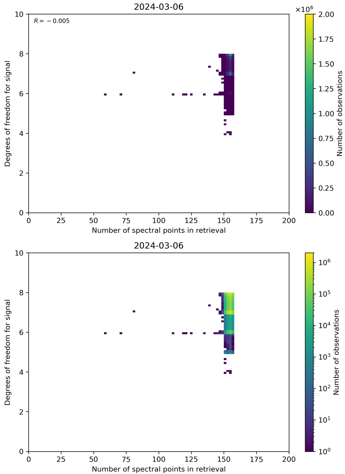
Figure 59: Scatter density plot of “Number of spectral points in retrieval” against “Degrees of freedom for signal” for 2024-03-05 to 2024-03-07.
