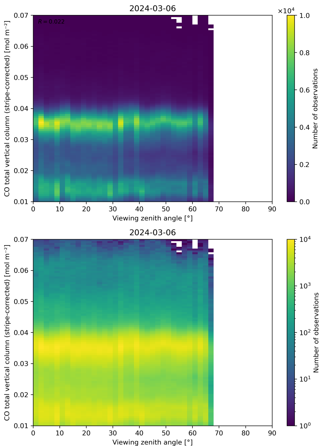
Figure 70: Scatter density plot of “Viewing zenith angle” against “CO total vertical column (stripe-corrected)” for 2024-03-05 to 2024-03-07.
