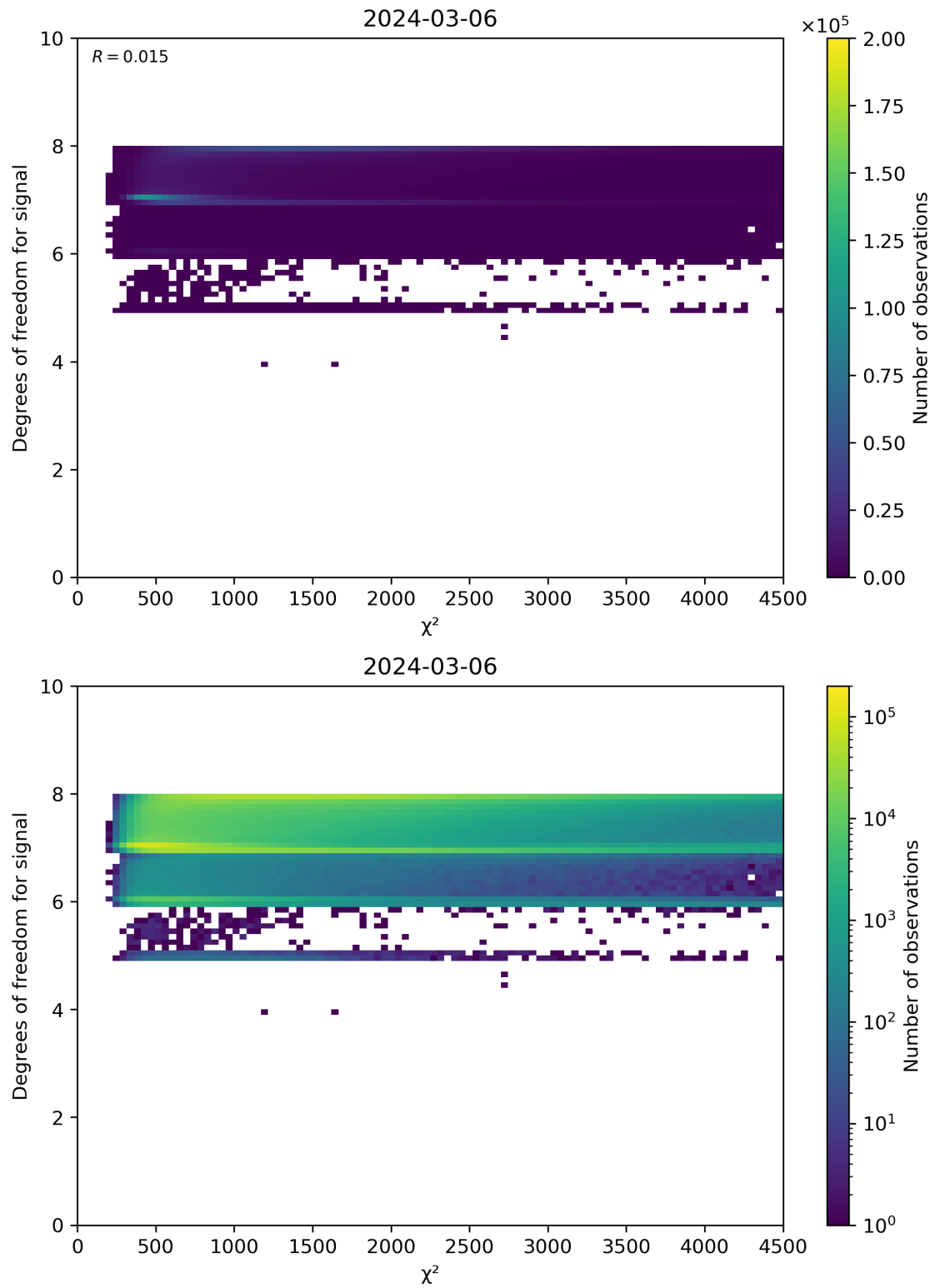
Figure 48: Scatter density plot of “ \chi^2 ” against “Degrees of freedom for signal” for 2024-03-05 to 2024-03-07.
