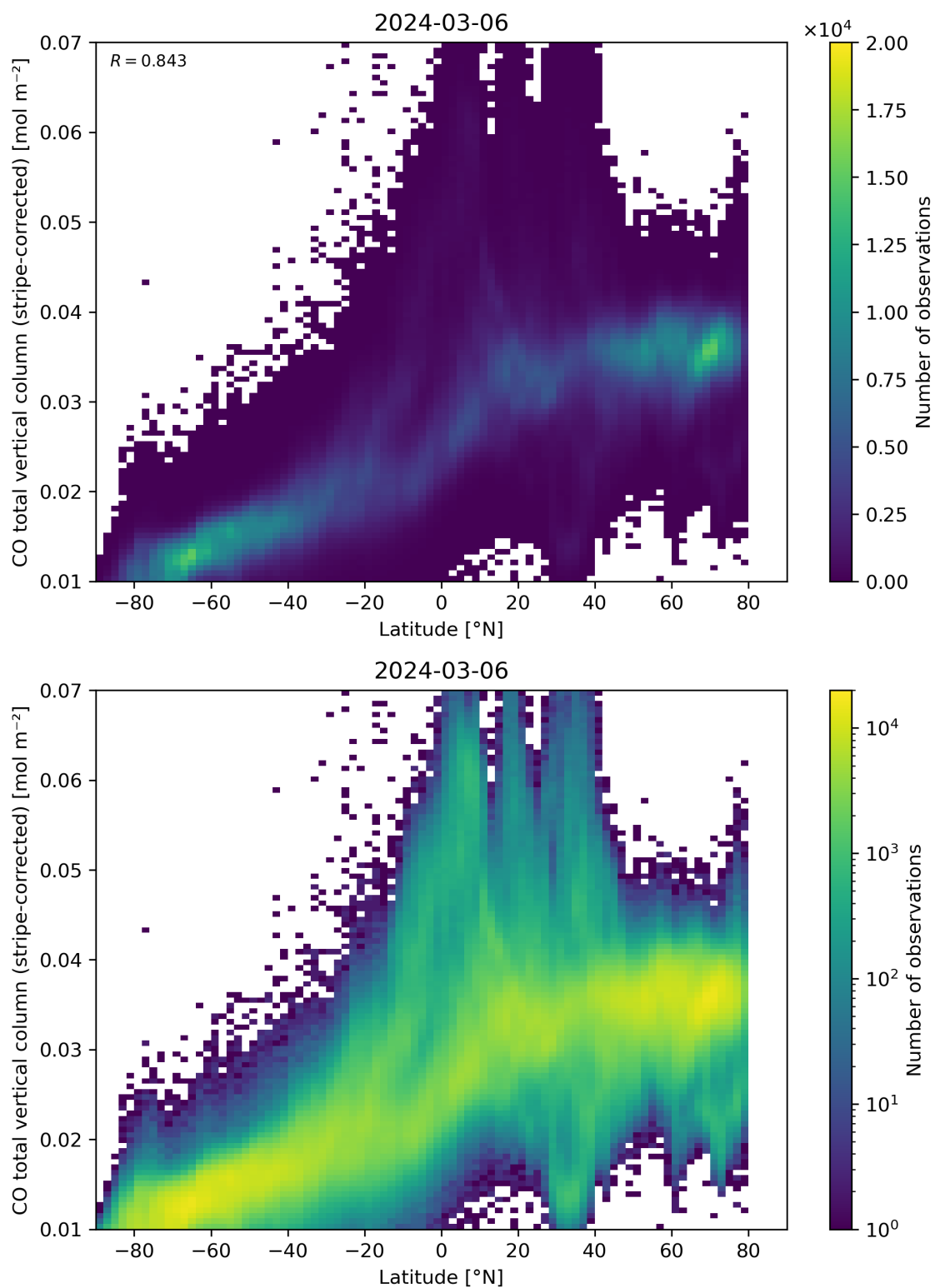
Figure 52: Scatter density plot of “Latitude” against “CO total vertical column (stripe-corrected)” for 2024-03-05 to 2024-03-07.
