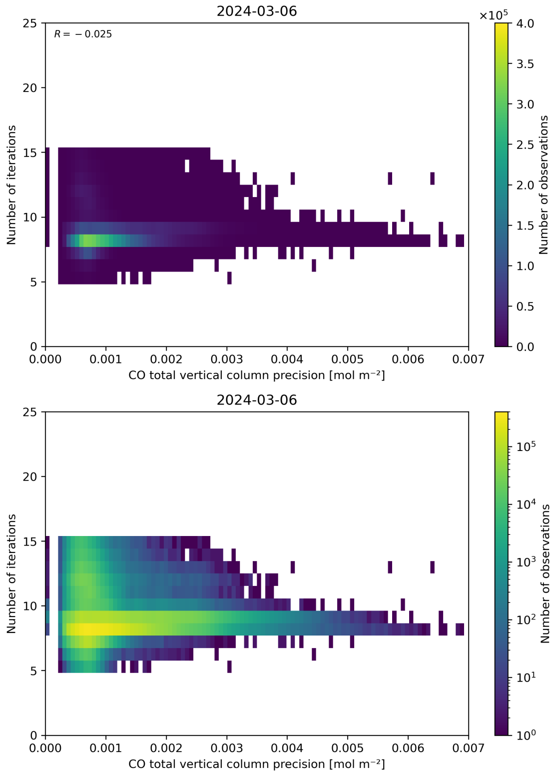
Figure 46: Scatter density plot of “CO total vertical column precision” against “Number of iterations” for 2024-03-05 to 2024-03-07.
