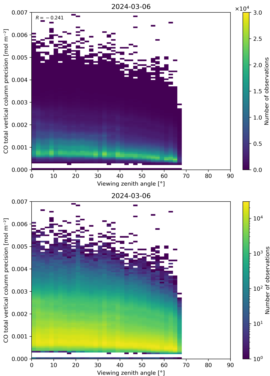
Figure 71: Scatter density plot of “Viewing zenith angle” against “CO total vertical column precision” for 2024-03-05 to 2024-03-07.
