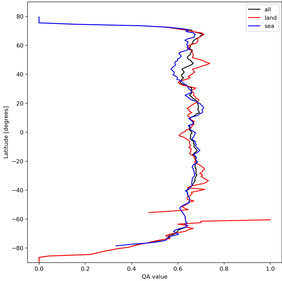
Figure 9: Zonal average of “QA value” for 2024-03-05 to 2024-03-07.
