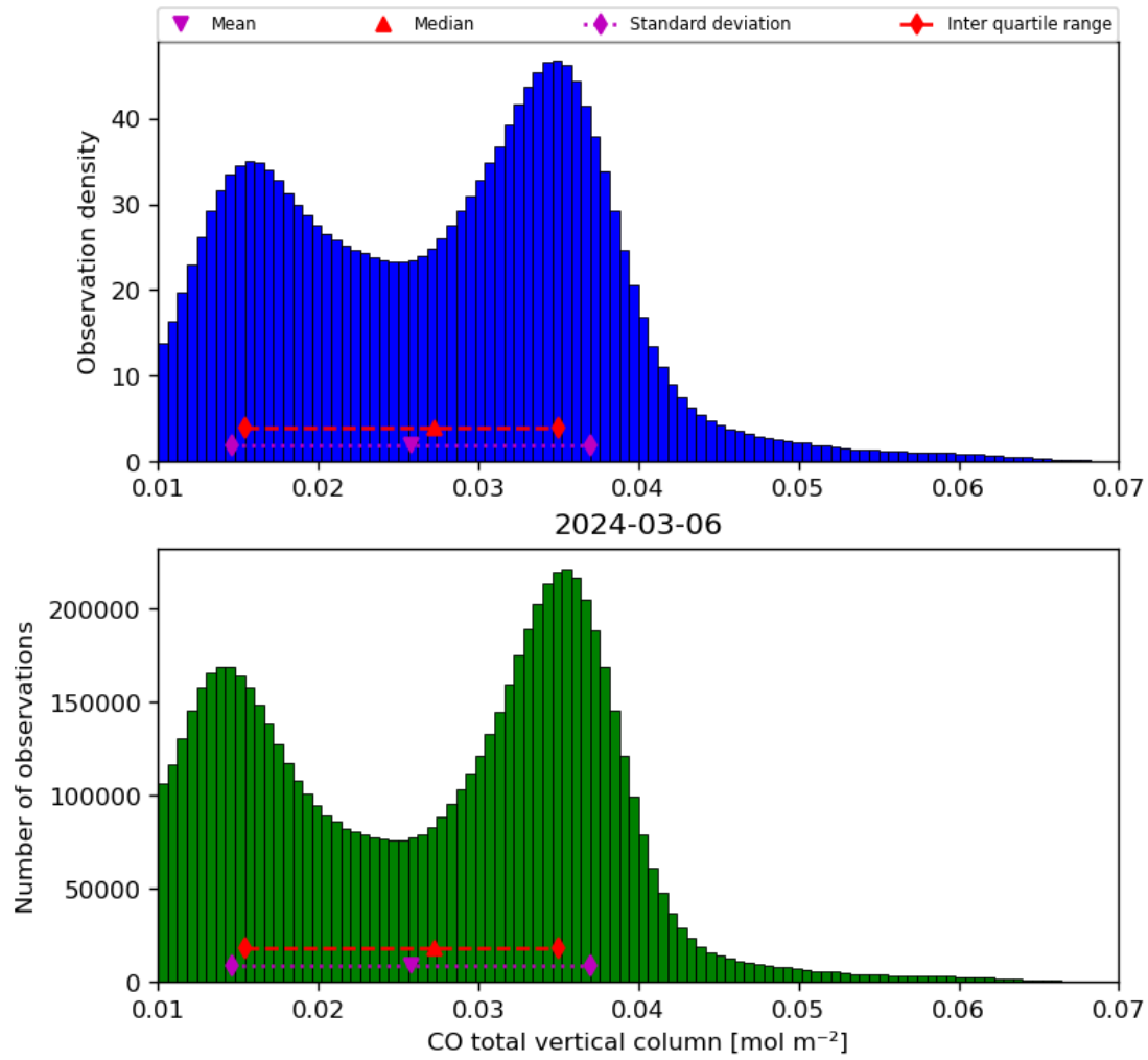
Figure 18: Histogram of “CO total vertical column” for 2024-03-05 to 2024-03-07
