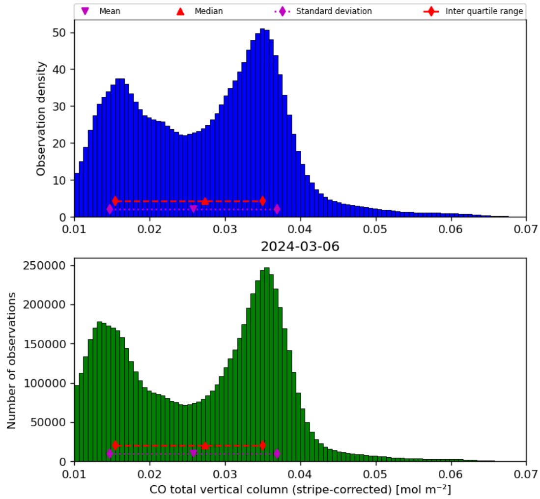
Figure 19: Histogram of “CO total vertical column (stripe-corrected)” for 2024-03-05 to 2024-03-07
