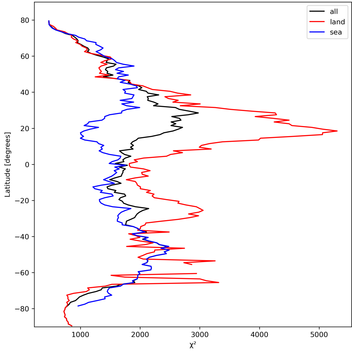
Figure 14: Zonal average of “ \chi^2 ” for 2024-03-05 to 2024-03-07.
