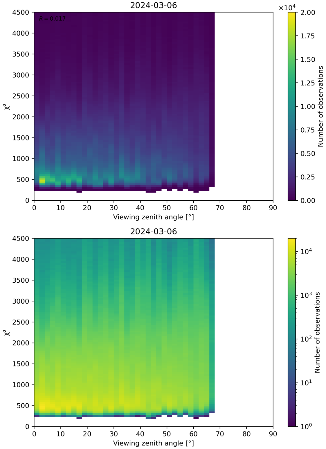
Figure 72: Scatter density plot of “Viewing zenith angle” against “ \chi^2 ” for 2024-03-05 to 2024-03-07.
