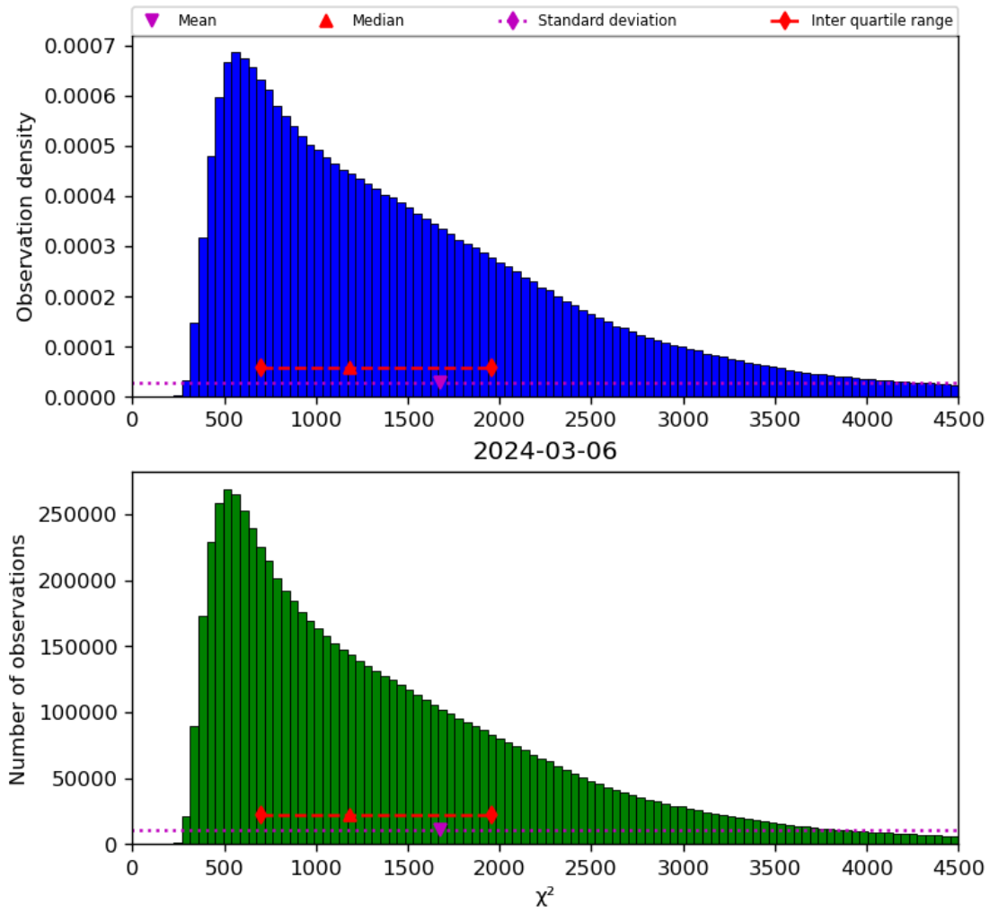
Figure 22: Histogram of “ \chi^2 ” for 2024-03-05 to 2024-03-07
