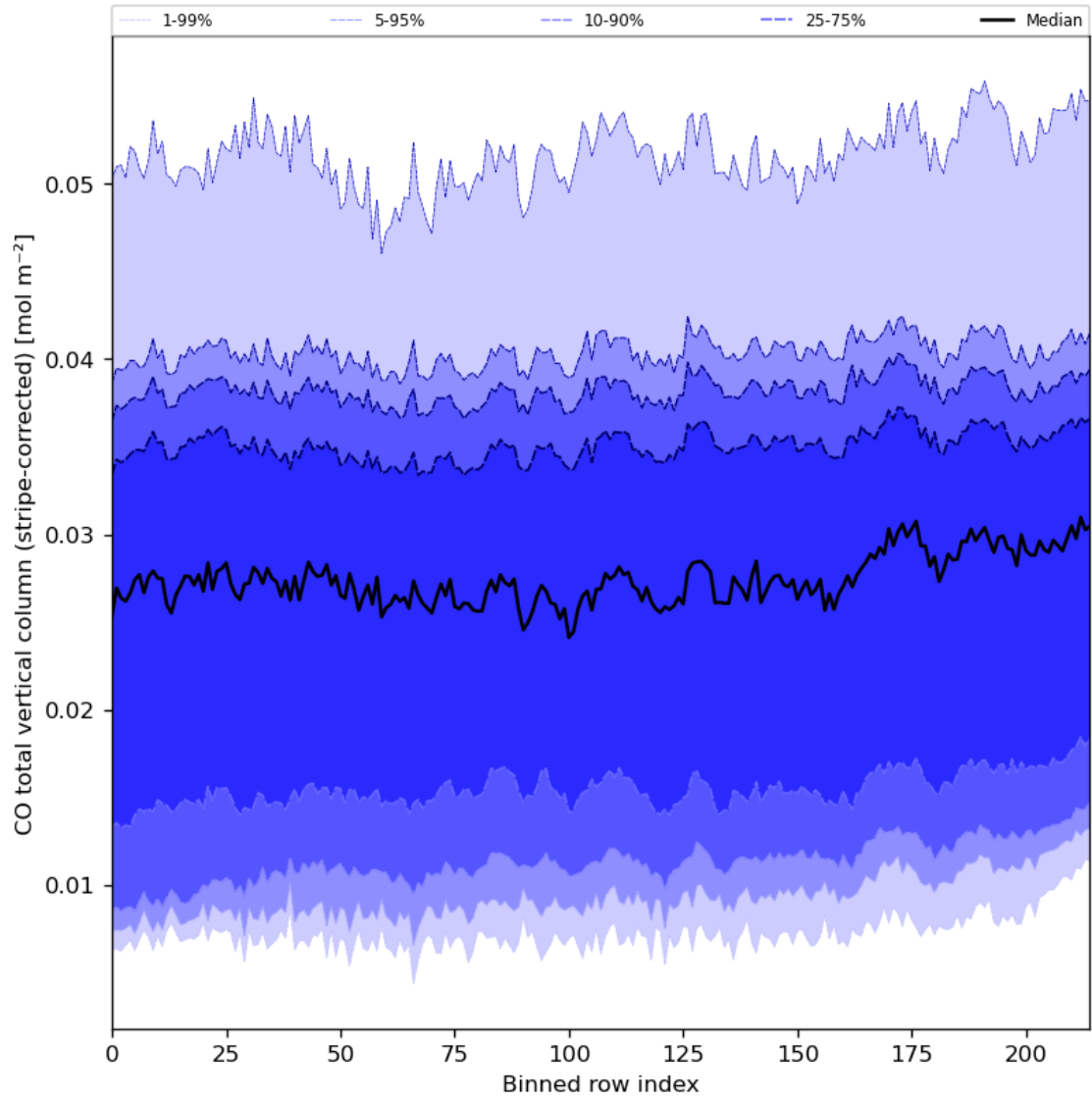
Figure 27: Along track statistics of “CO total vertical column (stripe-corrected)” for 2024-03-05 to 2024-03-07
