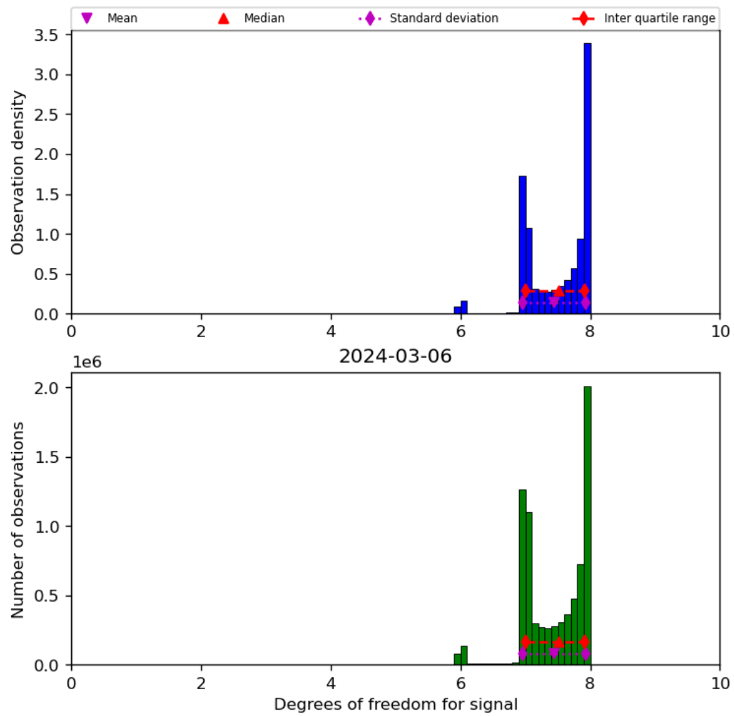
Figure 23: Histogram of “Degrees of freedom for signal” for 2024-03-05 to 2024-03-07
