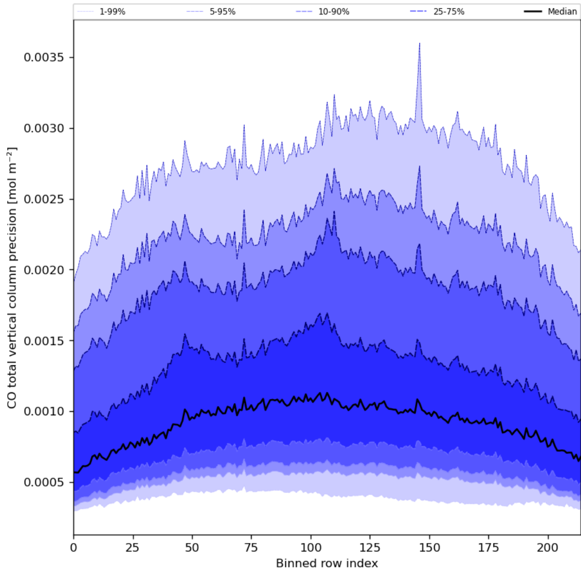
Figure 28: Along track statistics of “CO total vertical column precision” for 2024-03-05 to 2024-03-07
