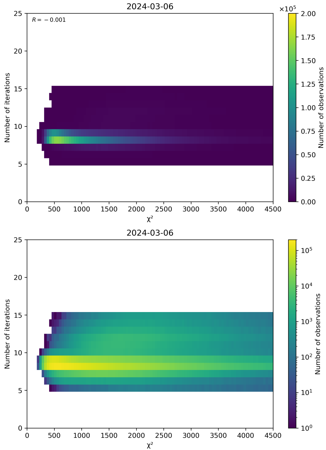
Figure 49: Scatter density plot of “ \chi^2 ” against “Number of iterations” for 2024-03-05 to 2024-03-07.
