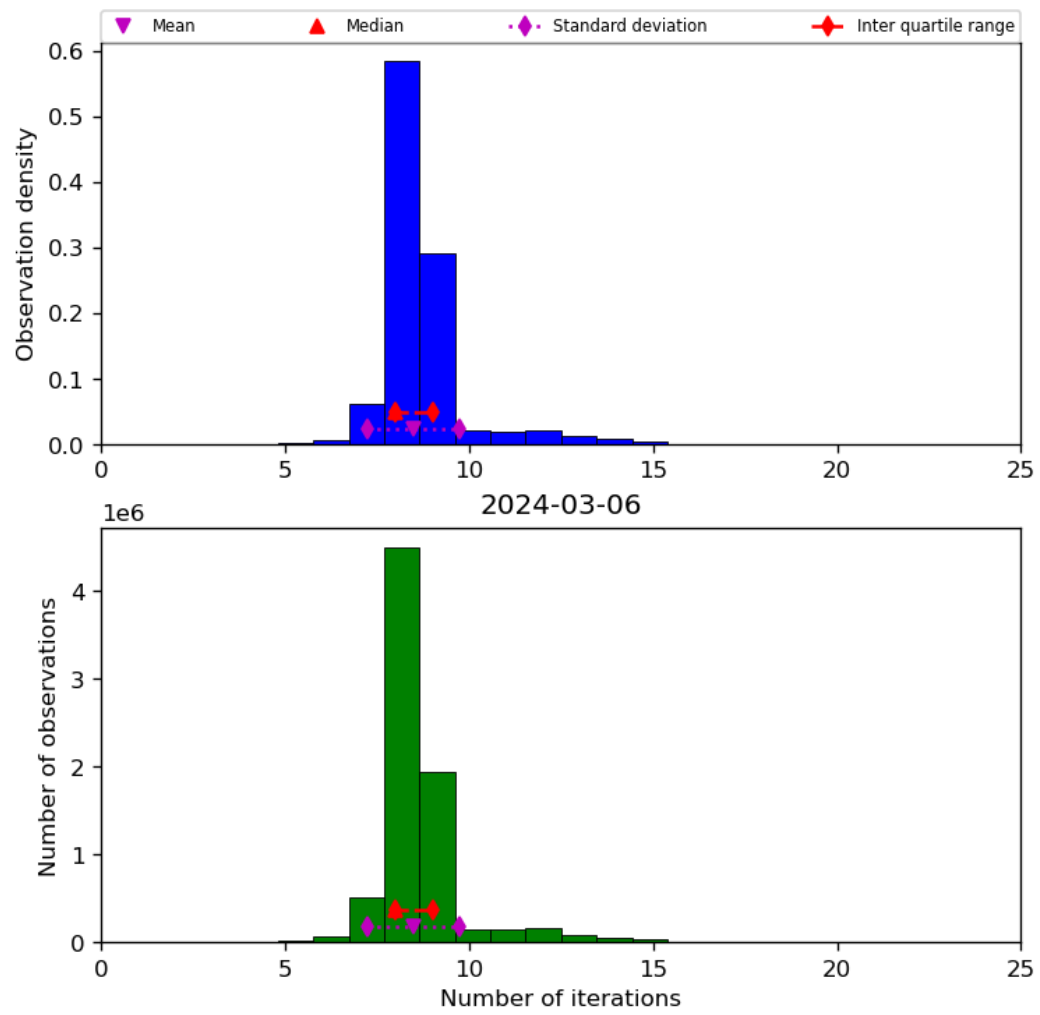
Figure 24: Histogram of “Number of iterations” for 2024-03-05 to 2024-03-07
