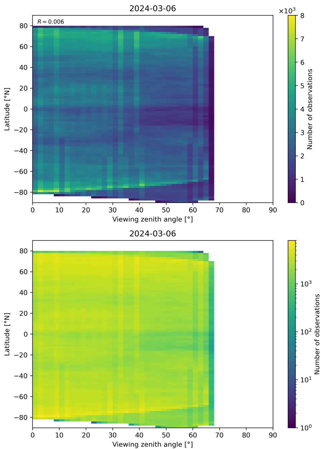
Figure 74: Scatter density plot of “Viewing zenith angle” against “Latitude” for 2024-03-05 to 2024-03-07.
