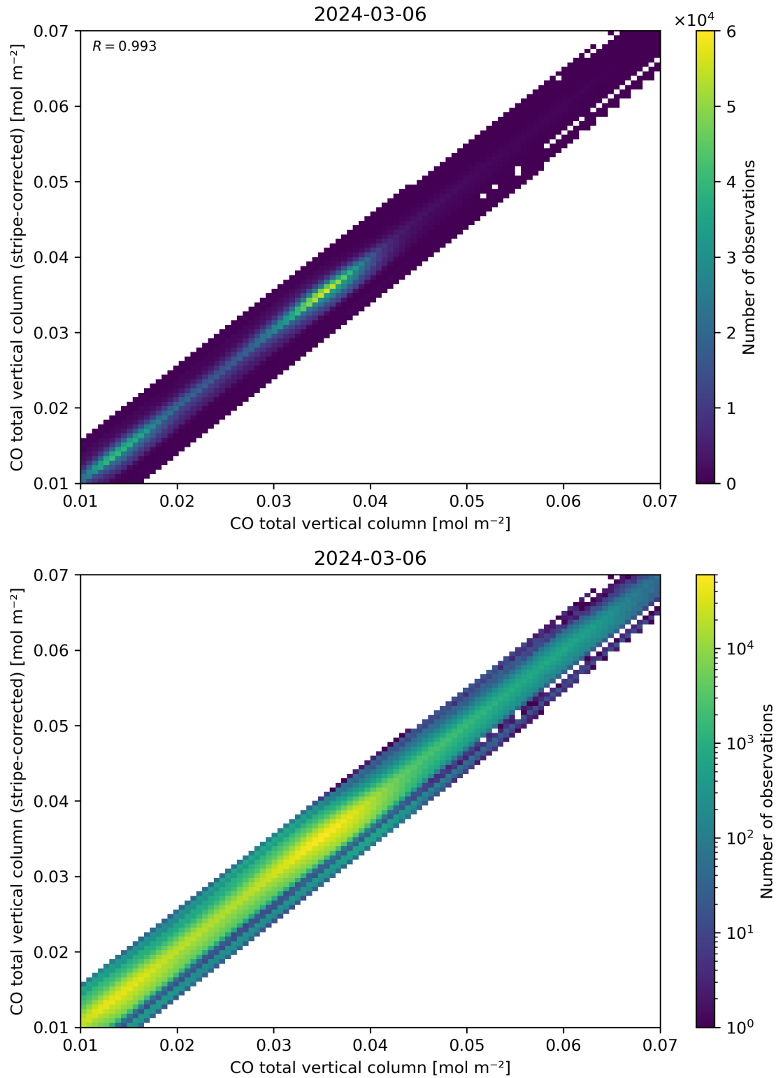
Figure 33: Scatter density plot of “CO total vertical column” against “CO total vertical column (stripe-corrected)” for 2024-03-05 to 2024-03-07.
