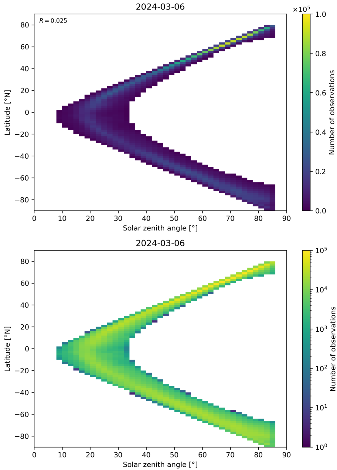
Figure 66: Scatter density plot of “Solar zenith angle” against “Latitude” for 2024-03-05 to 2024-03-07.
