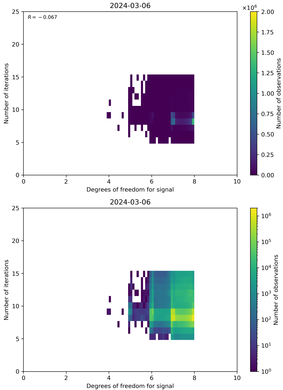
Figure 50: Scatter density plot of “Degrees of freedom for signal” against “Number of iterations” for 2024-03-05 to 2024-03-07.
