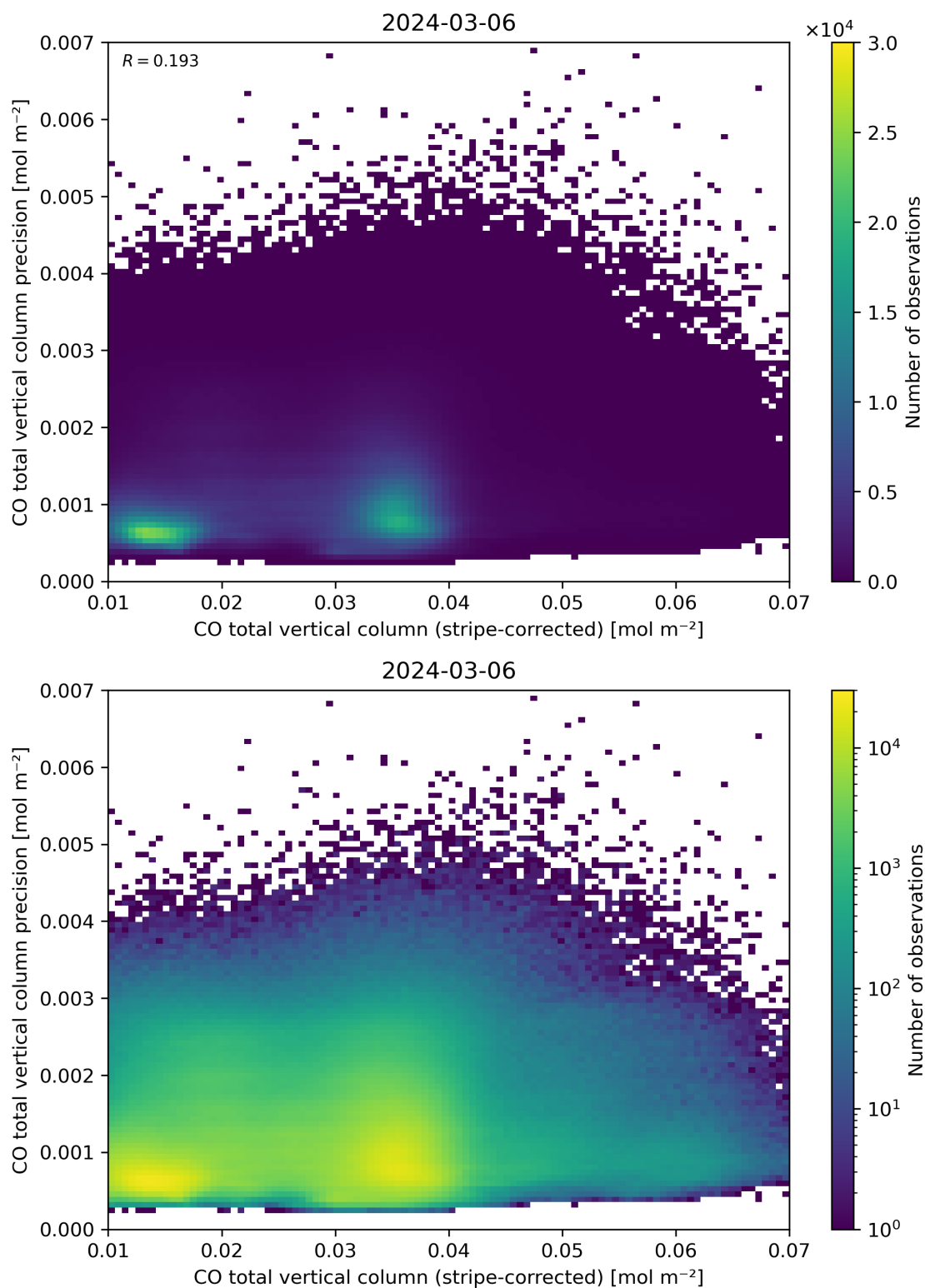
Figure 36: Scatter density plot of “CO total vertical column (stripe-corrected)” against “CO total vertical column precision” for 2024-03-05 to 2024-03-07.
