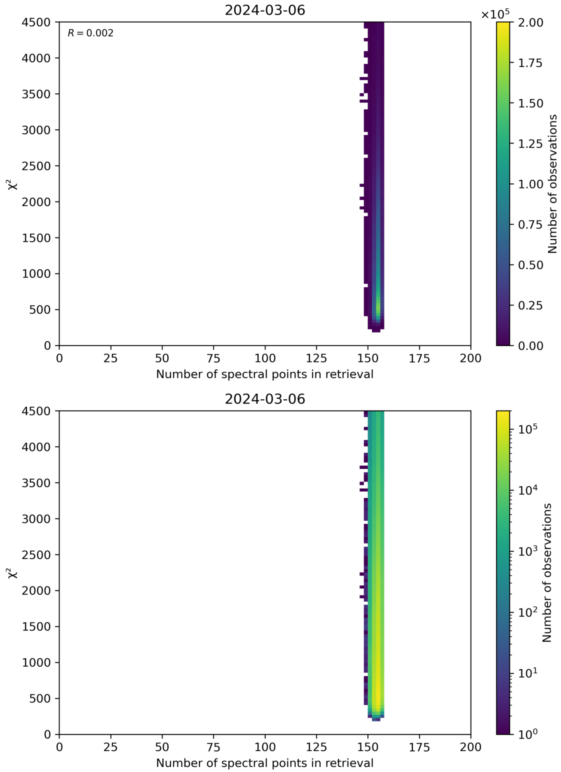
Figure 58: Scatter density plot of “Number of spectral points in retrieval” against “ \chi^2 ” for 2024-03-05 to 2024-03-07.
