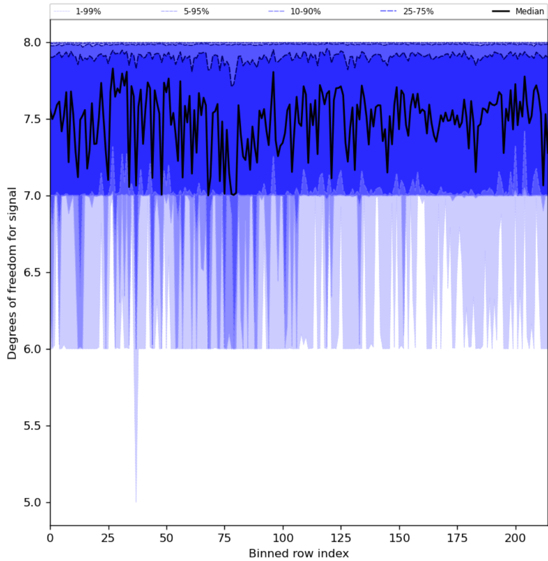
Figure 31: Along track statistics of “Degrees of freedom for signal” for 2024-03-05 to 2024-03-07
