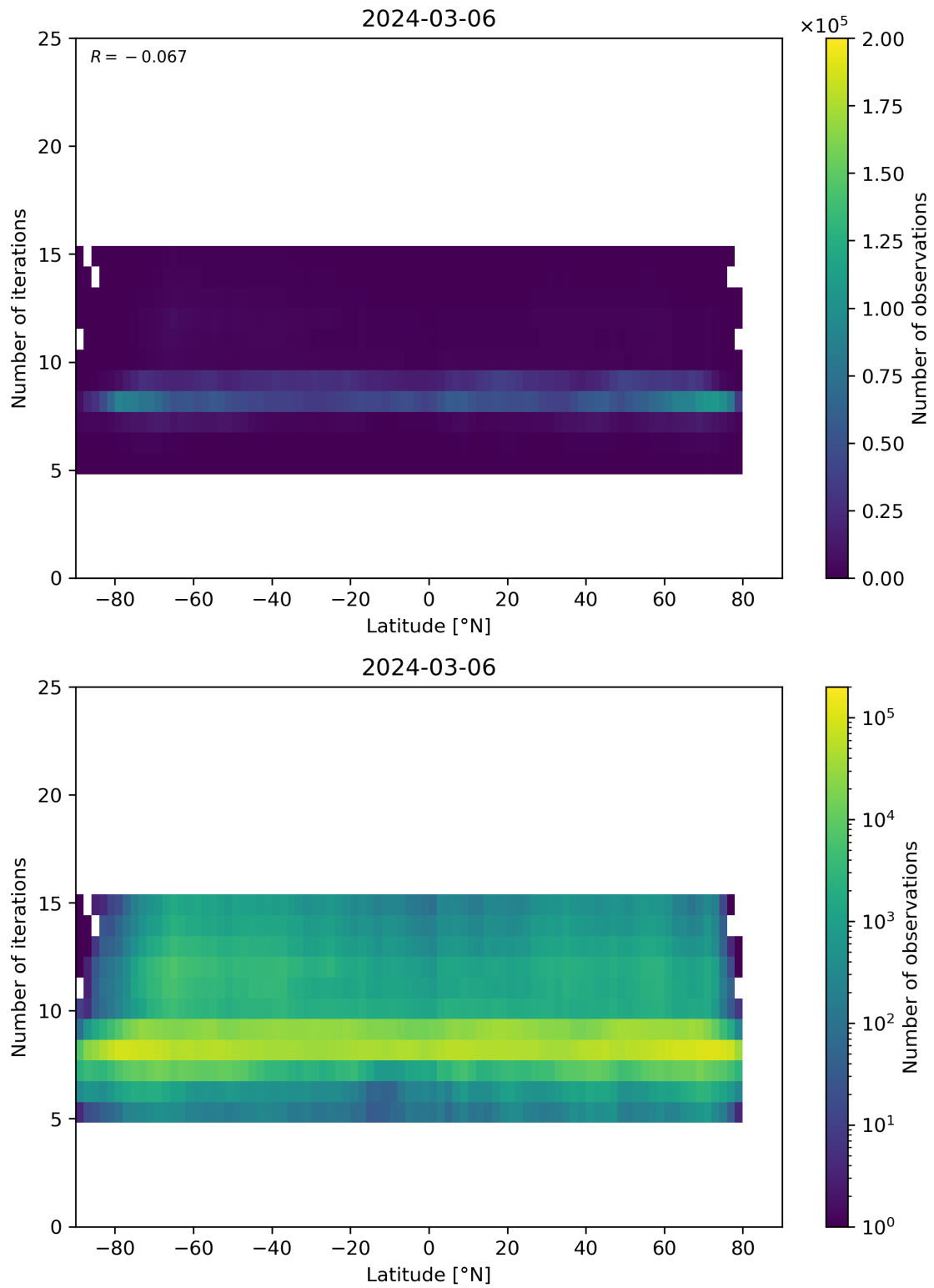
Figure 56: Scatter density plot of “Latitude” against “Number of iterations” for 2024-03-05 to 2024-03-07.
