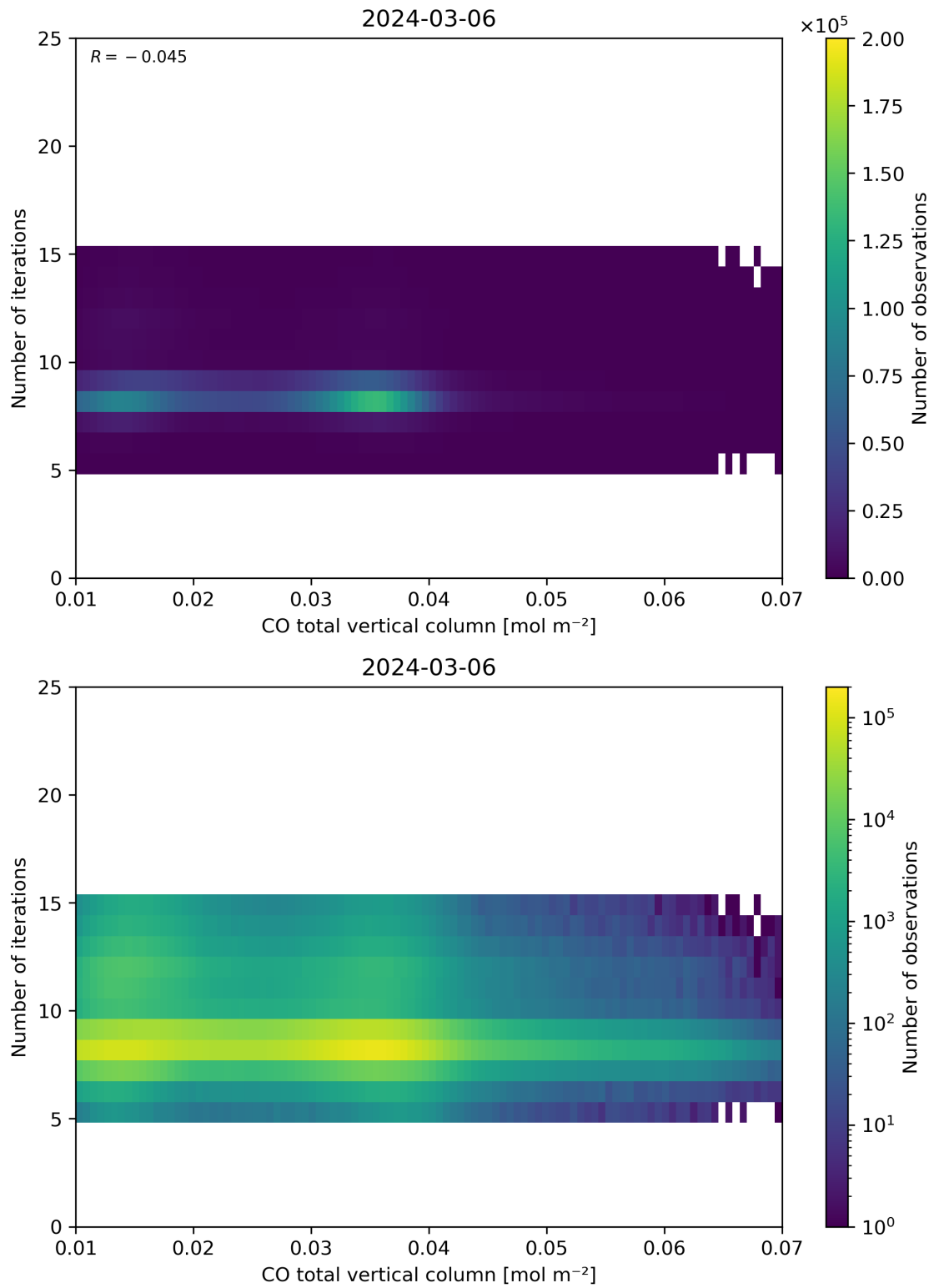
Figure 42: Scatter density plot of “CO total vertical column” against “Number of iterations” for 2024-03-05 to 2024-03-07.
