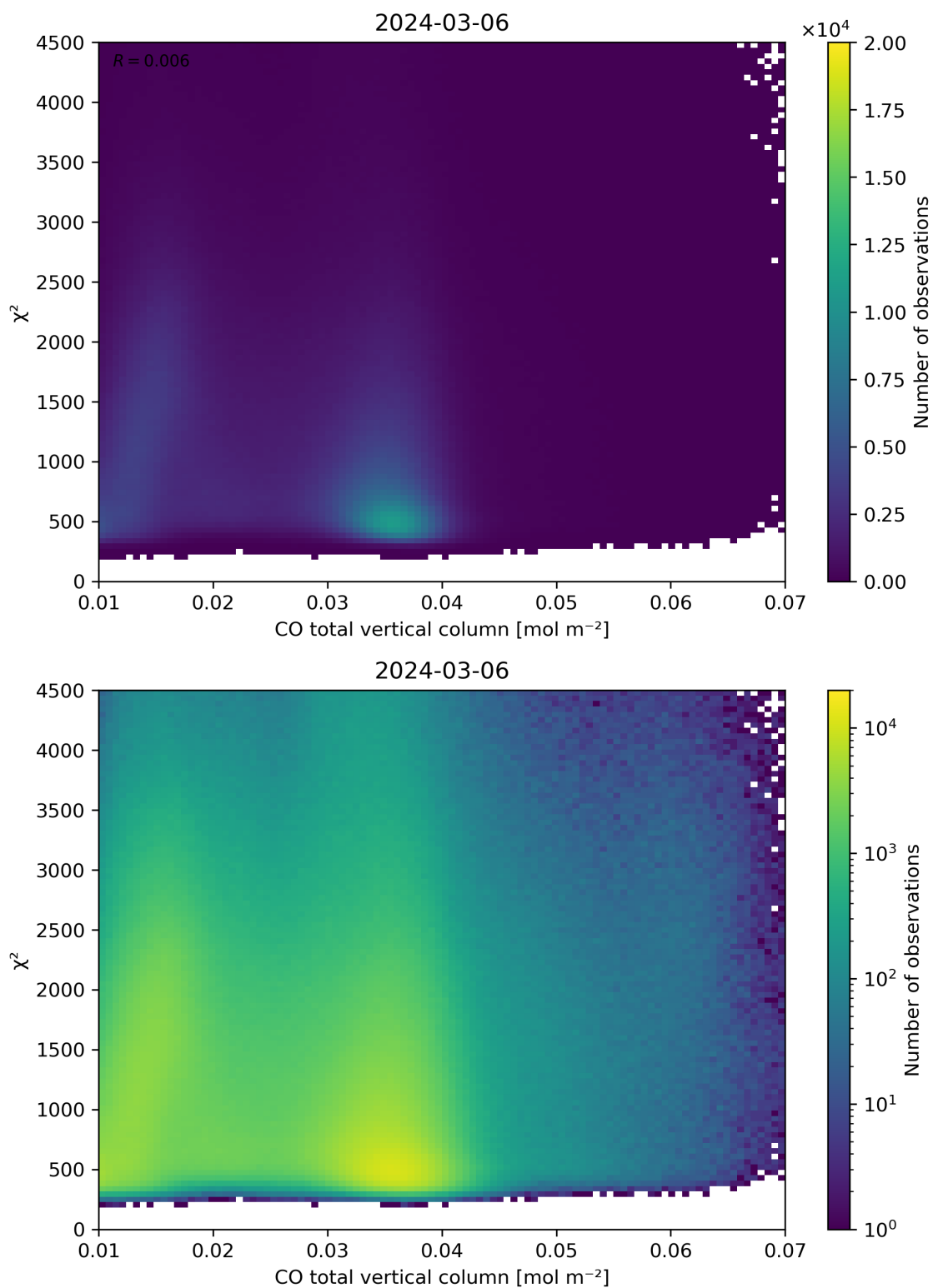
Figure 35: Scatter density plot of “CO total vertical column” against “ \chi^2 ” for 2024-03-05 to 2024-03-07.
