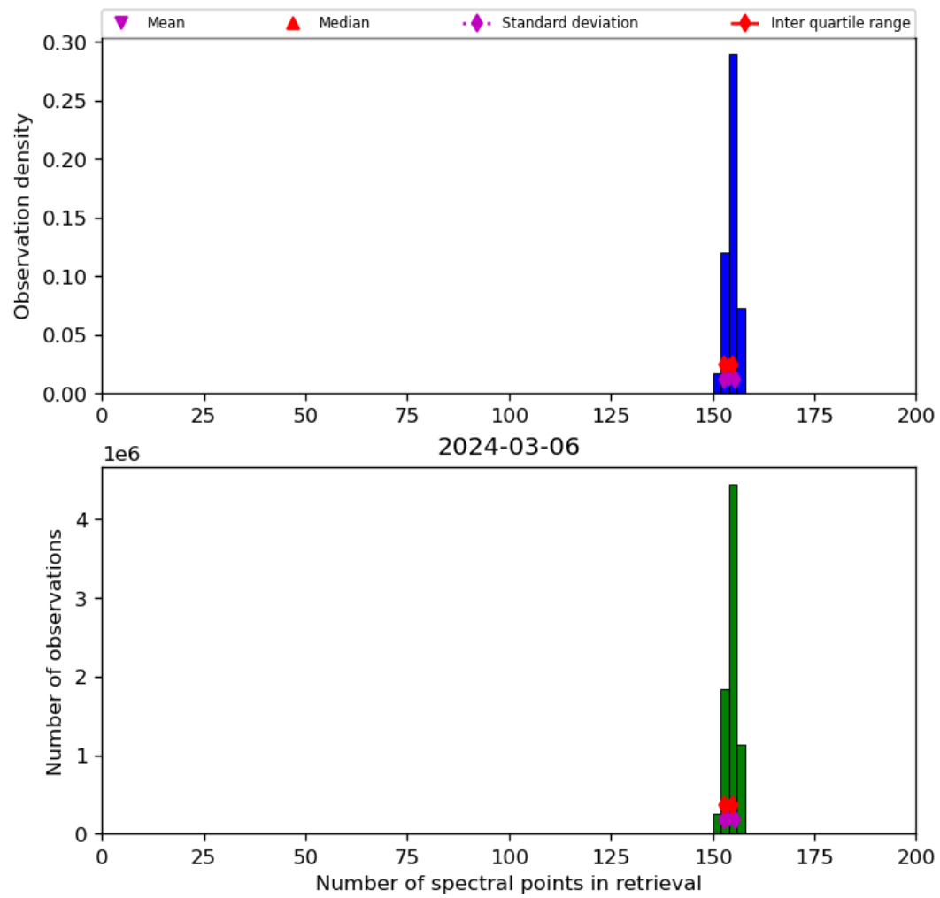
Figure 21: Histogram of “Number of spectral points in retrieval” for 2024-03-05 to 2024-03-07
