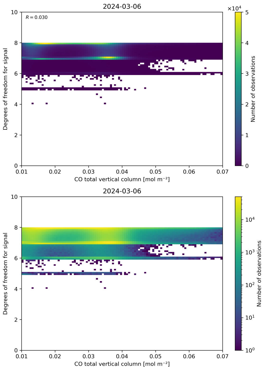
Figure 41: Scatter density plot of “CO total vertical column” against “Degrees of freedom for signal” for 2024-03-05 to 2024-03-07.
