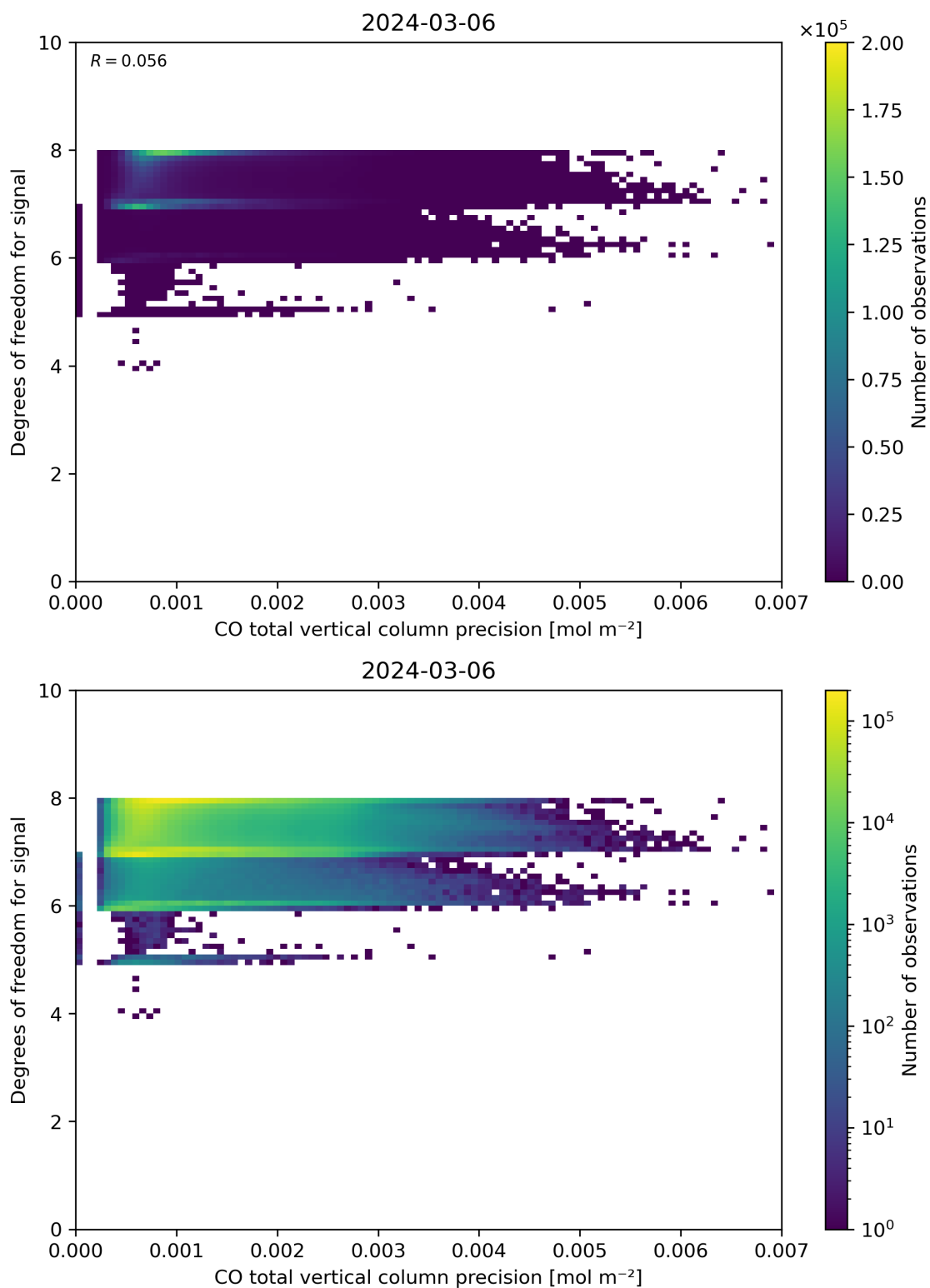
Figure 45: Scatter density plot of “CO total vertical column precision” against “Degrees of freedom for signal” for 2024-03-05 to 2024-03-07.
