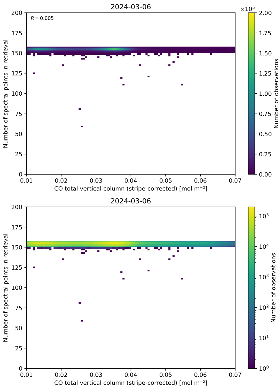
Figure 40: Scatter density plot of “CO total vertical column (stripe-corrected)” against “Number of spectral points in retrieval” for 2024-03-05 to 2024-03-07.
