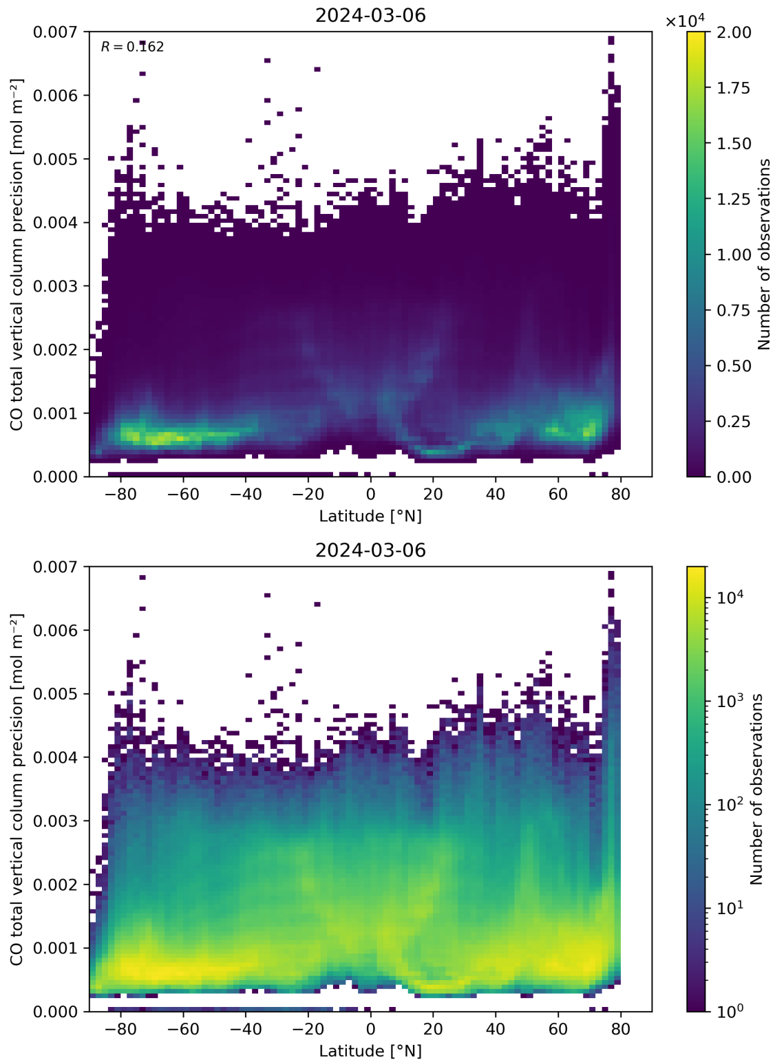
Figure 53: Scatter density plot of “Latitude” against “CO total vertical column precision” for 2024-03-05 to 2024-03-07.
