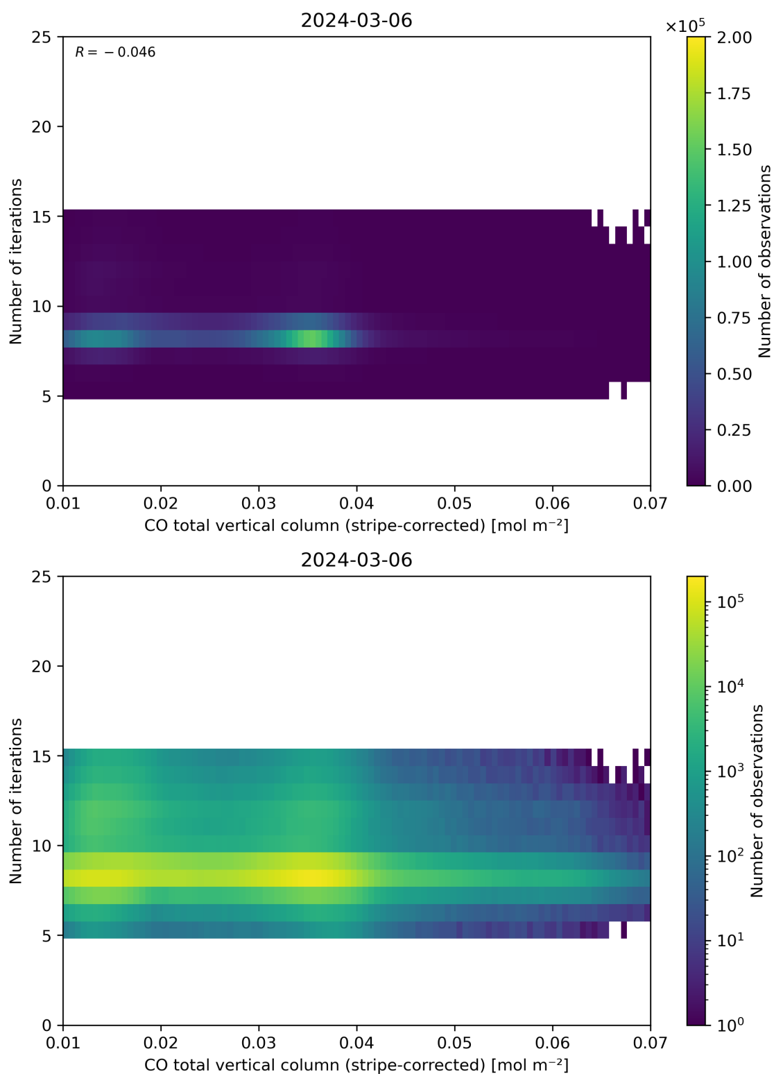
Figure 39: Scatter density plot of “CO total vertical column (stripe-corrected)” against “Number of iterations” for 2024-03-05 to 2024-03-07.
