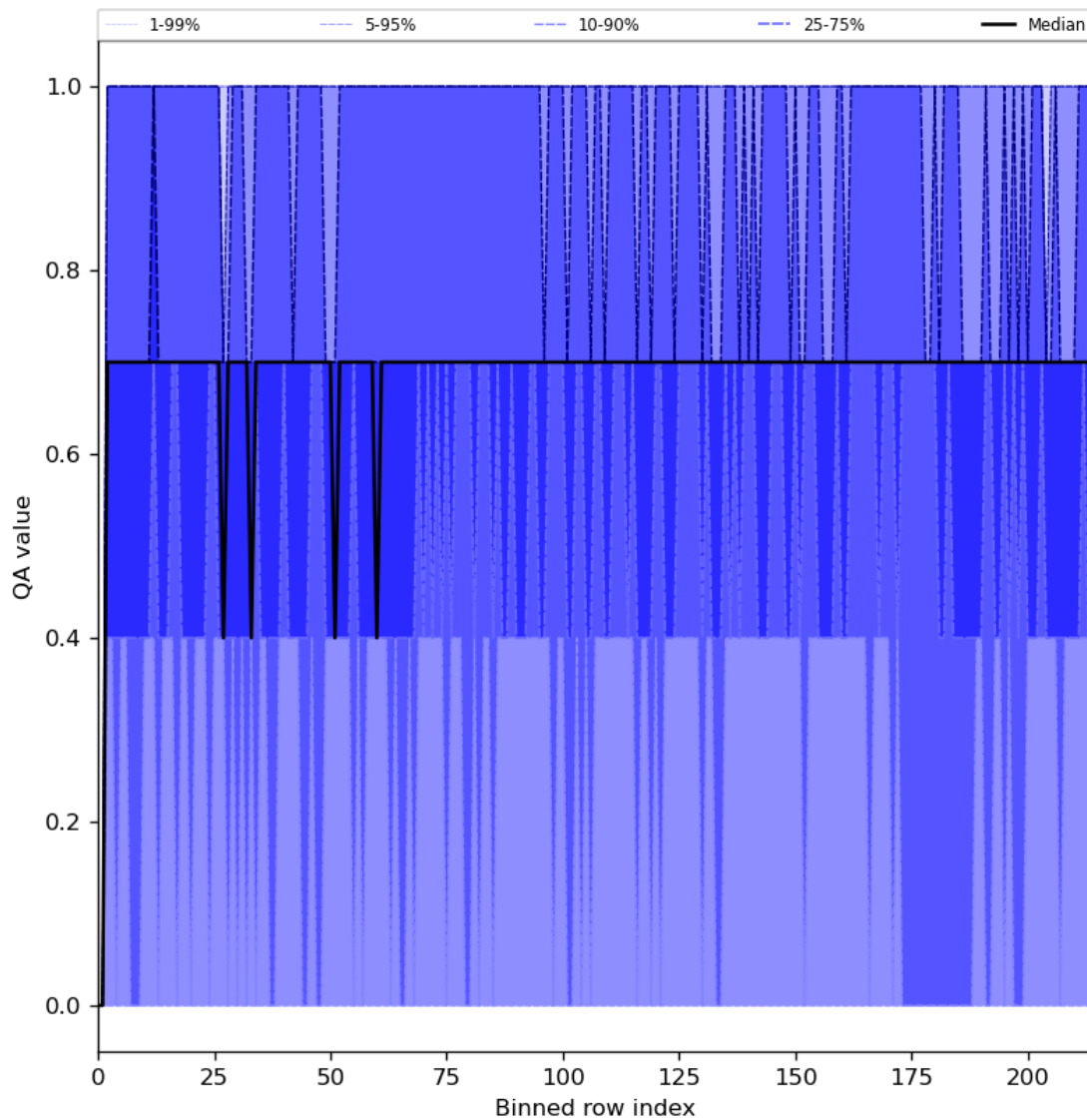
Figure 25: Along track statistics of “QA value” for 2024-03-05 to 2024-03-07
