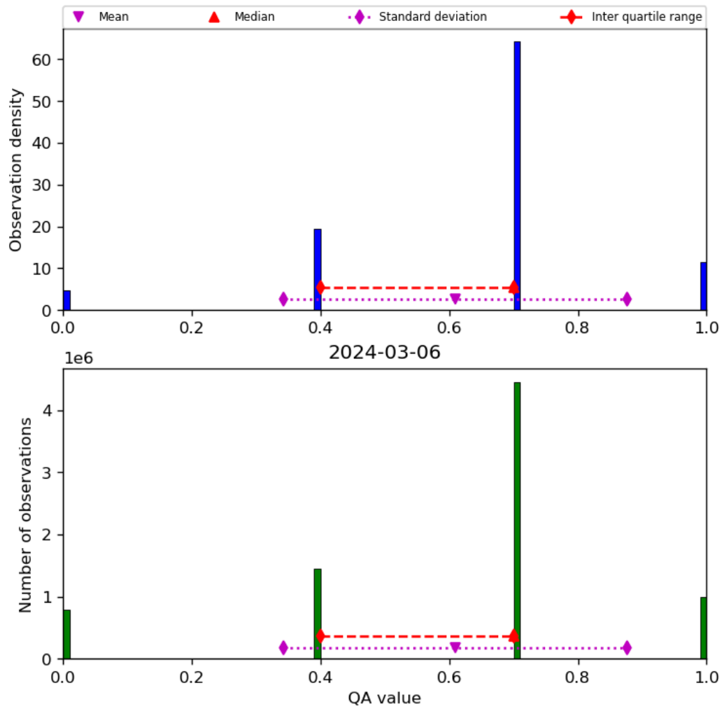
Figure 17: Histogram of “QA value” for 2024-03-05 to 2024-03-07
