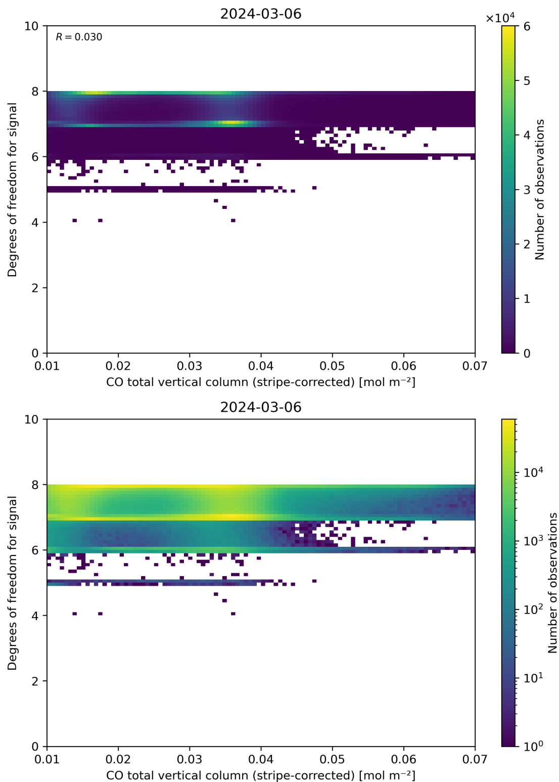
Figure 38: Scatter density plot of “CO total vertical column (stripe-corrected)” against “Degrees of freedom for signal” for 2024-03-05 to 2024-03-07.
