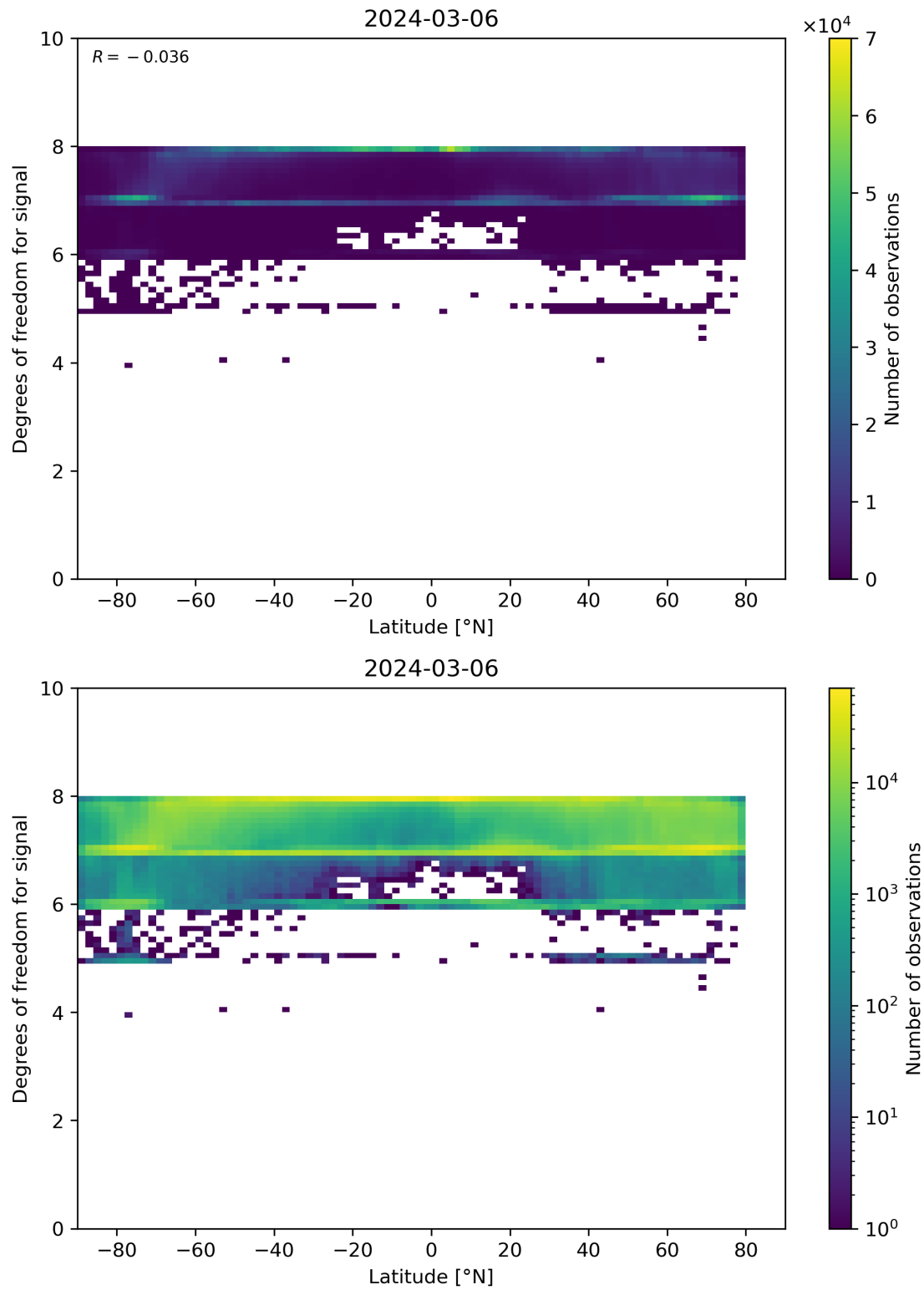
Figure 55: Scatter density plot of “Latitude” against “Degrees of freedom for signal” for 2024-03-05 to 2024-03-07.
