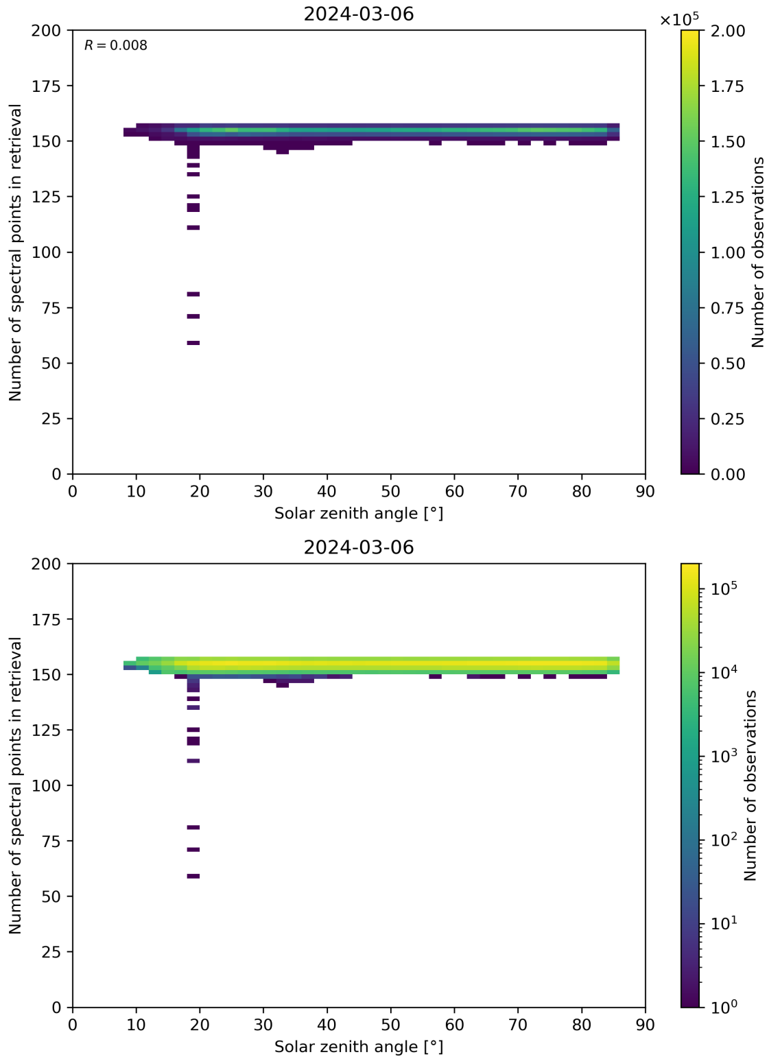
Figure 68: Scatter density plot of “Solar zenith angle” against “Number of spectral points in retrieval” for 2024-03-05 to 2024-03-07.
