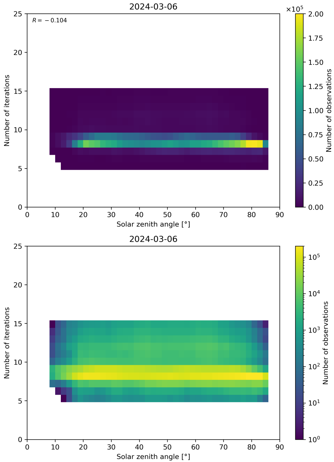
Figure 67: Scatter density plot of “Solar zenith angle” against “Number of iterations” for 2024-03-05 to 2024-03-07.
