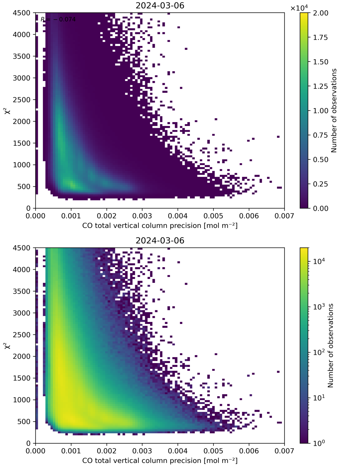
Figure 44: Scatter density plot of “CO total vertical column precision” against “ \chi^2 ” for 2024-03-05 to 2024-03-07.
