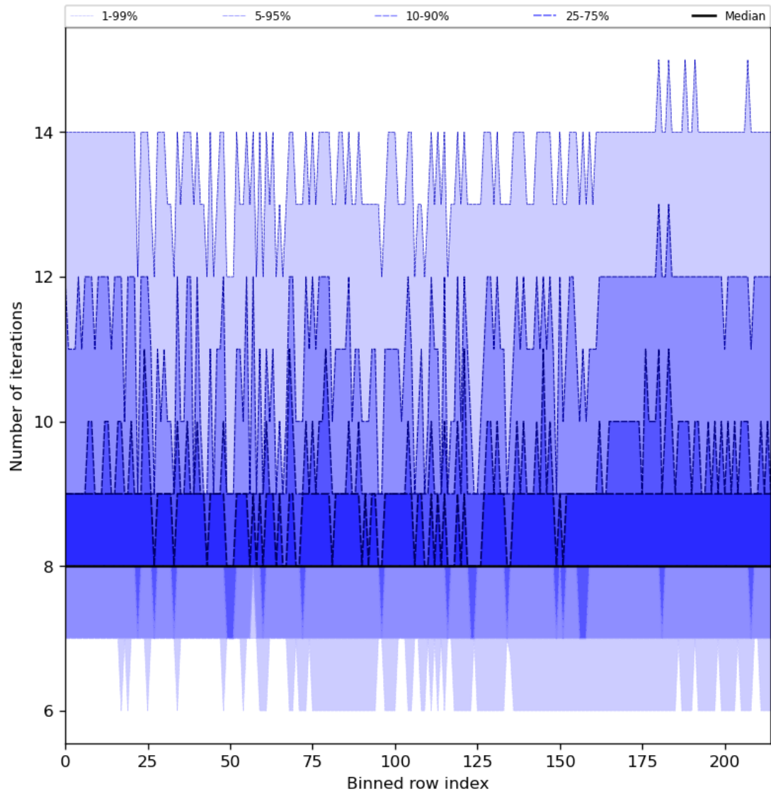
Figure 32: Along track statistics of “Number of iterations” for 2024-03-05 to 2024-03-07
