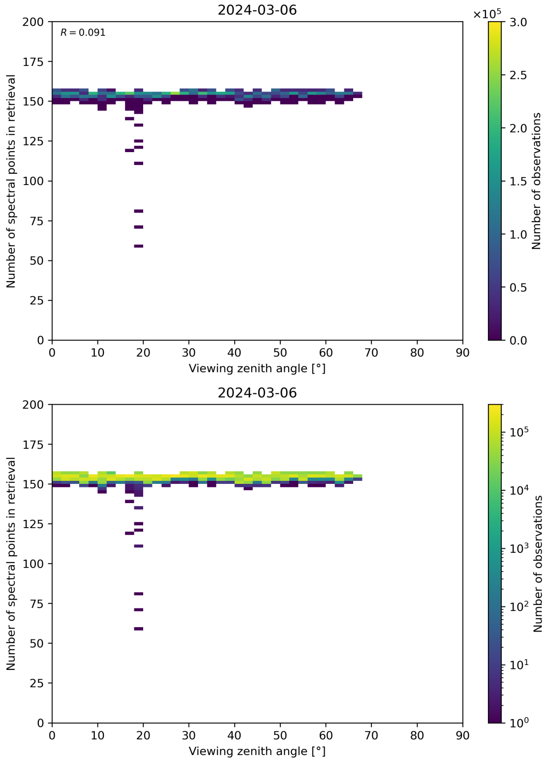
Figure 76: Scatter density plot of “Viewing zenith angle” against “Number of spectral points in retrieval” for 2024-03-05 to 2024-03-07.
