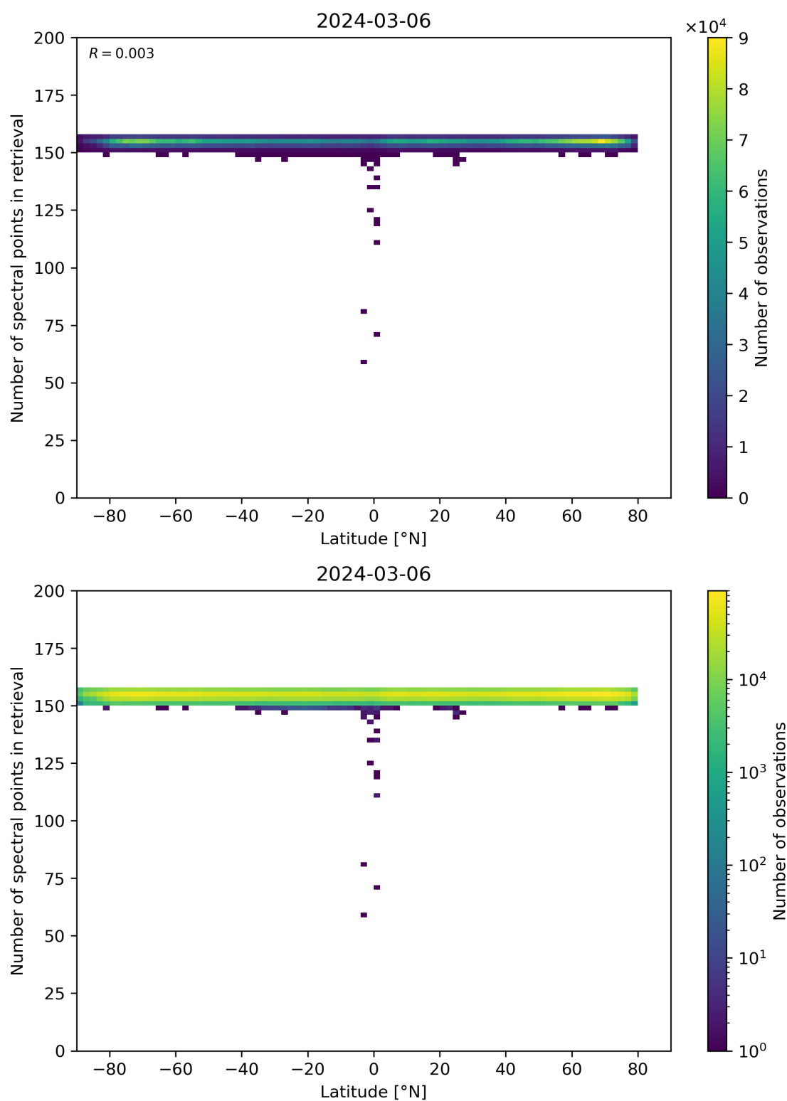
Figure 57: Scatter density plot of “Latitude” against “Number of spectral points in retrieval” for 2024-03-05 to 2024-03-07.
