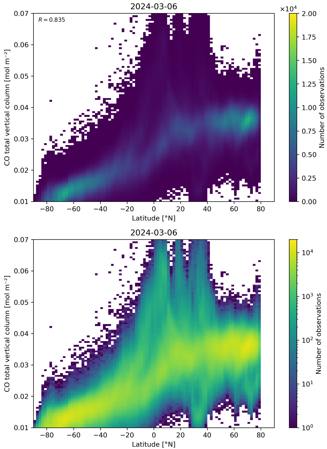
Figure 51: Scatter density plot of “Latitude” against “CO total vertical column” for 2024-03-05 to 2024-03-07.
