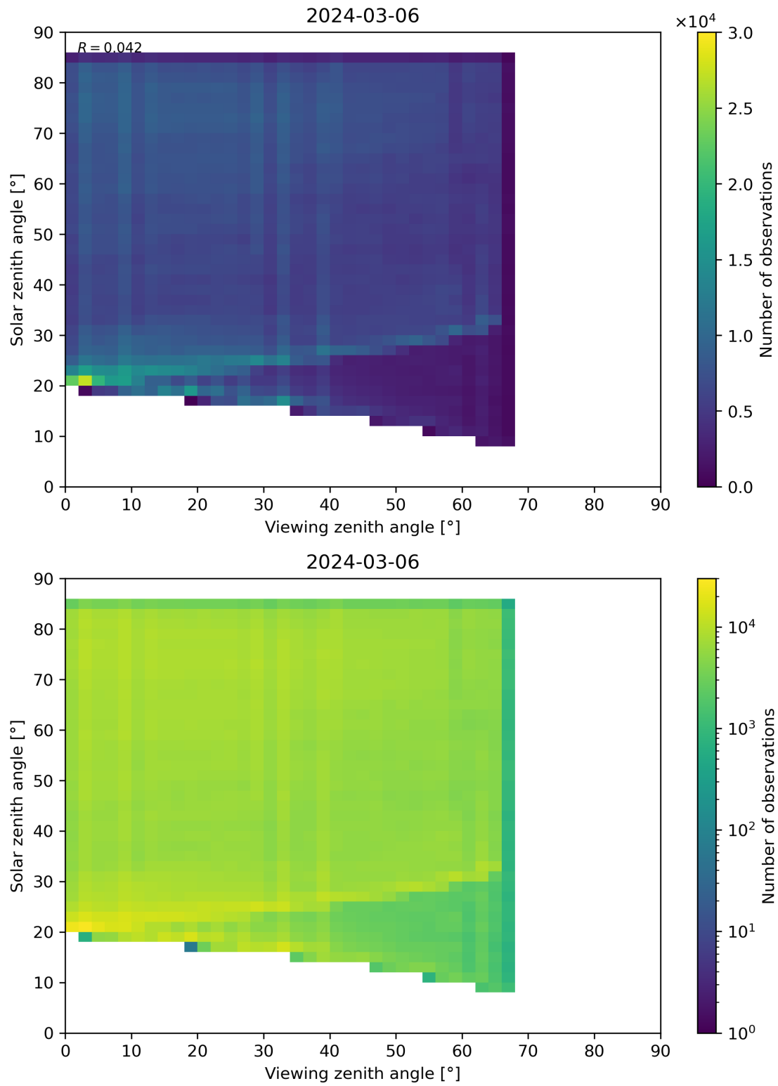
Figure 77: Scatter density plot of “Viewing zenith angle” against “Solar zenith angle” for 2024-03-05 to 2024-03-07.
