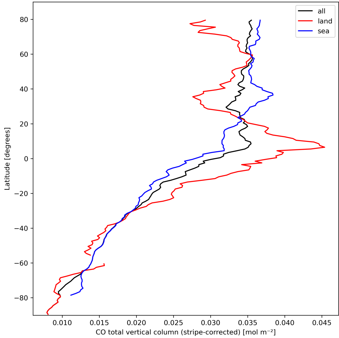
Figure 11: Zonal average of “CO total vertical column (stripe-corrected)” for 2024-03-05 to 2024-03-07.
