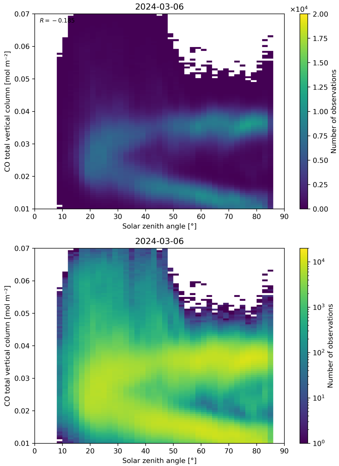
Figure 61: Scatter density plot of “Solar zenith angle” against “CO total vertical column” for 2024-03-05 to 2024-03-07.
