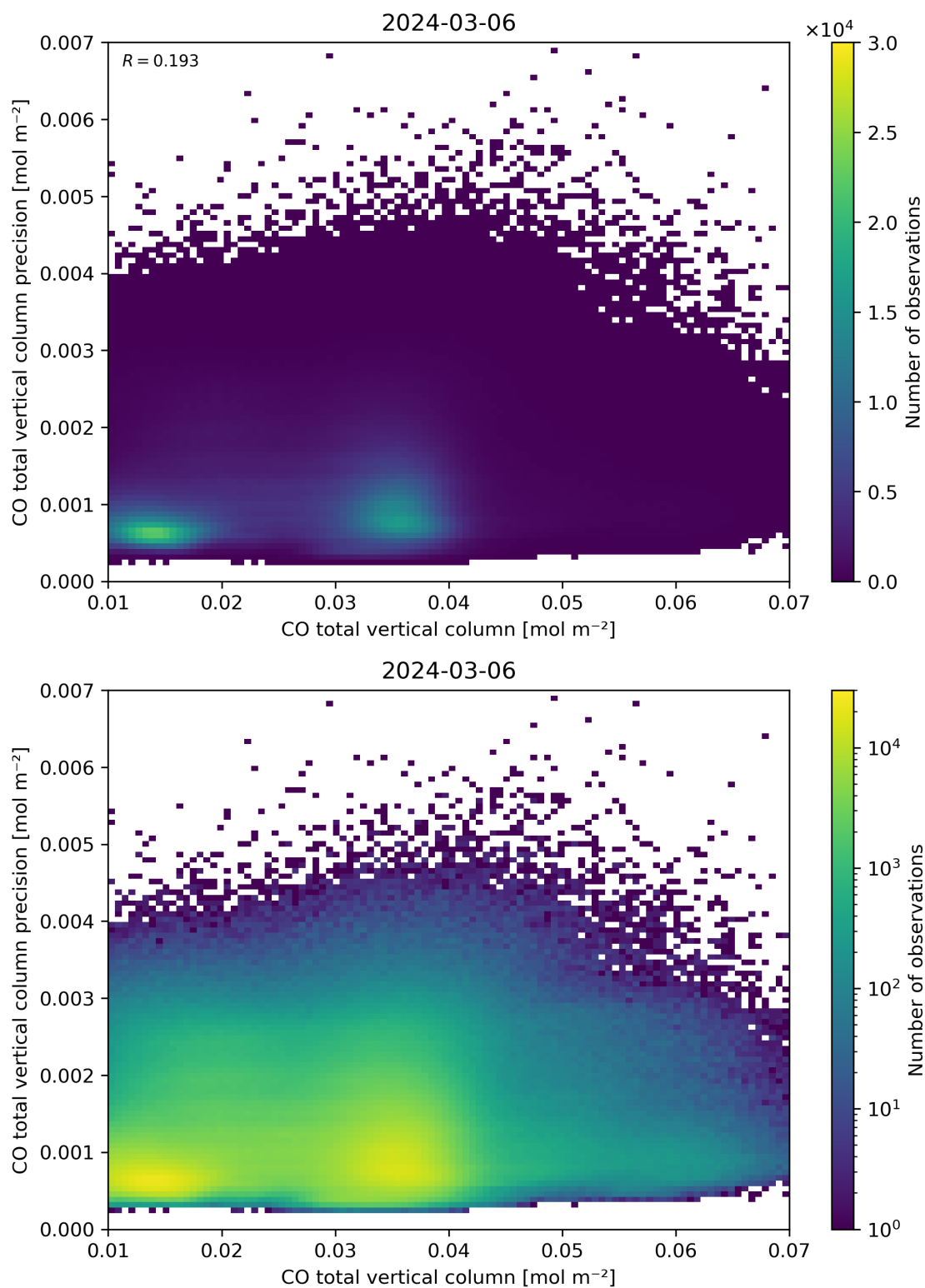
Figure 34: Scatter density plot of “CO total vertical column” against “CO total vertical column precision” for 2024-03-05 to 2024-03-07.
