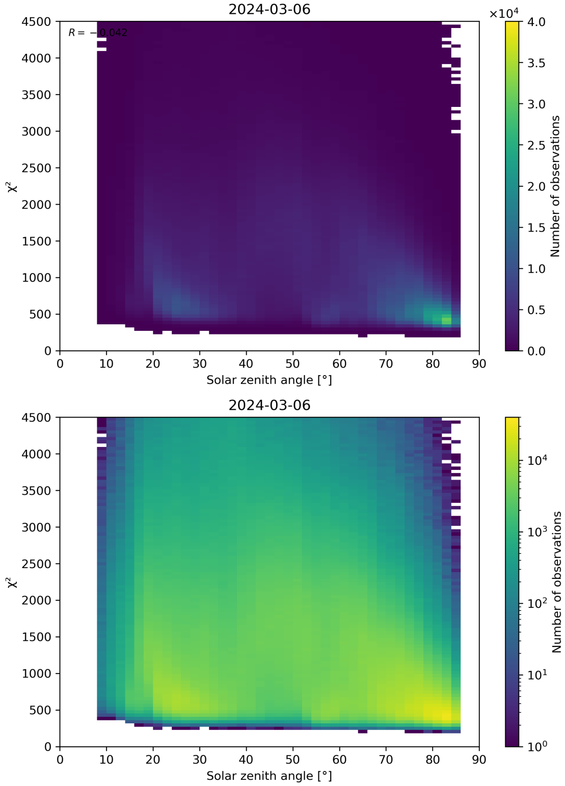
Figure 64: Scatter density plot of “Solar zenith angle” against “ \chi^2 ” for 2024-03-05 to 2024-03-07.
