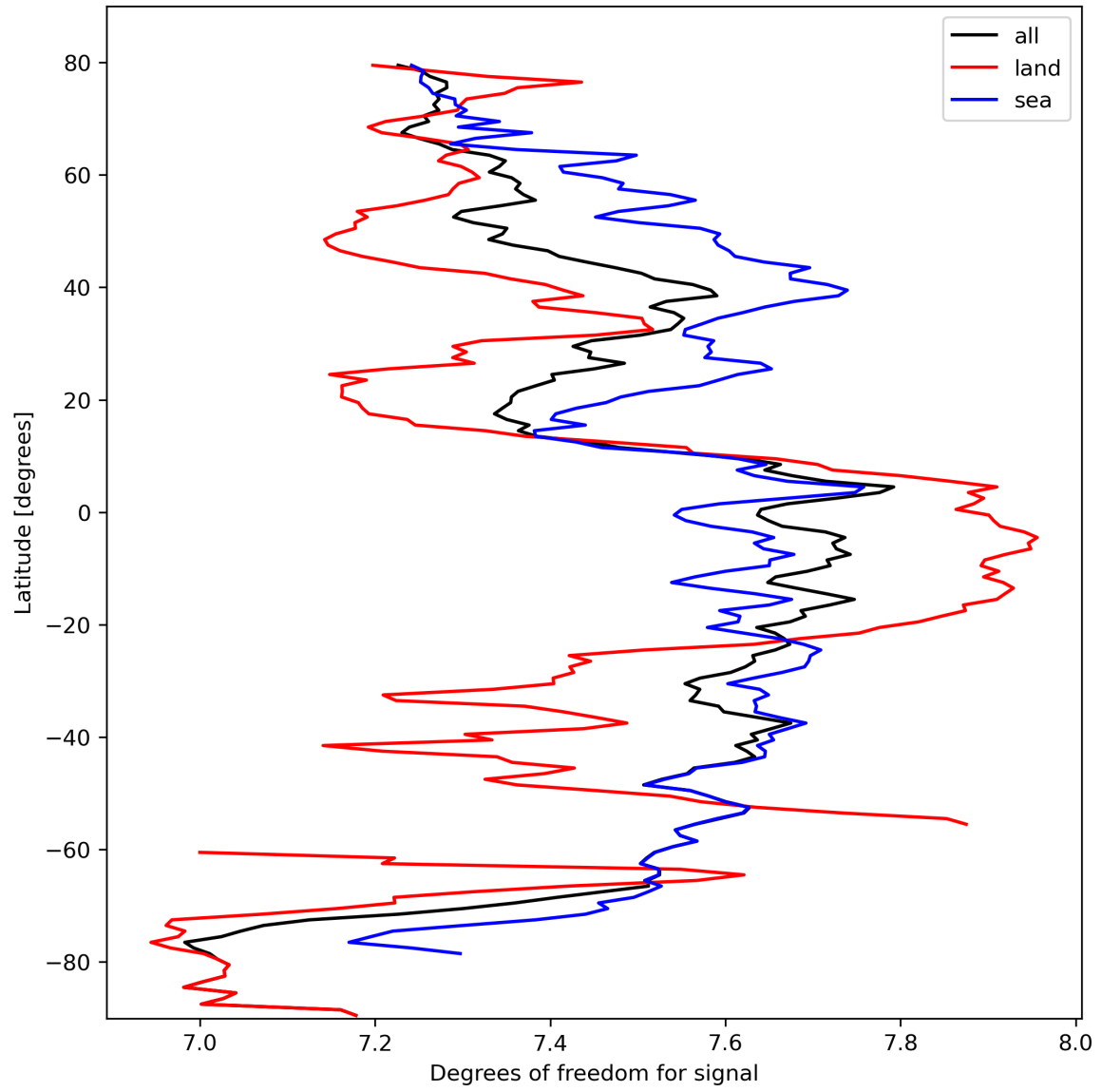
Figure 15: Zonal average of “Degrees of freedom for signal” for 2024-03-05 to 2024-03-07.
