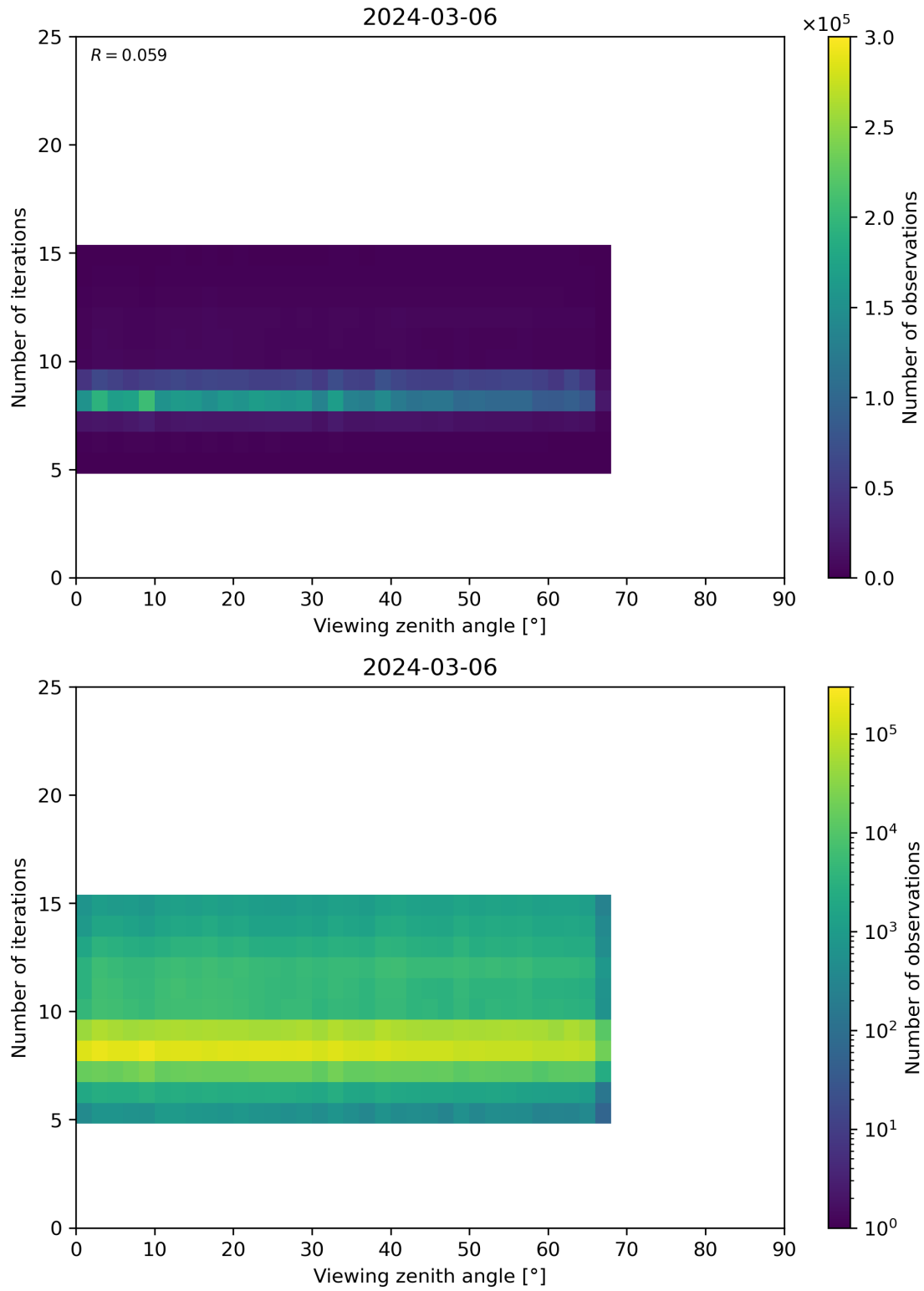
Figure 75: Scatter density plot of “Viewing zenith angle” against “Number of iterations” for 2024-03-05 to 2024-03-07.
