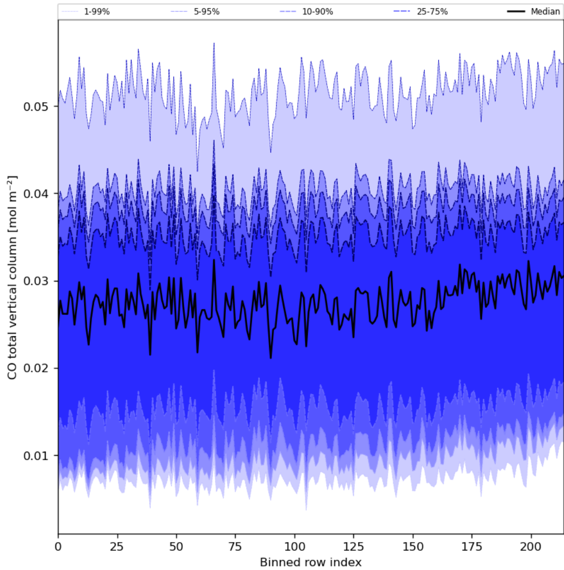
Figure 26: Along track statistics of “CO total vertical column” for 2024-03-05 to 2024-03-07
