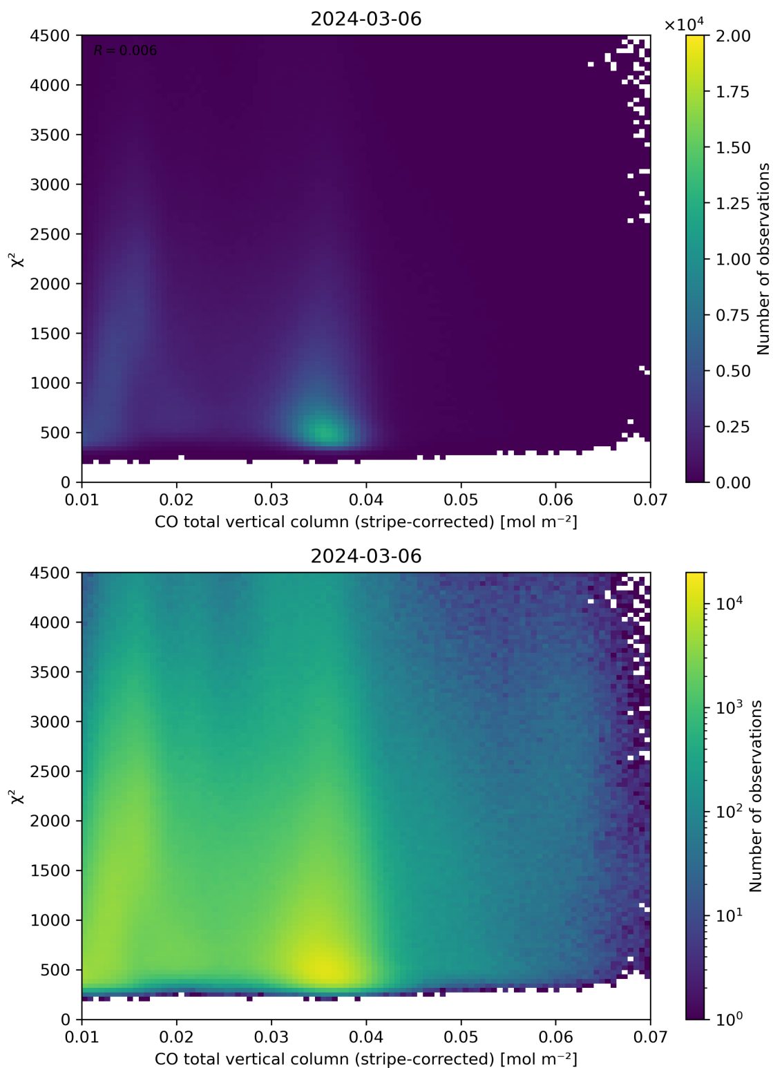
Figure 37: Scatter density plot of “CO total vertical column (stripe-corrected)” against “ \chi^2 ” for 2024-03-05 to 2024-03-07.
