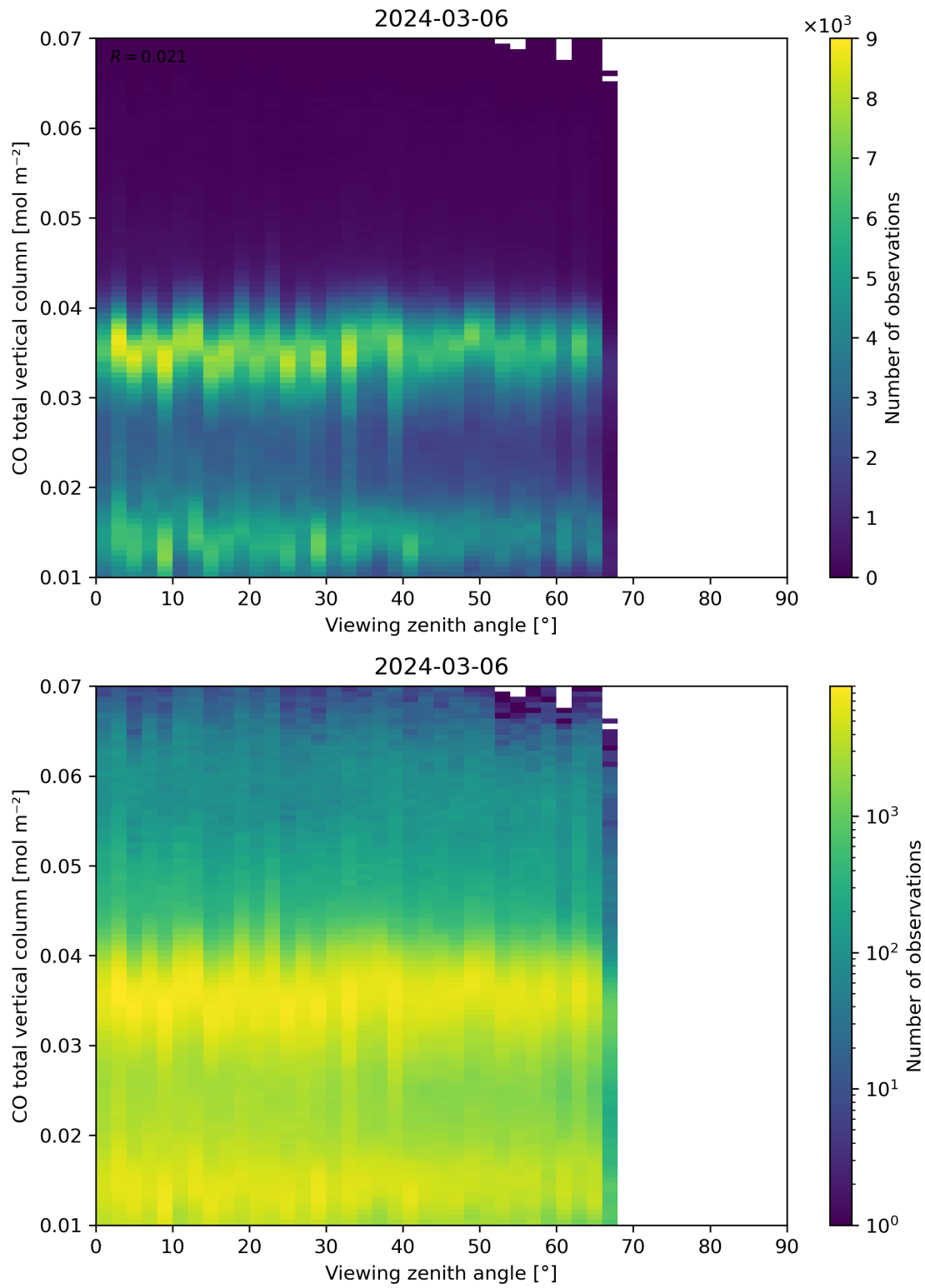
Figure 69: Scatter density plot of “Viewing zenith angle” against “CO total vertical column” for 2024-03-05 to 2024-03-07.
