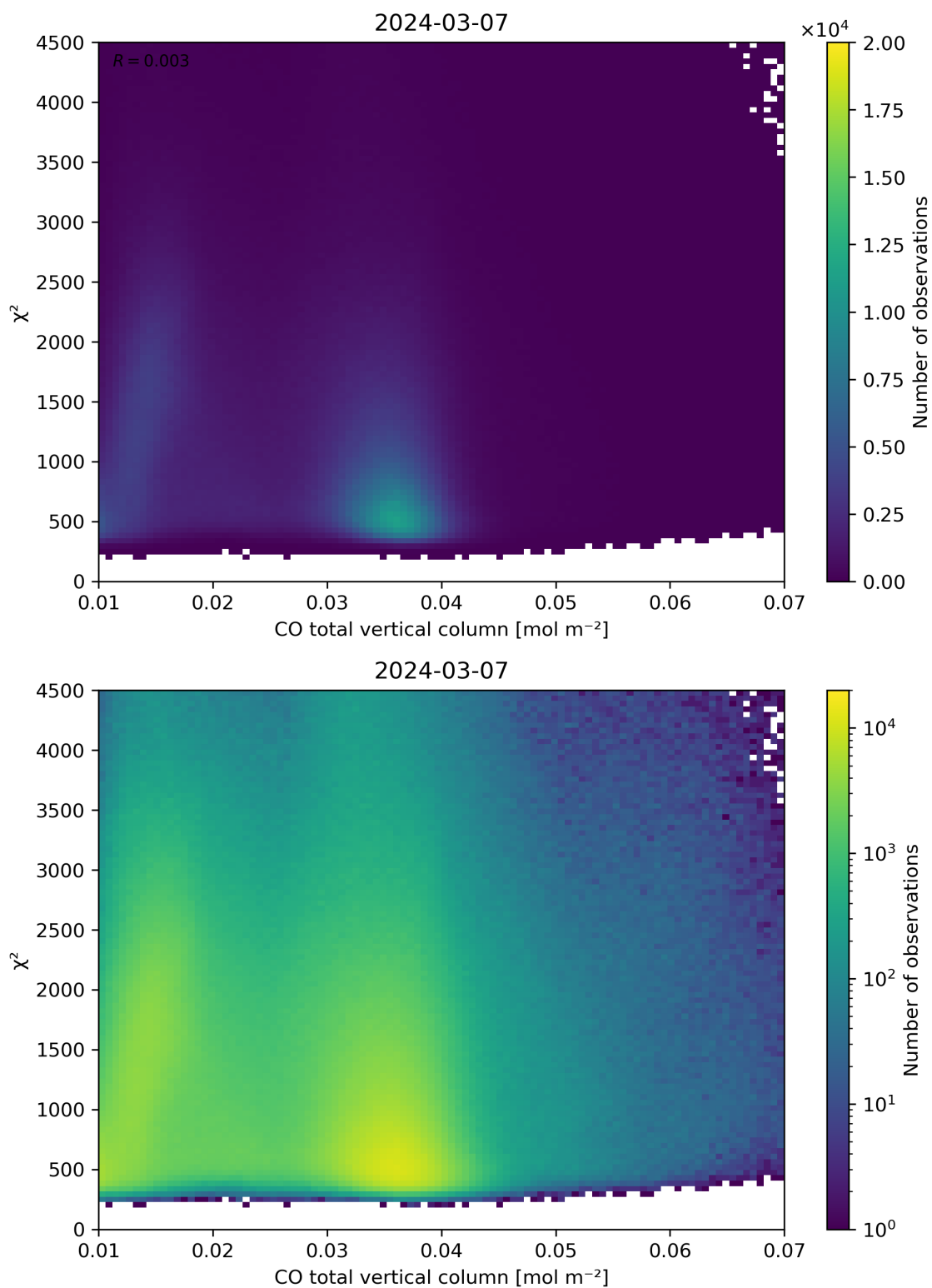
Figure 35: Scatter density plot of “CO total vertical column” against “ \chi^2 ” for 2024-03-06 to 2024-03-08.
