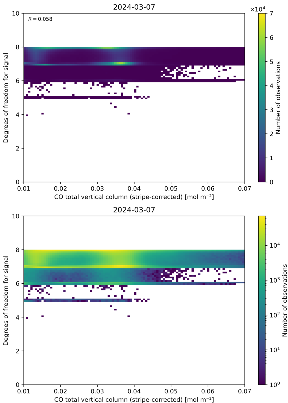
Figure 38: Scatter density plot of “CO total vertical column (stripe-corrected)” against “Degrees of freedom for signal” for 2024-03-06 to 2024-03-08.
