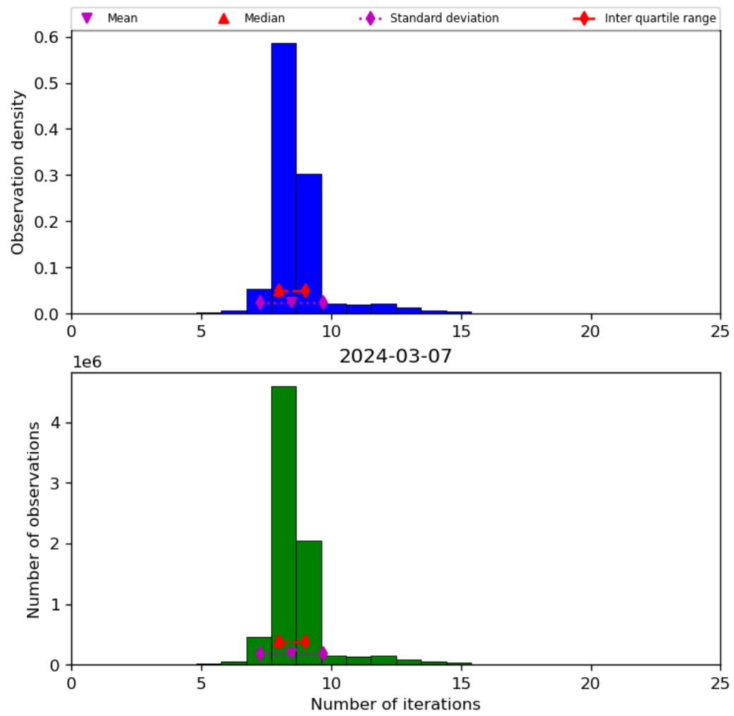
Figure 24: Histogram of “Number of iterations” for 2024-03-06 to 2024-03-08
