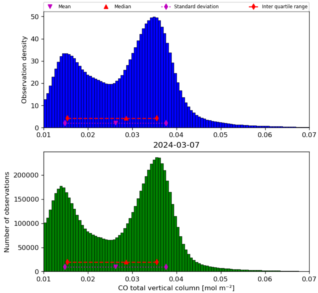
Figure 18: Histogram of “CO total vertical column” for 2024-03-06 to 2024-03-08
