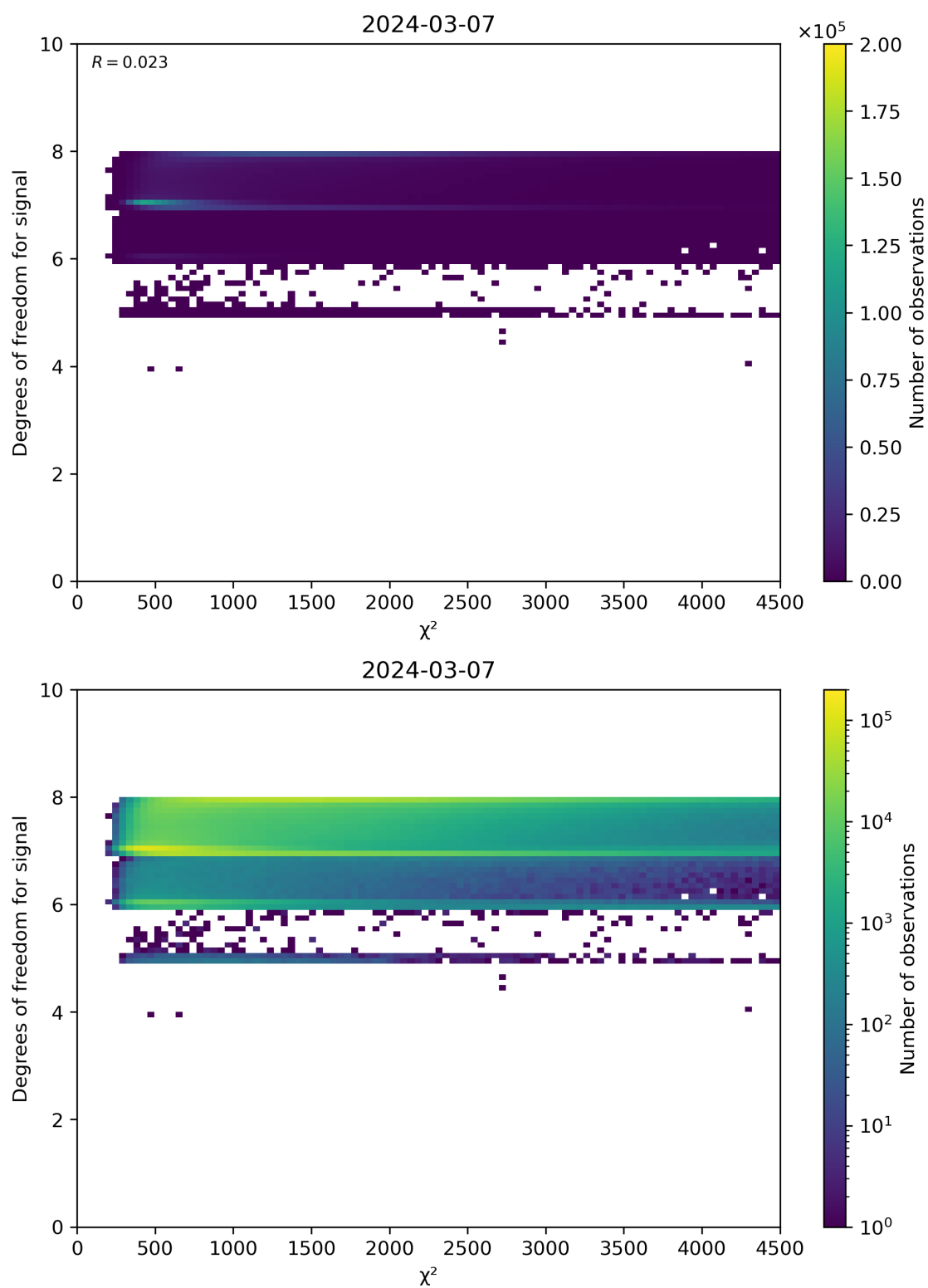
Figure 48: Scatter density plot of “ \chi^2 ” against “Degrees of freedom for signal” for 2024-03-06 to 2024-03-08.
