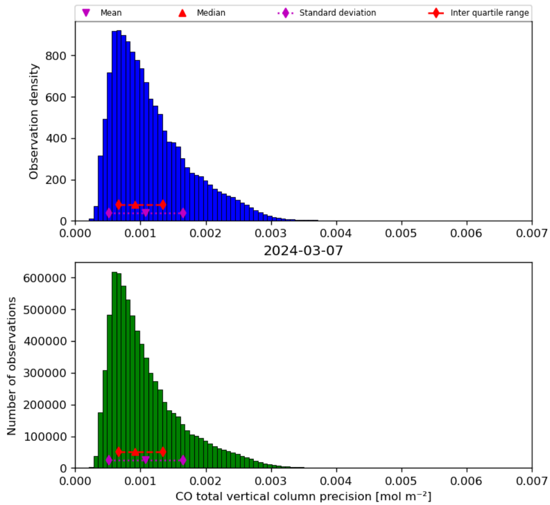
Figure 20: Histogram of “CO total vertical column precision” for 2024-03-06 to 2024-03-08
