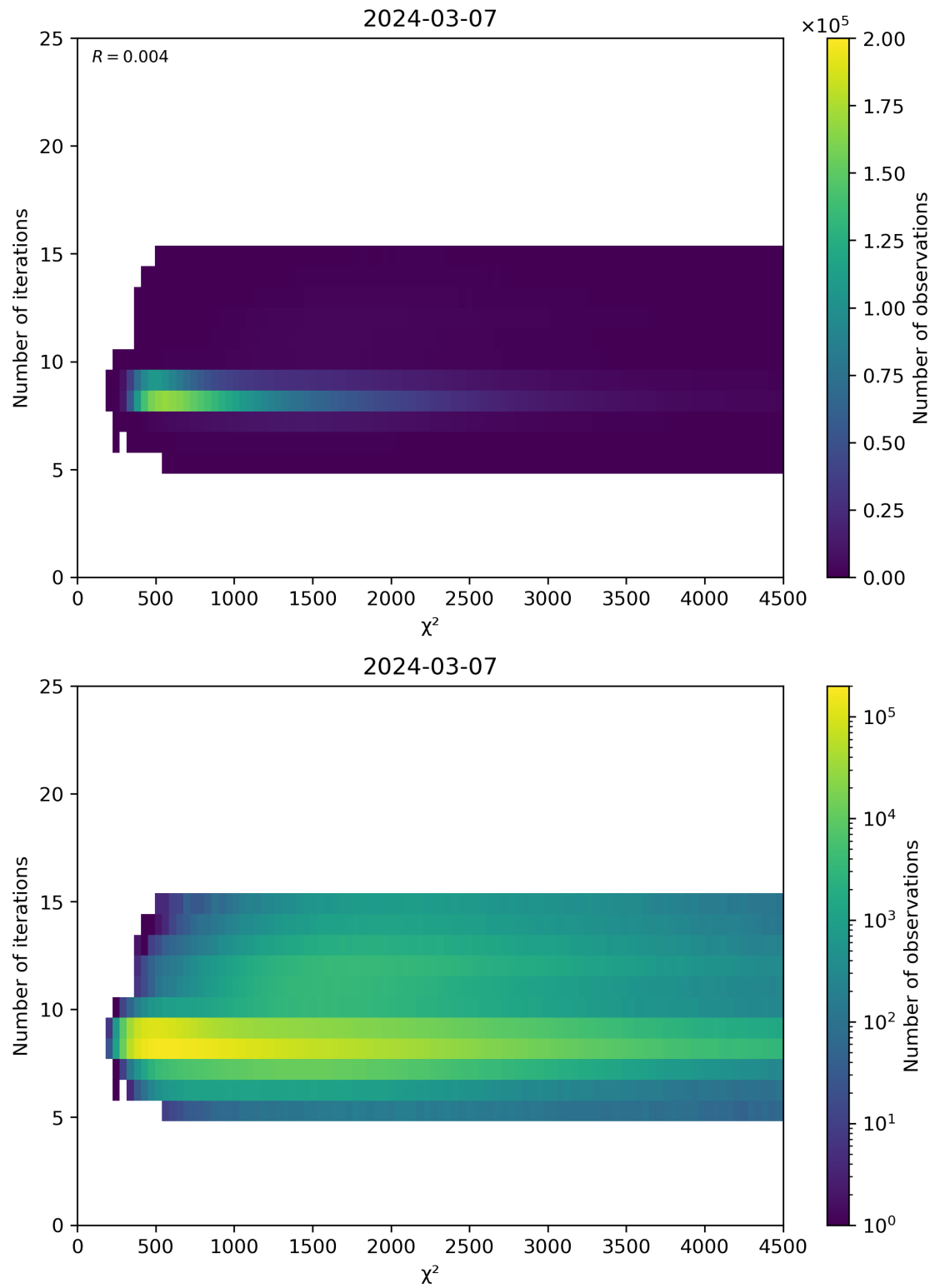
Figure 49: Scatter density plot of “ \chi^2 ” against “Number of iterations” for 2024-03-06 to 2024-03-08.
