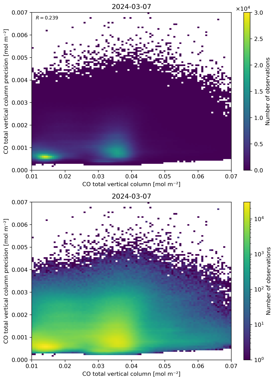
Figure 34: Scatter density plot of “CO total vertical column” against “CO total vertical column precision” for 2024-03-06 to 2024-03-08.
