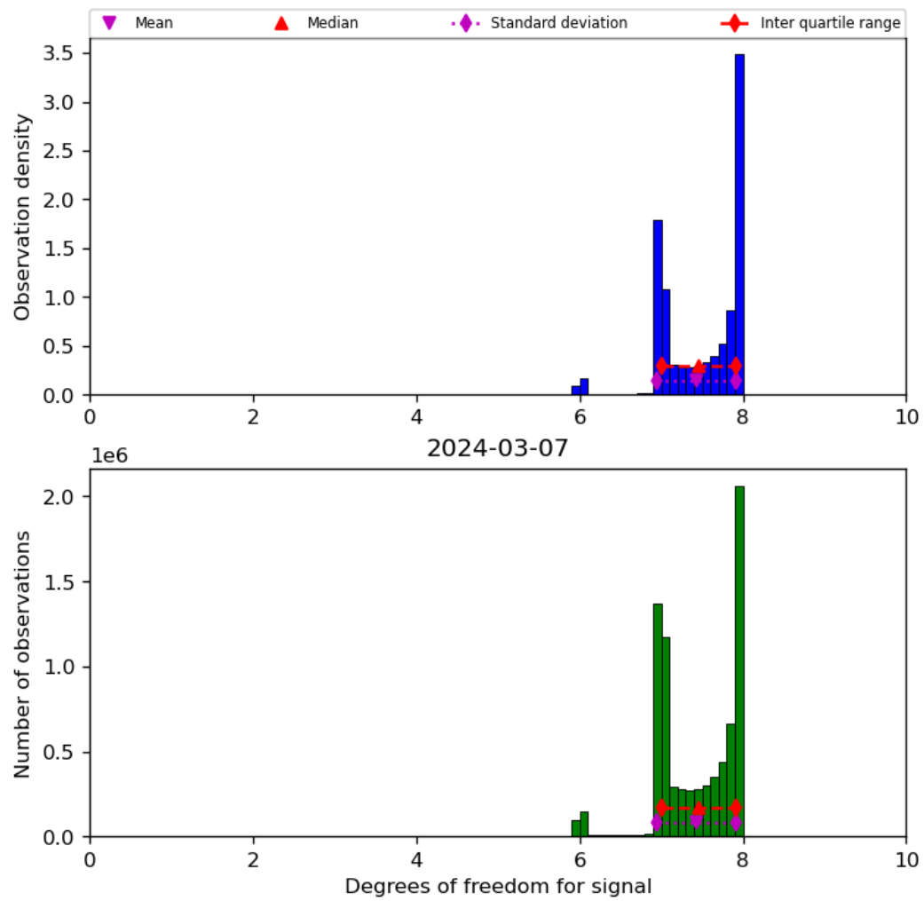
Figure 23: Histogram of “Degrees of freedom for signal” for 2024-03-06 to 2024-03-08
