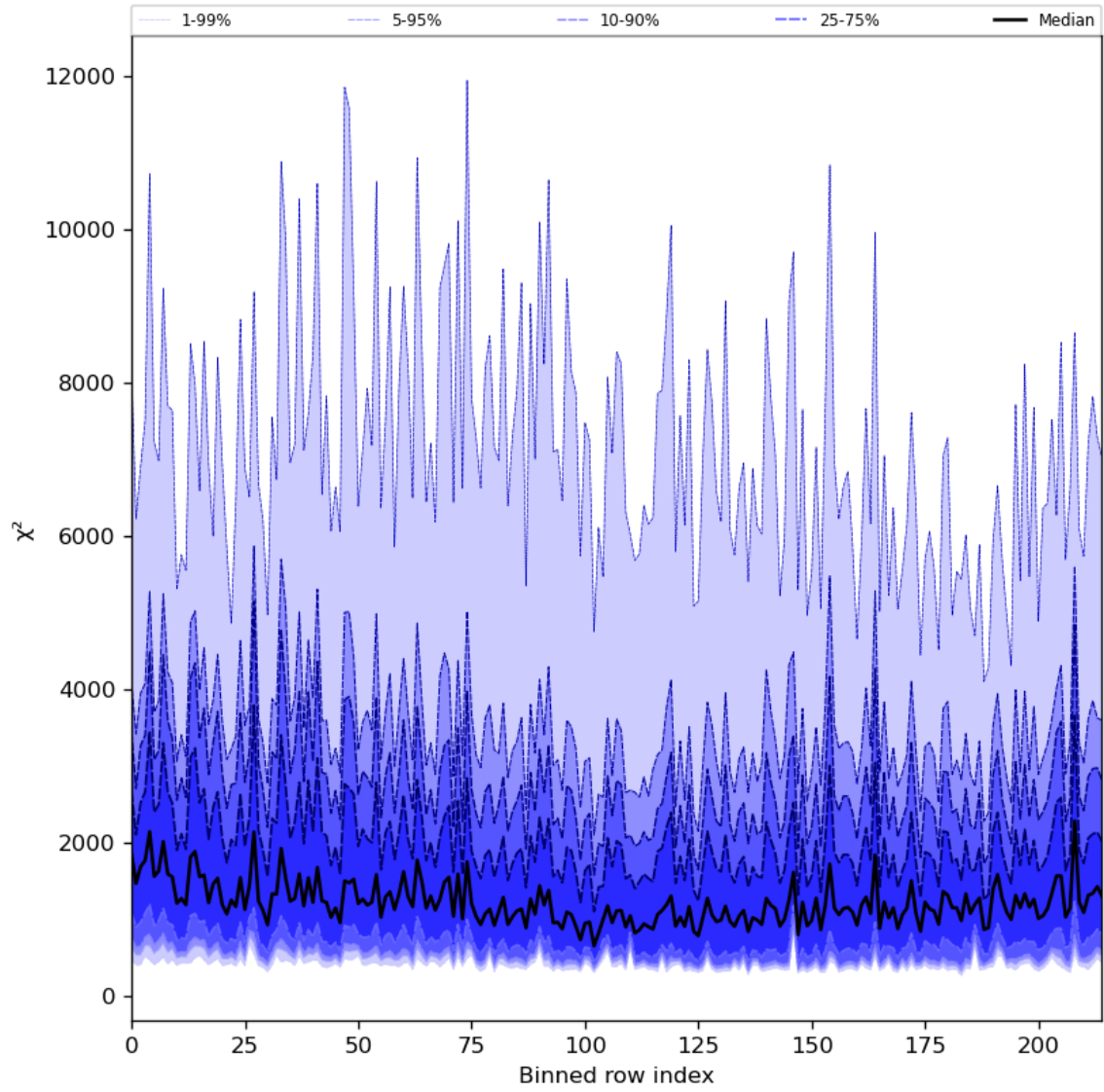
Figure 30: Along track statistics of “ \chi^2 ” for 2024-03-06 to 2024-03-08
