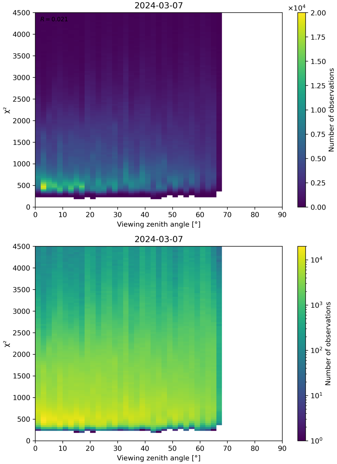
Figure 72: Scatter density plot of “Viewing zenith angle” against “ \chi^2 ” for 2024-03-06 to 2024-03-08.
