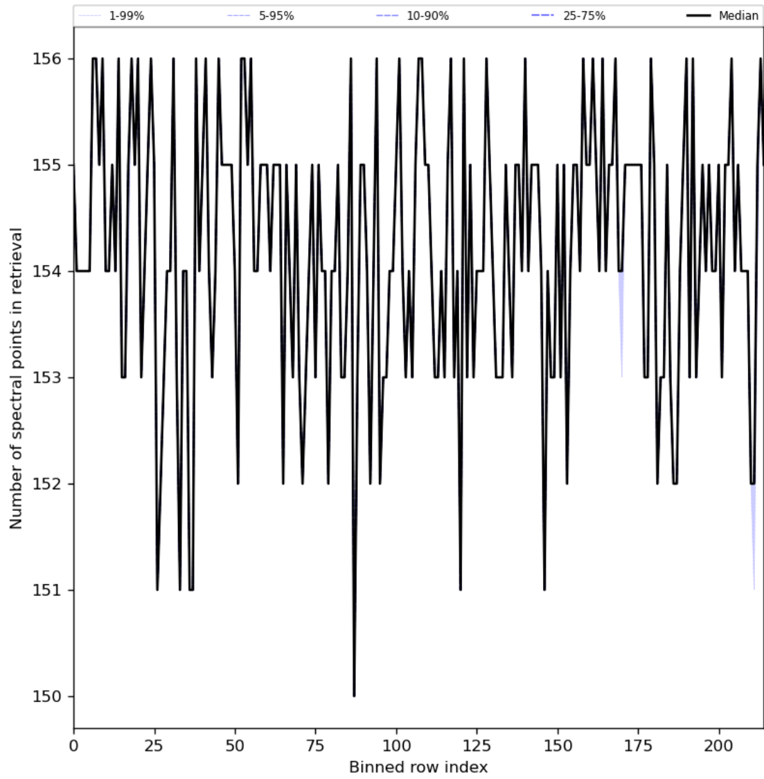
Figure 29: Along track statistics of “Number of spectral points in retrieval” for 2024-03-06 to 2024-03-08
