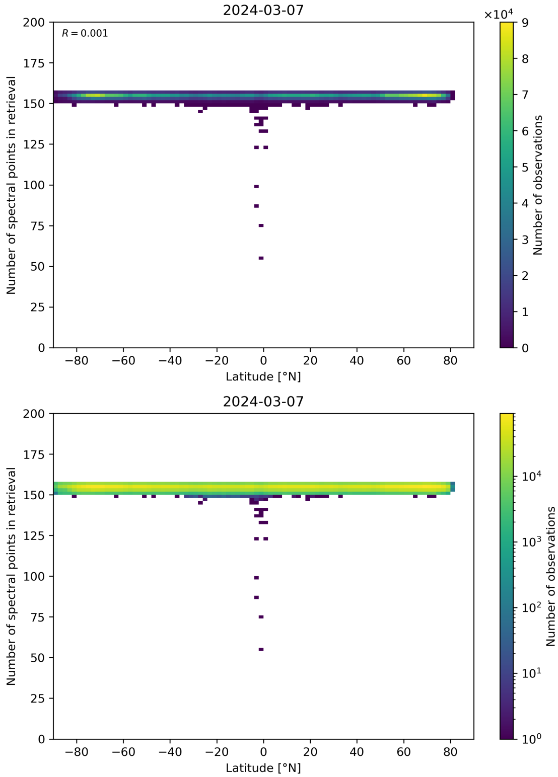
Figure 57: Scatter density plot of “Latitude” against “Number of spectral points in retrieval” for 2024-03-06 to 2024-03-08.
