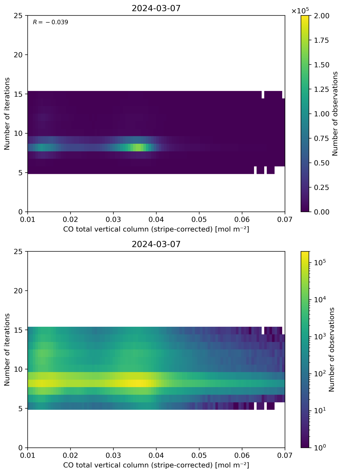
Figure 39: Scatter density plot of “CO total vertical column (stripe-corrected)” against “Number of iterations” for 2024-03-06 to 2024-03-08.
