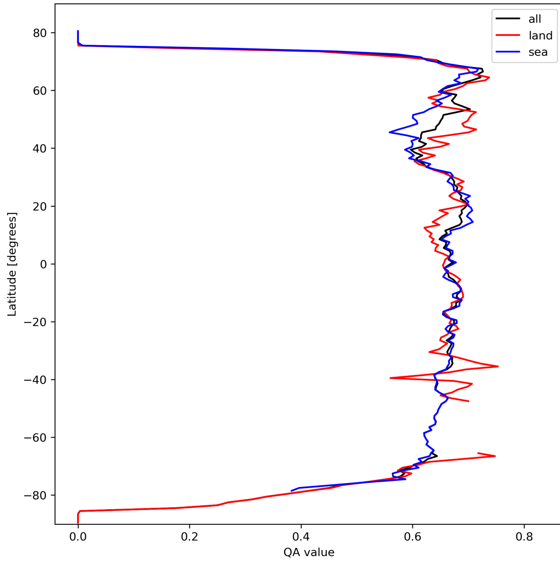
Figure 9: Zonal average of “QA value” for 2024-03-06 to 2024-03-08.
