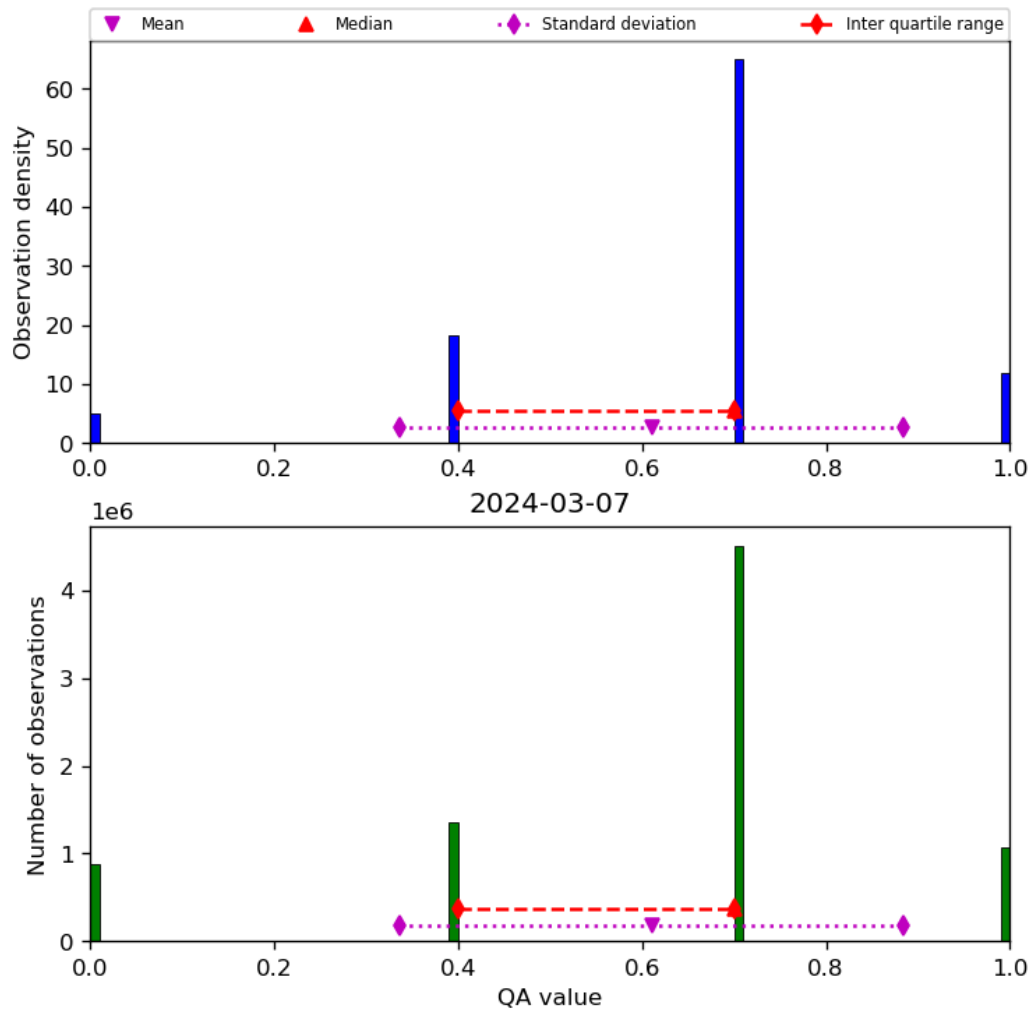
Figure 17: Histogram of “QA value” for 2024-03-06 to 2024-03-08
