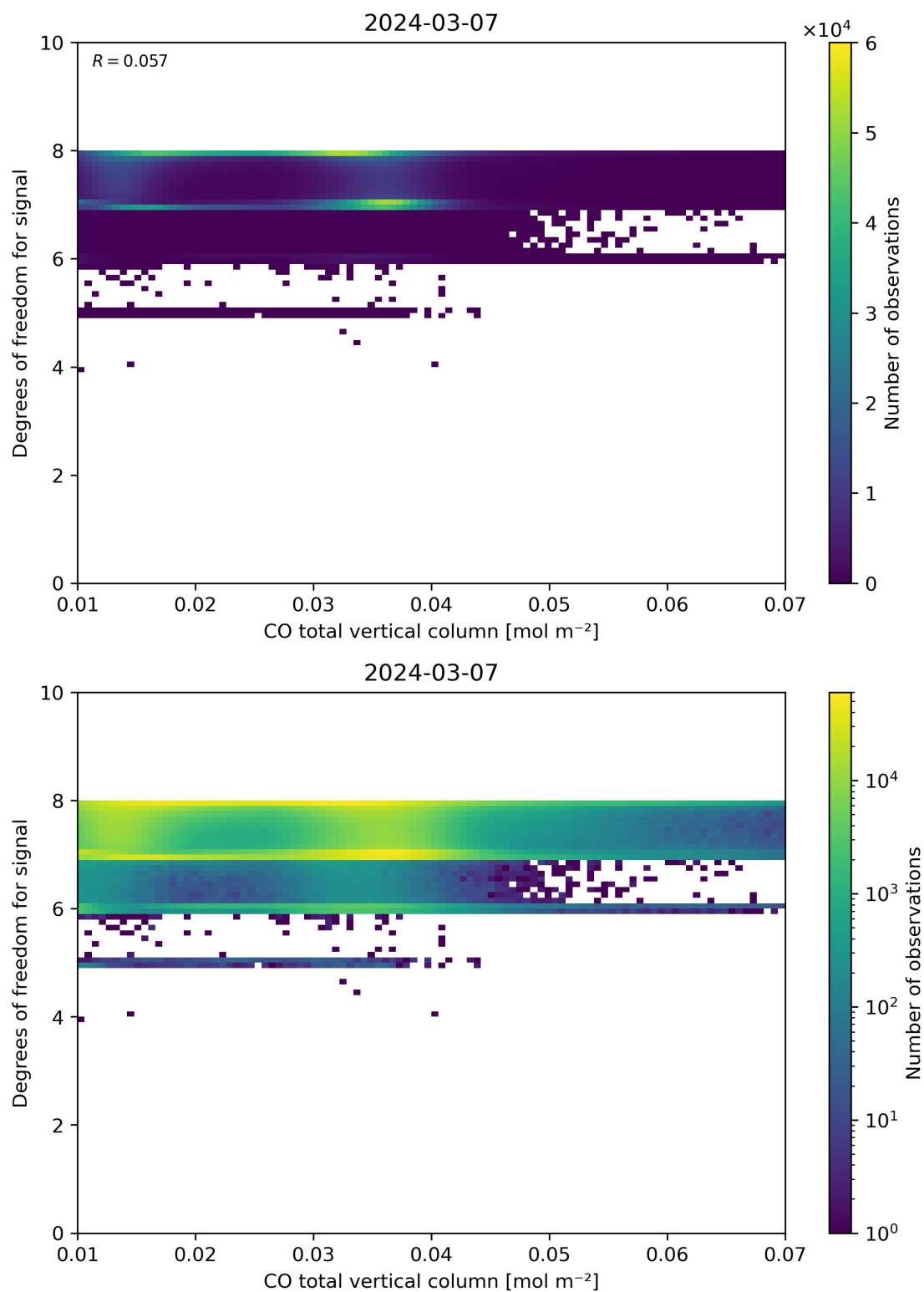
Figure 41: Scatter density plot of “CO total vertical column” against “Degrees of freedom for signal” for 2024-03-06 to 2024-03-08.
