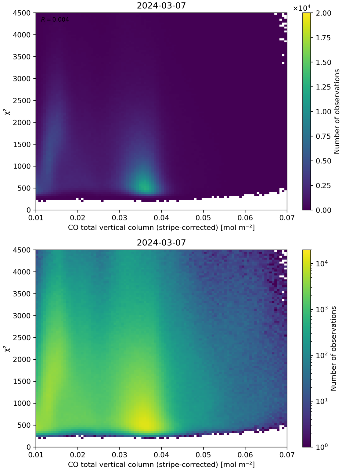
Figure 37: Scatter density plot of “CO total vertical column (stripe-corrected)” against “ \chi^2 ” for 2024-03-06 to 2024-03-08.
