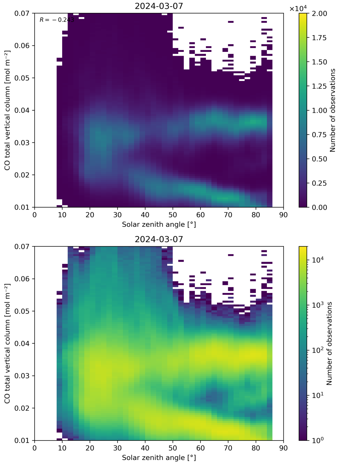
Figure 61: Scatter density plot of “Solar zenith angle” against “CO total vertical column” for 2024-03-06 to 2024-03-08.
