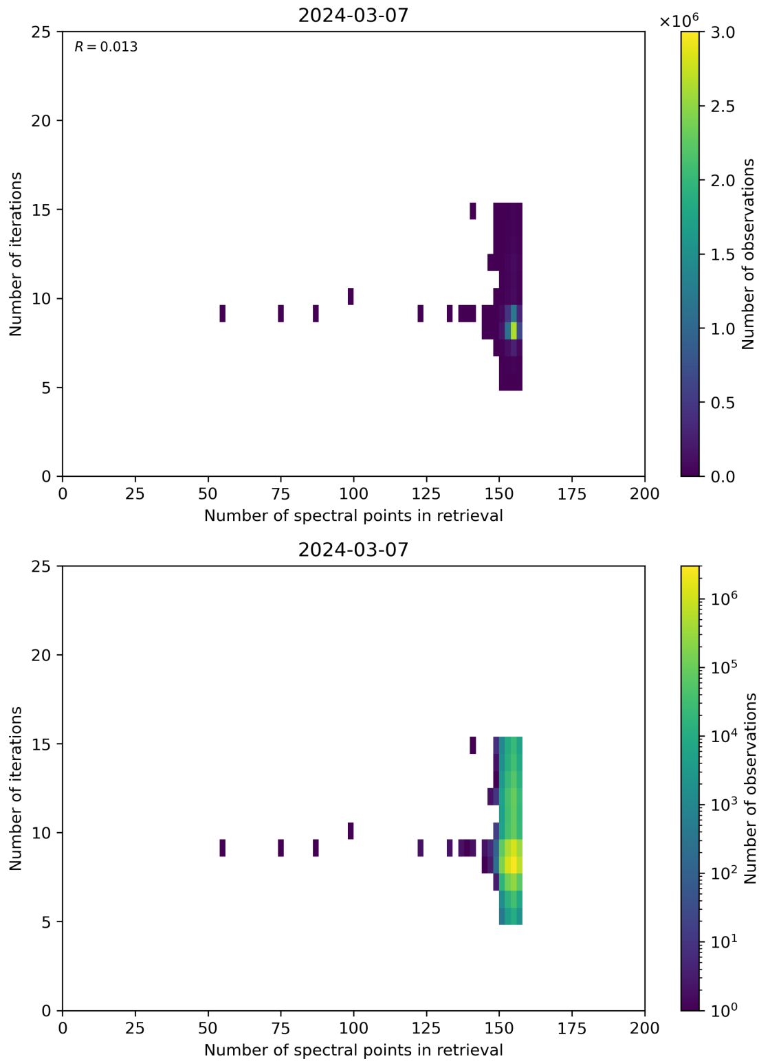
Figure 60: Scatter density plot of “Number of spectral points in retrieval” against “Number of iterations” for 2024-03-06 to 2024-03-08.
