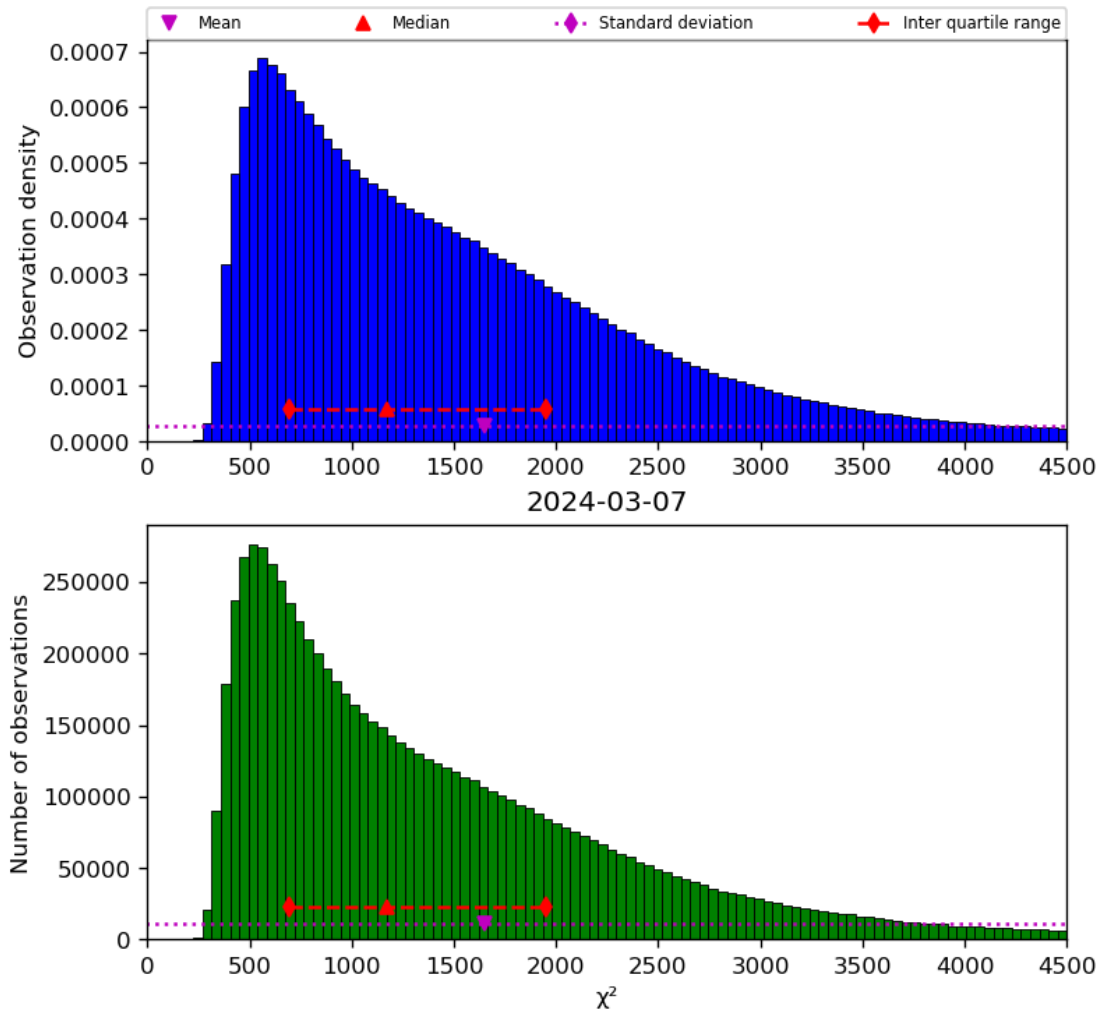
Figure 22: Histogram of “ \chi^2 ” for 2024-03-06 to 2024-03-08
