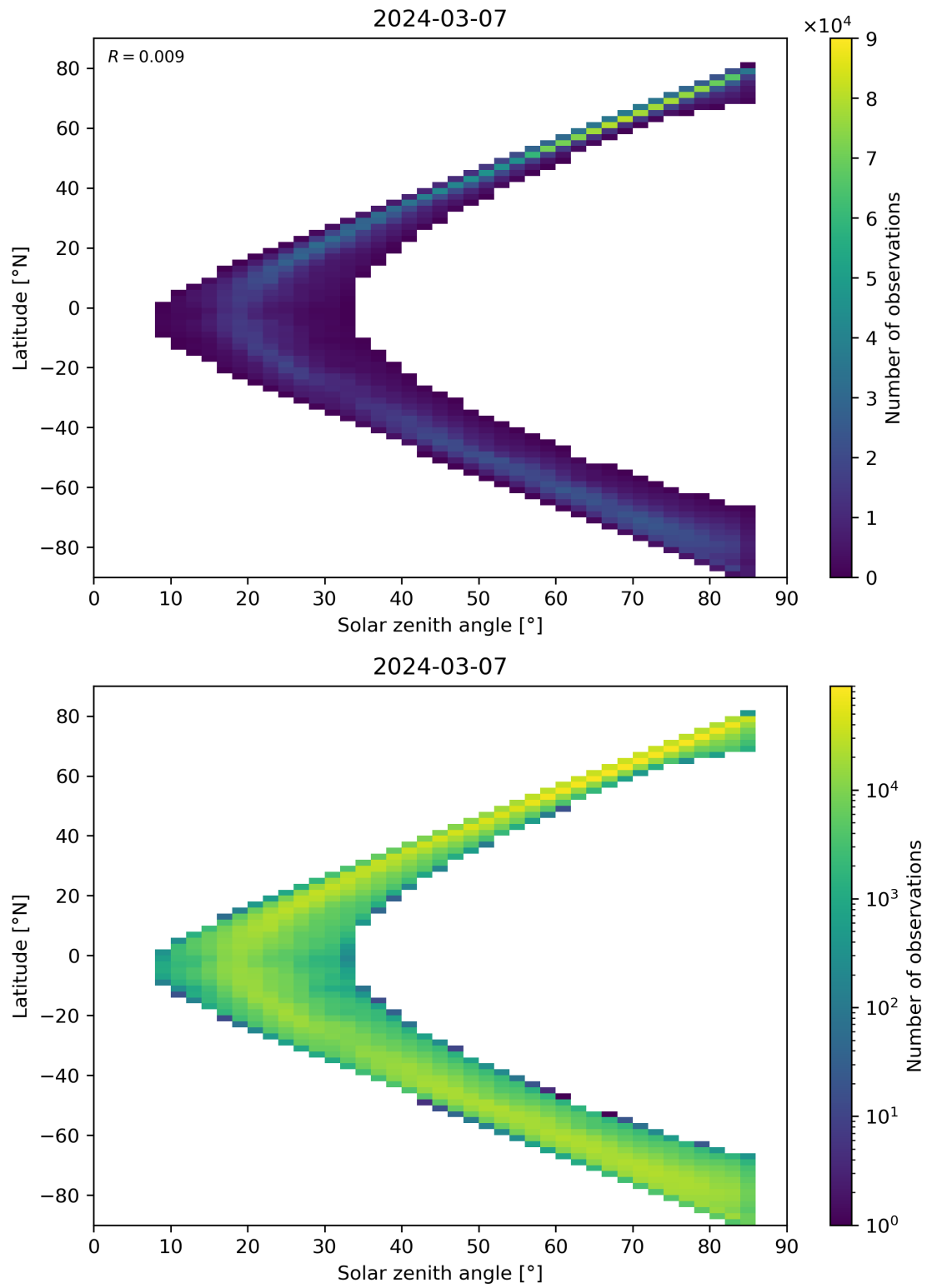
Figure 66: Scatter density plot of “Solar zenith angle” against “Latitude” for 2024-03-06 to 2024-03-08.
