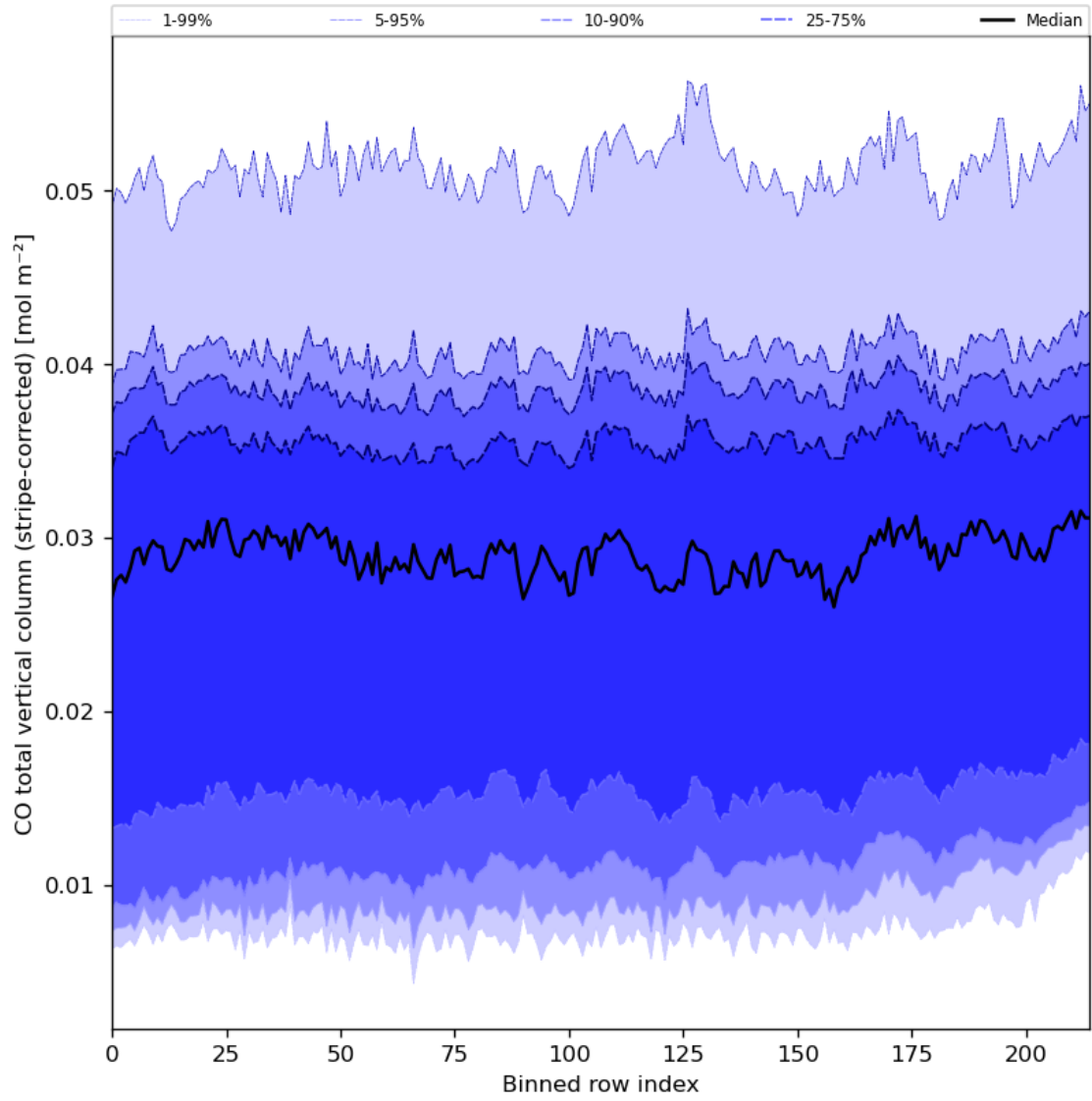
Figure 27: Along track statistics of “CO total vertical column (stripe-corrected)” for 2024-03-06 to 2024-03-08
