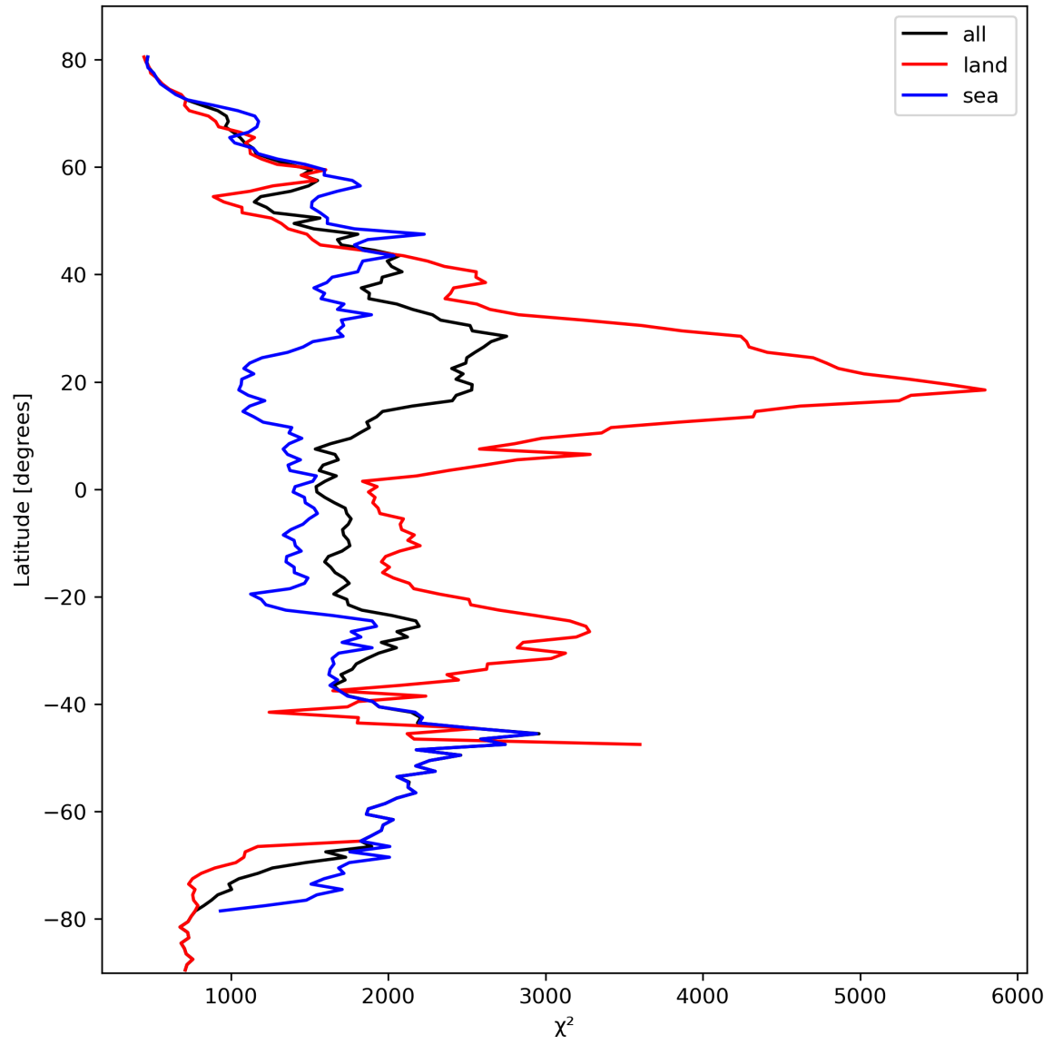
Figure 14: Zonal average of “ \chi^2 ” for 2024-03-06 to 2024-03-08.
