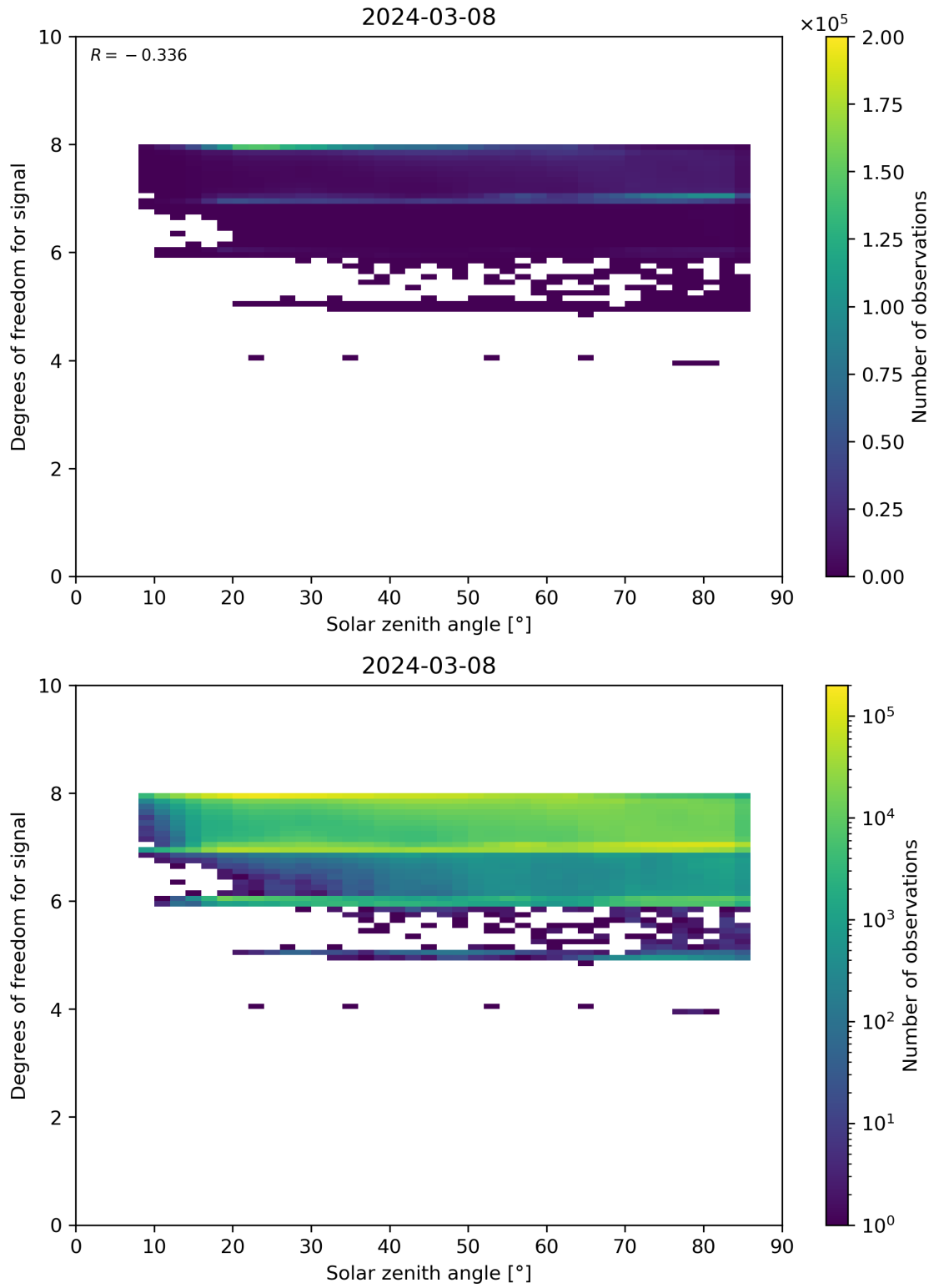
Figure 65: Scatter density plot of “Solar zenith angle” against “Degrees of freedom for signal” for 2024-03-07 to 2024-03-09.
