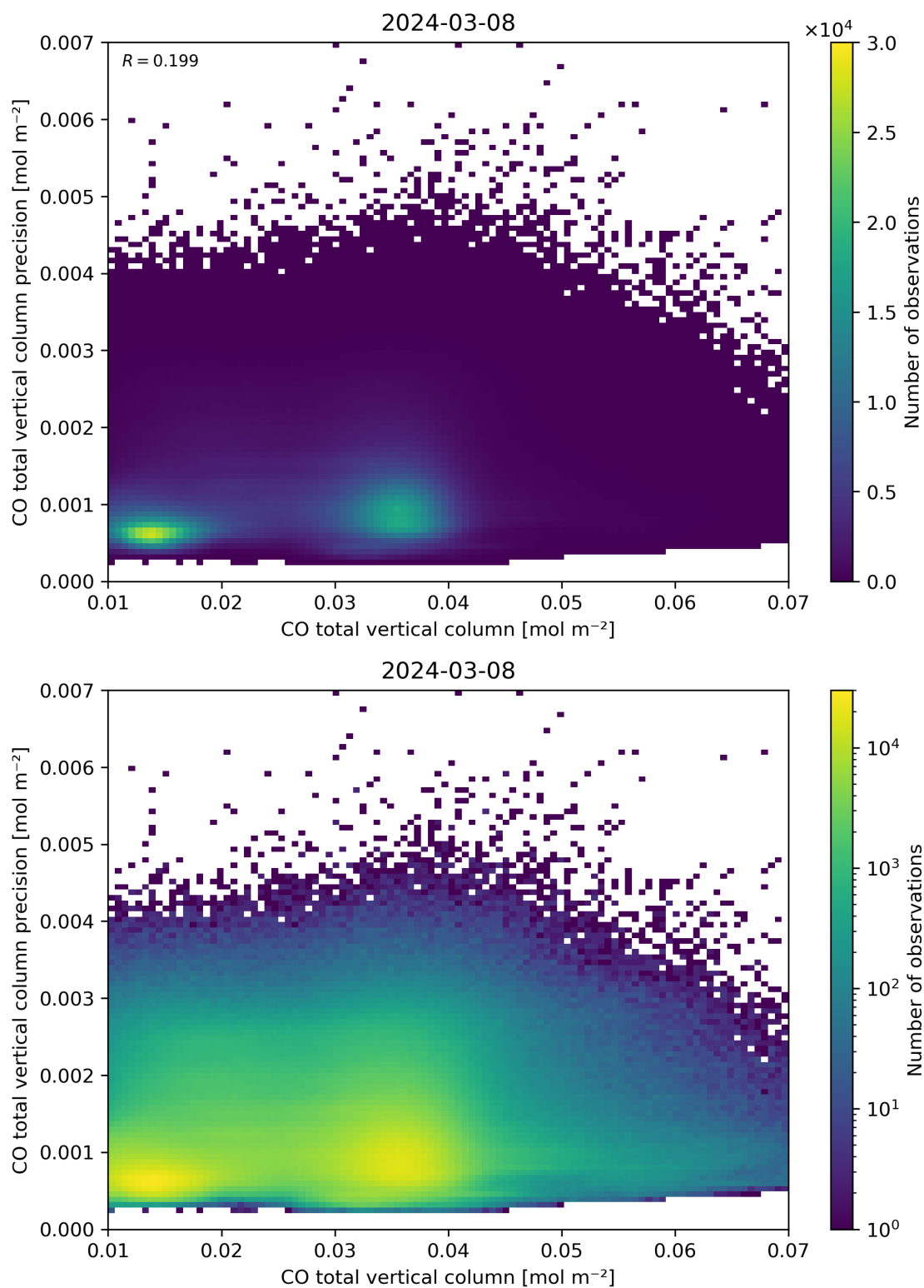
Figure 34: Scatter density plot of “CO total vertical column” against “CO total vertical column precision” for 2024-03-07 to 2024-03-09.
