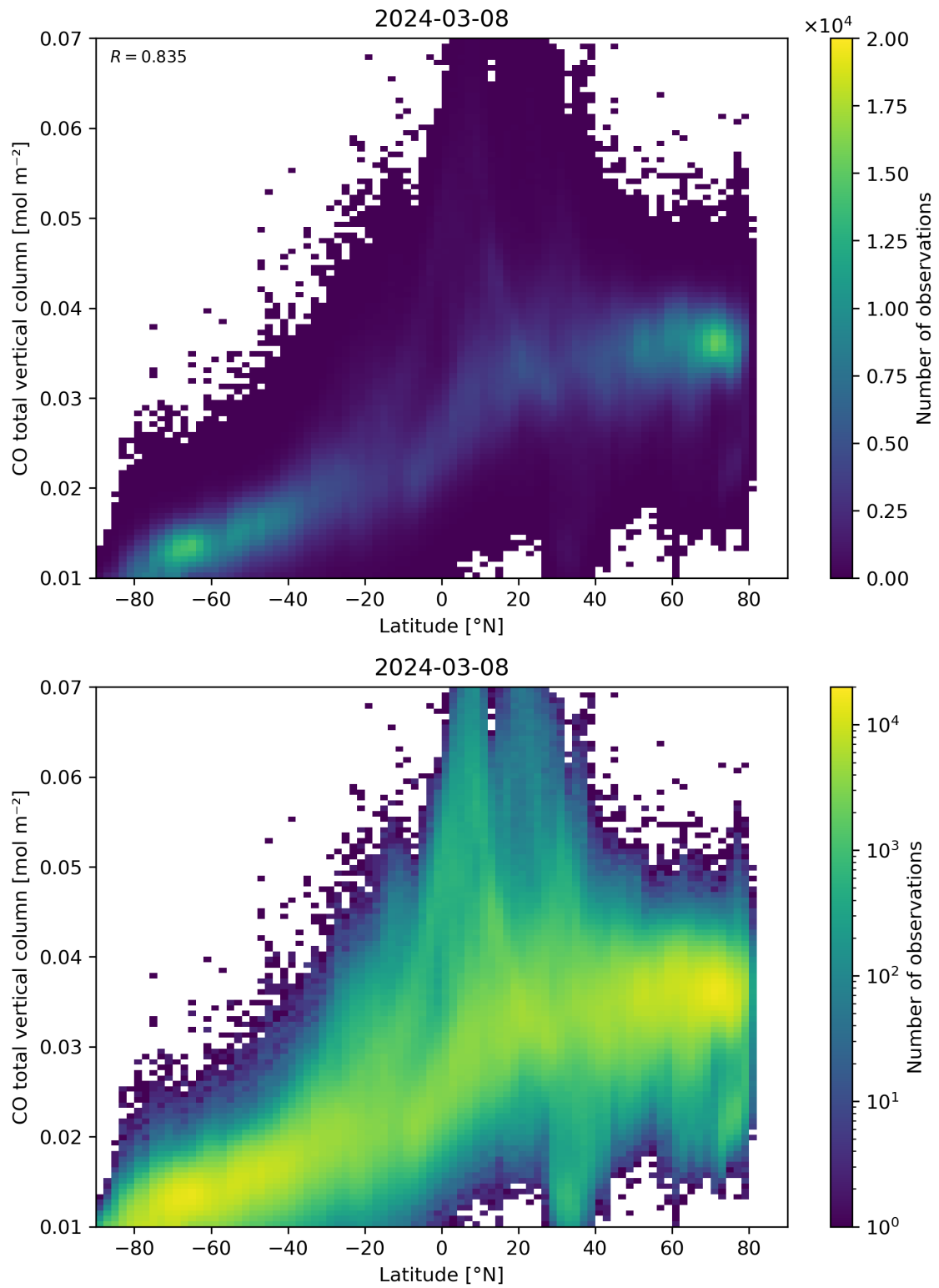
Figure 51: Scatter density plot of “Latitude” against “CO total vertical column” for 2024-03-07 to 2024-03-09.
