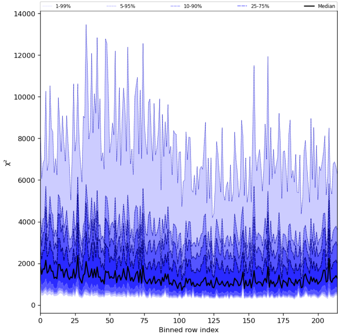
Figure 30: Along track statistics of “ \chi^2 ” for 2024-03-07 to 2024-03-09
