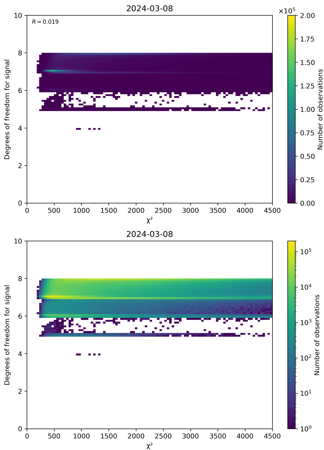
Figure 48: Scatter density plot of “ \chi^2 ” against “Degrees of freedom for signal” for 2024-03-07 to 2024-03-09.
