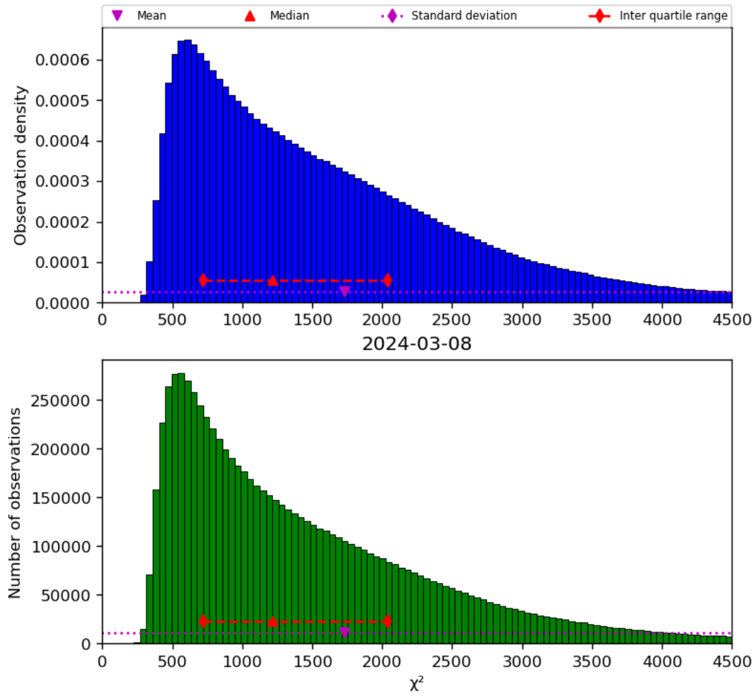
Figure 22: Histogram of “ \chi^2 ” for 2024-03-07 to 2024-03-09
