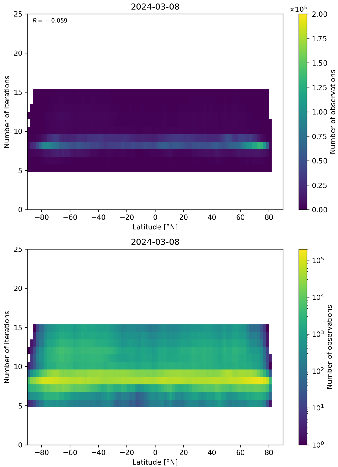
Figure 56: Scatter density plot of “Latitude” against “Number of iterations” for 2024-03-07 to 2024-03-09.
