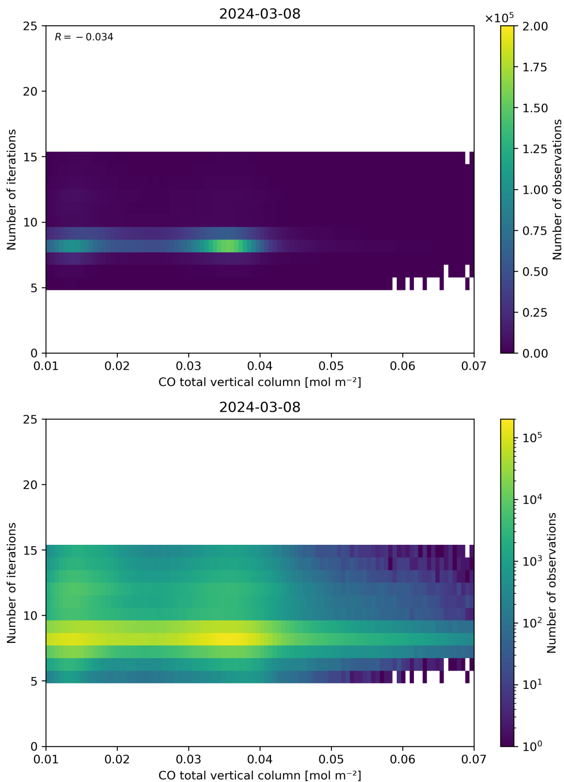
Figure 42: Scatter density plot of “CO total vertical column” against “Number of iterations” for 2024-03-07 to 2024-03-09.
