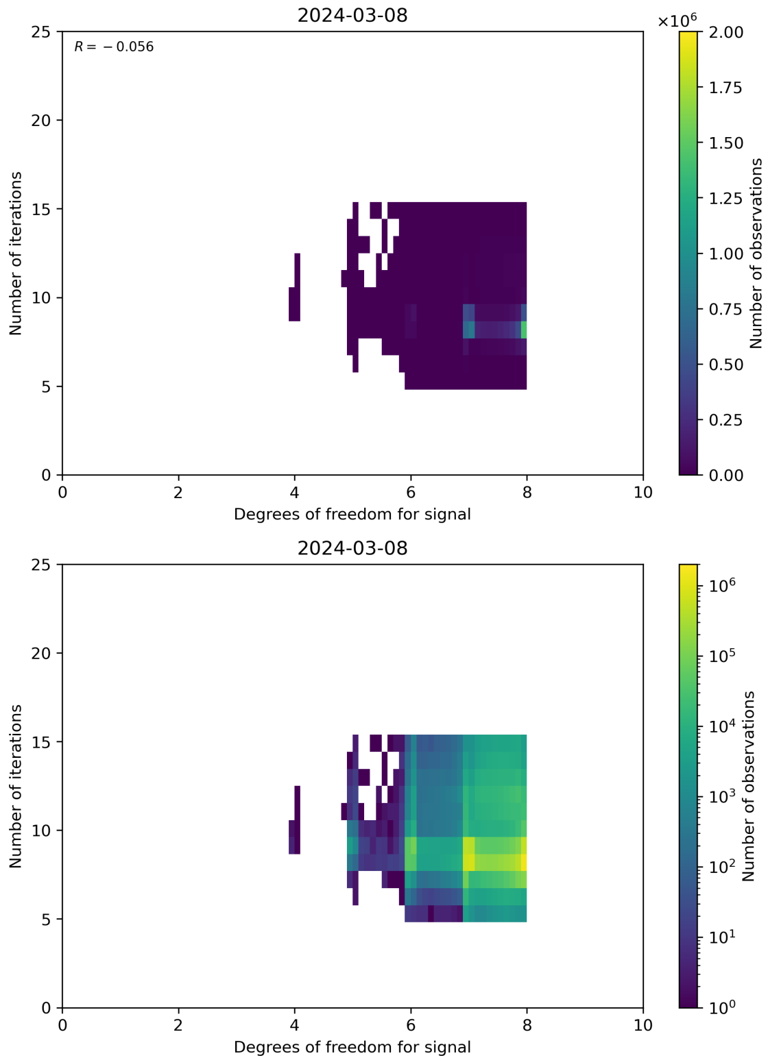
Figure 50: Scatter density plot of “Degrees of freedom for signal” against “Number of iterations” for 2024-03-07 to 2024-03-09.
