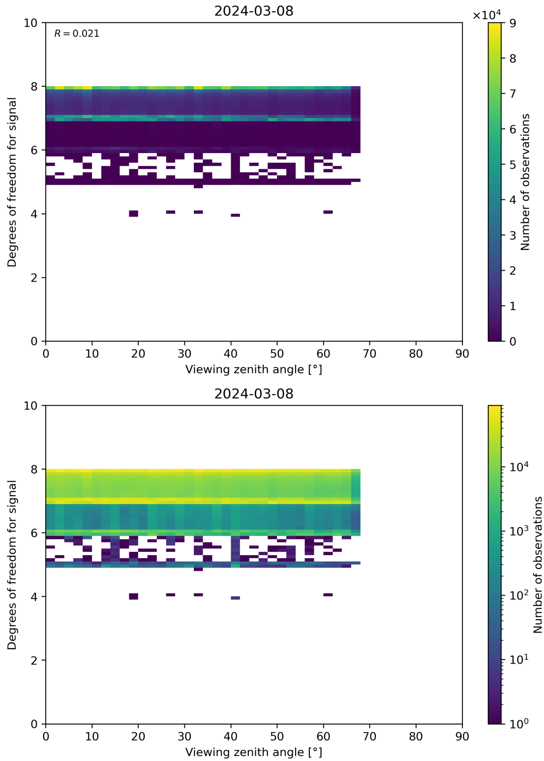
Figure 73: Scatter density plot of “Viewing zenith angle” against “Degrees of freedom for signal” for 2024-03-07 to 2024-03-09.
