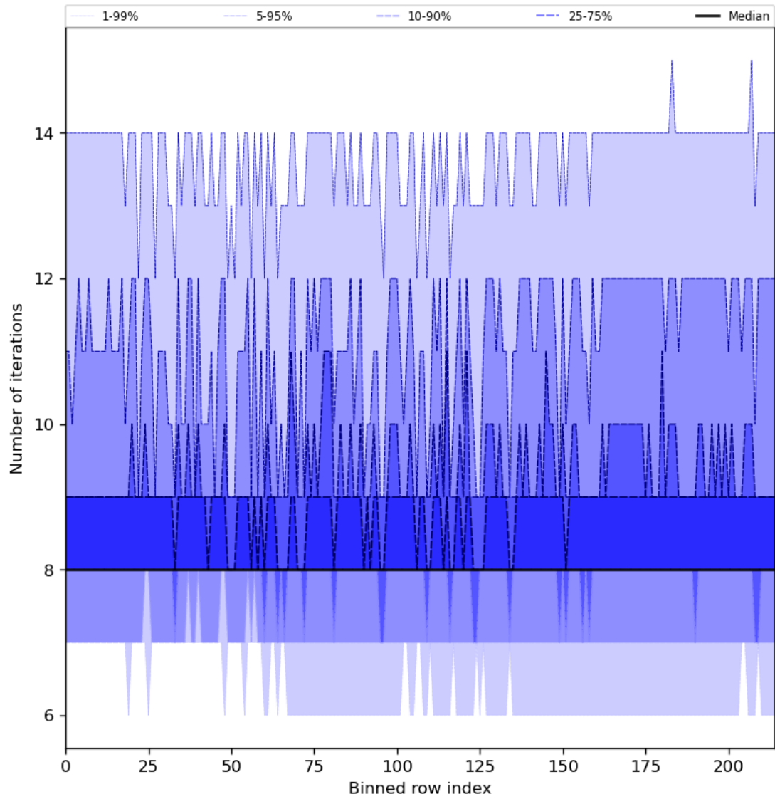
Figure 32: Along track statistics of “Number of iterations” for 2024-03-07 to 2024-03-09
