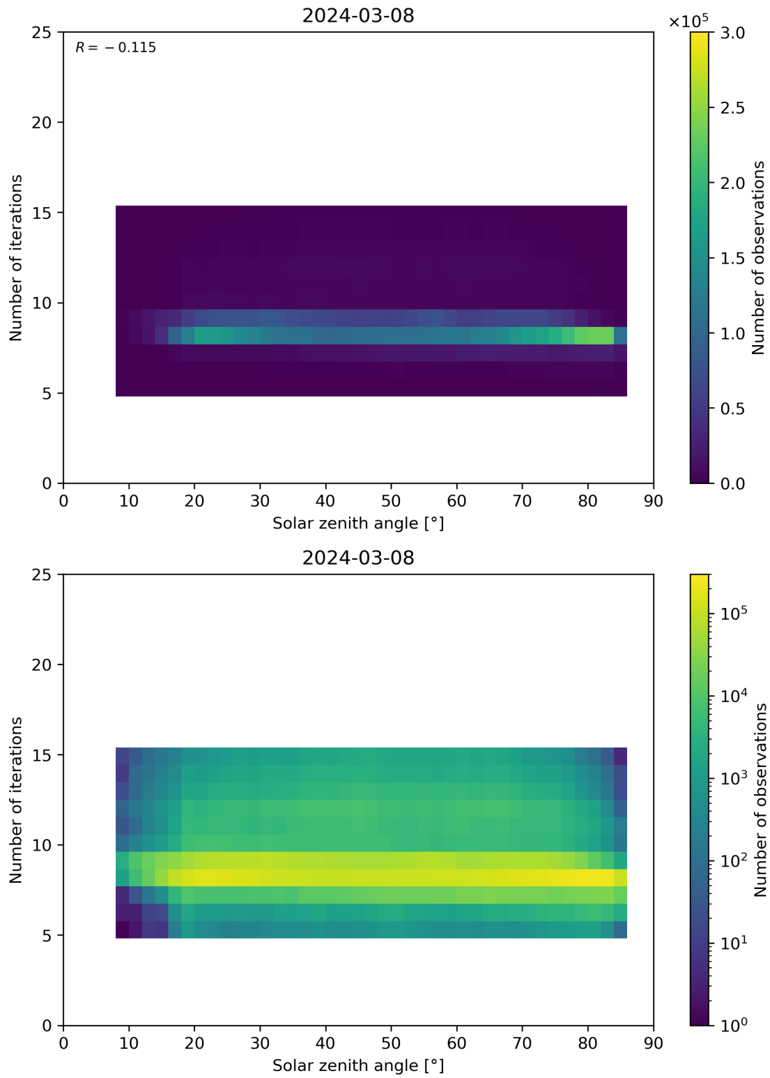
Figure 67: Scatter density plot of “Solar zenith angle” against “Number of iterations” for 2024-03-07 to 2024-03-09.
