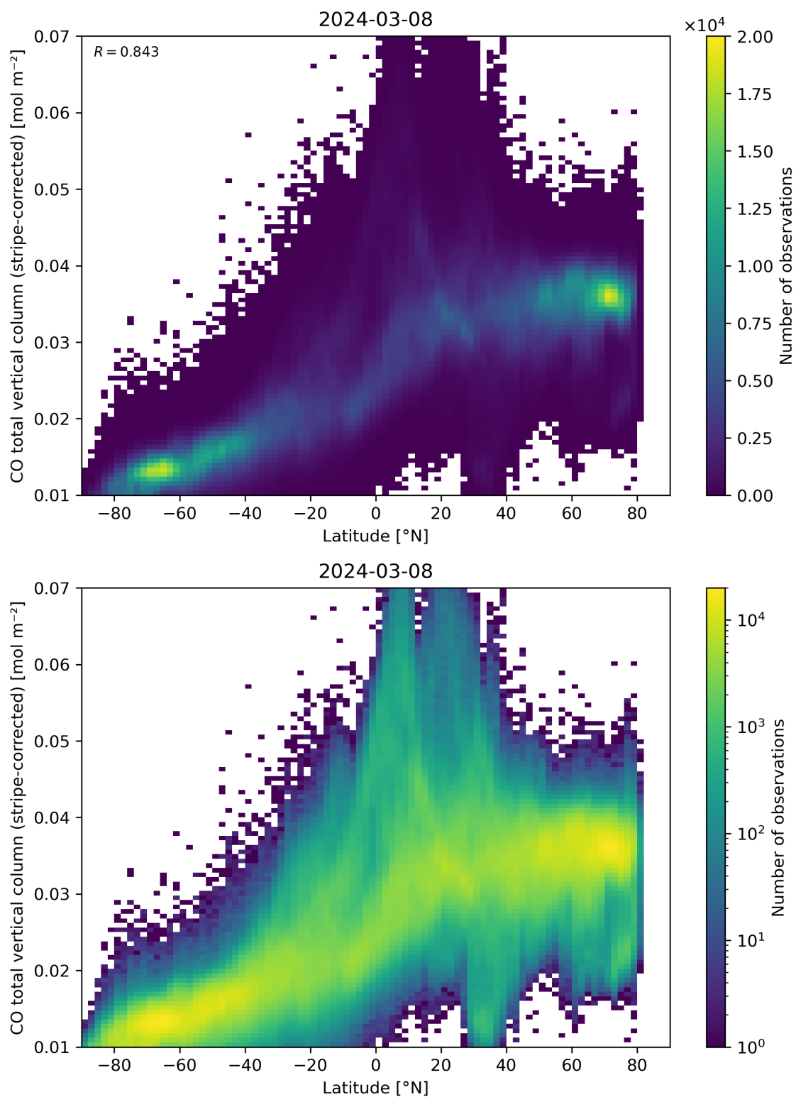
Figure 52: Scatter density plot of “Latitude” against “CO total vertical column (stripe-corrected)” for 2024-03-07 to 2024-03-09.
