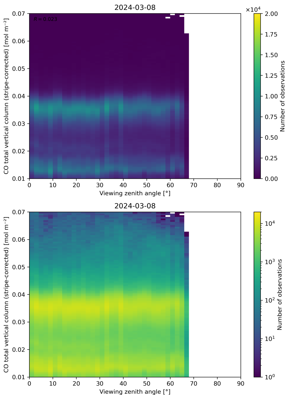
Figure 70: Scatter density plot of “Viewing zenith angle” against “CO total vertical column (stripe-corrected)” for 2024-03-07 to 2024-03-09.
