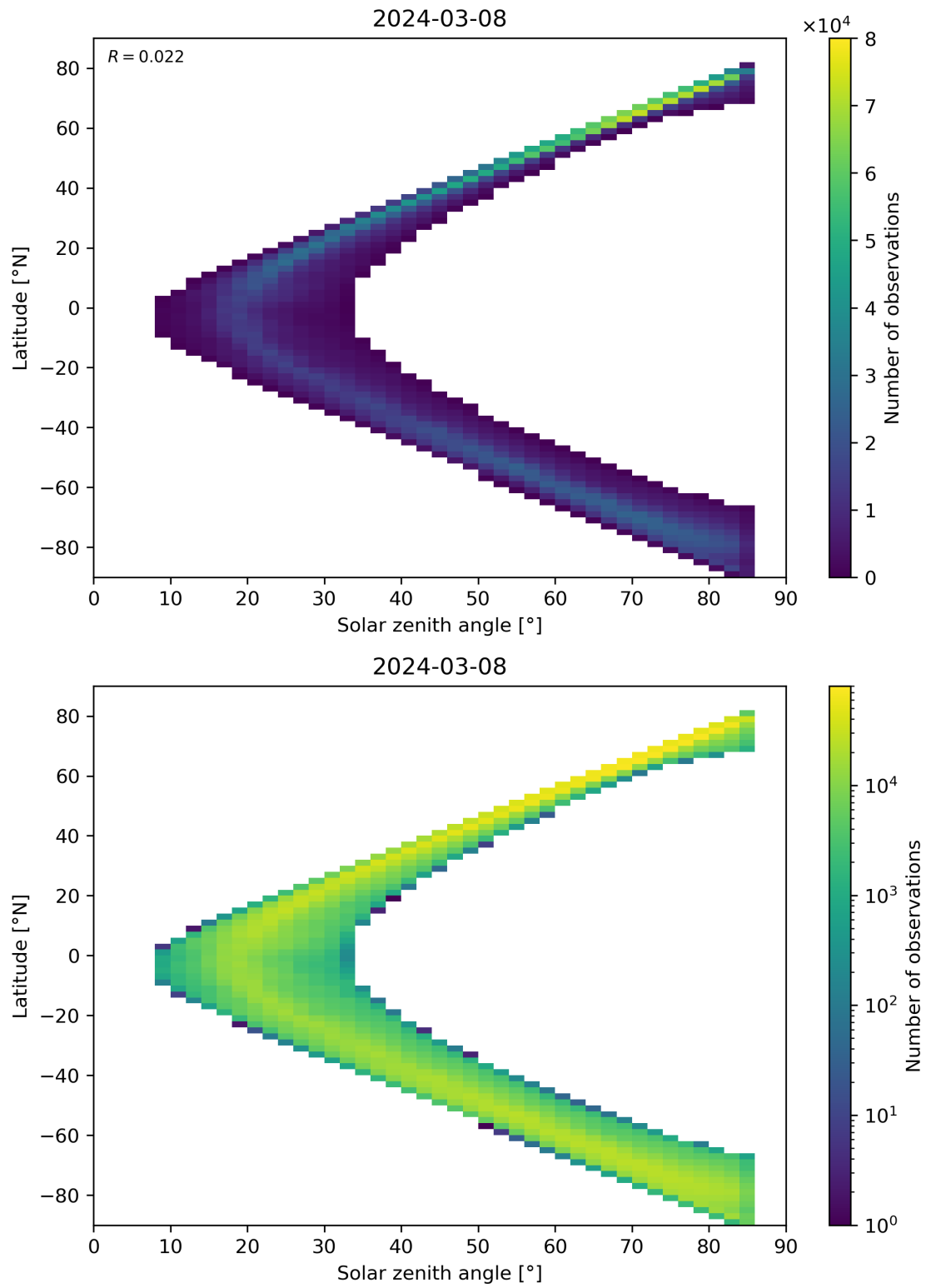
Figure 66: Scatter density plot of “Solar zenith angle” against “Latitude” for 2024-03-07 to 2024-03-09.
