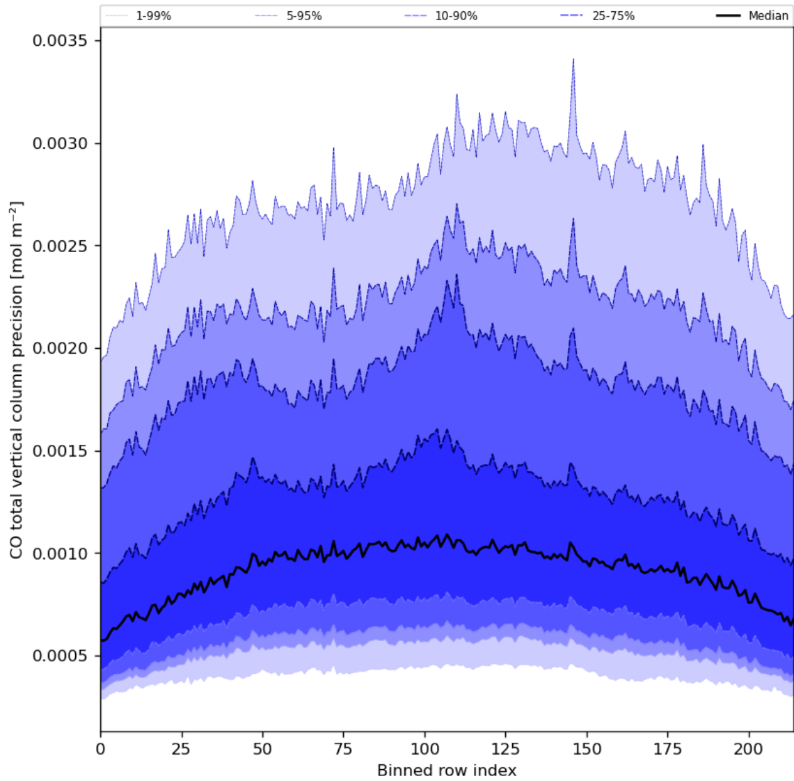
Figure 28: Along track statistics of “CO total vertical column precision” for 2024-03-07 to 2024-03-09
