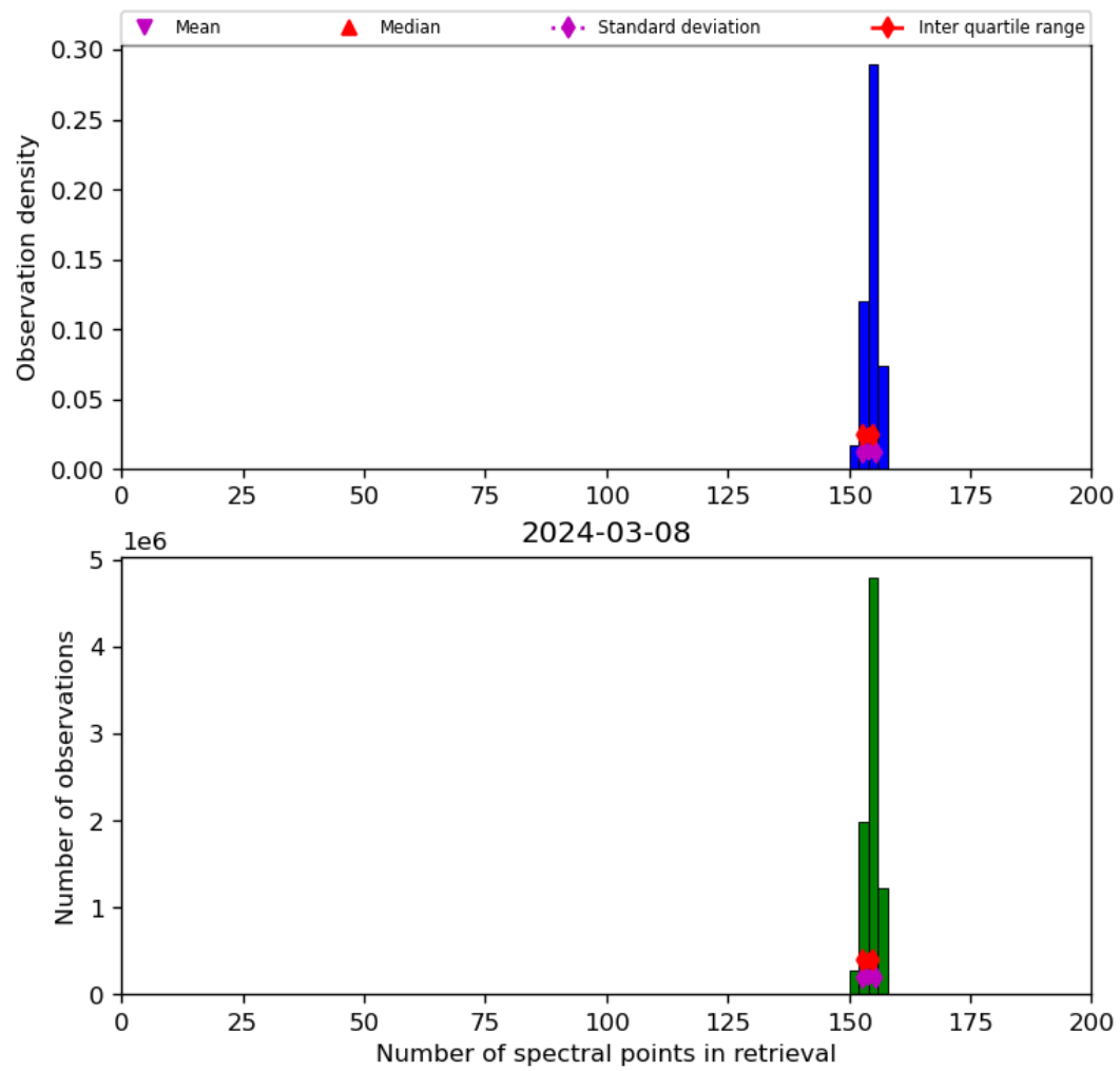
Figure 21: Histogram of “Number of spectral points in retrieval” for 2024-03-07 to 2024-03-09
