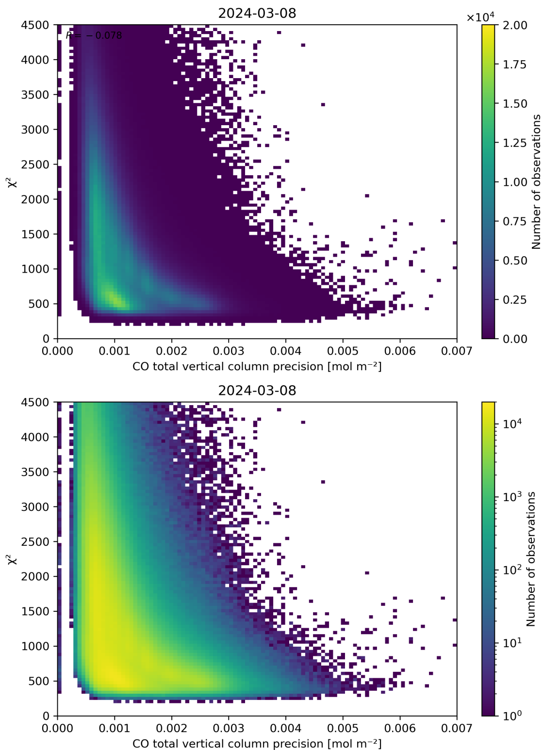
Figure 44: Scatter density plot of “CO total vertical column precision” against “ \chi^2 ” for 2024-03-07 to 2024-03-09.
