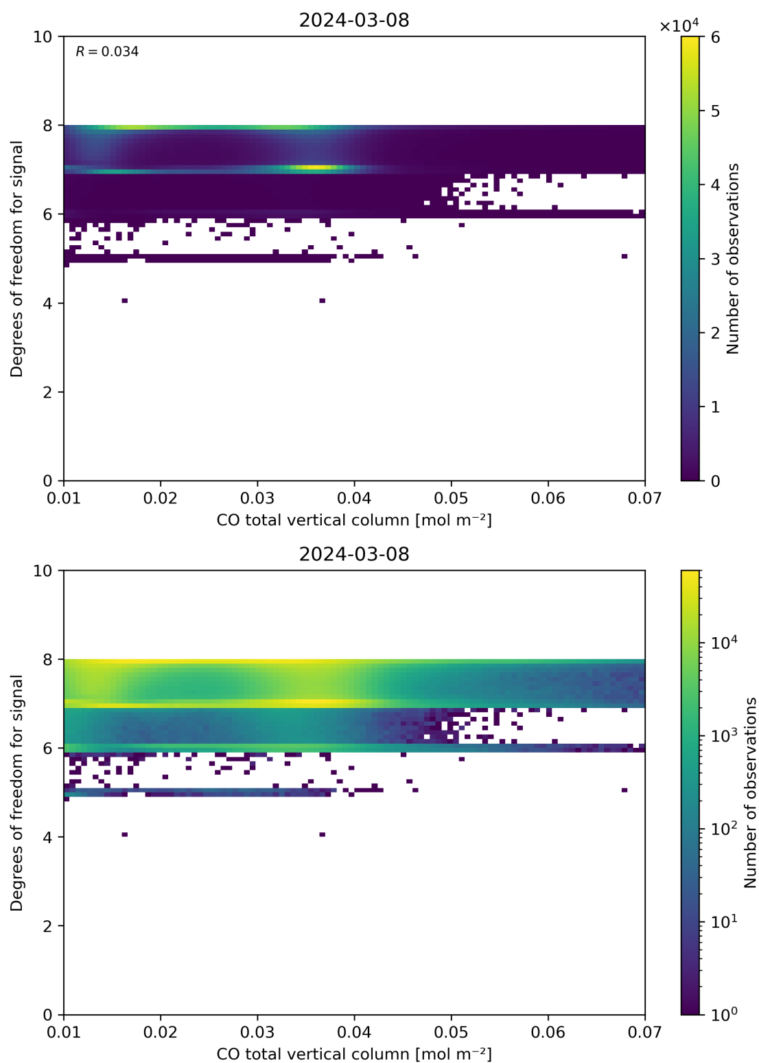
Figure 41: Scatter density plot of “CO total vertical column” against “Degrees of freedom for signal” for 2024-03-07 to 2024-03-09.
