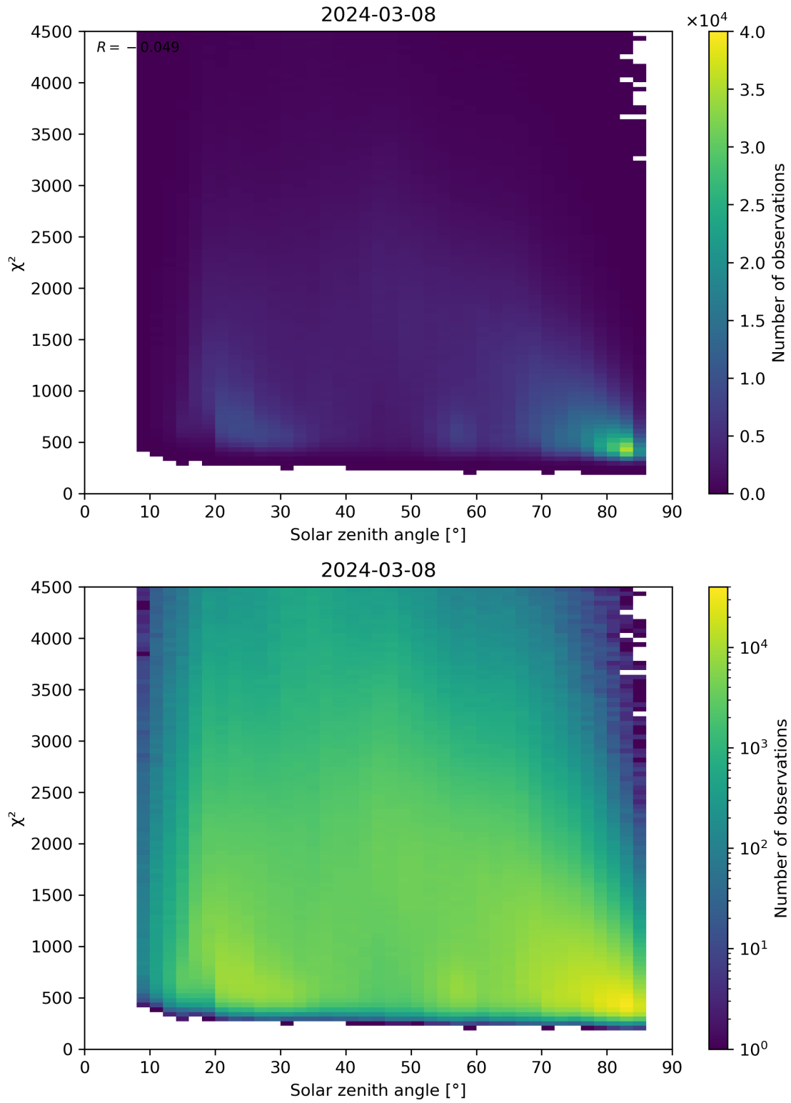
Figure 64: Scatter density plot of “Solar zenith angle” against “ \chi^2 ” for 2024-03-07 to 2024-03-09.
