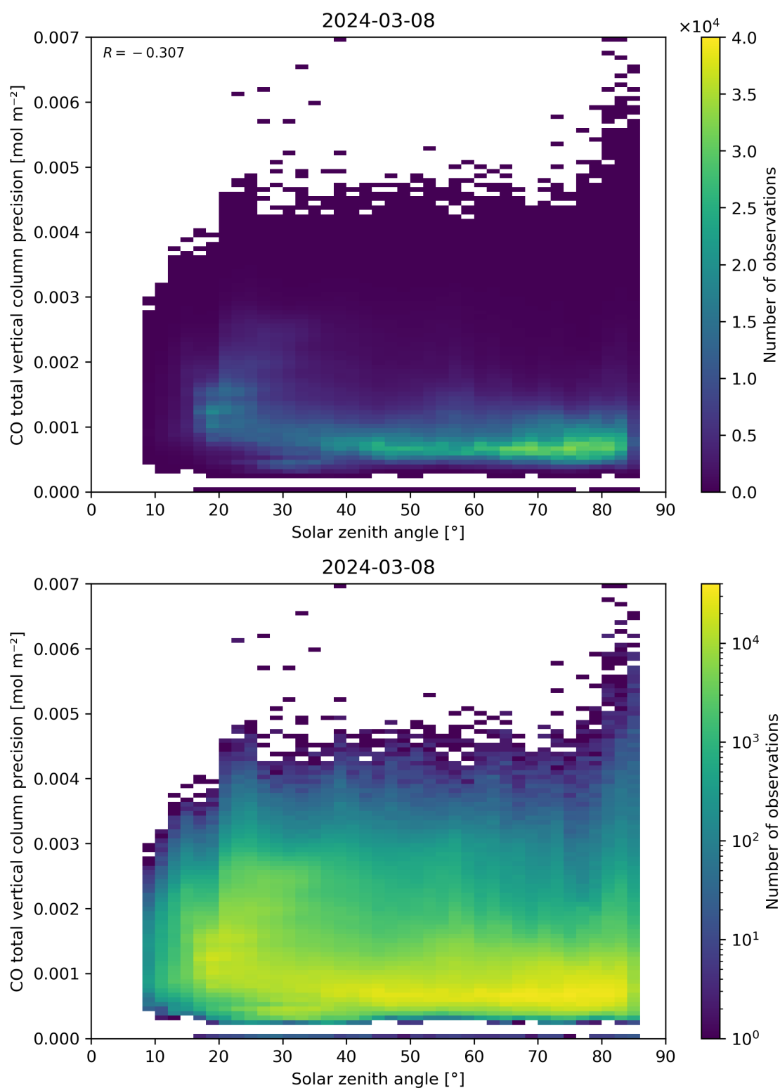
Figure 63: Scatter density plot of “Solar zenith angle” against “CO total vertical column precision” for 2024-03-07 to 2024-03-09.
