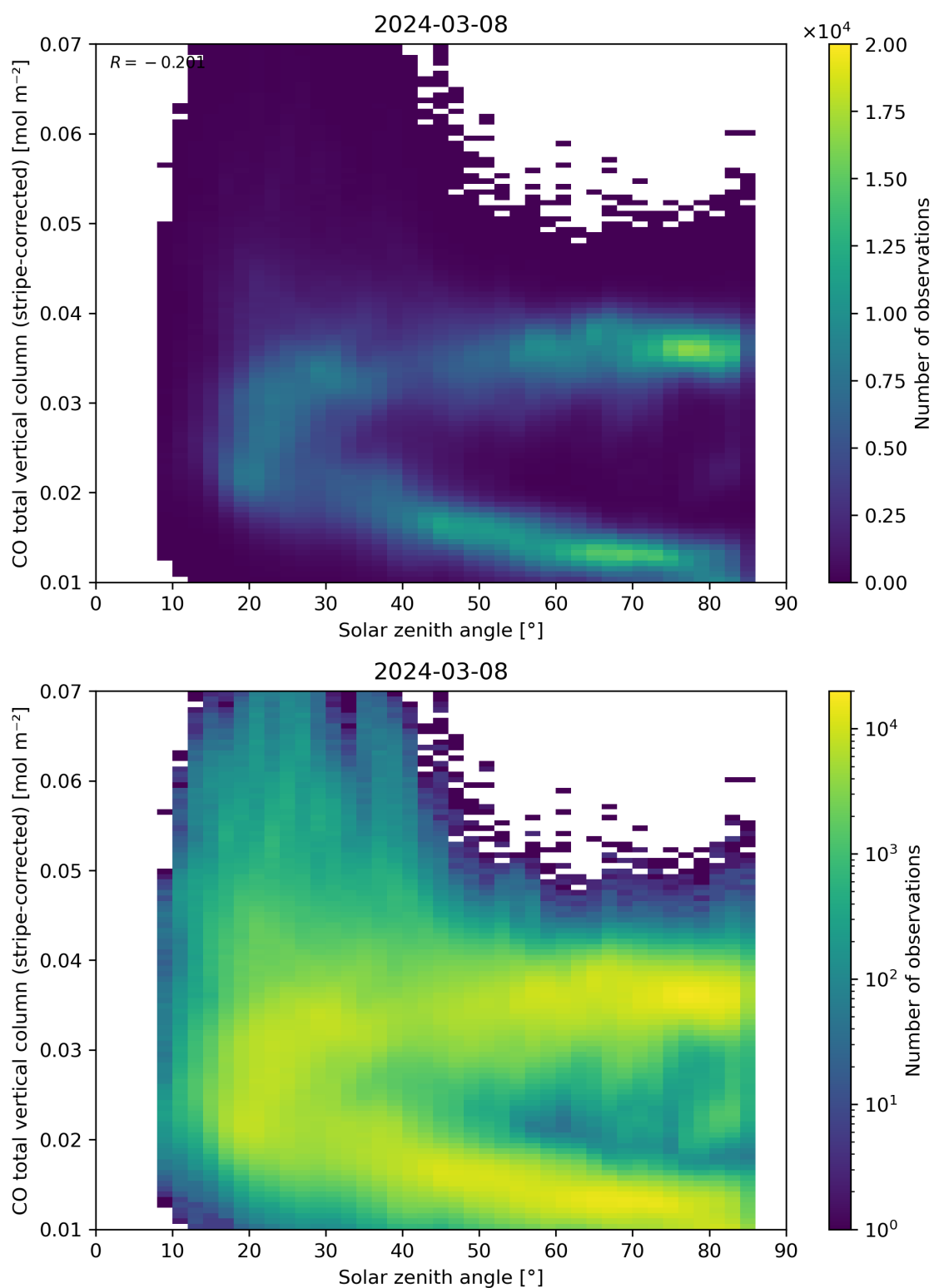
Figure 62: Scatter density plot of “Solar zenith angle” against “CO total vertical column (stripe-corrected)” for 2024-03-07 to 2024-03-09.
