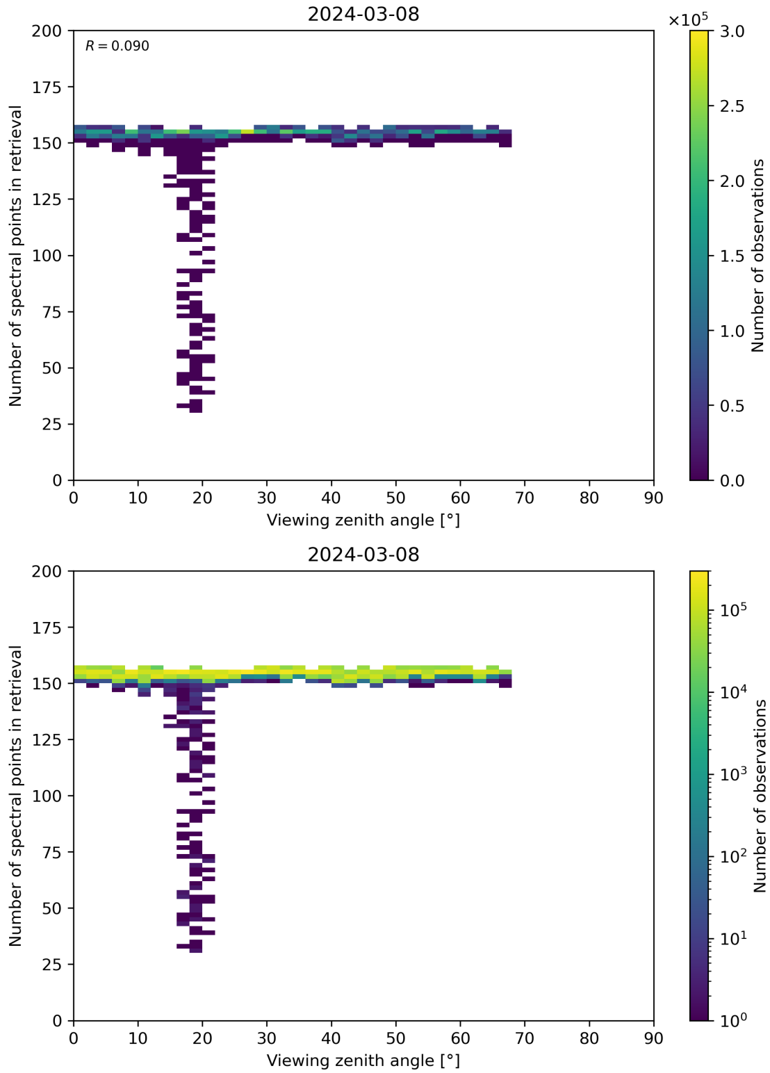
Figure 76: Scatter density plot of “Viewing zenith angle” against “Number of spectral points in retrieval” for 2024-03-07 to 2024-03-09.
