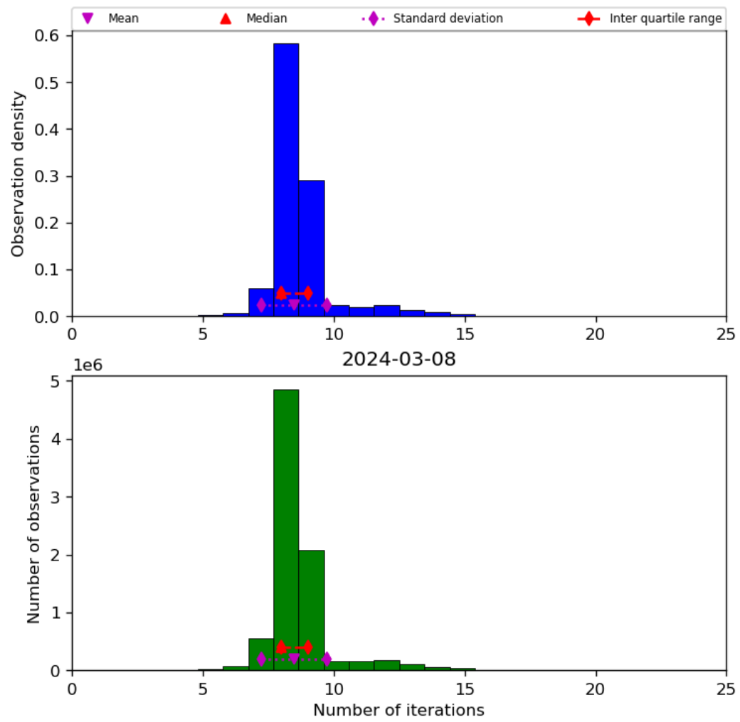
Figure 24: Histogram of “Number of iterations” for 2024-03-07 to 2024-03-09
