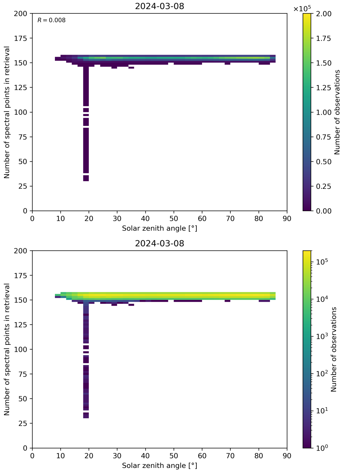
Figure 68: Scatter density plot of “Solar zenith angle” against “Number of spectral points in retrieval” for 2024-03-07 to 2024-03-09.
