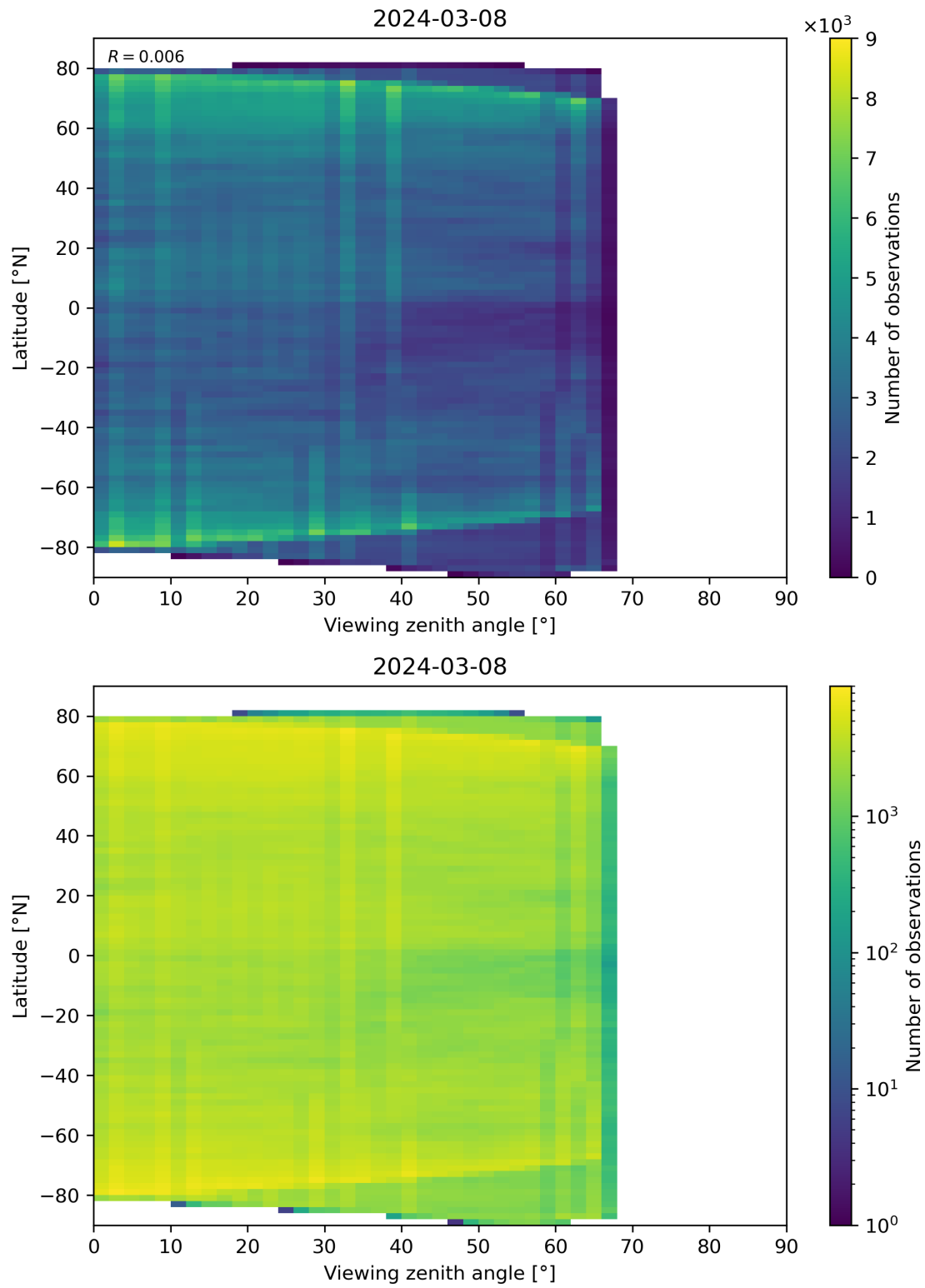
Figure 74: Scatter density plot of “Viewing zenith angle” against “Latitude” for 2024-03-07 to 2024-03-09.
