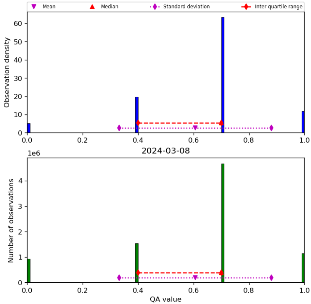
Figure 17: Histogram of “QA value” for 2024-03-07 to 2024-03-09
