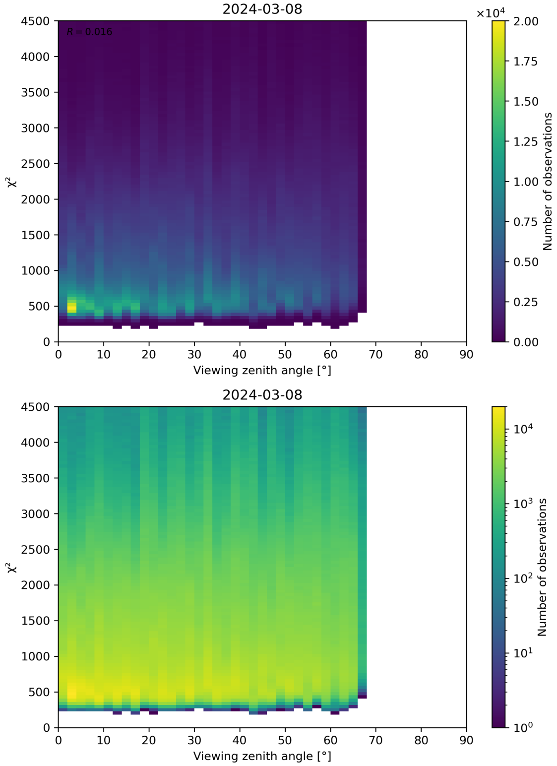
Figure 72: Scatter density plot of “Viewing zenith angle” against “ \chi^2 ” for 2024-03-07 to 2024-03-09.
