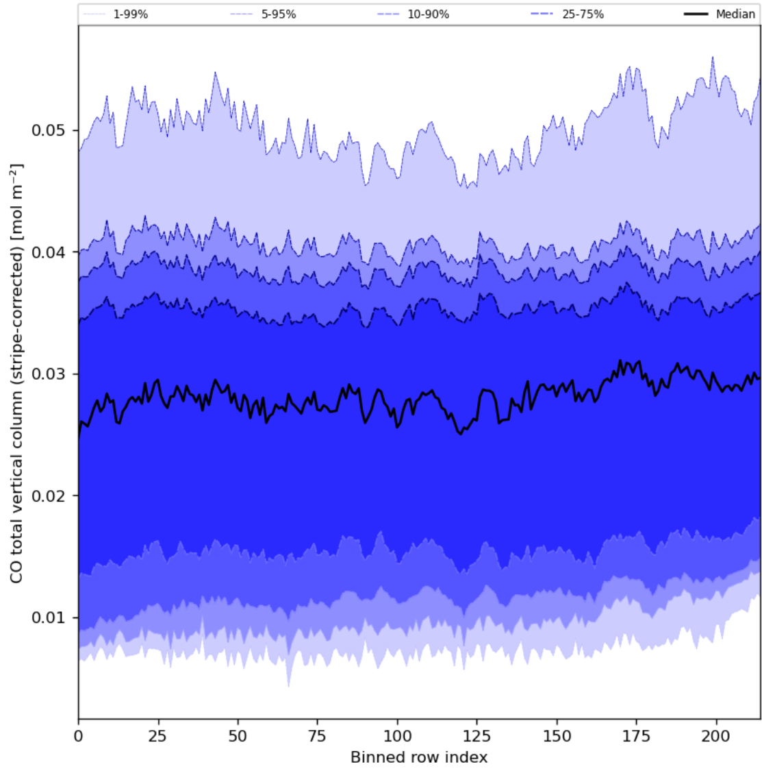
Figure 27: Along track statistics of “CO total vertical column (stripe-corrected)” for 2024-03-07 to 2024-03-09
