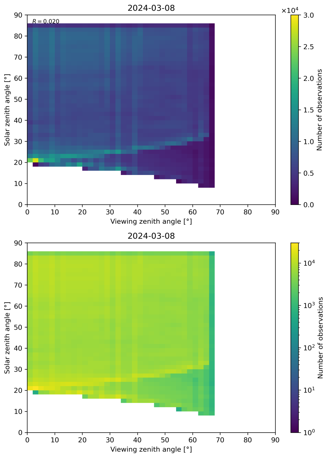
Figure 77: Scatter density plot of “Viewing zenith angle” against “Solar zenith angle” for 2024-03-07 to 2024-03-09.
