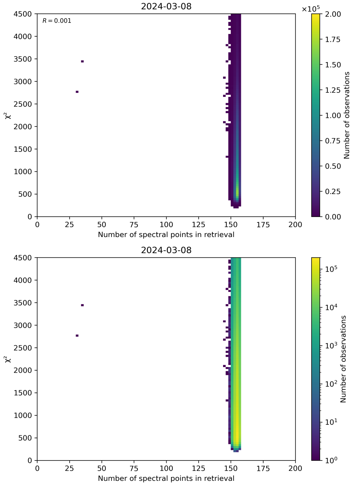
Figure 58: Scatter density plot of “Number of spectral points in retrieval” against “ \chi^2 ” for 2024-03-07 to 2024-03-09.
