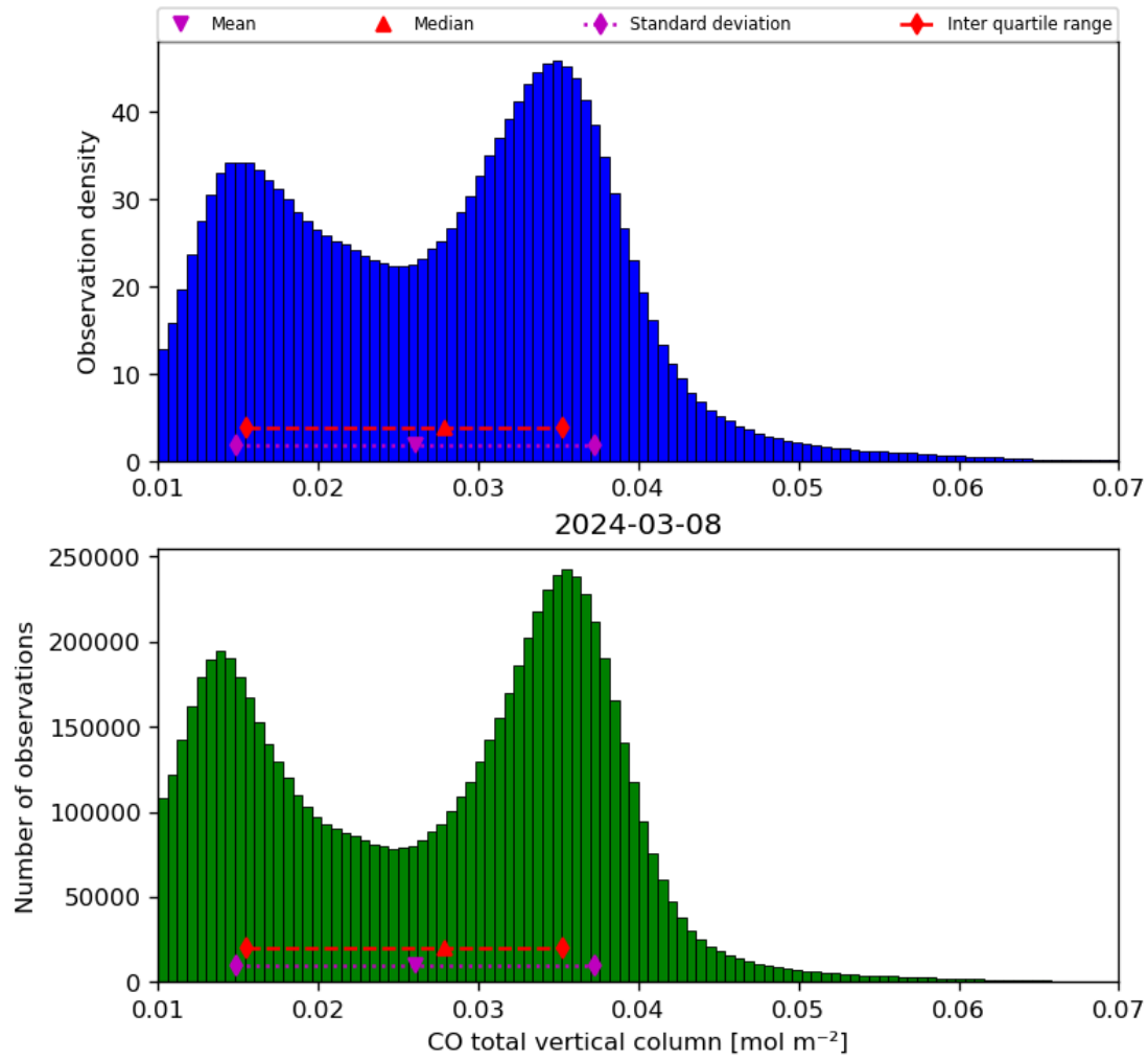
Figure 18: Histogram of “CO total vertical column” for 2024-03-07 to 2024-03-09
