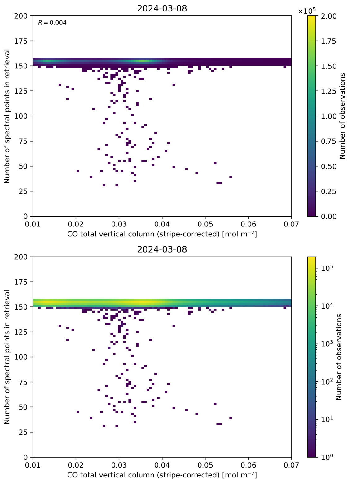
Figure 40: Scatter density plot of “CO total vertical column (stripe-corrected)” against “Number of spectral points in retrieval” for 2024-03-07 to 2024-03-09.
