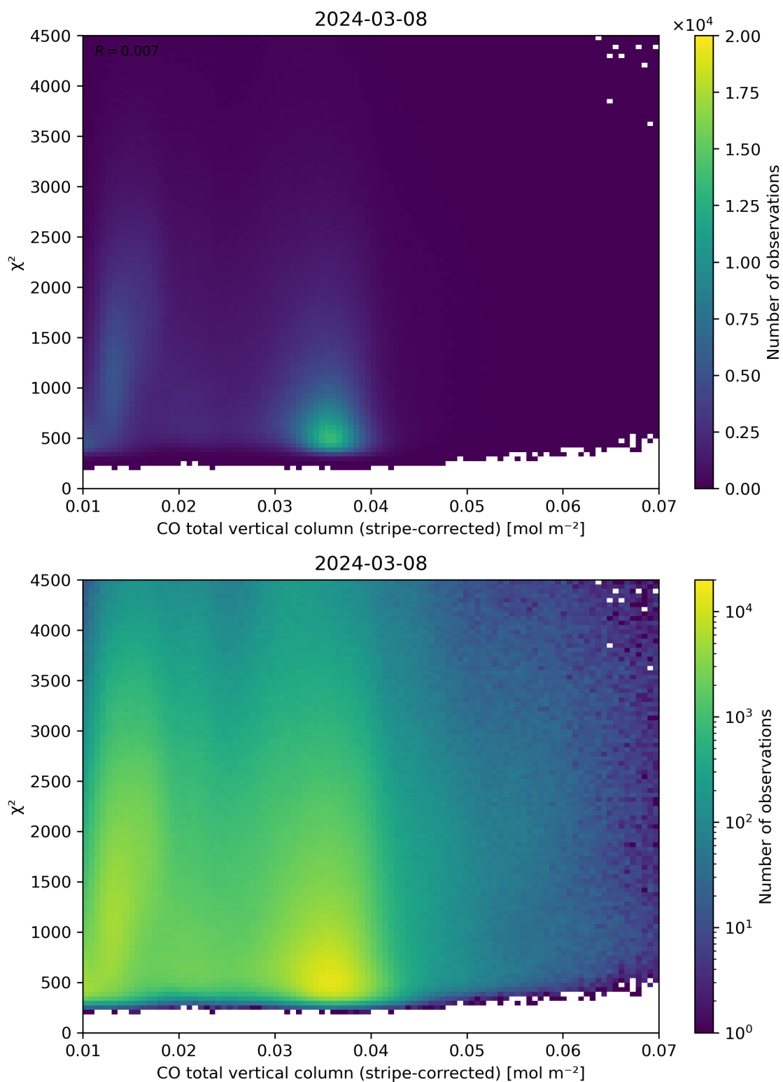
Figure 37: Scatter density plot of “CO total vertical column (stripe-corrected)” against “ \chi^2 ” for 2024-03-07 to 2024-03-09.
