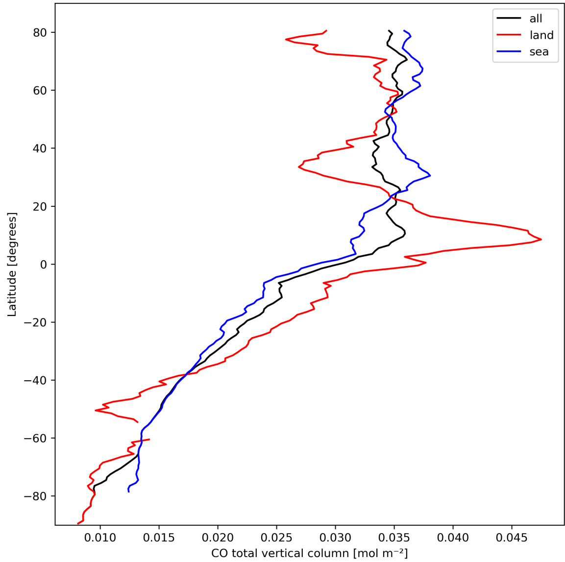
Figure 10: Zonal average of “CO total vertical column” for 2024-03-07 to 2024-03-09.
