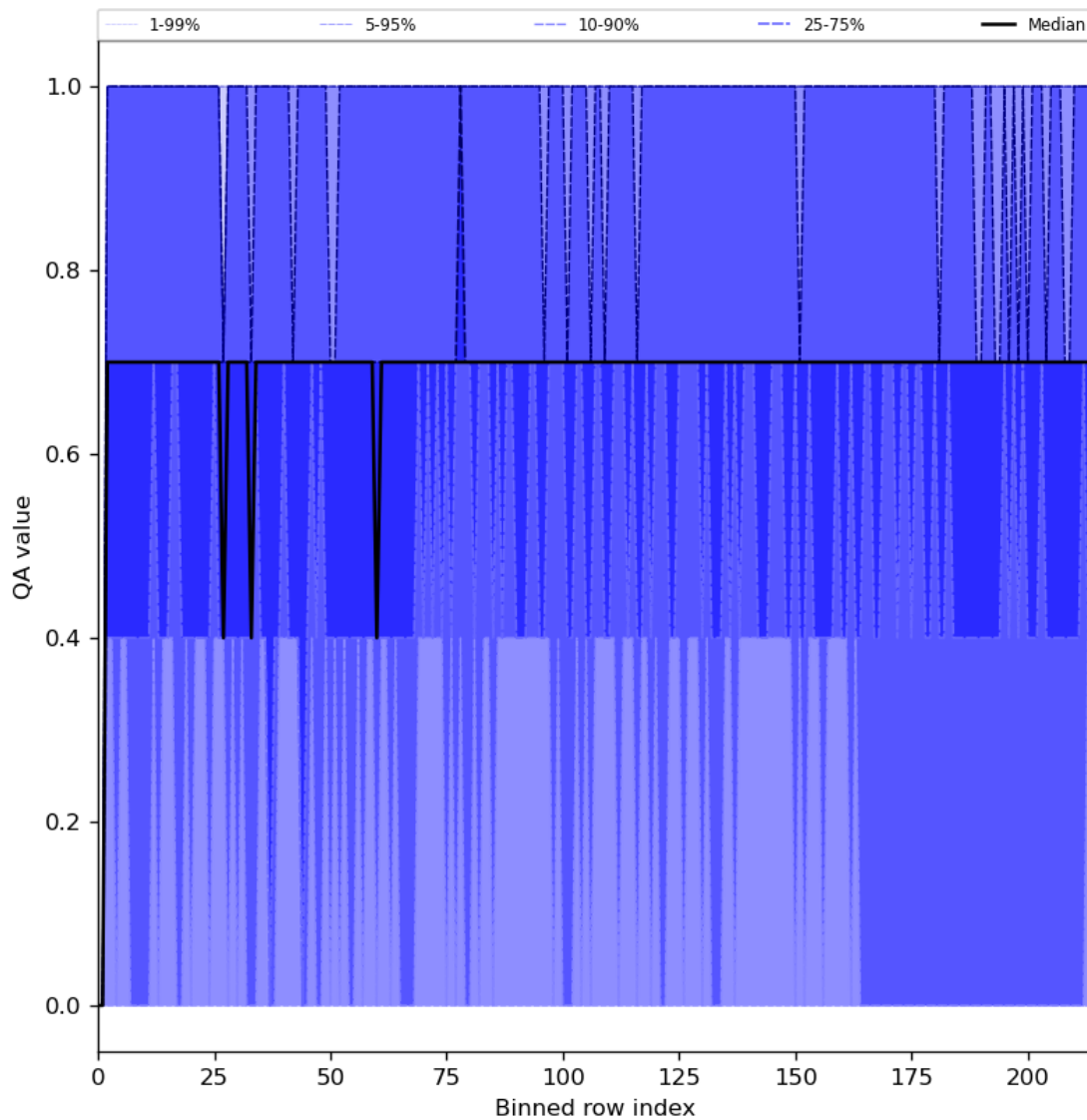
Figure 25: Along track statistics of “QA value” for 2024-03-07 to 2024-03-09
