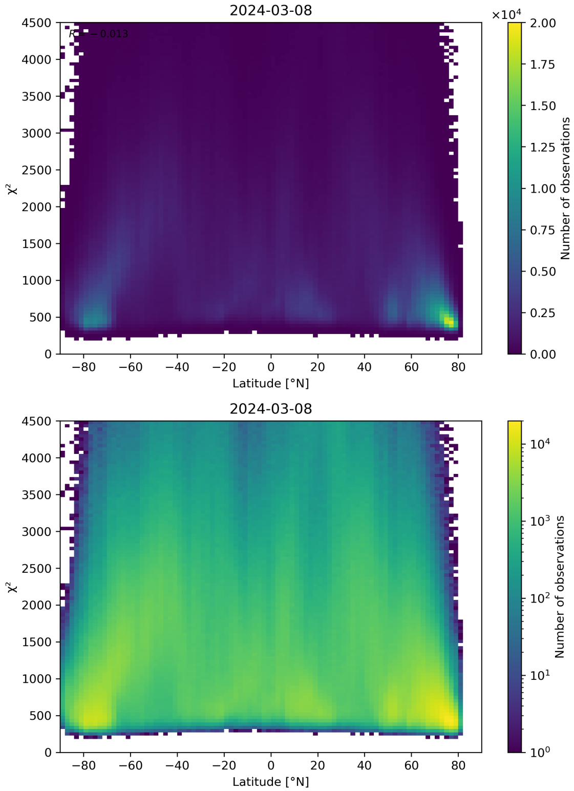
Figure 54: Scatter density plot of “Latitude” against “ \chi^2 ” for 2024-03-07 to 2024-03-09.
