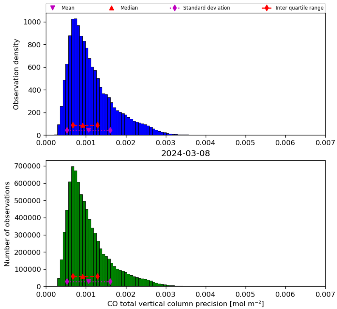
Figure 20: Histogram of “CO total vertical column precision” for 2024-03-07 to 2024-03-09
