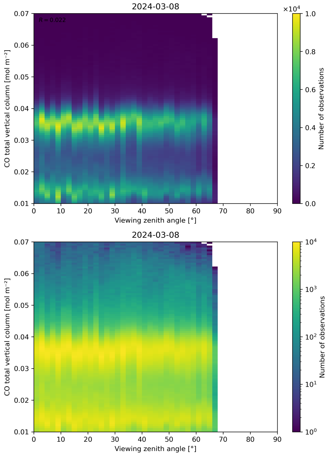
Figure 69: Scatter density plot of “Viewing zenith angle” against “CO total vertical column” for 2024-03-07 to 2024-03-09.
