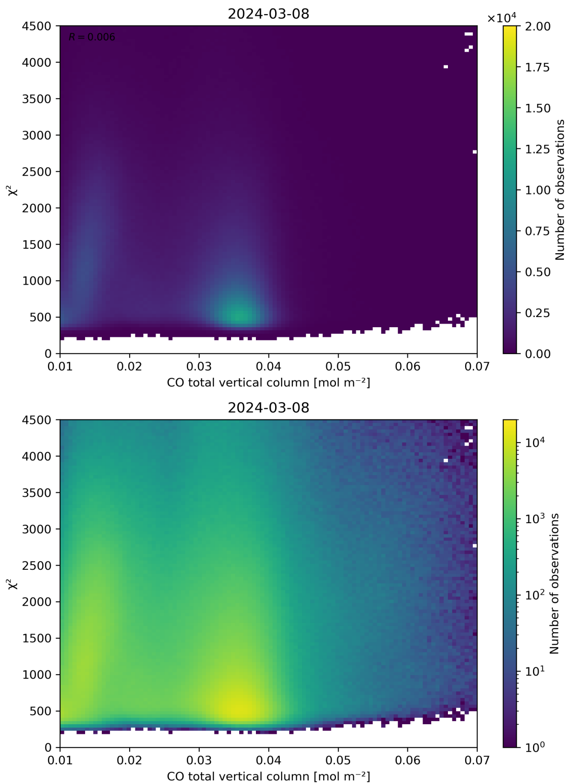
Figure 35: Scatter density plot of “CO total vertical column” against “ \chi^2 ” for 2024-03-07 to 2024-03-09.
