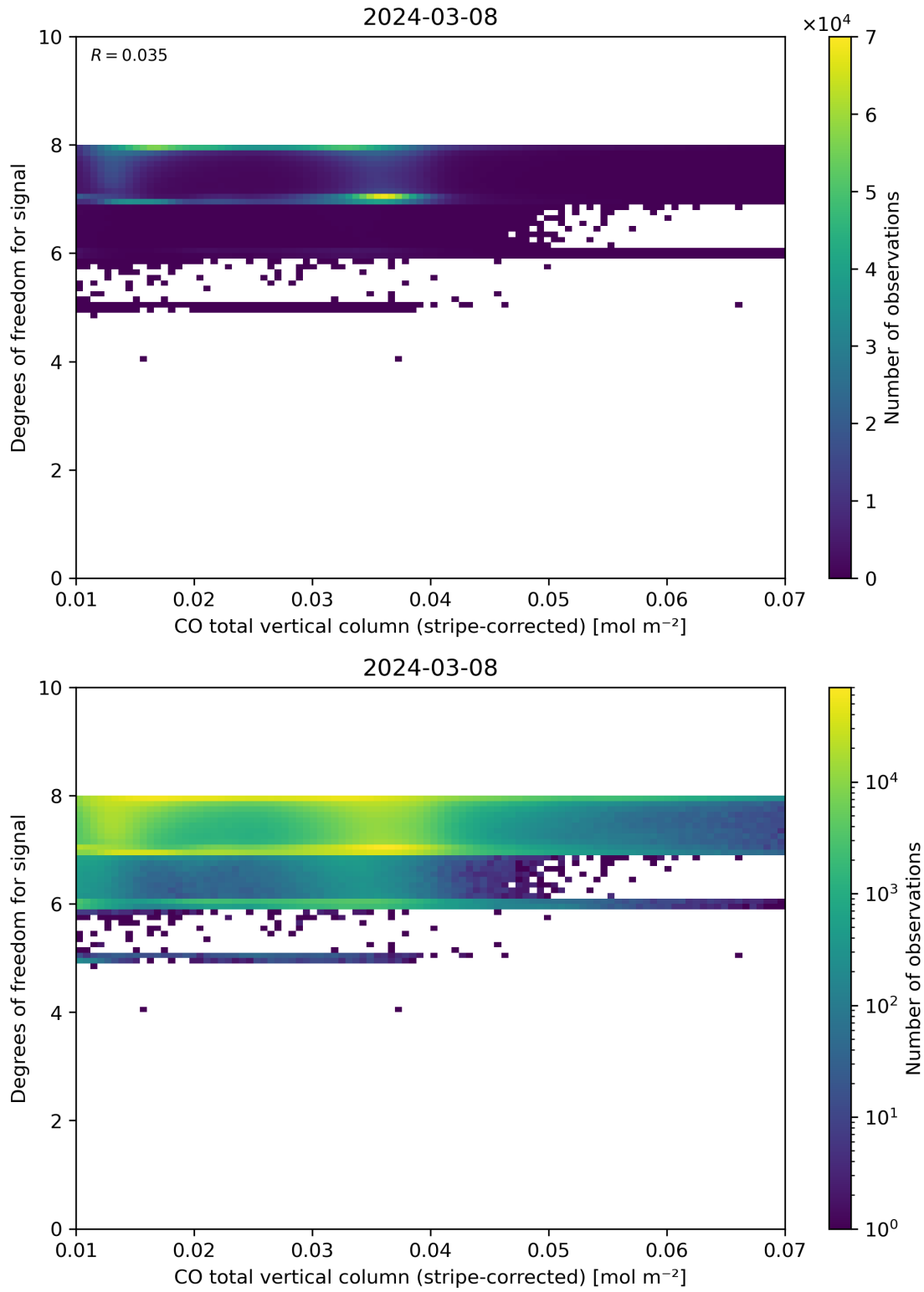
Figure 38: Scatter density plot of “CO total vertical column (stripe-corrected)” against “Degrees of freedom for signal” for 2024-03-07 to 2024-03-09.
