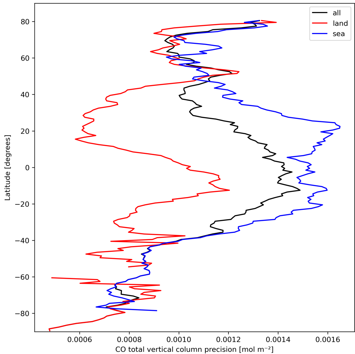
Figure 12: Zonal average of “CO total vertical column precision” for 2024-03-07 to 2024-03-09.
