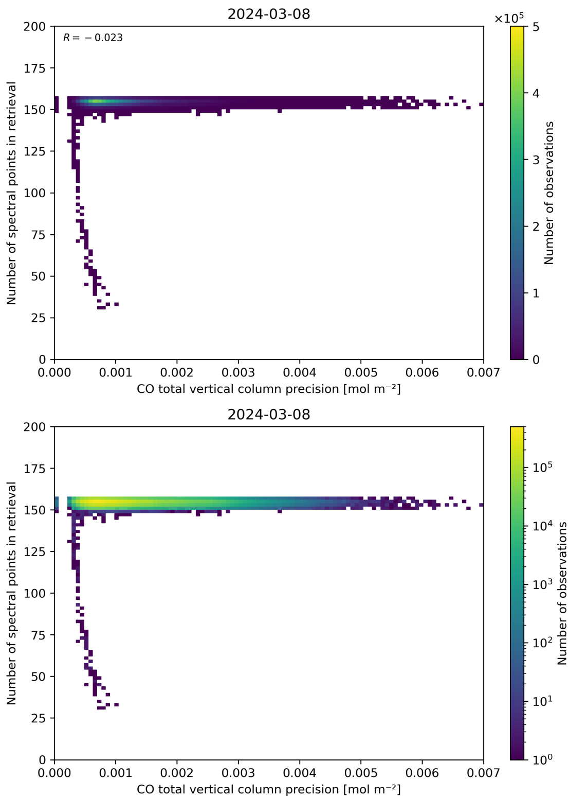
Figure 47: Scatter density plot of “CO total vertical column precision” against “Number of spectral points in retrieval” for 2024-03-07 to 2024-03-09.
