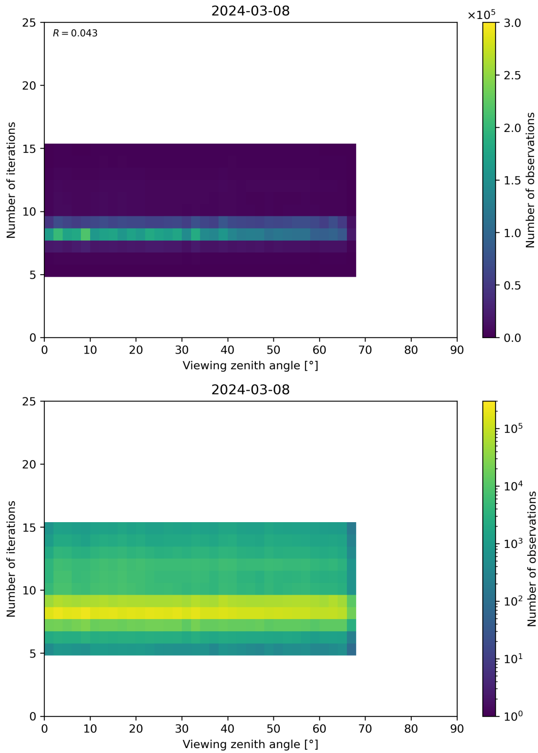
Figure 75: Scatter density plot of “Viewing zenith angle” against “Number of iterations” for 2024-03-07 to 2024-03-09.
