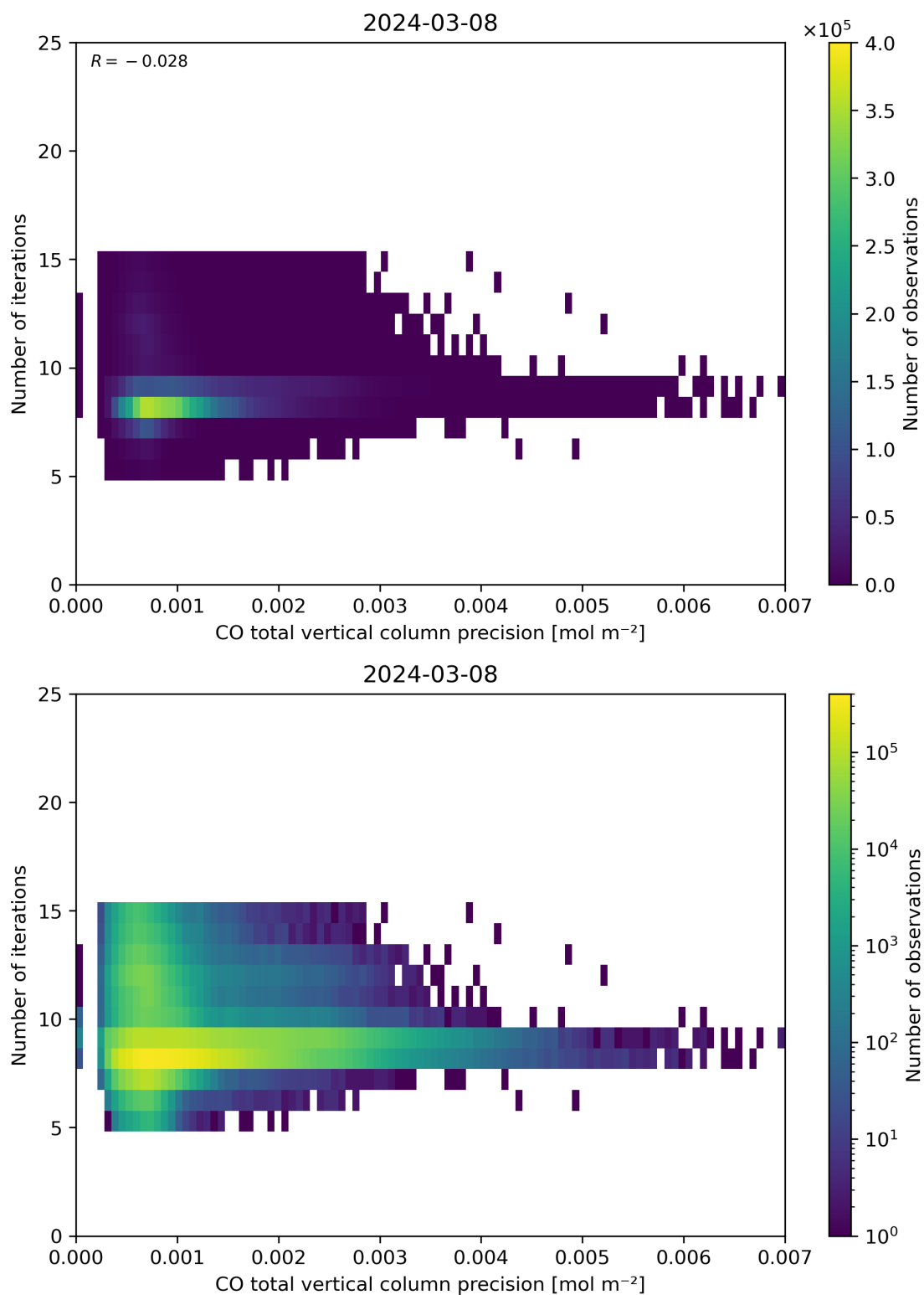
Figure 46: Scatter density plot of “CO total vertical column precision” against “Number of iterations” for 2024-03-07 to 2024-03-09.
