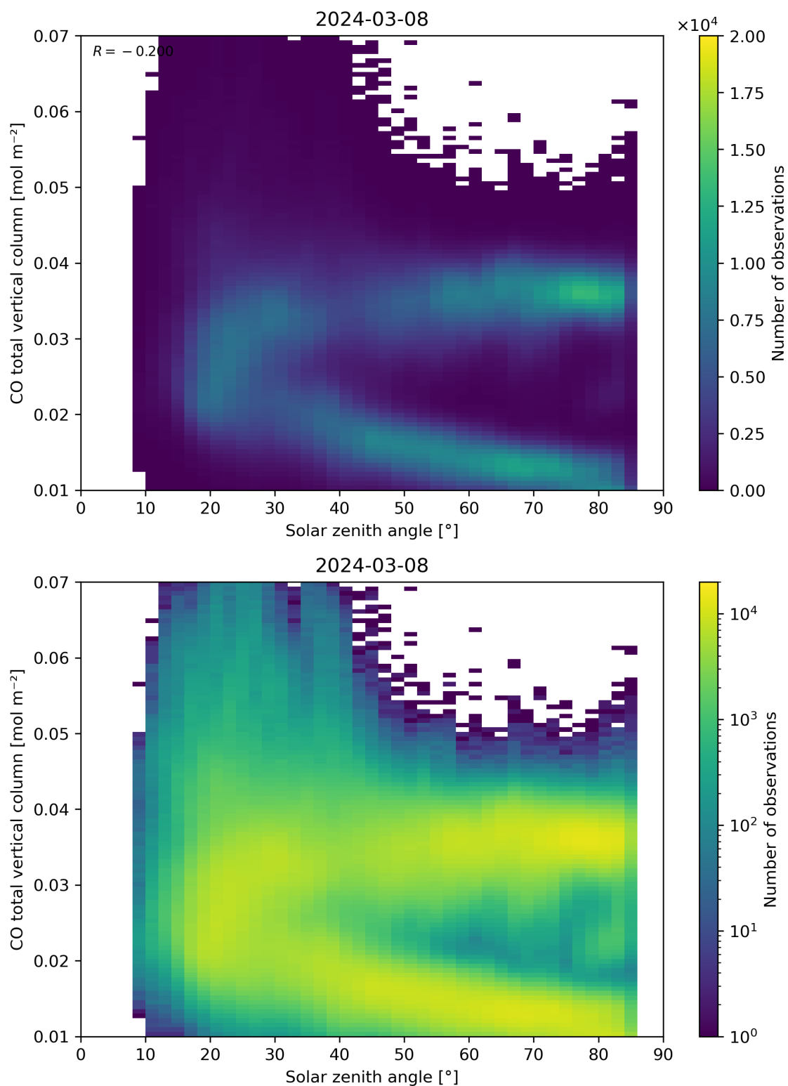
Figure 61: Scatter density plot of “Solar zenith angle” against “CO total vertical column” for 2024-03-07 to 2024-03-09.
