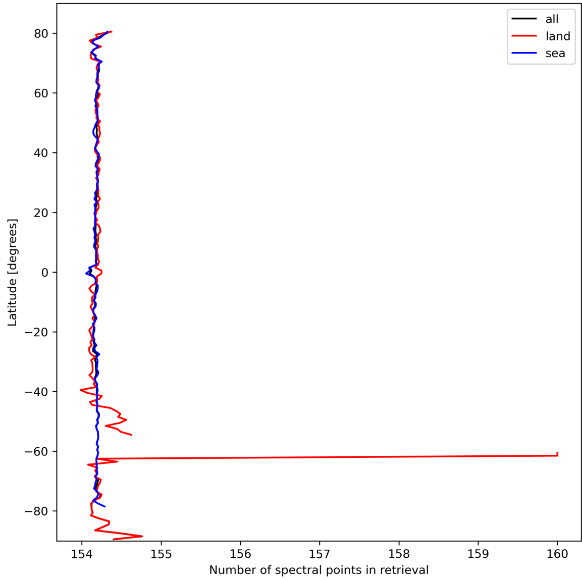
Figure 13: Zonal average of “Number of spectral points in retrieval” for 2024-03-07 to 2024-03-09.
