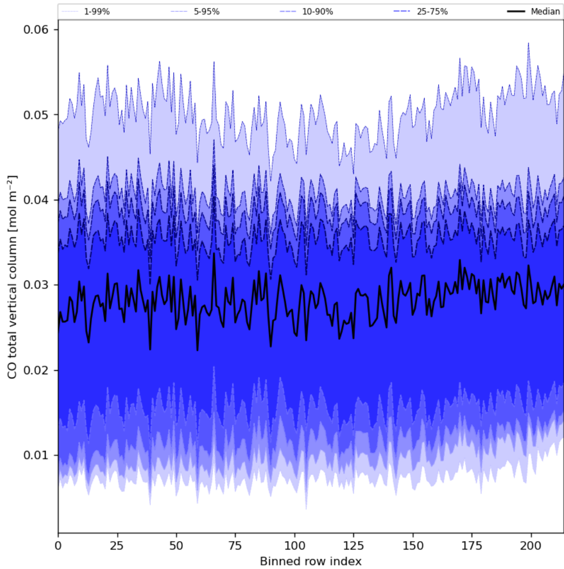
Figure 26: Along track statistics of "CO total vertical column" for 2024-03-07 to 2024-03-09
