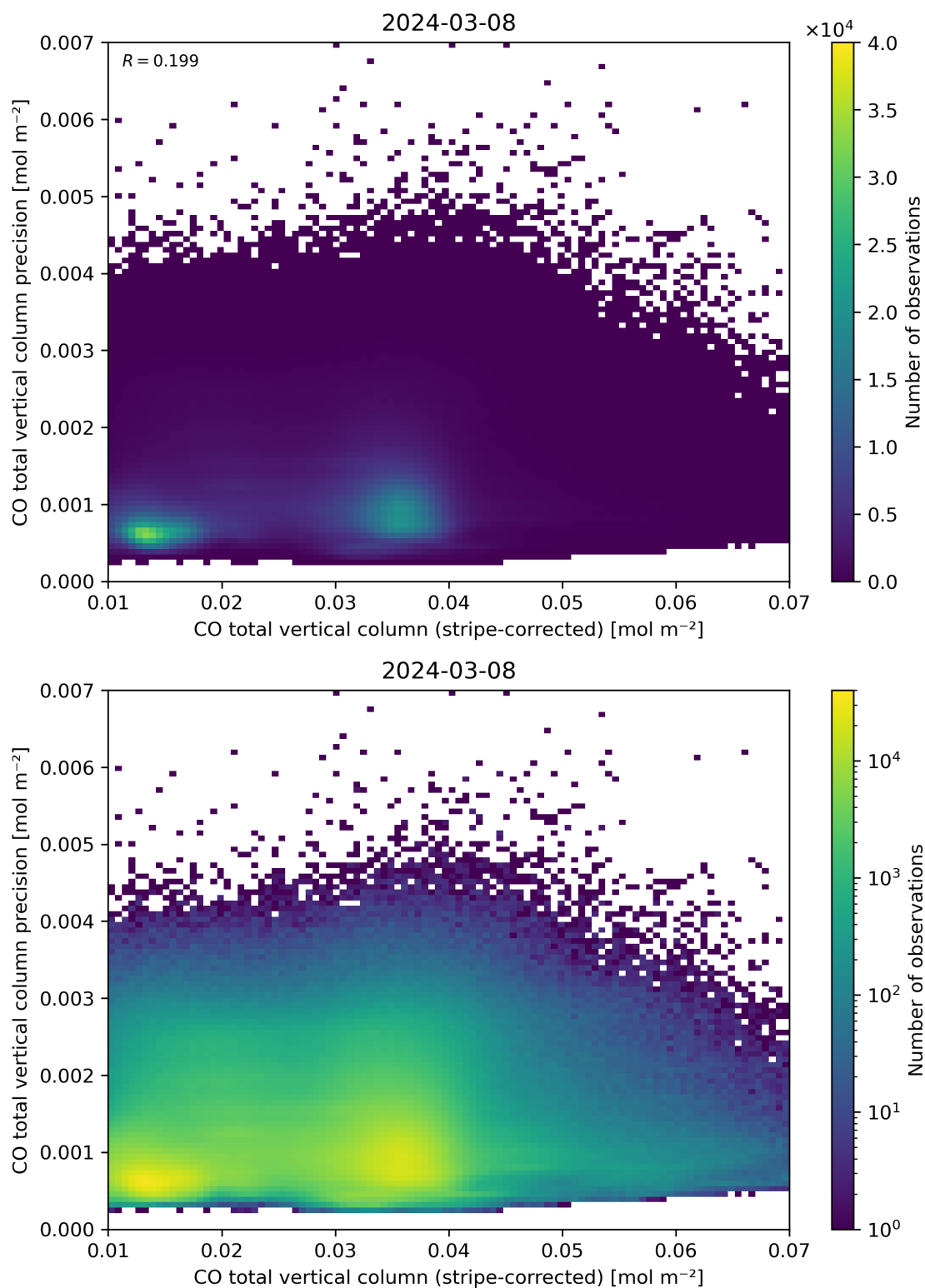
Figure 36: Scatter density plot of “CO total vertical column (stripe-corrected)” against “CO total vertical column precision” for 2024-03-07 to 2024-03-09.
