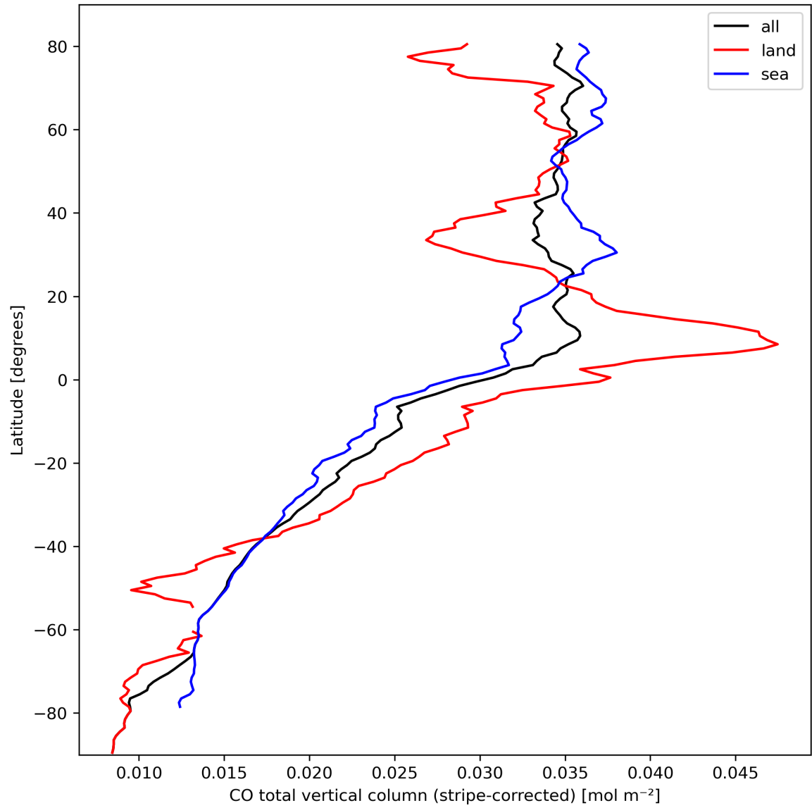
Figure 11: Zonal average of “CO total vertical column (stripe-corrected)” for 2024-03-07 to 2024-03-09.
