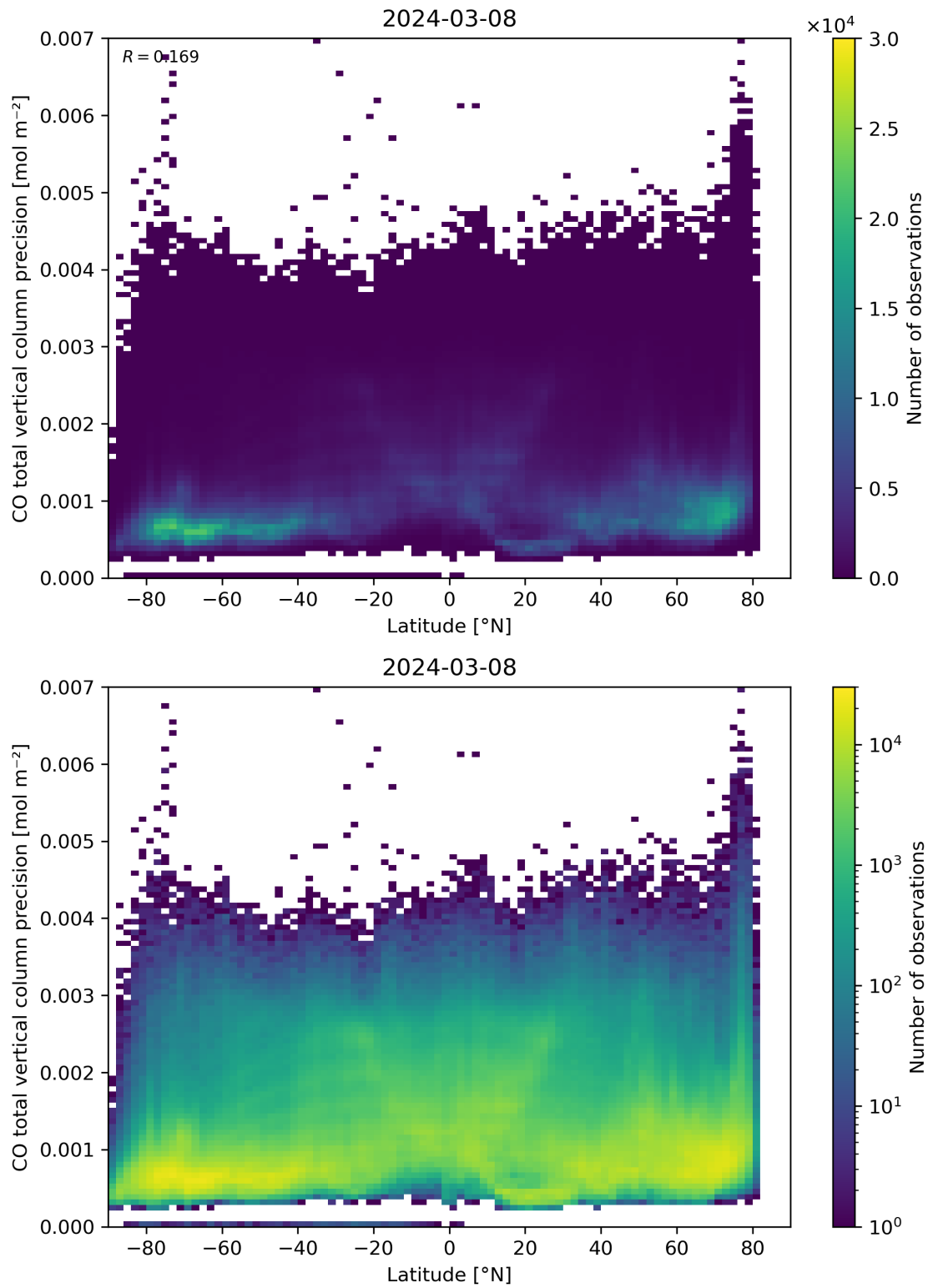
Figure 53: Scatter density plot of “Latitude” against “CO total vertical column precision” for 2024-03-07 to 2024-03-09.
