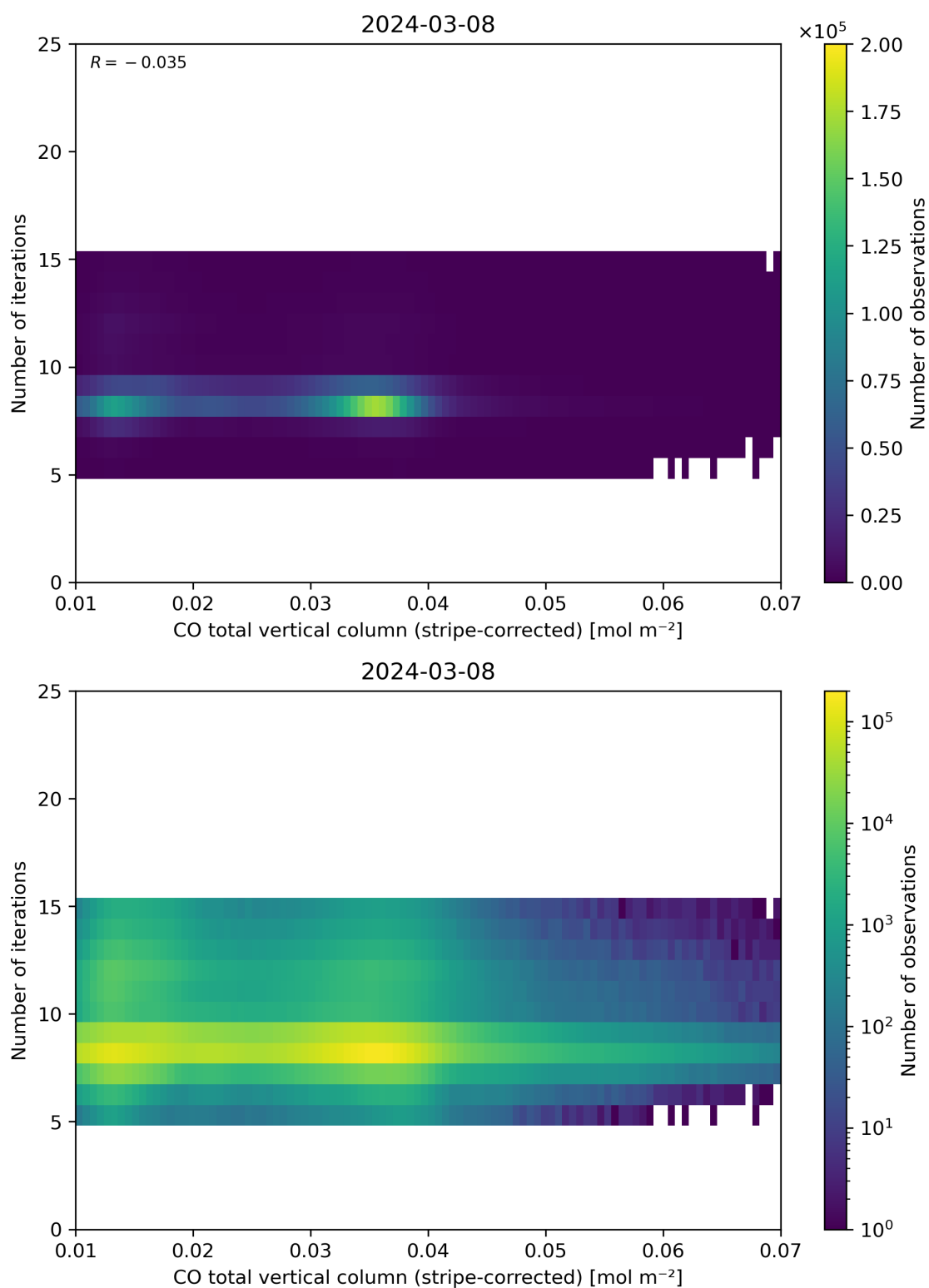
Figure 39: Scatter density plot of “CO total vertical column (stripe-corrected)” against “Number of iterations” for 2024-03-07 to 2024-03-09.
