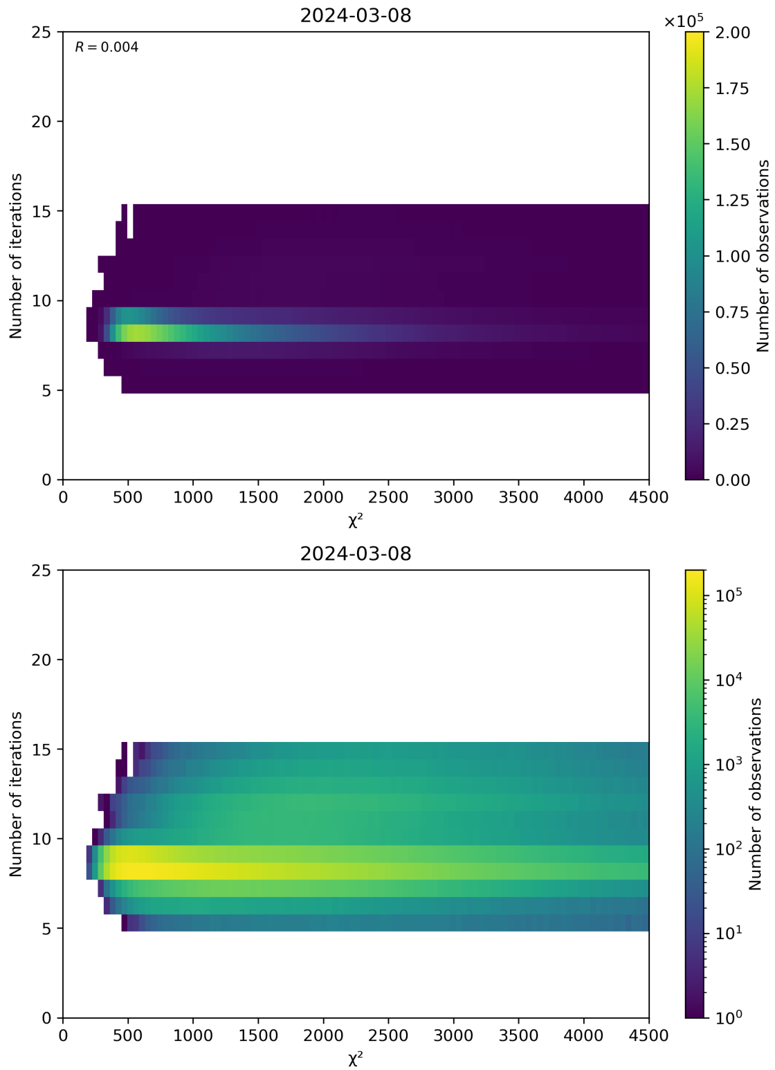
Figure 49: Scatter density plot of “ \chi^2 ” against “Number of iterations” for 2024-03-07 to 2024-03-09.
