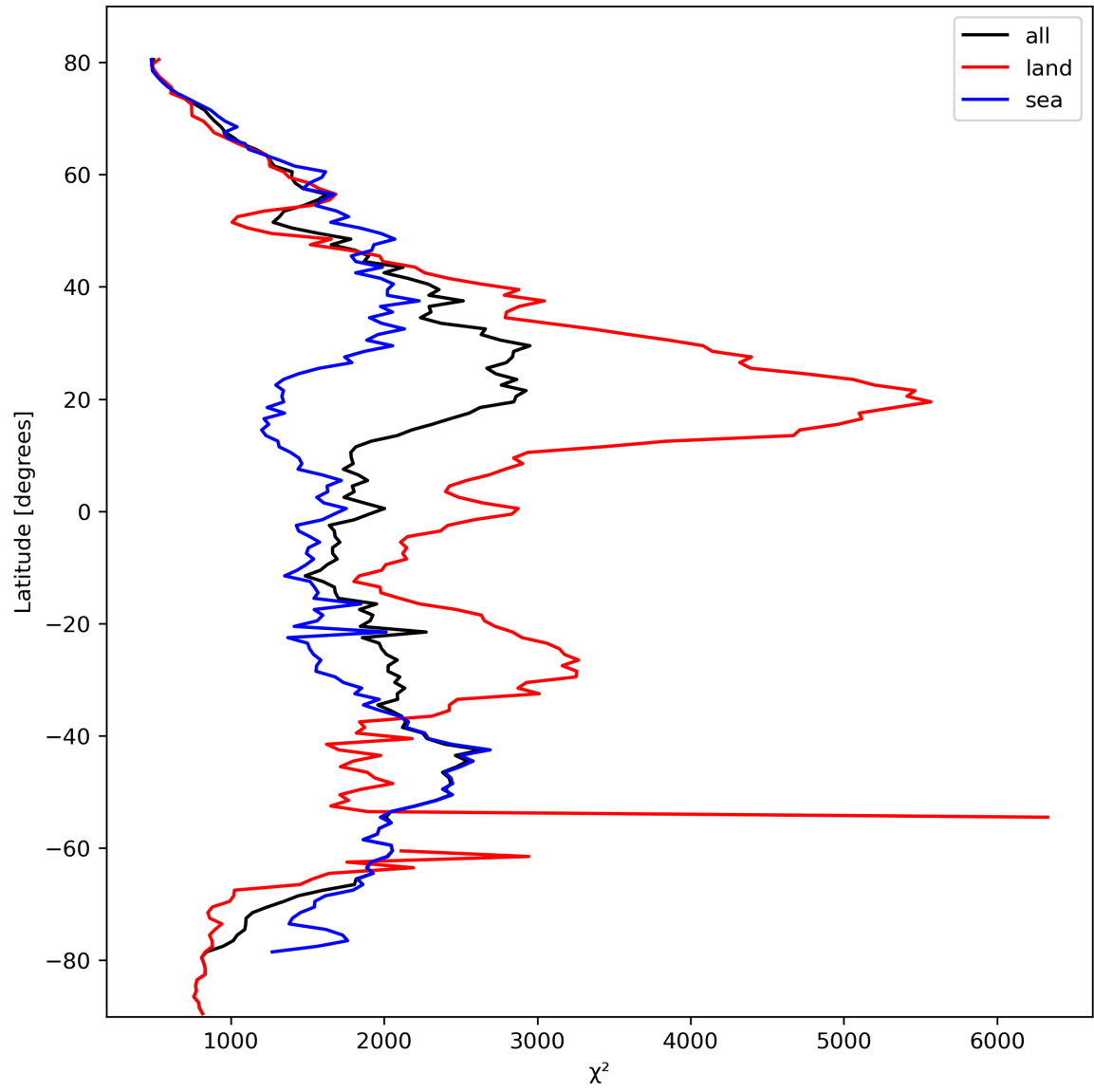
Figure 14: Zonal average of “ \chi^2 ” for 2024-03-07 to 2024-03-09.
