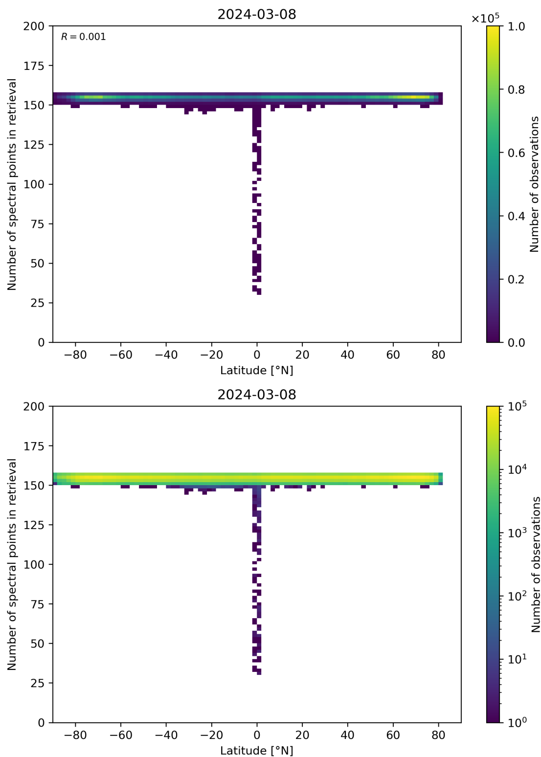
Figure 57: Scatter density plot of “Latitude” against “Number of spectral points in retrieval” for 2024-03-07 to 2024-03-09.
