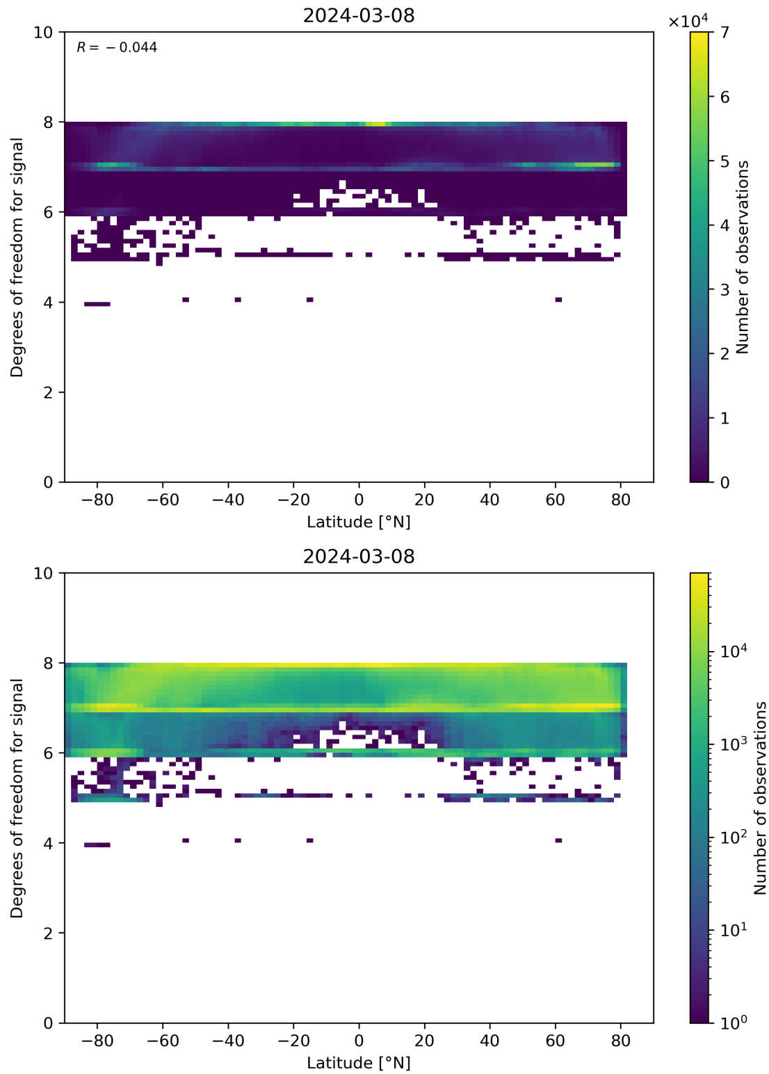
Figure 55: Scatter density plot of “Latitude” against “Degrees of freedom for signal” for 2024-03-07 to 2024-03-09.
