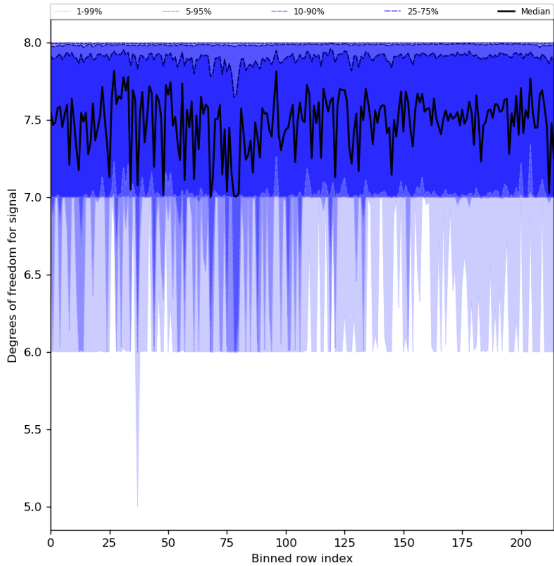
Figure 31: Along track statistics of “Degrees of freedom for signal” for 2024-03-07 to 2024-03-09
