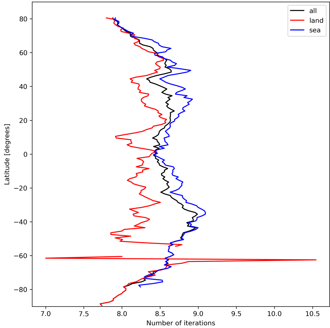
Figure 16: Zonal average of “Number of iterations” for 2024-03-07 to 2024-03-09.
