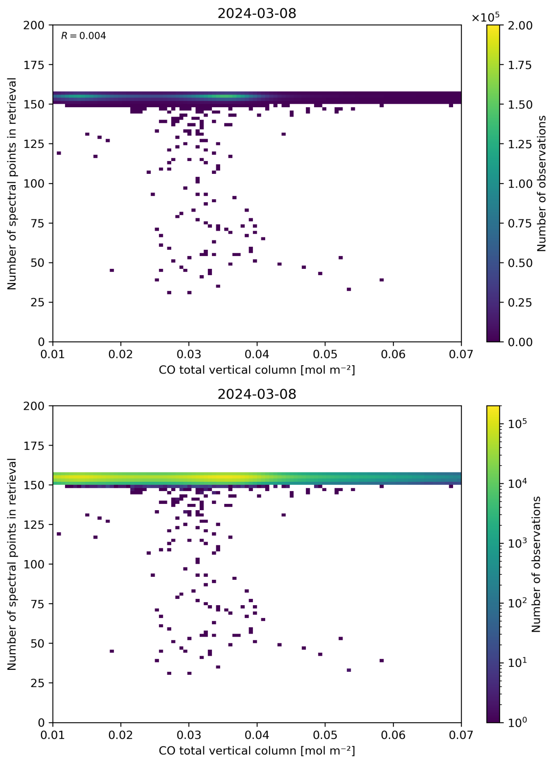
Figure 43: Scatter density plot of “CO total vertical column” against “Number of spectral points in retrieval” for 2024-03-07 to 2024-03-09.
