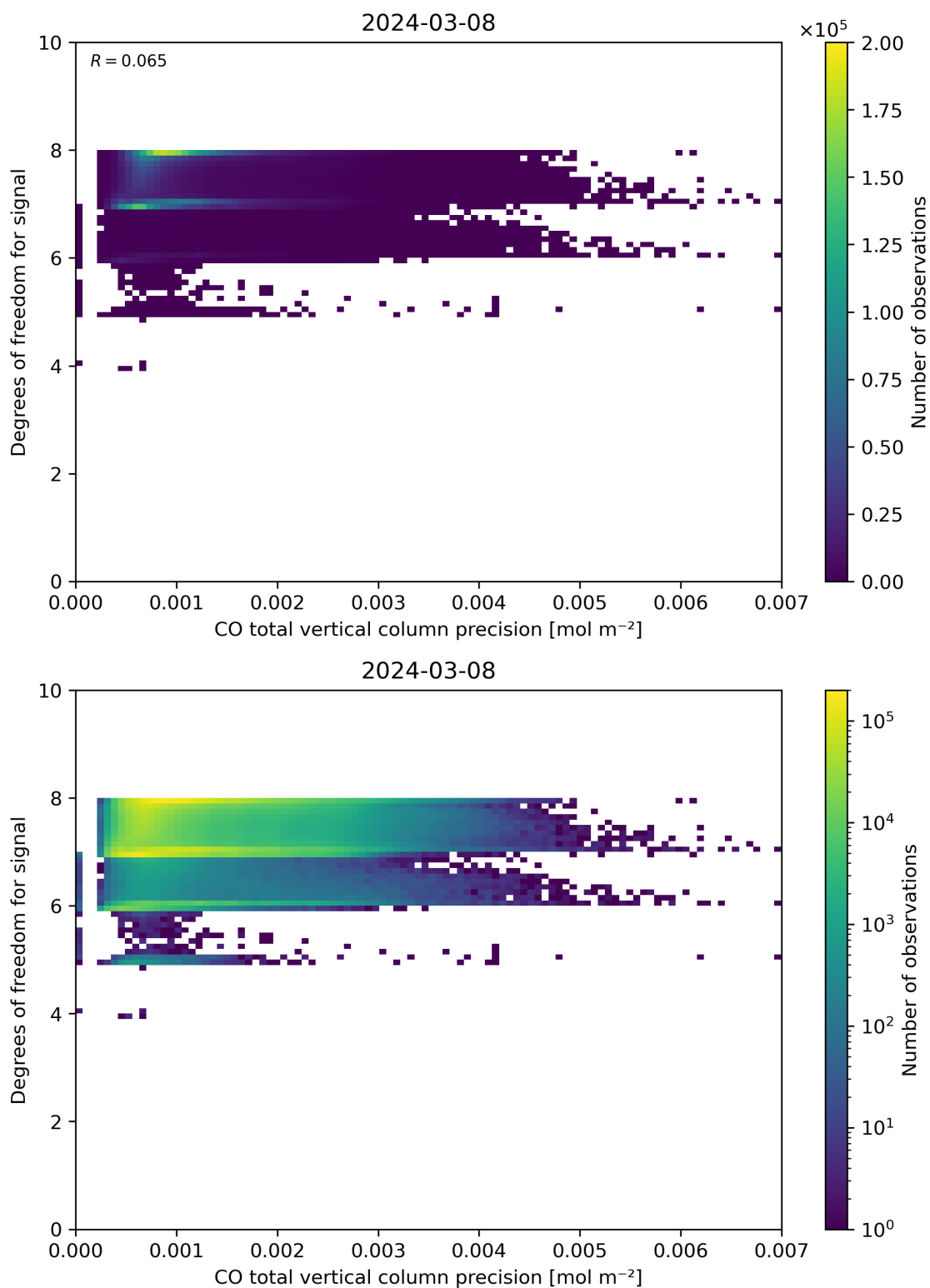
Figure 45: Scatter density plot of “CO total vertical column precision” against “Degrees of freedom for signal” for 2024-03-07 to 2024-03-09.
