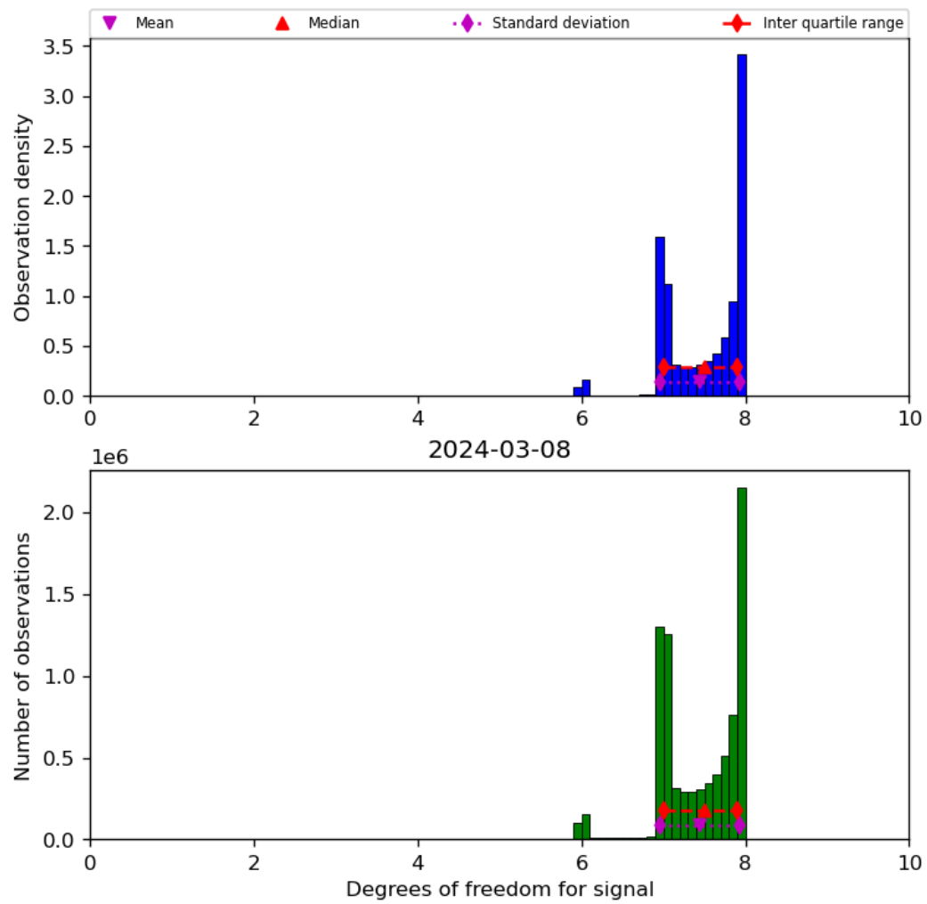
Figure 23: Histogram of “Degrees of freedom for signal” for 2024-03-07 to 2024-03-09
