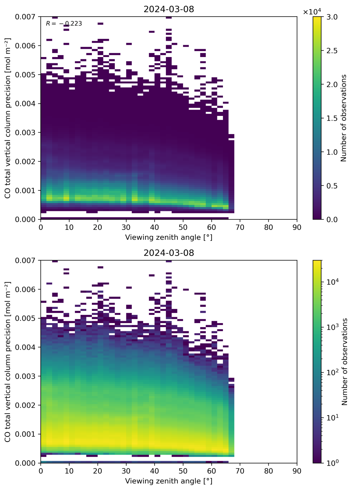
Figure 71: Scatter density plot of “Viewing zenith angle” against “CO total vertical column precision” for 2024-03-07 to 2024-03-09.
