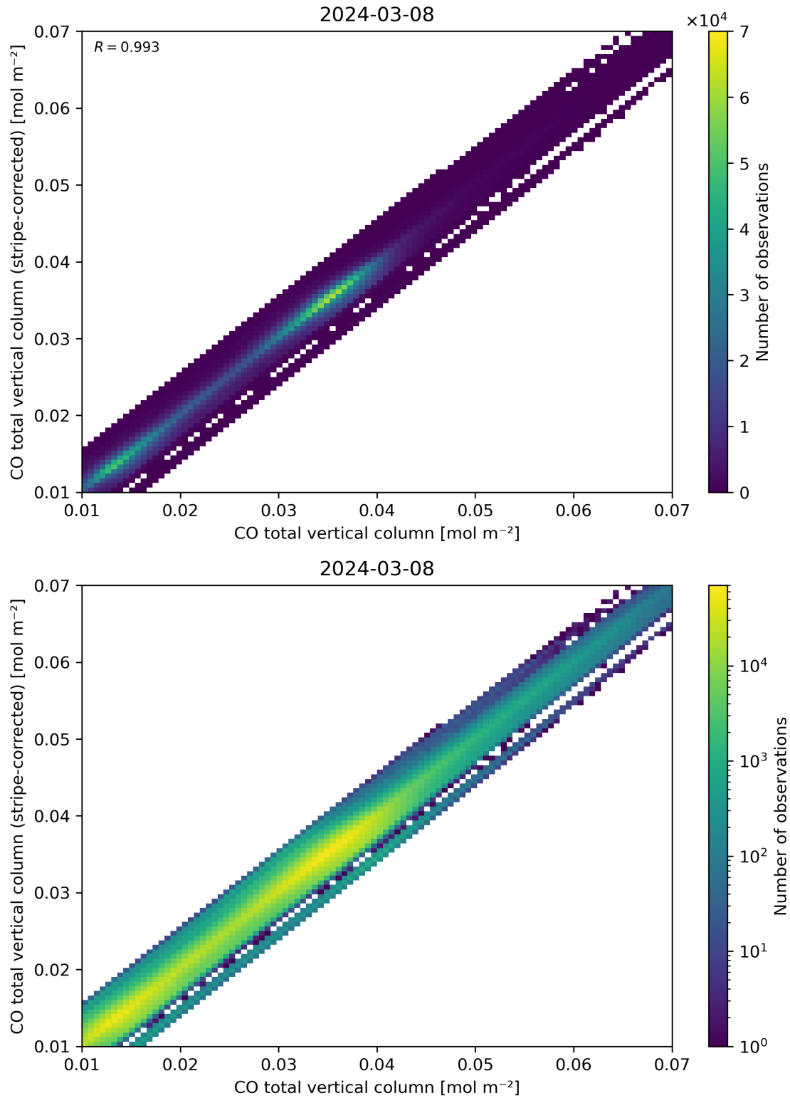
Figure 33: Scatter density plot of “CO total vertical column” against “CO total vertical column (stripe-corrected)” for 2024-03-07 to 2024-03-09.
