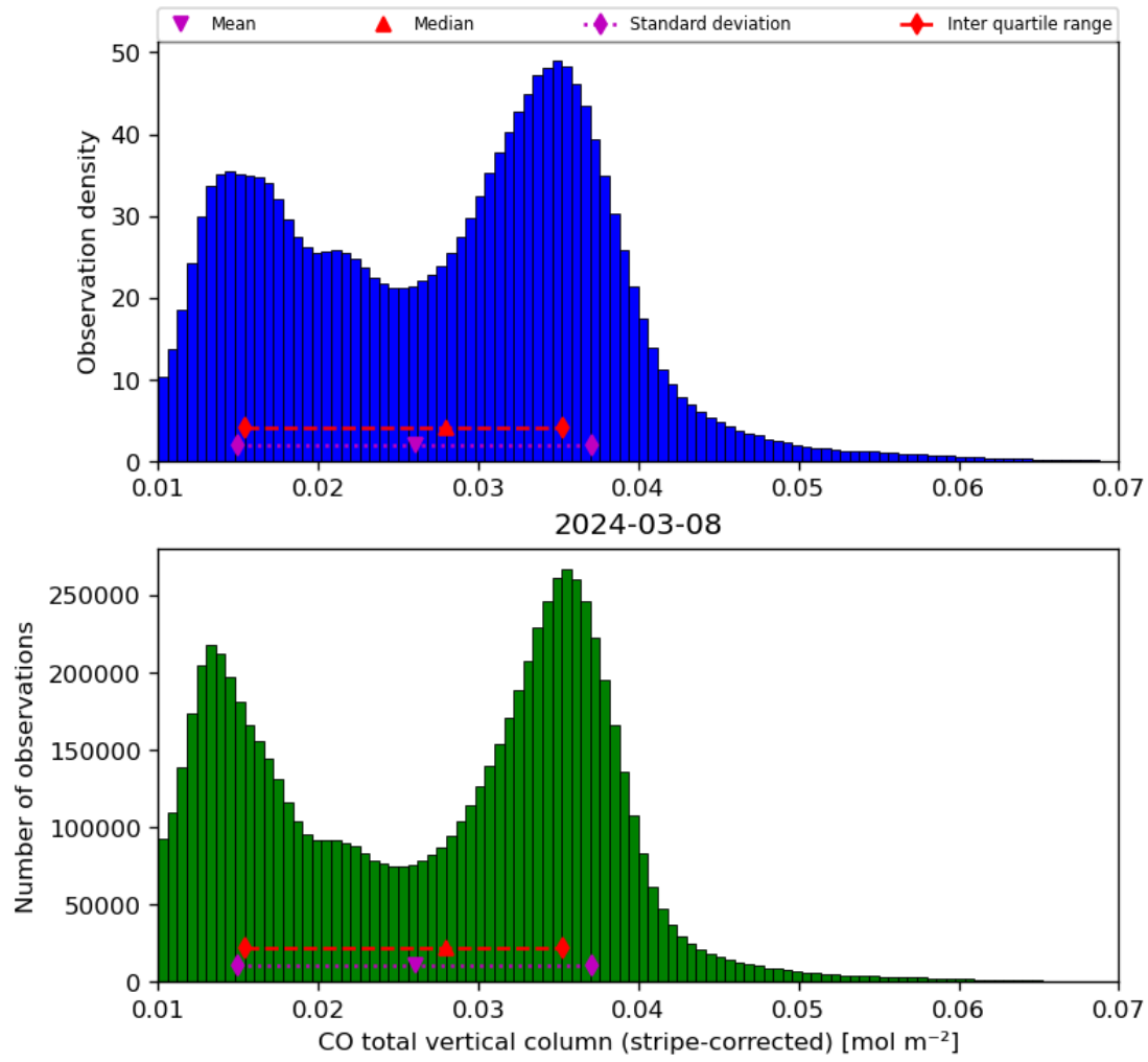
Figure 19: Histogram of “CO total vertical column (stripe-corrected)” for 2024-03-07 to 2024-03-09
