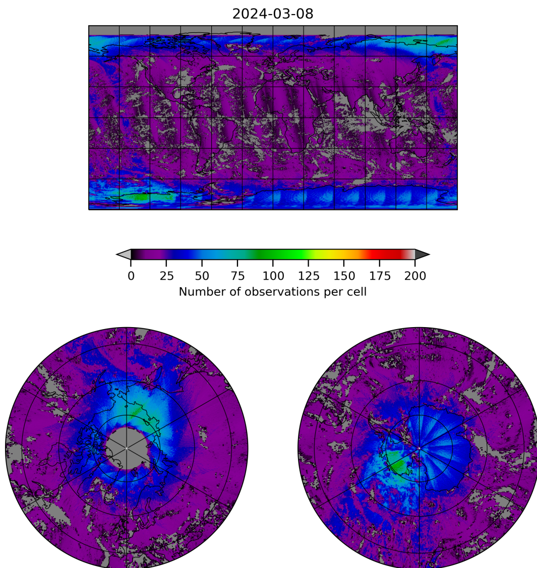
Figure 8: Map of the number of observations for 2024-03-07 to 2024-03-09
