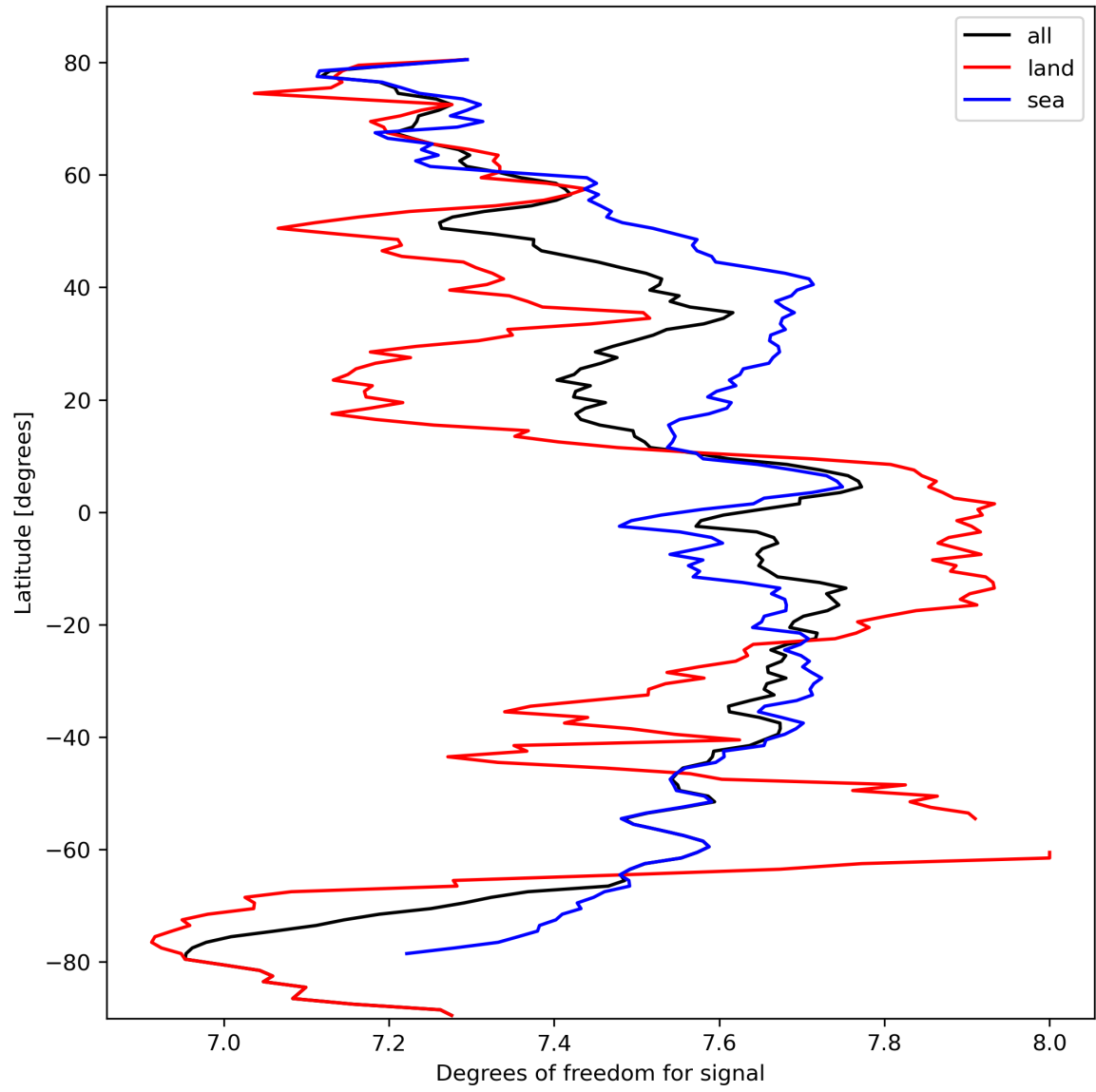
Figure 15: Zonal average of “Degrees of freedom for signal” for 2024-03-07 to 2024-03-09.
