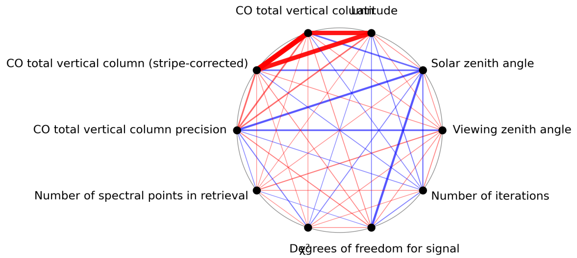
Figure 1: Map of correlation graph for 2024-03-07 to 2024-03-09.
