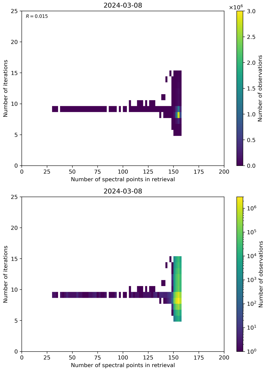
Figure 60: Scatter density plot of “Number of spectral points in retrieval” against “Number of iterations” for 2024-03-07 to 2024-03-09.
