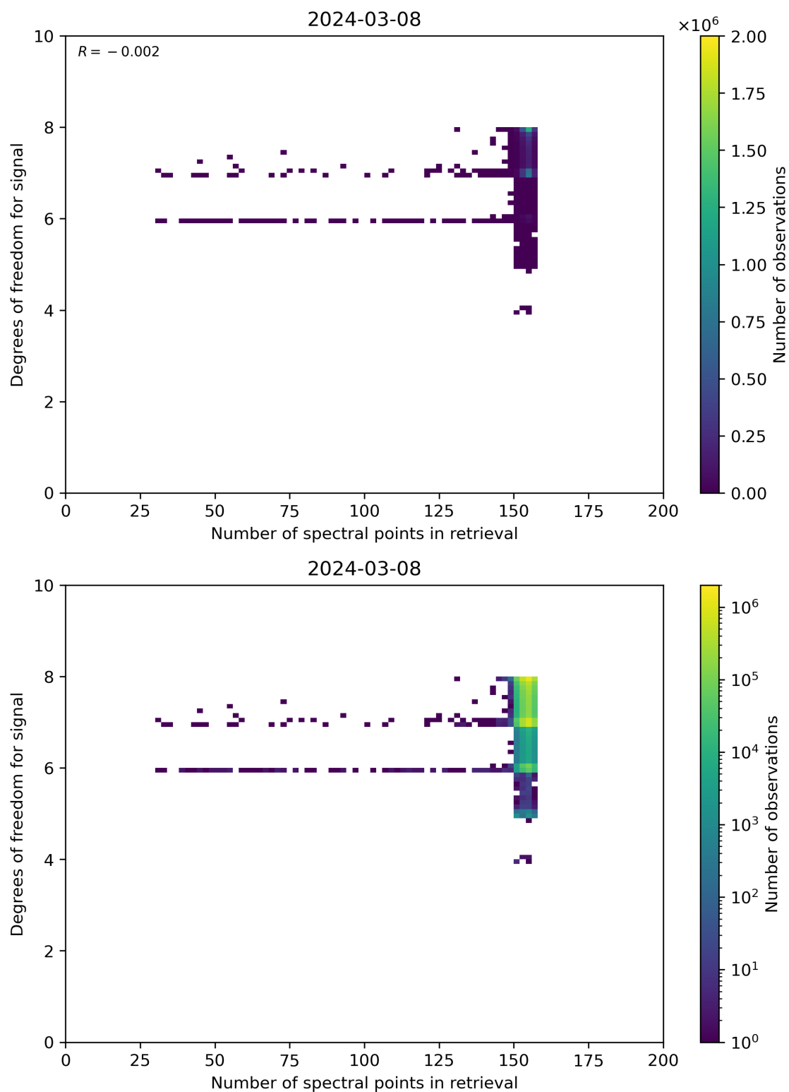
Figure 59: Scatter density plot of “Number of spectral points in retrieval” against “Degrees of freedom for signal” for 2024-03-07 to 2024-03-09.
