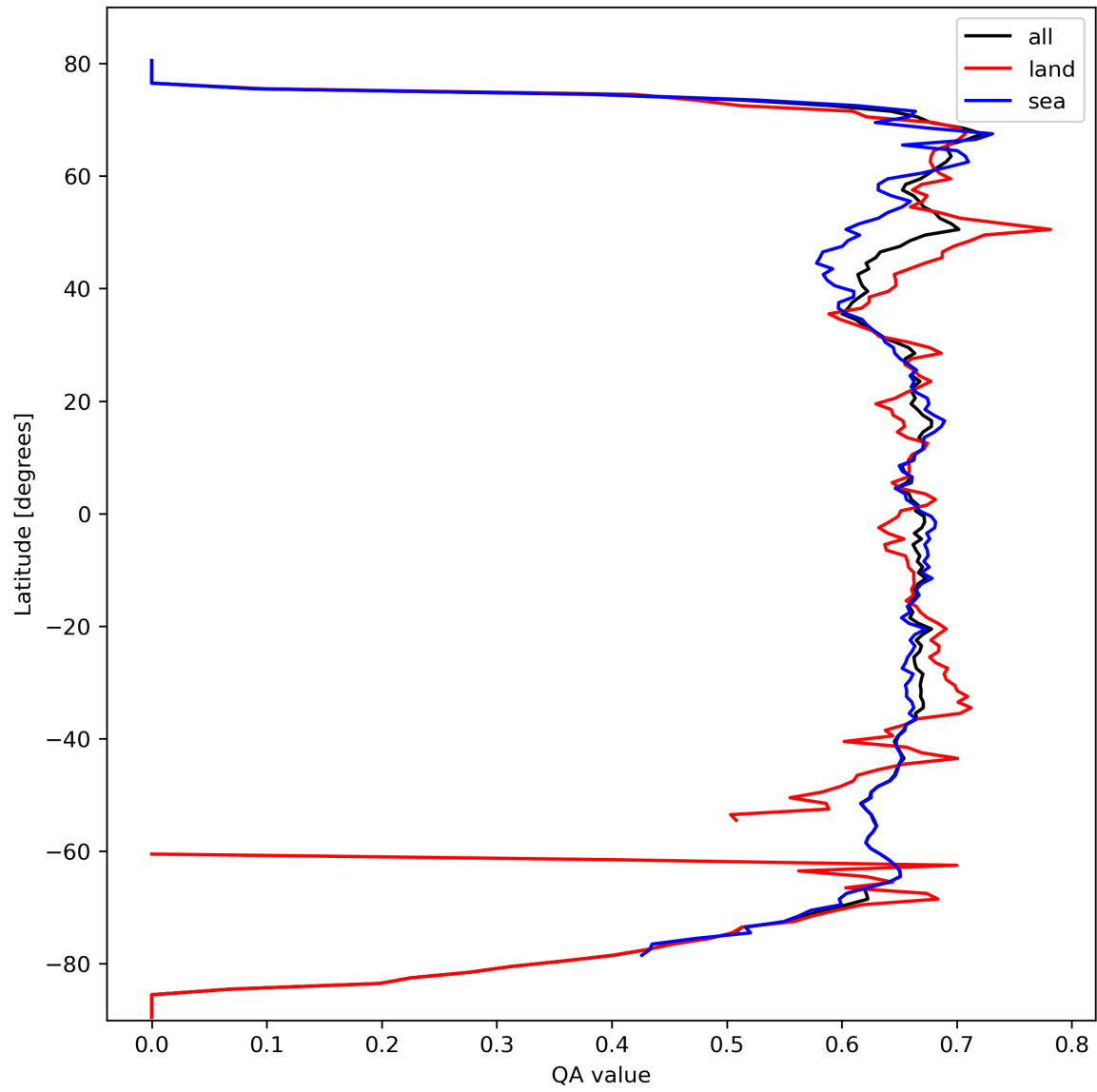
Figure 9: Zonal average of “QA value” for 2024-03-07 to 2024-03-09.
