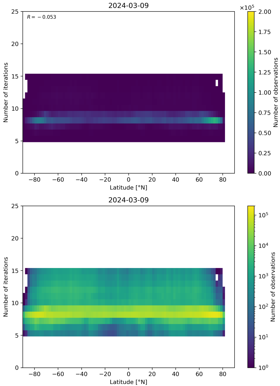
Figure 56: Scatter density plot of “Latitude” against “Number of iterations” for 2024-03-09 to 2024-03-10.
