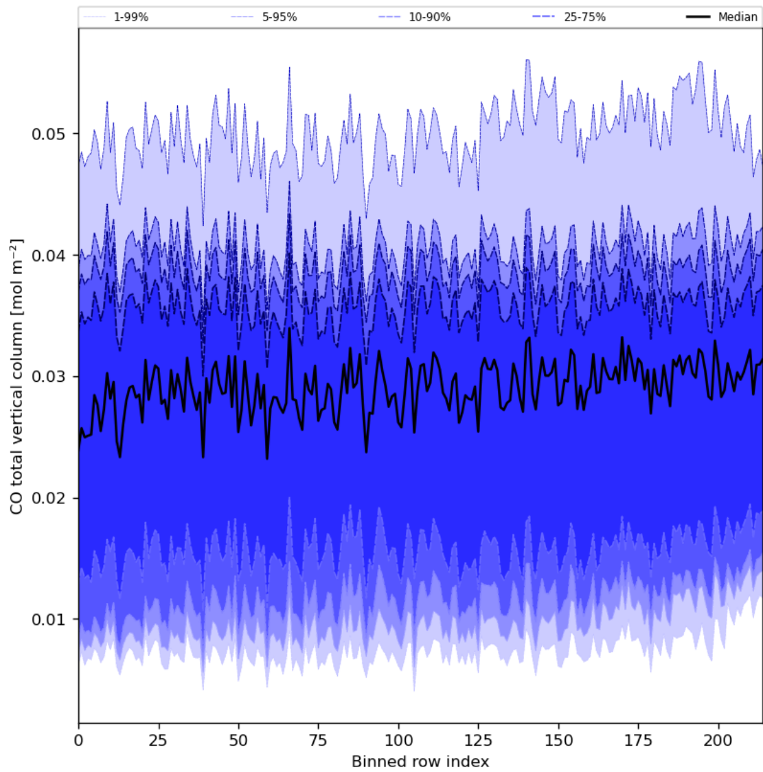
Figure 26: Along track statistics of “CO total vertical column” for 2024-03-09 to 2024-03-10
