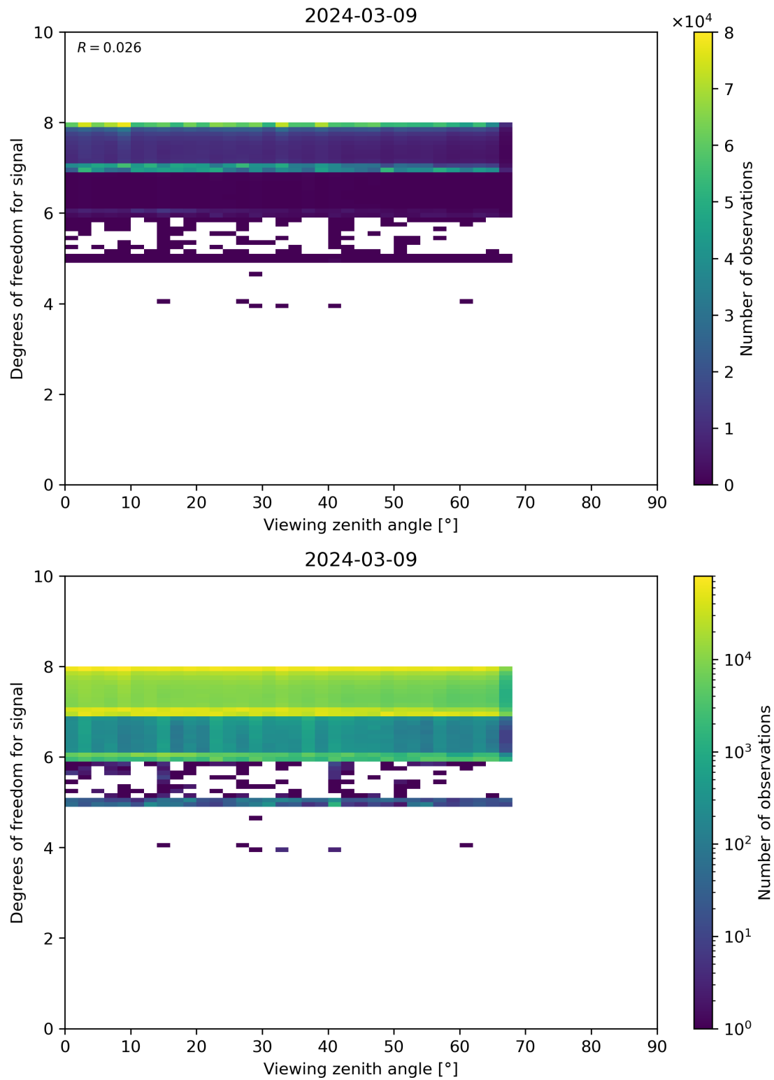
Figure 73: Scatter density plot of “Viewing zenith angle” against “Degrees of freedom for signal” for 2024-03-09 to 2024-03-10.
