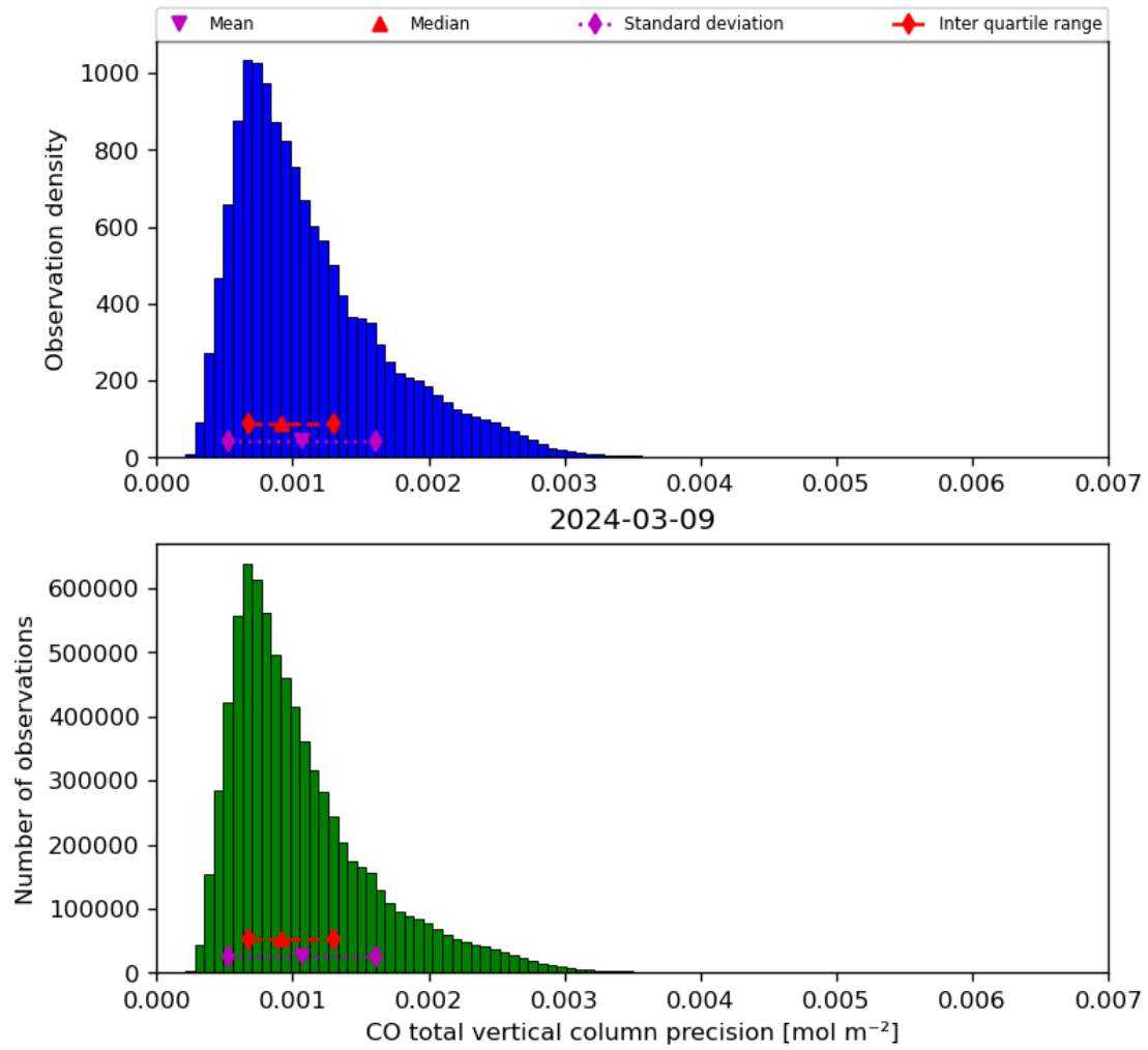
Figure 20: Histogram of “CO total vertical column precision” for 2024-03-09 to 2024-03-10
