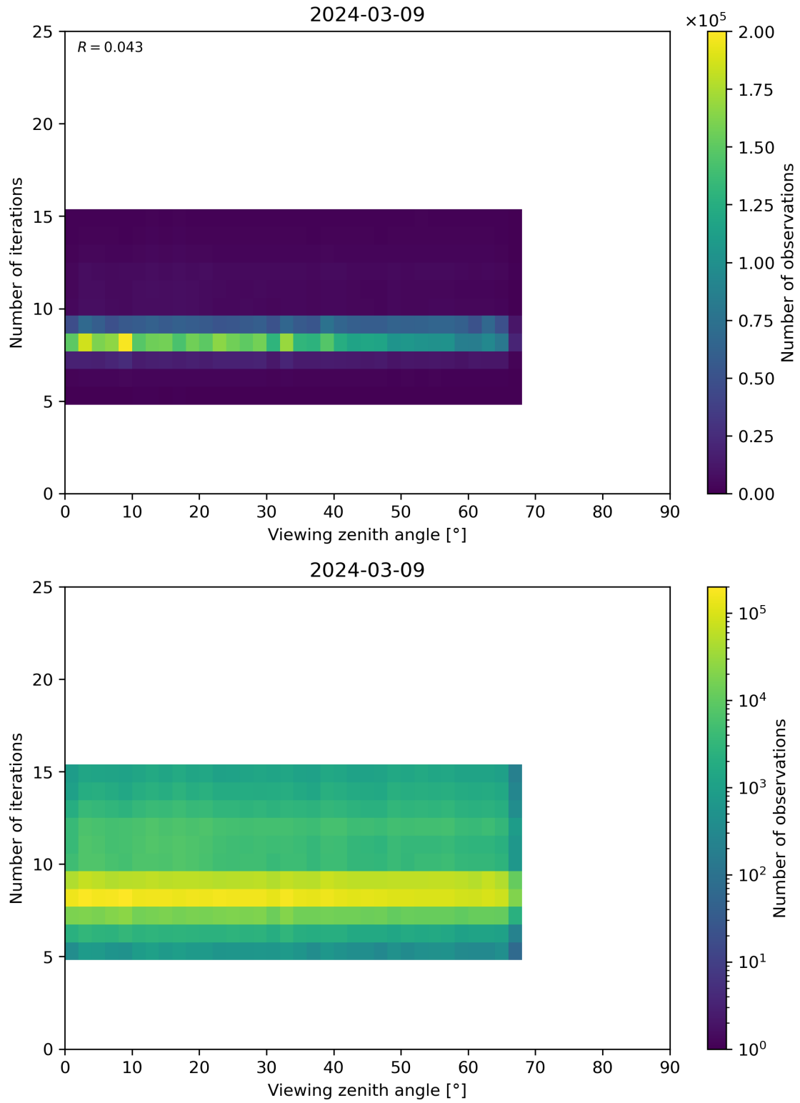
Figure 75: Scatter density plot of “Viewing zenith angle” against “Number of iterations” for 2024-03-09 to 2024-03-10.
