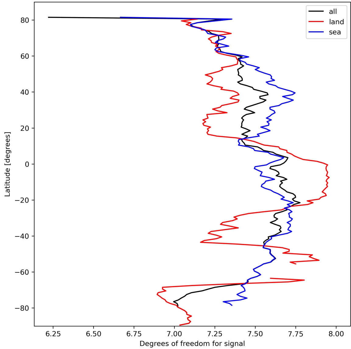
Figure 15: Zonal average of “Degrees of freedom for signal” for 2024-03-09 to 2024-03-10.
