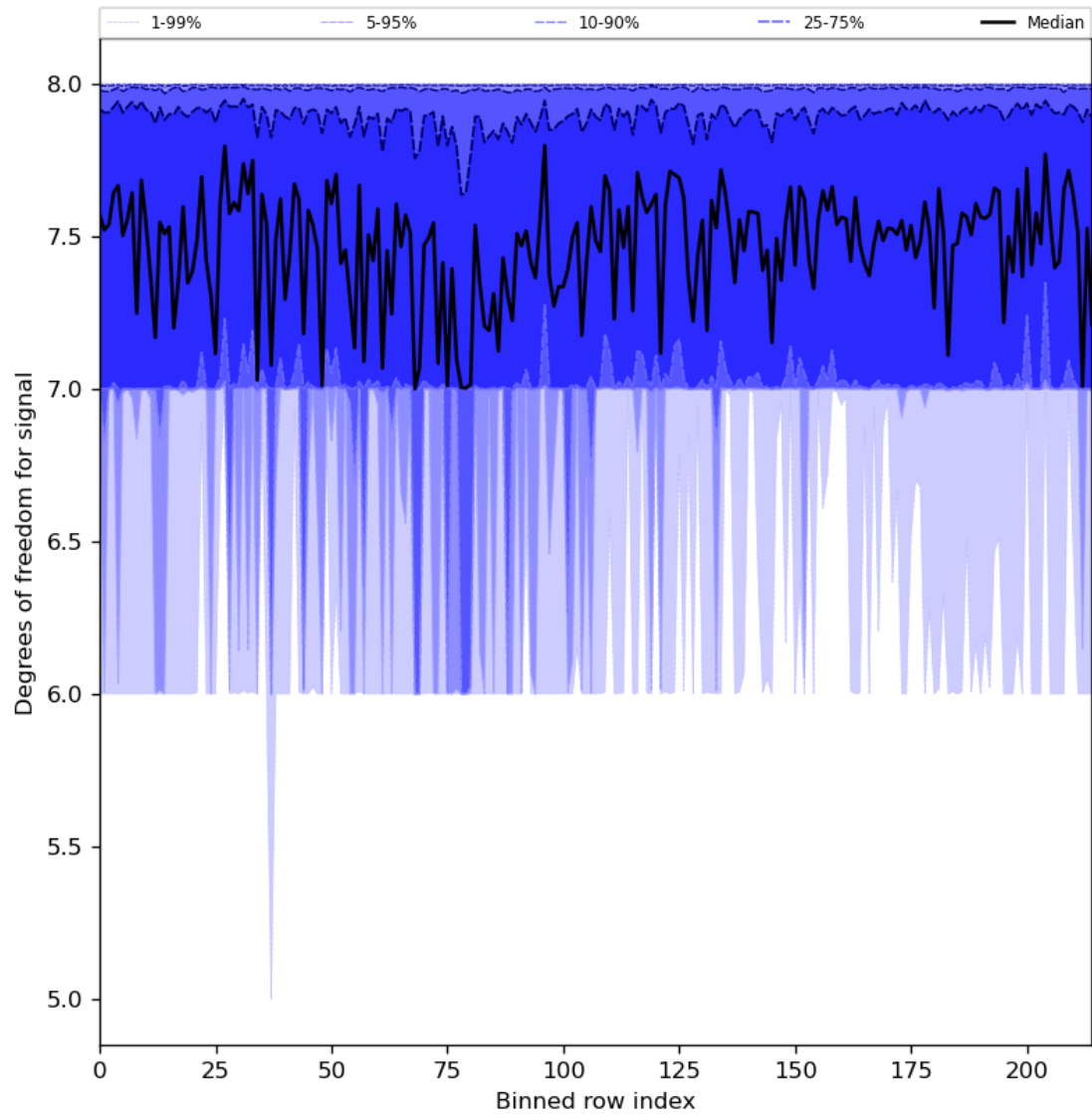
Figure 31: Along track statistics of “Degrees of freedom for signal” for 2024-03-09 to 2024-03-10
