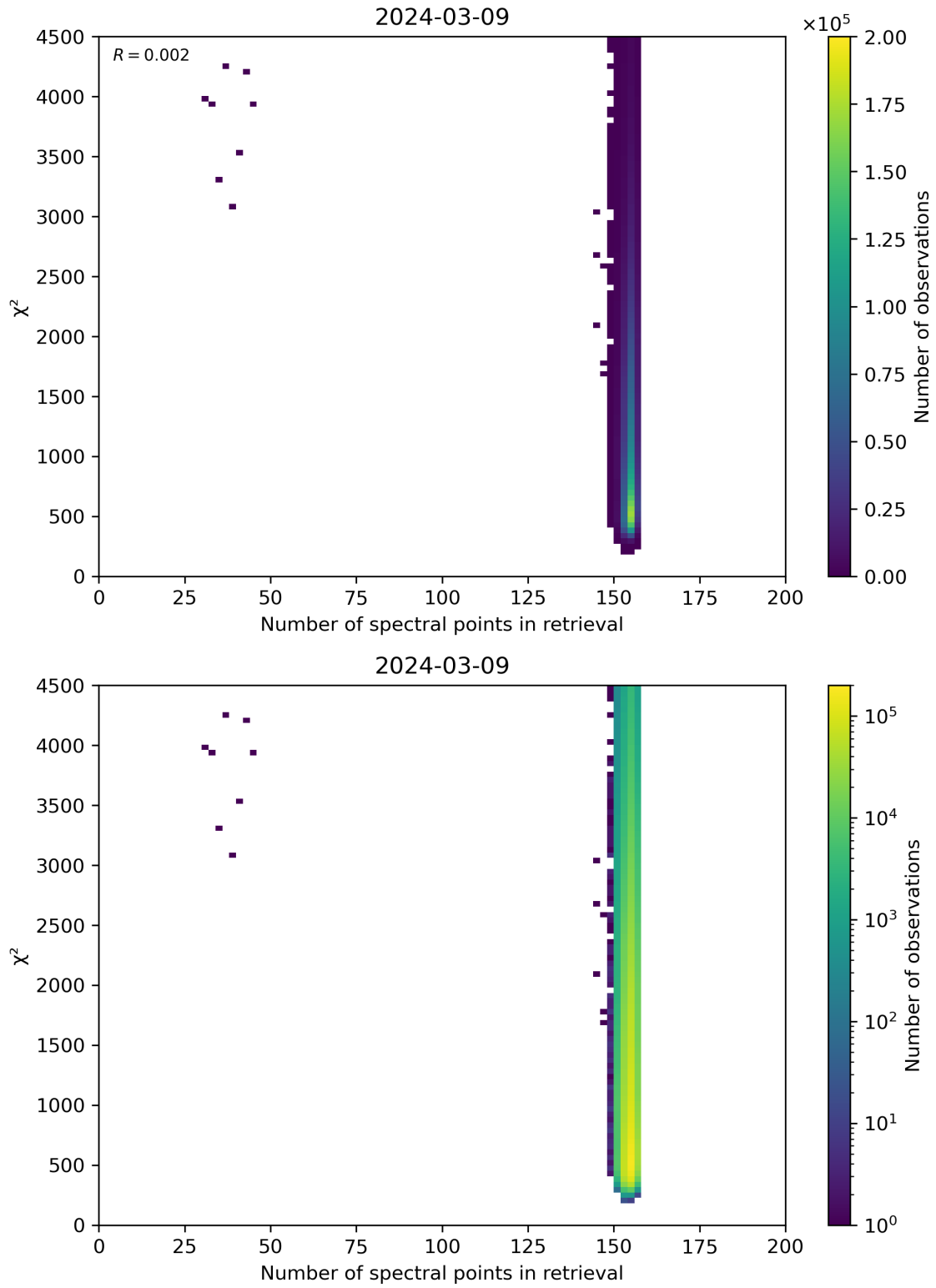
Figure 58: Scatter density plot of “Number of spectral points in retrieval” against “ \chi^2 ” for 2024-03-09 to 2024-03-10.
