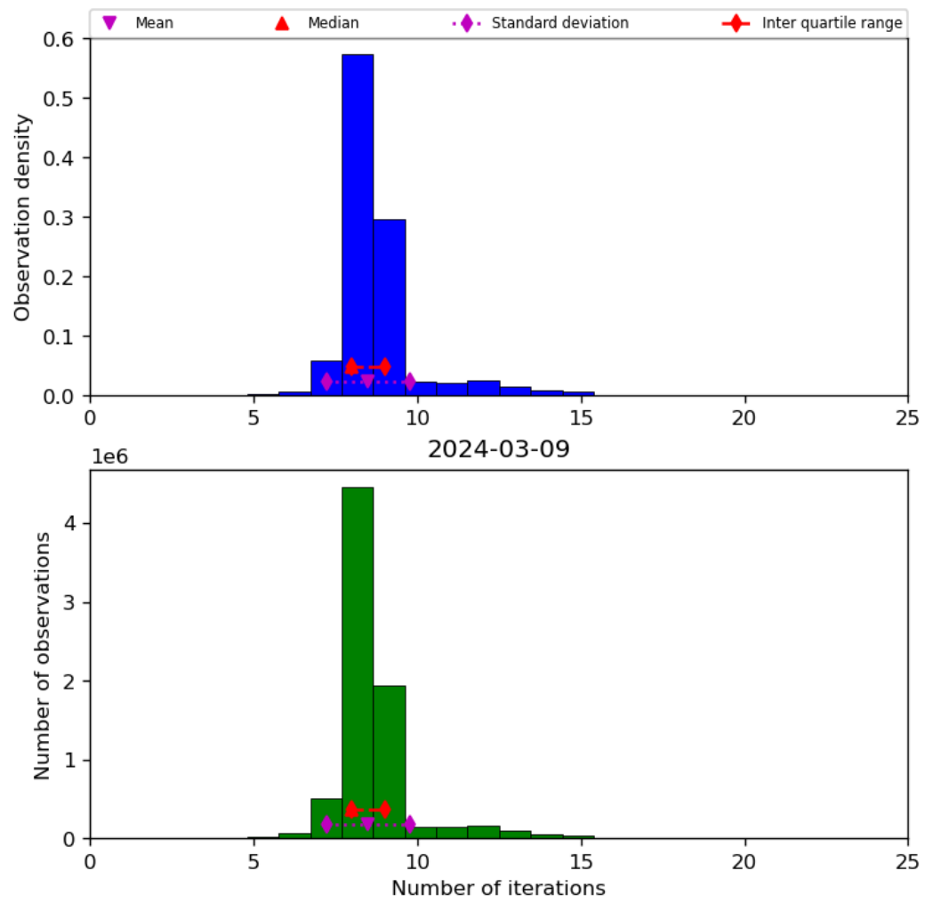
Figure 24: Histogram of “Number of iterations” for 2024-03-09 to 2024-03-10
