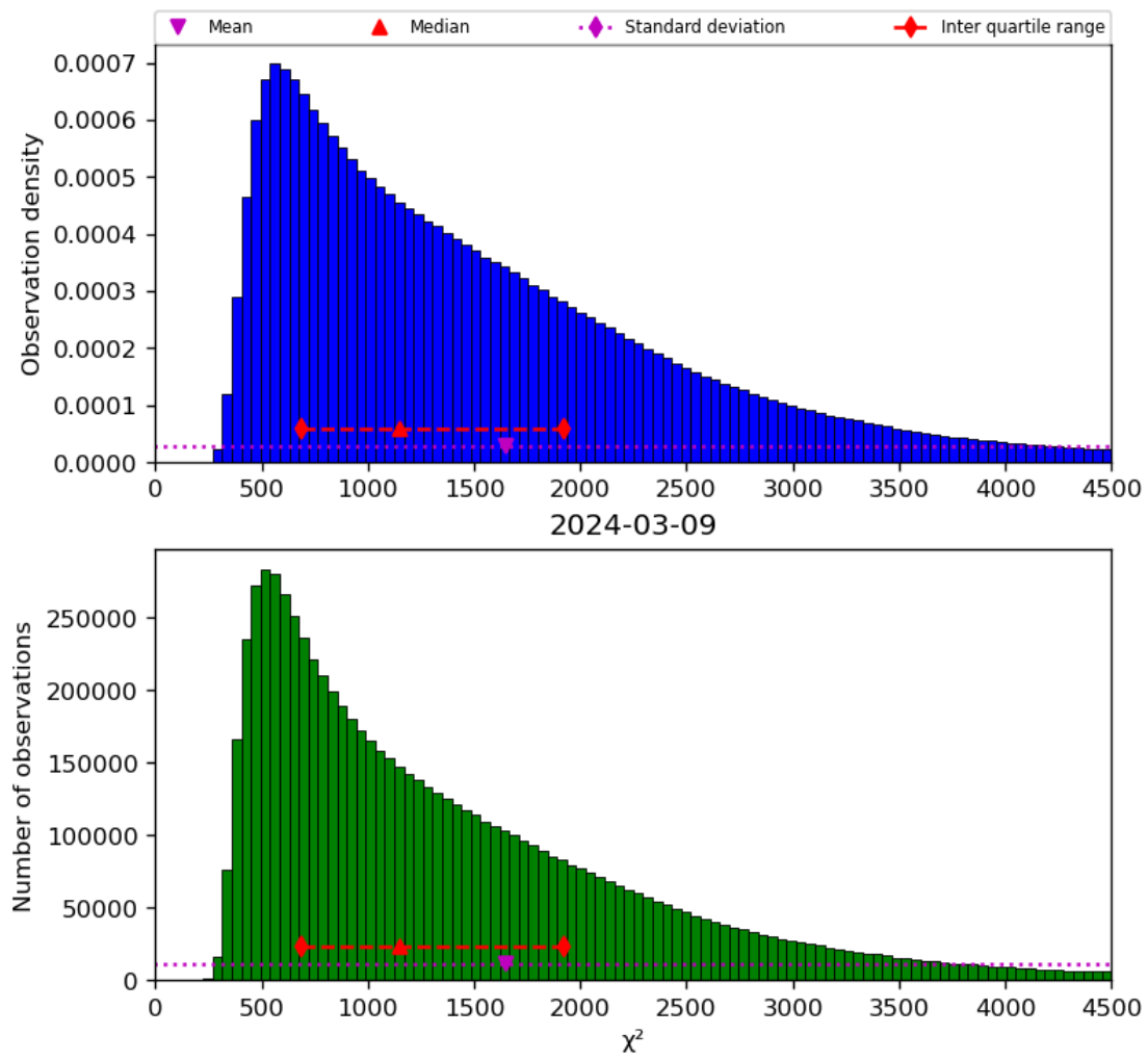
Figure 22: Histogram of “ \chi^2 ” for 2024-03-09 to 2024-03-10
