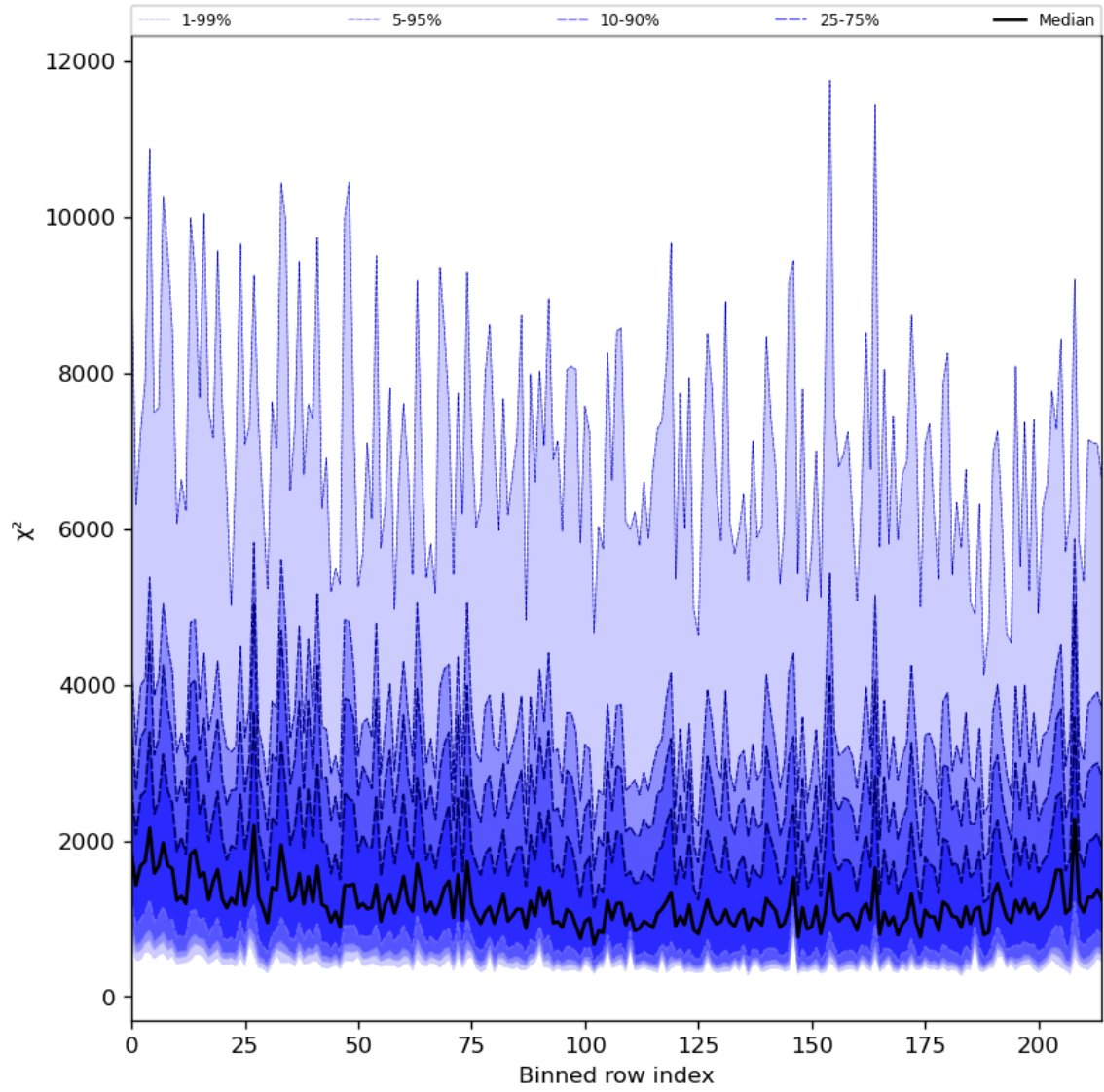
Figure 30: Along track statistics of “ \chi^2 ” for 2024-03-09 to 2024-03-10
