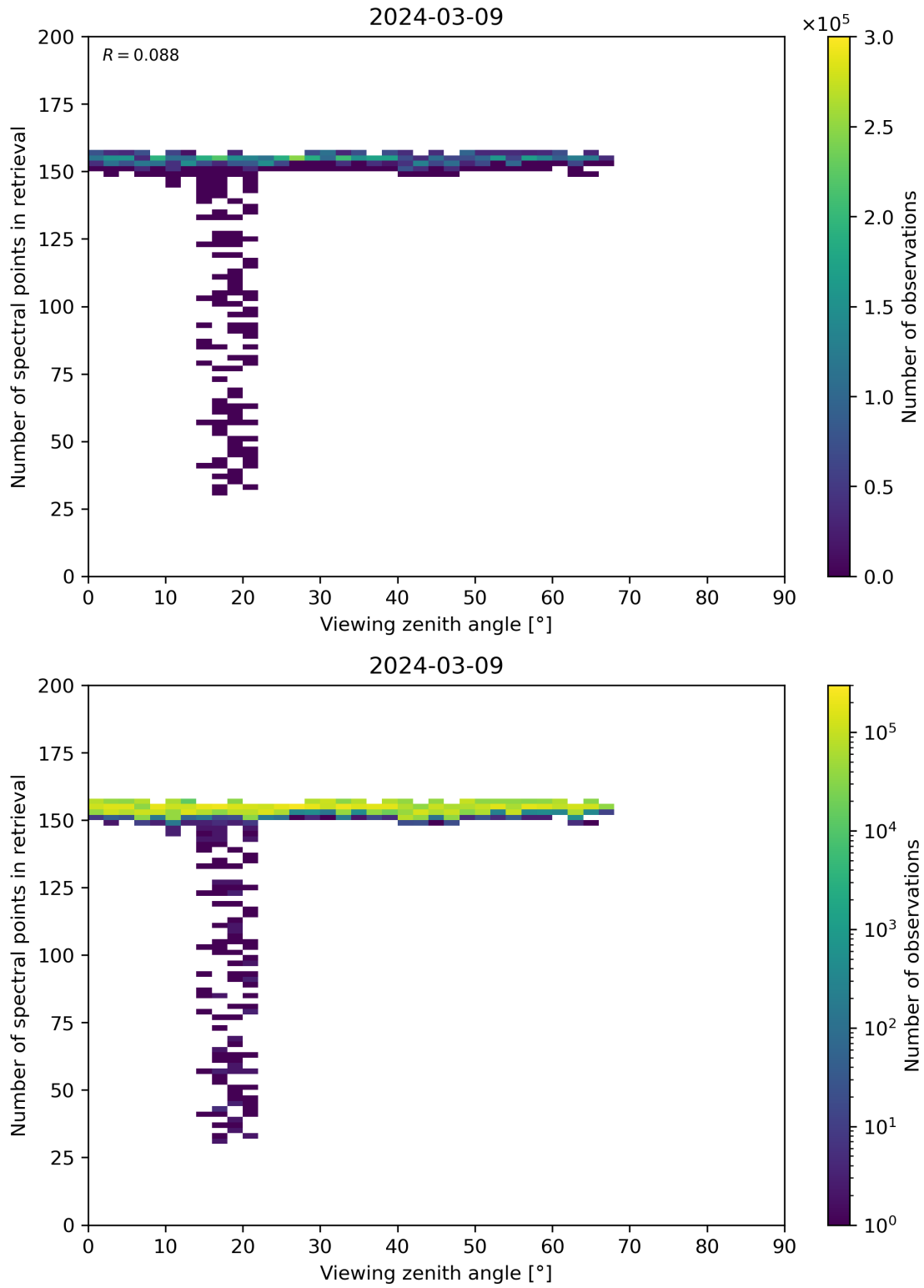
Figure 76: Scatter density plot of “Viewing zenith angle” against “Number of spectral points in retrieval” for 2024-03-09 to 2024-03-10.
