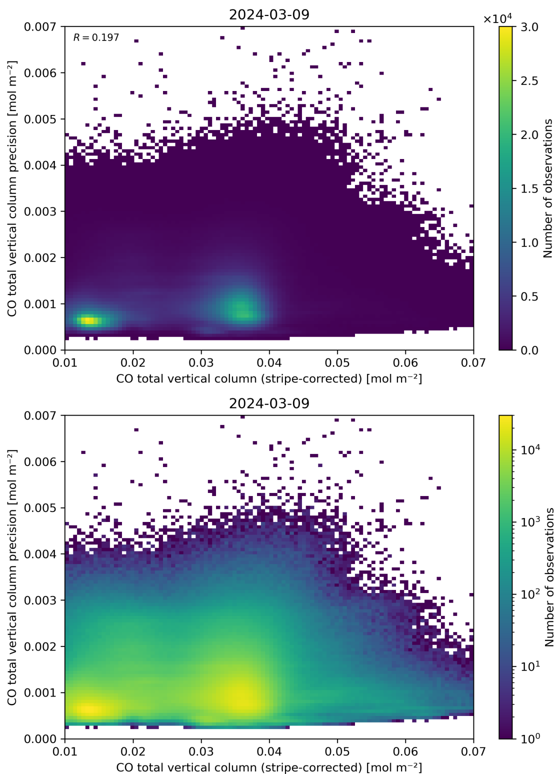
Figure 36: Scatter density plot of “CO total vertical column (stripe-corrected)” against “CO total vertical column precision” for 2024-03-09 to 2024-03-10.
