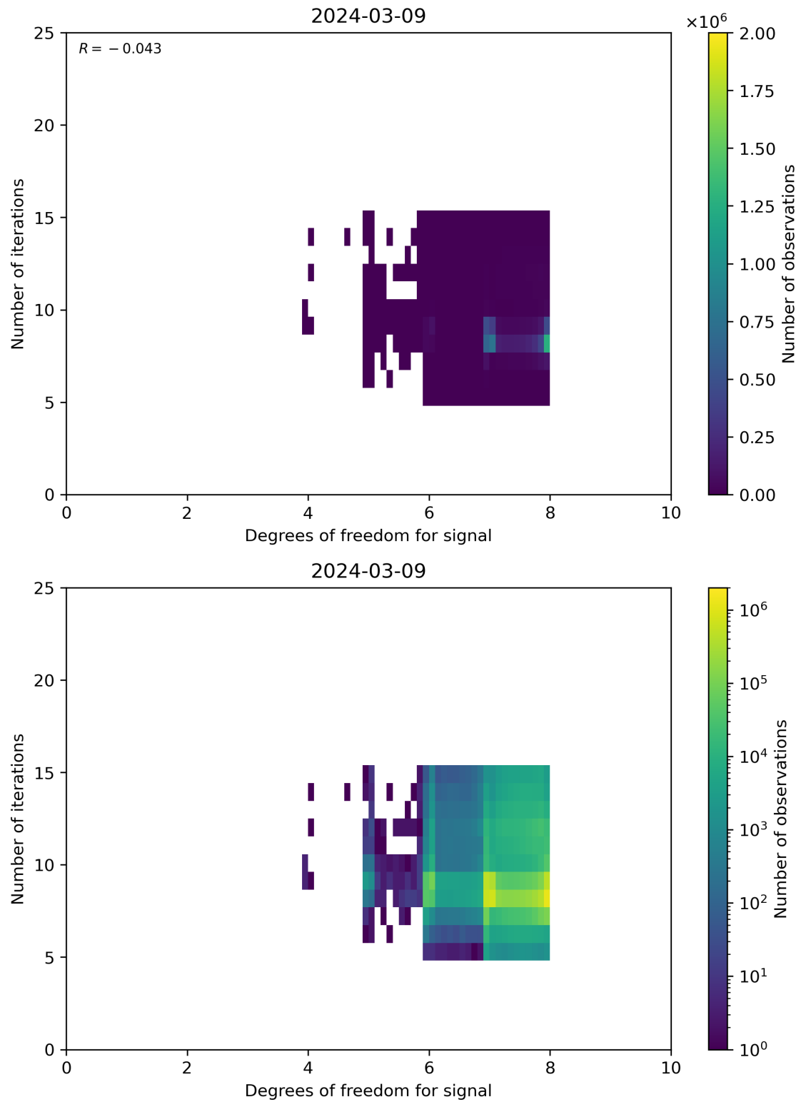
Figure 50: Scatter density plot of “Degrees of freedom for signal” against “Number of iterations” for 2024-03-09 to 2024-03-10.
