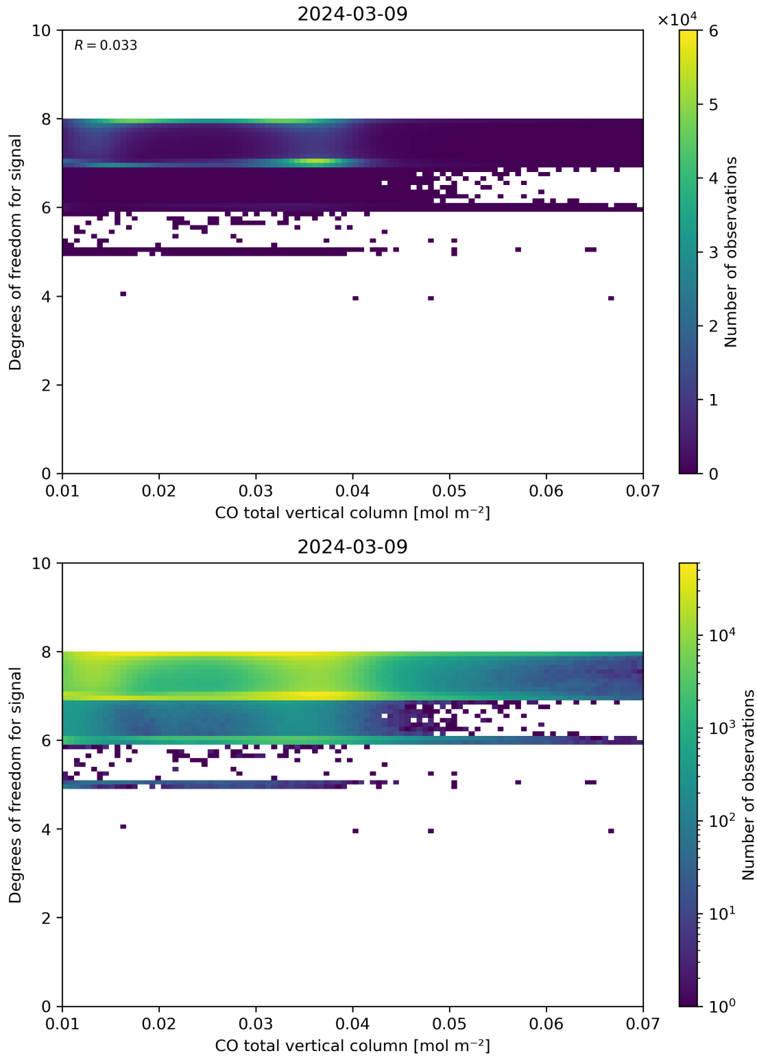
Figure 41: Scatter density plot of “CO total vertical column” against “Degrees of freedom for signal” for 2024-03-09 to 2024-03-10.
