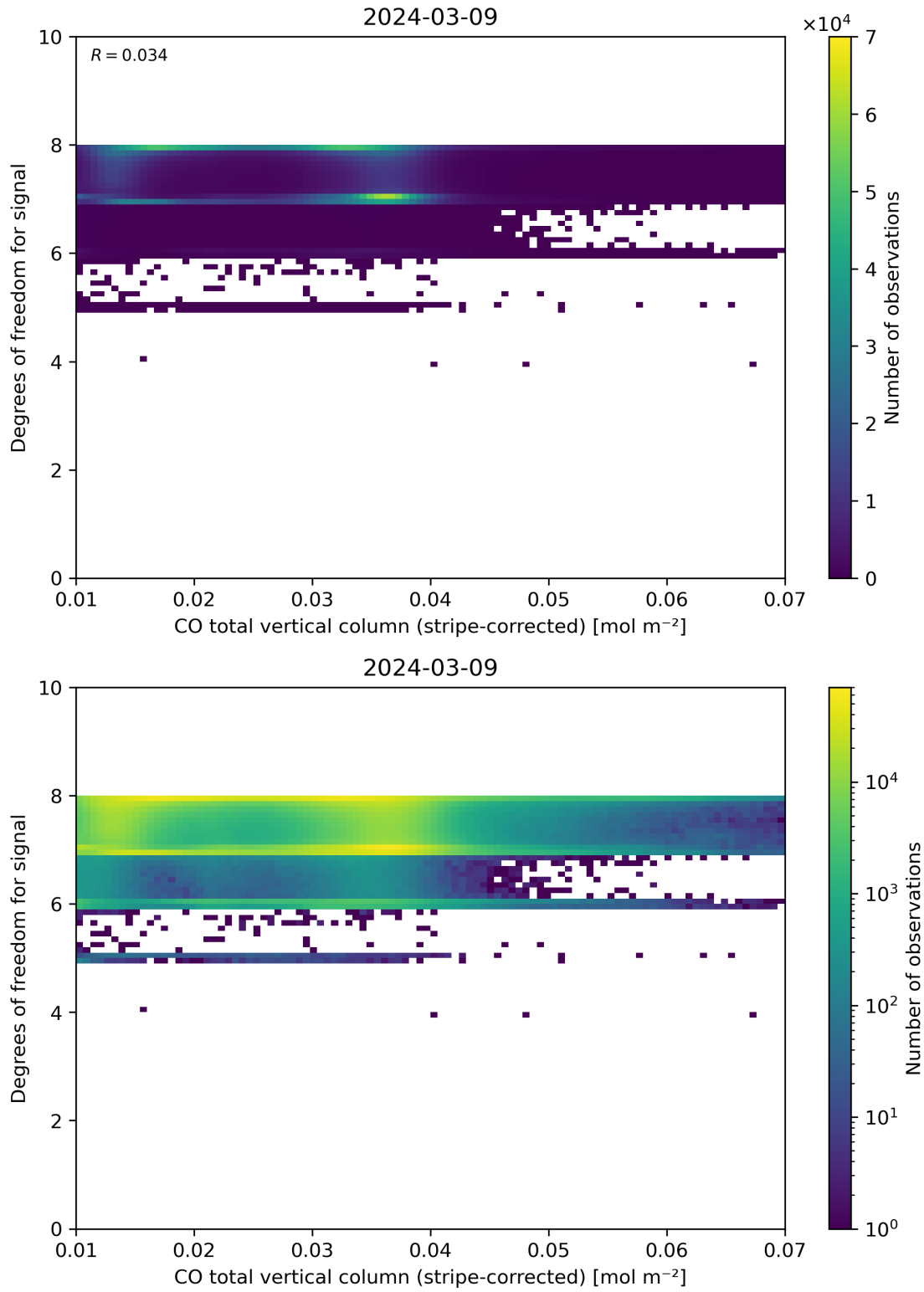
Figure 38: Scatter density plot of “CO total vertical column (stripe-corrected)” against “Degrees of freedom for signal” for 2024-03-09 to 2024-03-10.
