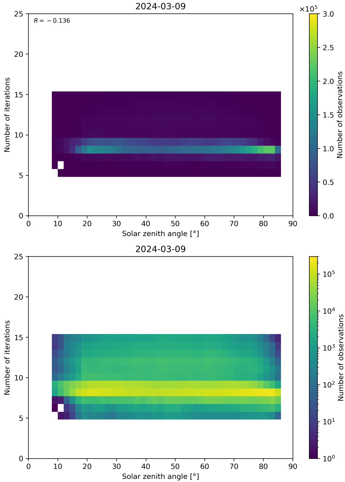
Figure 67: Scatter density plot of “Solar zenith angle” against “Number of iterations” for 2024-03-09 to 2024-03-10.
