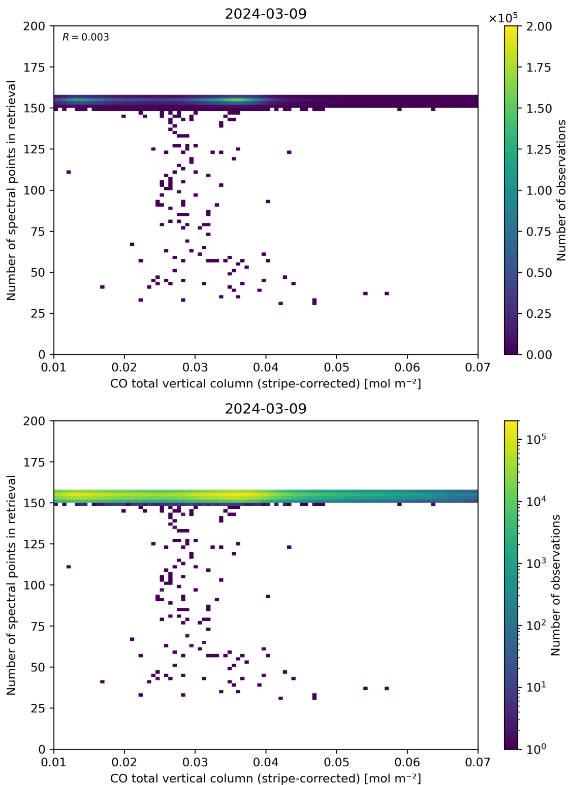
Figure 40: Scatter density plot of “CO total vertical column (stripe-corrected)” against “Number of spectral points in retrieval” for 2024-03-09 to 2024-03-10.
