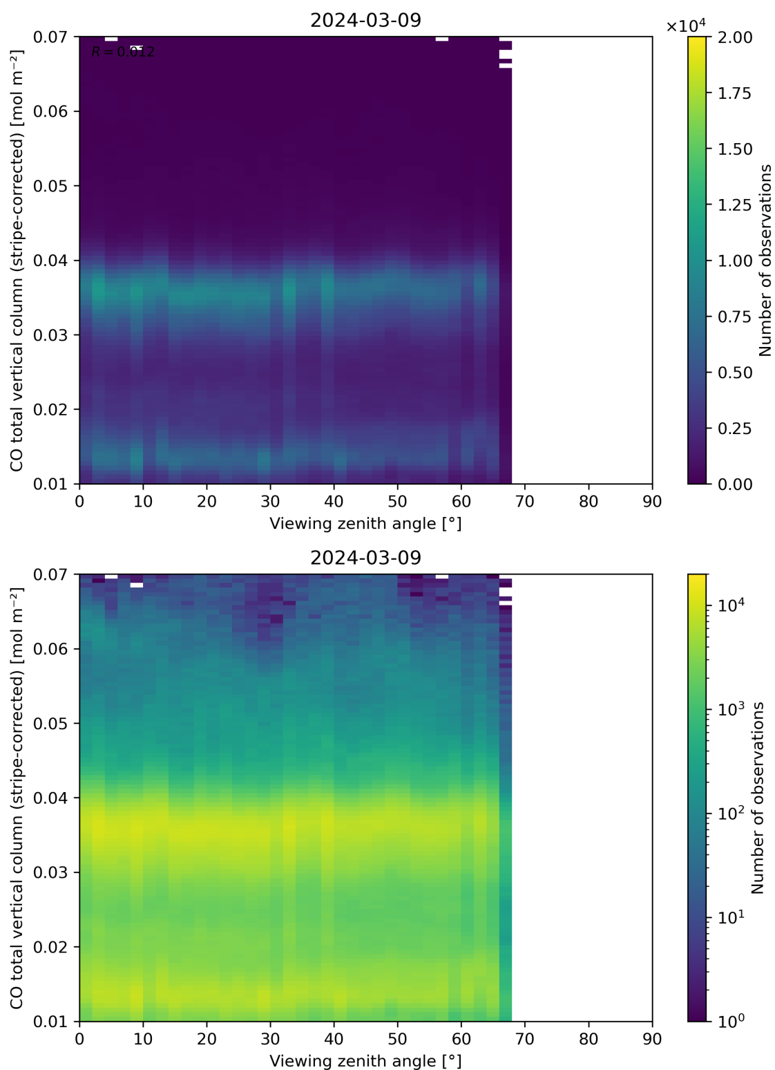
Figure 70: Scatter density plot of “Viewing zenith angle” against “CO total vertical column (stripe-corrected)” for 2024-03-09 to 2024-03-10.
