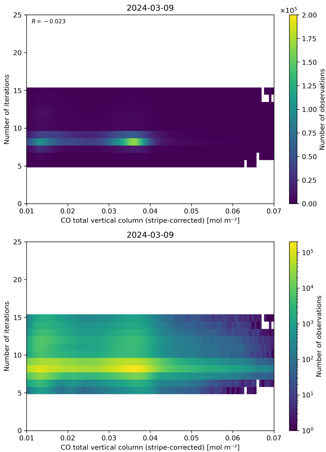
Figure 39: Scatter density plot of “CO total vertical column (stripe-corrected)” against “Number of iterations” for 2024-03-09 to 2024-03-10.
