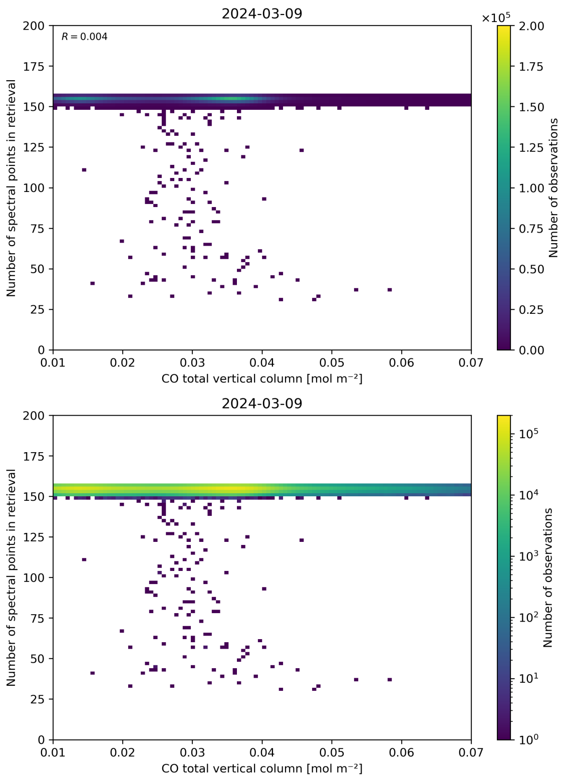
Figure 43: Scatter density plot of “CO total vertical column” against “Number of spectral points in retrieval” for 2024-03-09 to 2024-03-10.
