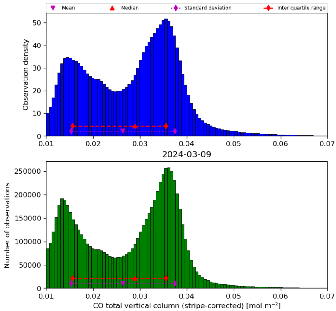
Figure 19: Histogram of “CO total vertical column (stripe-corrected)” for 2024-03-09 to 2024-03-10
