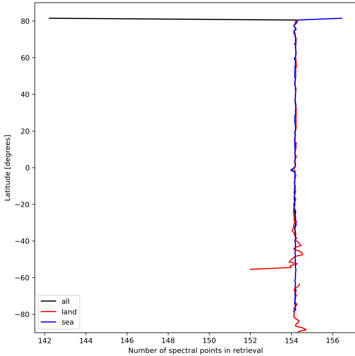
Figure 13: Zonal average of “Number of spectral points in retrieval” for 2024-03-09 to 2024-03-10.
