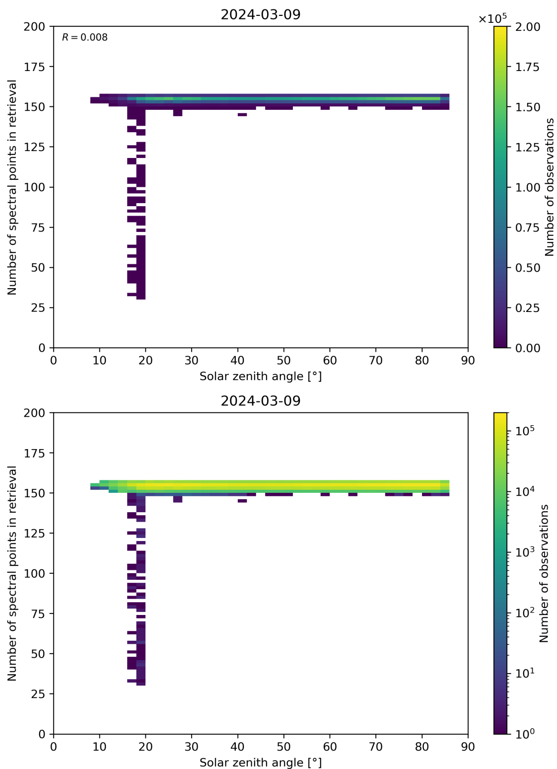
Figure 68: Scatter density plot of “Solar zenith angle” against “Number of spectral points in retrieval” for 2024-03-09 to 2024-03-10.
