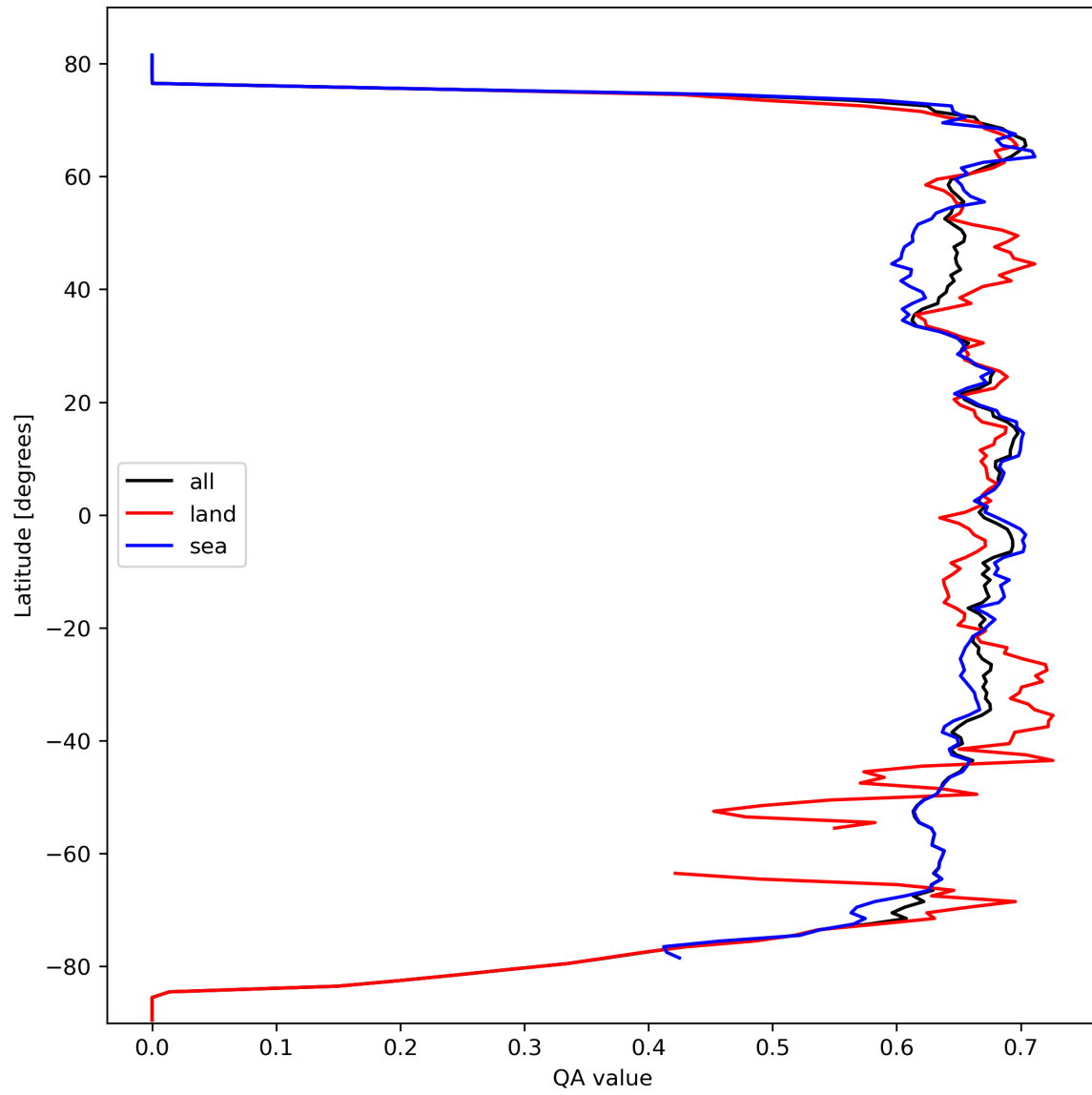
Figure 9: Zonal average of “QA value” for 2024-03-09 to 2024-03-10.
