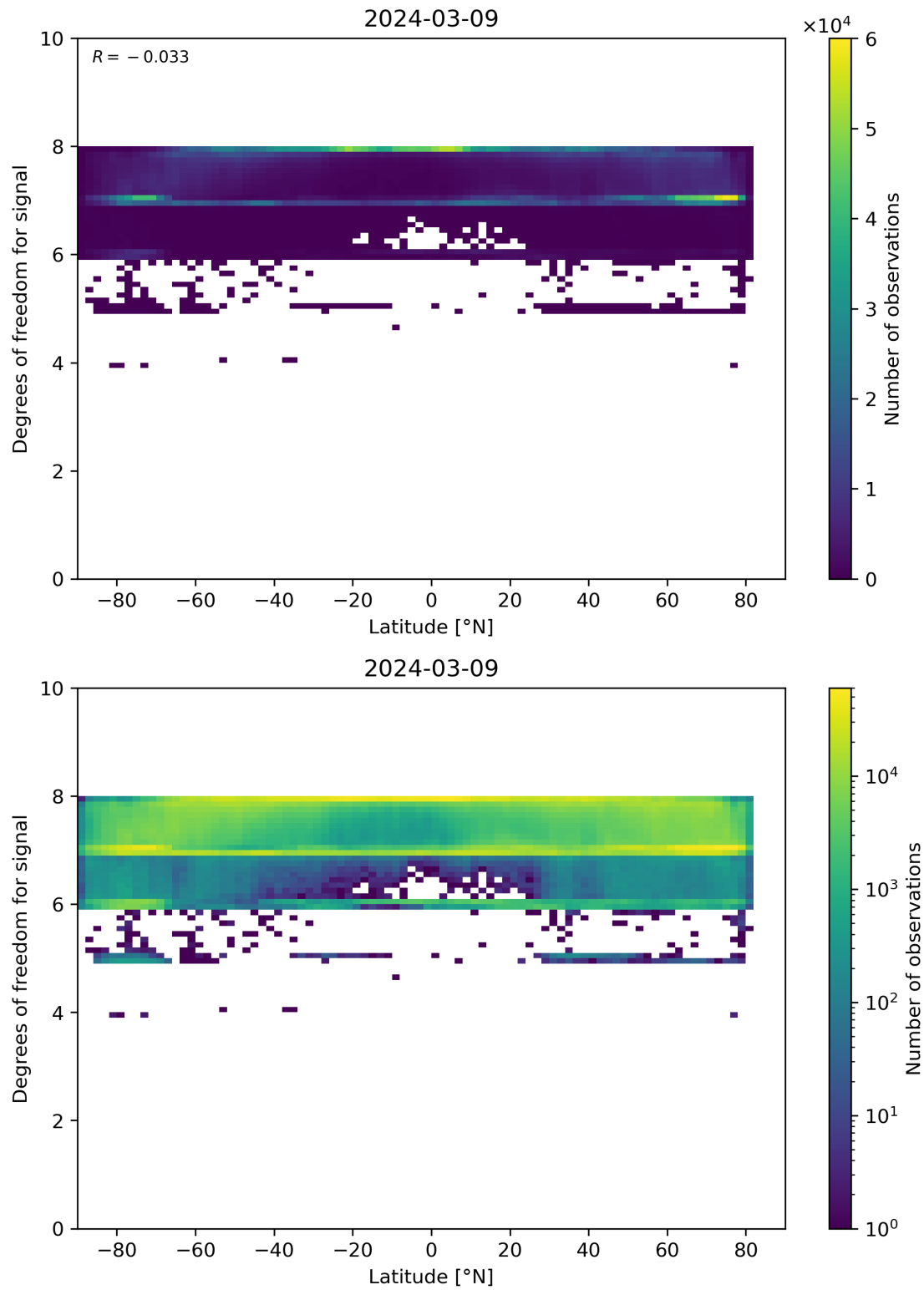
Figure 55: Scatter density plot of “Latitude” against “Degrees of freedom for signal” for 2024-03-09 to 2024-03-10.
