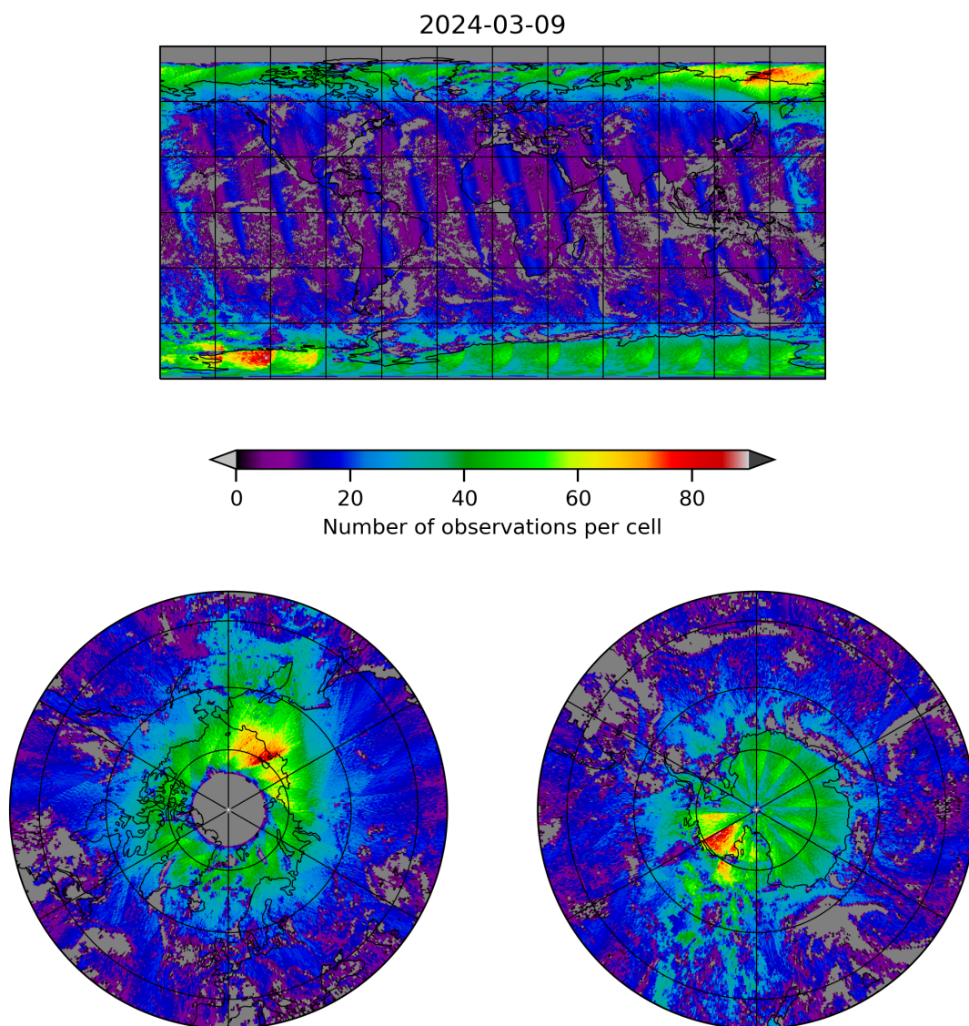
Figure 8: Map of the number of observations for 2024-03-09 to 2024-03-10
