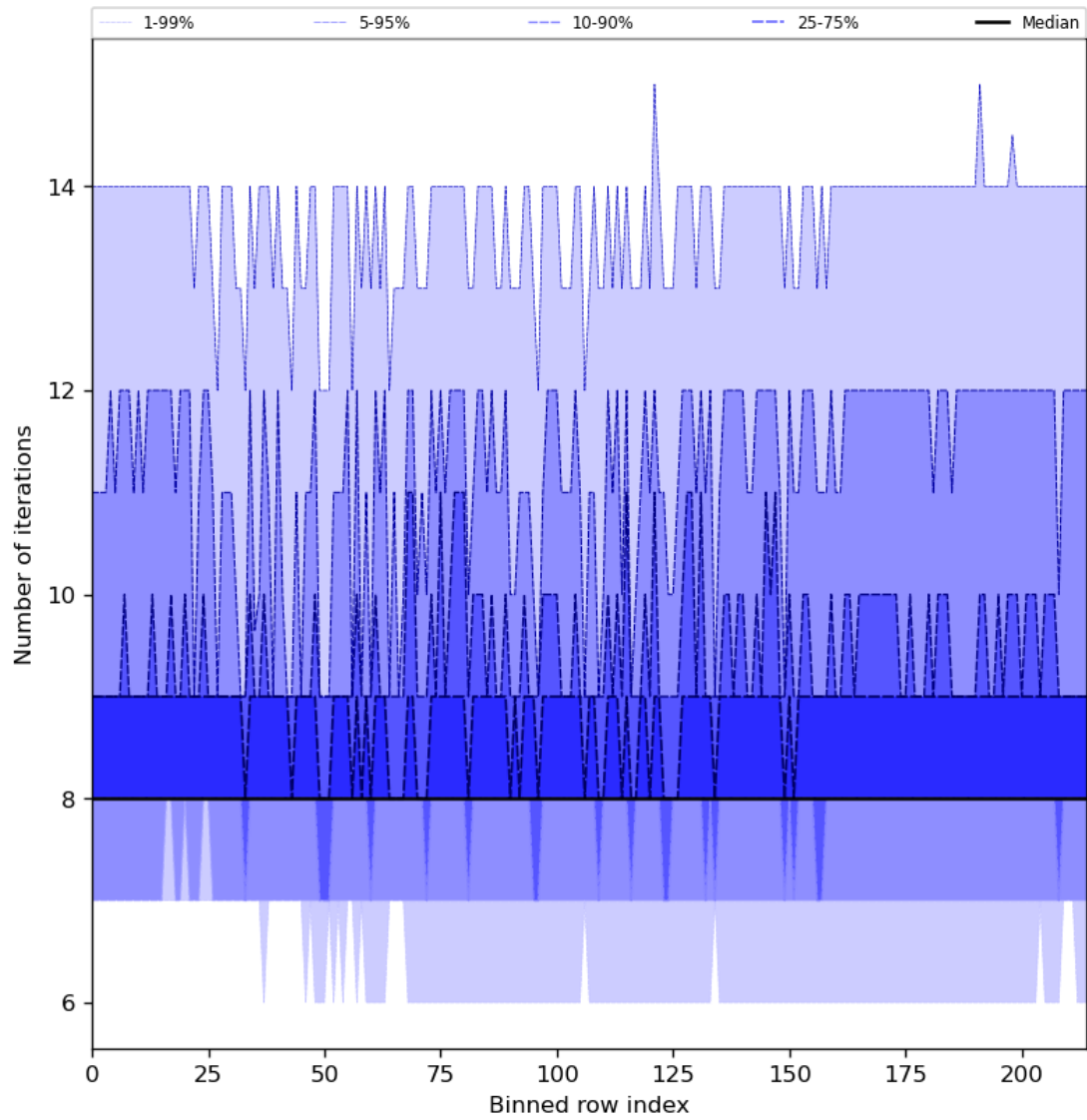
Figure 32: Along track statistics of “Number of iterations” for 2024-03-09 to 2024-03-10
