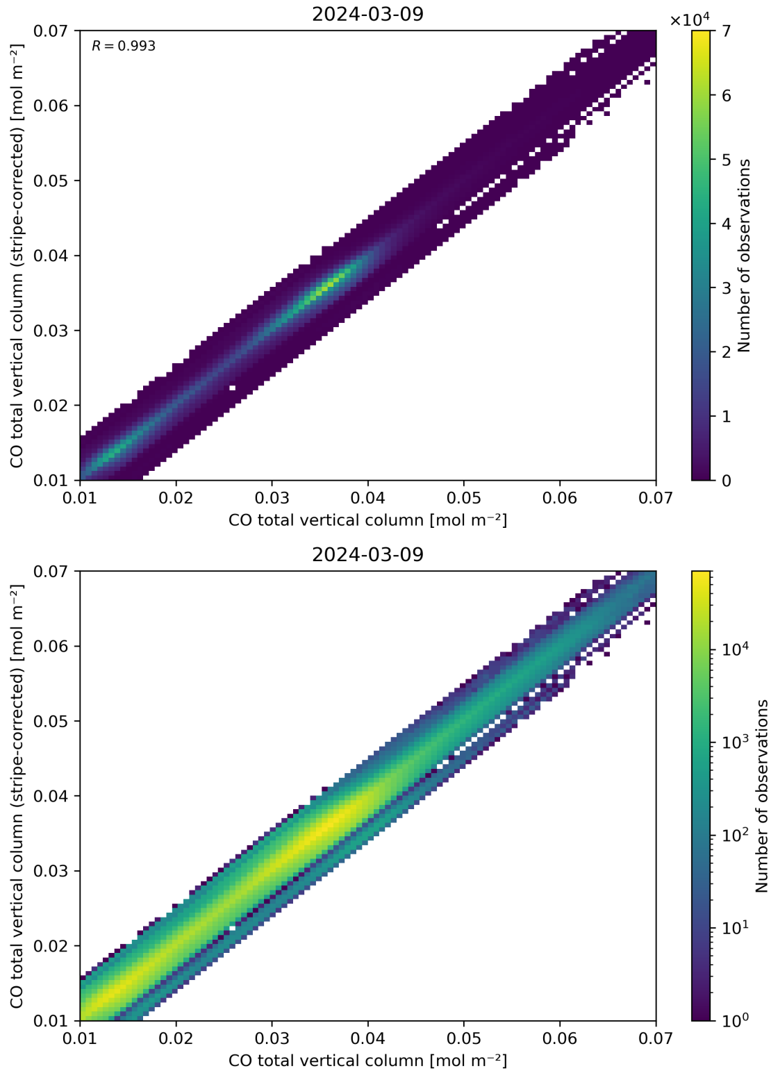
Figure 33: Scatter density plot of “CO total vertical column” against “CO total vertical column (stripe-corrected)” for 2024-03-09 to 2024-03-10.
