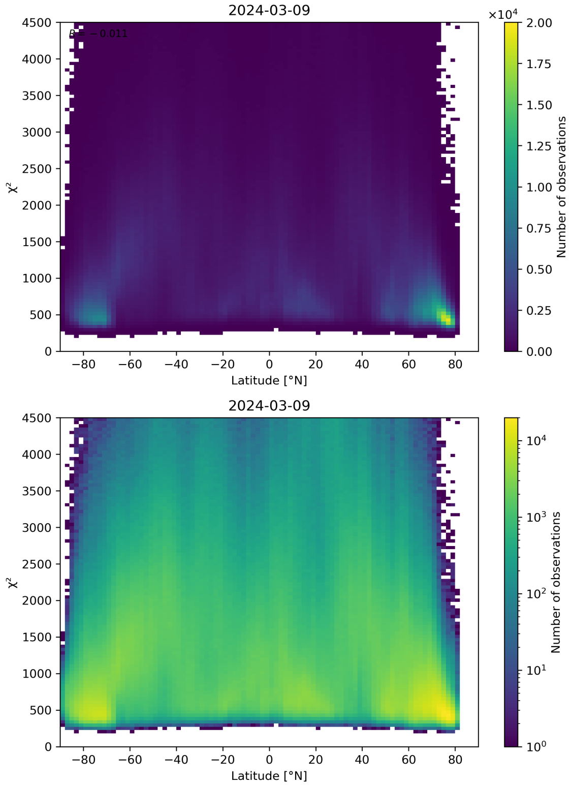
Figure 54: Scatter density plot of “Latitude” against “ \chi^2 ” for 2024-03-09 to 2024-03-10.
