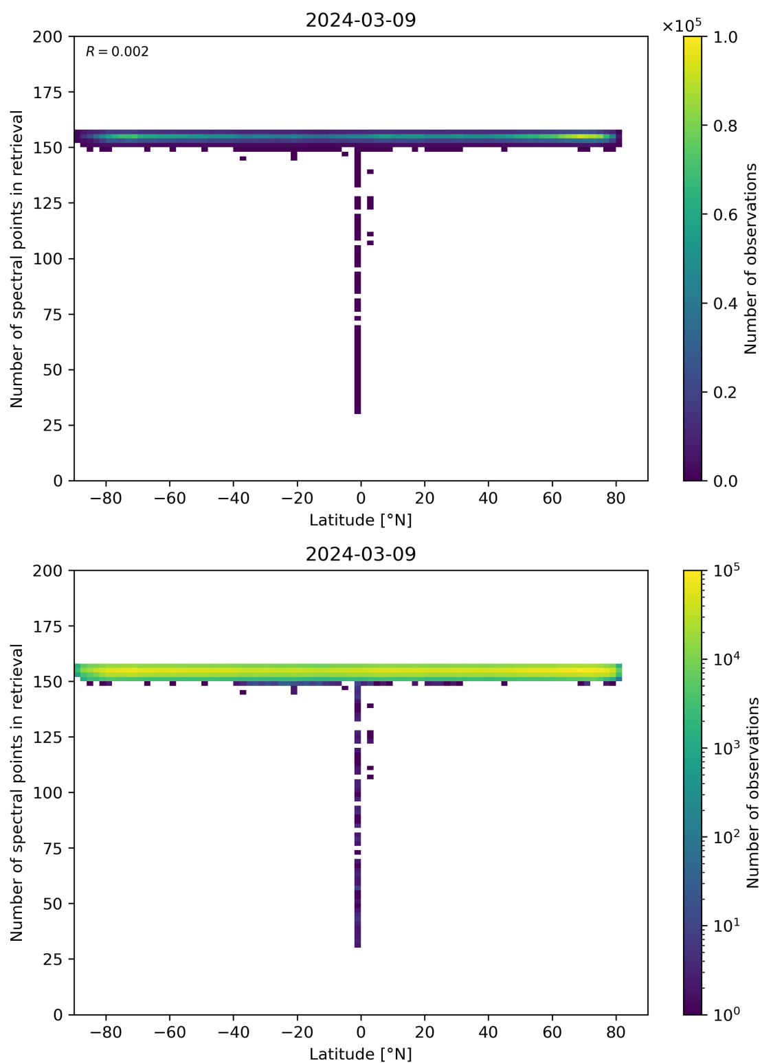
Figure 57: Scatter density plot of “Latitude” against “Number of spectral points in retrieval” for 2024-03-09 to 2024-03-10.
