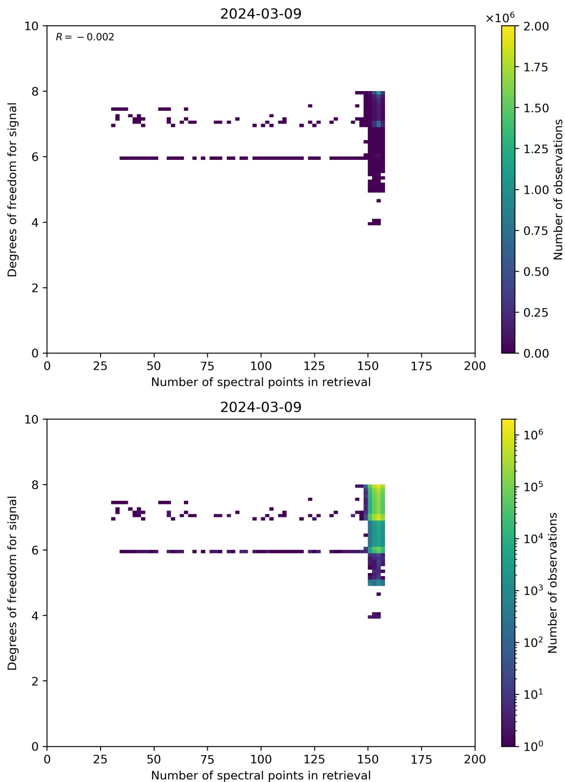
Figure 59: Scatter density plot of “Number of spectral points in retrieval” against “Degrees of freedom for signal” for 2024-03-09 to 2024-03-10.
