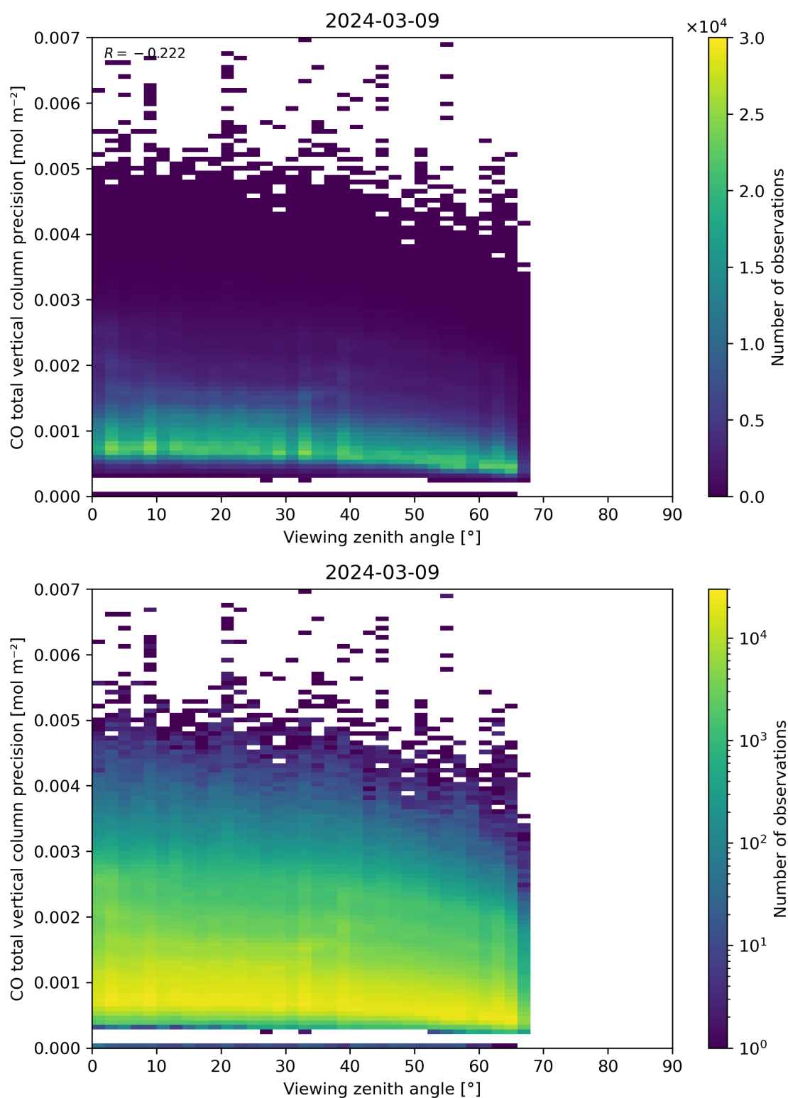
Figure 71: Scatter density plot of “Viewing zenith angle” against “CO total vertical column precision” for 2024-03-09 to 2024-03-10.
