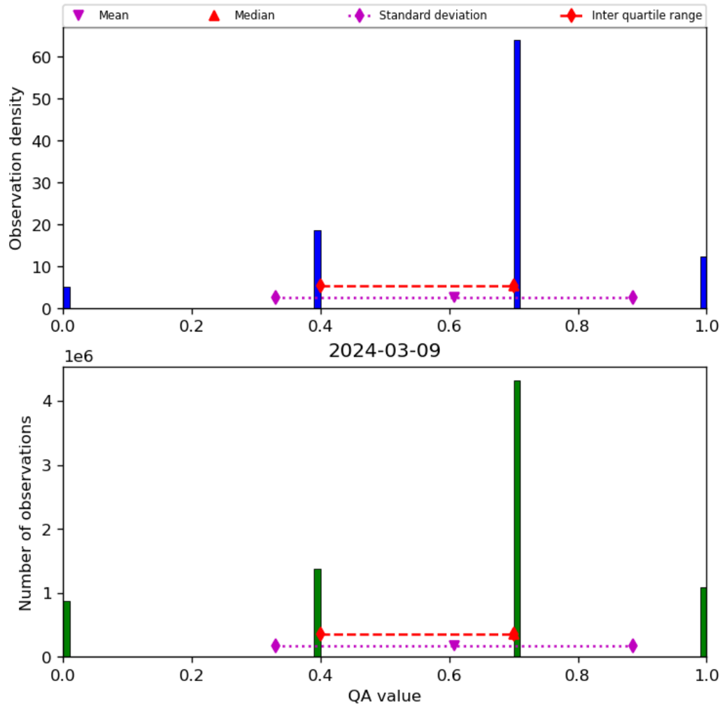
Figure 17: Histogram of “QA value” for 2024-03-09 to 2024-03-10
