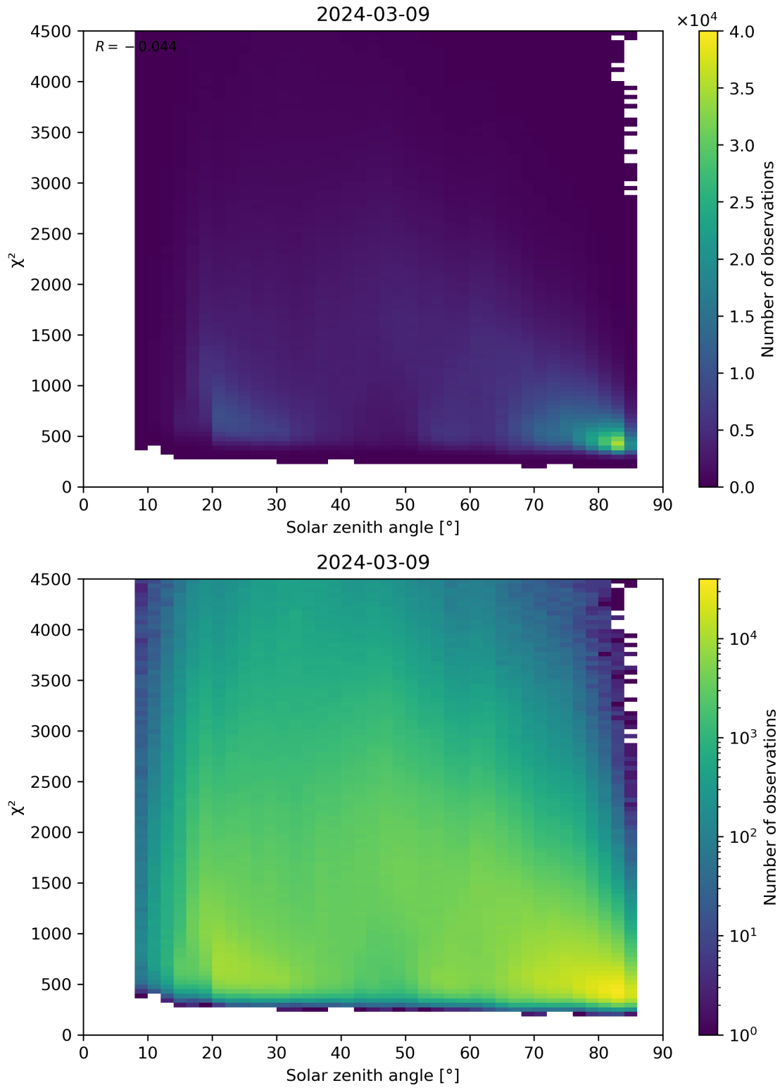
Figure 64: Scatter density plot of “Solar zenith angle” against “ \chi^2 ” for 2024-03-09 to 2024-03-10.
