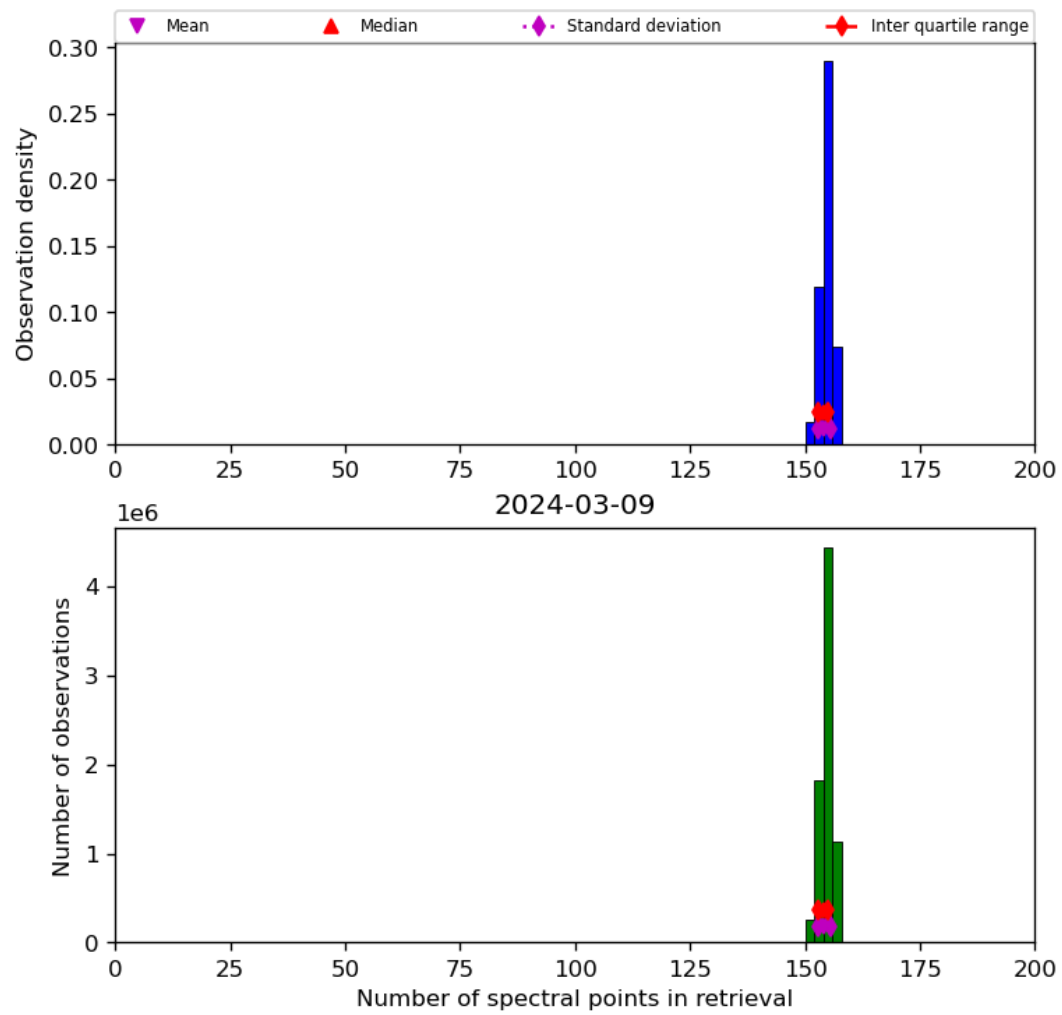
Figure 21: Histogram of “Number of spectral points in retrieval” for 2024-03-09 to 2024-03-10
