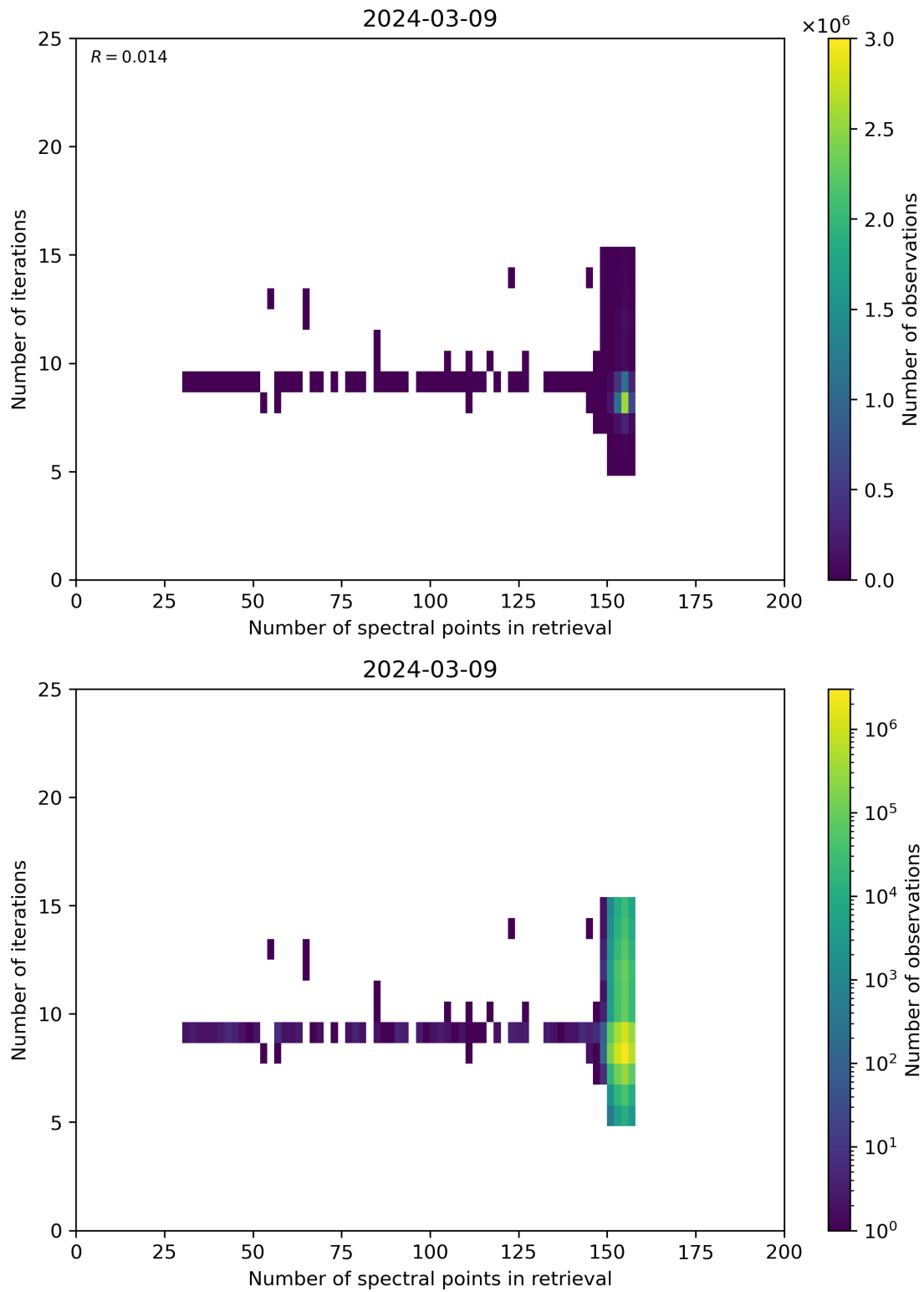
Figure 60: Scatter density plot of “Number of spectral points in retrieval” against “Number of iterations” for 2024-03-09 to 2024-03-10.
