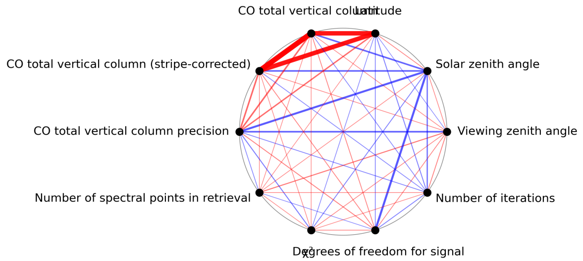
Figure 1: Map of correlation graph for 2024-03-09 to 2024-03-10.
