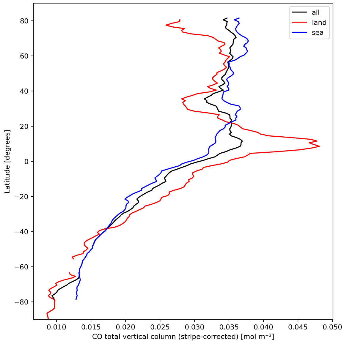
Figure 11: Zonal average of “CO total vertical column (stripe-corrected)” for 2024-03-09 to 2024-03-10.
