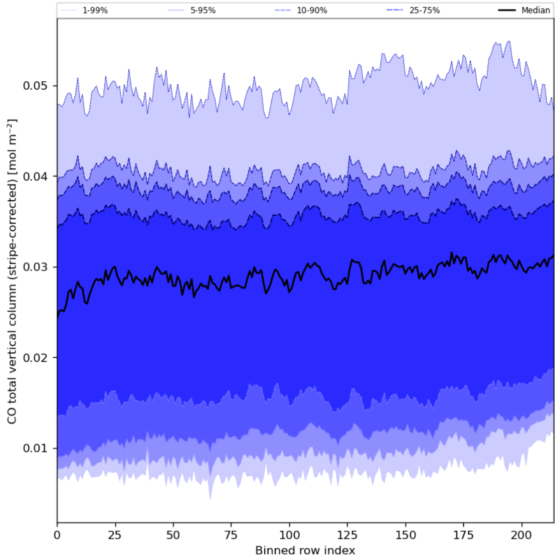
Figure 27: Along track statistics of “CO total vertical column (stripe-corrected)” for 2024-03-09 to 2024-03-10
