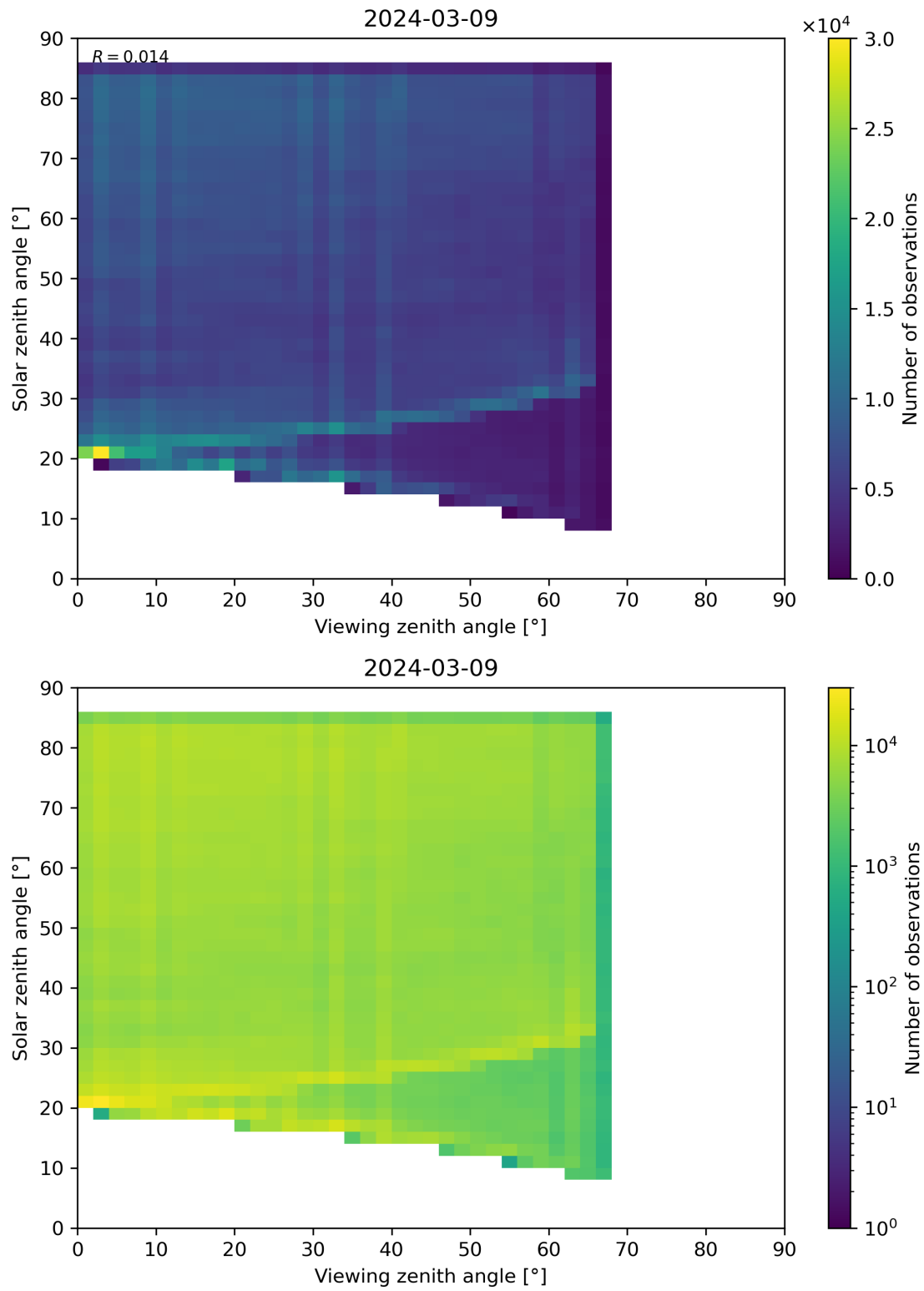
Figure 77: Scatter density plot of “Viewing zenith angle” against “Solar zenith angle” for 2024-03-09 to 2024-03-10.
