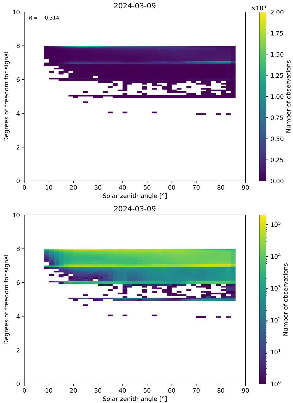
Figure 65: Scatter density plot of “Solar zenith angle” against “Degrees of freedom for signal” for 2024-03-09 to 2024-03-10.
