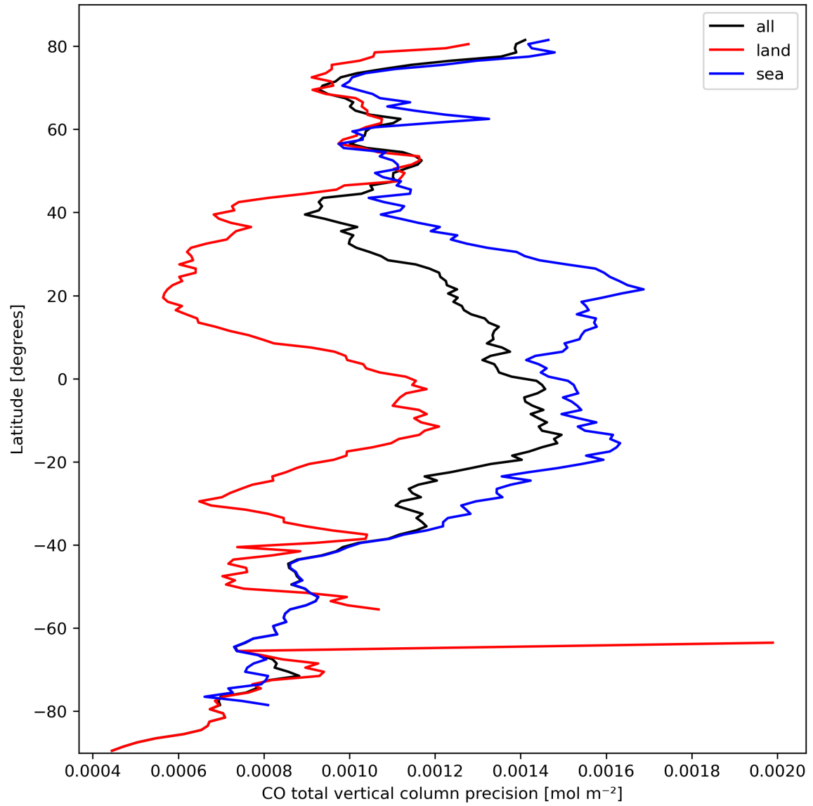
Figure 12: Zonal average of “CO total vertical column precision” for 2024-03-09 to 2024-03-10.
