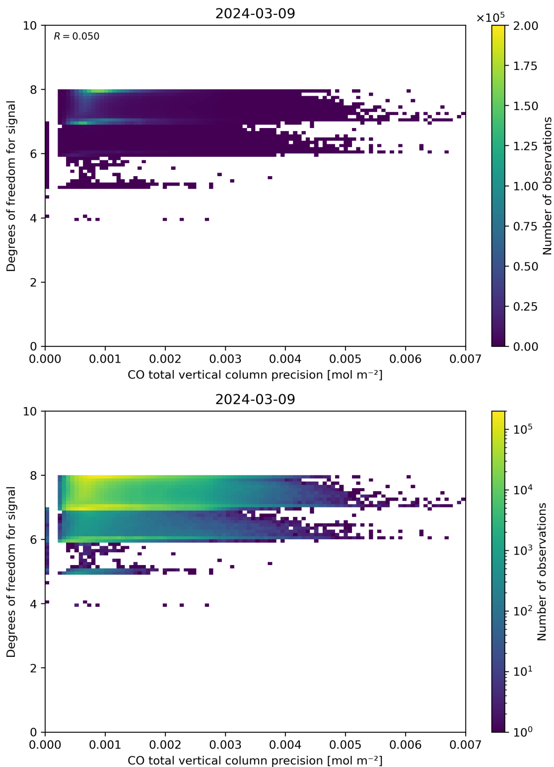
Figure 45: Scatter density plot of “CO total vertical column precision” against “Degrees of freedom for signal” for 2024-03-09 to 2024-03-10.
