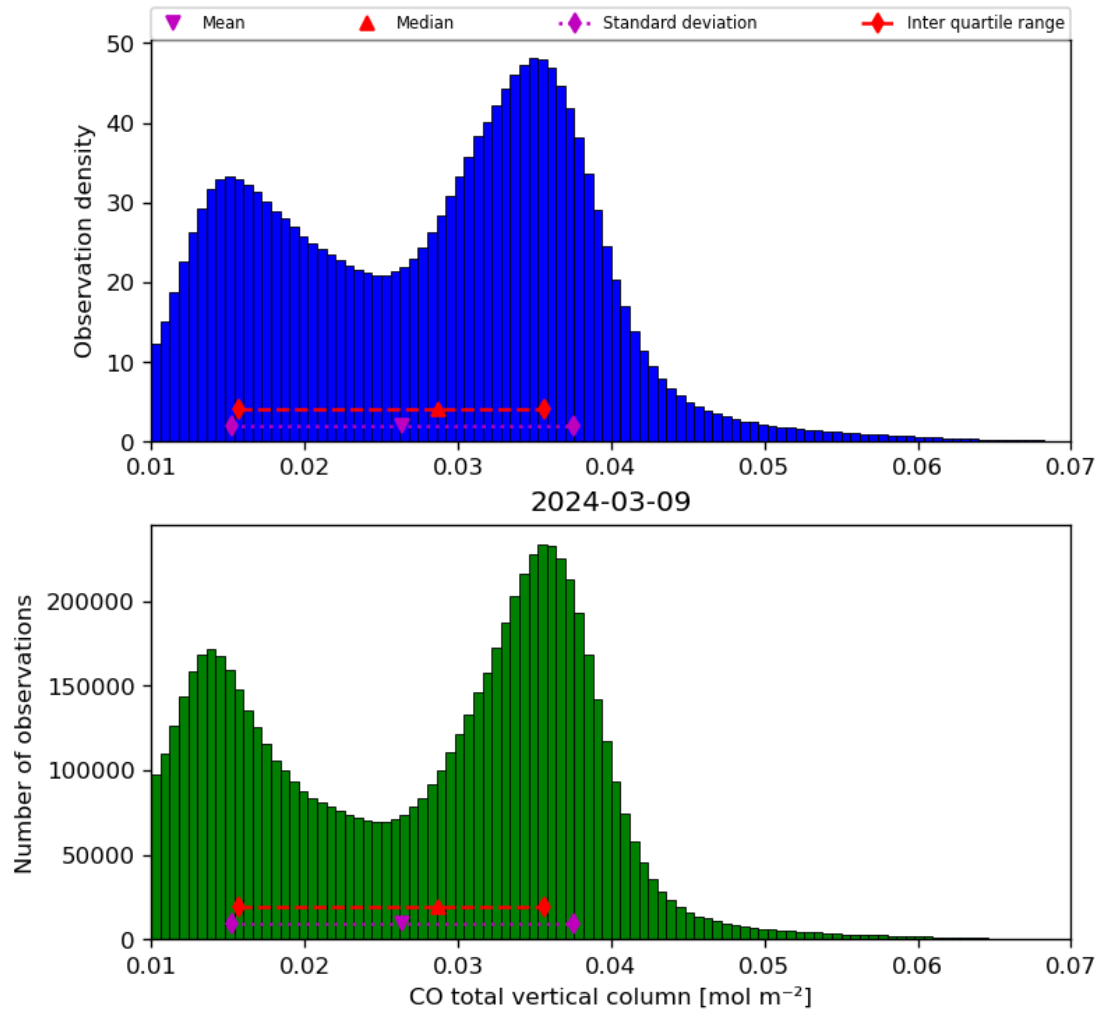
Figure 18: Histogram of “CO total vertical column” for 2024-03-09 to 2024-03-10
