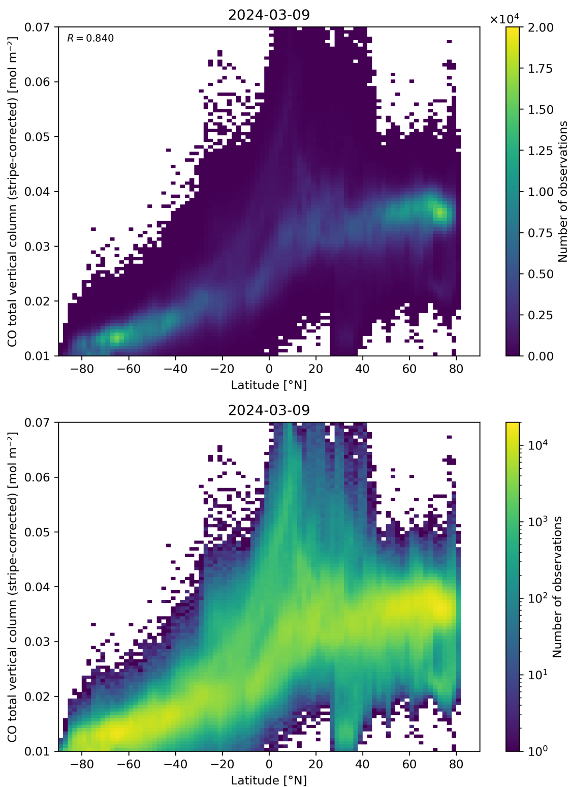
Figure 52: Scatter density plot of “Latitude” against “CO total vertical column (stripe-corrected)” for 2024-03-09 to 2024-03-10.
