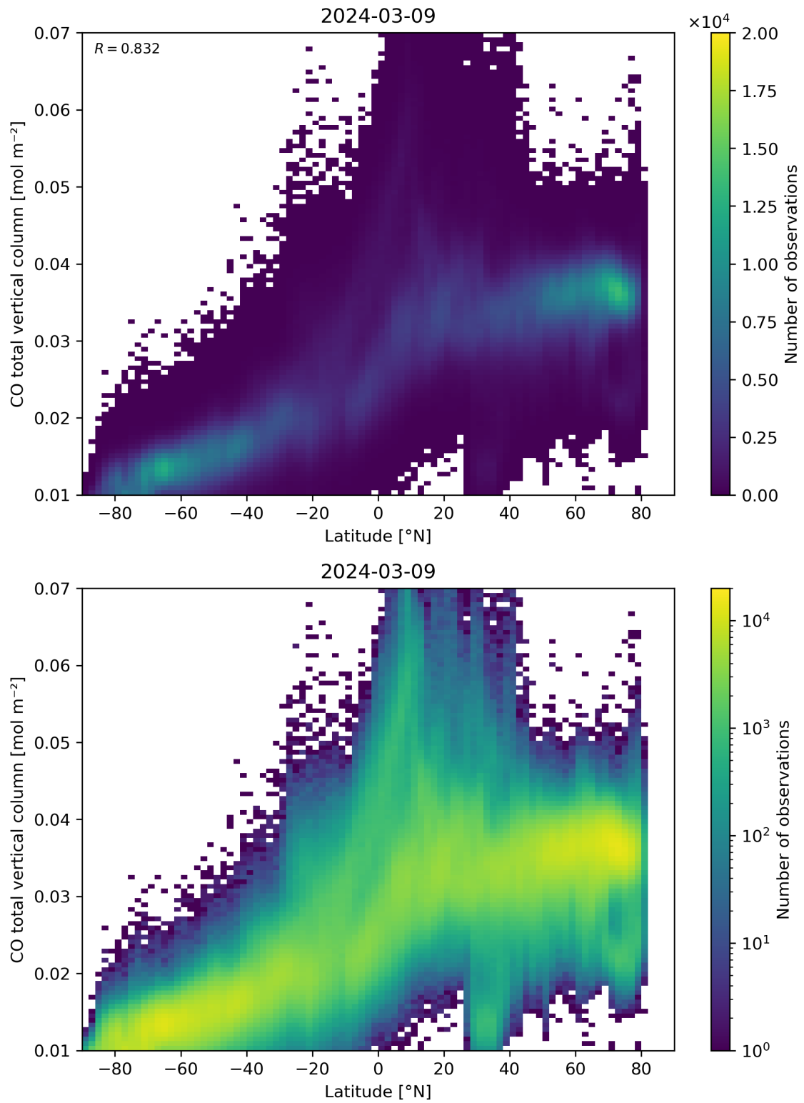
Figure 51: Scatter density plot of “Latitude” against “CO total vertical column” for 2024-03-09 to 2024-03-10.
