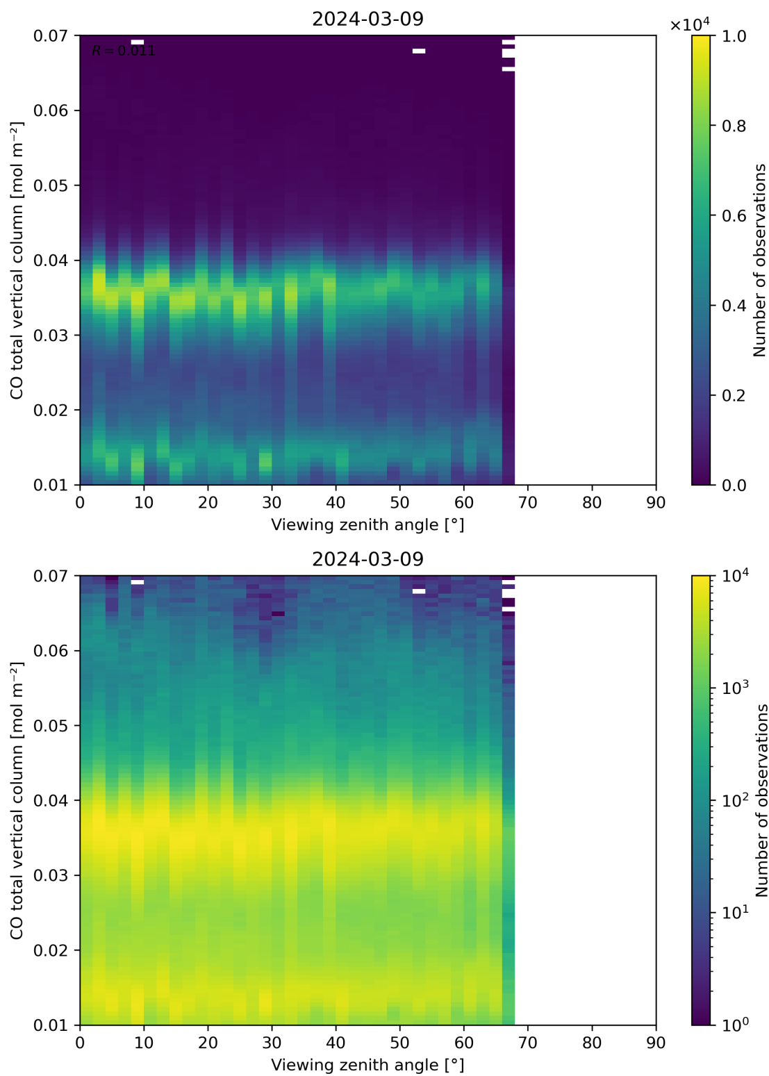
Figure 69: Scatter density plot of “Viewing zenith angle” against “CO total vertical column” for 2024-03-09 to 2024-03-10.
