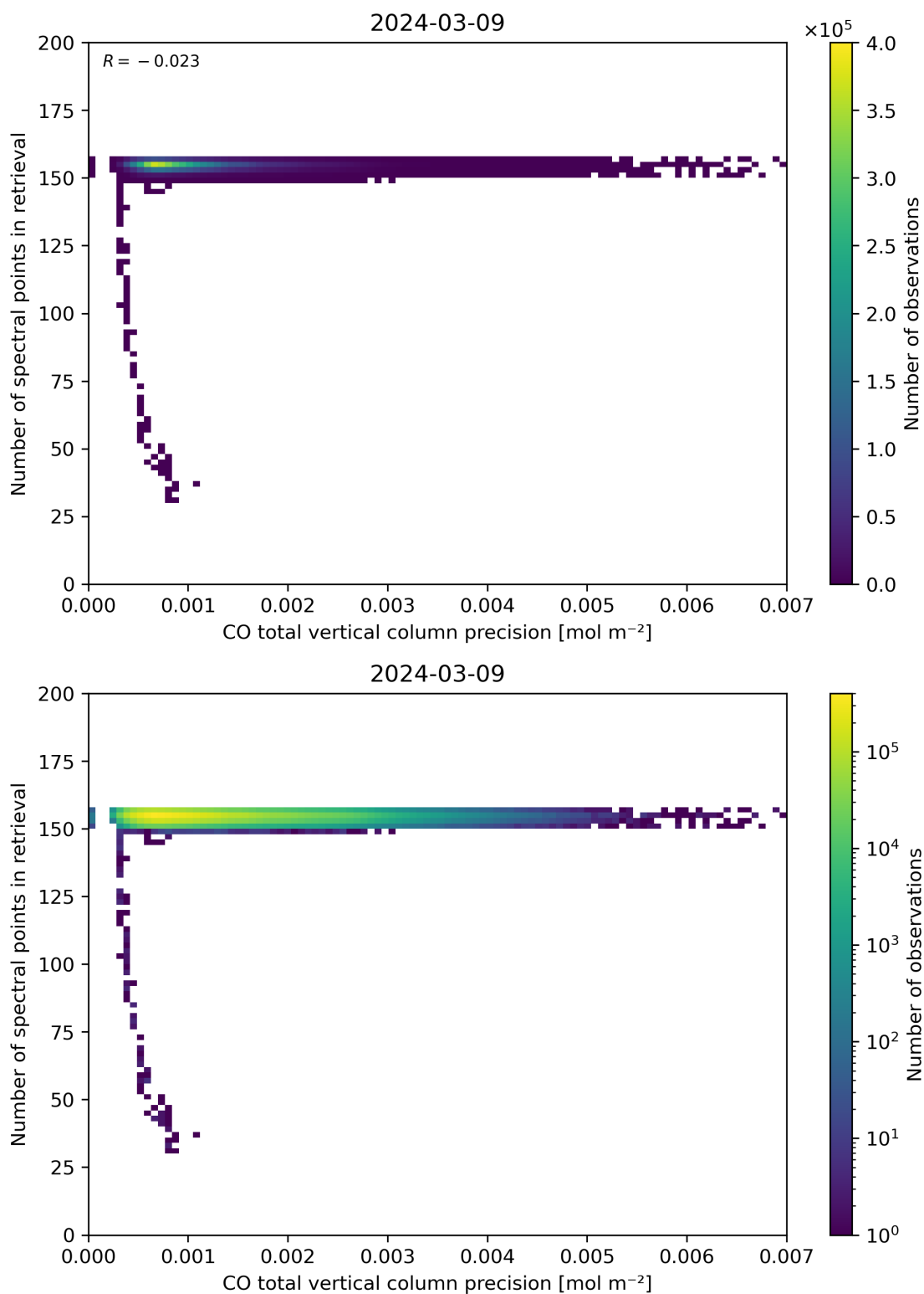
Figure 47: Scatter density plot of “CO total vertical column precision” against “Number of spectral points in retrieval” for 2024-03-09 to 2024-03-10.
