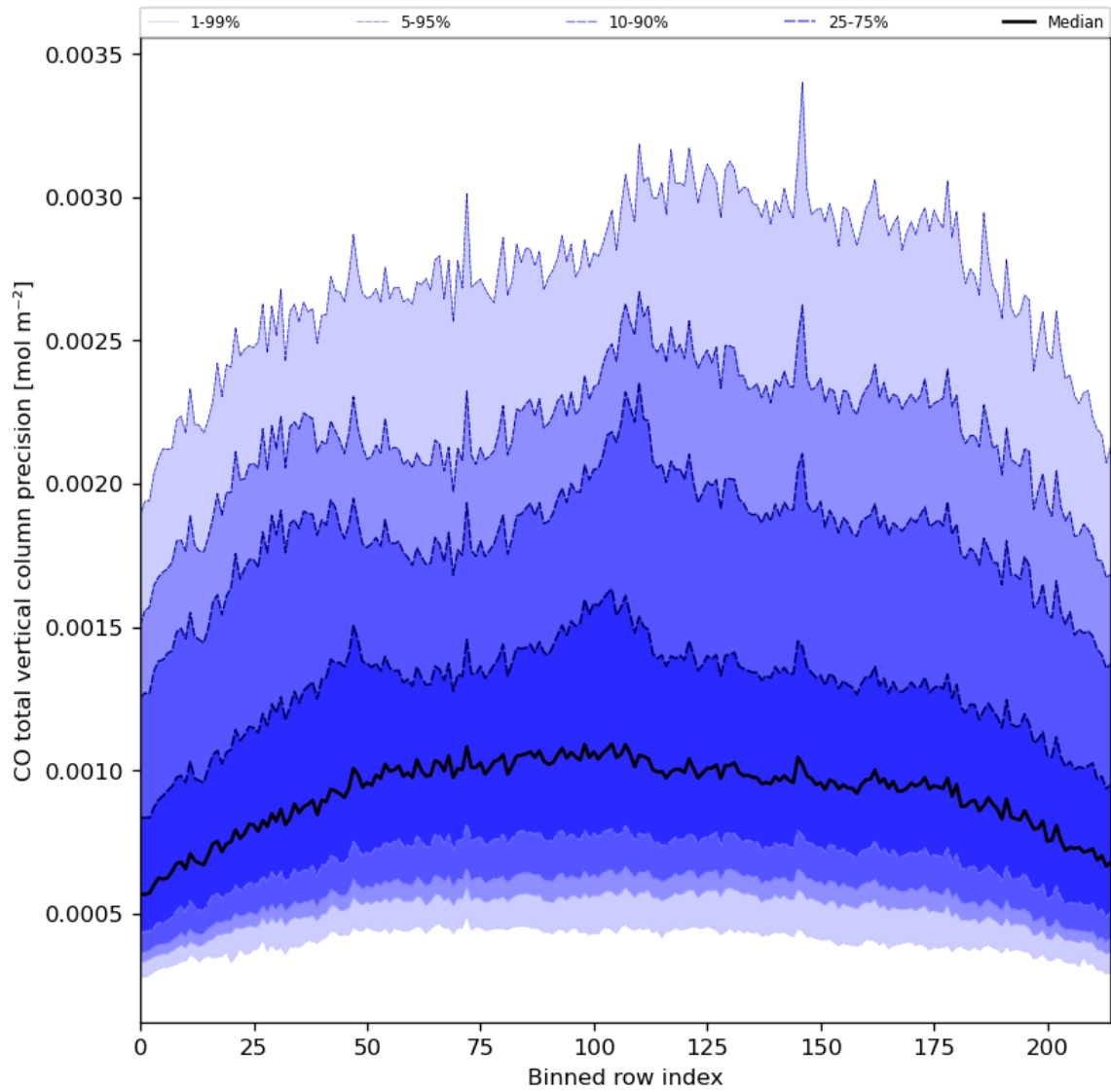
Figure 28: Along track statistics of “CO total vertical column precision” for 2024-03-09 to 2024-03-10
