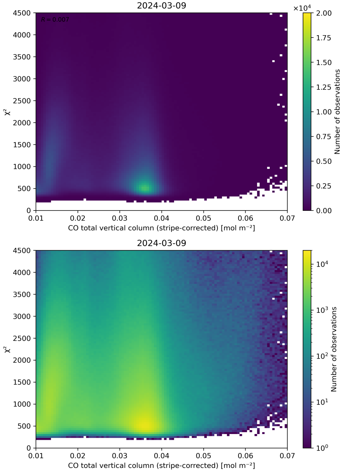
Figure 37: Scatter density plot of “CO total vertical column (stripe-corrected)” against “ \chi^2 ” for 2024-03-09 to 2024-03-10.
