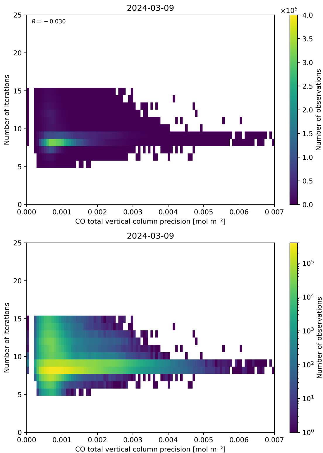
Figure 46: Scatter density plot of “CO total vertical column precision” against “Number of iterations” for 2024-03-09 to 2024-03-10.
