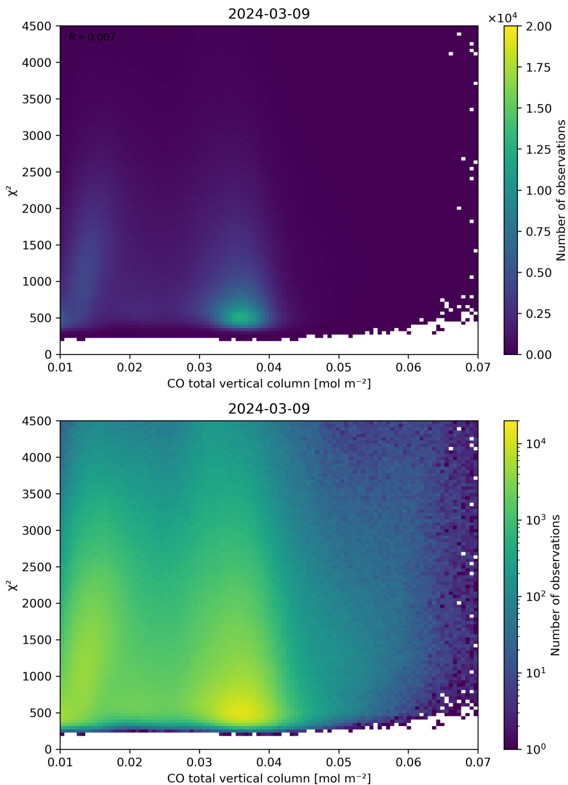
Figure 35: Scatter density plot of “CO total vertical column” against “ \chi^2 ” for 2024-03-09 to 2024-03-10.
