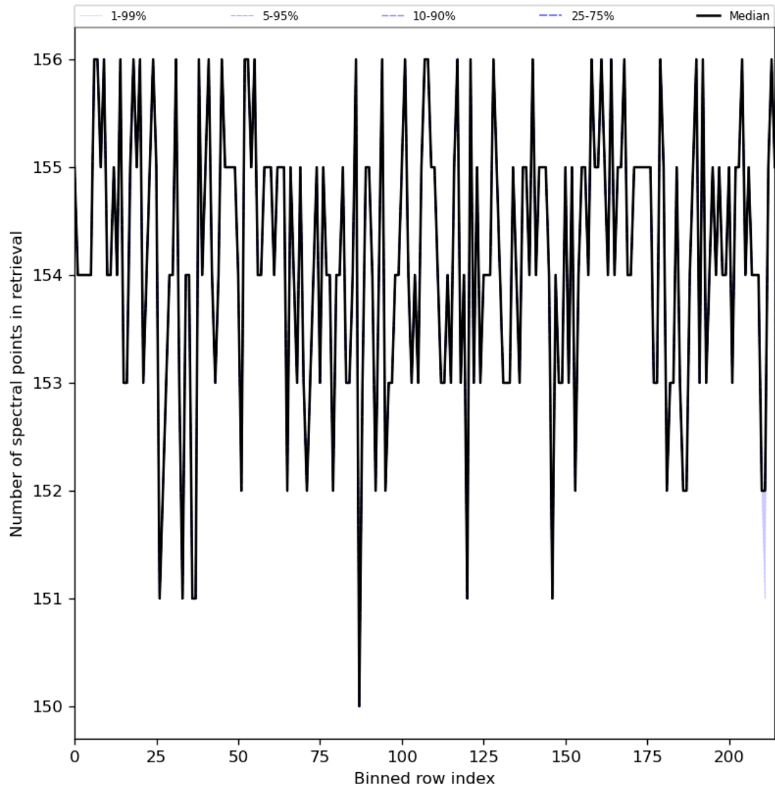
Figure 29: Along track statistics of “Number of spectral points in retrieval” for 2024-03-09 to 2024-03-10
