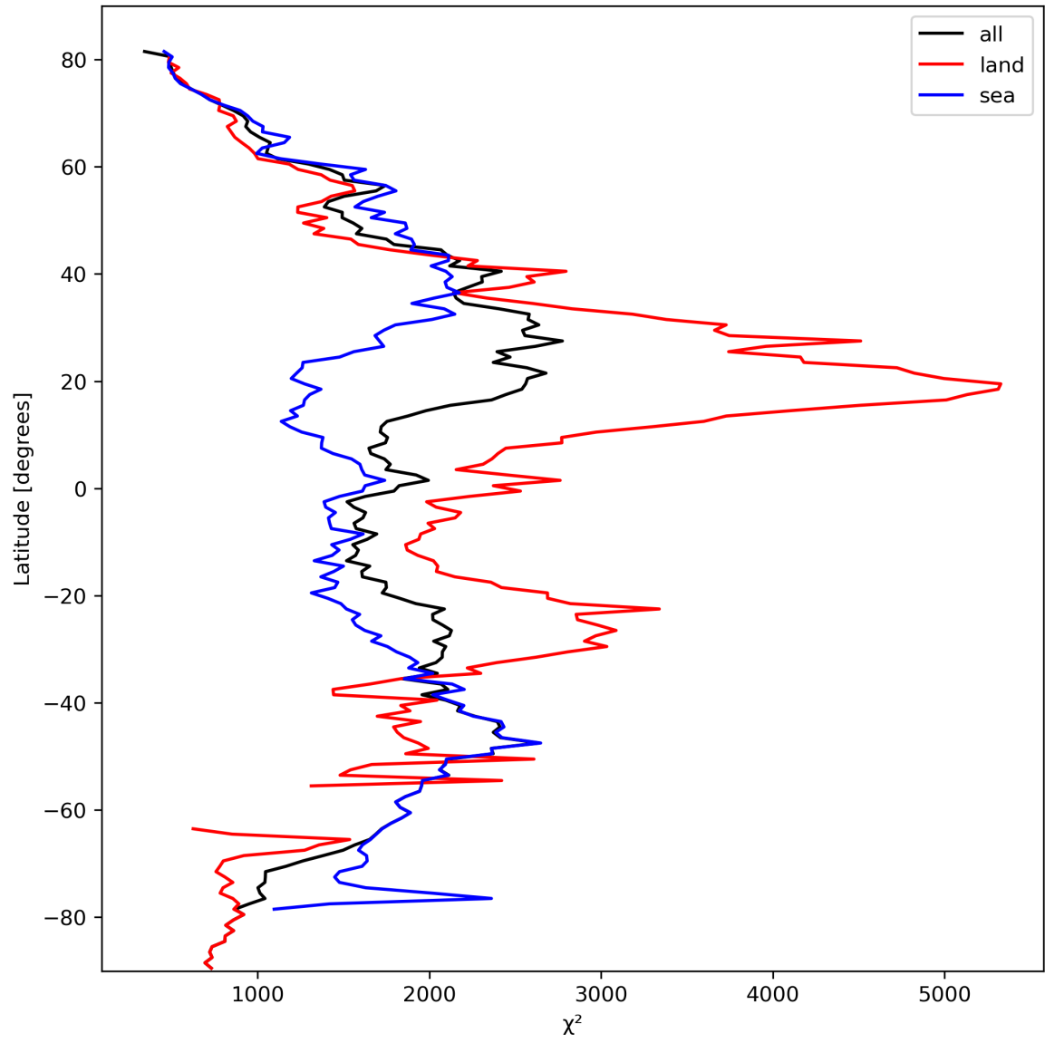
Figure 14: Zonal average of “ \chi^2 ” for 2024-03-09 to 2024-03-10.
