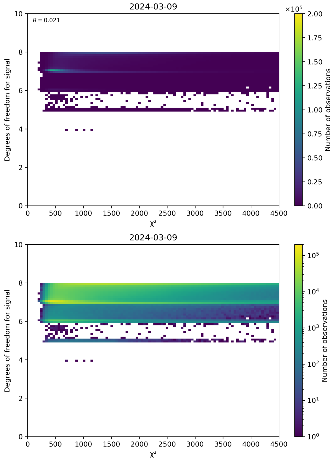
Figure 48: Scatter density plot of “ \chi^2 ” against “Degrees of freedom for signal” for 2024-03-09 to 2024-03-10.
