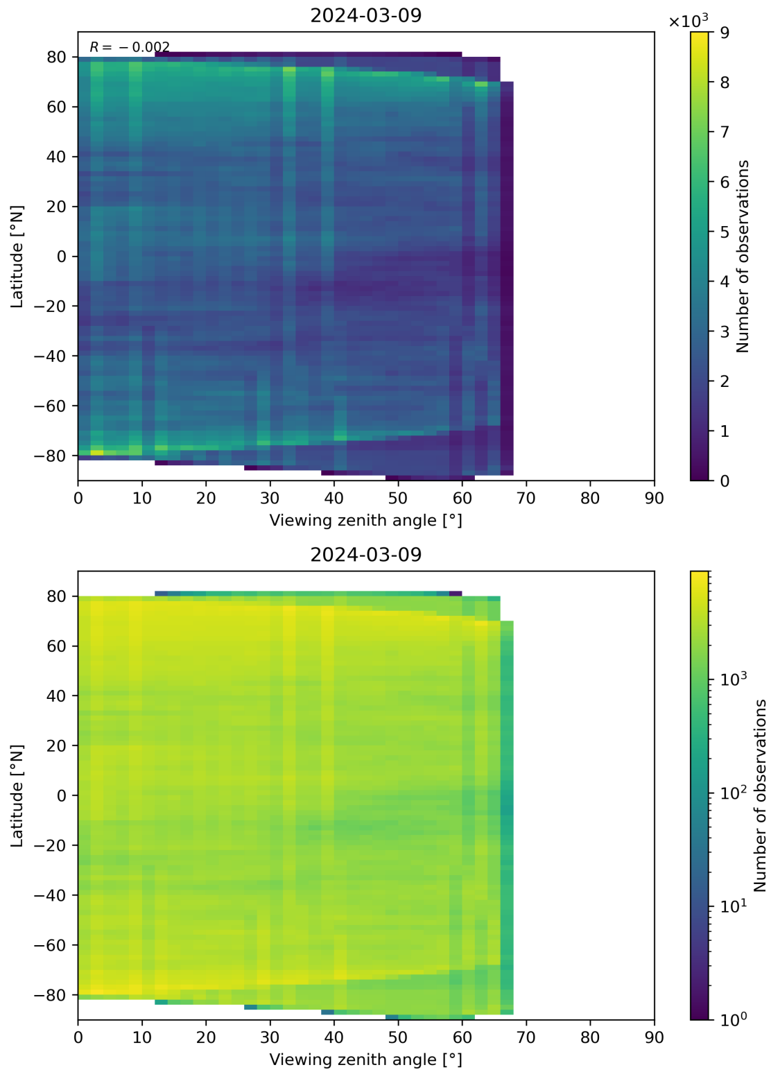
Figure 74: Scatter density plot of “Viewing zenith angle” against “Latitude” for 2024-03-09 to 2024-03-10.
