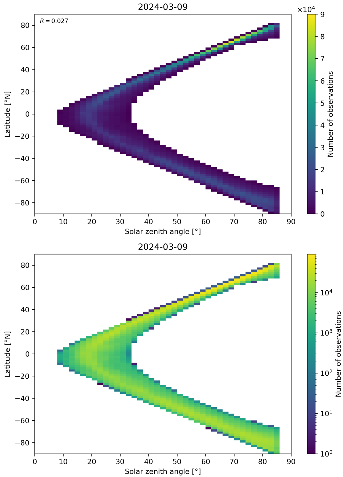
Figure 66: Scatter density plot of “Solar zenith angle” against “Latitude” for 2024-03-09 to 2024-03-10.
