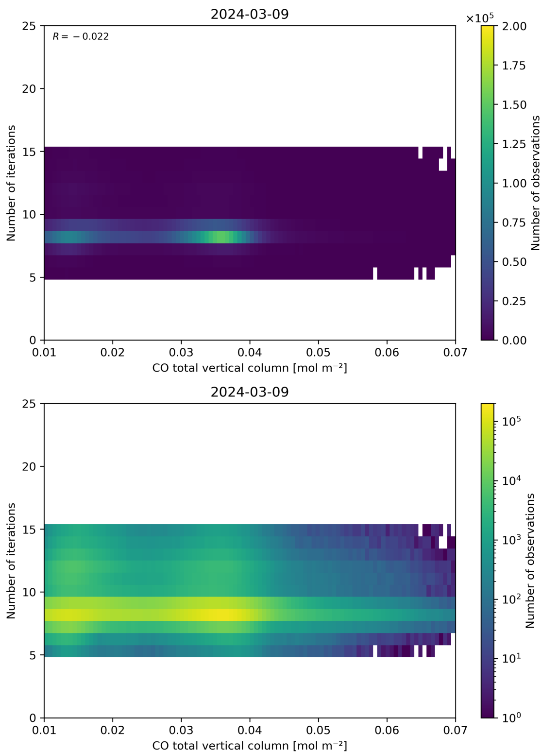
Figure 42: Scatter density plot of “CO total vertical column” against “Number of iterations” for 2024-03-09 to 2024-03-10.
