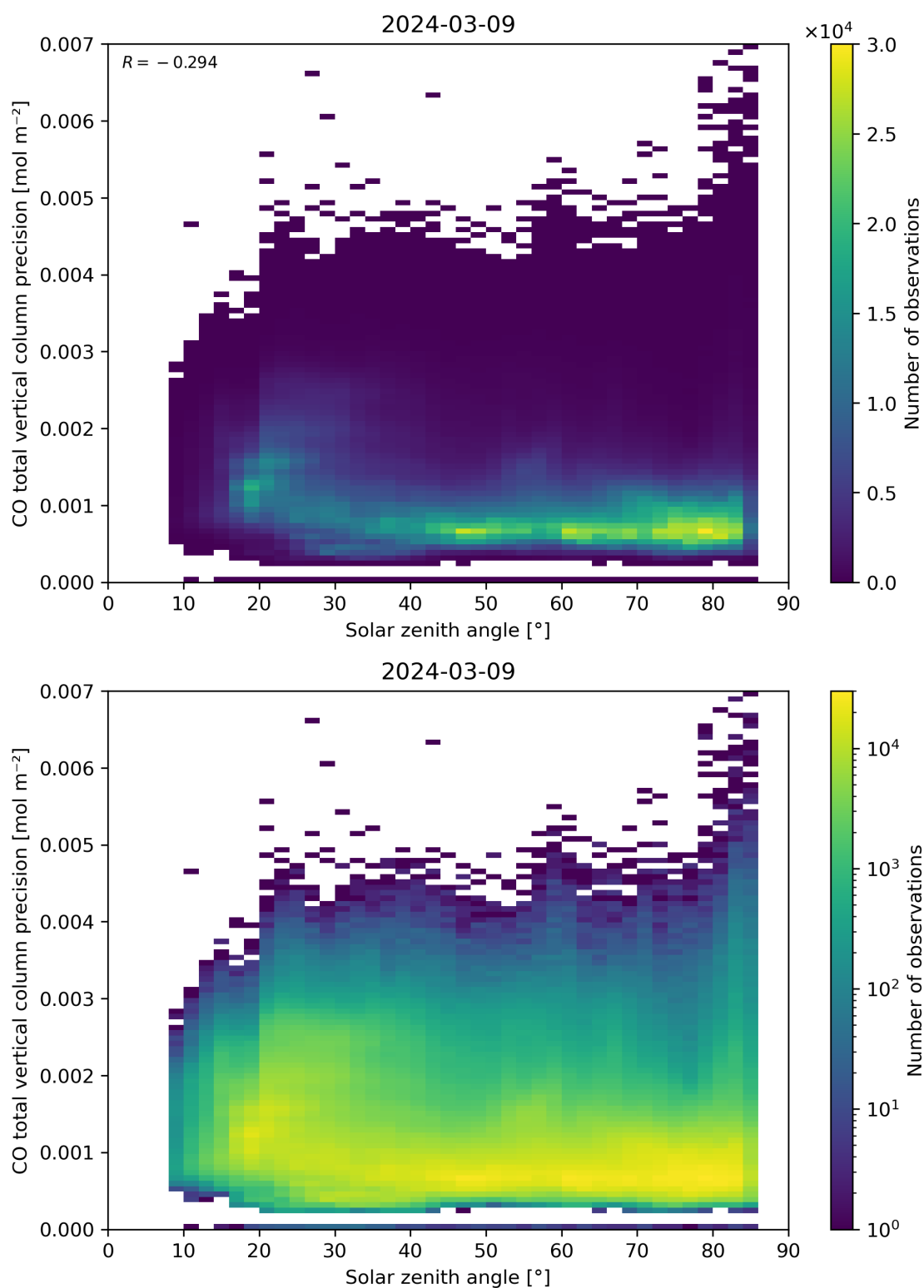
Figure 63: Scatter density plot of “Solar zenith angle” against “CO total vertical column precision” for 2024-03-09 to 2024-03-10.
