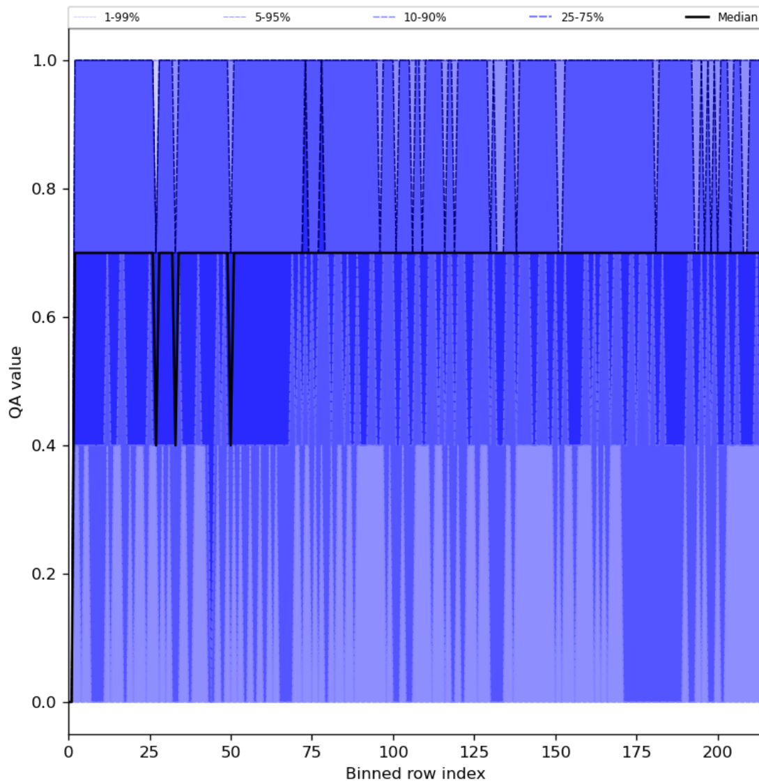
Figure 25: Along track statistics of “QA value” for 2024-03-09 to 2024-03-10
