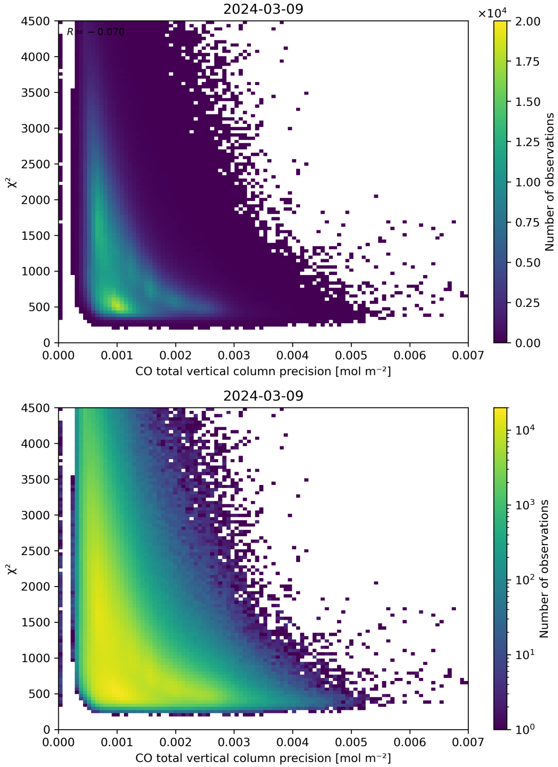
Figure 44: Scatter density plot of “CO total vertical column precision” against “ \chi^2 ” for 2024-03-09 to 2024-03-10.
