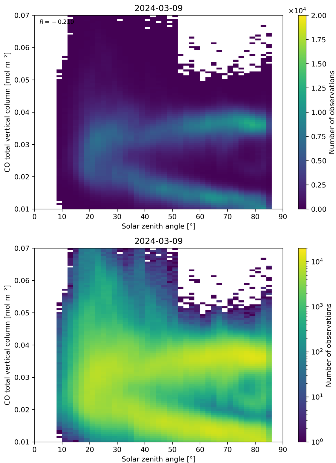
Figure 61: Scatter density plot of “Solar zenith angle” against “CO total vertical column” for 2024-03-09 to 2024-03-10.
