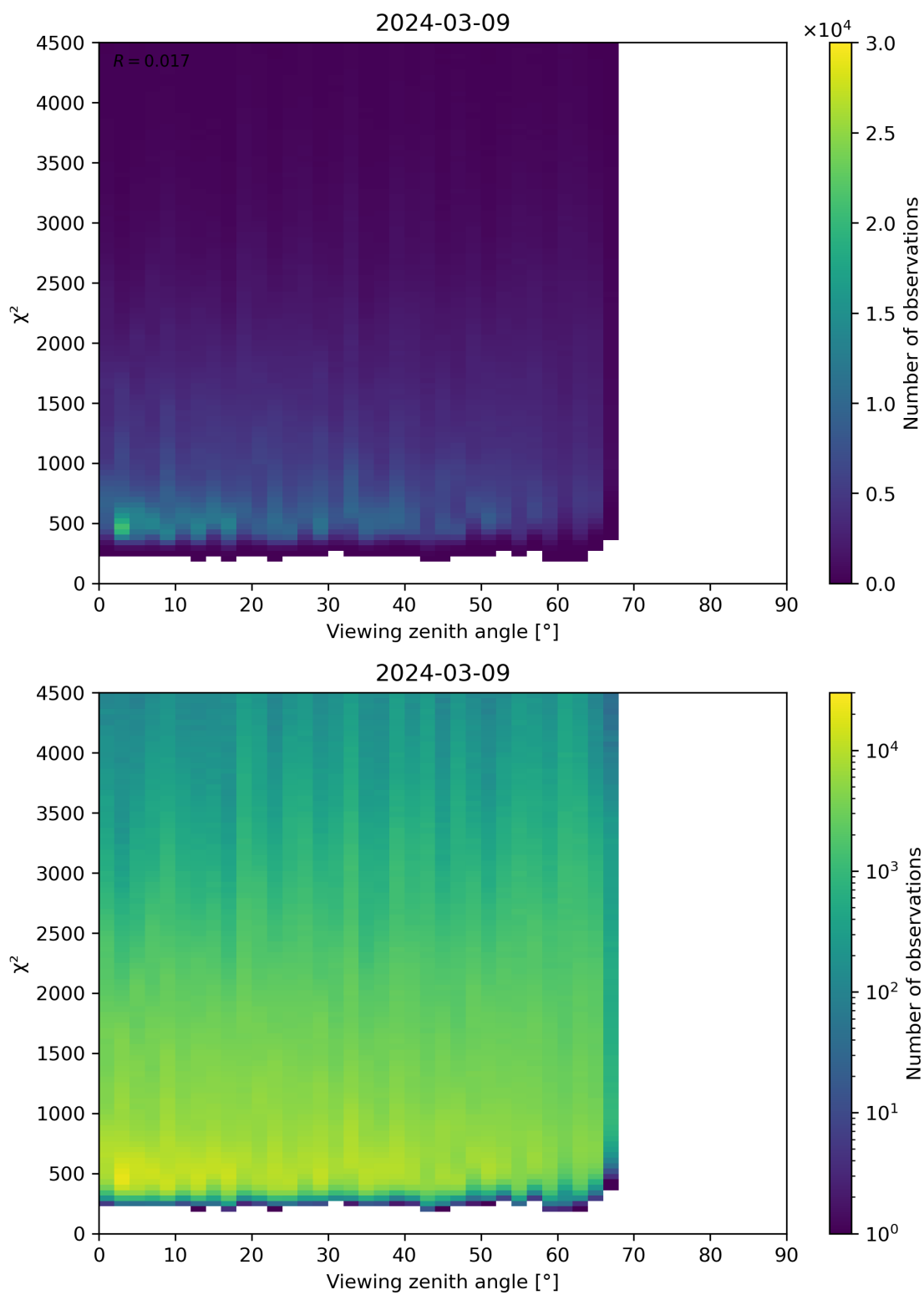
Figure 72: Scatter density plot of “Viewing zenith angle” against “ \chi^2 ” for 2024-03-09 to 2024-03-10.
