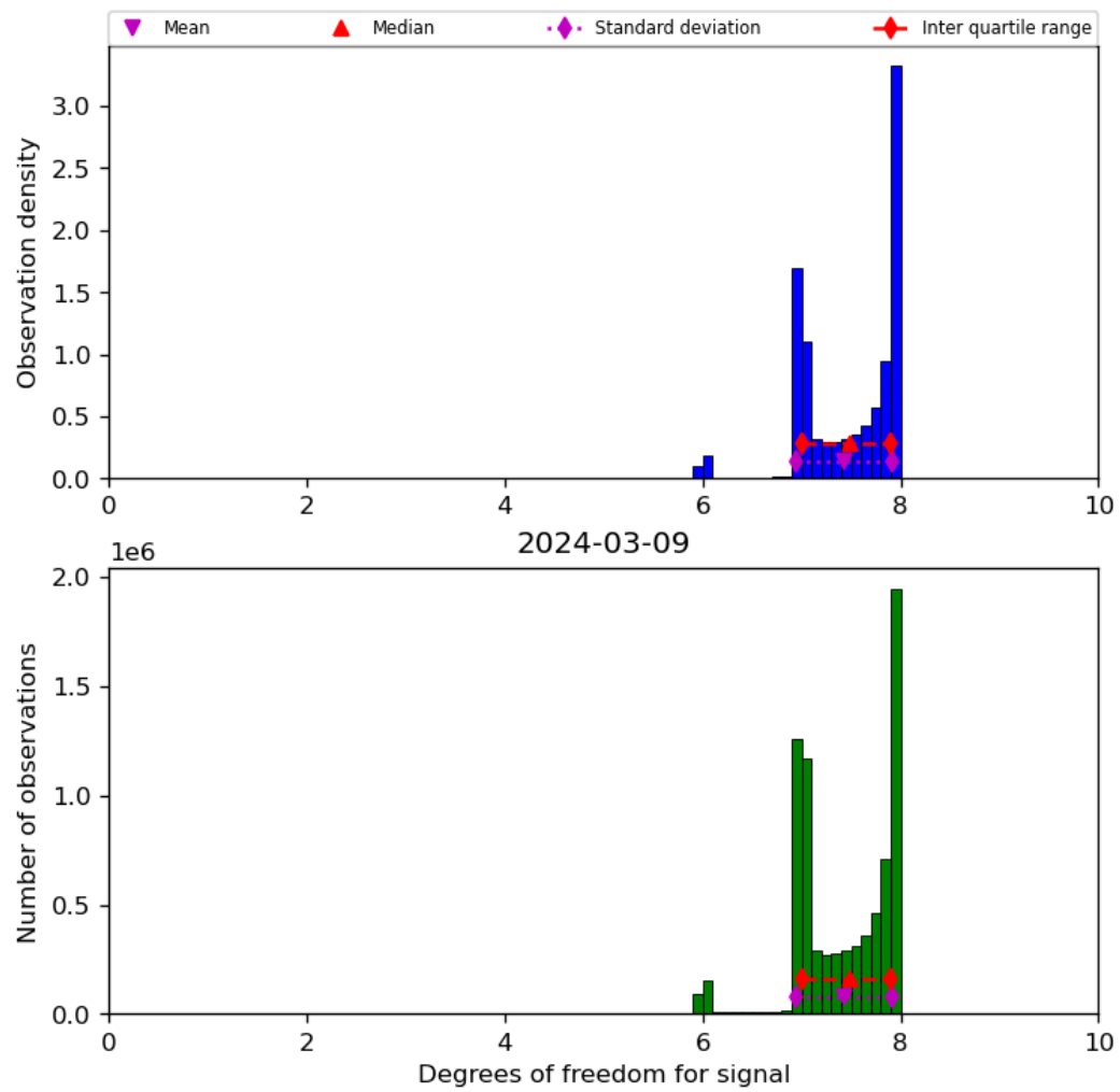
Figure 23: Histogram of “Degrees of freedom for signal” for 2024-03-09 to 2024-03-10
