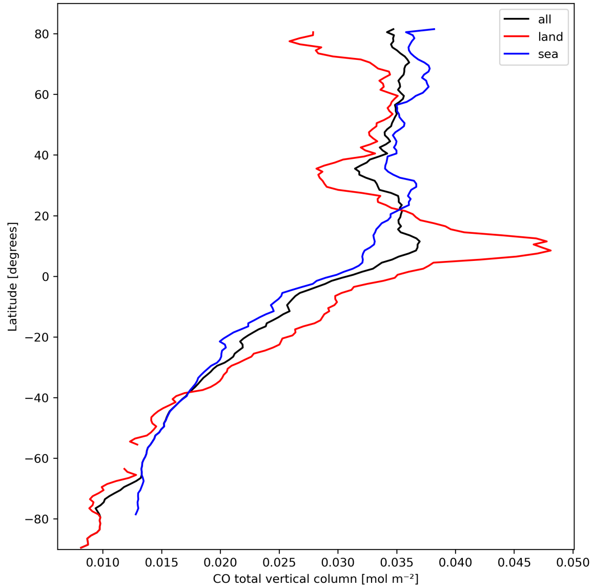
Figure 10: Zonal average of “CO total vertical column” for 2024-03-09 to 2024-03-10.
