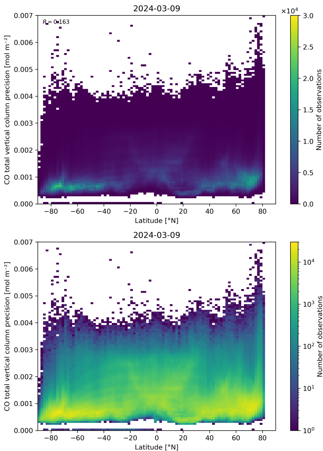
Figure 53: Scatter density plot of “Latitude” against “CO total vertical column precision” for 2024-03-09 to 2024-03-10.
