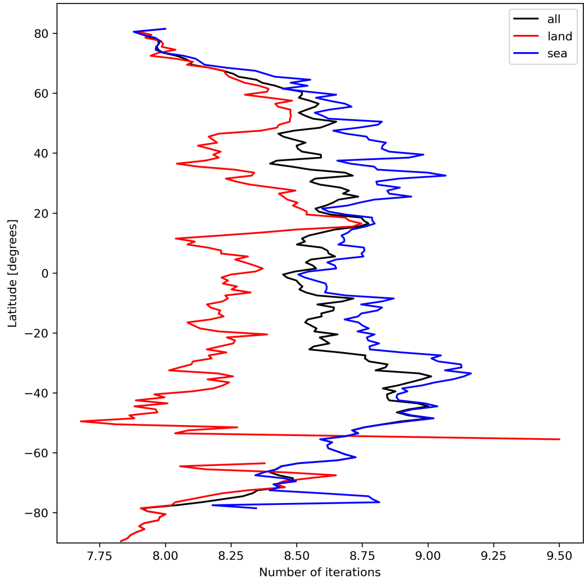
Figure 16: Zonal average of “Number of iterations” for 2024-03-09 to 2024-03-10.
