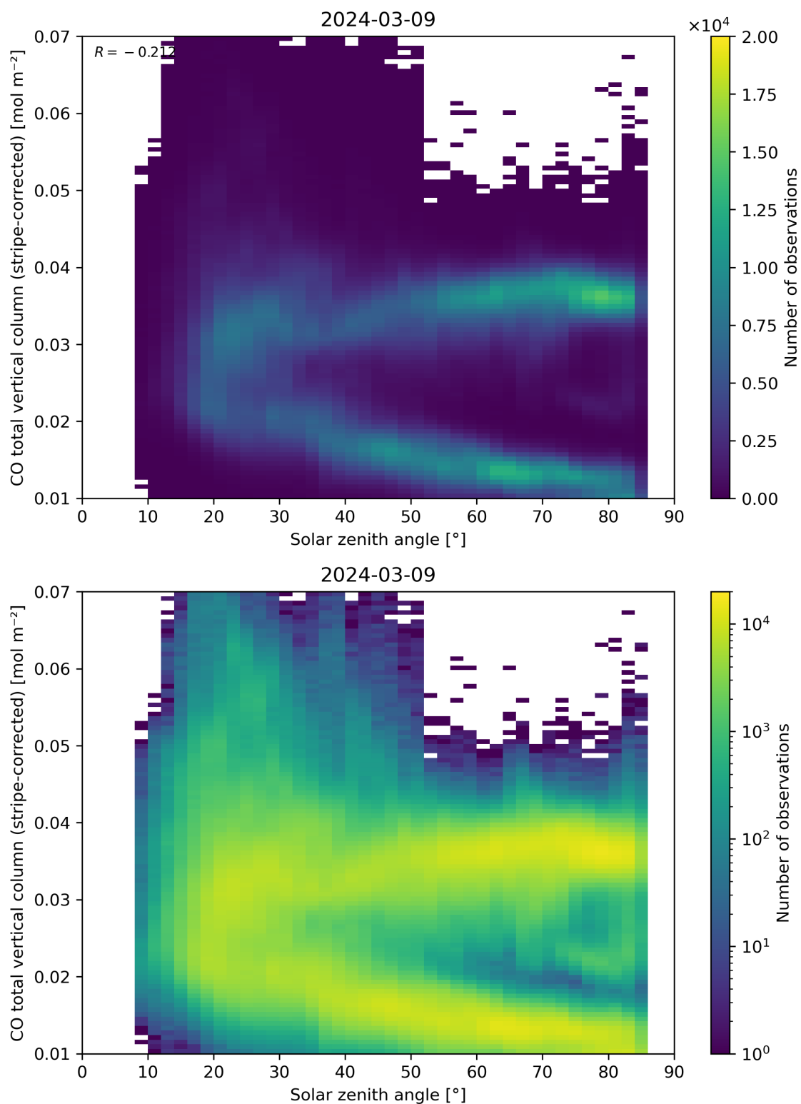
Figure 62: Scatter density plot of “Solar zenith angle” against “CO total vertical column (stripe-corrected)” for 2024-03-09 to 2024-03-10.
