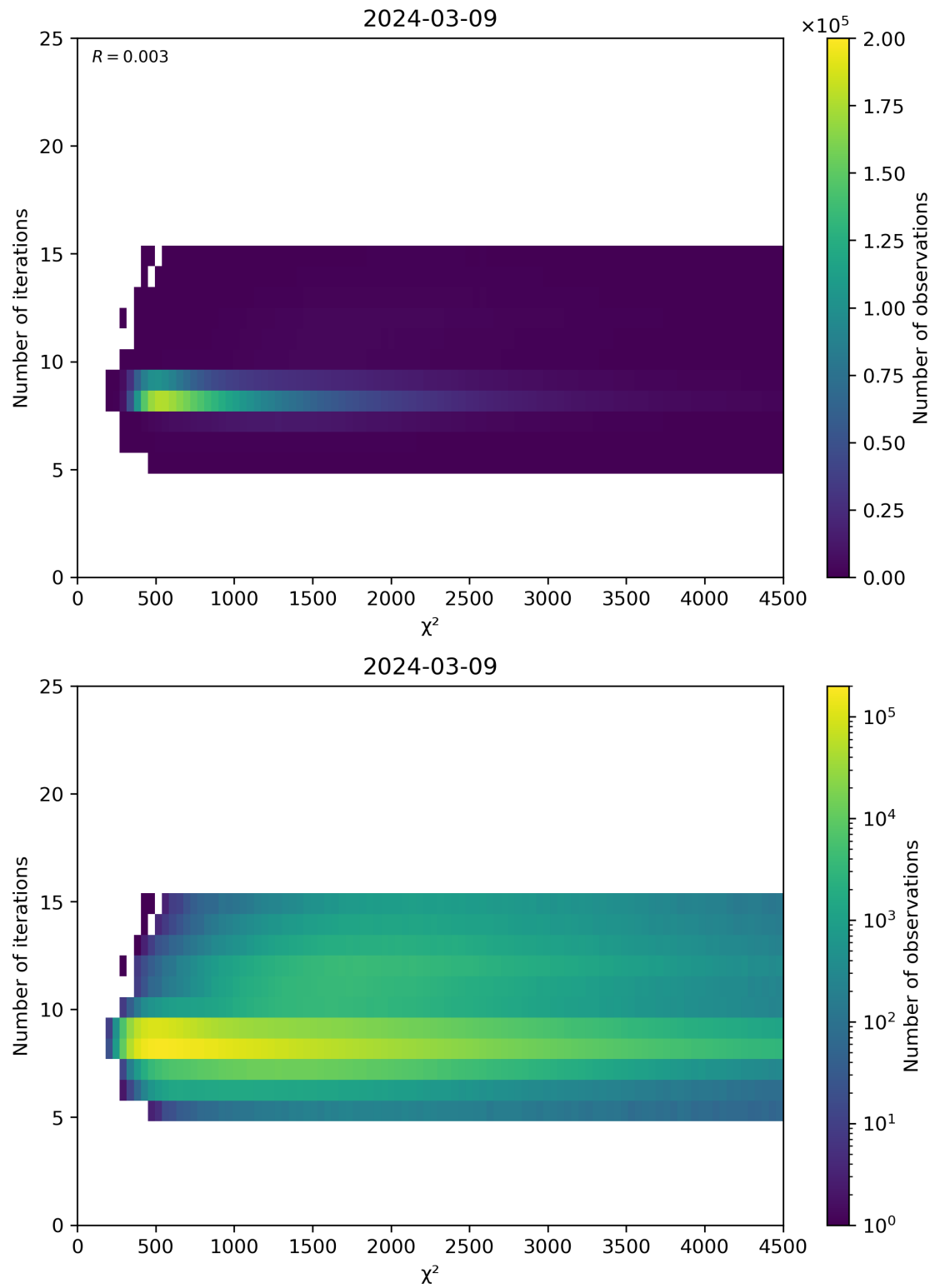
Figure 49: Scatter density plot of “ \chi^2 ” against “Number of iterations” for 2024-03-09 to 2024-03-10.
