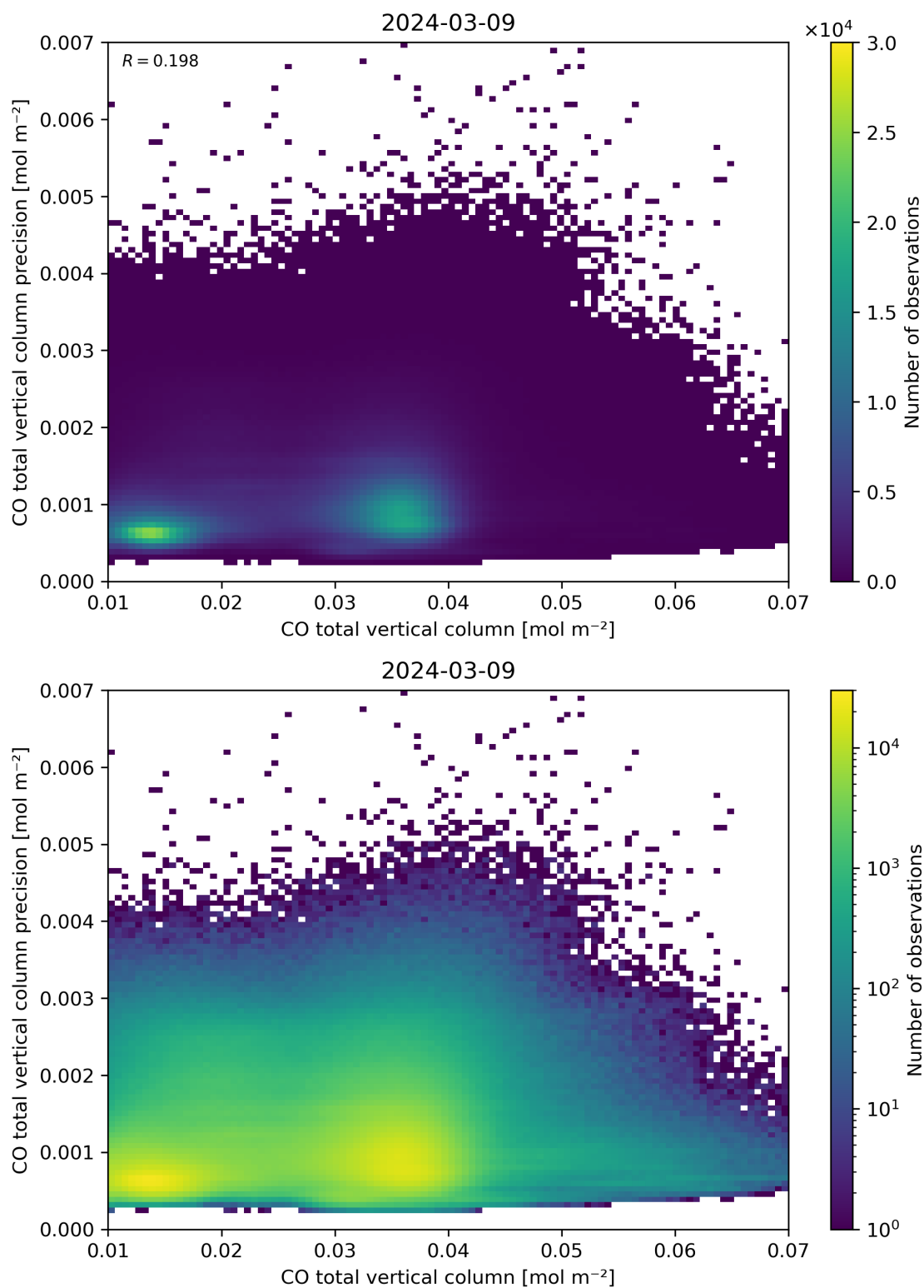
Figure 34: Scatter density plot of “CO total vertical column” against “CO total vertical column precision” for 2024-03-09 to 2024-03-10.
