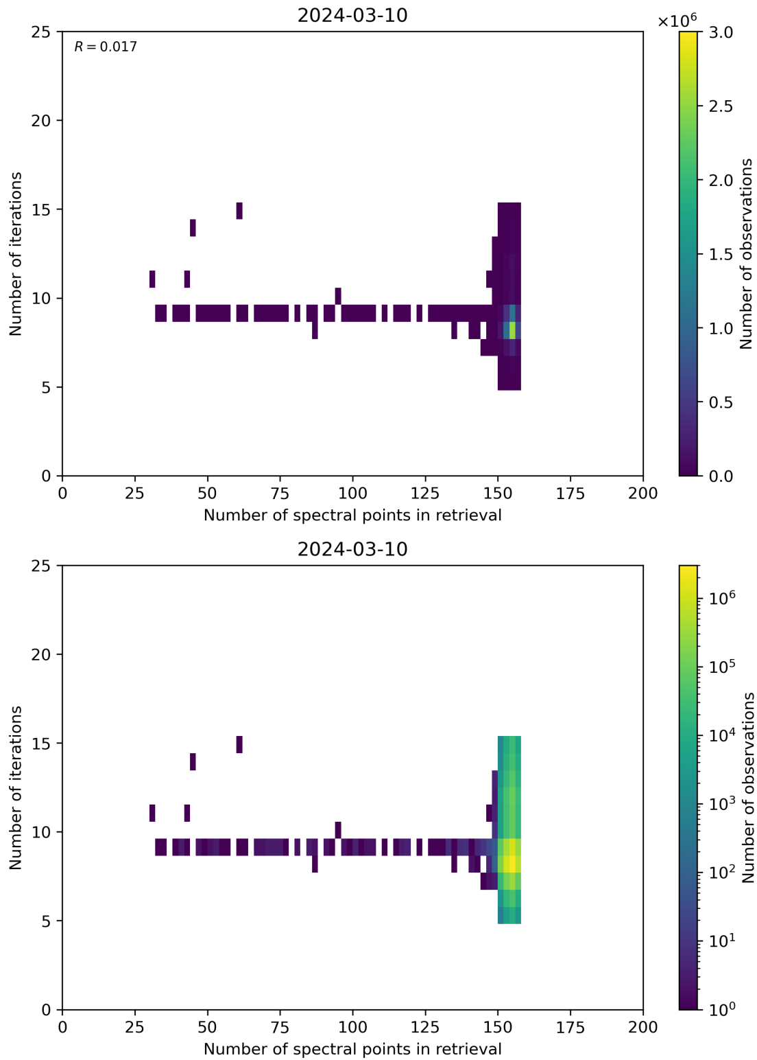
Figure 60: Scatter density plot of “Number of spectral points in retrieval” against “Number of iterations” for 2024-03-09 to 2024-03-11.
