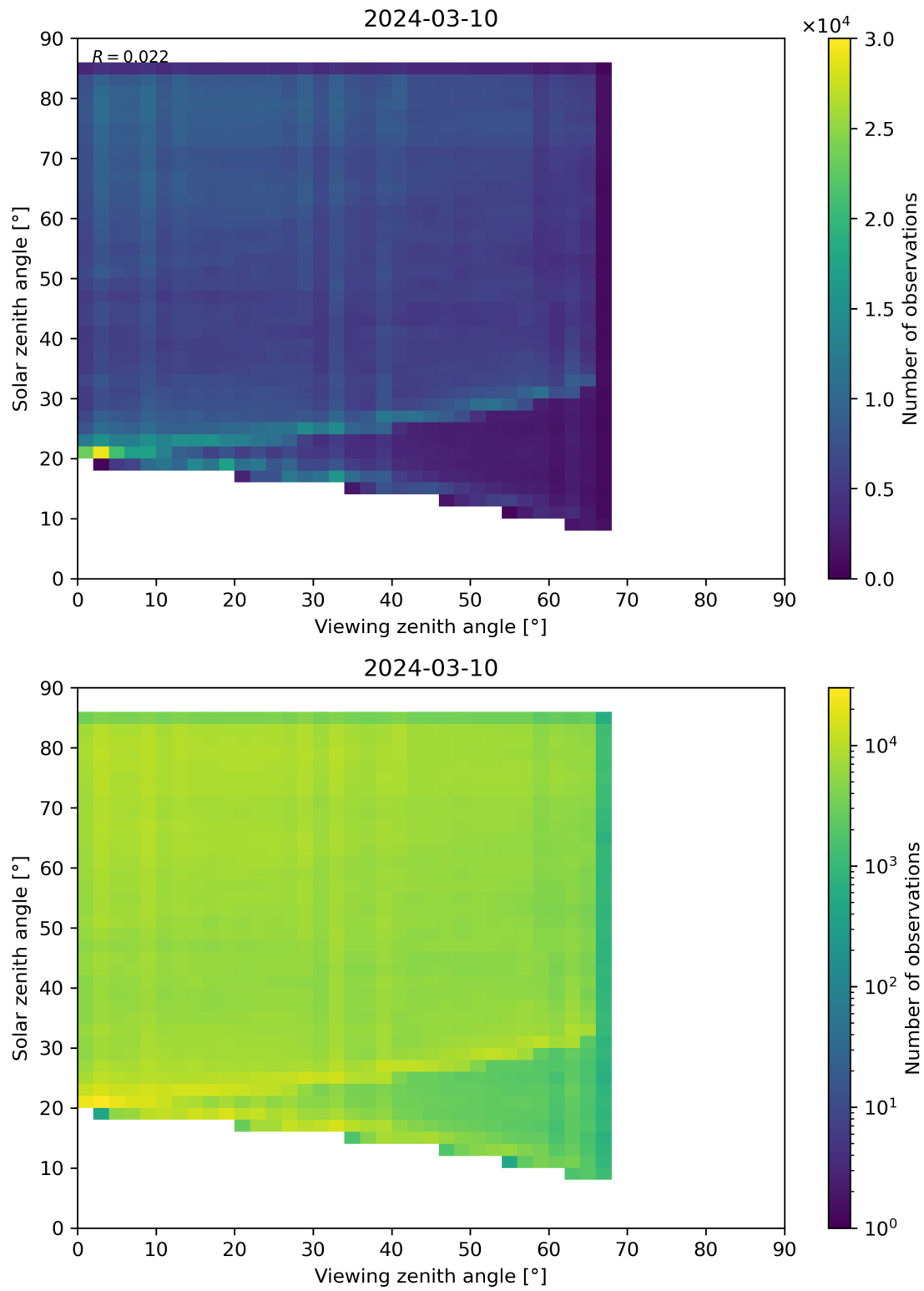
Figure 77: Scatter density plot of “Viewing zenith angle” against “Solar zenith angle” for 2024-03-09 to 2024-03-11.
