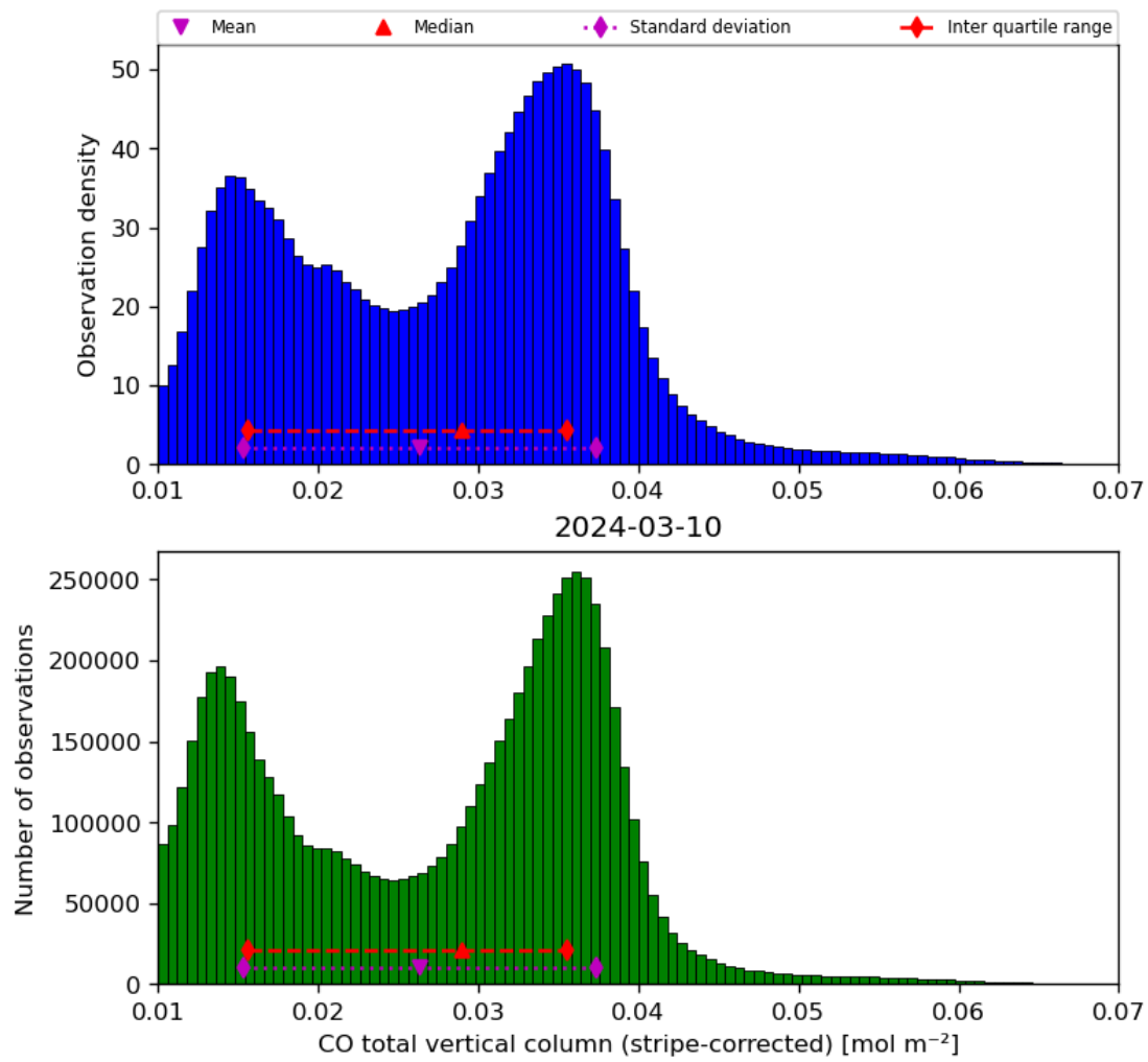
Figure 19: Histogram of “CO total vertical column (stripe-corrected)” for 2024-03-09 to 2024-03-11
