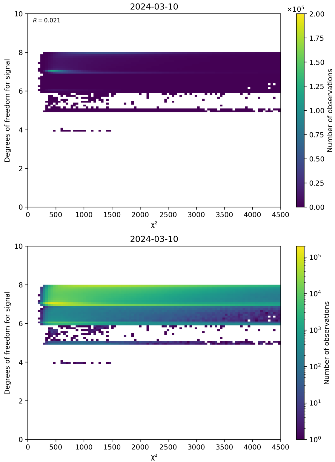
Figure 48: Scatter density plot of " \chi^2 " against "Degrees of freedom for signal" for 2024-03-09 to 2024-03-11.
