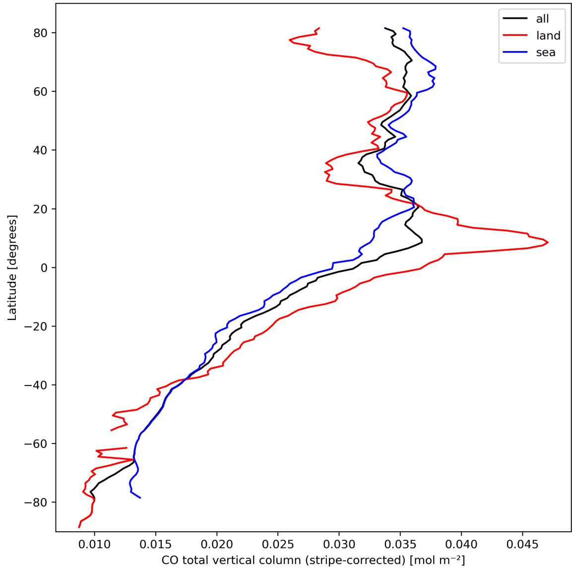
Figure 11: Zonal average of “CO total vertical column (stripe-corrected)” for 2024-03-09 to 2024-03-11.
