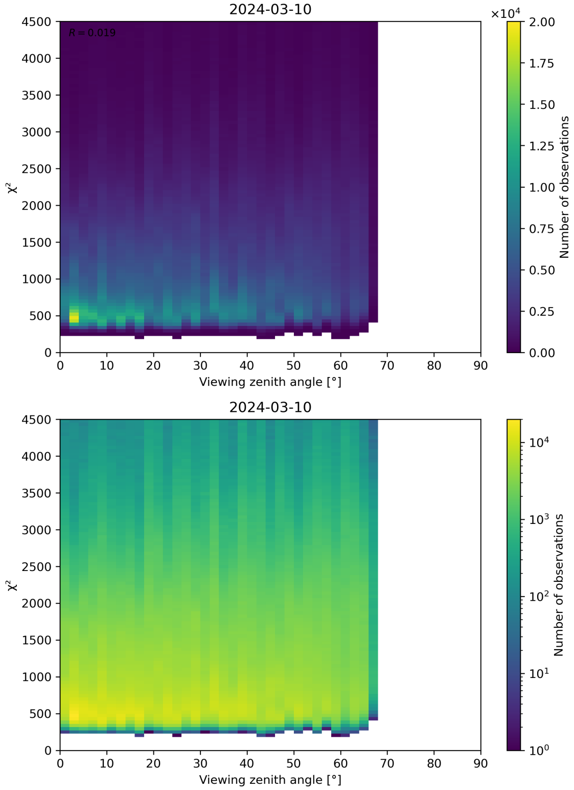
Figure 72: Scatter density plot of “Viewing zenith angle” against “ \chi^2 ” for 2024-03-09 to 2024-03-11.
