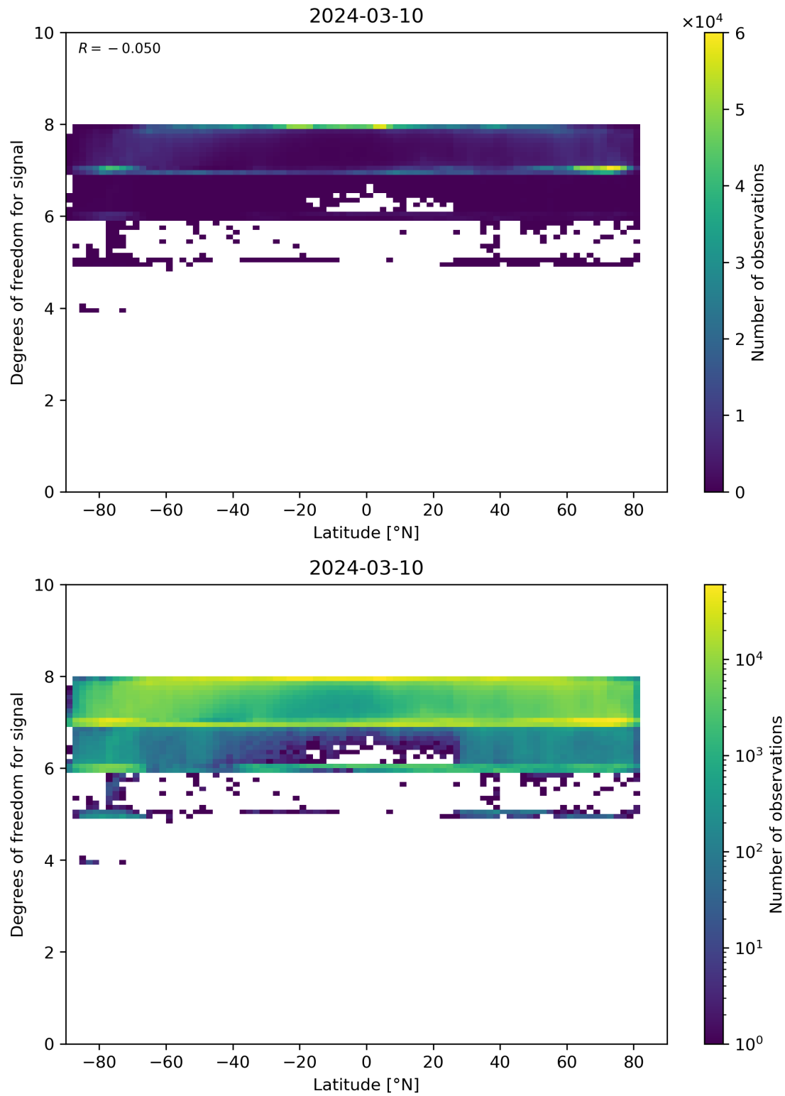
Figure 55: Scatter density plot of “Latitude” against “Degrees of freedom for signal” for 2024-03-09 to 2024-03-11.
