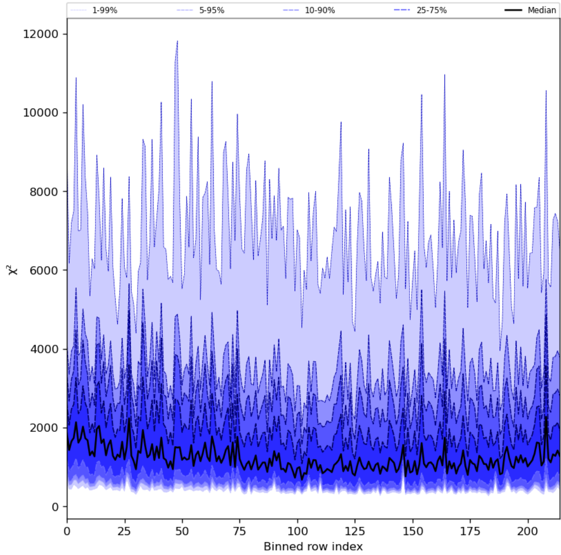
Figure 30: Along track statistics of “ \chi^2 ” for 2024-03-09 to 2024-03-11
