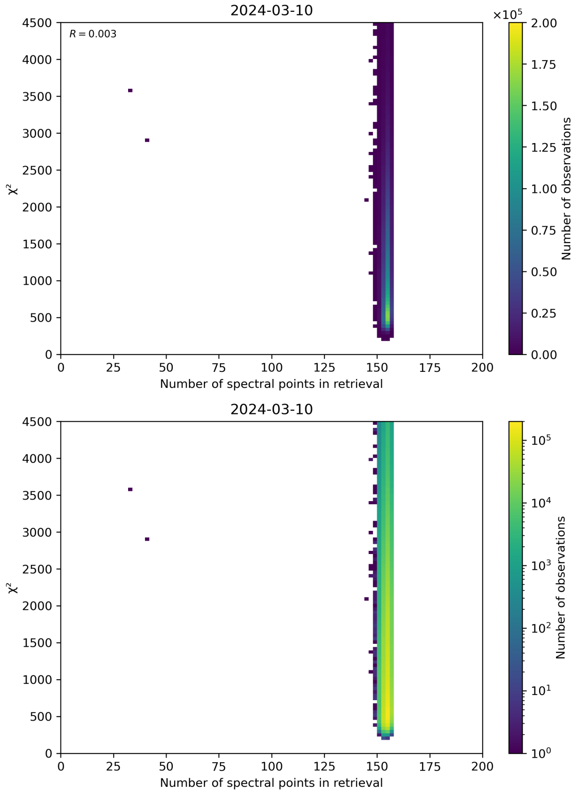
Figure 58: Scatter density plot of “Number of spectral points in retrieval” against “ \chi^2 ” for 2024-03-09 to 2024-03-11.
