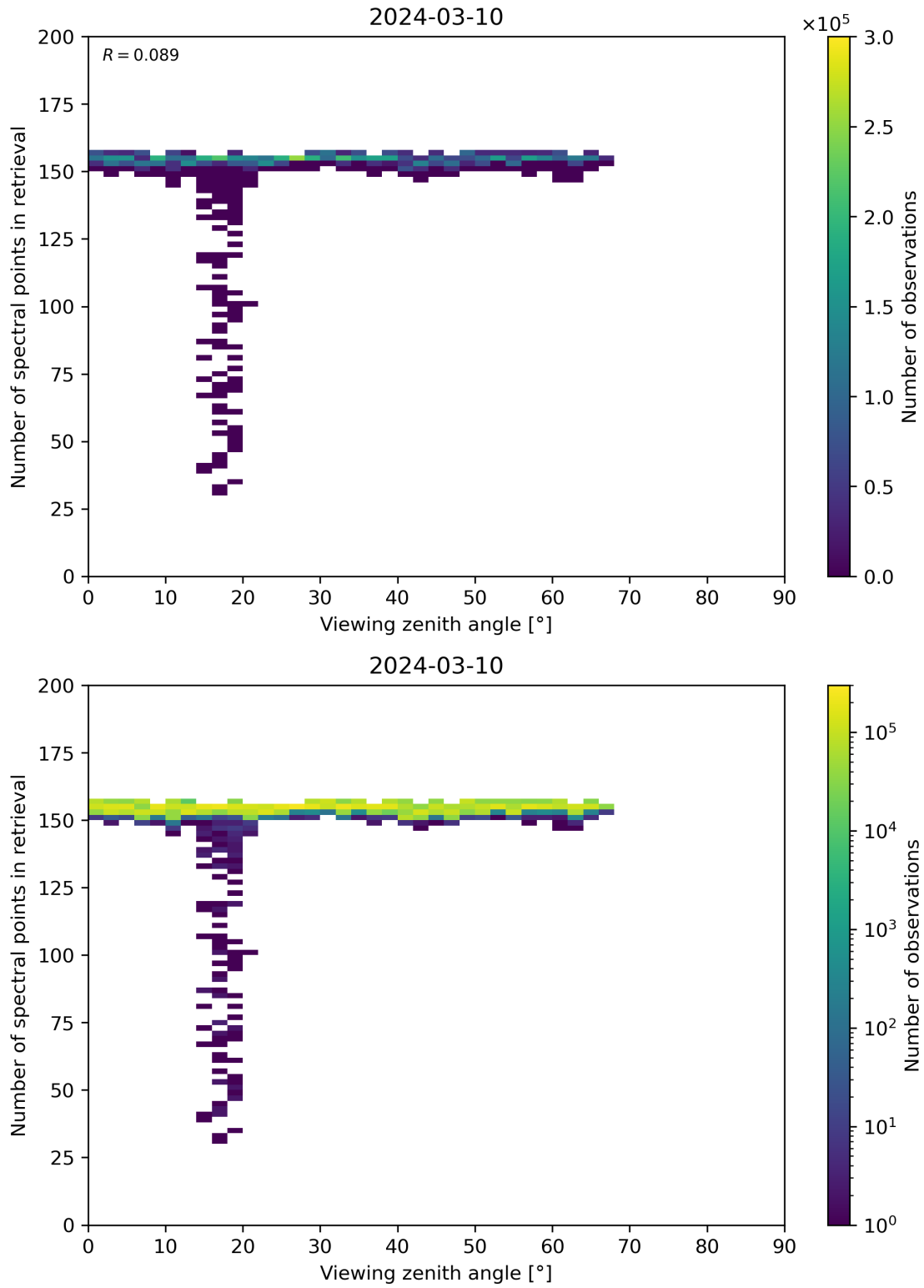
Figure 76: Scatter density plot of “Viewing zenith angle” against “Number of spectral points in retrieval” for 2024-03-09 to 2024-03-11.
