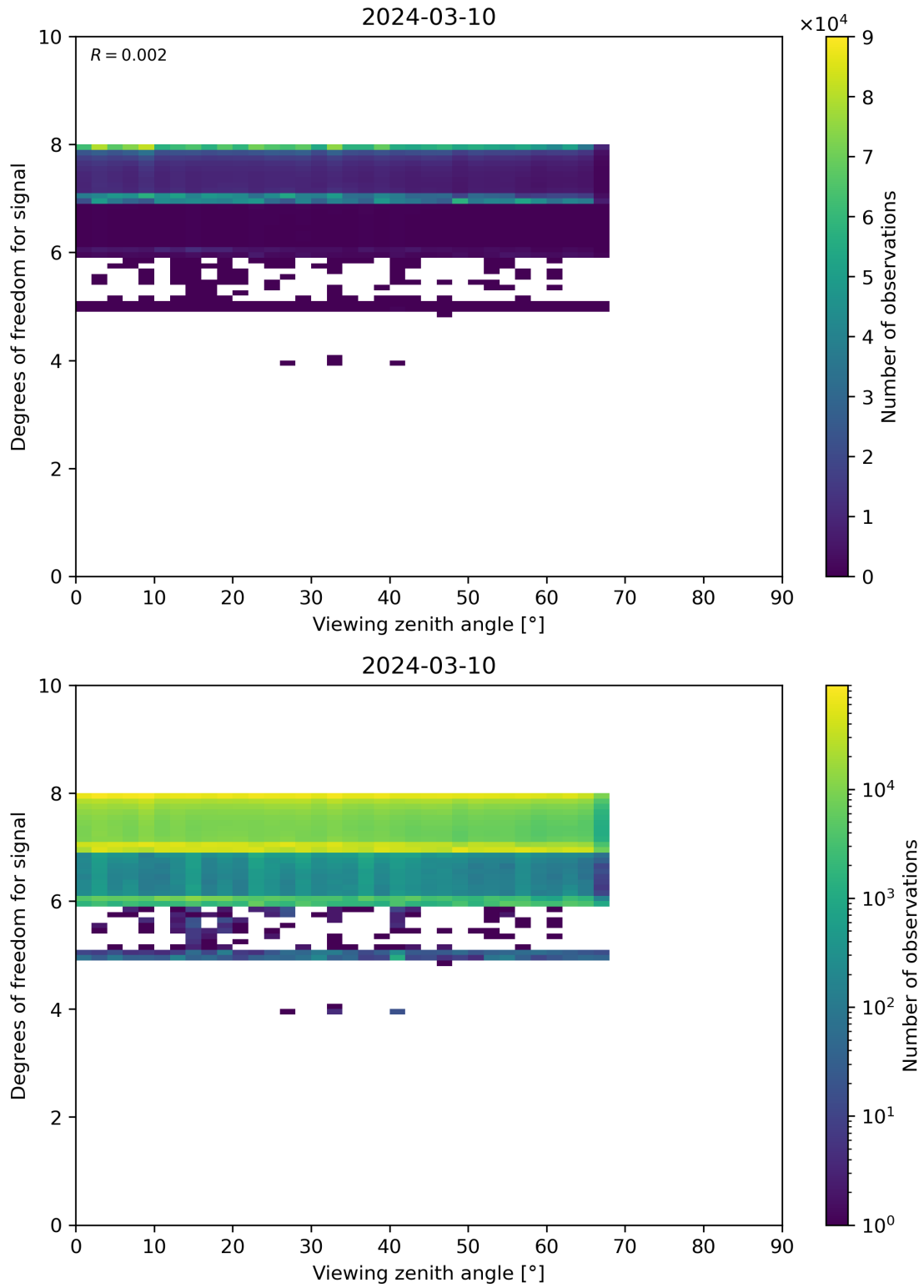
Figure 73: Scatter density plot of “Viewing zenith angle” against “Degrees of freedom for signal” for 2024-03-09 to 2024-03-11.
