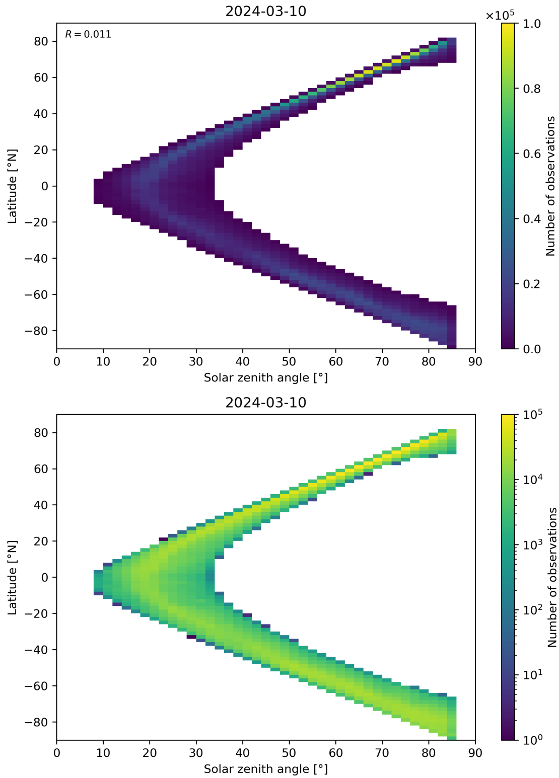
Figure 66: Scatter density plot of “Solar zenith angle” against “Latitude” for 2024-03-09 to 2024-03-11.
