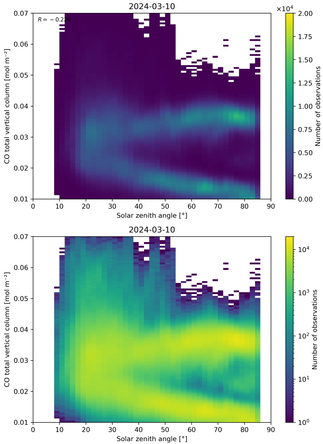
Figure 61: Scatter density plot of “Solar zenith angle” against “CO total vertical column” for 2024-03-09 to 2024-03-11.
