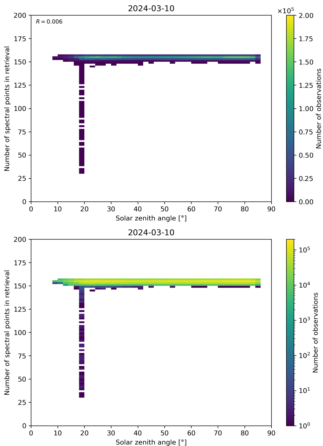
Figure 68: Scatter density plot of “Solar zenith angle” against “Number of spectral points in retrieval” for 2024-03-09 to 2024-03-11.
