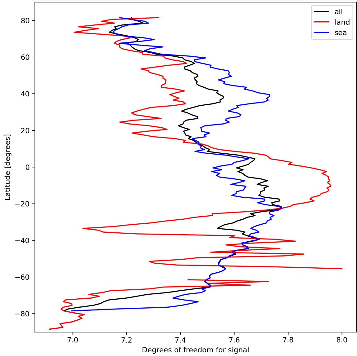
Figure 15: Zonal average of “Degrees of freedom for signal” for 2024-03-09 to 2024-03-11.
