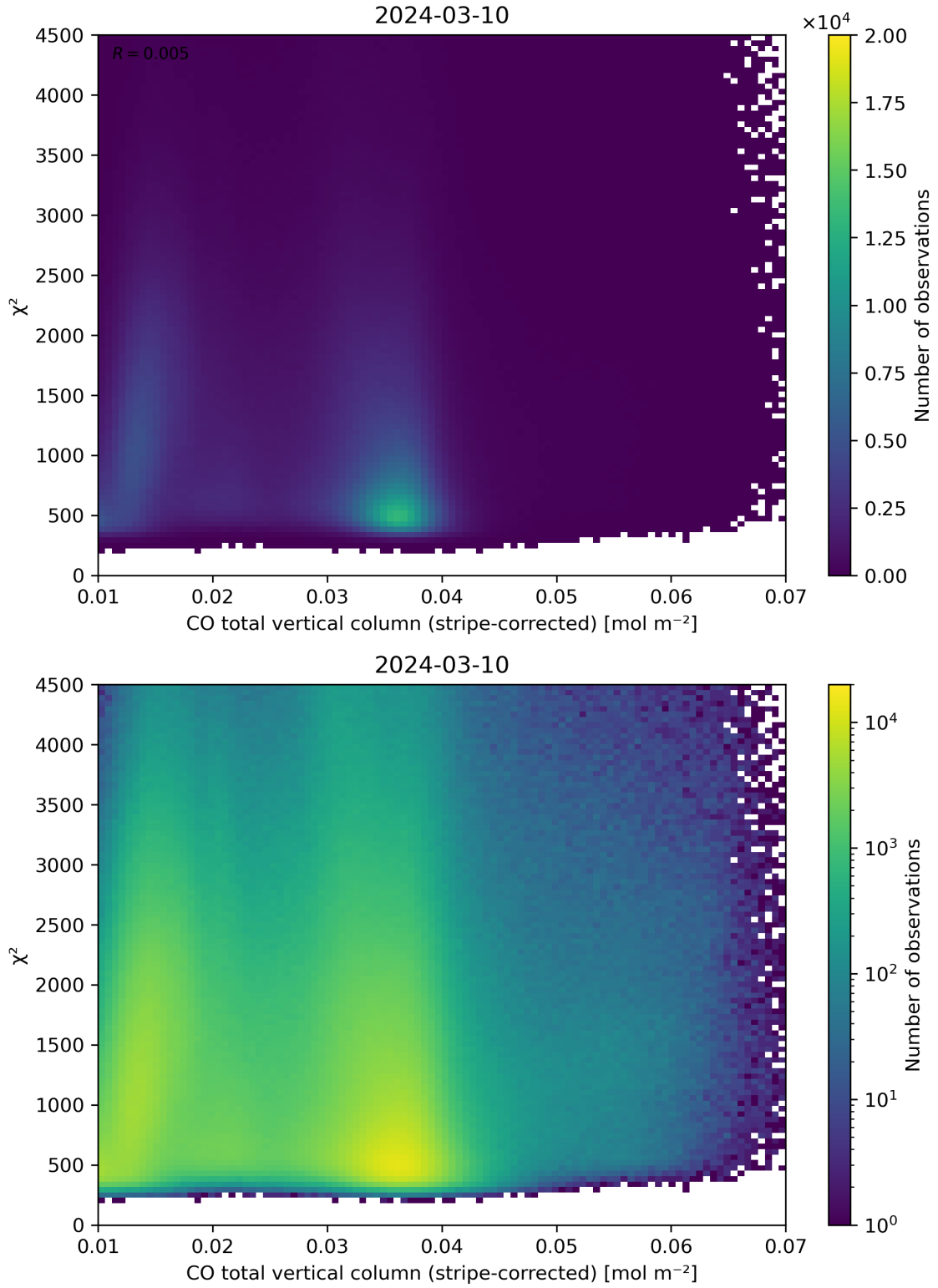
Figure 37: Scatter density plot of “CO total vertical column (stripe-corrected)” against “ \chi^2 ” for 2024-03-09 to 2024-03-11.
