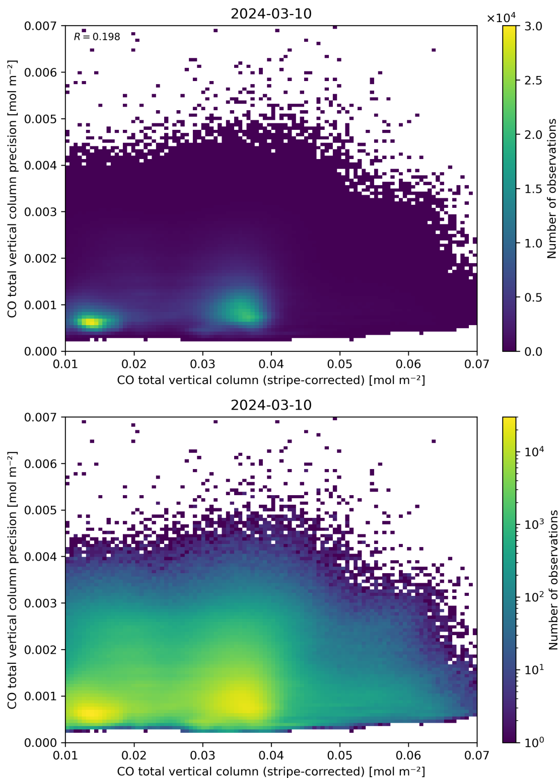
Figure 36: Scatter density plot of “CO total vertical column (stripe-corrected)” against “CO total vertical column precision” for 2024-03-09 to 2024-03-11.
