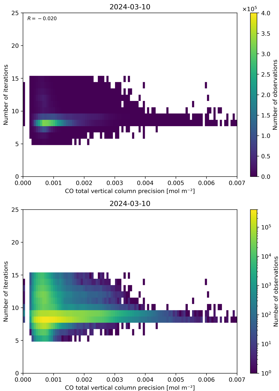
Figure 46: Scatter density plot of “CO total vertical column precision” against “Number of iterations” for 2024-03-09 to 2024-03-11.
