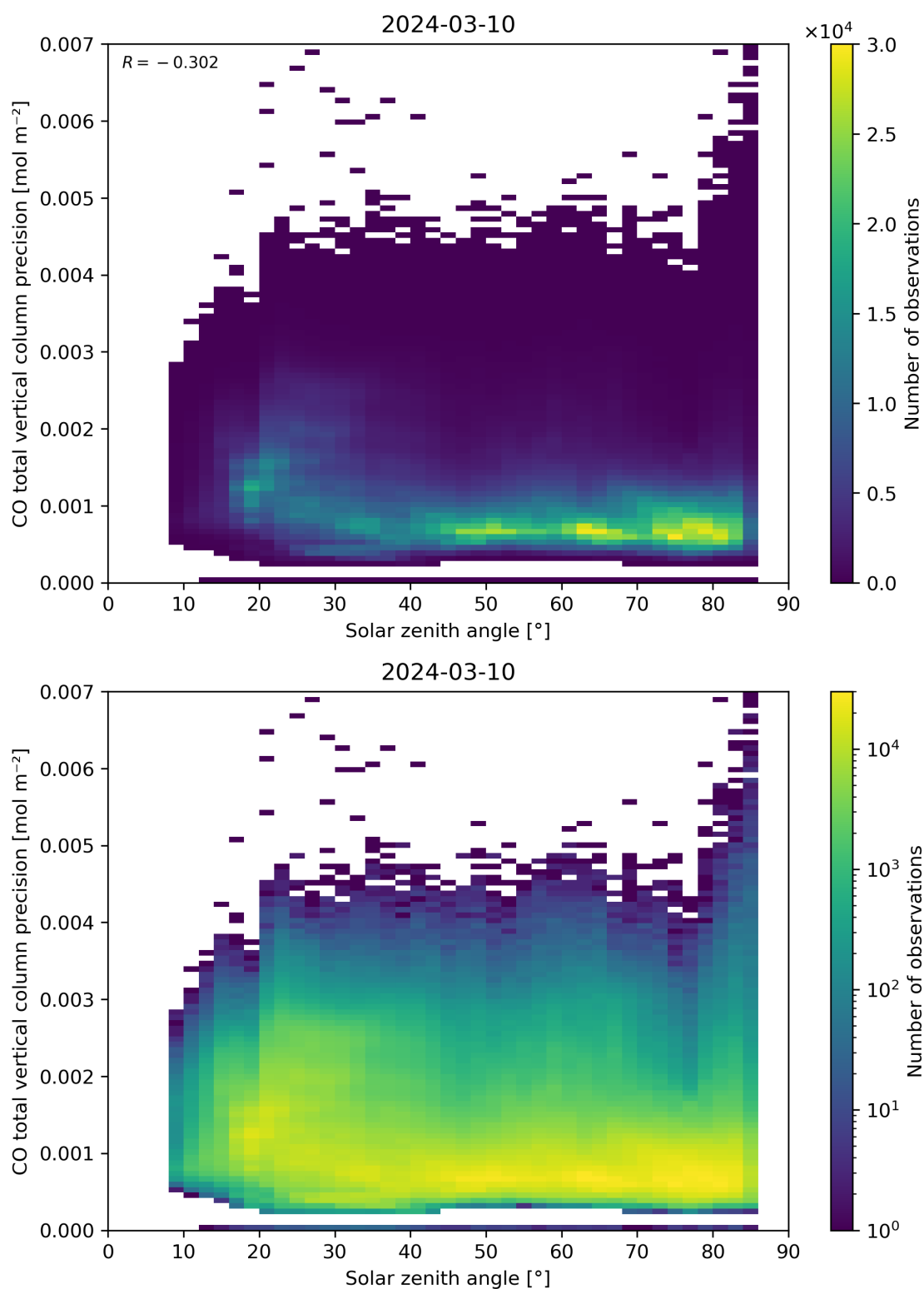
Figure 63: Scatter density plot of “Solar zenith angle” against “CO total vertical column precision” for 2024-03-09 to 2024-03-11.
