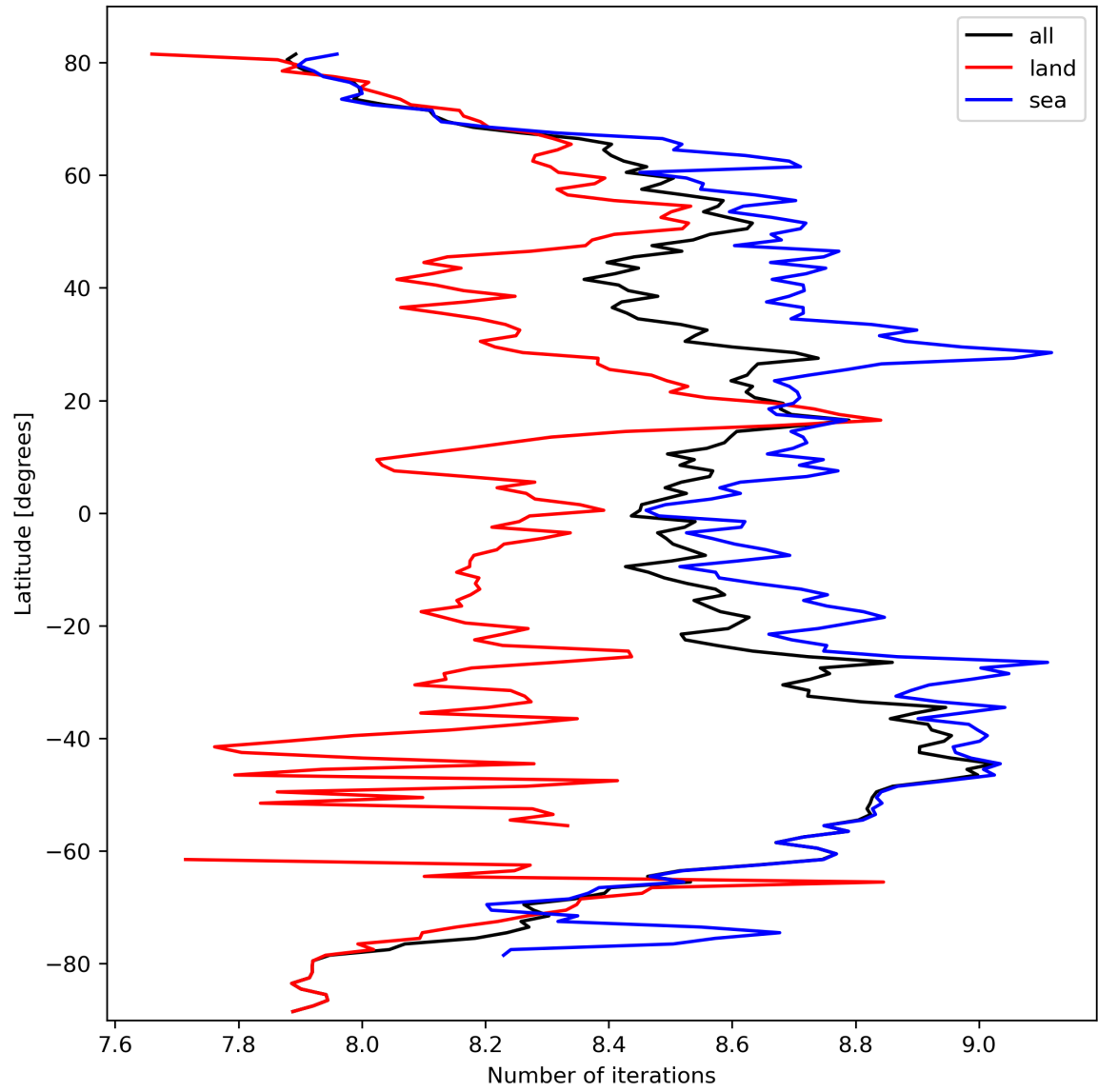
Figure 16: Zonal average of “Number of iterations” for 2024-03-09 to 2024-03-11.
