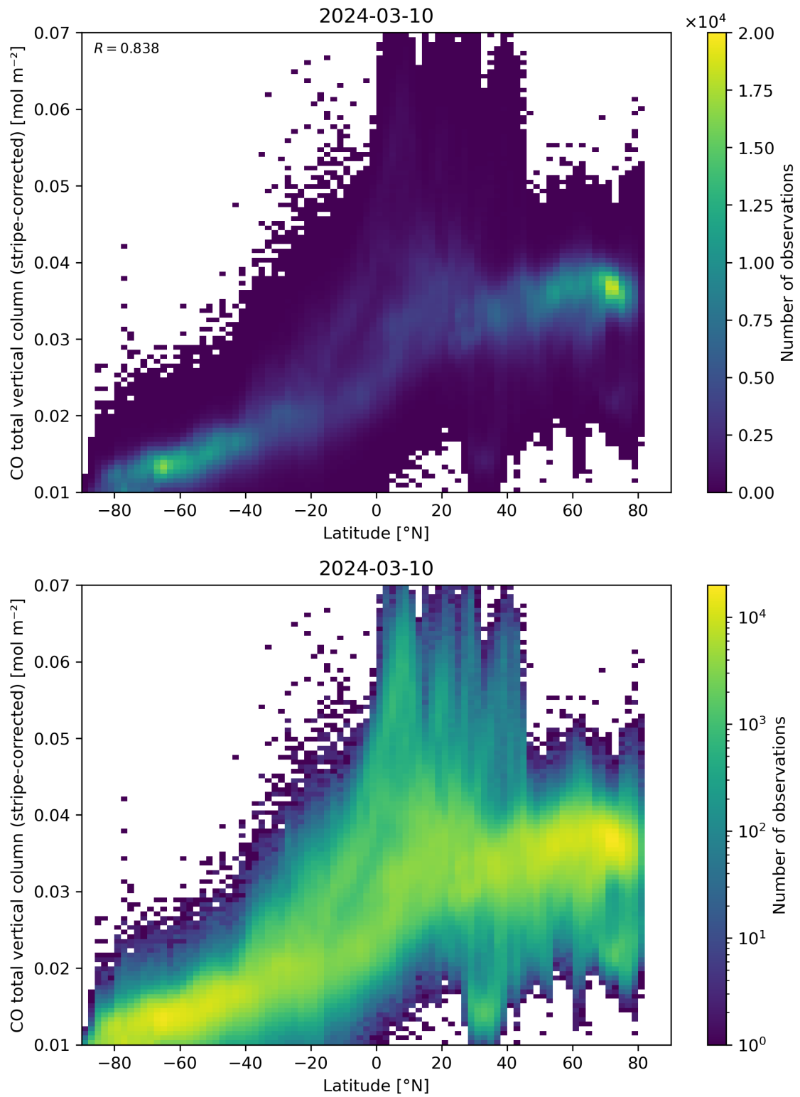
Figure 52: Scatter density plot of “Latitude” against “CO total vertical column (stripe-corrected)” for 2024-03-09 to 2024-03-11.
