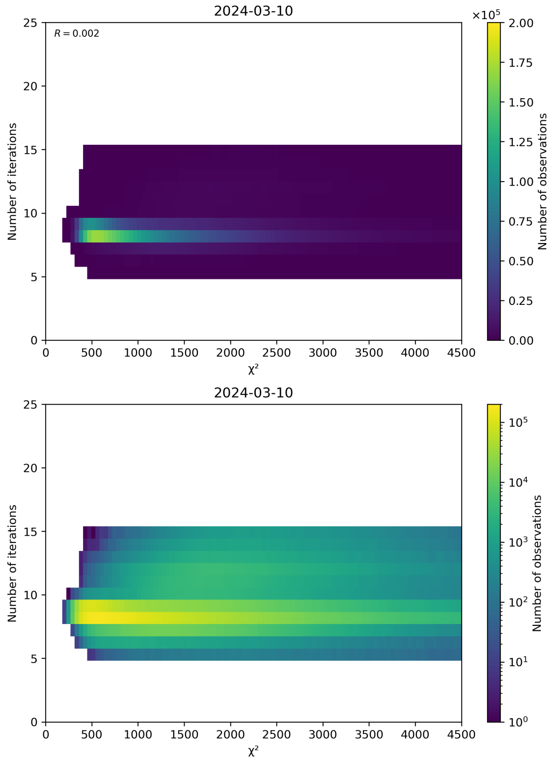
Figure 49: Scatter density plot of “ \chi^2 ” against “Number of iterations” for 2024-03-09 to 2024-03-11.
