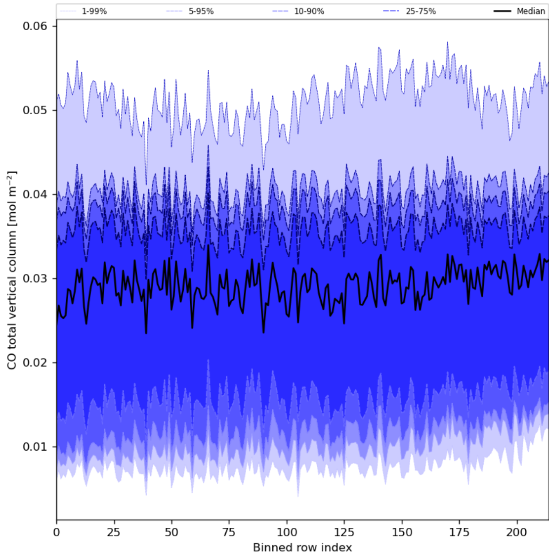
Figure 26: Along track statistics of “CO total vertical column” for 2024-03-09 to 2024-03-11
