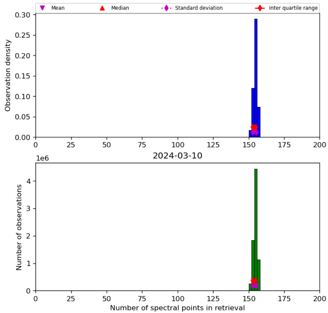
Figure 21: Histogram of “Number of spectral points in retrieval” for 2024-03-09 to 2024-03-11
