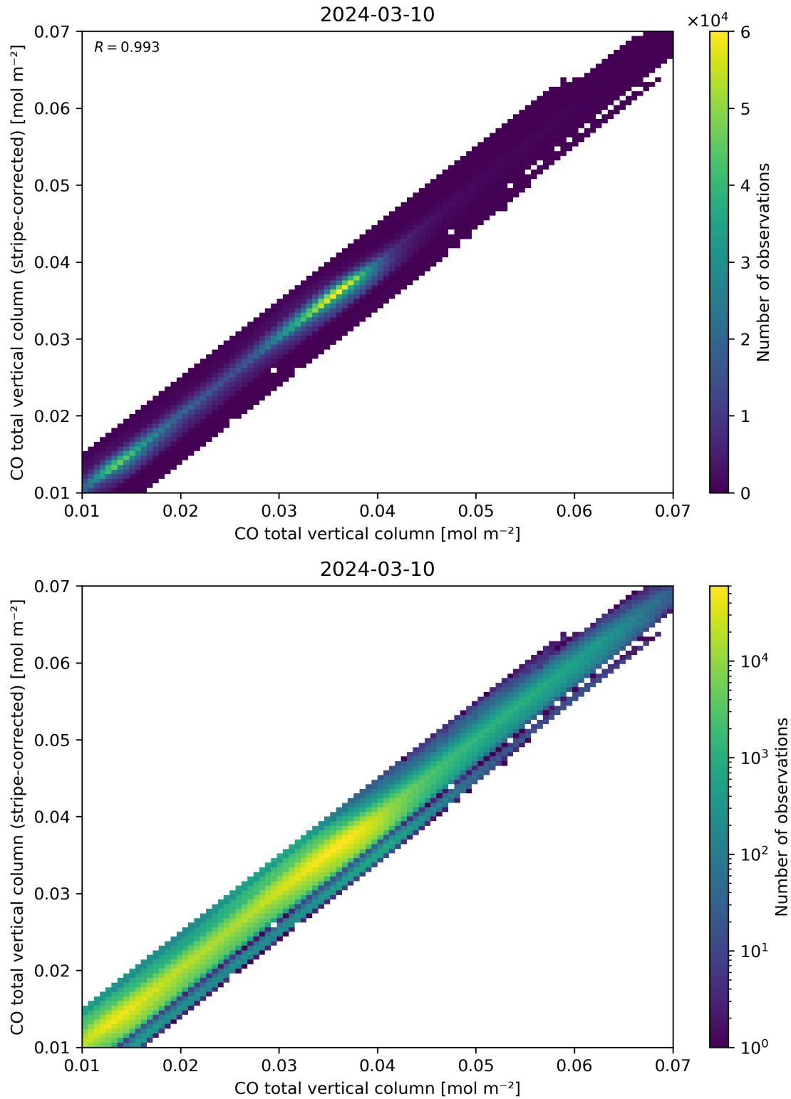
Figure 33: Scatter density plot of “CO total vertical column” against “CO total vertical column (stripe-corrected)” for 2024-03-09 to 2024-03-11.
