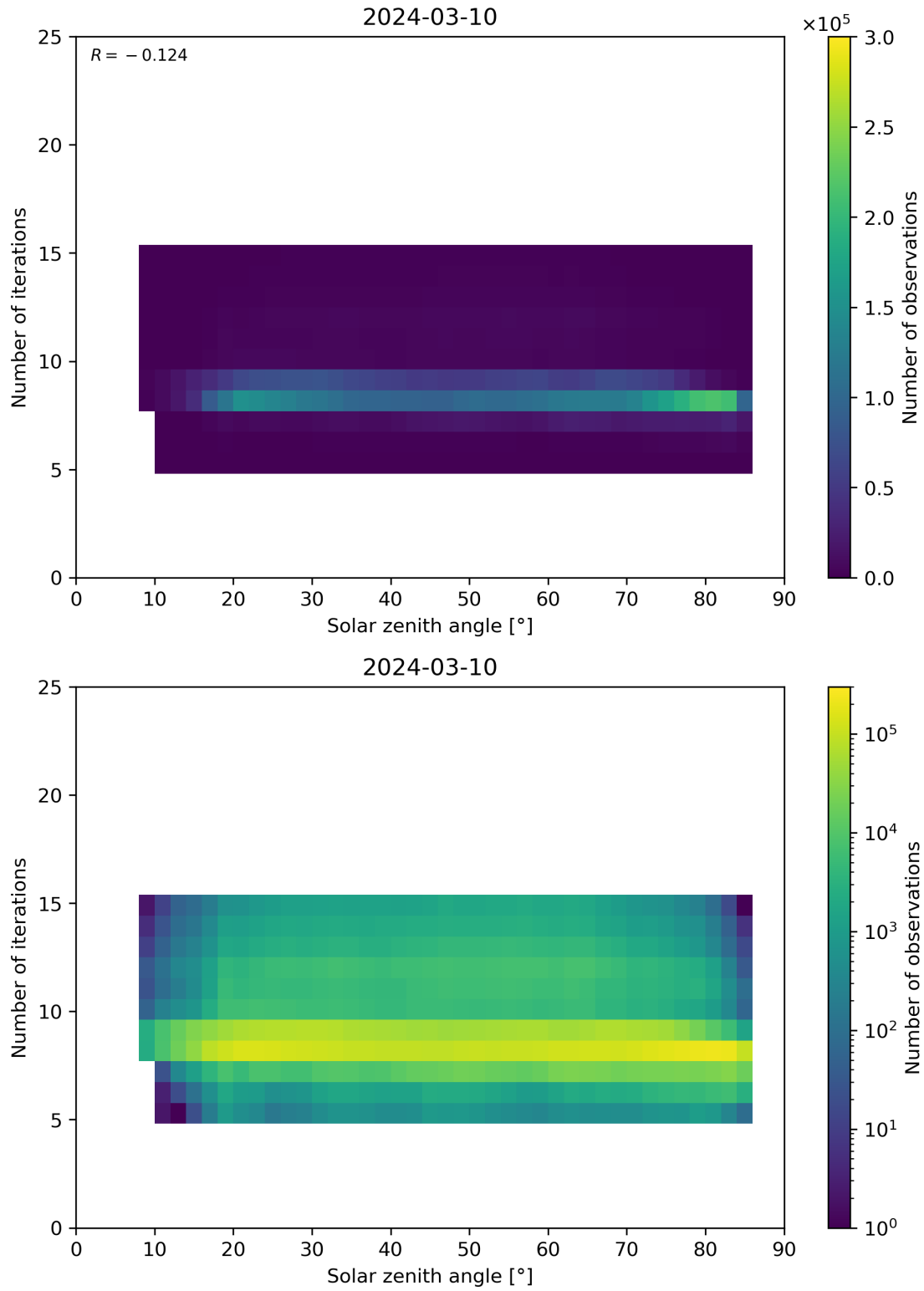
Figure 67: Scatter density plot of “Solar zenith angle” against “Number of iterations” for 2024-03-09 to 2024-03-11.
