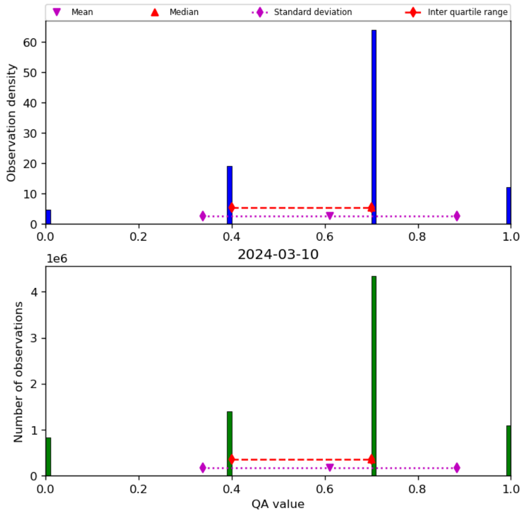
Figure 17: Histogram of “QA value” for 2024-03-09 to 2024-03-11
