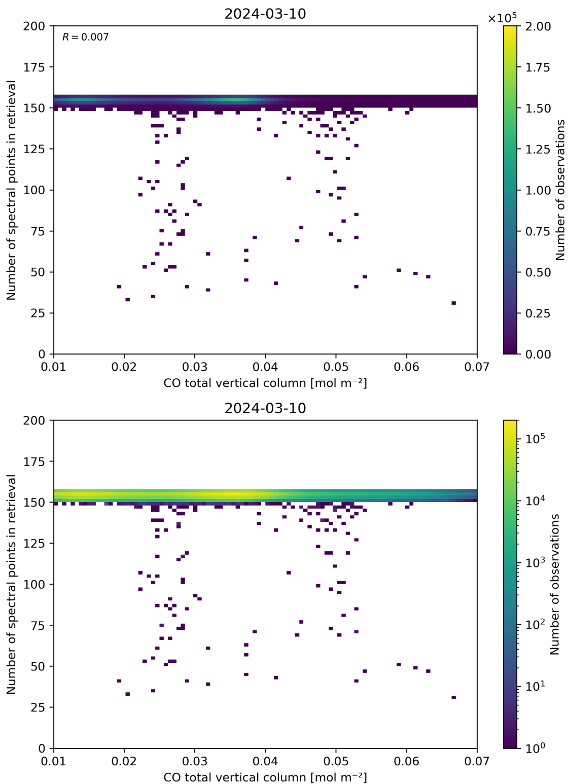
Figure 43: Scatter density plot of “CO total vertical column” against “Number of spectral points in retrieval” for 2024-03-09 to 2024-03-11.
