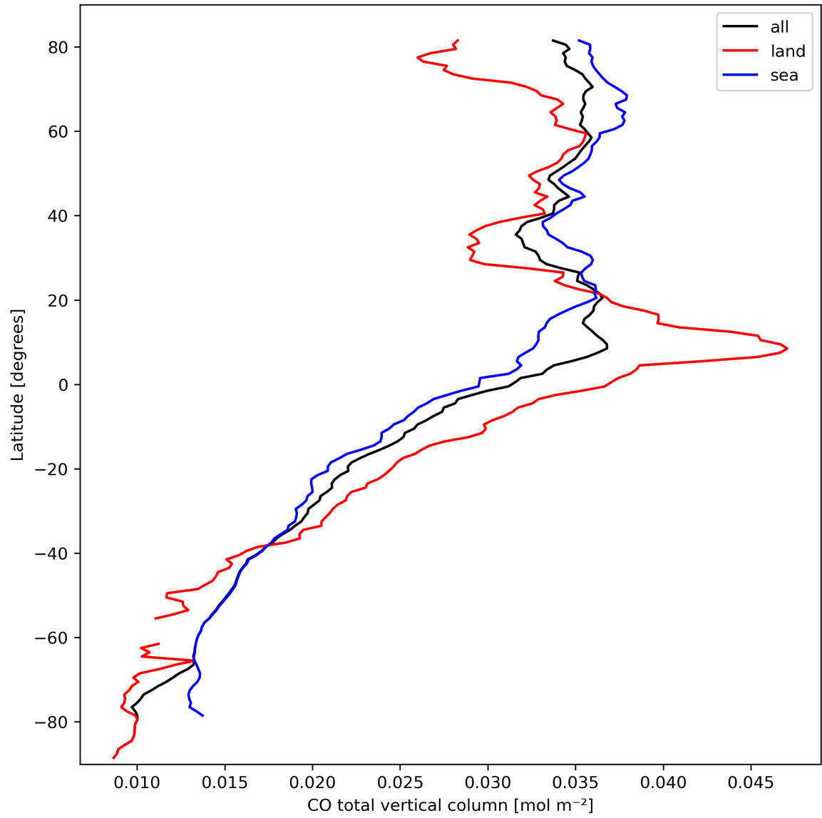
Figure 10: Zonal average of “CO total vertical column” for 2024-03-09 to 2024-03-11.
