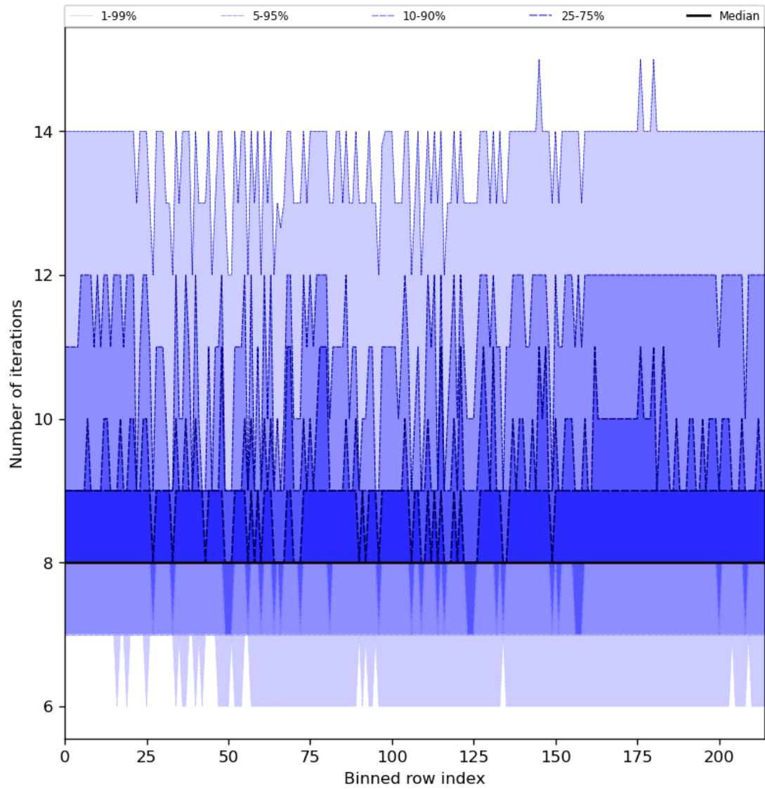
Figure 32: Along track statistics of “Number of iterations” for 2024-03-09 to 2024-03-11
