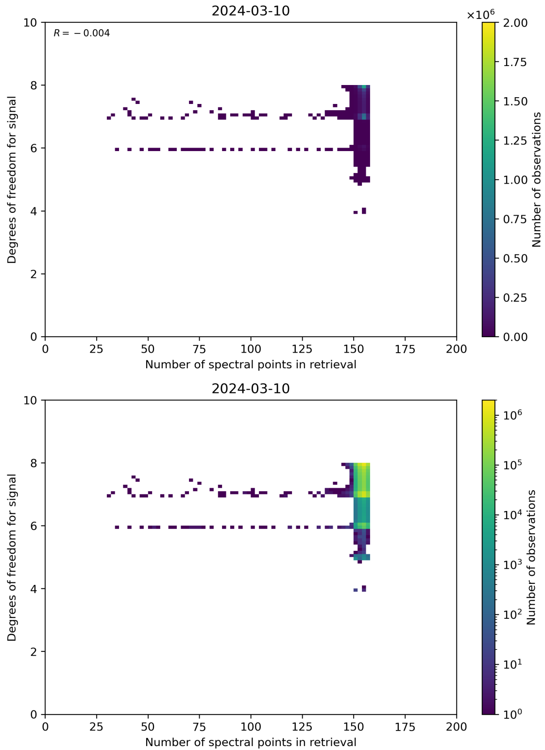
Figure 59: Scatter density plot of “Number of spectral points in retrieval” against “Degrees of freedom for signal” for 2024-03-09 to 2024-03-11.
