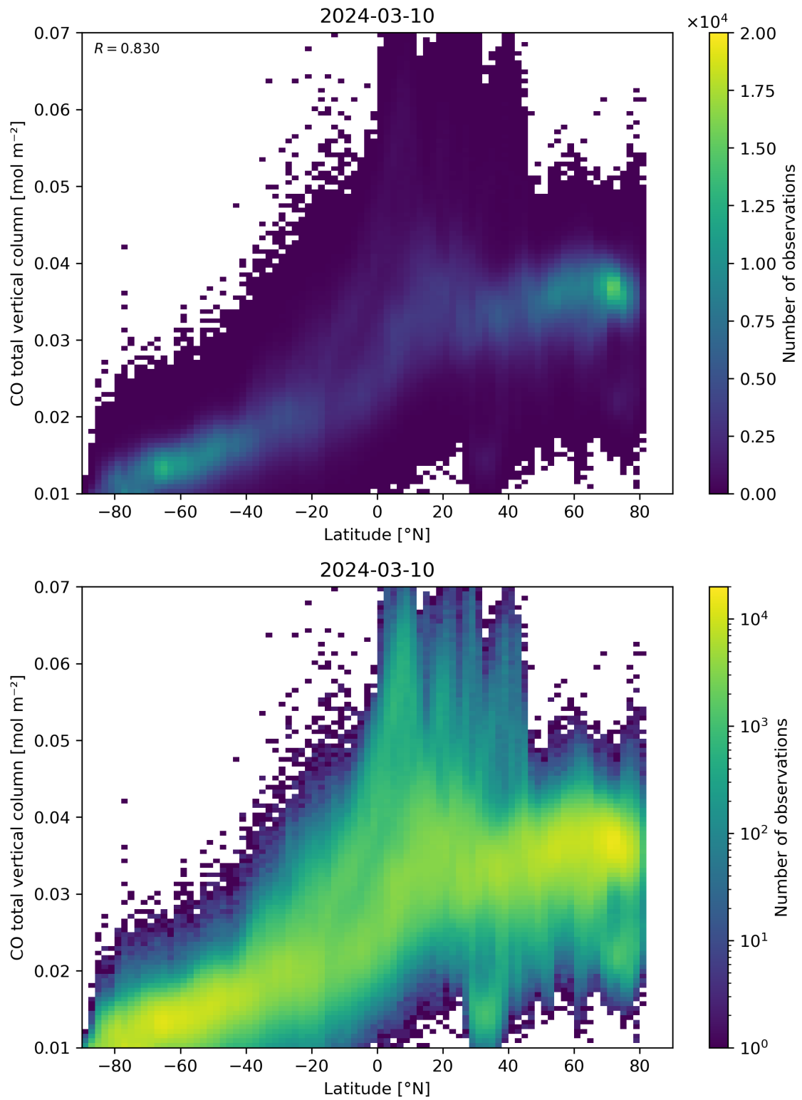
Figure 51: Scatter density plot of “Latitude” against “CO total vertical column” for 2024-03-09 to 2024-03-11.
