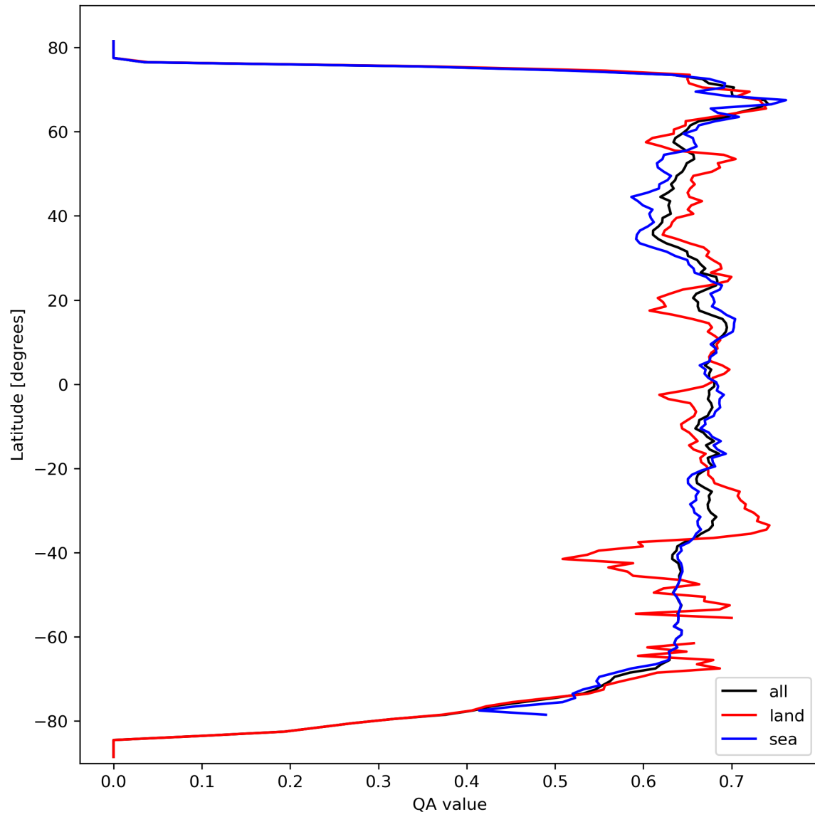
Figure 9: Zonal average of “QA value” for 2024-03-09 to 2024-03-11.
