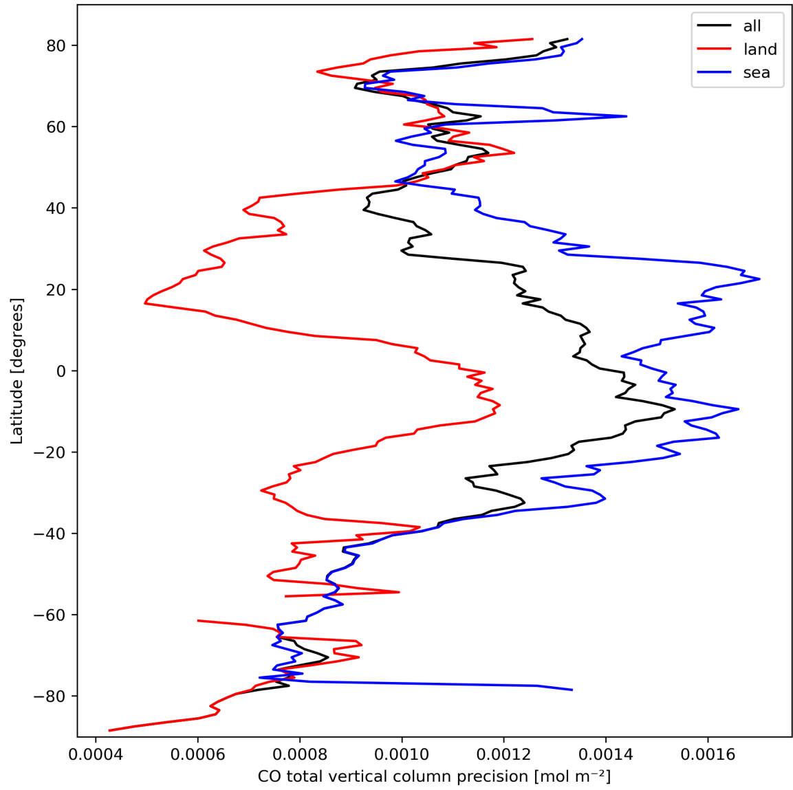
Figure 12: Zonal average of “CO total vertical column precision” for 2024-03-09 to 2024-03-11.
