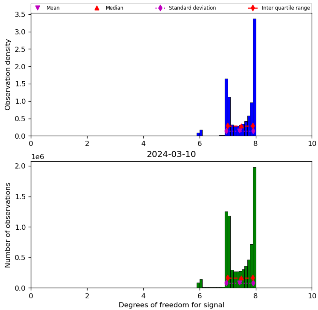
Figure 23: Histogram of “Degrees of freedom for signal” for 2024-03-09 to 2024-03-11
