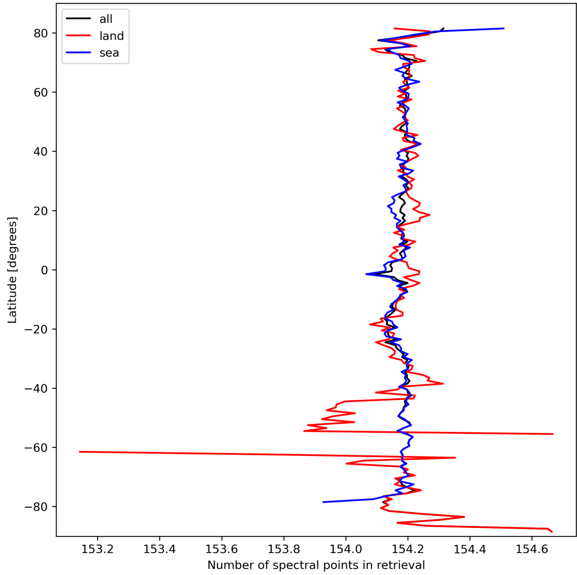
Figure 13: Zonal average of “Number of spectral points in retrieval” for 2024-03-09 to 2024-03-11.
