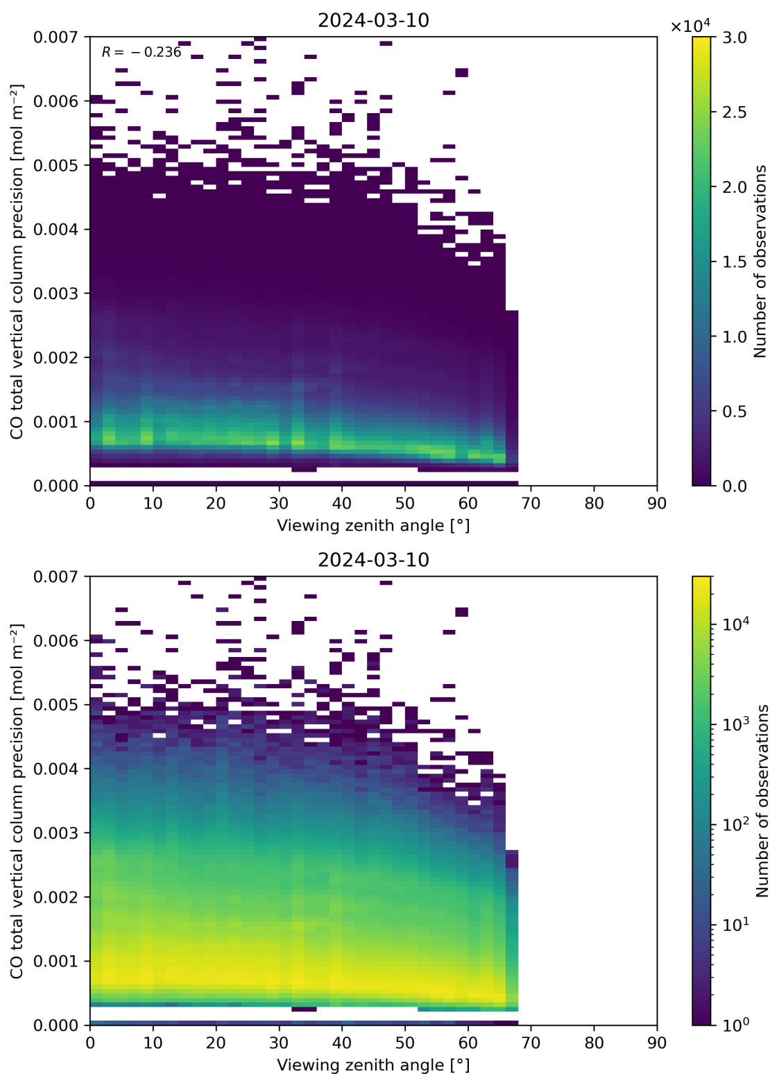
Figure 71: Scatter density plot of “Viewing zenith angle” against “CO total vertical column precision” for 2024-03-09 to 2024-03-11.
