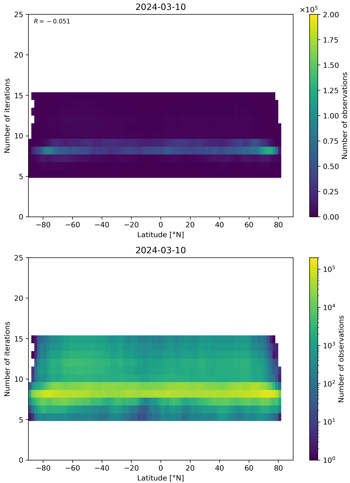
Figure 56: Scatter density plot of “Latitude” against “Number of iterations” for 2024-03-09 to 2024-03-11.
