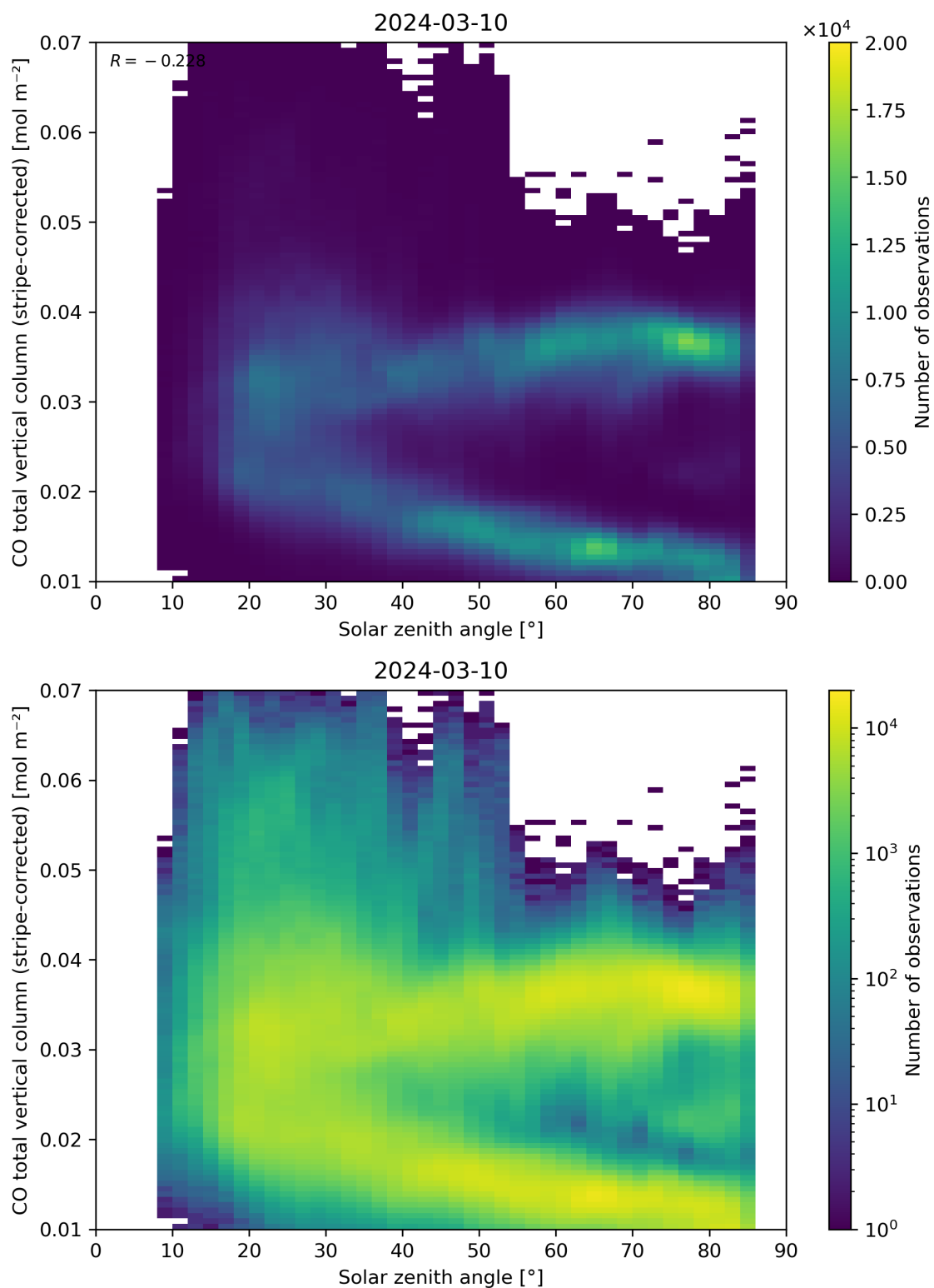
Figure 62: Scatter density plot of “Solar zenith angle” against “CO total vertical column (stripe-corrected)” for 2024-03-09 to 2024-03-11.
