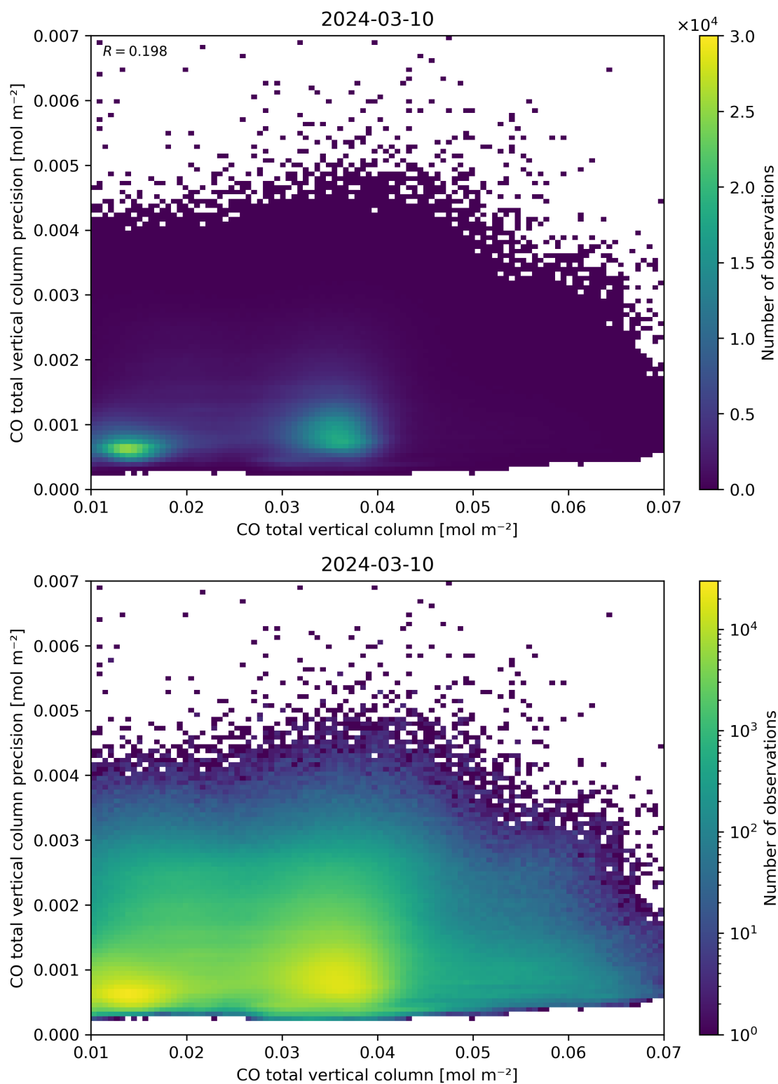
Figure 34: Scatter density plot of “CO total vertical column” against “CO total vertical column precision” for 2024-03-09 to 2024-03-11.
