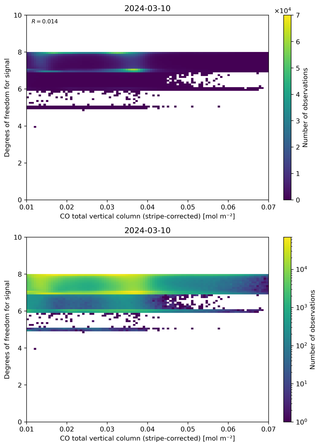
Figure 38: Scatter density plot of “CO total vertical column (stripe-corrected)” against “Degrees of freedom for signal” for 2024-03-09 to 2024-03-11.
