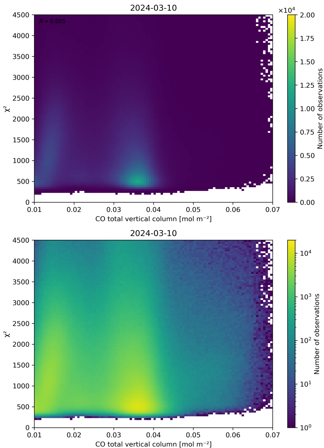
Figure 35: Scatter density plot of “CO total vertical column” against “ \chi^2 ” for 2024-03-09 to 2024-03-11.
