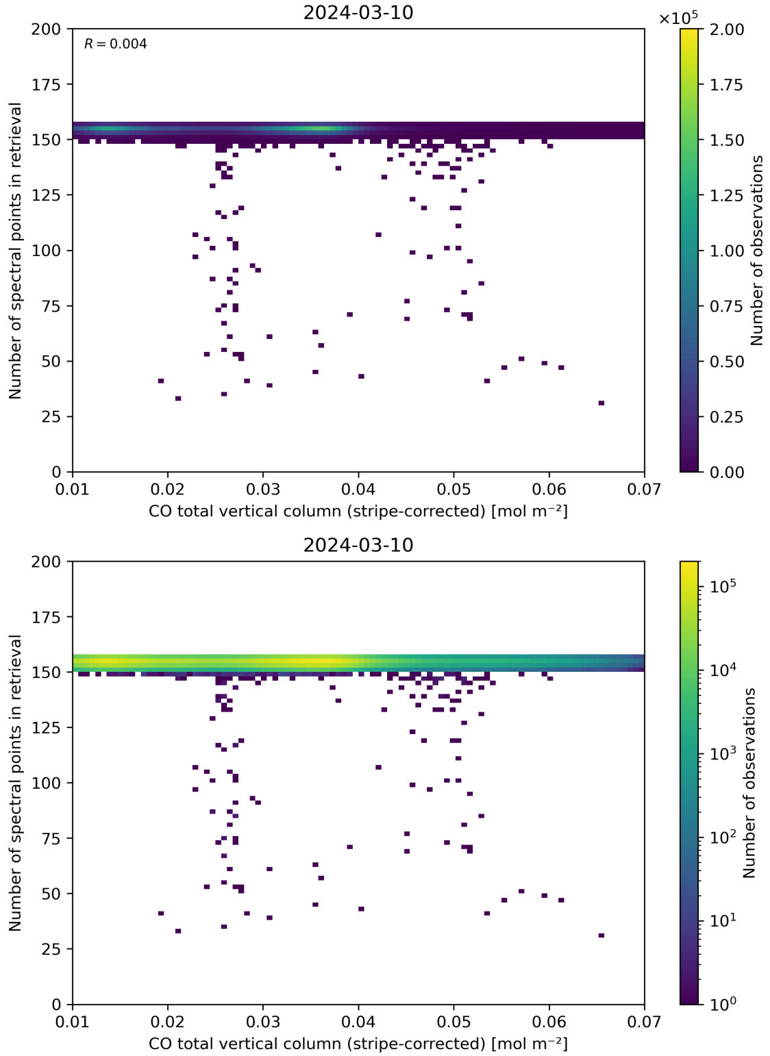
Figure 40: Scatter density plot of “CO total vertical column (stripe-corrected)” against “Number of spectral points in retrieval” for 2024-03-09 to 2024-03-11.
