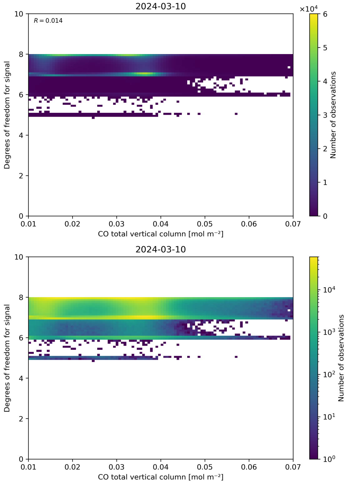
Figure 41: Scatter density plot of “CO total vertical column” against “Degrees of freedom for signal” for 2024-03-09 to 2024-03-11.
