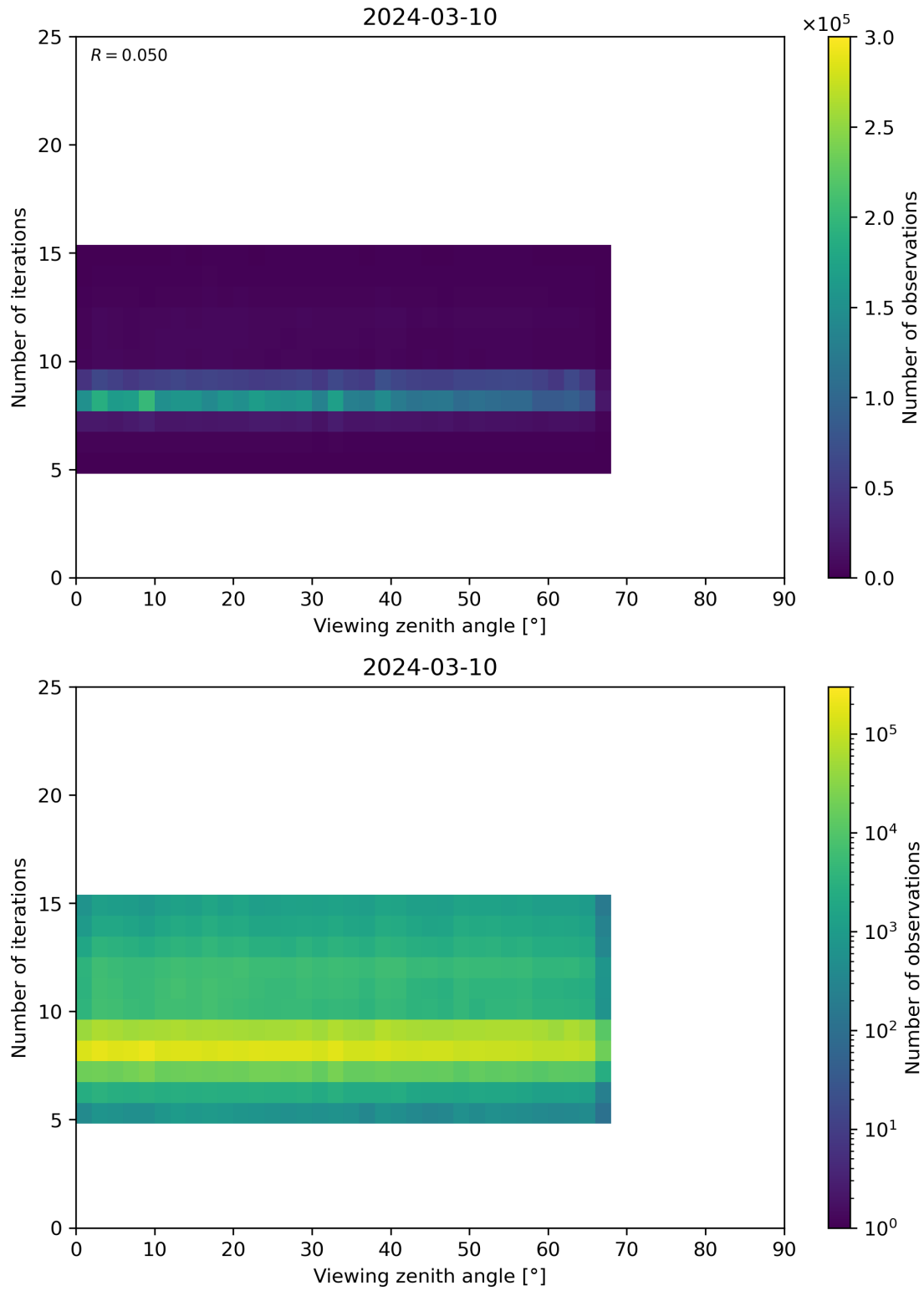
Figure 75: Scatter density plot of “Viewing zenith angle” against “Number of iterations” for 2024-03-09 to 2024-03-11.
