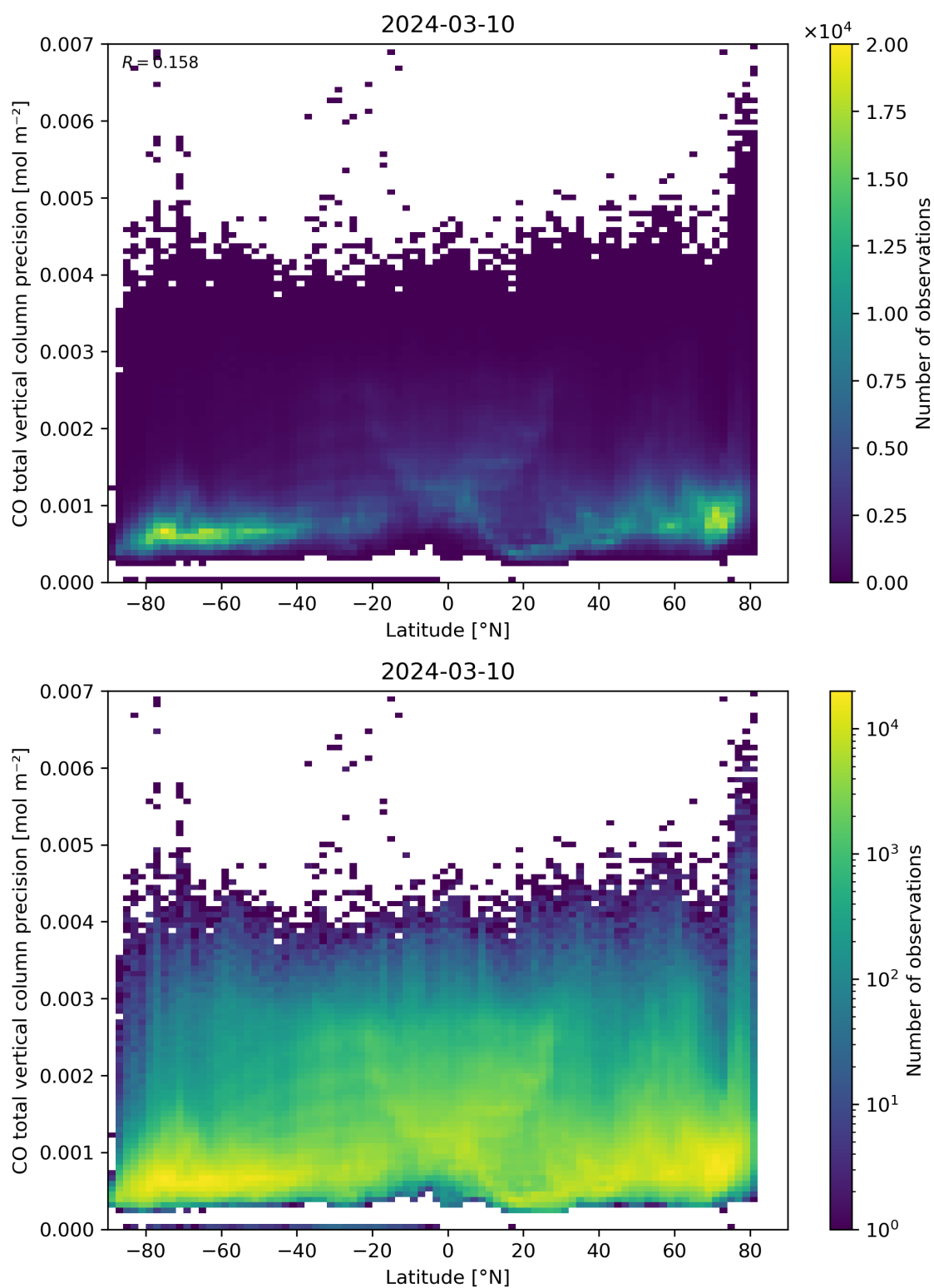
Figure 53: Scatter density plot of “Latitude” against “CO total vertical column precision” for 2024-03-09 to 2024-03-11.
