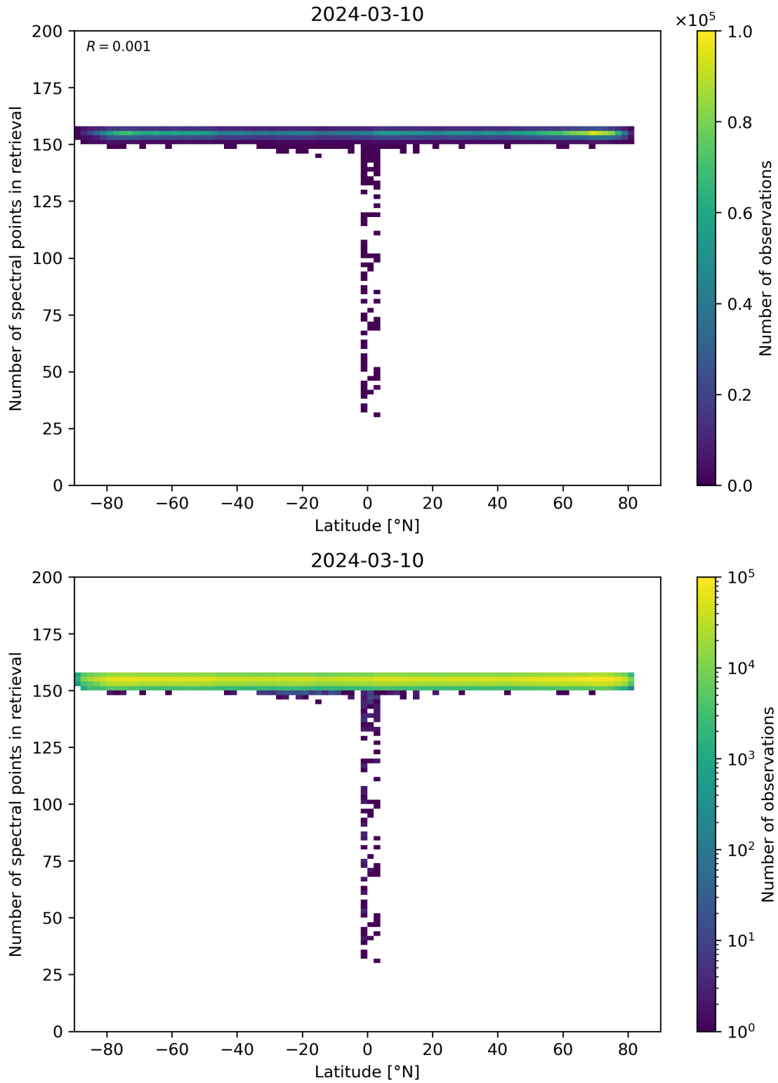
Figure 57: Scatter density plot of “Latitude” against “Number of spectral points in retrieval” for 2024-03-09 to 2024-03-11.
