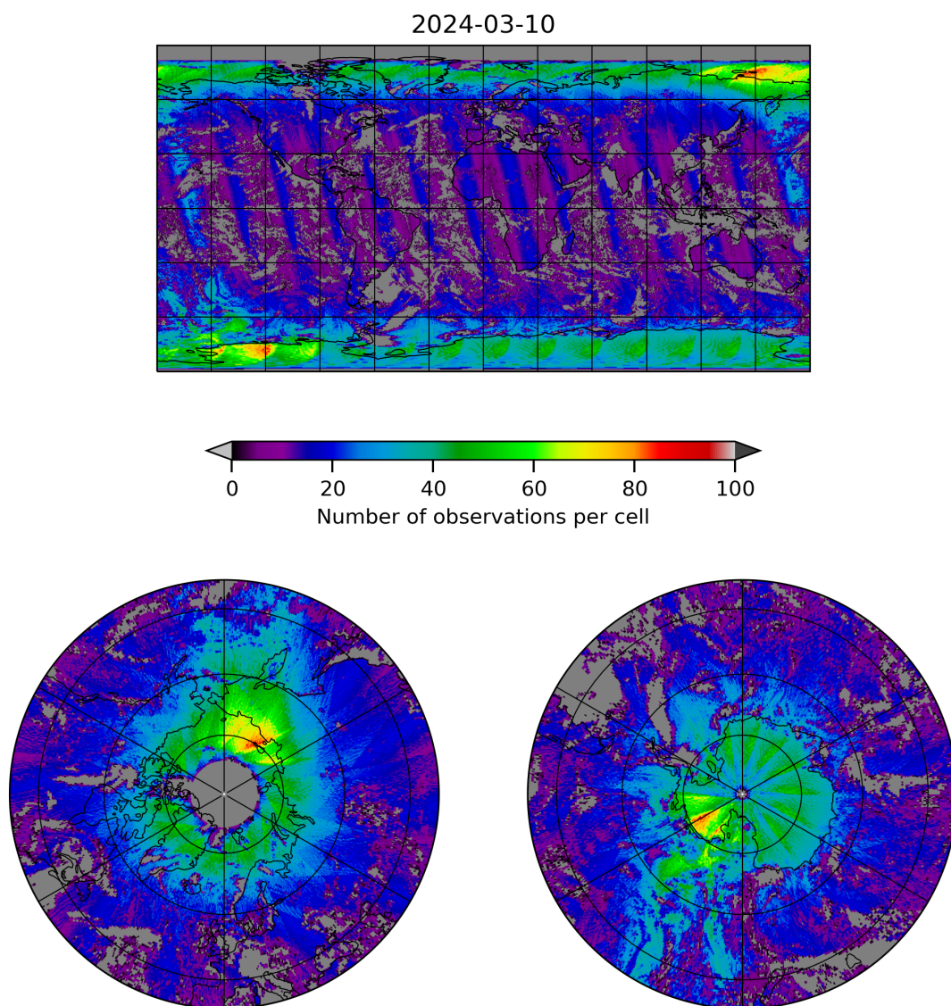
Figure 8: Map of the number of observations for 2024-03-09 to 2024-03-11
