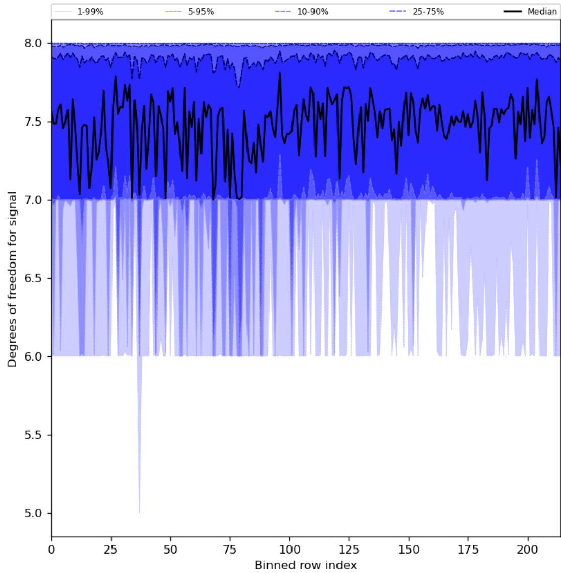
Figure 31: Along track statistics of “Degrees of freedom for signal” for 2024-03-09 to 2024-03-11
