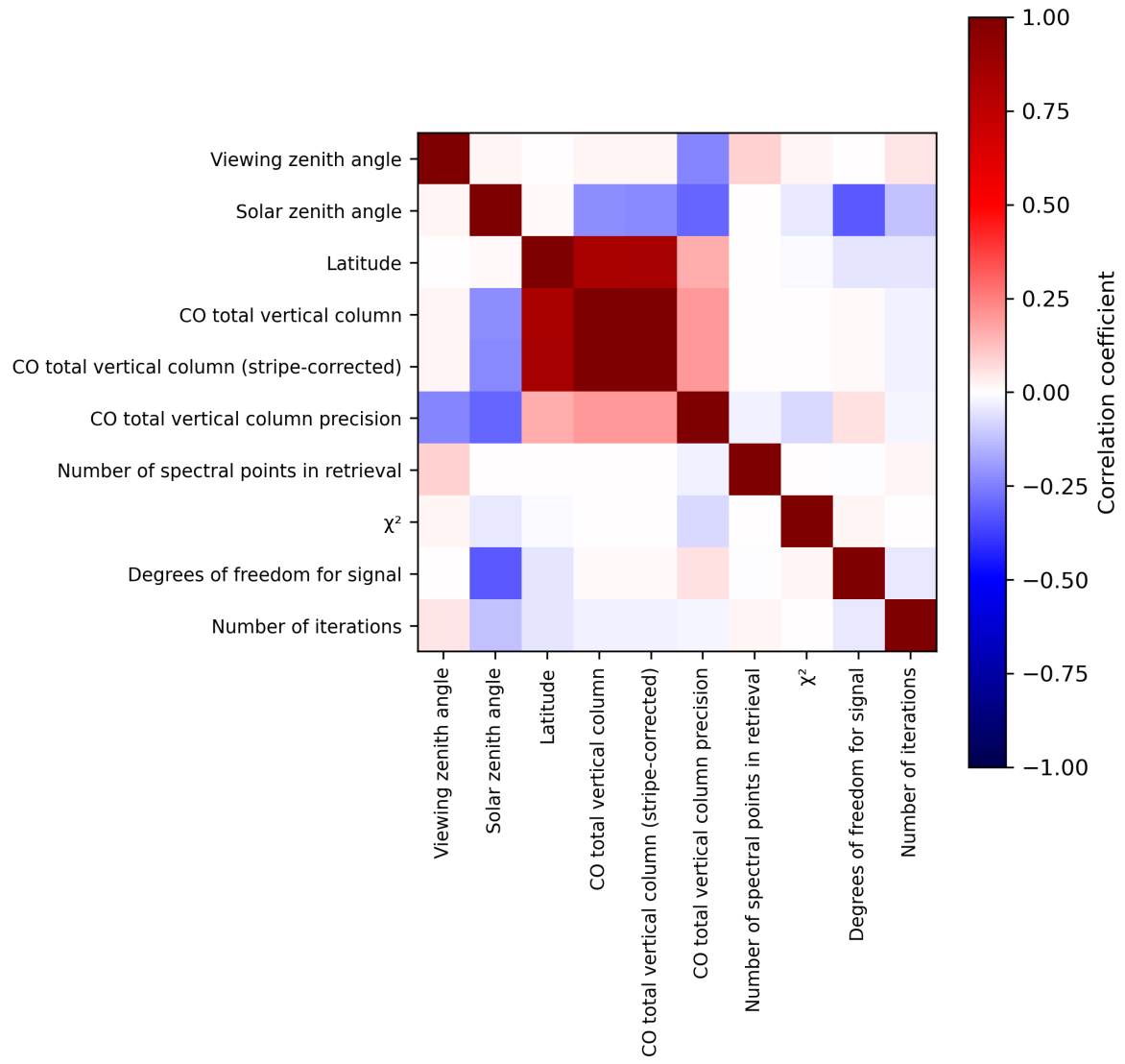
Figure 2: Map of correlation matrix for 2024-03-09 to 2024-03-11.
