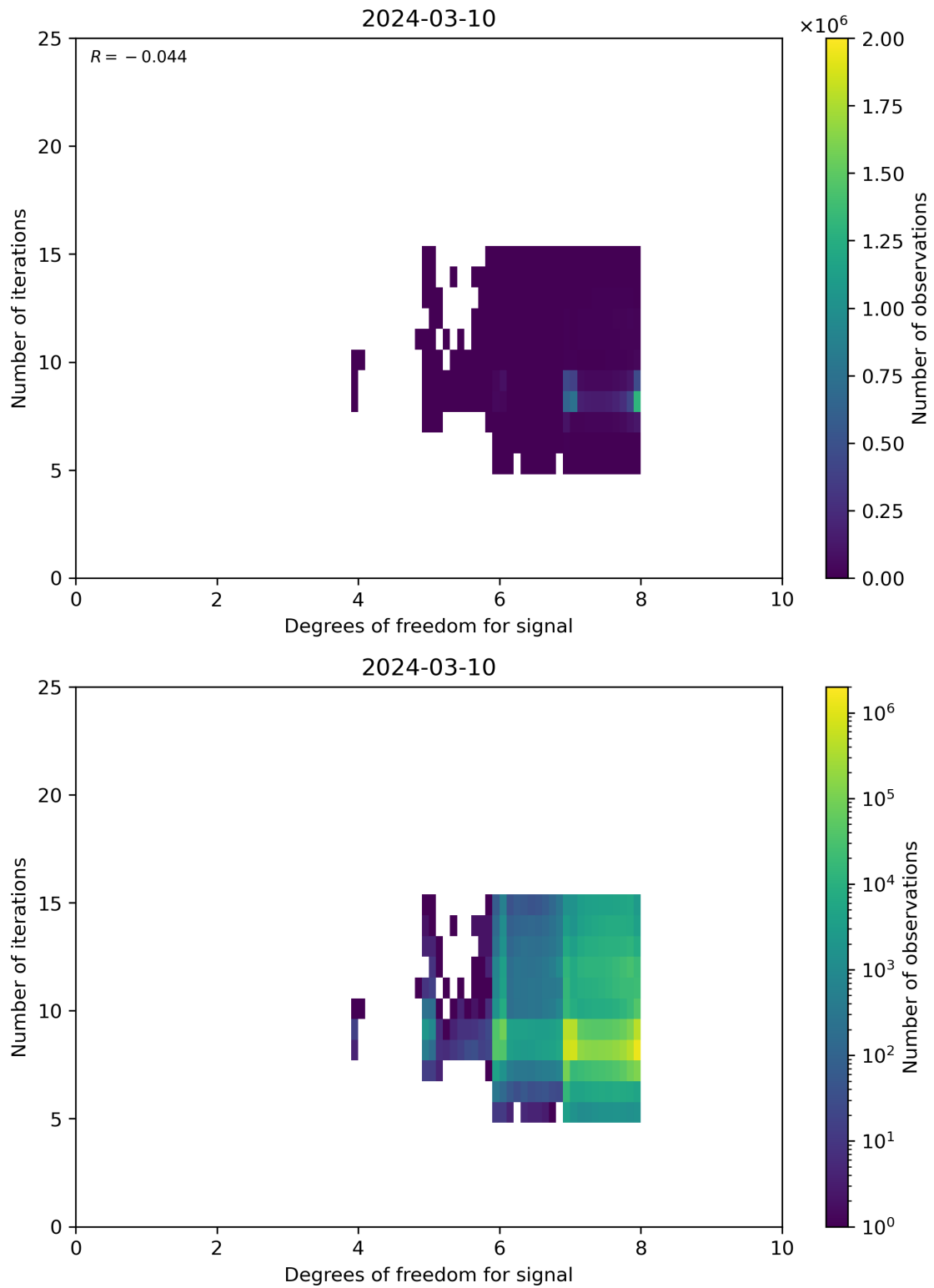
Figure 50: Scatter density plot of “Degrees of freedom for signal” against “Number of iterations” for 2024-03-09 to 2024-03-11.
