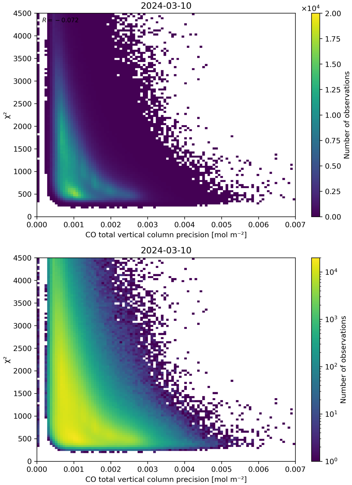
Figure 44: Scatter density plot of “CO total vertical column precision” against “ \chi^2 ” for 2024-03-09 to 2024-03-11.
