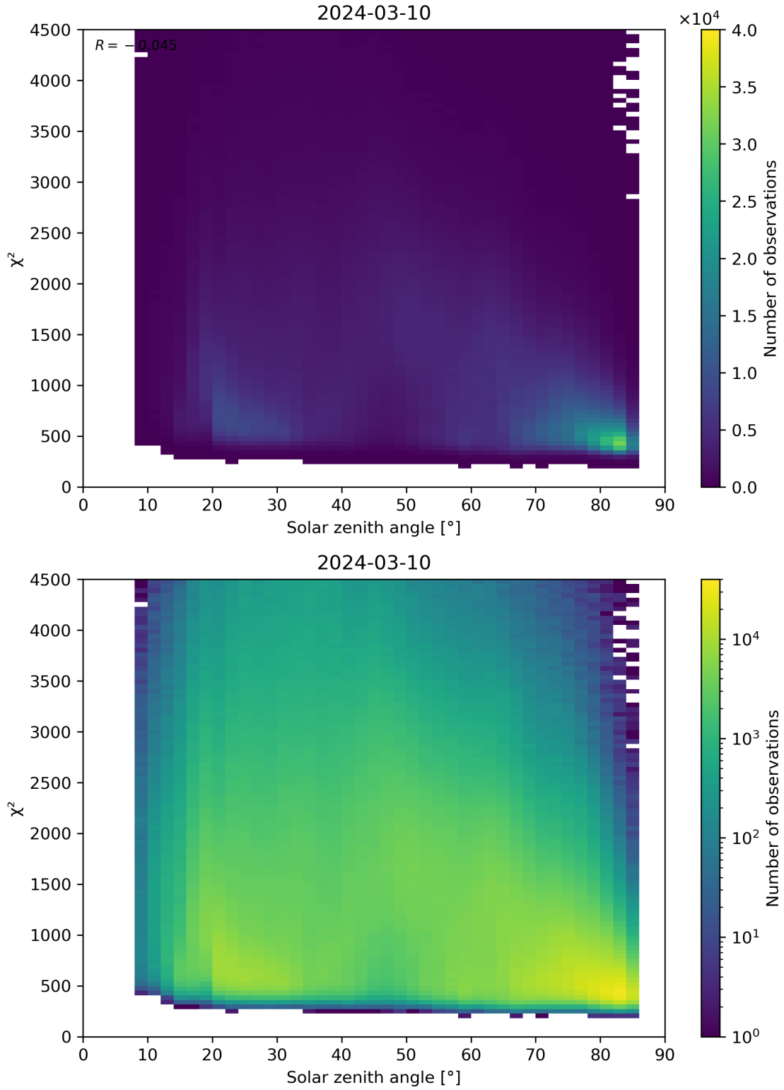
Figure 64: Scatter density plot of “Solar zenith angle” against “ \chi^2 ” for 2024-03-09 to 2024-03-11.
