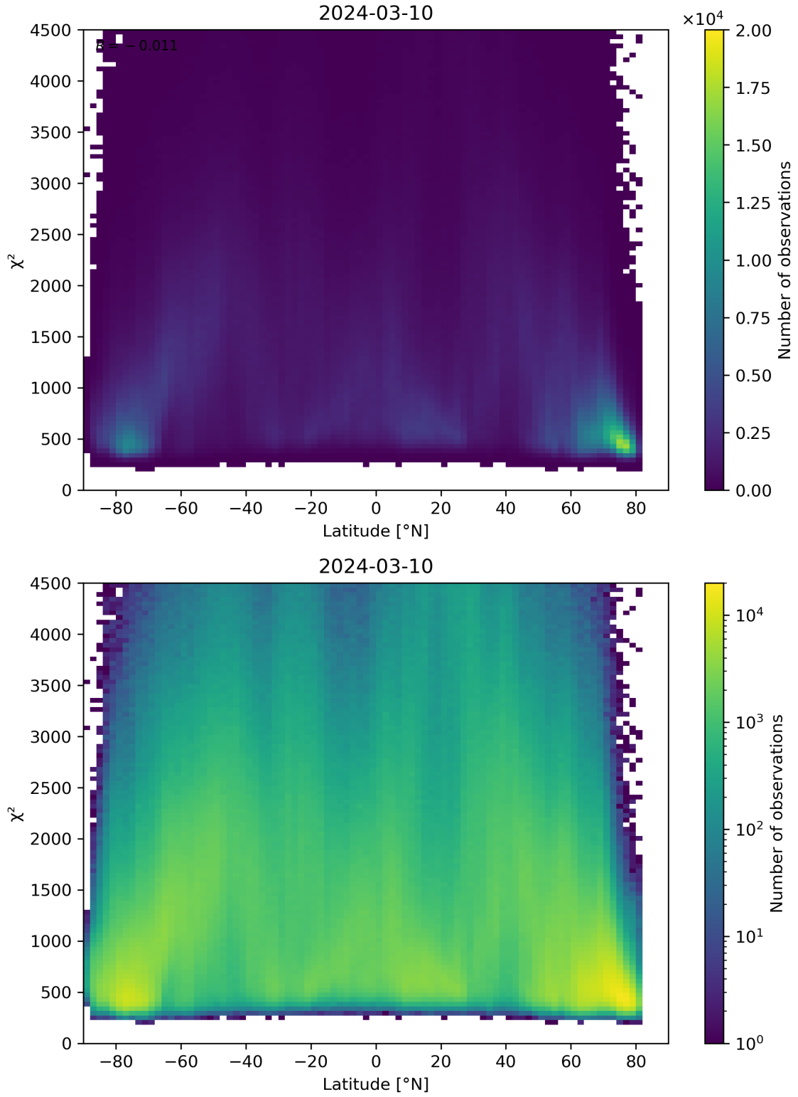
Figure 54: Scatter density plot of “Latitude” against “ \chi^2 ” for 2024-03-09 to 2024-03-11.
