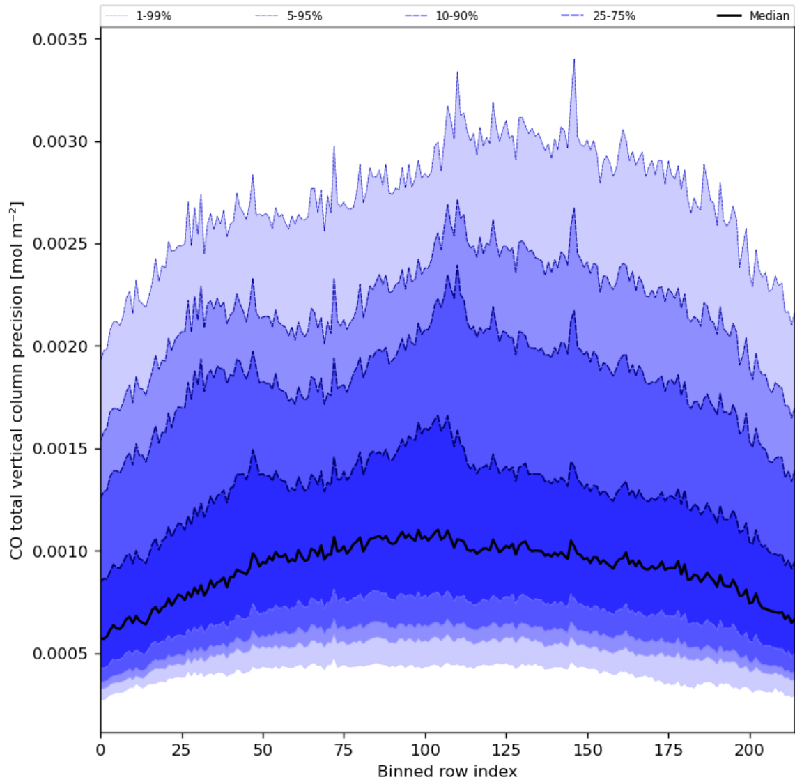
Figure 28: Along track statistics of “CO total vertical column precision” for 2024-03-09 to 2024-03-11
