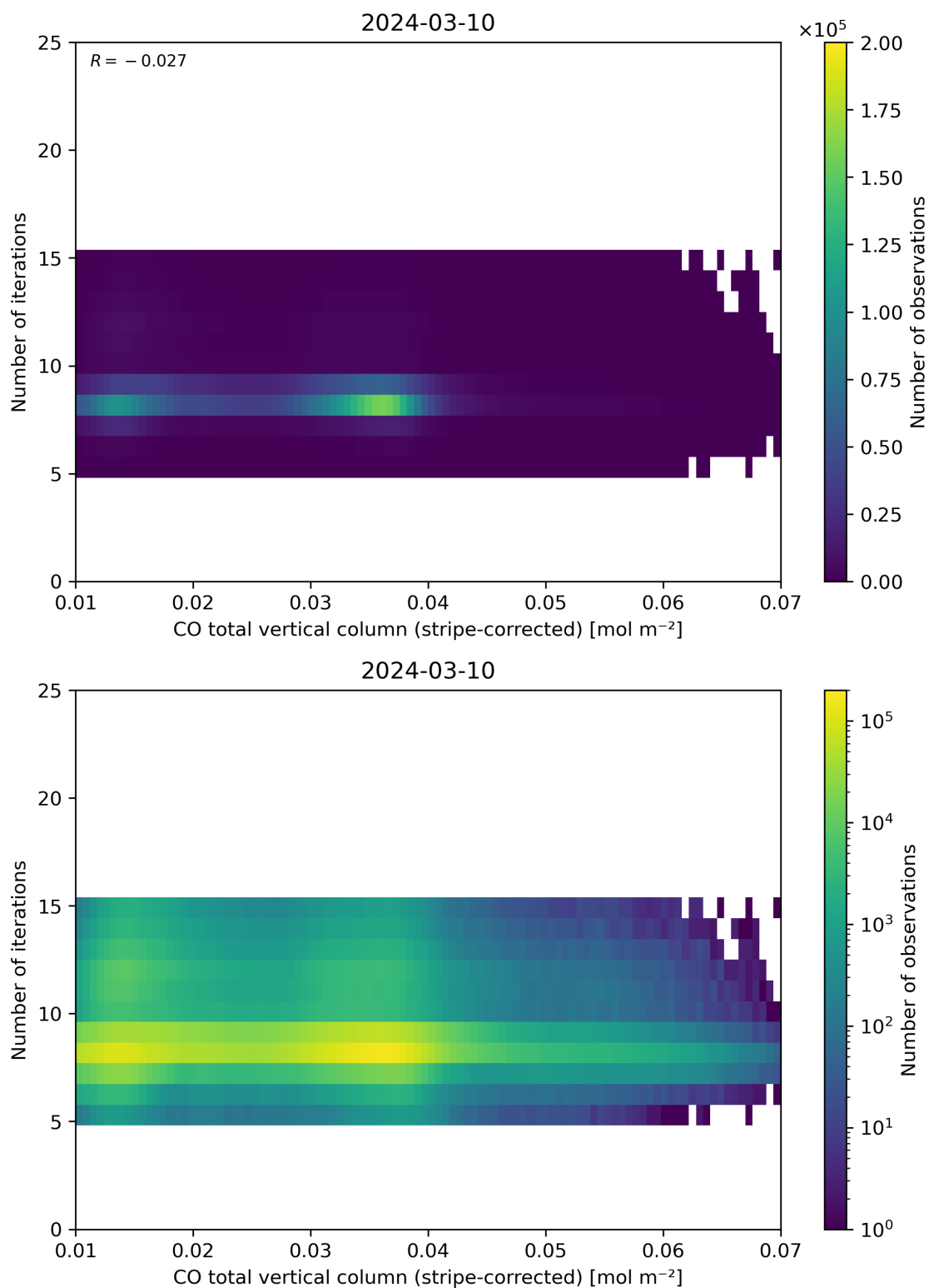
Figure 39: Scatter density plot of “CO total vertical column (stripe-corrected)” against “Number of iterations” for 2024-03-09 to 2024-03-11.
