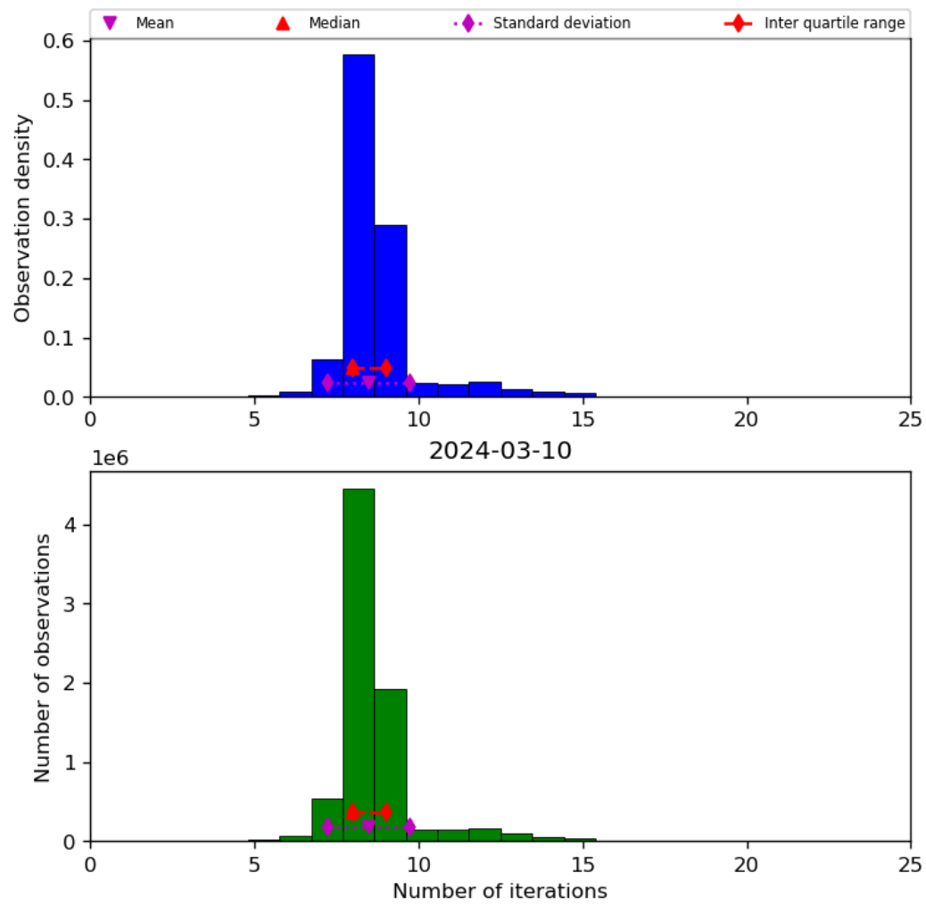
Figure 24: Histogram of “Number of iterations” for 2024-03-09 to 2024-03-11
