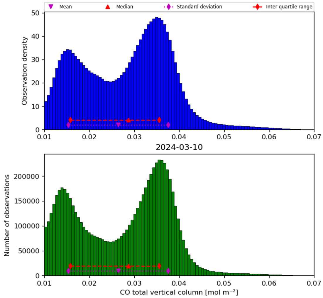
Figure 18: Histogram of “CO total vertical column” for 2024-03-09 to 2024-03-11
