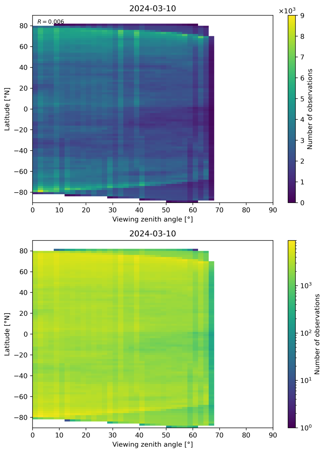
Figure 74: Scatter density plot of “Viewing zenith angle” against “Latitude” for 2024-03-09 to 2024-03-11.
