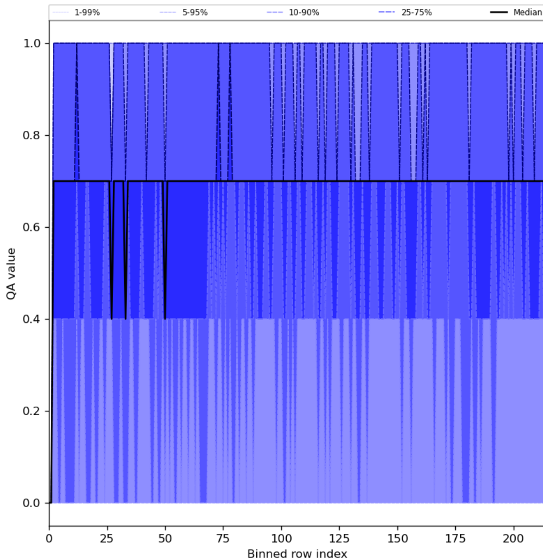
Figure 25: Along track statistics of “QA value” for 2024-03-09 to 2024-03-11
