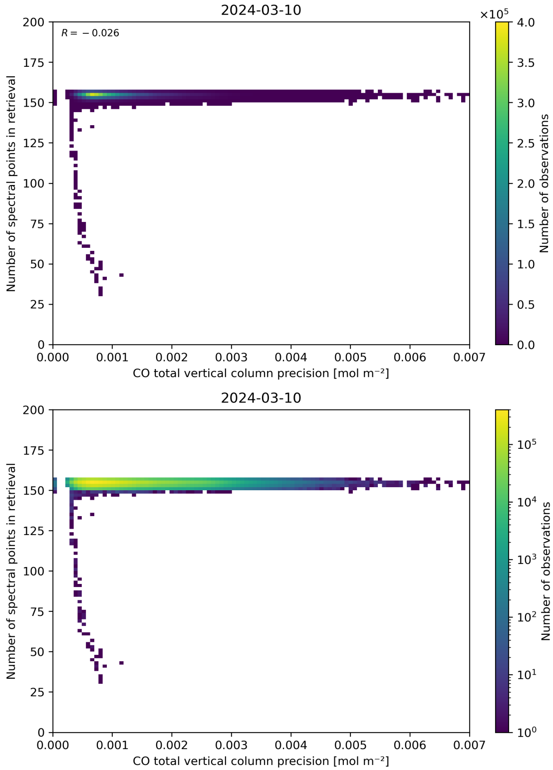
Figure 47: Scatter density plot of “CO total vertical column precision” against “Number of spectral points in retrieval” for 2024-03-09 to 2024-03-11.
