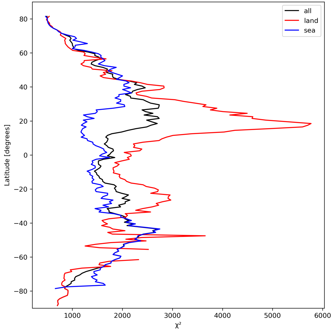
Figure 14: Zonal average of “ \chi^2 ” for 2024-03-09 to 2024-03-11.
