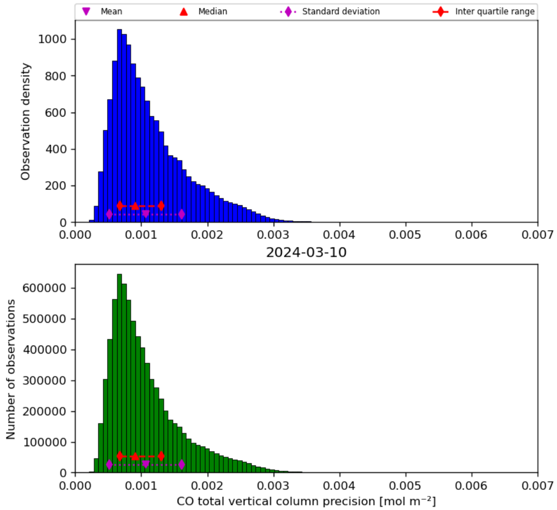
Figure 20: Histogram of “CO total vertical column precision” for 2024-03-09 to 2024-03-11
