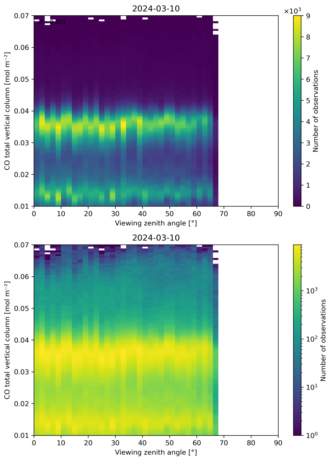
Figure 69: Scatter density plot of “Viewing zenith angle” against “CO total vertical column” for 2024-03-09 to 2024-03-11.
