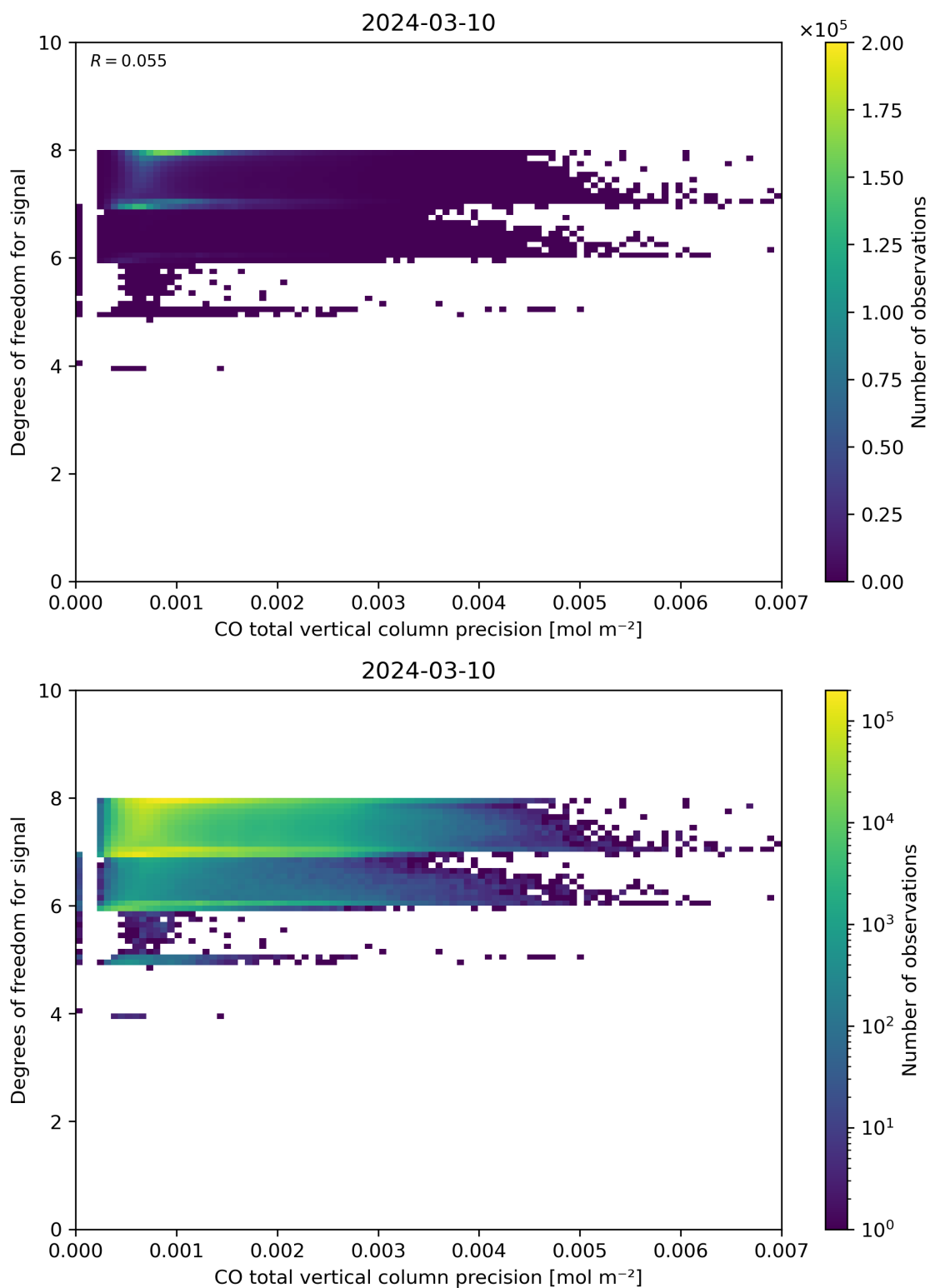
Figure 45: Scatter density plot of “CO total vertical column precision” against “Degrees of freedom for signal” for 2024-03-09 to 2024-03-11.
