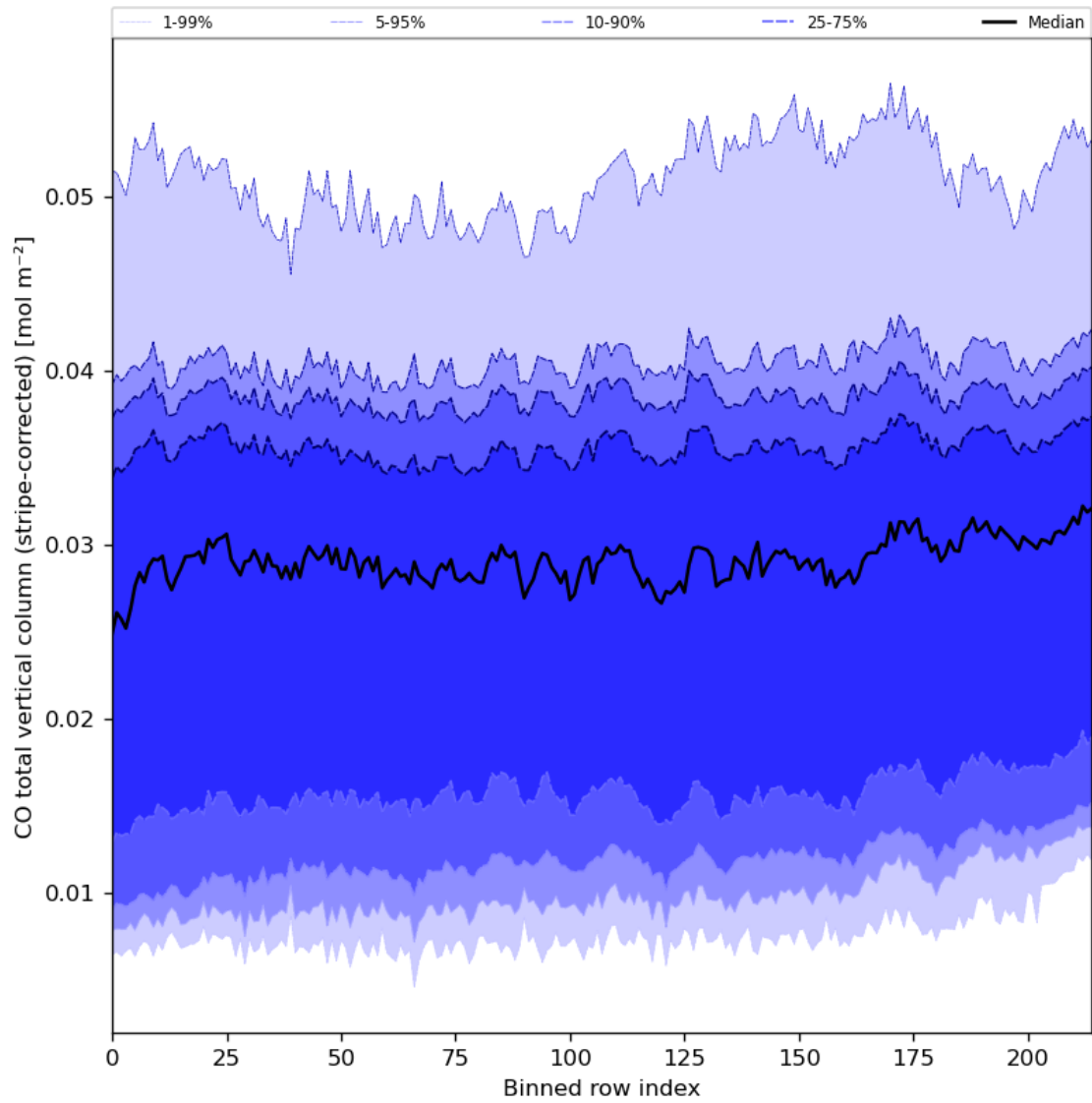
Figure 27: Along track statistics of “CO total vertical column (stripe-corrected)” for 2024-03-09 to 2024-03-11
