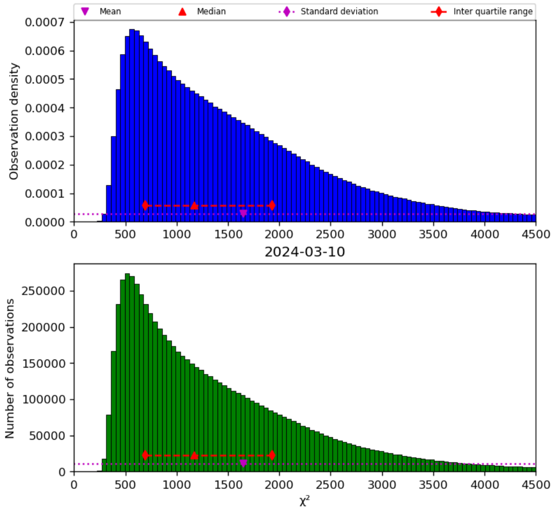
Figure 22: Histogram of “ \chi^2 ” for 2024-03-09 to 2024-03-11
