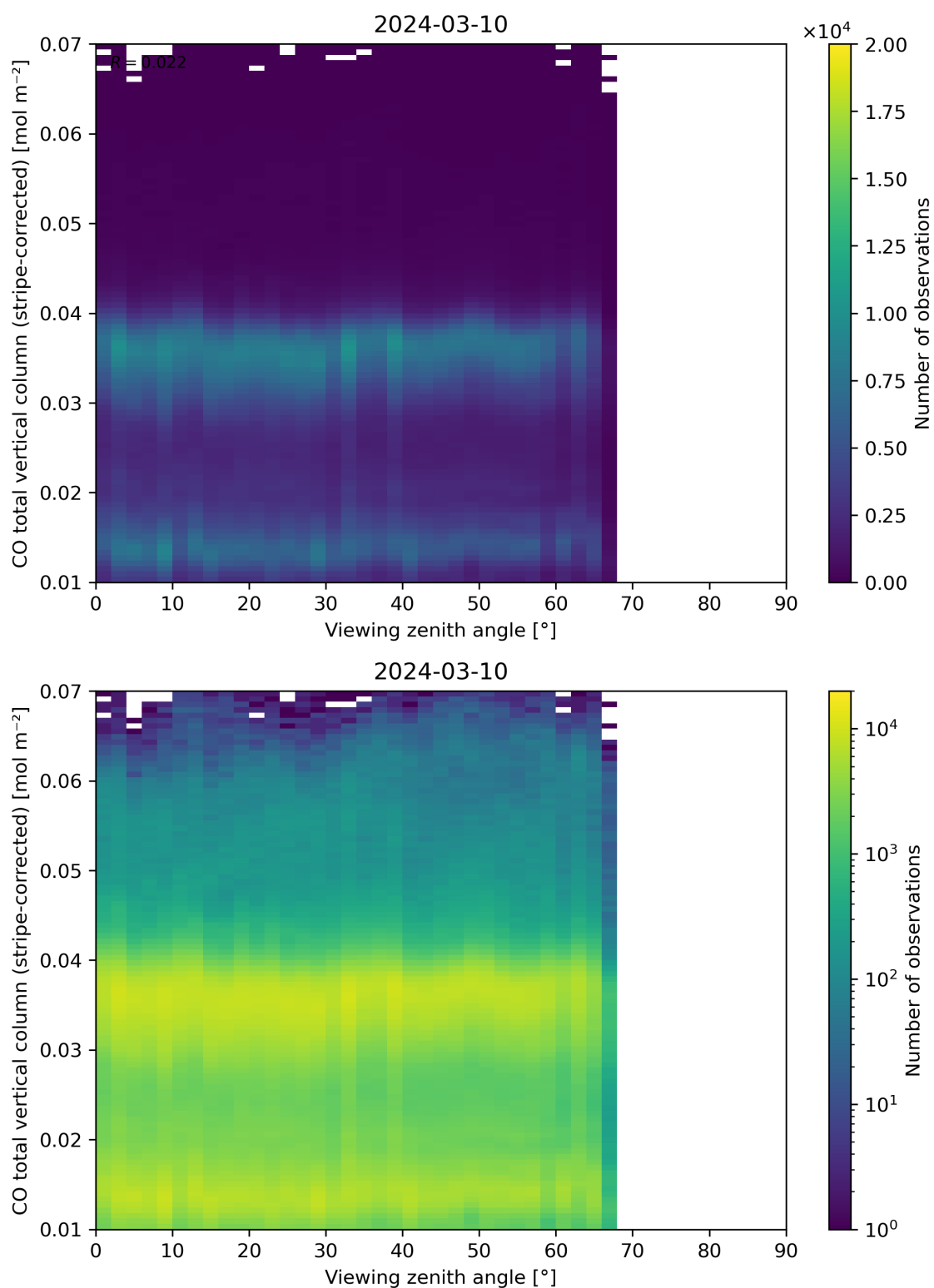
Figure 70: Scatter density plot of “Viewing zenith angle” against “CO total vertical column (stripe-corrected)” for 2024-03-09 to 2024-03-11.
