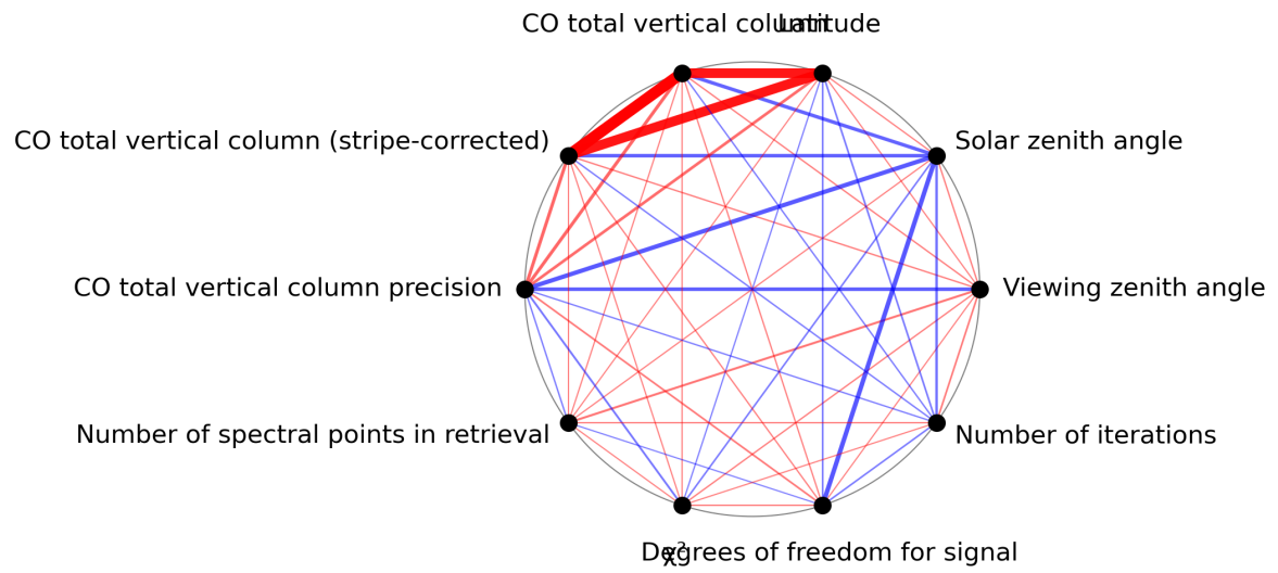
Figure 1: Map of correlation graph for 2024-03-09 to 2024-03-11.
