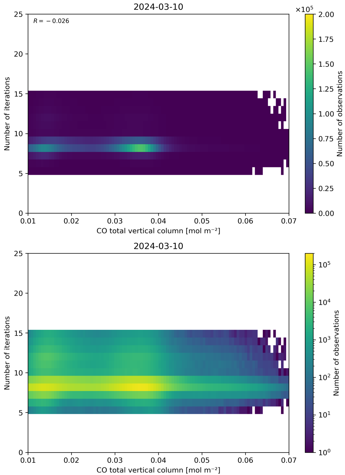
Figure 42: Scatter density plot of “CO total vertical column” against “Number of iterations” for 2024-03-09 to 2024-03-11.
