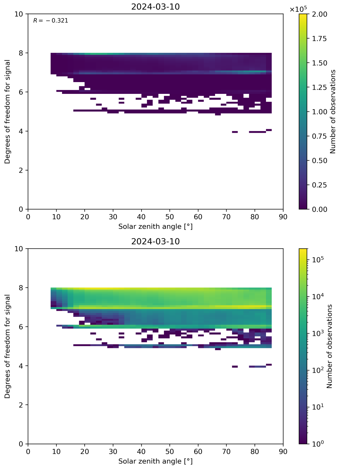
Figure 65: Scatter density plot of “Solar zenith angle” against “Degrees of freedom for signal” for 2024-03-09 to 2024-03-11.
