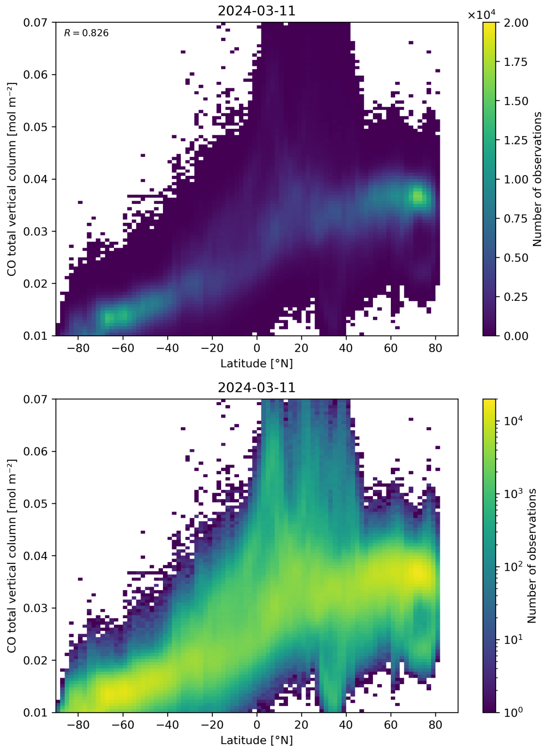
Figure 51: Scatter density plot of “Latitude” against “CO total vertical column” for 2024-03-10 to 2024-03-12.
