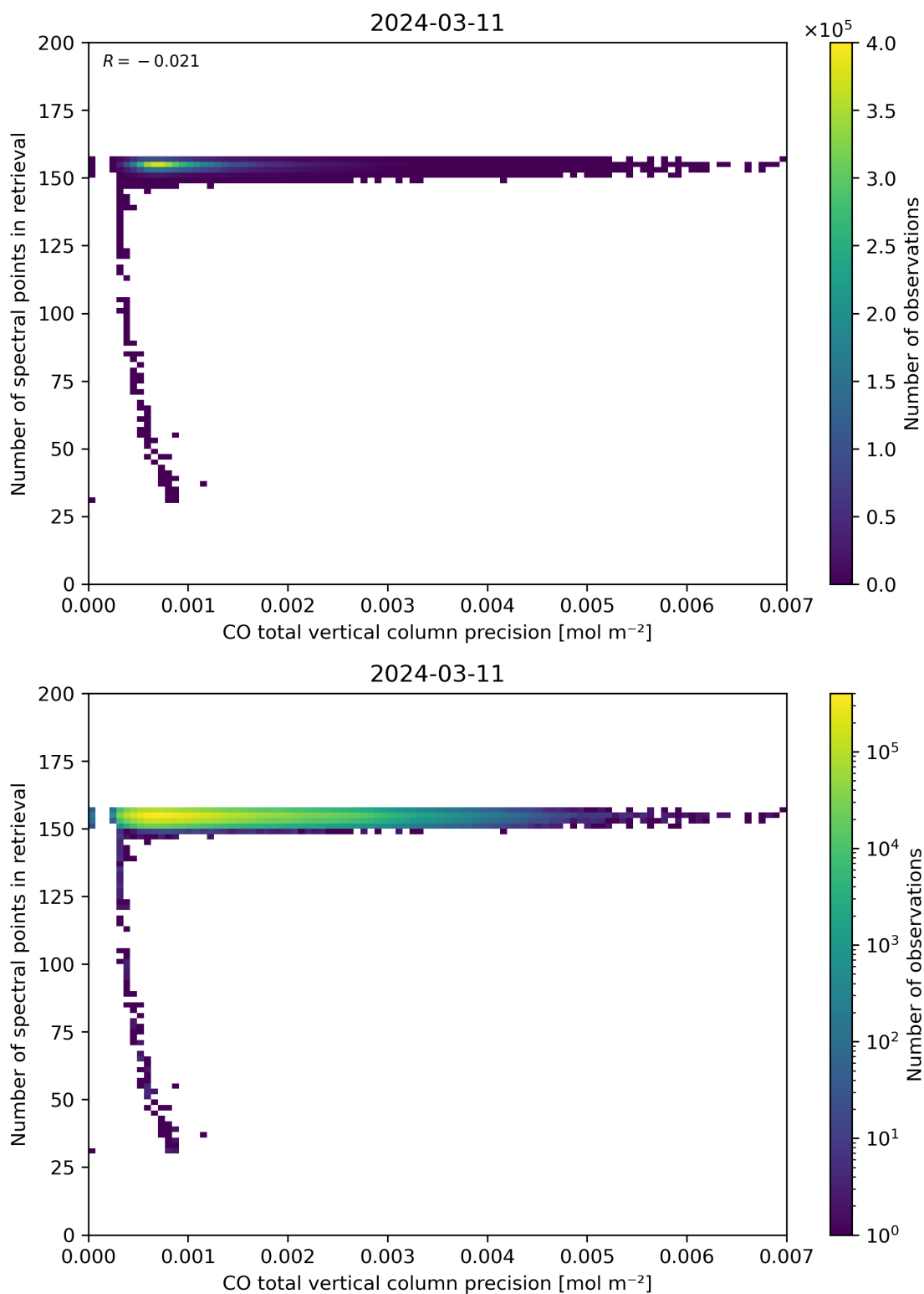
Figure 47: Scatter density plot of “CO total vertical column precision” against “Number of spectral points in retrieval” for 2024-03-10 to 2024-03-12.
