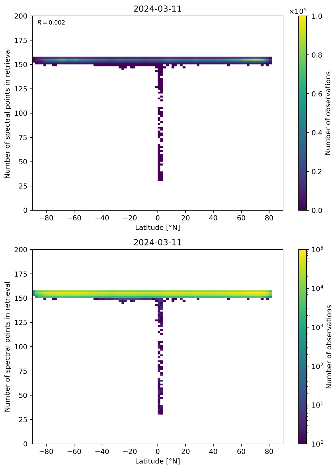
Figure 57: Scatter density plot of “Latitude” against “Number of spectral points in retrieval” for 2024-03-10 to 2024-03-12.
