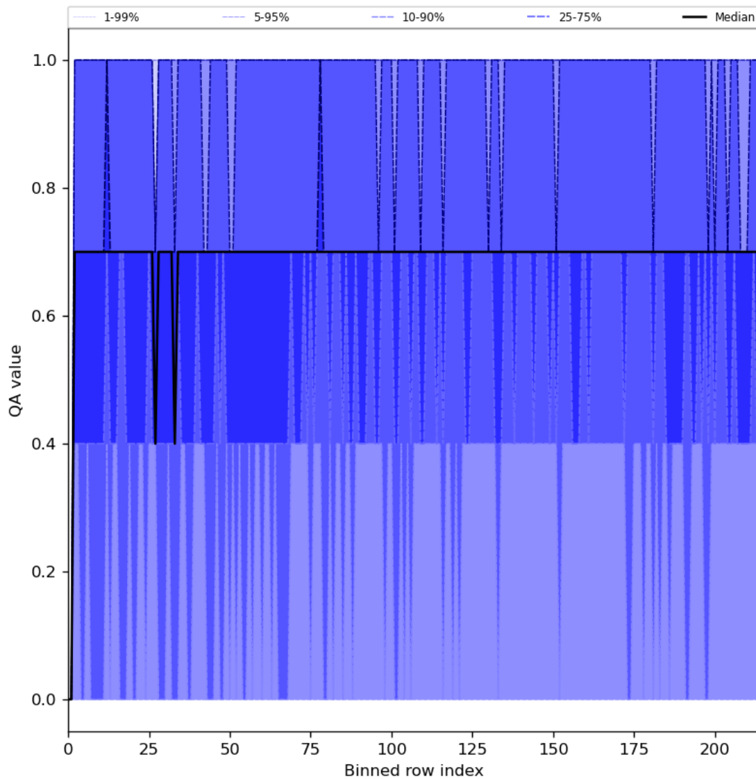
Figure 25: Along track statistics of “QA value” for 2024-03-10 to 2024-03-12
