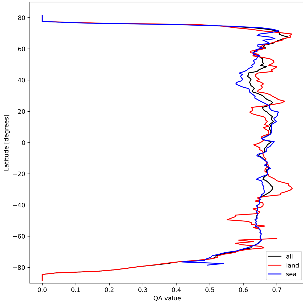
Figure 9: Zonal average of “QA value” for 2024-03-10 to 2024-03-12.
