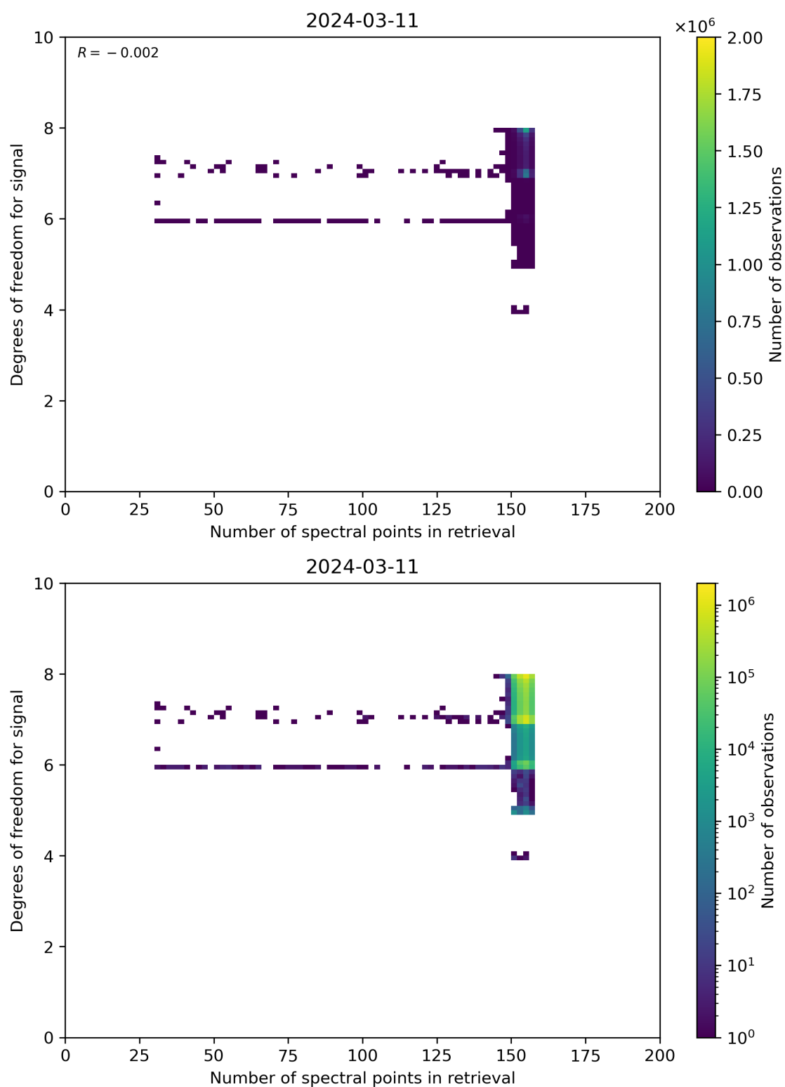
Figure 59: Scatter density plot of “Number of spectral points in retrieval” against “Degrees of freedom for signal” for 2024-03-10 to 2024-03-12.
