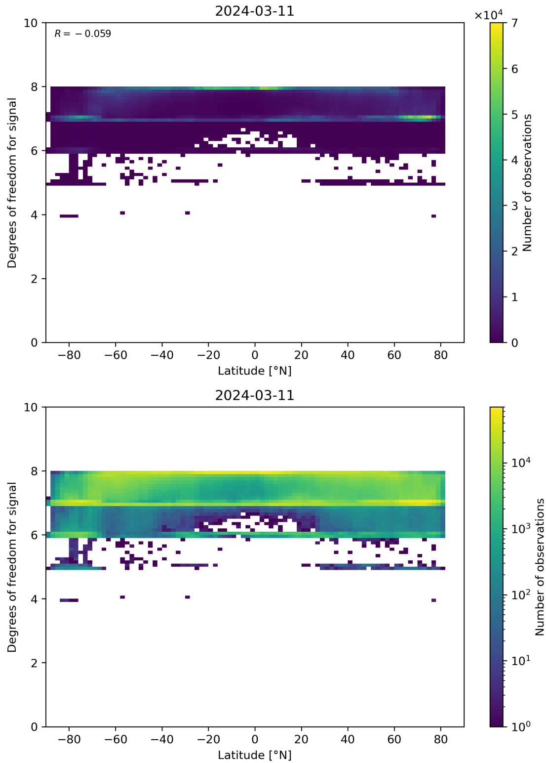
Figure 55: Scatter density plot of “Latitude” against “Degrees of freedom for signal” for 2024-03-10 to 2024-03-12.
