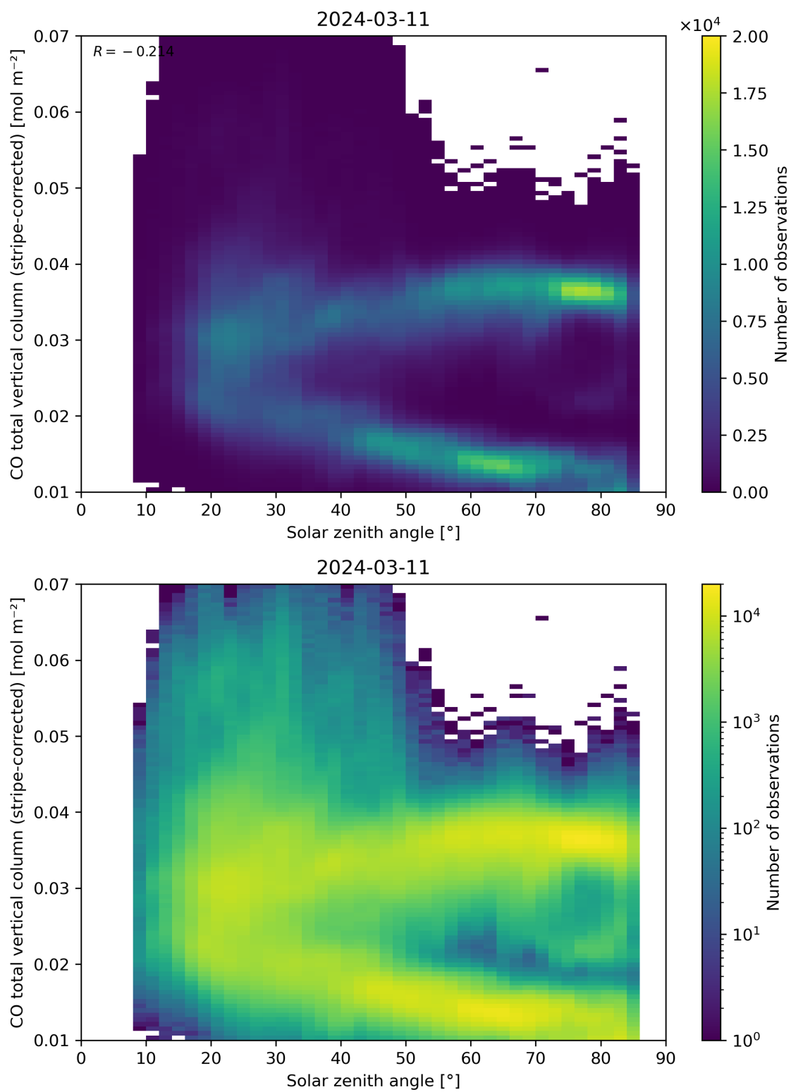
Figure 62: Scatter density plot of “Solar zenith angle” against “CO total vertical column (stripe-corrected)” for 2024-03-10 to 2024-03-12.
