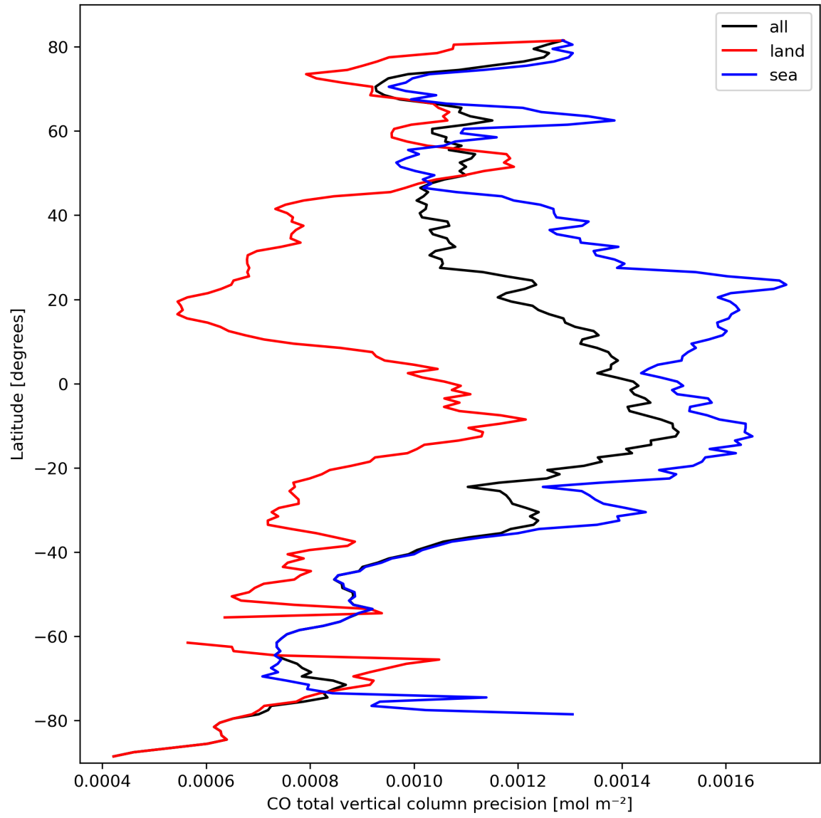
Figure 12: Zonal average of “CO total vertical column precision” for 2024-03-10 to 2024-03-12.
