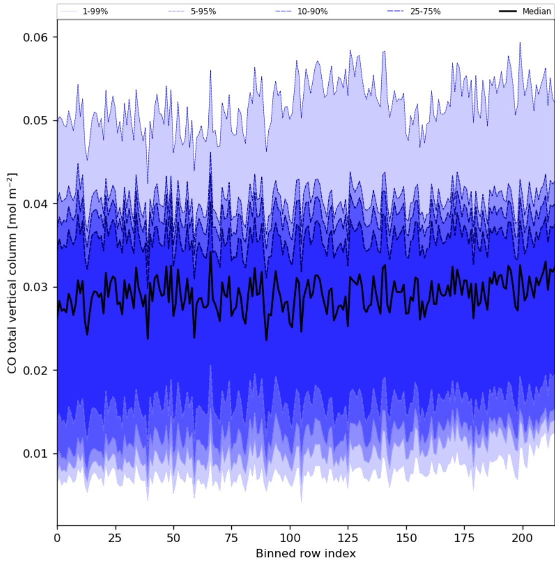
Figure 26: Along track statistics of “CO total vertical column” for 2024-03-10 to 2024-03-12
