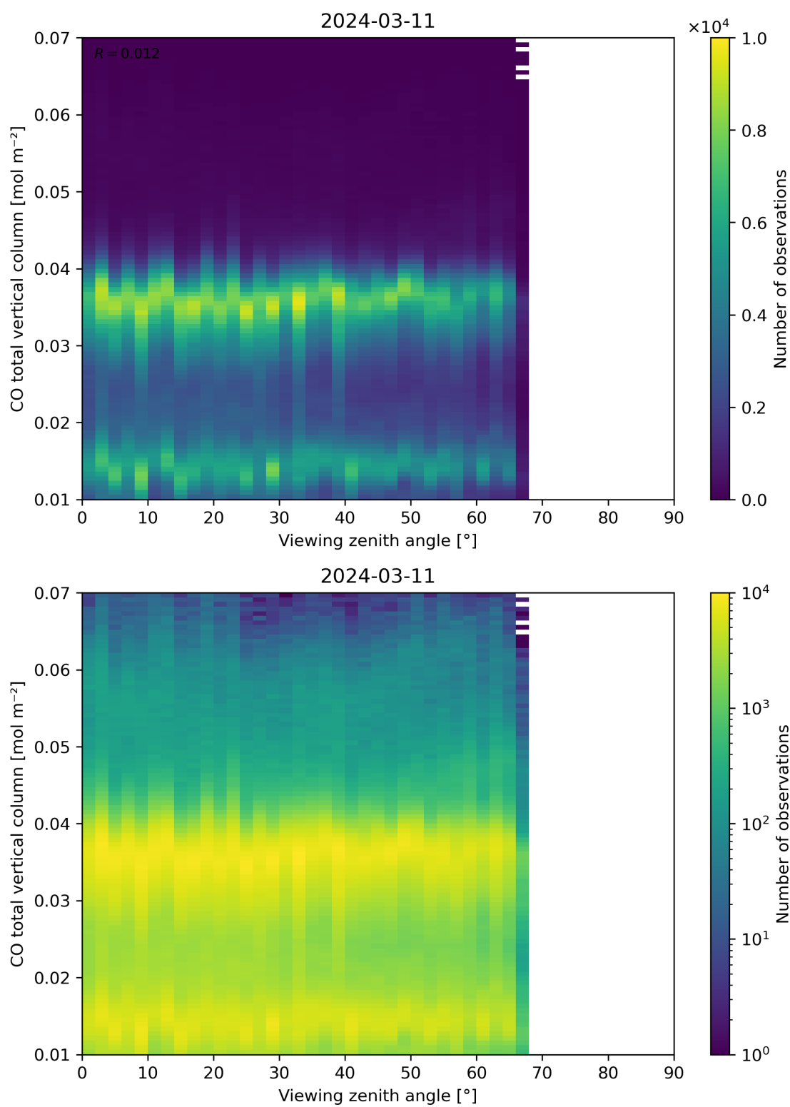
Figure 69: Scatter density plot of “Viewing zenith angle” against “CO total vertical column” for 2024-03-10 to 2024-03-12.
