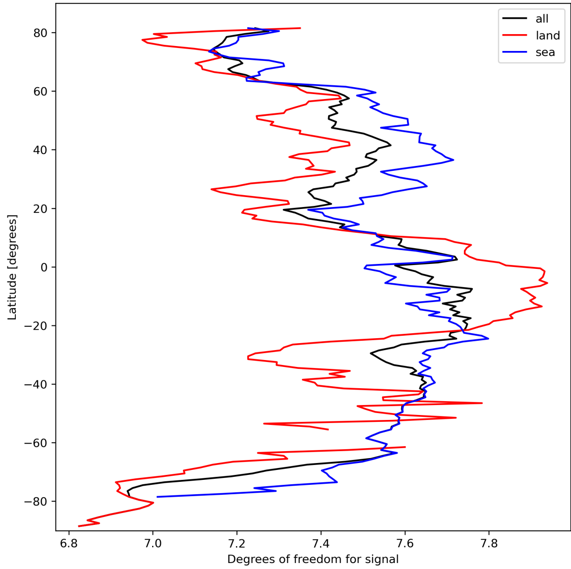
Figure 15: Zonal average of “Degrees of freedom for signal” for 2024-03-10 to 2024-03-12.
