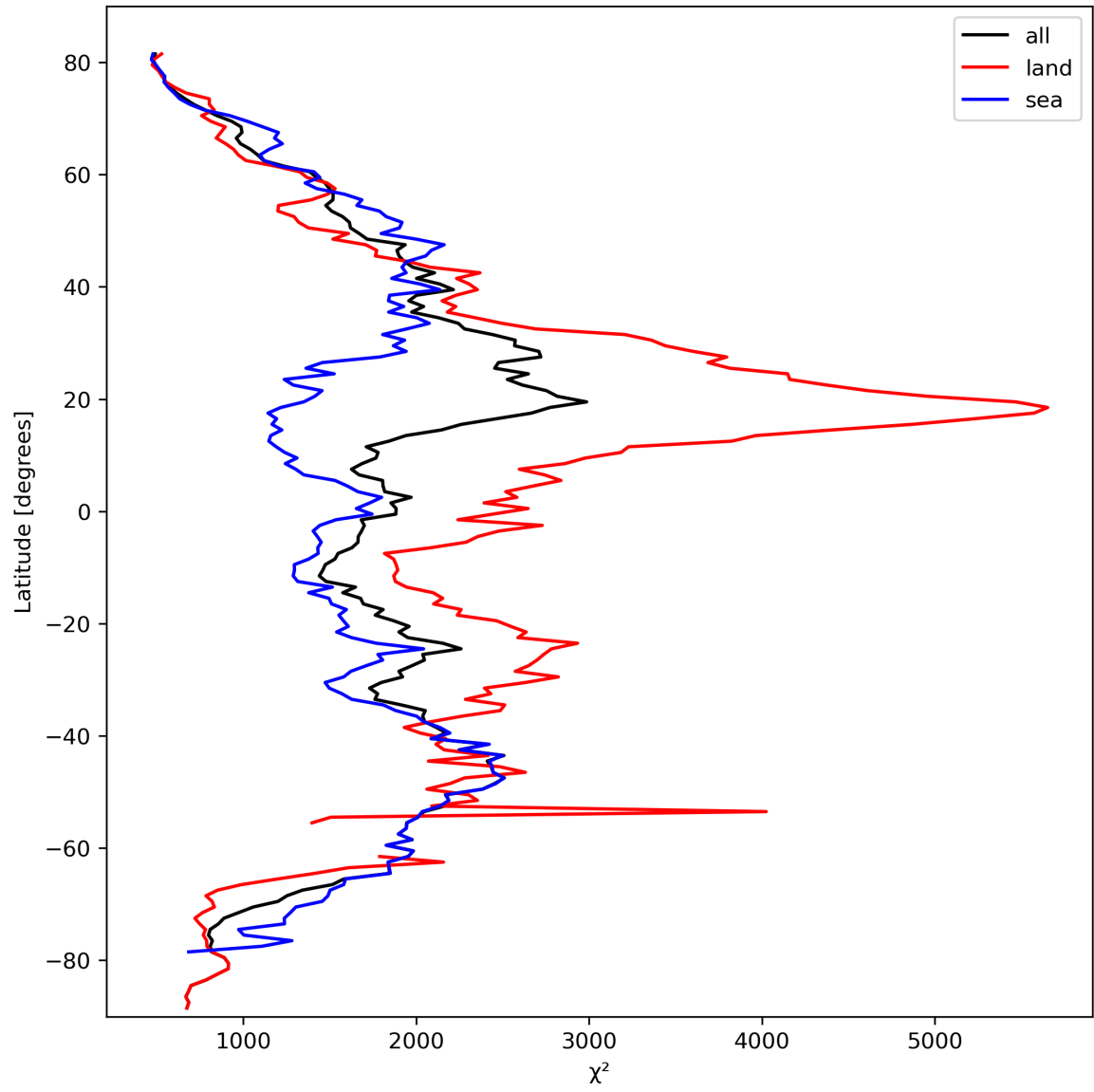
Figure 14: Zonal average of “ \chi^2 ” for 2024-03-10 to 2024-03-12.
