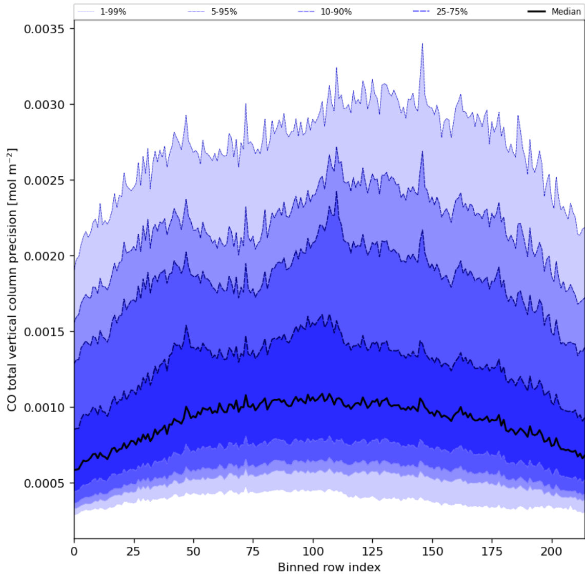
Figure 28: Along track statistics of “CO total vertical column precision” for 2024-03-10 to 2024-03-12
