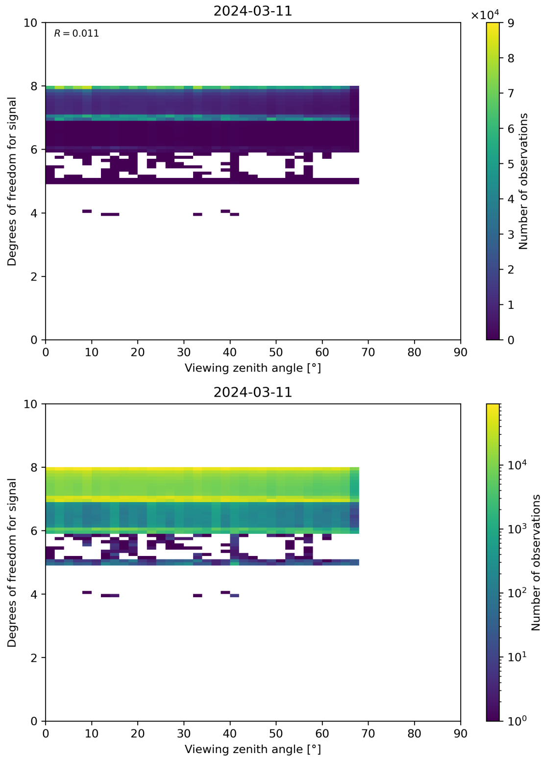
Figure 73: Scatter density plot of “Viewing zenith angle” against “Degrees of freedom for signal” for 2024-03-10 to 2024-03-12.
