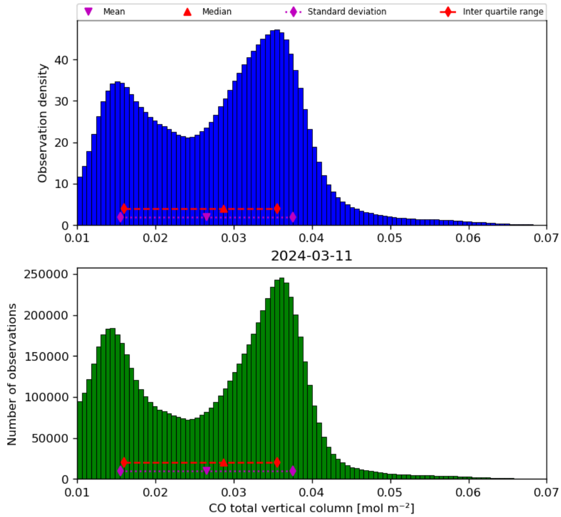
Figure 18: Histogram of “CO total vertical column” for 2024-03-10 to 2024-03-12
