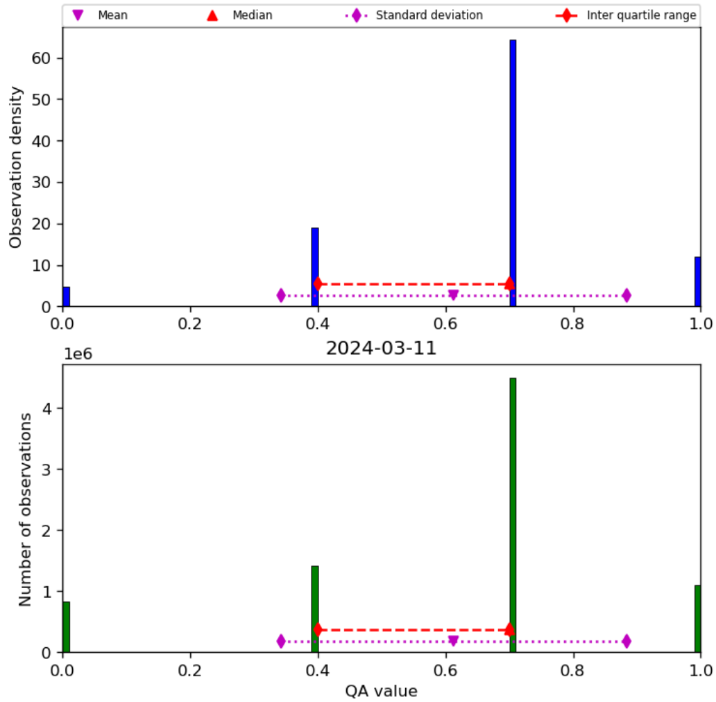
Figure 17: Histogram of “QA value” for 2024-03-10 to 2024-03-12
