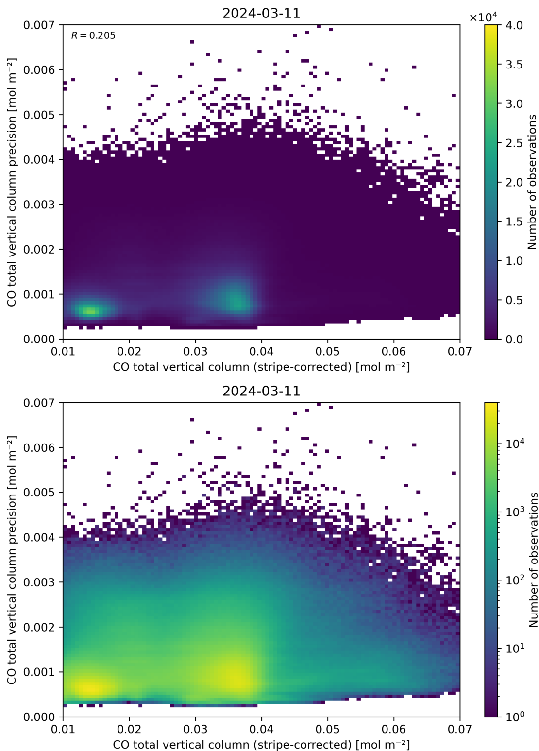
Figure 36: Scatter density plot of “CO total vertical column (stripe-corrected)” against “CO total vertical column precision” for 2024-03-10 to 2024-03-12.
