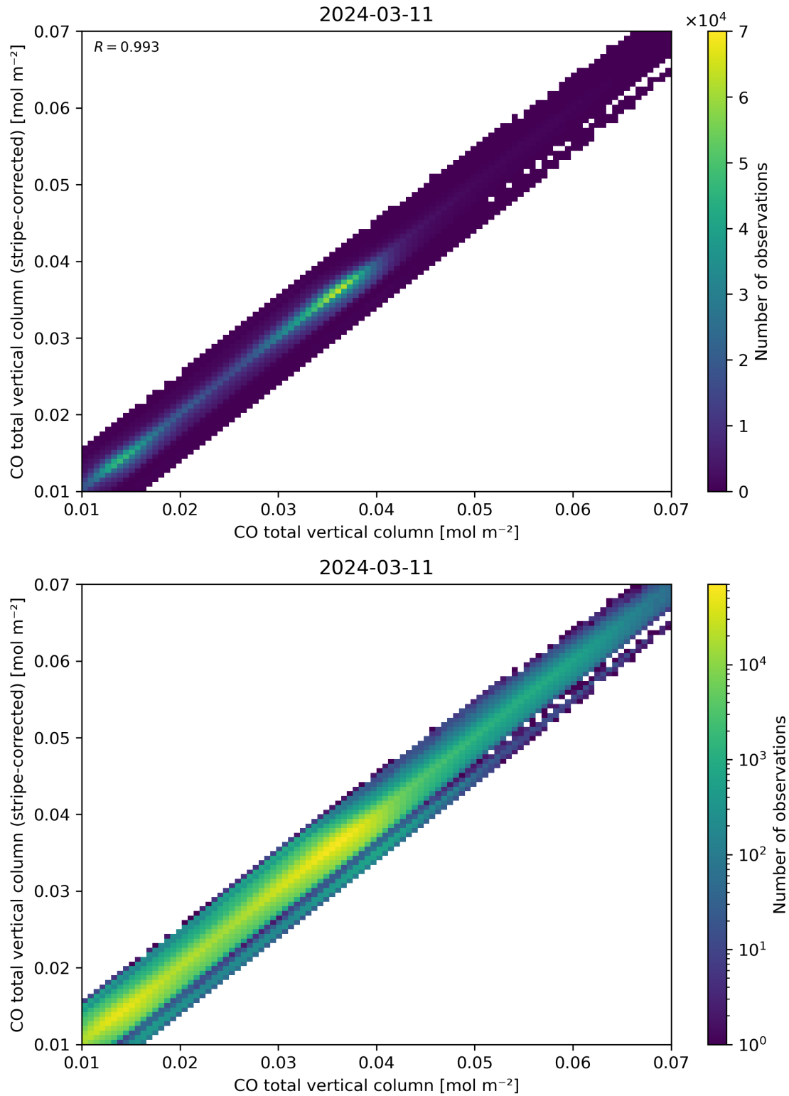
Figure 33: Scatter density plot of “CO total vertical column” against “CO total vertical column (stripe-corrected)” for 2024-03-10 to 2024-03-12.
