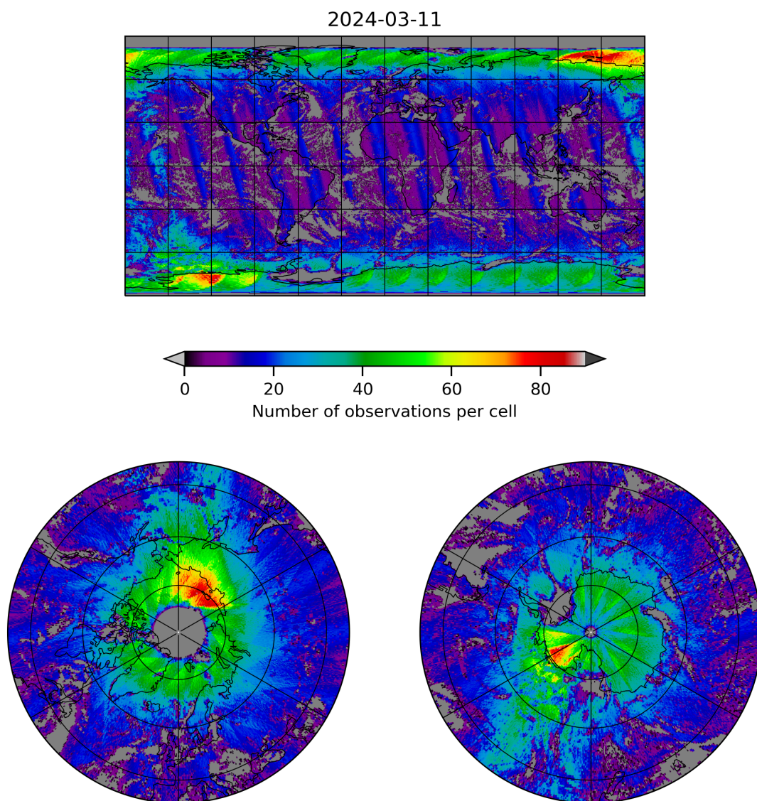
Figure 8: Map of the number of observations for 2024-03-10 to 2024-03-12
