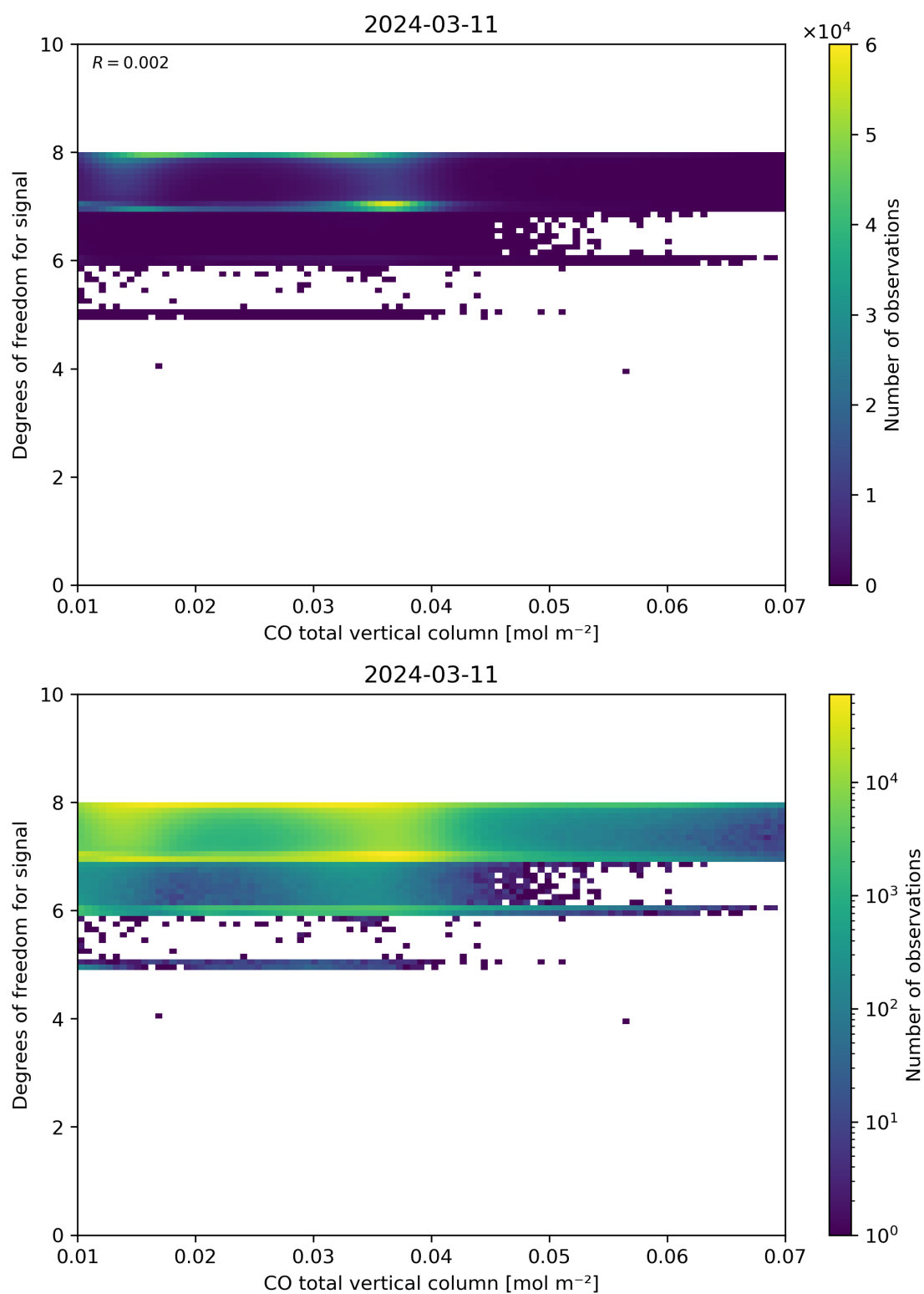
Figure 41: Scatter density plot of “CO total vertical column” against “Degrees of freedom for signal” for 2024-03-10 to 2024-03-12.
