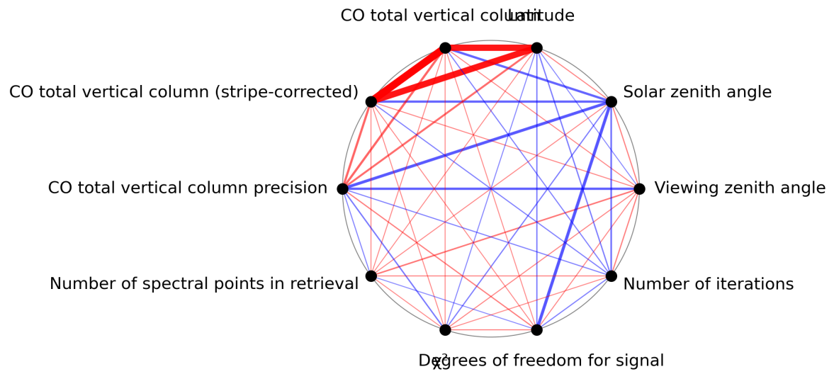
Figure 1: Map of correlation graph for 2024-03-10 to 2024-03-12.
