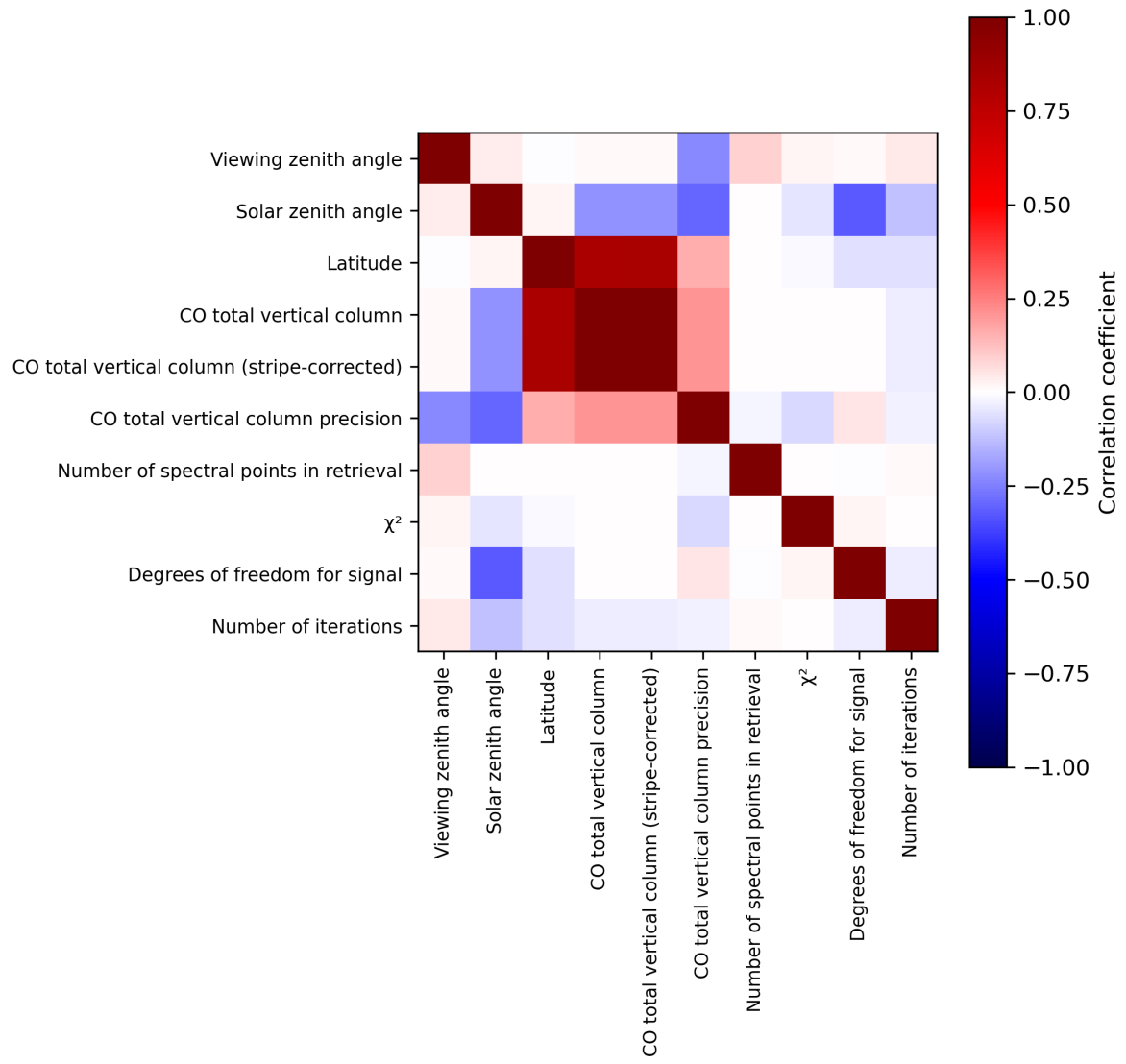
Figure 2: Map of correlation matrix for 2024-03-10 to 2024-03-12.
