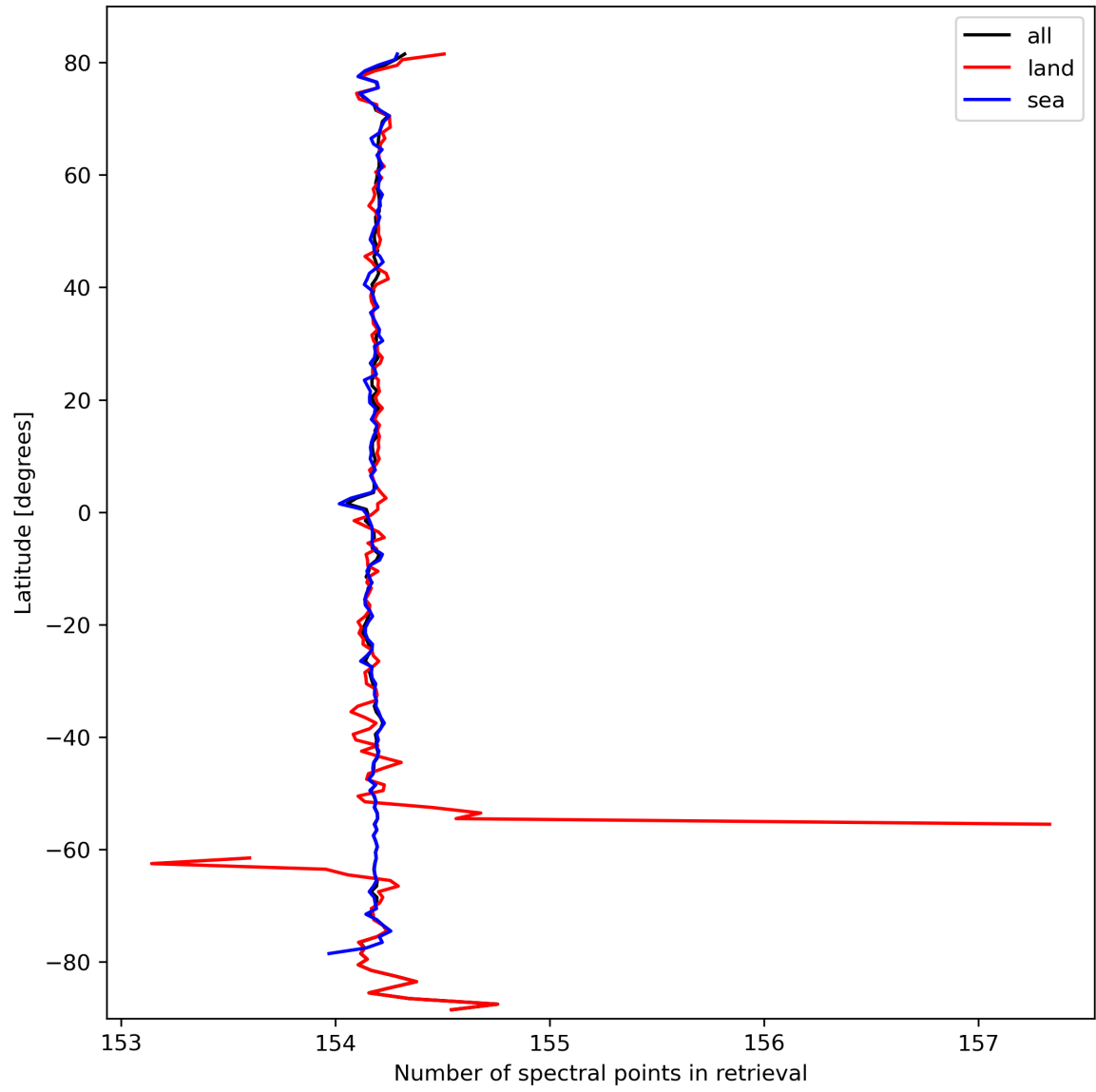
Figure 13: Zonal average of “Number of spectral points in retrieval” for 2024-03-10 to 2024-03-12.
