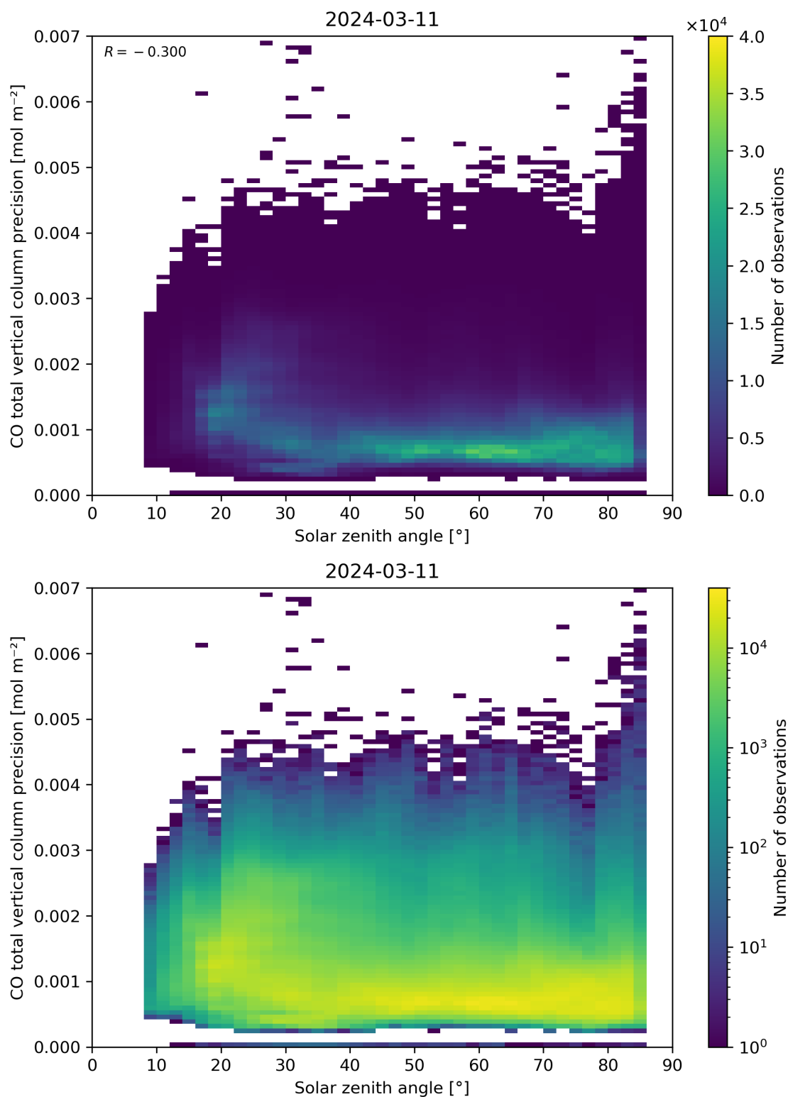
Figure 63: Scatter density plot of “Solar zenith angle” against “CO total vertical column precision” for 2024-03-10 to 2024-03-12.
