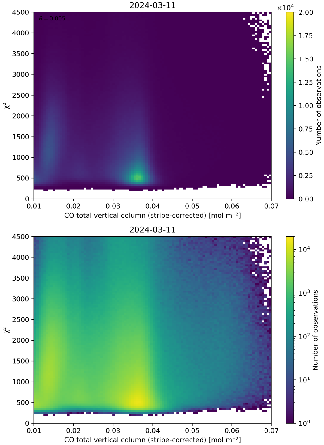
Figure 37: Scatter density plot of “CO total vertical column (stripe-corrected)” against “ \chi^2 ” for 2024-03-10 to 2024-03-12.
