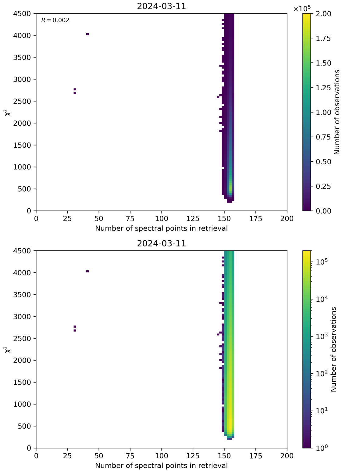
Figure 58: Scatter density plot of “Number of spectral points in retrieval” against “ \chi^2 ” for 2024-03-10 to 2024-03-12.
