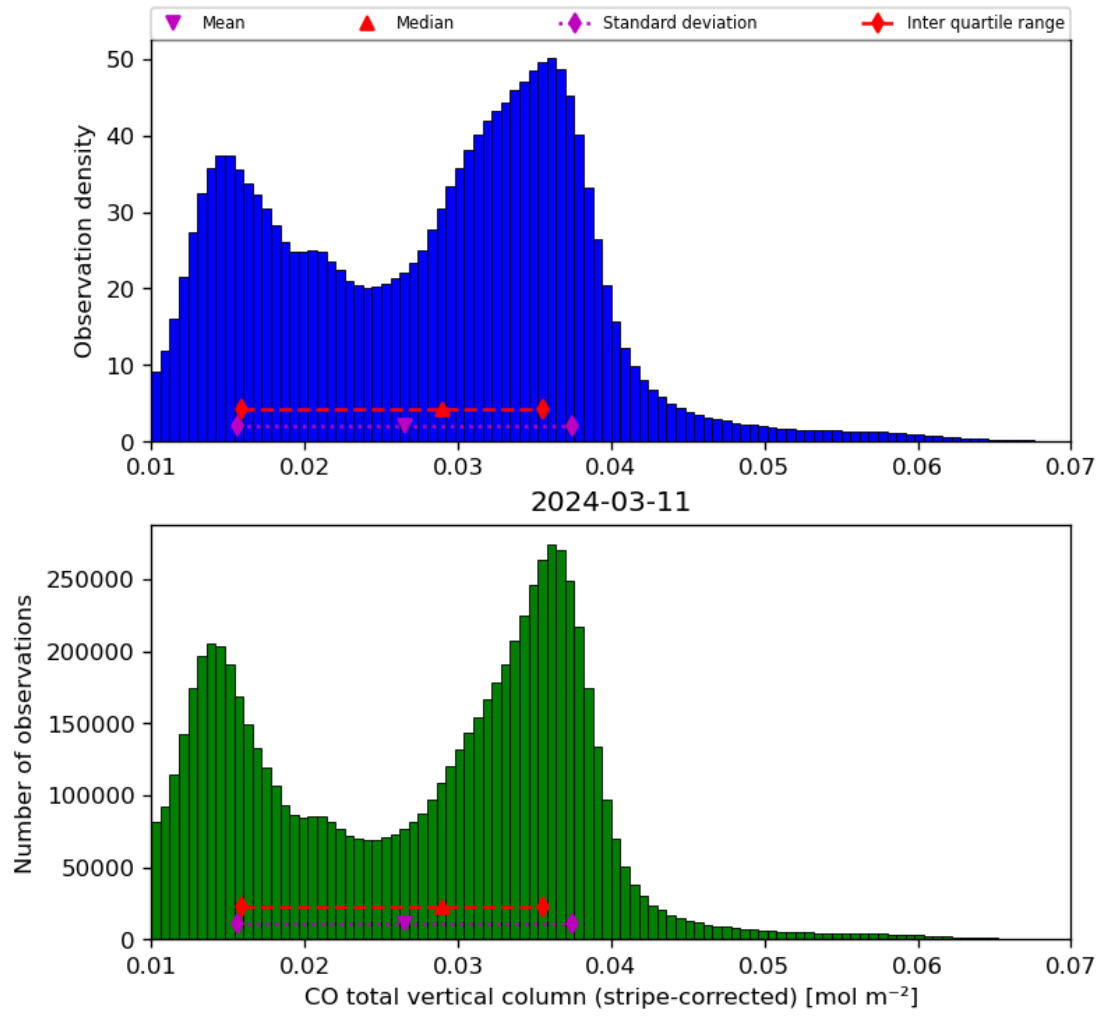
Figure 19: Histogram of “CO total vertical column (stripe-corrected)” for 2024-03-10 to 2024-03-12
