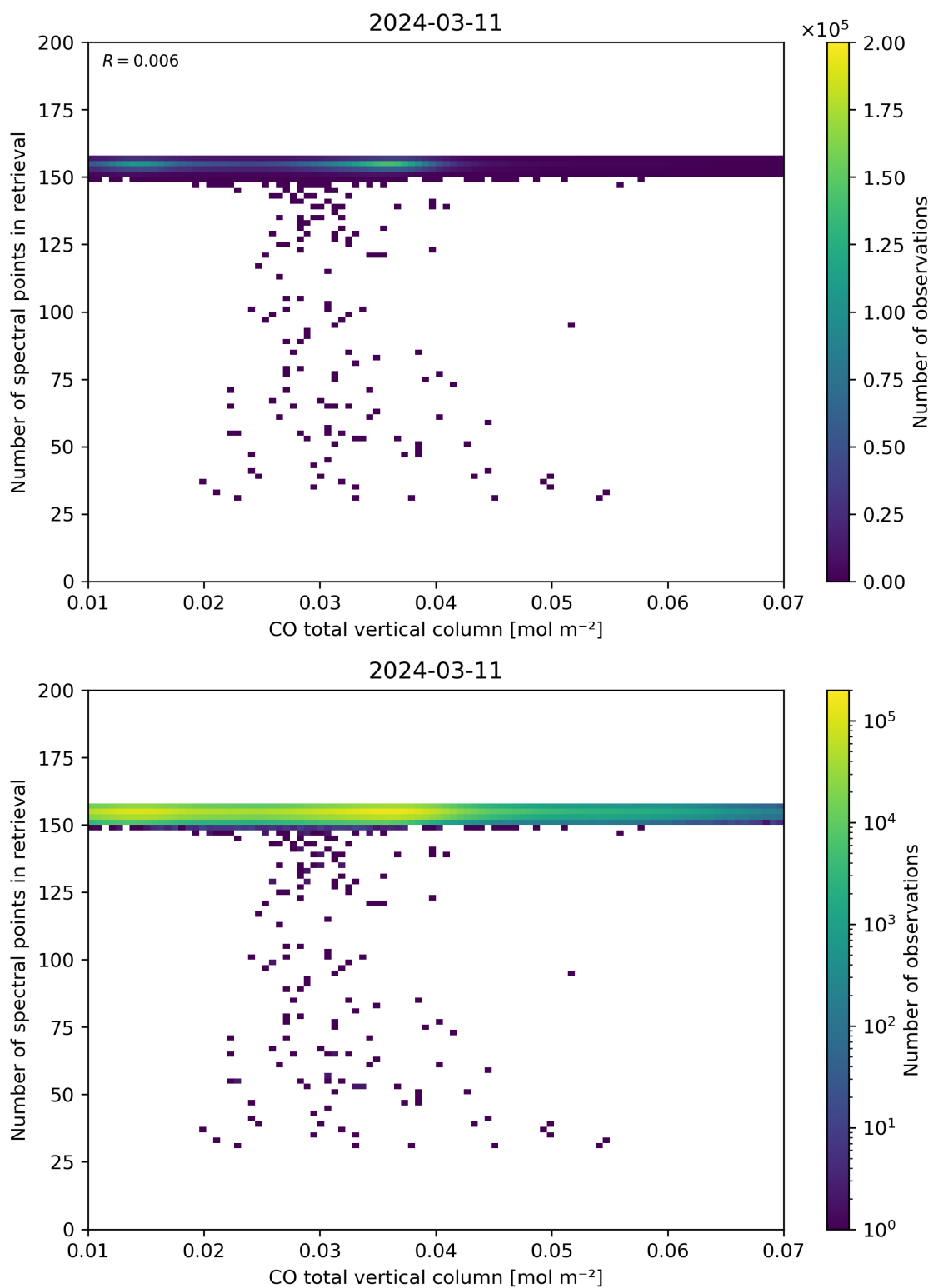
Figure 43: Scatter density plot of “CO total vertical column” against “Number of spectral points in retrieval” for 2024-03-10 to 2024-03-12.
