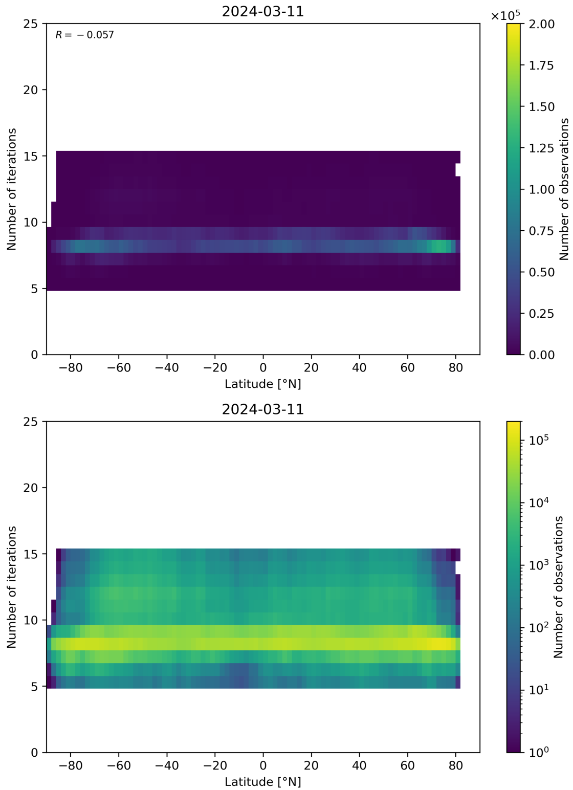
Figure 56: Scatter density plot of “Latitude” against “Number of iterations” for 2024-03-10 to 2024-03-12.
