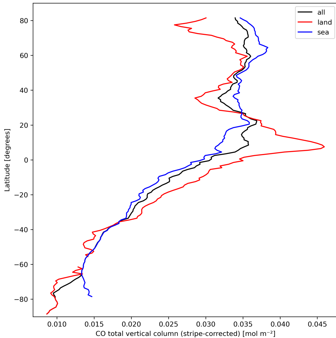
Figure 11: Zonal average of “CO total vertical column (stripe-corrected)” for 2024-03-10 to 2024-03-12.
