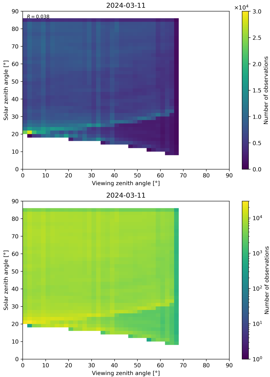
Figure 77: Scatter density plot of “Viewing zenith angle” against “Solar zenith angle” for 2024-03-10 to 2024-03-12.
