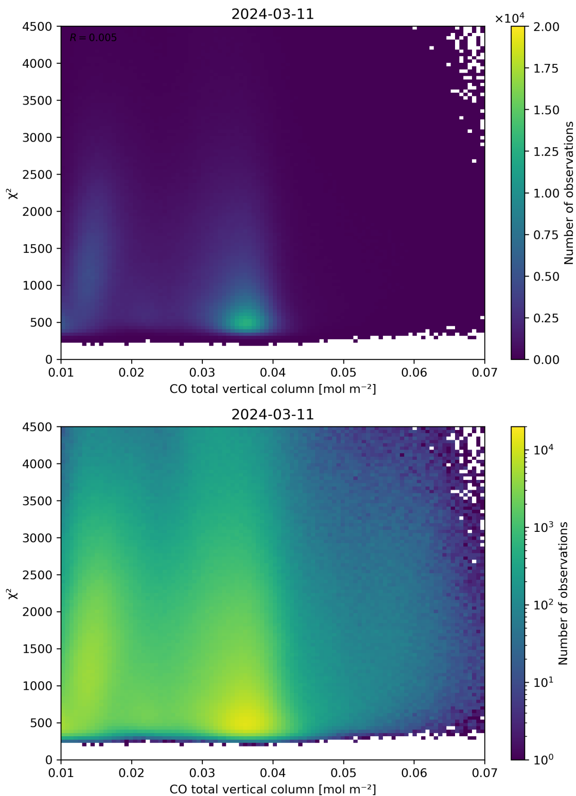
Figure 35: Scatter density plot of “CO total vertical column” against “ \chi^2 ” for 2024-03-10 to 2024-03-12.
