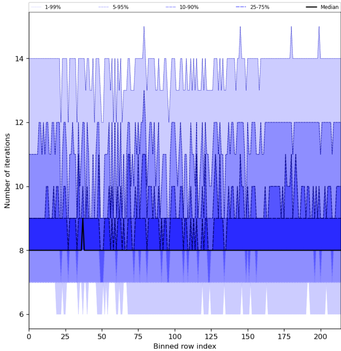
Figure 32: Along track statistics of “Number of iterations” for 2024-03-10 to 2024-03-12
