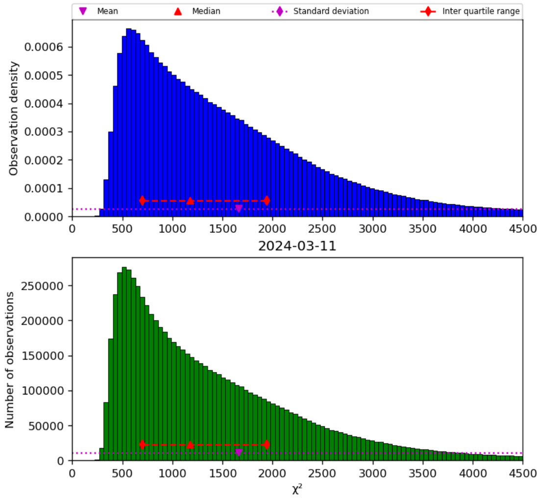
Figure 22: Histogram of “ \chi^2 ” for 2024-03-10 to 2024-03-12
