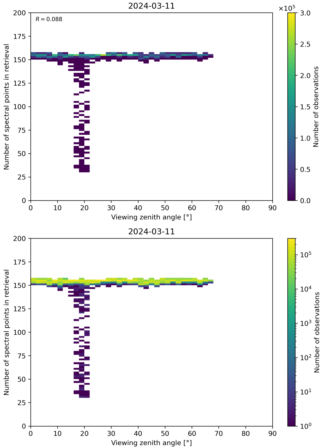
Figure 76: Scatter density plot of “Viewing zenith angle” against “Number of spectral points in retrieval” for 2024-03-10 to 2024-03-12.
