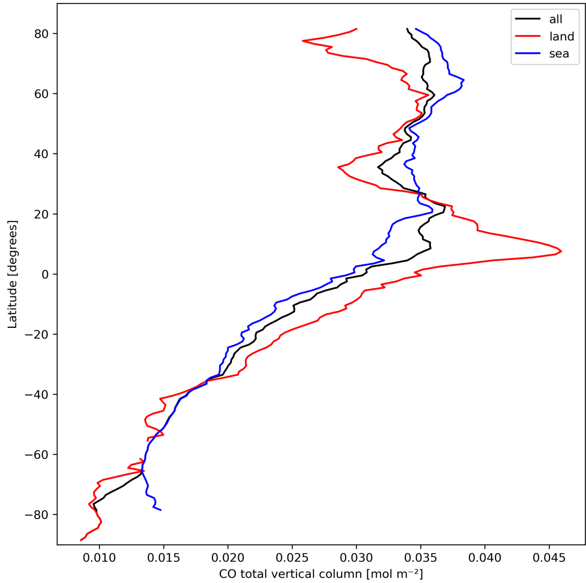
Figure 10: Zonal average of “CO total vertical column” for 2024-03-10 to 2024-03-12.
