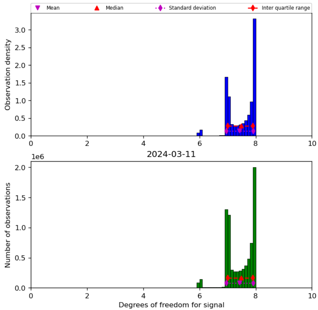
Figure 23: Histogram of “Degrees of freedom for signal” for 2024-03-10 to 2024-03-12
