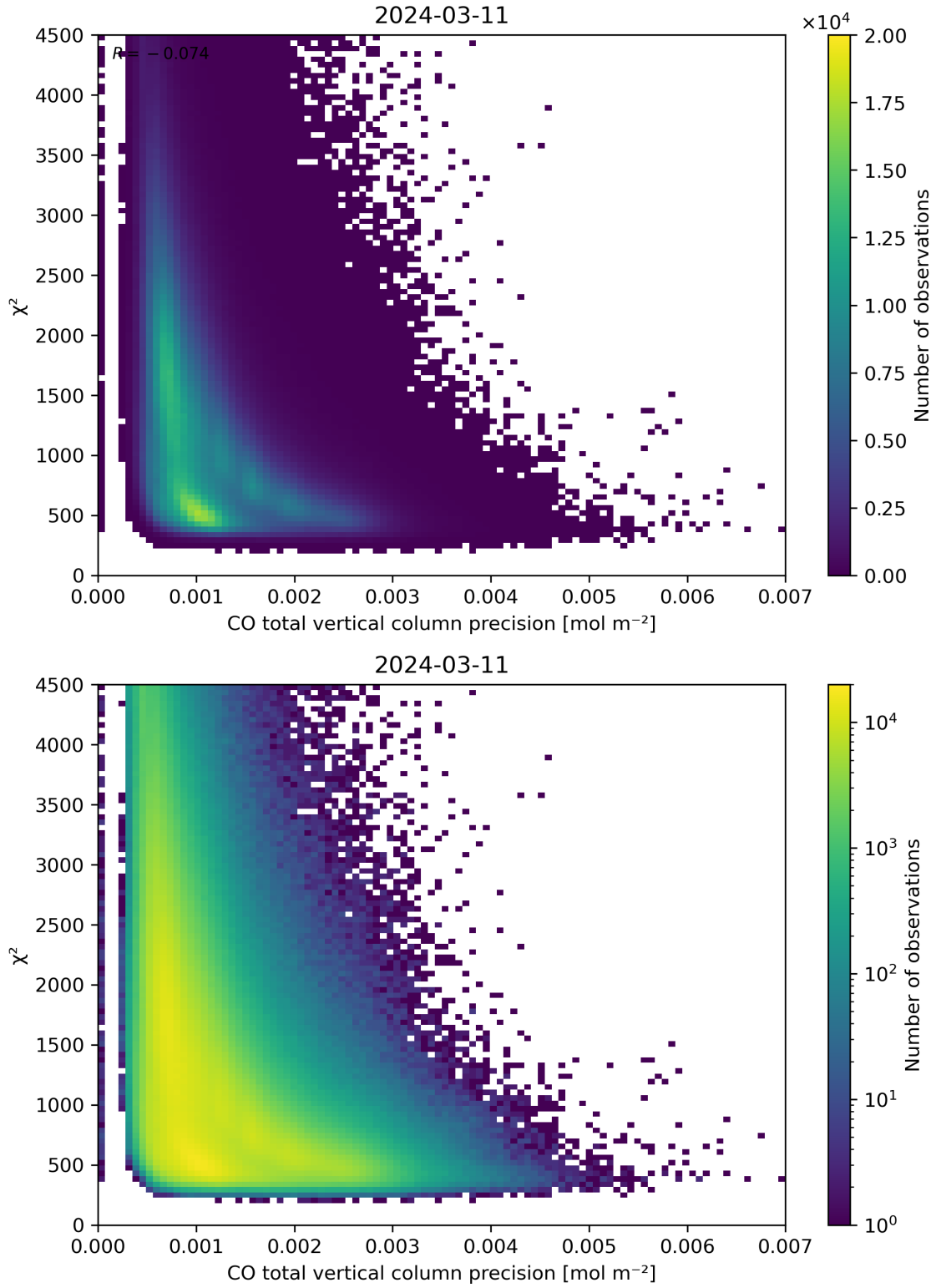
Figure 44: Scatter density plot of “CO total vertical column precision” against “ \chi^2 ” for 2024-03-10 to 2024-03-12.
