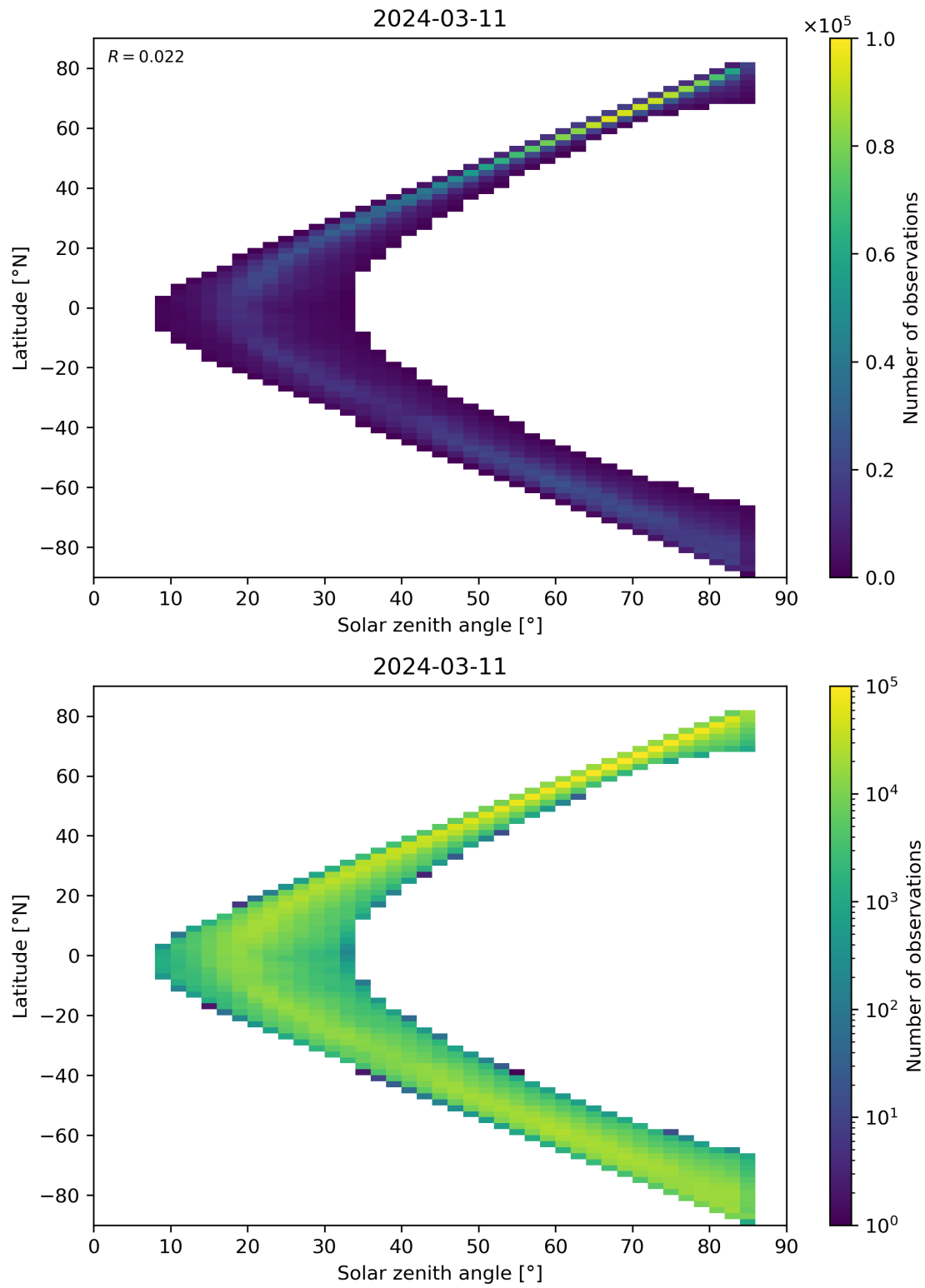
Figure 66: Scatter density plot of “Solar zenith angle” against “Latitude” for 2024-03-10 to 2024-03-12.
