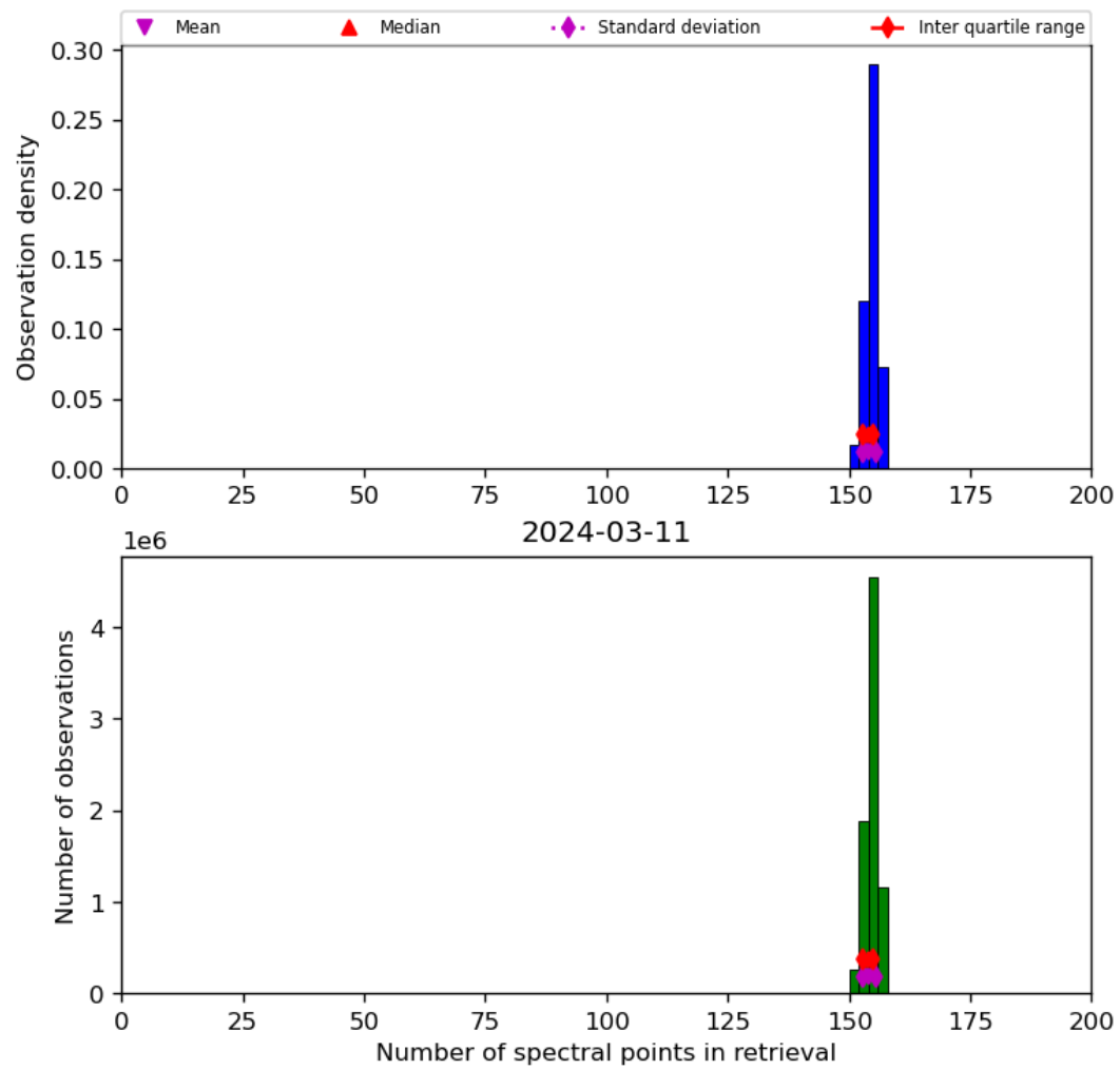
Figure 21: Histogram of “Number of spectral points in retrieval” for 2024-03-10 to 2024-03-12
