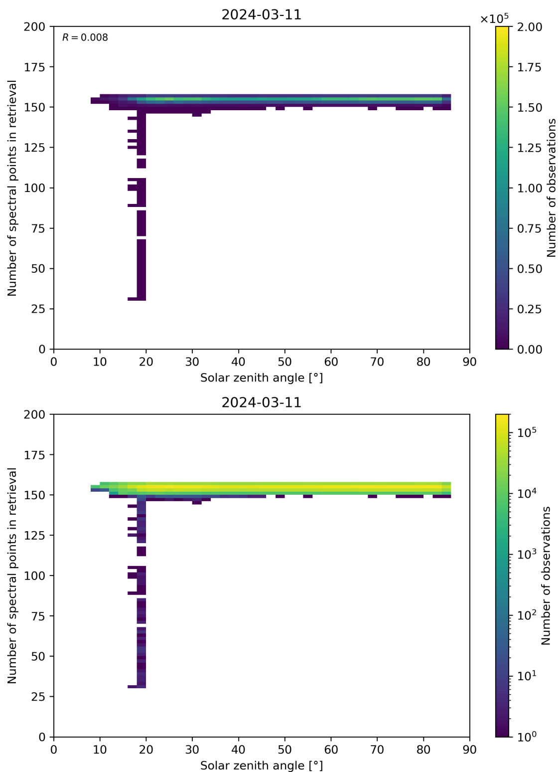
Figure 68: Scatter density plot of “Solar zenith angle” against “Number of spectral points in retrieval” for 2024-03-10 to 2024-03-12.
