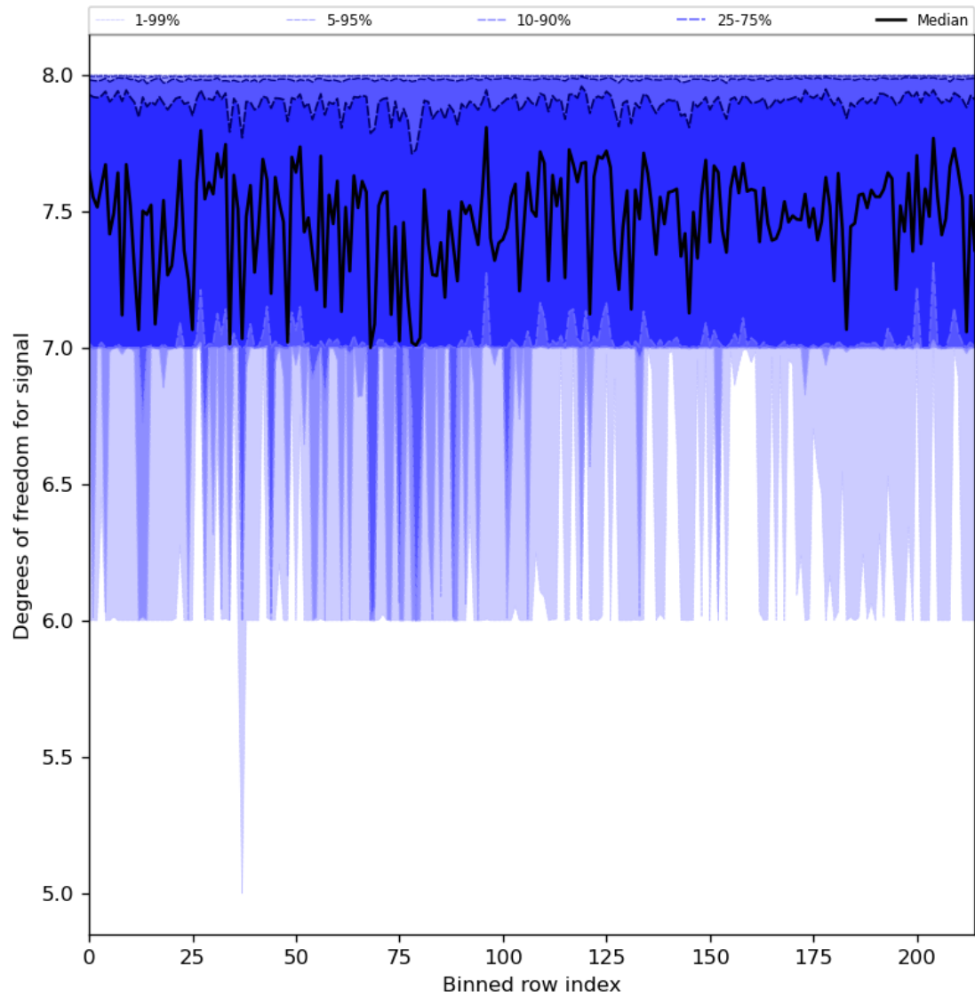
Figure 31: Along track statistics of “Degrees of freedom for signal” for 2024-03-10 to 2024-03-12
