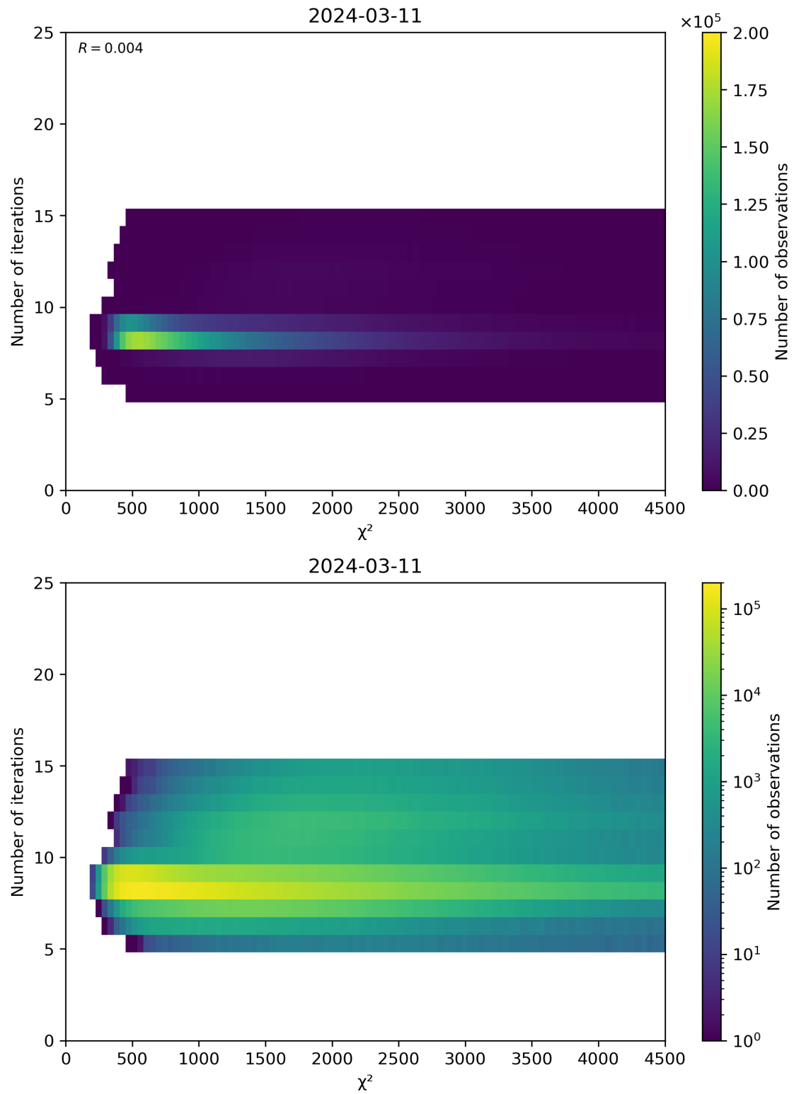
Figure 49: Scatter density plot of “ \chi^2 ” against “Number of iterations” for 2024-03-10 to 2024-03-12.
