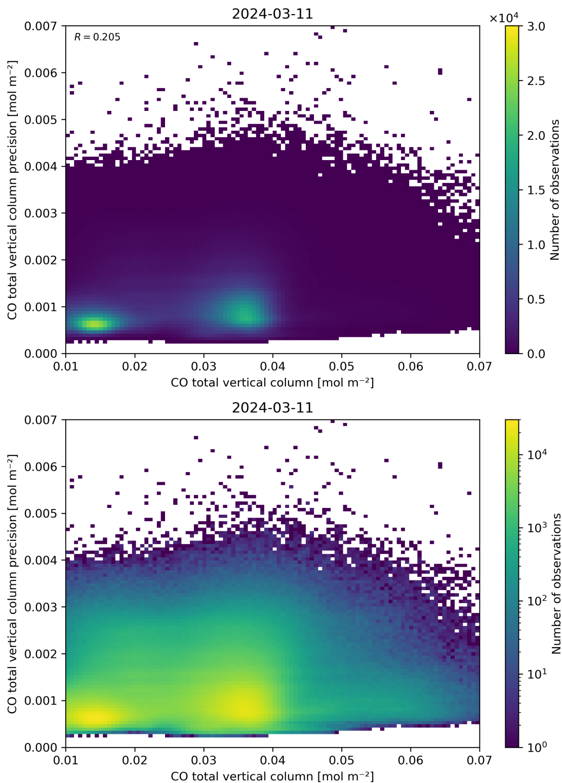
Figure 34: Scatter density plot of “CO total vertical column” against “CO total vertical column precision” for 2024-03-10 to 2024-03-12.
