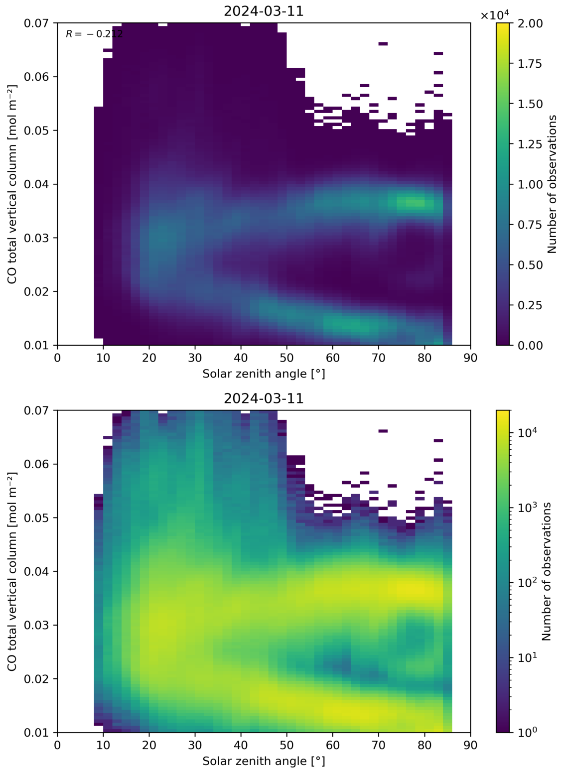
Figure 61: Scatter density plot of “Solar zenith angle” against “CO total vertical column” for 2024-03-10 to 2024-03-12.
