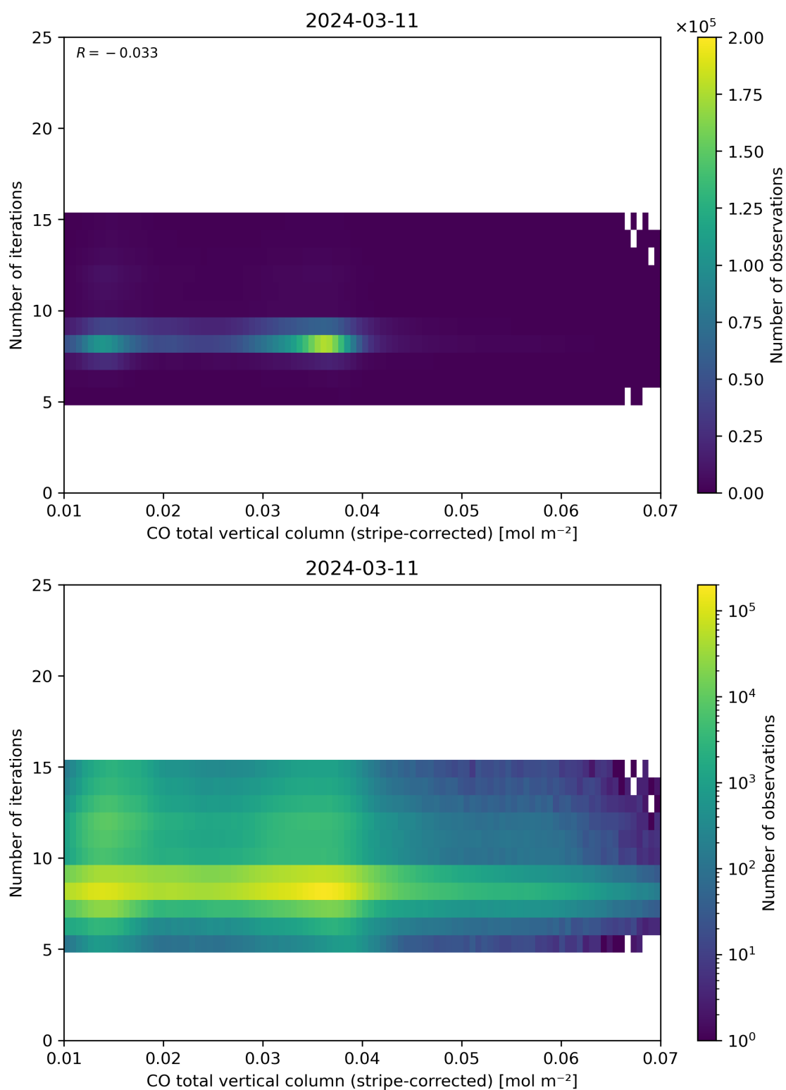
Figure 39: Scatter density plot of “CO total vertical column (stripe-corrected)” against “Number of iterations” for 2024-03-10 to 2024-03-12.
