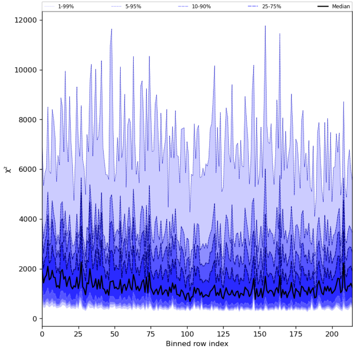
Figure 30: Along track statistics of “ \chi^2 ” for 2024-03-10 to 2024-03-12
