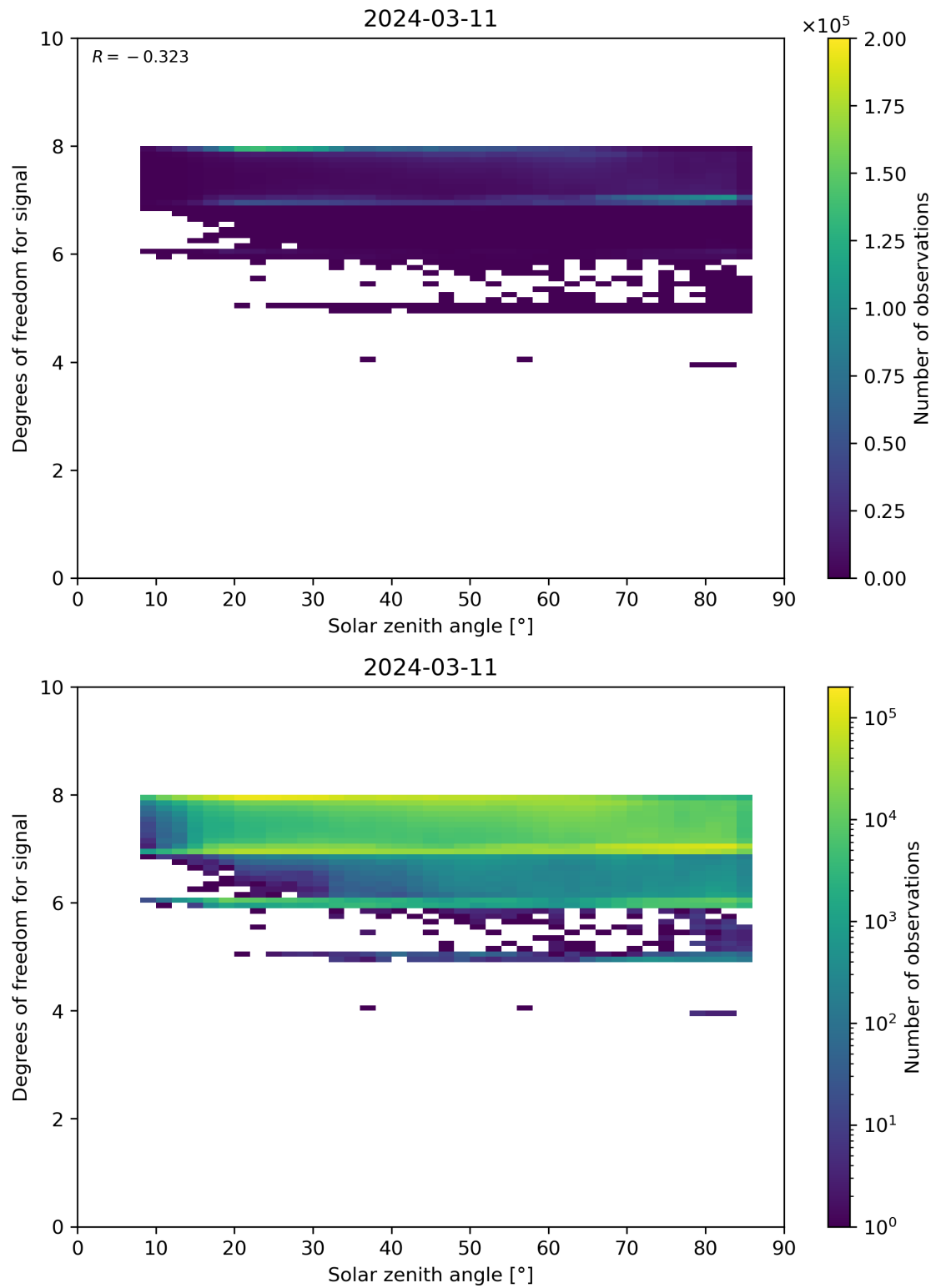
Figure 65: Scatter density plot of “Solar zenith angle” against “Degrees of freedom for signal” for 2024-03-10 to 2024-03-12.
