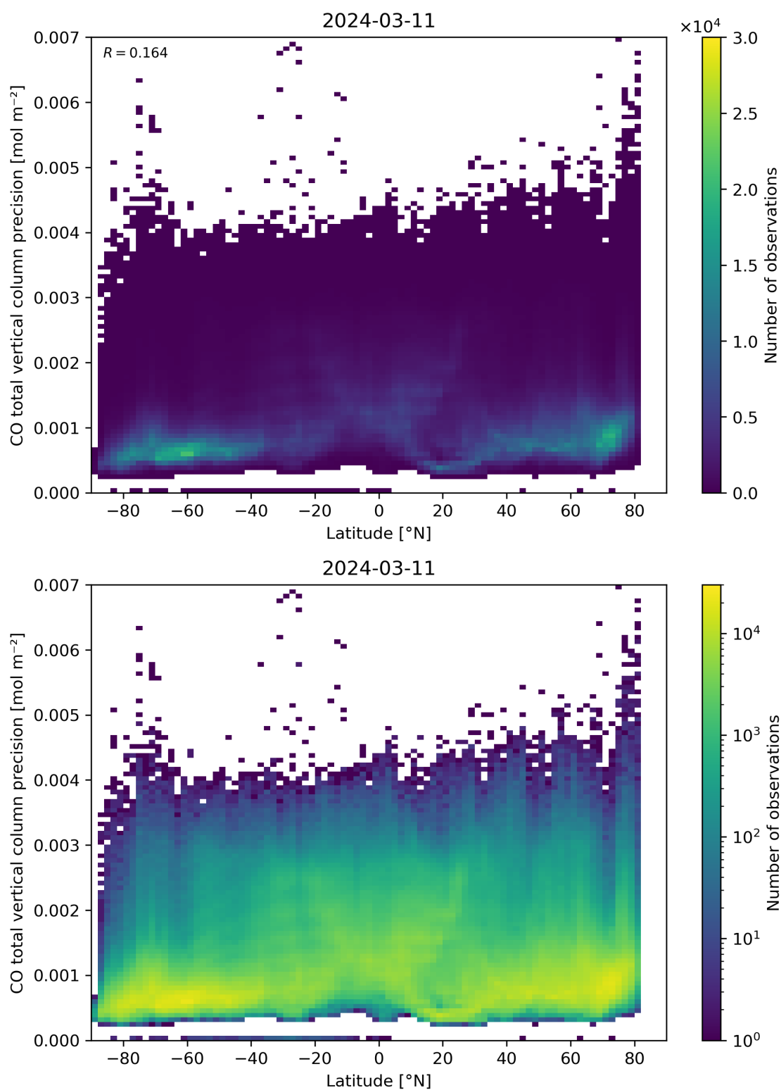
Figure 53: Scatter density plot of “Latitude” against “CO total vertical column precision” for 2024-03-10 to 2024-03-12.
