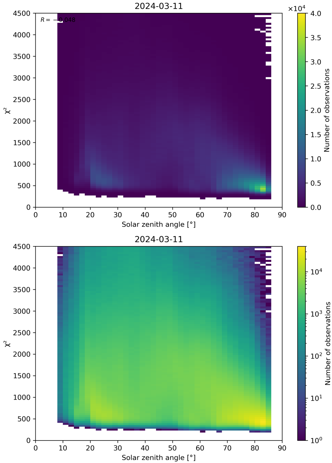
Figure 64: Scatter density plot of “Solar zenith angle” against “ \chi^2 ” for 2024-03-10 to 2024-03-12.
