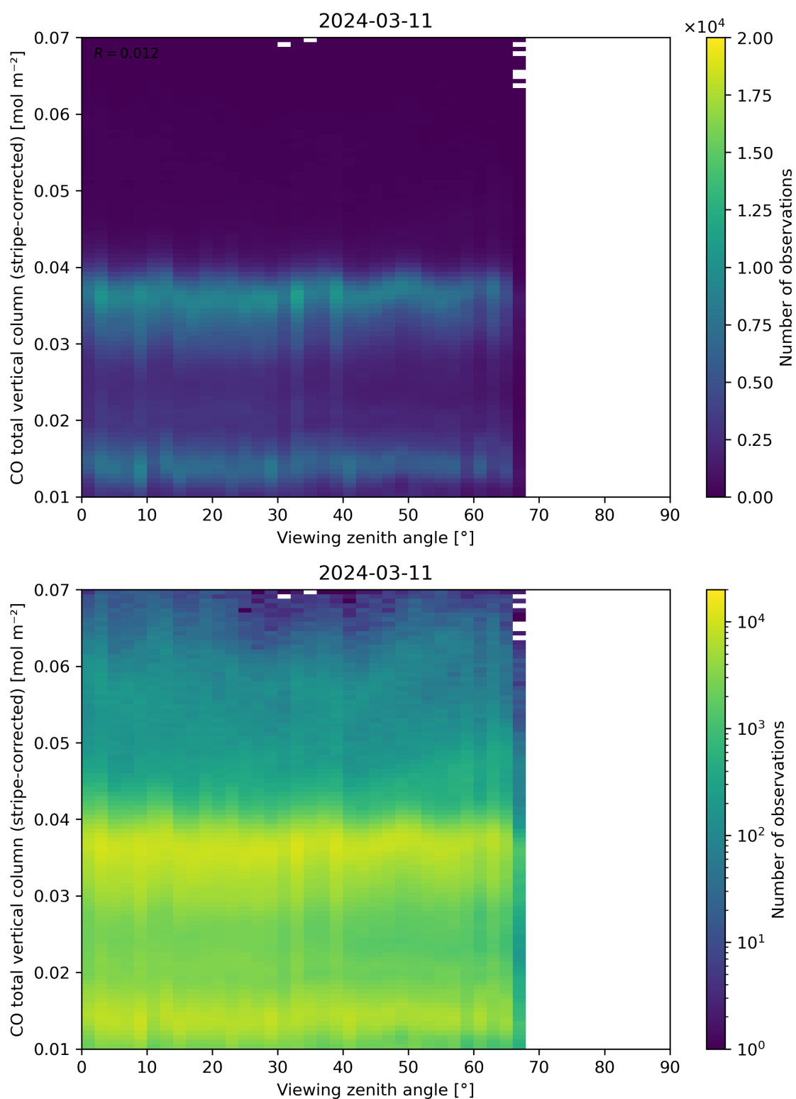
Figure 70: Scatter density plot of “Viewing zenith angle” against “CO total vertical column (stripe-corrected)” for 2024-03-10 to 2024-03-12.
