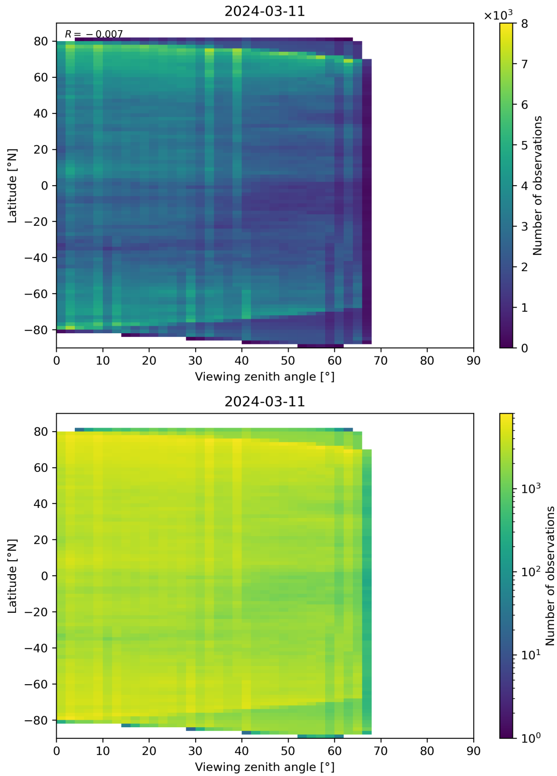
Figure 74: Scatter density plot of “Viewing zenith angle” against “Latitude” for 2024-03-10 to 2024-03-12.
