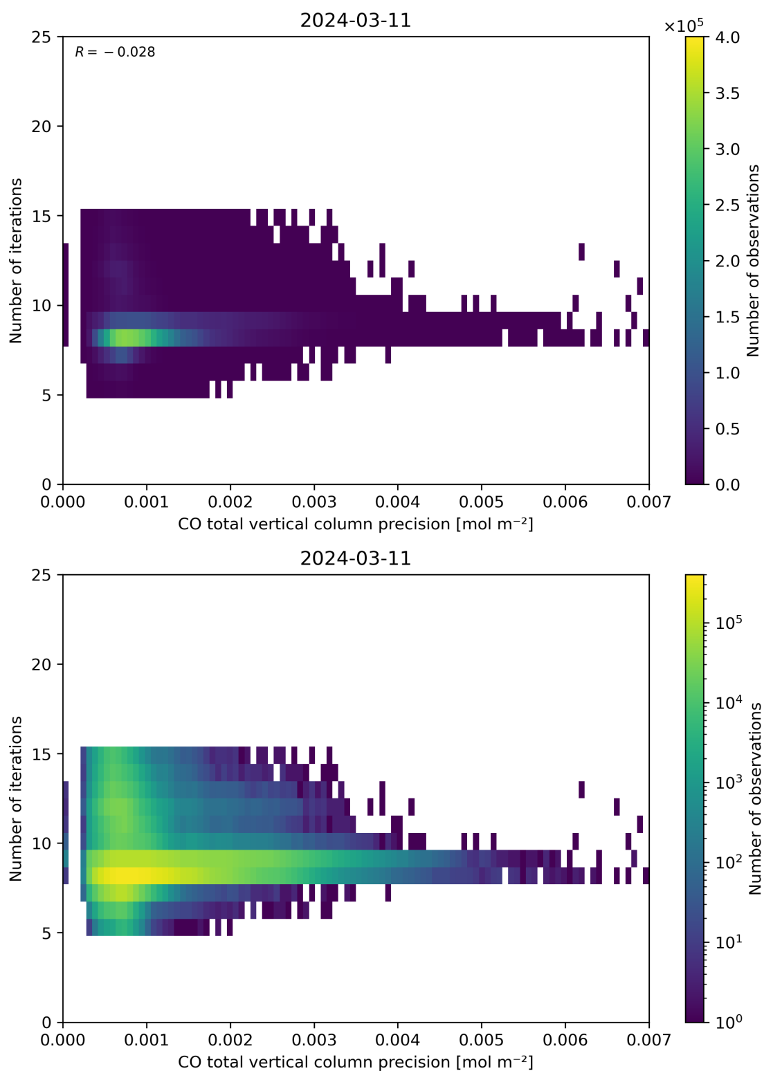
Figure 46: Scatter density plot of “CO total vertical column precision” against “Number of iterations” for 2024-03-10 to 2024-03-12.
