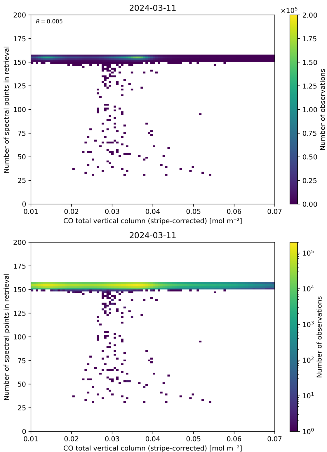
Figure 40: Scatter density plot of “CO total vertical column (stripe-corrected)” against “Number of spectral points in retrieval” for 2024-03-10 to 2024-03-12.
