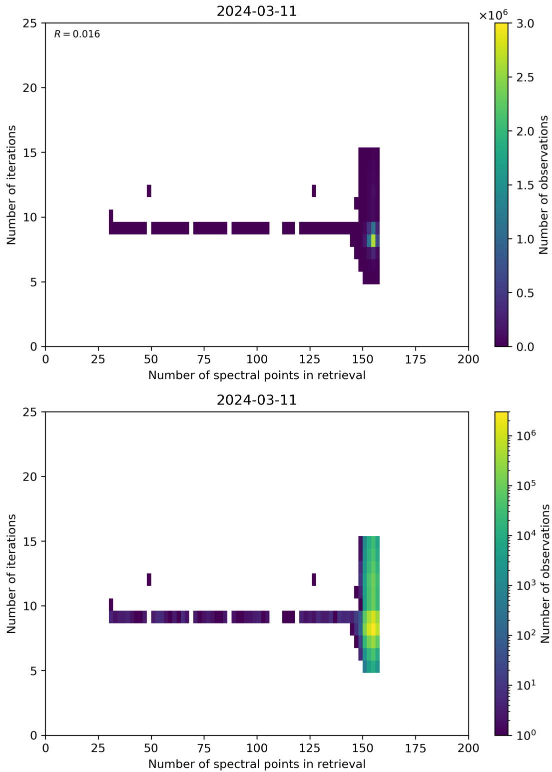
Figure 60: Scatter density plot of “Number of spectral points in retrieval” against “Number of iterations” for 2024-03-10 to 2024-03-12.
