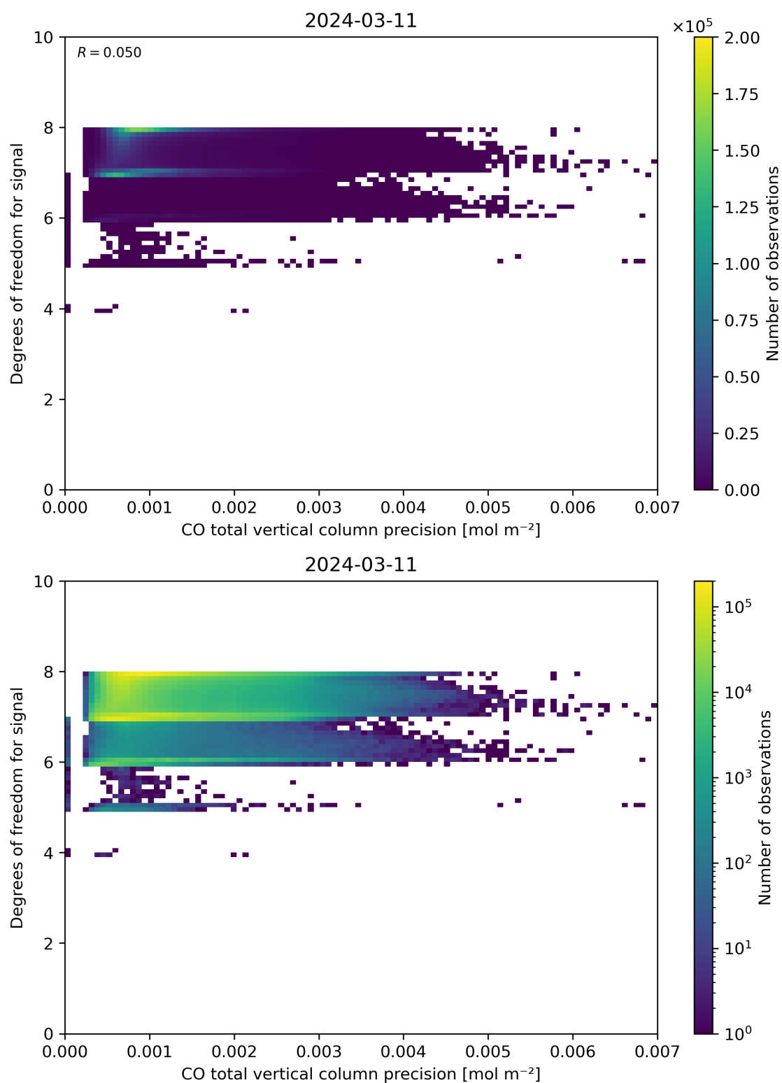
Figure 45: Scatter density plot of “CO total vertical column precision” against “Degrees of freedom for signal” for 2024-03-10 to 2024-03-12.
