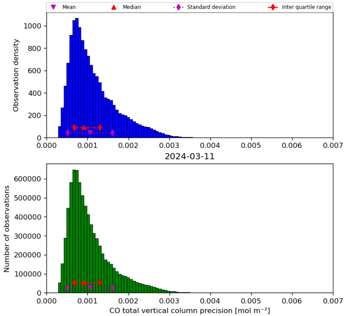
Figure 20: Histogram of “CO total vertical column precision” for 2024-03-10 to 2024-03-12
