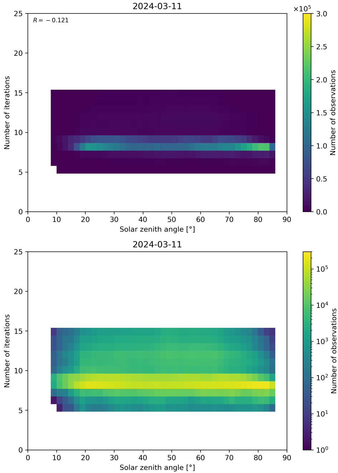
Figure 67: Scatter density plot of “Solar zenith angle” against “Number of iterations” for 2024-03-10 to 2024-03-12.
