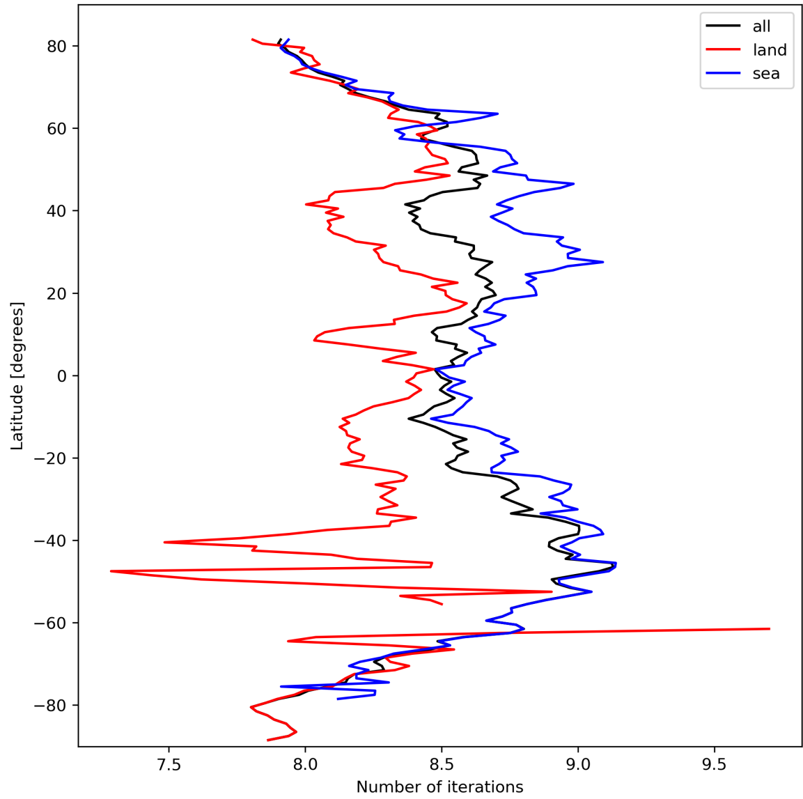
Figure 16: Zonal average of “Number of iterations” for 2024-03-10 to 2024-03-12.
