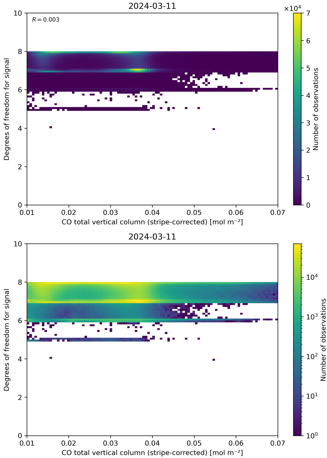
Figure 38: Scatter density plot of “CO total vertical column (stripe-corrected)” against “Degrees of freedom for signal” for 2024-03-10 to 2024-03-12.
