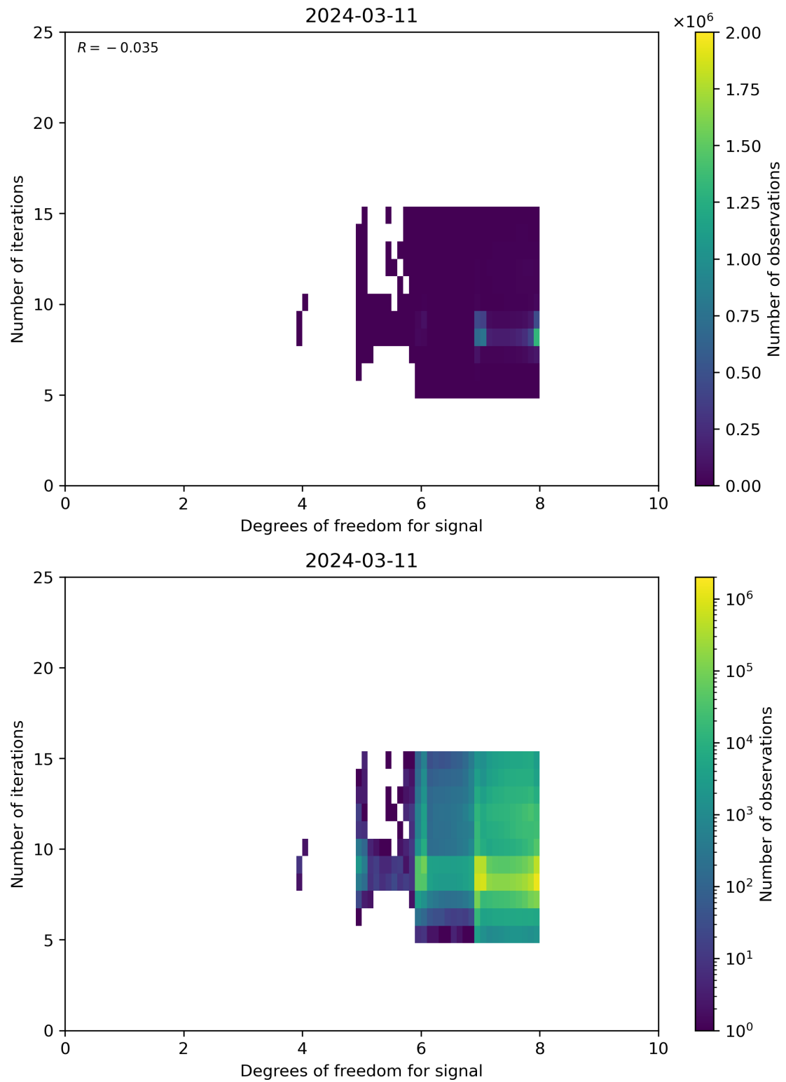
Figure 50: Scatter density plot of “Degrees of freedom for signal” against “Number of iterations” for 2024-03-10 to 2024-03-12.
