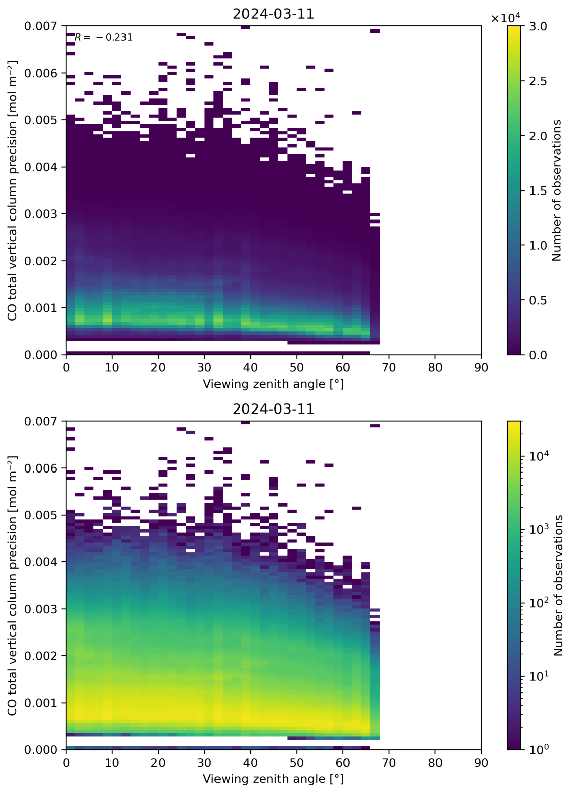
Figure 71: Scatter density plot of “Viewing zenith angle” against “CO total vertical column precision” for 2024-03-10 to 2024-03-12.
