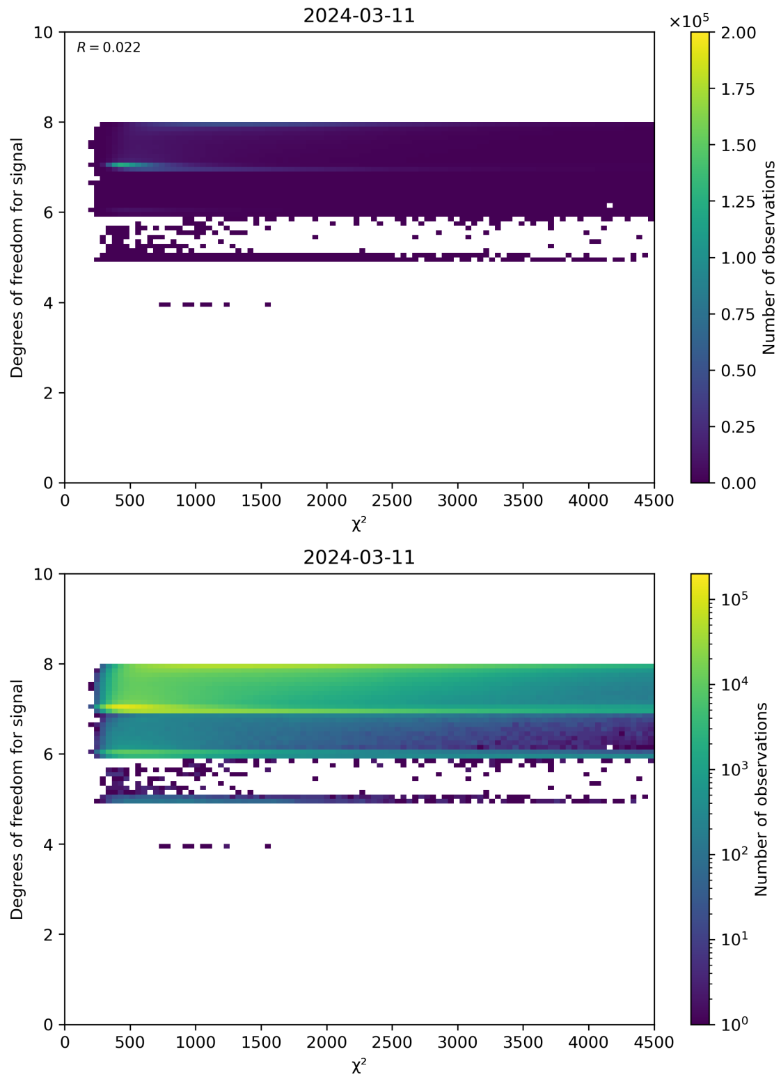
Figure 48: Scatter density plot of “ \chi^2 ” against “Degrees of freedom for signal” for 2024-03-10 to 2024-03-12.
