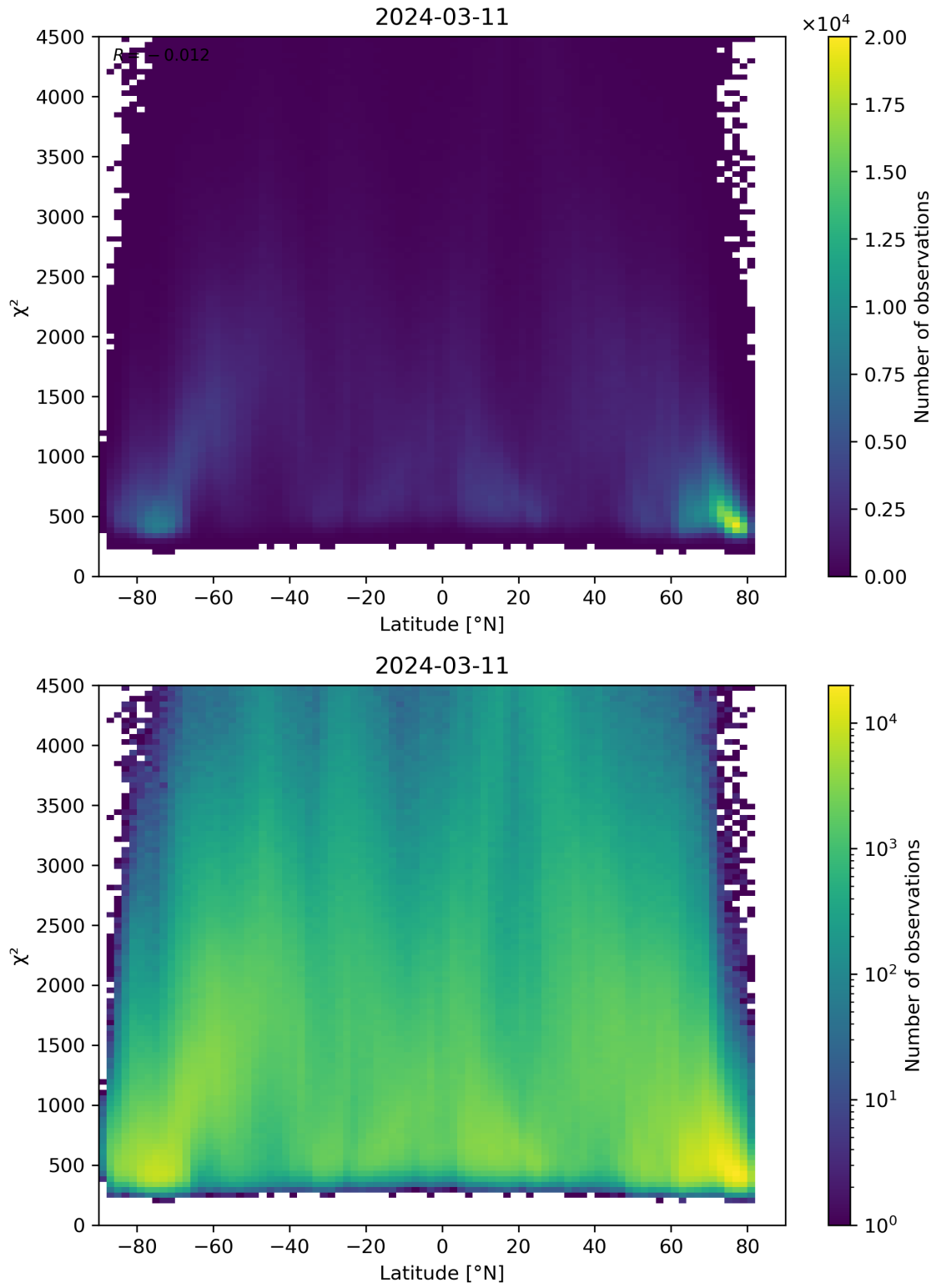
Figure 54: Scatter density plot of “Latitude” against “ \chi^2 ” for 2024-03-10 to 2024-03-12.
