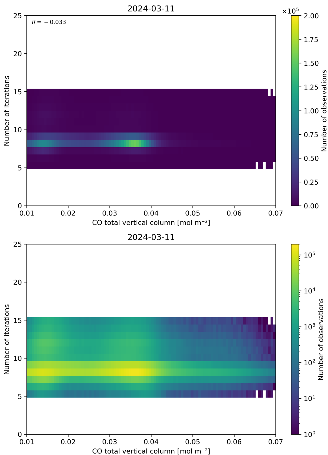
Figure 42: Scatter density plot of “CO total vertical column” against “Number of iterations” for 2024-03-10 to 2024-03-12.
