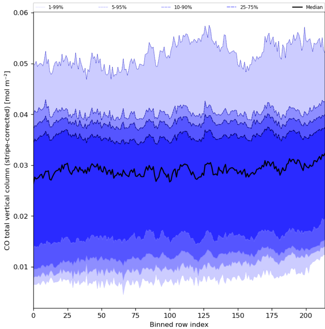
Figure 27: Along track statistics of “CO total vertical column (stripe-corrected)” for 2024-03-10 to 2024-03-12
