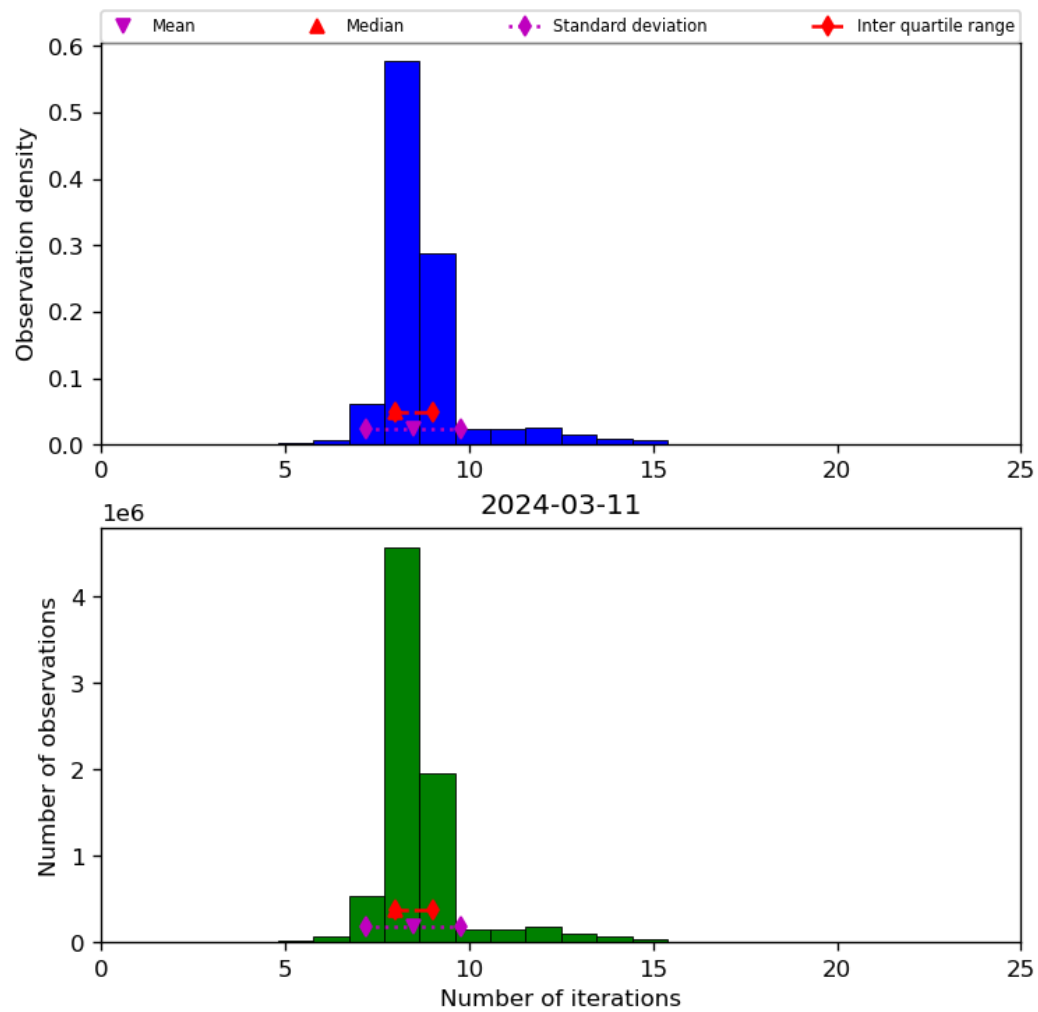
Figure 24: Histogram of “Number of iterations” for 2024-03-10 to 2024-03-12
