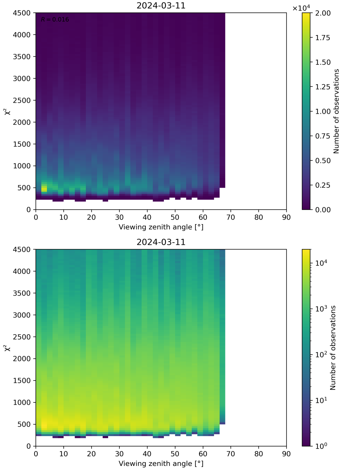
Figure 72: Scatter density plot of “Viewing zenith angle” against “ \chi^2 ” for 2024-03-10 to 2024-03-12.
