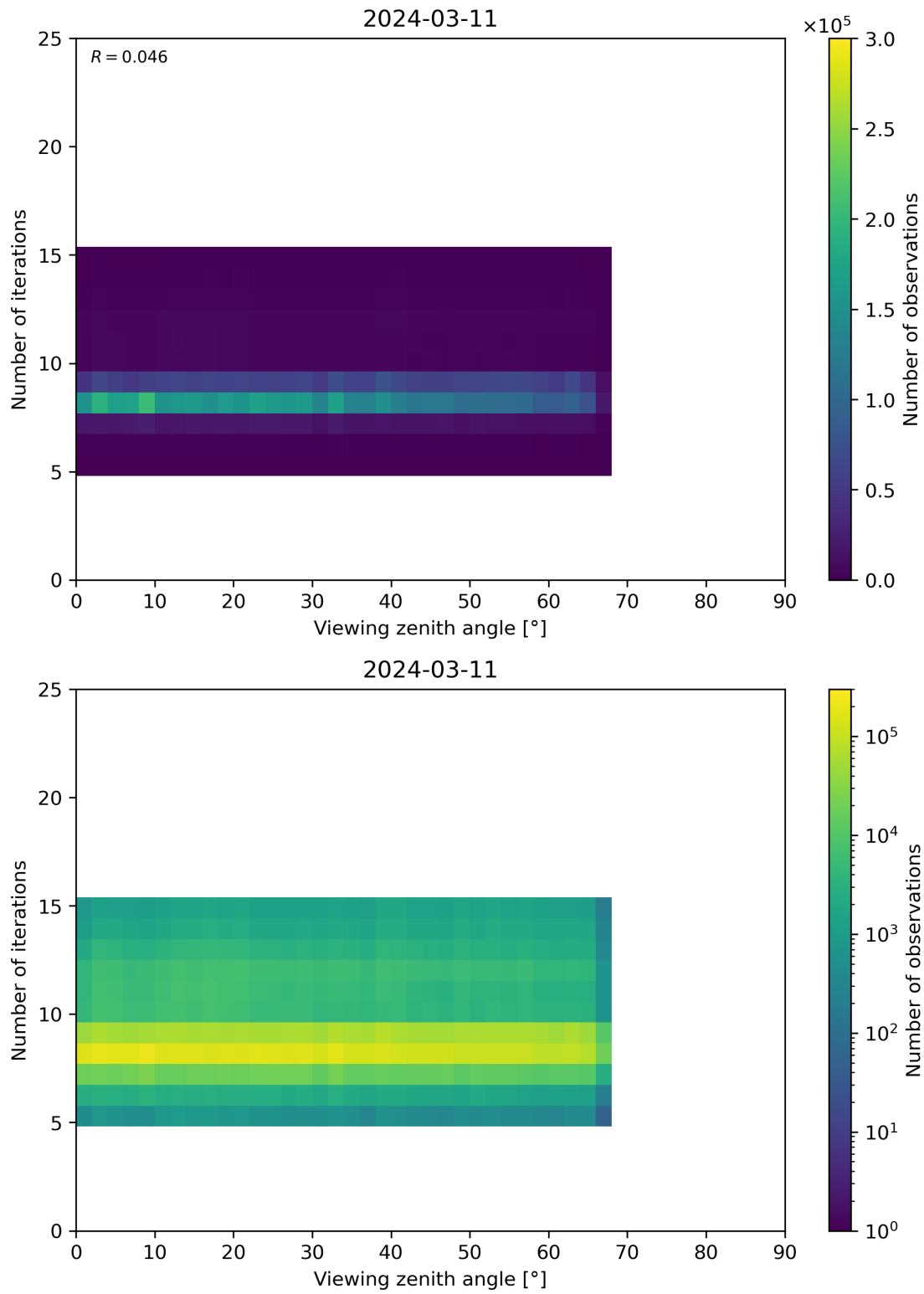
Figure 75: Scatter density plot of “Viewing zenith angle” against “Number of iterations” for 2024-03-10 to 2024-03-12.
