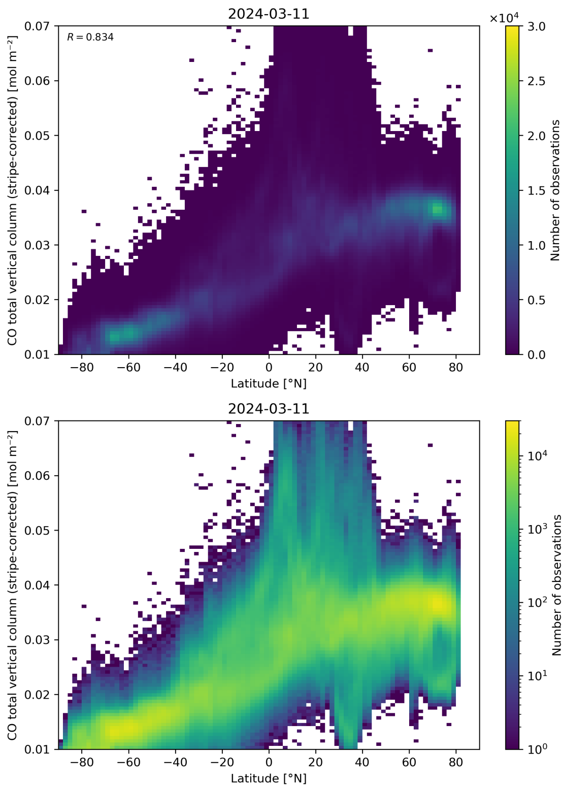
Figure 52: Scatter density plot of “Latitude” against “CO total vertical column (stripe-corrected)” for 2024-03-10 to 2024-03-12.
