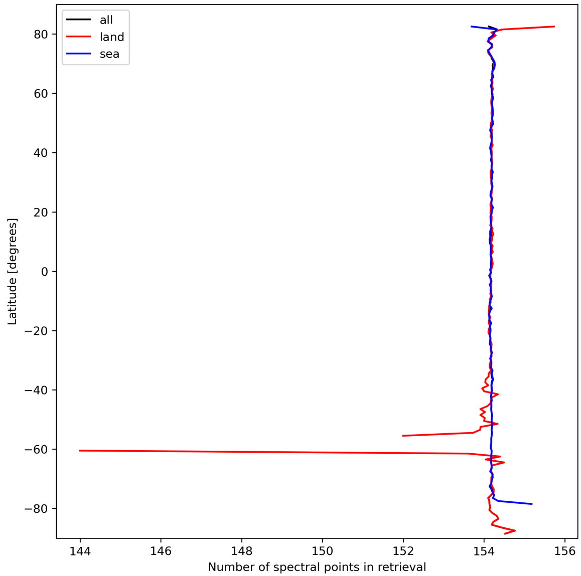
Figure 13: Zonal average of “Number of spectral points in retrieval” for 2024-03-11 to 2024-03-13.
