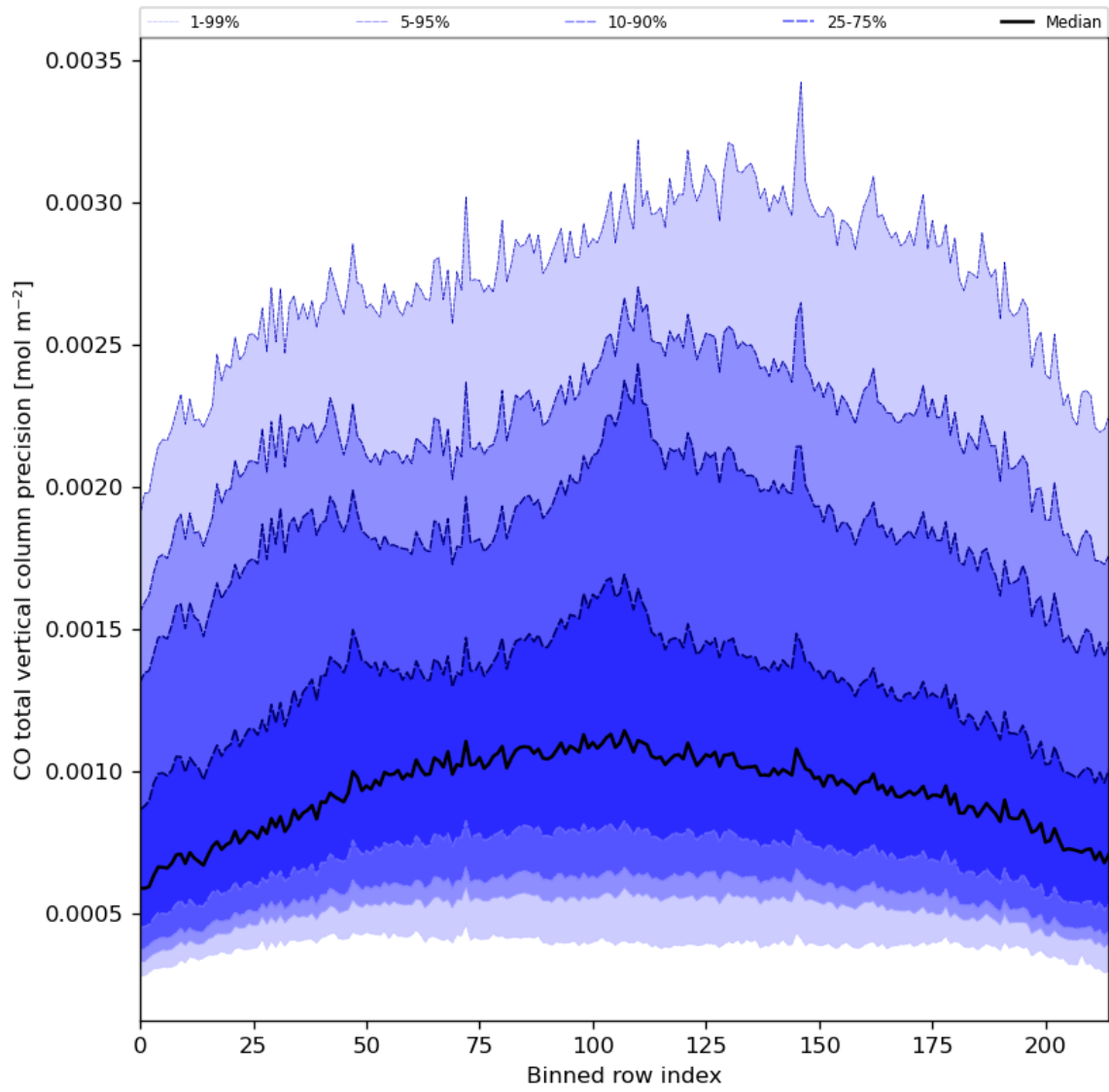
Figure 28: Along track statistics of “CO total vertical column precision” for 2024-03-11 to 2024-03-13
