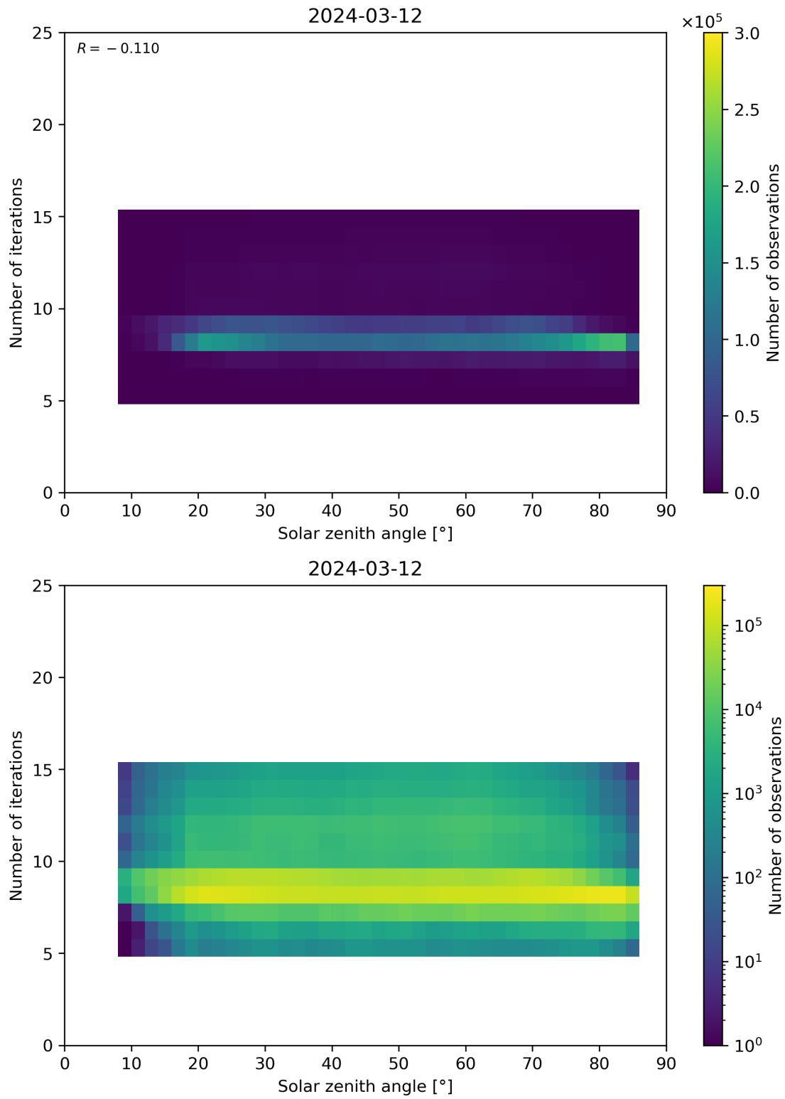
Figure 67: Scatter density plot of “Solar zenith angle” against “Number of iterations” for 2024-03-11 to 2024-03-13.
