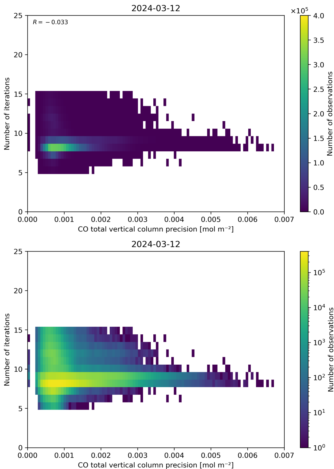
Figure 46: Scatter density plot of “CO total vertical column precision” against “Number of iterations” for 2024-03-11 to 2024-03-13.
