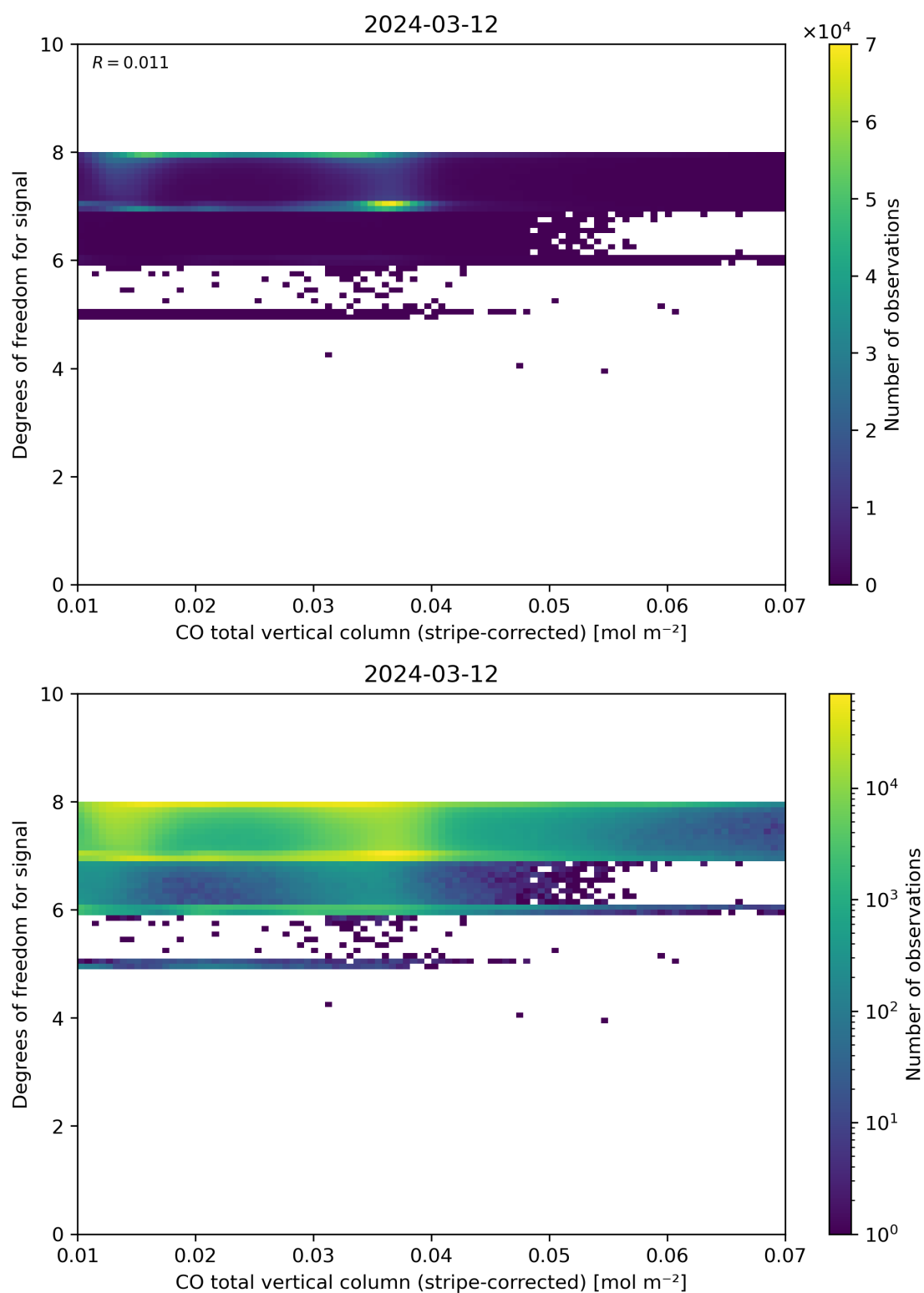
Figure 38: Scatter density plot of “CO total vertical column (stripe-corrected)” against “Degrees of freedom for signal” for 2024-03-11 to 2024-03-13.
