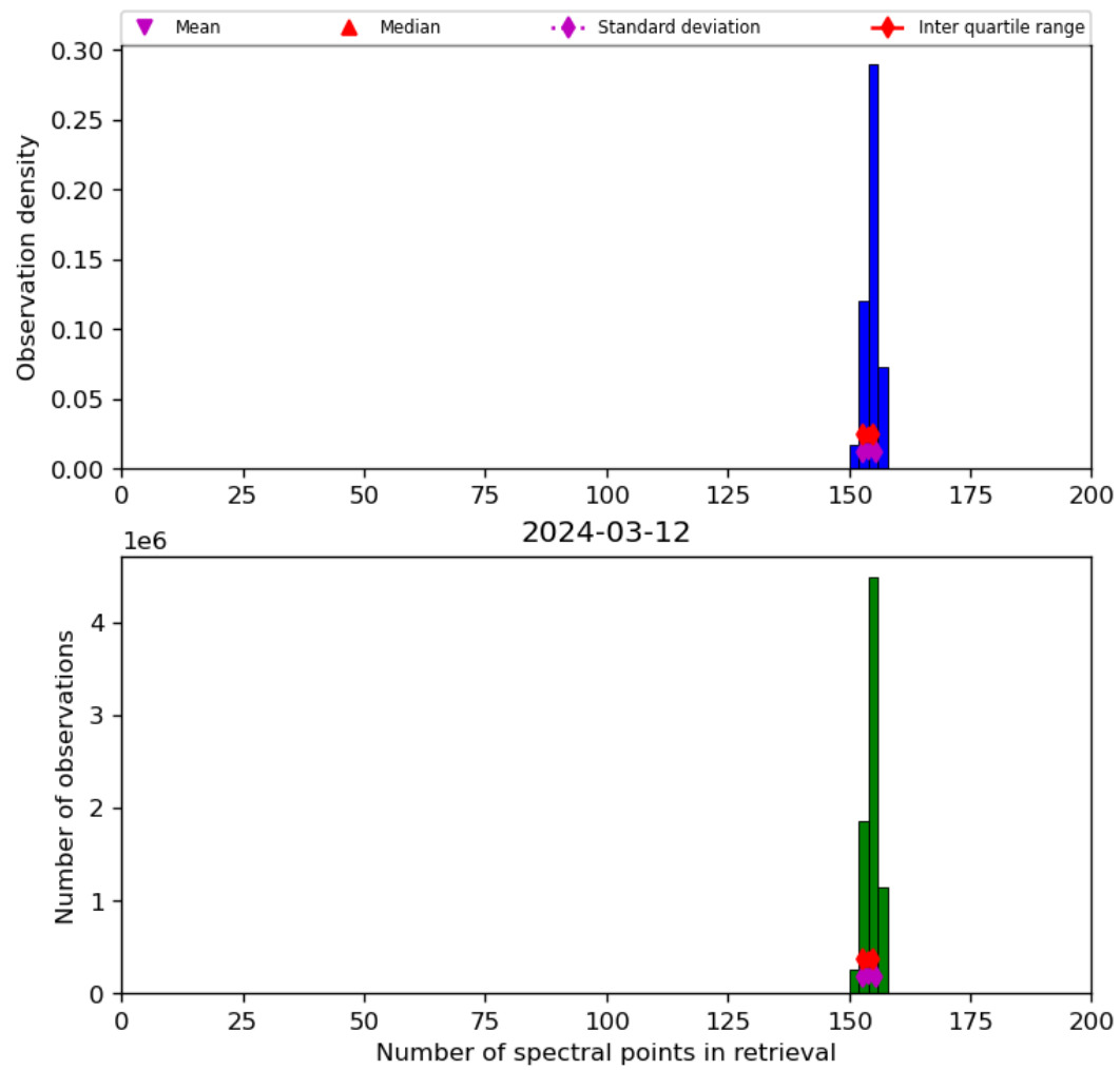
Figure 21: Histogram of “Number of spectral points in retrieval” for 2024-03-11 to 2024-03-13
