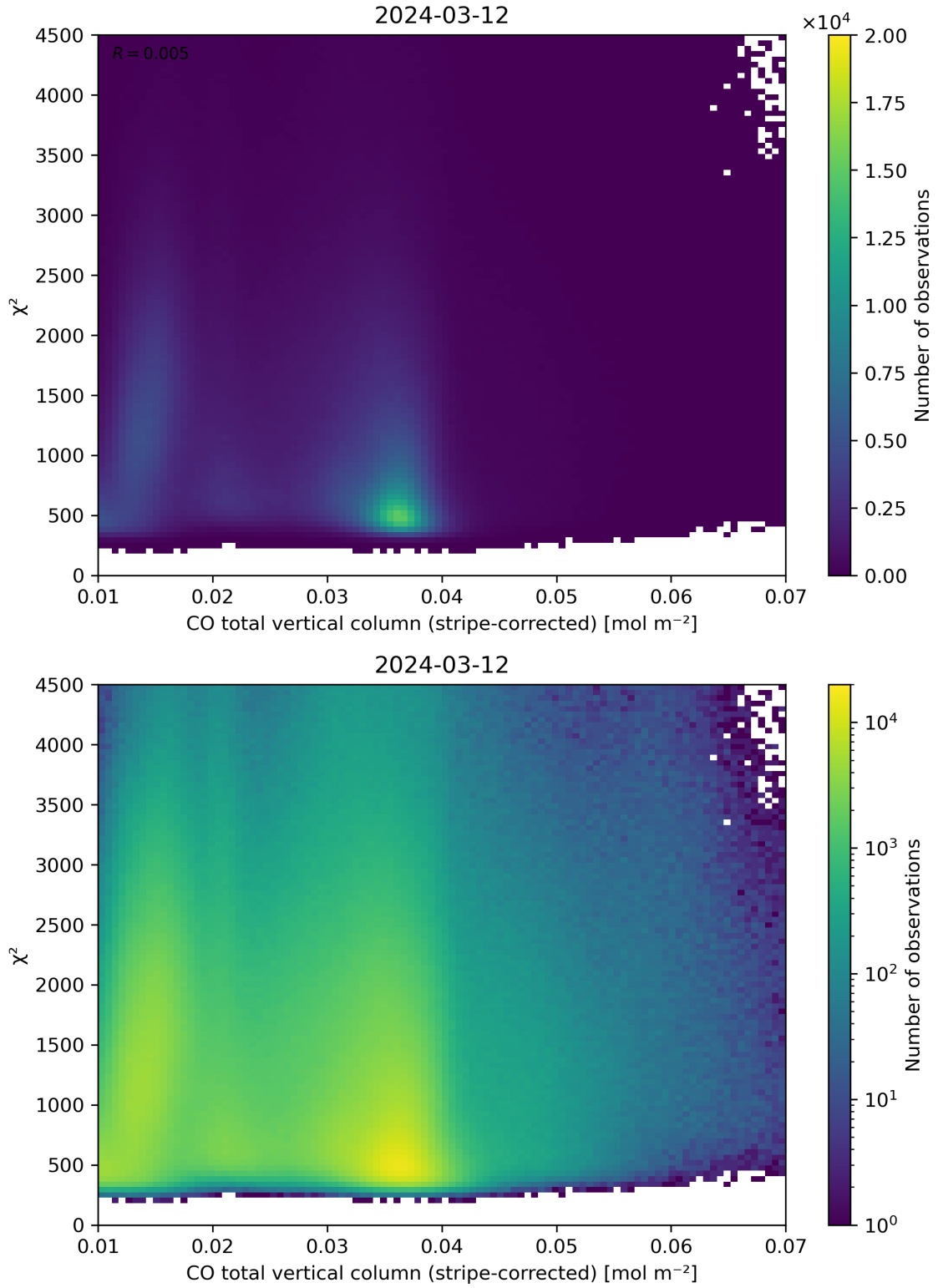
Figure 37: Scatter density plot of “CO total vertical column (stripe-corrected)” against “ \chi^2 ” for 2024-03-11 to 2024-03-13.
