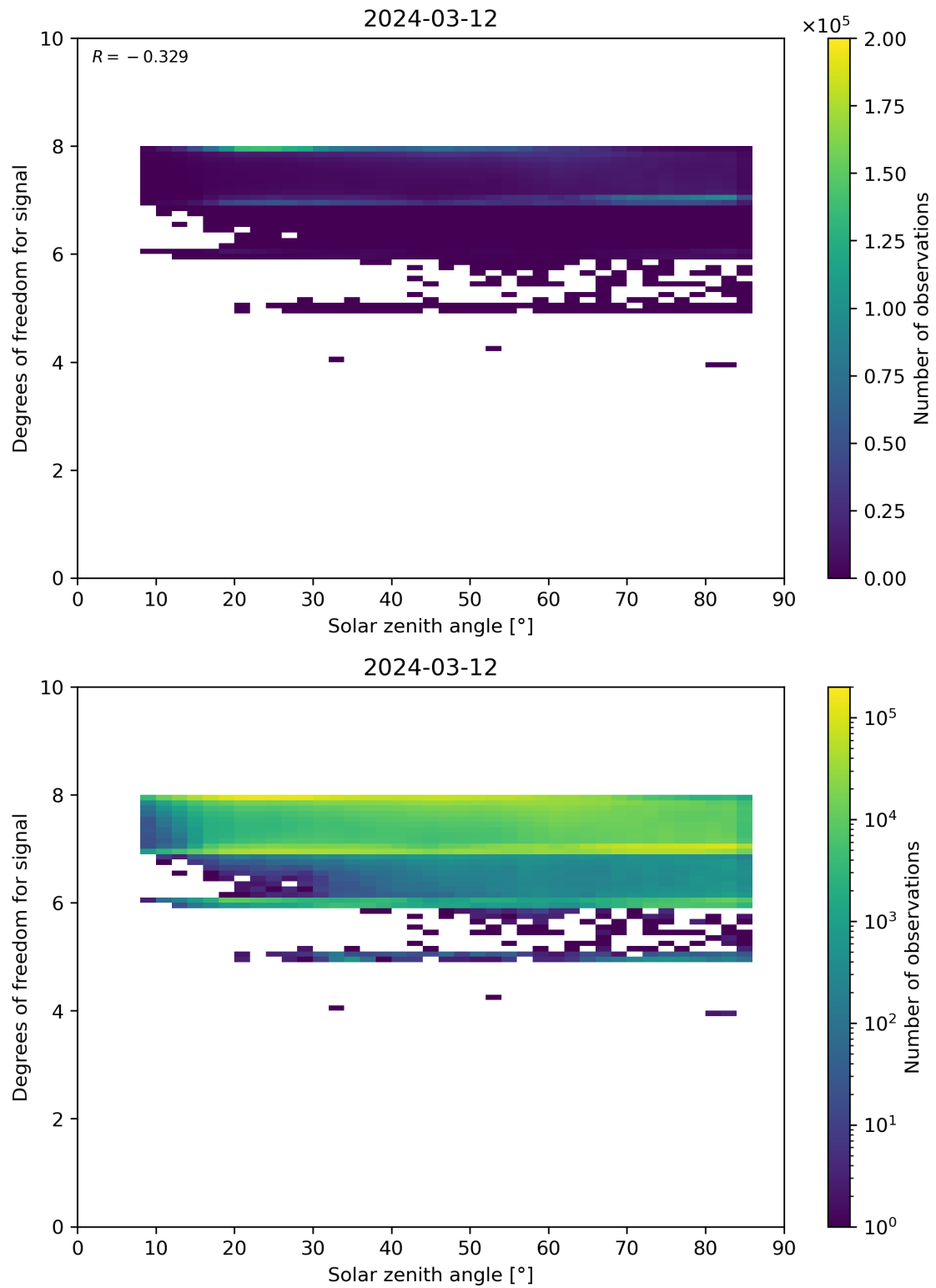
Figure 65: Scatter density plot of “Solar zenith angle” against “Degrees of freedom for signal” for 2024-03-11 to 2024-03-13.
