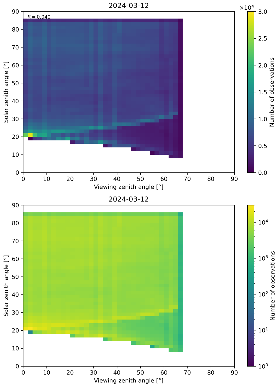
Figure 77: Scatter density plot of “Viewing zenith angle” against “Solar zenith angle” for 2024-03-11 to 2024-03-13.
