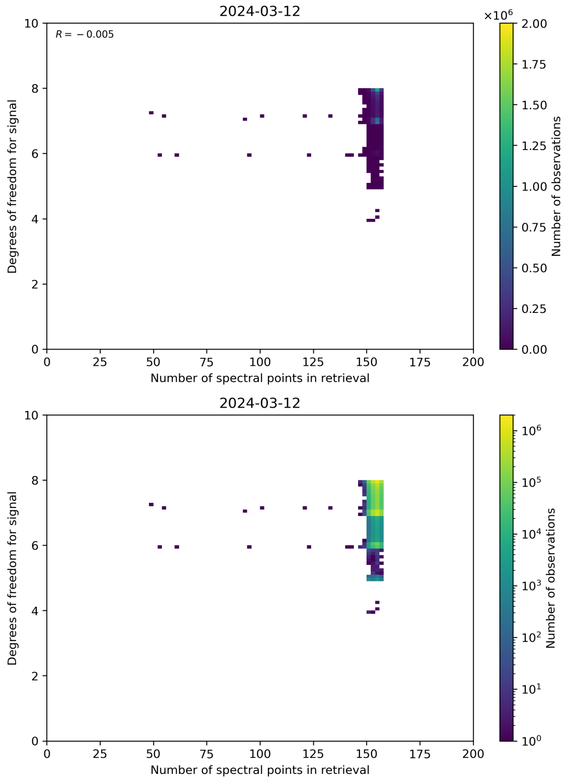
Figure 59: Scatter density plot of “Number of spectral points in retrieval” against “Degrees of freedom for signal” for 2024-03-11 to 2024-03-13.
