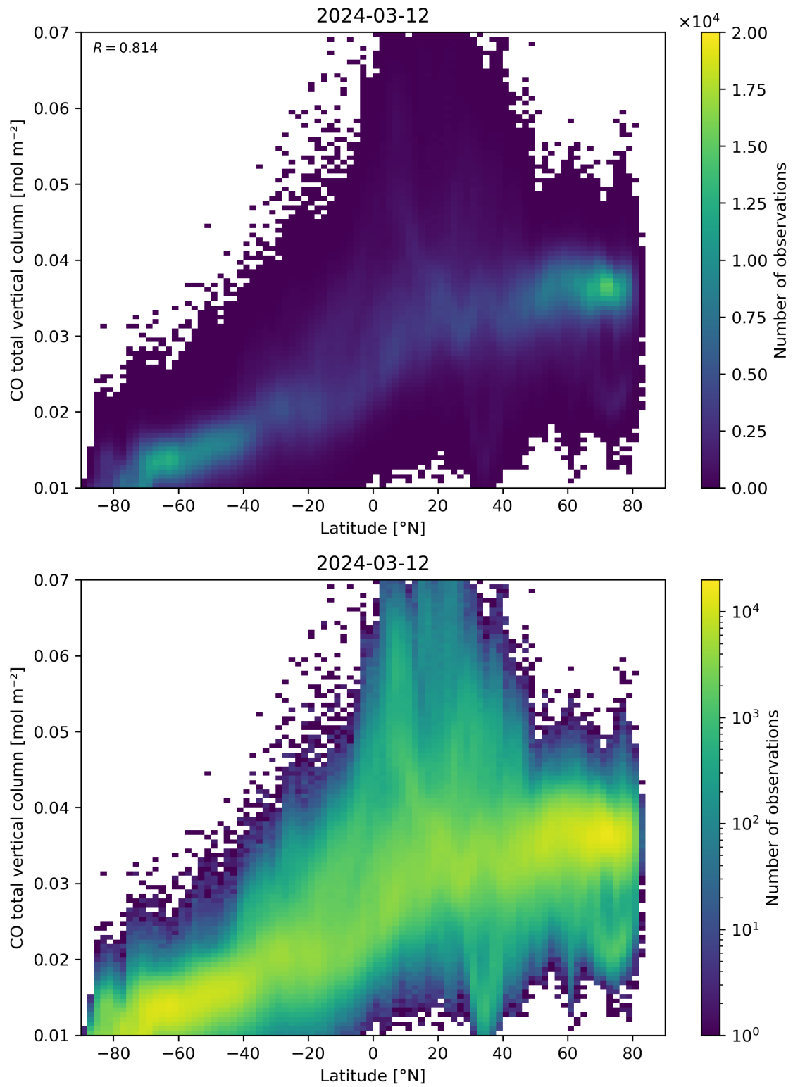
Figure 51: Scatter density plot of “Latitude” against “CO total vertical column” for 2024-03-11 to 2024-03-13.
