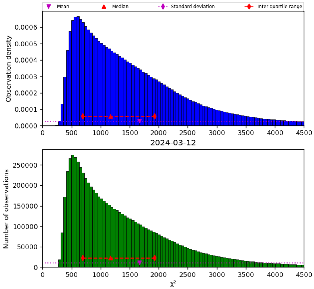
Figure 22: Histogram of “ \chi^2 ” for 2024-03-11 to 2024-03-13
