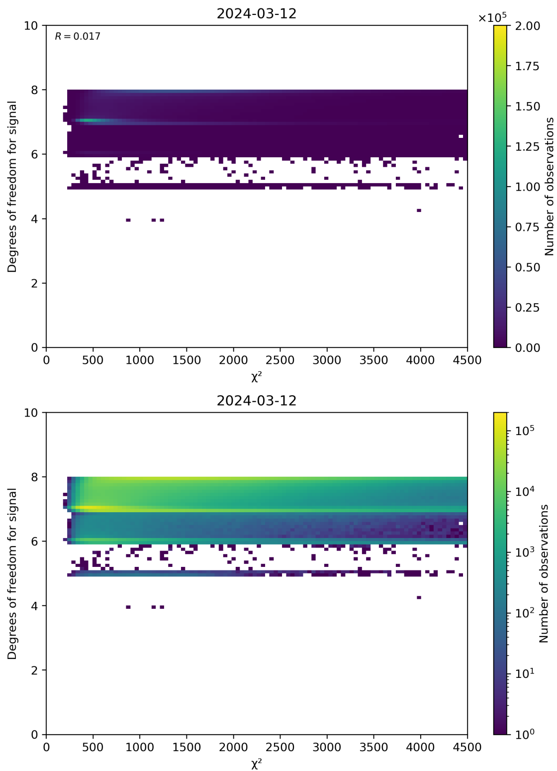
Figure 48: Scatter density plot of “ \chi^2 ” against “Degrees of freedom for signal” for 2024-03-11 to 2024-03-13.
