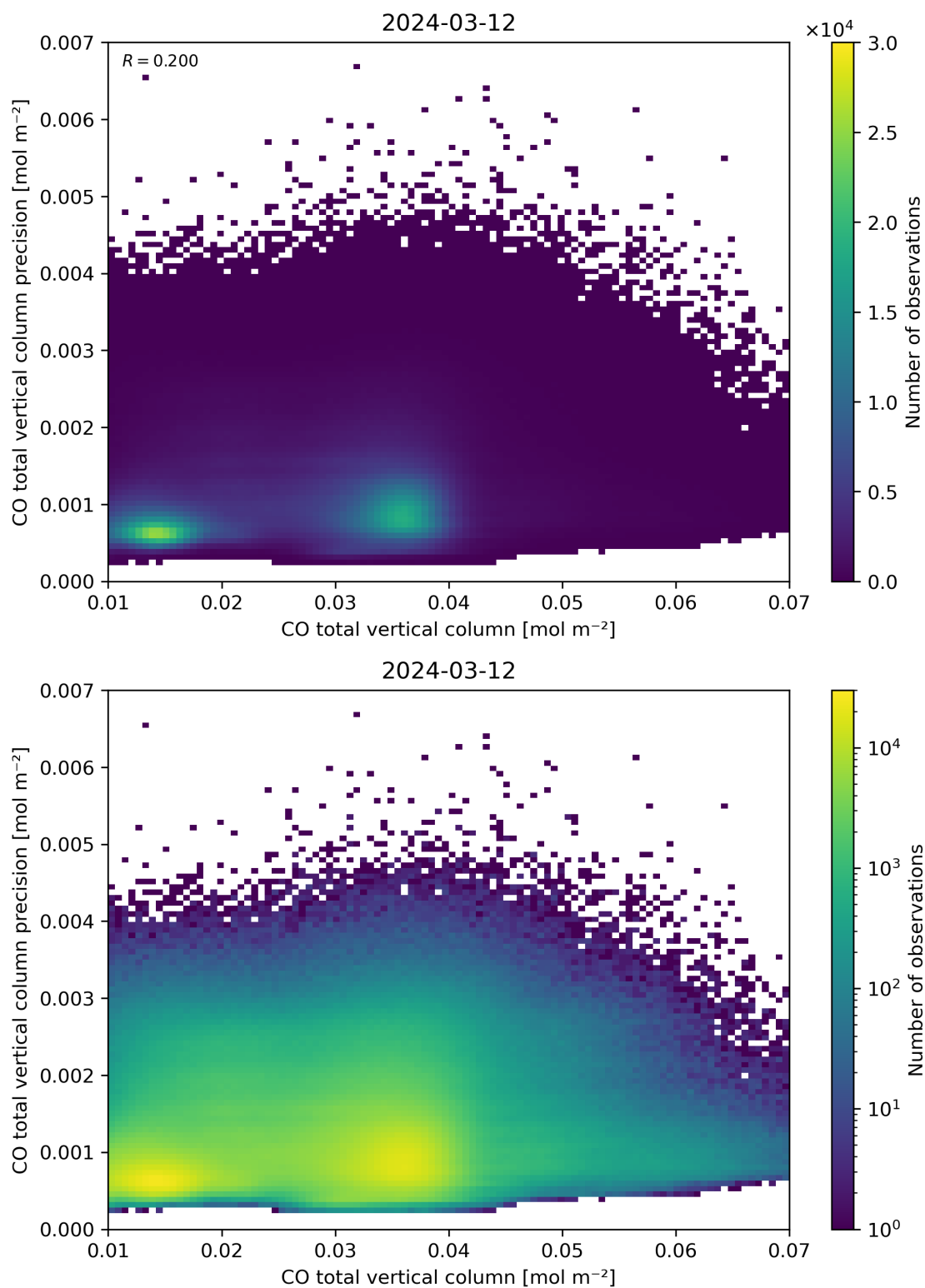
Figure 34: Scatter density plot of “CO total vertical column” against “CO total vertical column precision” for 2024-03-11 to 2024-03-13.
