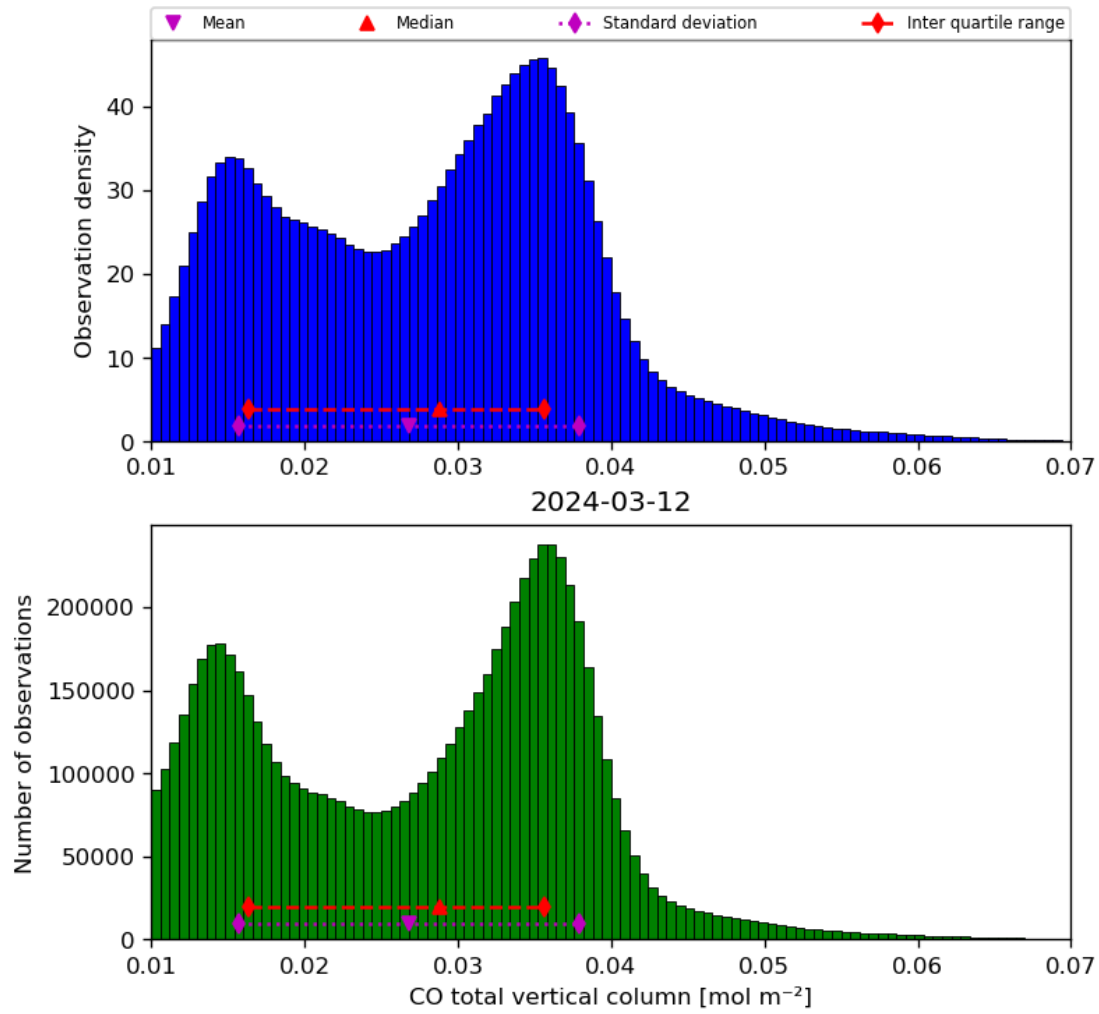
Figure 18: Histogram of “CO total vertical column” for 2024-03-11 to 2024-03-13
