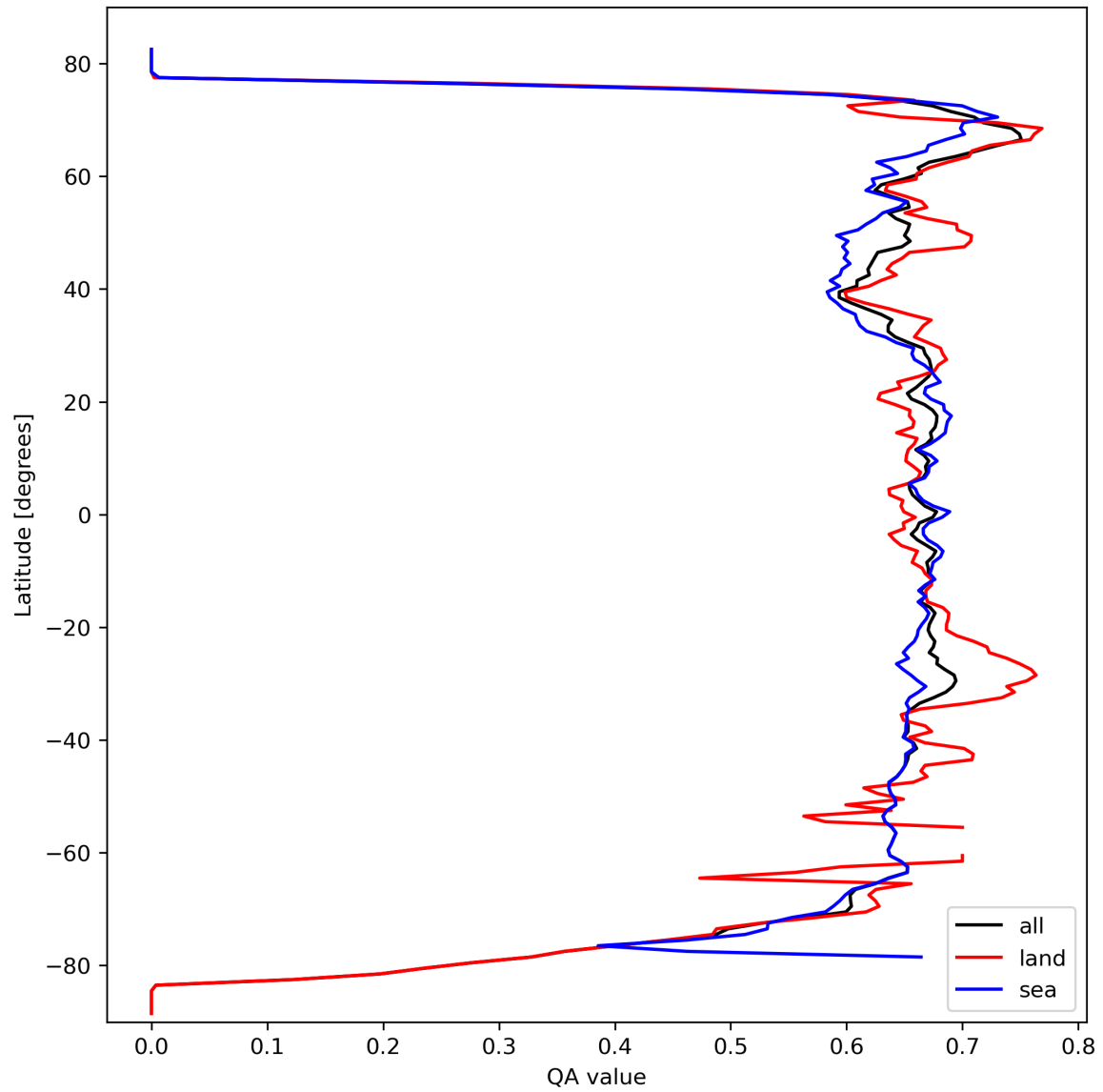
Figure 9: Zonal average of “QA value” for 2024-03-11 to 2024-03-13.
