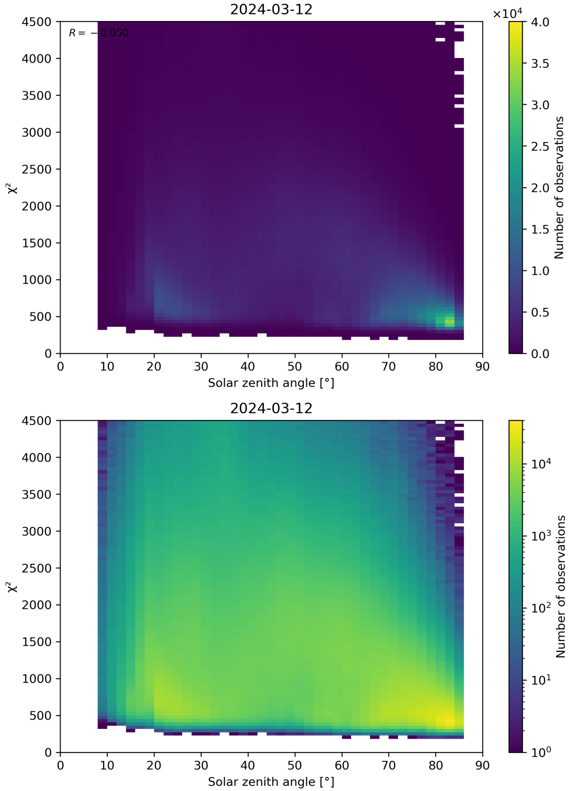
Figure 64: Scatter density plot of “Solar zenith angle” against “ \chi^2 ” for 2024-03-11 to 2024-03-13.
