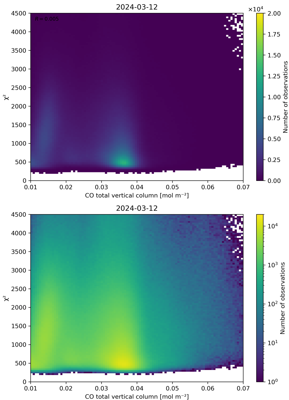
Figure 35: Scatter density plot of “CO total vertical column” against “ \chi^2 ” for 2024-03-11 to 2024-03-13.
