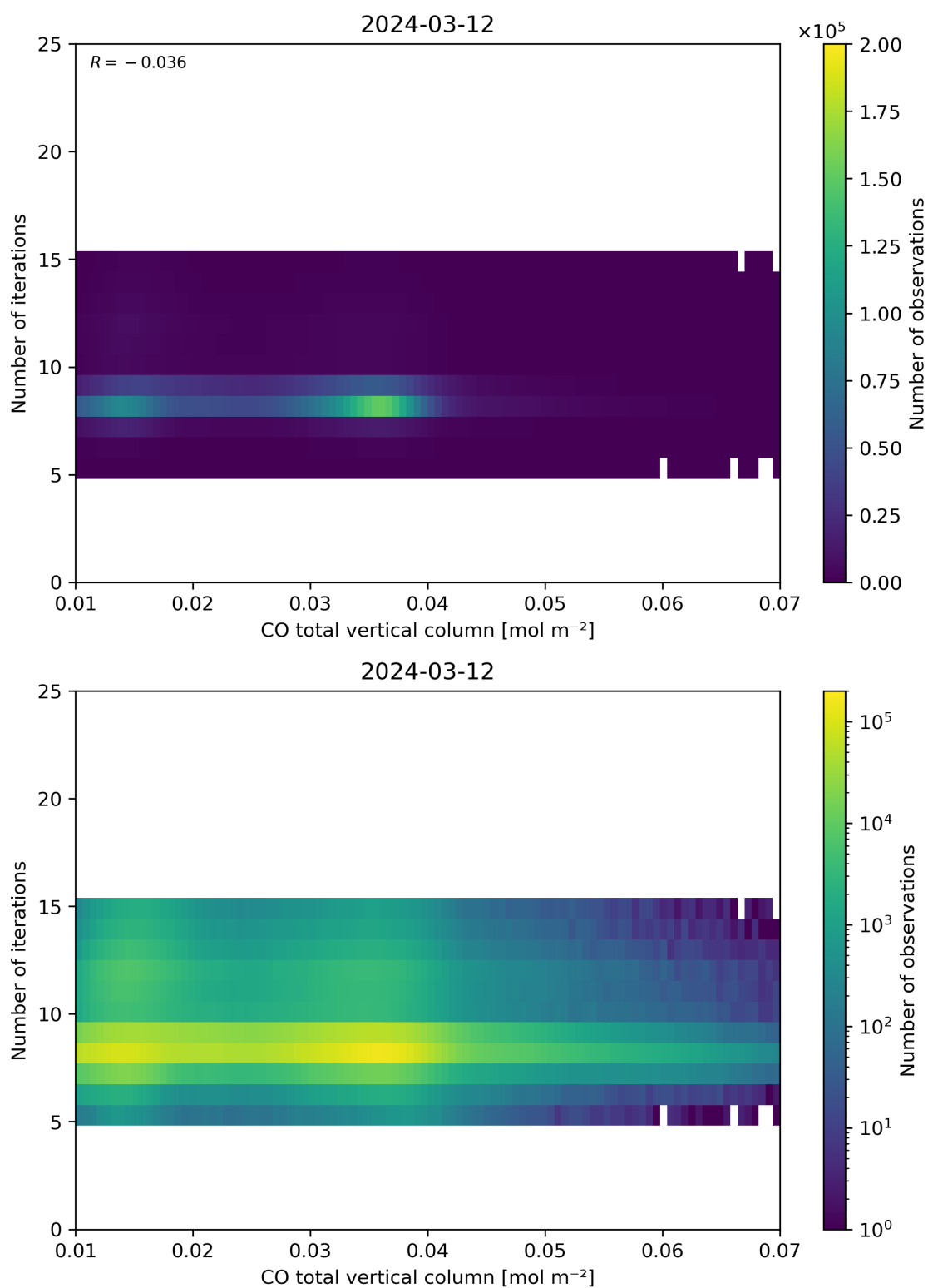
Figure 42: Scatter density plot of “CO total vertical column” against “Number of iterations” for 2024-03-11 to 2024-03-13.
