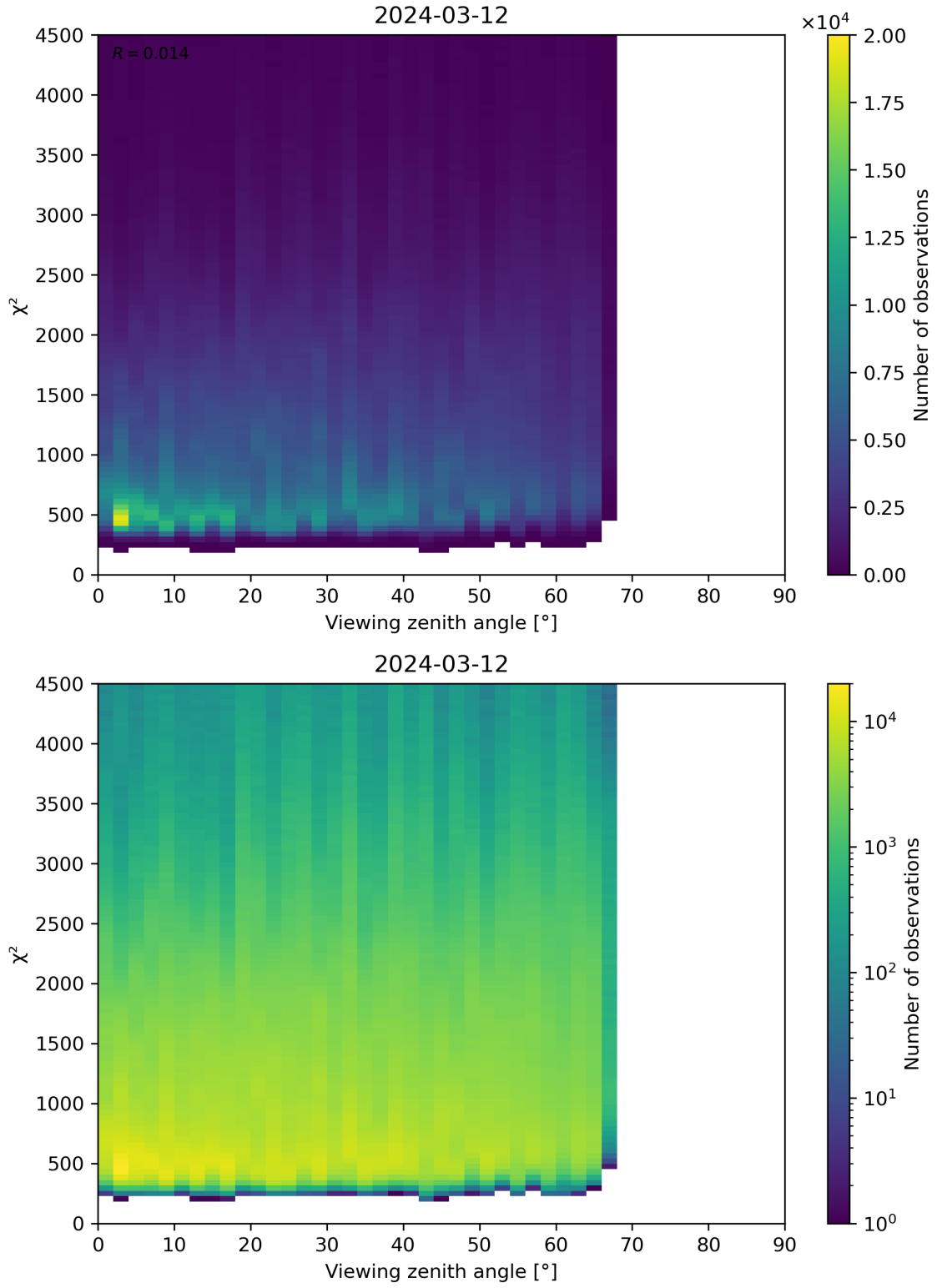
Figure 72: Scatter density plot of “Viewing zenith angle” against “ \chi^2 ” for 2024-03-11 to 2024-03-13.
