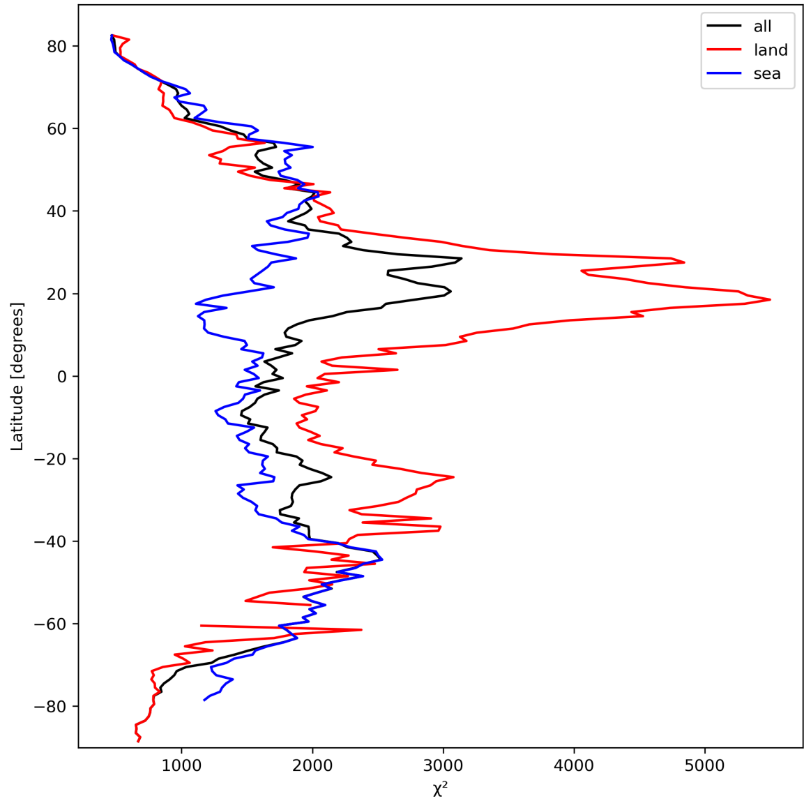
Figure 14: Zonal average of “ \chi^2 ” for 2024-03-11 to 2024-03-13.
