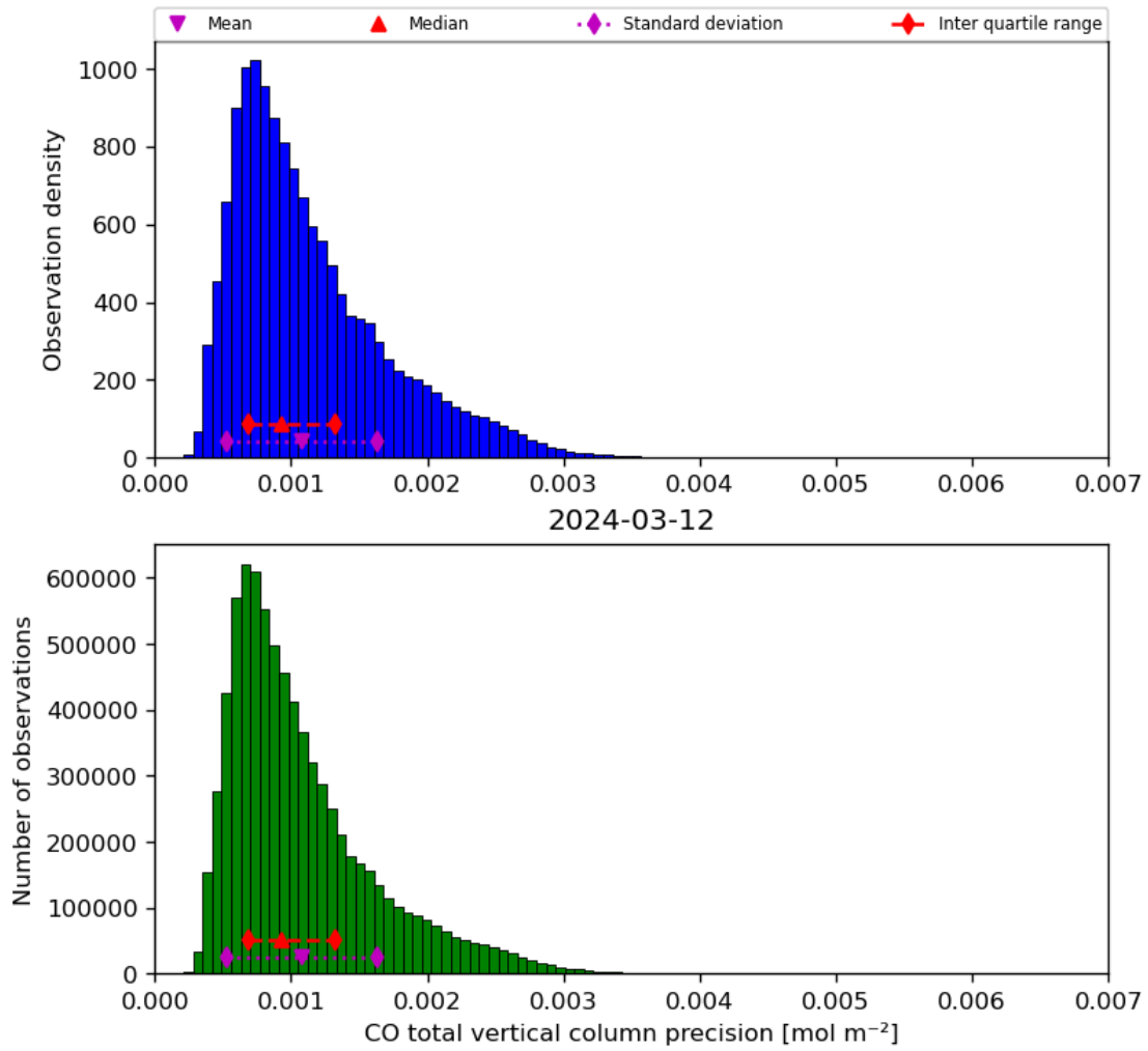
Figure 20: Histogram of “CO total vertical column precision” for 2024-03-11 to 2024-03-13
