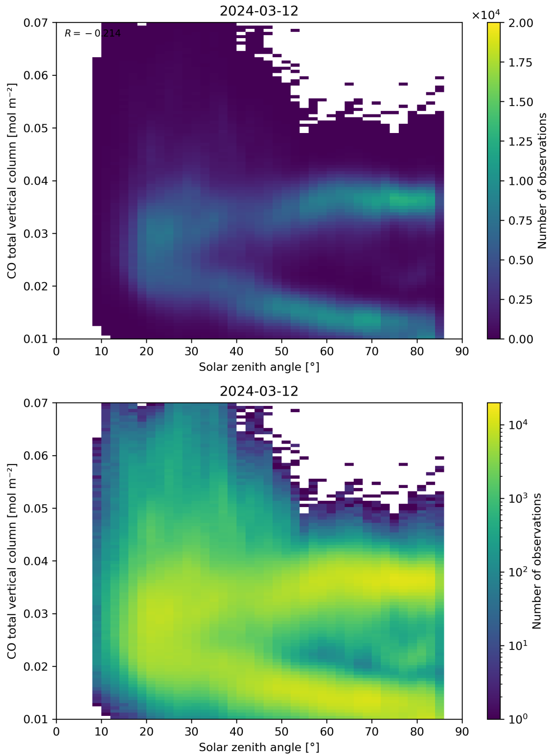
Figure 61: Scatter density plot of “Solar zenith angle” against “CO total vertical column” for 2024-03-11 to 2024-03-13.
