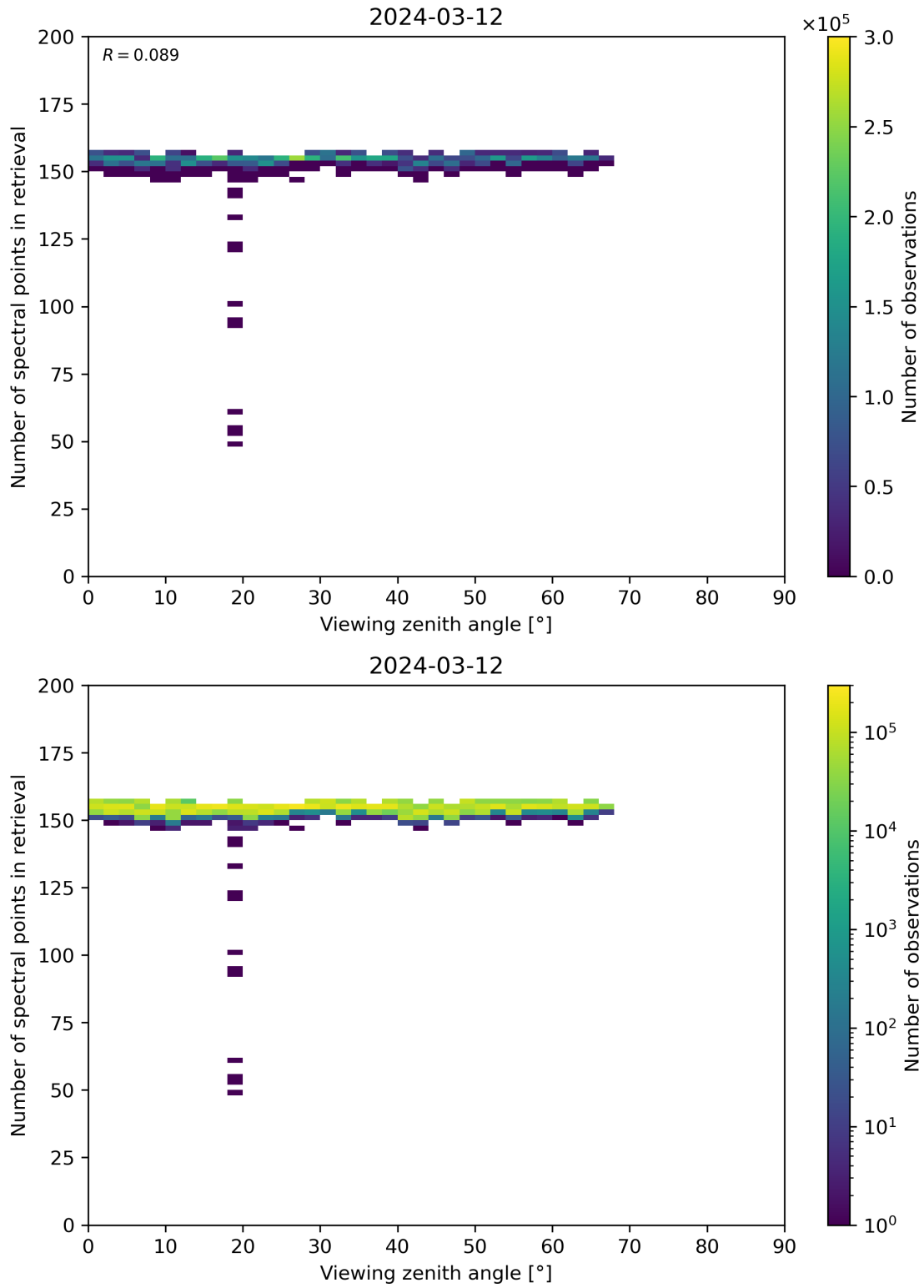
Figure 76: Scatter density plot of “Viewing zenith angle” against “Number of spectral points in retrieval” for 2024-03-11 to 2024-03-13.
