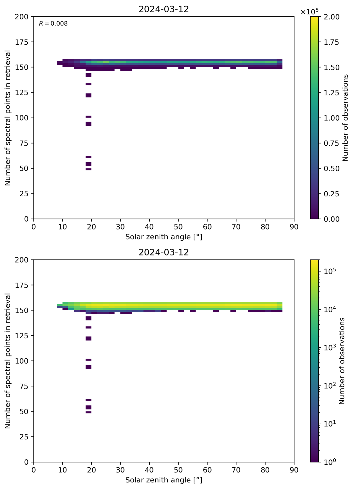
Figure 68: Scatter density plot of “Solar zenith angle” against “Number of spectral points in retrieval” for 2024-03-11 to 2024-03-13.
