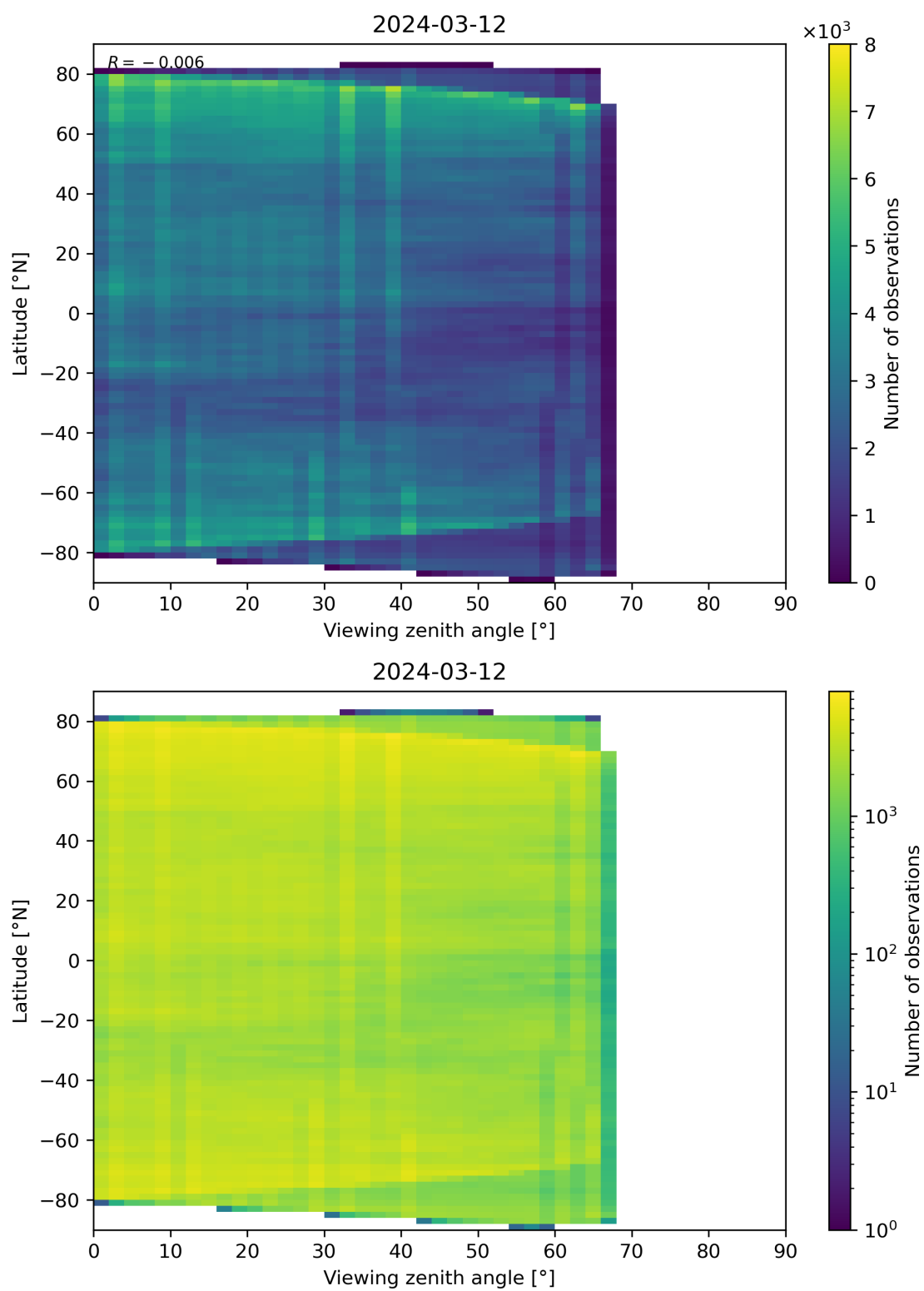
Figure 74: Scatter density plot of “Viewing zenith angle” against “Latitude” for 2024-03-11 to 2024-03-13.
