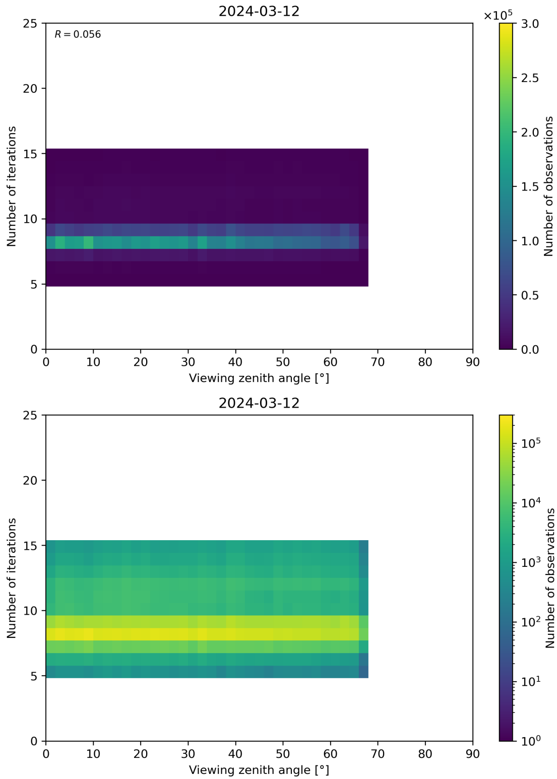
Figure 75: Scatter density plot of “Viewing zenith angle” against “Number of iterations” for 2024-03-11 to 2024-03-13.
