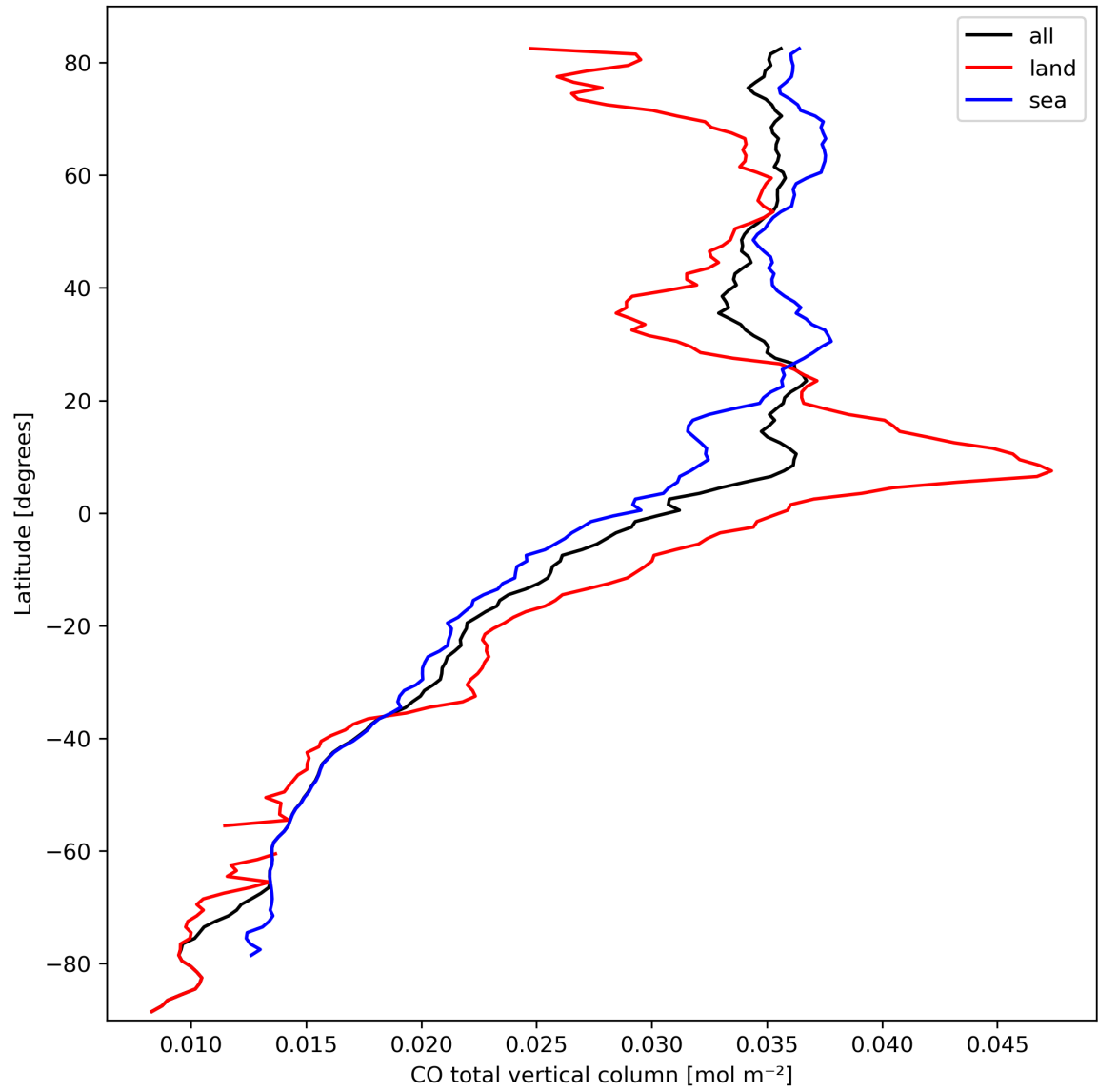
Figure 10: Zonal average of “CO total vertical column” for 2024-03-11 to 2024-03-13.
