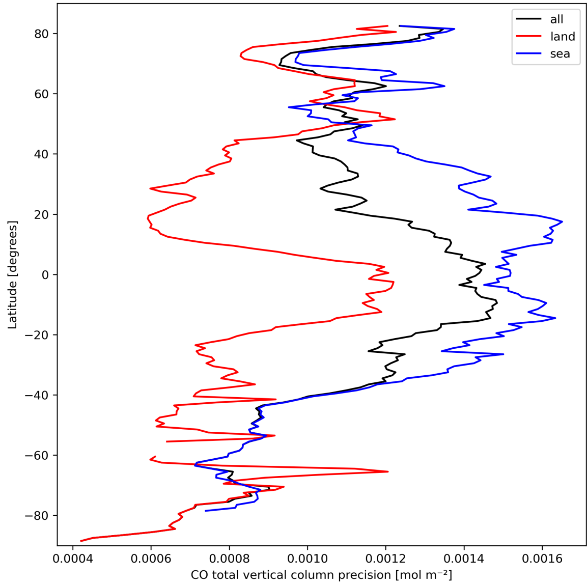
Figure 12: Zonal average of “CO total vertical column precision” for 2024-03-11 to 2024-03-13.
