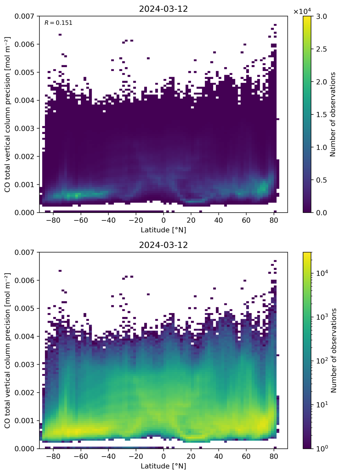
Figure 53: Scatter density plot of “Latitude” against “CO total vertical column precision” for 2024-03-11 to 2024-03-13.
