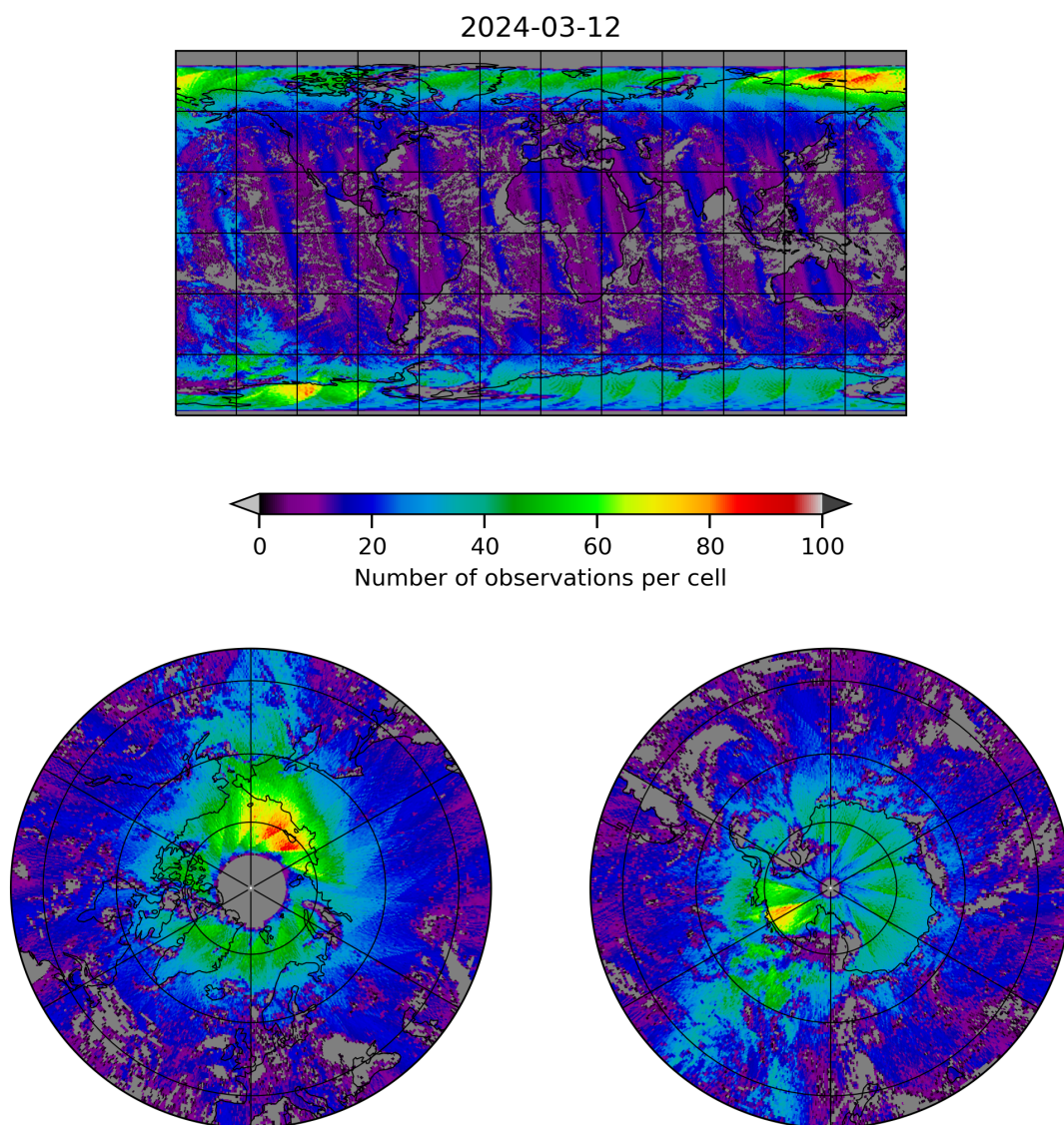
Figure 8: Map of the number of observations for 2024-03-11 to 2024-03-13
