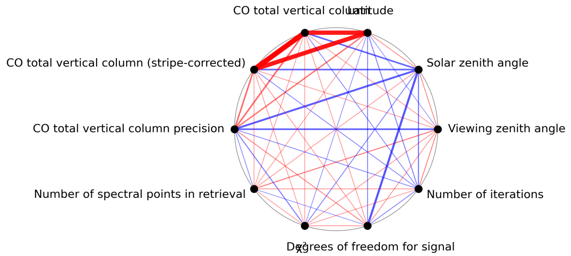
Figure 1: Map of correlation graph for 2024-03-11 to 2024-03-13.
