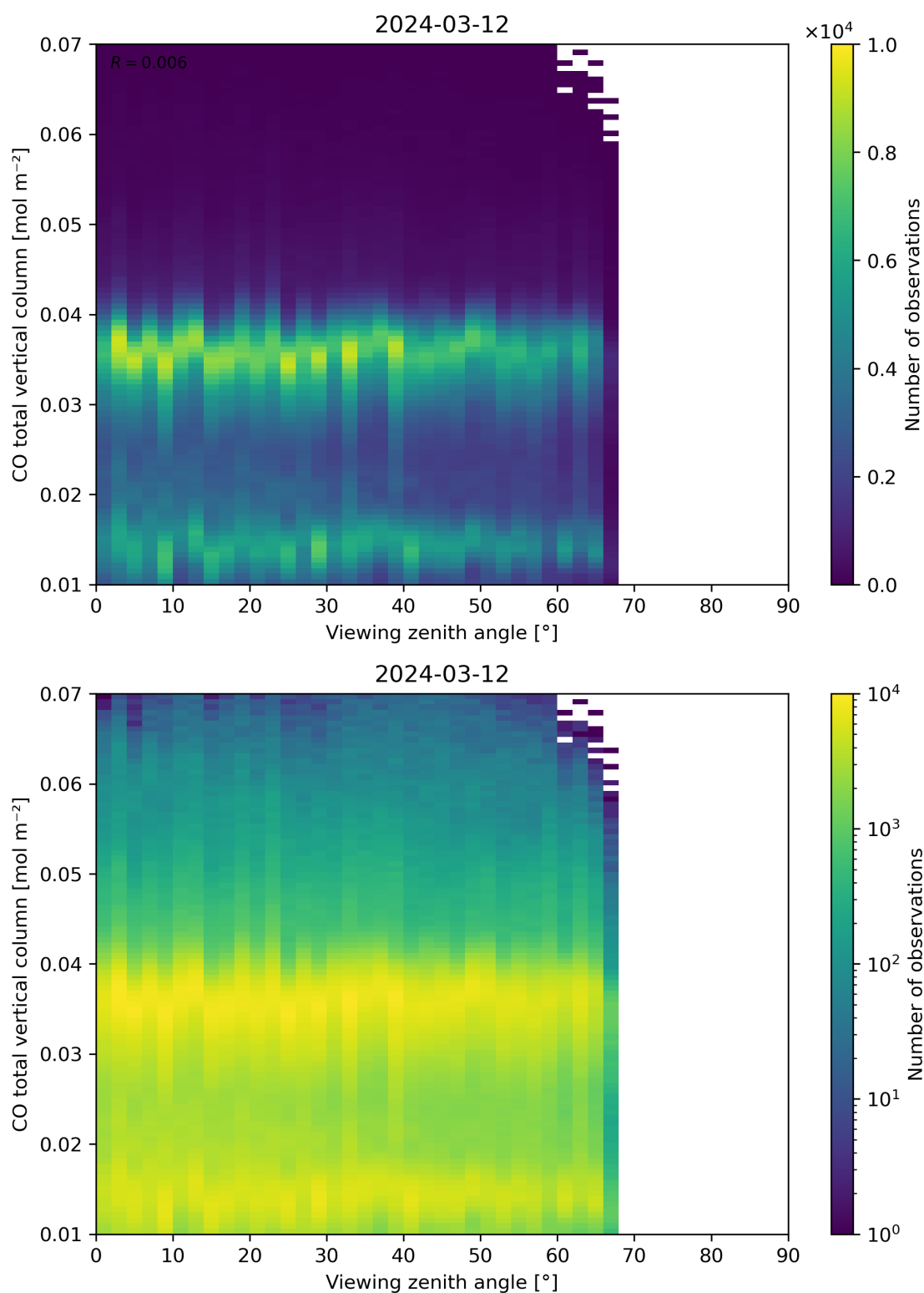
Figure 69: Scatter density plot of “Viewing zenith angle” against “CO total vertical column” for 2024-03-11 to 2024-03-13.
