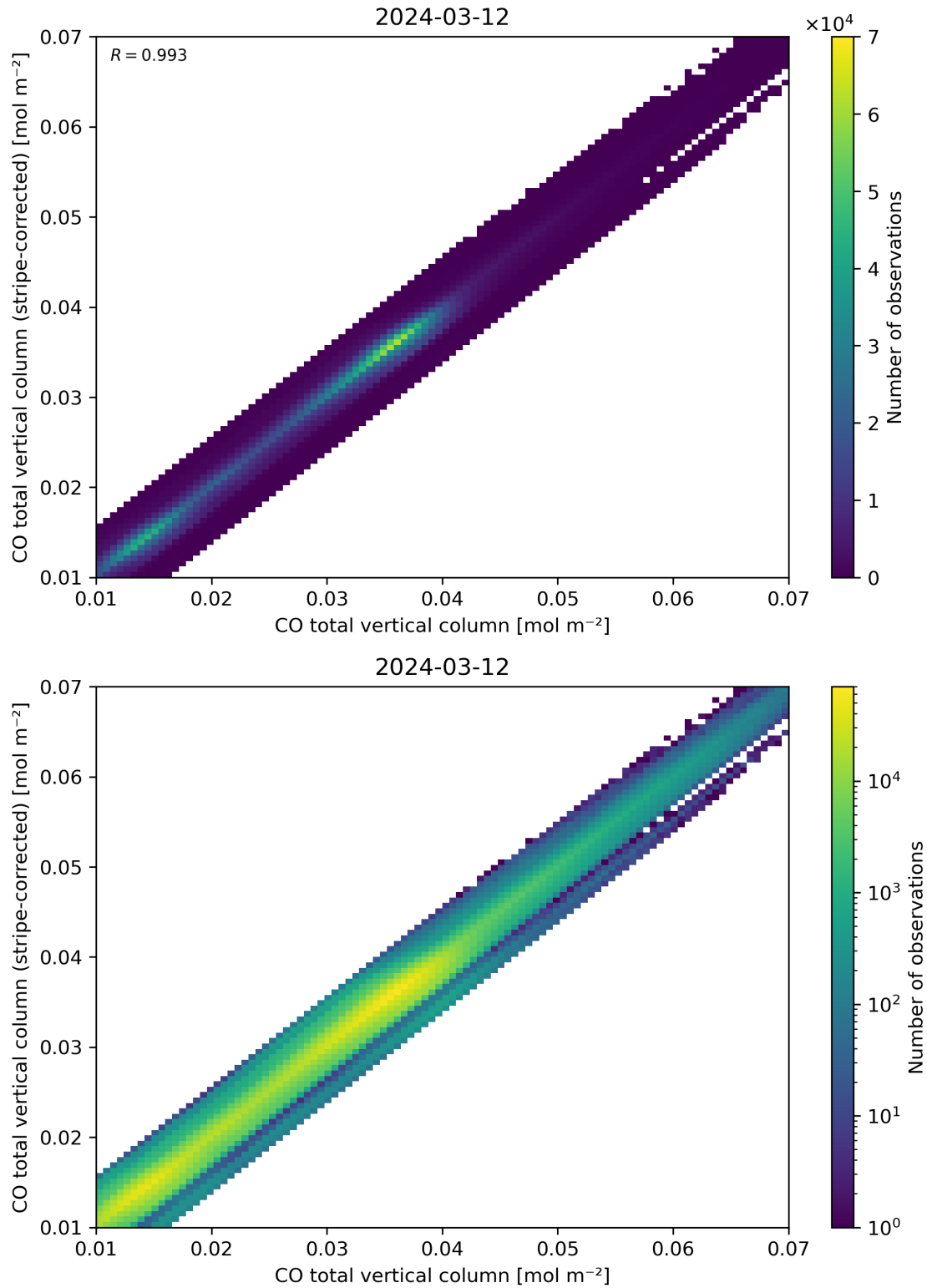
Figure 33: Scatter density plot of “CO total vertical column” against “CO total vertical column (stripe-corrected)” for 2024-03-11 to 2024-03-13.
