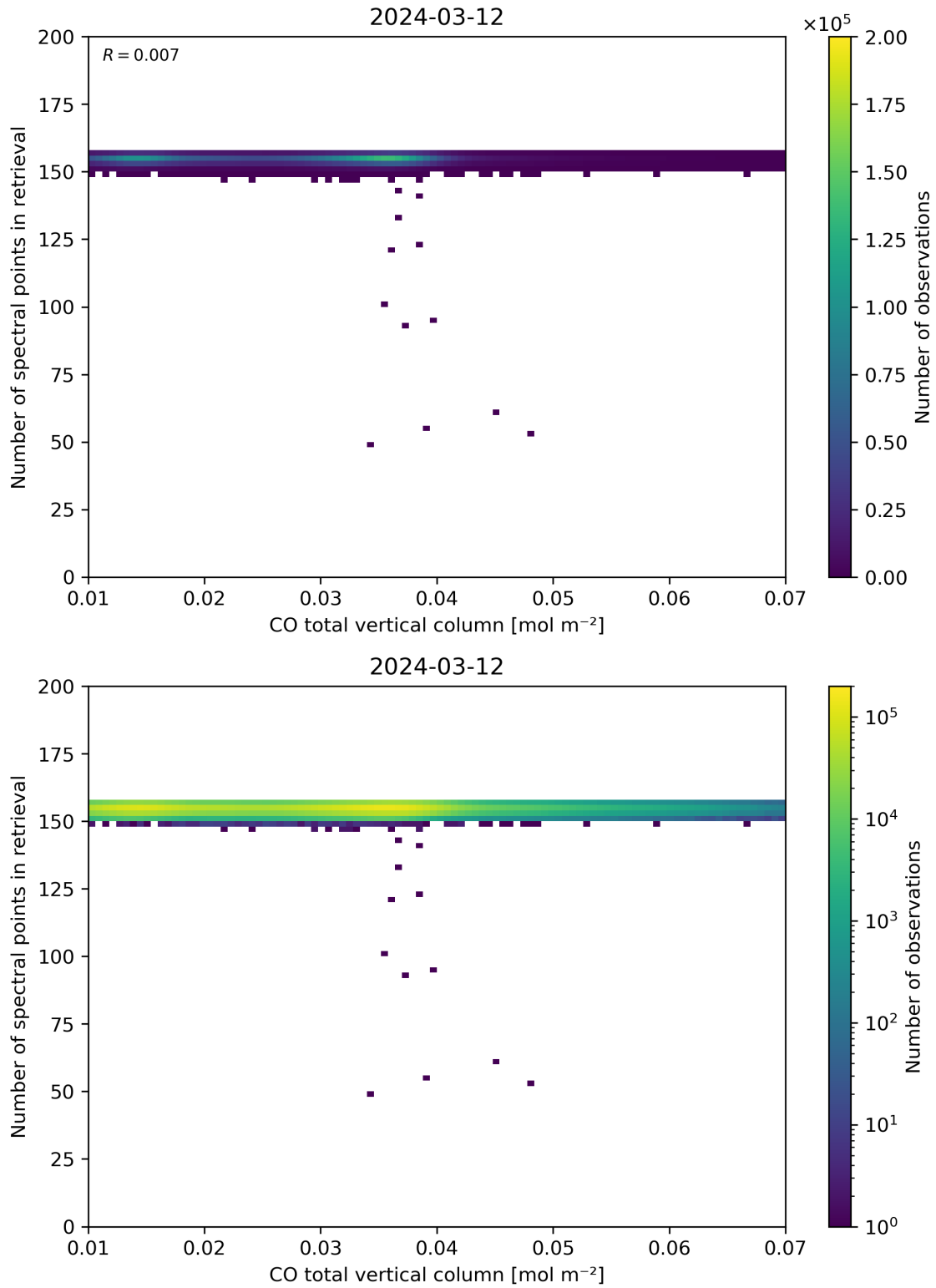
Figure 43: Scatter density plot of “CO total vertical column” against “Number of spectral points in retrieval” for 2024-03-11 to 2024-03-13.
