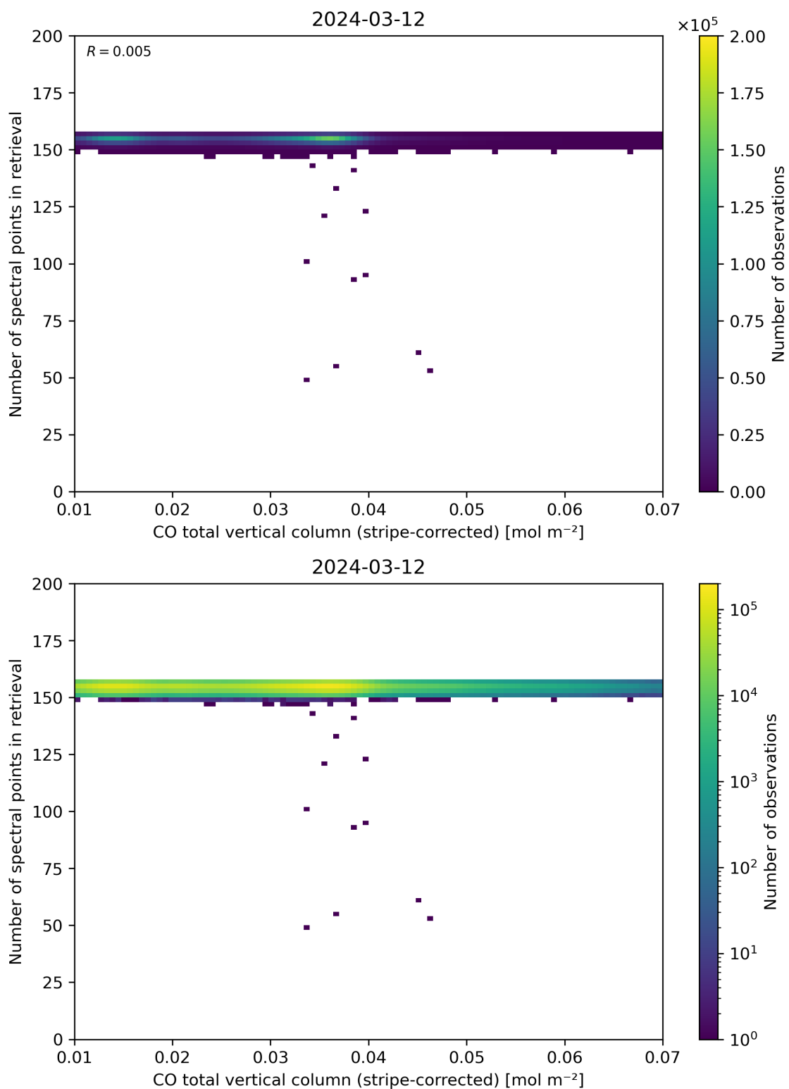
Figure 40: Scatter density plot of “CO total vertical column (stripe-corrected)” against “Number of spectral points in retrieval” for 2024-03-11 to 2024-03-13.
