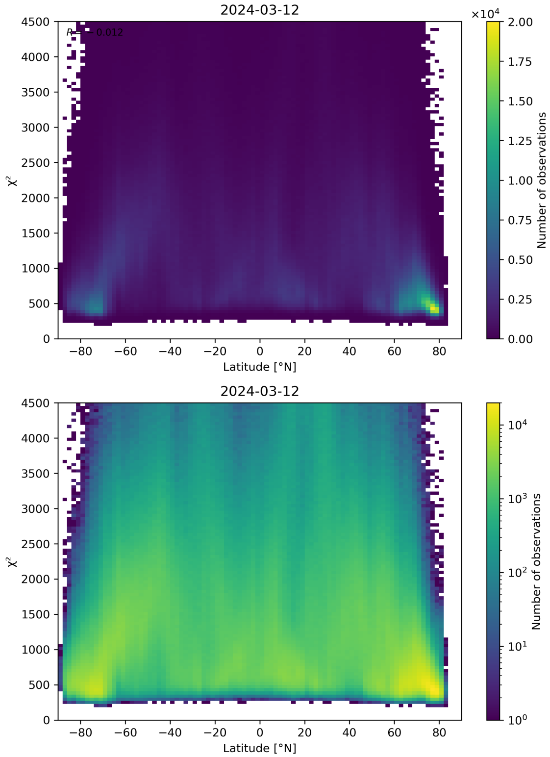
Figure 54: Scatter density plot of “Latitude” against “ \chi^2 ” for 2024-03-11 to 2024-03-13.
