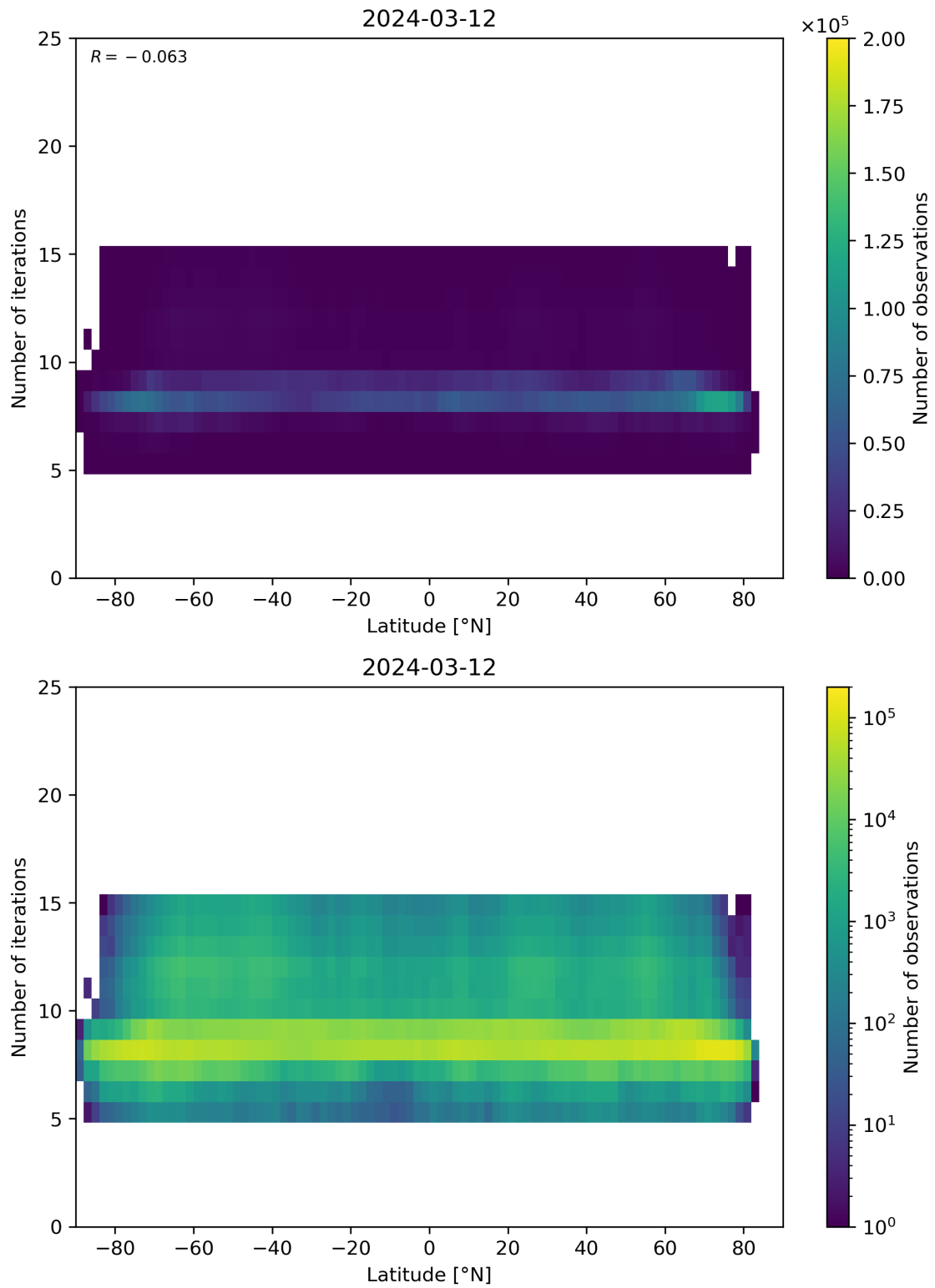
Figure 56: Scatter density plot of “Latitude” against “Number of iterations” for 2024-03-11 to 2024-03-13.
