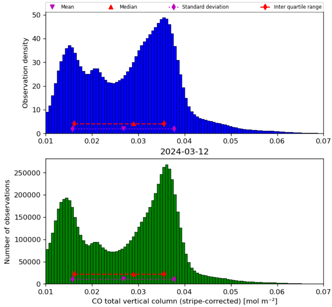
Figure 19: Histogram of “CO total vertical column (stripe-corrected)” for 2024-03-11 to 2024-03-13
