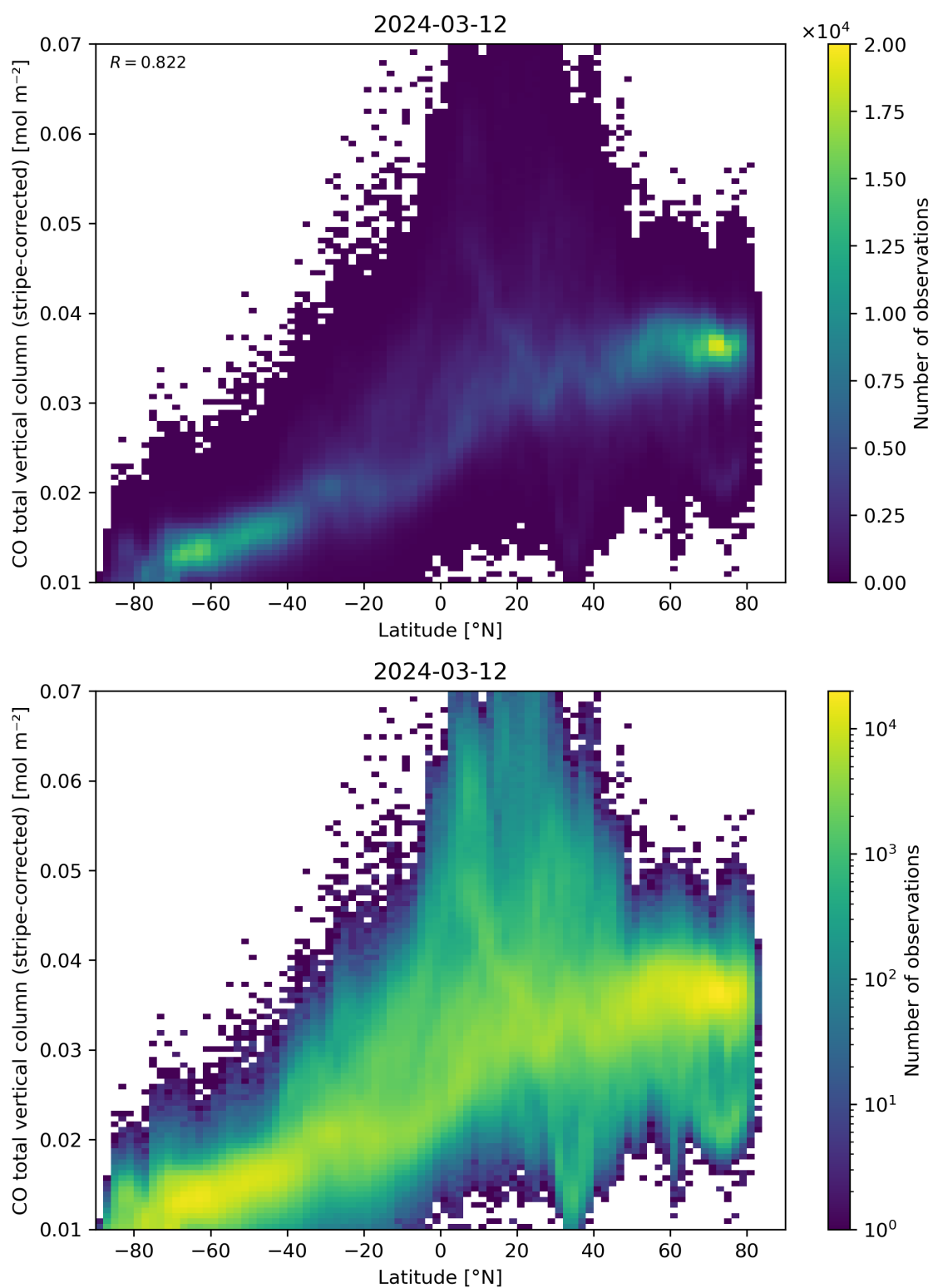
Figure 52: Scatter density plot of “Latitude” against “CO total vertical column (stripe-corrected)” for 2024-03-11 to 2024-03-13.
