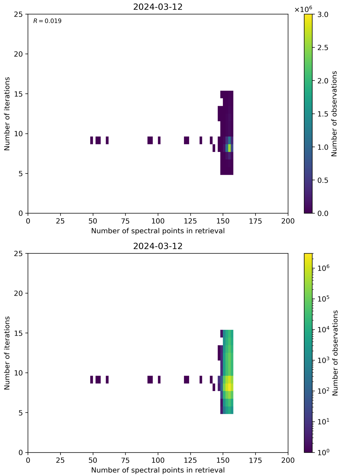
Figure 60: Scatter density plot of “Number of spectral points in retrieval” against “Number of iterations” for 2024-03-11 to 2024-03-13.
