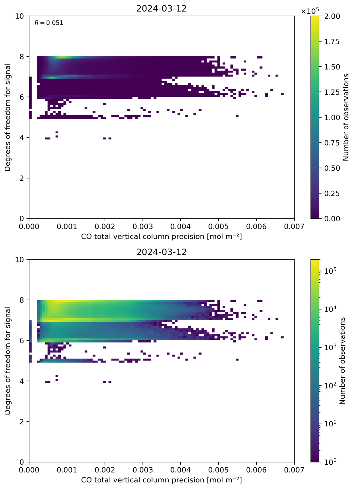
Figure 45: Scatter density plot of “CO total vertical column precision” against “Degrees of freedom for signal” for 2024-03-11 to 2024-03-13.
