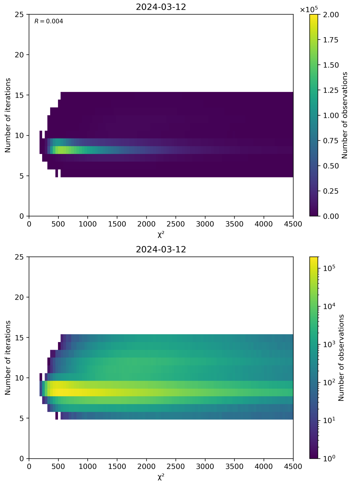
Figure 49: Scatter density plot of “ \chi^2 ” against “Number of iterations” for 2024-03-11 to 2024-03-13.
