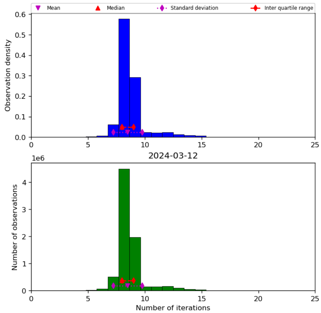
Figure 24: Histogram of “Number of iterations” for 2024-03-11 to 2024-03-13
