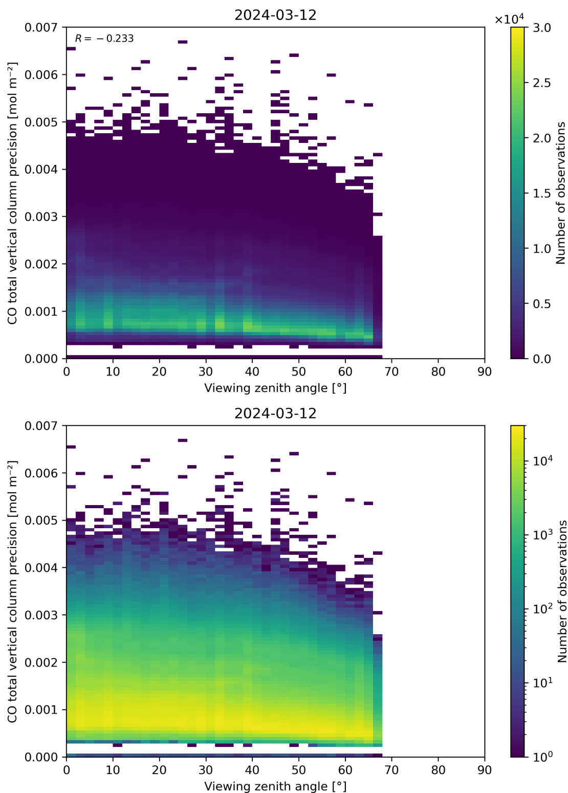
Figure 71: Scatter density plot of “Viewing zenith angle” against “CO total vertical column precision” for 2024-03-11 to 2024-03-13.
