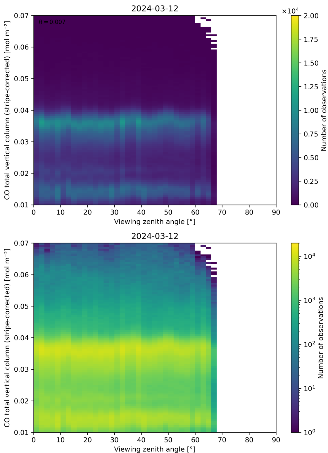
Figure 70: Scatter density plot of “Viewing zenith angle” against “CO total vertical column (stripe-corrected)” for 2024-03-11 to 2024-03-13.
