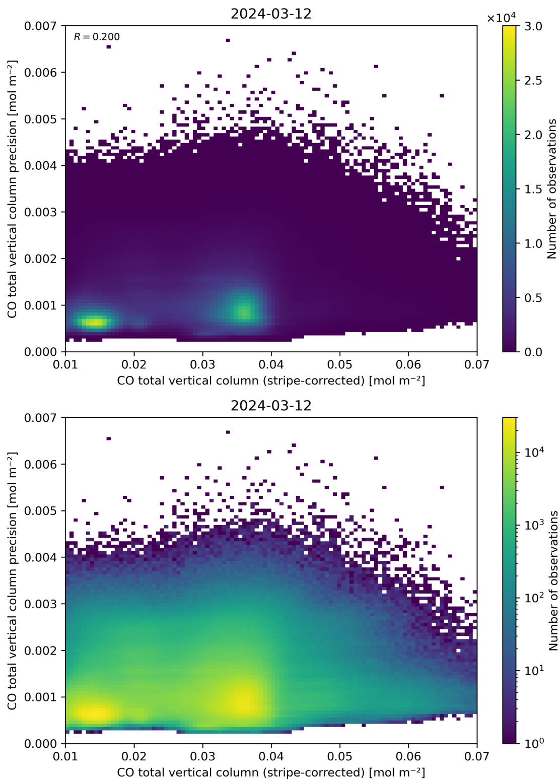
Figure 36: Scatter density plot of “CO total vertical column (stripe-corrected)” against “CO total vertical column precision” for 2024-03-11 to 2024-03-13.
