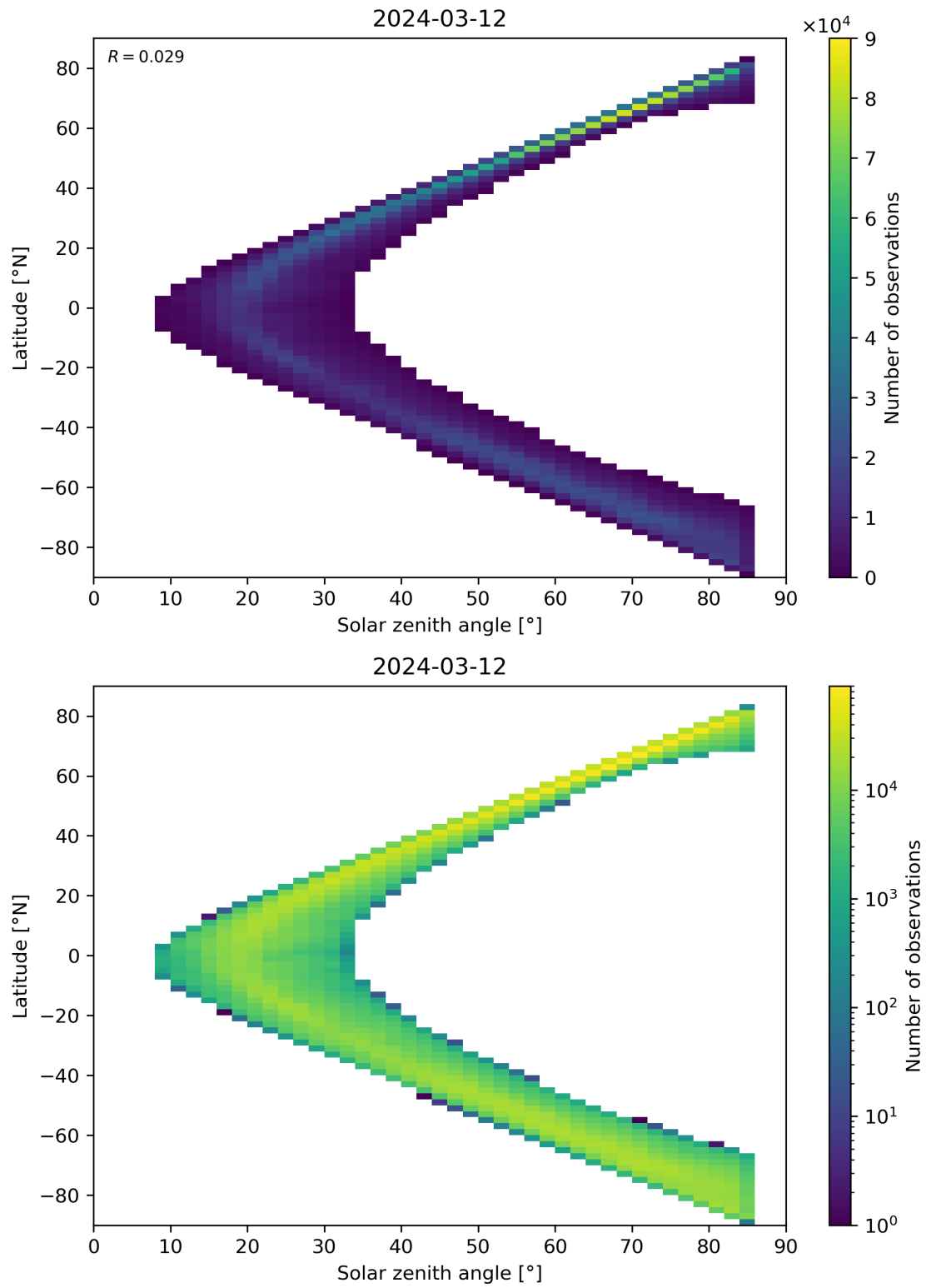
Figure 66: Scatter density plot of “Solar zenith angle” against “Latitude” for 2024-03-11 to 2024-03-13.
