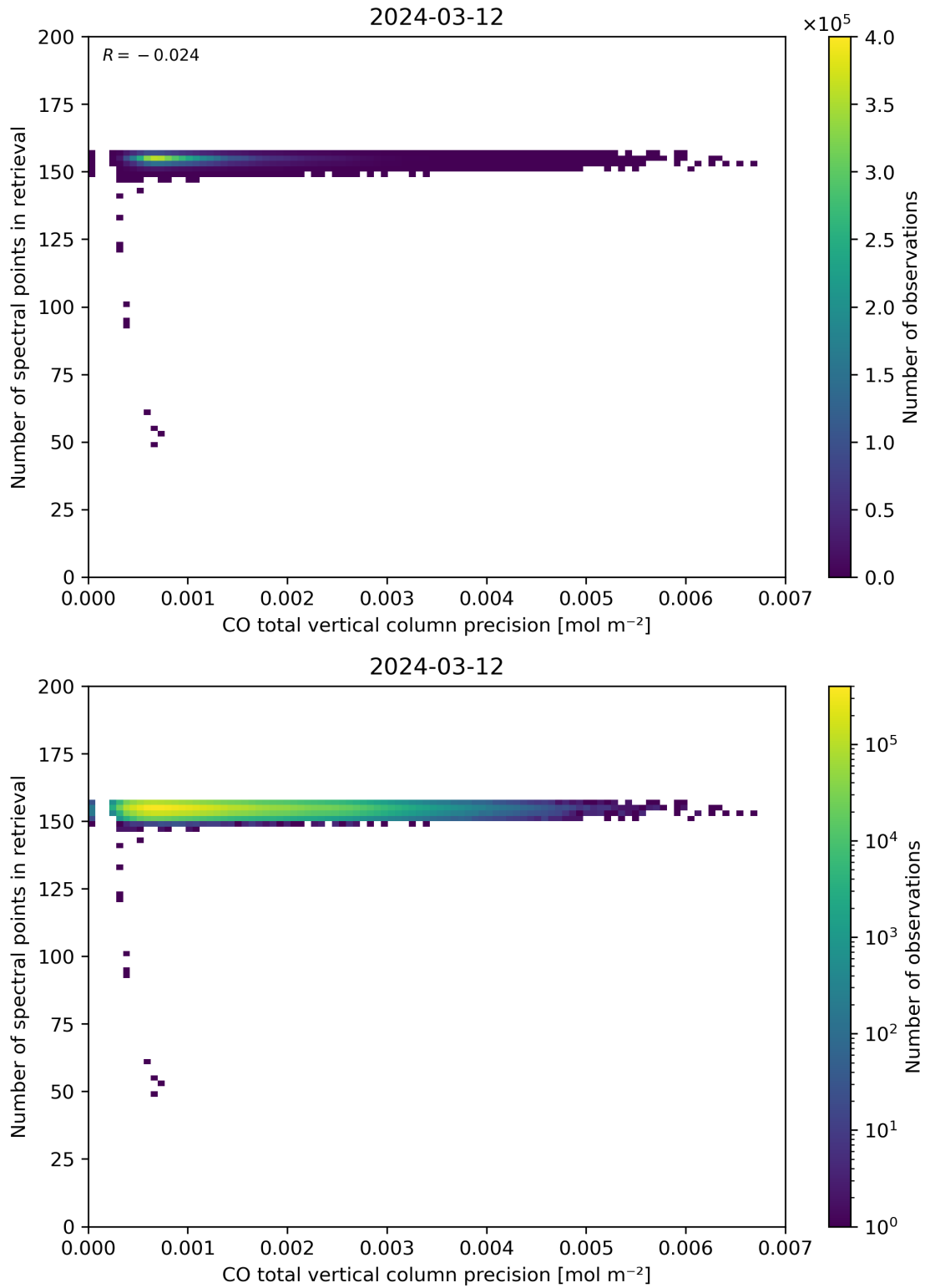
Figure 47: Scatter density plot of “CO total vertical column precision” against “Number of spectral points in retrieval” for 2024-03-11 to 2024-03-13.
