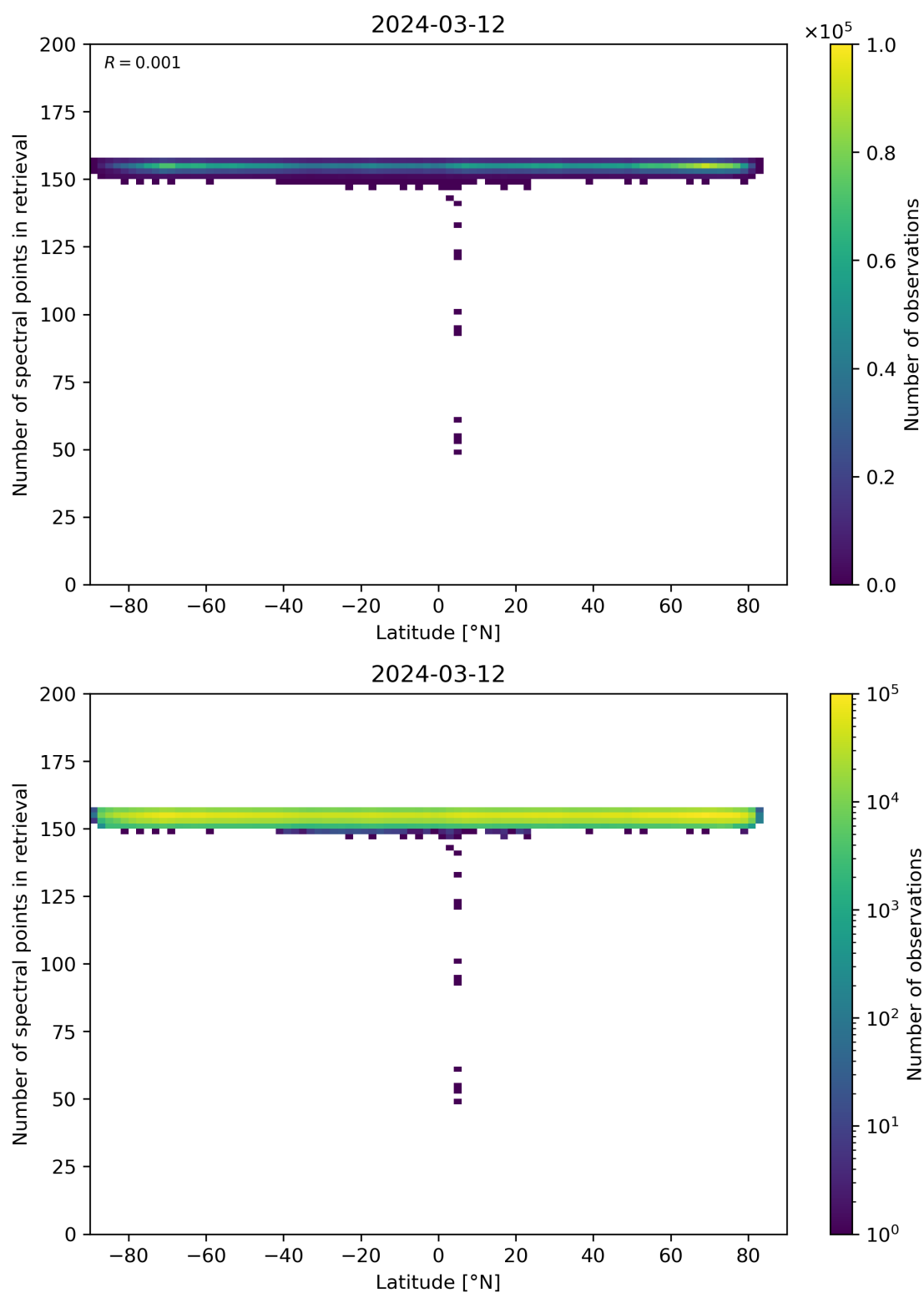
Figure 57: Scatter density plot of “Latitude” against “Number of spectral points in retrieval” for 2024-03-11 to 2024-03-13.
