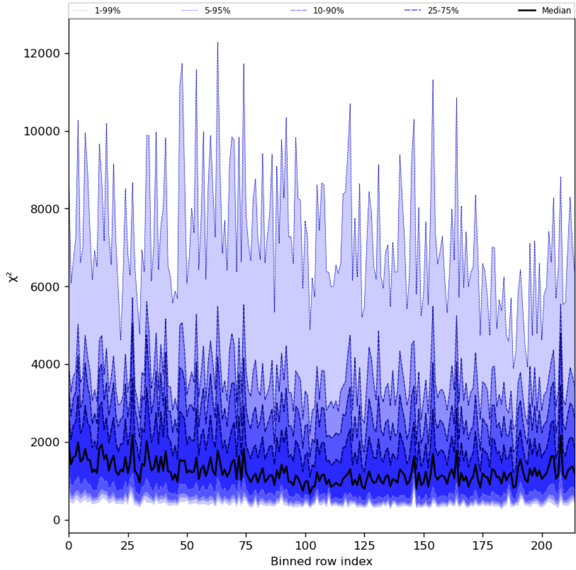
Figure 30: Along track statistics of “ \chi^2 ” for 2024-03-11 to 2024-03-13
