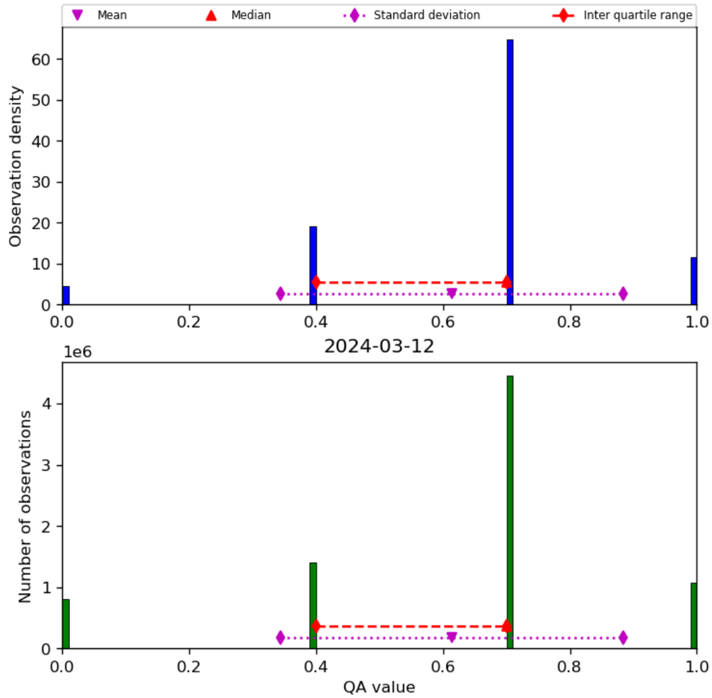
Figure 17: Histogram of “QA value” for 2024-03-11 to 2024-03-13
