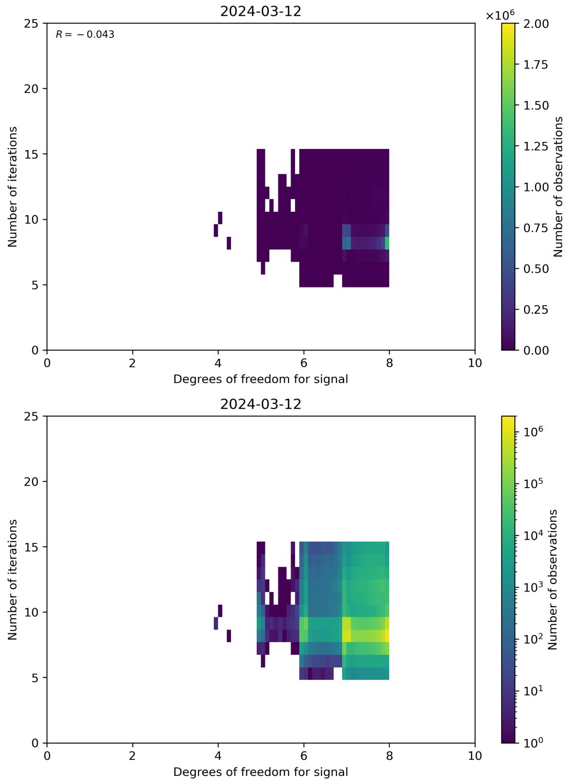
Figure 50: Scatter density plot of “Degrees of freedom for signal” against “Number of iterations” for 2024-03-11 to 2024-03-13.
