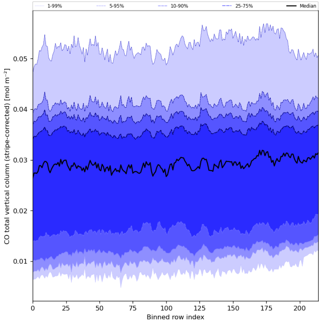
Figure 27: Along track statistics of “CO total vertical column (stripe-corrected)” for 2024-03-11 to 2024-03-13
