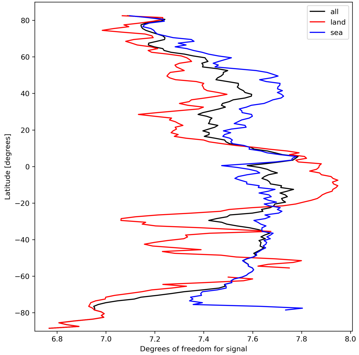
Figure 15: Zonal average of “Degrees of freedom for signal” for 2024-03-11 to 2024-03-13.
