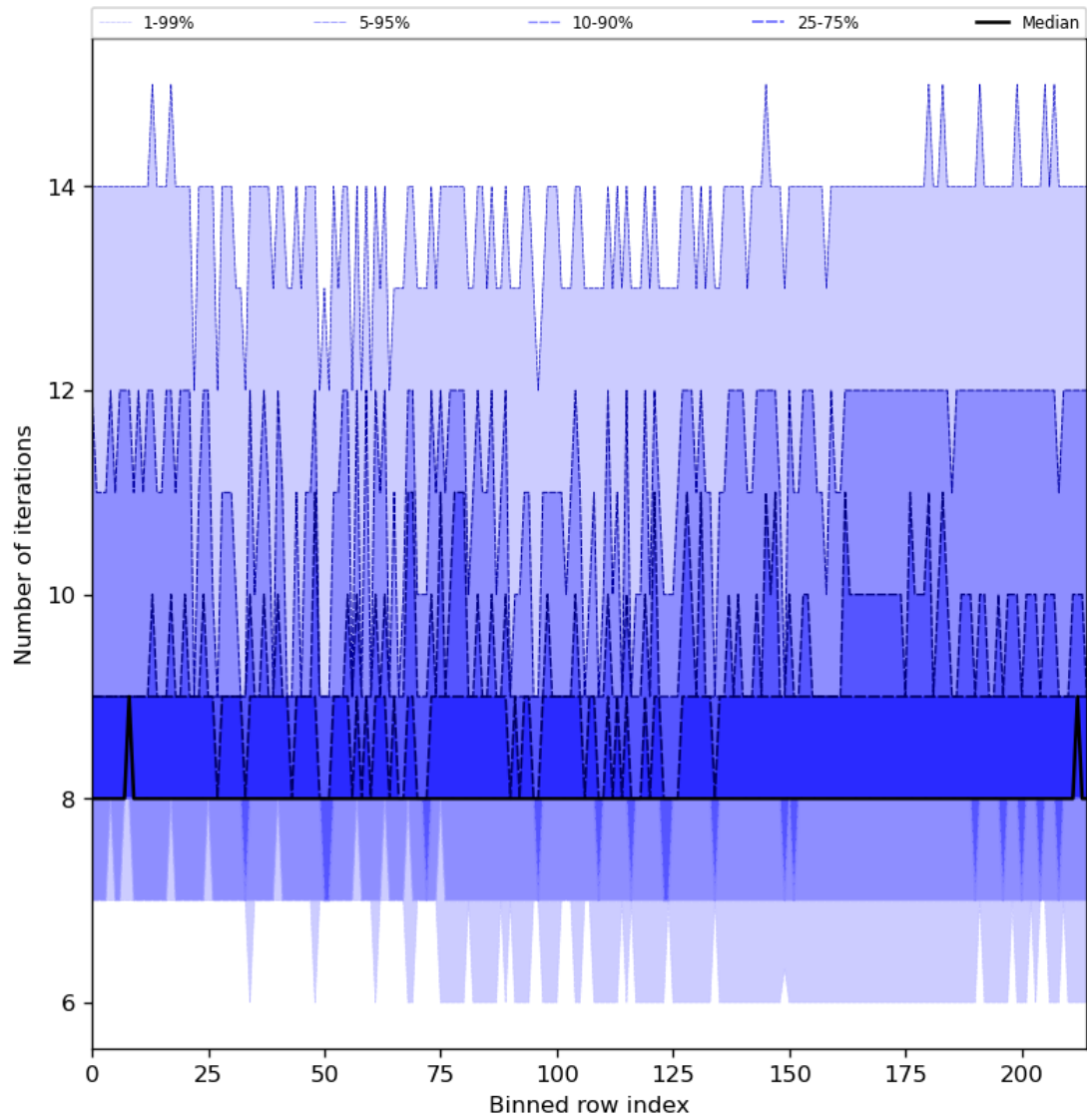
Figure 32: Along track statistics of “Number of iterations” for 2024-03-11 to 2024-03-13
