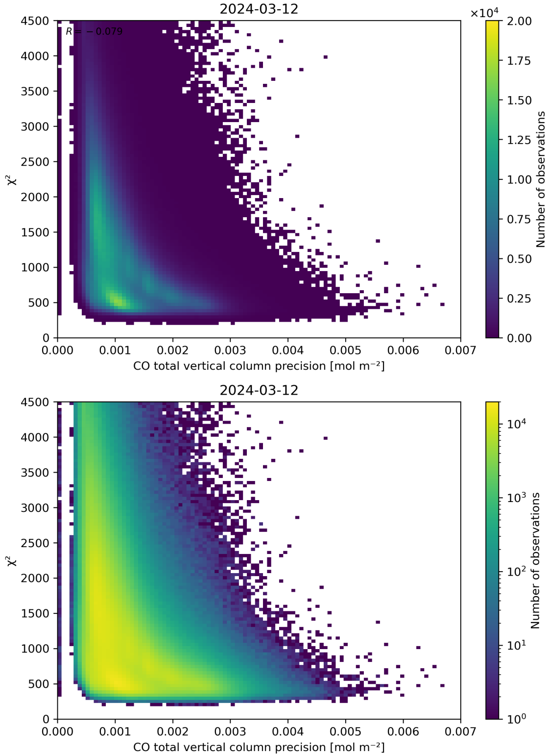
Figure 44: Scatter density plot of “CO total vertical column precision” against “ \chi^2 ” for 2024-03-11 to 2024-03-13.
