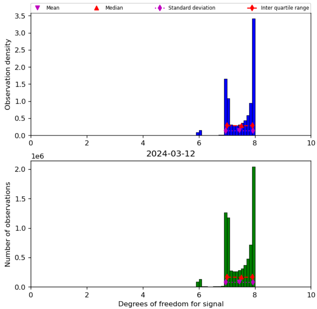
Figure 23: Histogram of “Degrees of freedom for signal” for 2024-03-11 to 2024-03-13
