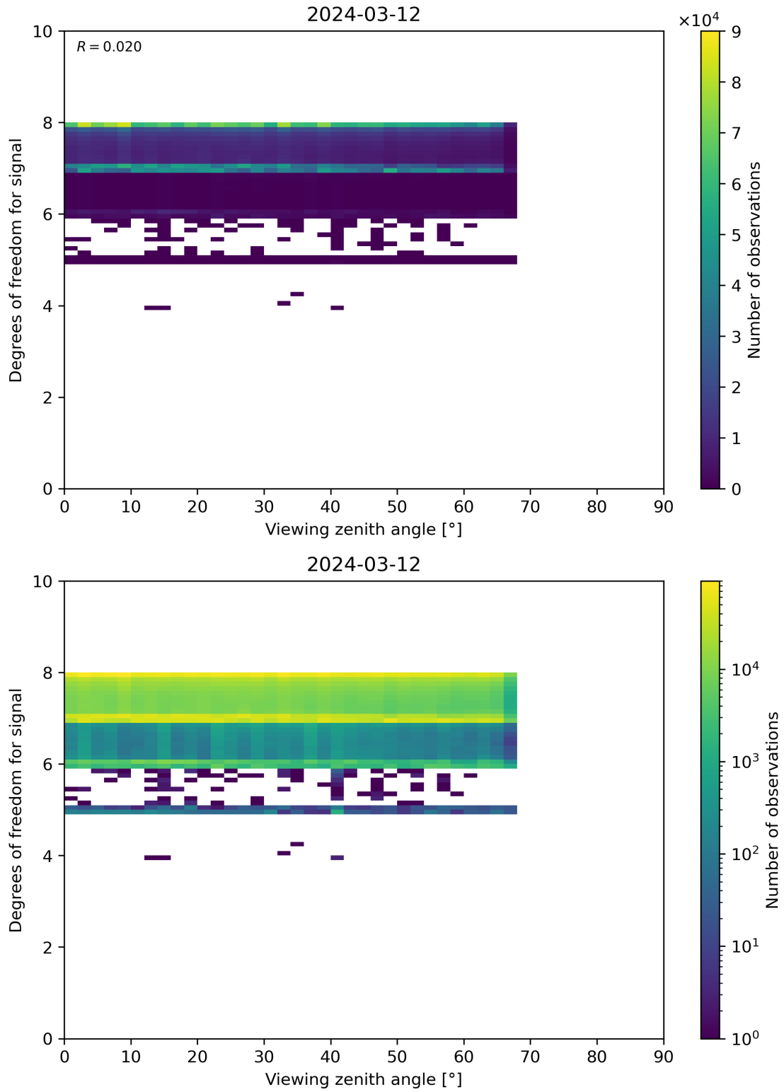
Figure 73: Scatter density plot of “Viewing zenith angle” against “Degrees of freedom for signal” for 2024-03-11 to 2024-03-13.
