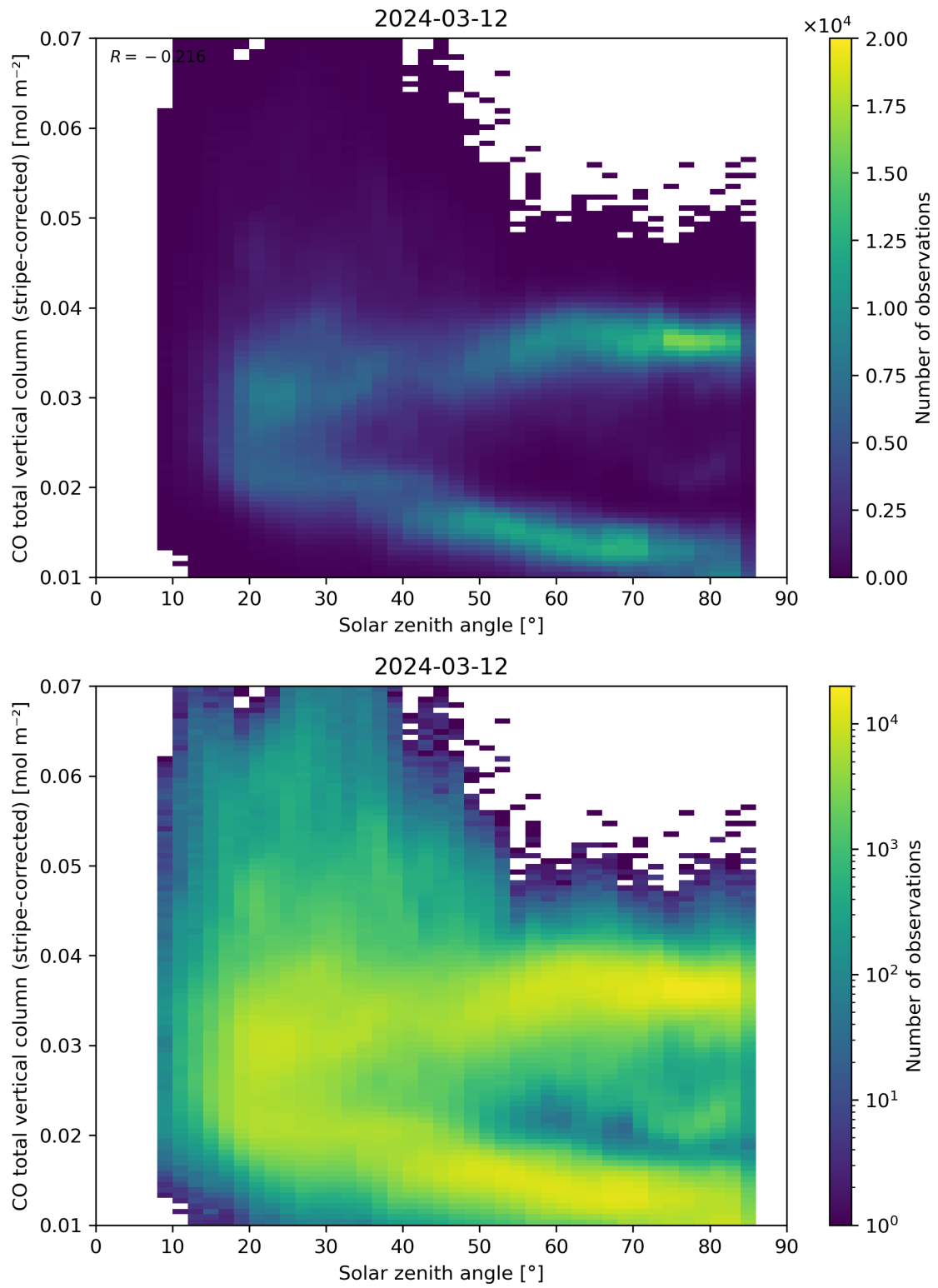
Figure 62: Scatter density plot of “Solar zenith angle” against “CO total vertical column (stripe-corrected)” for 2024-03-11 to 2024-03-13.
