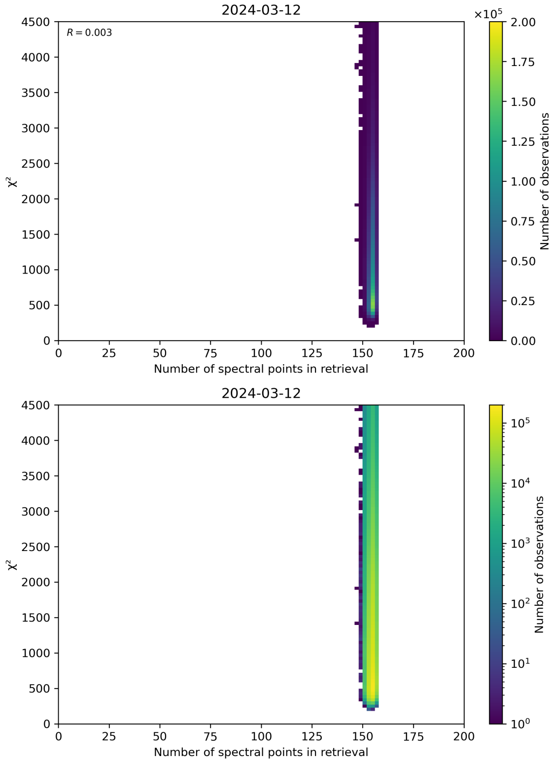
Figure 58: Scatter density plot of “Number of spectral points in retrieval” against “ \chi^2 ” for 2024-03-11 to 2024-03-13.
