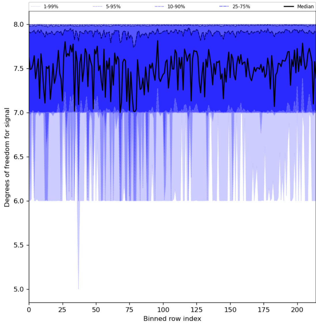
Figure 31: Along track statistics of “Degrees of freedom for signal” for 2024-03-11 to 2024-03-13
