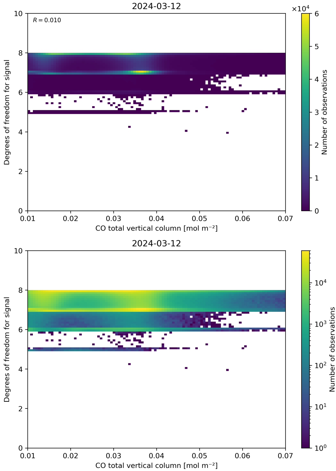
Figure 41: Scatter density plot of “CO total vertical column” against “Degrees of freedom for signal” for 2024-03-11 to 2024-03-13.
