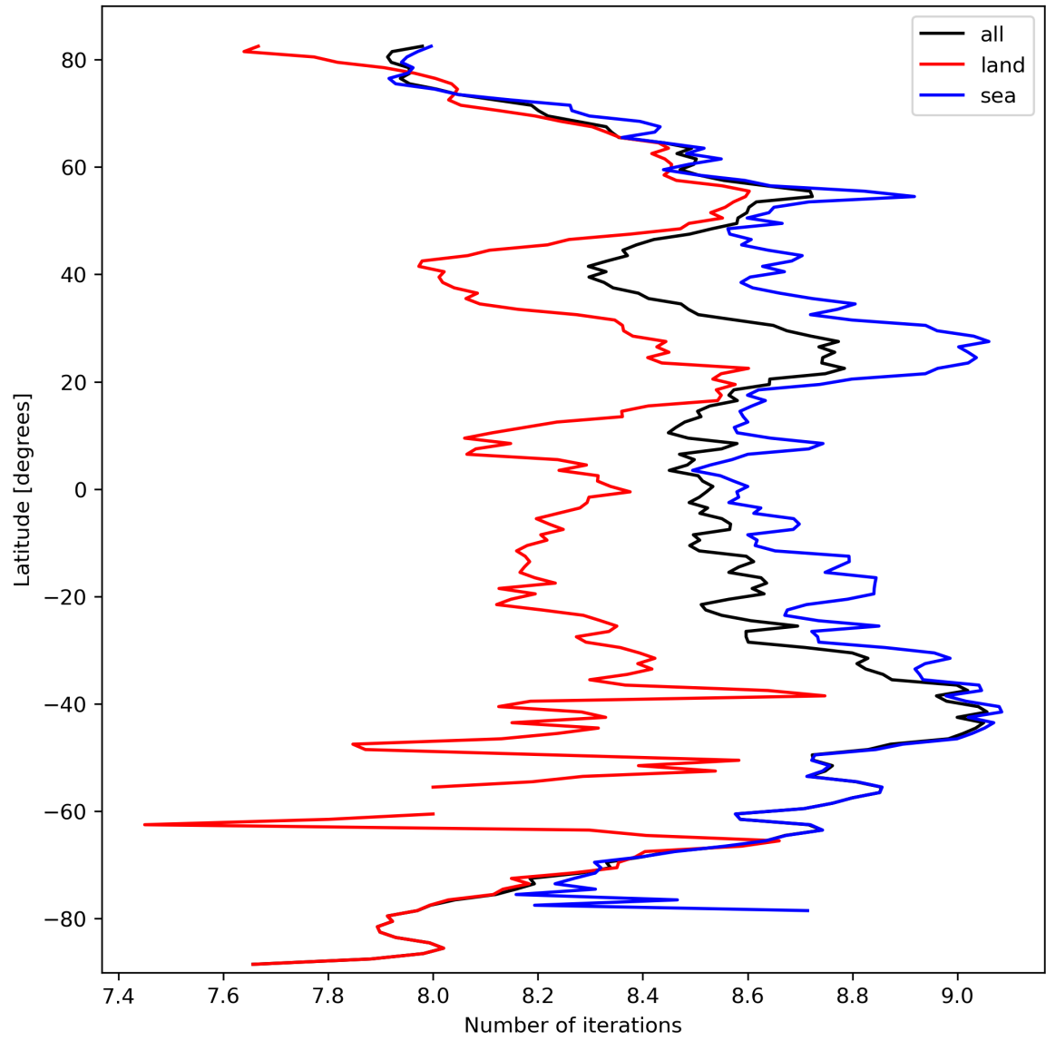
Figure 16: Zonal average of “Number of iterations” for 2024-03-11 to 2024-03-13.
