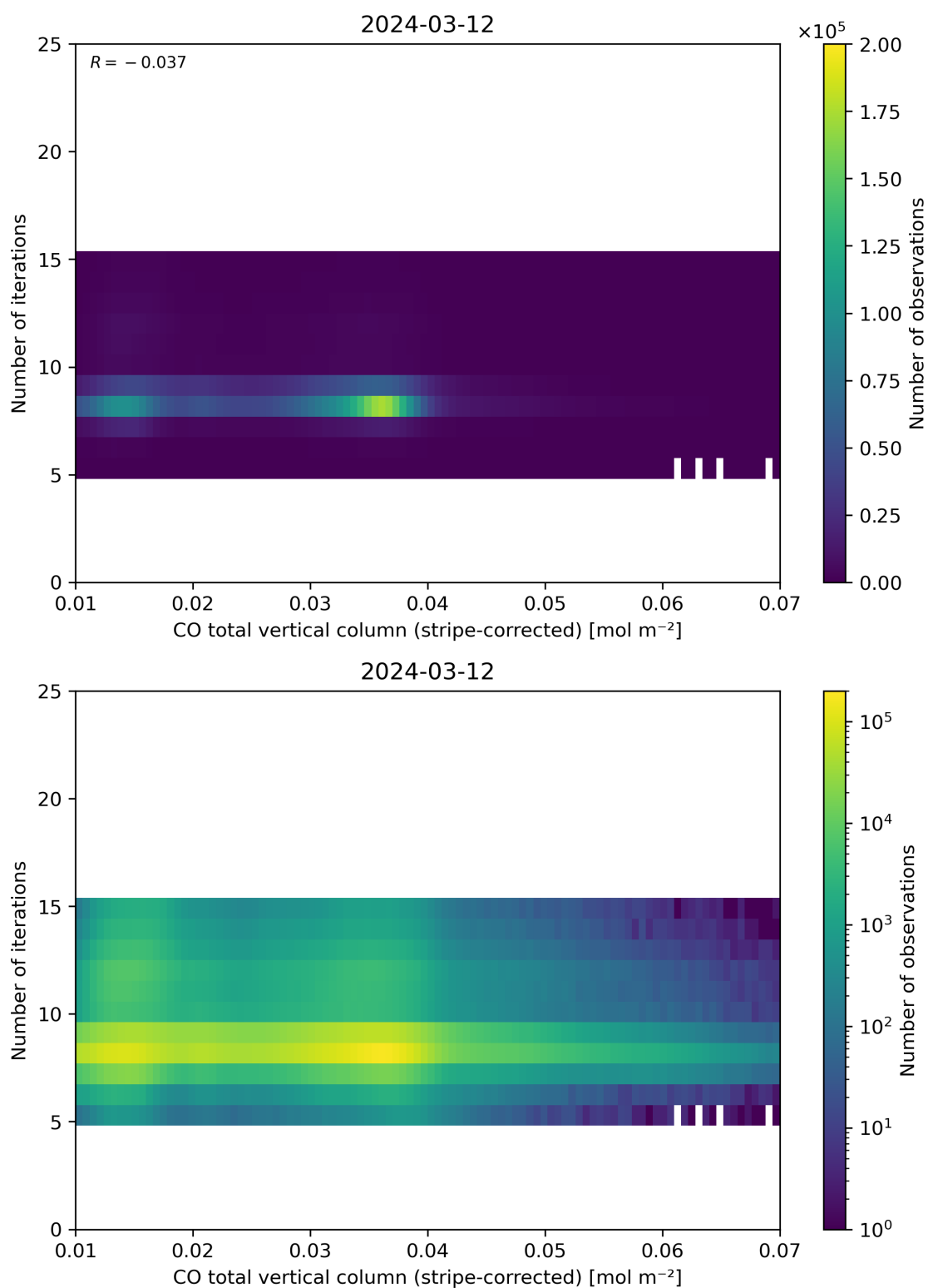
Figure 39: Scatter density plot of “CO total vertical column (stripe-corrected)” against “Number of iterations” for 2024-03-11 to 2024-03-13.
