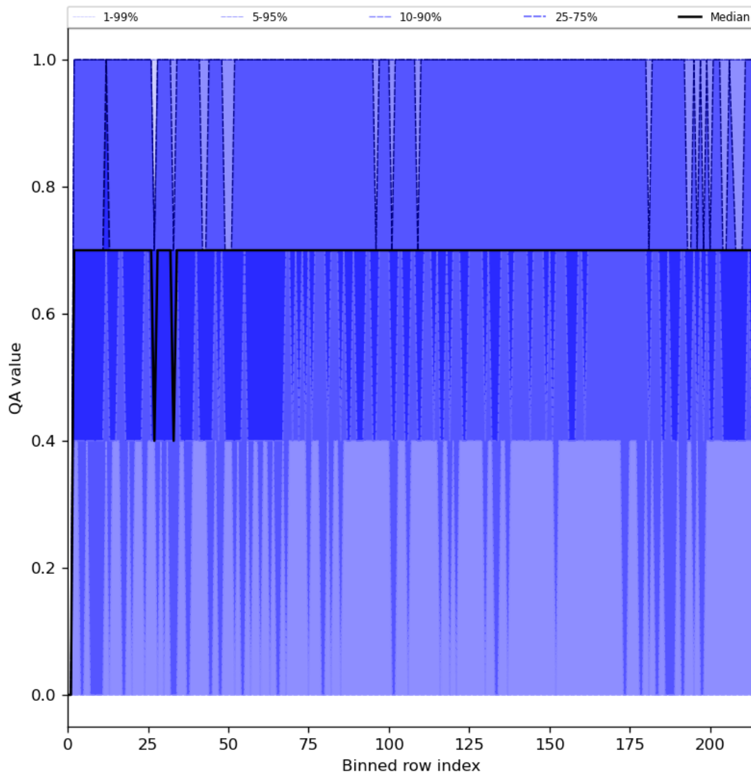
Figure 25: Along track statistics of “QA value” for 2024-03-11 to 2024-03-13
