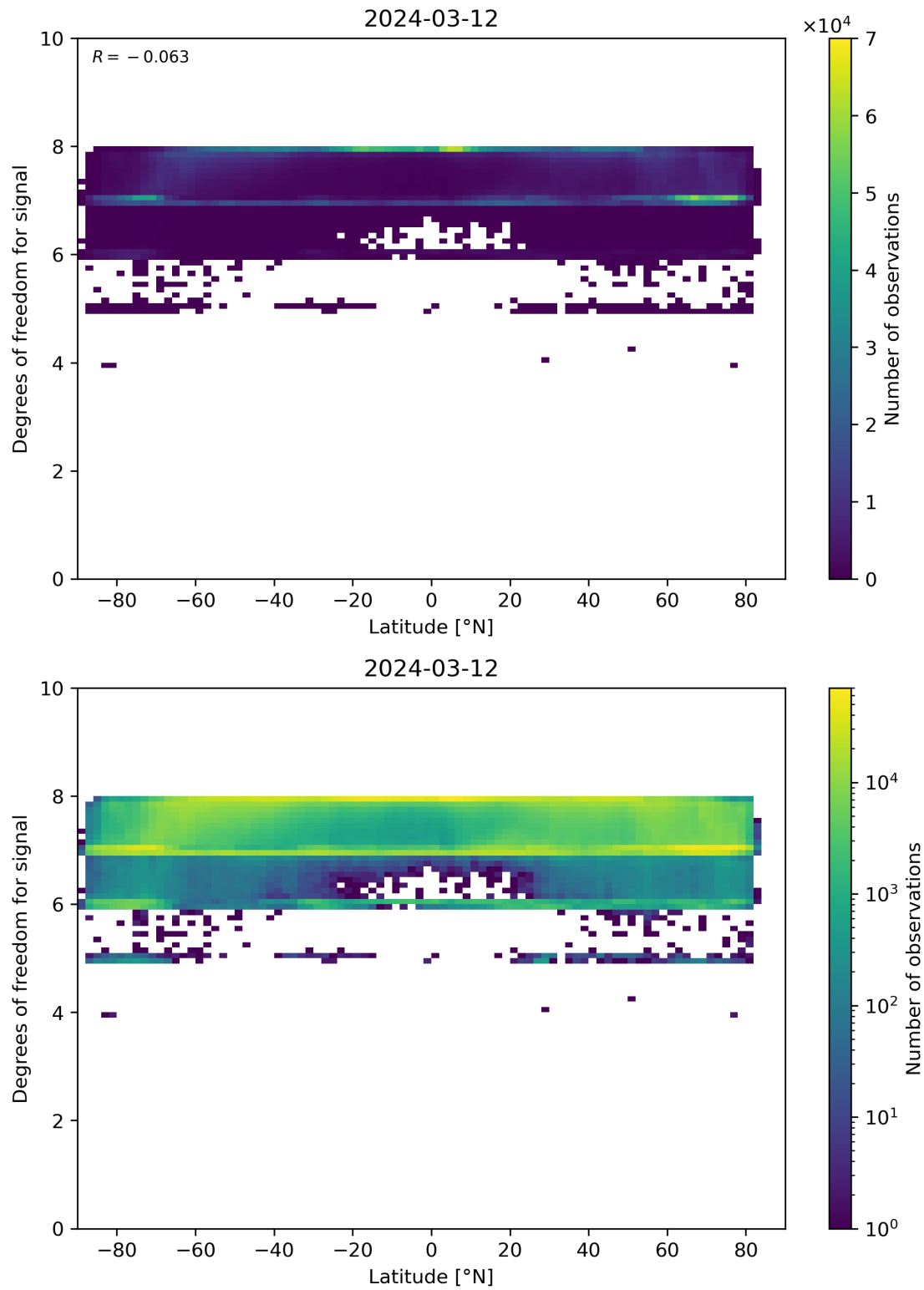
Figure 55: Scatter density plot of “Latitude” against “Degrees of freedom for signal” for 2024-03-11 to 2024-03-13.
