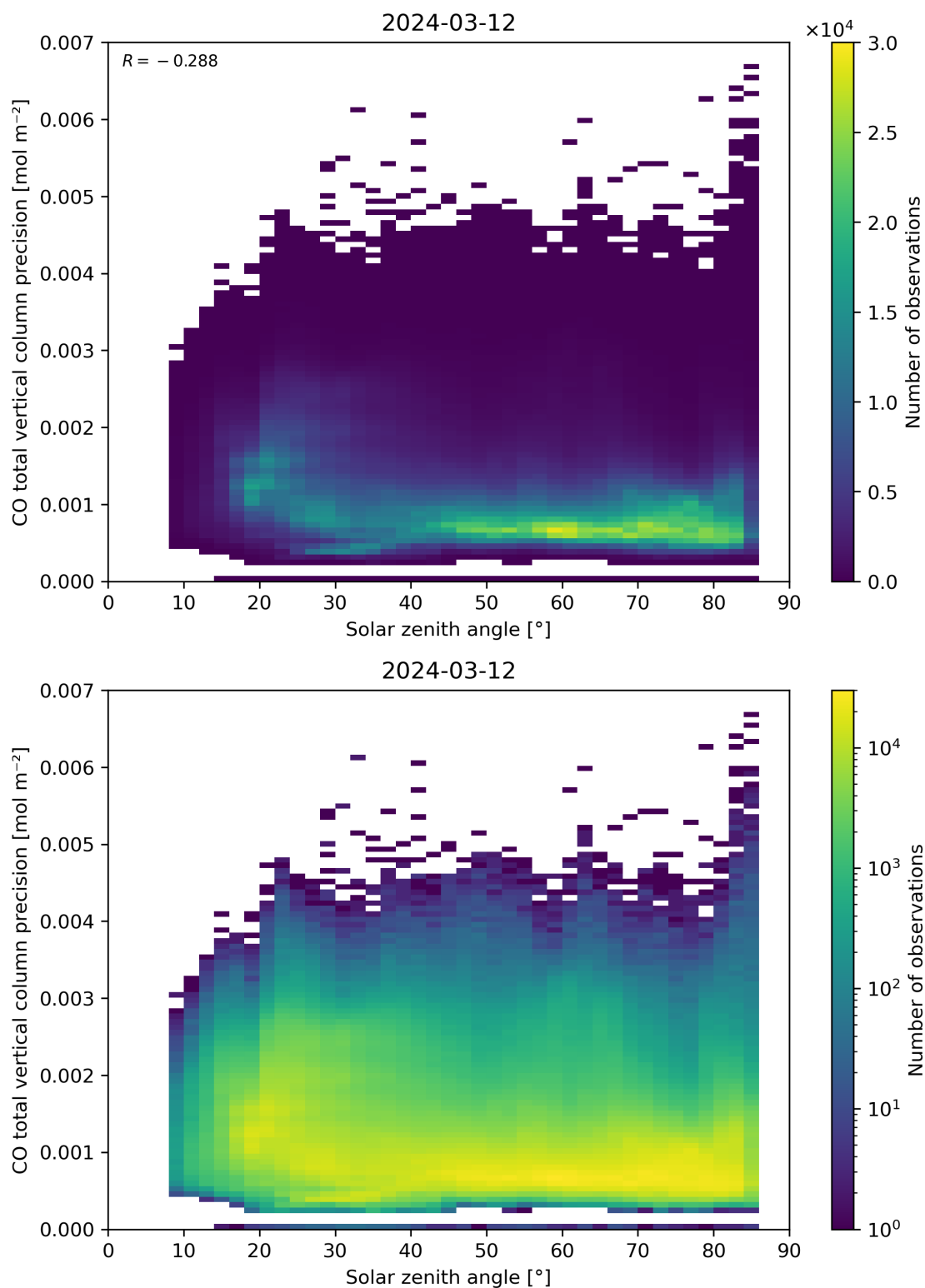
Figure 63: Scatter density plot of “Solar zenith angle” against “CO total vertical column precision” for 2024-03-11 to 2024-03-13.
