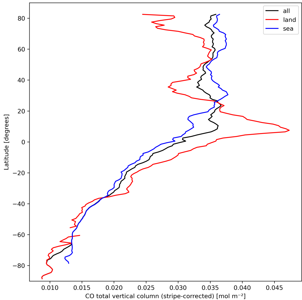
Figure 11: Zonal average of “CO total vertical column (stripe-corrected)” for 2024-03-11 to 2024-03-13.
