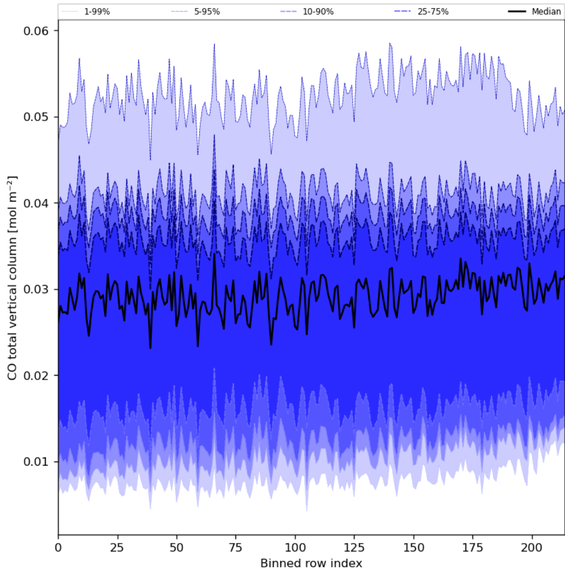
Figure 26: Along track statistics of “CO total vertical column” for 2024-03-11 to 2024-03-13
