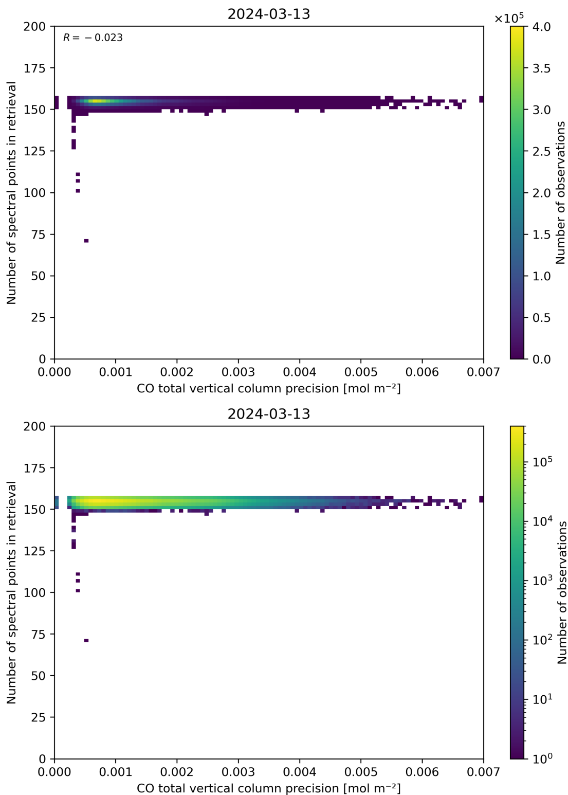
Figure 47: Scatter density plot of “CO total vertical column precision” against “Number of spectral points in retrieval” for 2024-03-12 to 2024-03-14.
