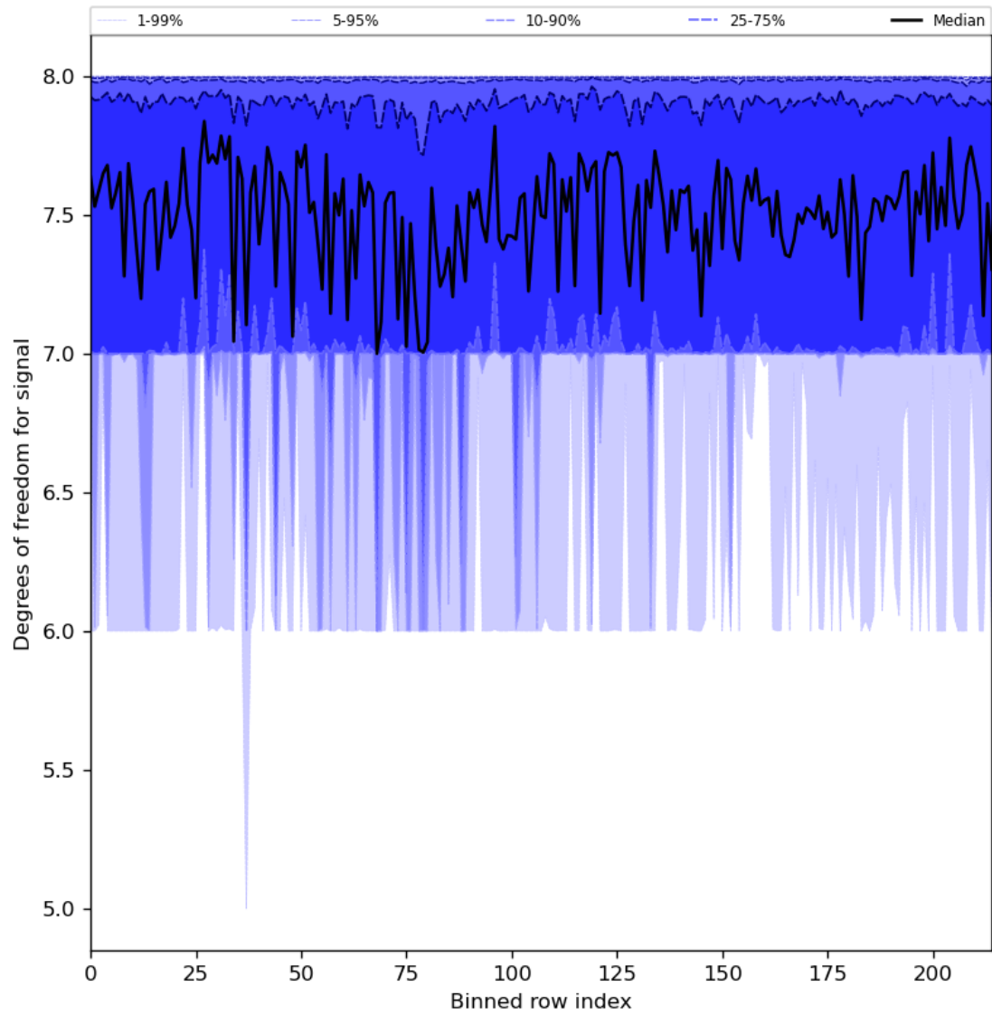
Figure 31: Along track statistics of “Degrees of freedom for signal” for 2024-03-12 to 2024-03-14
