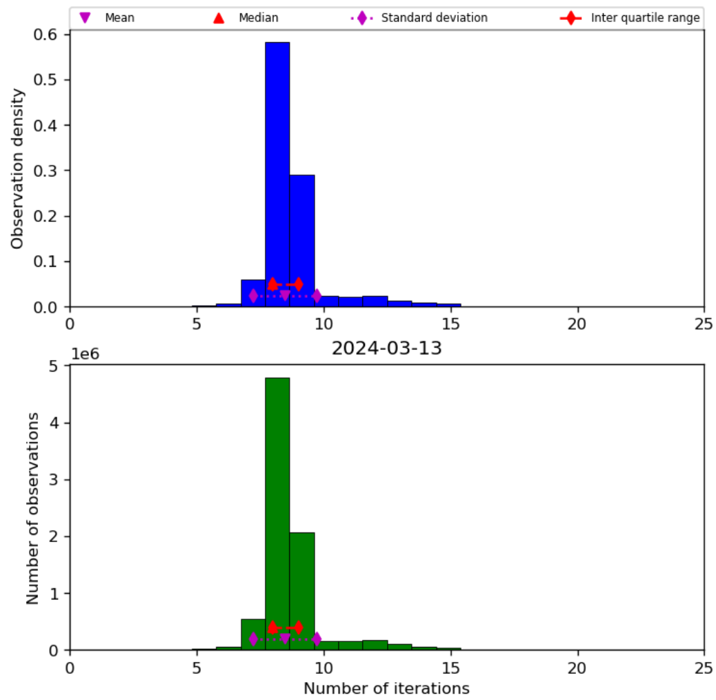
Figure 24: Histogram of “Number of iterations” for 2024-03-12 to 2024-03-14
