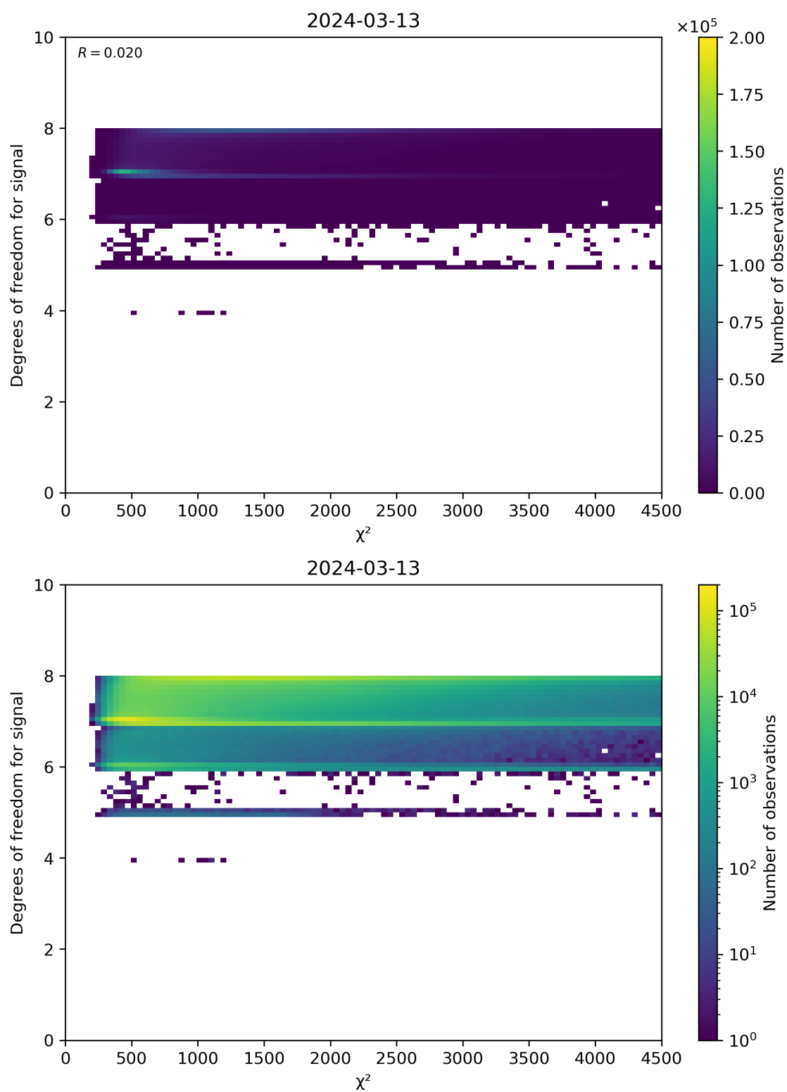
Figure 48: Scatter density plot of “ \chi^2 ” against “Degrees of freedom for signal” for 2024-03-12 to 2024-03-14.
