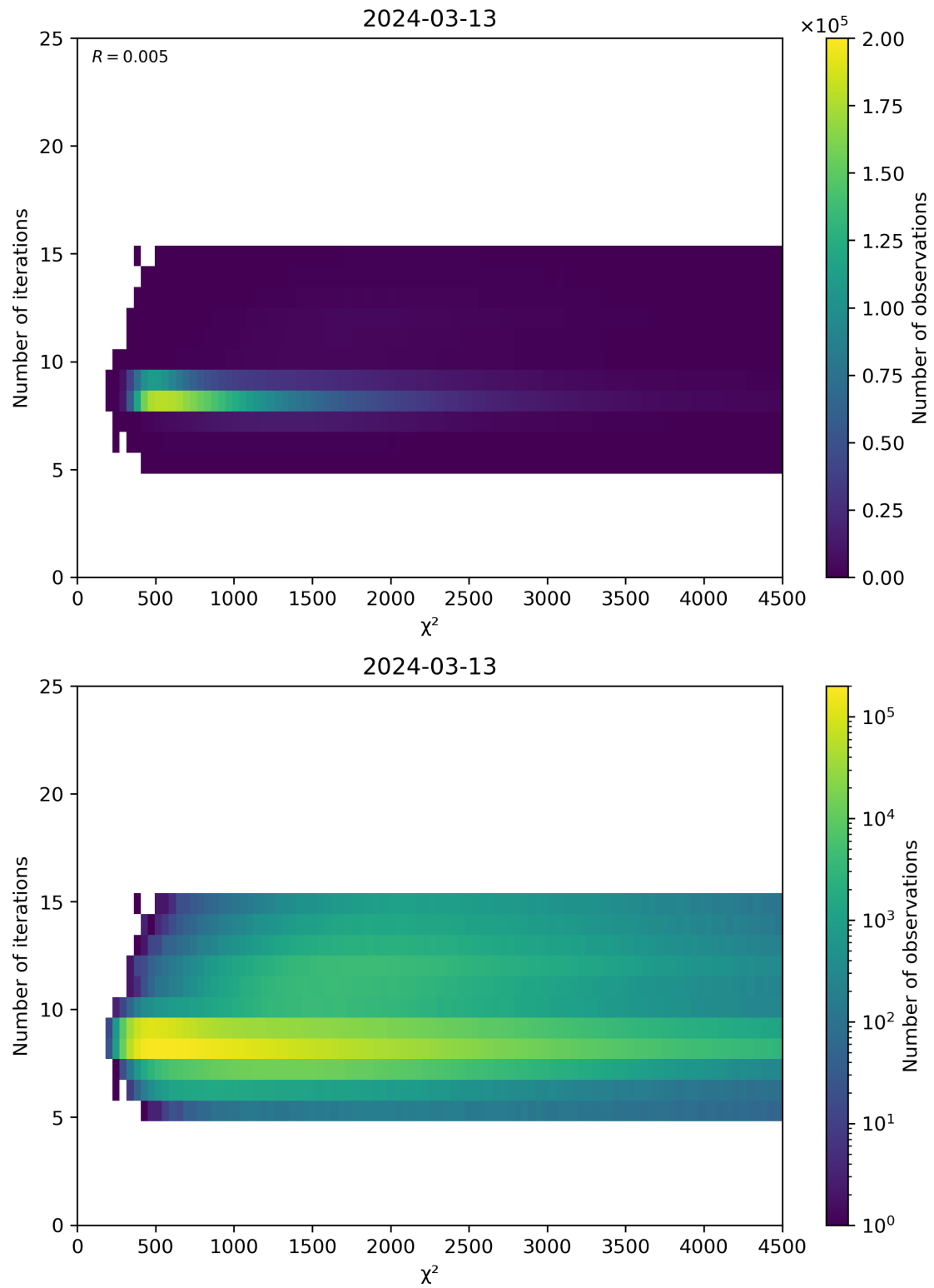
Figure 49: Scatter density plot of “ \chi^2 ” against “Number of iterations” for 2024-03-12 to 2024-03-14.
