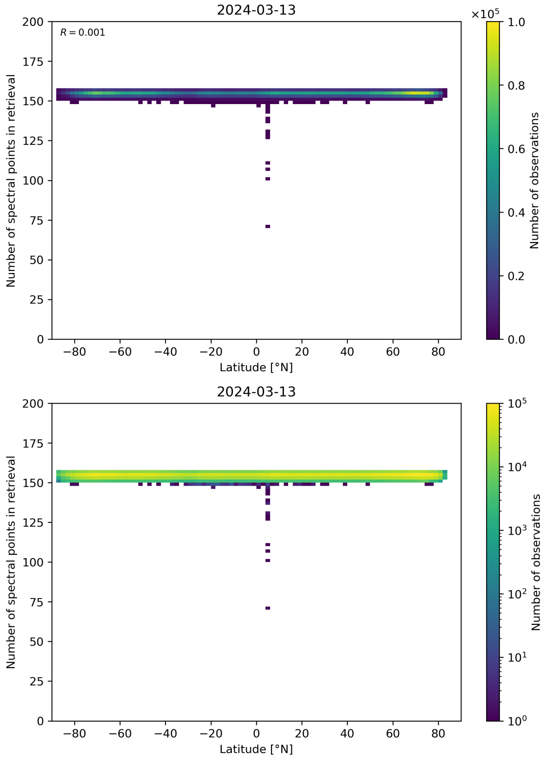
Figure 57: Scatter density plot of “Latitude” against “Number of spectral points in retrieval” for 2024-03-12 to 2024-03-14.
