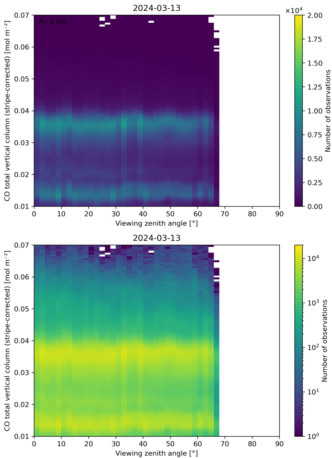
Figure 70: Scatter density plot of “Viewing zenith angle” against “CO total vertical column (stripe-corrected)” for 2024-03-12 to 2024-03-14.
