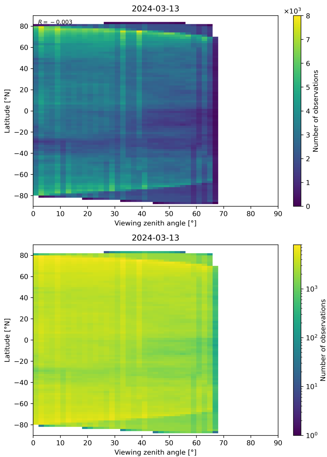
Figure 74: Scatter density plot of “Viewing zenith angle” against “Latitude” for 2024-03-12 to 2024-03-14.
