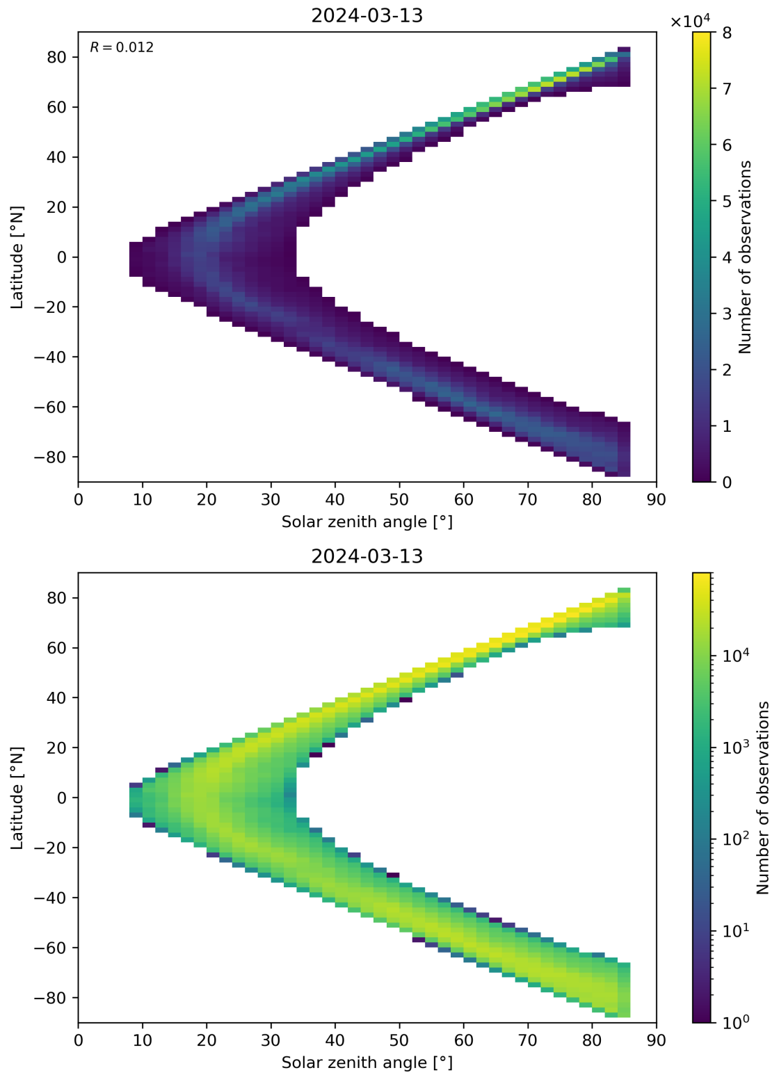
Figure 66: Scatter density plot of “Solar zenith angle” against “Latitude” for 2024-03-12 to 2024-03-14.
