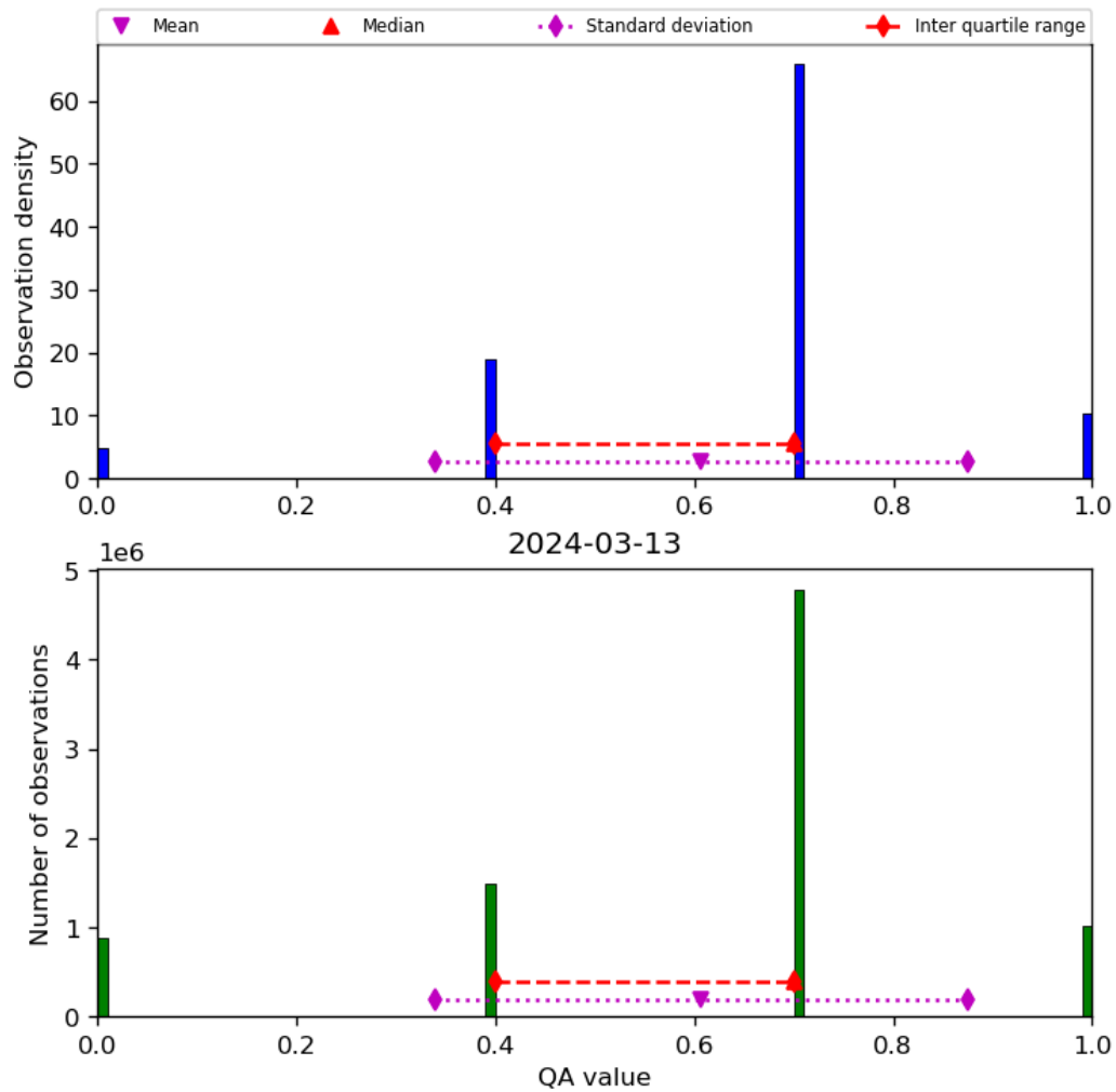
Figure 17: Histogram of “QA value” for 2024-03-12 to 2024-03-14
