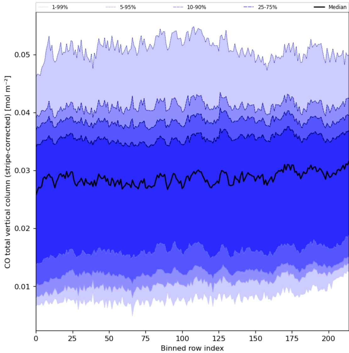
Figure 27: Along track statistics of “CO total vertical column (stripe-corrected)” for 2024-03-12 to 2024-03-14
