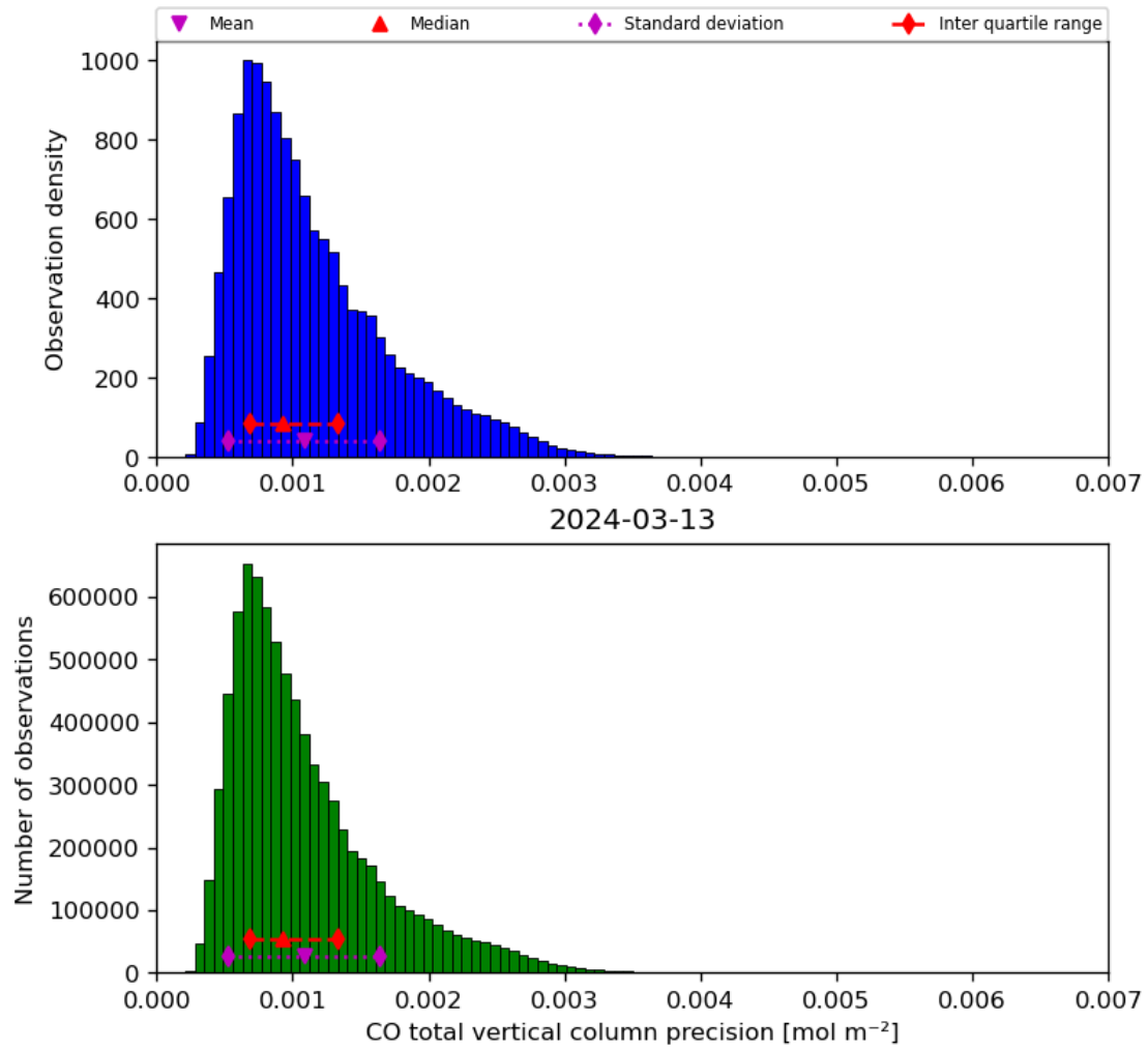
Figure 20: Histogram of “CO total vertical column precision” for 2024-03-12 to 2024-03-14
