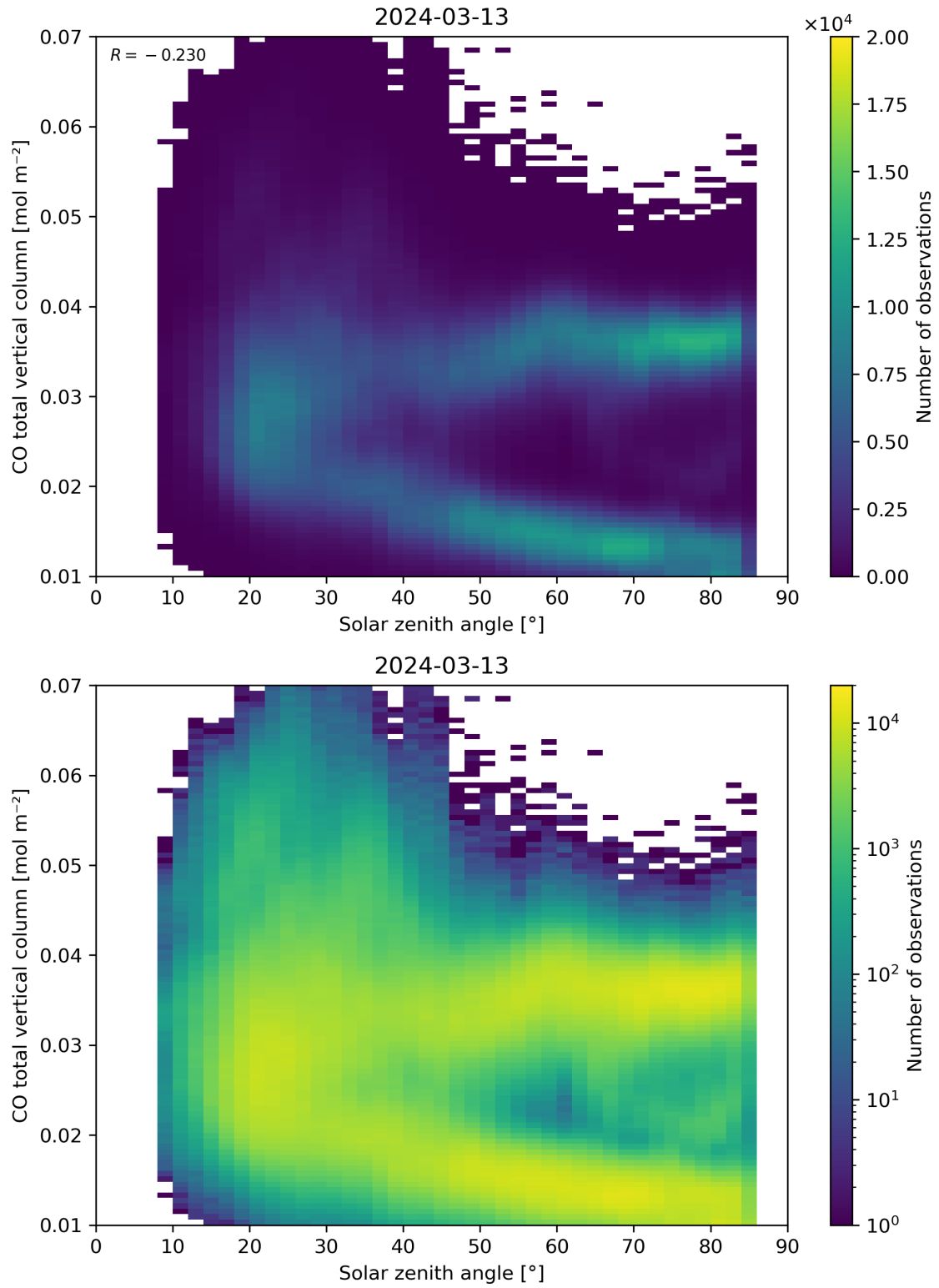
Figure 61: Scatter density plot of “Solar zenith angle” against “CO total vertical column” for 2024-03-12 to 2024-03-14.
