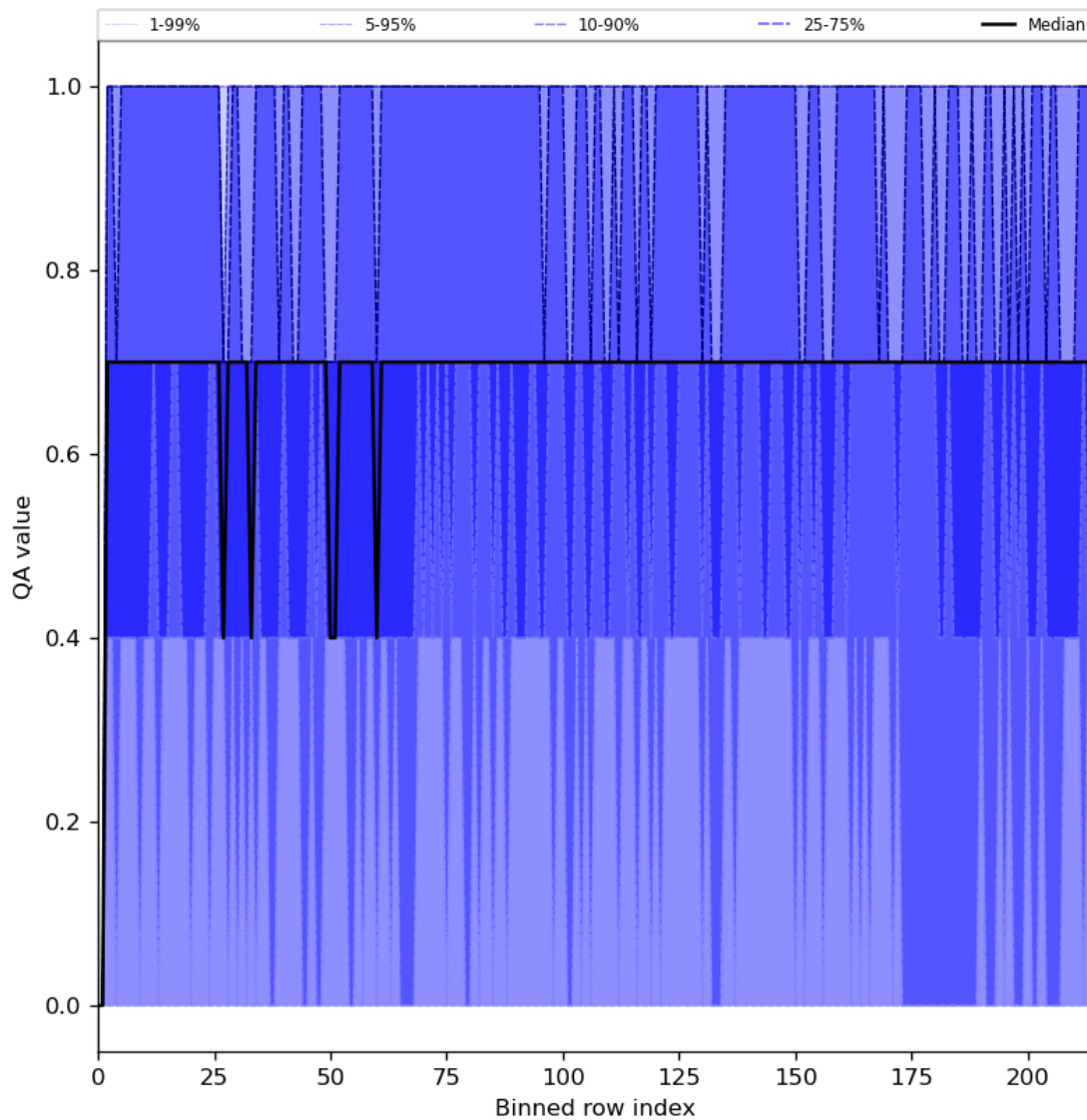
Figure 25: Along track statistics of “QA value” for 2024-03-12 to 2024-03-14
