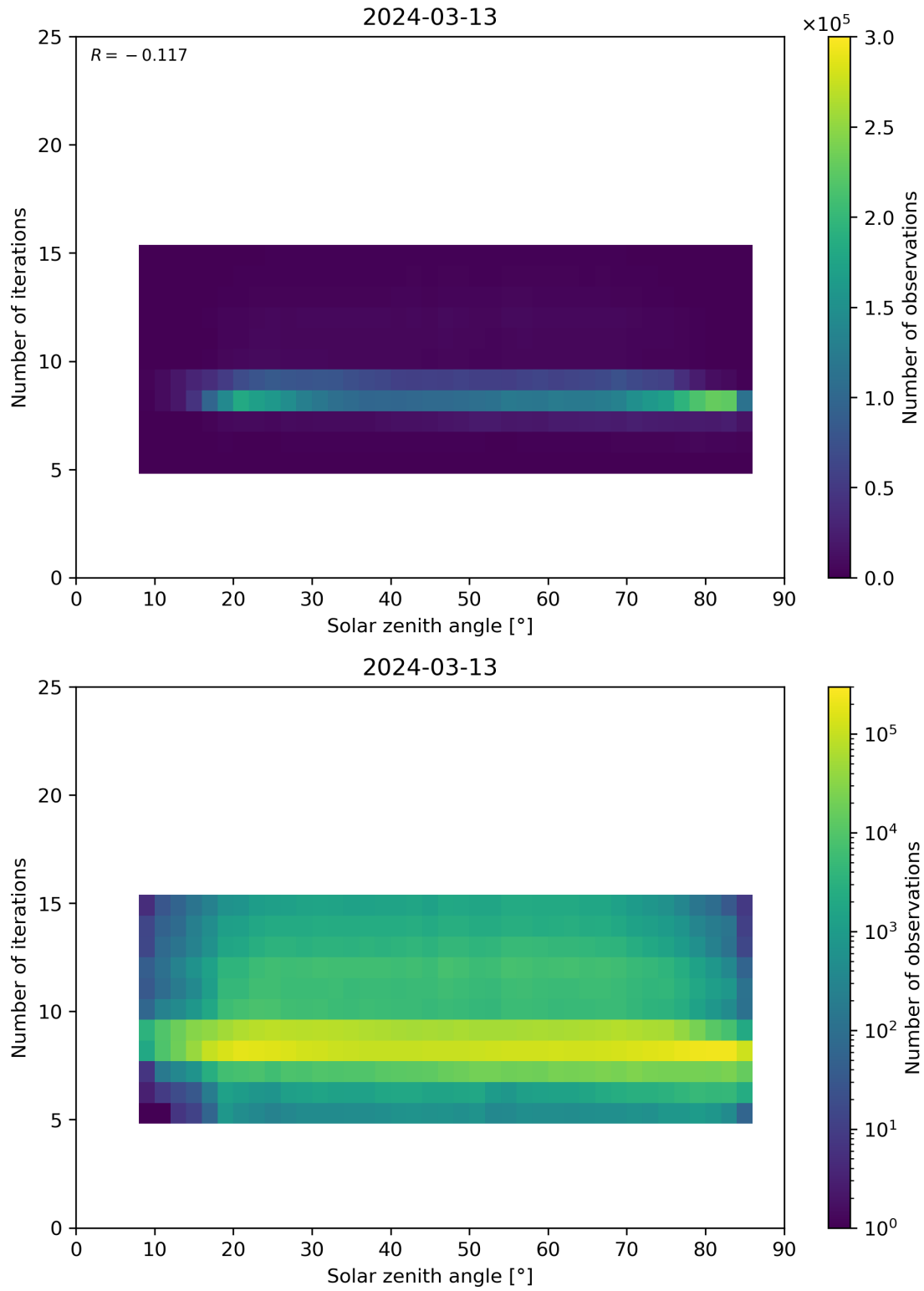
Figure 67: Scatter density plot of “Solar zenith angle” against “Number of iterations” for 2024-03-12 to 2024-03-14.
