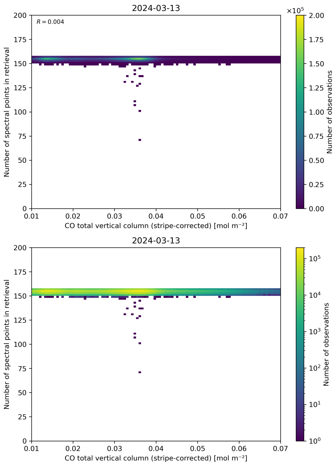
Figure 40: Scatter density plot of “CO total vertical column (stripe-corrected)” against “Number of spectral points in retrieval” for 2024-03-12 to 2024-03-14.
