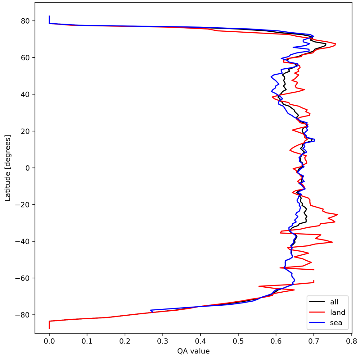
Figure 9: Zonal average of “QA value” for 2024-03-12 to 2024-03-14.
