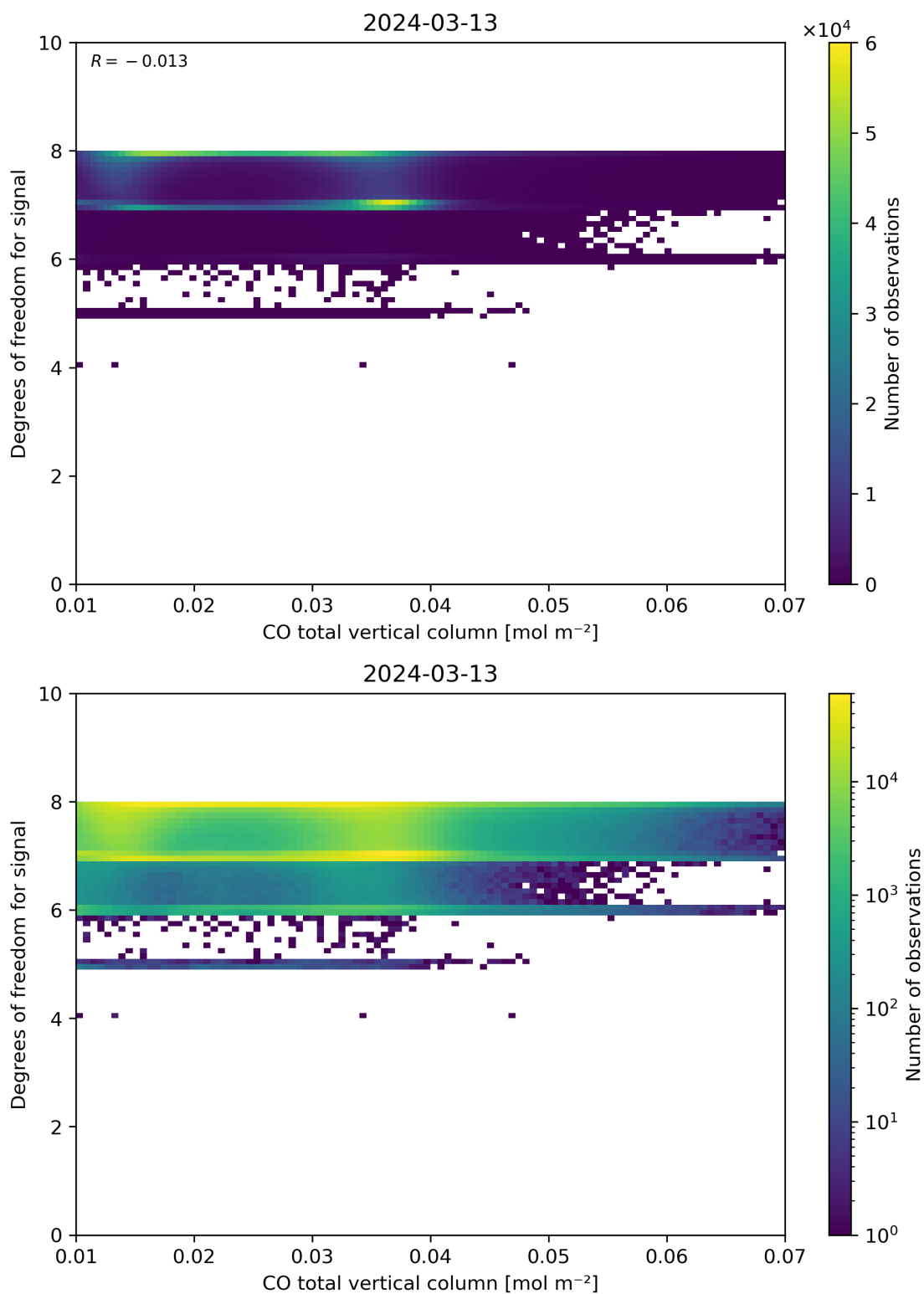
Figure 41: Scatter density plot of “CO total vertical column” against “Degrees of freedom for signal” for 2024-03-12 to 2024-03-14.
