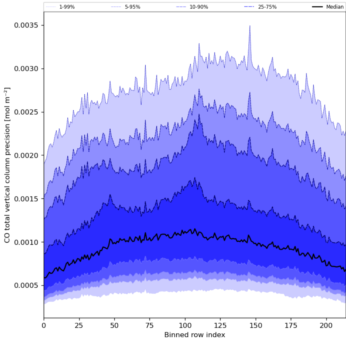
Figure 28: Along track statistics of “CO total vertical column precision” for 2024-03-12 to 2024-03-14
