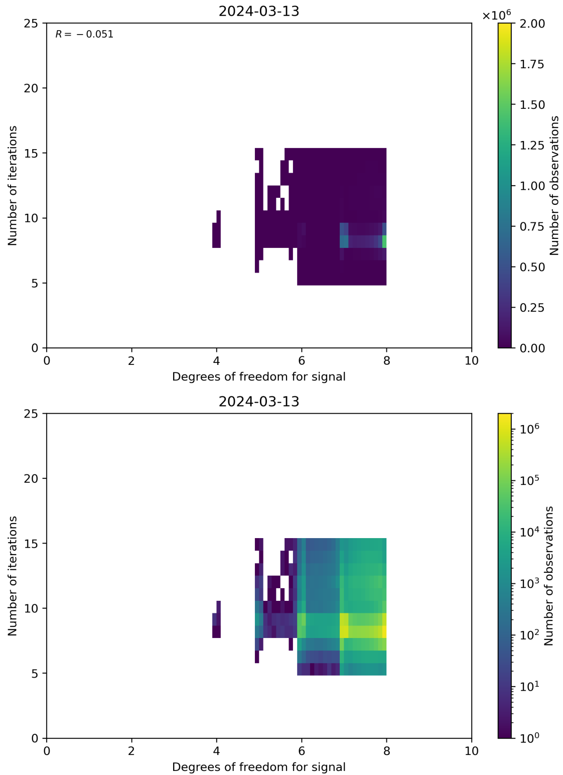
Figure 50: Scatter density plot of “Degrees of freedom for signal” against “Number of iterations” for 2024-03-12 to 2024-03-14.
