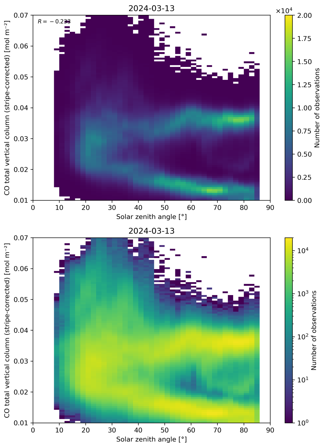
Figure 62: Scatter density plot of “Solar zenith angle” against “CO total vertical column (stripe-corrected)” for 2024-03-12 to 2024-03-14.
