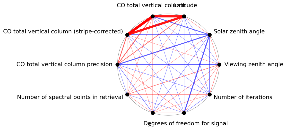
Figure 1: Map of correlation graph for 2024-03-12 to 2024-03-14.
