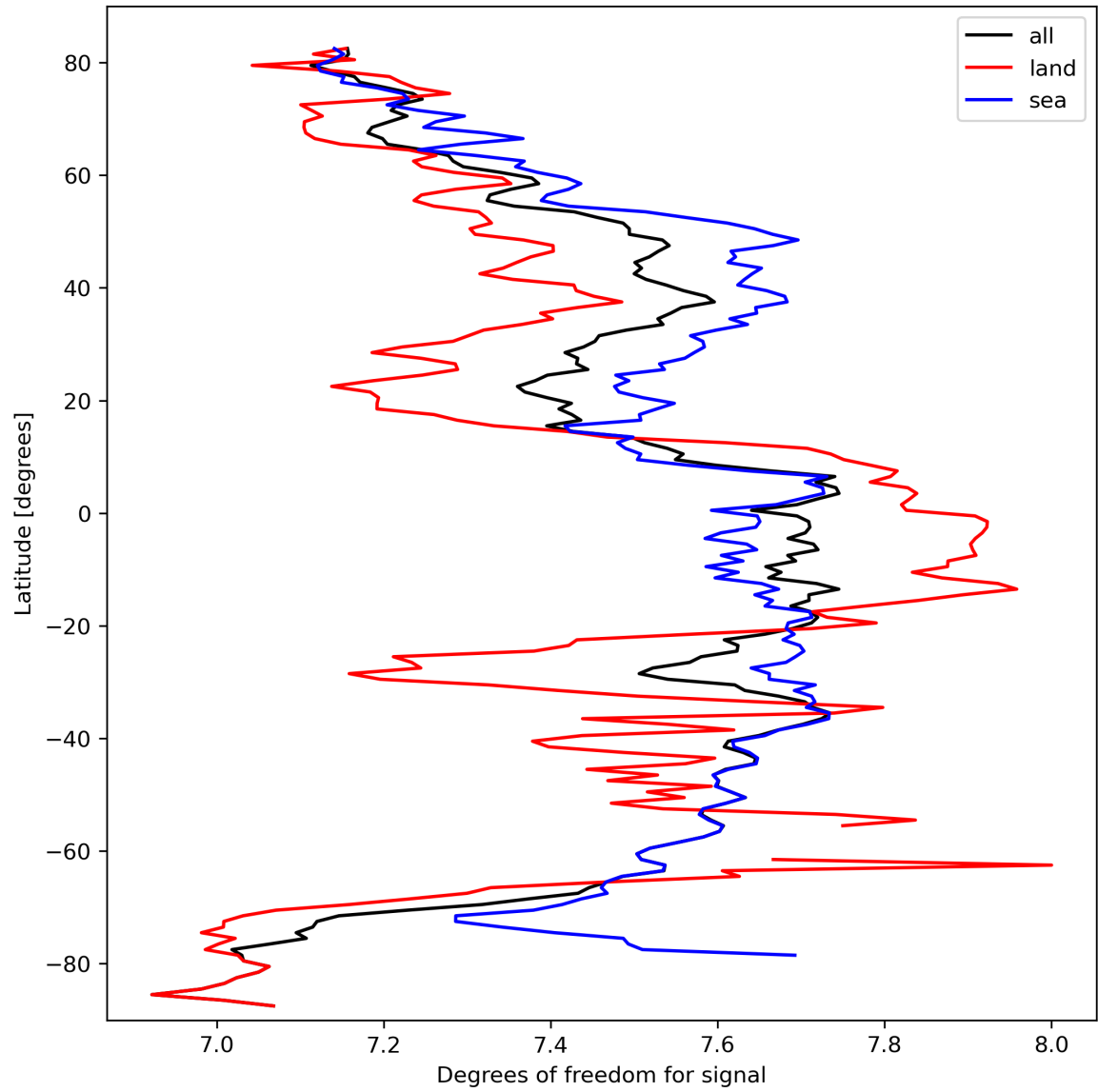
Figure 15: Zonal average of “Degrees of freedom for signal” for 2024-03-12 to 2024-03-14.
