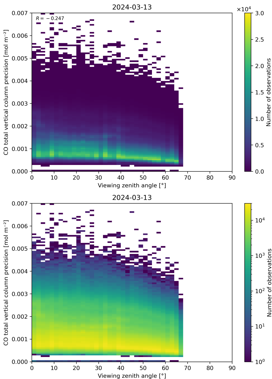
Figure 71: Scatter density plot of “Viewing zenith angle” against “CO total vertical column precision” for 2024-03-12 to 2024-03-14.
