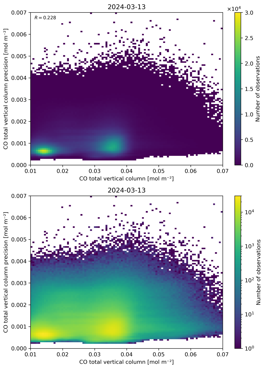
Figure 34: Scatter density plot of “CO total vertical column” against “CO total vertical column precision” for 2024-03-12 to 2024-03-14.
