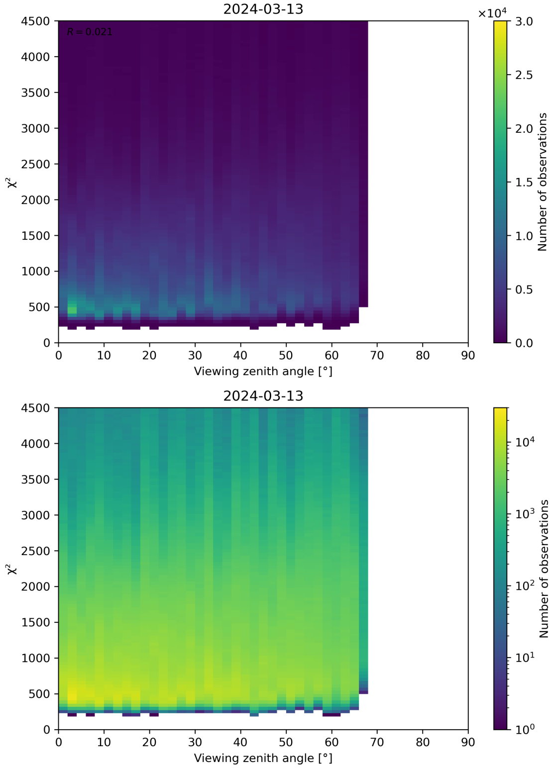
Figure 72: Scatter density plot of “Viewing zenith angle” against “ \chi^2 ” for 2024-03-12 to 2024-03-14.
