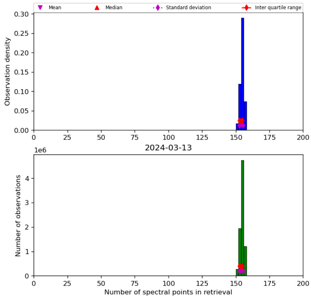
Figure 21: Histogram of “Number of spectral points in retrieval” for 2024-03-12 to 2024-03-14
