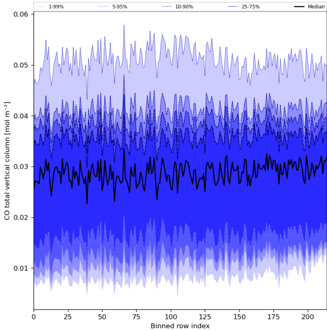
Figure 26: Along track statistics of “CO total vertical column” for 2024-03-12 to 2024-03-14
