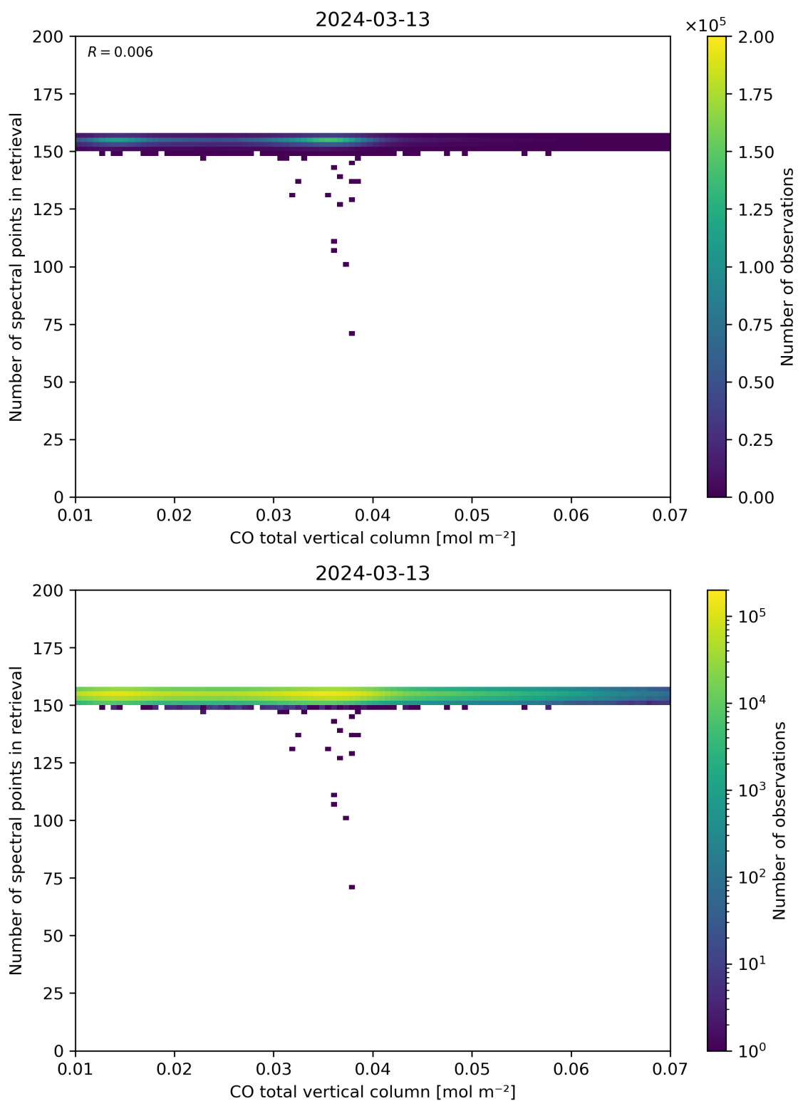
Figure 43: Scatter density plot of “CO total vertical column” against “Number of spectral points in retrieval” for 2024-03-12 to 2024-03-14.
