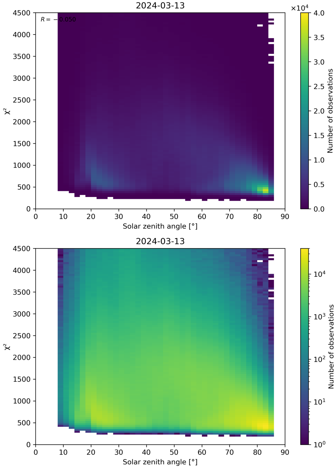
Figure 64: Scatter density plot of “Solar zenith angle” against “ \chi^2 ” for 2024-03-12 to 2024-03-14.
