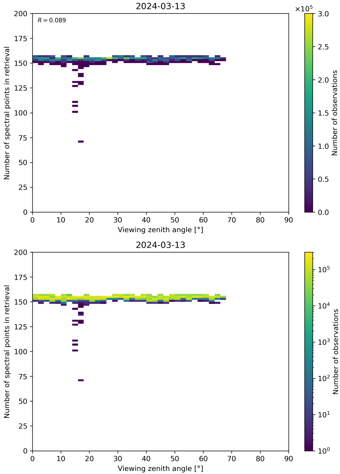
Figure 76: Scatter density plot of “Viewing zenith angle” against “Number of spectral points in retrieval” for 2024-03-12 to 2024-03-14.
