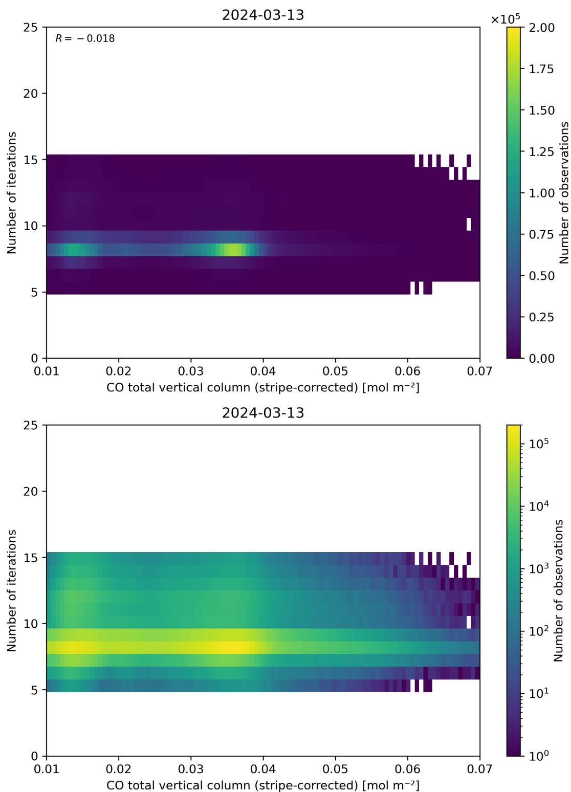
Figure 39: Scatter density plot of “CO total vertical column (stripe-corrected)” against “Number of iterations” for 2024-03-12 to 2024-03-14.
