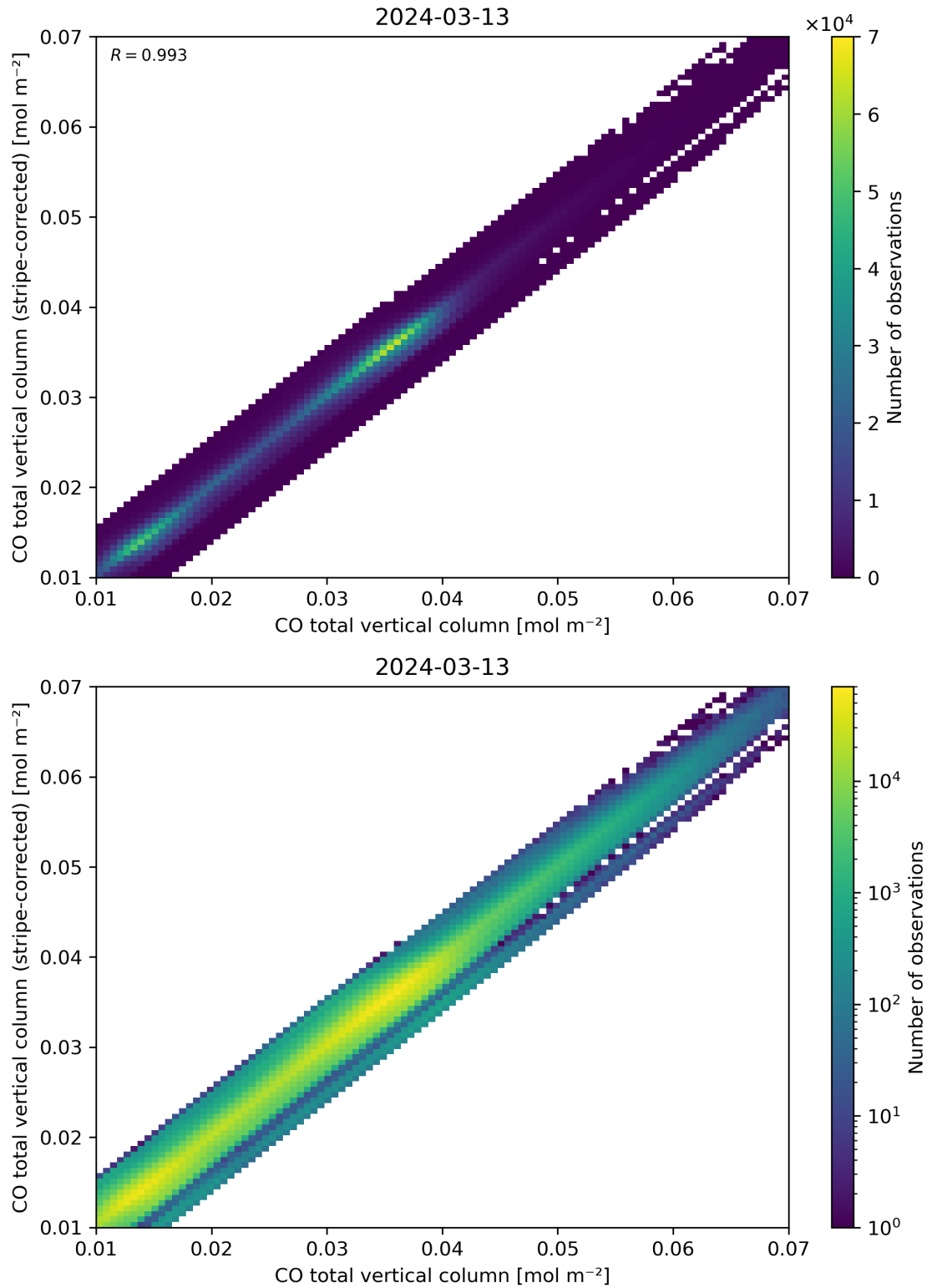
Figure 33: Scatter density plot of “CO total vertical column” against “CO total vertical column (stripe-corrected)” for 2024-03-12 to 2024-03-14.
