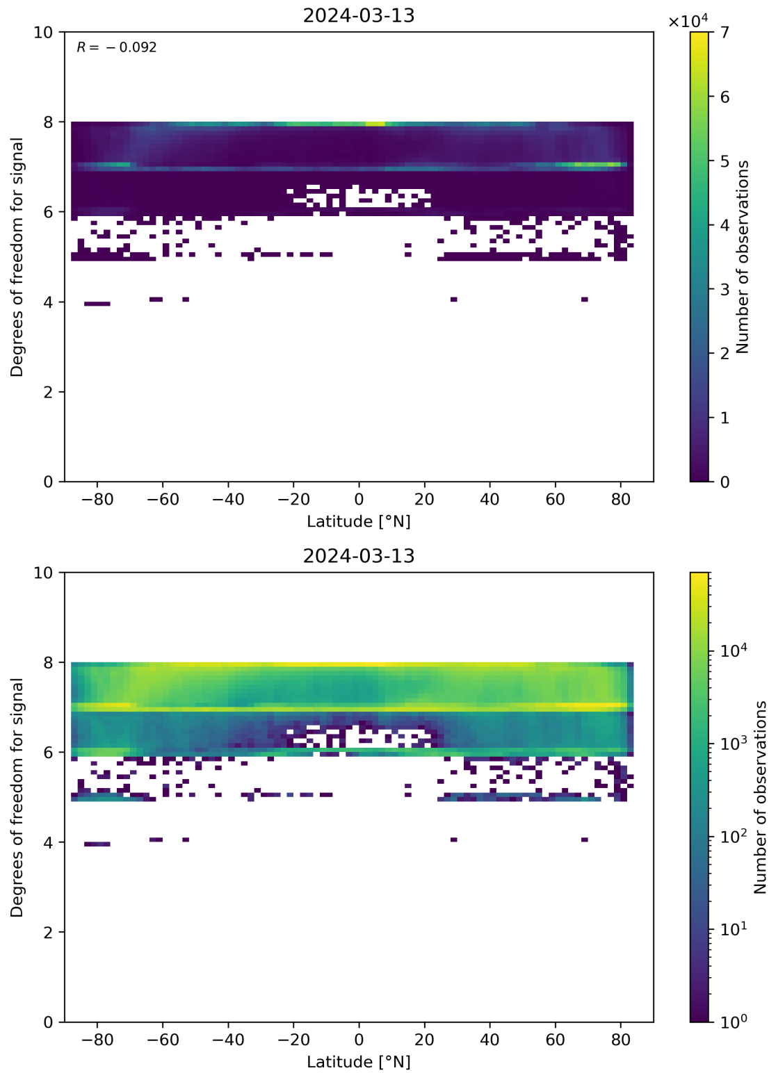
Figure 55: Scatter density plot of “Latitude” against “Degrees of freedom for signal” for 2024-03-12 to 2024-03-14.
