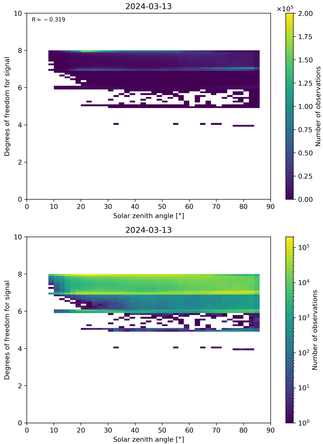
Figure 65: Scatter density plot of “Solar zenith angle” against “Degrees of freedom for signal” for 2024-03-12 to 2024-03-14.
