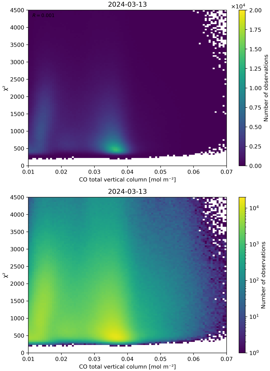
Figure 35: Scatter density plot of “CO total vertical column” against “ \chi^2 ” for 2024-03-12 to 2024-03-14.
