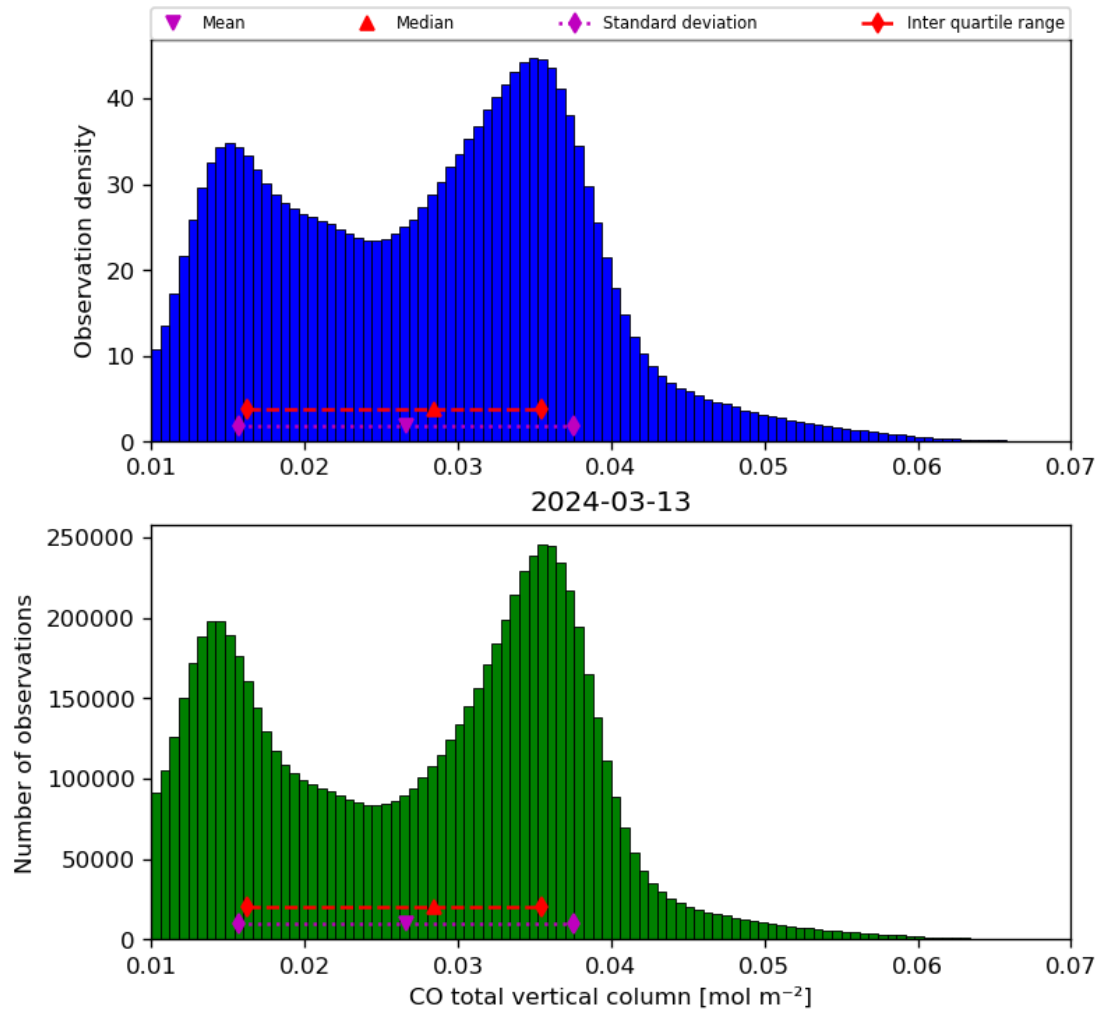
Figure 18: Histogram of “CO total vertical column” for 2024-03-12 to 2024-03-14
