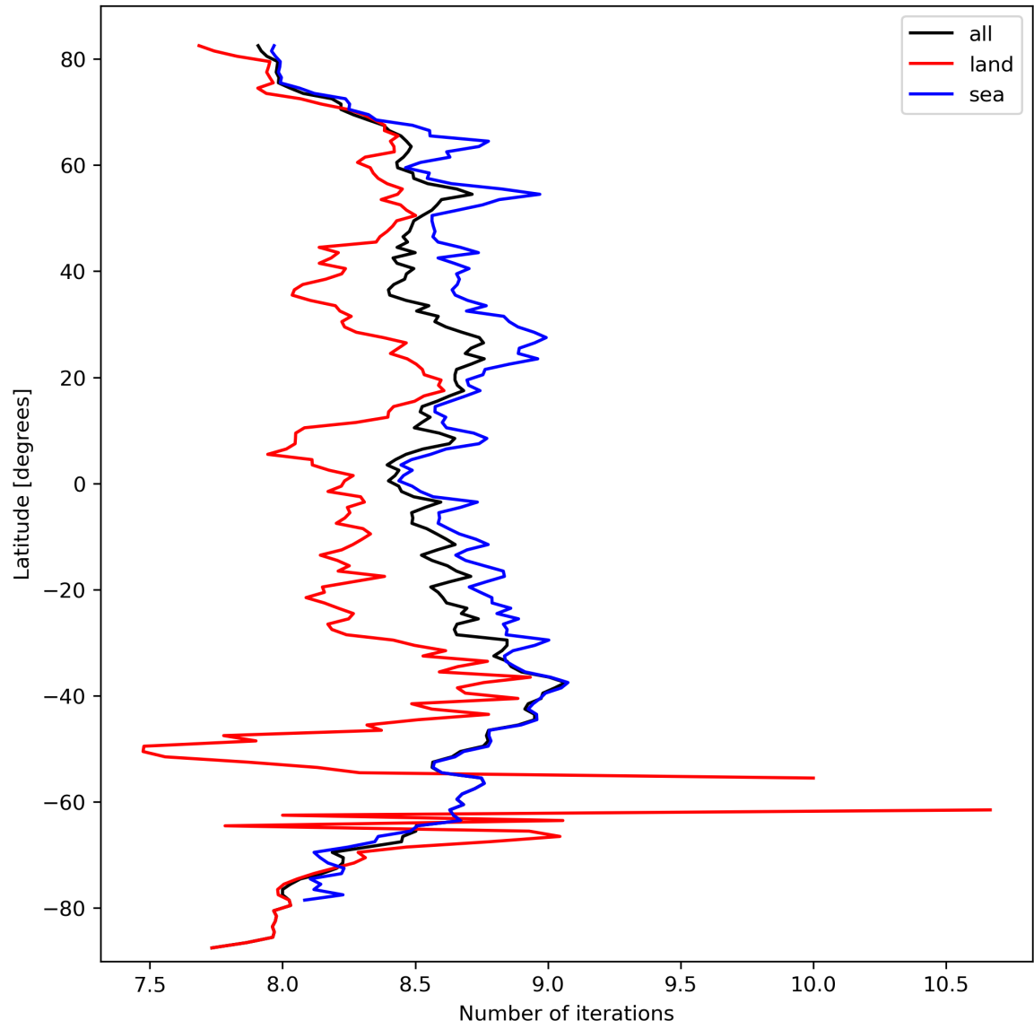
Figure 16: Zonal average of “Number of iterations” for 2024-03-12 to 2024-03-14.
