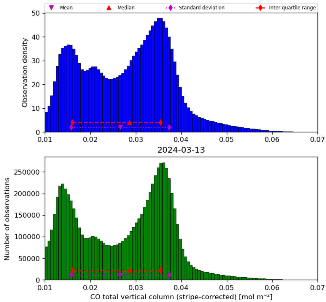
Figure 19: Histogram of “CO total vertical column (stripe-corrected)” for 2024-03-12 to 2024-03-14
