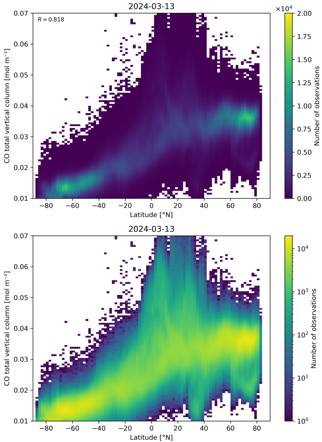
Figure 51: Scatter density plot of “Latitude” against “CO total vertical column” for 2024-03-12 to 2024-03-14.
