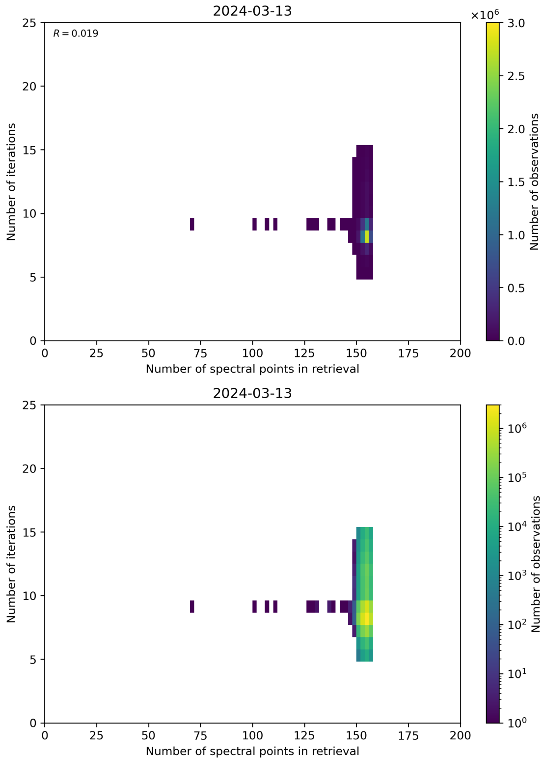
Figure 60: Scatter density plot of “Number of spectral points in retrieval” against “Number of iterations” for 2024-03-12 to 2024-03-14.
