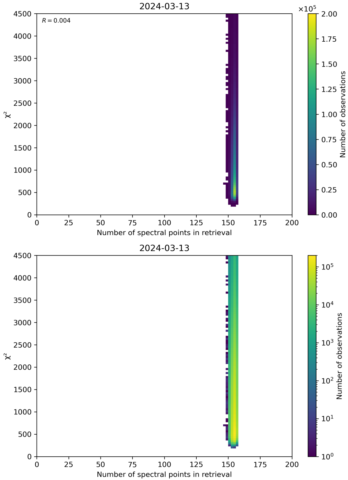
Figure 58: Scatter density plot of “Number of spectral points in retrieval” against “ \chi^2 ” for 2024-03-12 to 2024-03-14.
