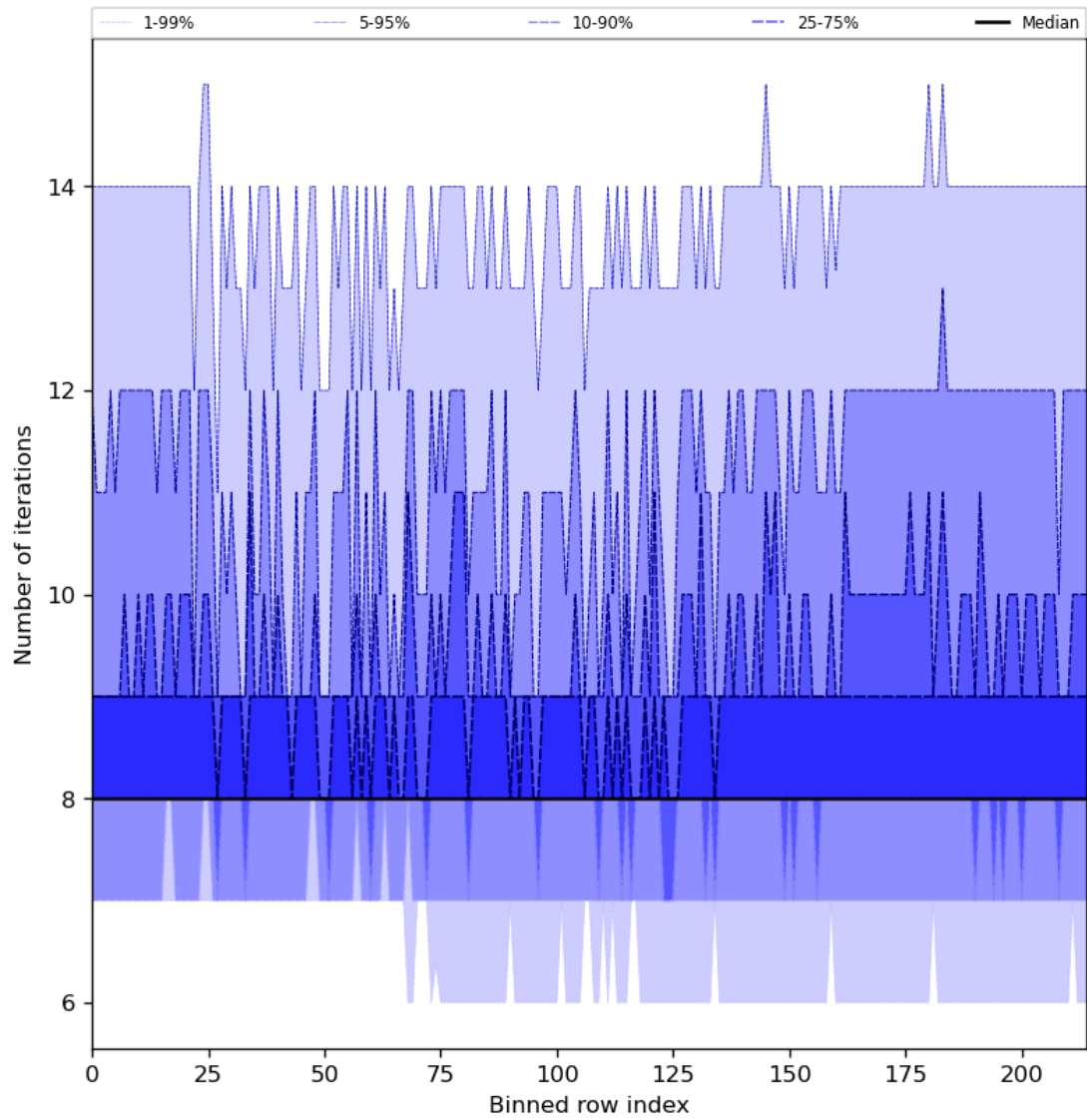
Figure 32: Along track statistics of “Number of iterations” for 2024-03-12 to 2024-03-14
