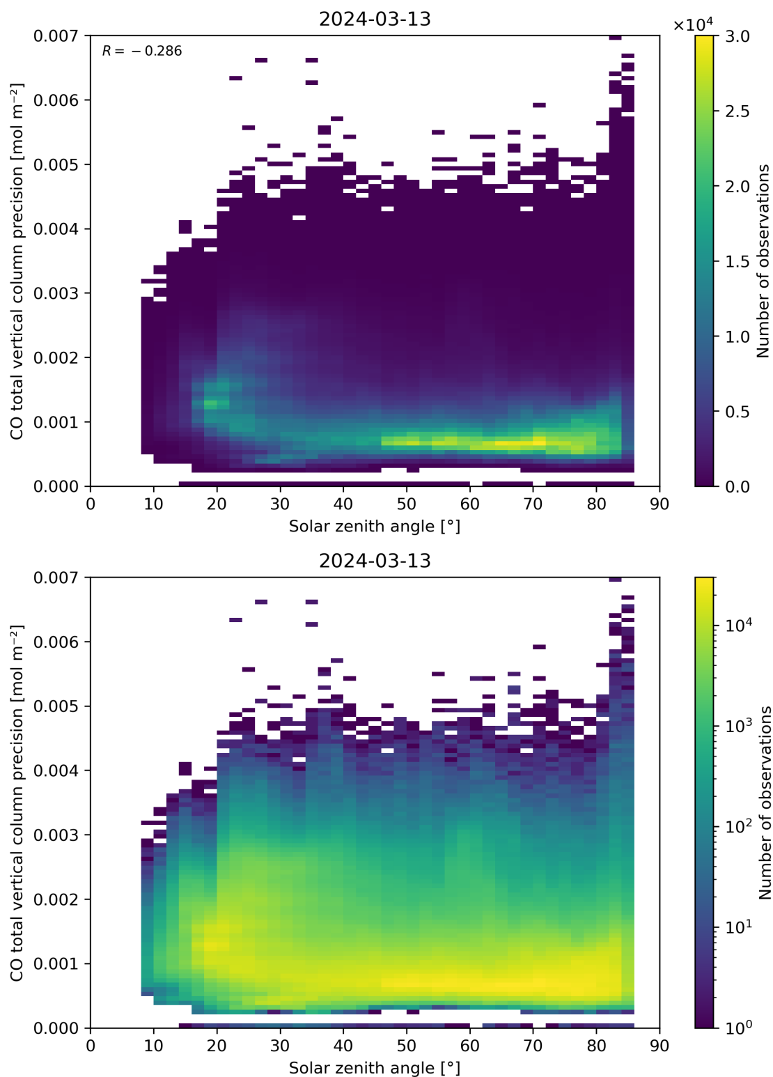
Figure 63: Scatter density plot of “Solar zenith angle” against “CO total vertical column precision” for 2024-03-12 to 2024-03-14.
