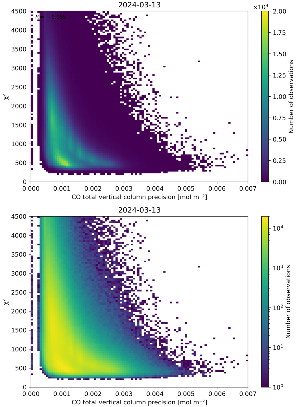
Figure 44: Scatter density plot of “CO total vertical column precision” against “ \chi^2 ” for 2024-03-12 to 2024-03-14.
