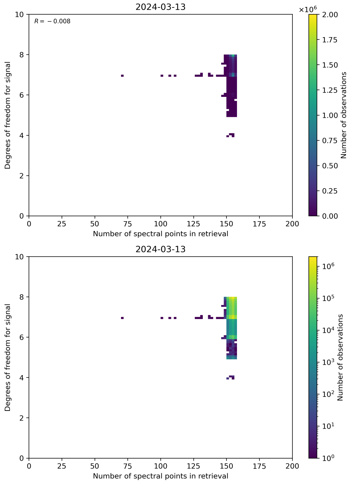
Figure 59: Scatter density plot of “Number of spectral points in retrieval” against “Degrees of freedom for signal” for 2024-03-12 to 2024-03-14.
