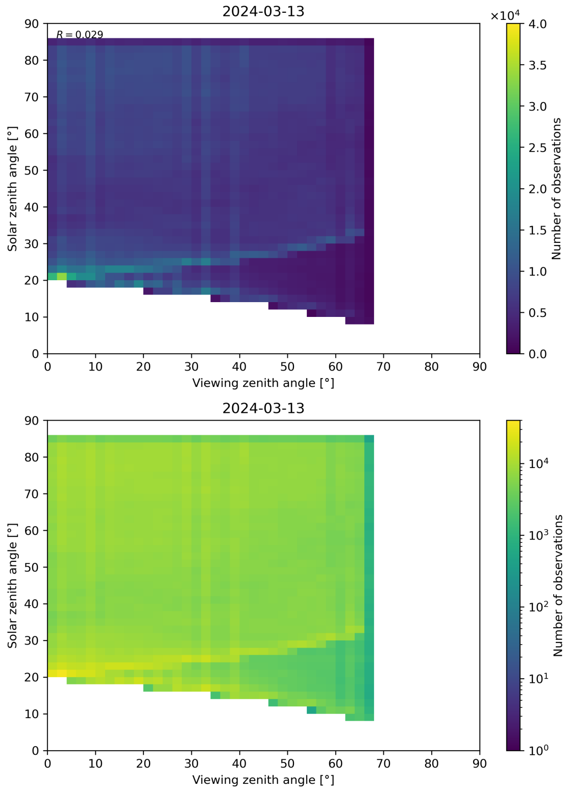
Figure 77: Scatter density plot of “Viewing zenith angle” against “Solar zenith angle” for 2024-03-12 to 2024-03-14.
