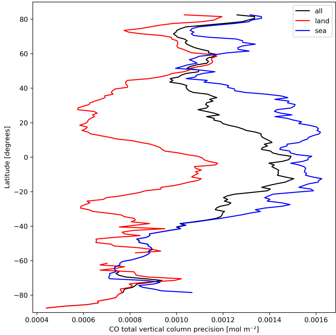
Figure 12: Zonal average of "CO total vertical column precision" for 2024-03-12 to 2024-03-14.
