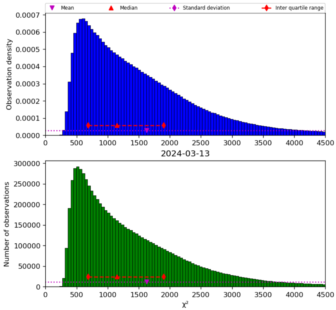
Figure 22: Histogram of “ \chi^2 ” for 2024-03-12 to 2024-03-14
