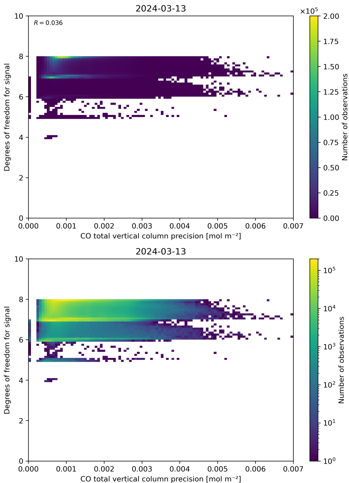
Figure 45: Scatter density plot of “CO total vertical column precision” against “Degrees of freedom for signal” for 2024-03-12 to 2024-03-14.
