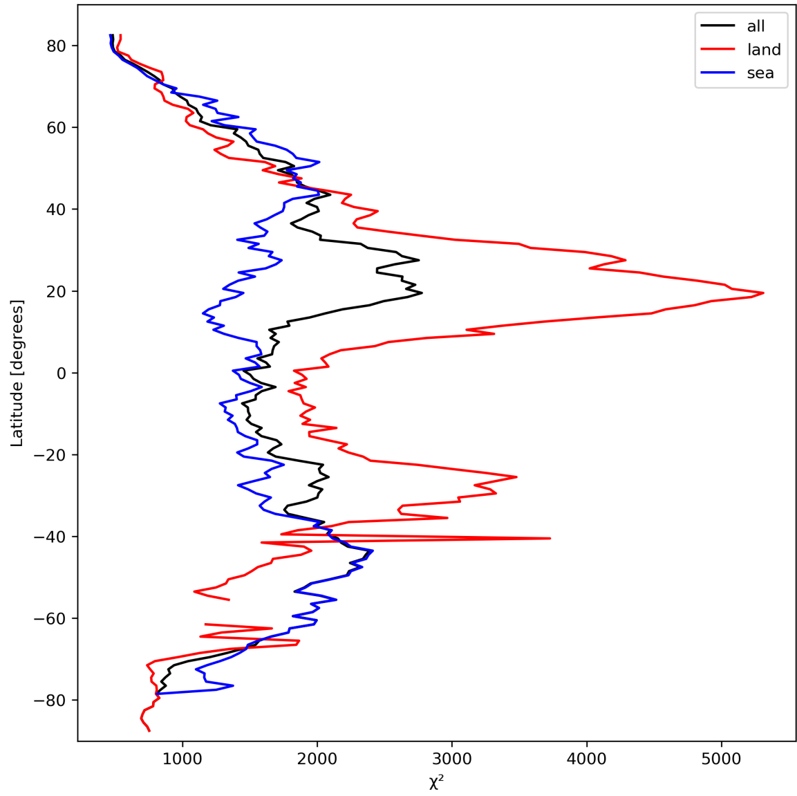
Figure 14: Zonal average of “ \chi^2 ” for 2024-03-12 to 2024-03-14.
