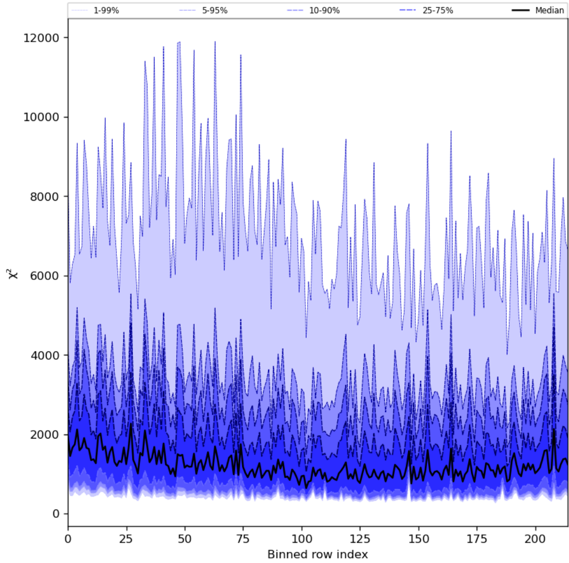
Figure 30: Along track statistics of “ \chi^2 ” for 2024-03-12 to 2024-03-14
