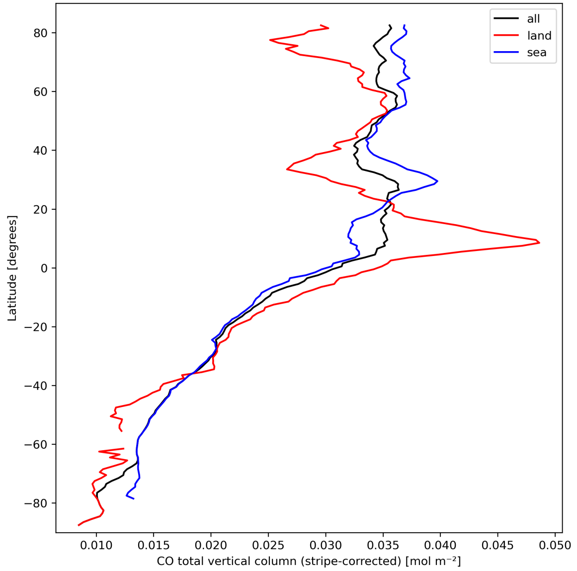
Figure 11: Zonal average of “CO total vertical column (stripe-corrected)” for 2024-03-12 to 2024-03-14.
