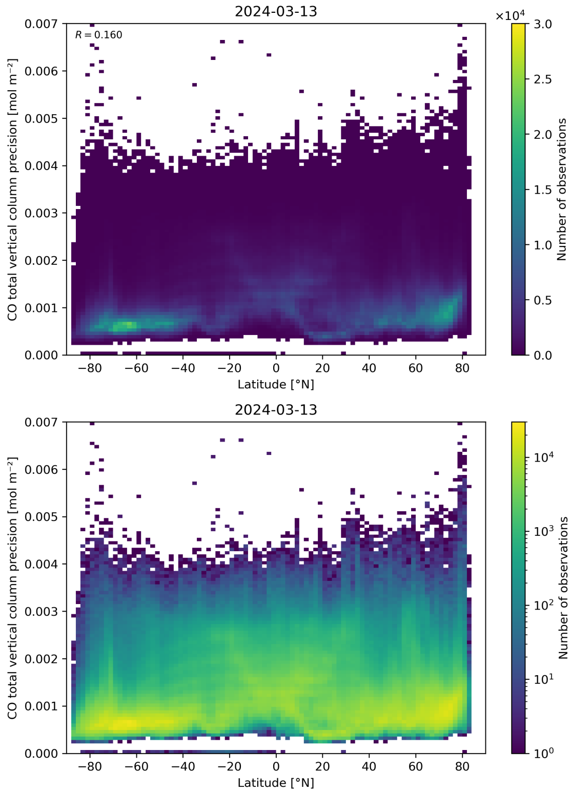
Figure 53: Scatter density plot of “Latitude” against “CO total vertical column precision” for 2024-03-12 to 2024-03-14.
