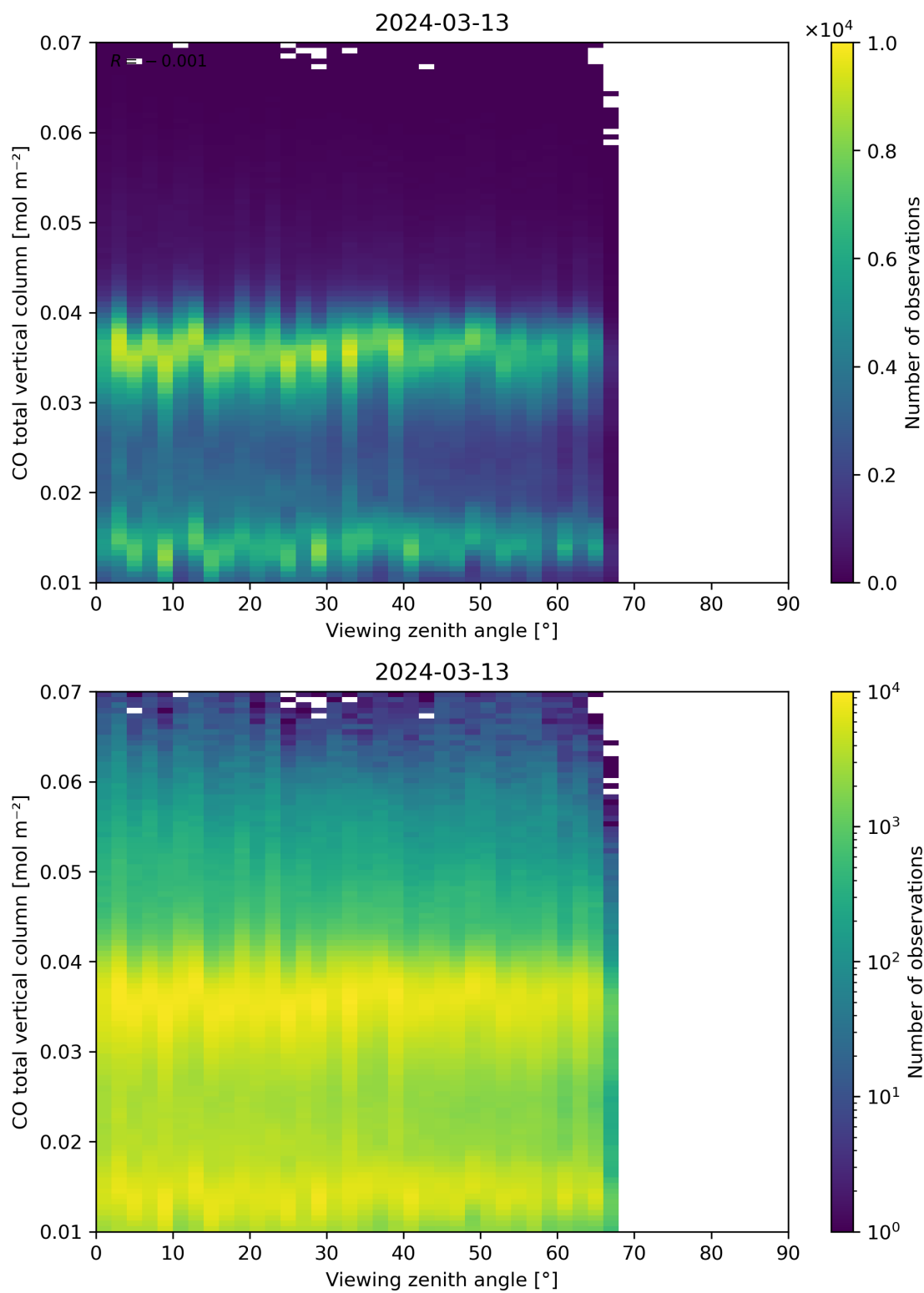
Figure 69: Scatter density plot of “Viewing zenith angle” against “CO total vertical column” for 2024-03-12 to 2024-03-14.
