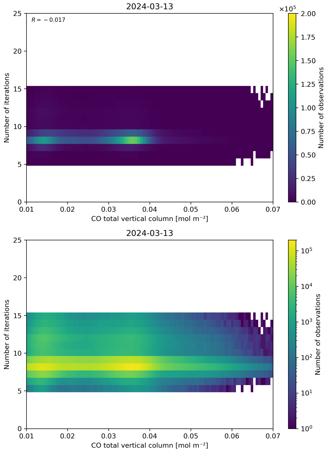
Figure 42: Scatter density plot of “CO total vertical column” against “Number of iterations” for 2024-03-12 to 2024-03-14.
