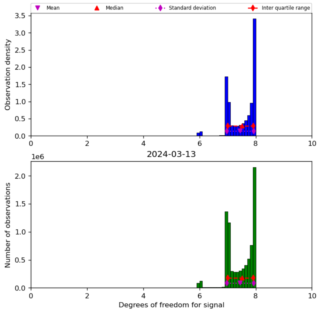
Figure 23: Histogram of “Degrees of freedom for signal” for 2024-03-12 to 2024-03-14
