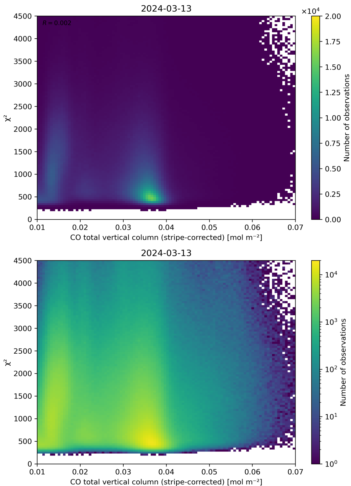
Figure 37: Scatter density plot of “CO total vertical column (stripe-corrected)” against “ \chi^2 ” for 2024-03-12 to 2024-03-14.
