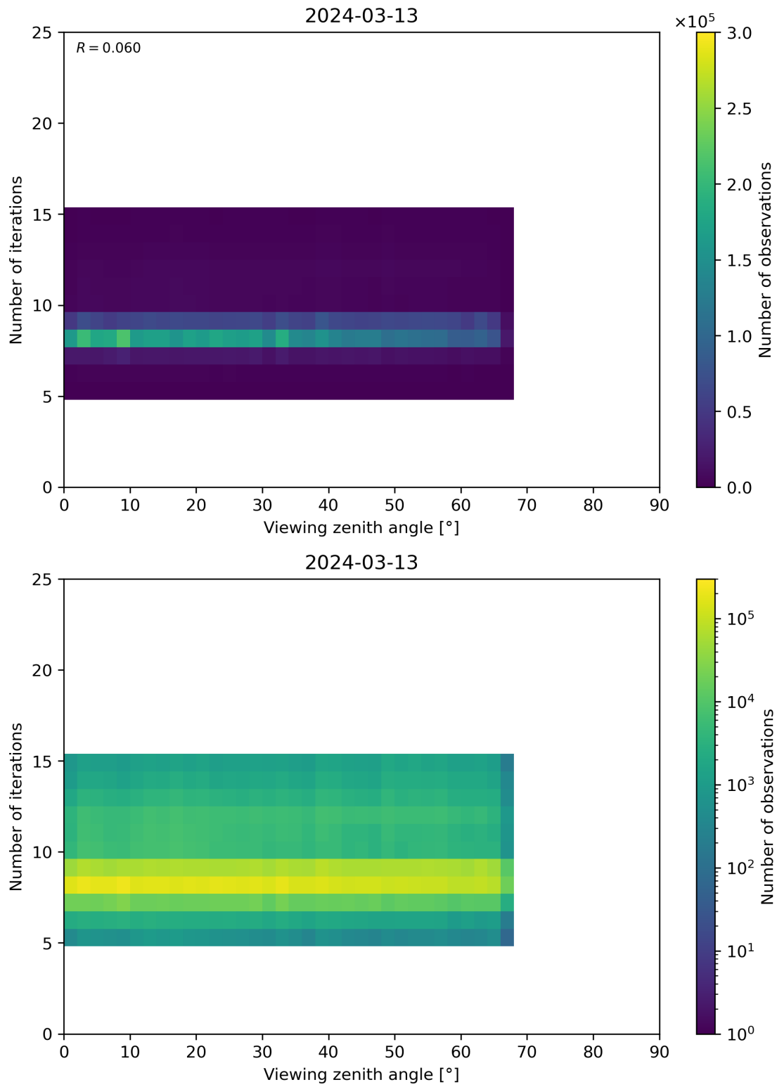
Figure 75: Scatter density plot of “Viewing zenith angle” against “Number of iterations” for 2024-03-12 to 2024-03-14.
