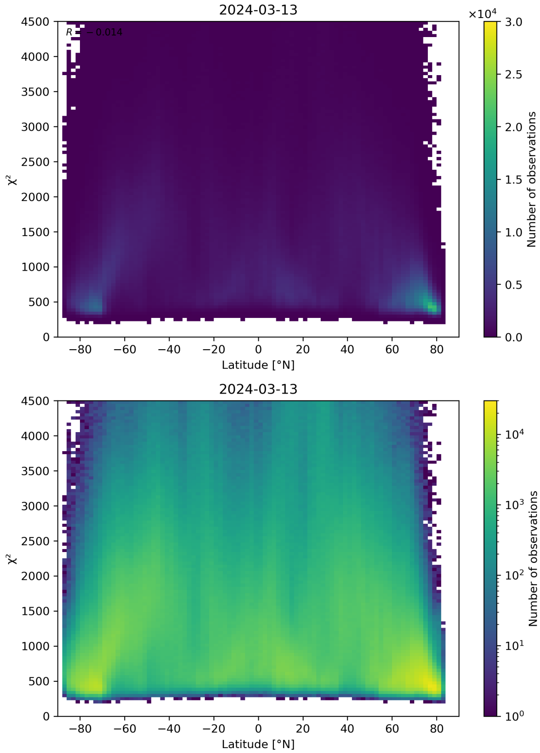
Figure 54: Scatter density plot of “Latitude” against “ \chi^2 ” for 2024-03-12 to 2024-03-14.
