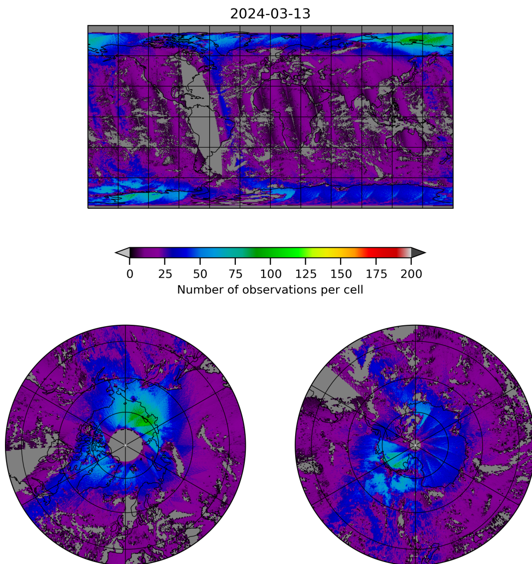
Figure 8: Map of the number of observations for 2024-03-12 to 2024-03-14
