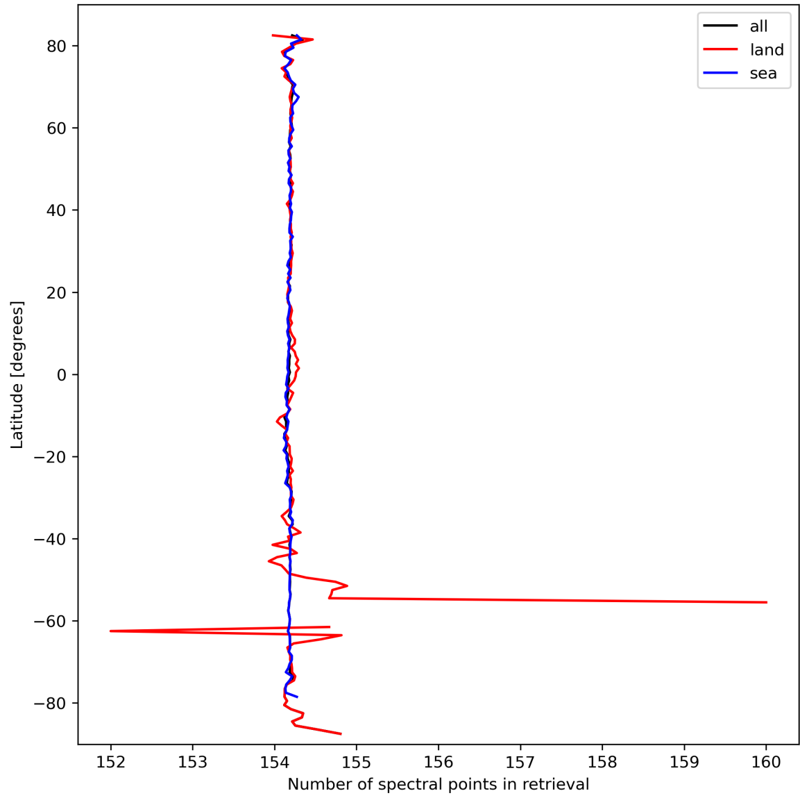
Figure 13: Zonal average of “Number of spectral points in retrieval” for 2024-03-12 to 2024-03-14.
