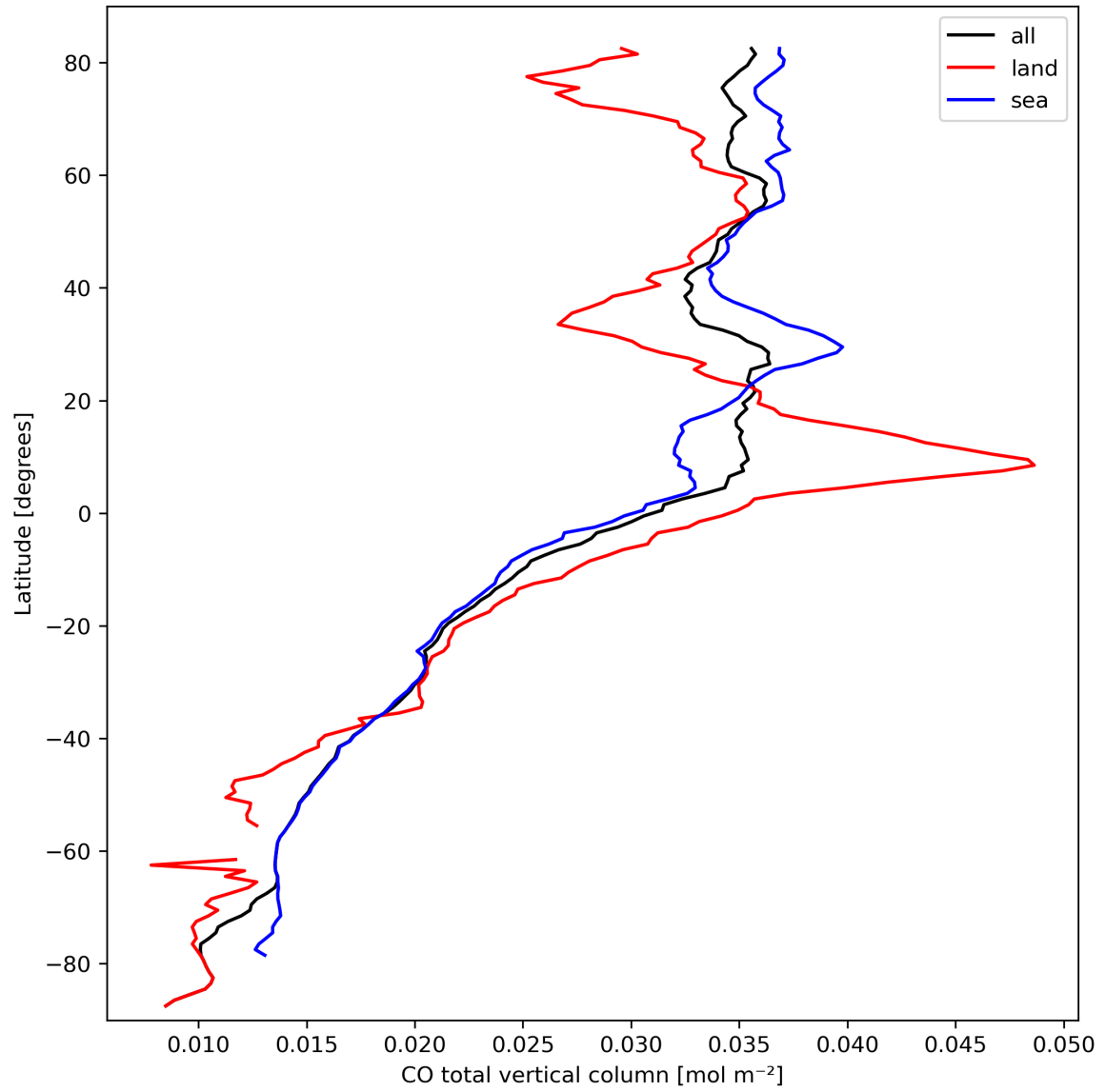
Figure 10: Zonal average of “CO total vertical column” for 2024-03-12 to 2024-03-14.
