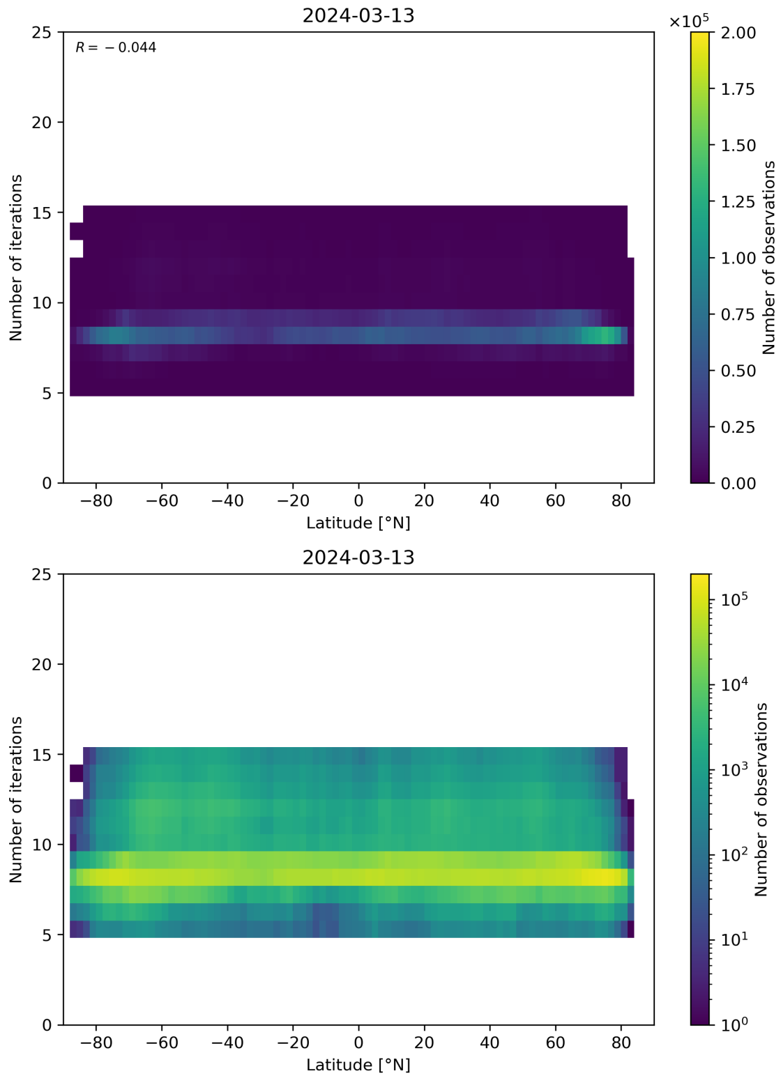
Figure 56: Scatter density plot of “Latitude” against “Number of iterations” for 2024-03-12 to 2024-03-14.
