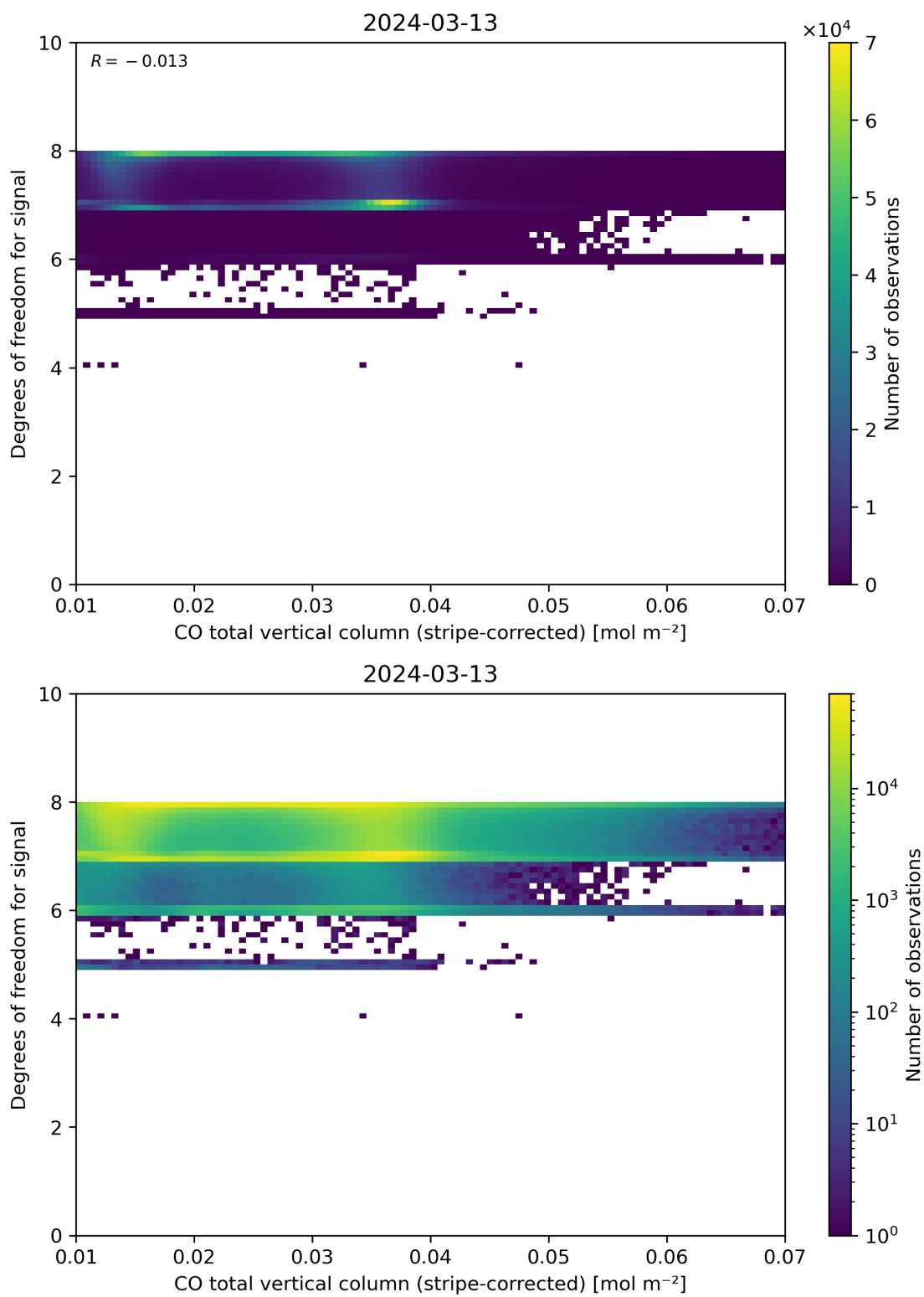
Figure 38: Scatter density plot of “CO total vertical column (stripe-corrected)” against “Degrees of freedom for signal” for 2024-03-12 to 2024-03-14.
