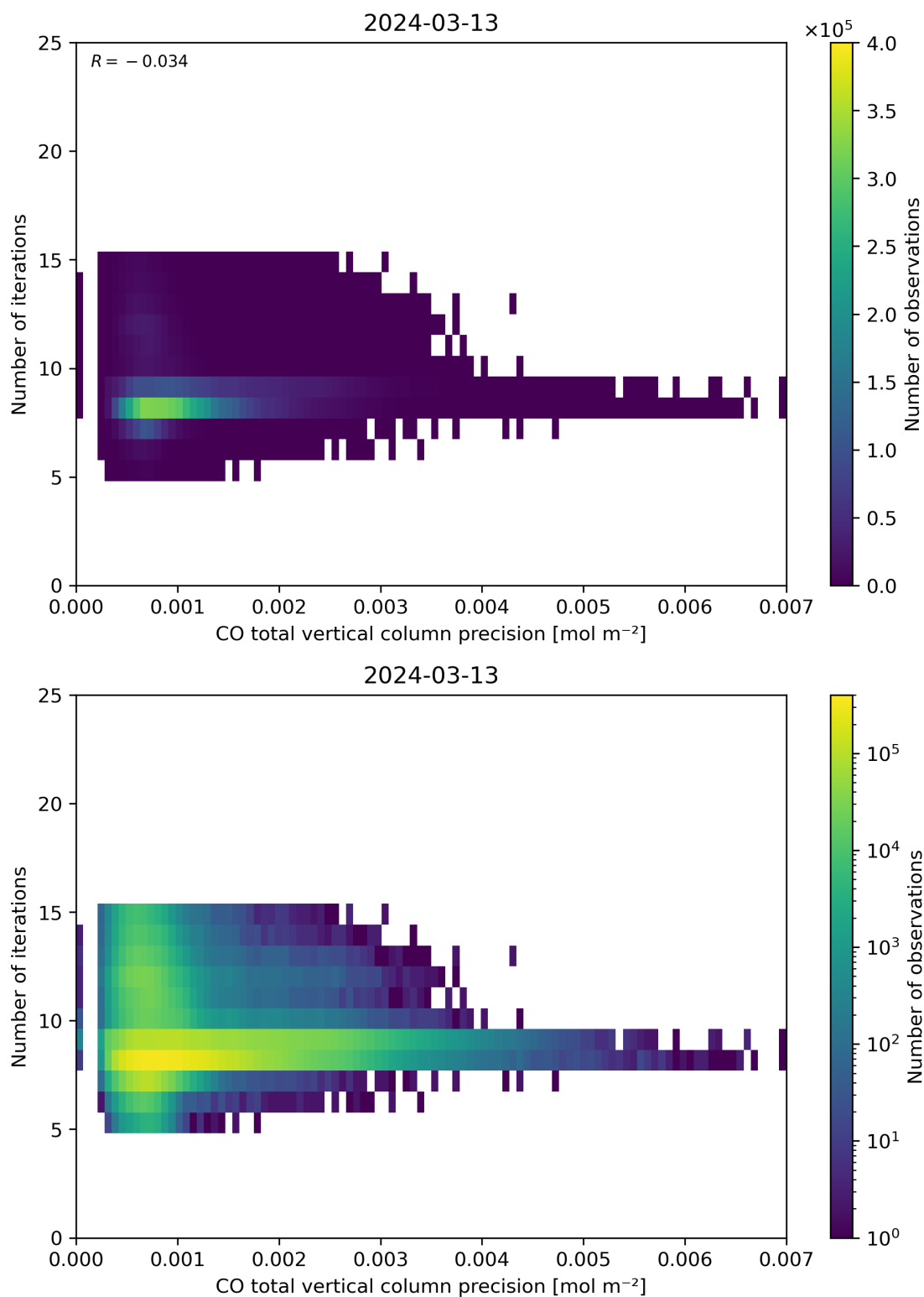
Figure 46: Scatter density plot of “CO total vertical column precision” against “Number of iterations” for 2024-03-12 to 2024-03-14.
