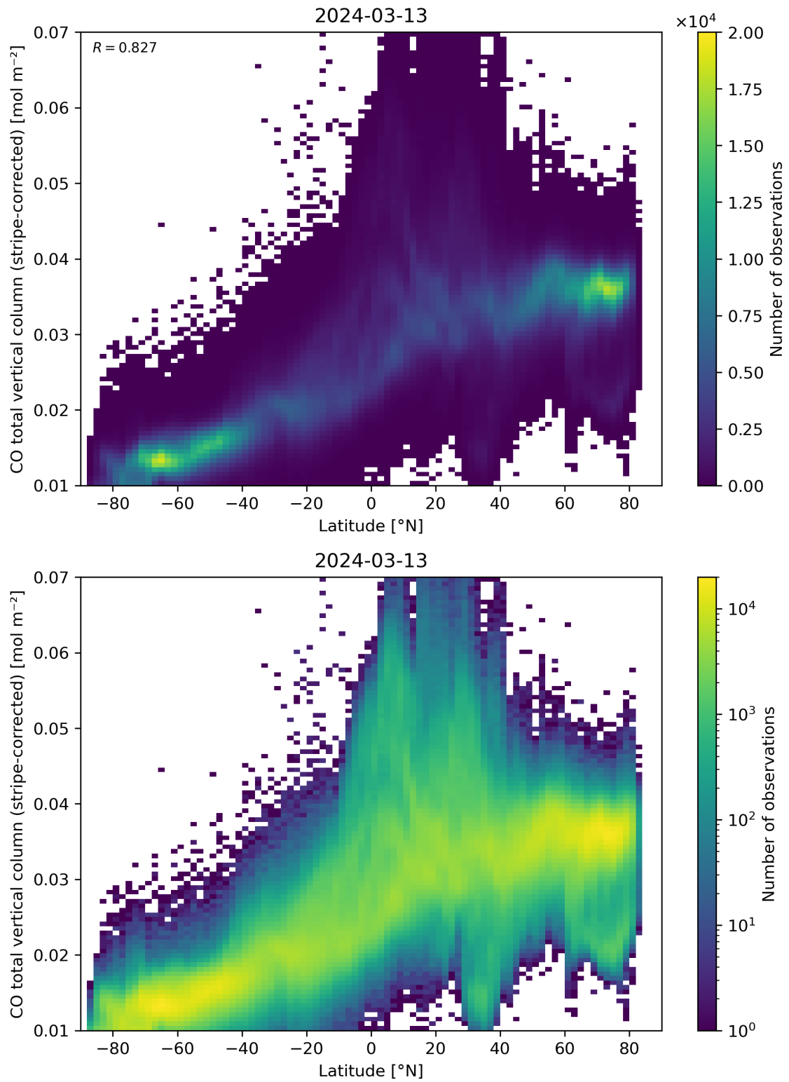
Figure 52: Scatter density plot of “Latitude” against “CO total vertical column (stripe-corrected)” for 2024-03-12 to 2024-03-14.
