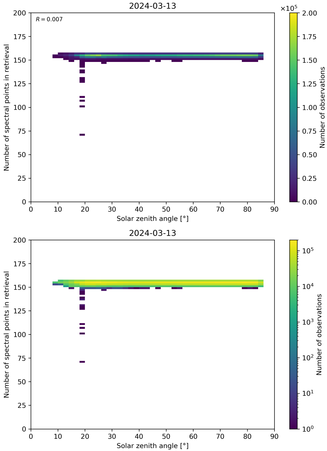
Figure 68: Scatter density plot of “Solar zenith angle” against “Number of spectral points in retrieval” for 2024-03-12 to 2024-03-14.
