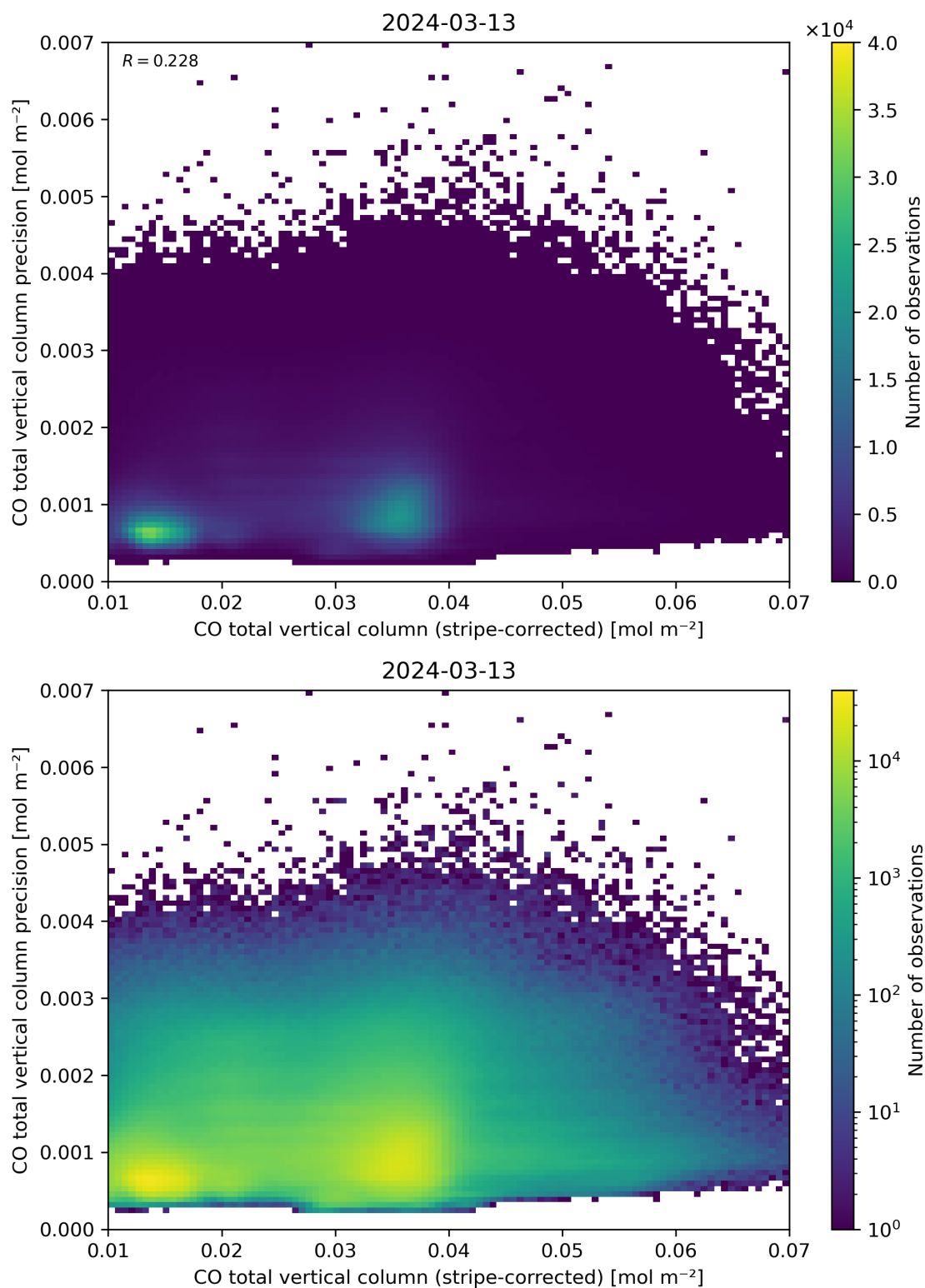
Figure 36: Scatter density plot of “CO total vertical column (stripe-corrected)” against “CO total vertical column precision” for 2024-03-12 to 2024-03-14.
