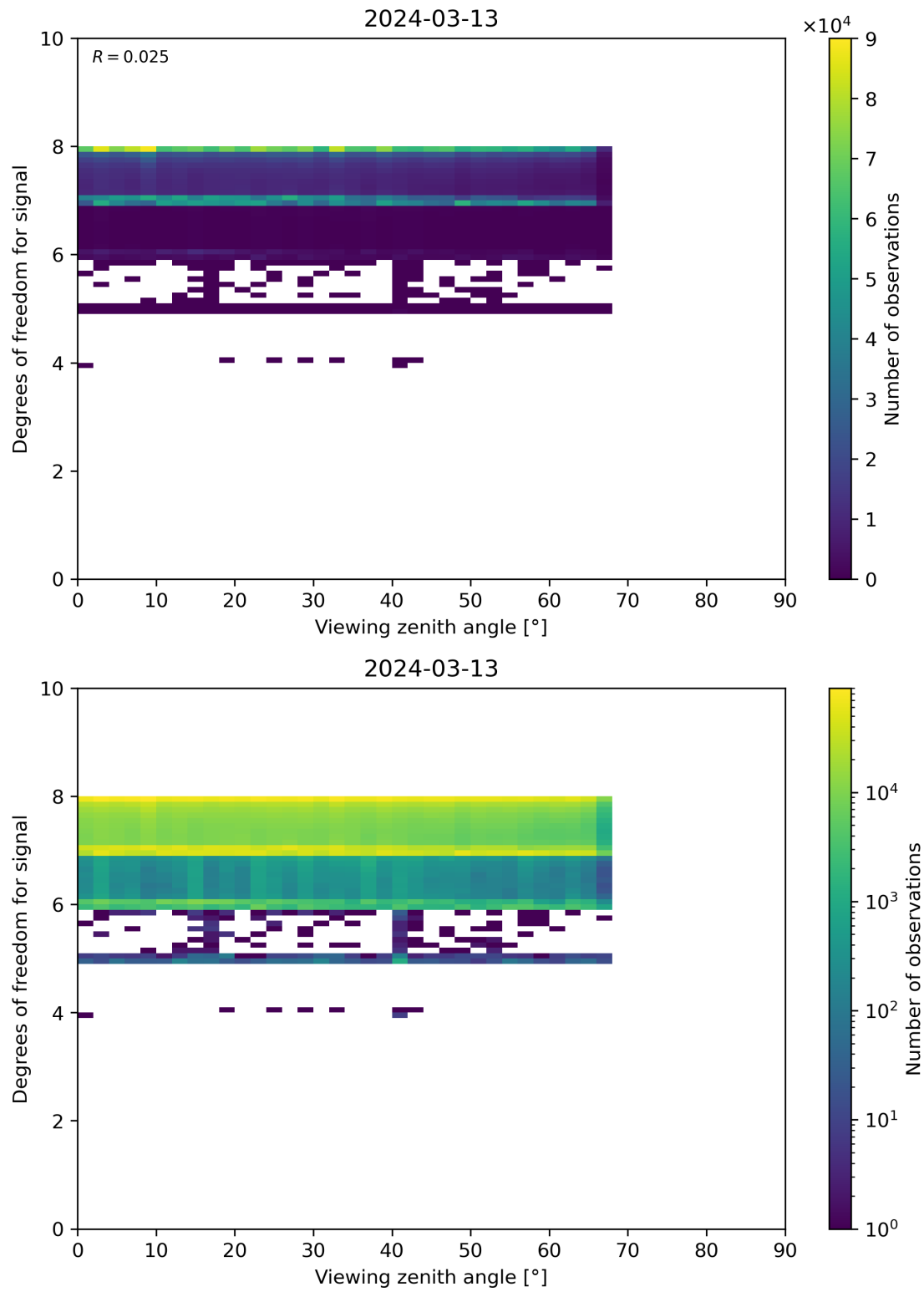
Figure 73: Scatter density plot of “Viewing zenith angle” against “Degrees of freedom for signal” for 2024-03-12 to 2024-03-14.
