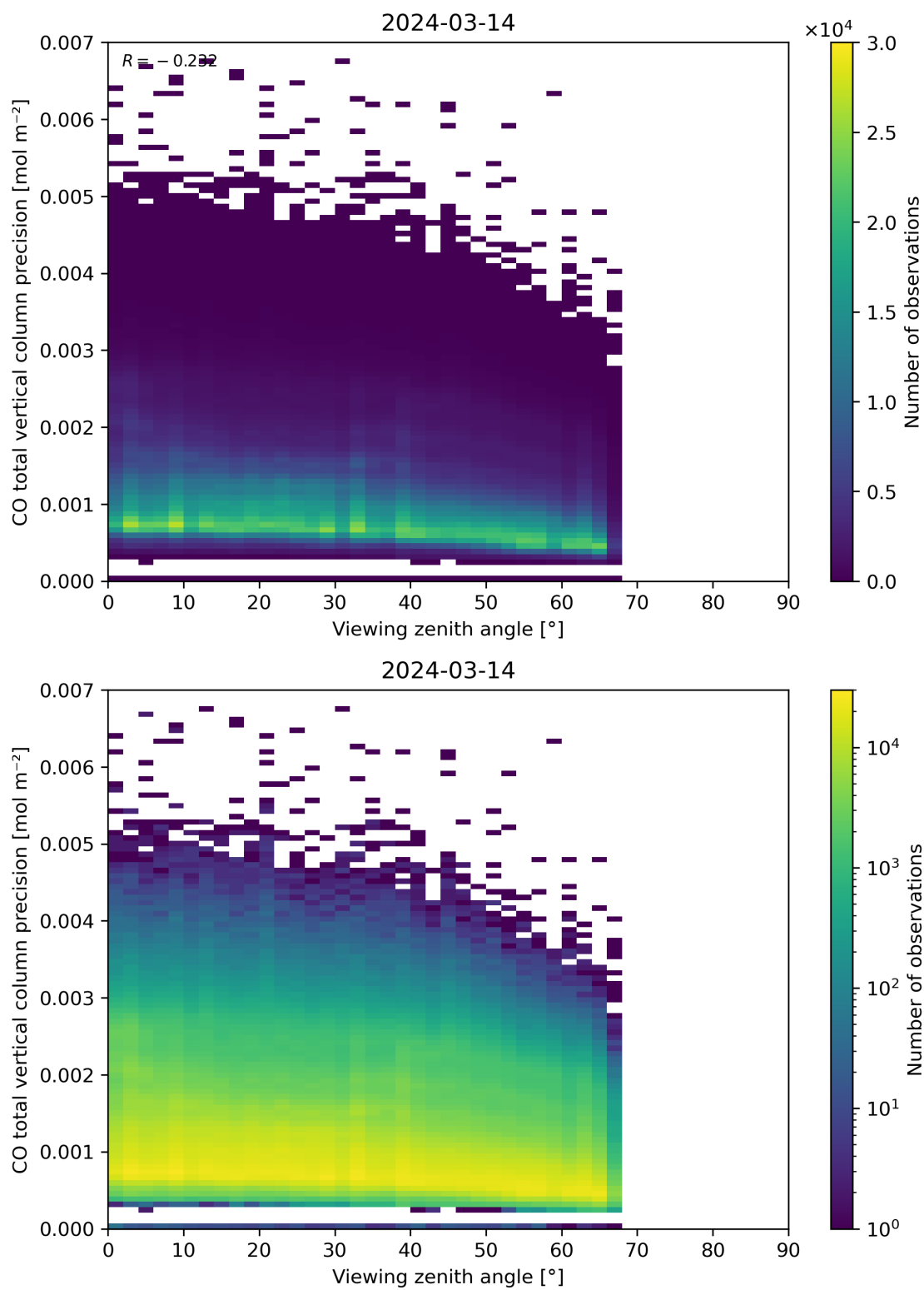
Figure 71: Scatter density plot of “Viewing zenith angle” against “CO total vertical column precision” for 2024-03-14 to 2024-03-15.
