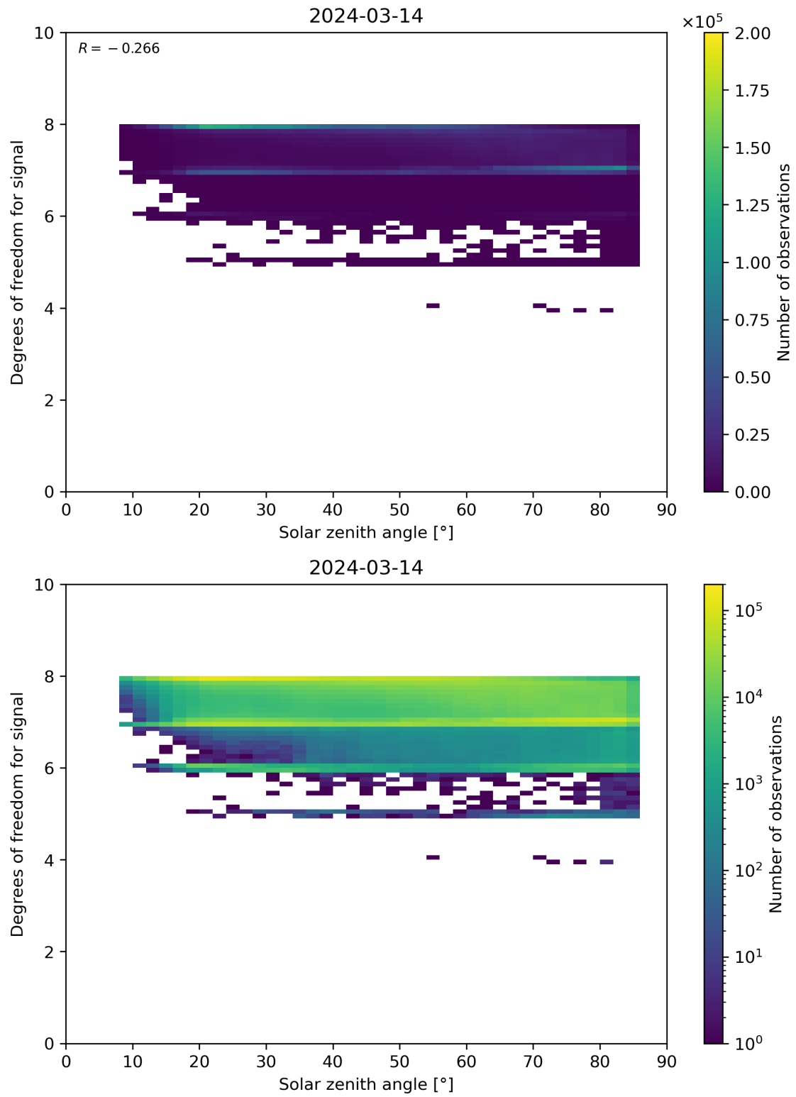
Figure 65: Scatter density plot of “Solar zenith angle” against “Degrees of freedom for signal” for 2024-03-14 to 2024-03-15.
