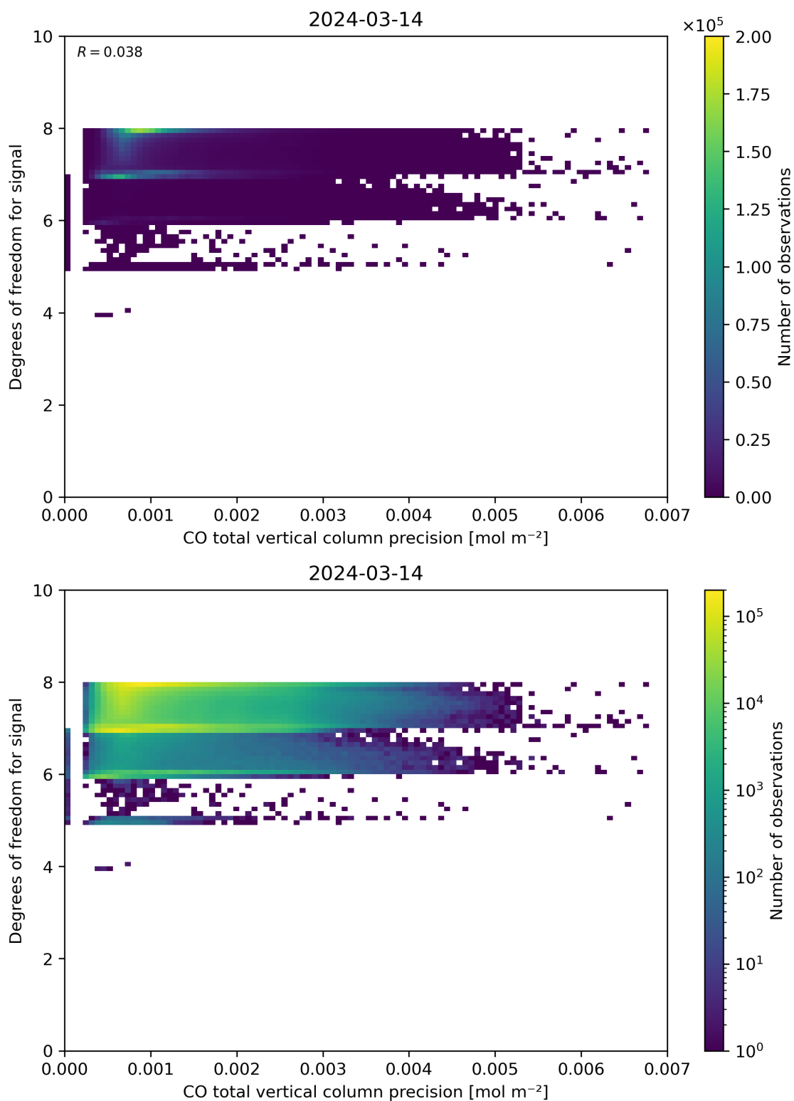
Figure 45: Scatter density plot of “CO total vertical column precision” against “Degrees of freedom for signal” for 2024-03-14 to 2024-03-15.
