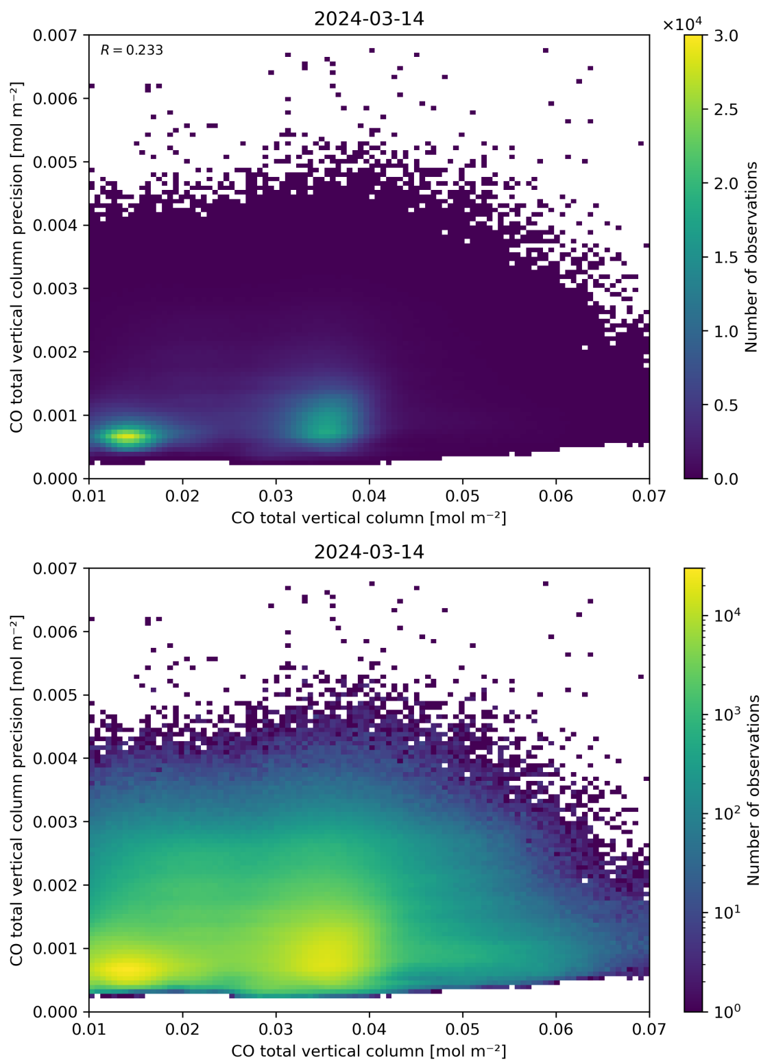
Figure 34: Scatter density plot of “CO total vertical column” against “CO total vertical column precision” for 2024-03-14 to 2024-03-15.
