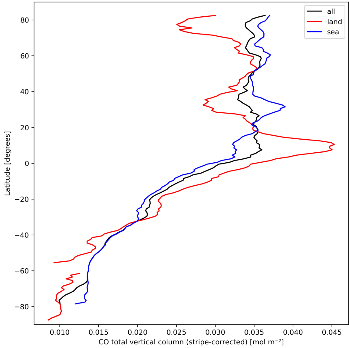
Figure 11: Zonal average of “CO total vertical column (stripe-corrected)” for 2024-03-14 to 2024-03-15.
