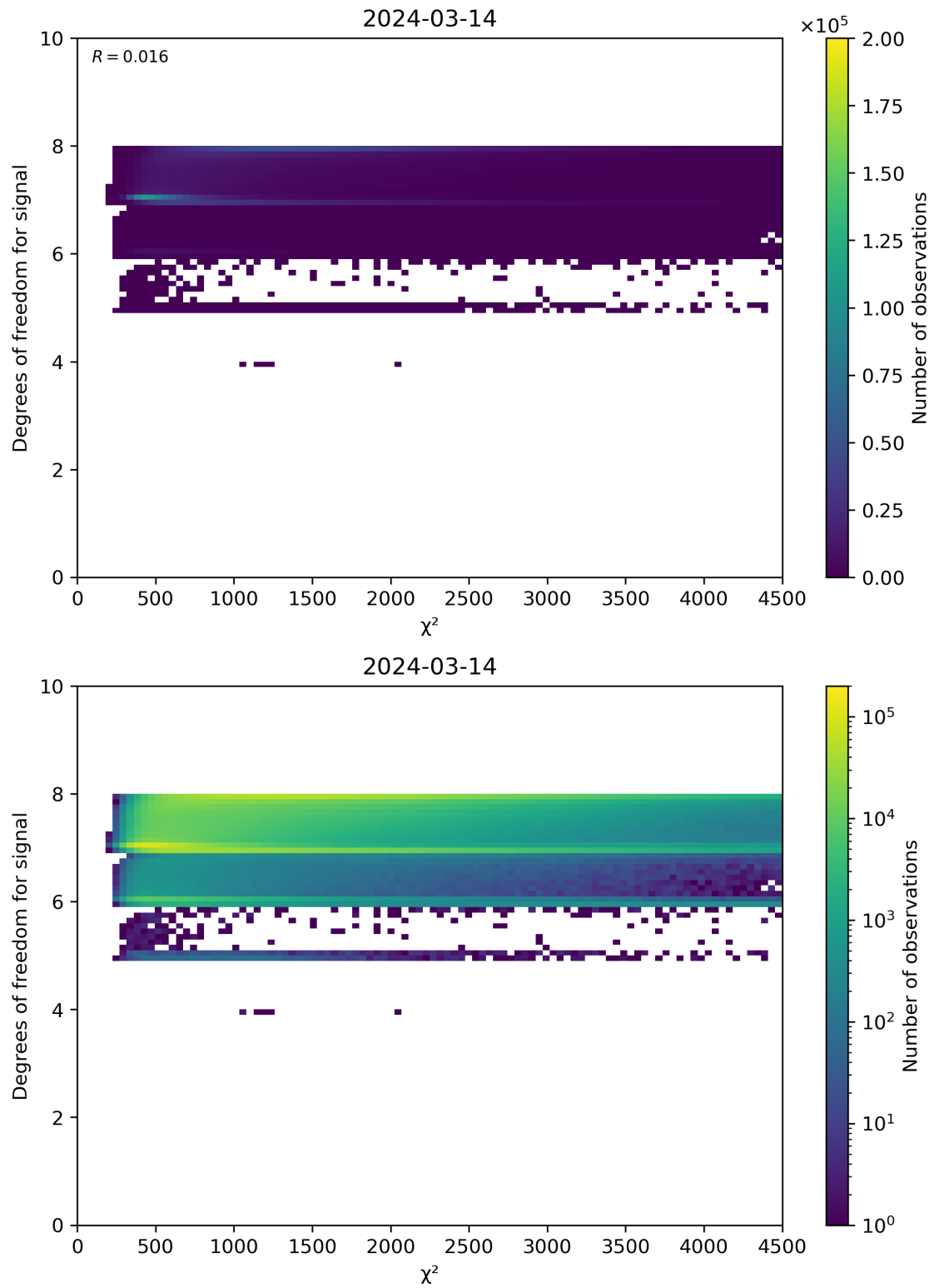
Figure 48: Scatter density plot of " \chi^2 " against "Degrees of freedom for signal" for 2024-03-14 to 2024-03-15.
