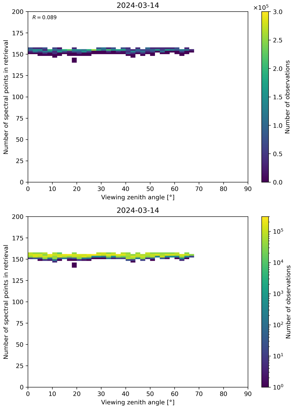
Figure 76: Scatter density plot of “Viewing zenith angle” against “Number of spectral points in retrieval” for 2024-03-14 to 2024-03-15.
