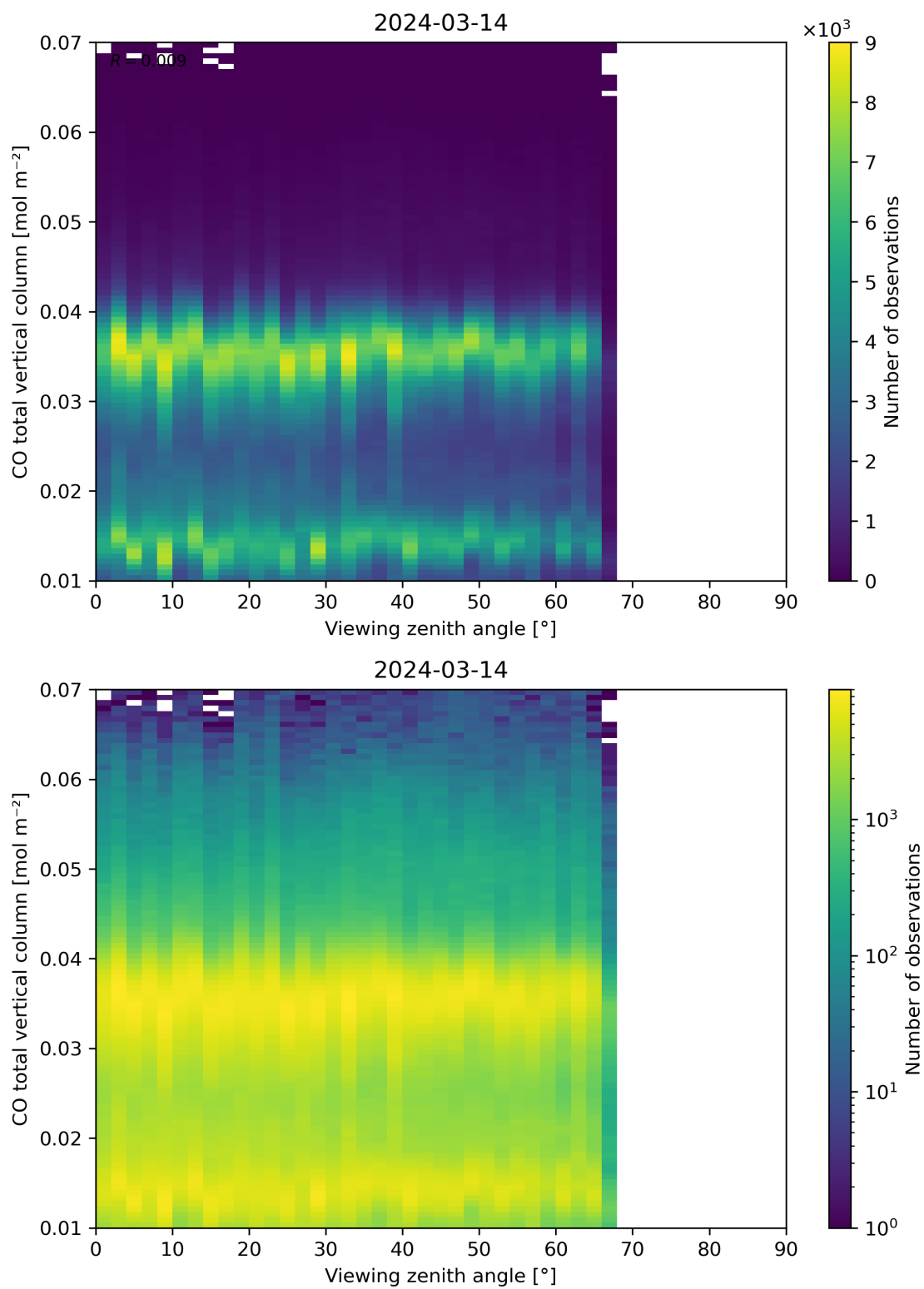
Figure 69: Scatter density plot of “Viewing zenith angle” against “CO total vertical column” for 2024-03-14 to 2024-03-15.
