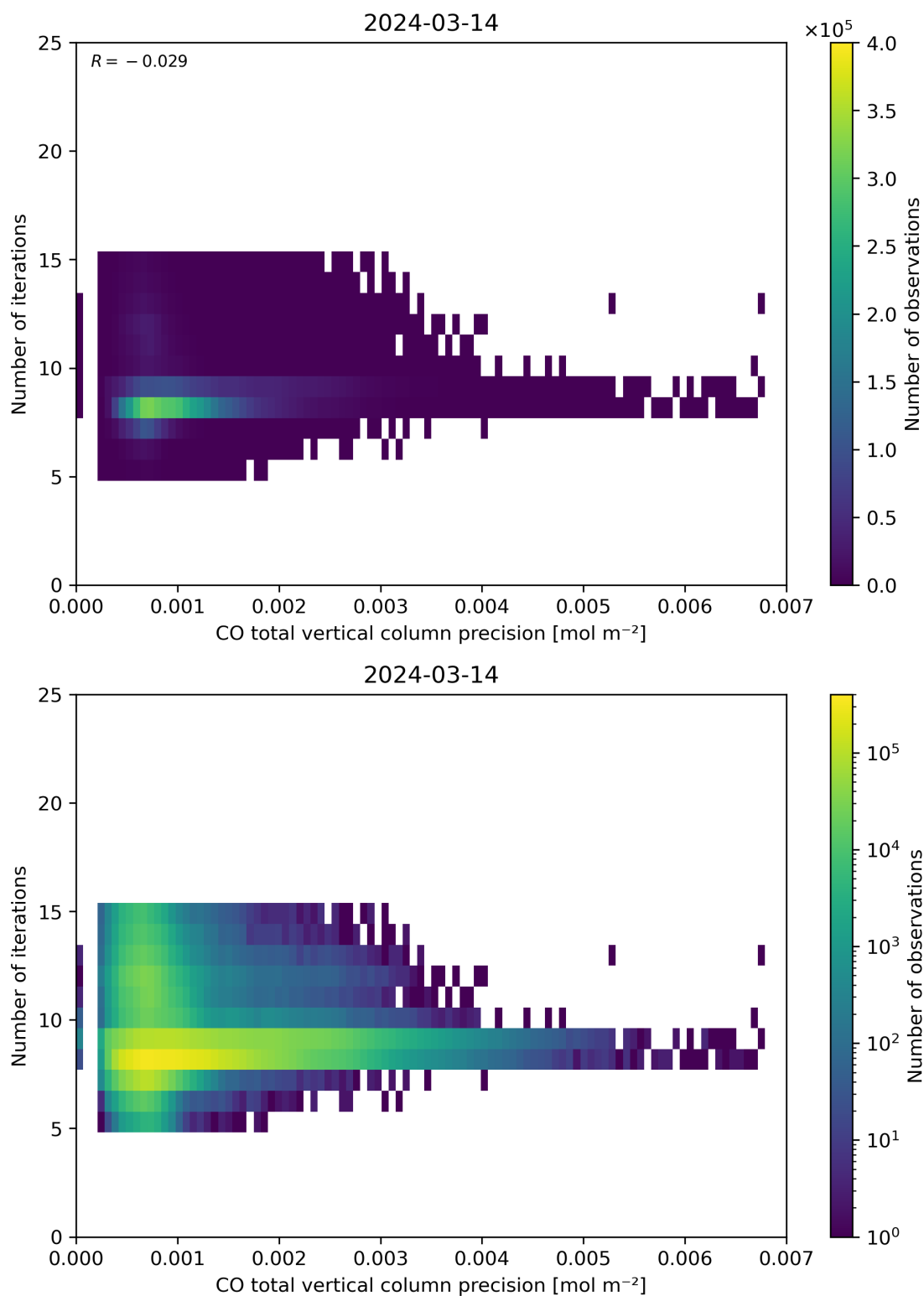
Figure 46: Scatter density plot of “CO total vertical column precision” against “Number of iterations” for 2024-03-14 to 2024-03-15.
