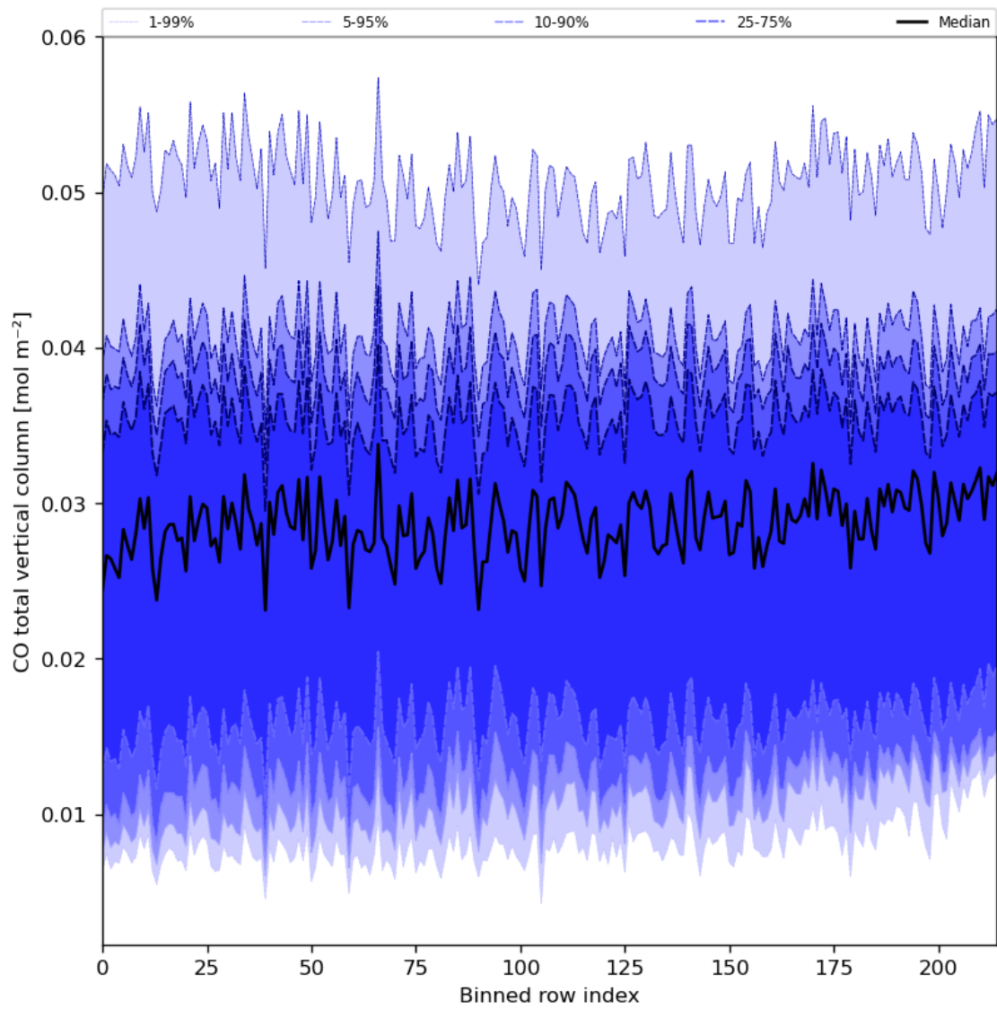
Figure 26: Along track statistics of “CO total vertical column” for 2024-03-14 to 2024-03-15
