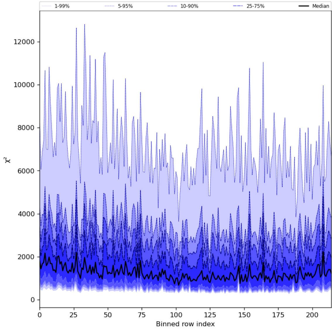
Figure 30: Along track statistics of “ \chi^2 ” for 2024-03-14 to 2024-03-15
