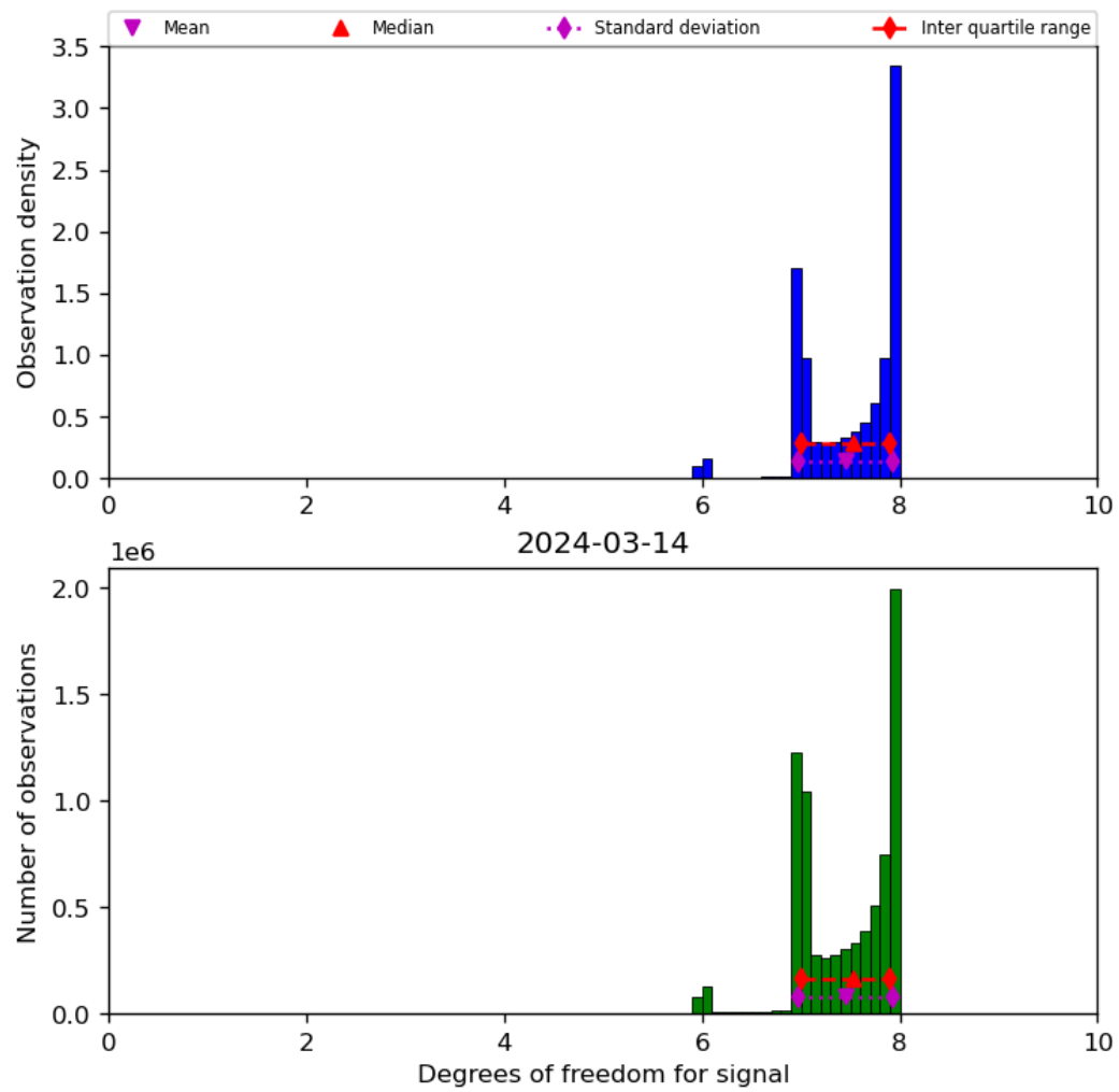
Figure 23: Histogram of “Degrees of freedom for signal” for 2024-03-14 to 2024-03-15
