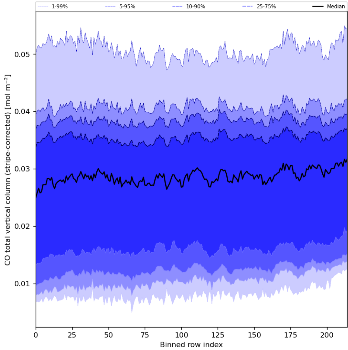
Figure 27: Along track statistics of “CO total vertical column (stripe-corrected)” for 2024-03-14 to 2024-03-15
