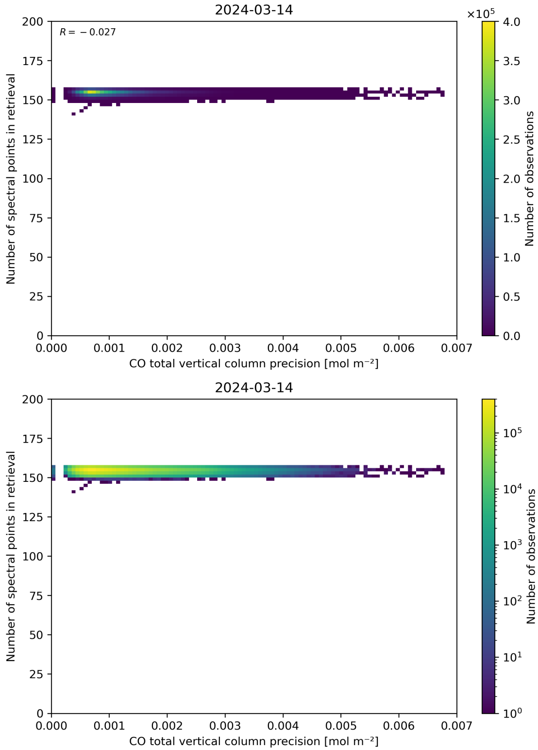
Figure 47: Scatter density plot of “CO total vertical column precision” against “Number of spectral points in retrieval” for 2024-03-14 to 2024-03-15.
