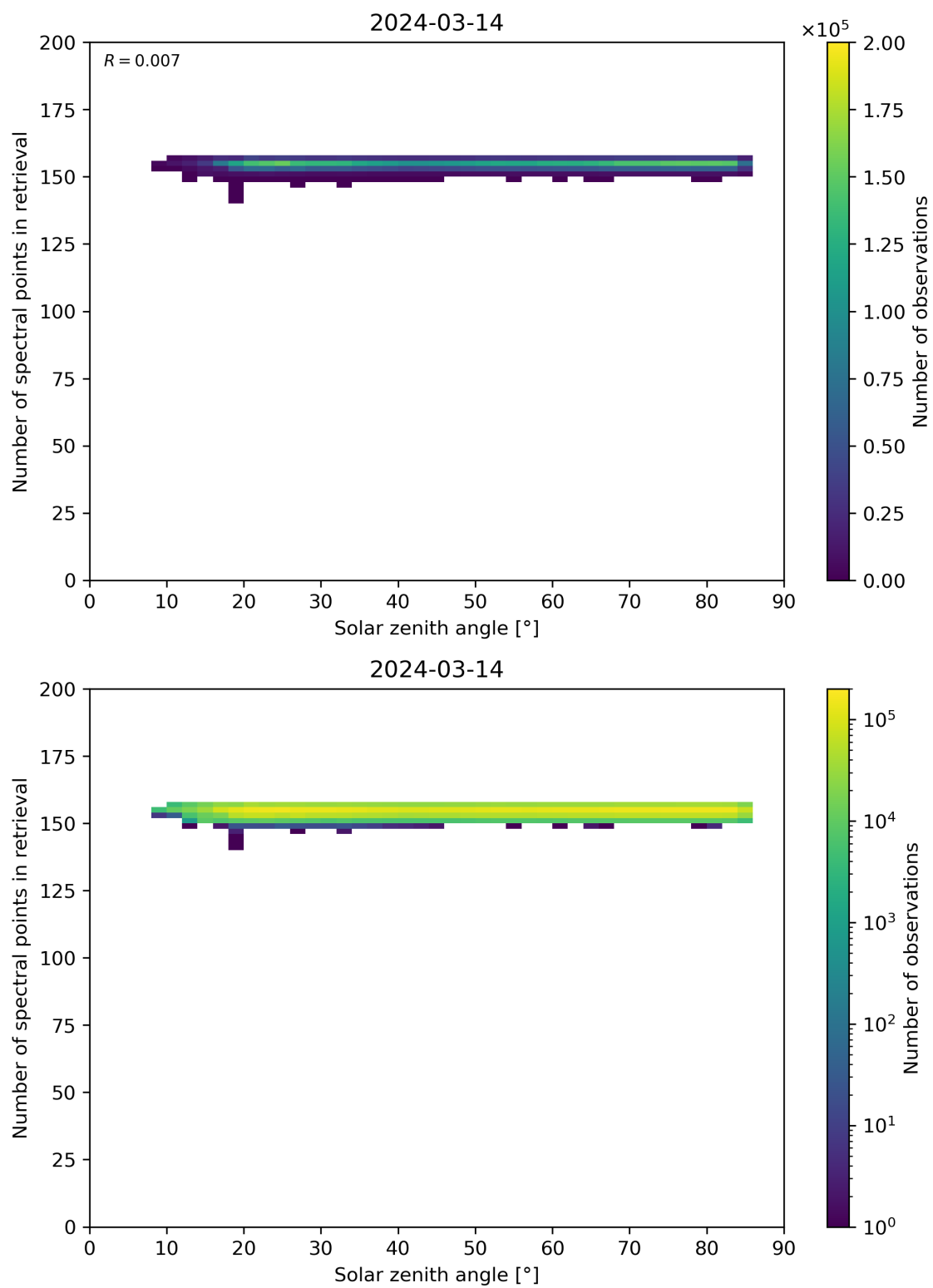
Figure 68: Scatter density plot of “Solar zenith angle” against “Number of spectral points in retrieval” for 2024-03-14 to 2024-03-15.
