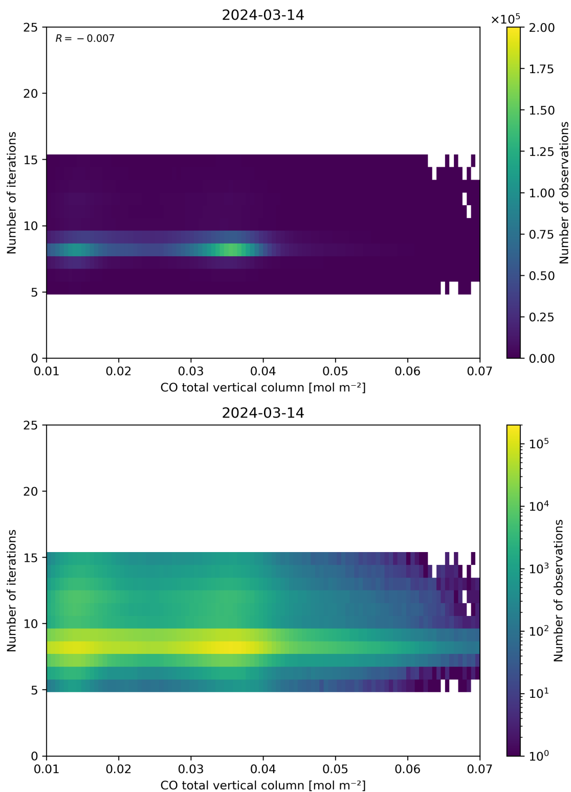
Figure 42: Scatter density plot of “CO total vertical column” against “Number of iterations” for 2024-03-14 to 2024-03-15.
