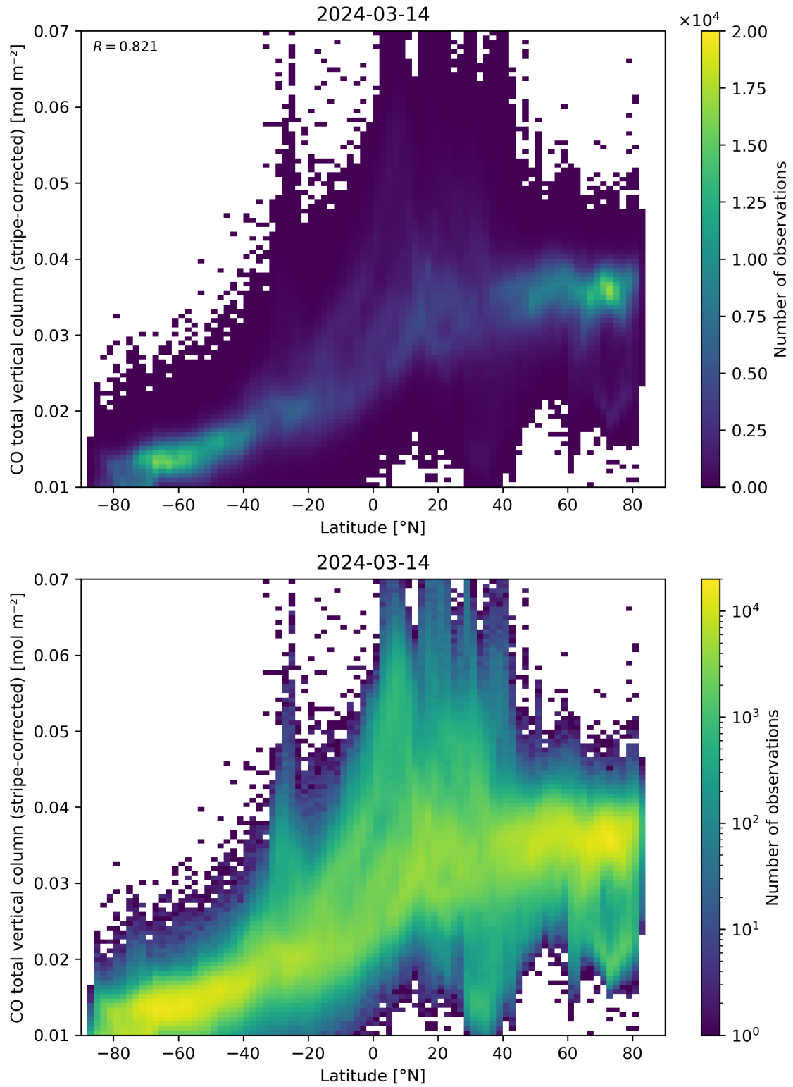
Figure 52: Scatter density plot of “Latitude” against “CO total vertical column (stripe-corrected)” for 2024-03-14 to 2024-03-15.
