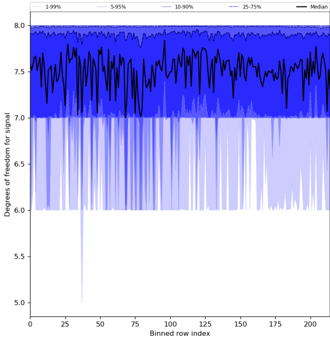
Figure 31: Along track statistics of “Degrees of freedom for signal” for 2024-03-14 to 2024-03-15
