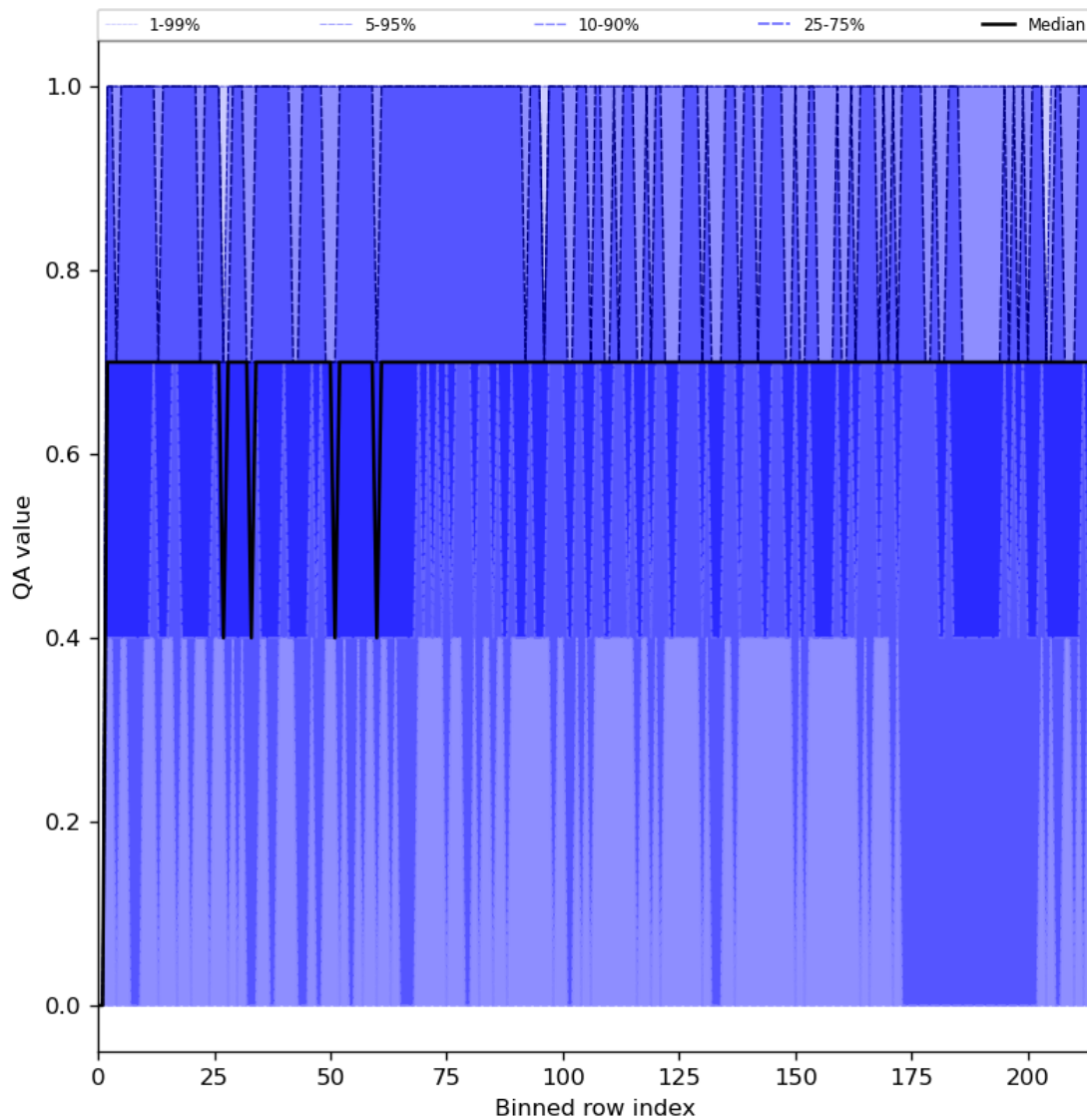
Figure 25: Along track statistics of “QA value” for 2024-03-14 to 2024-03-15
