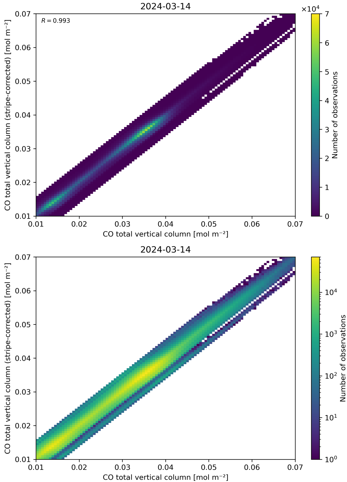
Figure 33: Scatter density plot of “CO total vertical column” against “CO total vertical column (stripe-corrected)” for 2024-03-14 to 2024-03-15.
