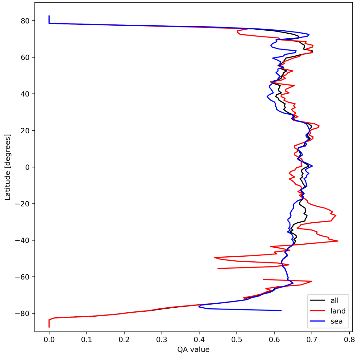
Figure 9: Zonal average of “QA value” for 2024-03-14 to 2024-03-15.
