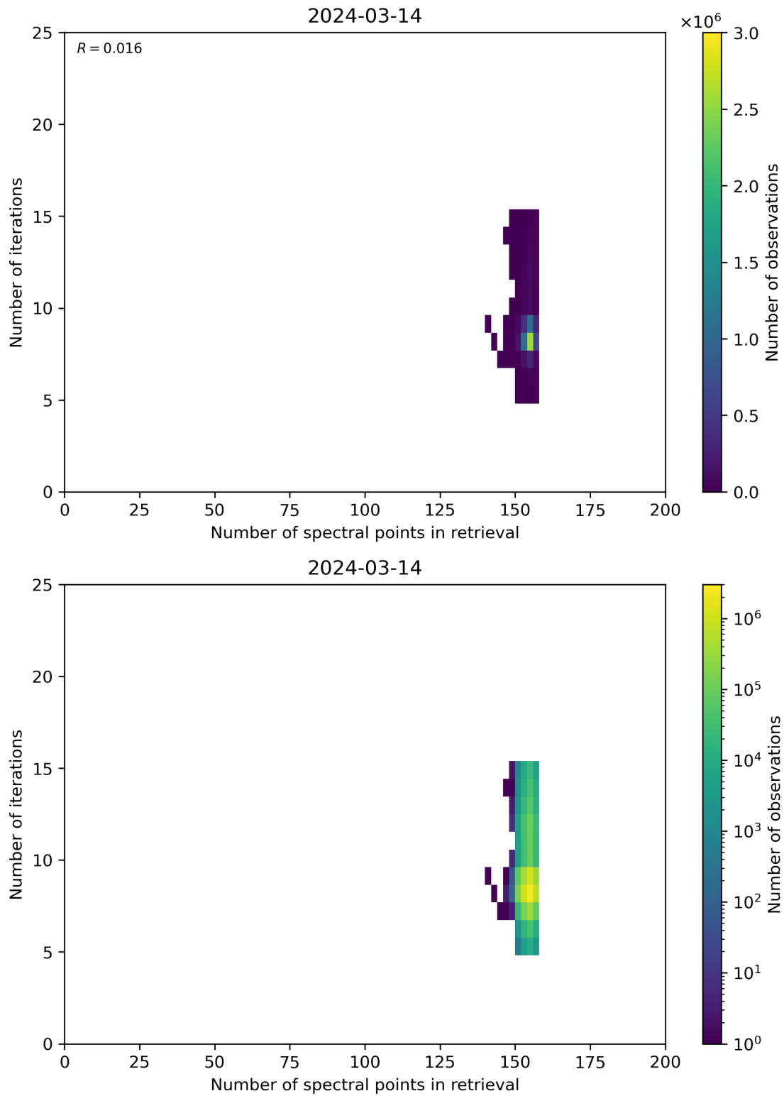
Figure 60: Scatter density plot of “Number of spectral points in retrieval” against “Number of iterations” for 2024-03-14 to 2024-03-15.
