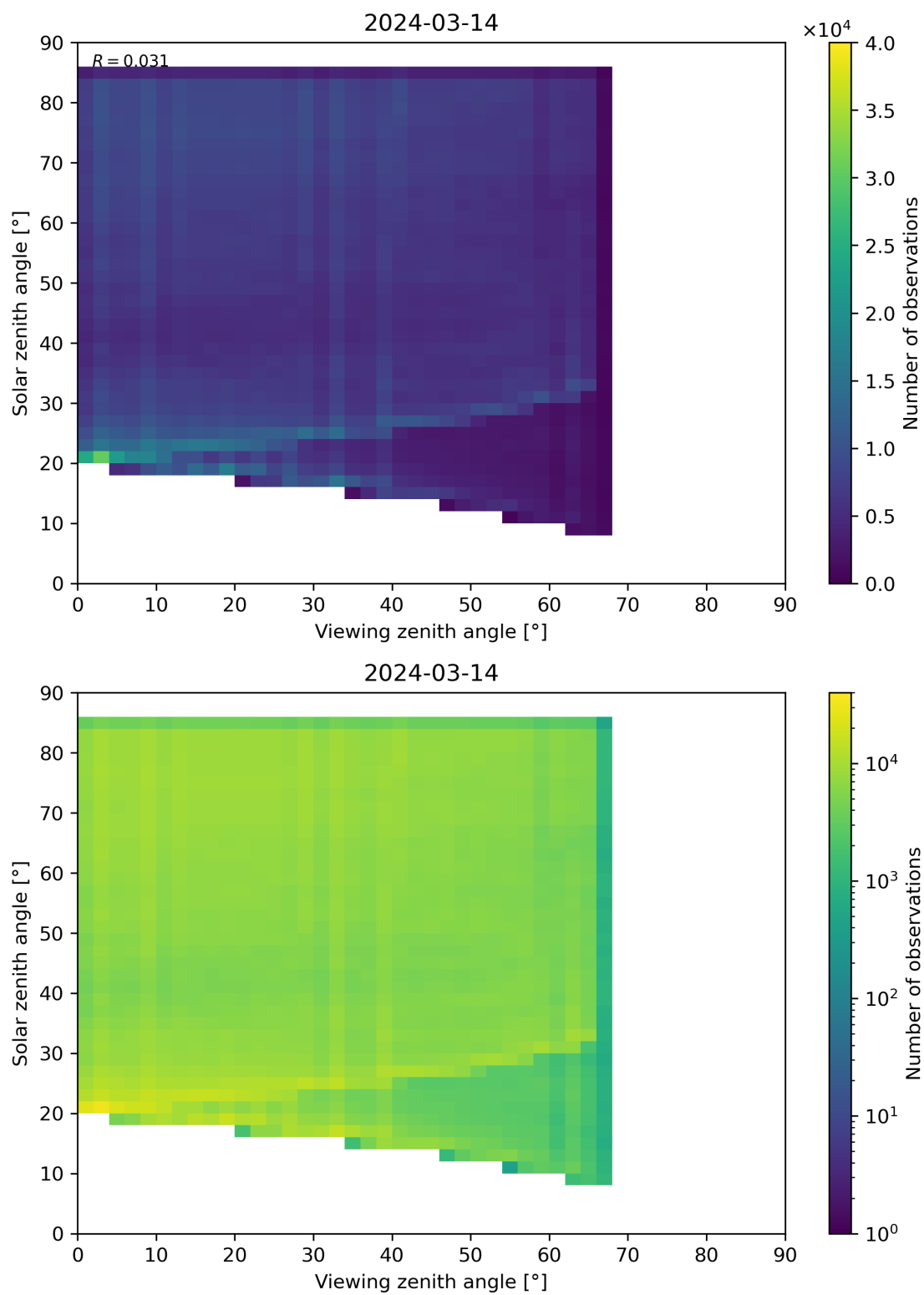
Figure 77: Scatter density plot of “Viewing zenith angle” against “Solar zenith angle” for 2024-03-14 to 2024-03-15.
