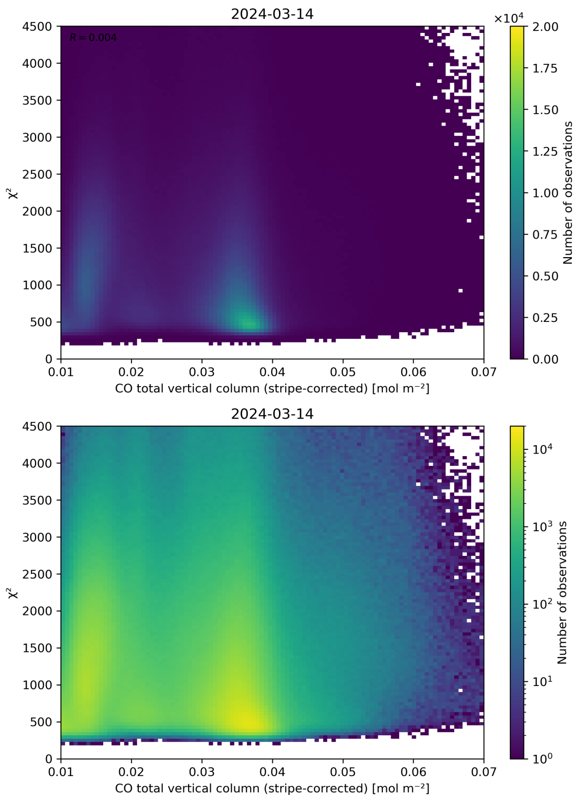
Figure 37: Scatter density plot of “CO total vertical column (stripe-corrected)” against “ \chi^2 ” for 2024-03-14 to 2024-03-15.
