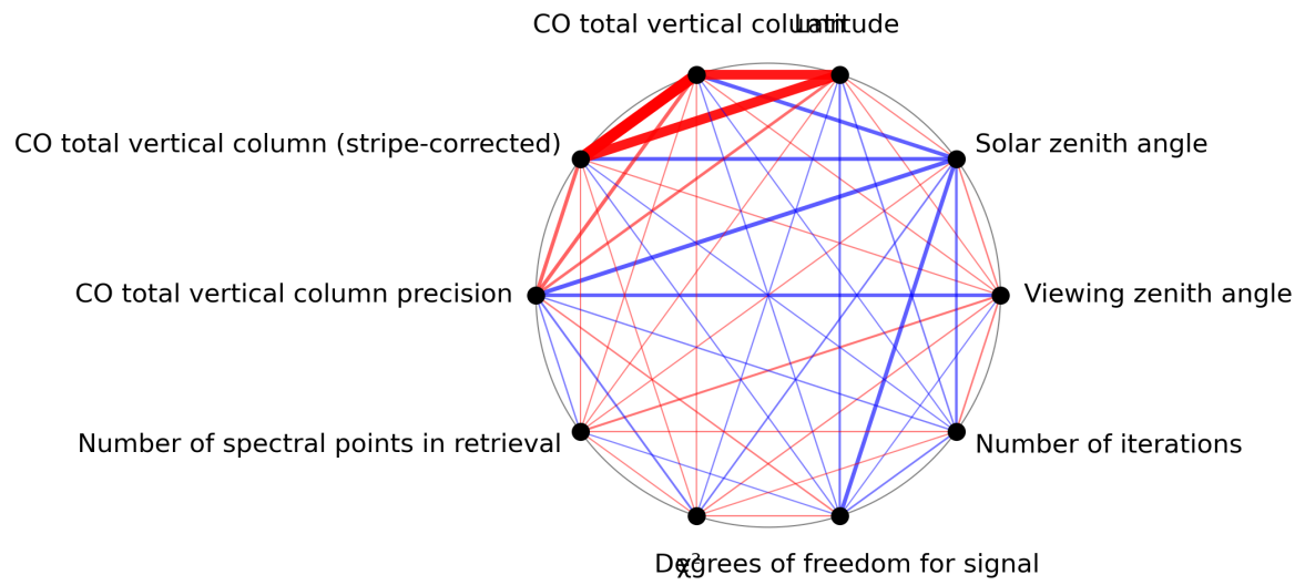
Figure 1: Map of correlation graph for 2024-03-14 to 2024-03-15.
