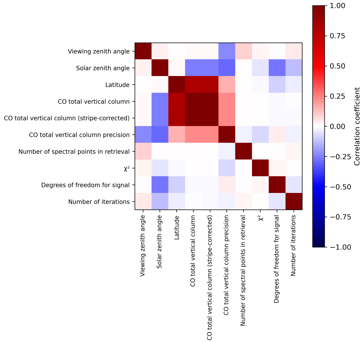
Figure 2: Map of correlation matrix for 2024-03-14 to 2024-03-15.
