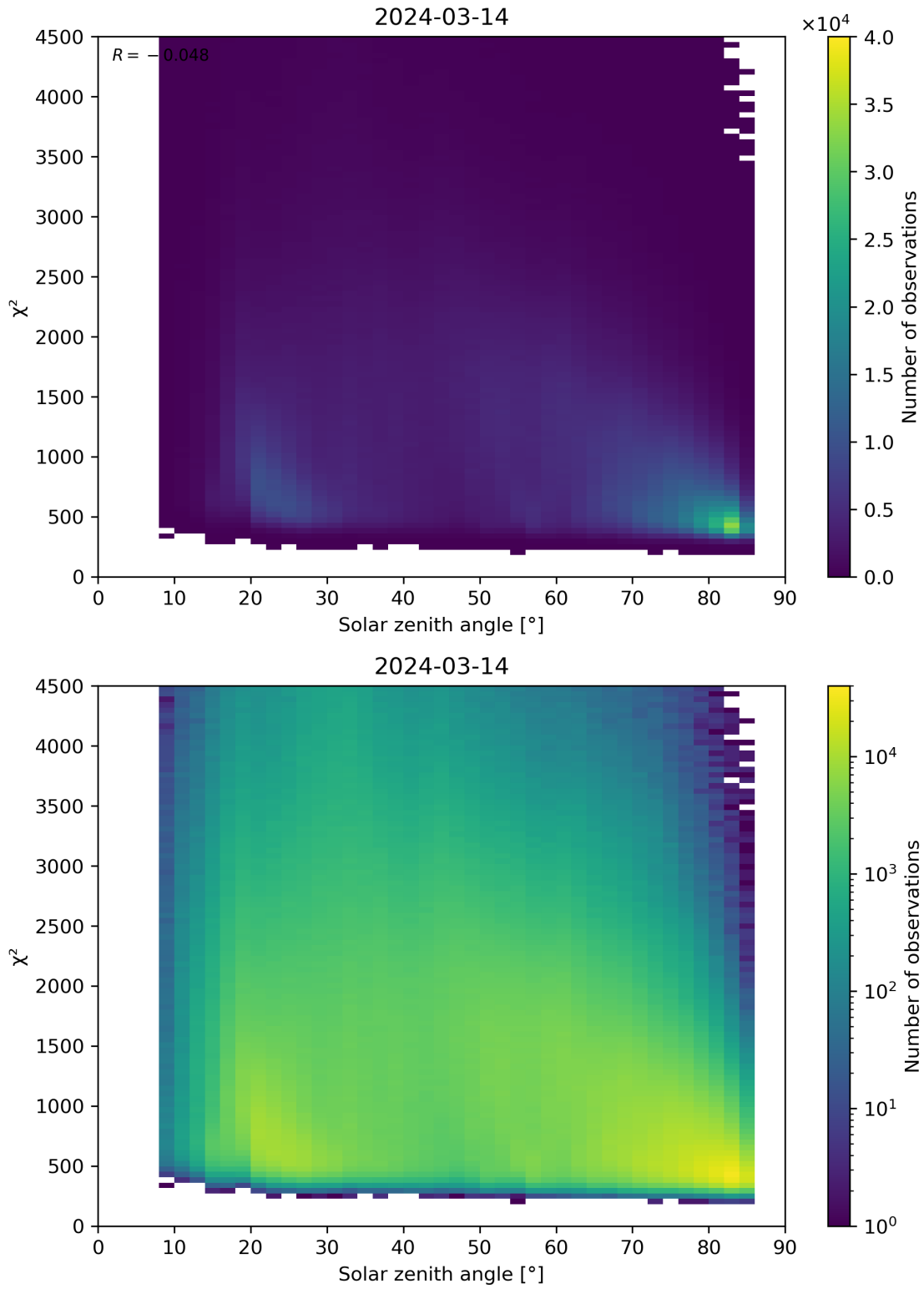
Figure 64: Scatter density plot of “Solar zenith angle” against “ \chi^2 ” for 2024-03-14 to 2024-03-15.
