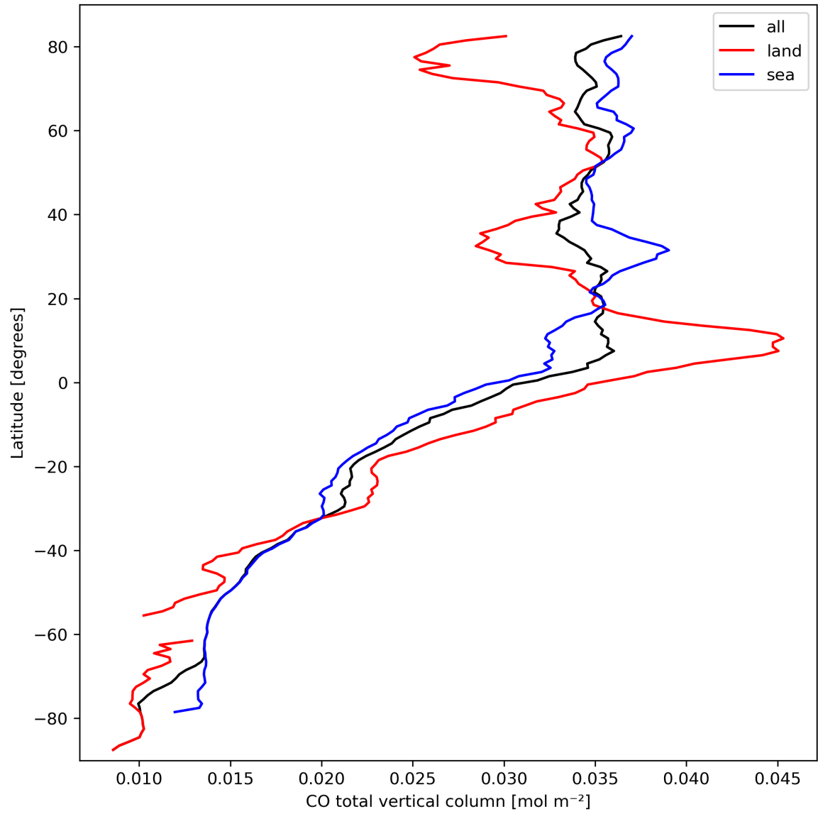
Figure 10: Zonal average of “CO total vertical column” for 2024-03-14 to 2024-03-15.
