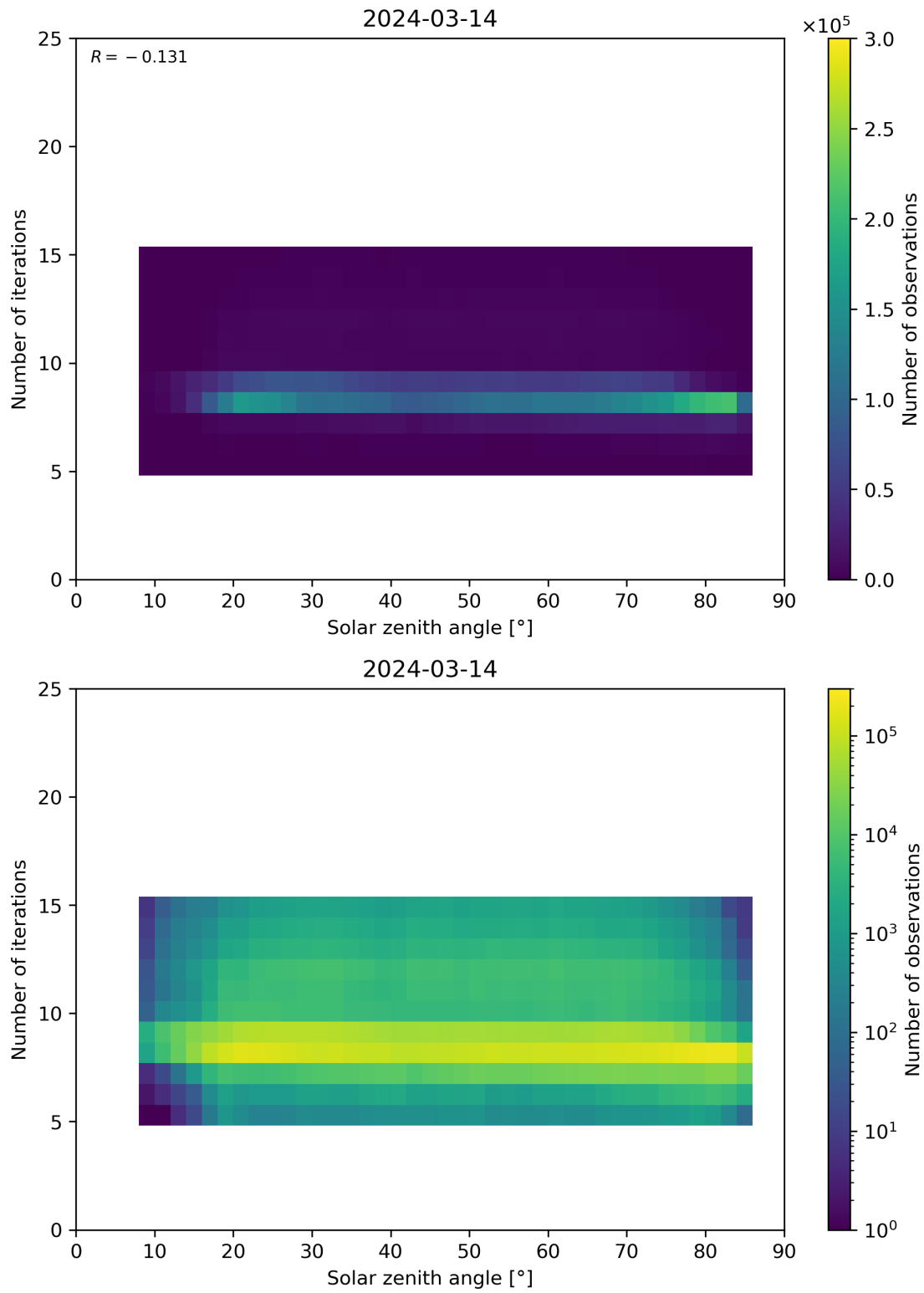
Figure 67: Scatter density plot of “Solar zenith angle” against “Number of iterations” for 2024-03-14 to 2024-03-15.
