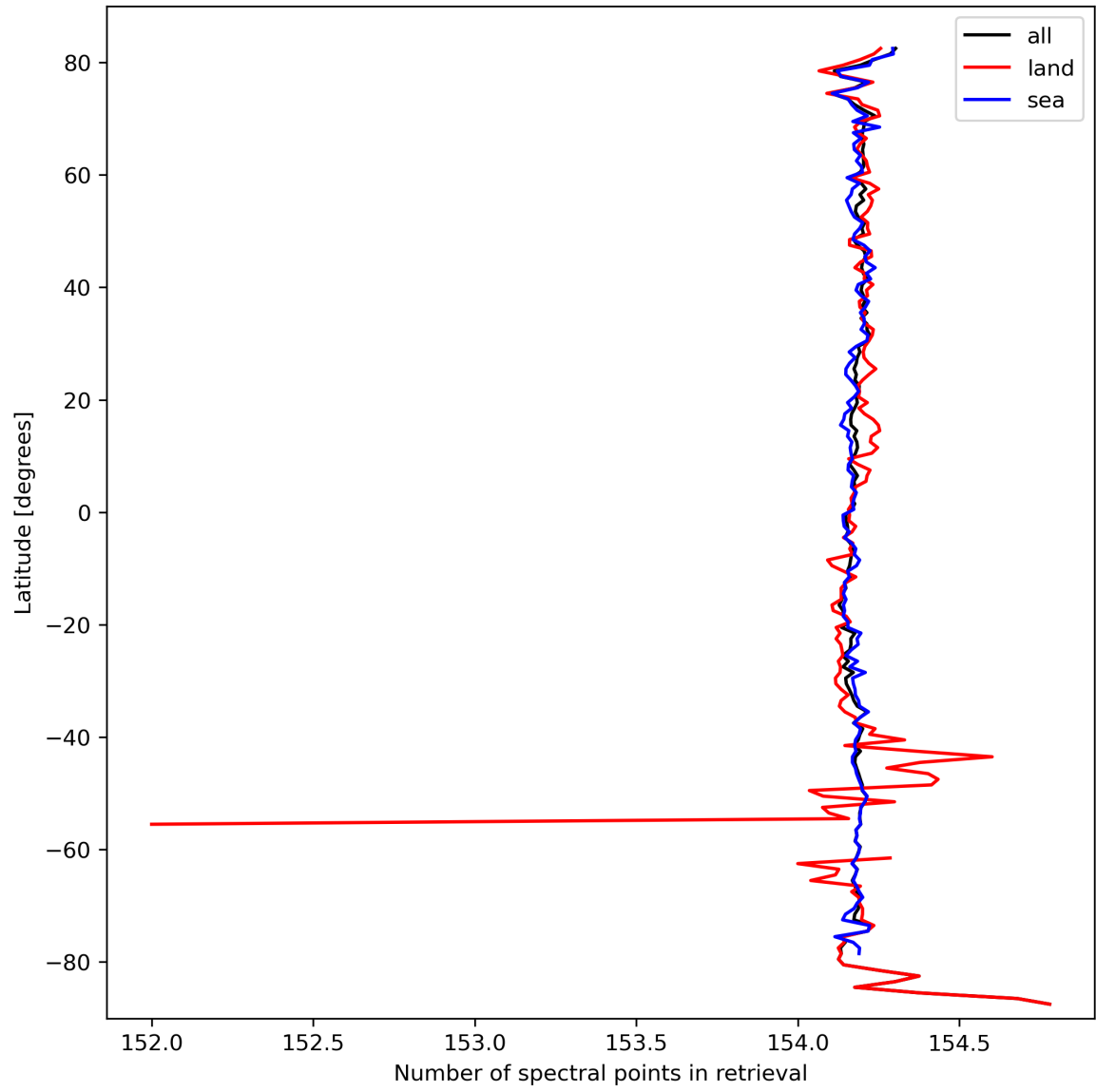
Figure 13: Zonal average of “Number of spectral points in retrieval” for 2024-03-14 to 2024-03-15.
