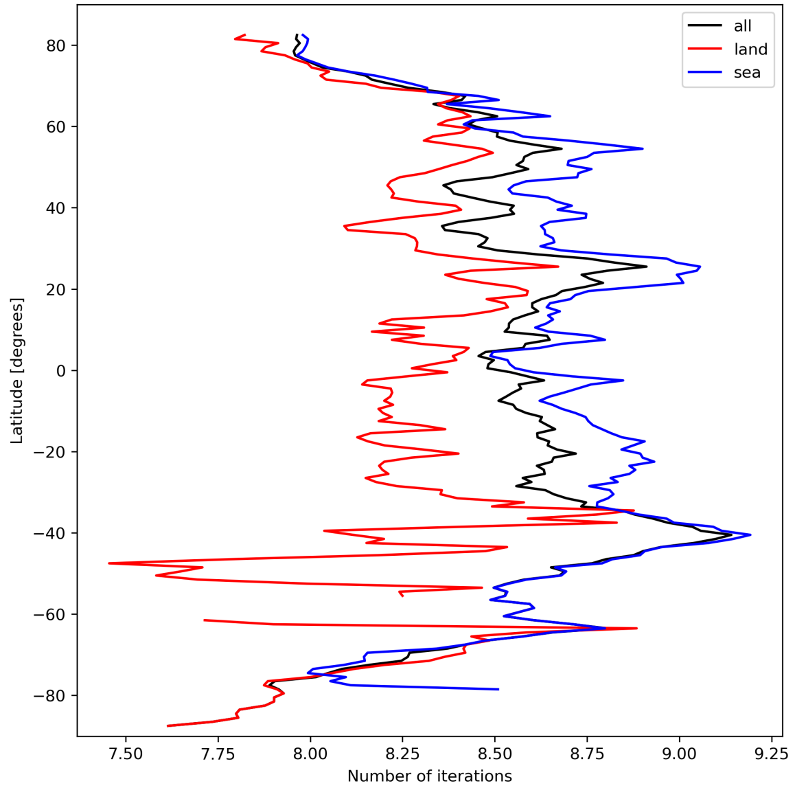
Figure 16: Zonal average of “Number of iterations” for 2024-03-14 to 2024-03-15.
