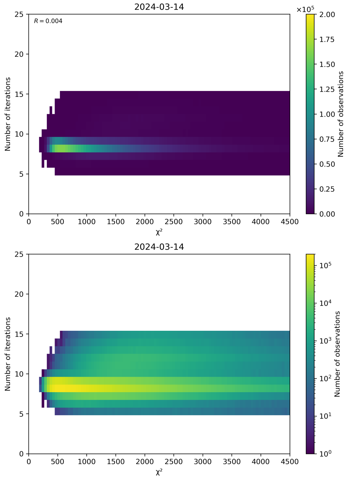
Figure 49: Scatter density plot of “ \chi^2 ” against “Number of iterations” for 2024-03-14 to 2024-03-15.
