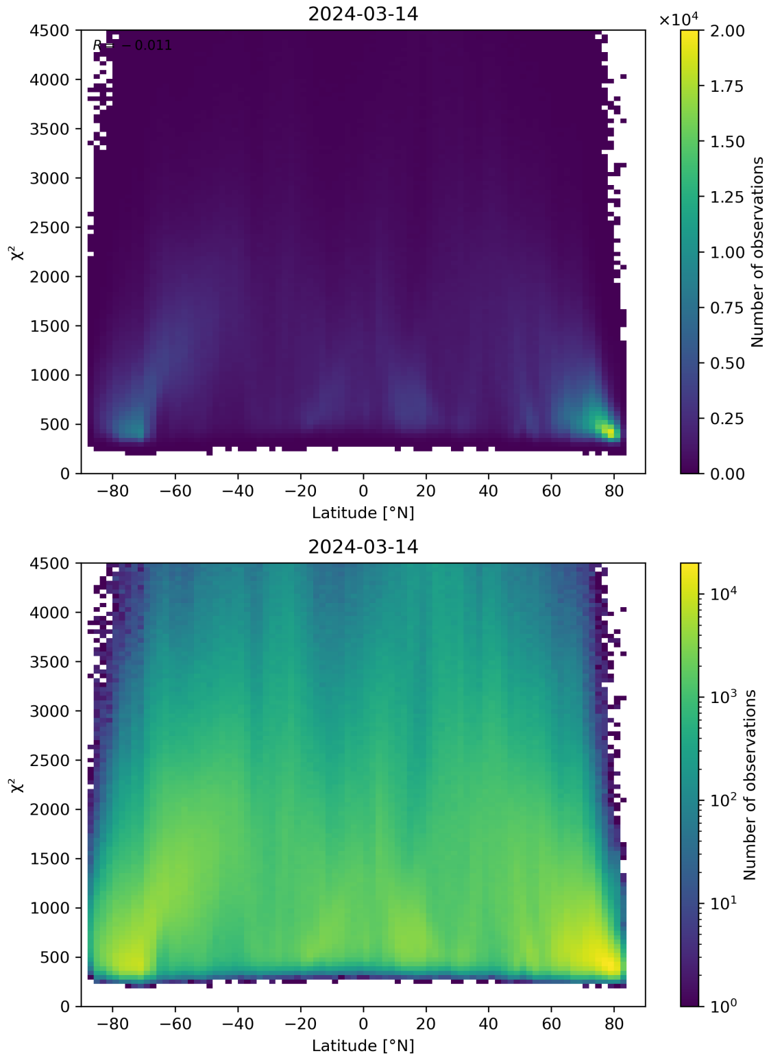
Figure 54: Scatter density plot of “Latitude” against “ \chi^2 ” for 2024-03-14 to 2024-03-15.
