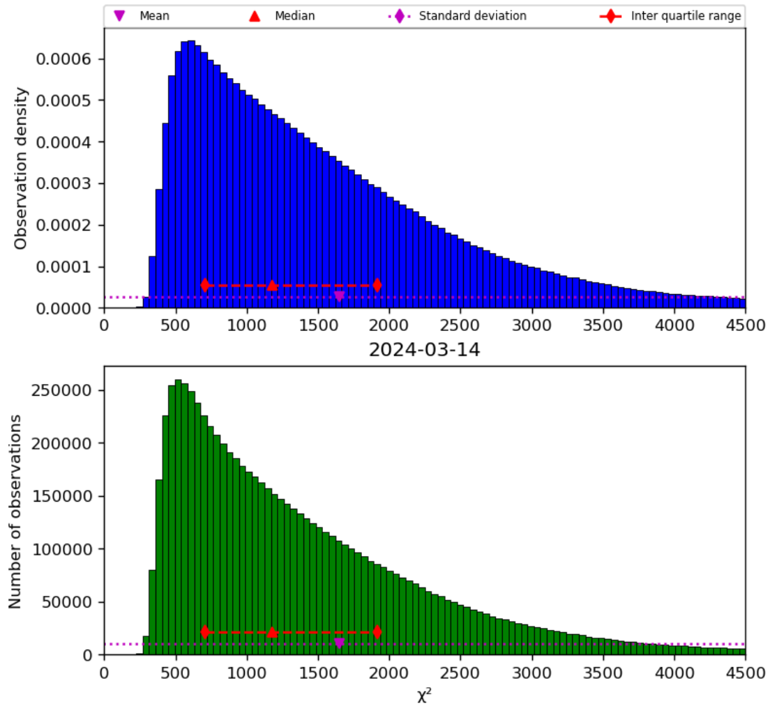
Figure 22: Histogram of “ \chi^2 ” for 2024-03-14 to 2024-03-15
