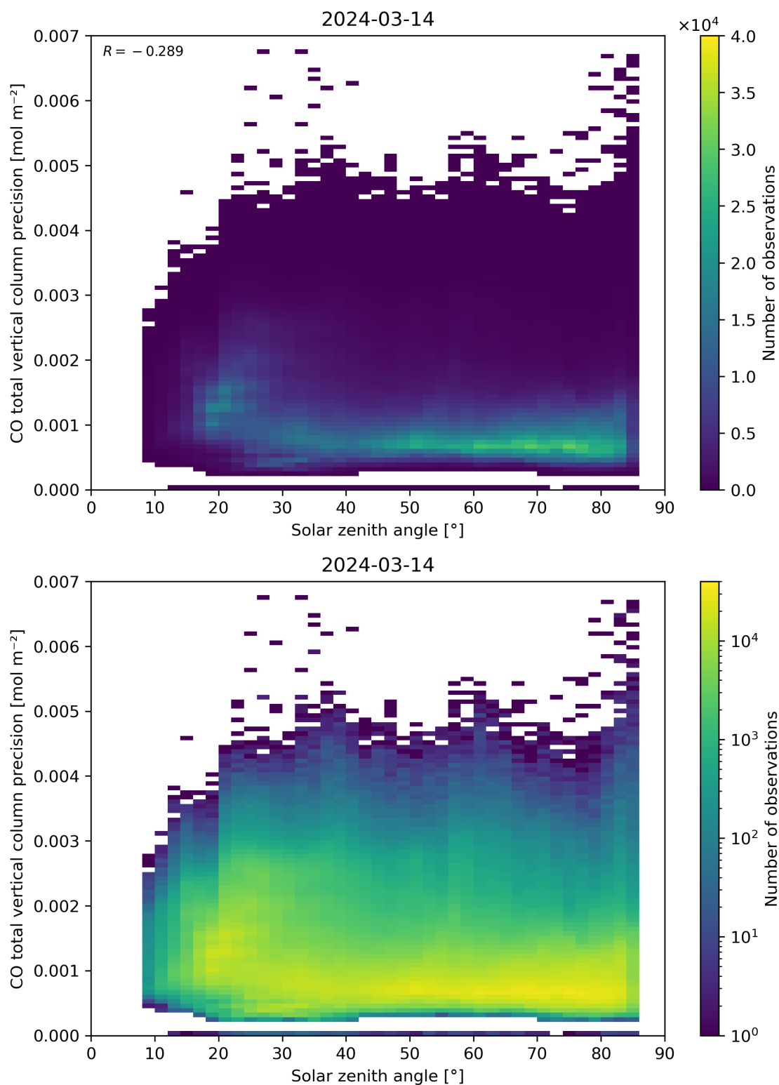
Figure 63: Scatter density plot of “Solar zenith angle” against “CO total vertical column precision” for 2024-03-14 to 2024-03-15.
