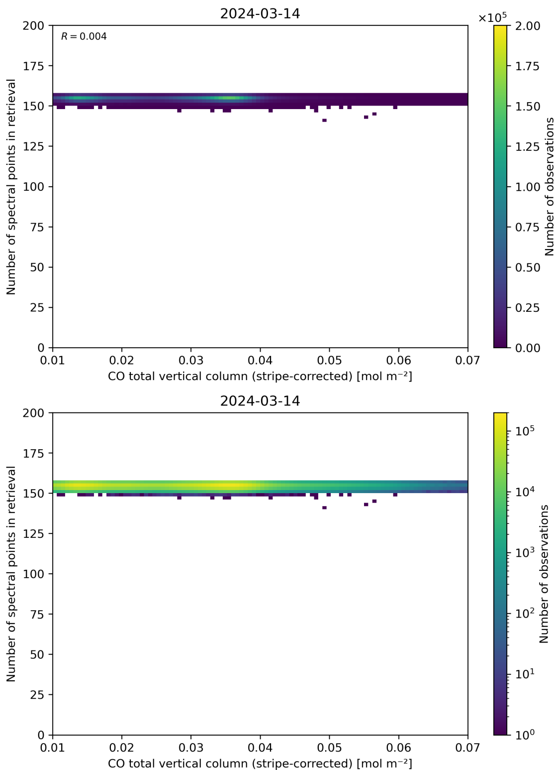
Figure 40: Scatter density plot of “CO total vertical column (stripe-corrected)” against “Number of spectral points in retrieval” for 2024-03-14 to 2024-03-15.
