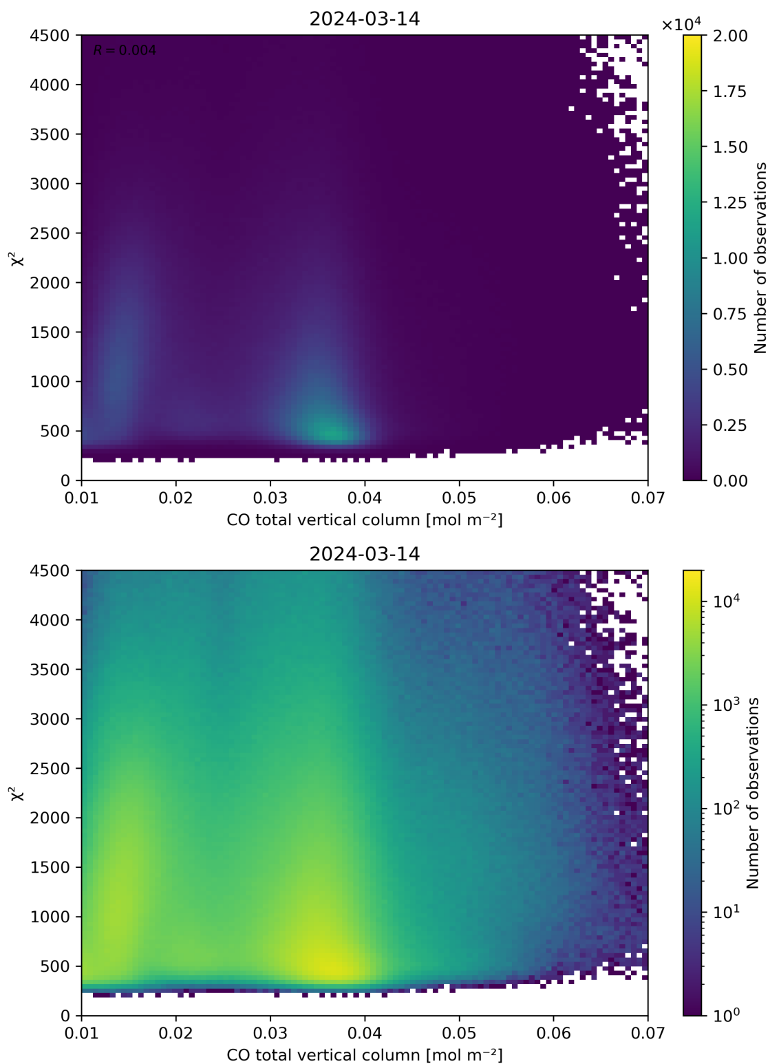
Figure 35: Scatter density plot of “CO total vertical column” against “ \chi^2 ” for 2024-03-14 to 2024-03-15.
