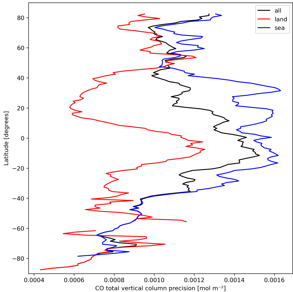
Figure 12: Zonal average of “CO total vertical column precision” for 2024-03-14 to 2024-03-15.
