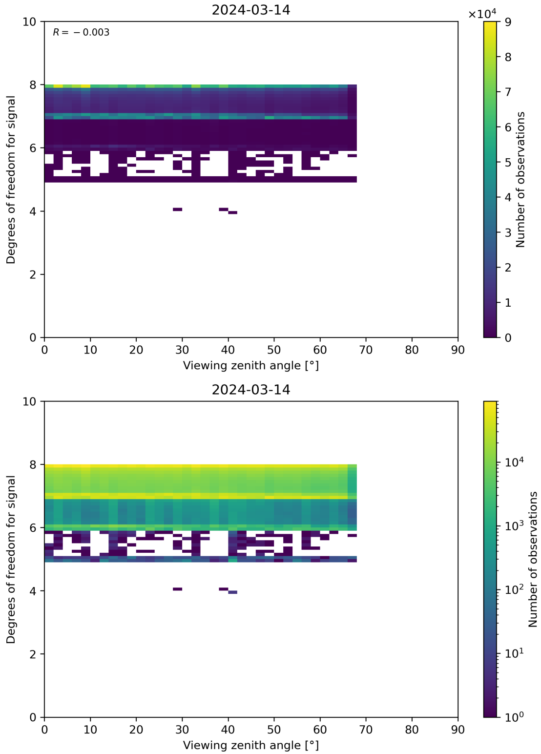
Figure 73: Scatter density plot of “Viewing zenith angle” against “Degrees of freedom for signal” for 2024-03-14 to 2024-03-15.
