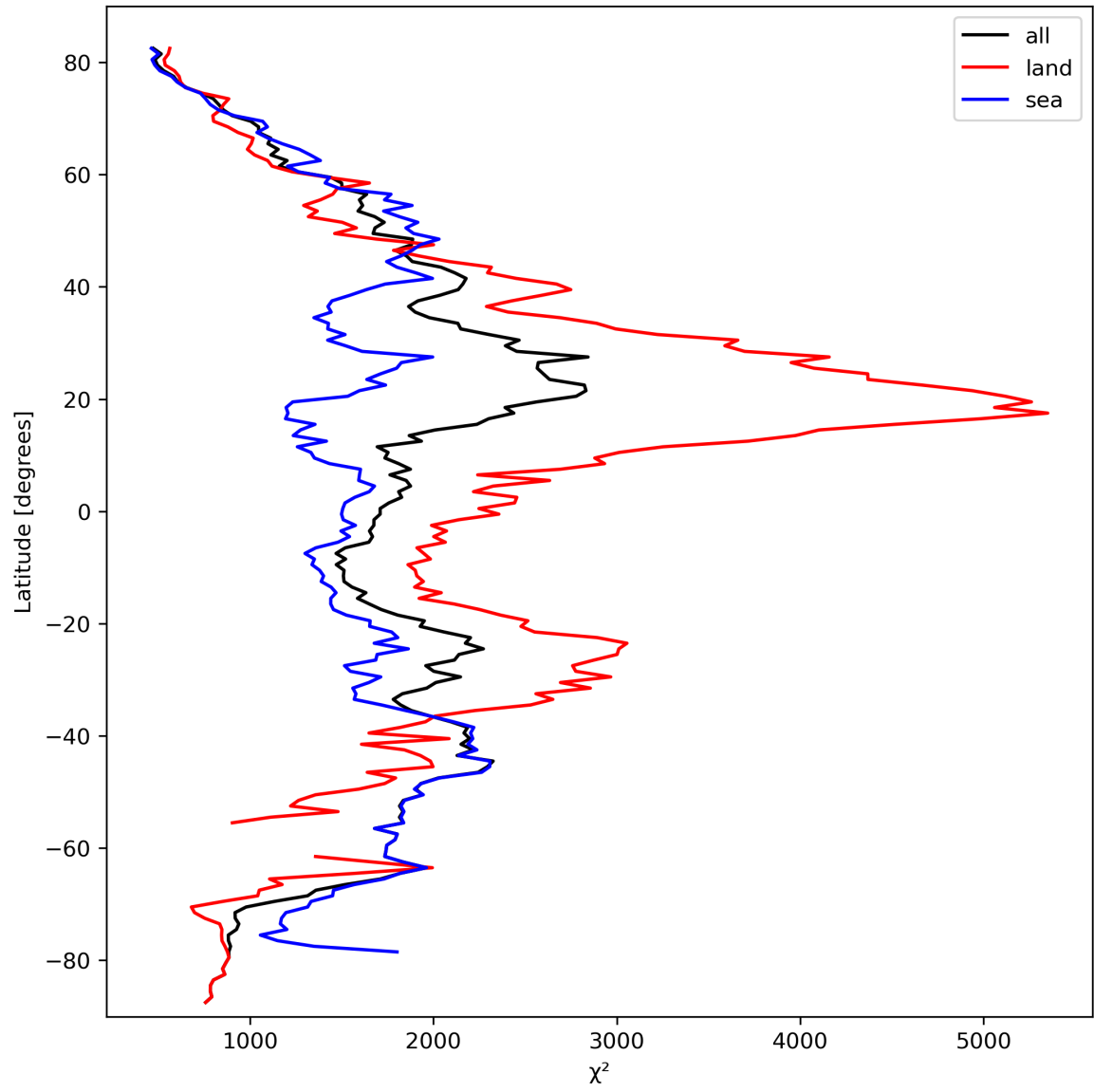
Figure 14: Zonal average of “ \chi^2 ” for 2024-03-14 to 2024-03-15.
