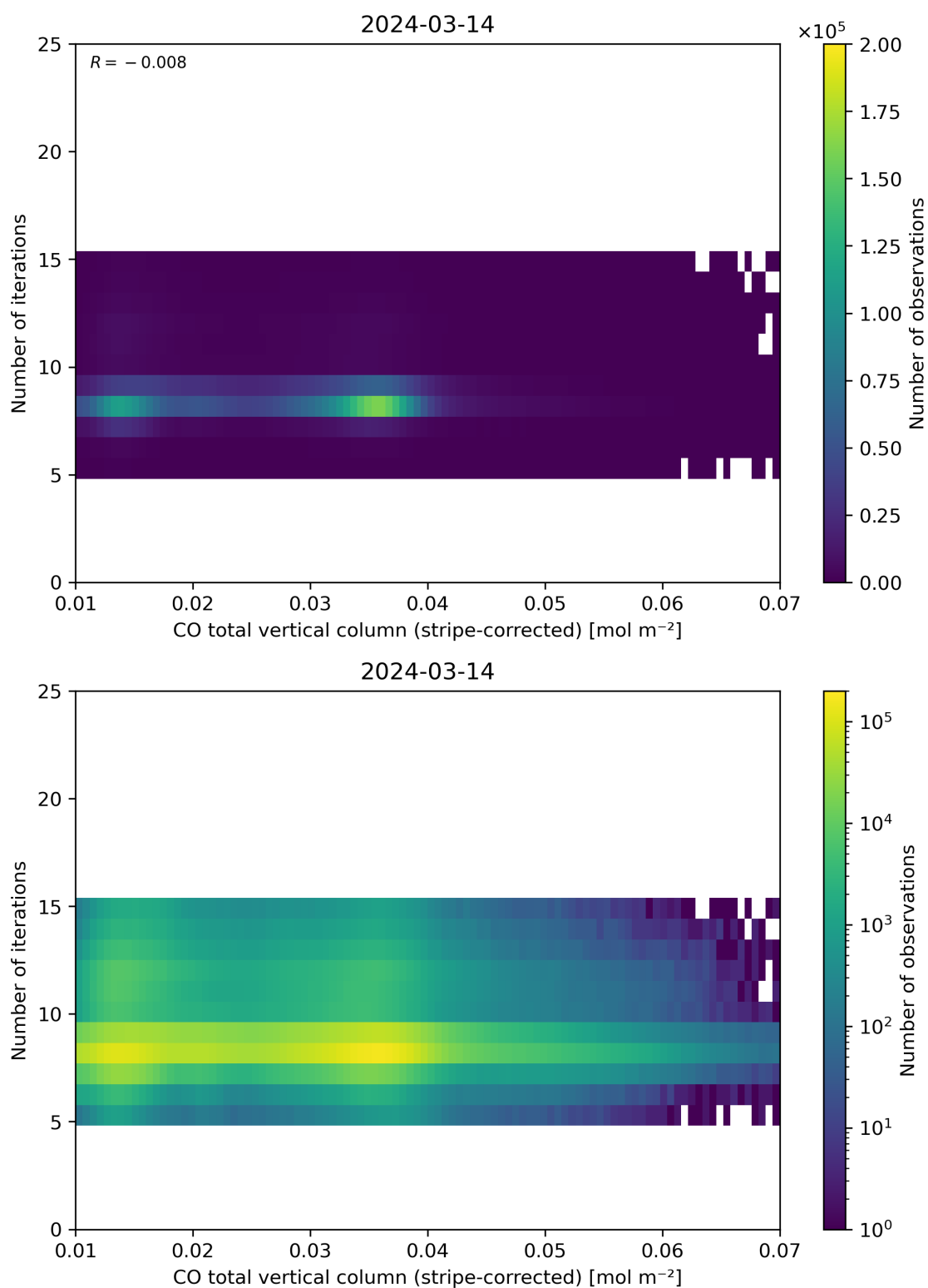
Figure 39: Scatter density plot of “CO total vertical column (stripe-corrected)” against “Number of iterations” for 2024-03-14 to 2024-03-15.
