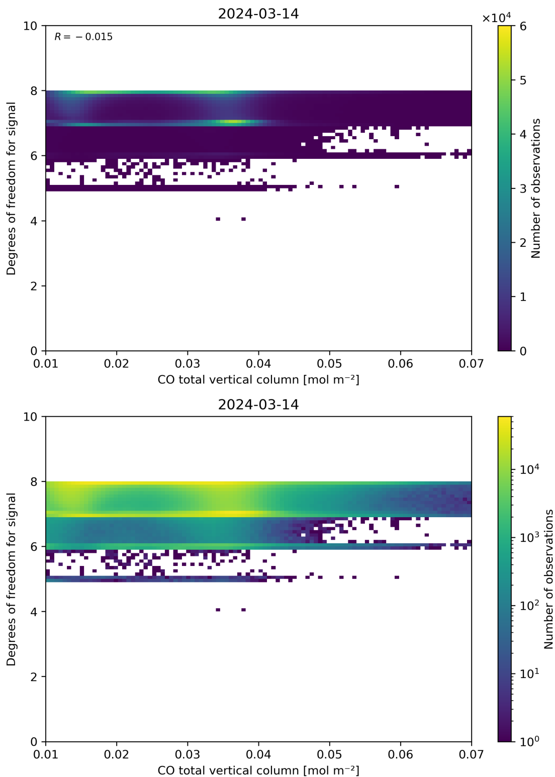
Figure 41: Scatter density plot of “CO total vertical column” against “Degrees of freedom for signal” for 2024-03-14 to 2024-03-15.
