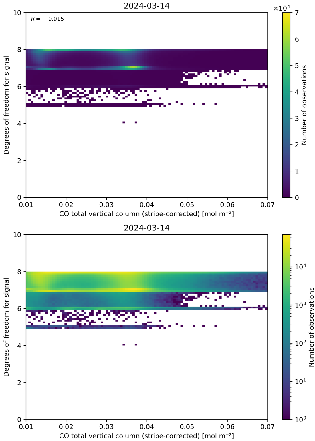
Figure 38: Scatter density plot of “CO total vertical column (stripe-corrected)” against “Degrees of freedom for signal” for 2024-03-14 to 2024-03-15.
