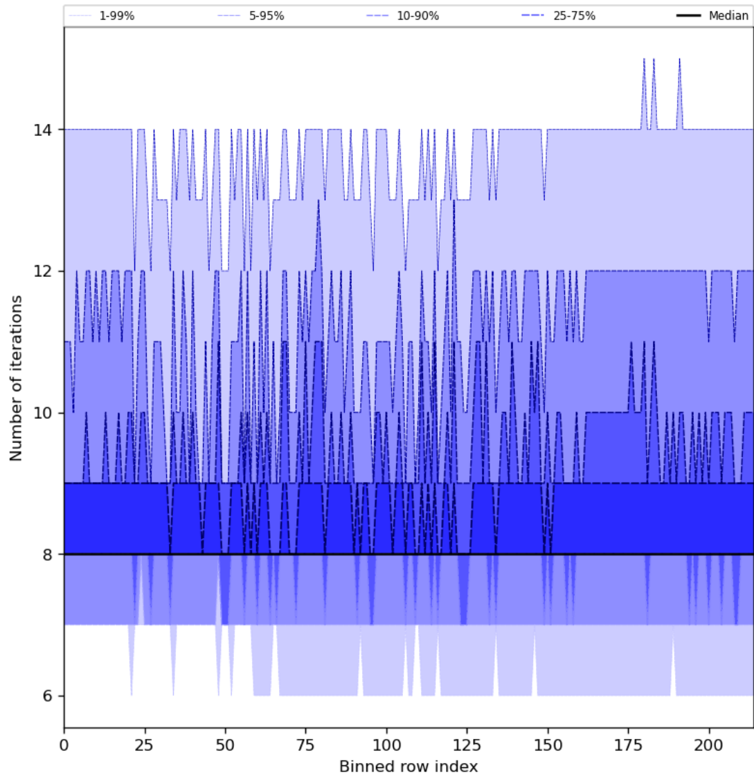
Figure 32: Along track statistics of “Number of iterations” for 2024-03-14 to 2024-03-15
