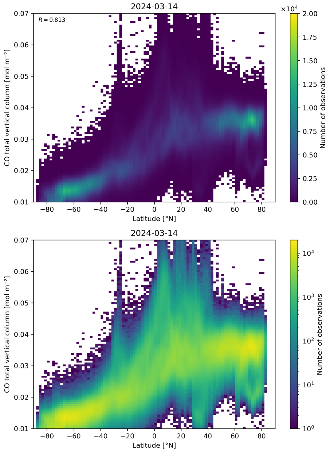
Figure 51: Scatter density plot of “Latitude” against “CO total vertical column” for 2024-03-14 to 2024-03-15.
