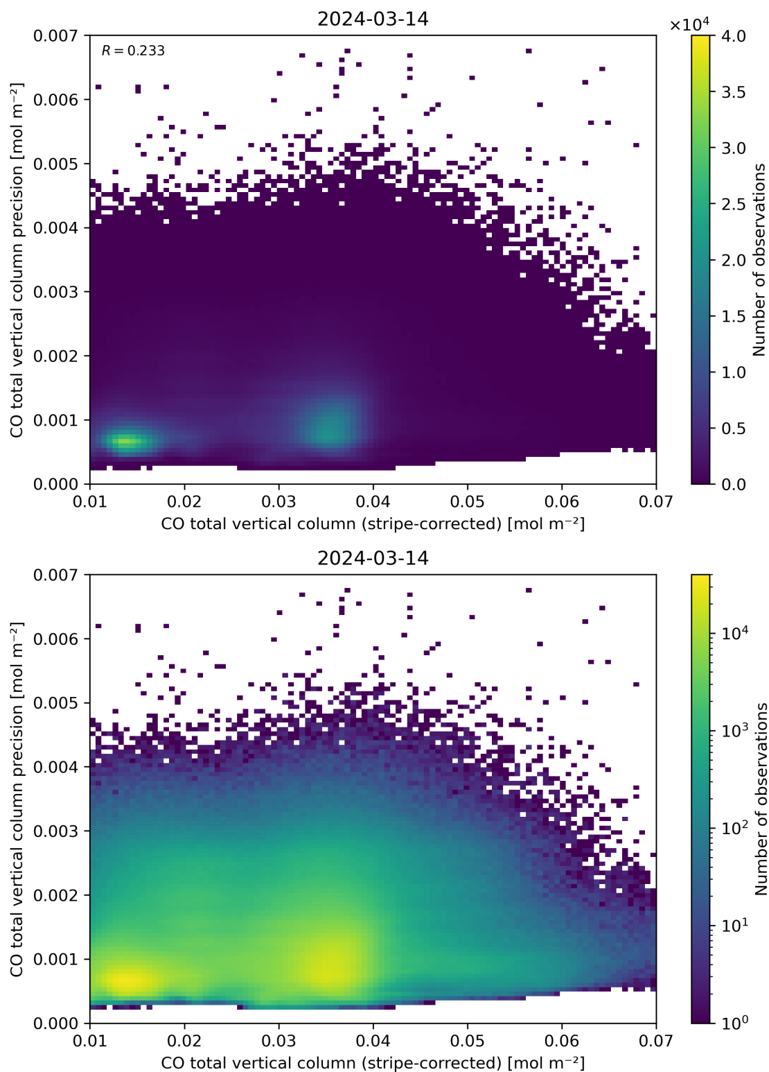
Figure 36: Scatter density plot of “CO total vertical column (stripe-corrected)” against “CO total vertical column precision” for 2024-03-14 to 2024-03-15.
