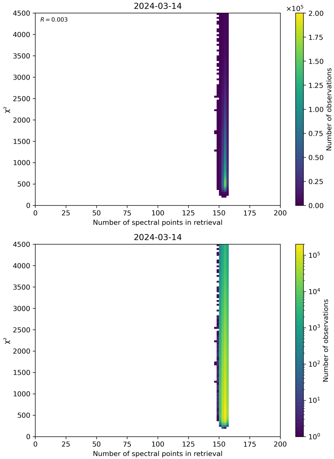
Figure 58: Scatter density plot of “Number of spectral points in retrieval” against “ \chi^2 ” for 2024-03-14 to 2024-03-15.
