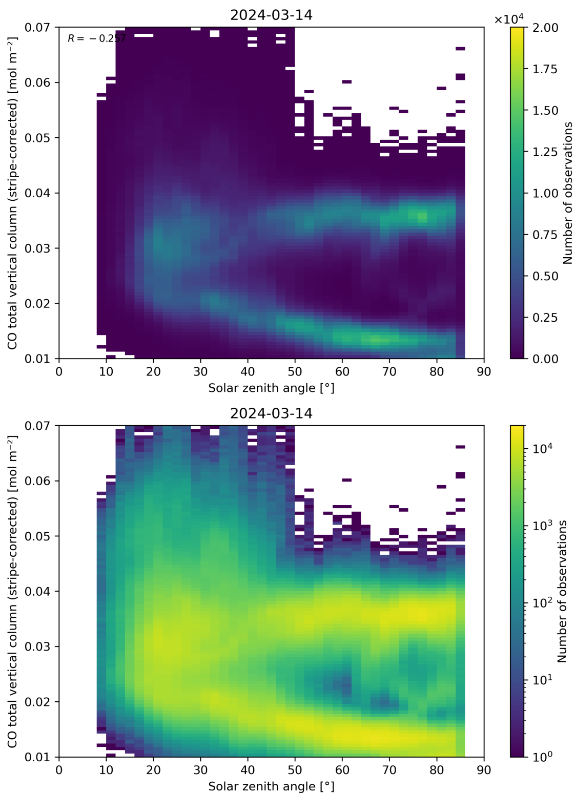
Figure 62: Scatter density plot of “Solar zenith angle” against “CO total vertical column (stripe-corrected)” for 2024-03-14 to 2024-03-15.
