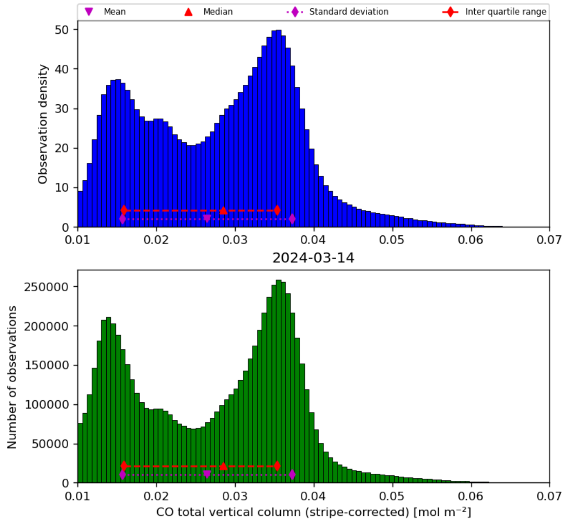
Figure 19: Histogram of “CO total vertical column (stripe-corrected)” for 2024-03-14 to 2024-03-15
