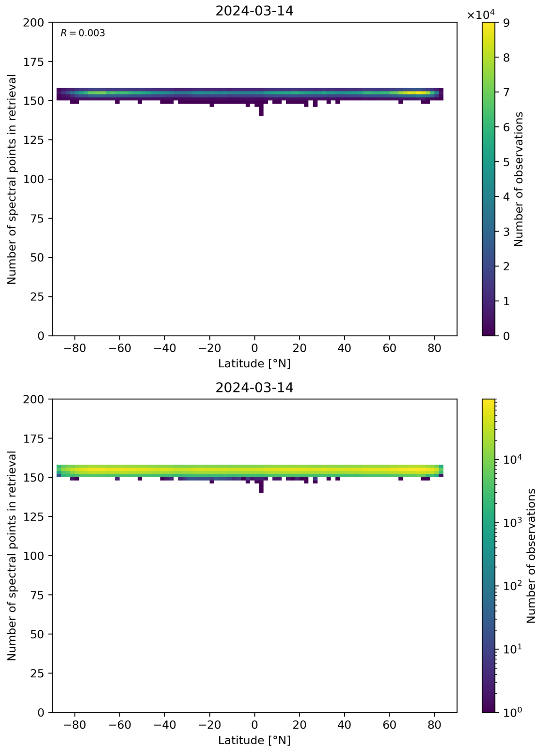
Figure 57: Scatter density plot of “Latitude” against “Number of spectral points in retrieval” for 2024-03-14 to 2024-03-15.
