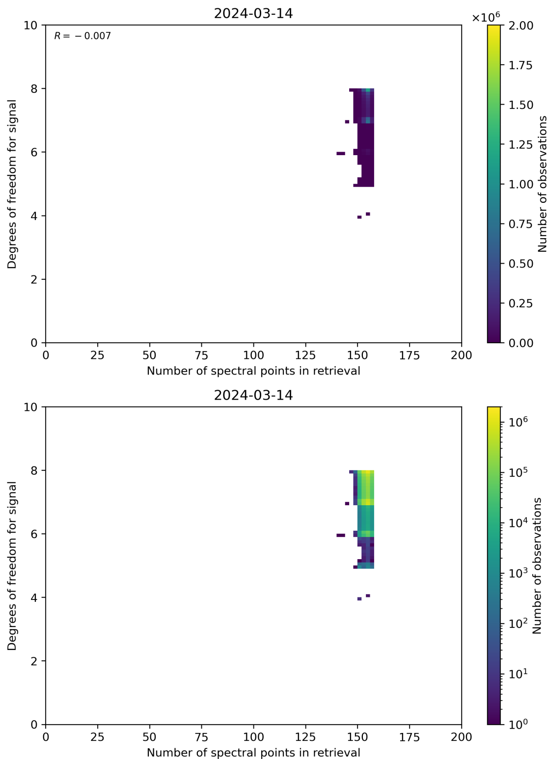
Figure 59: Scatter density plot of “Number of spectral points in retrieval” against “Degrees of freedom for signal” for 2024-03-14 to 2024-03-15.
