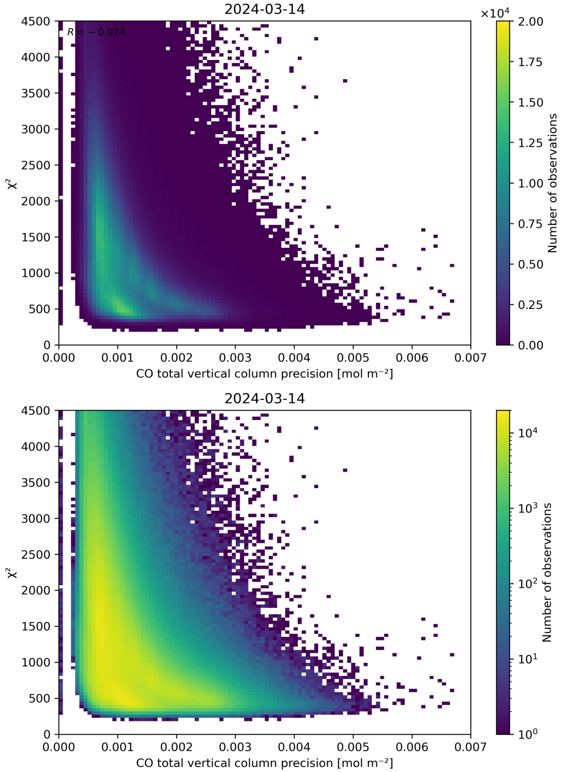
Figure 44: Scatter density plot of “CO total vertical column precision” against “ \chi^2 ” for 2024-03-14 to 2024-03-15.
