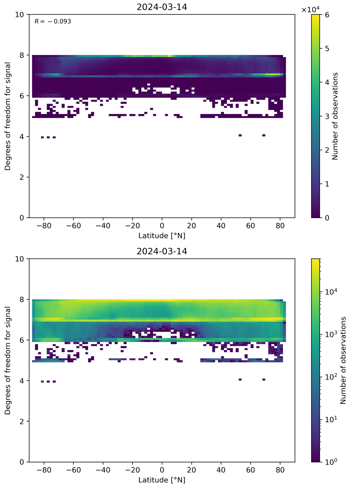
Figure 55: Scatter density plot of “Latitude” against “Degrees of freedom for signal” for 2024-03-14 to 2024-03-15.
