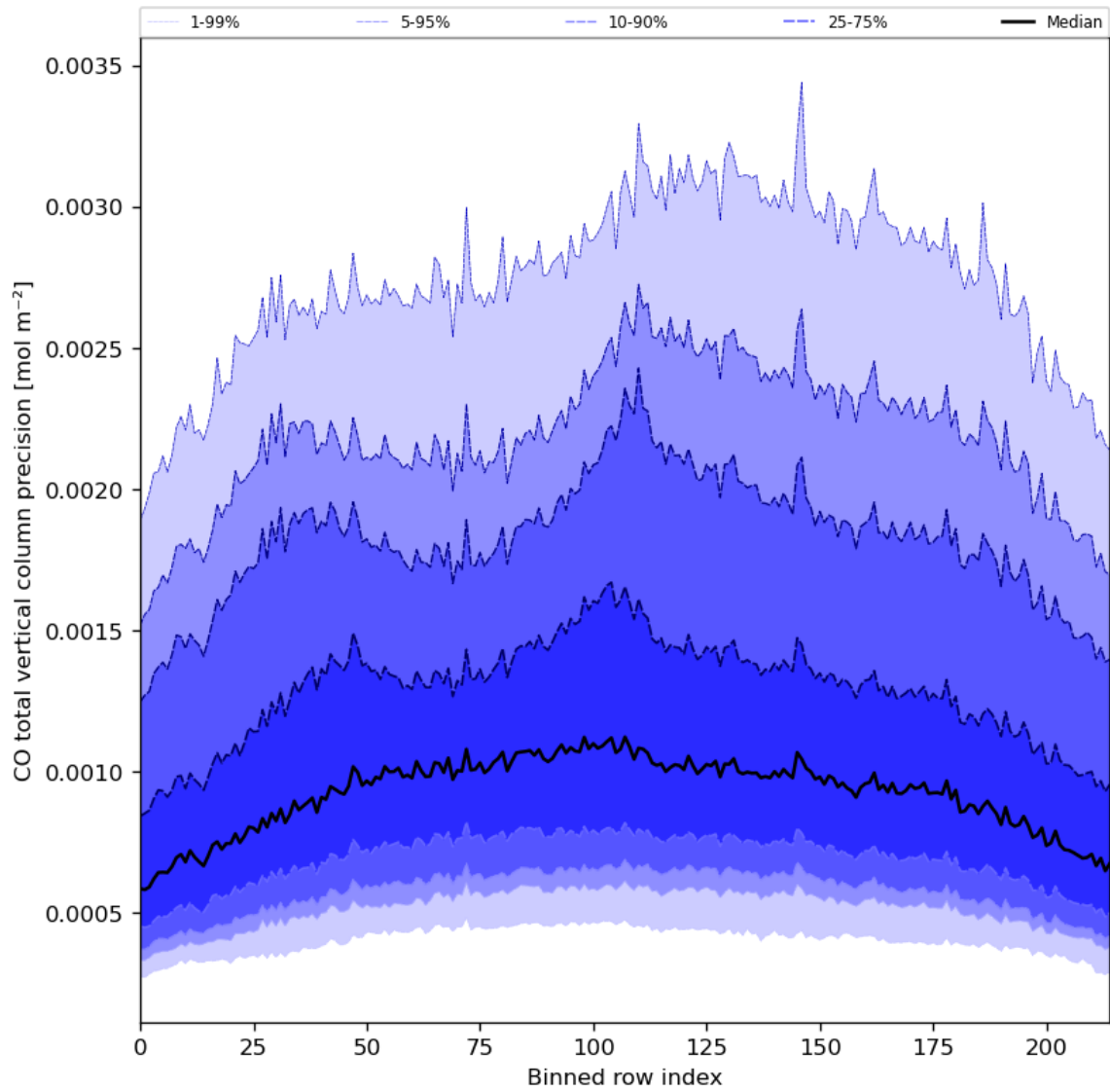
Figure 28: Along track statistics of “CO total vertical column precision” for 2024-03-14 to 2024-03-15
