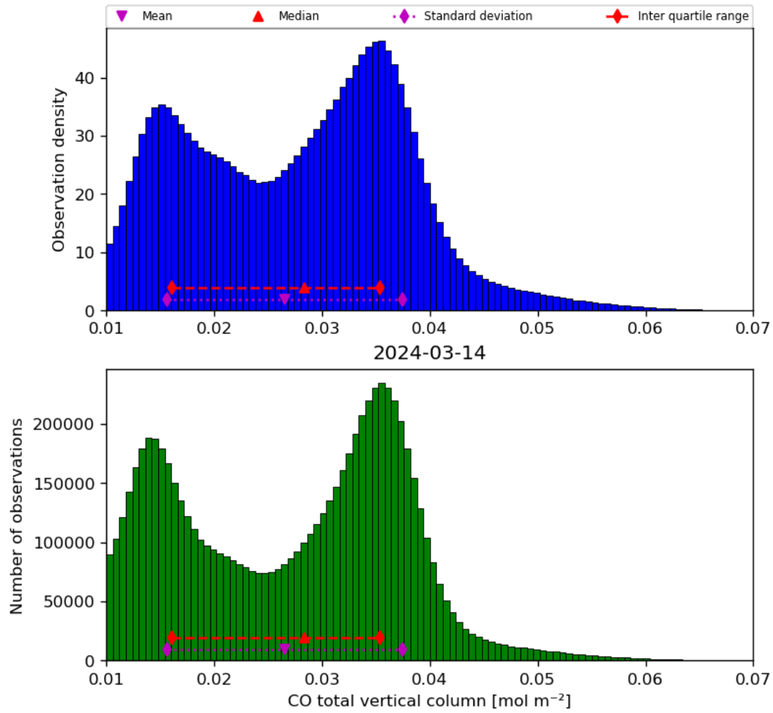
Figure 18: Histogram of “CO total vertical column” for 2024-03-14 to 2024-03-15
