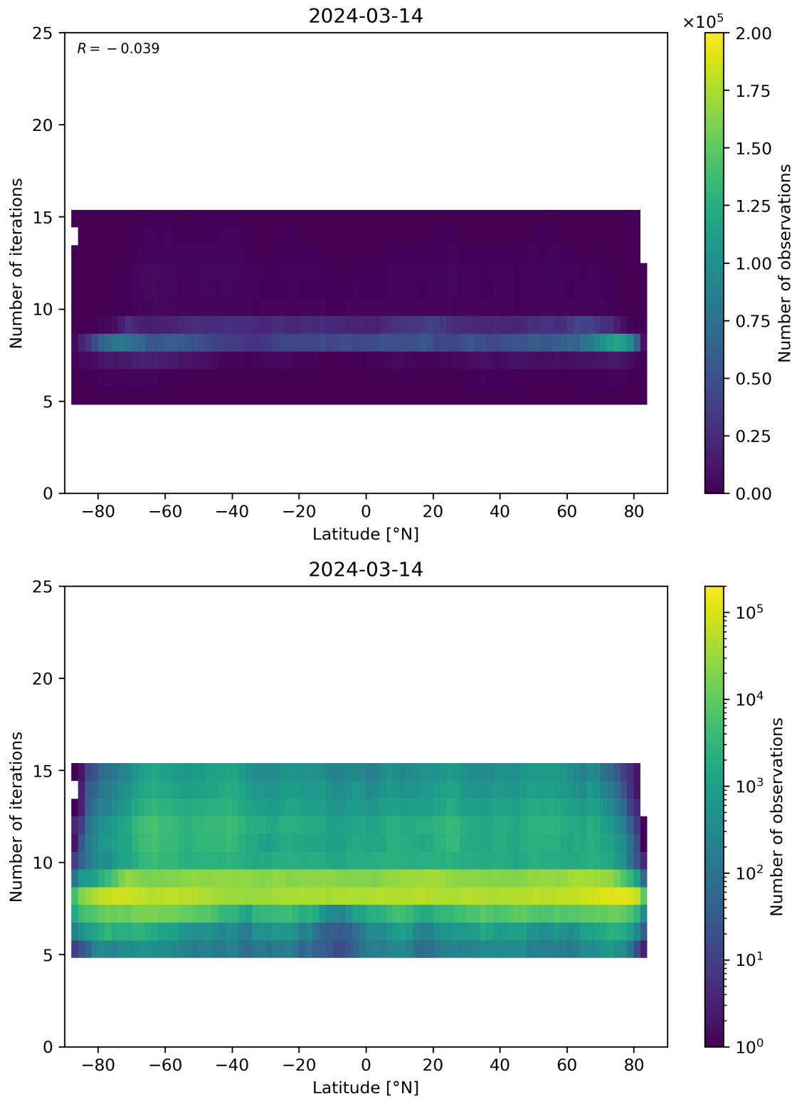
Figure 56: Scatter density plot of “Latitude” against “Number of iterations” for 2024-03-14 to 2024-03-15.
