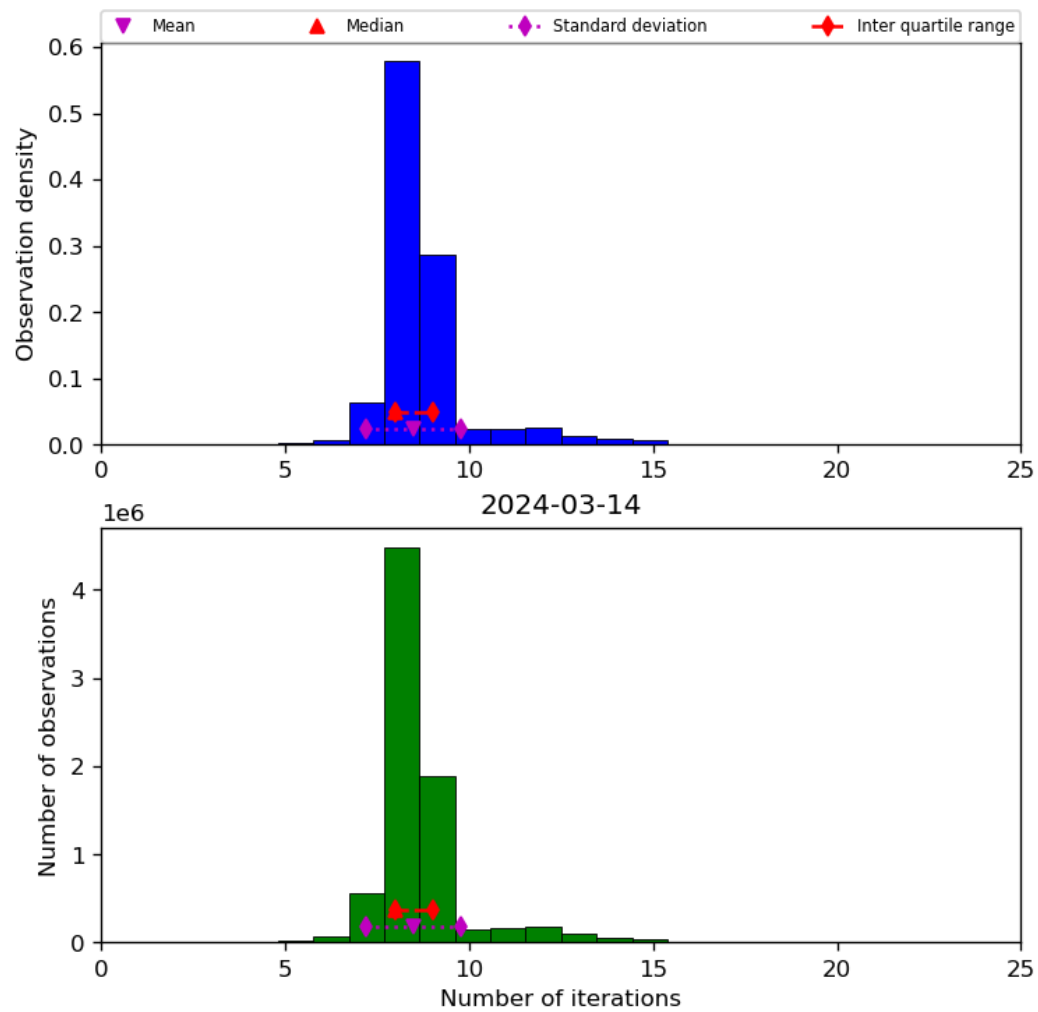
Figure 24: Histogram of “Number of iterations” for 2024-03-14 to 2024-03-15
