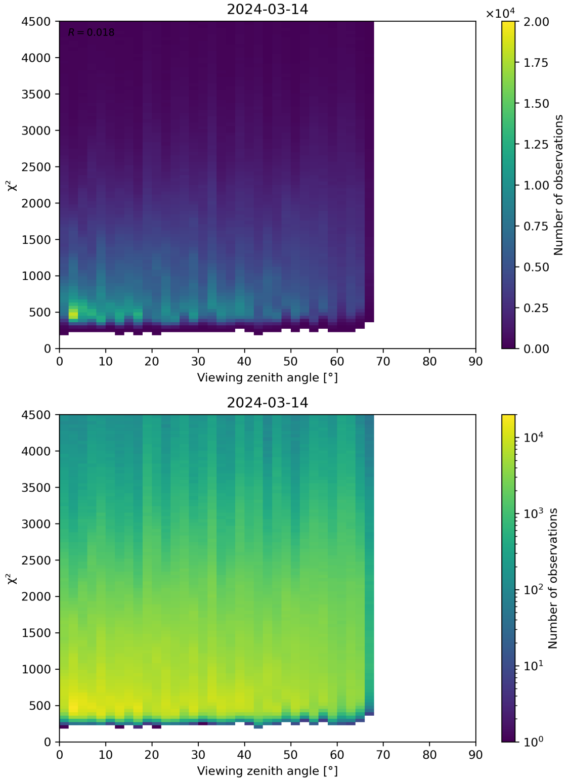
Figure 72: Scatter density plot of “Viewing zenith angle” against “ \chi^2 ” for 2024-03-14 to 2024-03-15.
