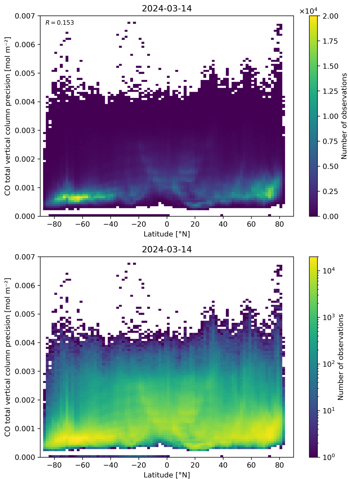
Figure 53: Scatter density plot of “Latitude” against “CO total vertical column precision” for 2024-03-14 to 2024-03-15.
