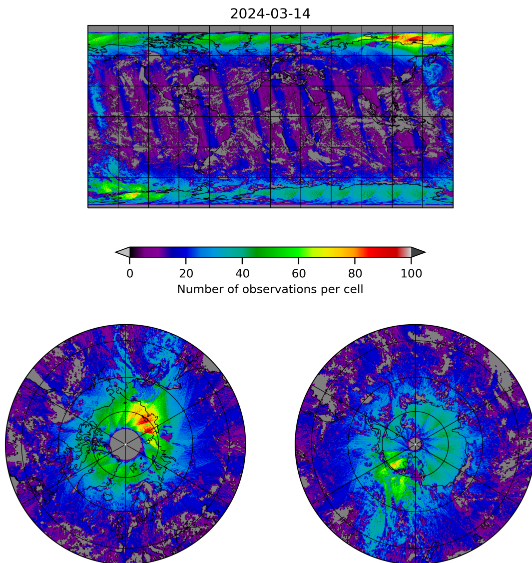
Figure 8: Map of the number of observations for 2024-03-14 to 2024-03-15
