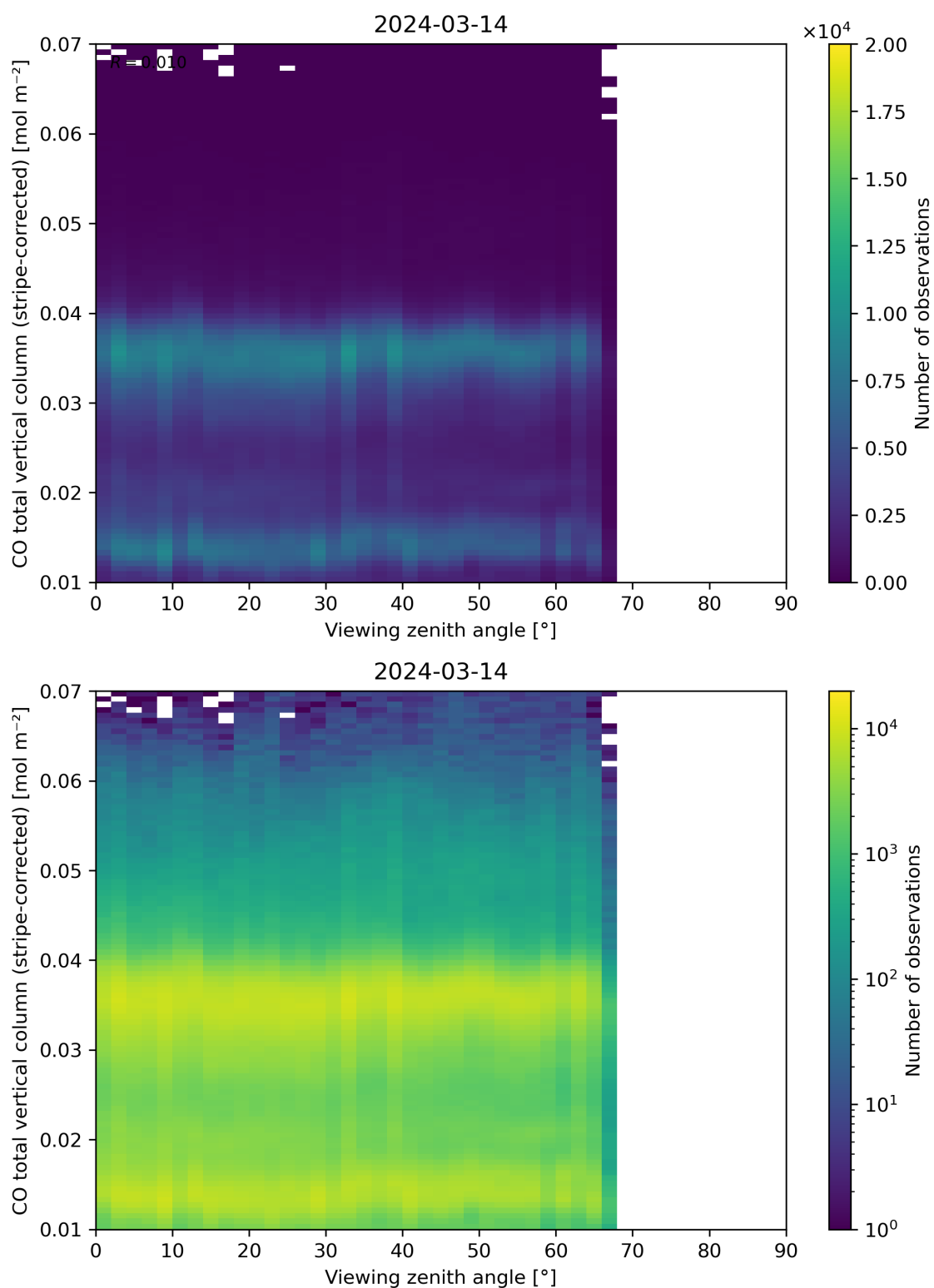
Figure 70: Scatter density plot of “Viewing zenith angle” against “CO total vertical column (stripe-corrected)” for 2024-03-14 to 2024-03-15.
