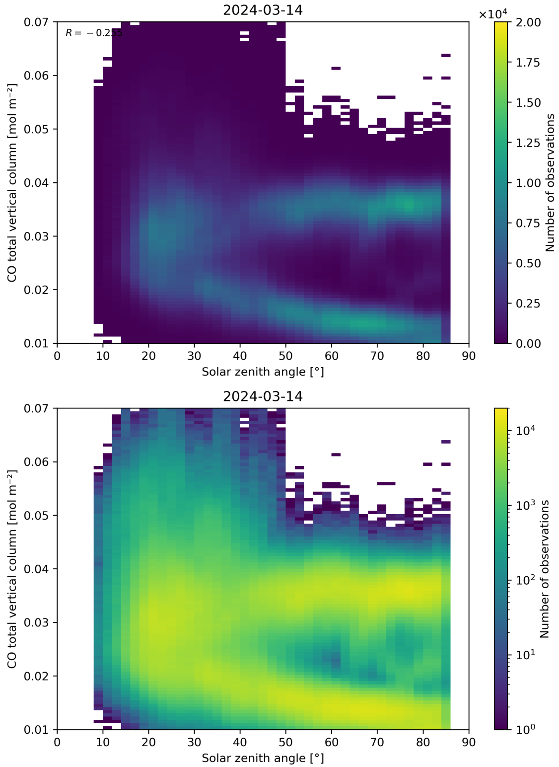
Figure 61: Scatter density plot of “Solar zenith angle” against “CO total vertical column” for 2024-03-14 to 2024-03-15.
