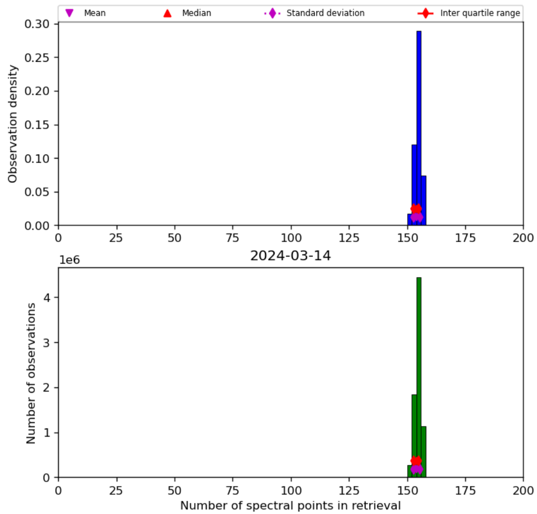
Figure 21: Histogram of “Number of spectral points in retrieval” for 2024-03-14 to 2024-03-15
