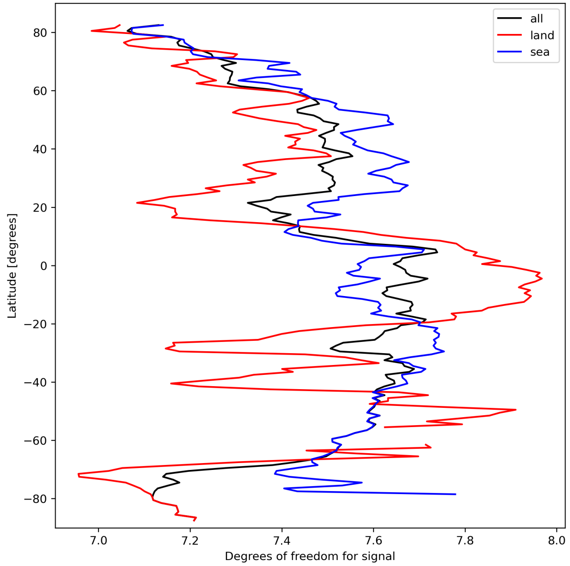
Figure 15: Zonal average of “Degrees of freedom for signal” for 2024-03-14 to 2024-03-15.
