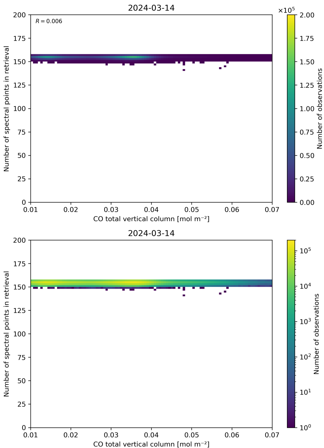
Figure 43: Scatter density plot of “CO total vertical column” against “Number of spectral points in retrieval” for 2024-03-14 to 2024-03-15.
