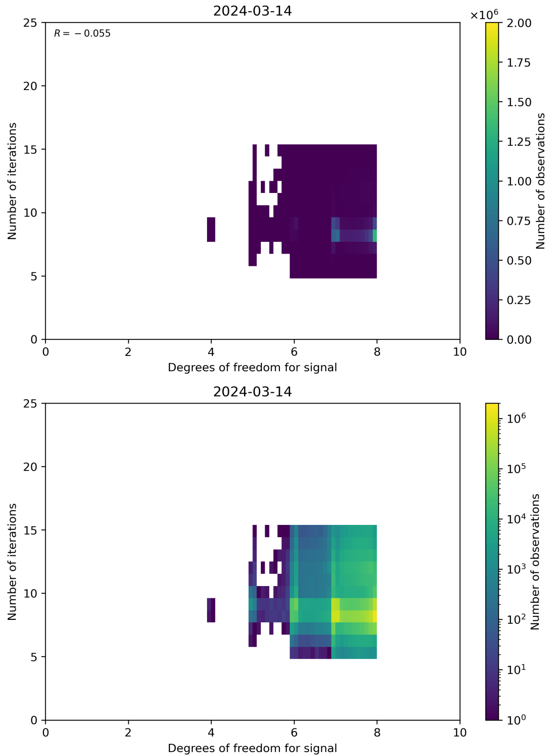
Figure 50: Scatter density plot of “Degrees of freedom for signal” against “Number of iterations” for 2024-03-14 to 2024-03-15.
