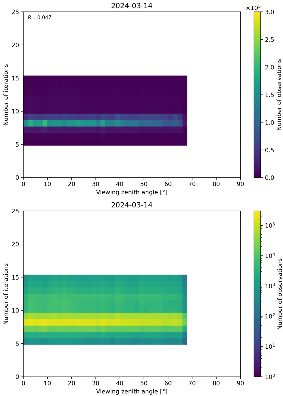
Figure 75: Scatter density plot of “Viewing zenith angle” against “Number of iterations” for 2024-03-14 to 2024-03-15.
