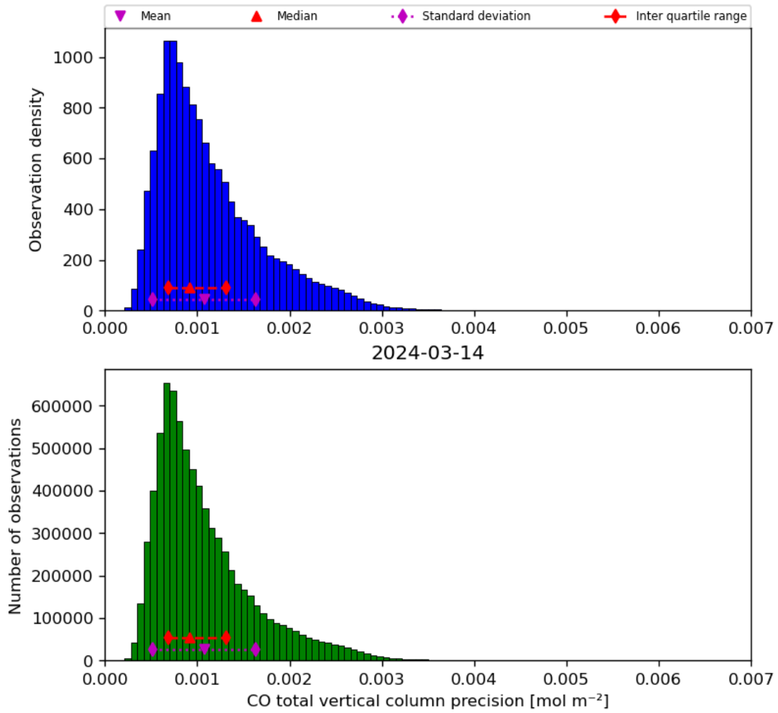
Figure 20: Histogram of “CO total vertical column precision” for 2024-03-14 to 2024-03-15
