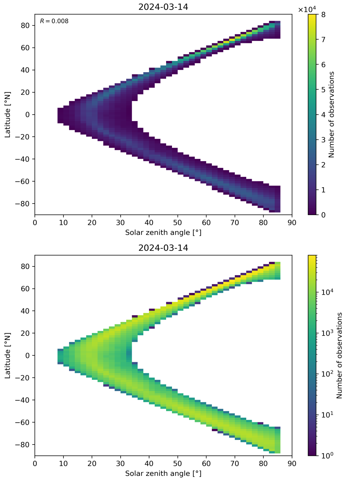
Figure 66: Scatter density plot of “Solar zenith angle” against “Latitude” for 2024-03-14 to 2024-03-15.
