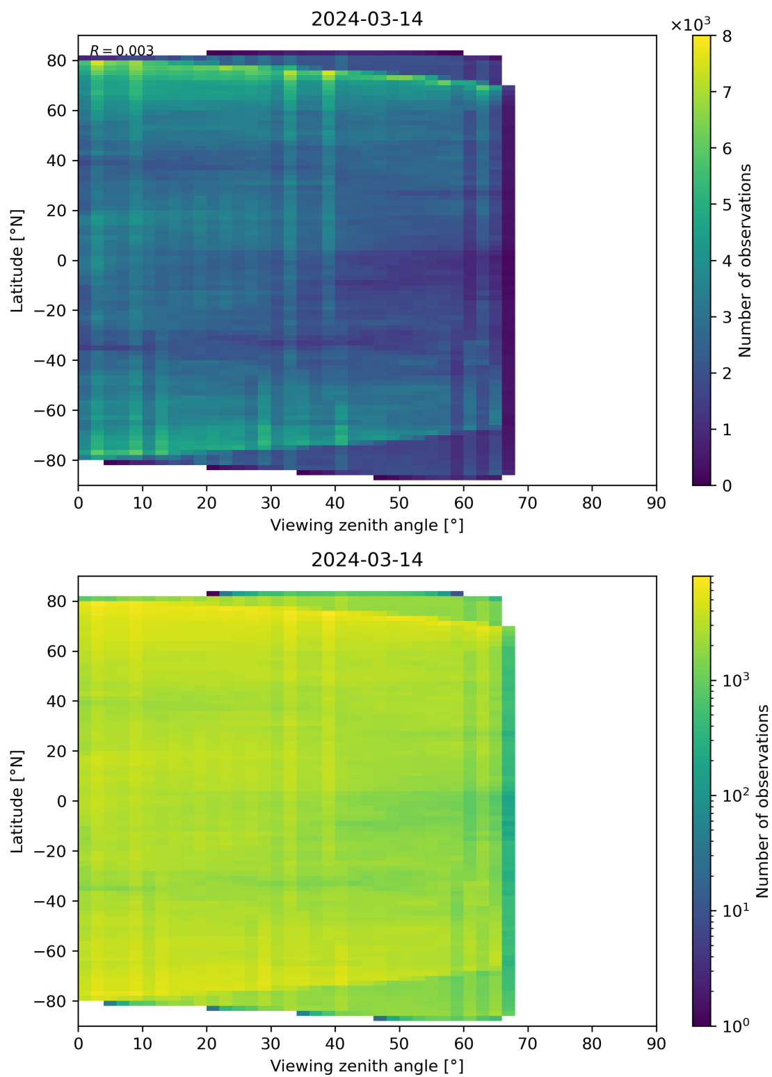
Figure 74: Scatter density plot of “Viewing zenith angle” against “Latitude” for 2024-03-14 to 2024-03-15.
