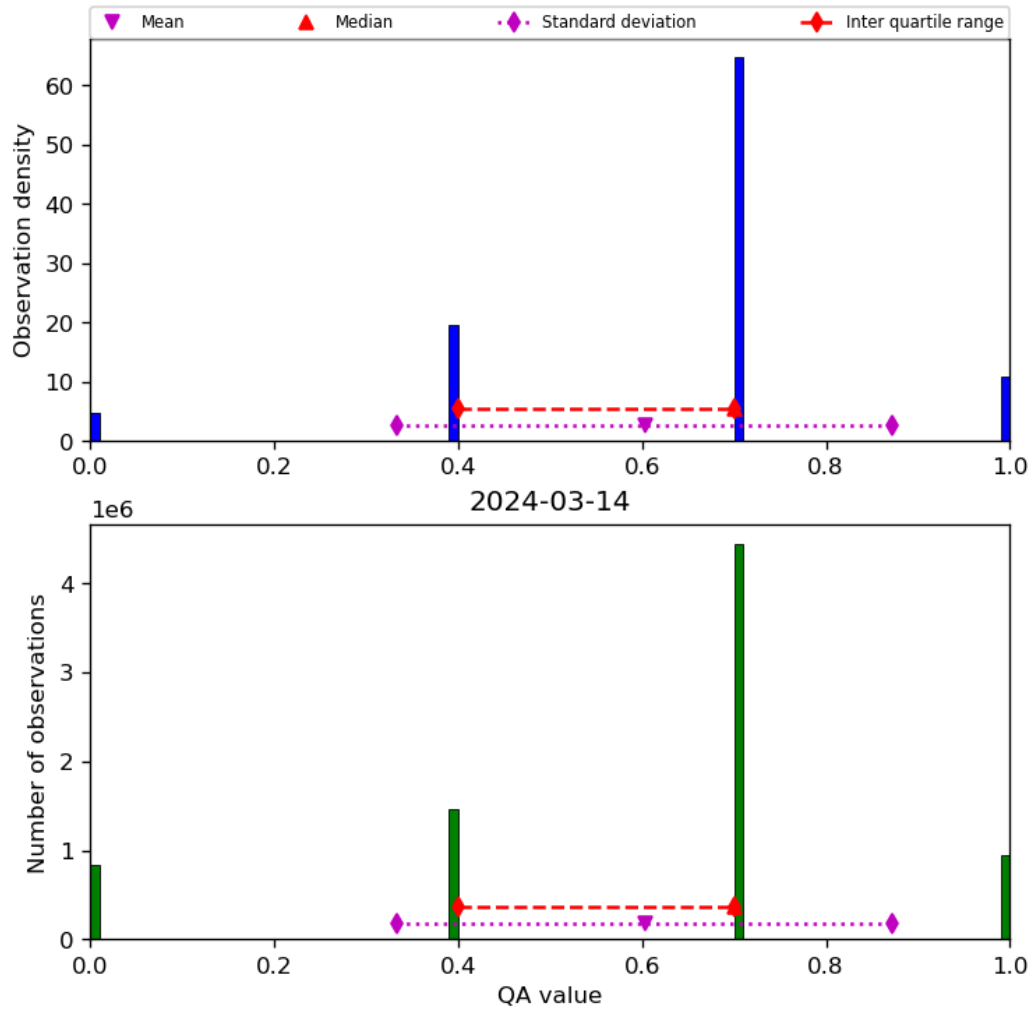
Figure 17: Histogram of “QA value” for 2024-03-14 to 2024-03-15
