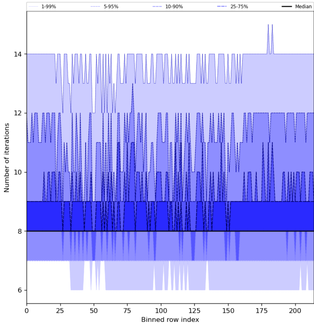
Figure 32: Along track statistics of “Number of iterations” for 2024-03-14 to 2024-03-16
