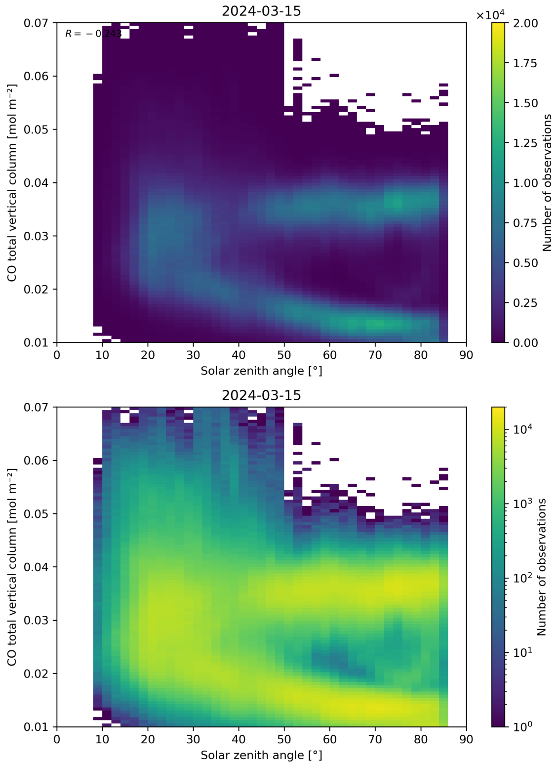
Figure 61: Scatter density plot of “Solar zenith angle” against “CO total vertical column” for 2024-03-14 to 2024-03-16.
