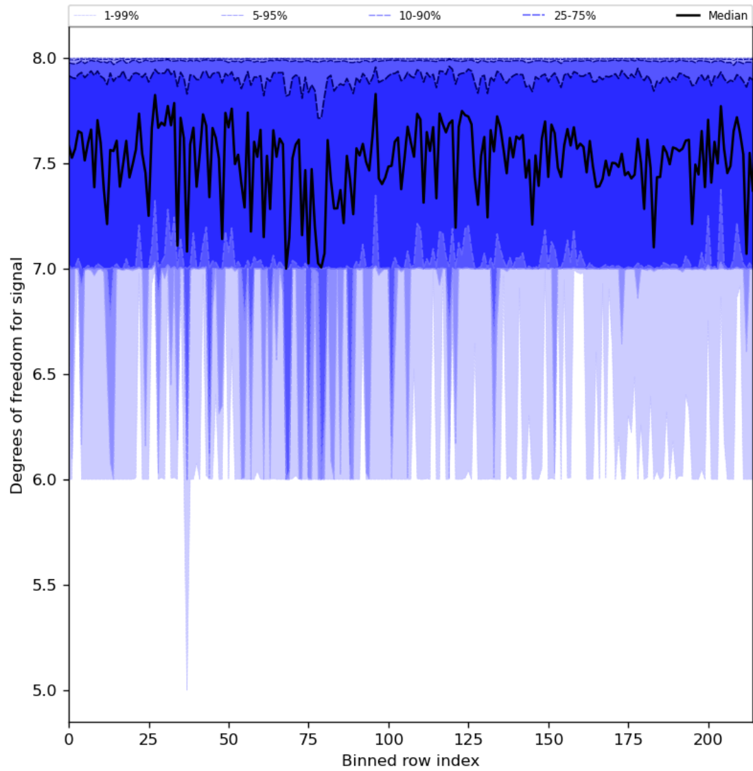
Figure 31: Along track statistics of “Degrees of freedom for signal” for 2024-03-14 to 2024-03-16
