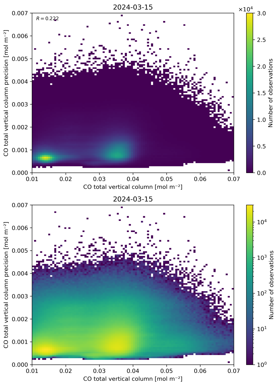
Figure 34: Scatter density plot of “CO total vertical column” against “CO total vertical column precision” for 2024-03-14 to 2024-03-16.
