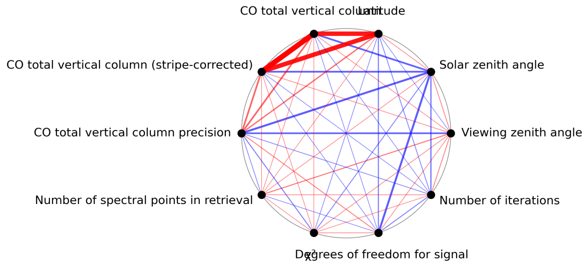
Figure 1: Map of correlation graph for 2024-03-14 to 2024-03-16.
