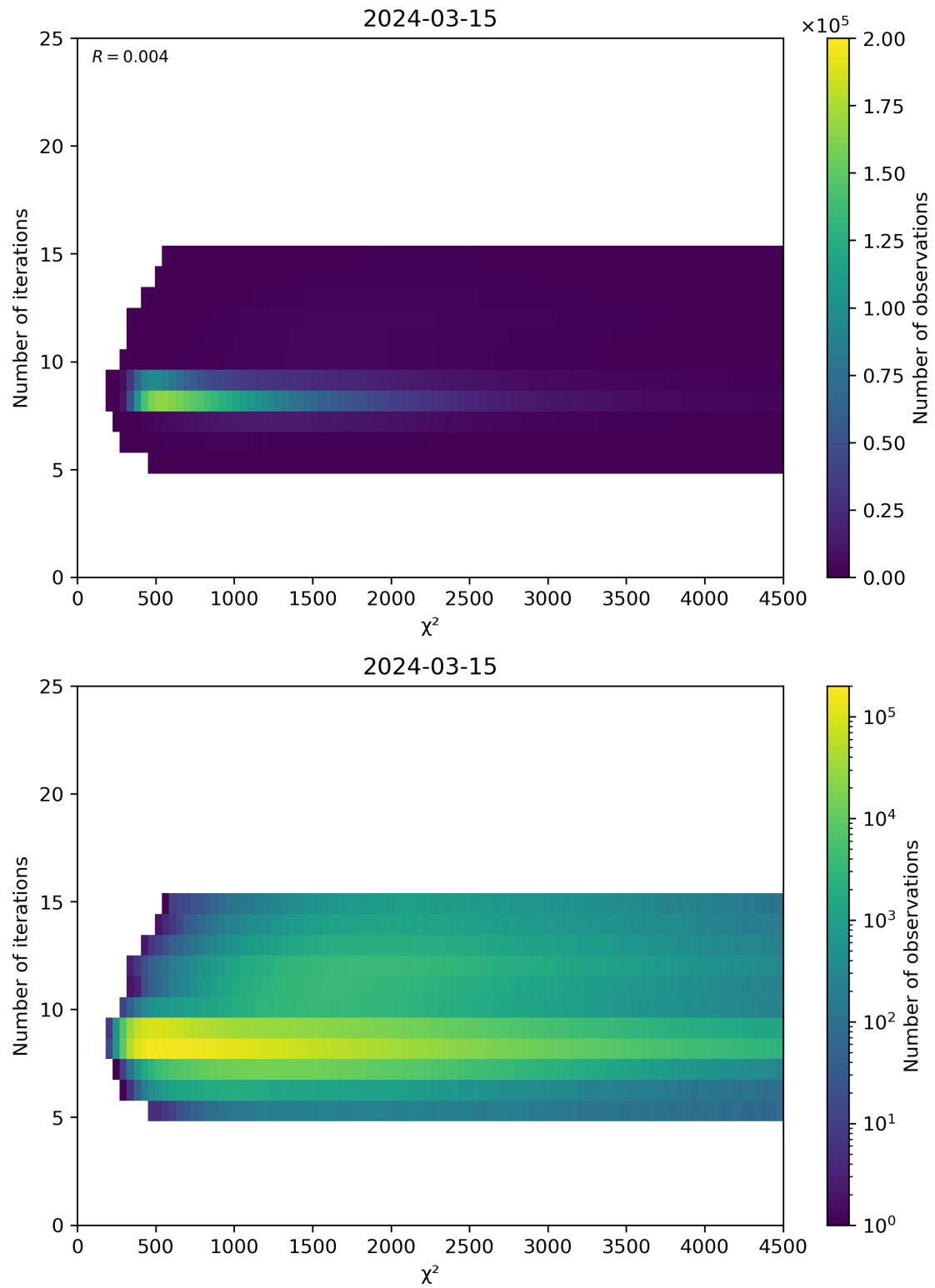
Figure 49: Scatter density plot of “ \chi^2 ” against “Number of iterations” for 2024-03-14 to 2024-03-16.
