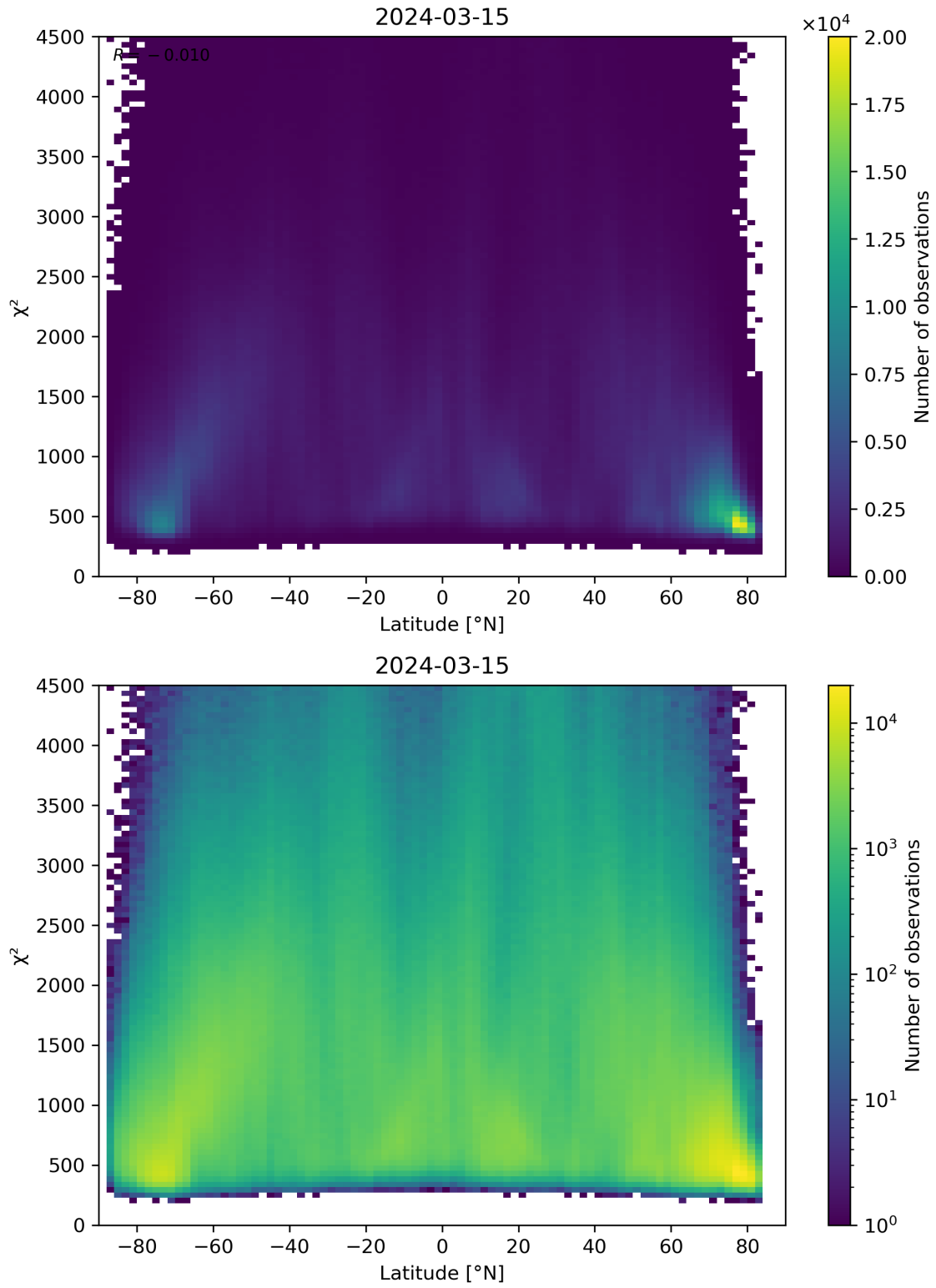
Figure 54: Scatter density plot of “Latitude” against “ \chi^2 ” for 2024-03-14 to 2024-03-16.
