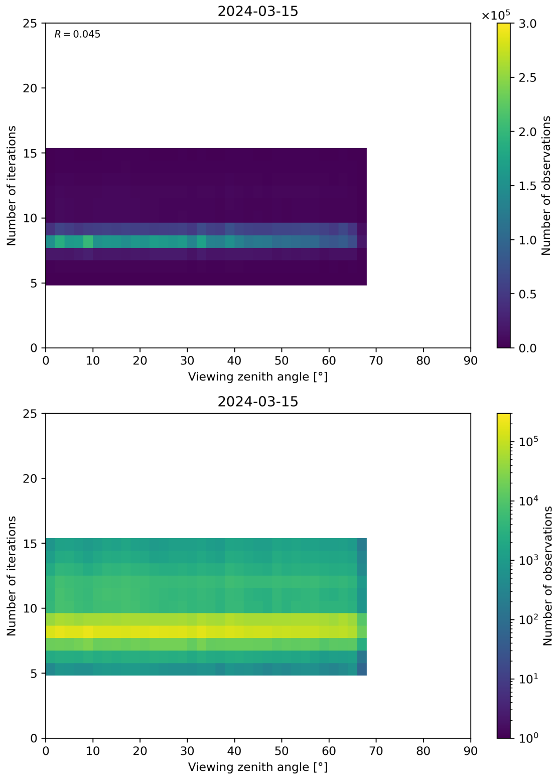
Figure 75: Scatter density plot of “Viewing zenith angle” against “Number of iterations” for 2024-03-14 to 2024-03-16.
