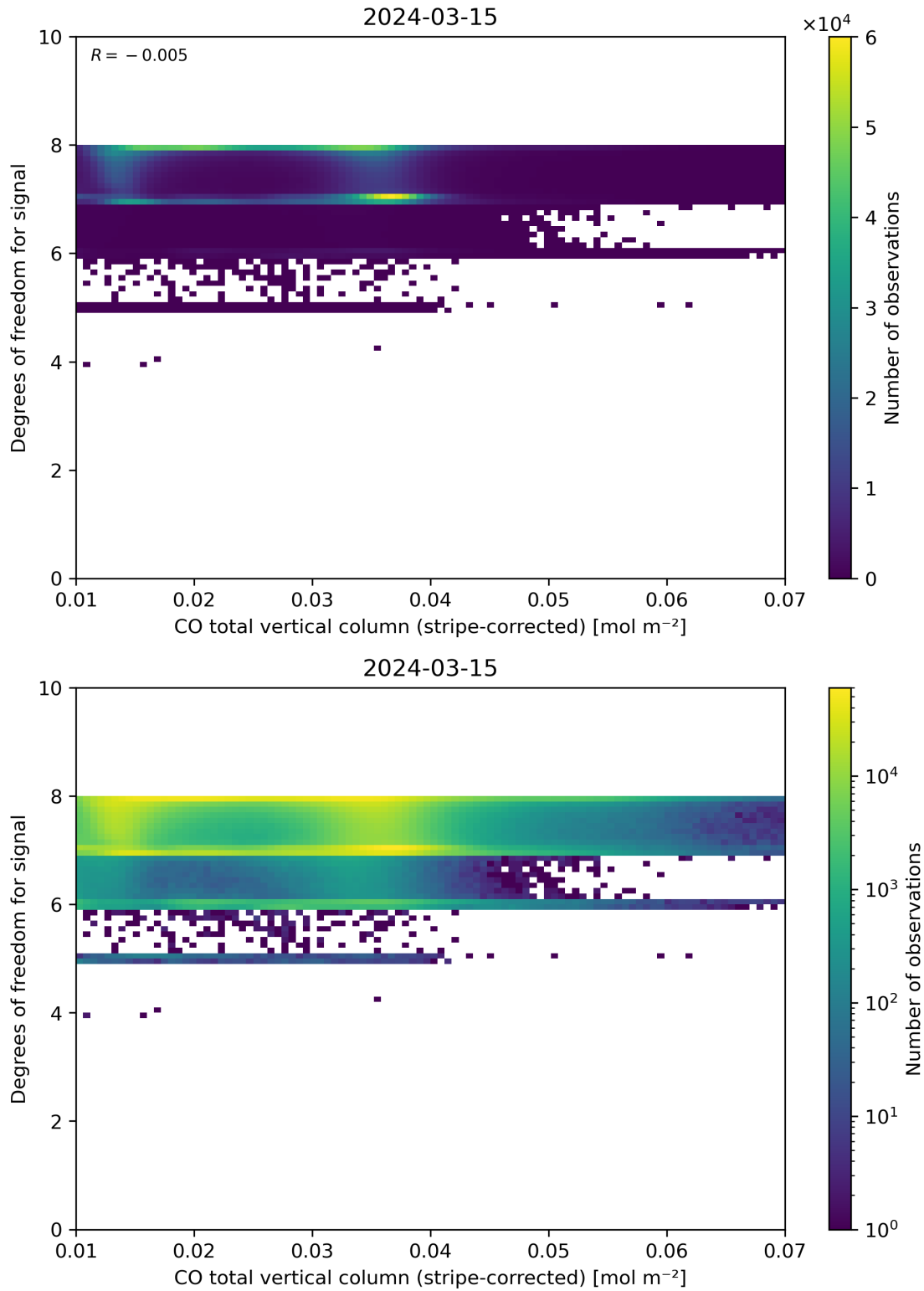
Figure 38: Scatter density plot of “CO total vertical column (stripe-corrected)” against “Degrees of freedom for signal” for 2024-03-14 to 2024-03-16.
