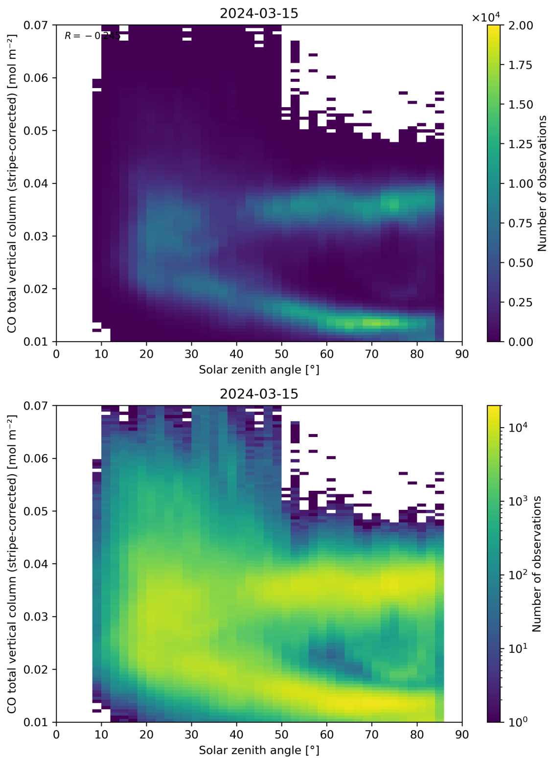
Figure 62: Scatter density plot of “Solar zenith angle” against “CO total vertical column (stripe-corrected)” for 2024-03-14 to 2024-03-16.
