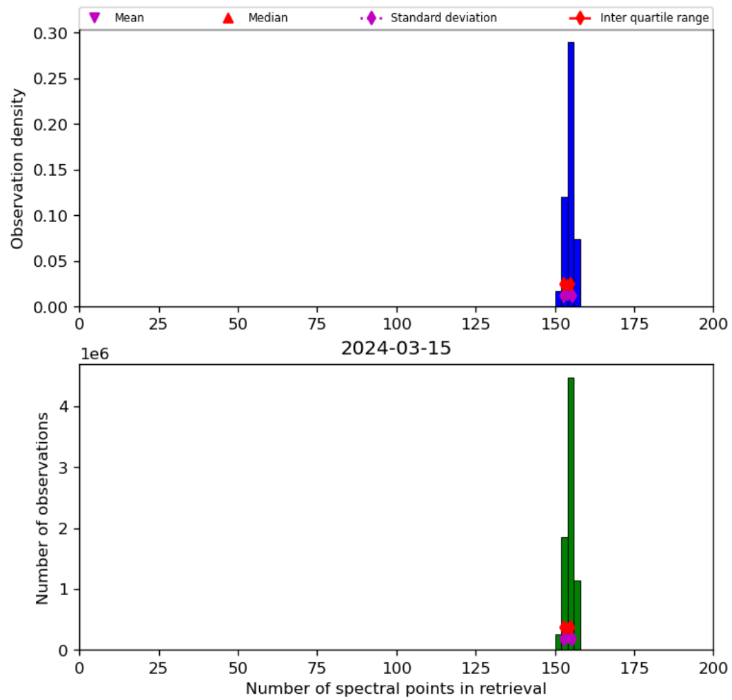
Figure 21: Histogram of “Number of spectral points in retrieval” for 2024-03-14 to 2024-03-16
