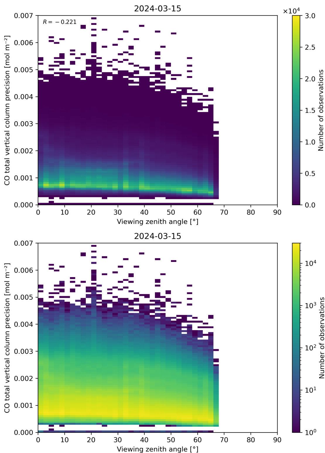
Figure 71: Scatter density plot of “Viewing zenith angle” against “CO total vertical column precision” for 2024-03-14 to 2024-03-16.
