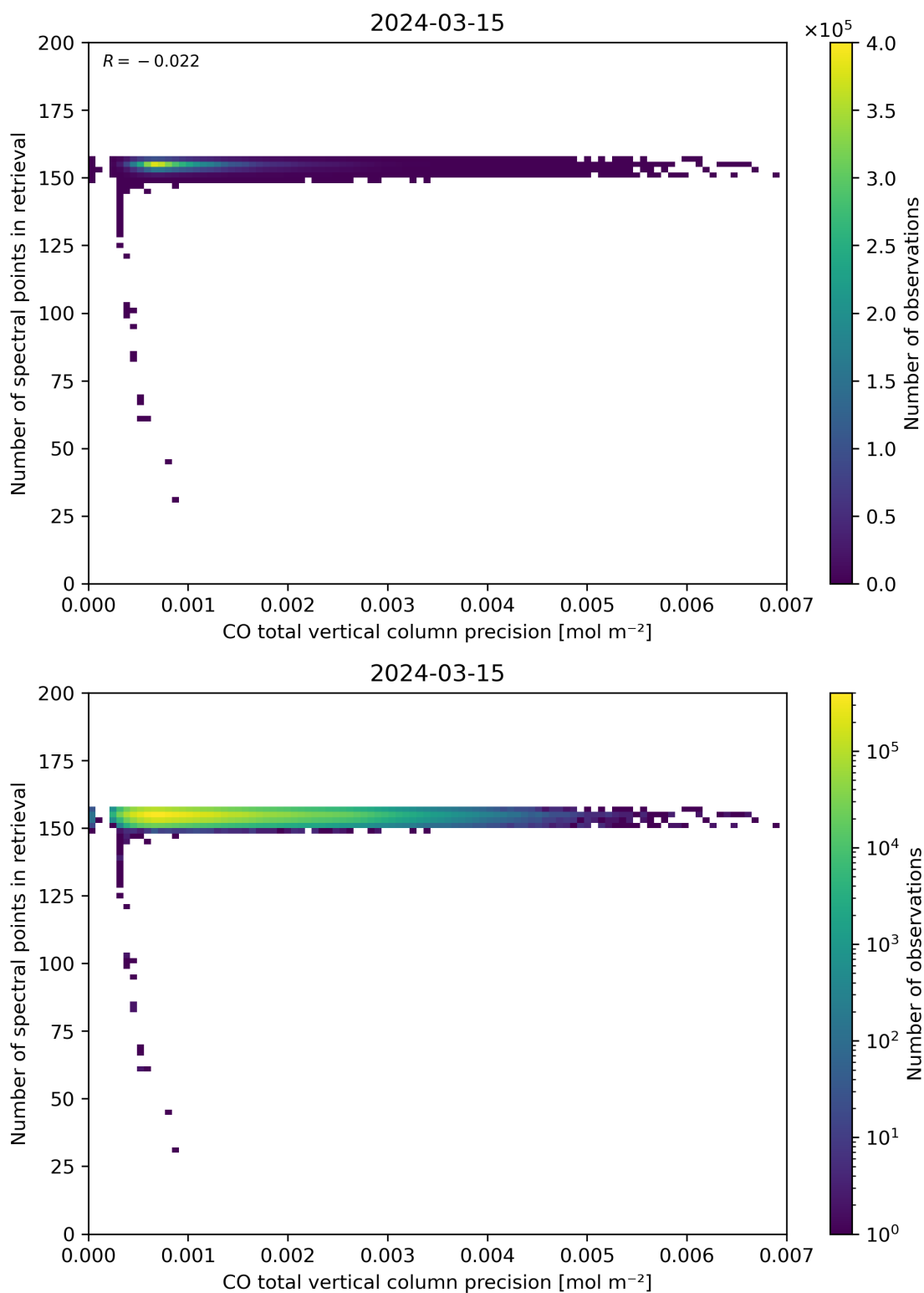
Figure 47: Scatter density plot of “CO total vertical column precision” against “Number of spectral points in retrieval” for 2024-03-14 to 2024-03-16.
