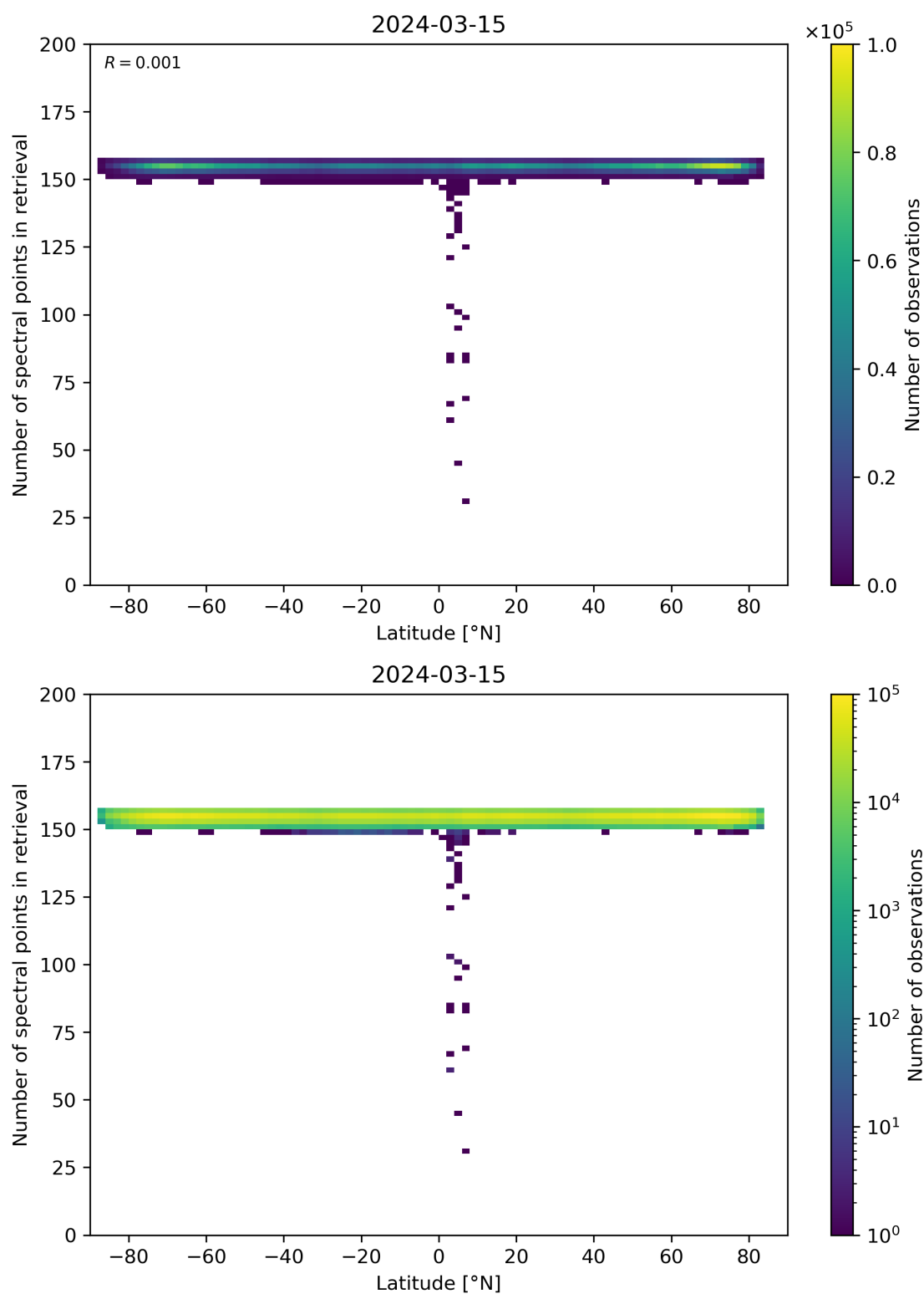
Figure 57: Scatter density plot of “Latitude” against “Number of spectral points in retrieval” for 2024-03-14 to 2024-03-16.
