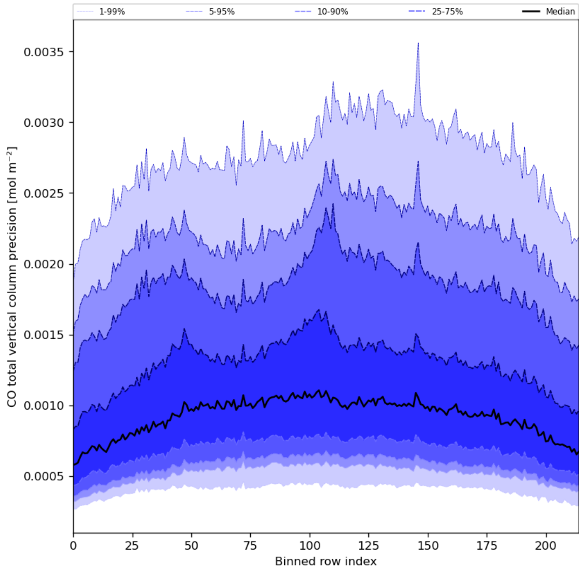
Figure 28: Along track statistics of “CO total vertical column precision” for 2024-03-14 to 2024-03-16
