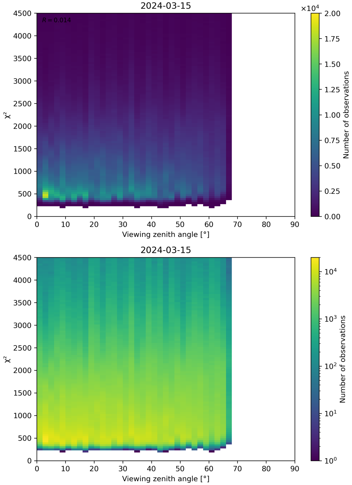
Figure 72: Scatter density plot of “Viewing zenith angle” against “ \chi^2 ” for 2024-03-14 to 2024-03-16.
