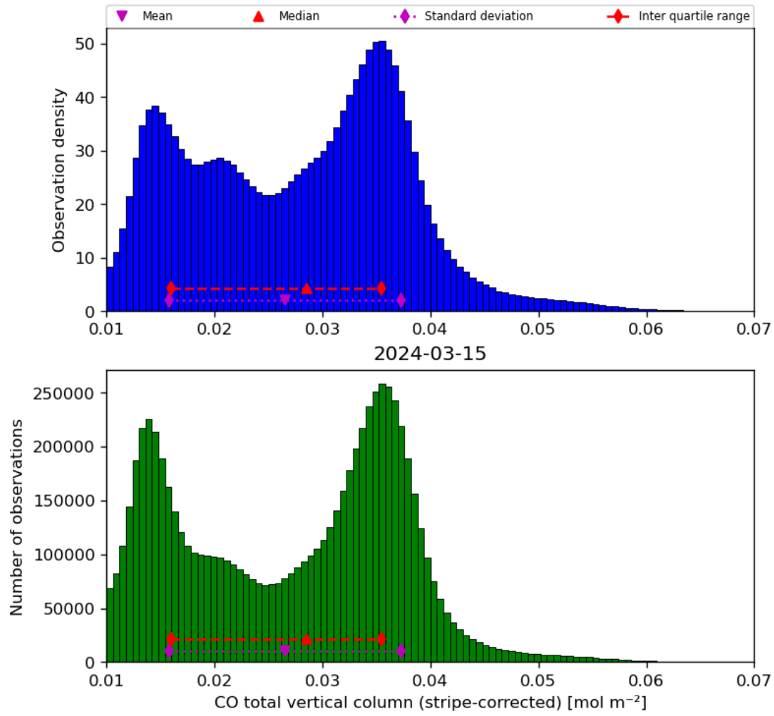
Figure 19: Histogram of “CO total vertical column (stripe-corrected)” for 2024-03-14 to 2024-03-16
