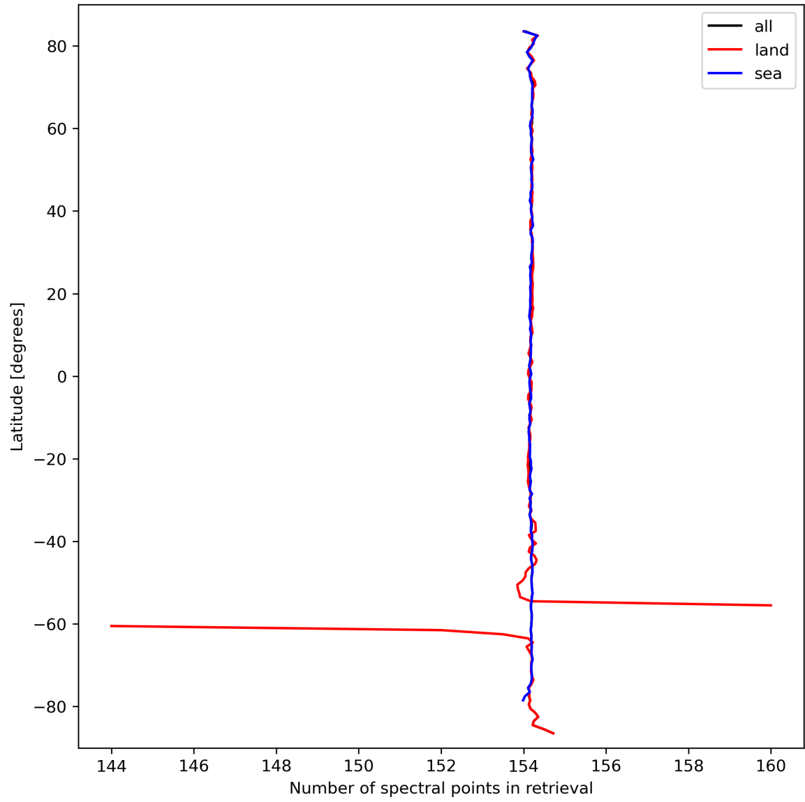
Figure 13: Zonal average of “Number of spectral points in retrieval” for 2024-03-14 to 2024-03-16.
