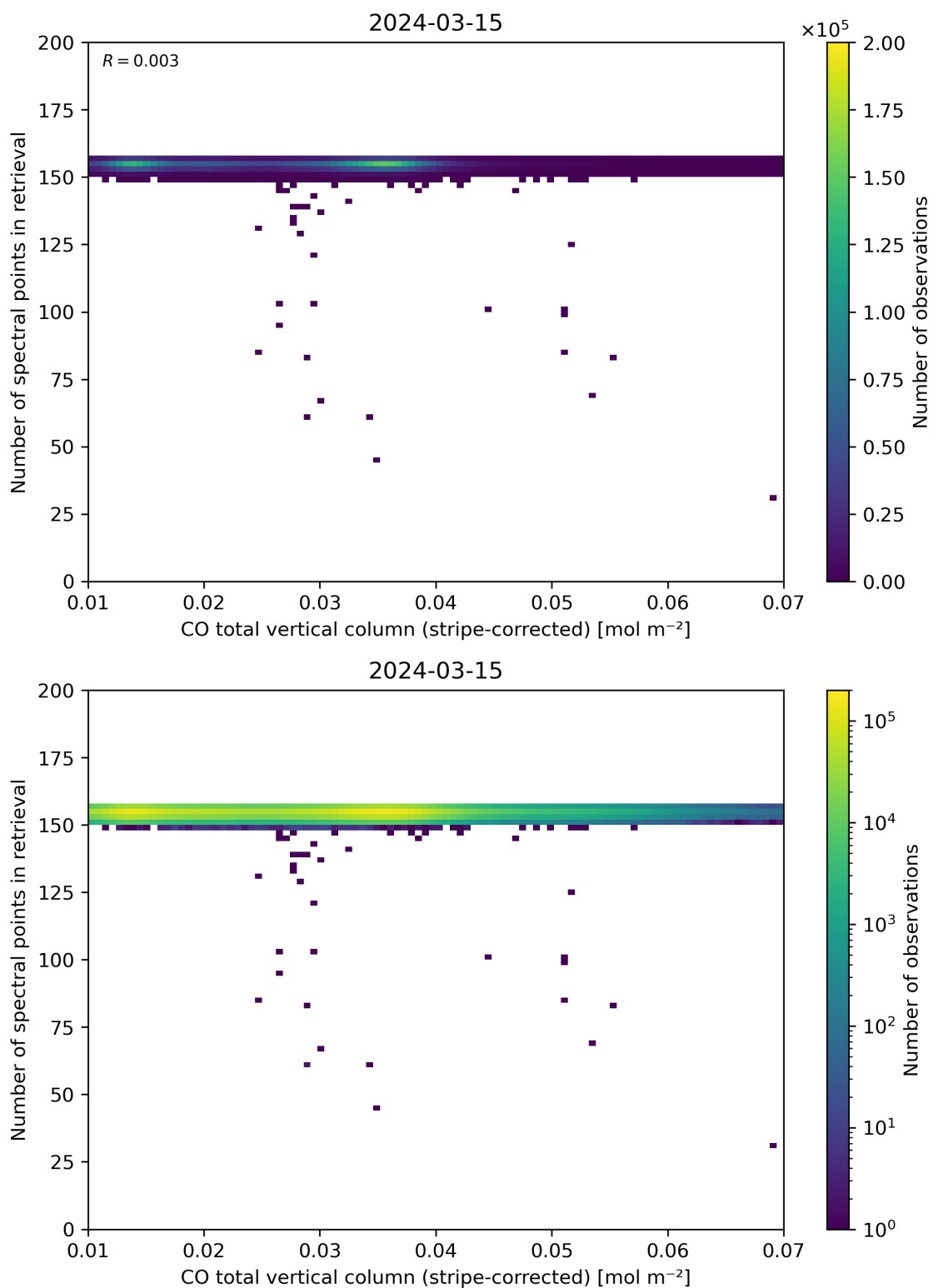
Figure 40: Scatter density plot of “CO total vertical column (stripe-corrected)” against “Number of spectral points in retrieval” for 2024-03-14 to 2024-03-16.
