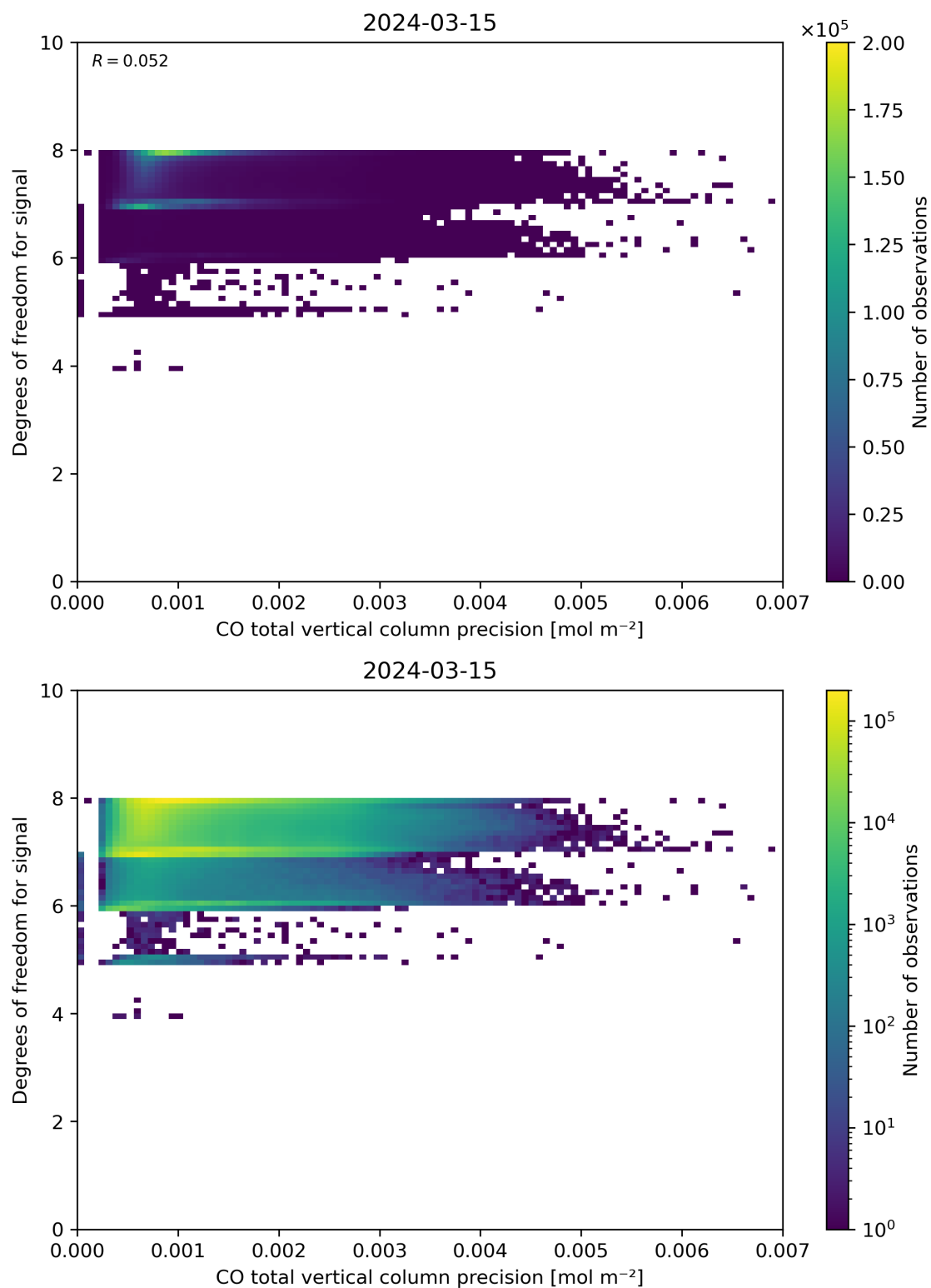
Figure 45: Scatter density plot of “CO total vertical column precision” against “Degrees of freedom for signal” for 2024-03-14 to 2024-03-16.
