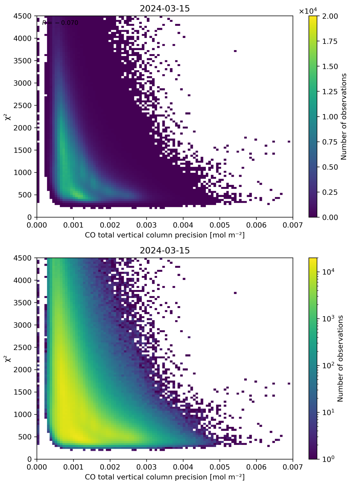
Figure 44: Scatter density plot of “CO total vertical column precision” against “ \chi^2 ” for 2024-03-14 to 2024-03-16.
