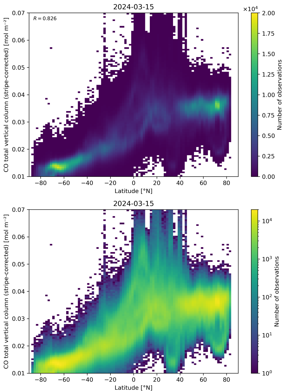
Figure 52: Scatter density plot of “Latitude” against “CO total vertical column (stripe-corrected)” for 2024-03-14 to 2024-03-16.
