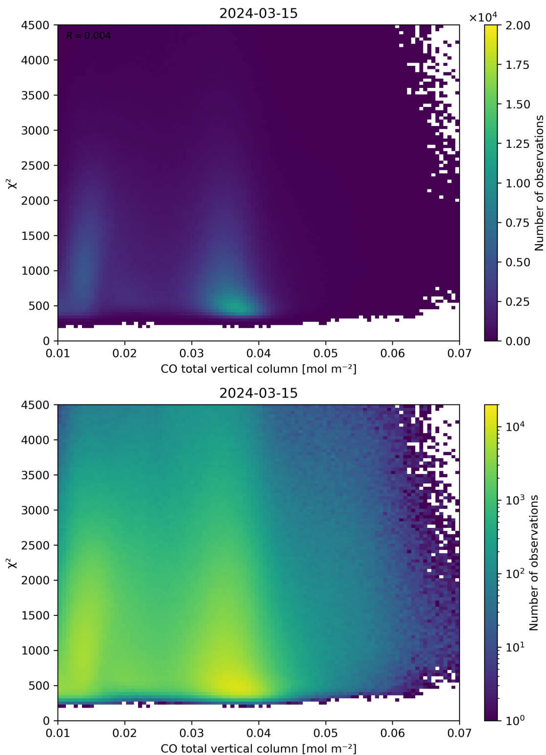
Figure 35: Scatter density plot of “CO total vertical column” against “ \chi^2 ” for 2024-03-14 to 2024-03-16.
