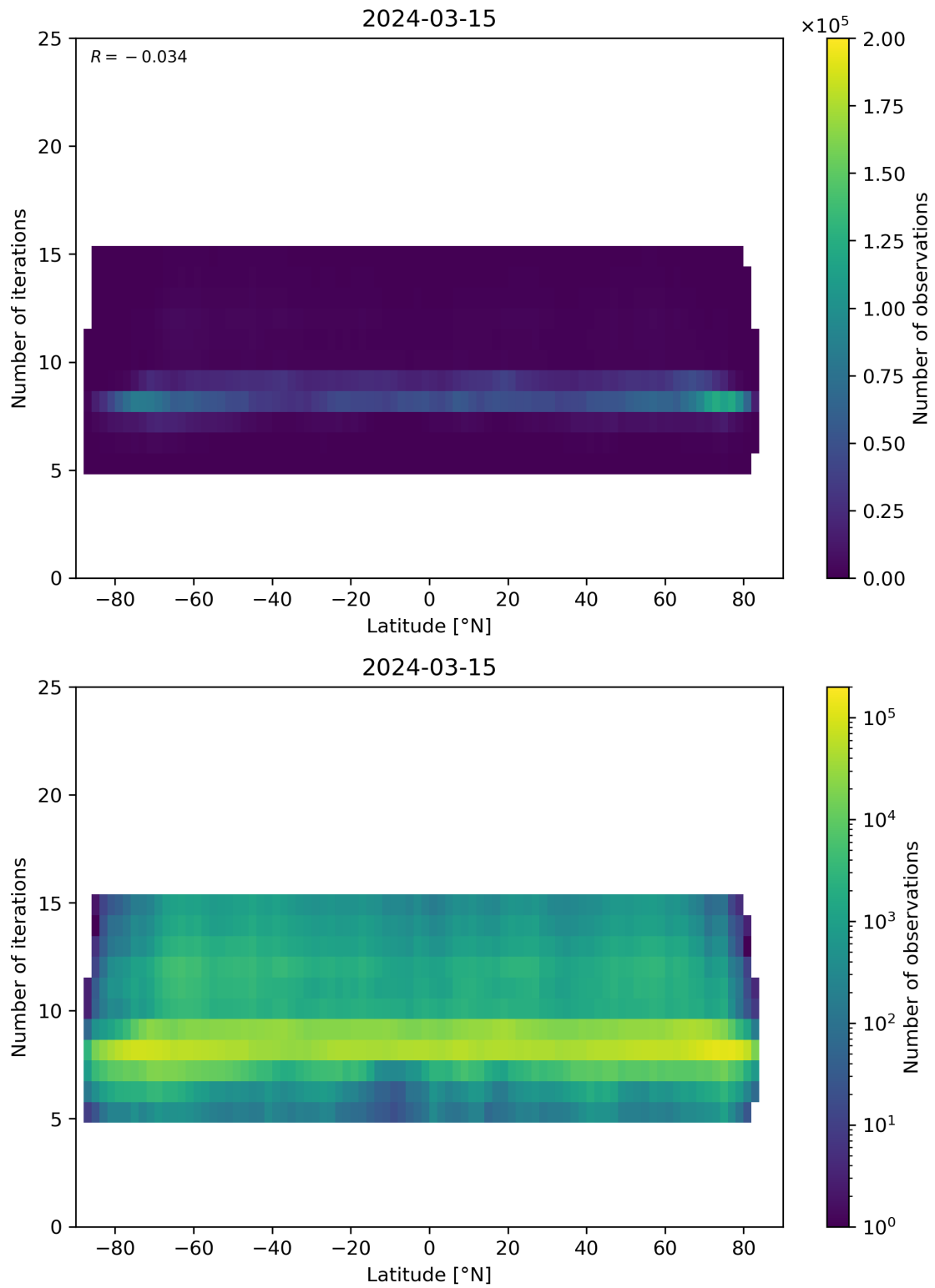
Figure 56: Scatter density plot of “Latitude” against “Number of iterations” for 2024-03-14 to 2024-03-16.
