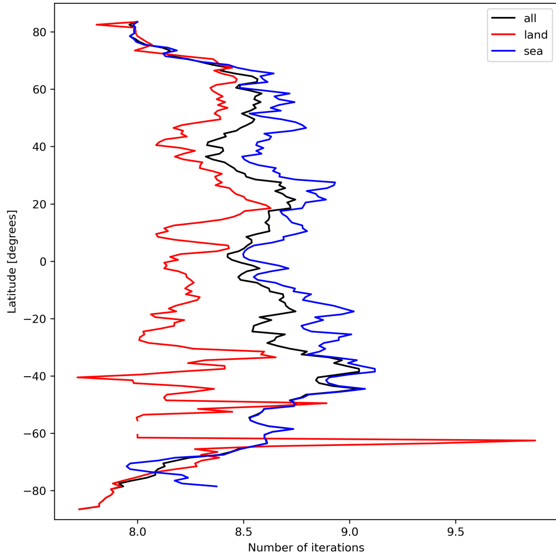
Figure 16: Zonal average of “Number of iterations” for 2024-03-14 to 2024-03-16.
