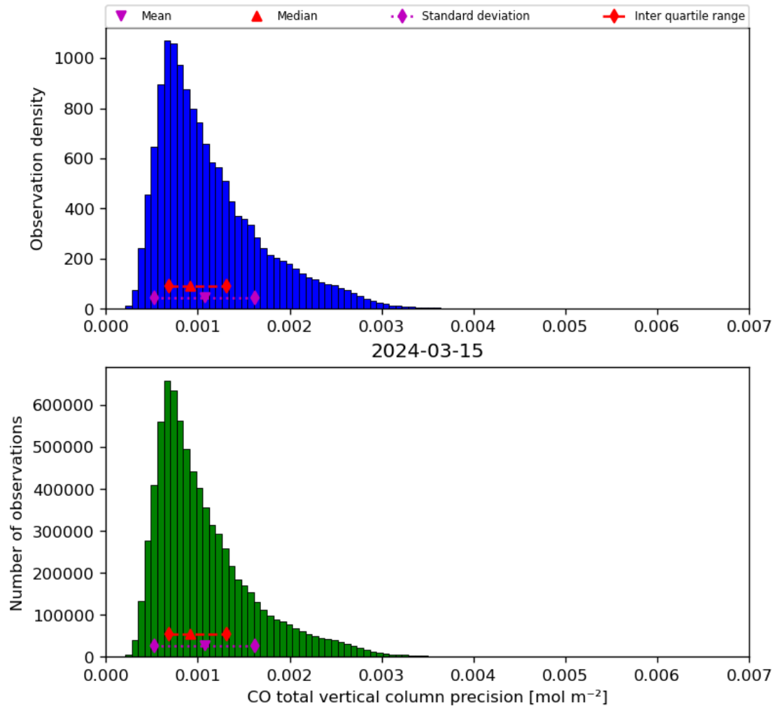
Figure 20: Histogram of “CO total vertical column precision” for 2024-03-14 to 2024-03-16
