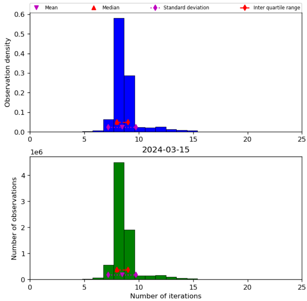
Figure 24: Histogram of “Number of iterations” for 2024-03-14 to 2024-03-16
