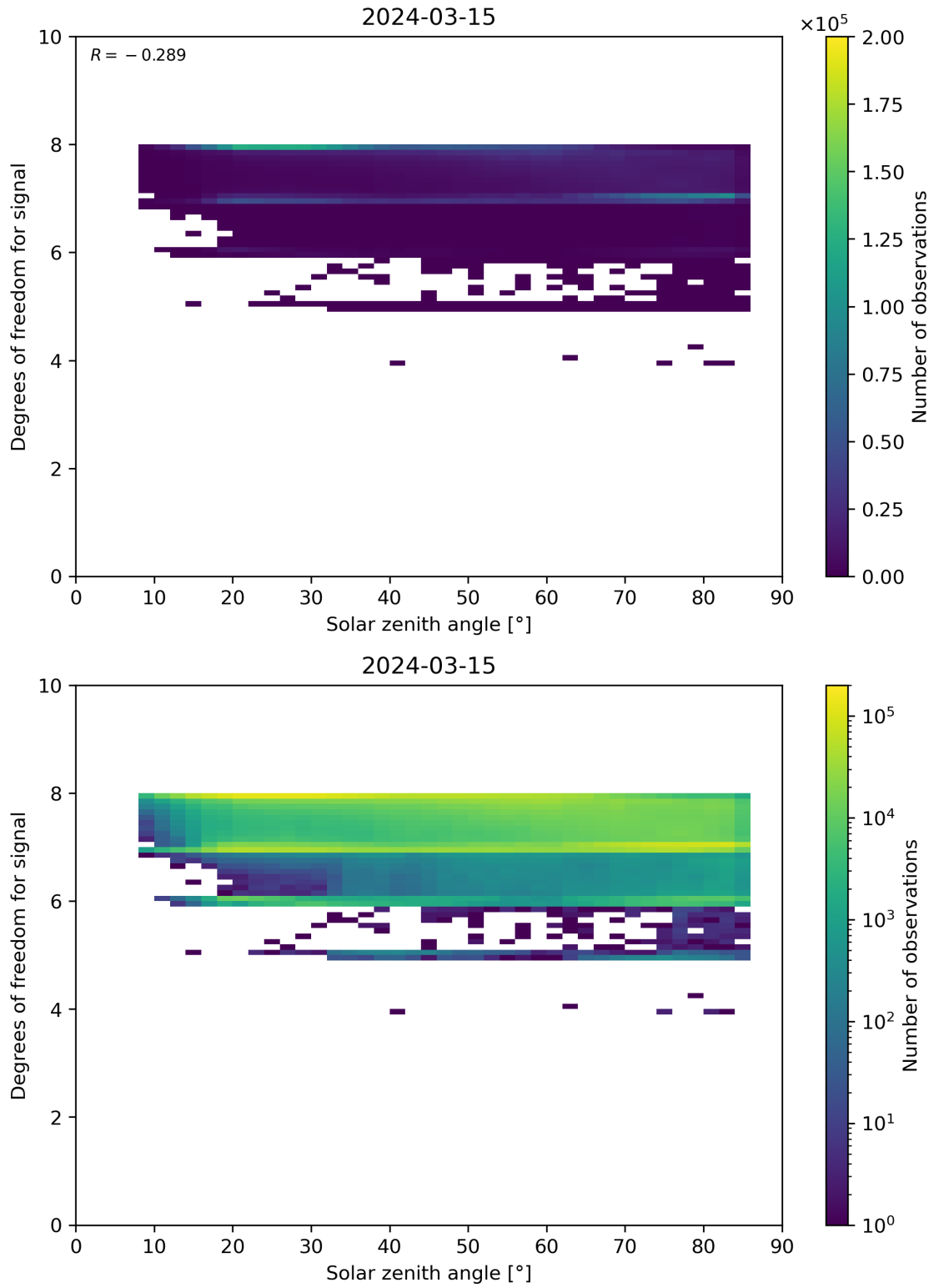
Figure 65: Scatter density plot of “Solar zenith angle” against “Degrees of freedom for signal” for 2024-03-14 to 2024-03-16.
