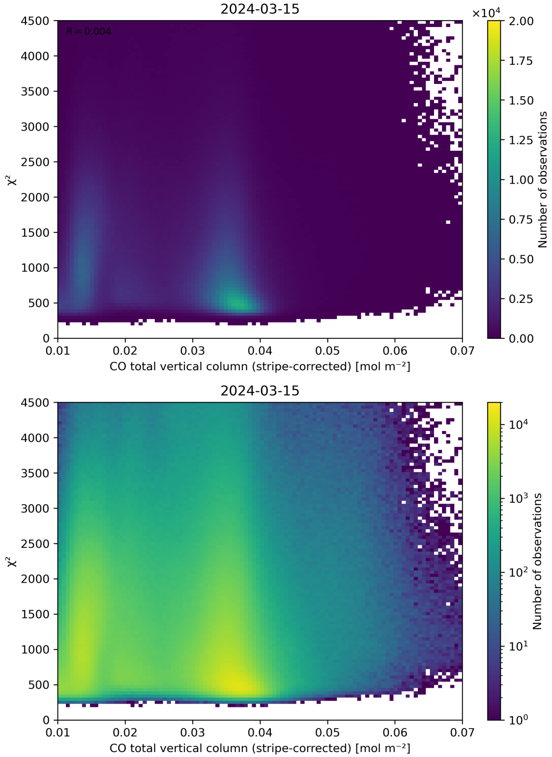
Figure 37: Scatter density plot of “CO total vertical column (stripe-corrected)” against “ \chi^2 ” for 2024-03-14 to 2024-03-16.
