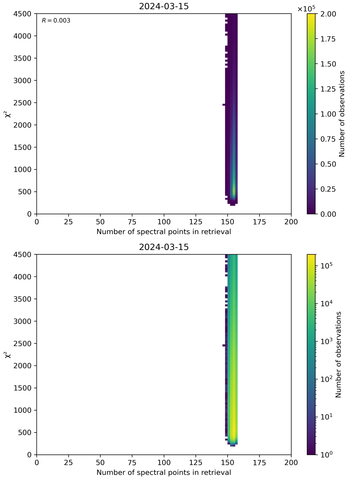
Figure 58: Scatter density plot of “Number of spectral points in retrieval” against “ \chi^2 ” for 2024-03-14 to 2024-03-16.
