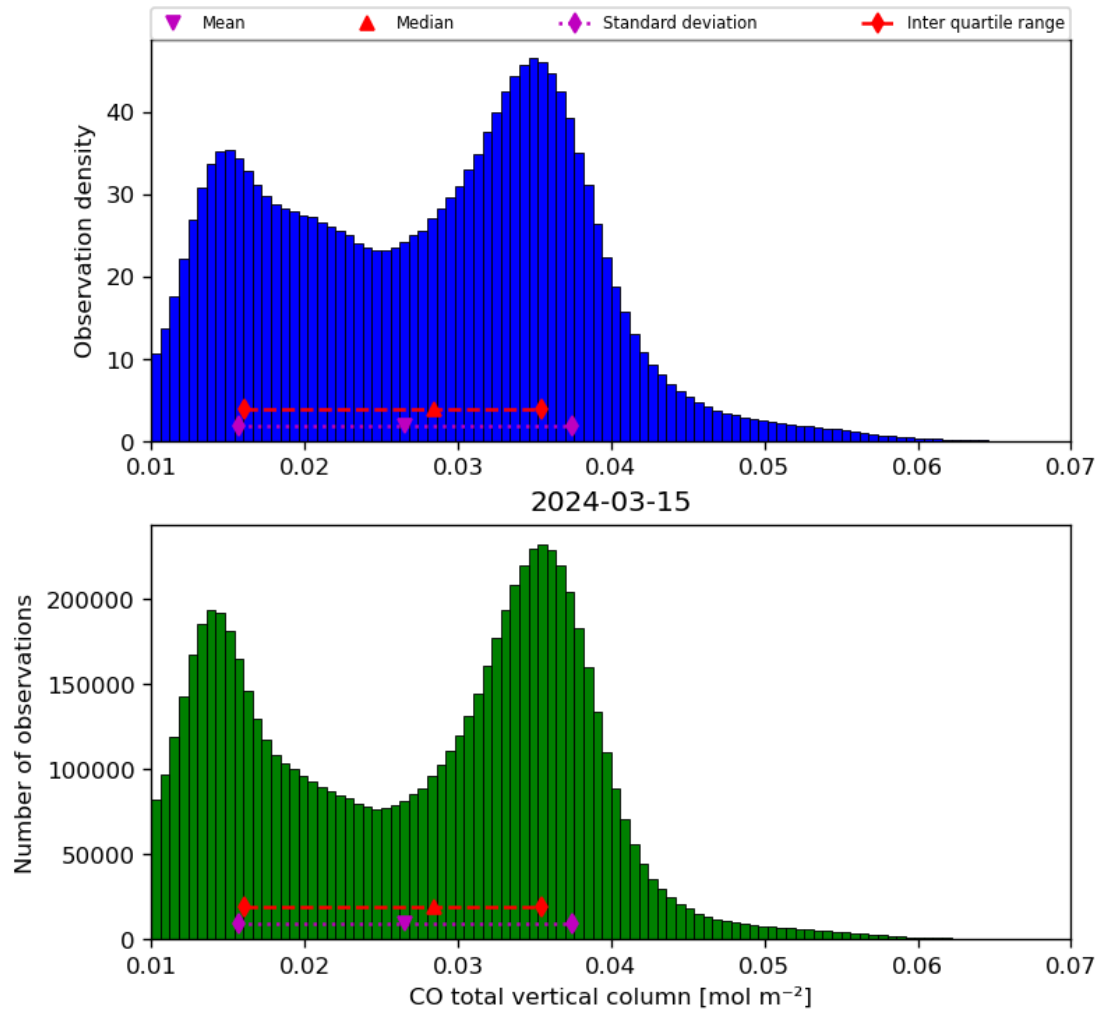
Figure 18: Histogram of “CO total vertical column” for 2024-03-14 to 2024-03-16
