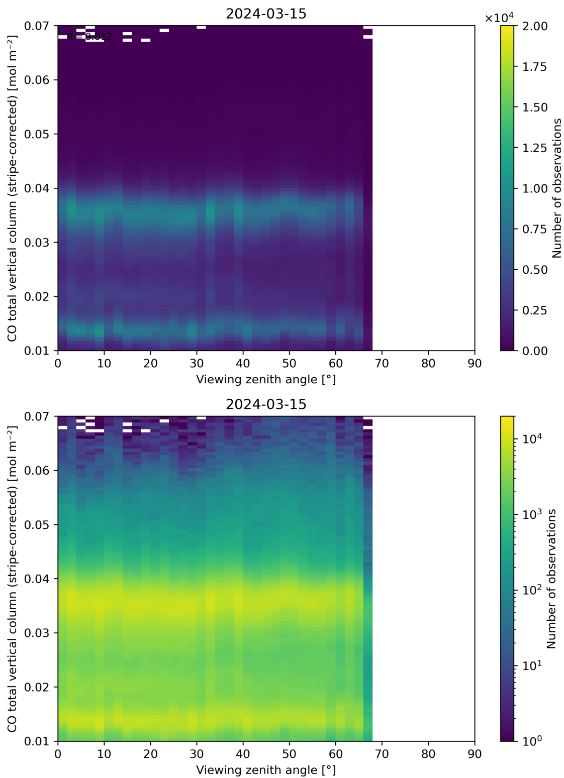
Figure 70: Scatter density plot of “Viewing zenith angle” against “CO total vertical column (stripe-corrected)” for 2024-03-14 to 2024-03-16.
