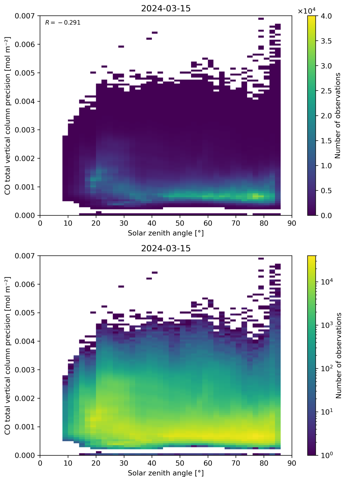
Figure 63: Scatter density plot of “Solar zenith angle” against “CO total vertical column precision” for 2024-03-14 to 2024-03-16.
