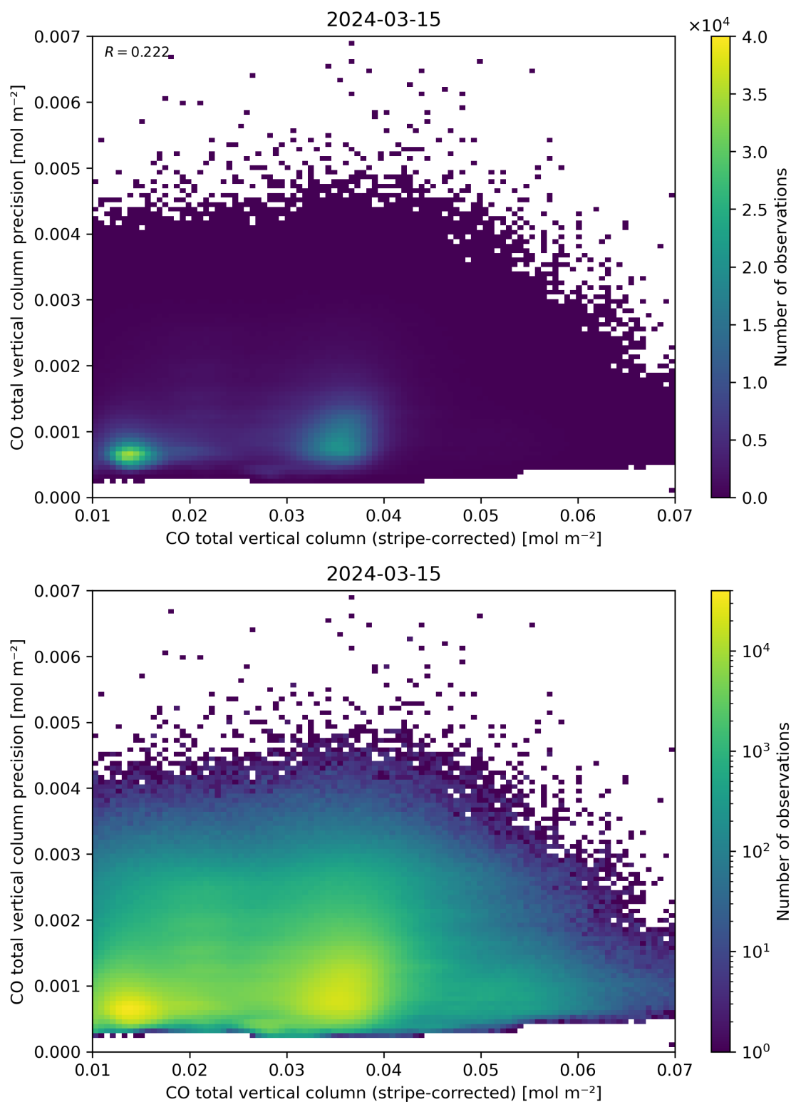
Figure 36: Scatter density plot of “CO total vertical column (stripe-corrected)” against “CO total vertical column precision” for 2024-03-14 to 2024-03-16.
