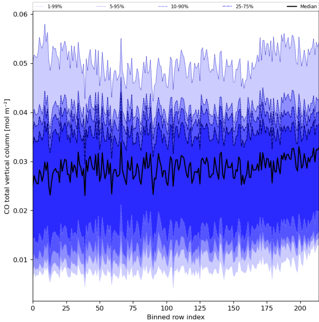
Figure 26: Along track statistics of “CO total vertical column” for 2024-03-14 to 2024-03-16
