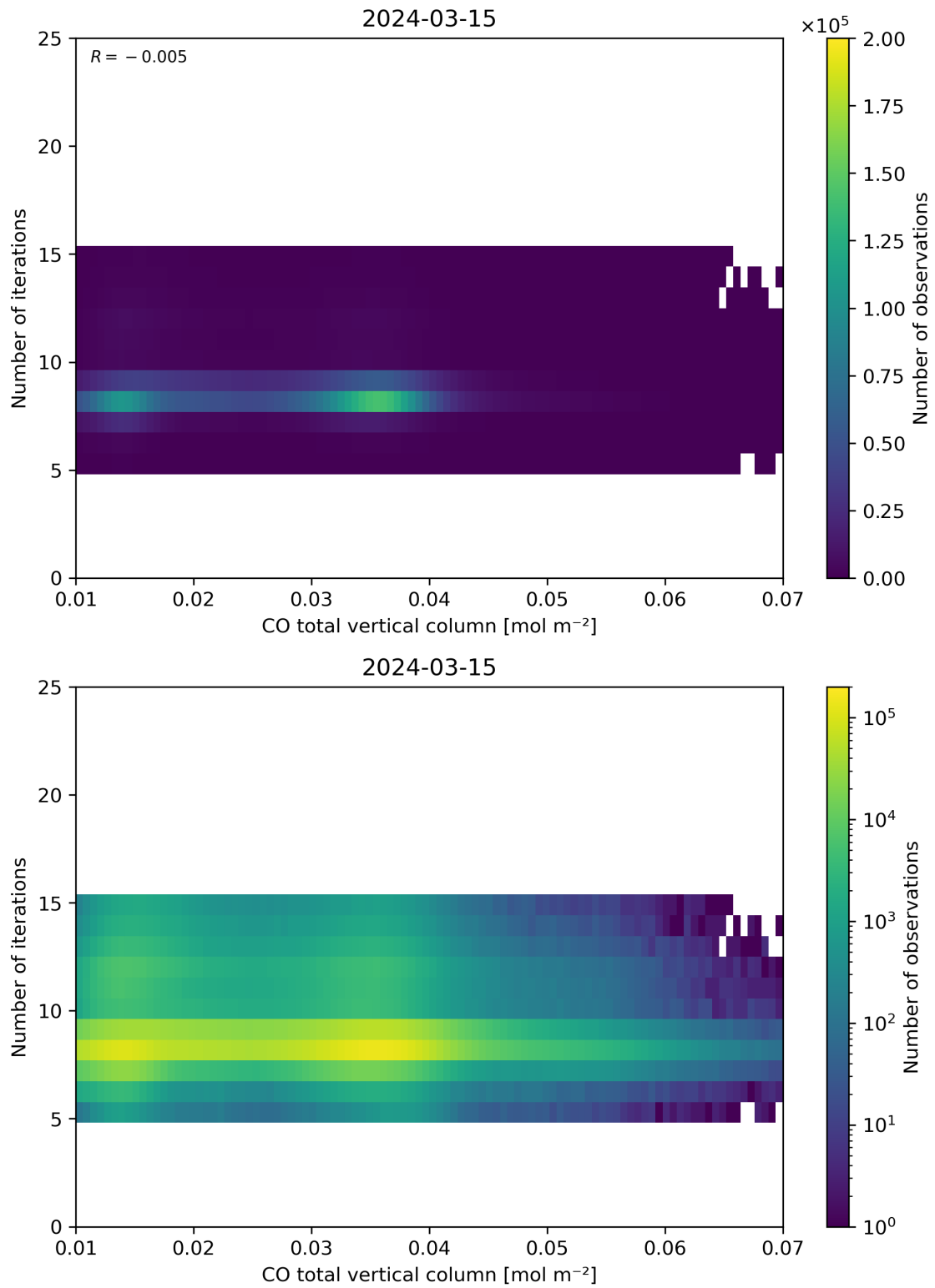
Figure 42: Scatter density plot of “CO total vertical column” against “Number of iterations” for 2024-03-14 to 2024-03-16.
