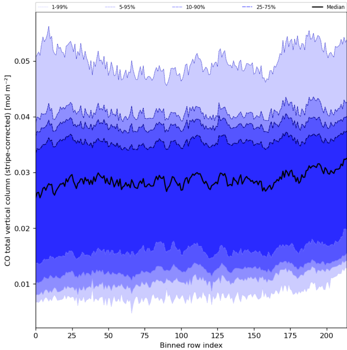
Figure 27: Along track statistics of “CO total vertical column (stripe-corrected)” for 2024-03-14 to 2024-03-16
