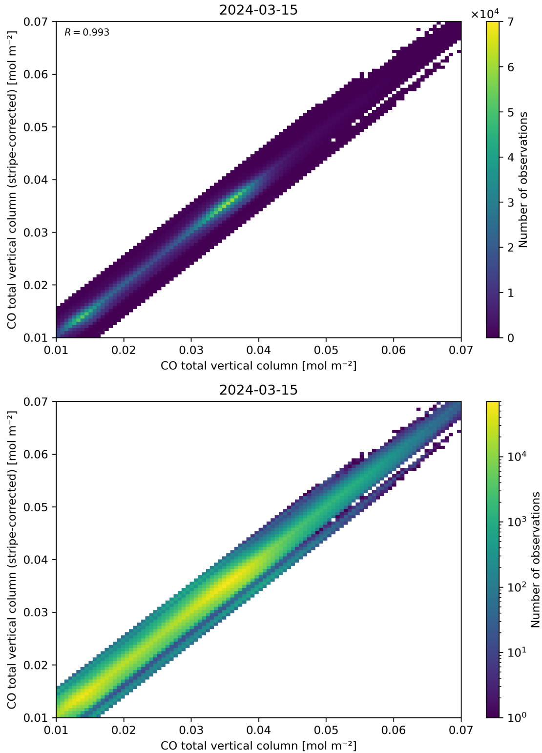
Figure 33: Scatter density plot of “CO total vertical column” against “CO total vertical column (stripe-corrected)” for 2024-03-14 to 2024-03-16.
