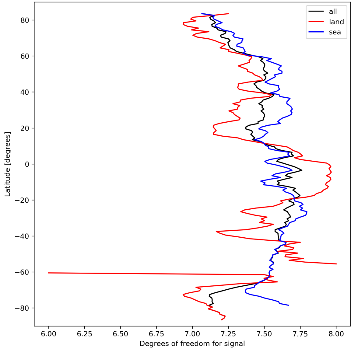
Figure 15: Zonal average of “Degrees of freedom for signal” for 2024-03-14 to 2024-03-16.
