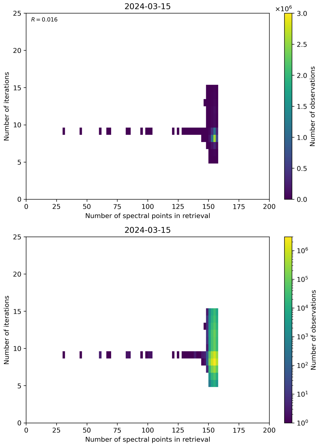
Figure 60: Scatter density plot of “Number of spectral points in retrieval” against “Number of iterations” for 2024-03-14 to 2024-03-16.
