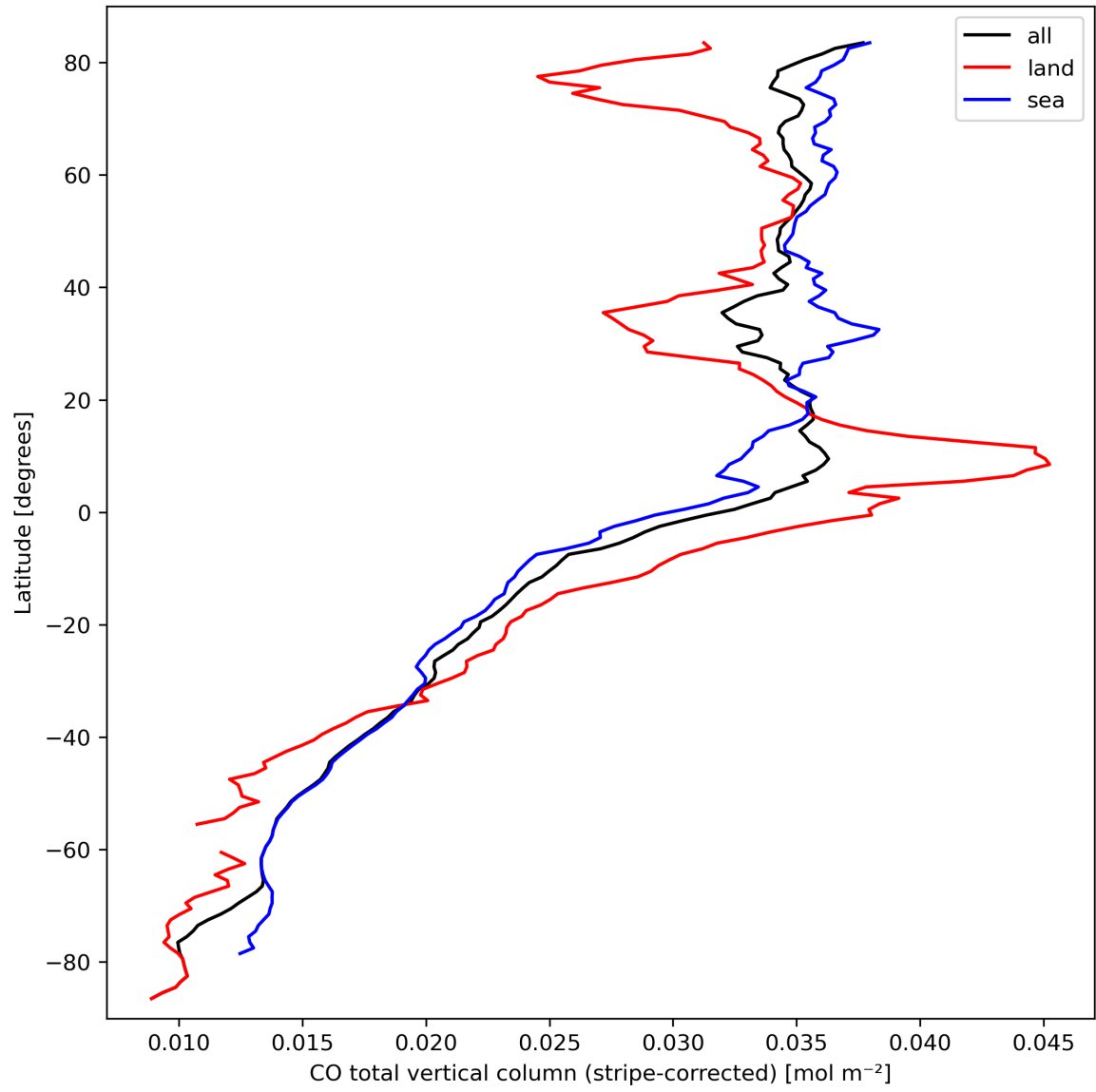
Figure 11: Zonal average of “CO total vertical column (stripe-corrected)” for 2024-03-14 to 2024-03-16.
