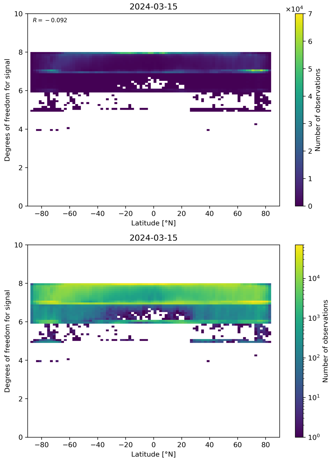
Figure 55: Scatter density plot of “Latitude” against “Degrees of freedom for signal” for 2024-03-14 to 2024-03-16.
