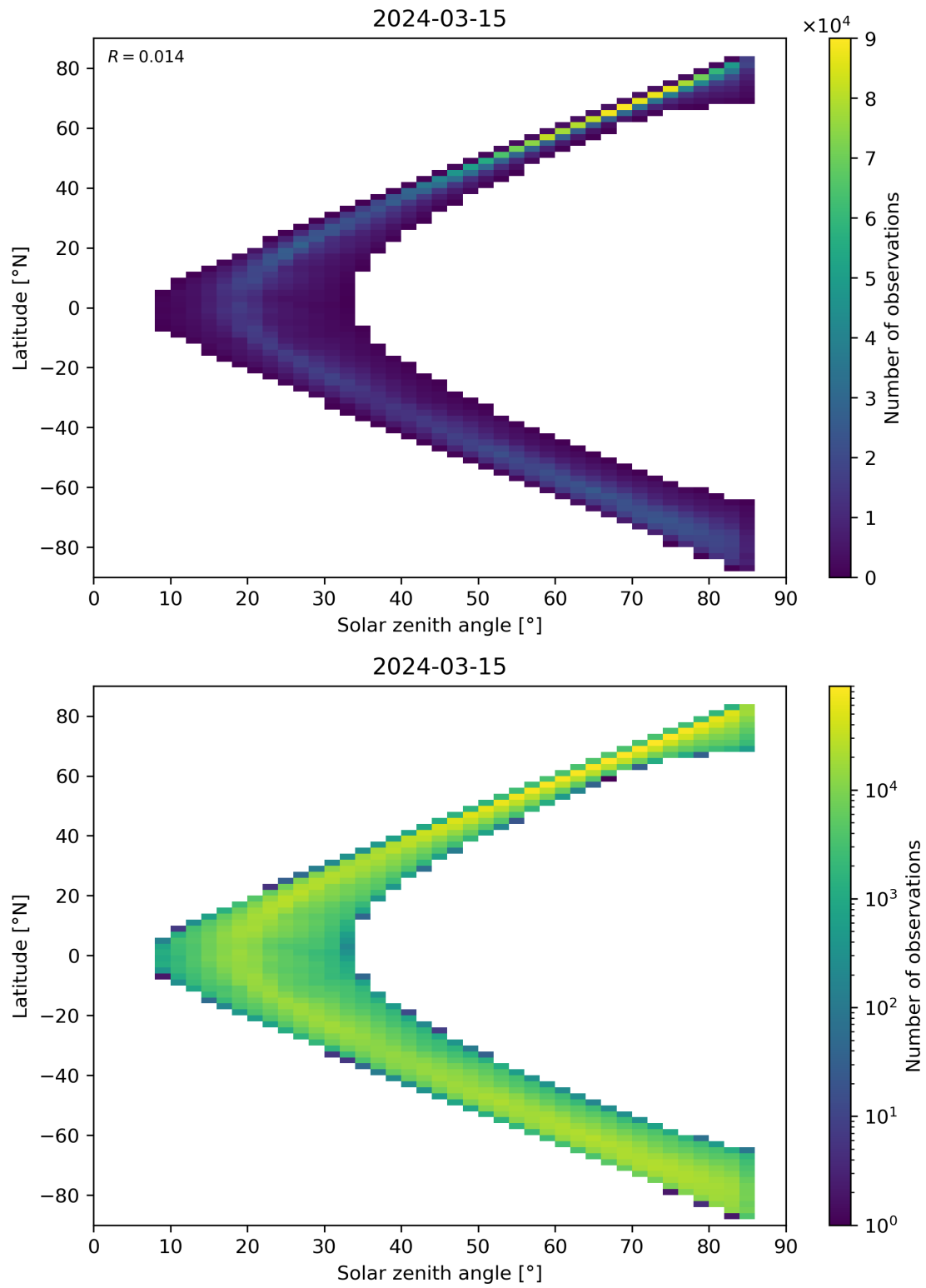
Figure 66: Scatter density plot of “Solar zenith angle” against “Latitude” for 2024-03-14 to 2024-03-16.
