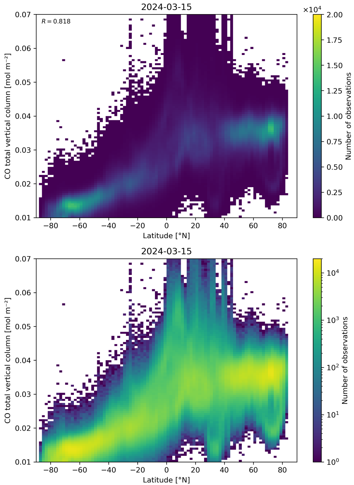
Figure 51: Scatter density plot of “Latitude” against “CO total vertical column” for 2024-03-14 to 2024-03-16.
