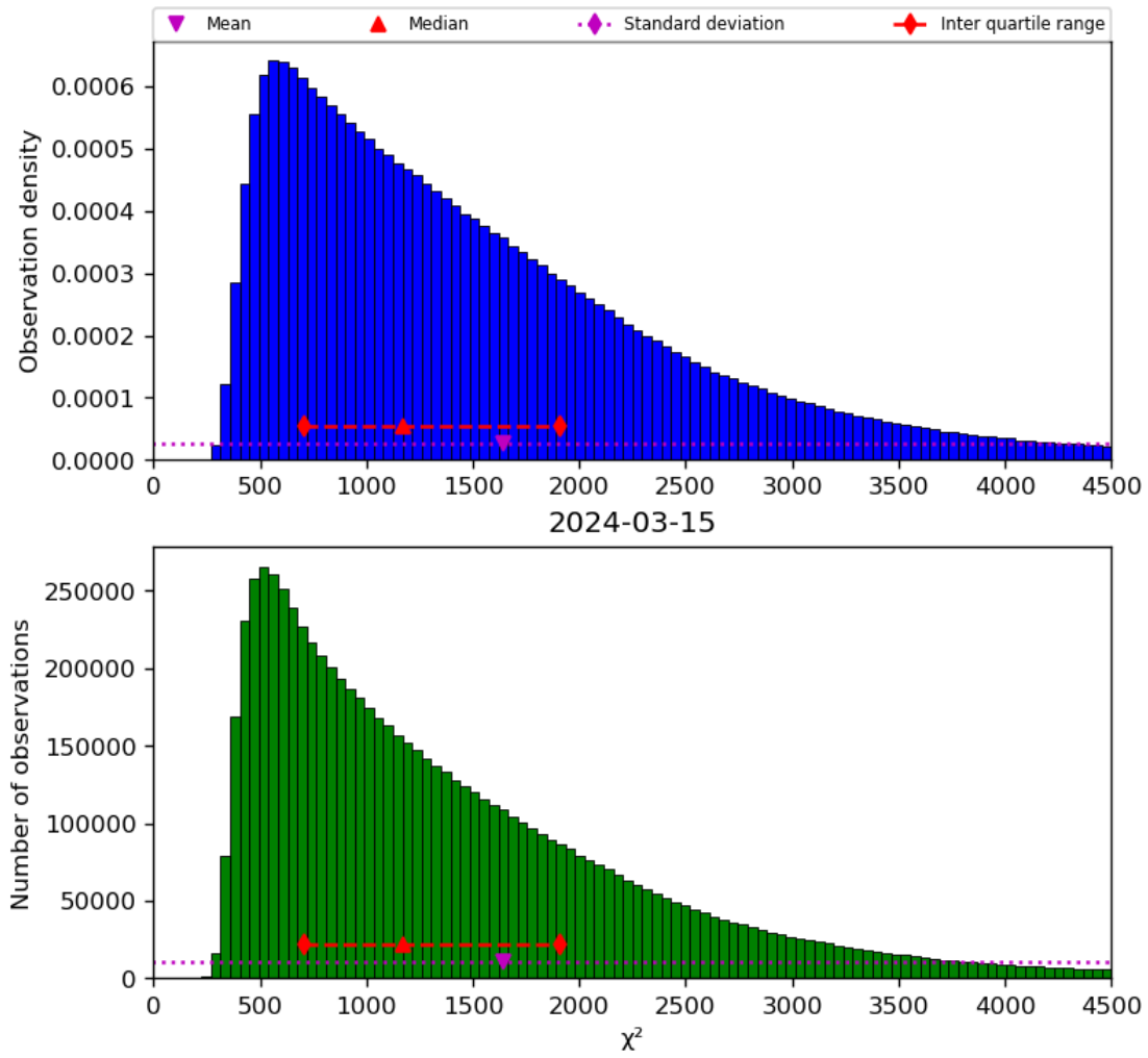
Figure 22: Histogram of “ \chi^2 ” for 2024-03-14 to 2024-03-16
