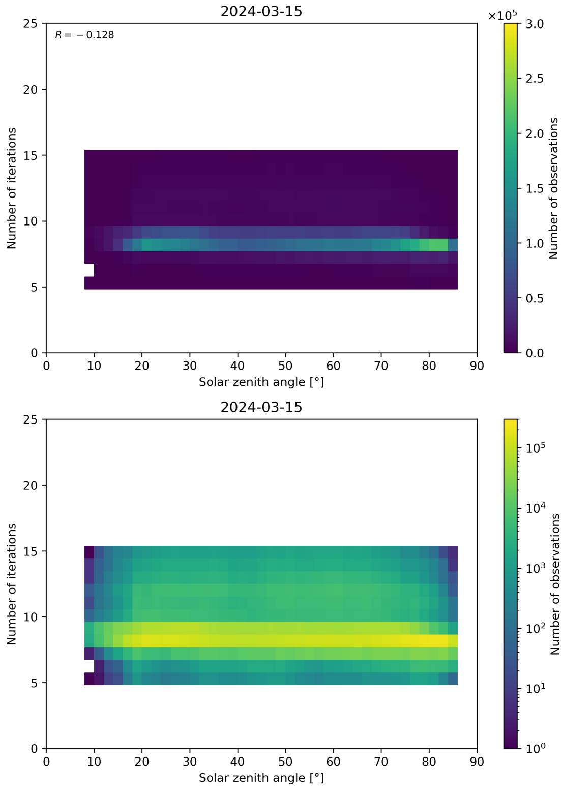
Figure 67: Scatter density plot of “Solar zenith angle” against “Number of iterations” for 2024-03-14 to 2024-03-16.
