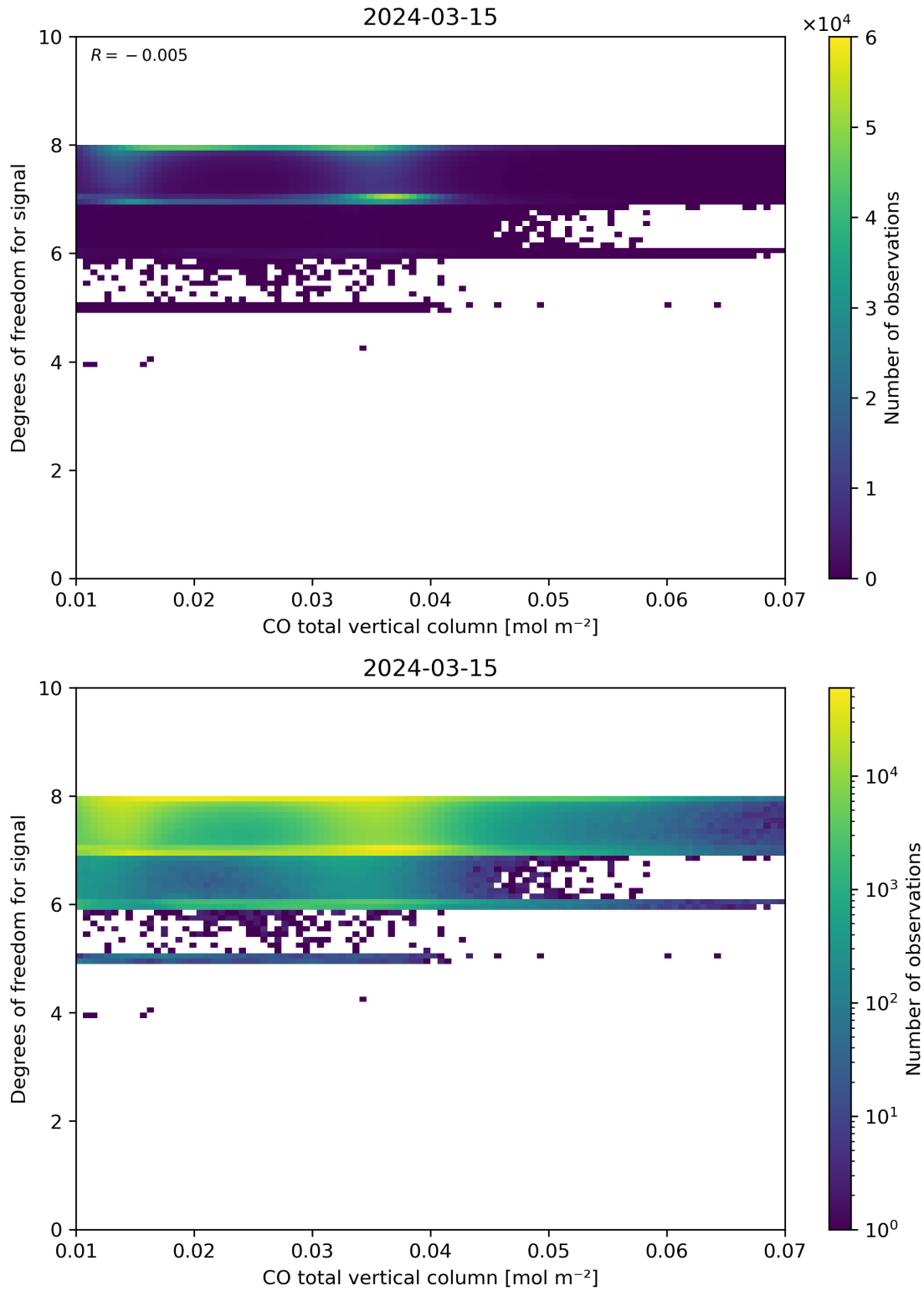
Figure 41: Scatter density plot of “CO total vertical column” against “Degrees of freedom for signal” for 2024-03-14 to 2024-03-16.
