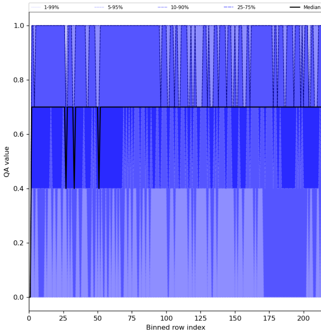
Figure 25: Along track statistics of “QA value” for 2024-03-14 to 2024-03-16
