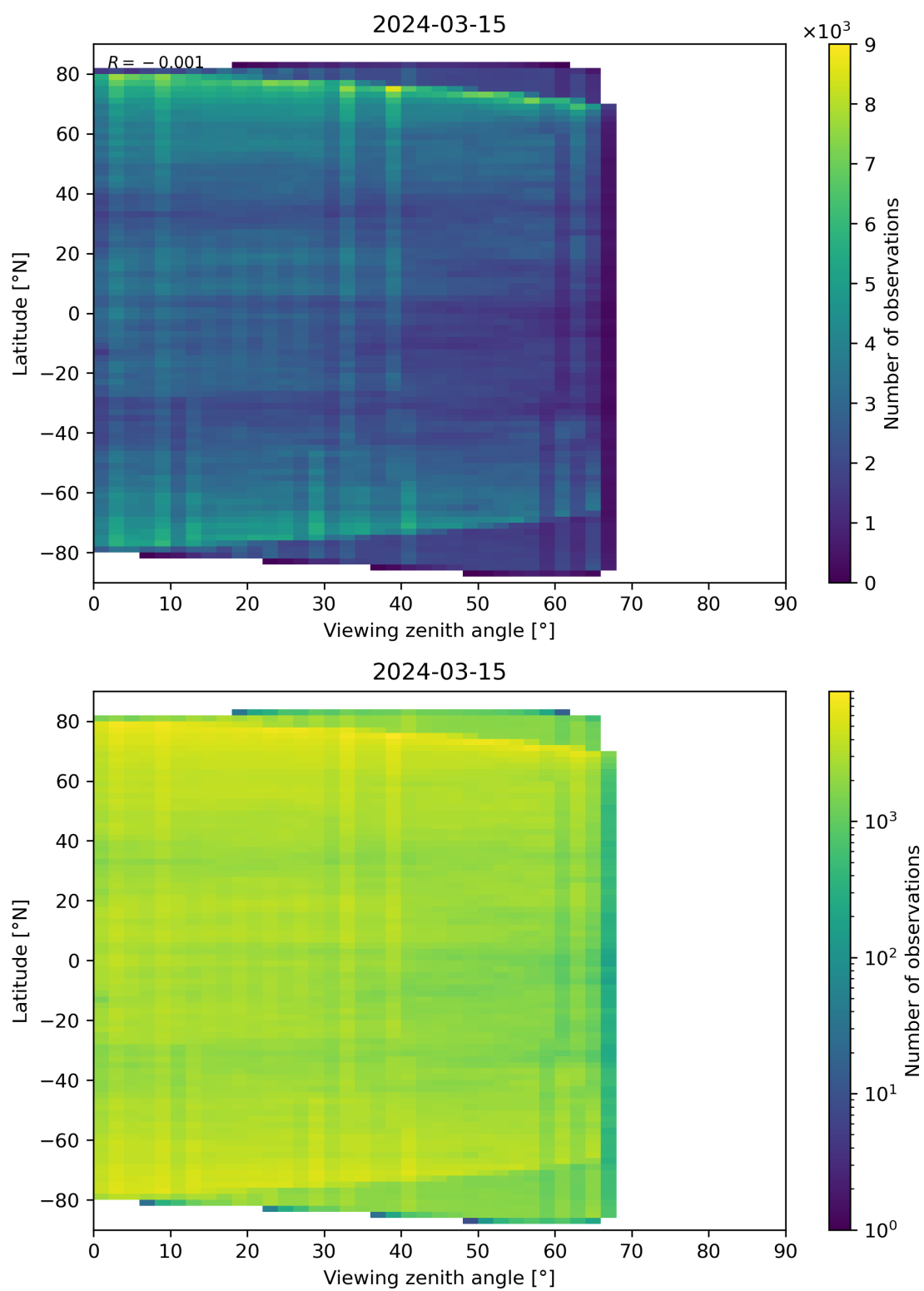
Figure 74: Scatter density plot of “Viewing zenith angle” against “Latitude” for 2024-03-14 to 2024-03-16.
