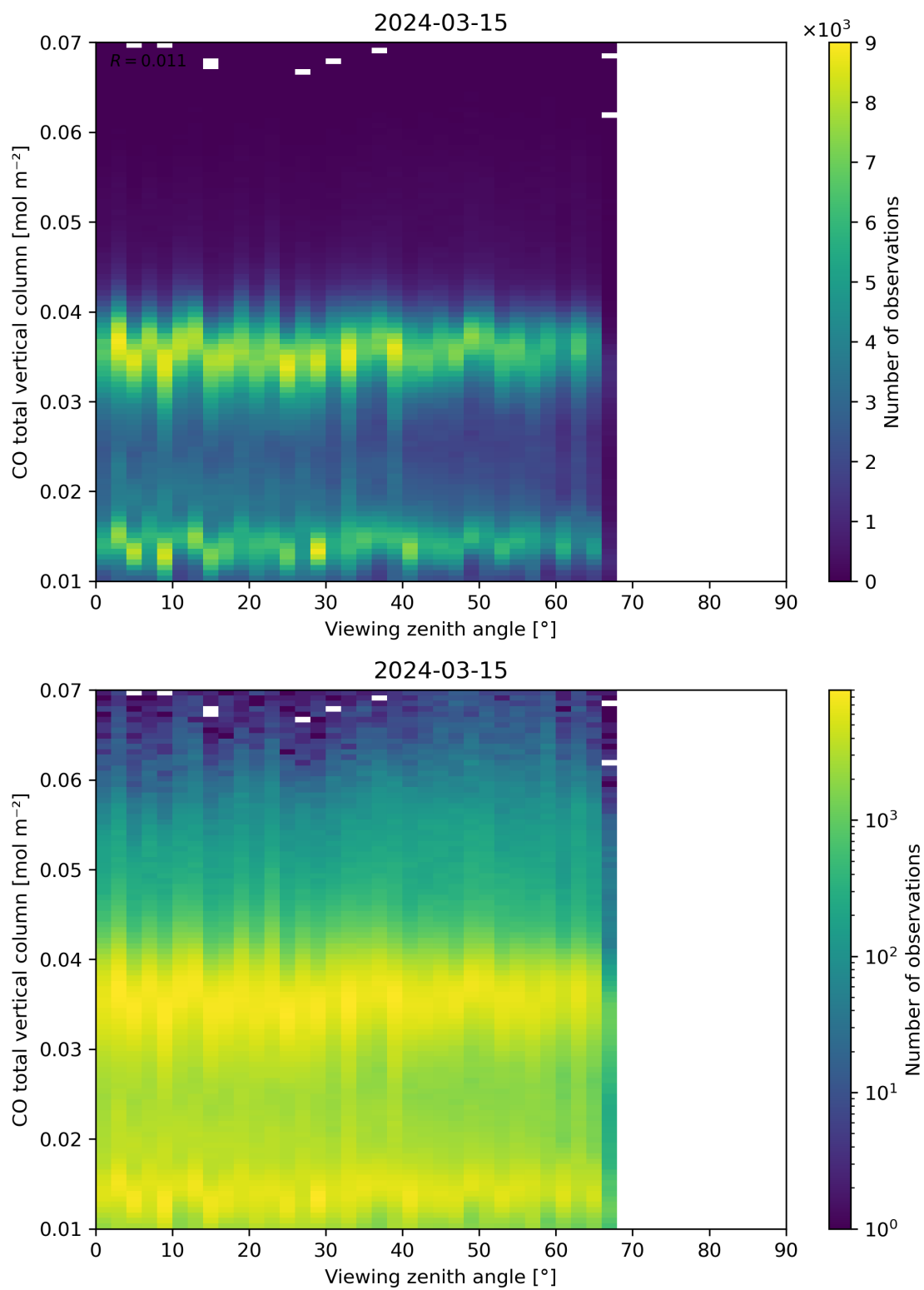
Figure 69: Scatter density plot of “Viewing zenith angle” against “CO total vertical column” for 2024-03-14 to 2024-03-16.
