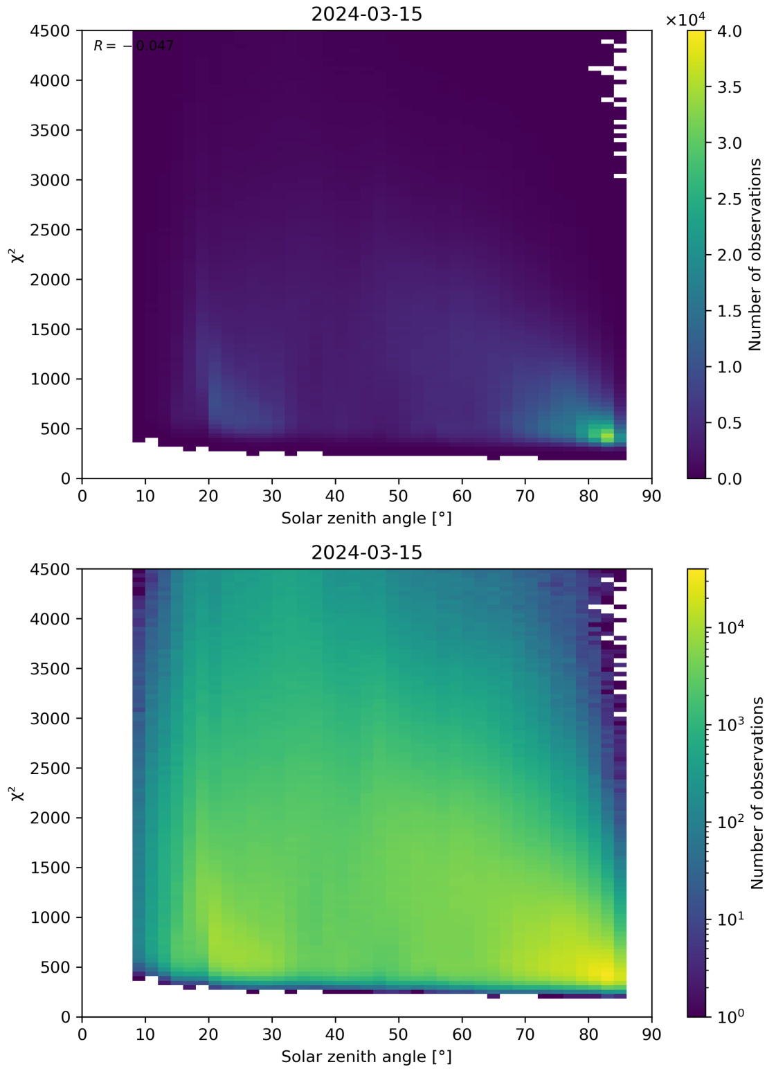
Figure 64: Scatter density plot of “Solar zenith angle” against “ \chi^2 ” for 2024-03-14 to 2024-03-16.
