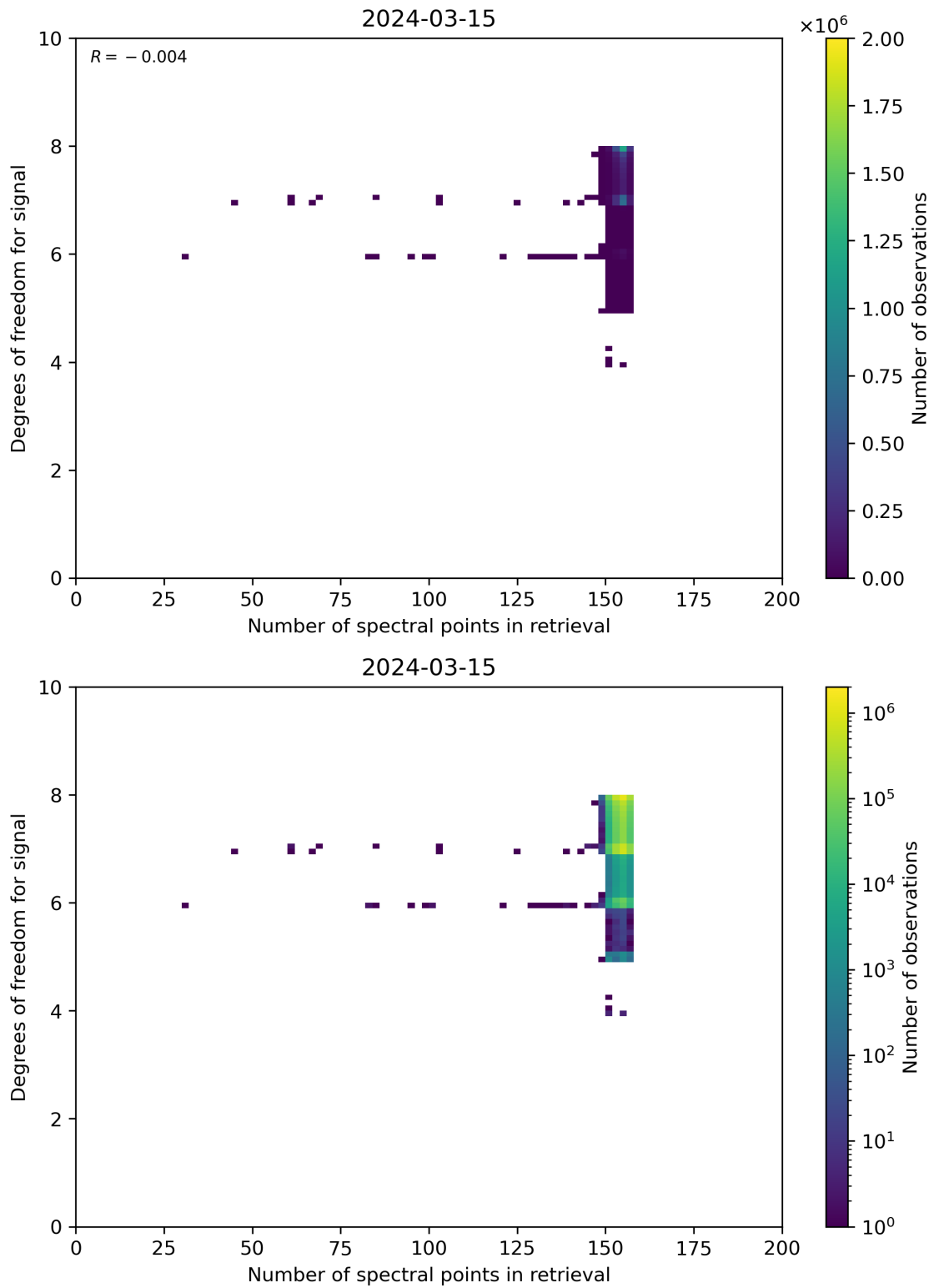
Figure 59: Scatter density plot of “Number of spectral points in retrieval” against “Degrees of freedom for signal” for 2024-03-14 to 2024-03-16.
