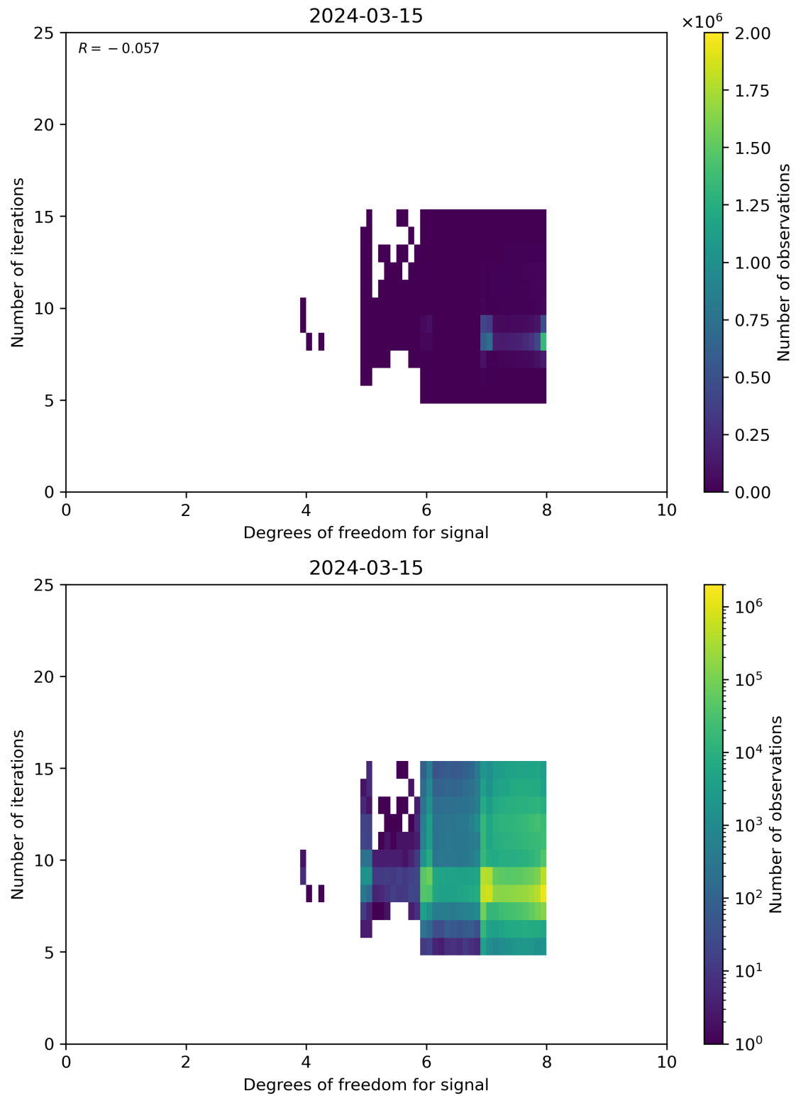
Figure 50: Scatter density plot of “Degrees of freedom for signal” against “Number of iterations” for 2024-03-14 to 2024-03-16.
