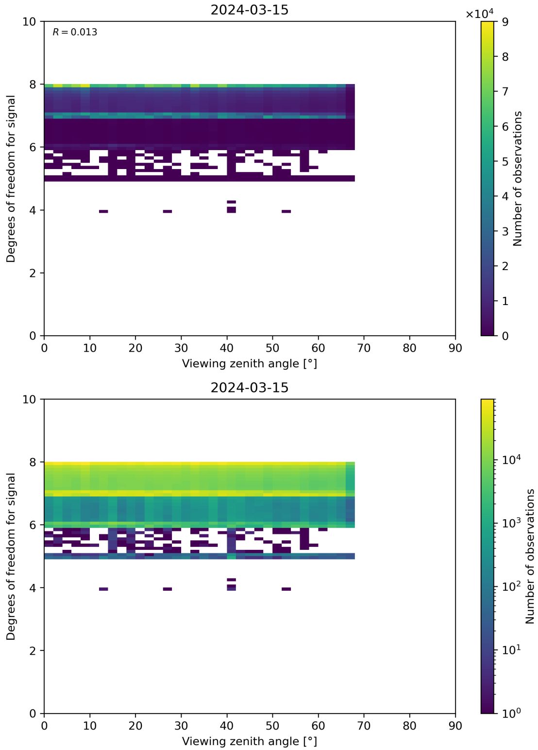
Figure 73: Scatter density plot of “Viewing zenith angle” against “Degrees of freedom for signal” for 2024-03-14 to 2024-03-16.
