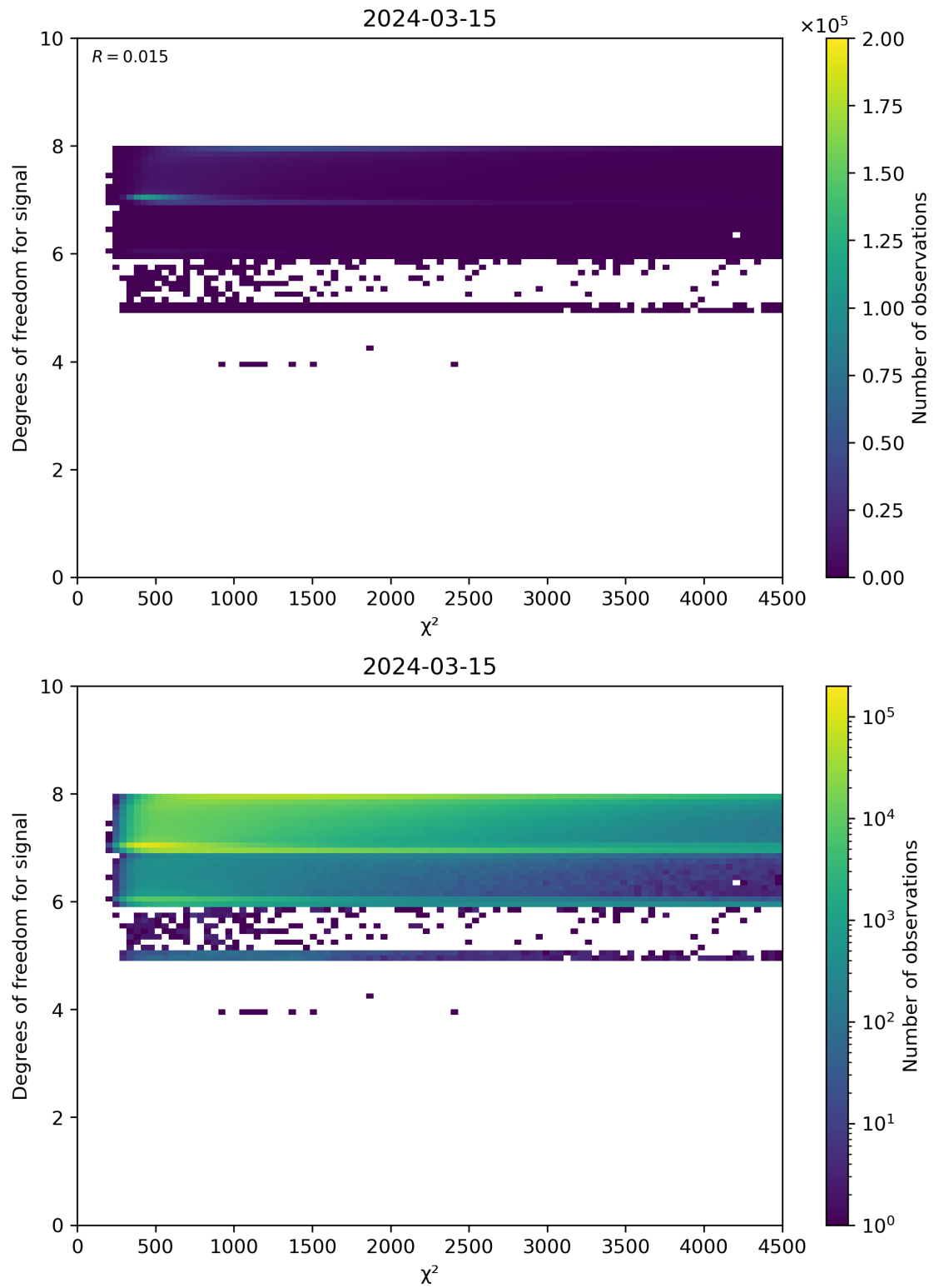
Figure 48: Scatter density plot of “ \chi^2 ” against “Degrees of freedom for signal” for 2024-03-14 to 2024-03-16.
