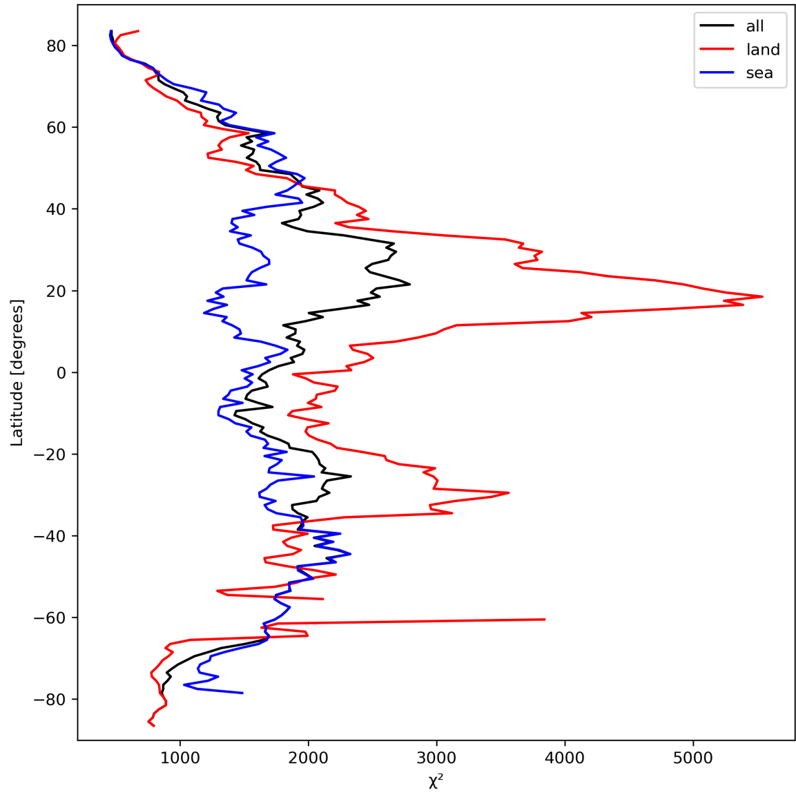
Figure 14: Zonal average of “ \chi^2 ” for 2024-03-14 to 2024-03-16.
