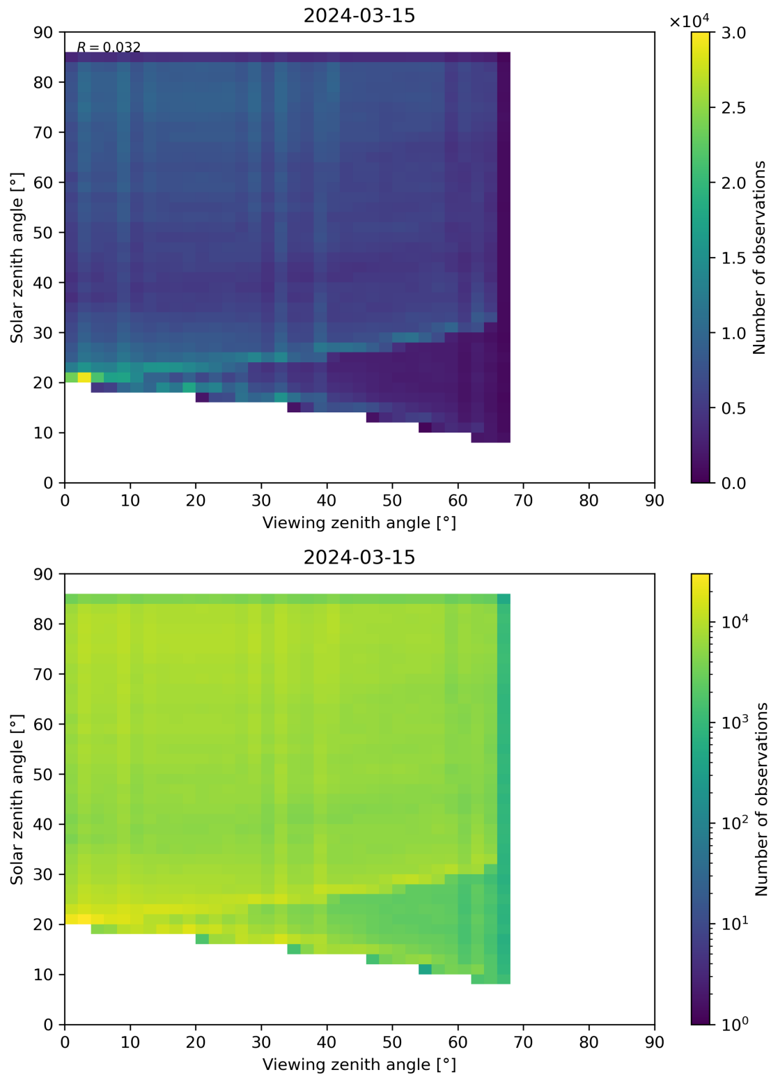
Figure 77: Scatter density plot of “Viewing zenith angle” against “Solar zenith angle” for 2024-03-14 to 2024-03-16.
