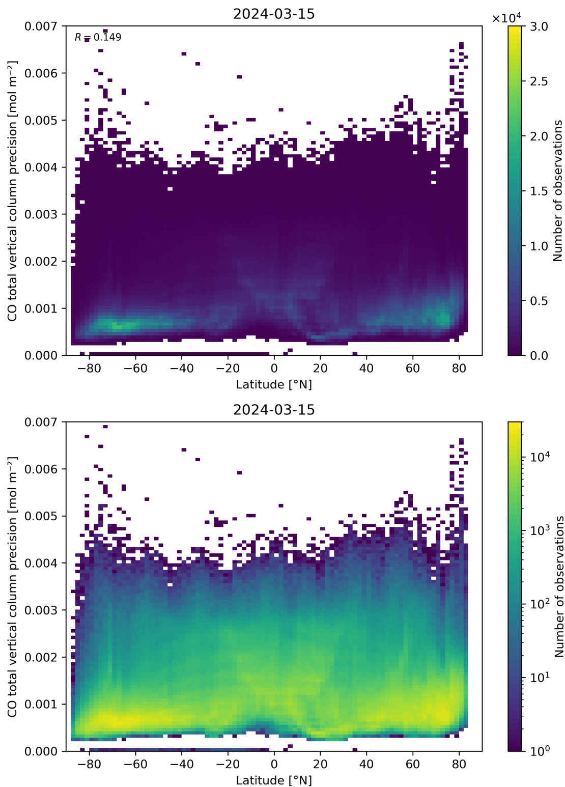
Figure 53: Scatter density plot of “Latitude” against “CO total vertical column precision” for 2024-03-14 to 2024-03-16.
