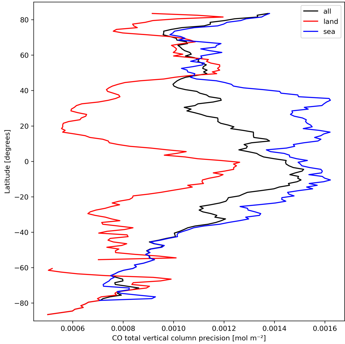
Figure 12: Zonal average of “CO total vertical column precision” for 2024-03-14 to 2024-03-16.
