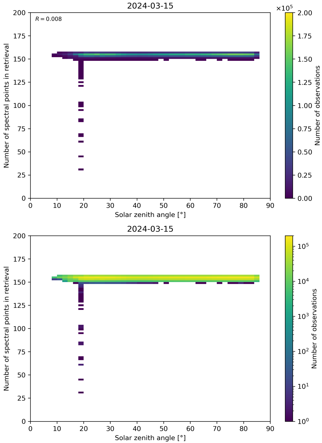
Figure 68: Scatter density plot of “Solar zenith angle” against “Number of spectral points in retrieval” for 2024-03-14 to 2024-03-16.
