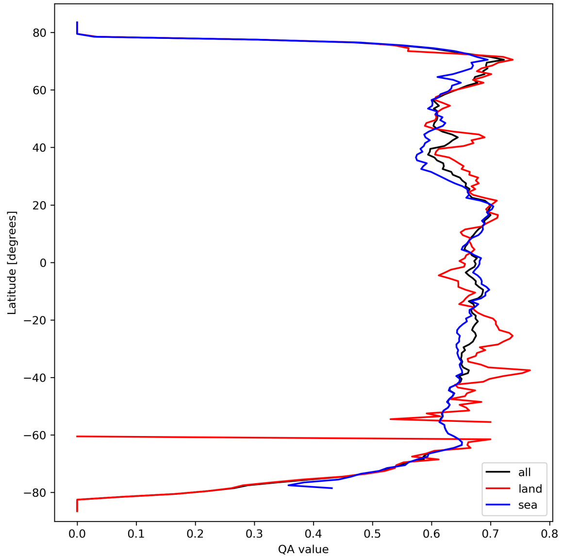
Figure 9: Zonal average of “QA value” for 2024-03-14 to 2024-03-16.
