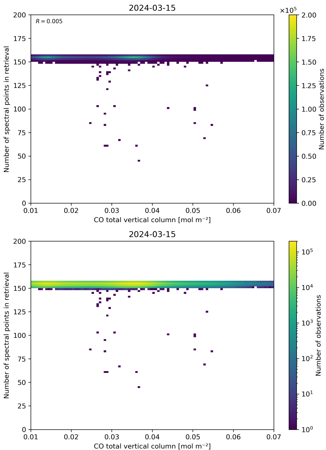
Figure 43: Scatter density plot of “CO total vertical column” against “Number of spectral points in retrieval” for 2024-03-14 to 2024-03-16.
