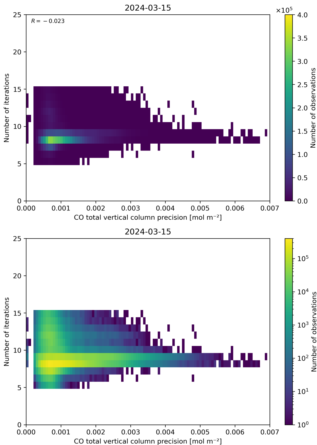
Figure 46: Scatter density plot of “CO total vertical column precision” against “Number of iterations” for 2024-03-14 to 2024-03-16.
