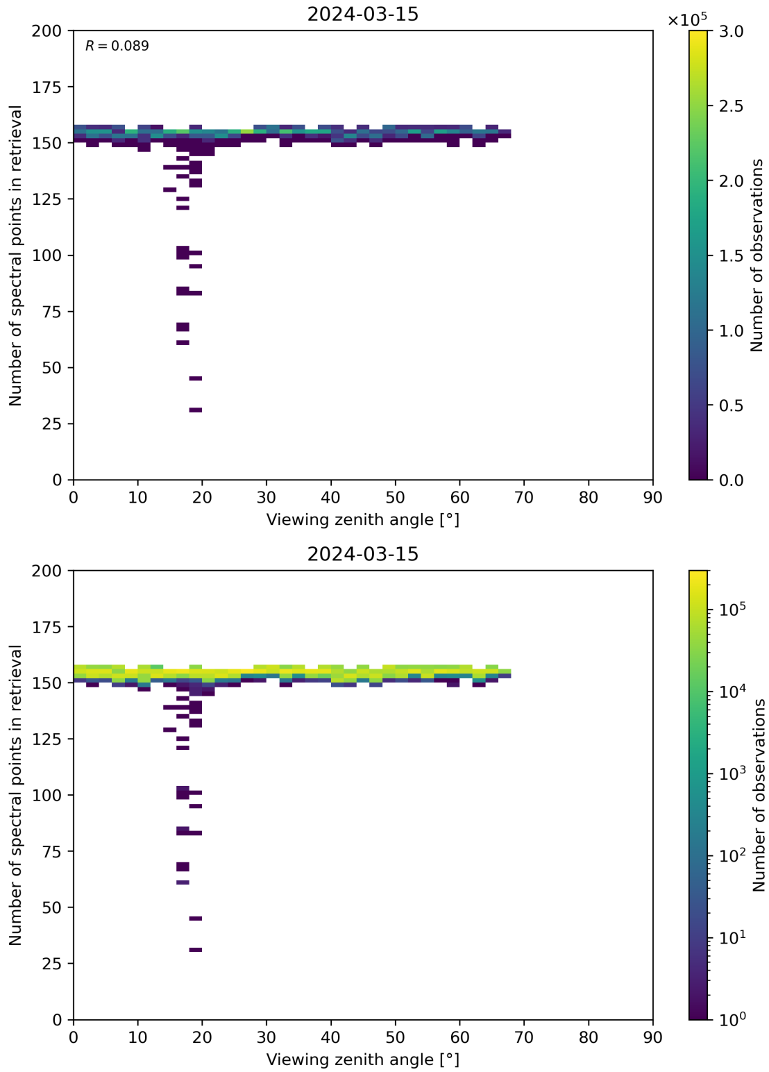
Figure 76: Scatter density plot of “Viewing zenith angle” against “Number of spectral points in retrieval” for 2024-03-14 to 2024-03-16.
