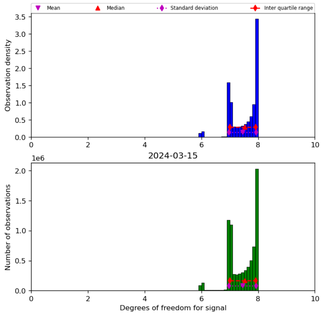
Figure 23: Histogram of “Degrees of freedom for signal” for 2024-03-14 to 2024-03-16
