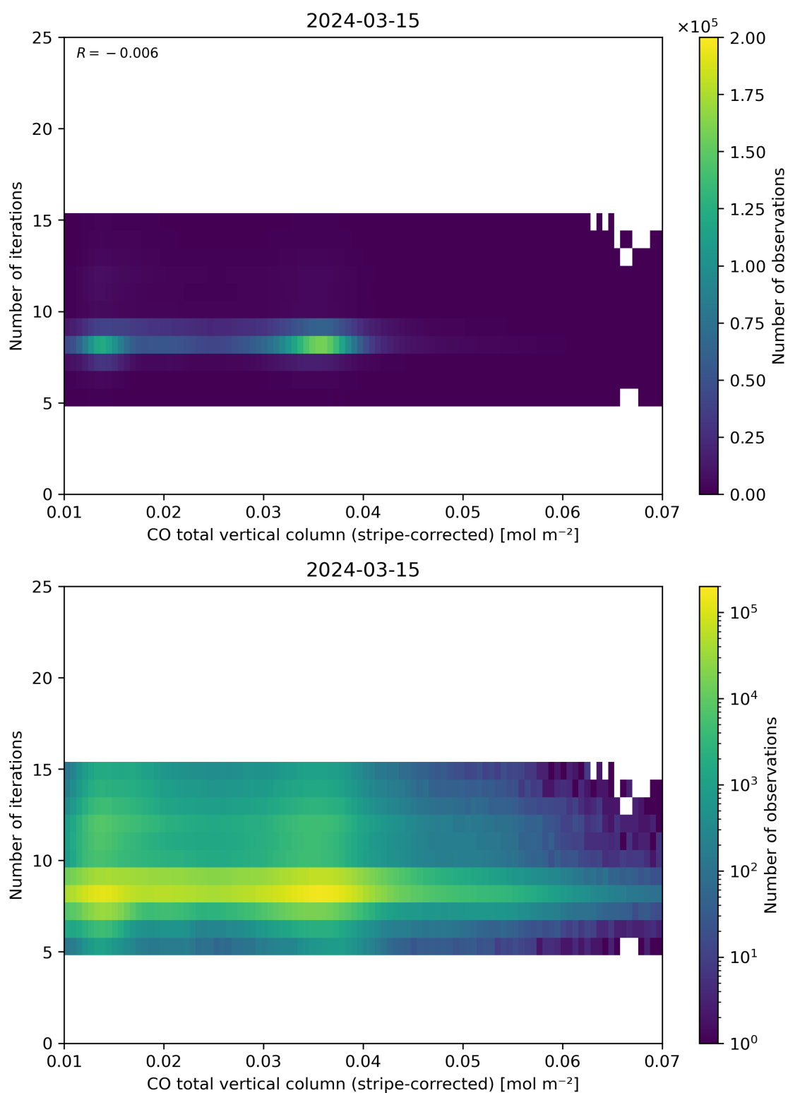
Figure 39: Scatter density plot of “CO total vertical column (stripe-corrected)” against “Number of iterations” for 2024-03-14 to 2024-03-16.
