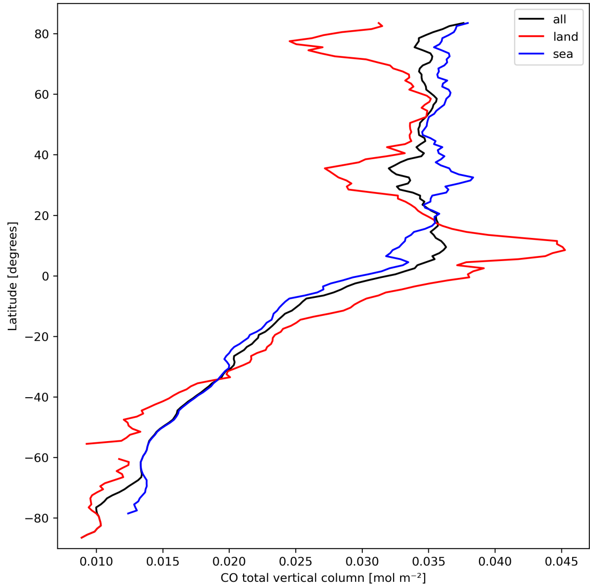
Figure 10: Zonal average of “CO total vertical column” for 2024-03-14 to 2024-03-16.
