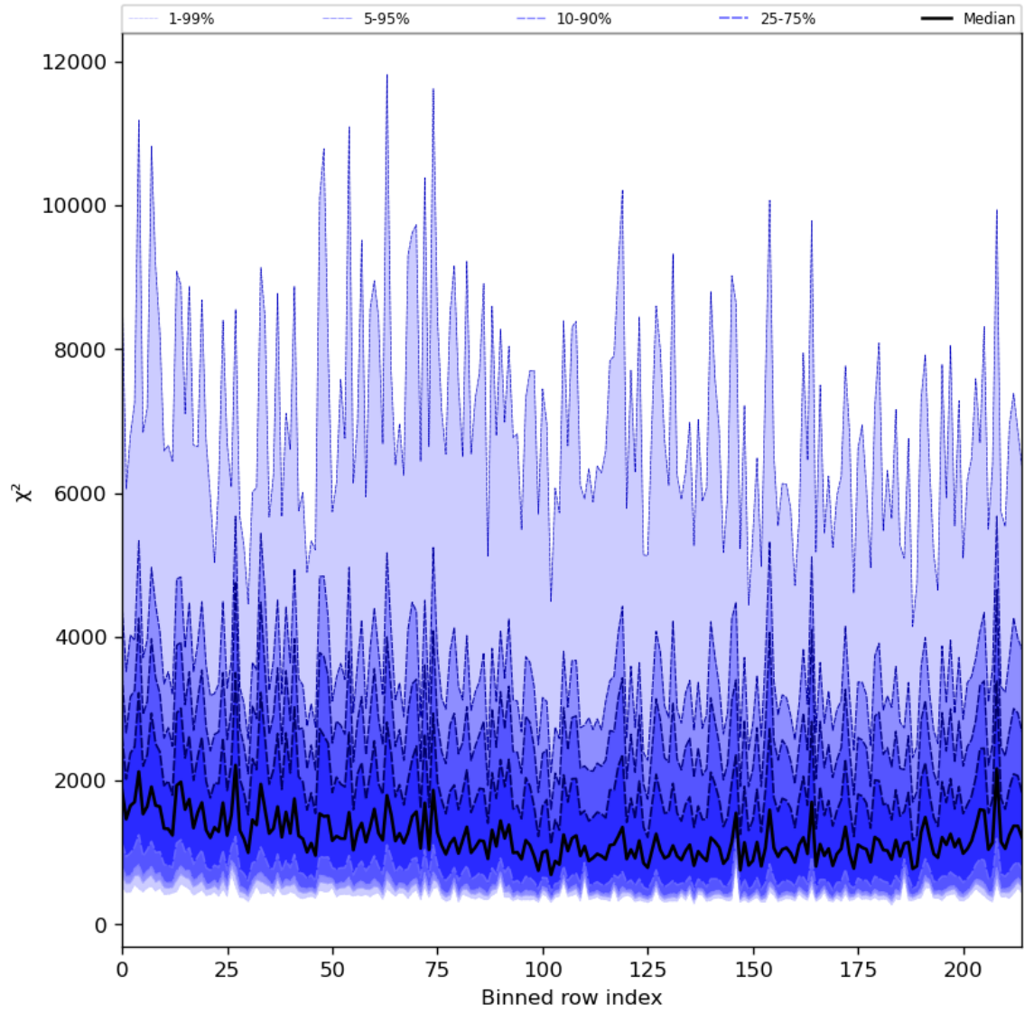
Figure 30: Along track statistics of “ \chi^2 ” for 2024-03-14 to 2024-03-16
