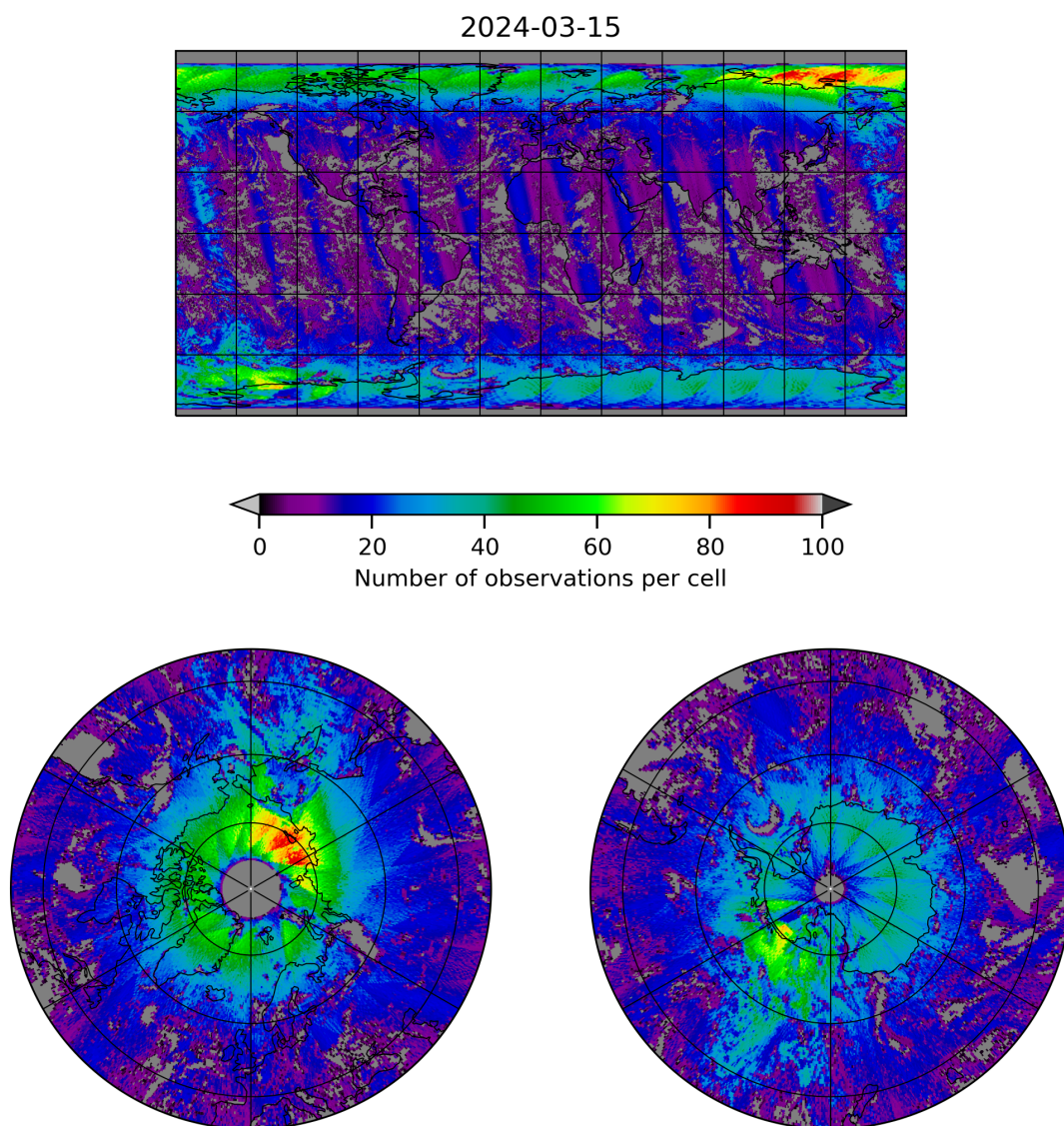
Figure 8: Map of the number of observations for 2024-03-14 to 2024-03-16
