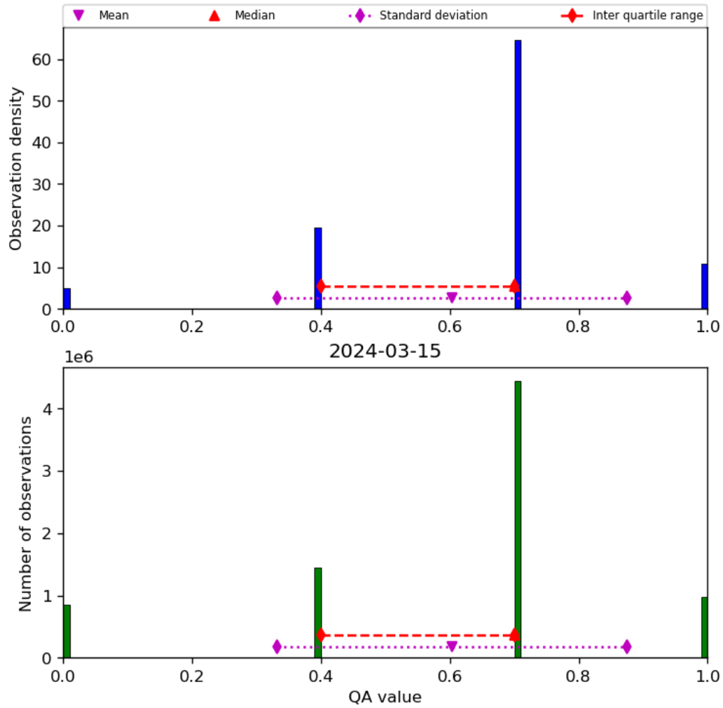
Figure 17: Histogram of “QA value” for 2024-03-14 to 2024-03-16
