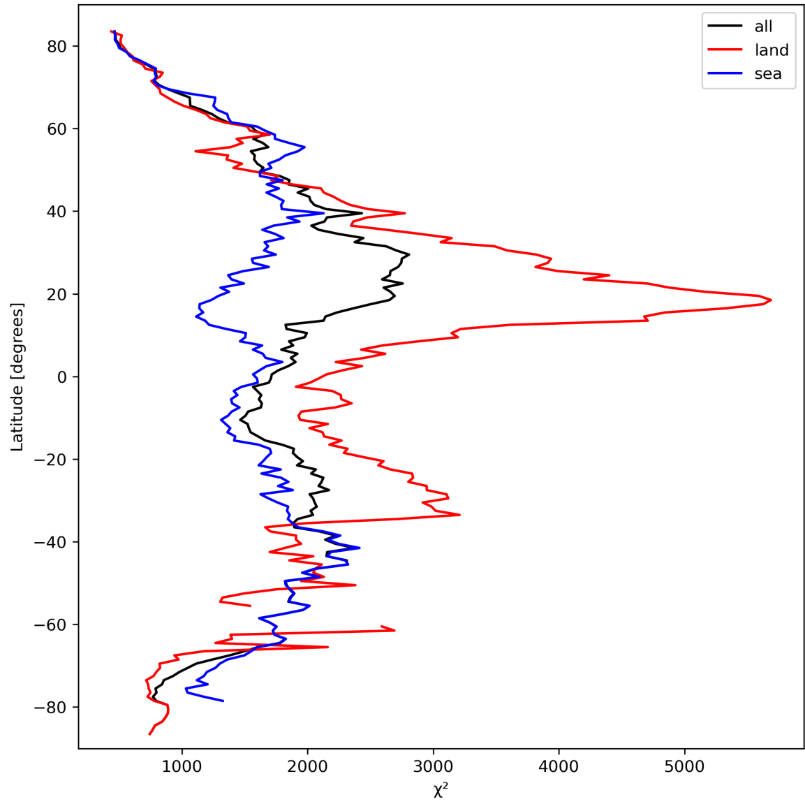
Figure 14: Zonal average of “ \chi^2 ” for 2024-03-15 to 2024-03-17.
