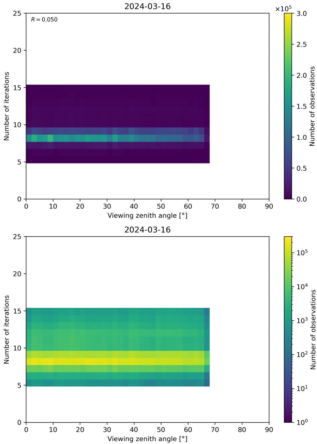
Figure 75: Scatter density plot of “Viewing zenith angle” against “Number of iterations” for 2024-03-15 to 2024-03-17.
