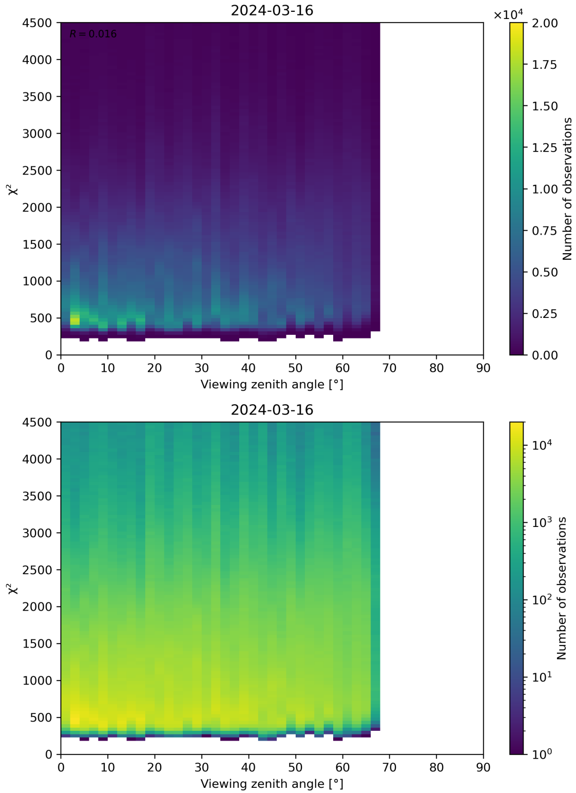
Figure 72: Scatter density plot of “Viewing zenith angle” against “ \chi^2 ” for 2024-03-15 to 2024-03-17.
