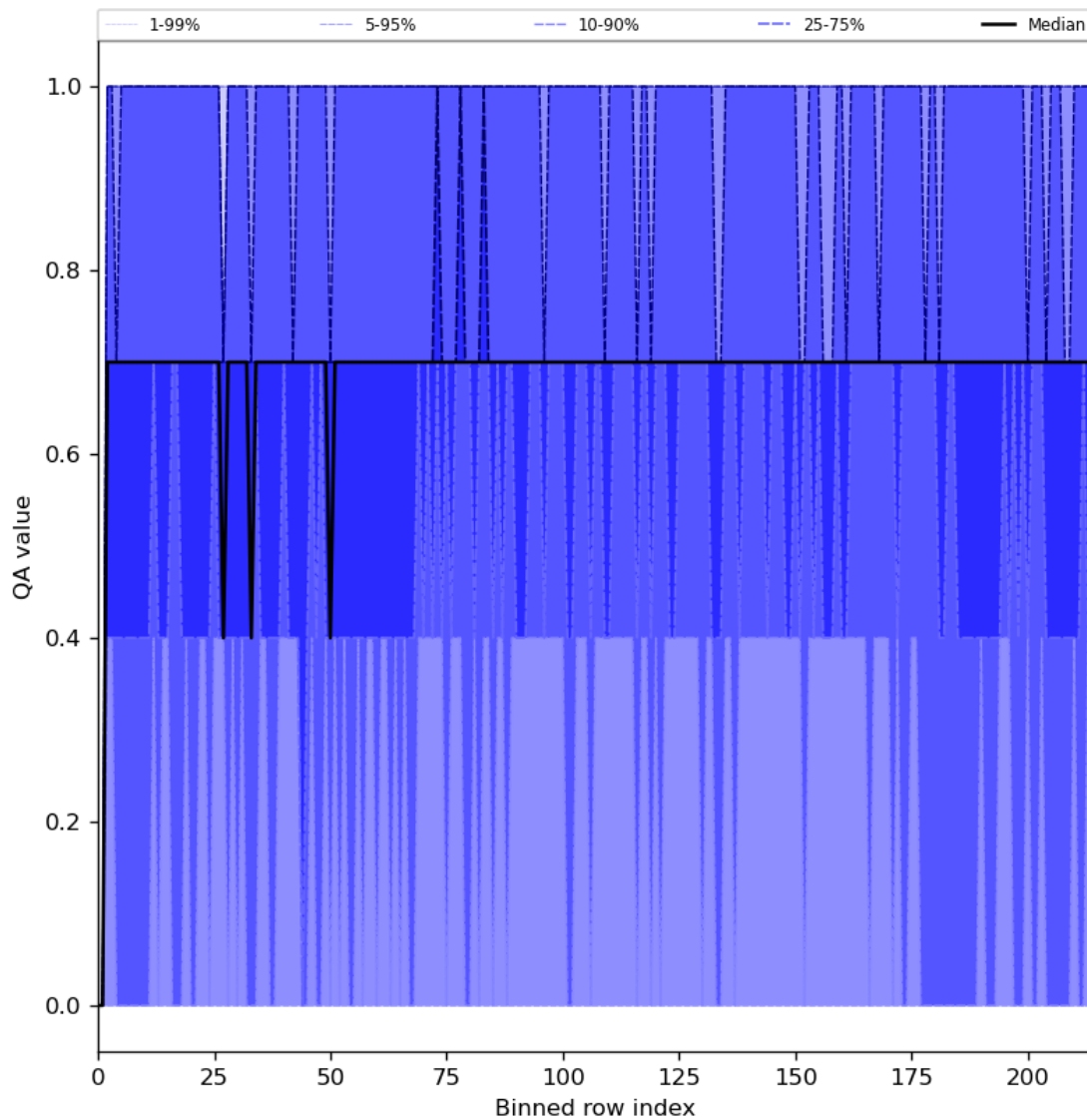
Figure 25: Along track statistics of “QA value” for 2024-03-15 to 2024-03-17
