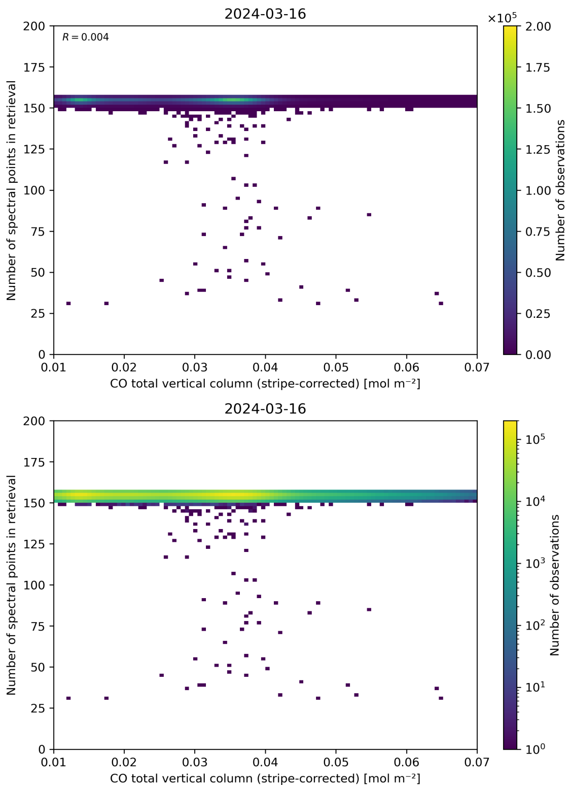
Figure 40: Scatter density plot of “CO total vertical column (stripe-corrected)” against “Number of spectral points in retrieval” for 2024-03-15 to 2024-03-17.
