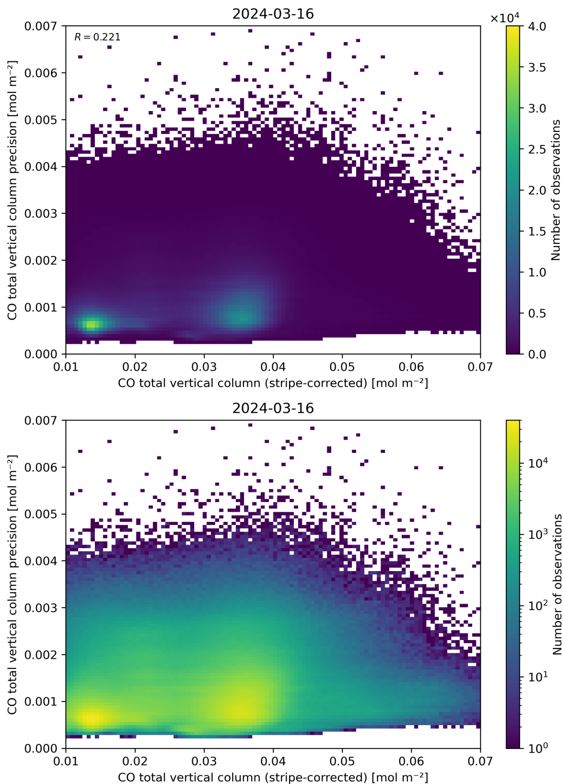
Figure 36: Scatter density plot of “CO total vertical column (stripe-corrected)” against “CO total vertical column precision” for 2024-03-15 to 2024-03-17.
