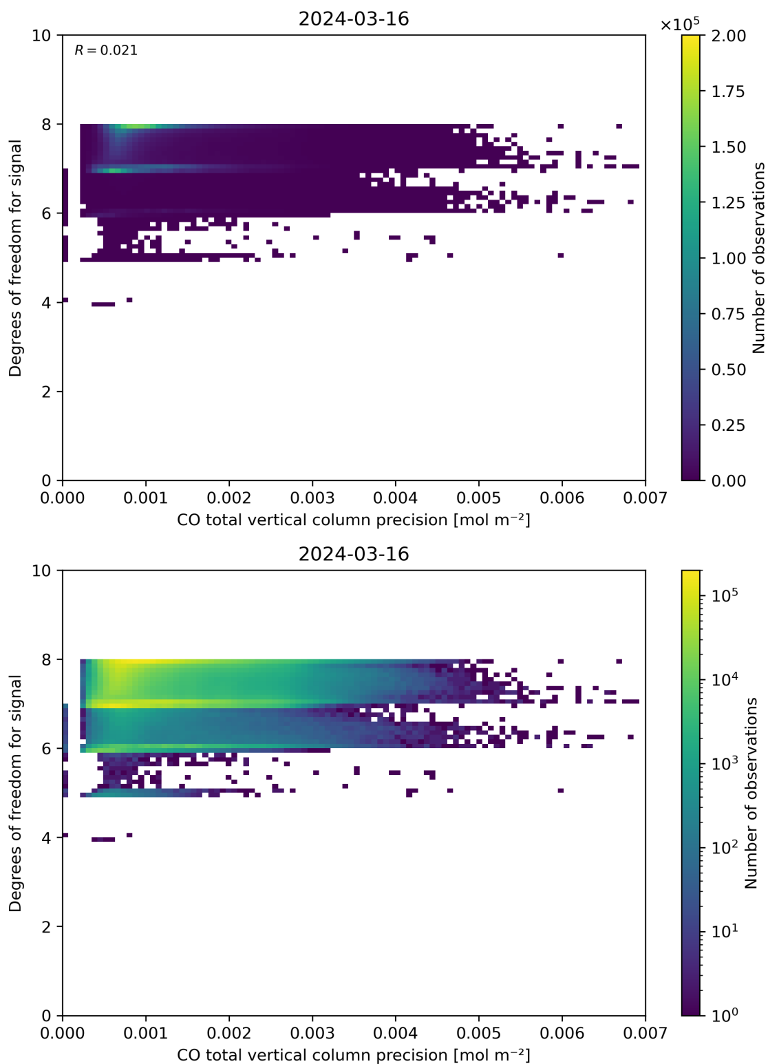
Figure 45: Scatter density plot of “CO total vertical column precision” against “Degrees of freedom for signal” for 2024-03-15 to 2024-03-17.
