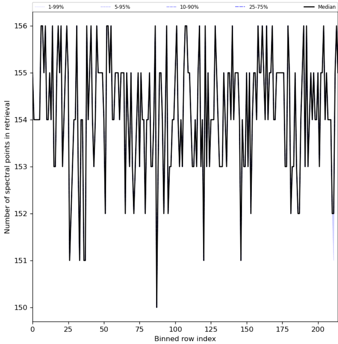
Figure 29: Along track statistics of “Number of spectral points in retrieval” for 2024-03-15 to 2024-03-17
