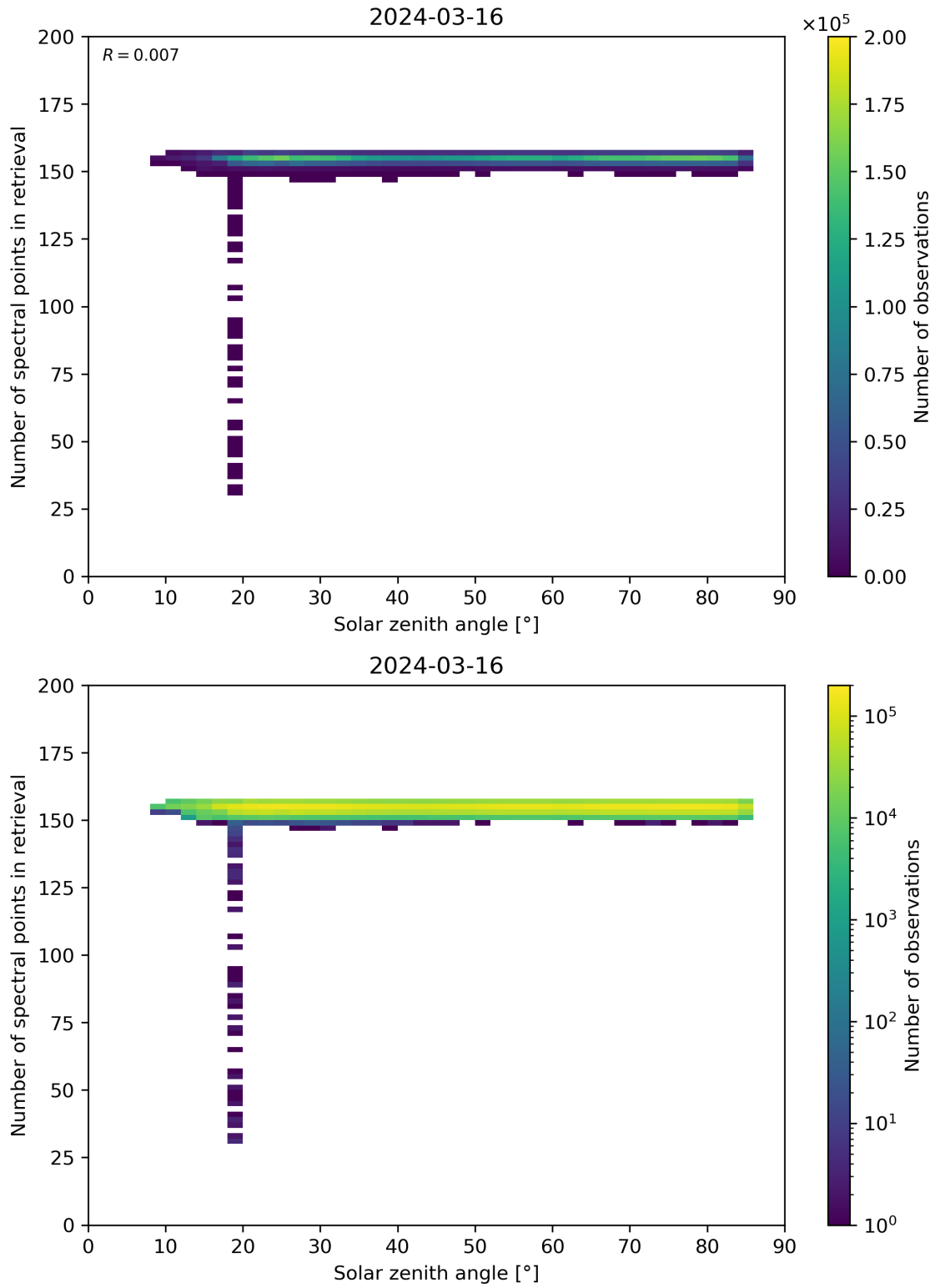
Figure 68: Scatter density plot of “Solar zenith angle” against “Number of spectral points in retrieval” for 2024-03-15 to 2024-03-17.
