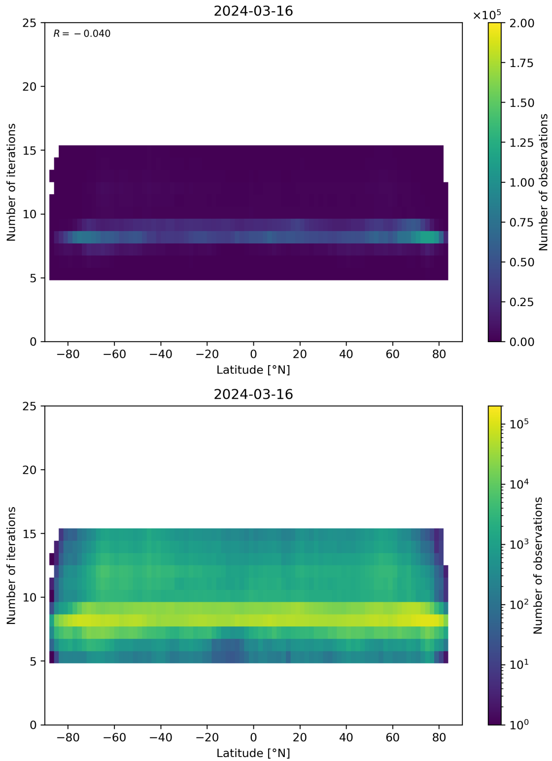
Figure 56: Scatter density plot of “Latitude” against “Number of iterations” for 2024-03-15 to 2024-03-17.
