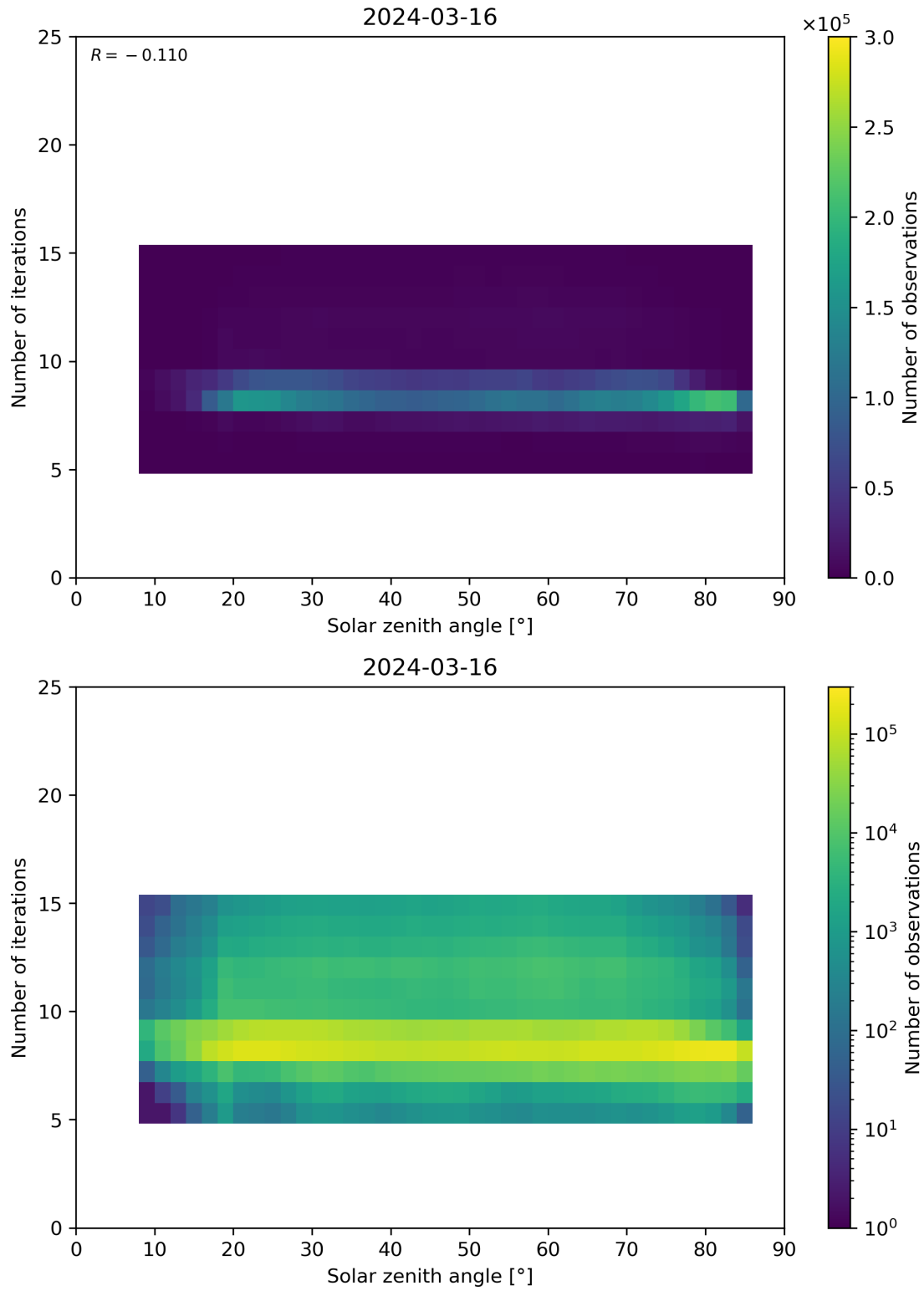
Figure 67: Scatter density plot of “Solar zenith angle” against “Number of iterations” for 2024-03-15 to 2024-03-17.
