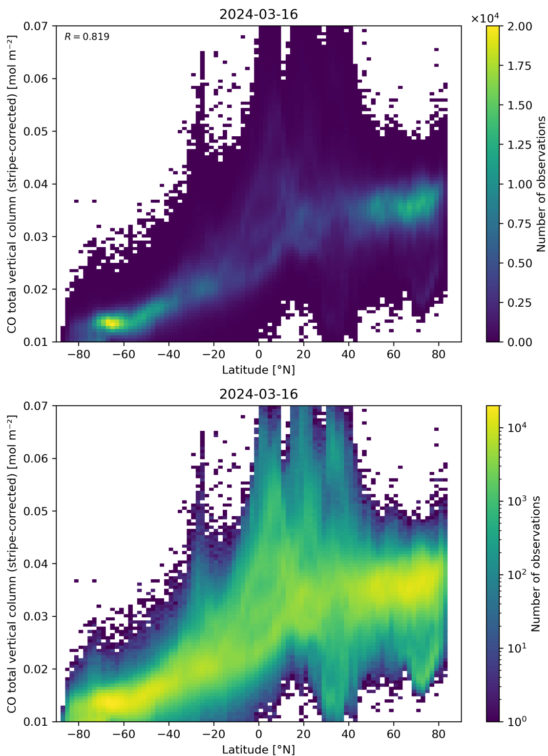
Figure 52: Scatter density plot of “Latitude” against “CO total vertical column (stripe-corrected)” for 2024-03-15 to 2024-03-17.
