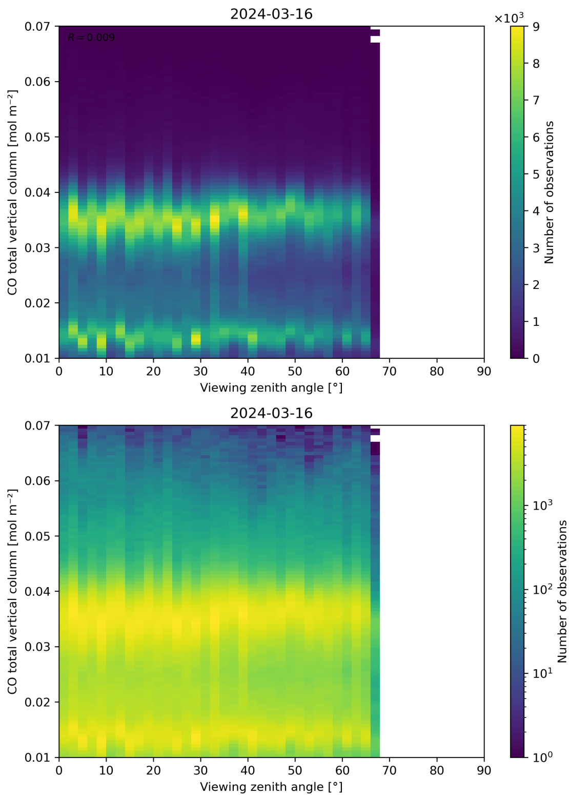
Figure 69: Scatter density plot of “Viewing zenith angle” against “CO total vertical column” for 2024-03-15 to 2024-03-17.
