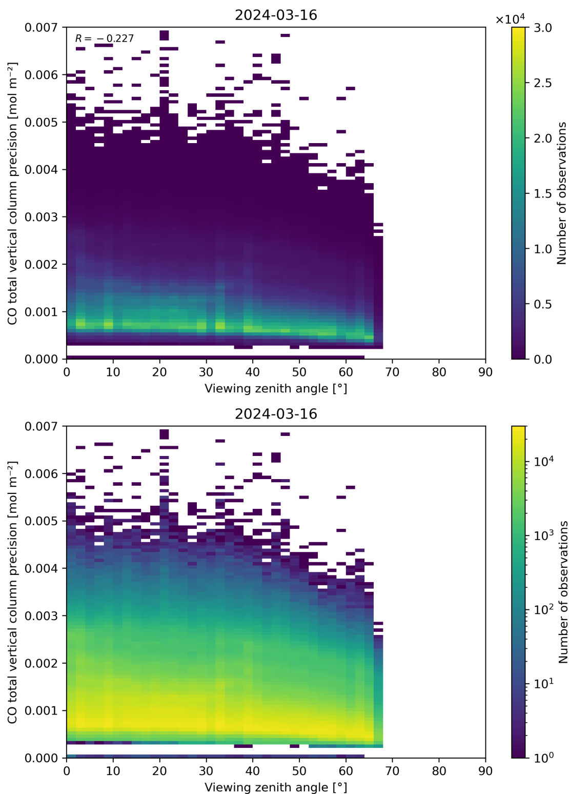
Figure 71: Scatter density plot of “Viewing zenith angle” against “CO total vertical column precision” for 2024-03-15 to 2024-03-17.
