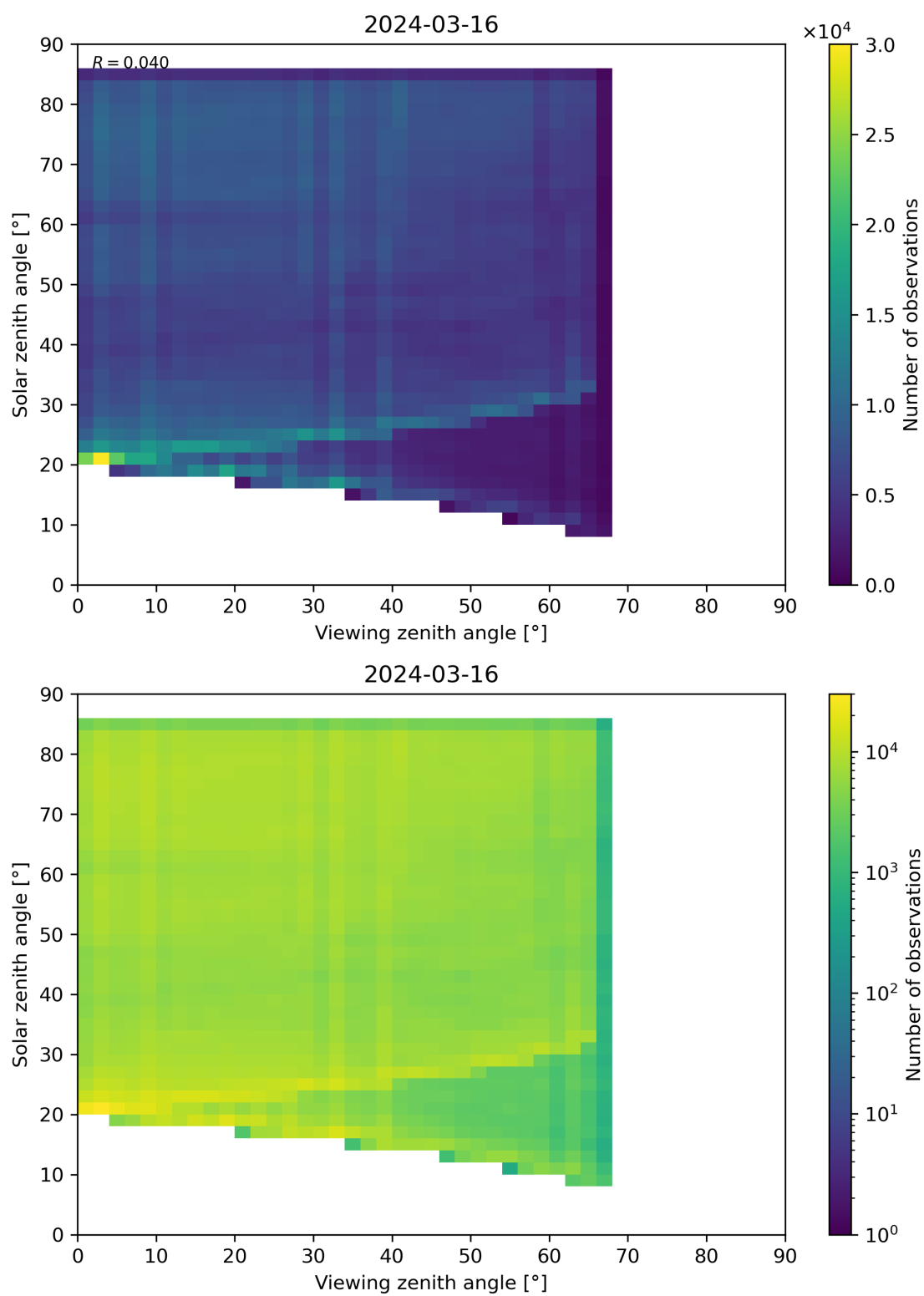
Figure 77: Scatter density plot of “Viewing zenith angle” against “Solar zenith angle” for 2024-03-15 to 2024-03-17.
