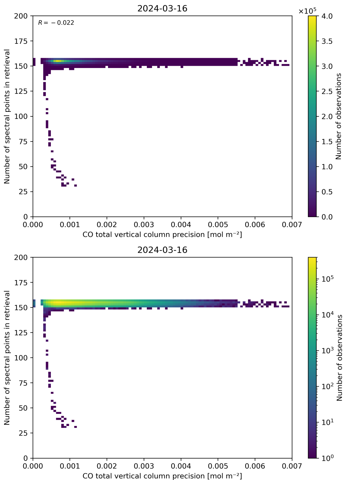
Figure 47: Scatter density plot of “CO total vertical column precision” against “Number of spectral points in retrieval” for 2024-03-15 to 2024-03-17.
