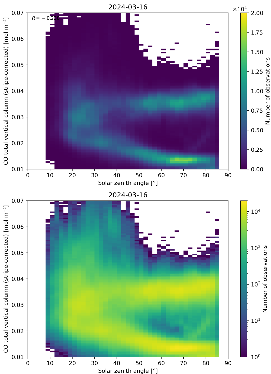
Figure 62: Scatter density plot of “Solar zenith angle” against “CO total vertical column (stripe-corrected)” for 2024-03-15 to 2024-03-17.
