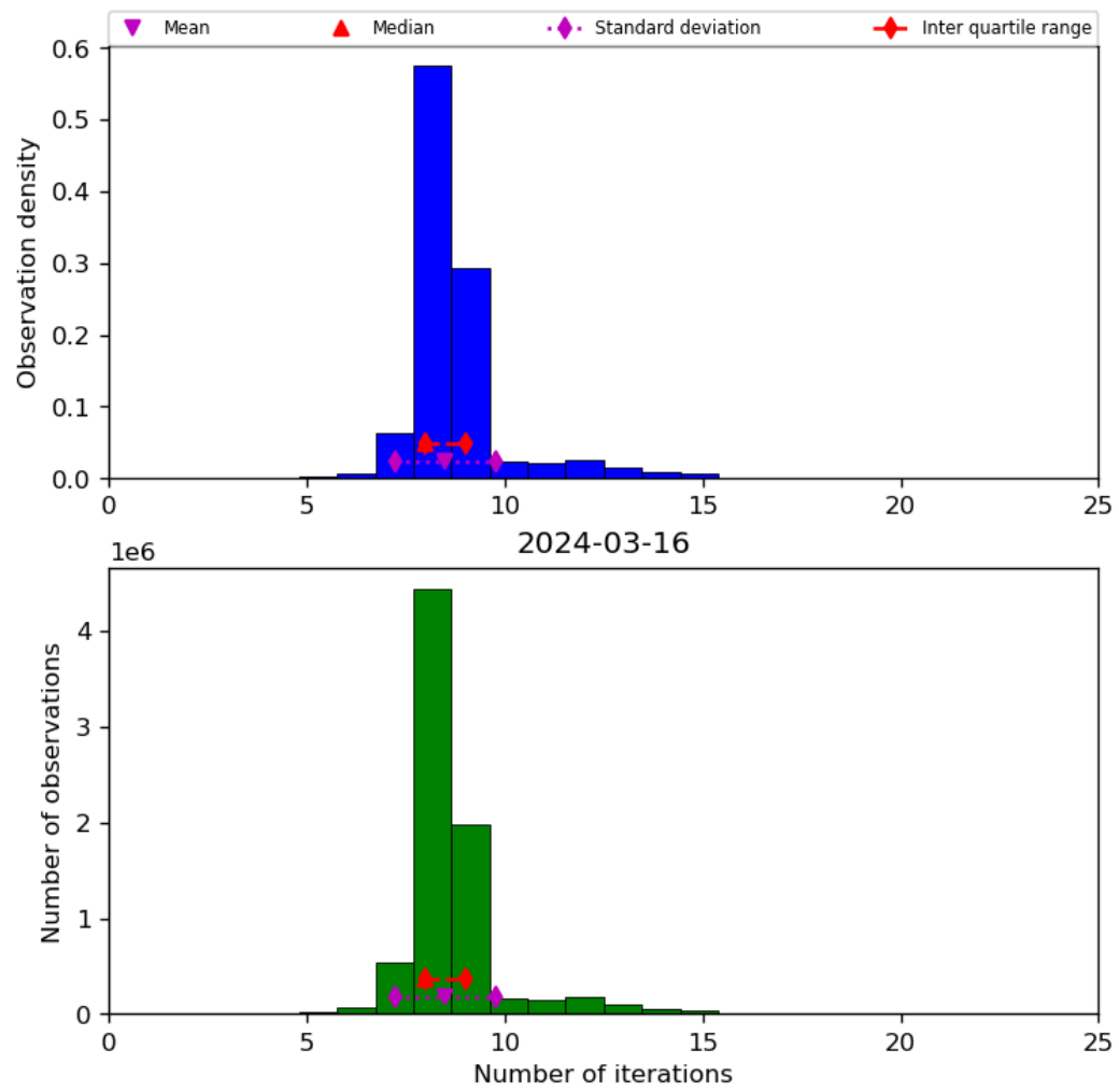
Figure 24: Histogram of “Number of iterations” for 2024-03-15 to 2024-03-17
