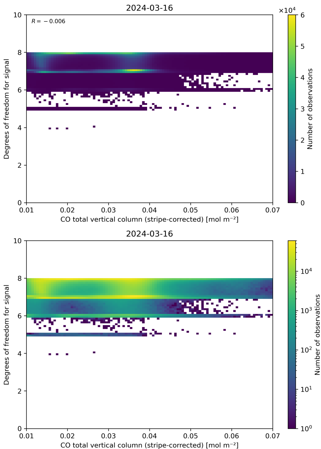
Figure 38: Scatter density plot of “CO total vertical column (stripe-corrected)” against “Degrees of freedom for signal” for 2024-03-15 to 2024-03-17.
