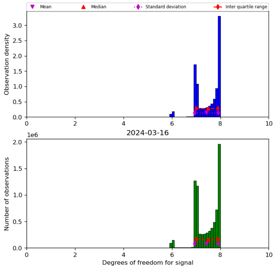
Figure 23: Histogram of “Degrees of freedom for signal” for 2024-03-15 to 2024-03-17
