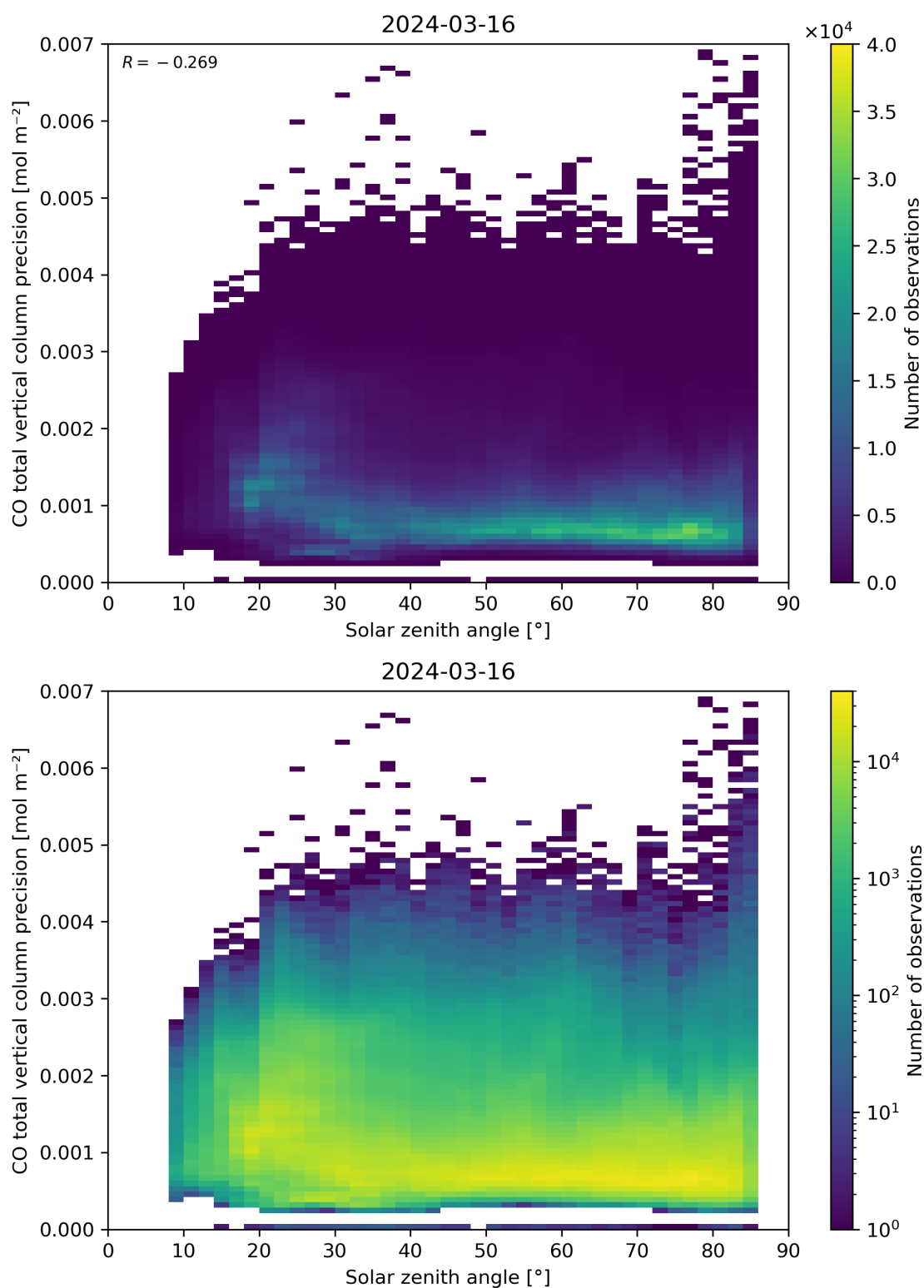
Figure 63: Scatter density plot of “Solar zenith angle” against “CO total vertical column precision” for 2024-03-15 to 2024-03-17.
