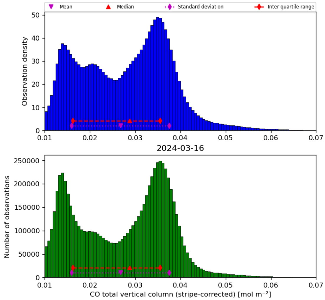
Figure 19: Histogram of “CO total vertical column (stripe-corrected)” for 2024-03-15 to 2024-03-17
