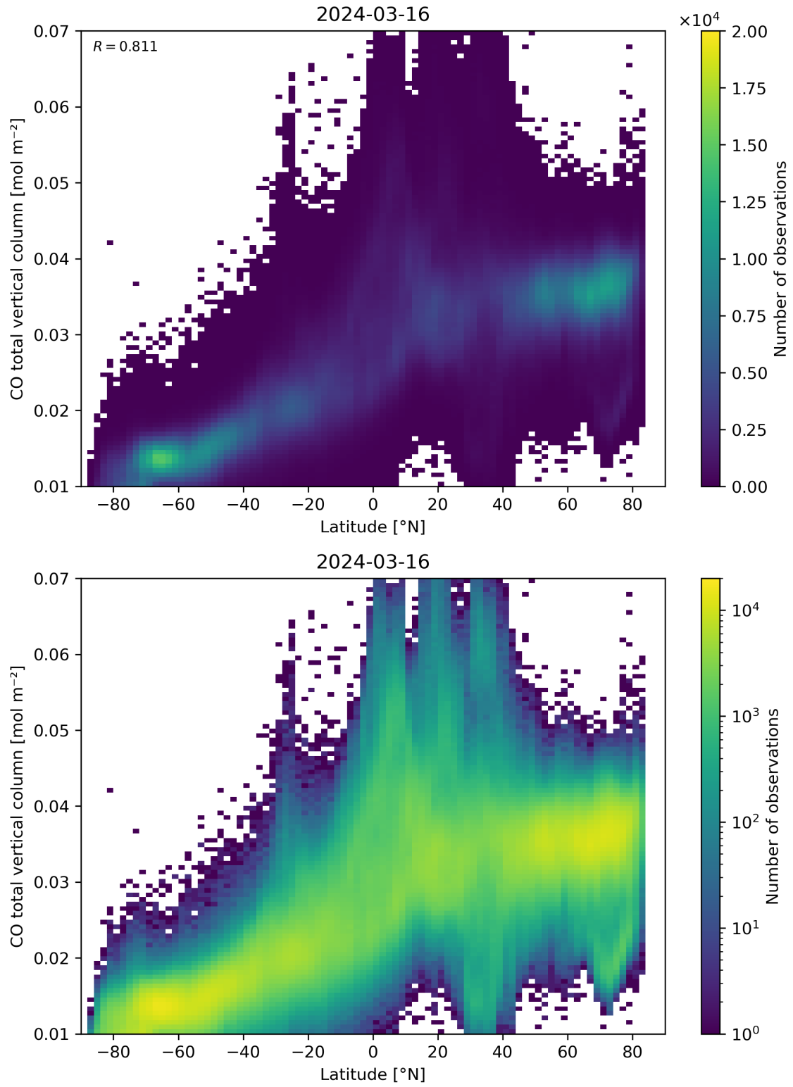
Figure 51: Scatter density plot of “Latitude” against “CO total vertical column” for 2024-03-15 to 2024-03-17.
