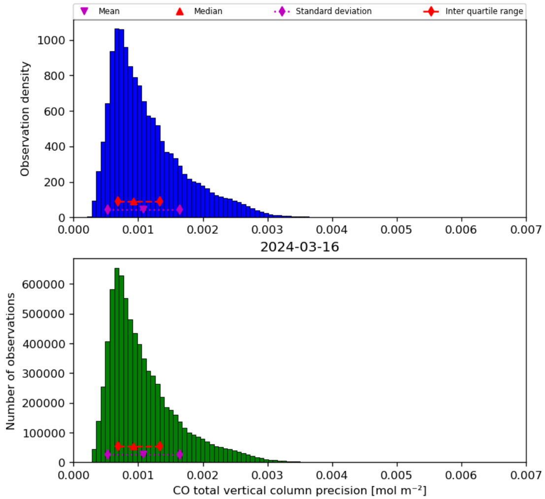
Figure 20: Histogram of “CO total vertical column precision” for 2024-03-15 to 2024-03-17
