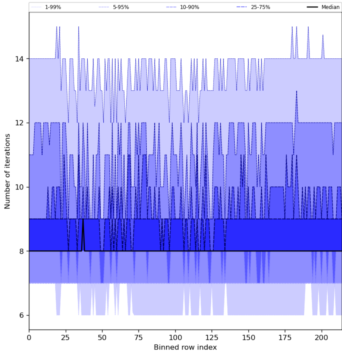
Figure 32: Along track statistics of “Number of iterations” for 2024-03-15 to 2024-03-17
