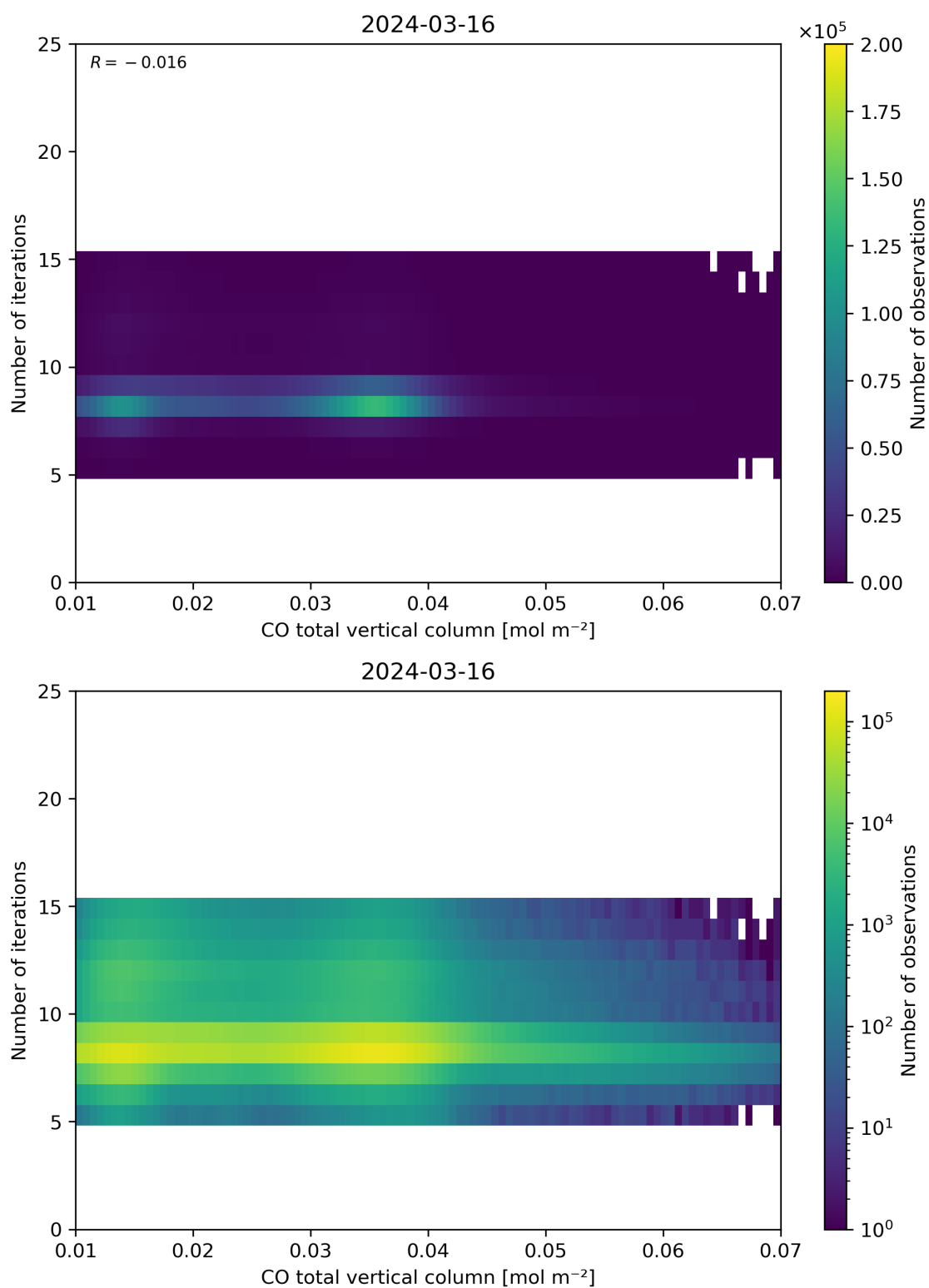
Figure 42: Scatter density plot of “CO total vertical column” against “Number of iterations” for 2024-03-15 to 2024-03-17.
