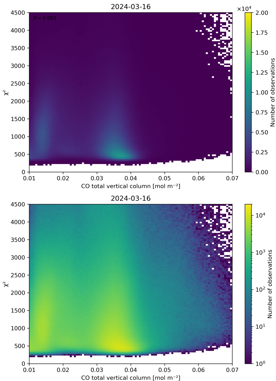
Figure 35: Scatter density plot of “CO total vertical column” against “ \chi^2 ” for 2024-03-15 to 2024-03-17.
