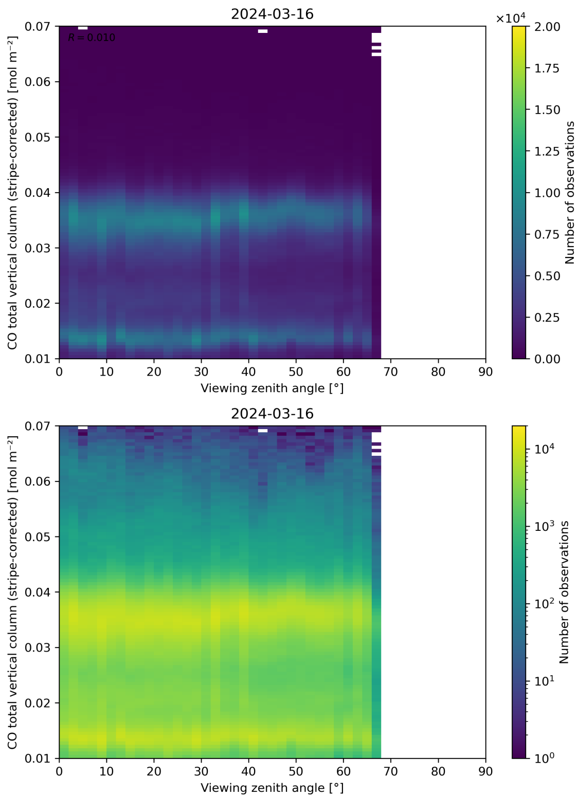
Figure 70: Scatter density plot of “Viewing zenith angle” against “CO total vertical column (stripe-corrected)” for 2024-03-15 to 2024-03-17.
