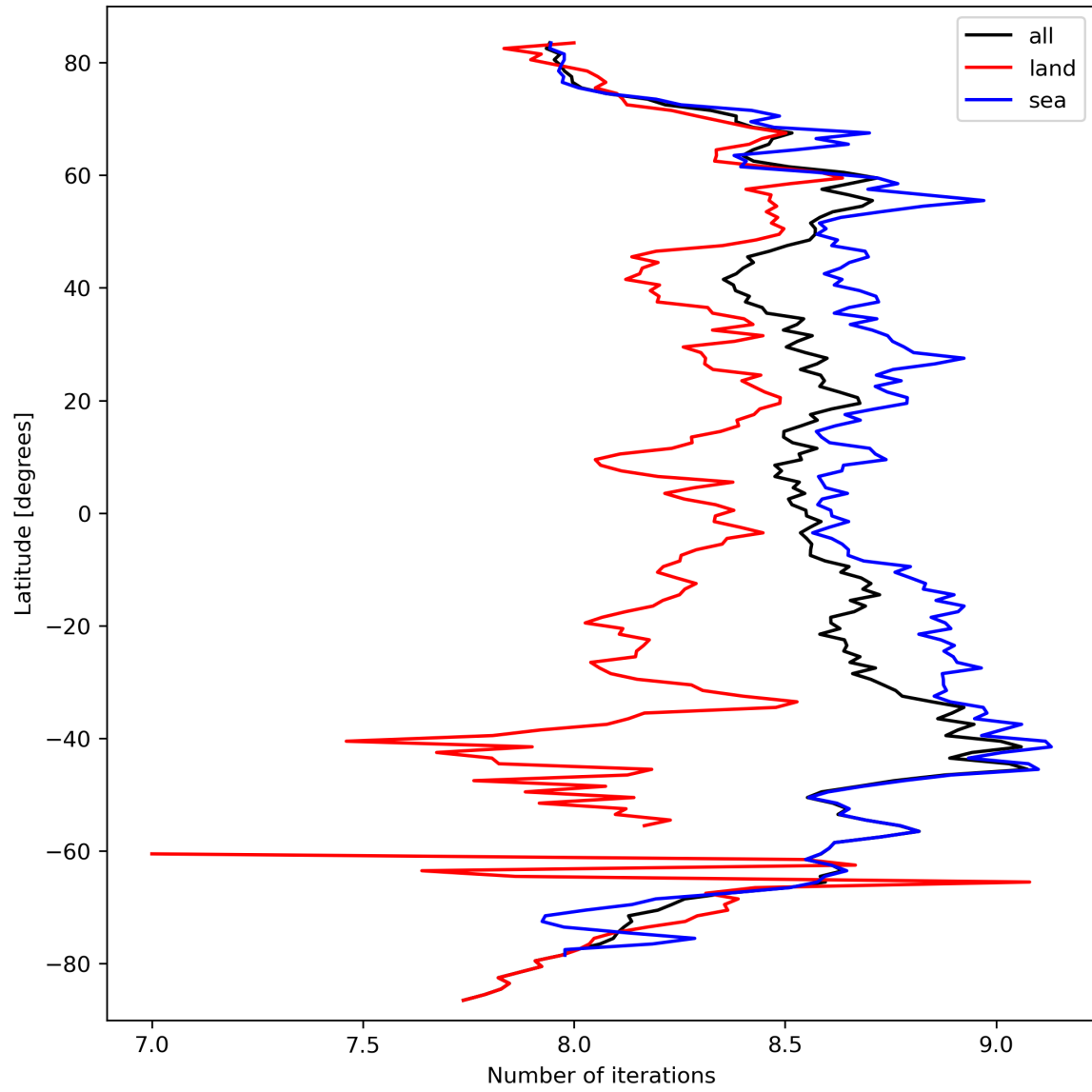
Figure 16: Zonal average of “Number of iterations” for 2024-03-15 to 2024-03-17.
