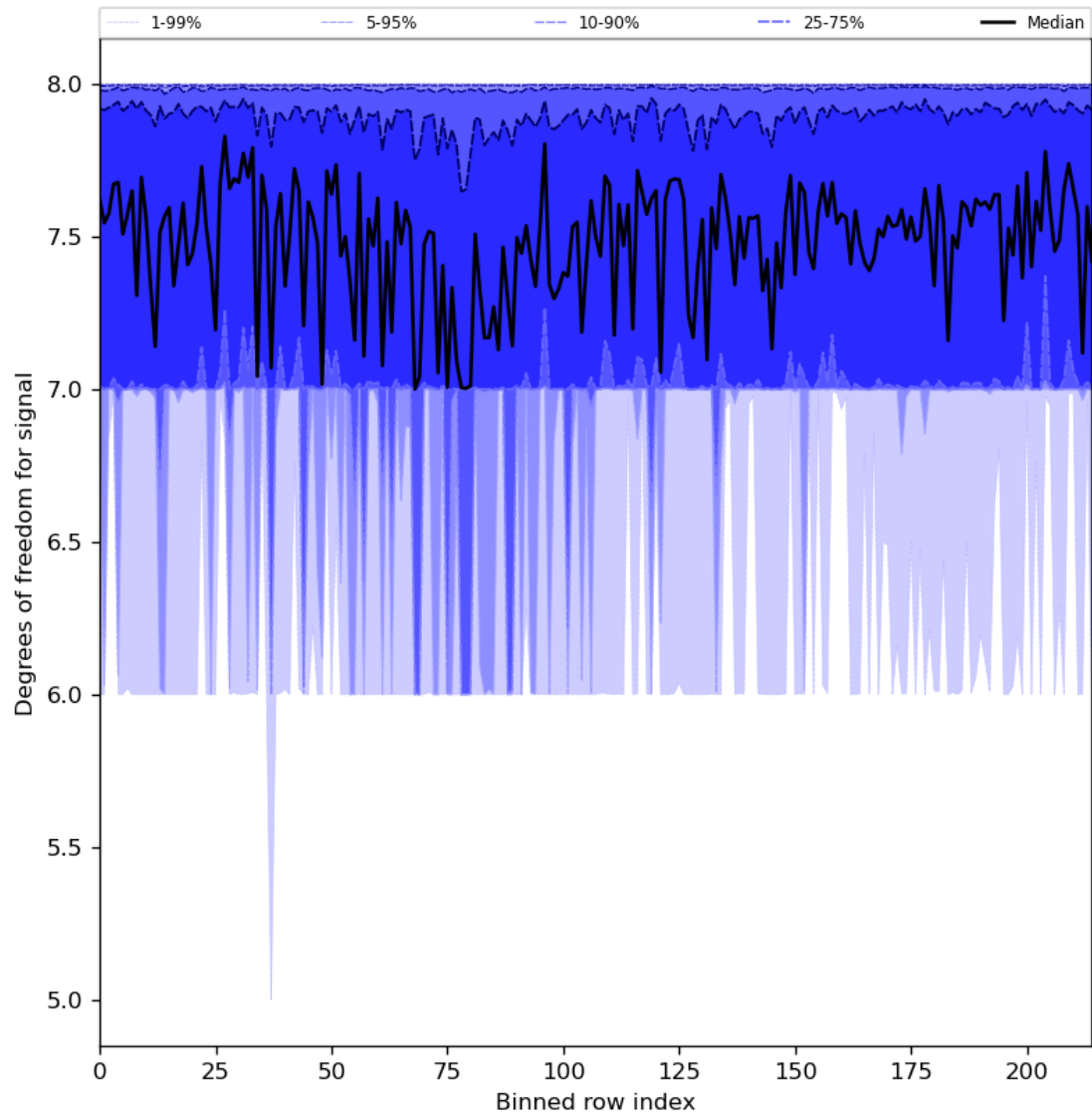
Figure 31: Along track statistics of “Degrees of freedom for signal” for 2024-03-15 to 2024-03-17
