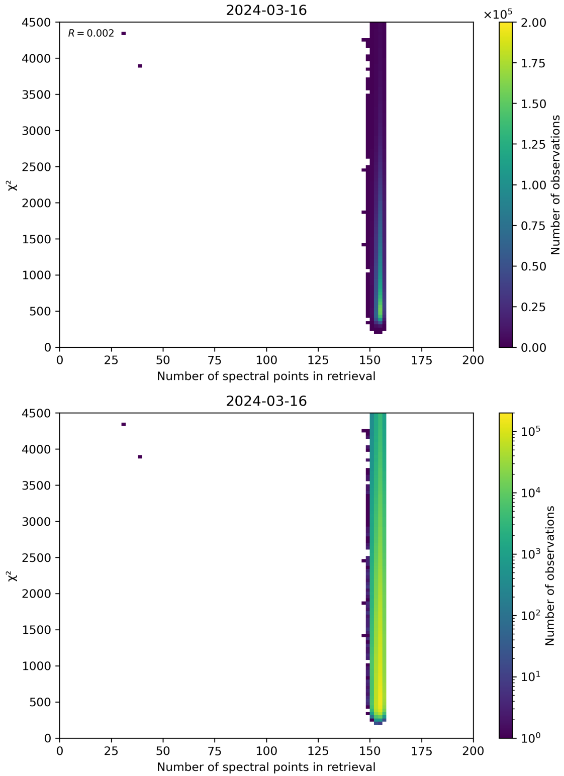
Figure 58: Scatter density plot of “Number of spectral points in retrieval” against “ \chi^2 ” for 2024-03-15 to 2024-03-17.
