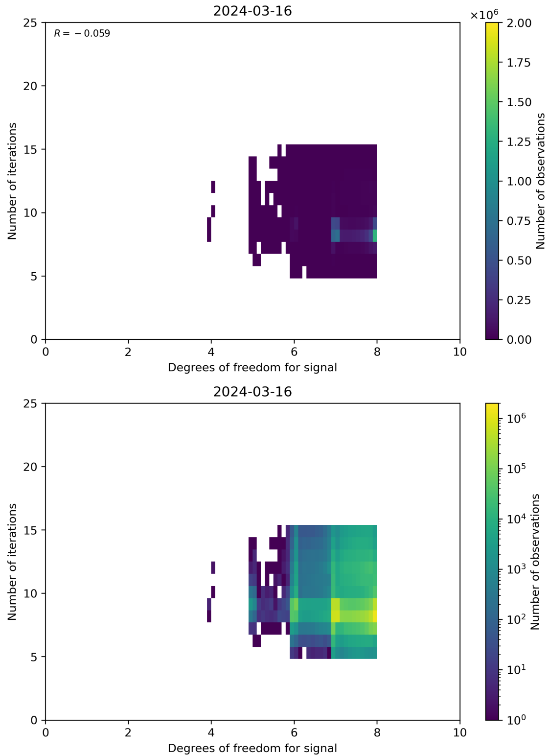
Figure 50: Scatter density plot of “Degrees of freedom for signal” against “Number of iterations” for 2024-03-15 to 2024-03-17.
