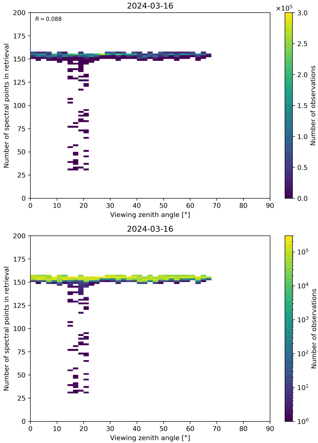
Figure 76: Scatter density plot of “Viewing zenith angle” against “Number of spectral points in retrieval” for 2024-03-15 to 2024-03-17.
