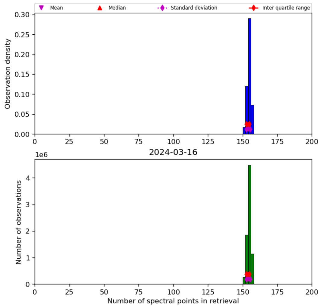
Figure 21: Histogram of “Number of spectral points in retrieval” for 2024-03-15 to 2024-03-17
