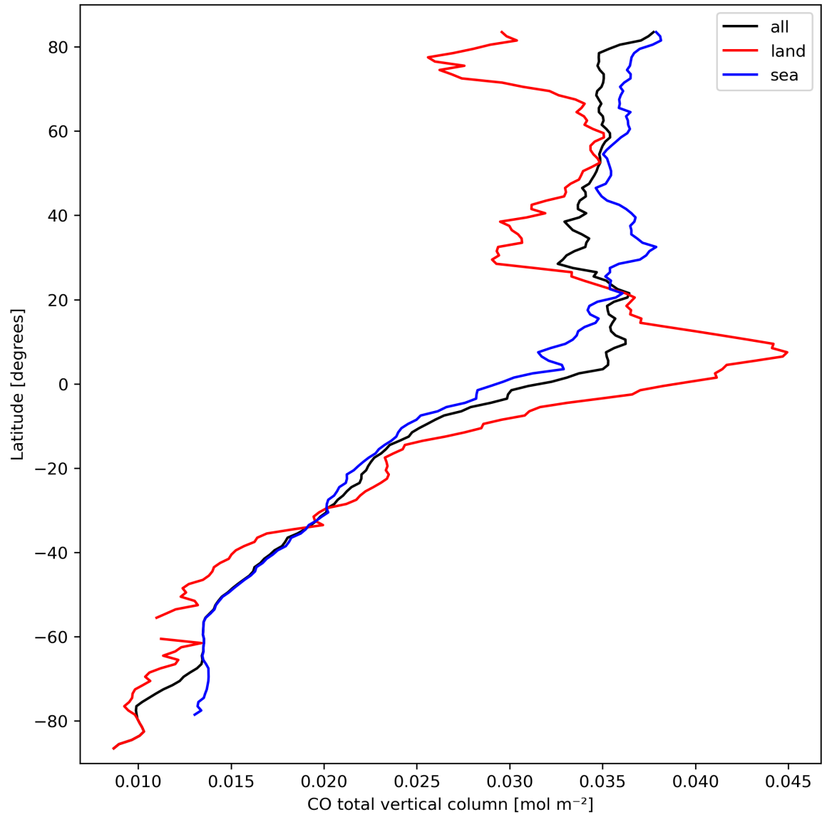
Figure 10: Zonal average of “CO total vertical column” for 2024-03-15 to 2024-03-17.
