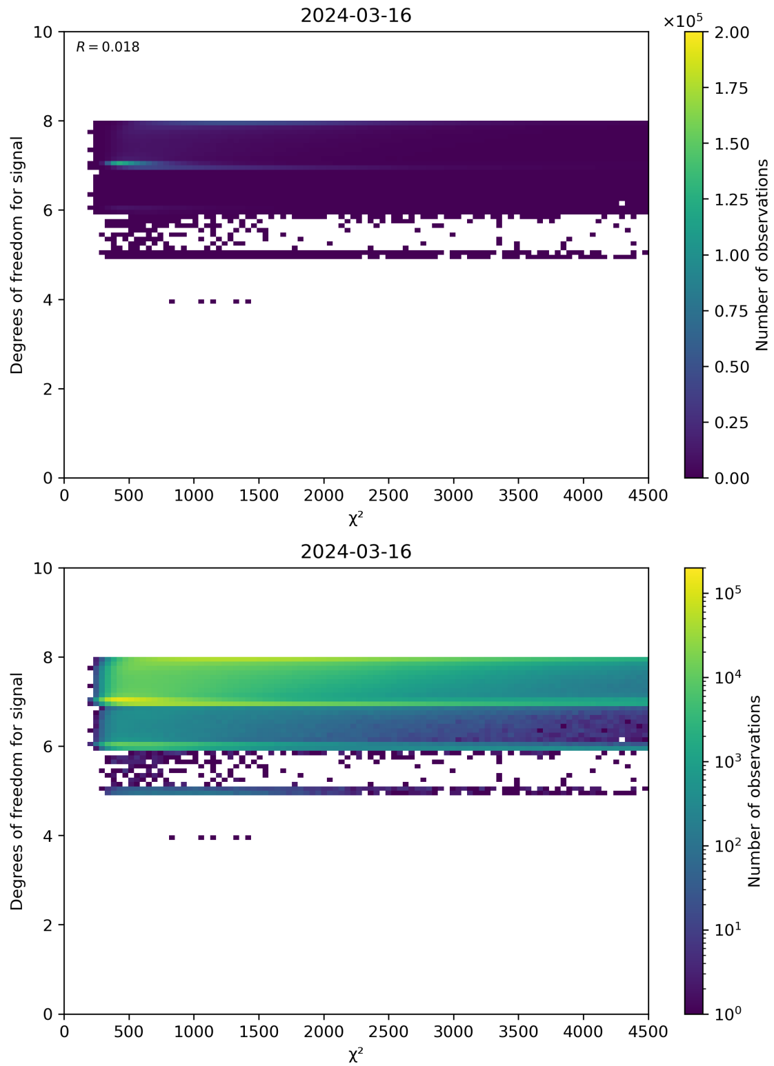
Figure 48: Scatter density plot of “ \chi^2 ” against “Degrees of freedom for signal” for 2024-03-15 to 2024-03-17.
