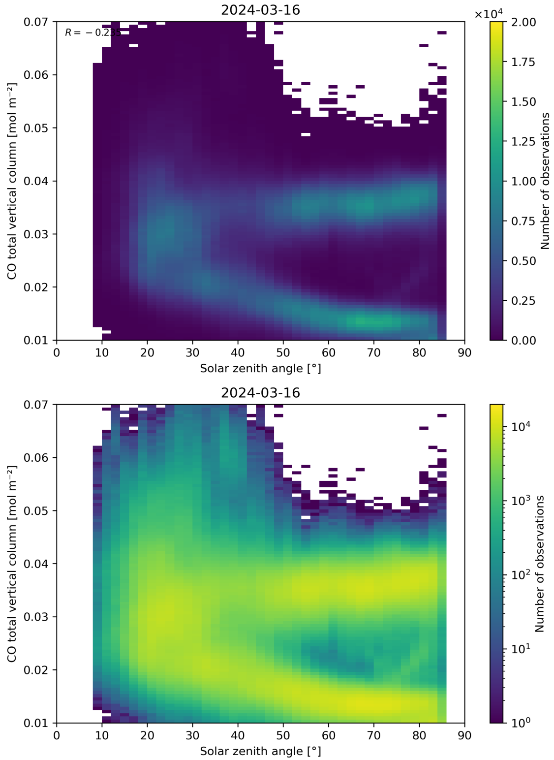
Figure 61: Scatter density plot of “Solar zenith angle” against “CO total vertical column” for 2024-03-15 to 2024-03-17.
