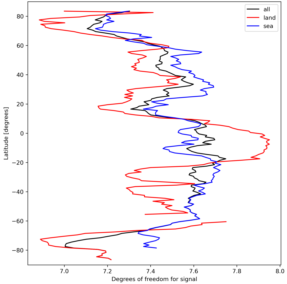
Figure 15: Zonal average of “Degrees of freedom for signal” for 2024-03-15 to 2024-03-17.
