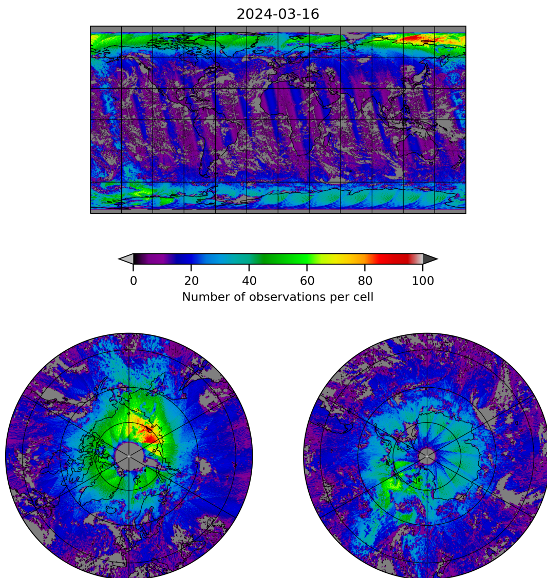
Figure 8: Map of the number of observations for 2024-03-15 to 2024-03-17
