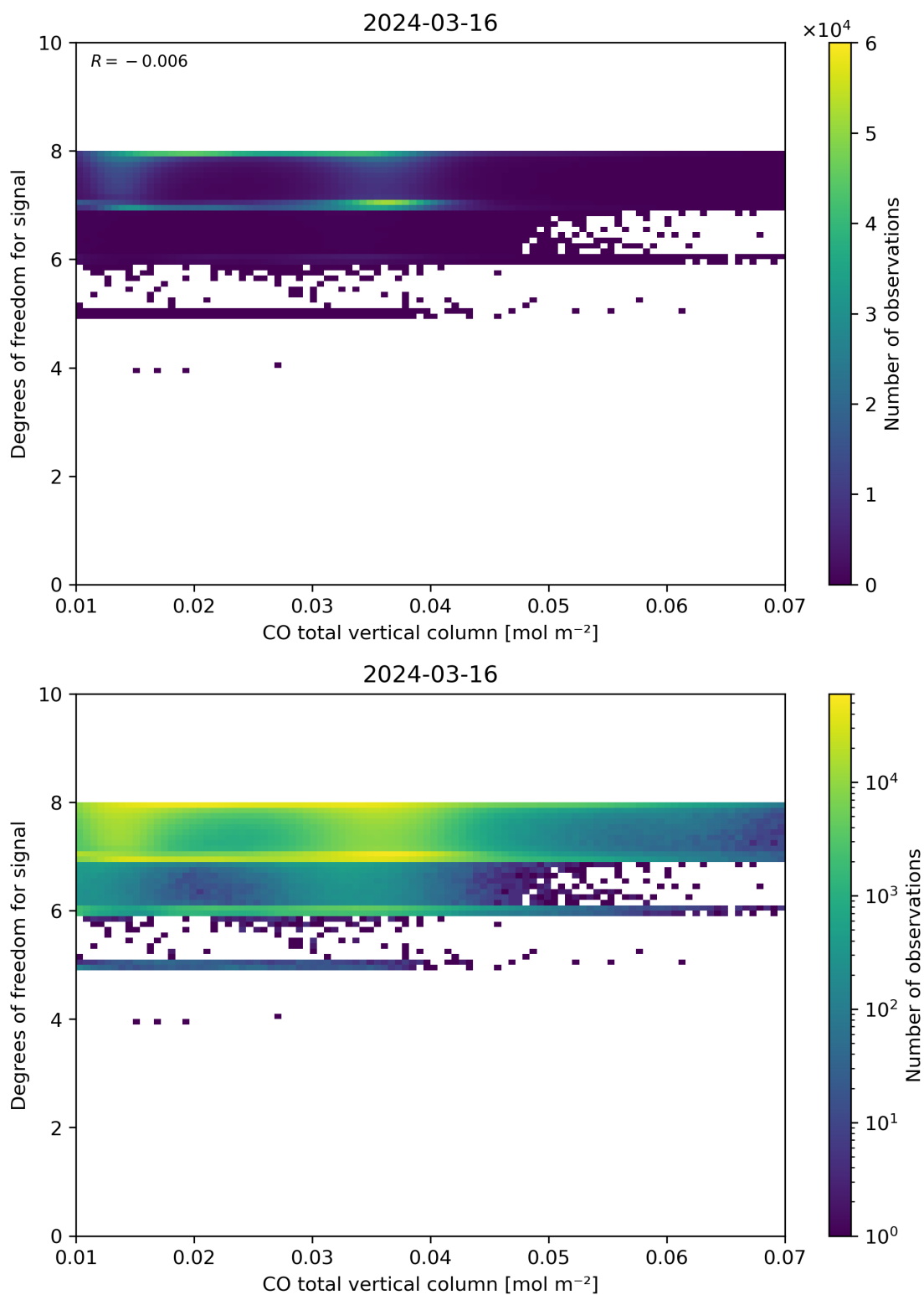
Figure 41: Scatter density plot of “CO total vertical column” against “Degrees of freedom for signal” for 2024-03-15 to 2024-03-17.
