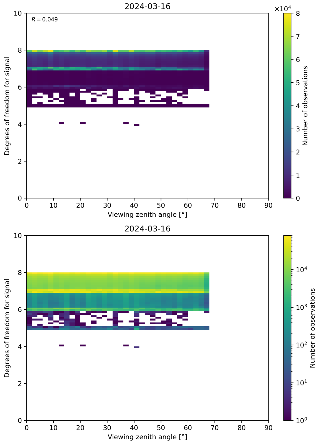
Figure 73: Scatter density plot of “Viewing zenith angle” against “Degrees of freedom for signal” for 2024-03-15 to 2024-03-17.
