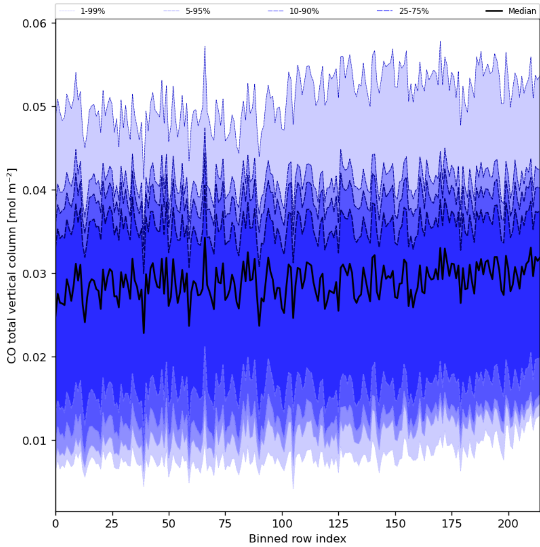
Figure 26: Along track statistics of “CO total vertical column” for 2024-03-15 to 2024-03-17
