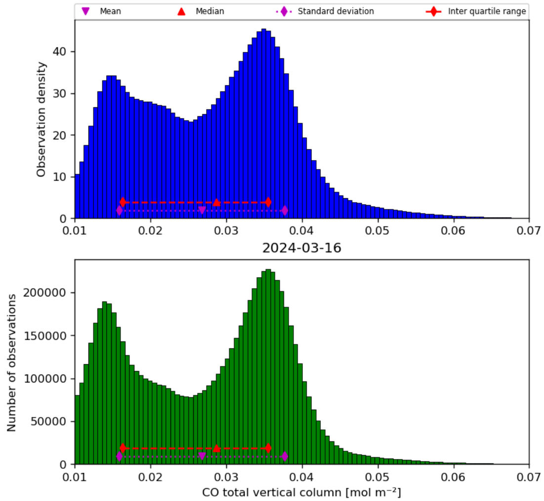
Figure 18: Histogram of “CO total vertical column” for 2024-03-15 to 2024-03-17
