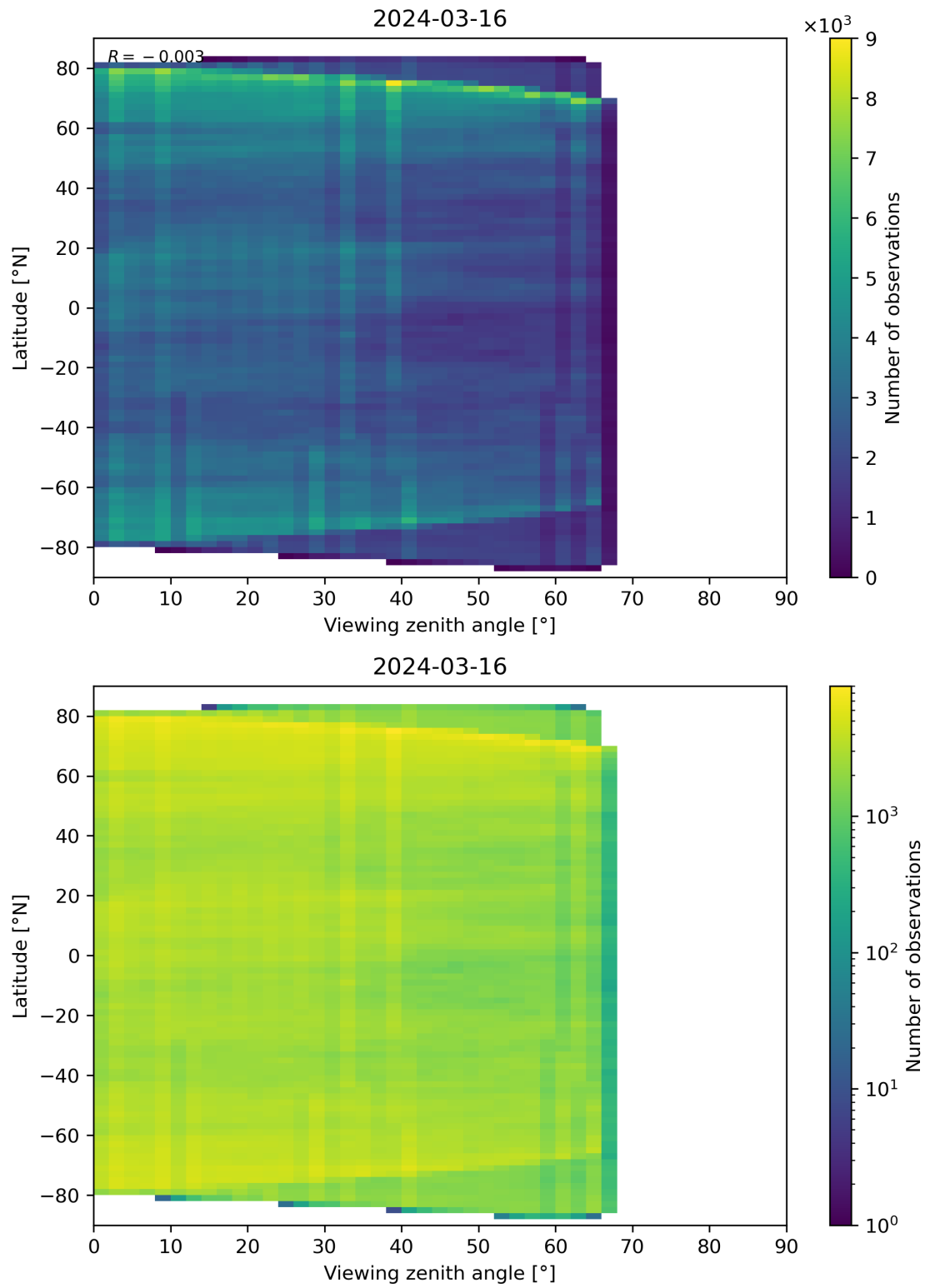
Figure 74: Scatter density plot of “Viewing zenith angle” against “Latitude” for 2024-03-15 to 2024-03-17.
