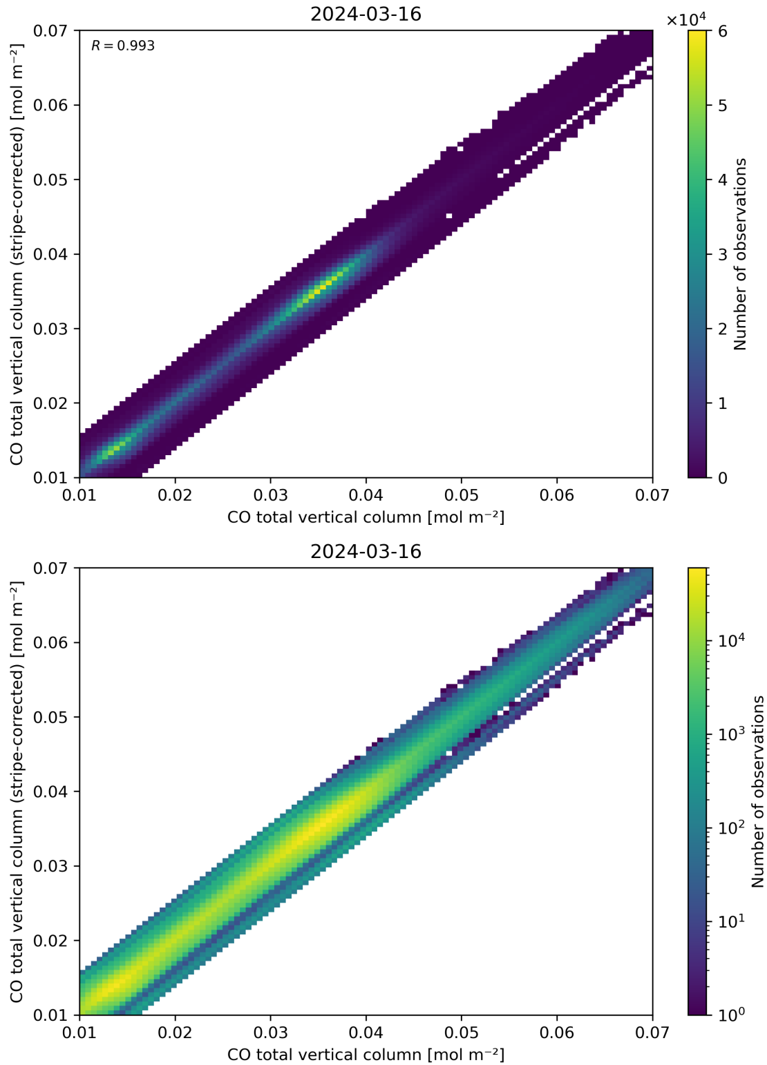
Figure 33: Scatter density plot of “CO total vertical column” against “CO total vertical column (stripe-corrected)” for 2024-03-15 to 2024-03-17.
