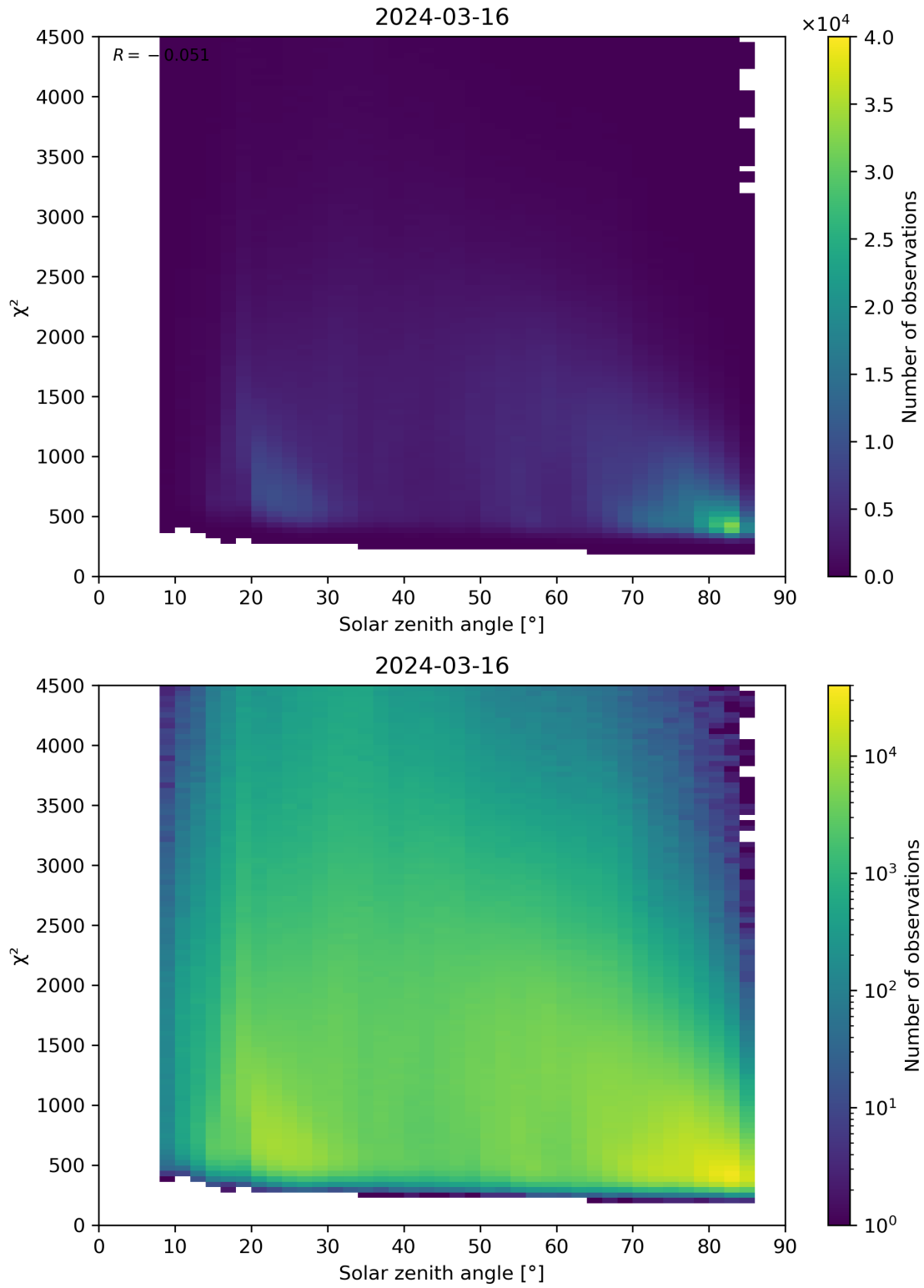
Figure 64: Scatter density plot of “Solar zenith angle” against “ \chi^2 ” for 2024-03-15 to 2024-03-17.
