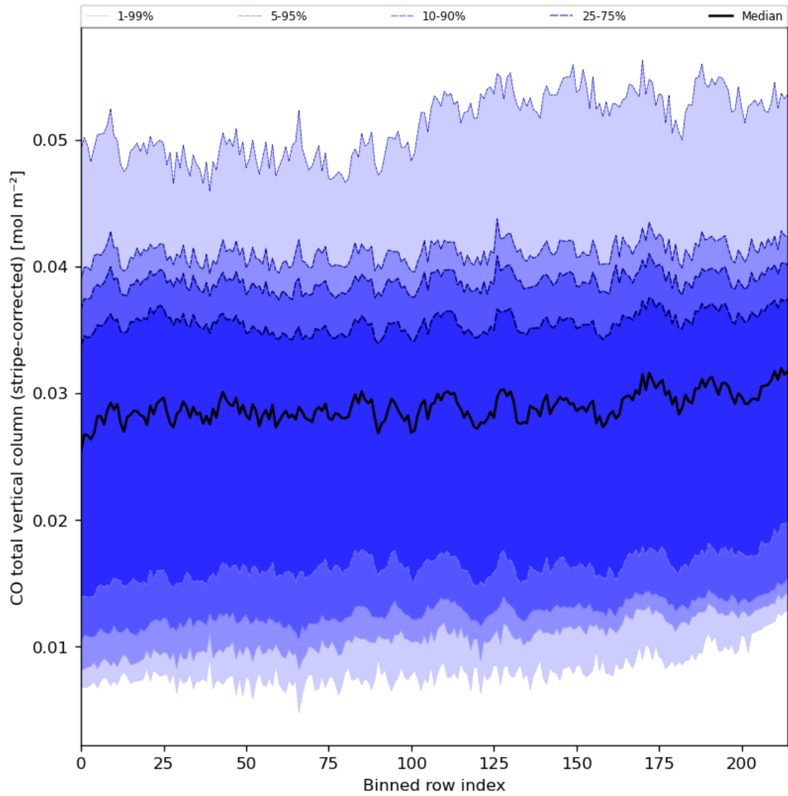
Figure 27: Along track statistics of “CO total vertical column (stripe-corrected)” for 2024-03-15 to 2024-03-17
