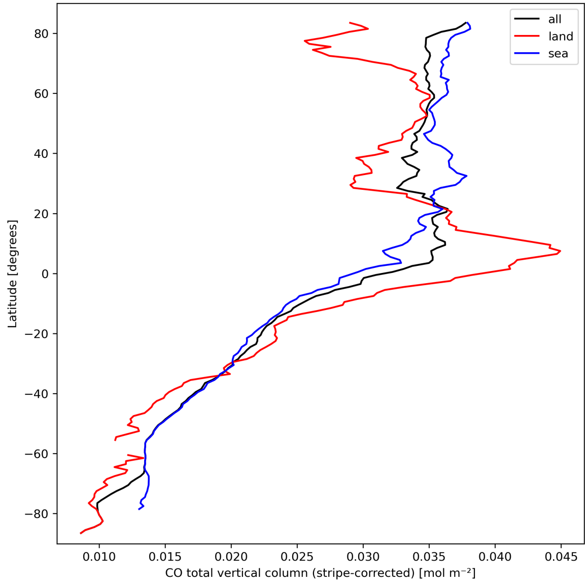
Figure 11: Zonal average of “CO total vertical column (stripe-corrected)” for 2024-03-15 to 2024-03-17.
