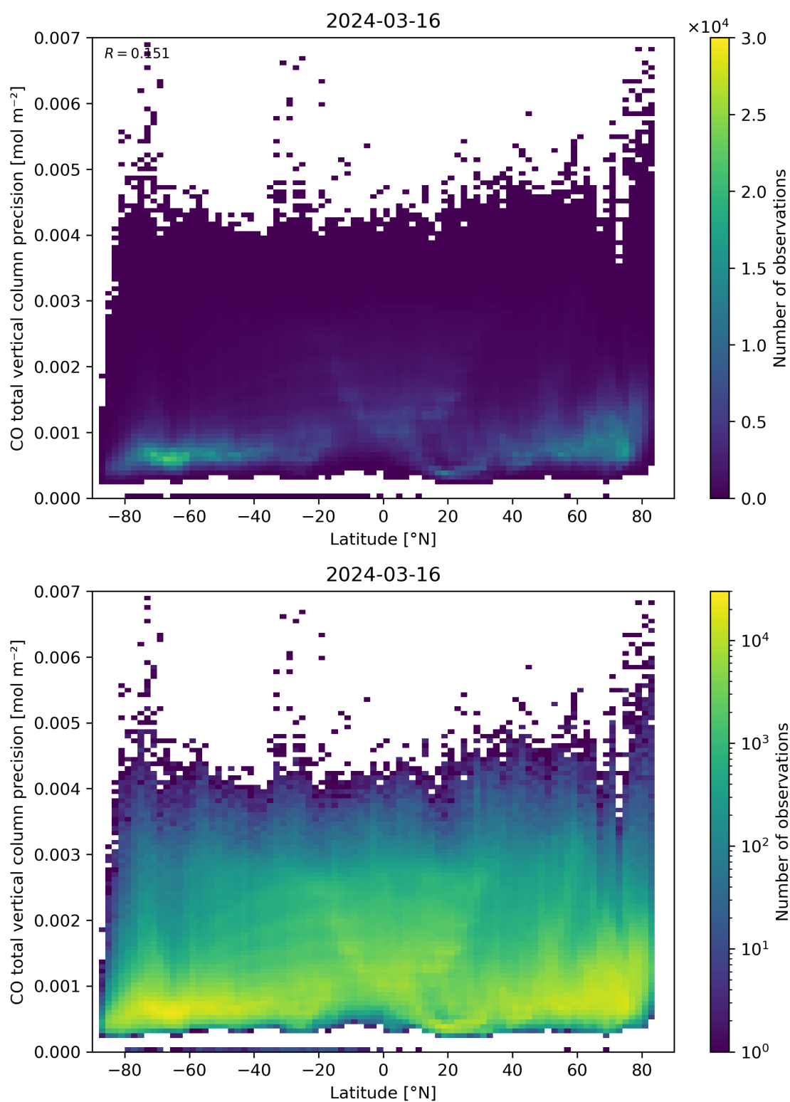
Figure 53: Scatter density plot of “Latitude” against “CO total vertical column precision” for 2024-03-15 to 2024-03-17.
