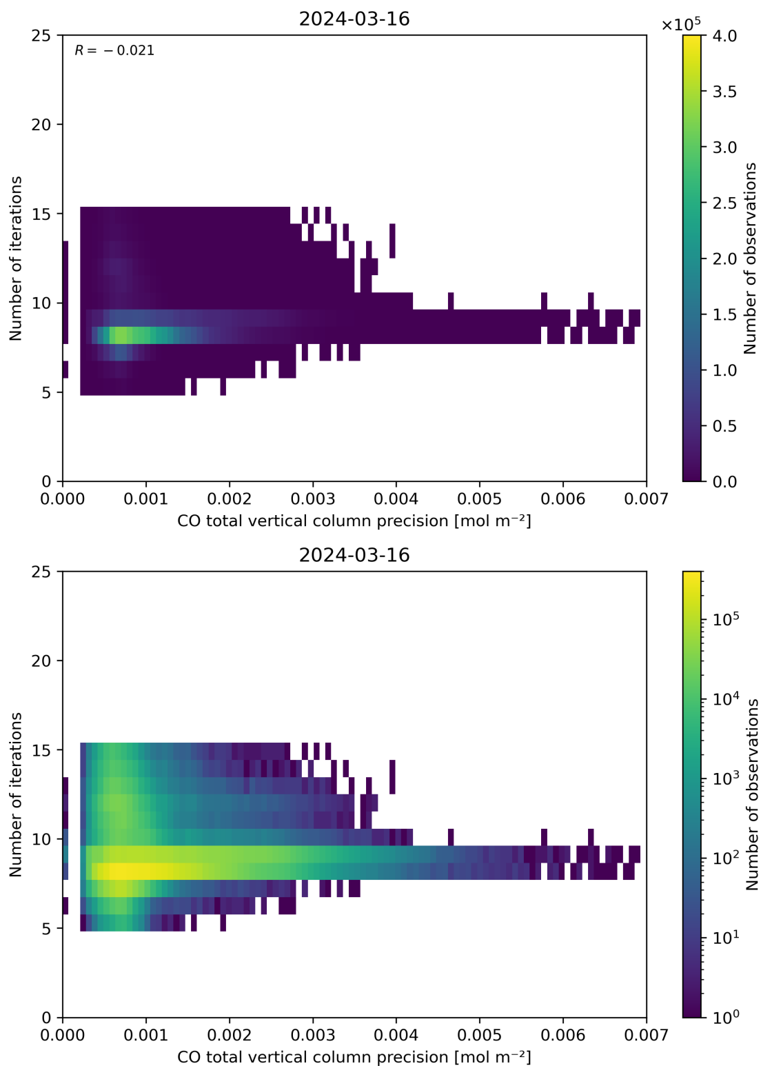
Figure 46: Scatter density plot of “CO total vertical column precision” against “Number of iterations” for 2024-03-15 to 2024-03-17.
