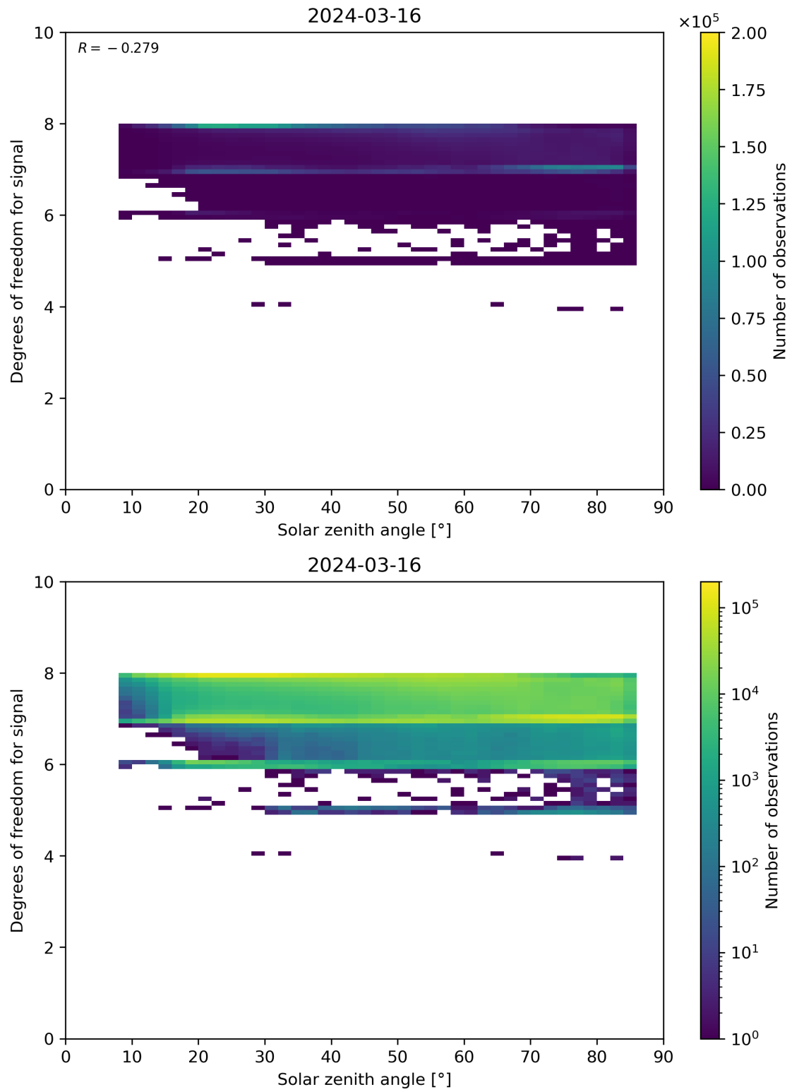
Figure 65: Scatter density plot of “Solar zenith angle” against “Degrees of freedom for signal” for 2024-03-15 to 2024-03-17.
