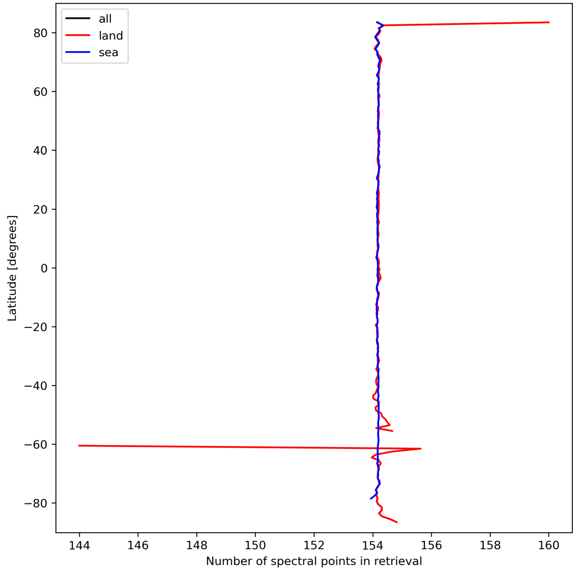
Figure 13: Zonal average of “Number of spectral points in retrieval” for 2024-03-15 to 2024-03-17.
