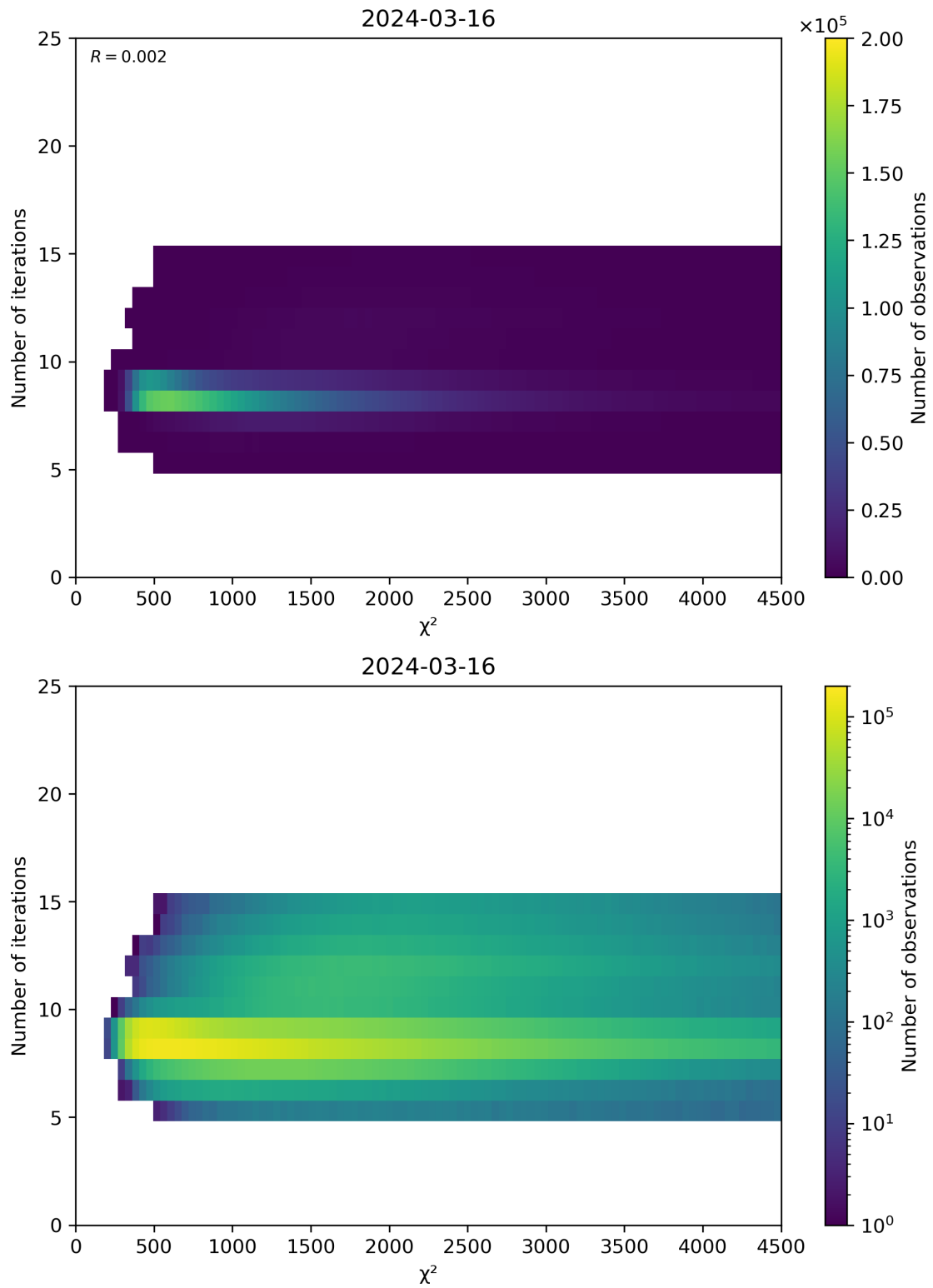
Figure 49: Scatter density plot of “ \chi^2 ” against “Number of iterations” for 2024-03-15 to 2024-03-17.
