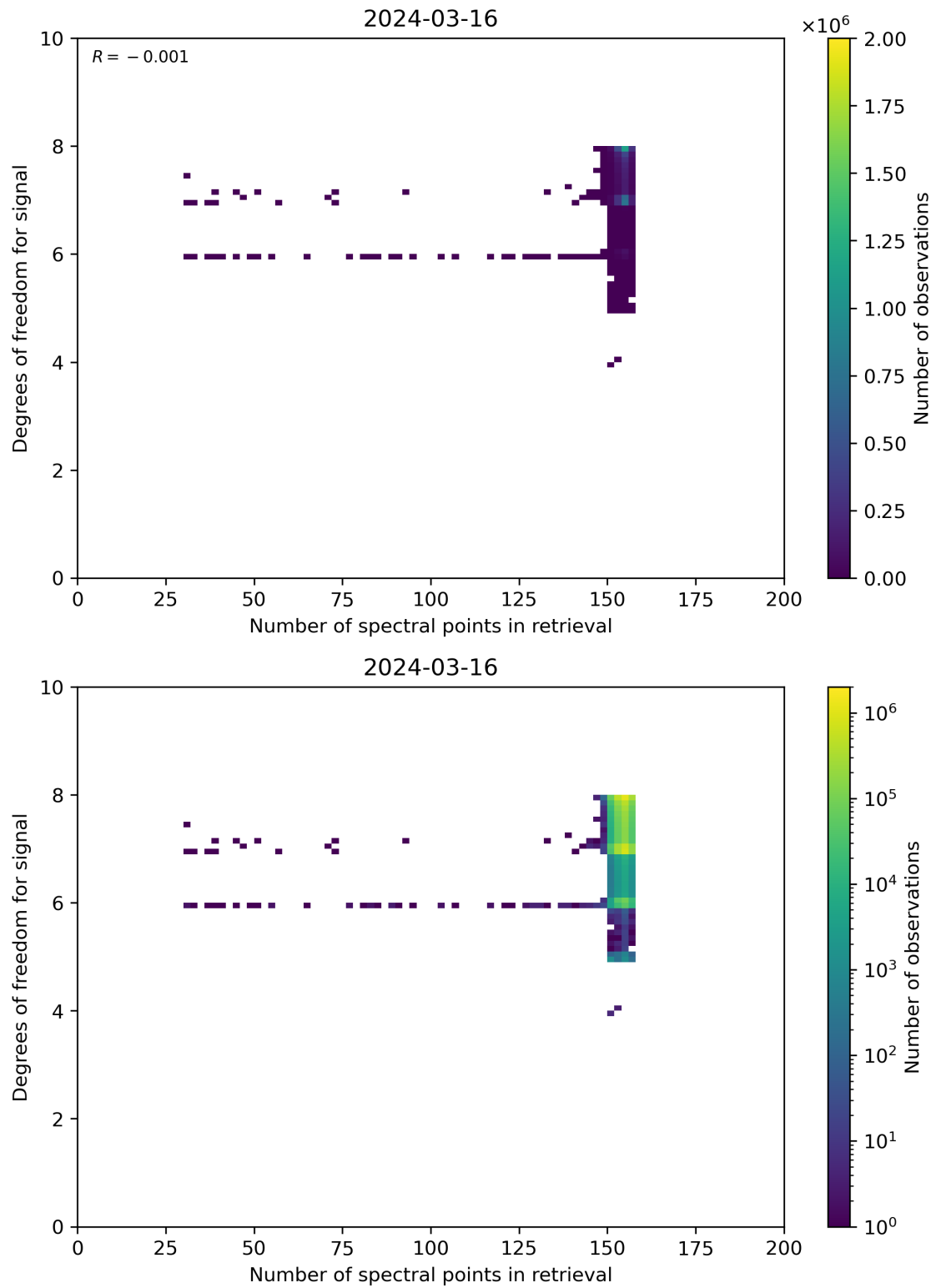
Figure 59: Scatter density plot of “Number of spectral points in retrieval” against “Degrees of freedom for signal” for 2024-03-15 to 2024-03-17.
