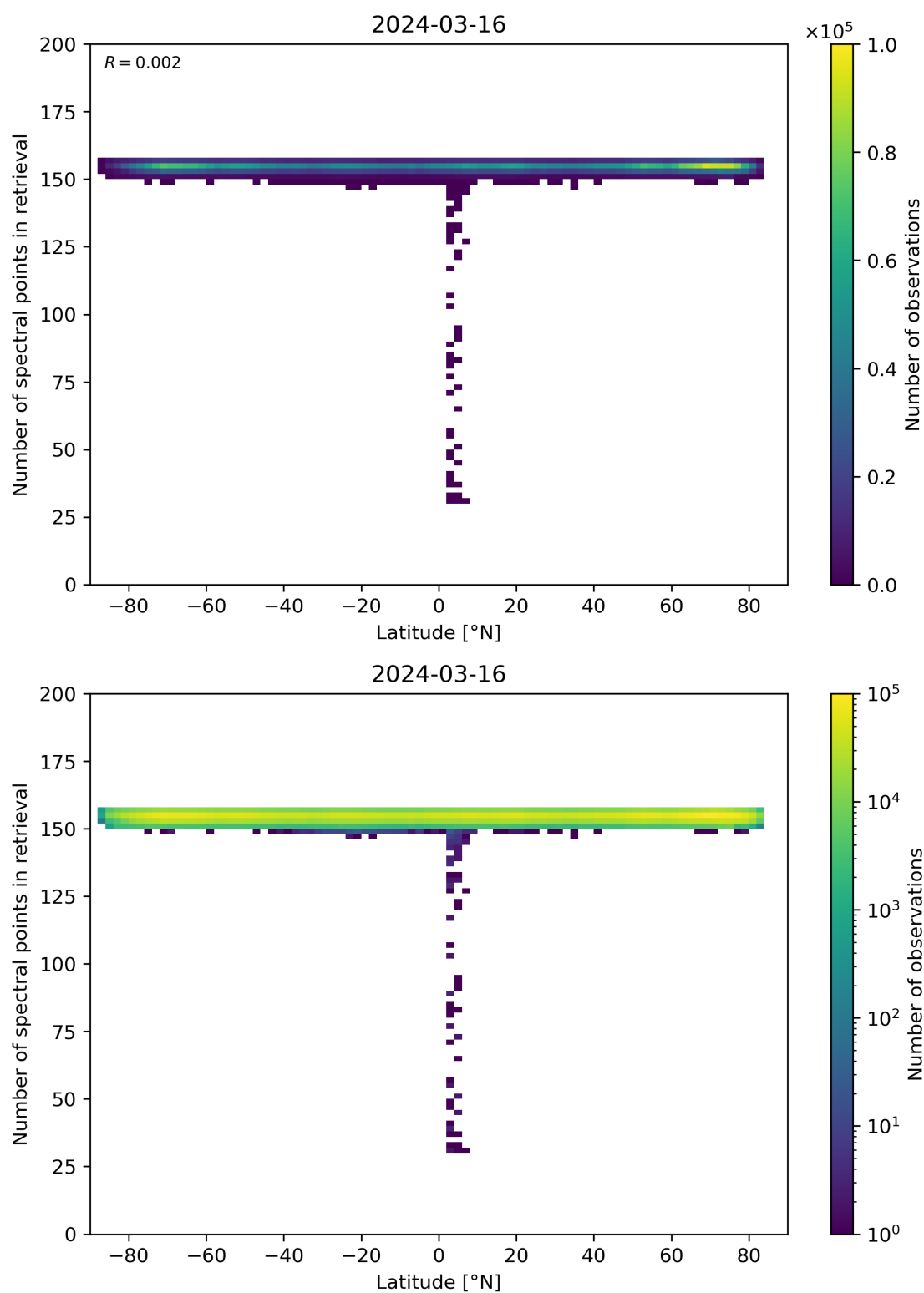
Figure 57: Scatter density plot of “Latitude” against “Number of spectral points in retrieval” for 2024-03-15 to 2024-03-17.
