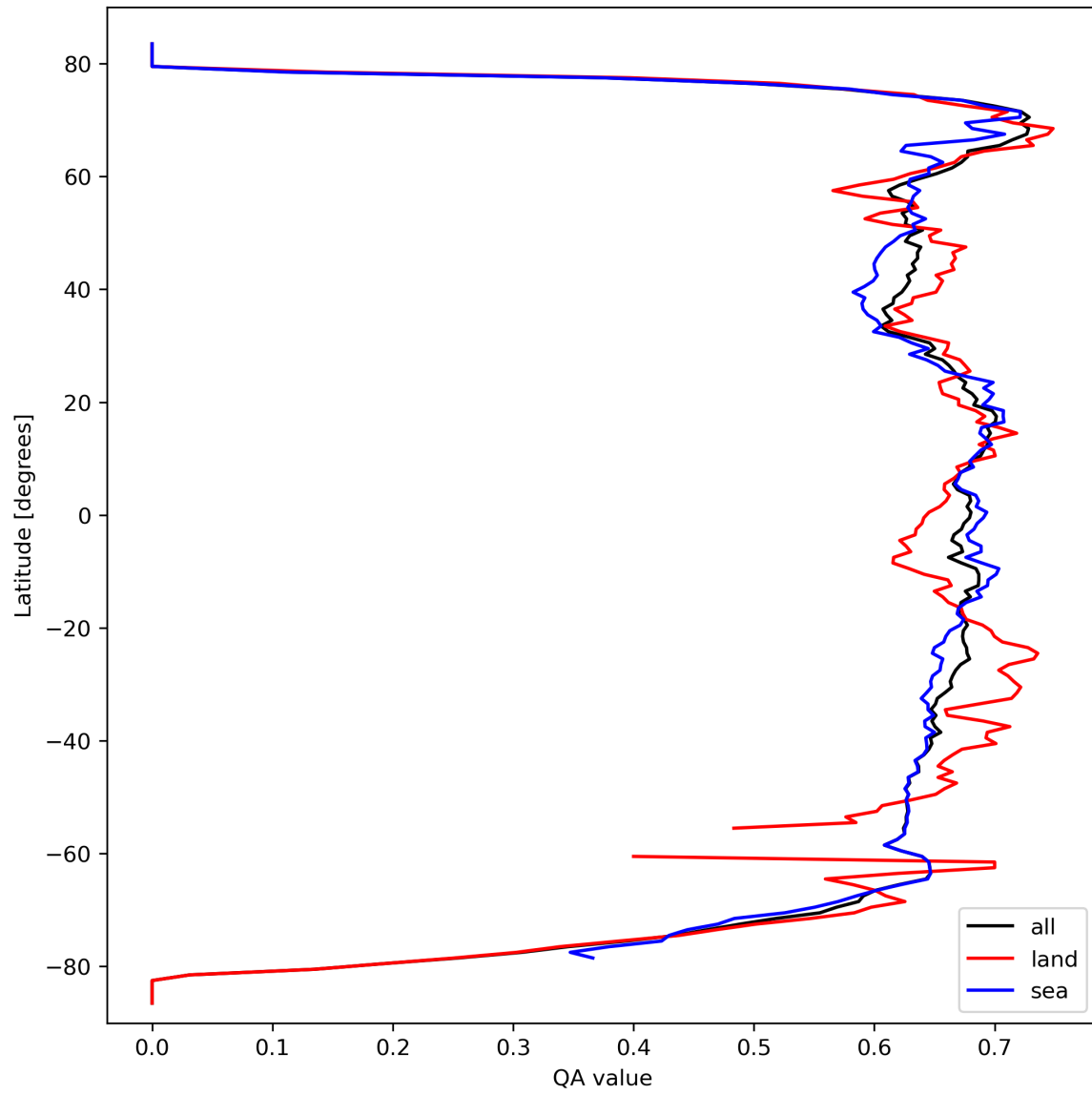
Figure 9: Zonal average of “QA value” for 2024-03-15 to 2024-03-17.
