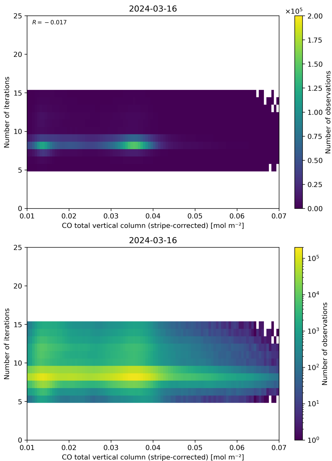
Figure 39: Scatter density plot of “CO total vertical column (stripe-corrected)” against “Number of iterations” for 2024-03-15 to 2024-03-17.
