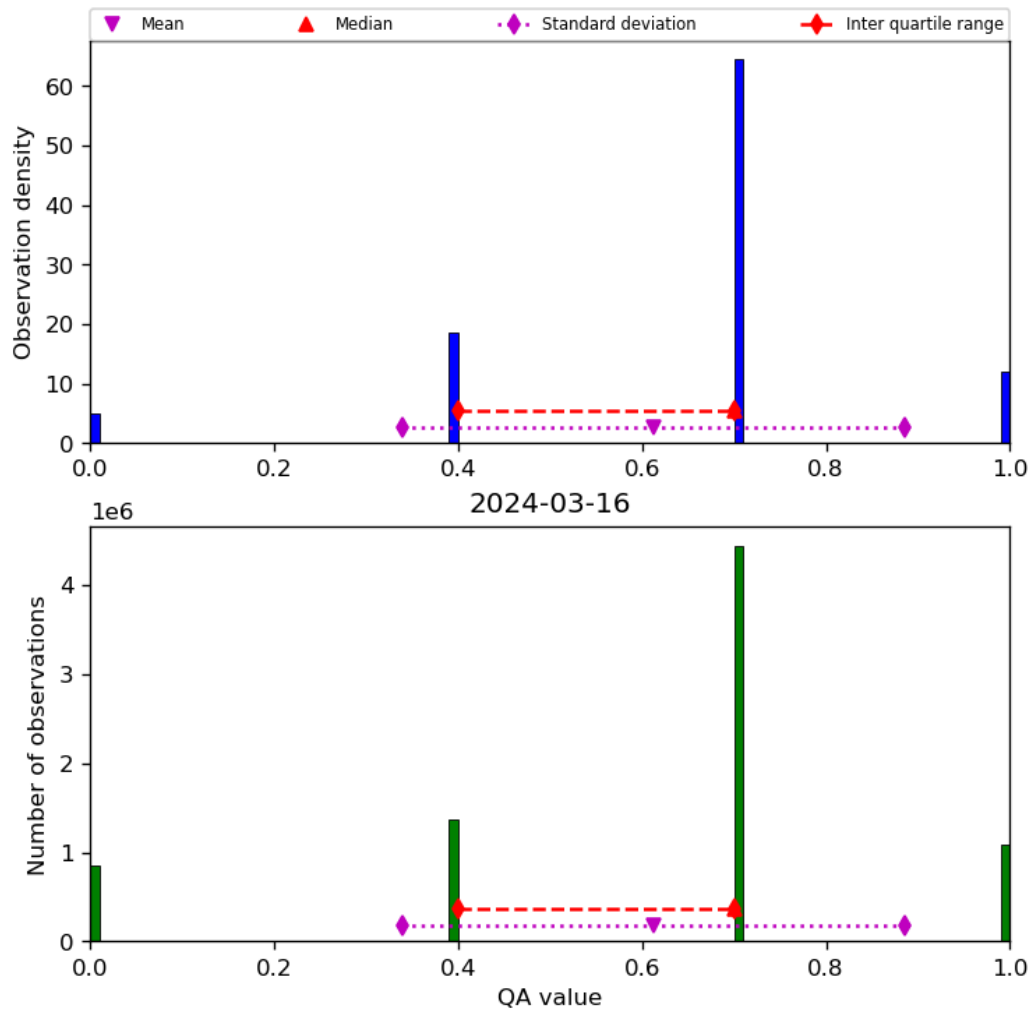
Figure 17: Histogram of “QA value” for 2024-03-15 to 2024-03-17
