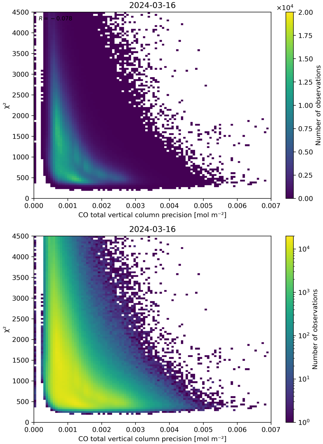
Figure 44: Scatter density plot of “CO total vertical column precision” against “ \chi^2 ” for 2024-03-15 to 2024-03-17.
