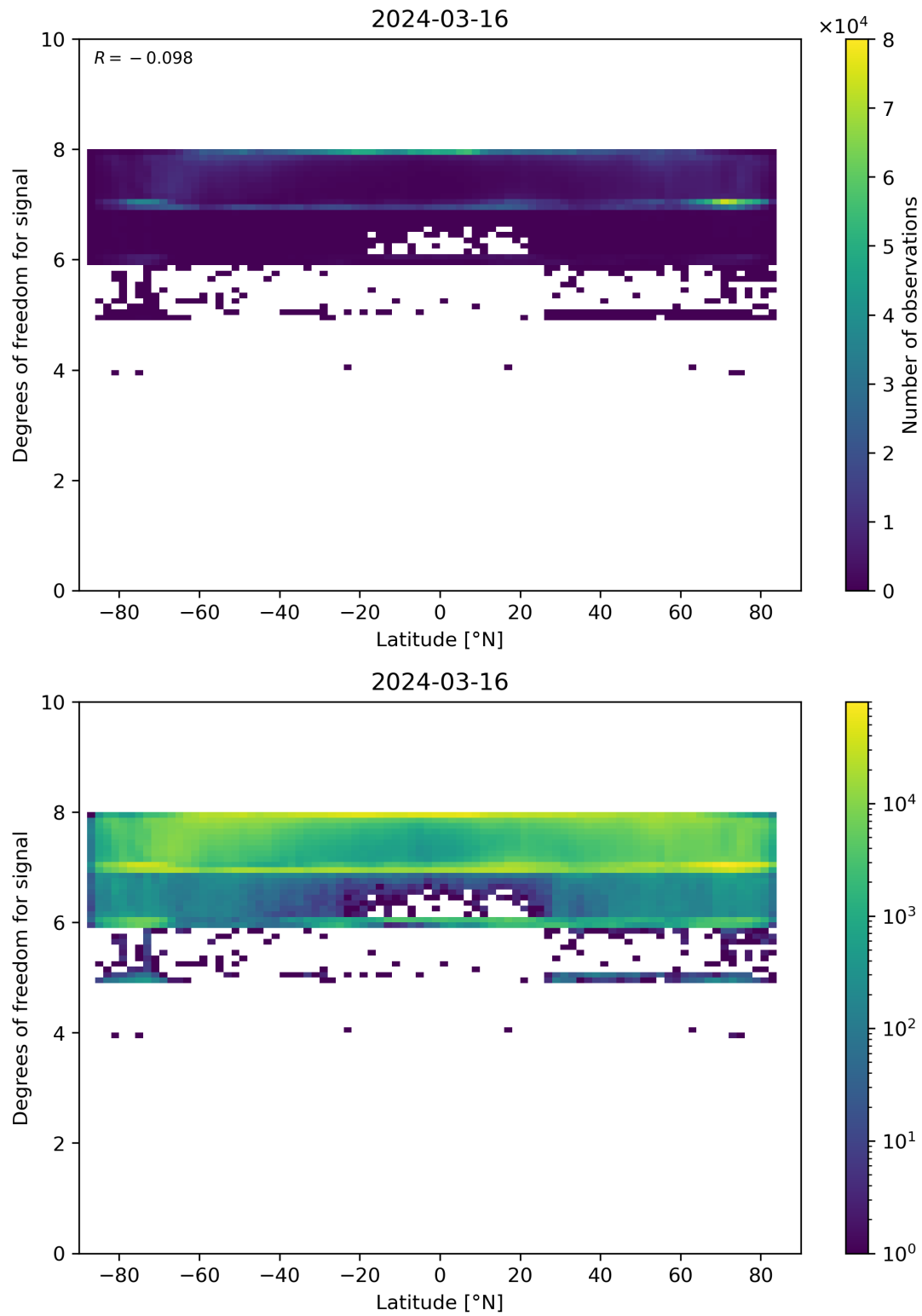
Figure 55: Scatter density plot of “Latitude” against “Degrees of freedom for signal” for 2024-03-15 to 2024-03-17.
