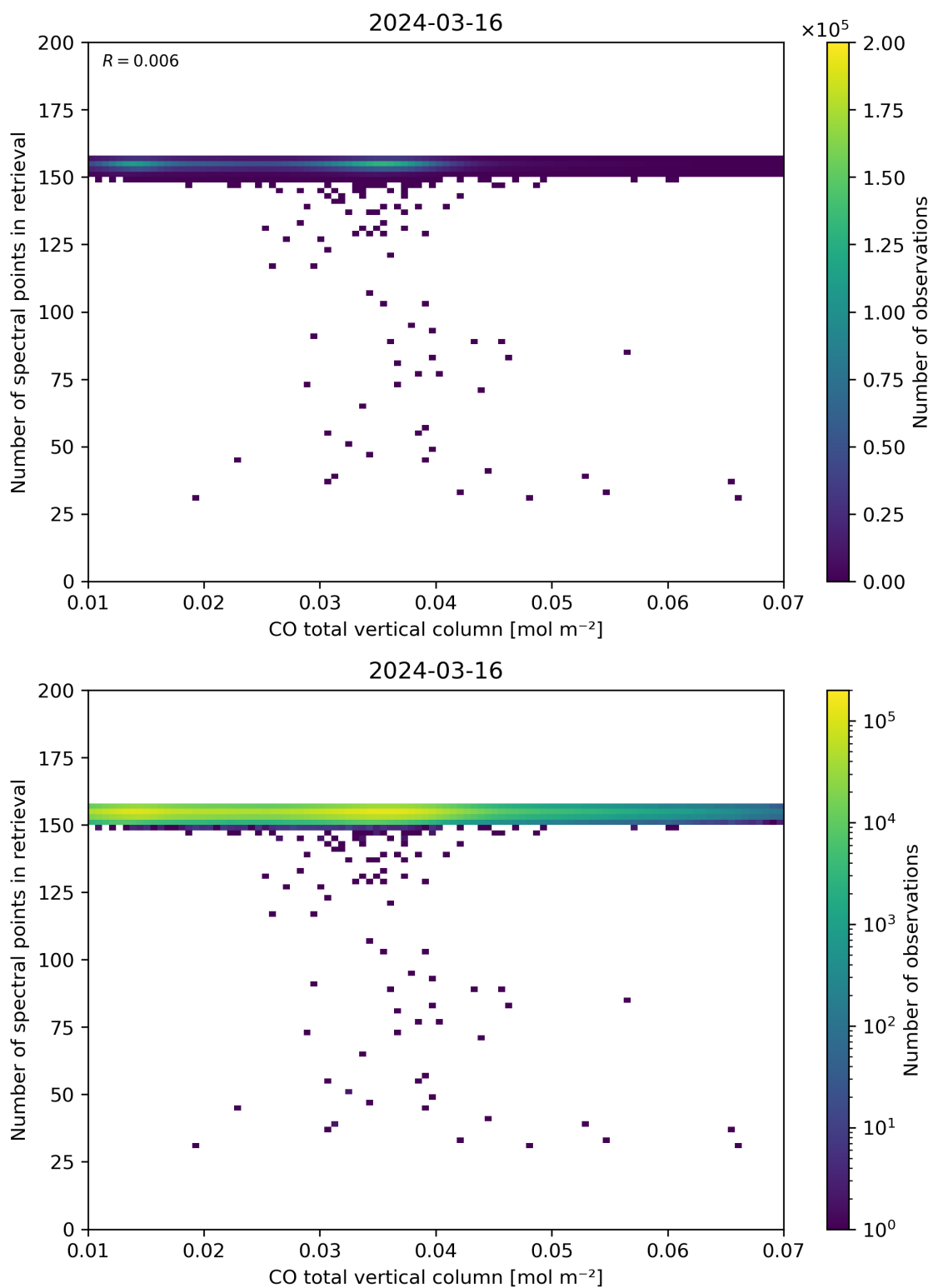
Figure 43: Scatter density plot of “CO total vertical column” against “Number of spectral points in retrieval” for 2024-03-15 to 2024-03-17.
