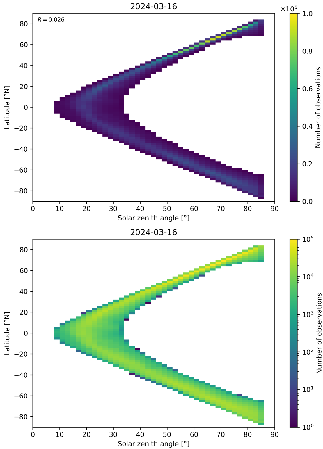
Figure 66: Scatter density plot of “Solar zenith angle” against “Latitude” for 2024-03-15 to 2024-03-17.
