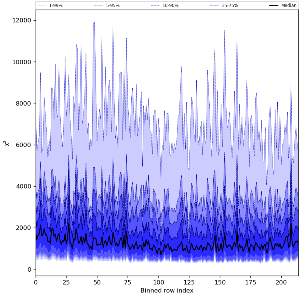
Figure 30: Along track statistics of “ \chi^2 ” for 2024-03-15 to 2024-03-17
