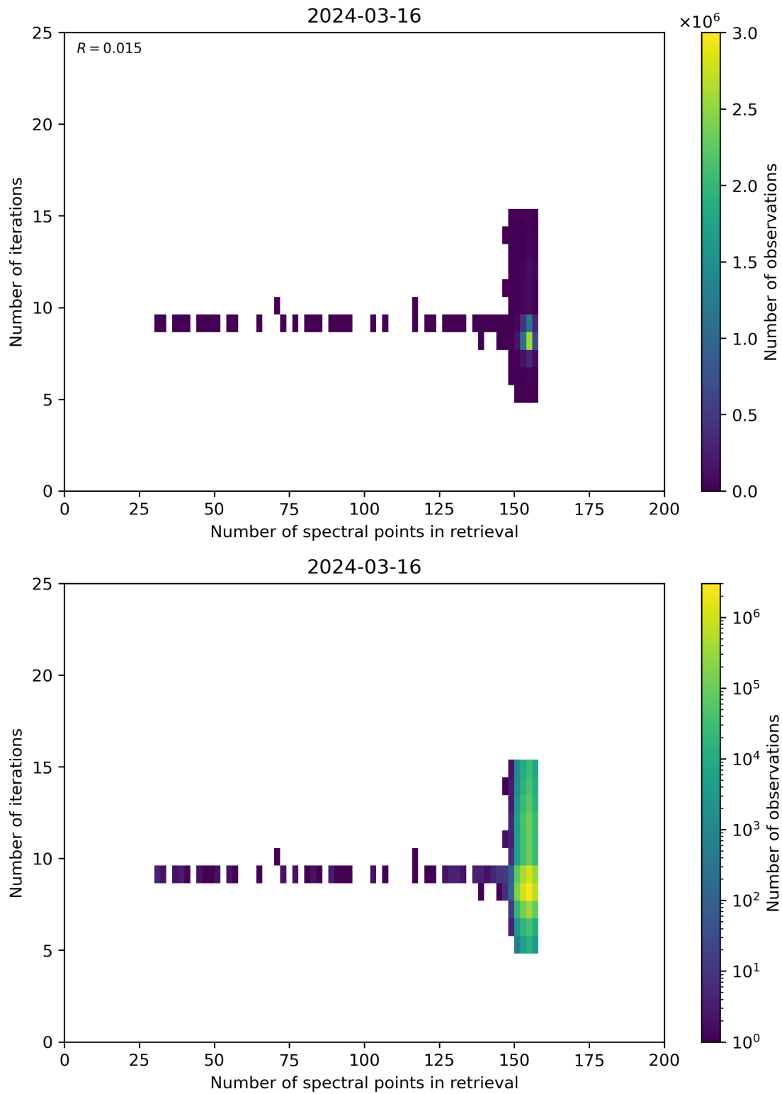
Figure 60: Scatter density plot of “Number of spectral points in retrieval” against “Number of iterations” for 2024-03-15 to 2024-03-17.
