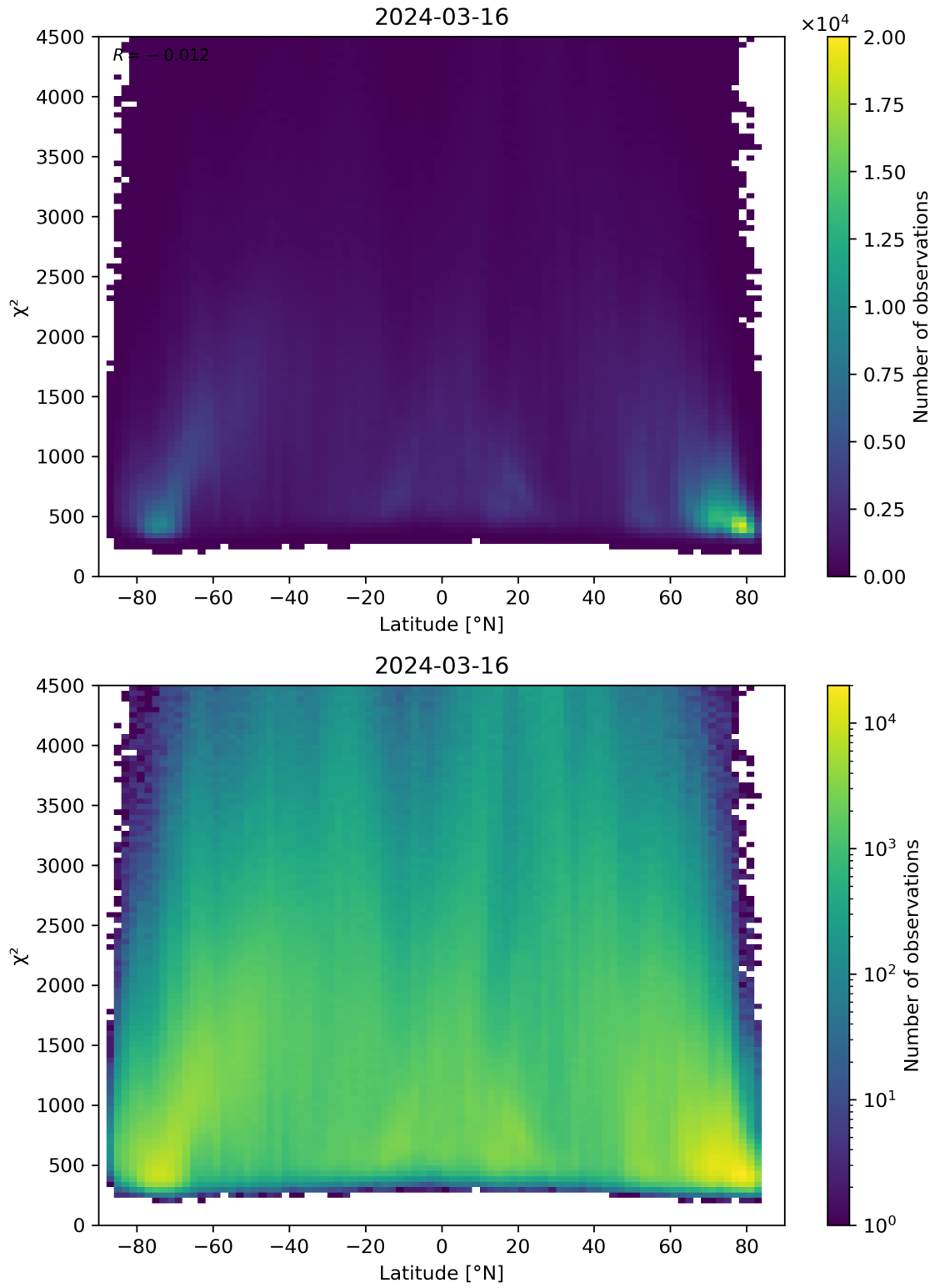
Figure 54: Scatter density plot of “Latitude” against “ \chi^2 ” for 2024-03-15 to 2024-03-17.
