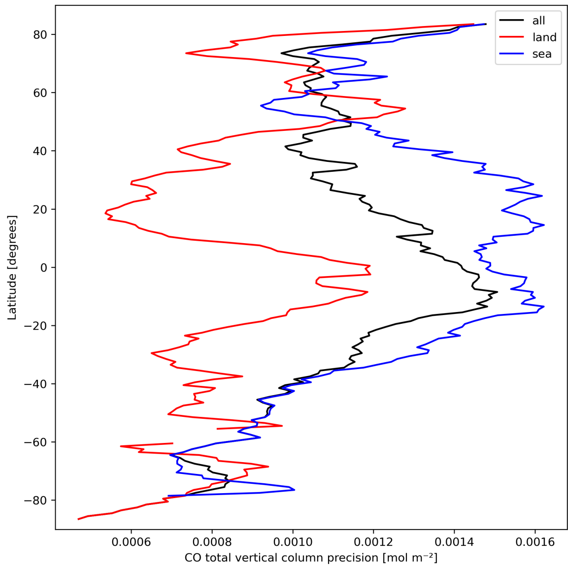
Figure 12: Zonal average of “CO total vertical column precision” for 2024-03-15 to 2024-03-17.
