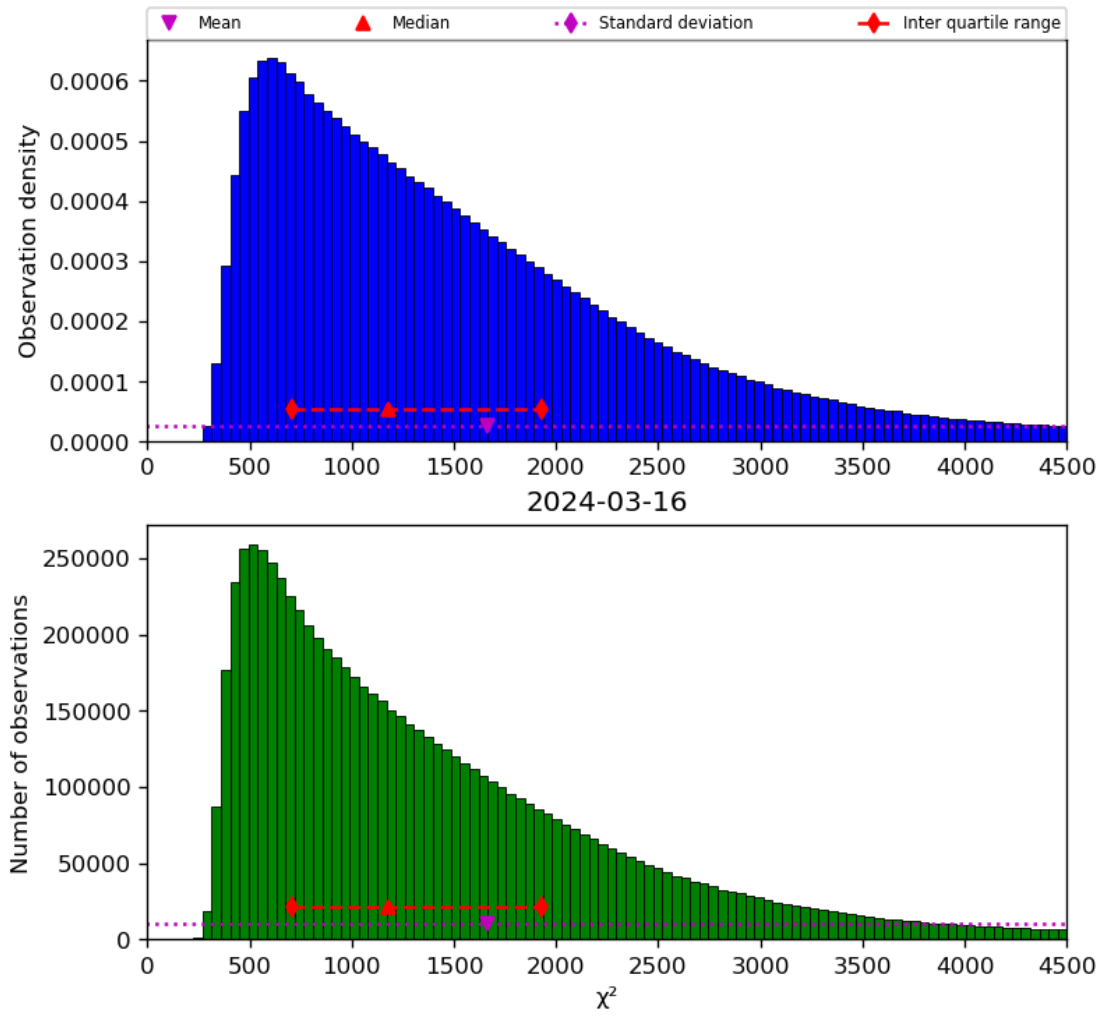
Figure 22: Histogram of “ \chi^2 ” for 2024-03-15 to 2024-03-17
