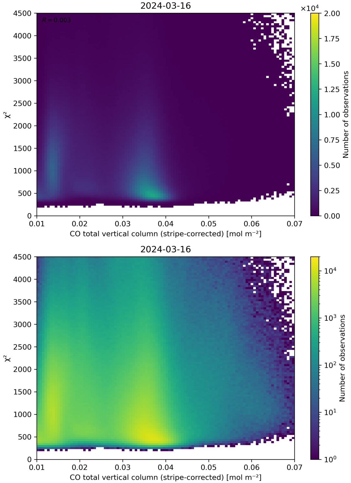
Figure 37: Scatter density plot of “CO total vertical column (stripe-corrected)” against “ \chi^2 ” for 2024-03-15 to 2024-03-17.
