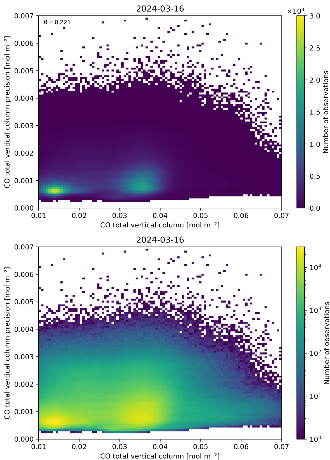
Figure 34: Scatter density plot of “CO total vertical column” against “CO total vertical column precision” for 2024-03-15 to 2024-03-17.
