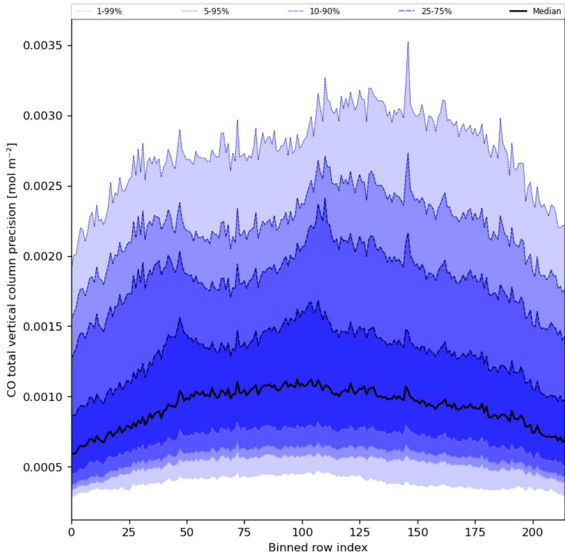
Figure 28: Along track statistics of “CO total vertical column precision” for 2024-03-15 to 2024-03-17
