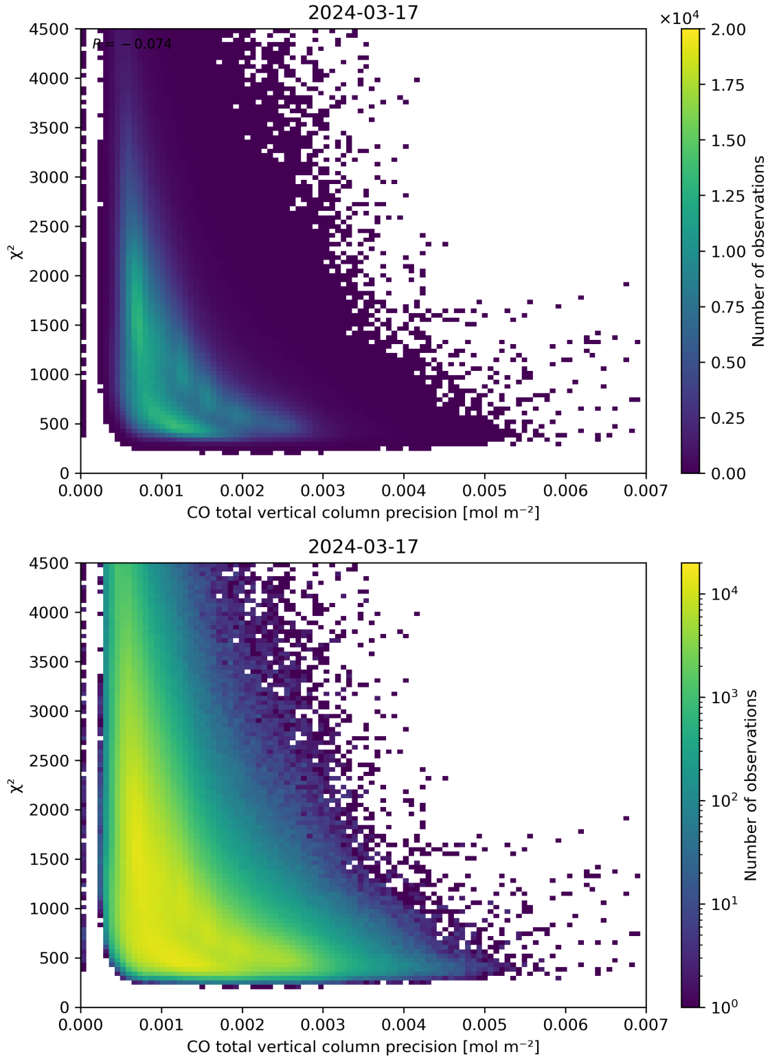
Figure 44: Scatter density plot of “CO total vertical column precision” against “ \chi^2 ” for 2024-03-16 to 2024-03-18.
