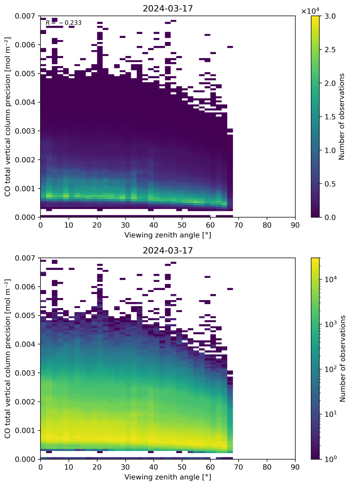
Figure 71: Scatter density plot of “Viewing zenith angle” against “CO total vertical column precision” for 2024-03-16 to 2024-03-18.
