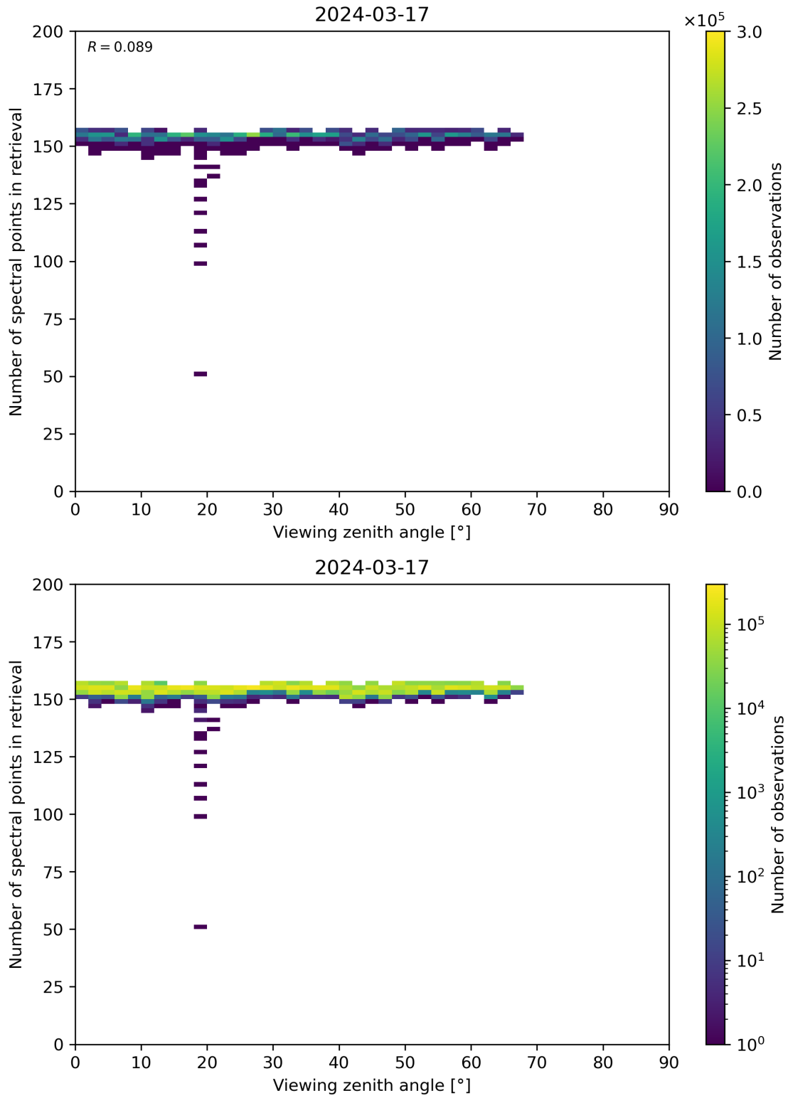
Figure 76: Scatter density plot of “Viewing zenith angle” against “Number of spectral points in retrieval” for 2024-03-16 to 2024-03-18.
