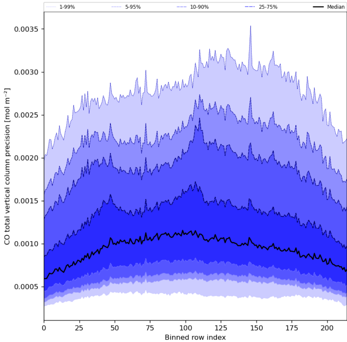
Figure 28: Along track statistics of “CO total vertical column precision” for 2024-03-16 to 2024-03-18
