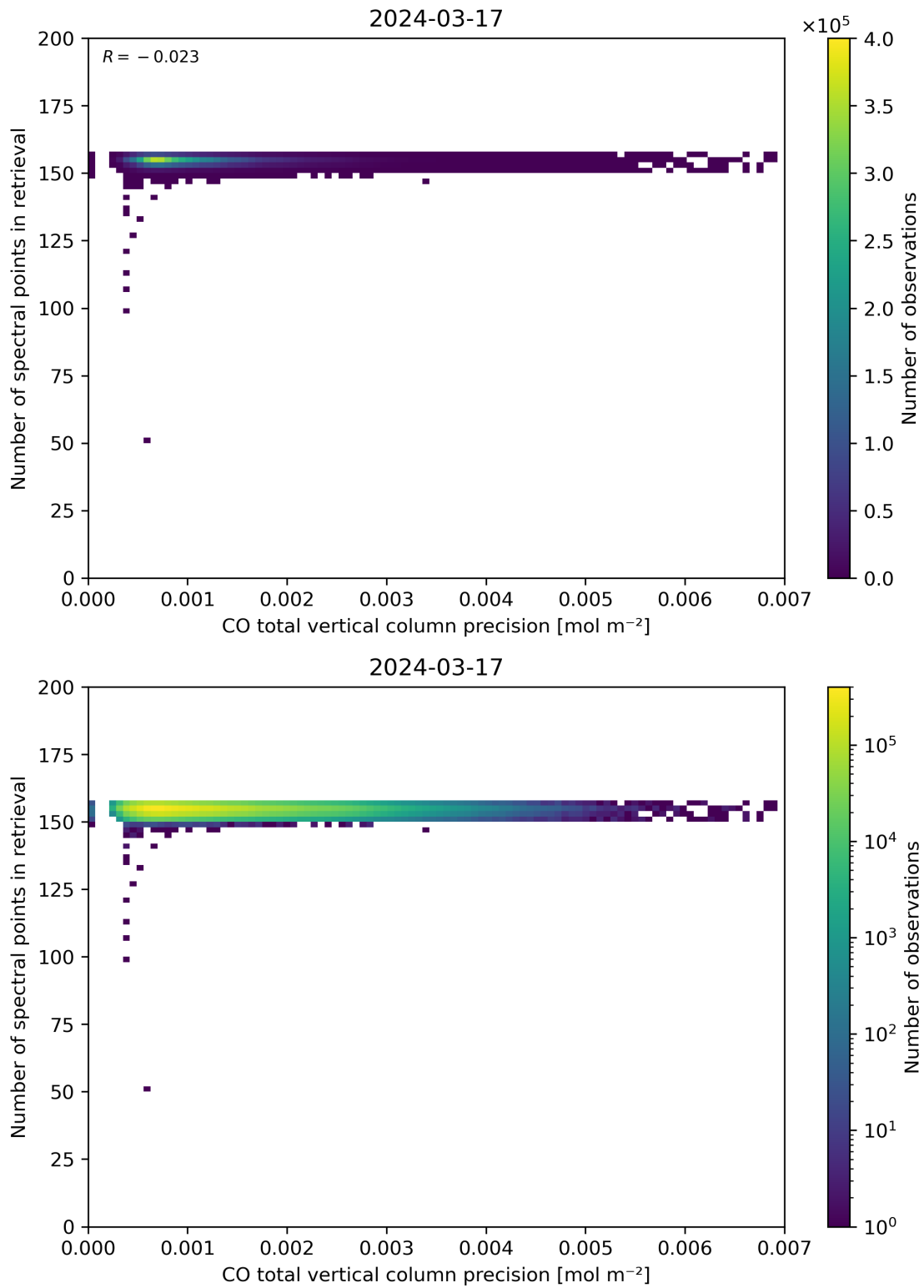
Figure 47: Scatter density plot of “CO total vertical column precision” against “Number of spectral points in retrieval” for 2024-03-16 to 2024-03-18.
