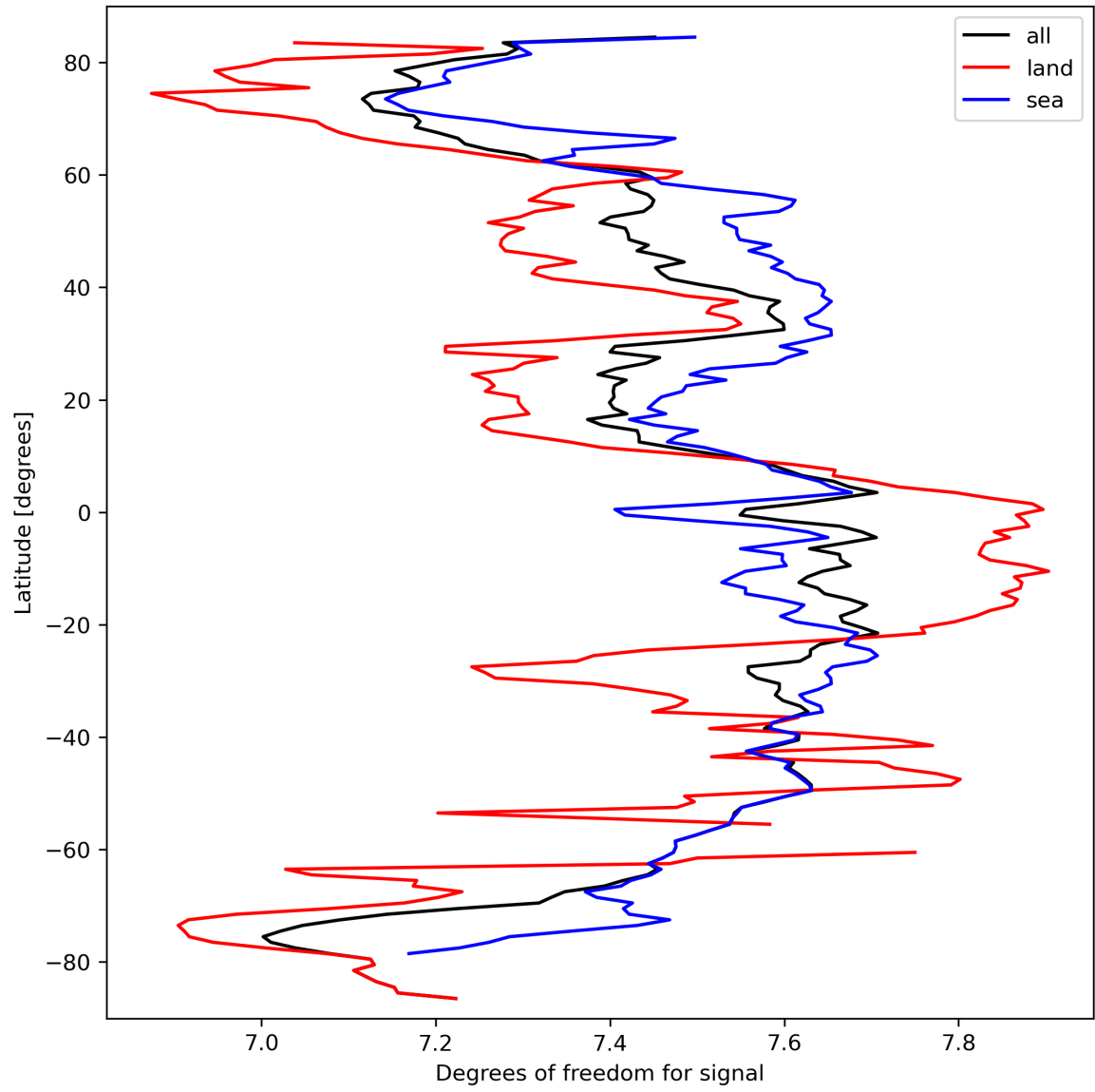
Figure 15: Zonal average of “Degrees of freedom for signal” for 2024-03-16 to 2024-03-18.
