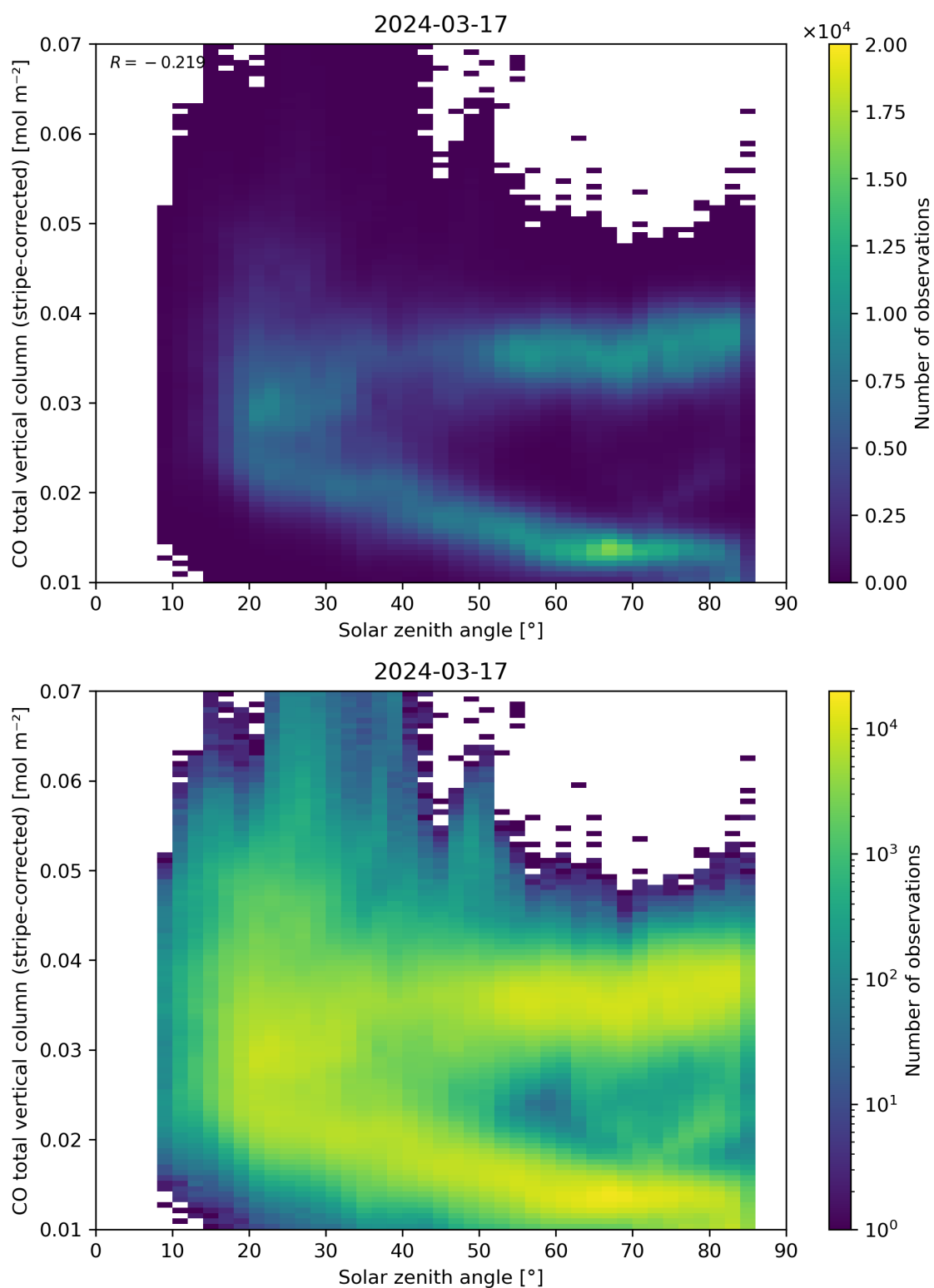
Figure 62: Scatter density plot of “Solar zenith angle” against “CO total vertical column (stripe-corrected)” for 2024-03-16 to 2024-03-18.
