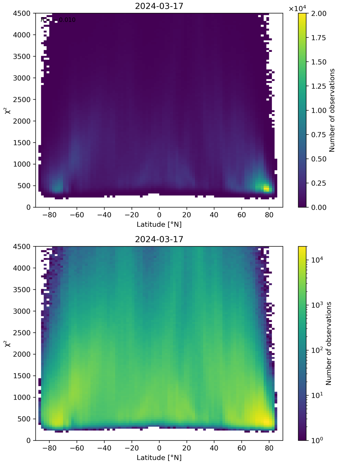
Figure 54: Scatter density plot of “Latitude” against “ \chi^2 ” for 2024-03-16 to 2024-03-18.
