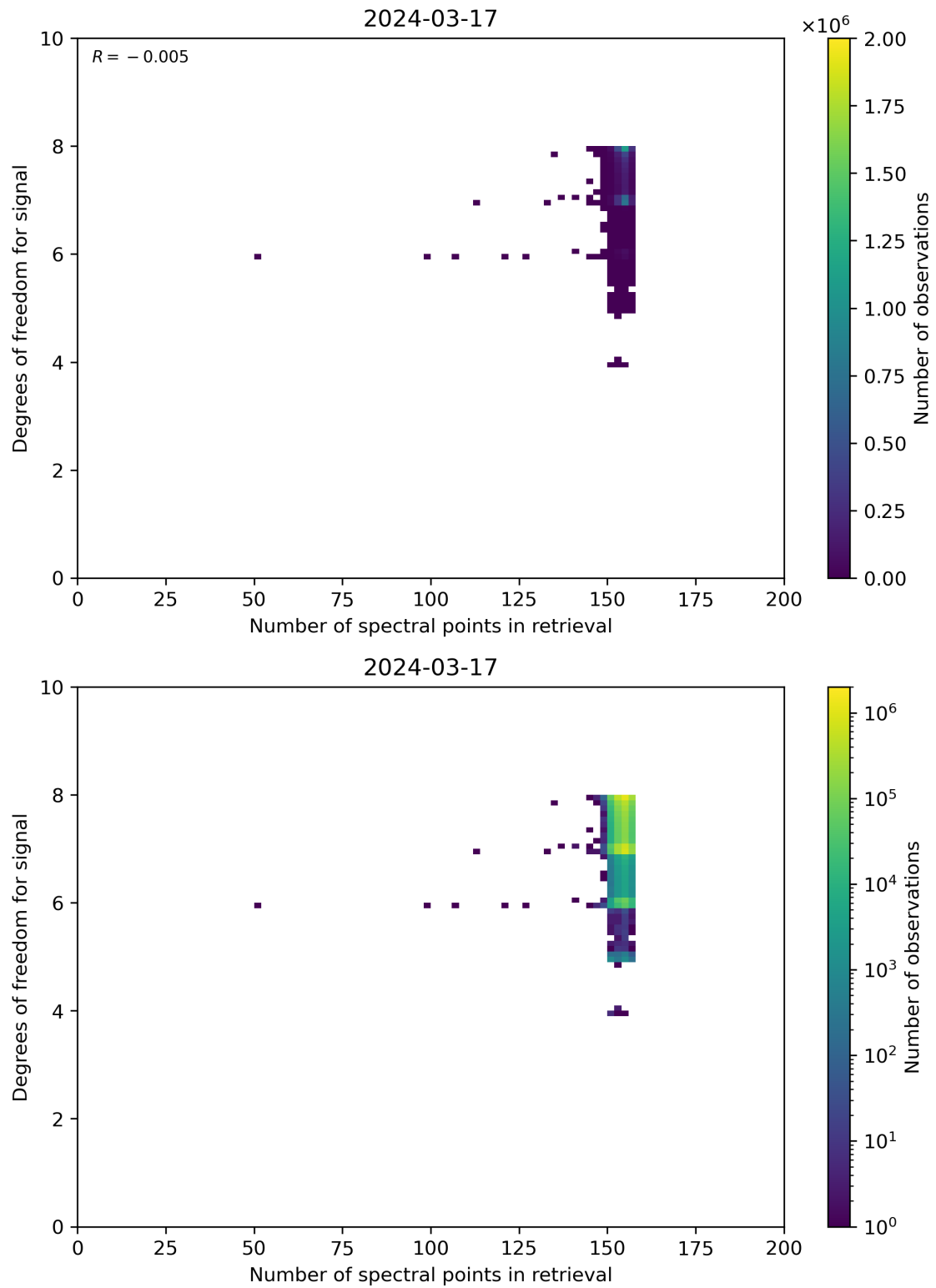
Figure 59: Scatter density plot of “Number of spectral points in retrieval” against “Degrees of freedom for signal” for 2024-03-16 to 2024-03-18.
