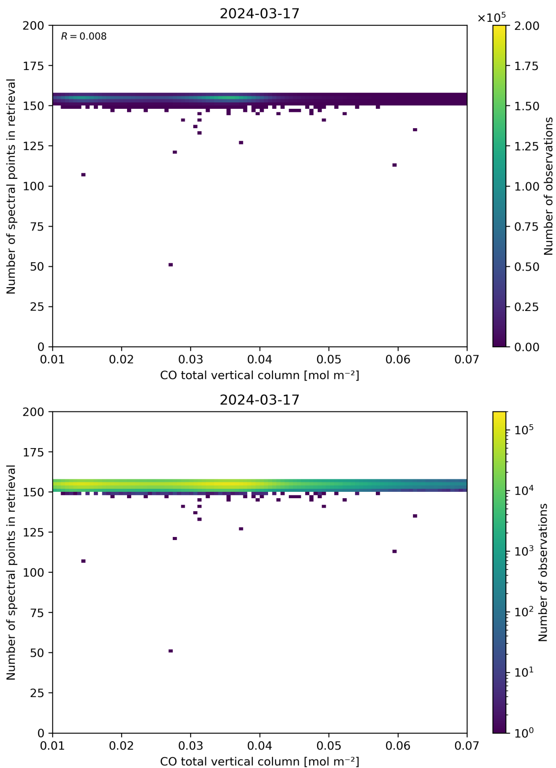
Figure 43: Scatter density plot of “CO total vertical column” against “Number of spectral points in retrieval” for 2024-03-16 to 2024-03-18.
