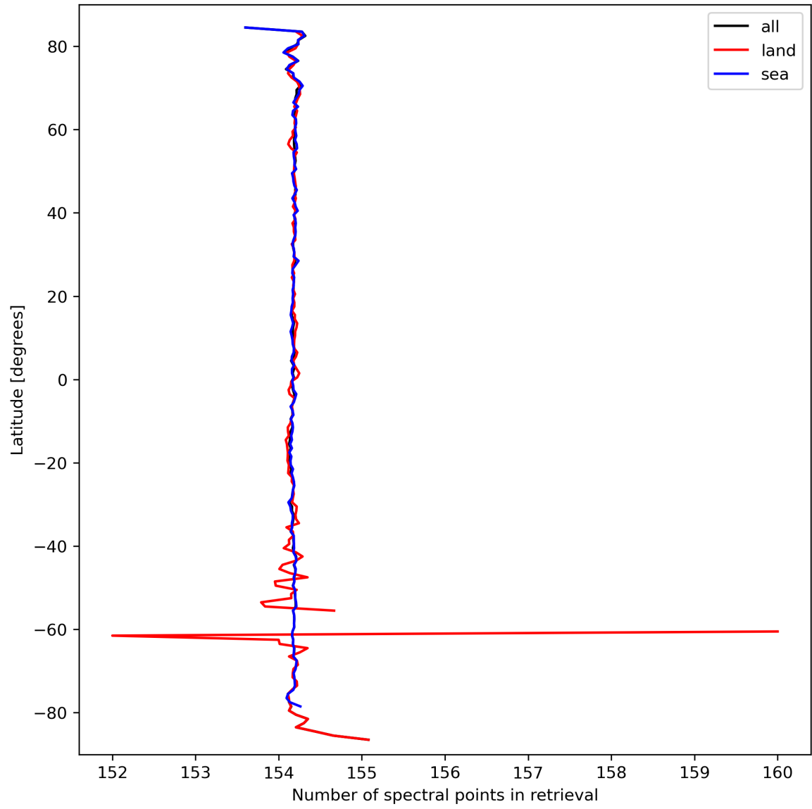
Figure 13: Zonal average of “Number of spectral points in retrieval” for 2024-03-16 to 2024-03-18.
