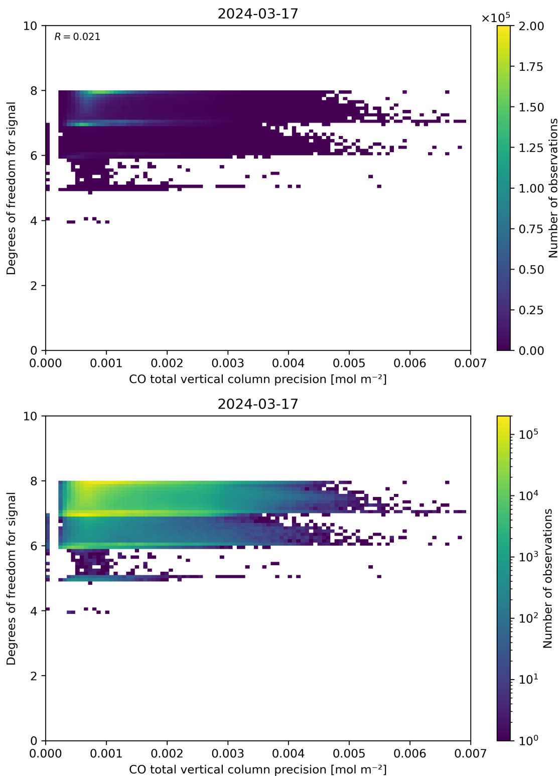
Figure 45: Scatter density plot of “CO total vertical column precision” against “Degrees of freedom for signal” for 2024-03-16 to 2024-03-18.
