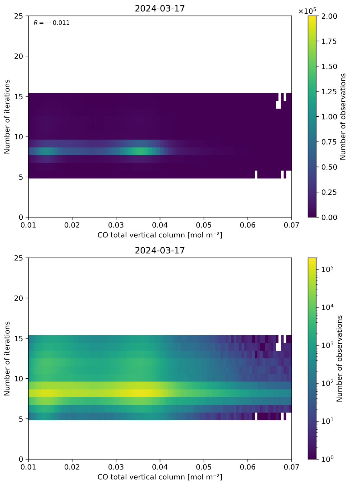
Figure 42: Scatter density plot of “CO total vertical column” against “Number of iterations” for 2024-03-16 to 2024-03-18.
