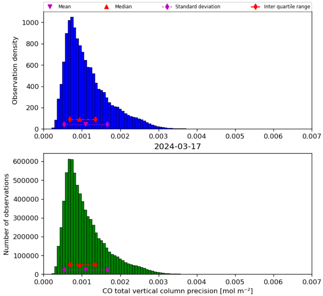
Figure 20: Histogram of “CO total vertical column precision” for 2024-03-16 to 2024-03-18
