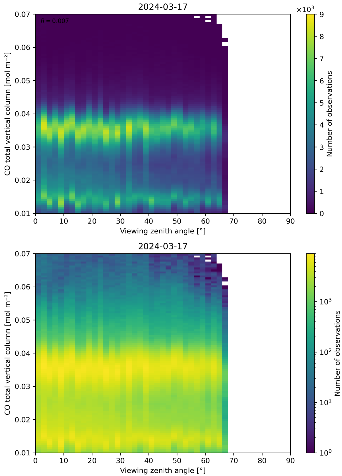
Figure 69: Scatter density plot of “Viewing zenith angle” against “CO total vertical column” for 2024-03-16 to 2024-03-18.
