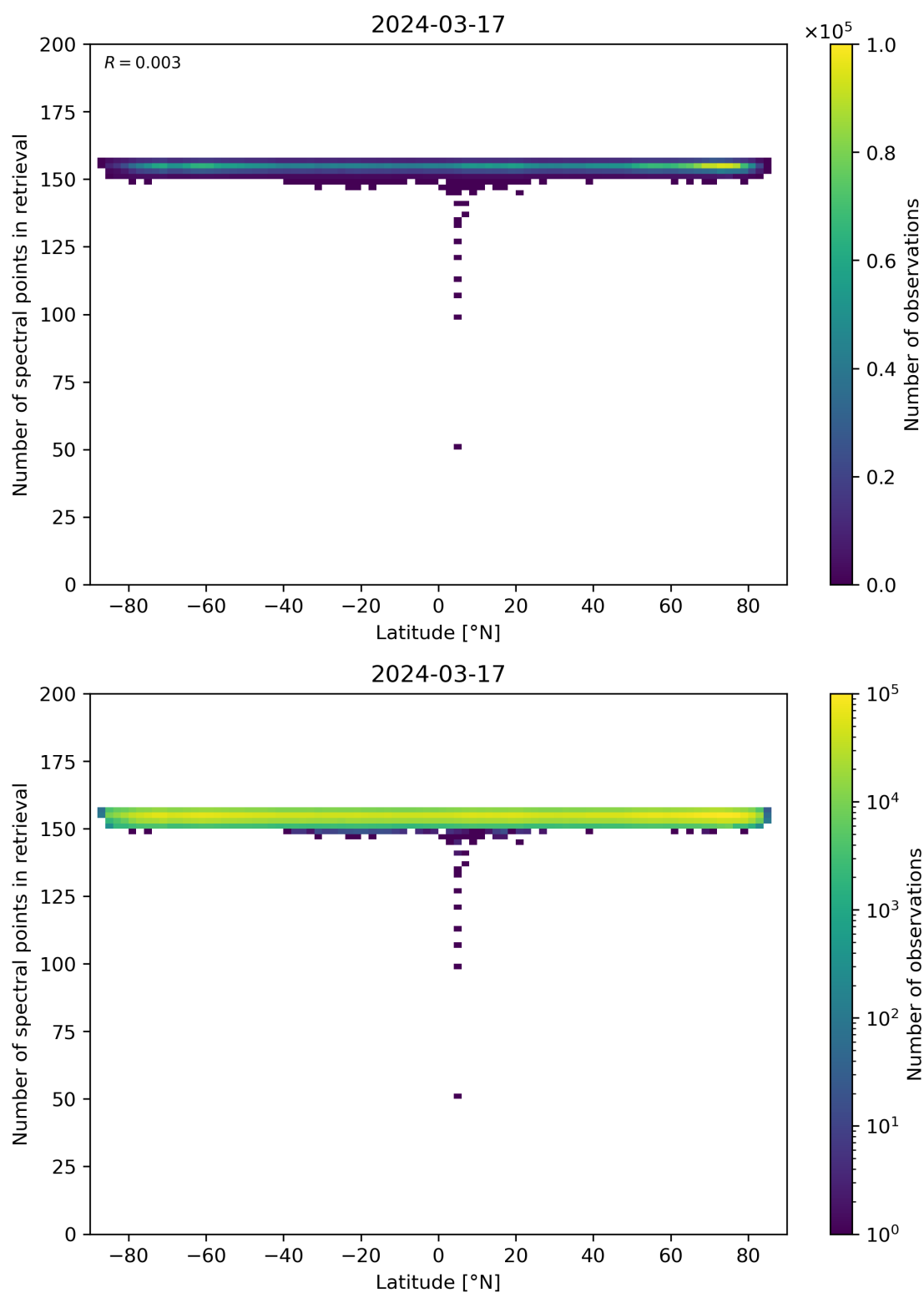
Figure 57: Scatter density plot of “Latitude” against “Number of spectral points in retrieval” for 2024-03-16 to 2024-03-18.
