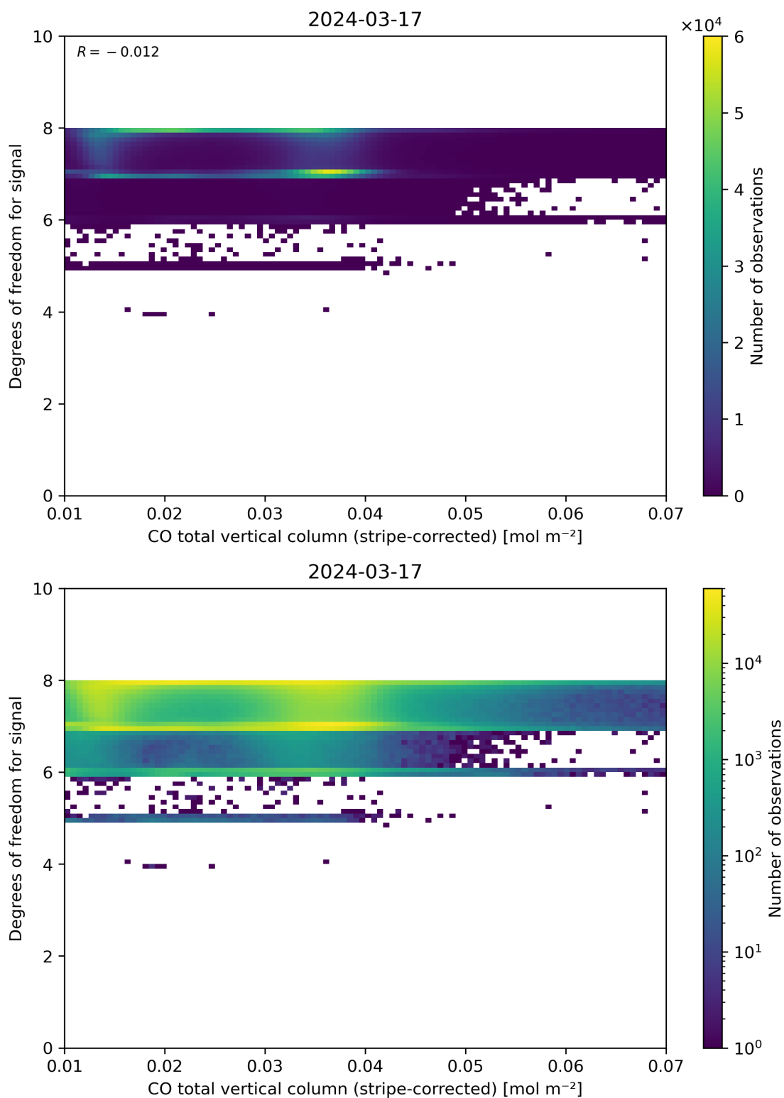
Figure 38: Scatter density plot of “CO total vertical column (stripe-corrected)” against “Degrees of freedom for signal” for 2024-03-16 to 2024-03-18.
