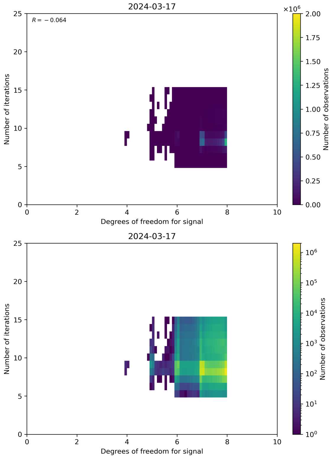
Figure 50: Scatter density plot of “Degrees of freedom for signal” against “Number of iterations” for 2024-03-16 to 2024-03-18.
