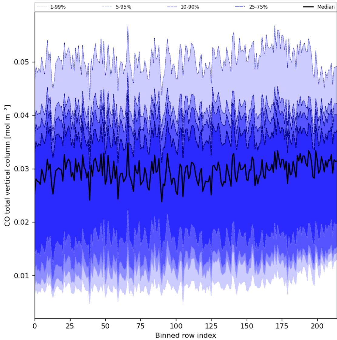
Figure 26: Along track statistics of “CO total vertical column” for 2024-03-16 to 2024-03-18
