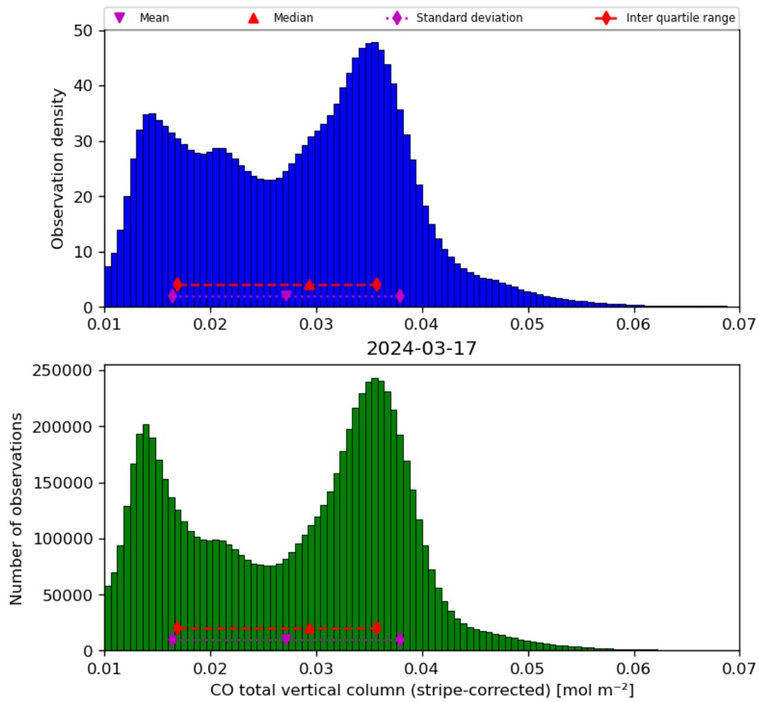
Figure 19: Histogram of “CO total vertical column (stripe-corrected)” for 2024-03-16 to 2024-03-18
