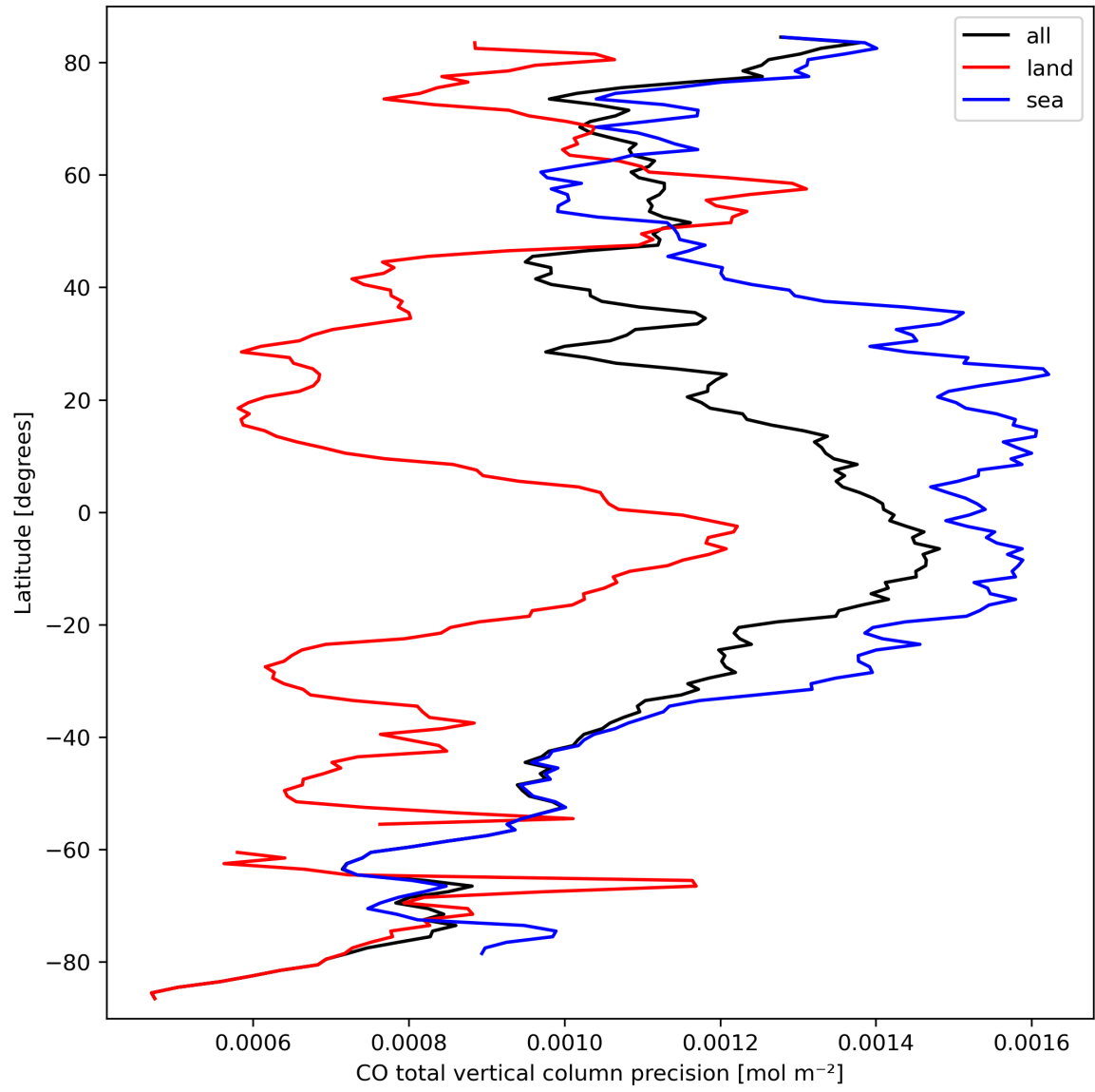
Figure 12: Zonal average of “CO total vertical column precision” for 2024-03-16 to 2024-03-18.
