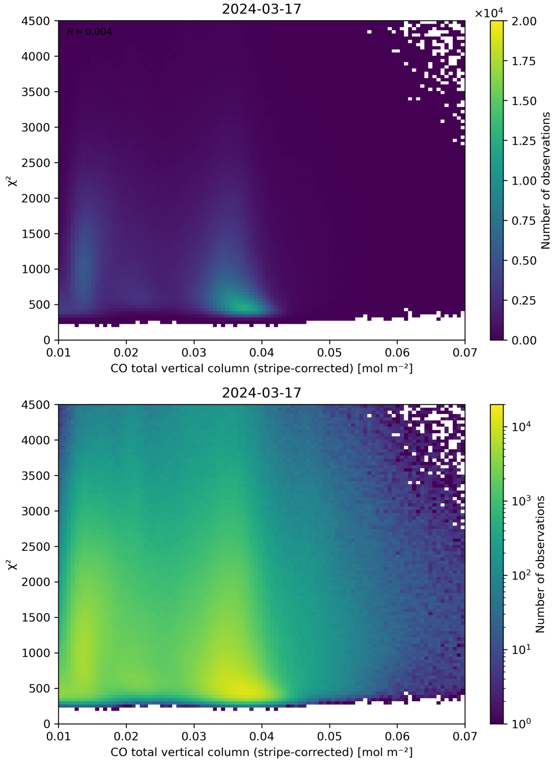
Figure 37: Scatter density plot of “CO total vertical column (stripe-corrected)” against “ \chi^2 ” for 2024-03-16 to 2024-03-18.
