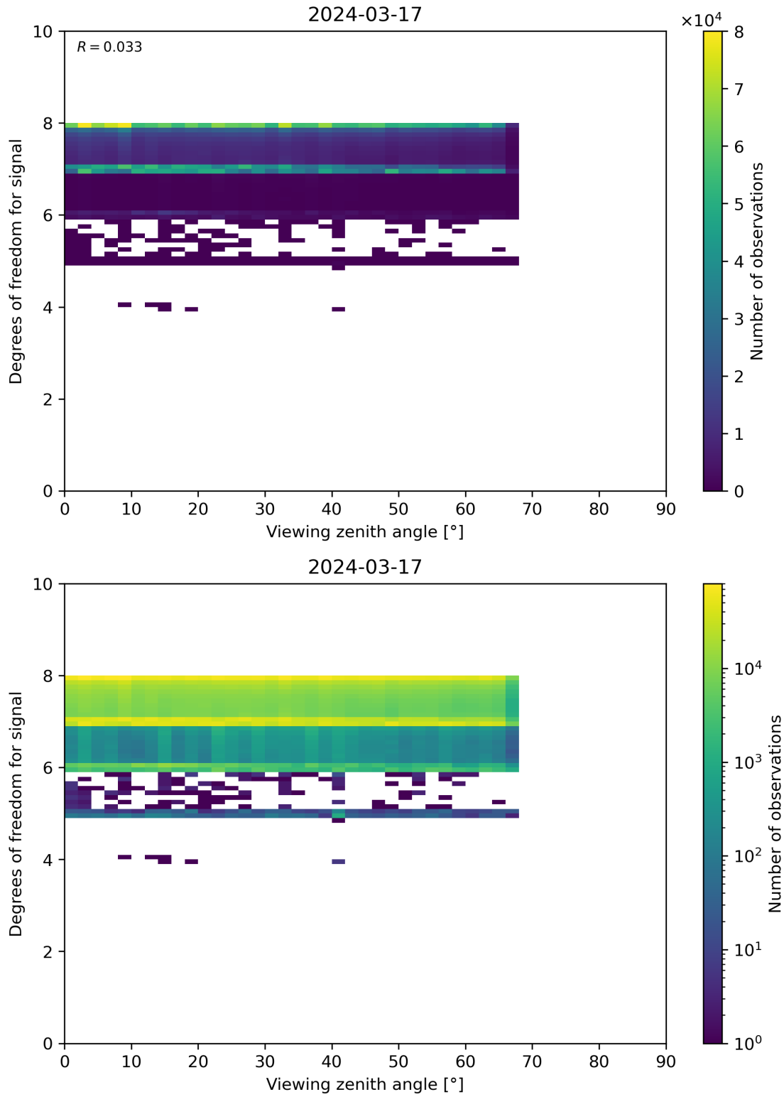
Figure 73: Scatter density plot of “Viewing zenith angle” against “Degrees of freedom for signal” for 2024-03-16 to 2024-03-18.
