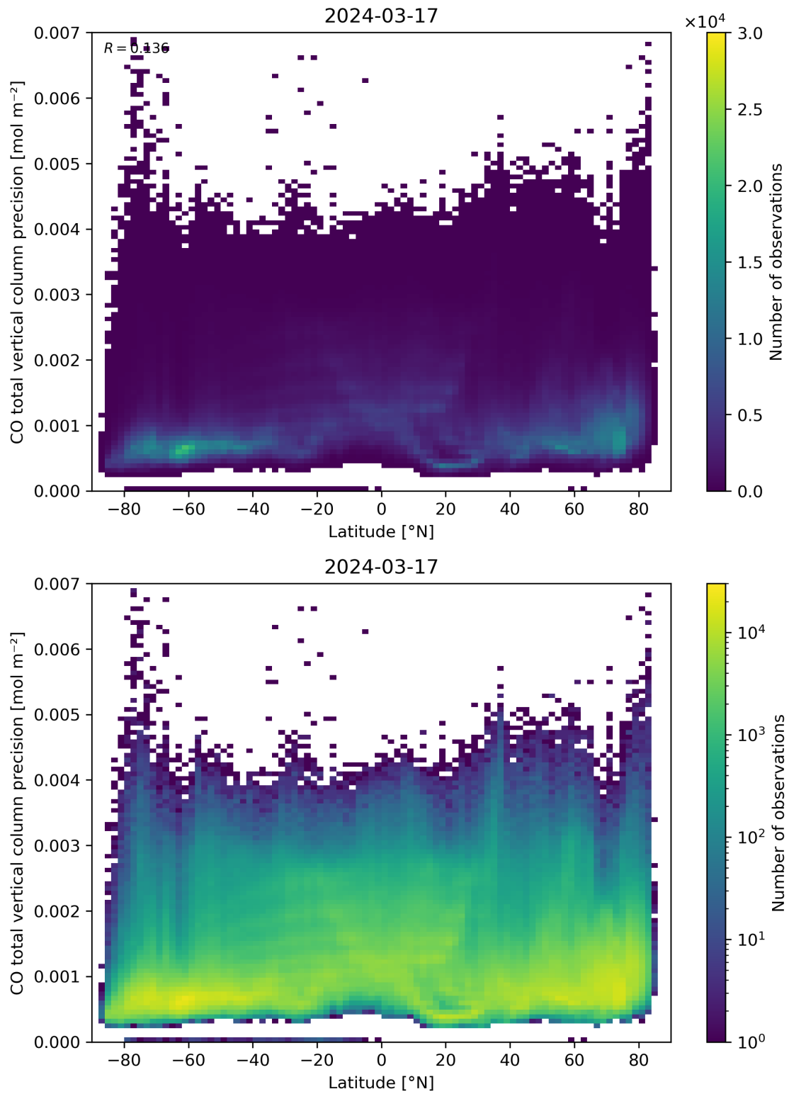
Figure 53: Scatter density plot of “Latitude” against “CO total vertical column precision” for 2024-03-16 to 2024-03-18.
