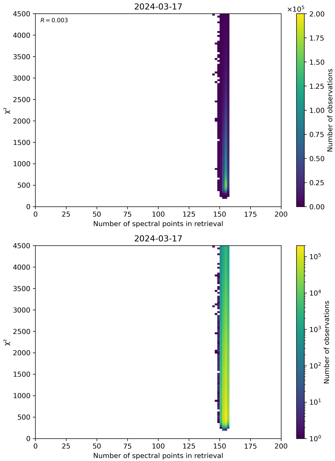
Figure 58: Scatter density plot of “Number of spectral points in retrieval” against “ \chi^2 ” for 2024-03-16 to 2024-03-18.
