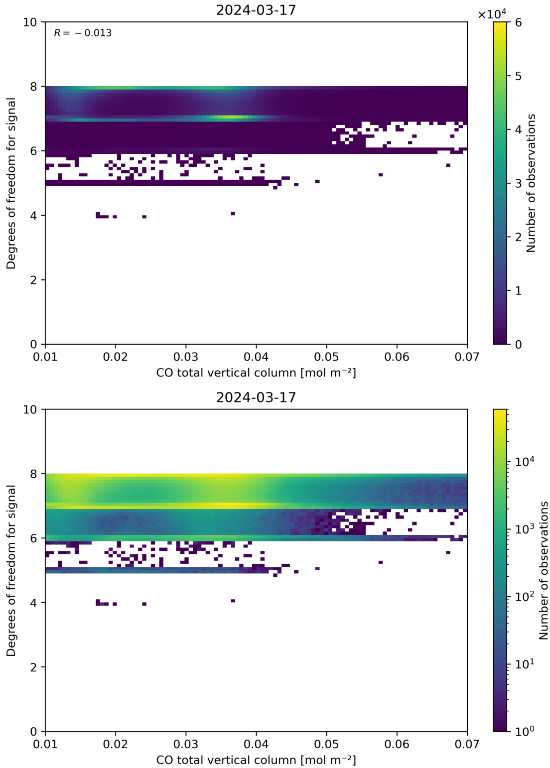
Figure 41: Scatter density plot of “CO total vertical column” against “Degrees of freedom for signal” for 2024-03-16 to 2024-03-18.
