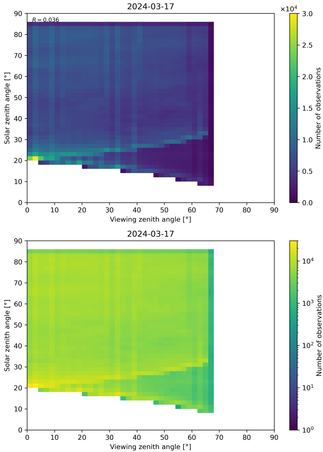
Figure 77: Scatter density plot of “Viewing zenith angle” against “Solar zenith angle” for 2024-03-16 to 2024-03-18.
