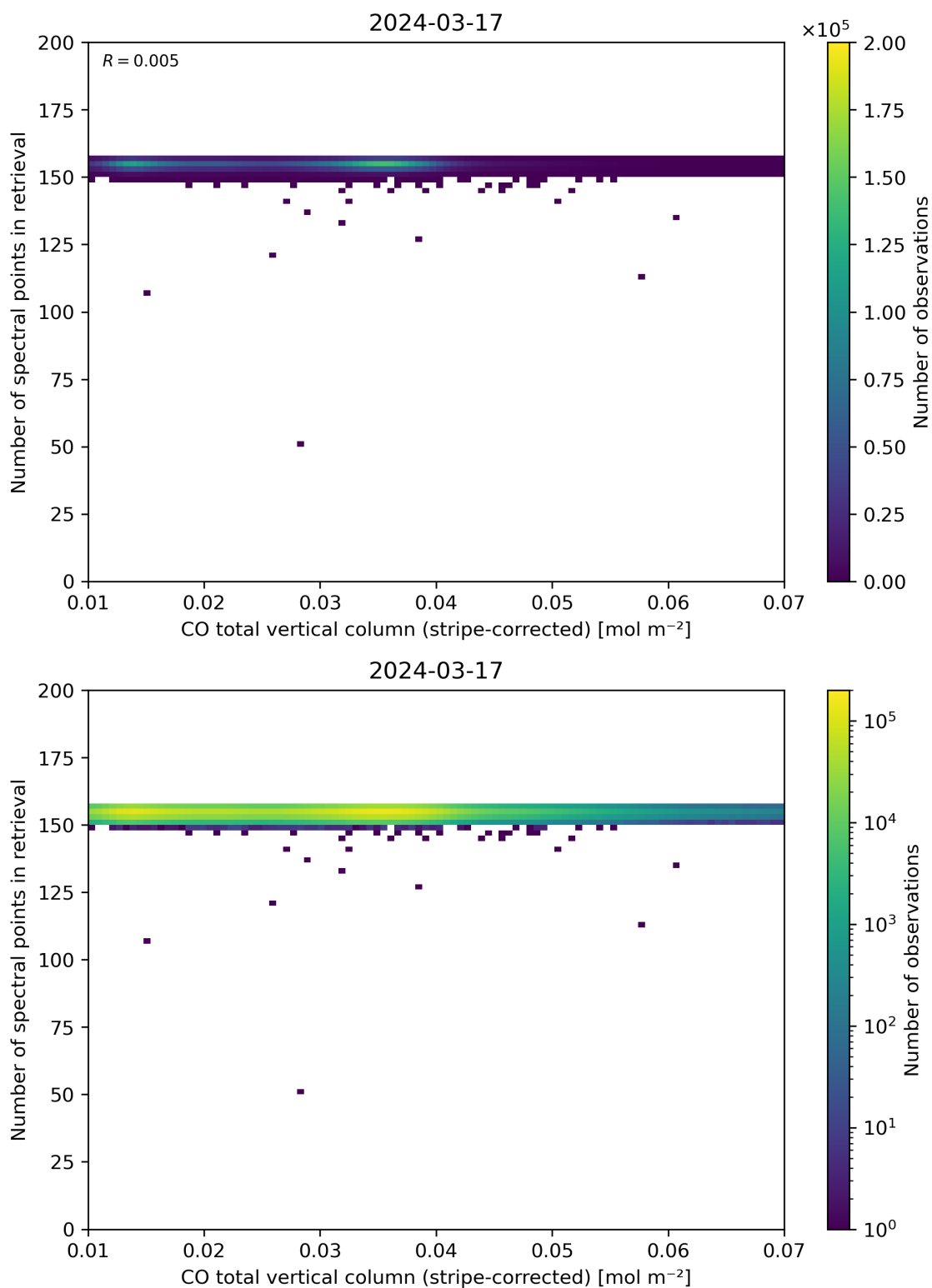
Figure 40: Scatter density plot of “CO total vertical column (stripe-corrected)” against “Number of spectral points in retrieval” for 2024-03-16 to 2024-03-18.
