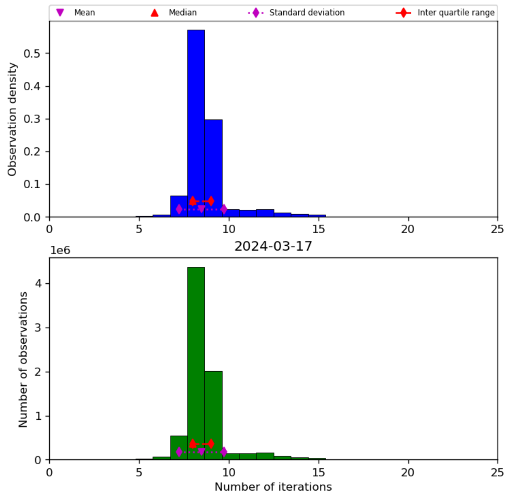
Figure 24: Histogram of “Number of iterations” for 2024-03-16 to 2024-03-18
