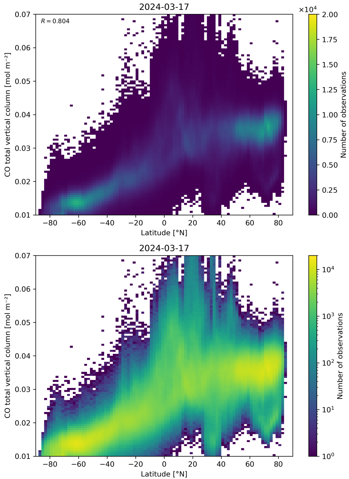
Figure 51: Scatter density plot of “Latitude” against “CO total vertical column” for 2024-03-16 to 2024-03-18.
