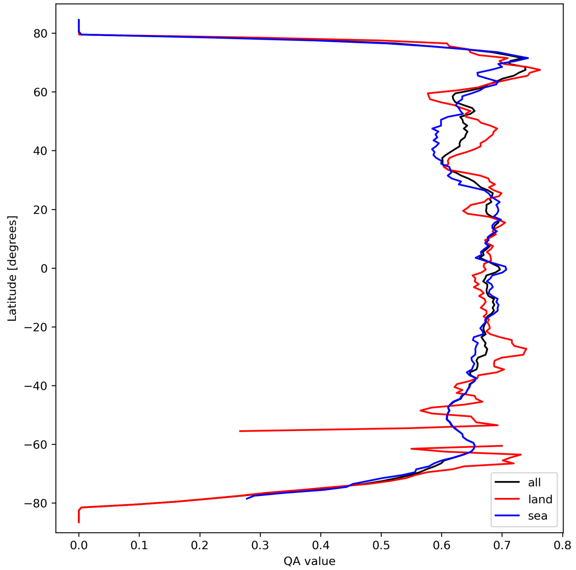
Figure 9: Zonal average of “QA value” for 2024-03-16 to 2024-03-18.
