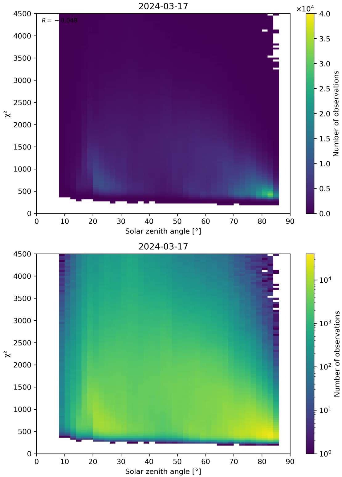
Figure 64: Scatter density plot of “Solar zenith angle” against “ \chi^2 ” for 2024-03-16 to 2024-03-18.
