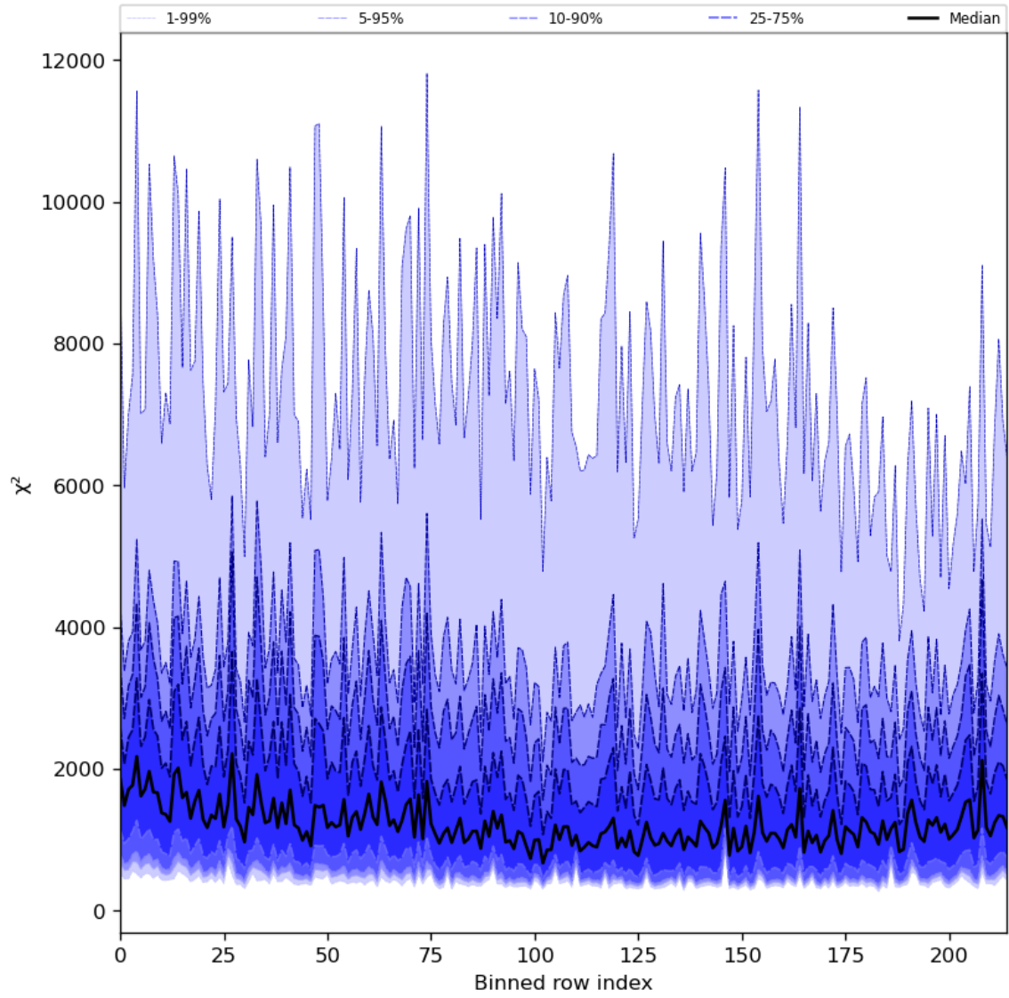
Figure 30: Along track statistics of “ \chi^2 ” for 2024-03-16 to 2024-03-18
