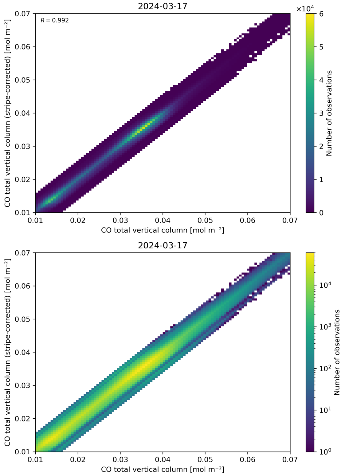
Figure 33: Scatter density plot of “CO total vertical column” against “CO total vertical column (stripe-corrected)” for 2024-03-16 to 2024-03-18.
