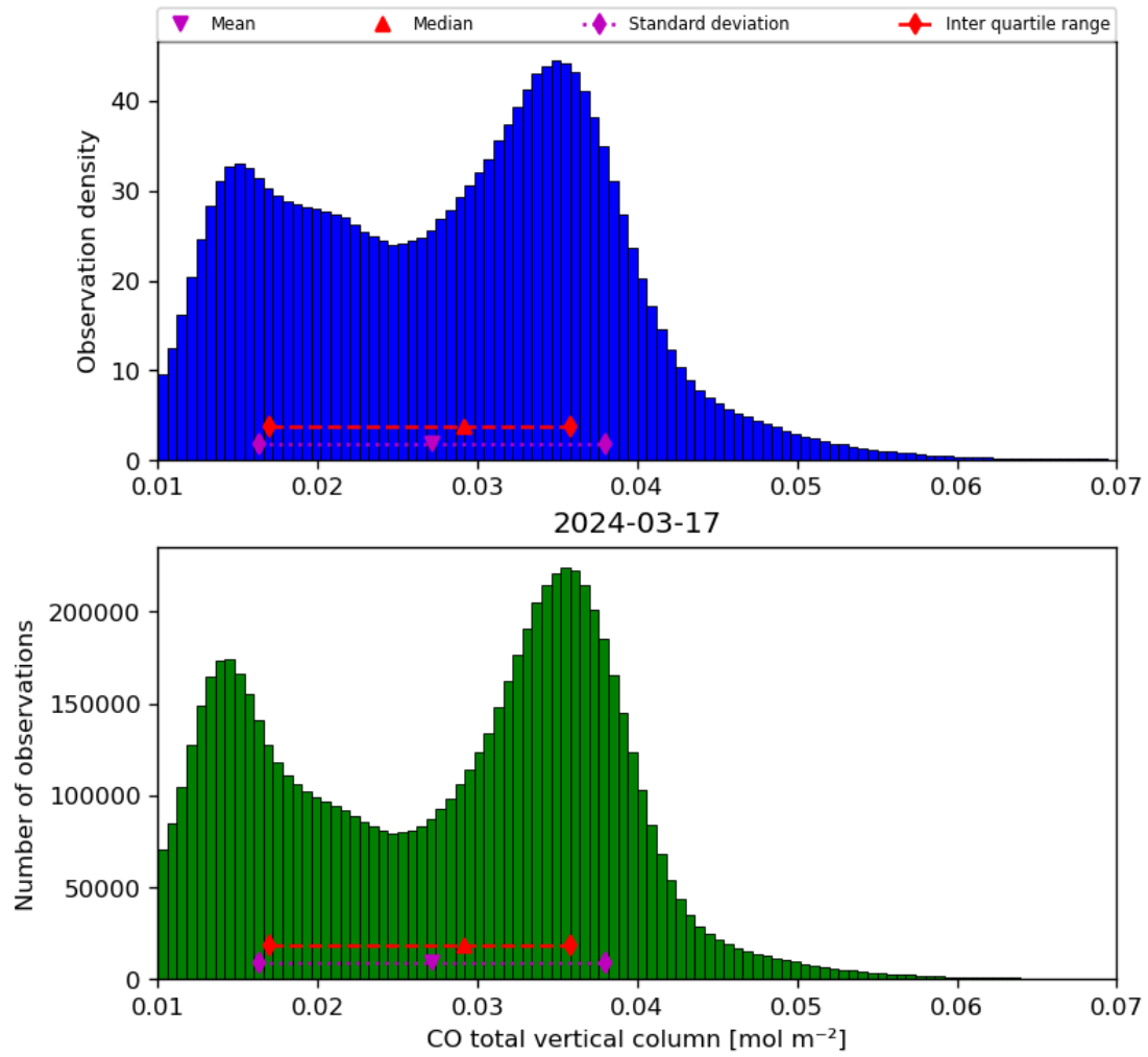
Figure 18: Histogram of “CO total vertical column” for 2024-03-16 to 2024-03-18
