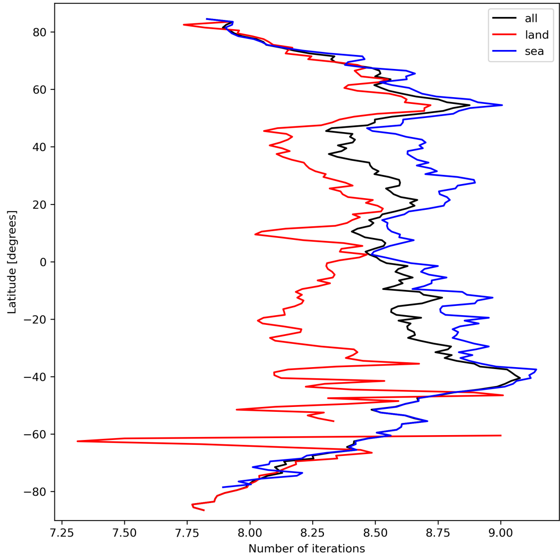
Figure 16: Zonal average of “Number of iterations” for 2024-03-16 to 2024-03-18.
