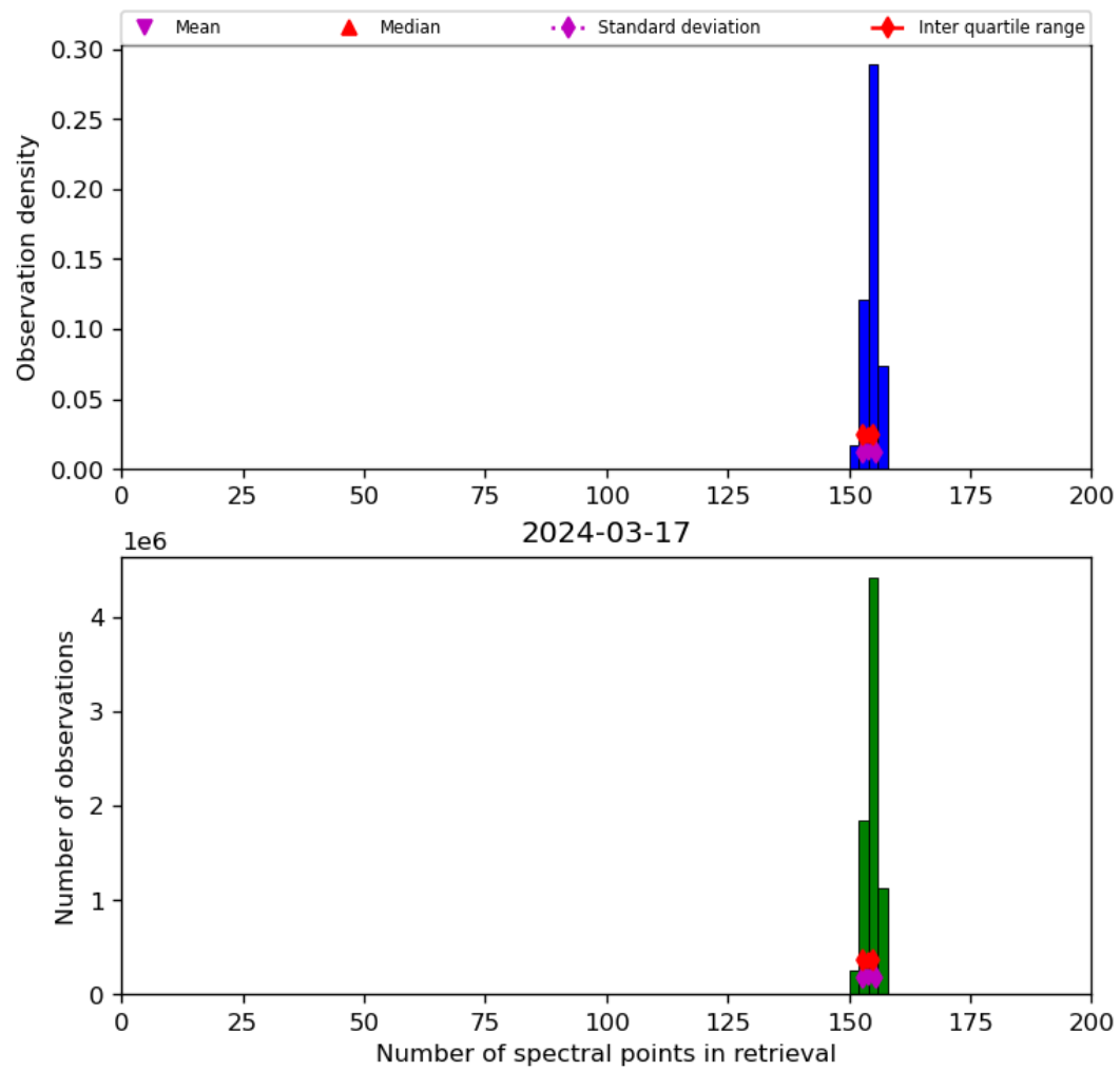
Figure 21: Histogram of “Number of spectral points in retrieval” for 2024-03-16 to 2024-03-18
