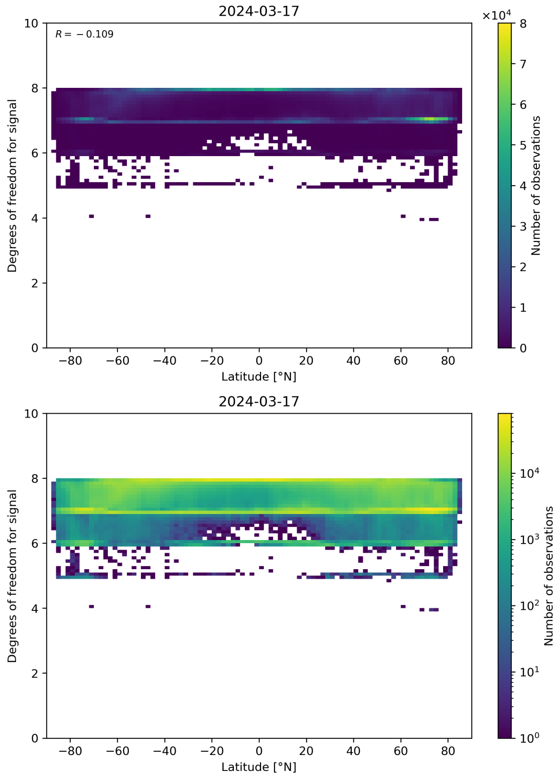
Figure 55: Scatter density plot of “Latitude” against “Degrees of freedom for signal” for 2024-03-16 to 2024-03-18.
