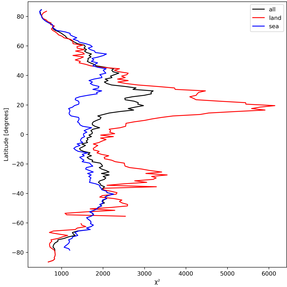
Figure 14: Zonal average of “ \chi^2 ” for 2024-03-16 to 2024-03-18.
