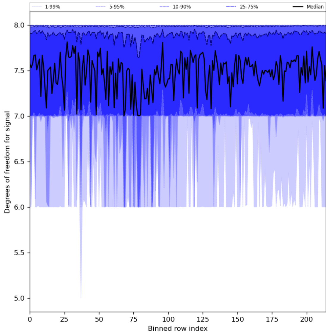
Figure 31: Along track statistics of “Degrees of freedom for signal” for 2024-03-16 to 2024-03-18
