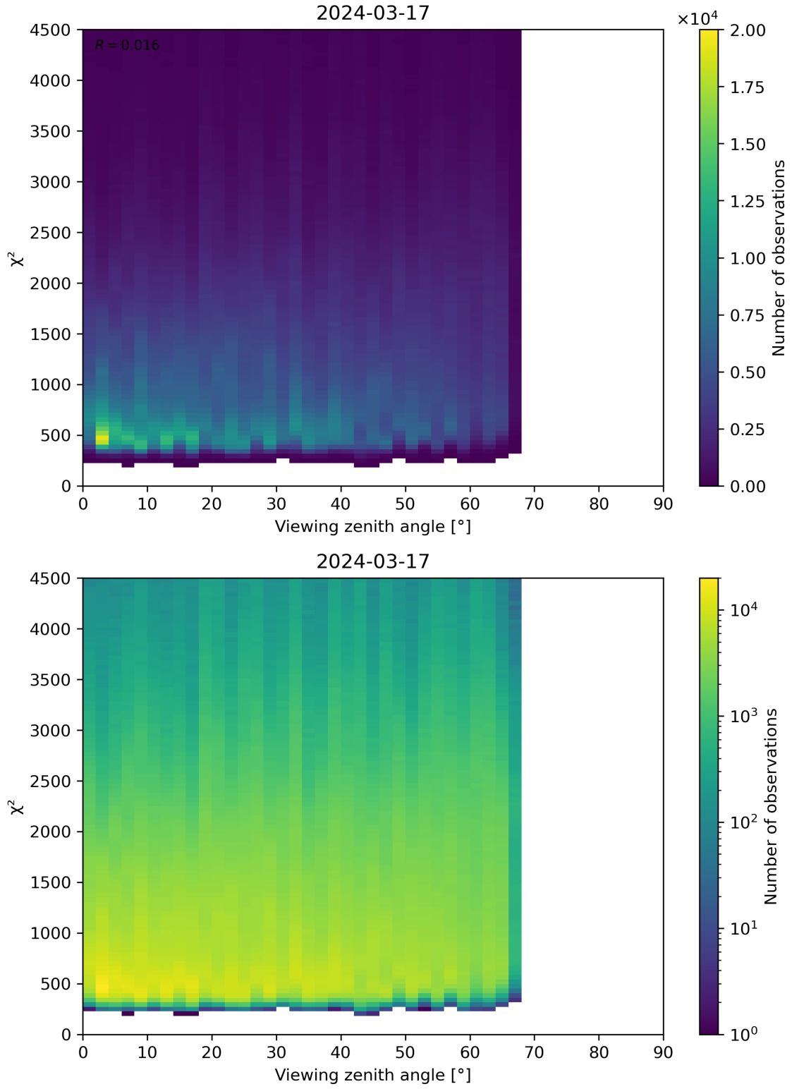
Figure 72: Scatter density plot of “Viewing zenith angle” against “ \chi^2 ” for 2024-03-16 to 2024-03-18.
