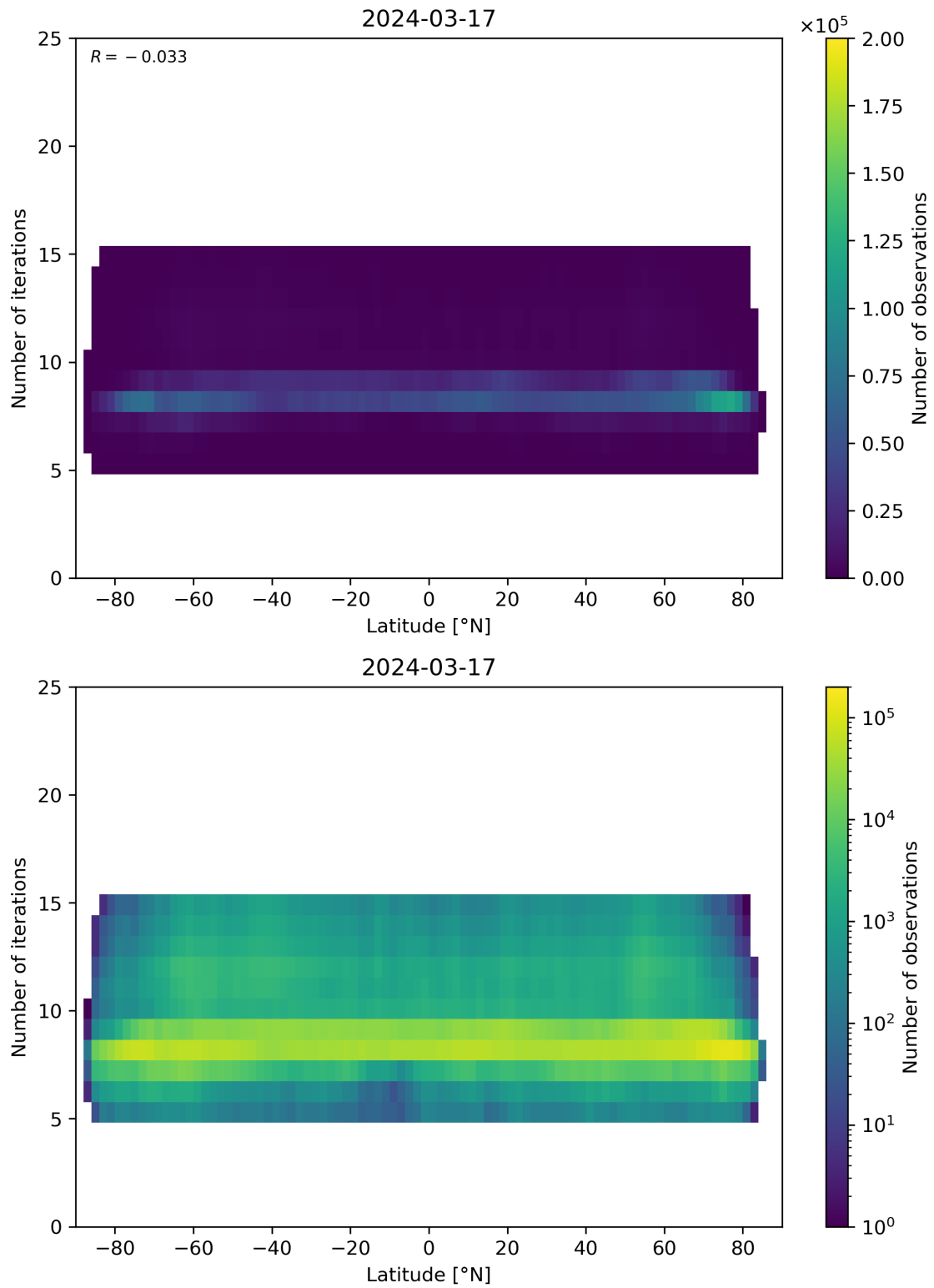
Figure 56: Scatter density plot of “Latitude” against “Number of iterations” for 2024-03-16 to 2024-03-18.
