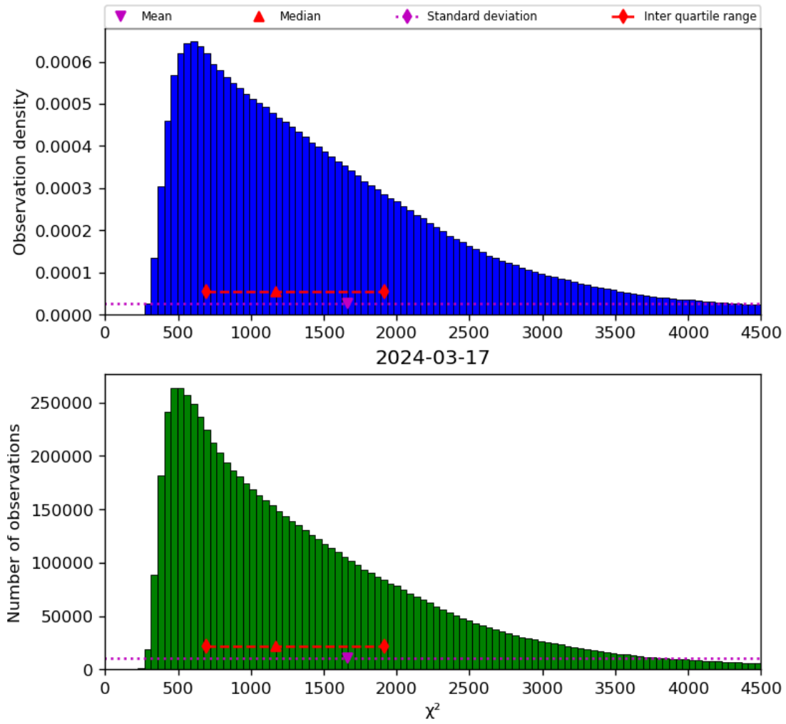
Figure 22: Histogram of “ \chi^2 ” for 2024-03-16 to 2024-03-18
