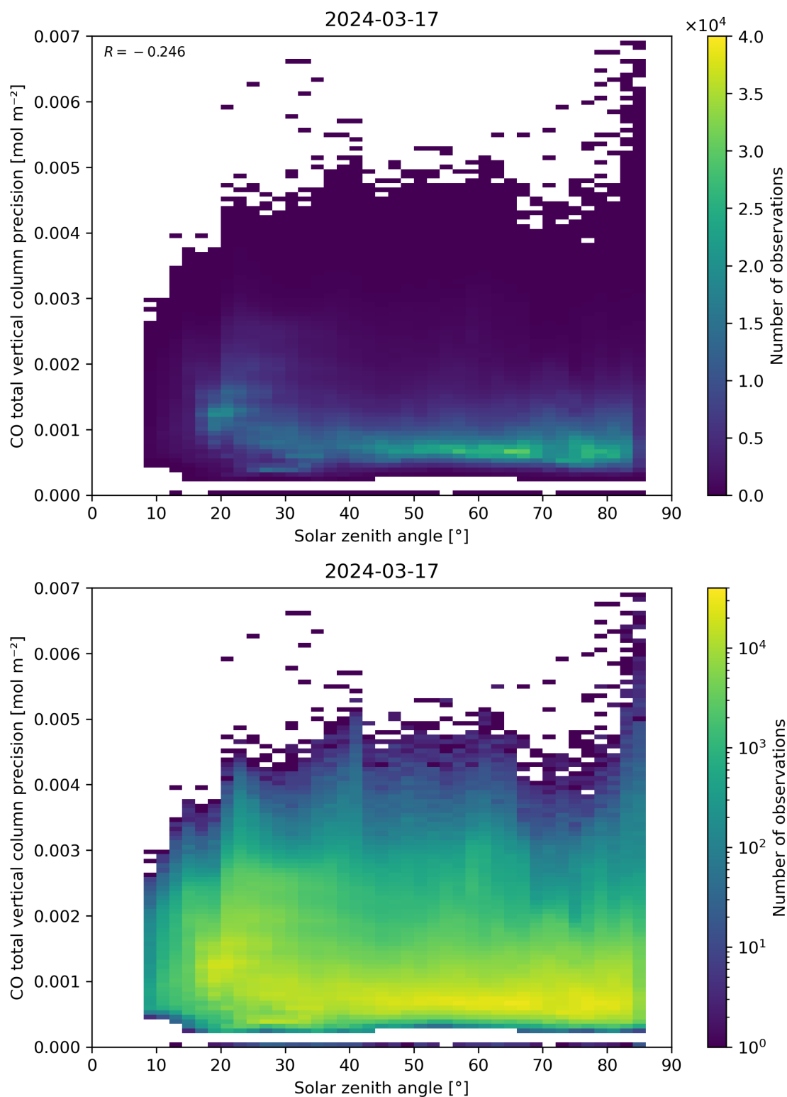
Figure 63: Scatter density plot of “Solar zenith angle” against “CO total vertical column precision” for 2024-03-16 to 2024-03-18.
