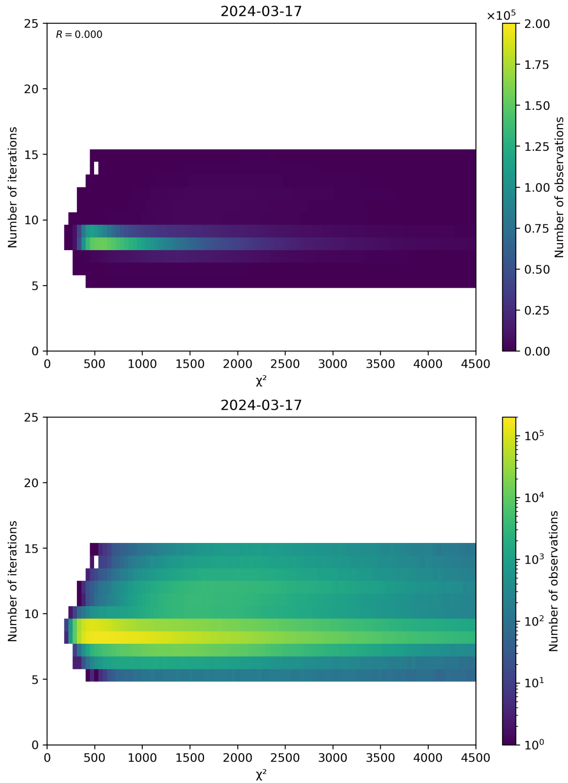
Figure 49: Scatter density plot of “ \chi^2 ” against “Number of iterations” for 2024-03-16 to 2024-03-18.
