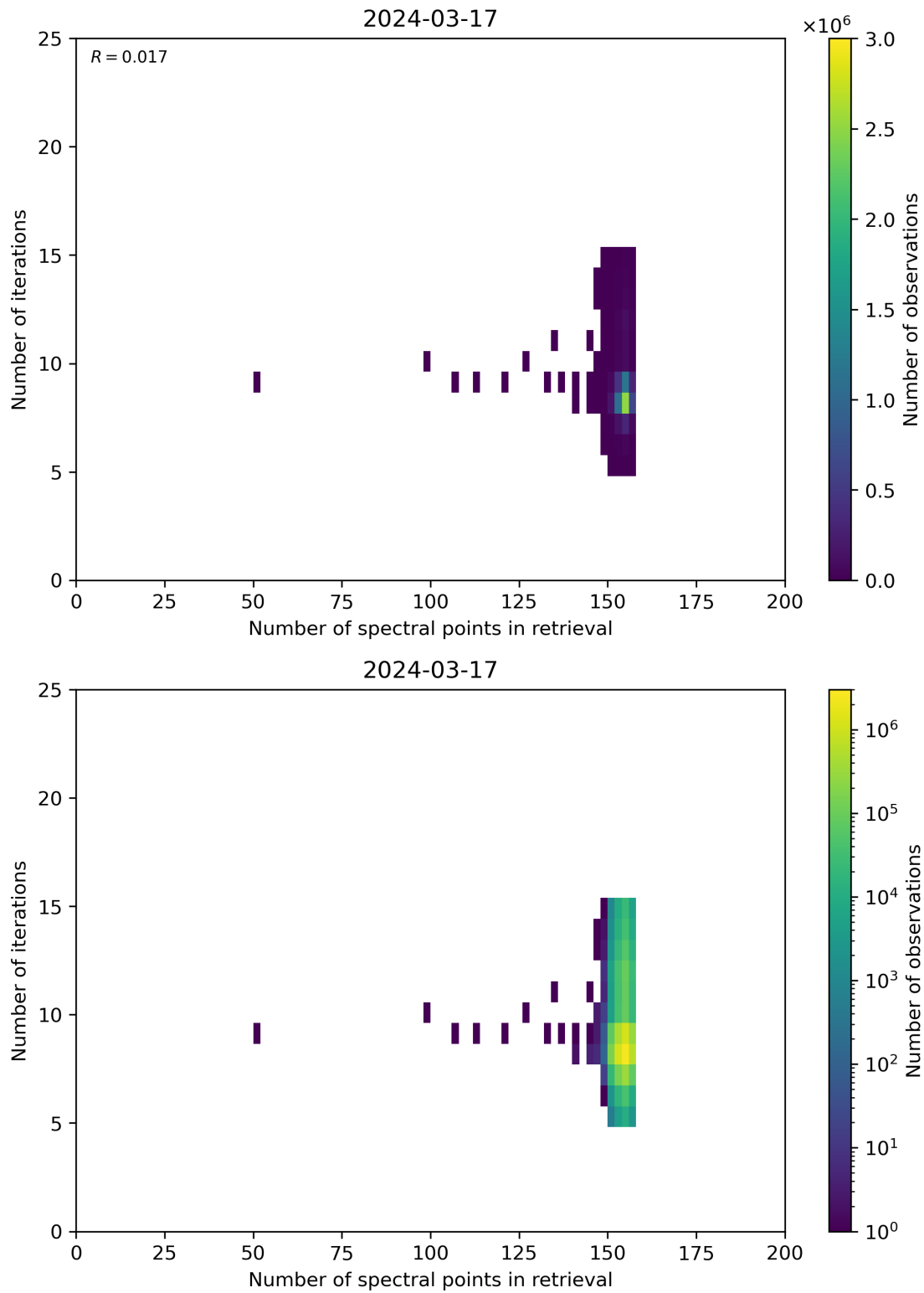
Figure 60: Scatter density plot of “Number of spectral points in retrieval” against “Number of iterations” for 2024-03-16 to 2024-03-18.
