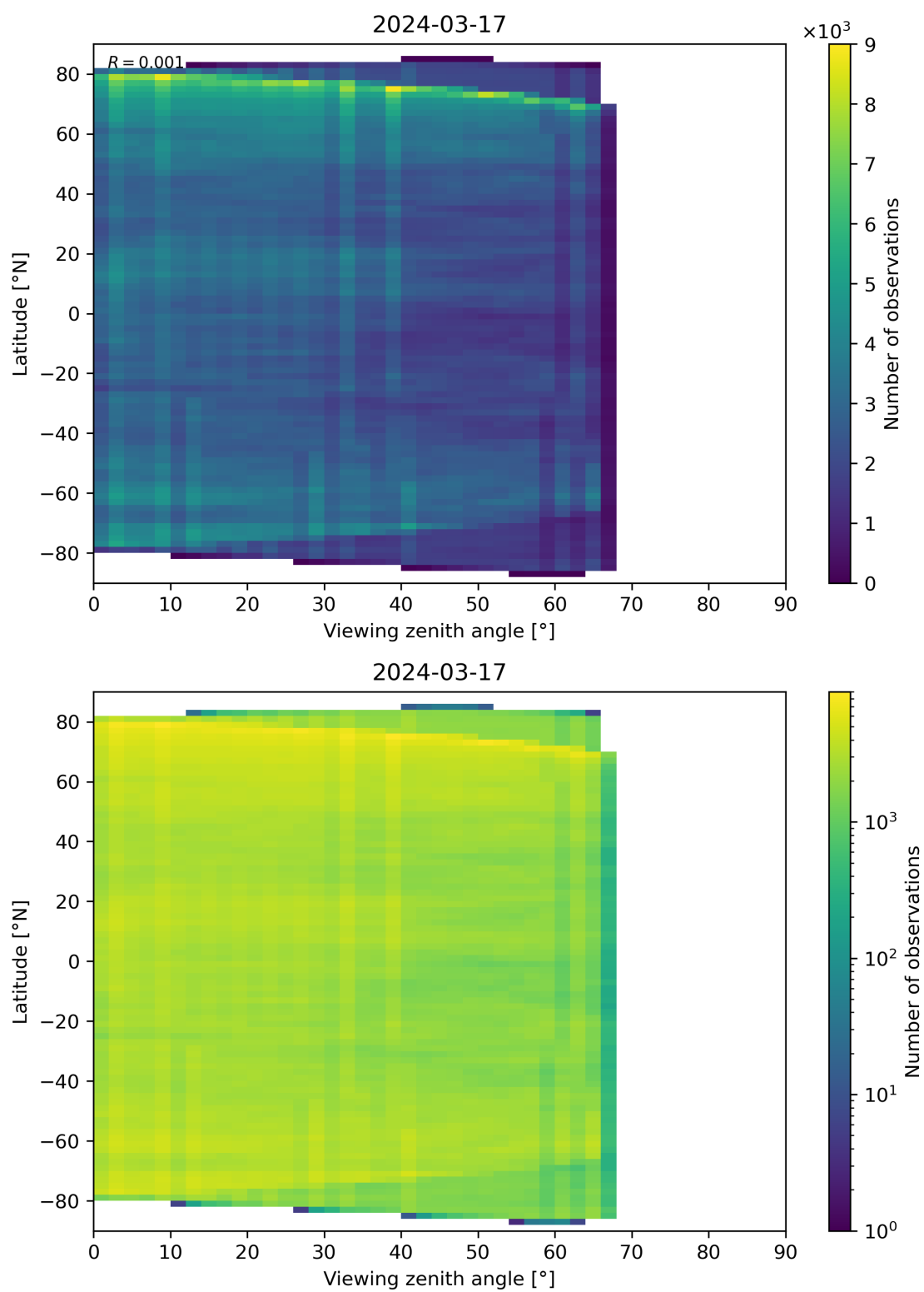
Figure 74: Scatter density plot of “Viewing zenith angle” against “Latitude” for 2024-03-16 to 2024-03-18.
