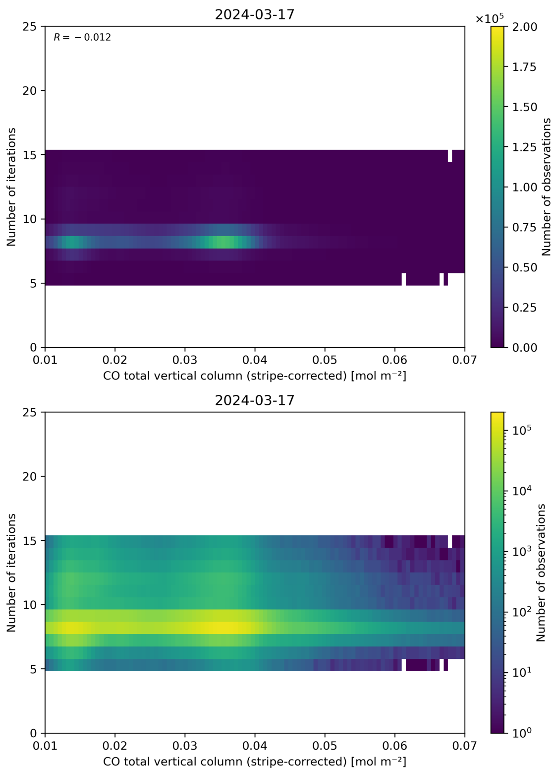
Figure 39: Scatter density plot of “CO total vertical column (stripe-corrected)” against “Number of iterations” for 2024-03-16 to 2024-03-18.
