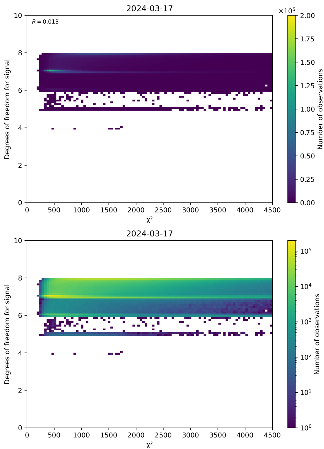
Figure 48: Scatter density plot of “ \chi^2 ” against “Degrees of freedom for signal” for 2024-03-16 to 2024-03-18.
