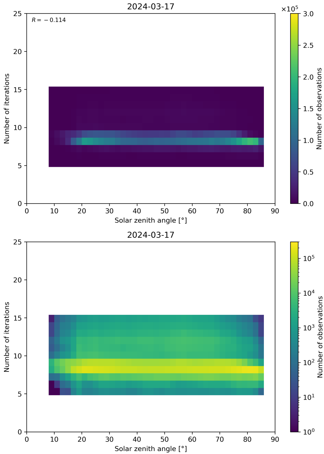
Figure 67: Scatter density plot of “Solar zenith angle” against “Number of iterations” for 2024-03-16 to 2024-03-18.
