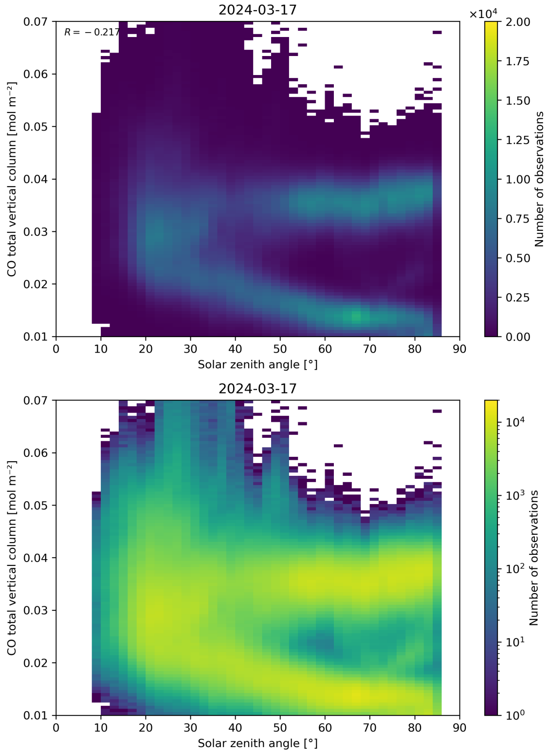
Figure 61: Scatter density plot of “Solar zenith angle” against “CO total vertical column” for 2024-03-16 to 2024-03-18.
