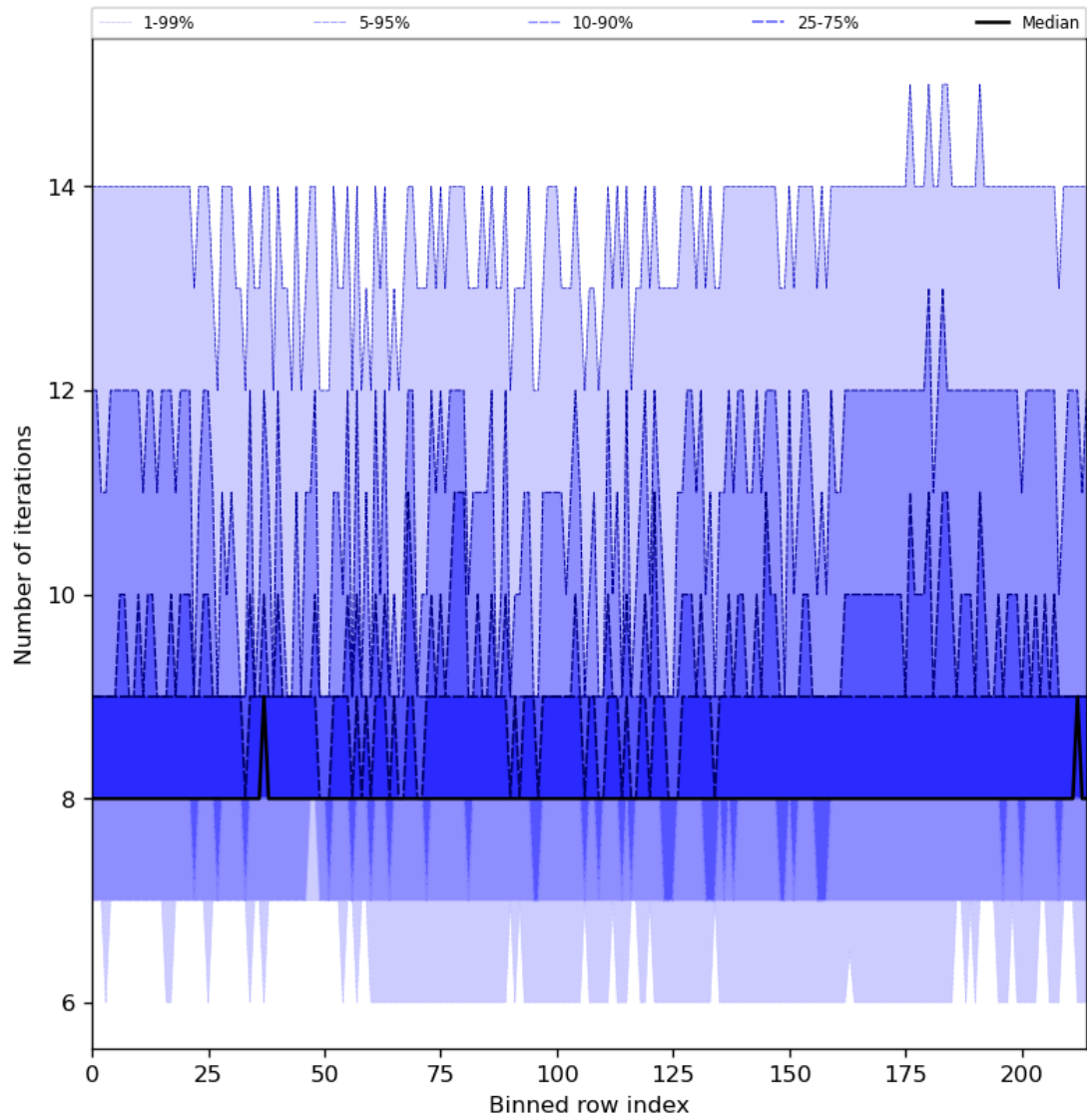
Figure 32: Along track statistics of “Number of iterations” for 2024-03-16 to 2024-03-18
