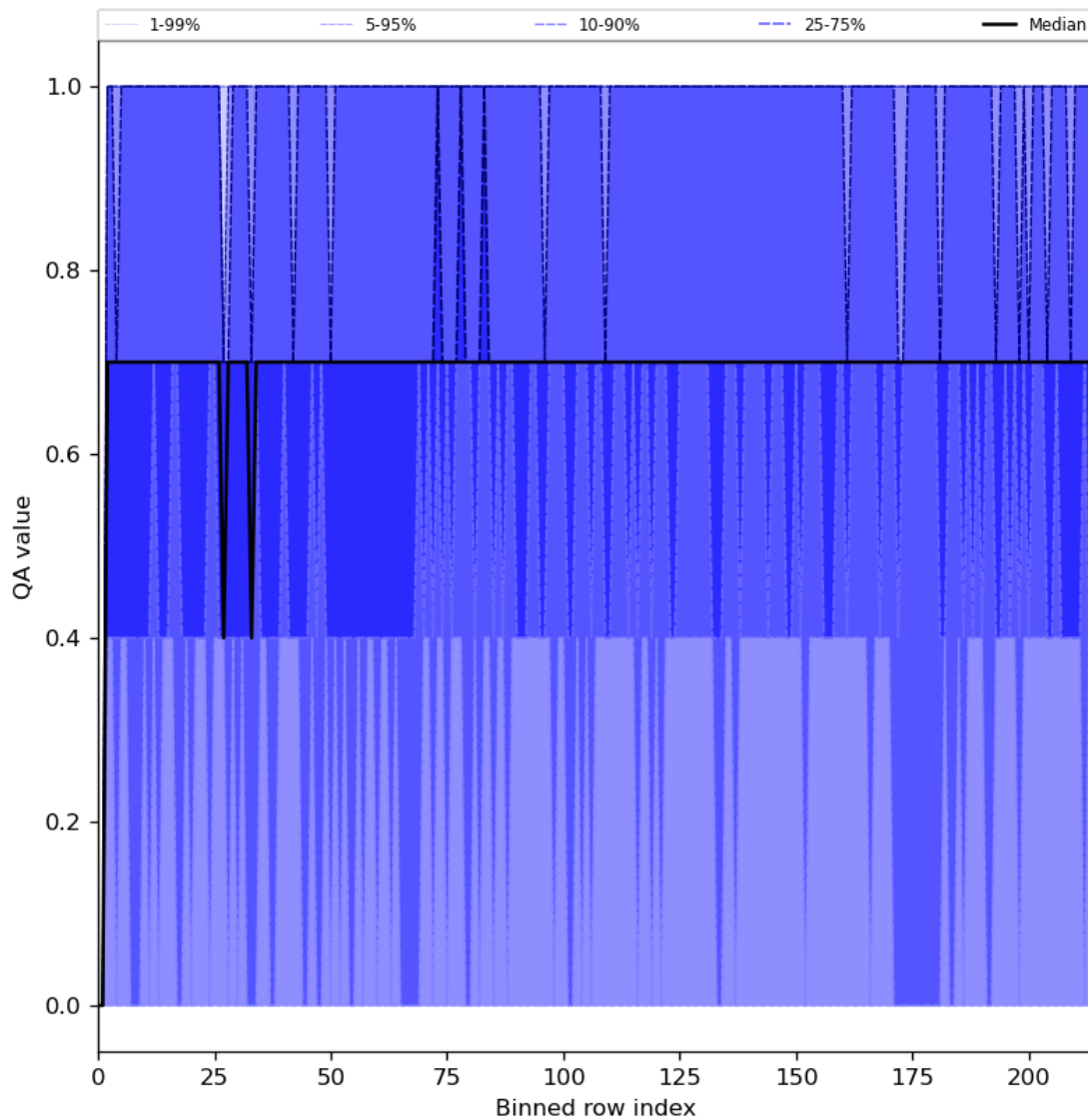
Figure 25: Along track statistics of “QA value” for 2024-03-16 to 2024-03-18
