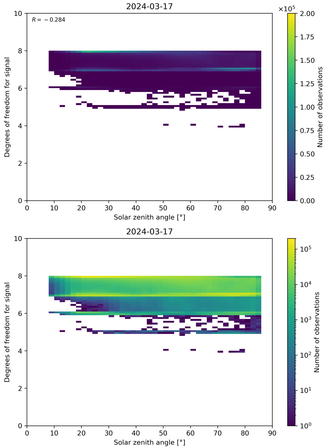
Figure 65: Scatter density plot of “Solar zenith angle” against “Degrees of freedom for signal” for 2024-03-16 to 2024-03-18.
