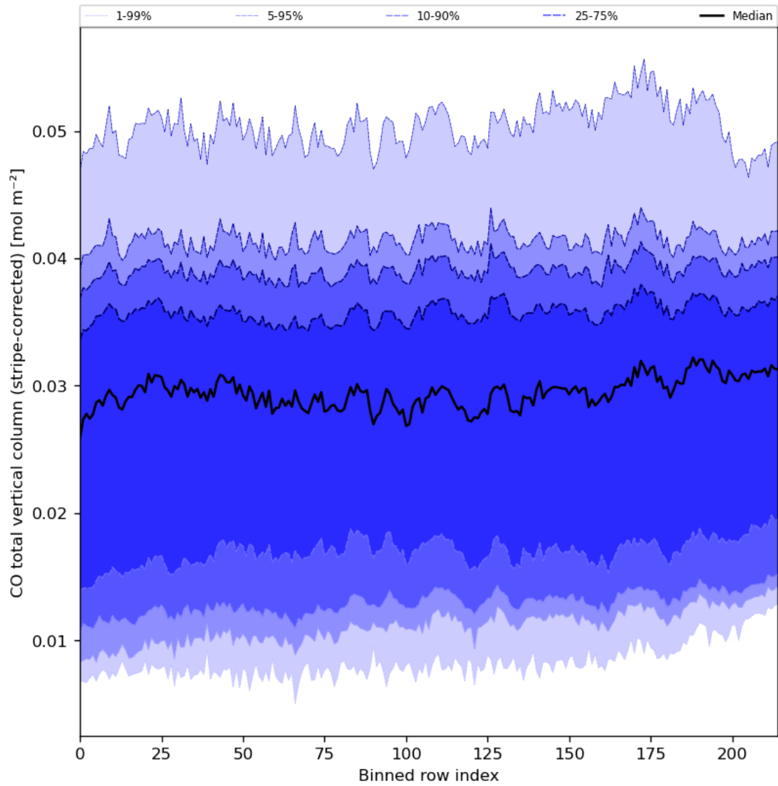
Figure 27: Along track statistics of “CO total vertical column (stripe-corrected)” for 2024-03-16 to 2024-03-18
