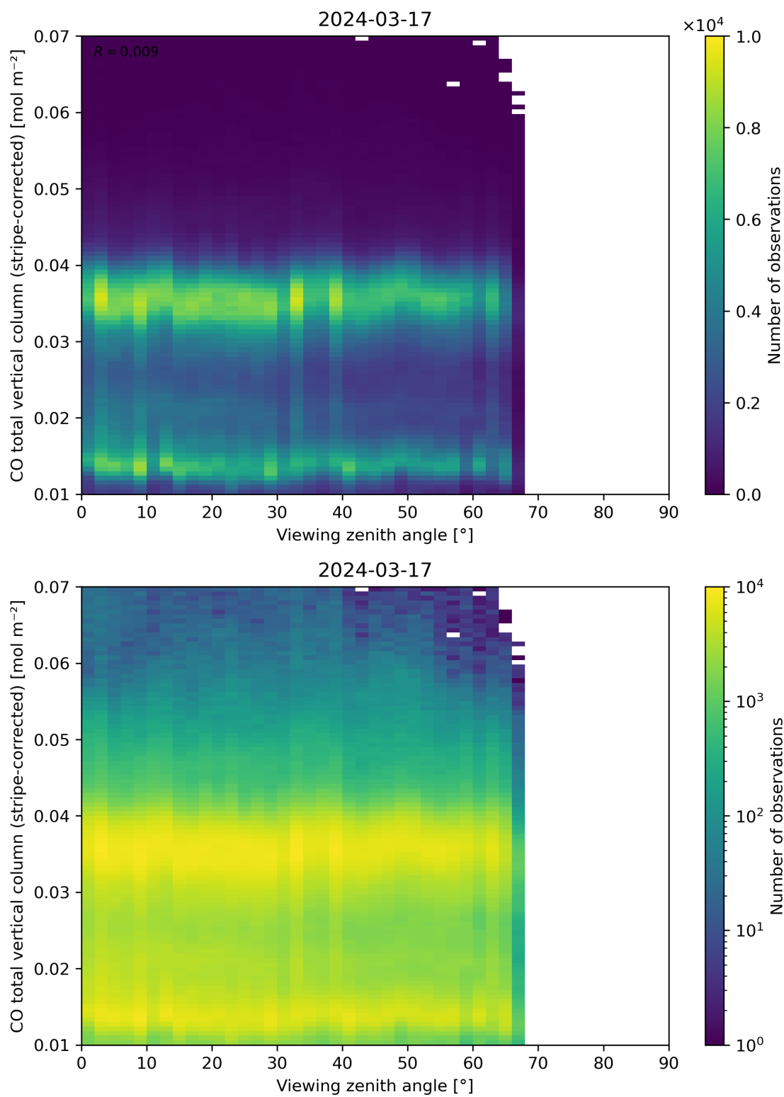
Figure 70: Scatter density plot of “Viewing zenith angle” against “CO total vertical column (stripe-corrected)” for 2024-03-16 to 2024-03-18.
