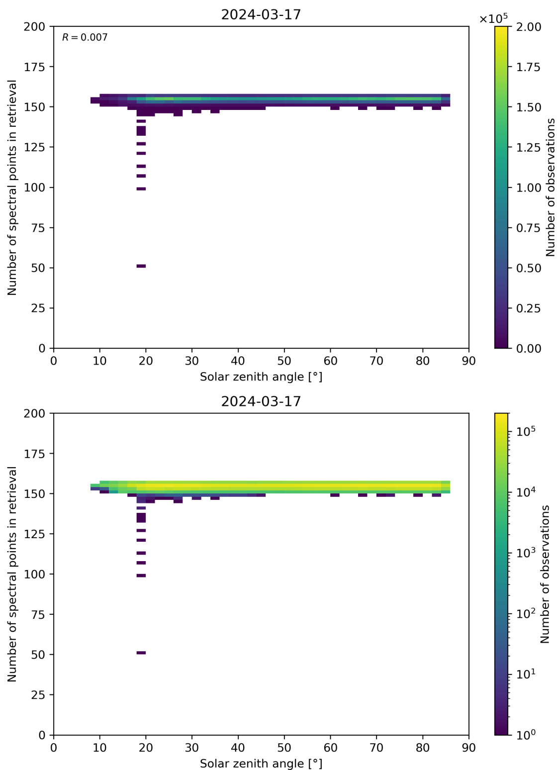
Figure 68: Scatter density plot of “Solar zenith angle” against “Number of spectral points in retrieval” for 2024-03-16 to 2024-03-18.
