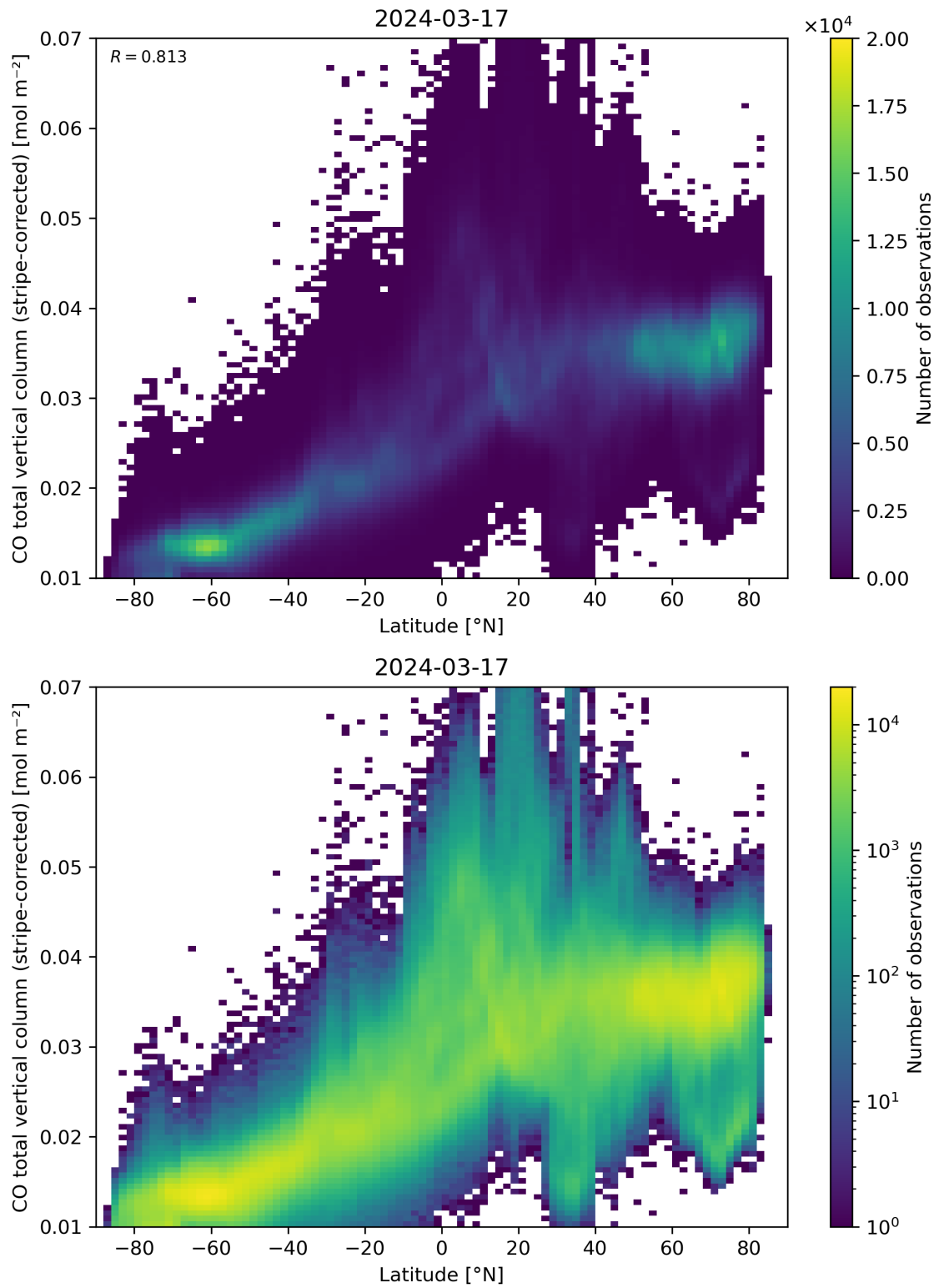
Figure 52: Scatter density plot of “Latitude” against “CO total vertical column (stripe-corrected)” for 2024-03-16 to 2024-03-18.
