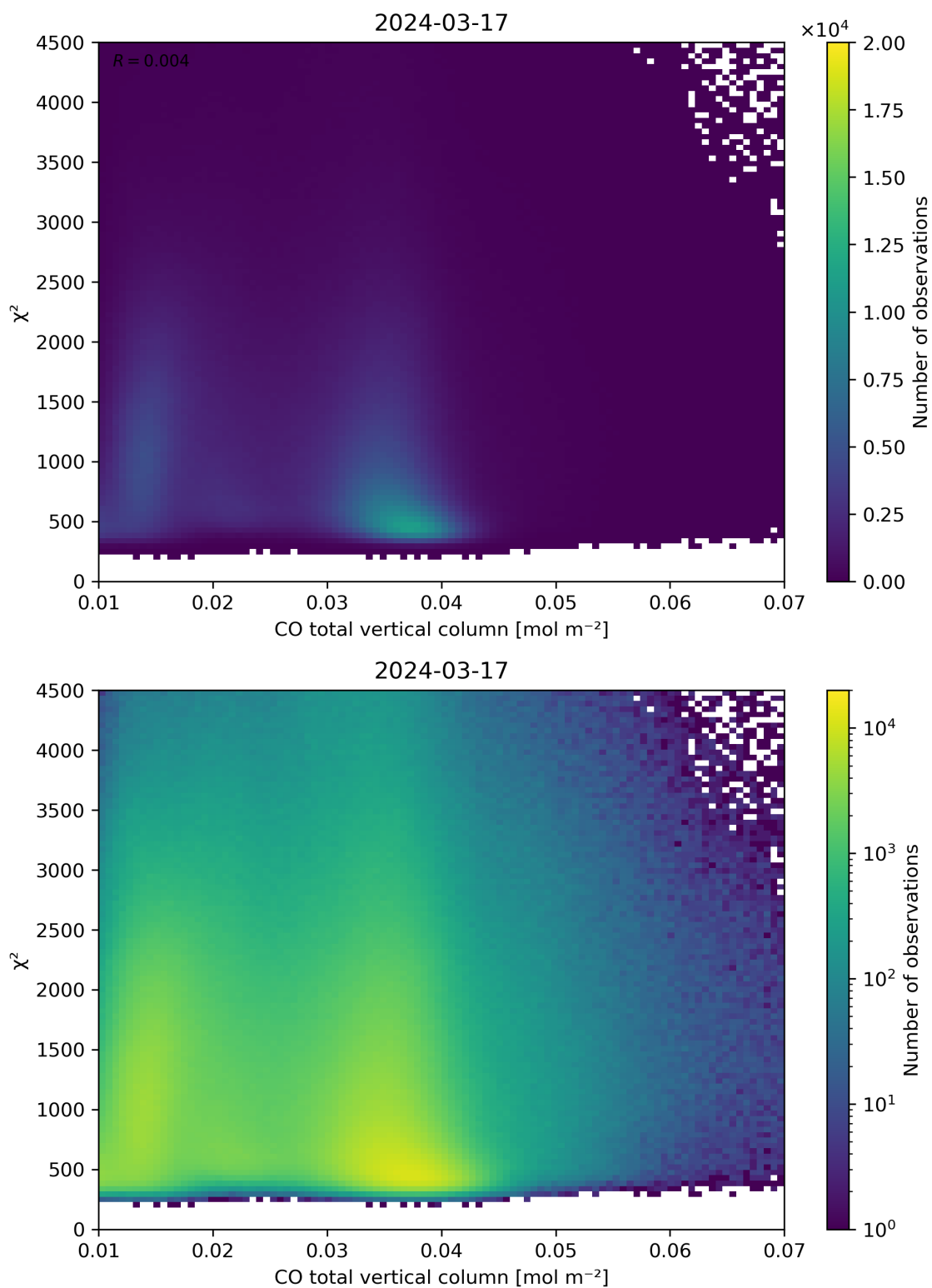
Figure 35: Scatter density plot of “CO total vertical column” against “ \chi^2 ” for 2024-03-16 to 2024-03-18.
