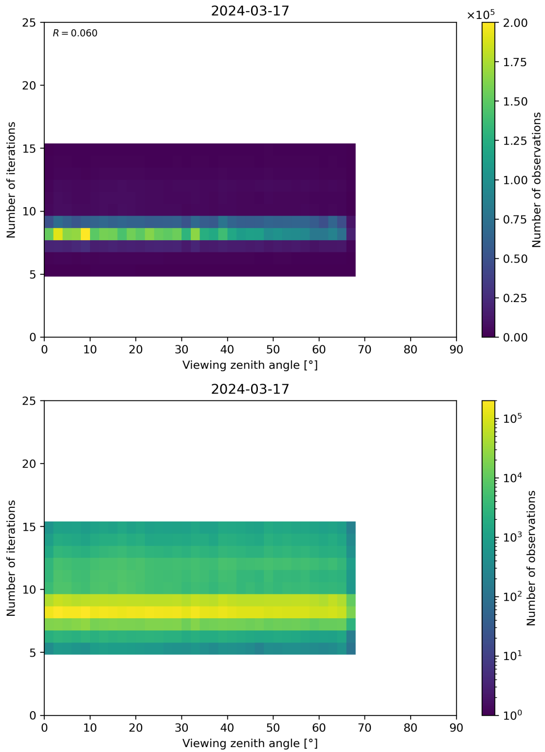
Figure 75: Scatter density plot of “Viewing zenith angle” against “Number of iterations” for 2024-03-16 to 2024-03-18.
