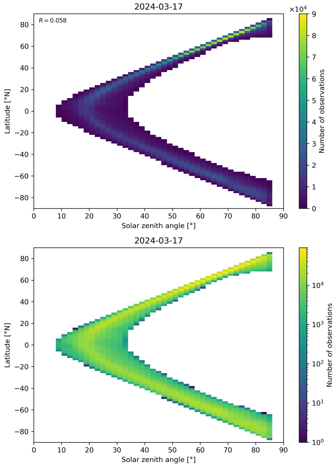
Figure 66: Scatter density plot of “Solar zenith angle” against “Latitude” for 2024-03-16 to 2024-03-18.
