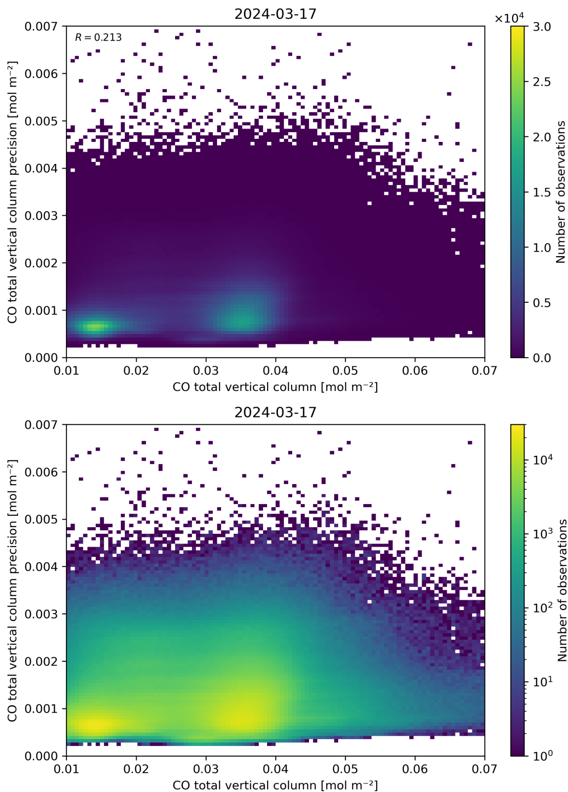
Figure 34: Scatter density plot of “CO total vertical column” against “CO total vertical column precision” for 2024-03-16 to 2024-03-18.
