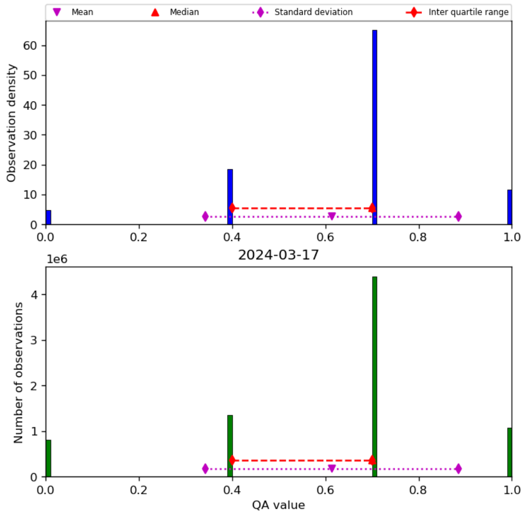
Figure 17: Histogram of “QA value” for 2024-03-16 to 2024-03-18
