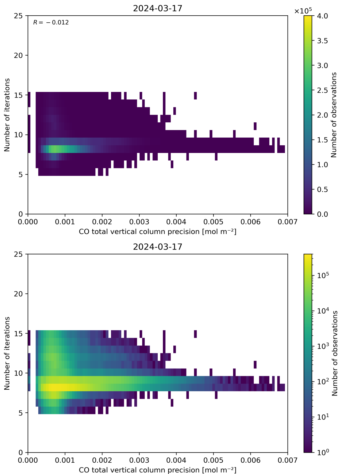
Figure 46: Scatter density plot of “CO total vertical column precision” against “Number of iterations” for 2024-03-16 to 2024-03-18.
