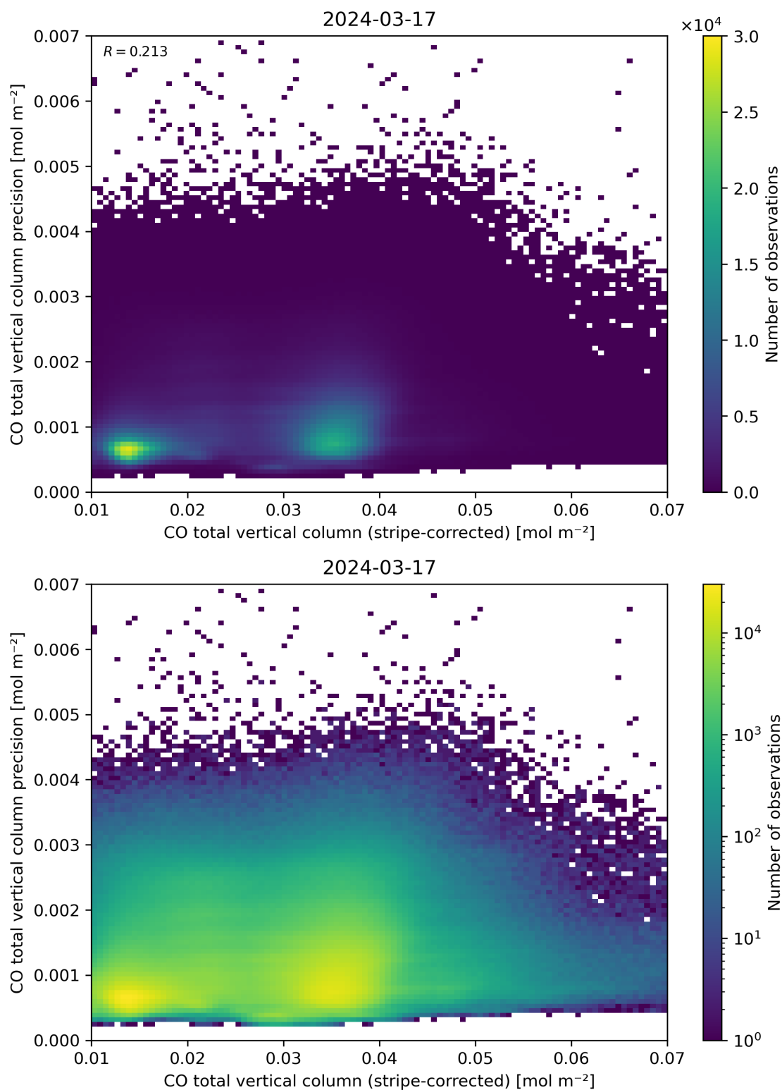
Figure 36: Scatter density plot of “CO total vertical column (stripe-corrected)” against “CO total vertical column precision” for 2024-03-16 to 2024-03-18.
