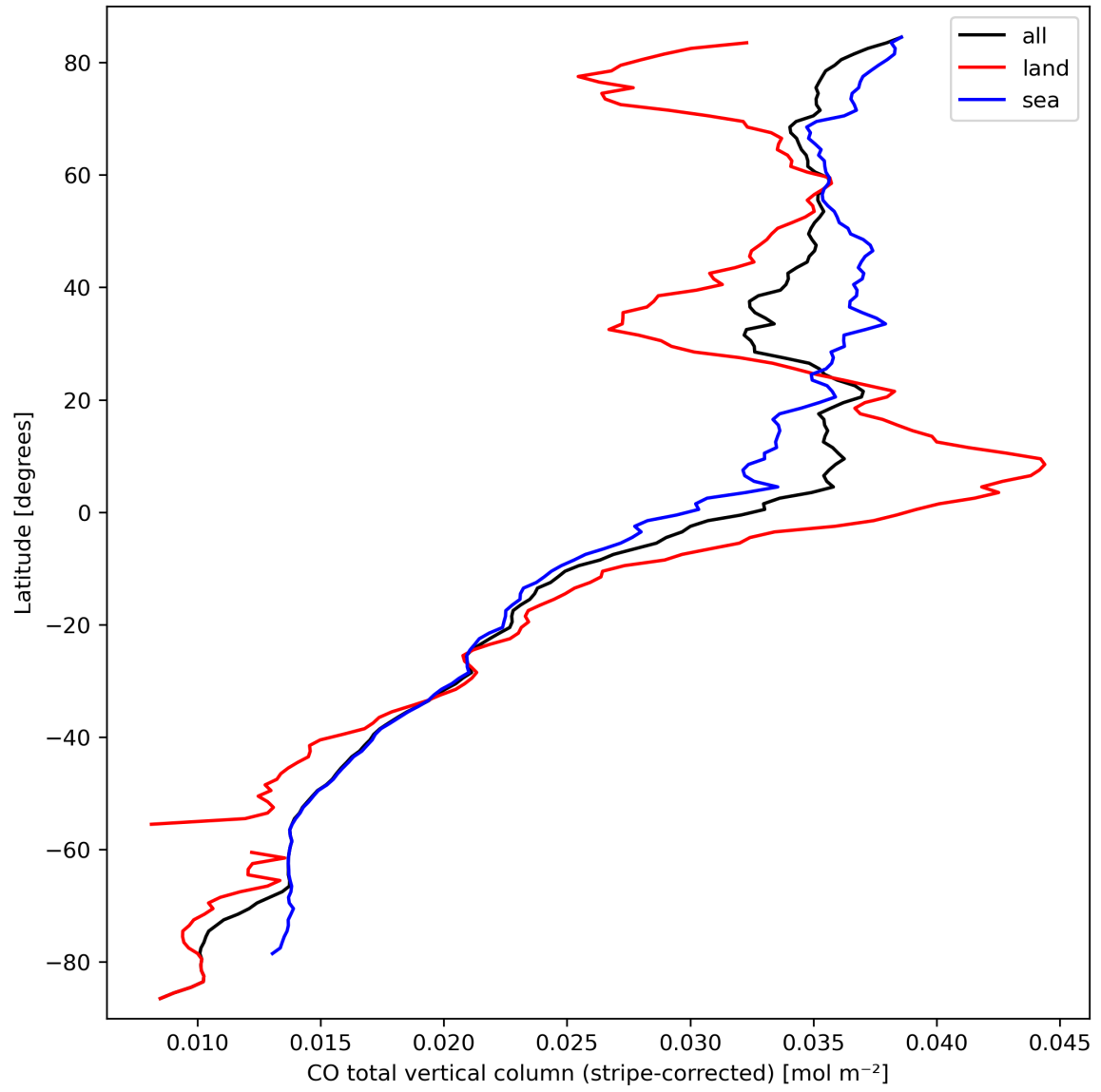
Figure 11: Zonal average of “CO total vertical column (stripe-corrected)” for 2024-03-16 to 2024-03-18.
