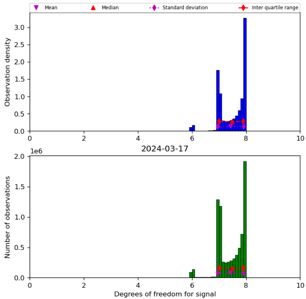
Figure 23: Histogram of “Degrees of freedom for signal” for 2024-03-16 to 2024-03-18
