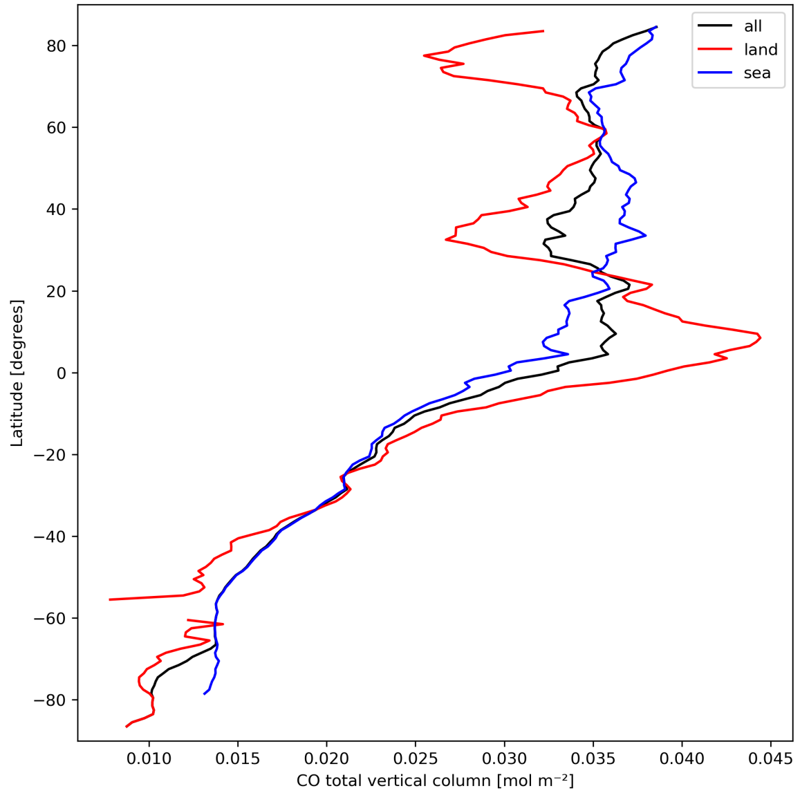
Figure 10: Zonal average of “CO total vertical column” for 2024-03-16 to 2024-03-18.
