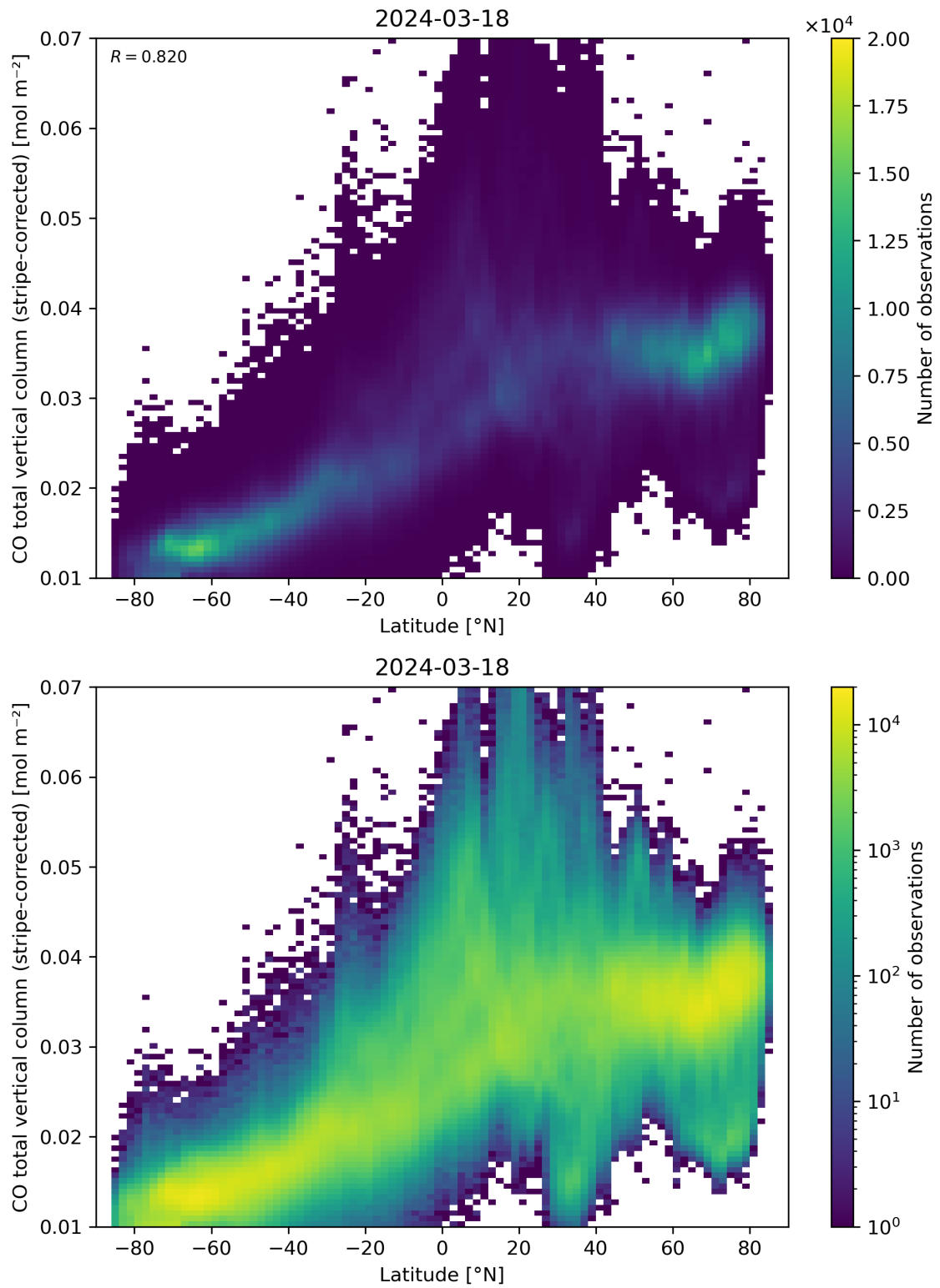
Figure 52: Scatter density plot of “Latitude” against “CO total vertical column (stripe-corrected)” for 2024-03-17 to 2024-03-19.
