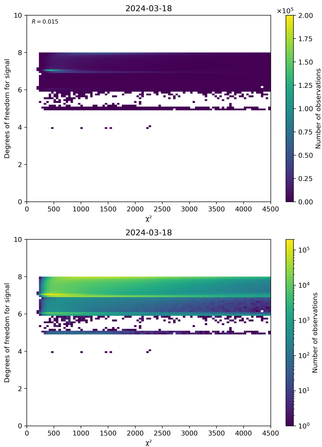
Figure 48: Scatter density plot of “ \chi^2 ” against “Degrees of freedom for signal” for 2024-03-17 to 2024-03-19.
