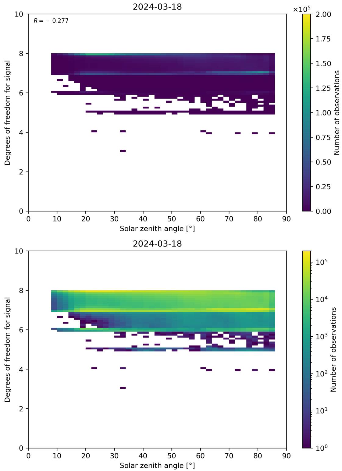
Figure 65: Scatter density plot of “Solar zenith angle” against “Degrees of freedom for signal” for 2024-03-17 to 2024-03-19.
