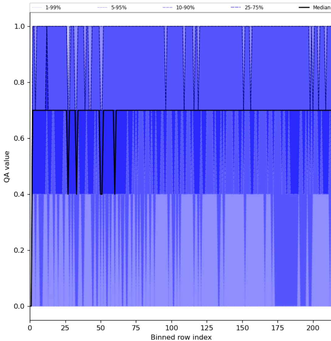
Figure 25: Along track statistics of “QA value” for 2024-03-17 to 2024-03-19
