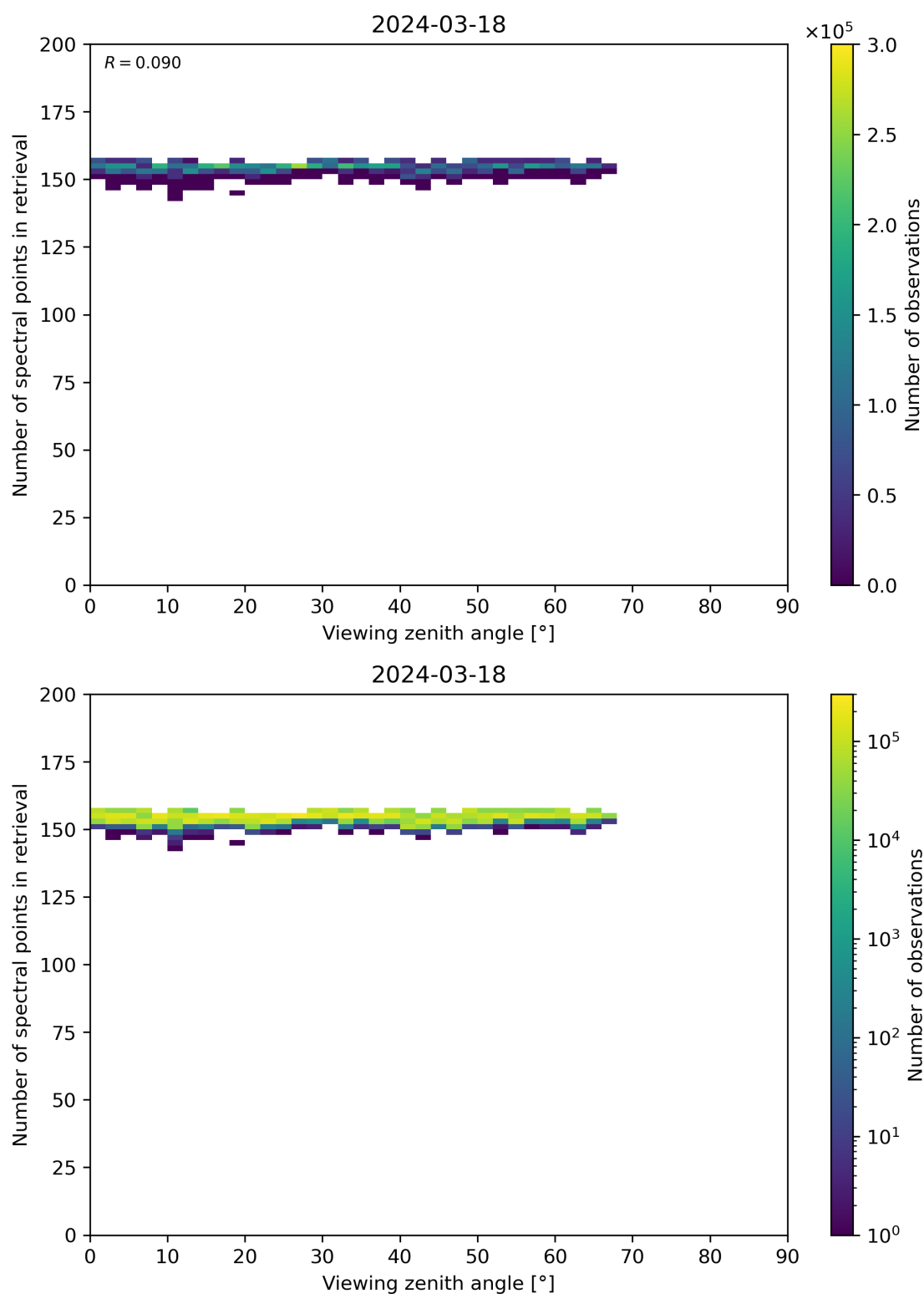
Figure 76: Scatter density plot of “Viewing zenith angle” against “Number of spectral points in retrieval” for 2024-03-17 to 2024-03-19.
