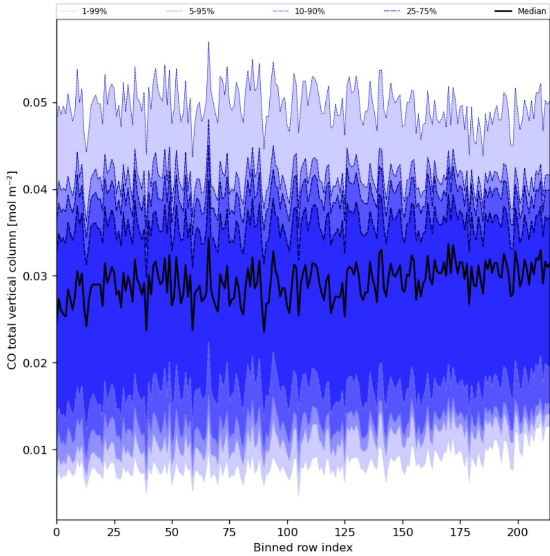
Figure 26: Along track statistics of “CO total vertical column” for 2024-03-17 to 2024-03-19
