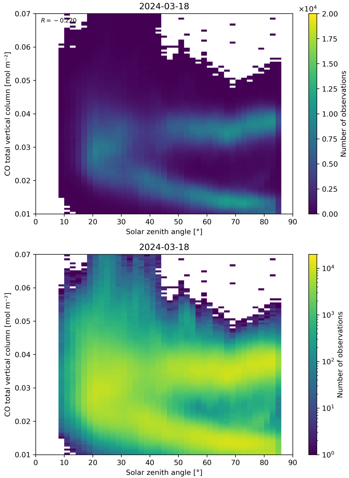
Figure 61: Scatter density plot of “Solar zenith angle” against “CO total vertical column” for 2024-03-17 to 2024-03-19.
