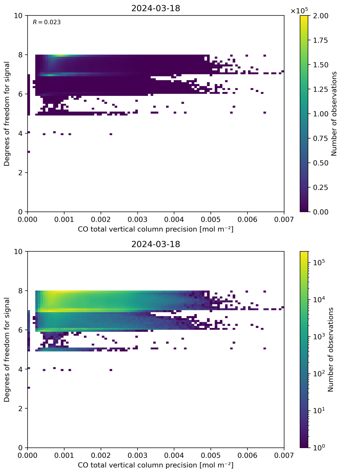
Figure 45: Scatter density plot of “CO total vertical column precision” against “Degrees of freedom for signal” for 2024-03-17 to 2024-03-19.
