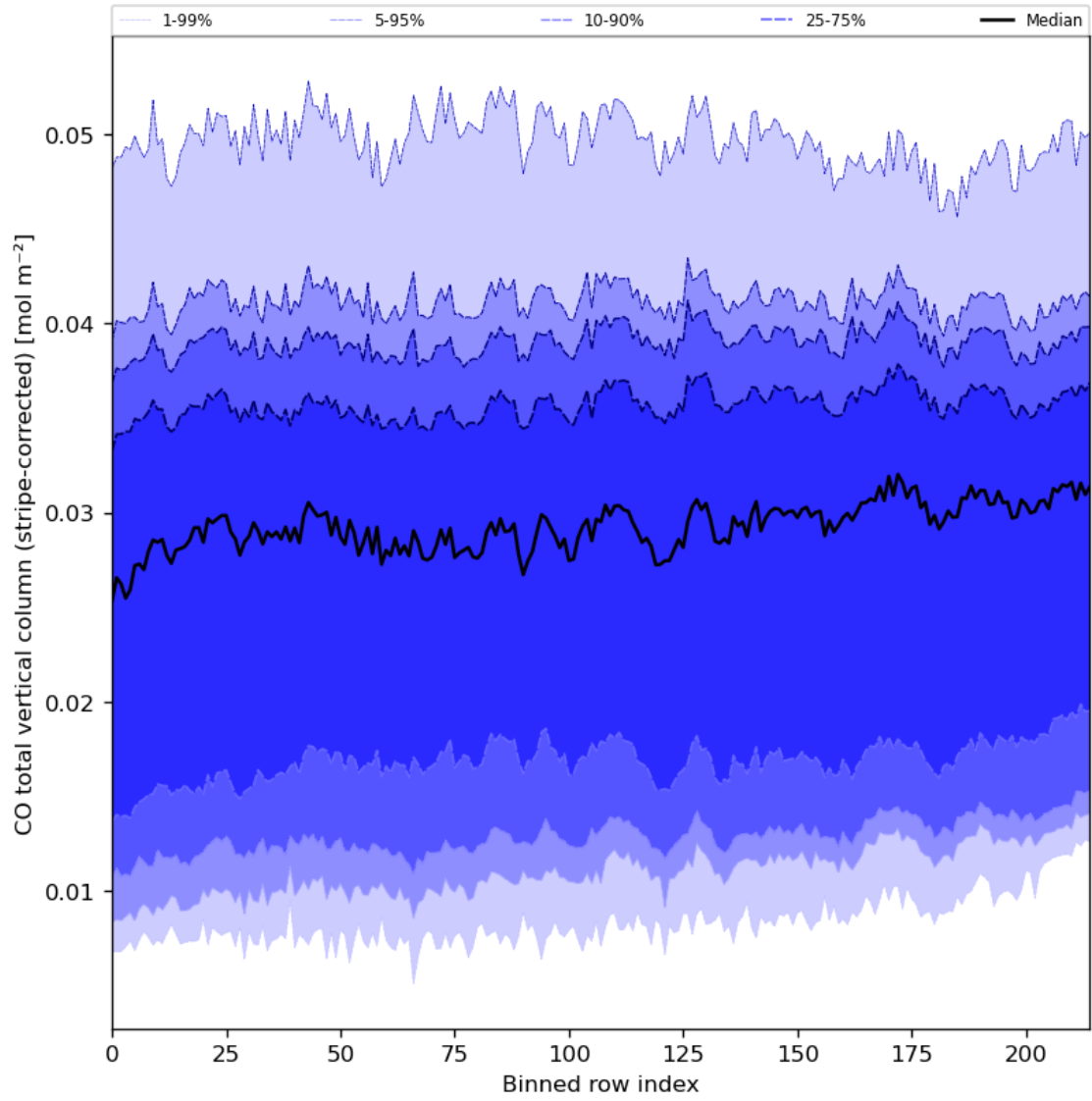
Figure 27: Along track statistics of “CO total vertical column (stripe-corrected)” for 2024-03-17 to 2024-03-19
