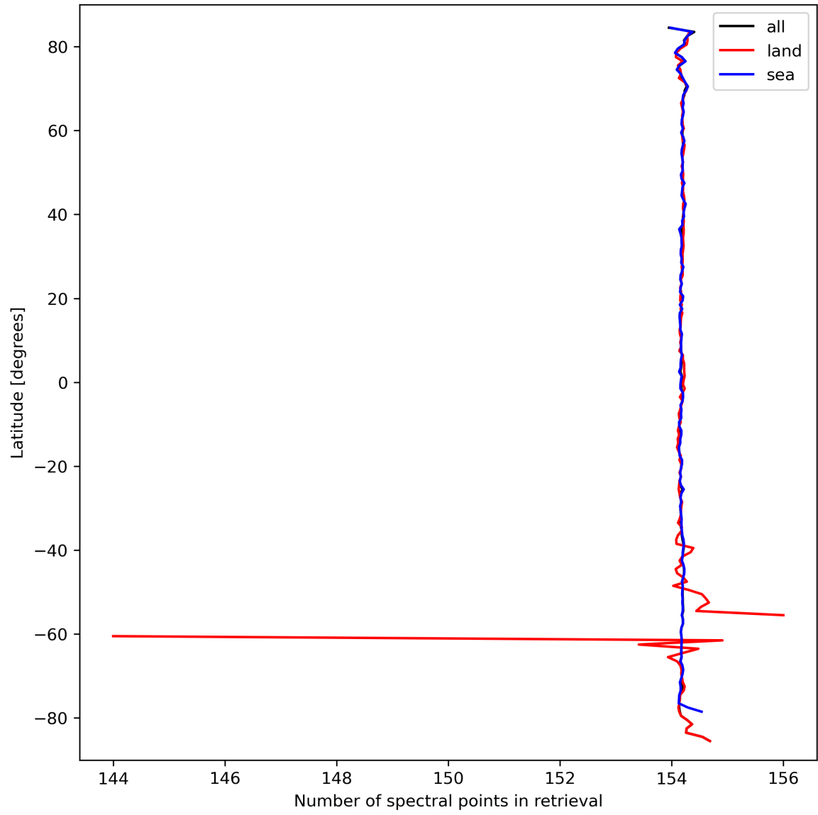
Figure 13: Zonal average of “Number of spectral points in retrieval” for 2024-03-17 to 2024-03-19.
