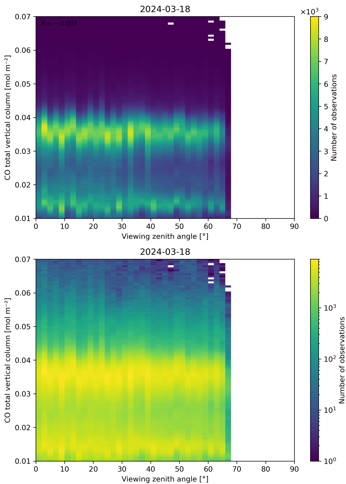
Figure 69: Scatter density plot of “Viewing zenith angle” against “CO total vertical column” for 2024-03-17 to 2024-03-19.
