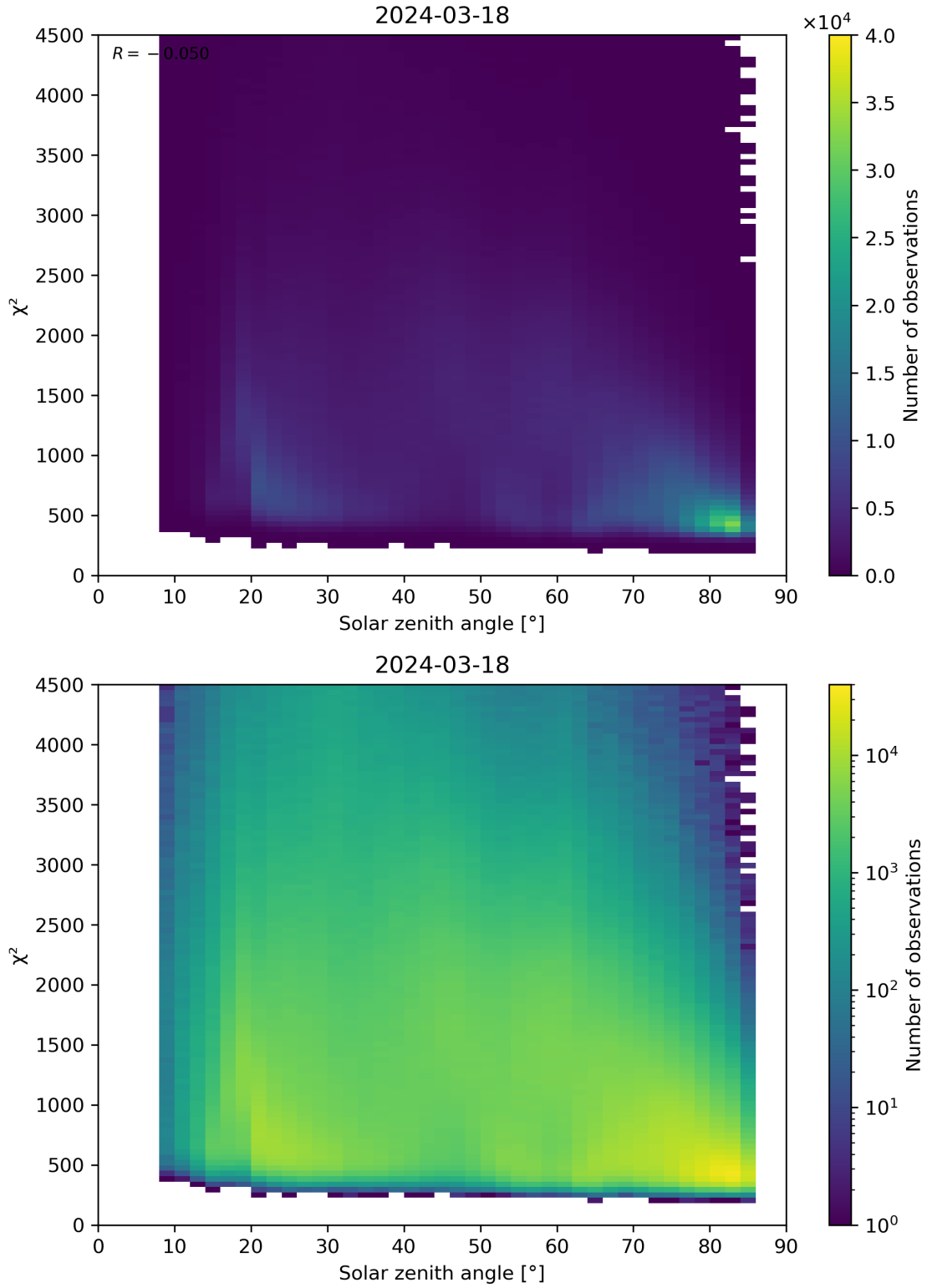
Figure 64: Scatter density plot of “Solar zenith angle” against “ \chi^2 ” for 2024-03-17 to 2024-03-19.
