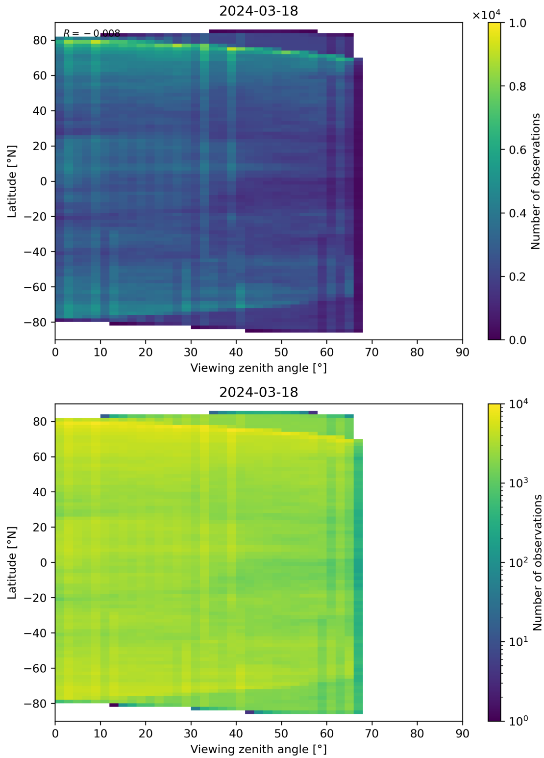
Figure 74: Scatter density plot of “Viewing zenith angle” against “Latitude” for 2024-03-17 to 2024-03-19.
