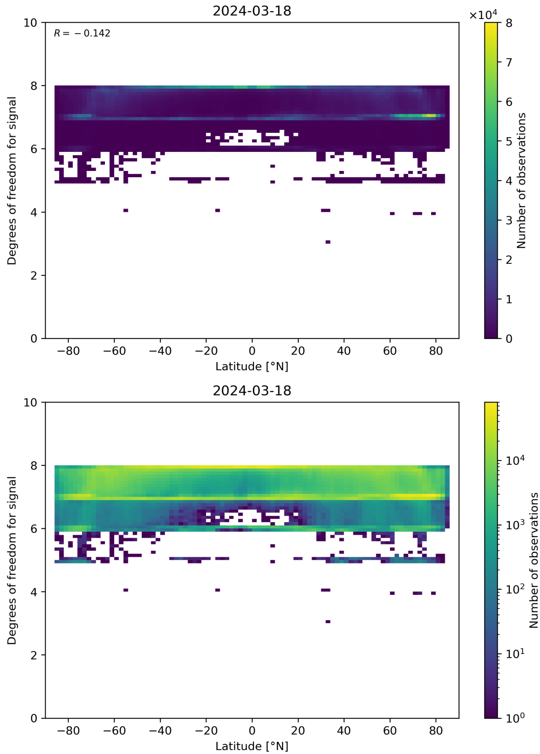
Figure 55: Scatter density plot of “Latitude” against “Degrees of freedom for signal” for 2024-03-17 to 2024-03-19.
