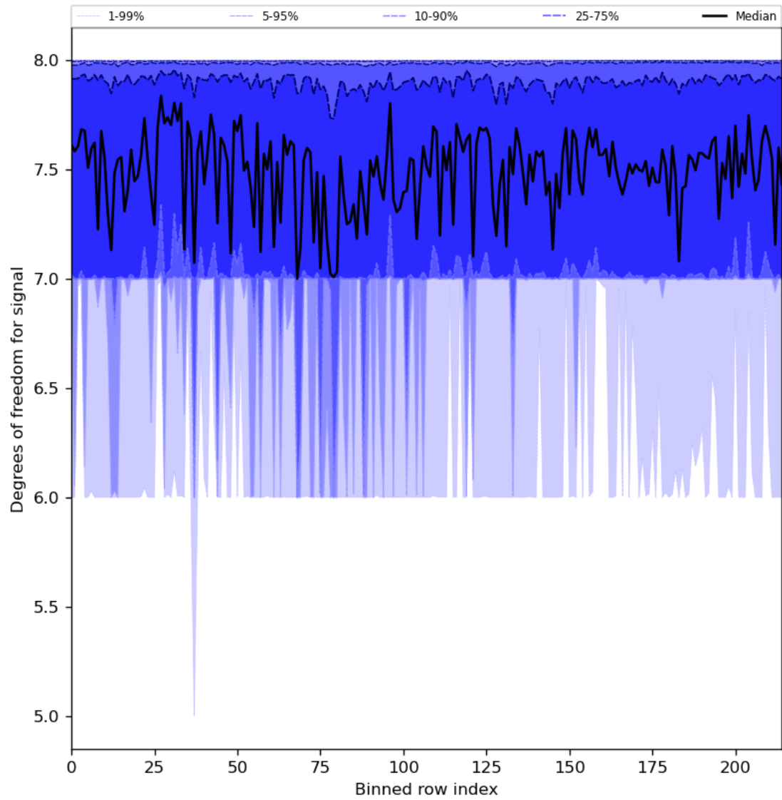
Figure 31: Along track statistics of “Degrees of freedom for signal” for 2024-03-17 to 2024-03-19
