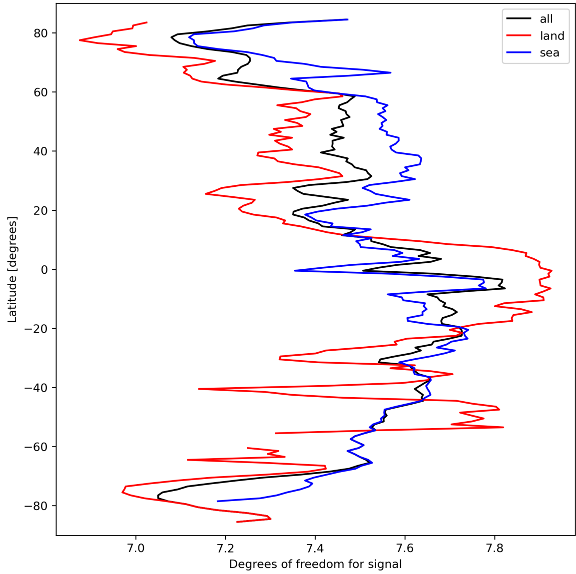
Figure 15: Zonal average of “Degrees of freedom for signal” for 2024-03-17 to 2024-03-19.
