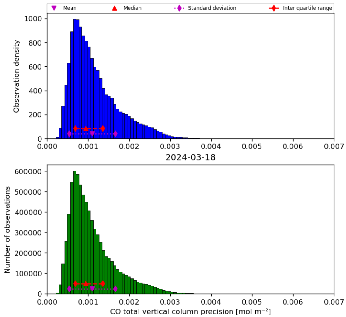
Figure 20: Histogram of “CO total vertical column precision” for 2024-03-17 to 2024-03-19
