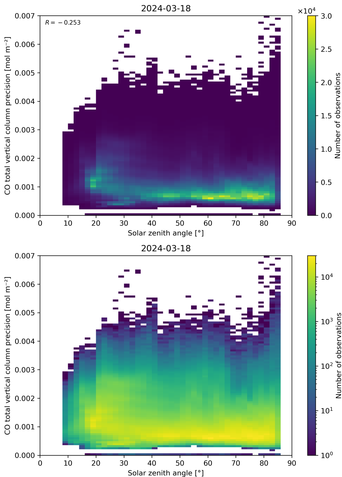
Figure 63: Scatter density plot of “Solar zenith angle” against “CO total vertical column precision” for 2024-03-17 to 2024-03-19.
