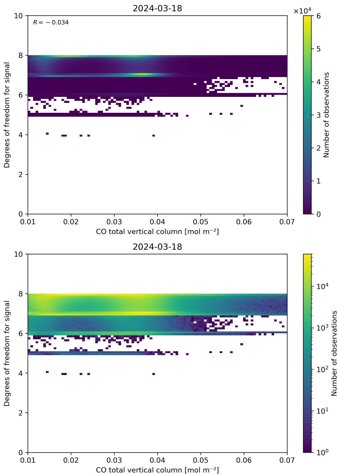
Figure 41: Scatter density plot of “CO total vertical column” against “Degrees of freedom for signal” for 2024-03-17 to 2024-03-19.
