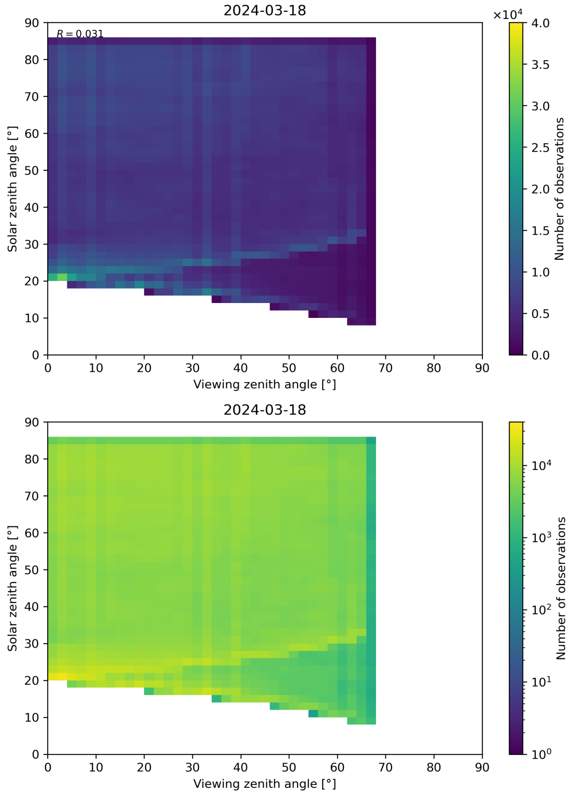
Figure 77: Scatter density plot of “Viewing zenith angle” against “Solar zenith angle” for 2024-03-17 to 2024-03-19.
