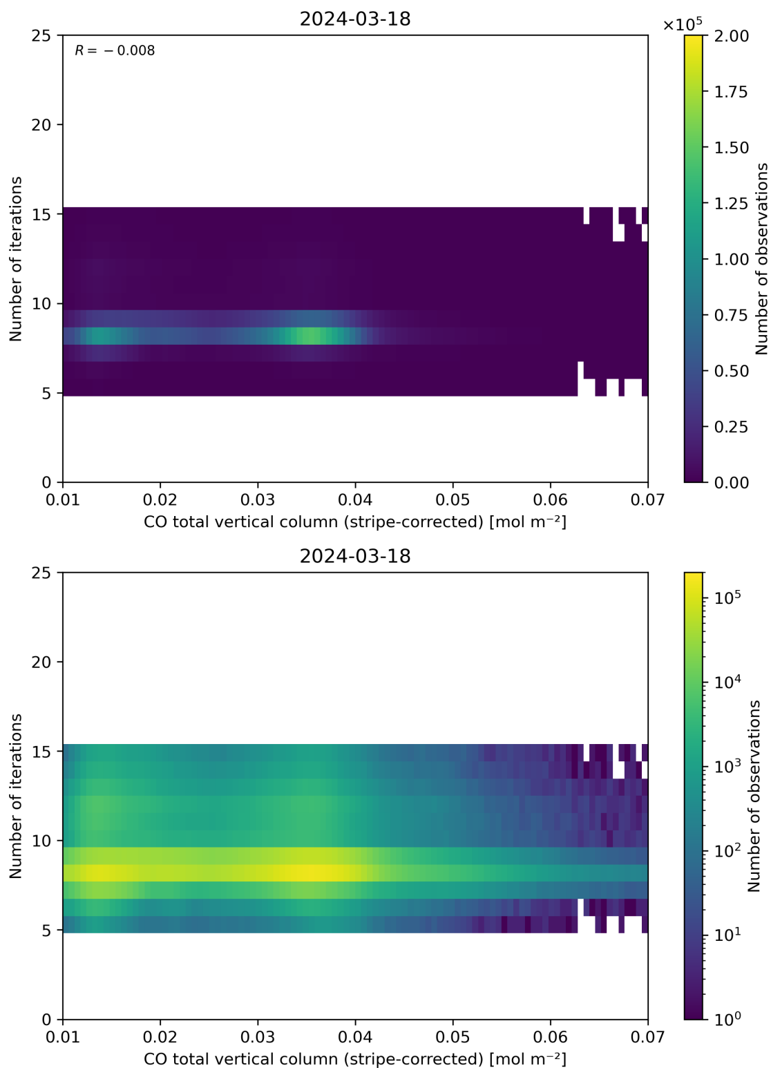
Figure 39: Scatter density plot of “CO total vertical column (stripe-corrected)” against “Number of iterations” for 2024-03-17 to 2024-03-19.
