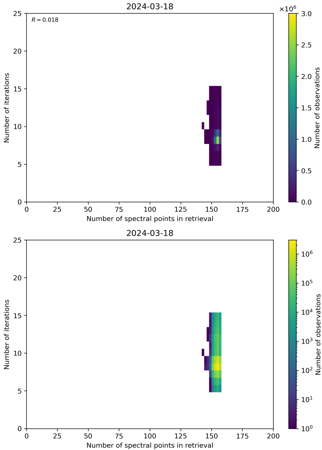
Figure 60: Scatter density plot of “Number of spectral points in retrieval” against “Number of iterations” for 2024-03-17 to 2024-03-19.
