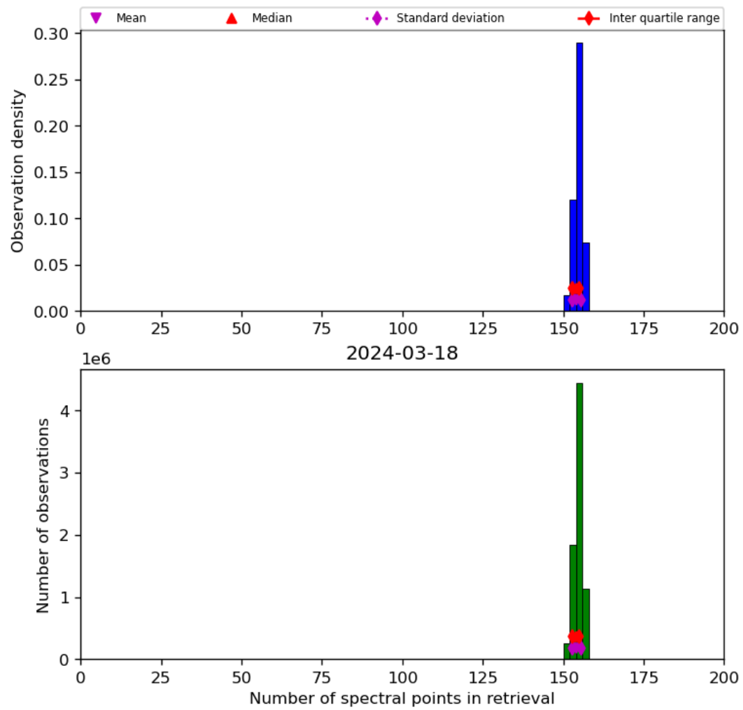
Figure 21: Histogram of “Number of spectral points in retrieval” for 2024-03-17 to 2024-03-19
