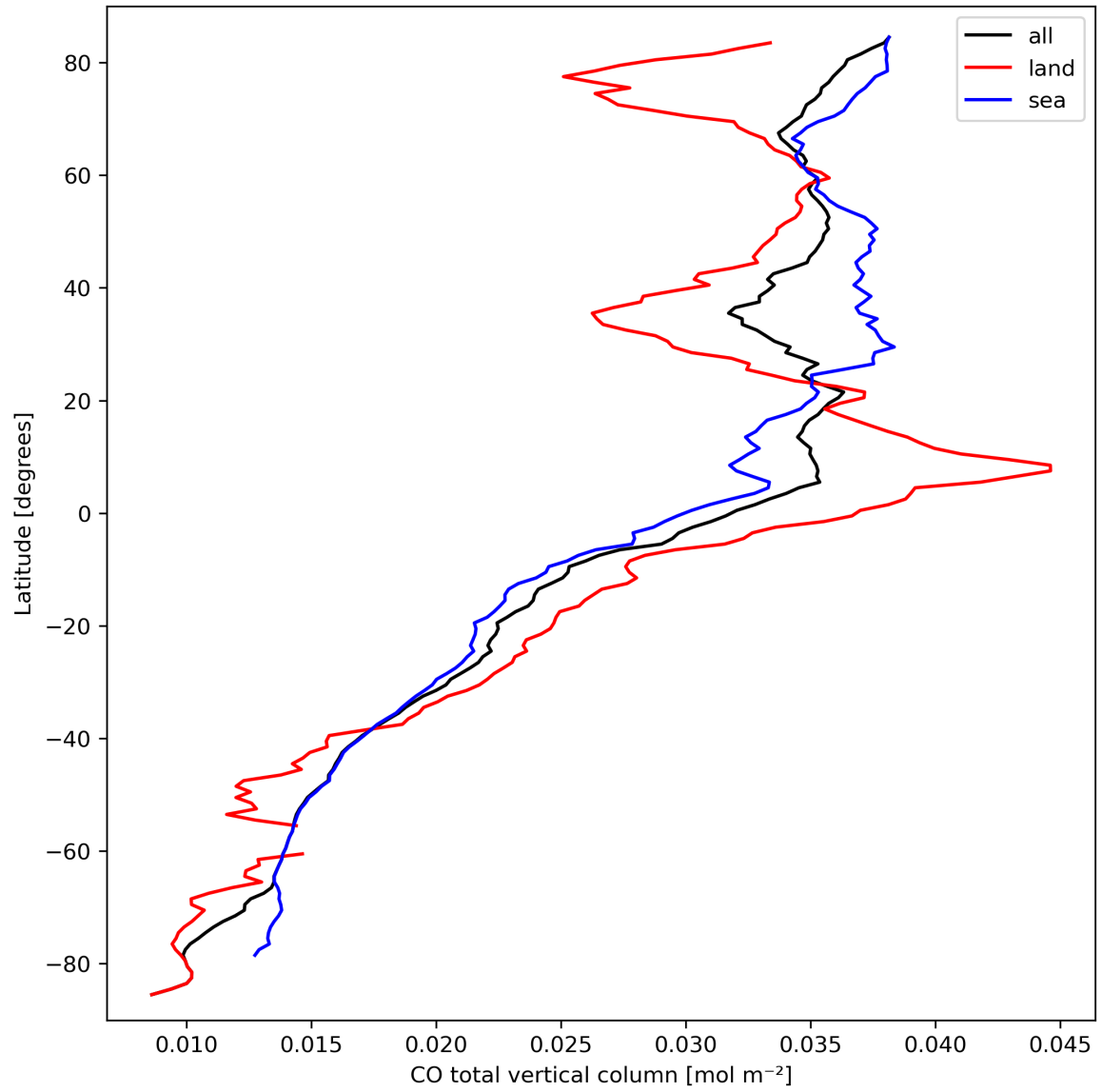
Figure 10: Zonal average of “CO total vertical column” for 2024-03-17 to 2024-03-19.
