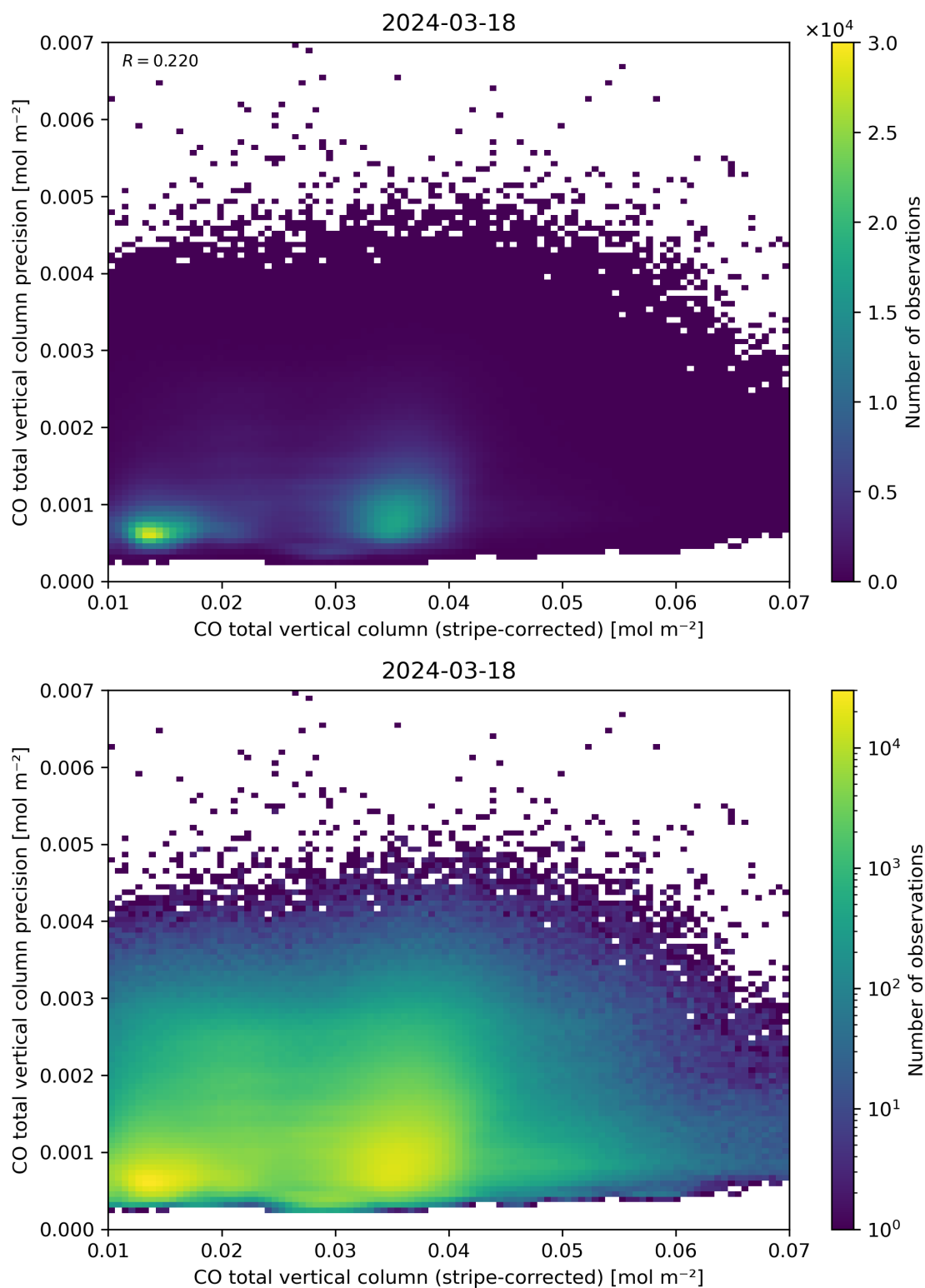
Figure 36: Scatter density plot of “CO total vertical column (stripe-corrected)” against “CO total vertical column precision” for 2024-03-17 to 2024-03-19.
