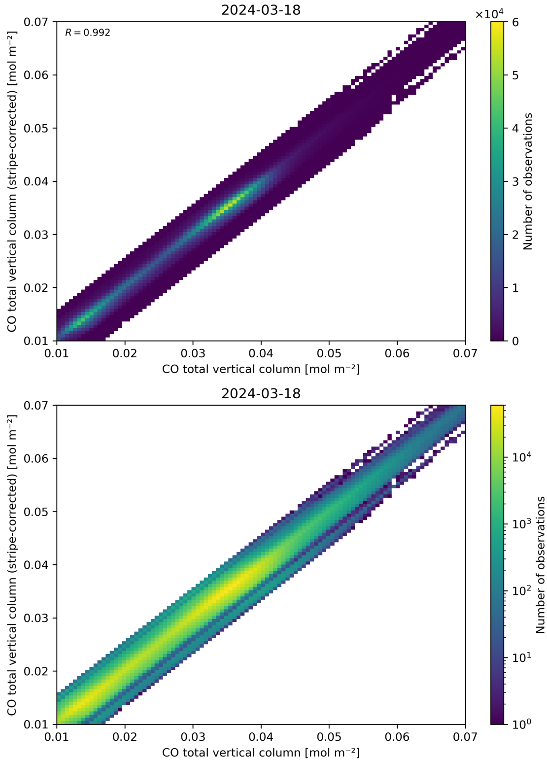
Figure 33: Scatter density plot of “CO total vertical column” against “CO total vertical column (stripe-corrected)” for 2024-03-17 to 2024-03-19.
