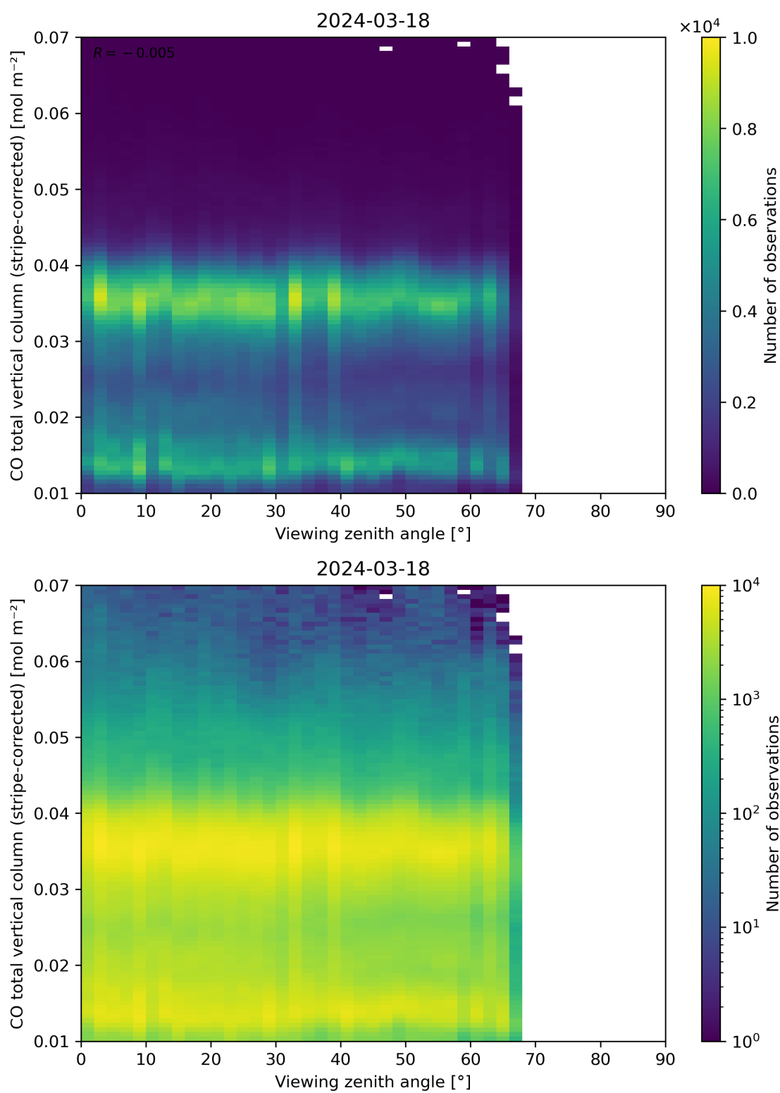
Figure 70: Scatter density plot of “Viewing zenith angle” against “CO total vertical column (stripe-corrected)” for 2024-03-17 to 2024-03-19.
