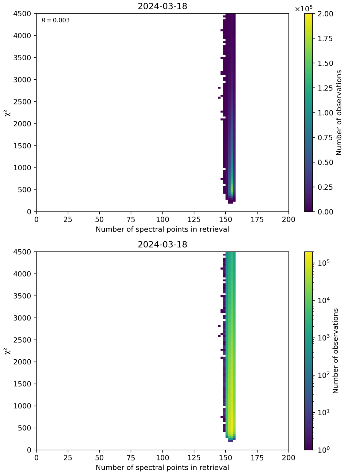
Figure 58: Scatter density plot of “Number of spectral points in retrieval” against “ \chi^2 ” for 2024-03-17 to 2024-03-19.
