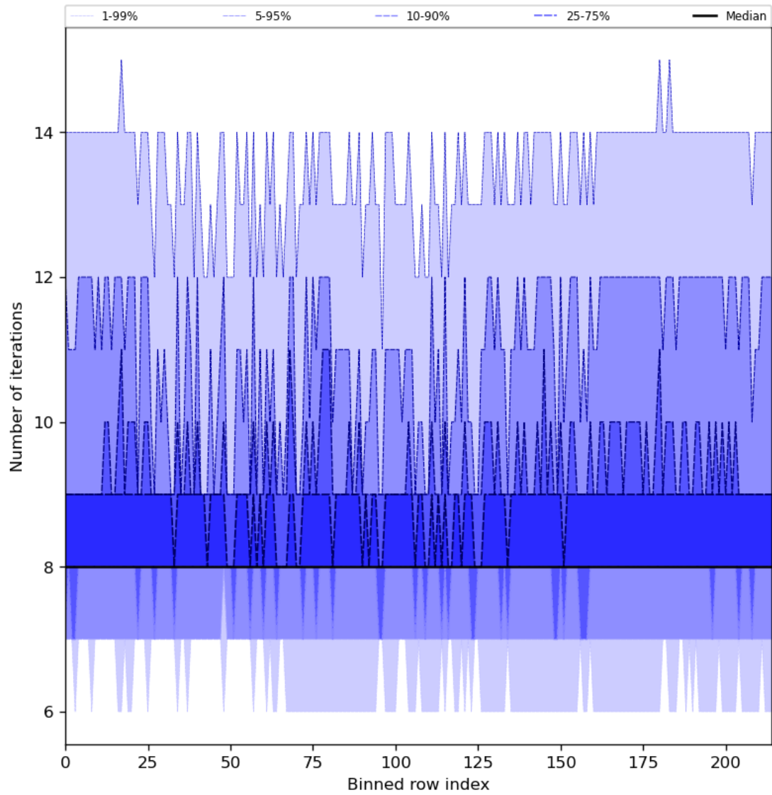
Figure 32: Along track statistics of “Number of iterations” for 2024-03-17 to 2024-03-19
