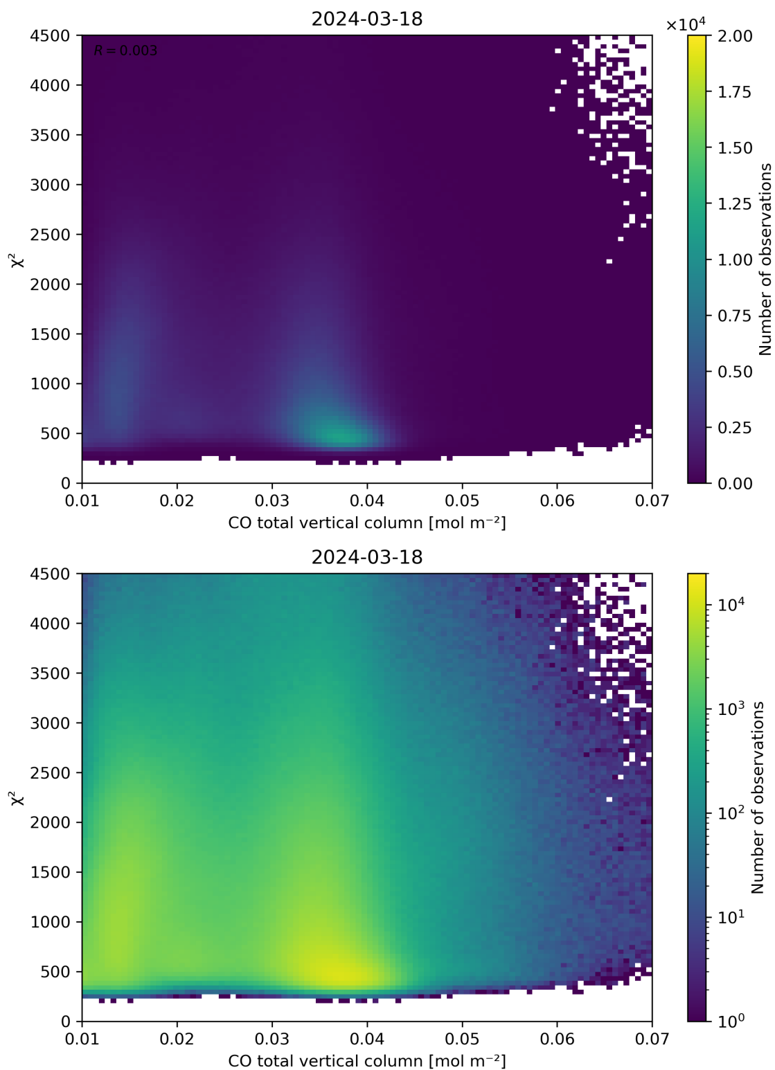
Figure 35: Scatter density plot of “CO total vertical column” against “ \chi^2 ” for 2024-03-17 to 2024-03-19.
