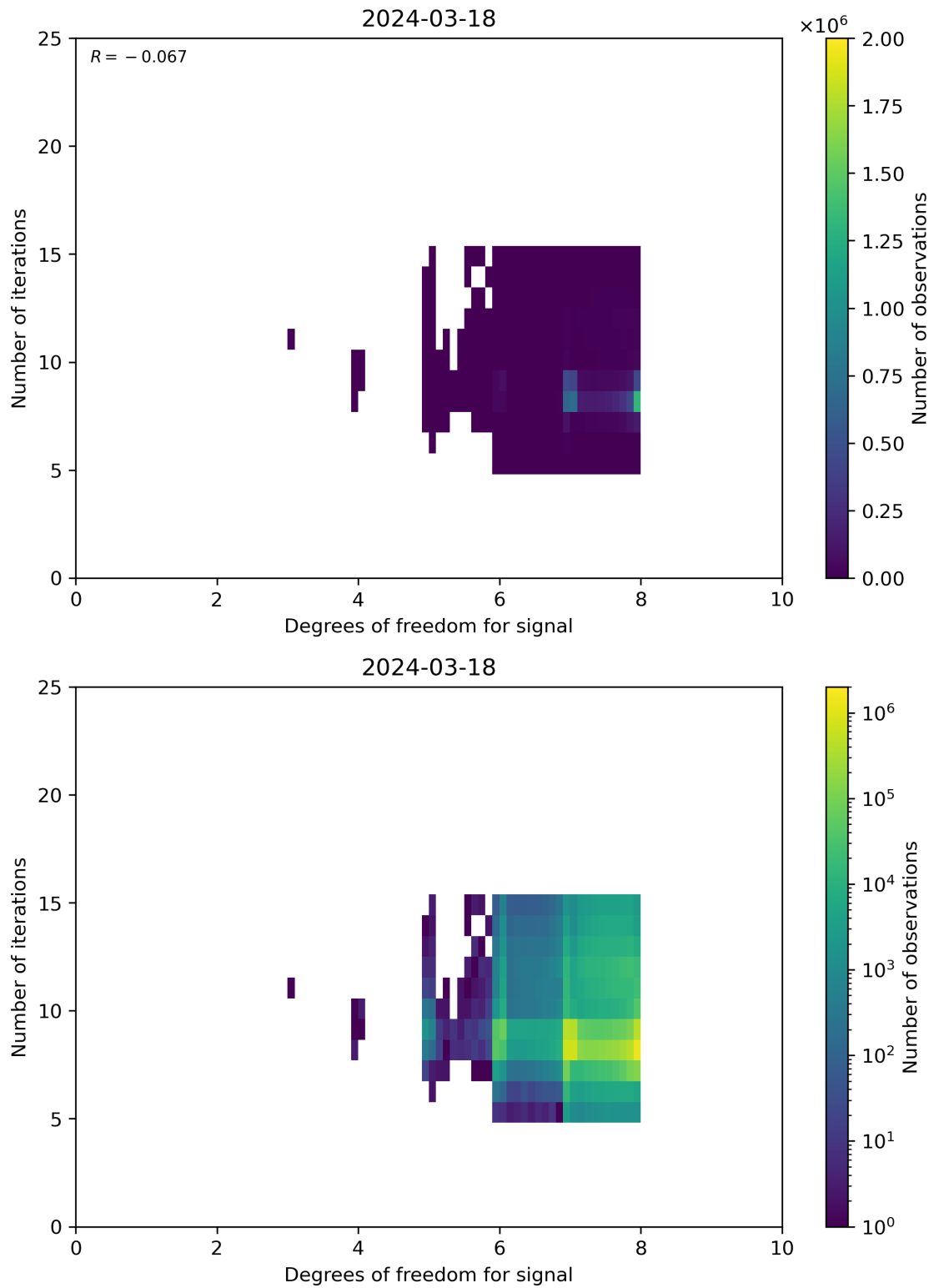
Figure 50: Scatter density plot of “Degrees of freedom for signal” against “Number of iterations” for 2024-03-17 to 2024-03-19.
