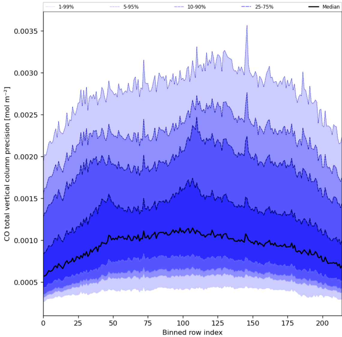
Figure 28: Along track statistics of “CO total vertical column precision” for 2024-03-17 to 2024-03-19
