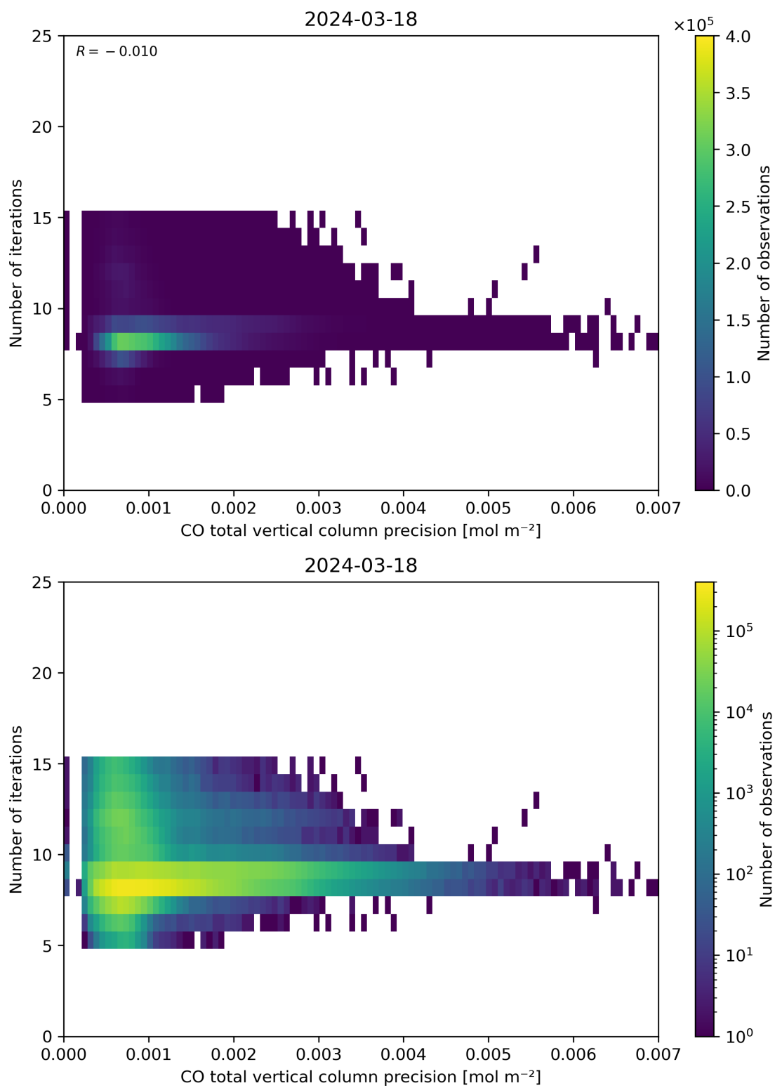
Figure 46: Scatter density plot of “CO total vertical column precision” against “Number of iterations” for 2024-03-17 to 2024-03-19.
