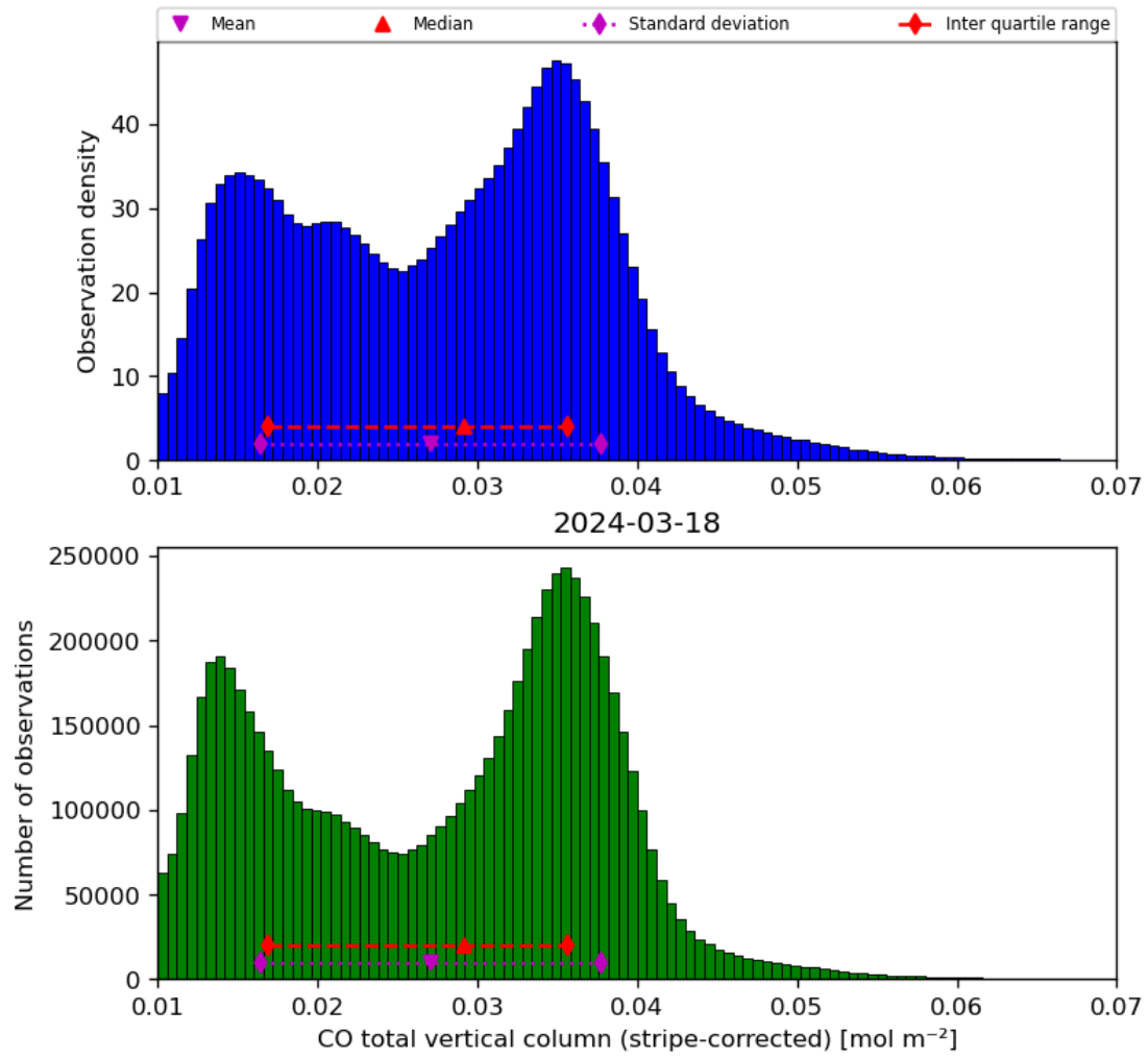
Figure 19: Histogram of “CO total vertical column (stripe-corrected)” for 2024-03-17 to 2024-03-19
