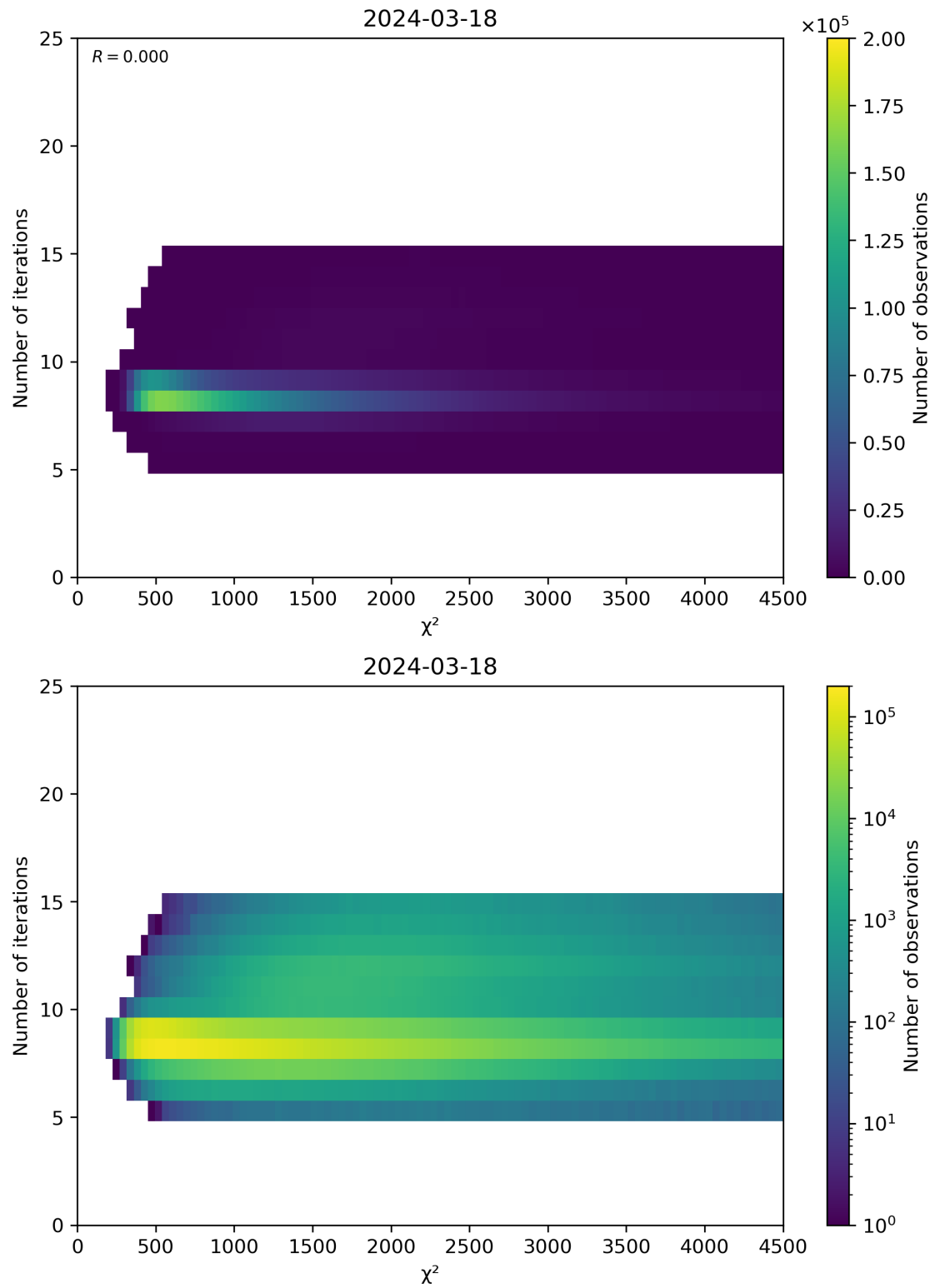
Figure 49: Scatter density plot of “ \chi^2 ” against “Number of iterations” for 2024-03-17 to 2024-03-19.
