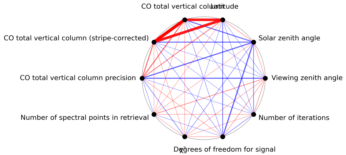
Figure 1: Map of correlation graph for 2024-03-17 to 2024-03-19.
