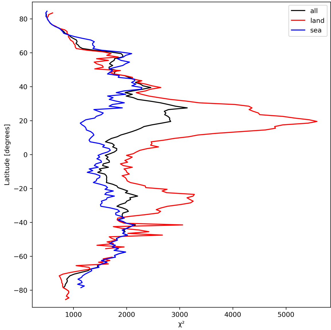
Figure 14: Zonal average of “ \chi^2 ” for 2024-03-17 to 2024-03-19.
