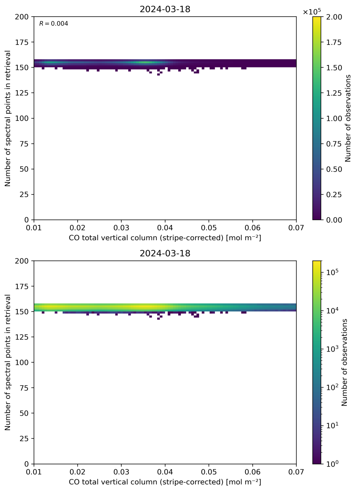
Figure 40: Scatter density plot of “CO total vertical column (stripe-corrected)” against “Number of spectral points in retrieval” for 2024-03-17 to 2024-03-19.
