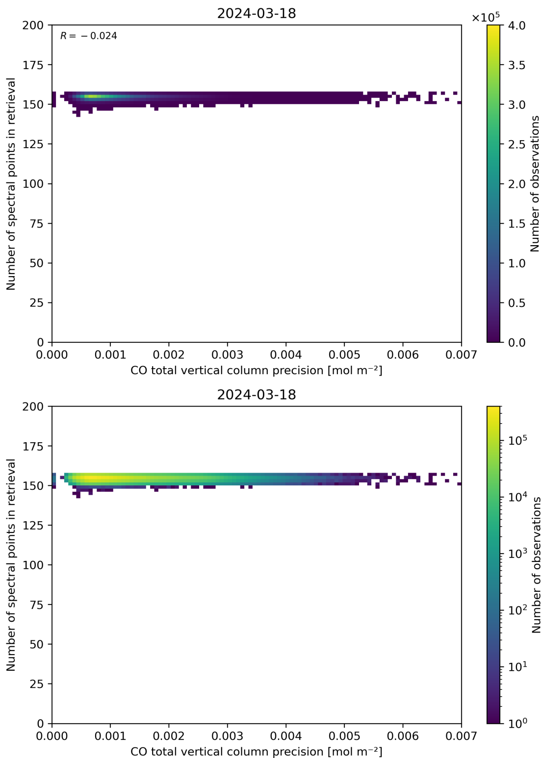
Figure 47: Scatter density plot of “CO total vertical column precision” against “Number of spectral points in retrieval” for 2024-03-17 to 2024-03-19.
