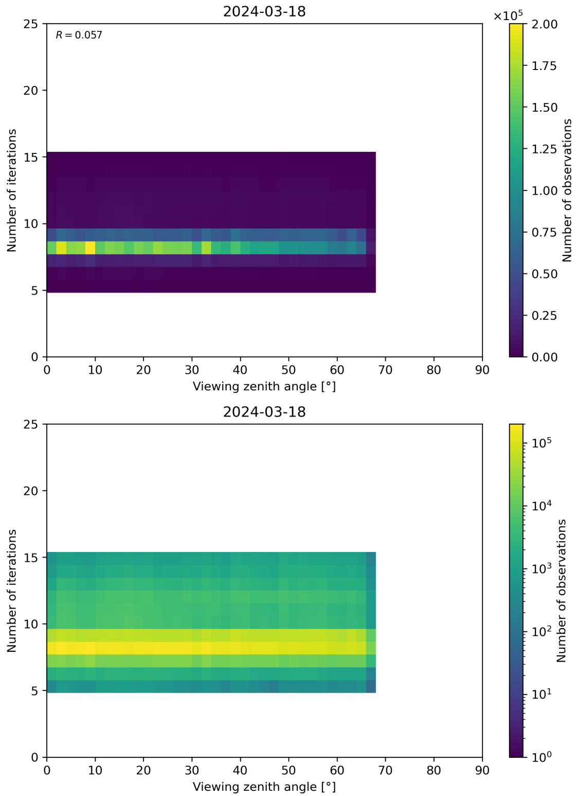
Figure 75: Scatter density plot of “Viewing zenith angle” against “Number of iterations” for 2024-03-17 to 2024-03-19.
