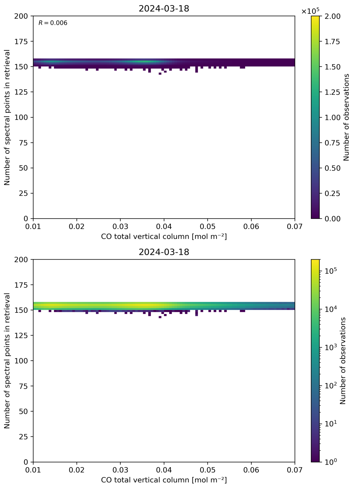
Figure 43: Scatter density plot of “CO total vertical column” against “Number of spectral points in retrieval” for 2024-03-17 to 2024-03-19.
