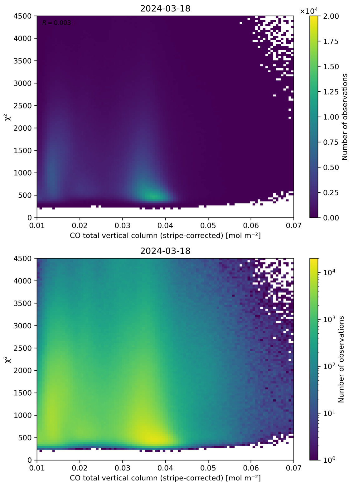
Figure 37: Scatter density plot of “CO total vertical column (stripe-corrected)” against “ \chi^2 ” for 2024-03-17 to 2024-03-19.
