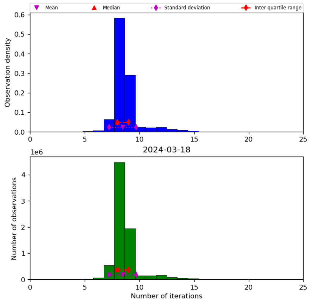
Figure 24: Histogram of “Number of iterations” for 2024-03-17 to 2024-03-19
