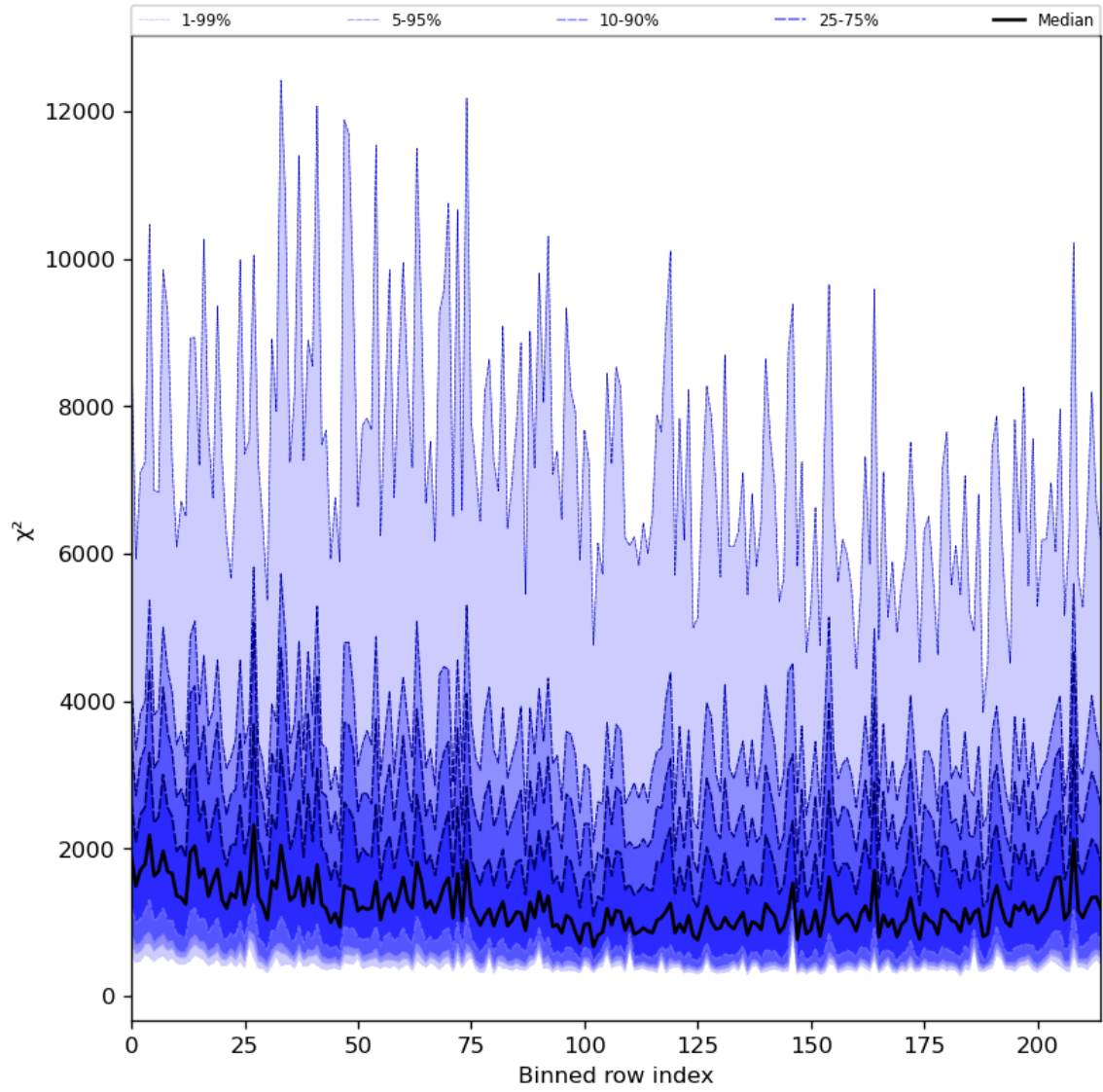
Figure 30: Along track statistics of “ \chi^2 ” for 2024-03-17 to 2024-03-19
