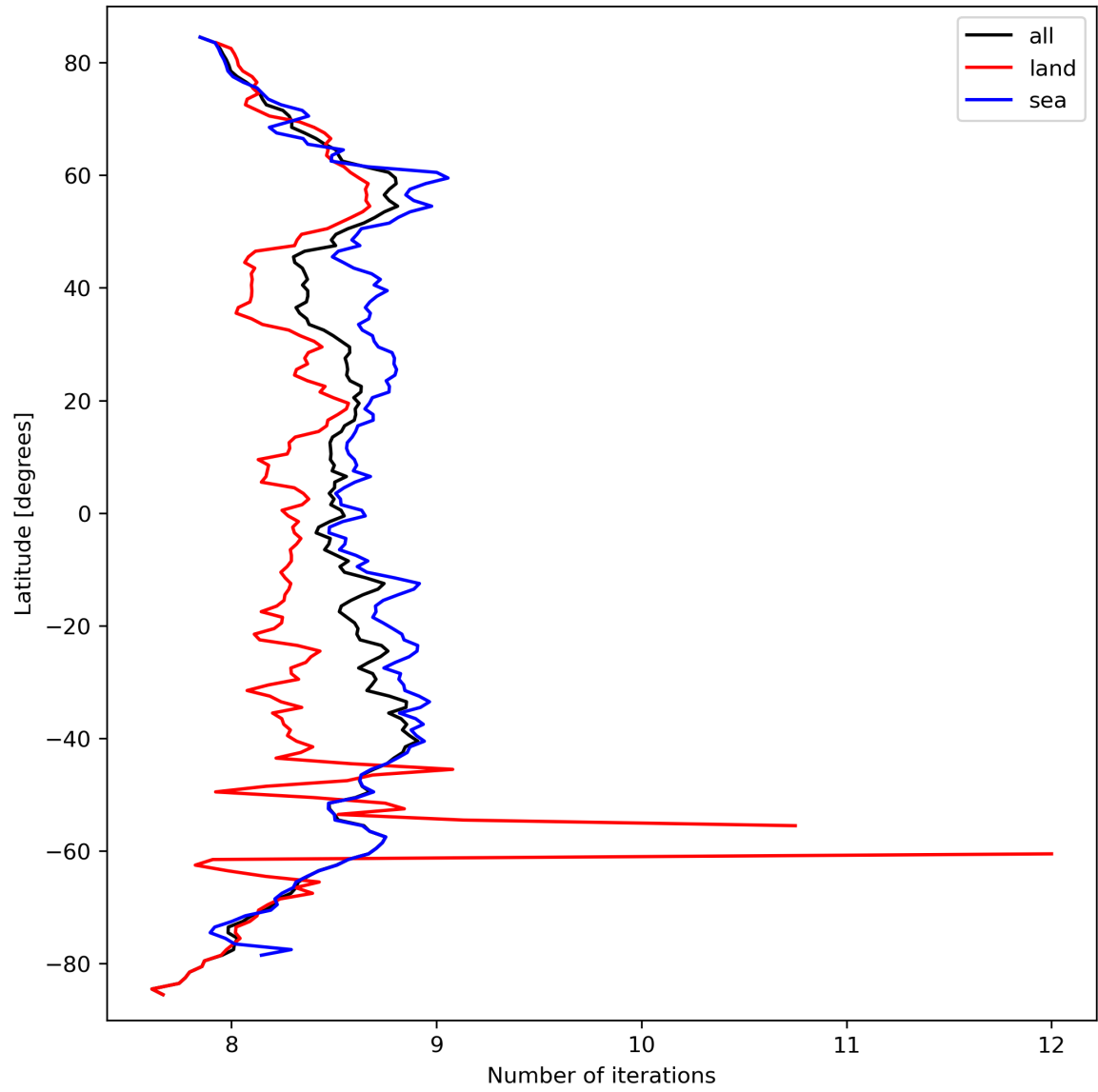
Figure 16: Zonal average of “Number of iterations” for 2024-03-17 to 2024-03-19.
