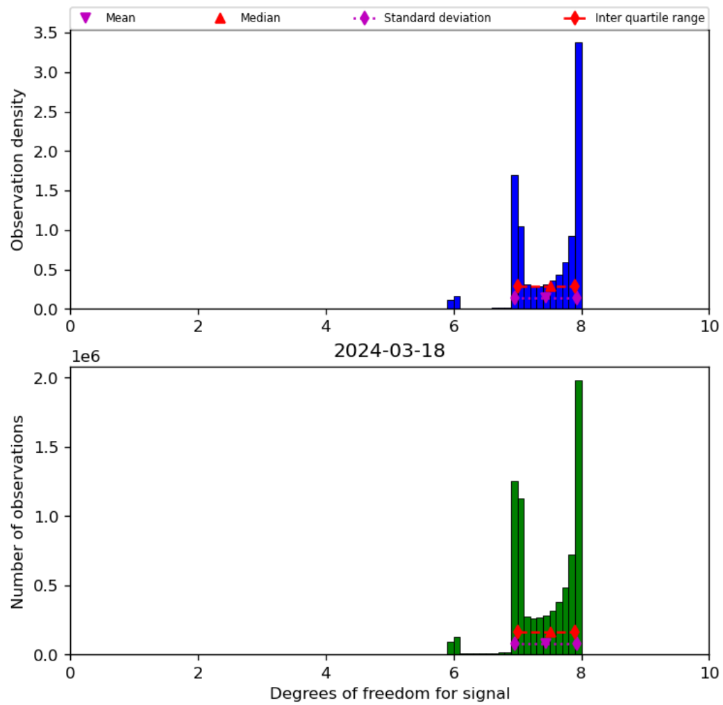
Figure 23: Histogram of “Degrees of freedom for signal” for 2024-03-17 to 2024-03-19
