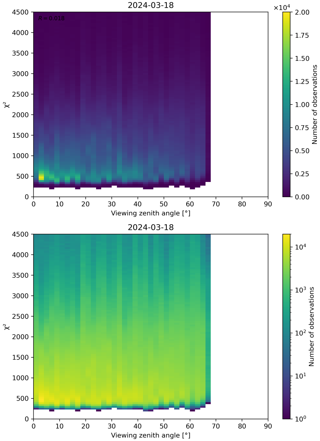
Figure 72: Scatter density plot of “Viewing zenith angle” against “ \chi^2 ” for 2024-03-17 to 2024-03-19.
