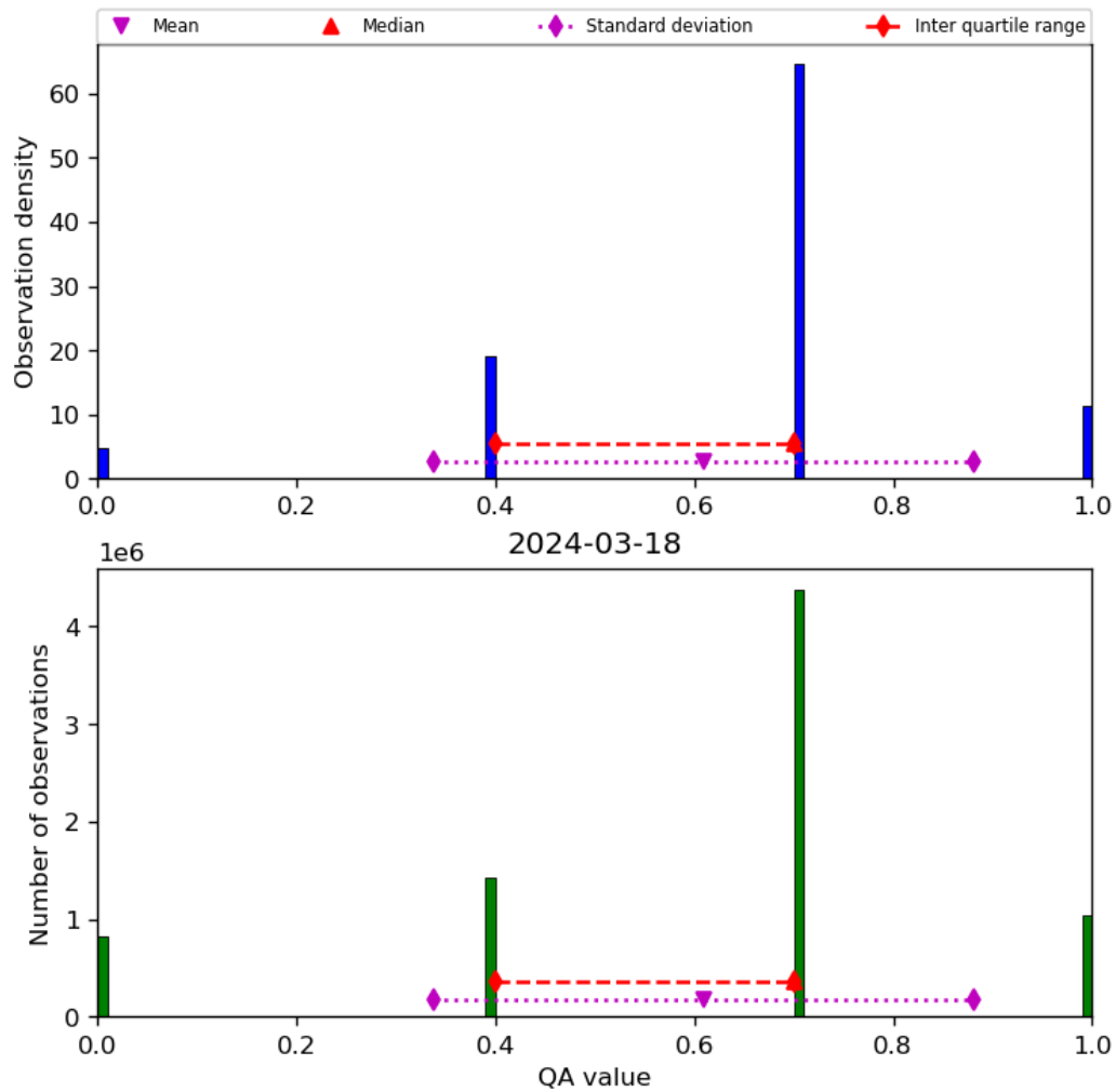
Figure 17: Histogram of “QA value” for 2024-03-17 to 2024-03-19
