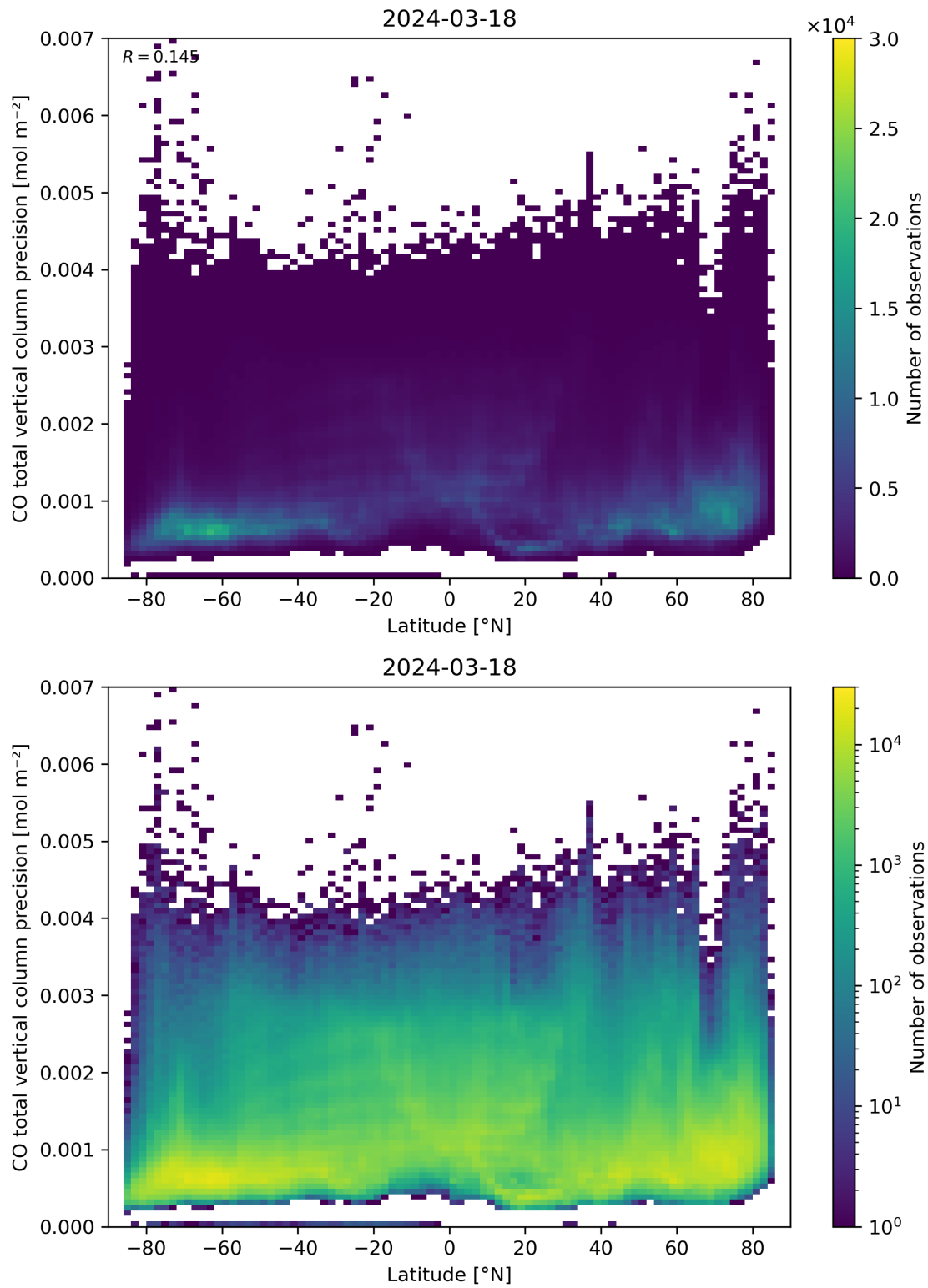
Figure 53: Scatter density plot of “Latitude” against “CO total vertical column precision” for 2024-03-17 to 2024-03-19.
