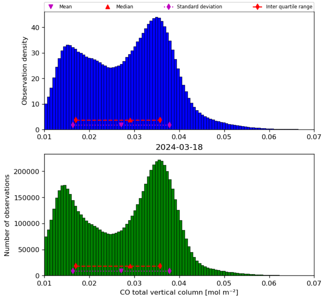
Figure 18: Histogram of “CO total vertical column” for 2024-03-17 to 2024-03-19
