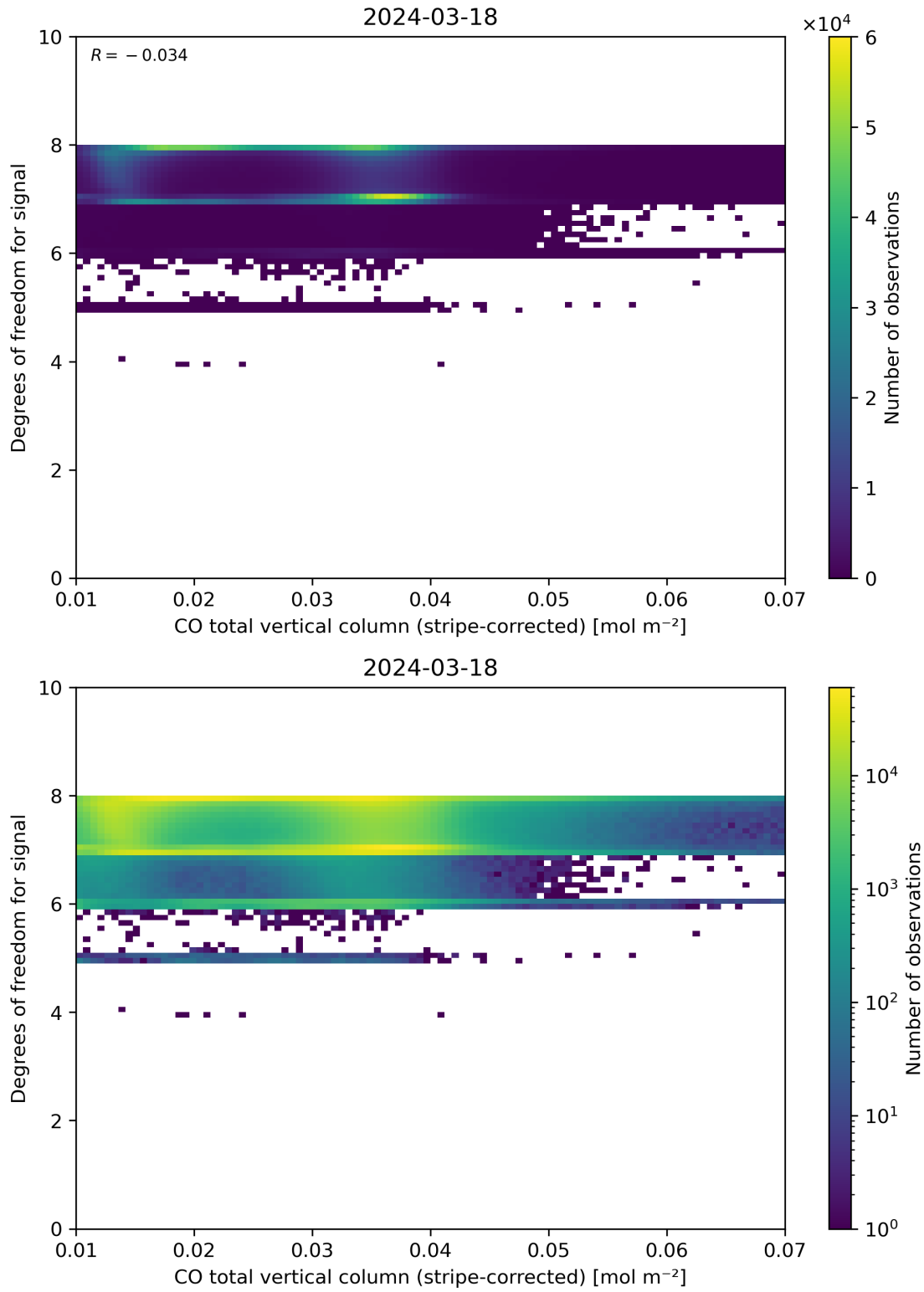
Figure 38: Scatter density plot of “CO total vertical column (stripe-corrected)” against “Degrees of freedom for signal” for 2024-03-17 to 2024-03-19.
