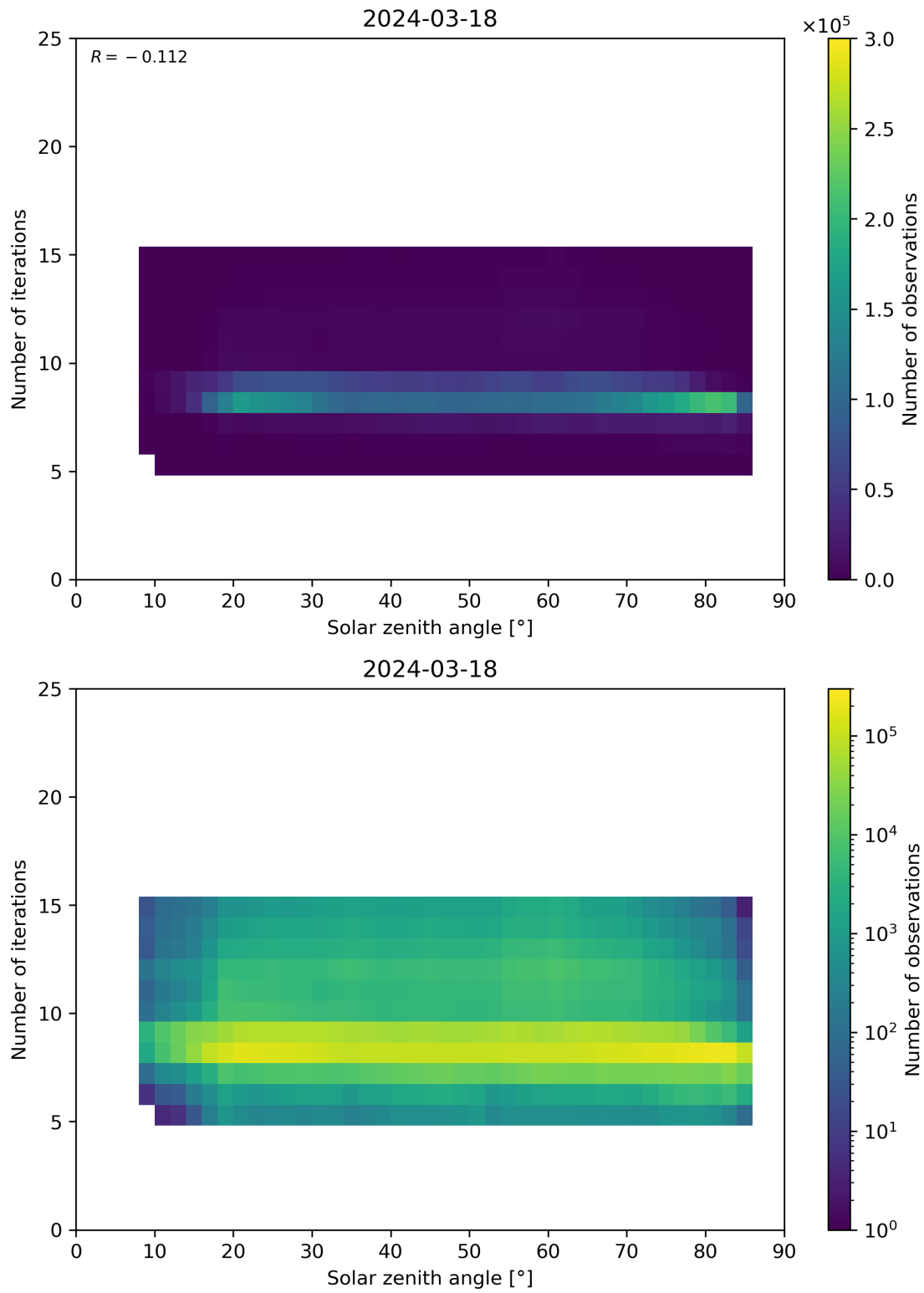
Figure 67: Scatter density plot of “Solar zenith angle” against “Number of iterations” for 2024-03-17 to 2024-03-19.
