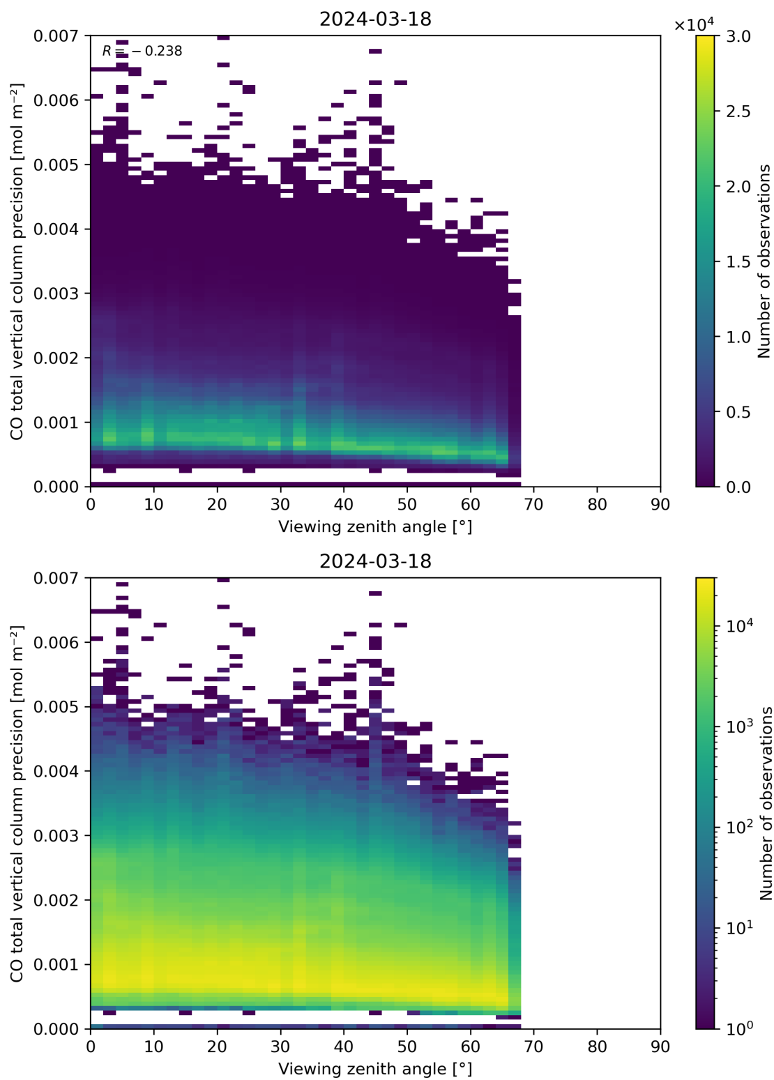
Figure 71: Scatter density plot of “Viewing zenith angle” against “CO total vertical column precision” for 2024-03-17 to 2024-03-19.
