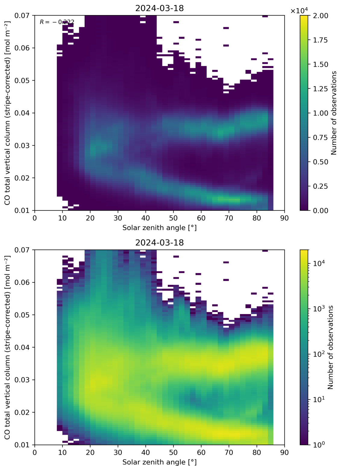
Figure 62: Scatter density plot of “Solar zenith angle” against “CO total vertical column (stripe-corrected)” for 2024-03-17 to 2024-03-19.
