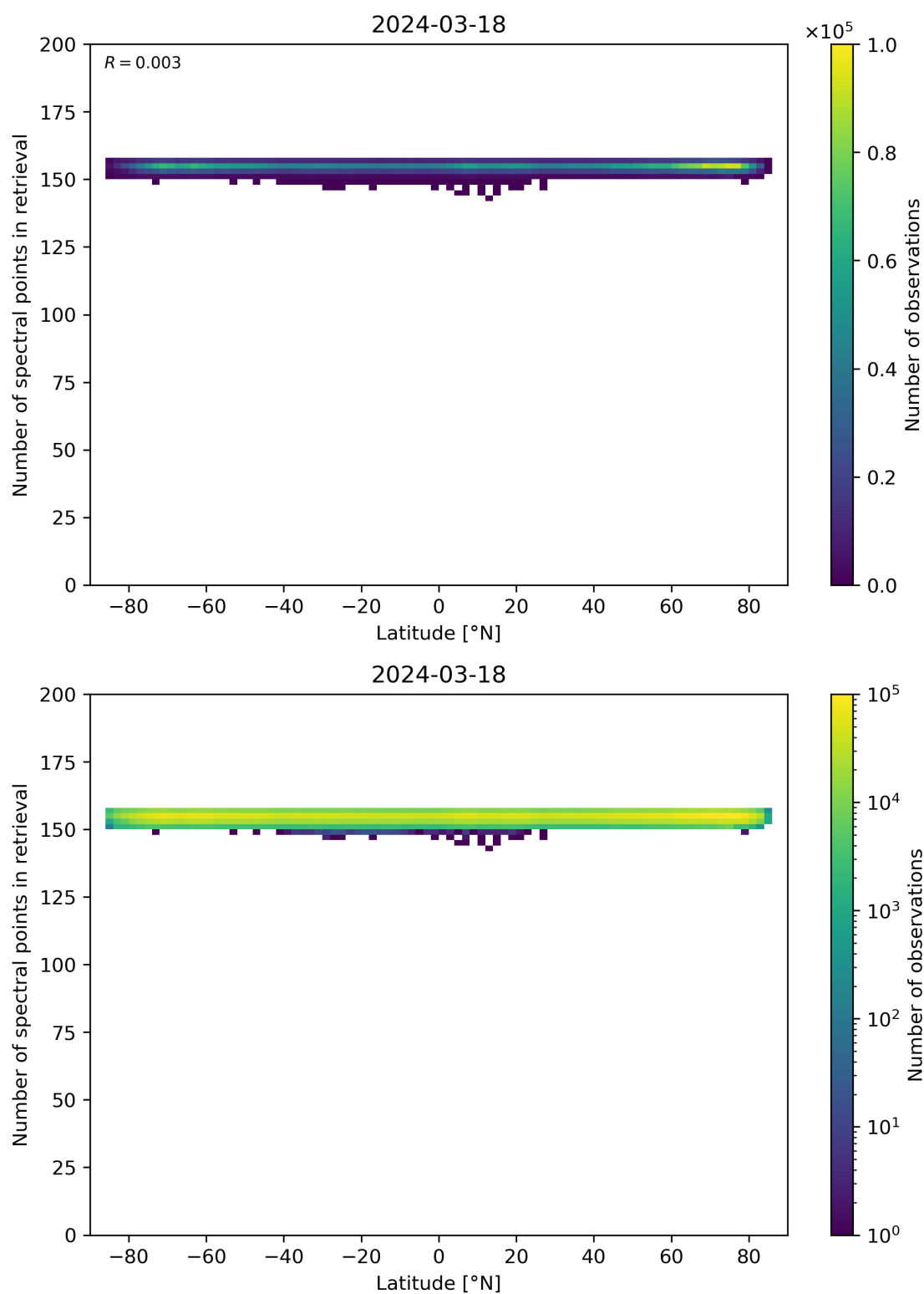
Figure 57: Scatter density plot of “Latitude” against “Number of spectral points in retrieval” for 2024-03-17 to 2024-03-19.
