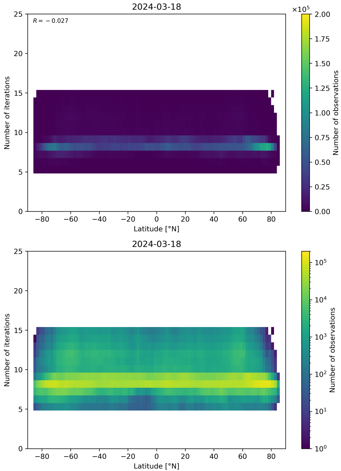
Figure 56: Scatter density plot of “Latitude” against “Number of iterations” for 2024-03-17 to 2024-03-19.
