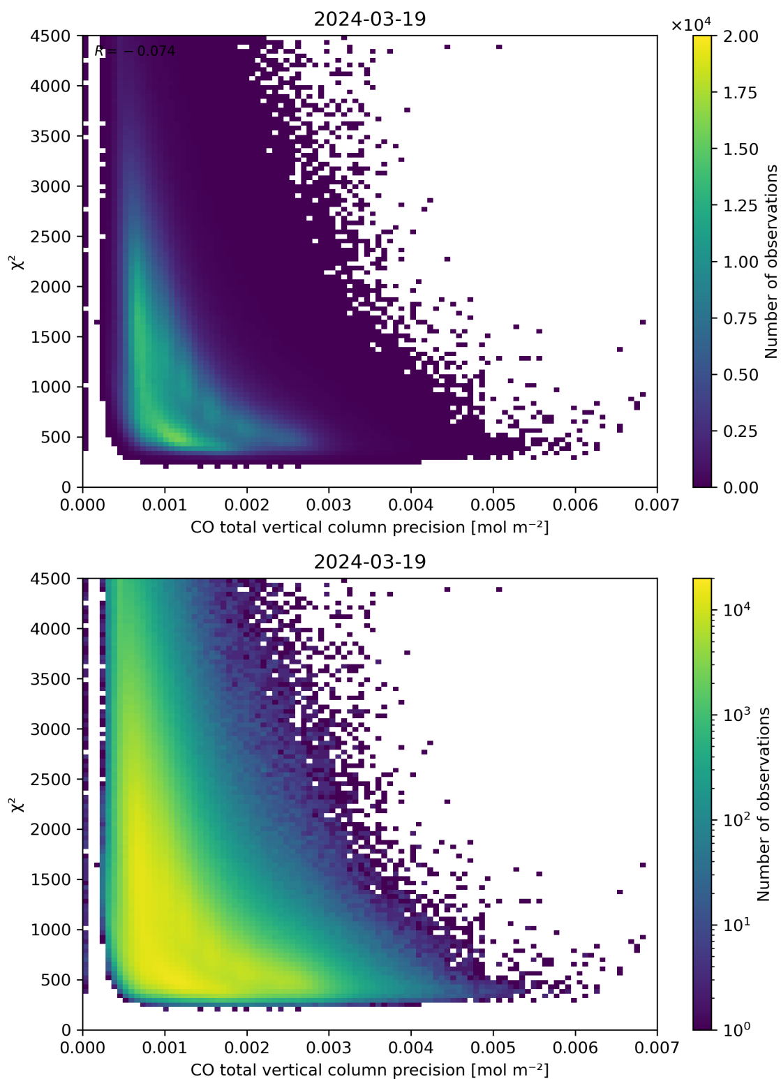
Figure 44: Scatter density plot of “CO total vertical column precision” against “ \chi^2 ” for 2024-03-18 to 2024-03-20.
