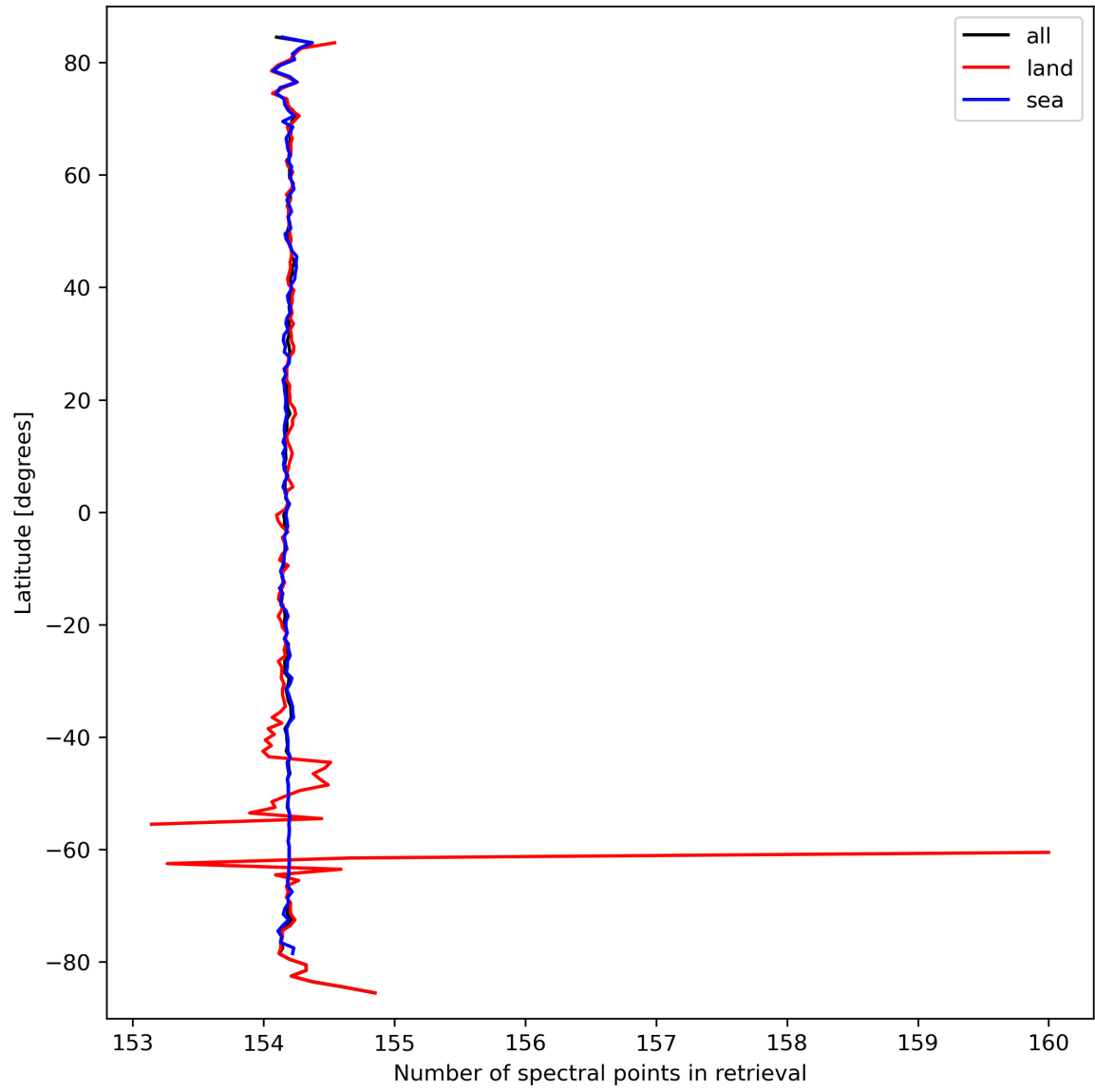
Figure 13: Zonal average of “Number of spectral points in retrieval” for 2024-03-18 to 2024-03-20.
