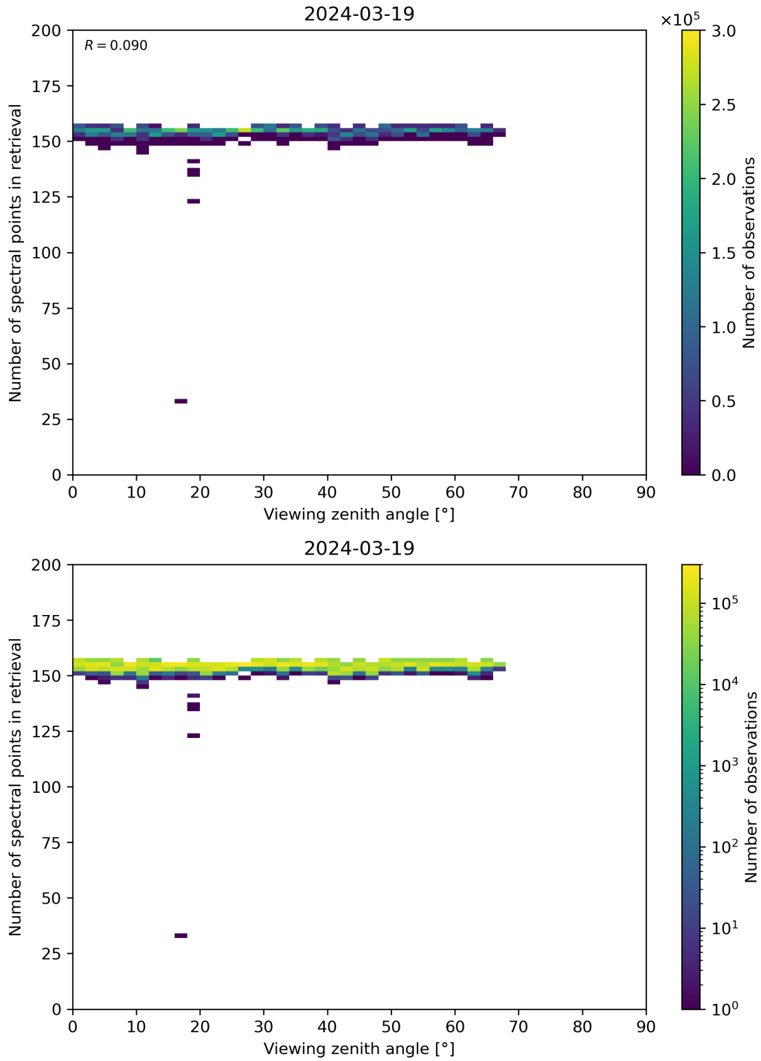
Figure 76: Scatter density plot of “Viewing zenith angle” against “Number of spectral points in retrieval” for 2024-03-18 to 2024-03-20.
