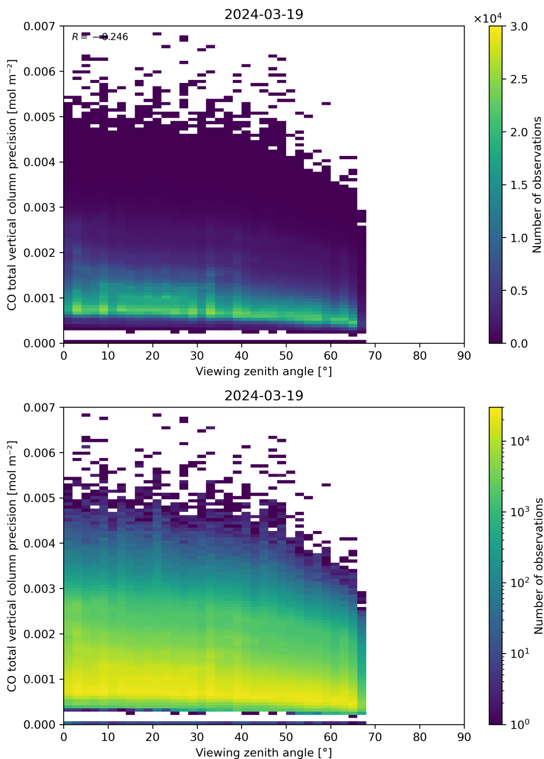
Figure 71: Scatter density plot of “Viewing zenith angle” against “CO total vertical column precision” for 2024-03-18 to 2024-03-20.
