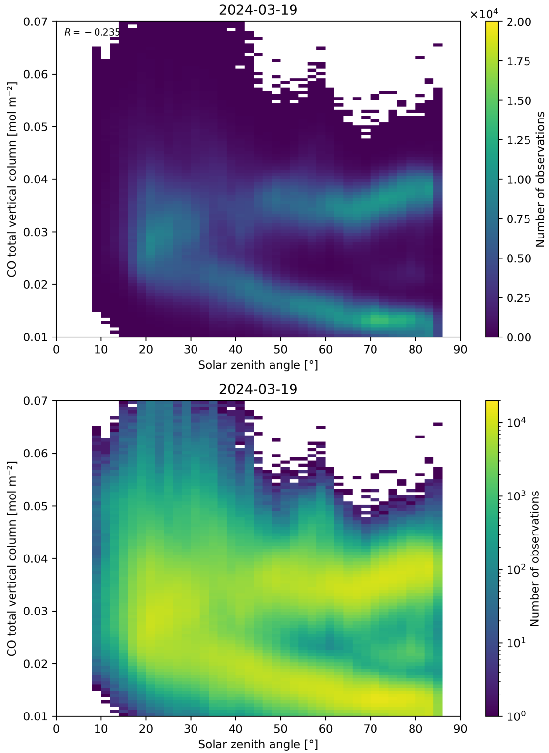
Figure 61: Scatter density plot of “Solar zenith angle” against “CO total vertical column” for 2024-03-18 to 2024-03-20.
