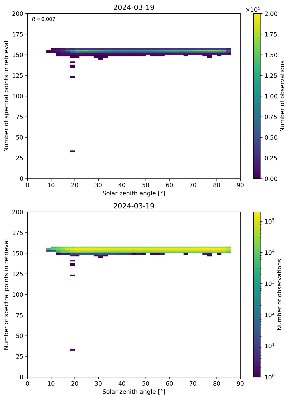
Figure 68: Scatter density plot of “Solar zenith angle” against “Number of spectral points in retrieval” for 2024-03-18 to 2024-03-20.
