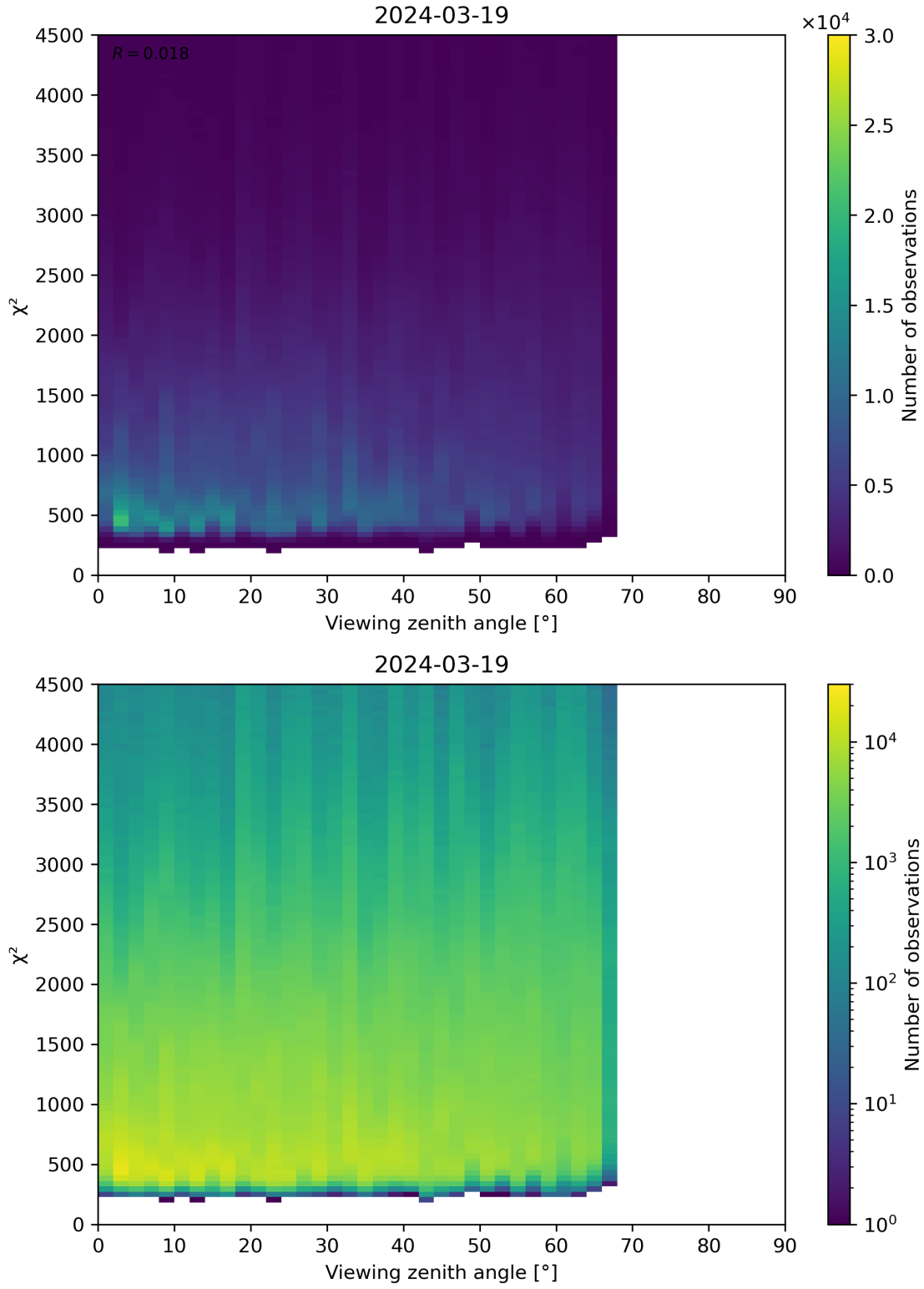
Figure 72: Scatter density plot of “Viewing zenith angle” against “ \chi^2 ” for 2024-03-18 to 2024-03-20.
