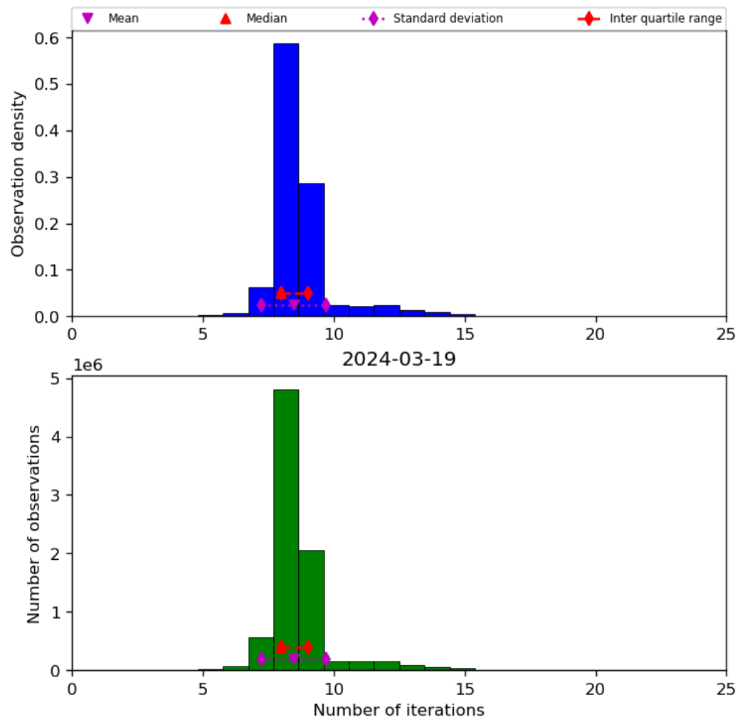
Figure 24: Histogram of “Number of iterations” for 2024-03-18 to 2024-03-20
