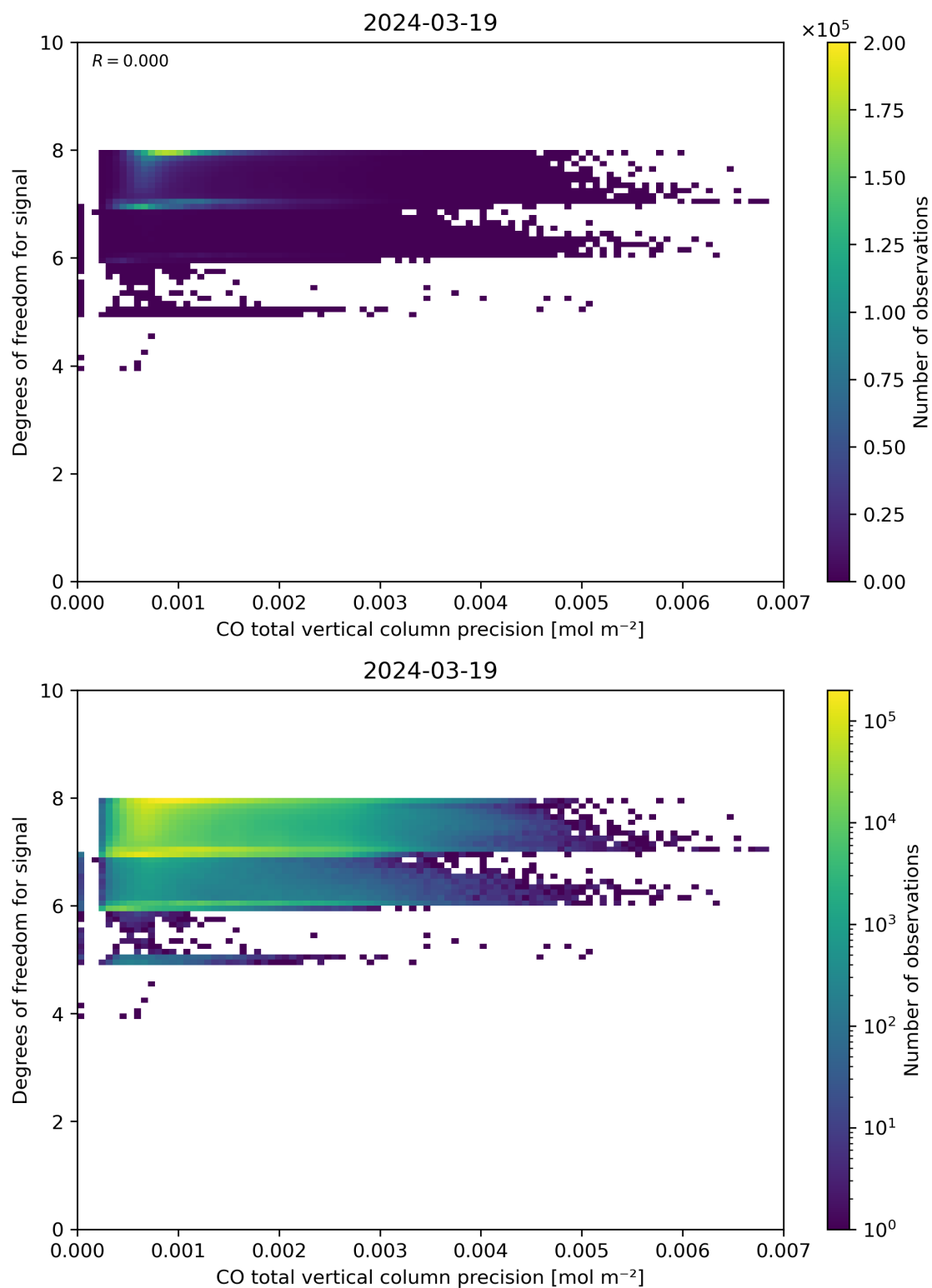
Figure 45: Scatter density plot of “CO total vertical column precision” against “Degrees of freedom for signal” for 2024-03-18 to 2024-03-20.
