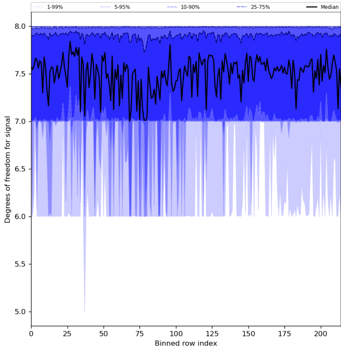
Figure 31: Along track statistics of “Degrees of freedom for signal” for 2024-03-18 to 2024-03-20
