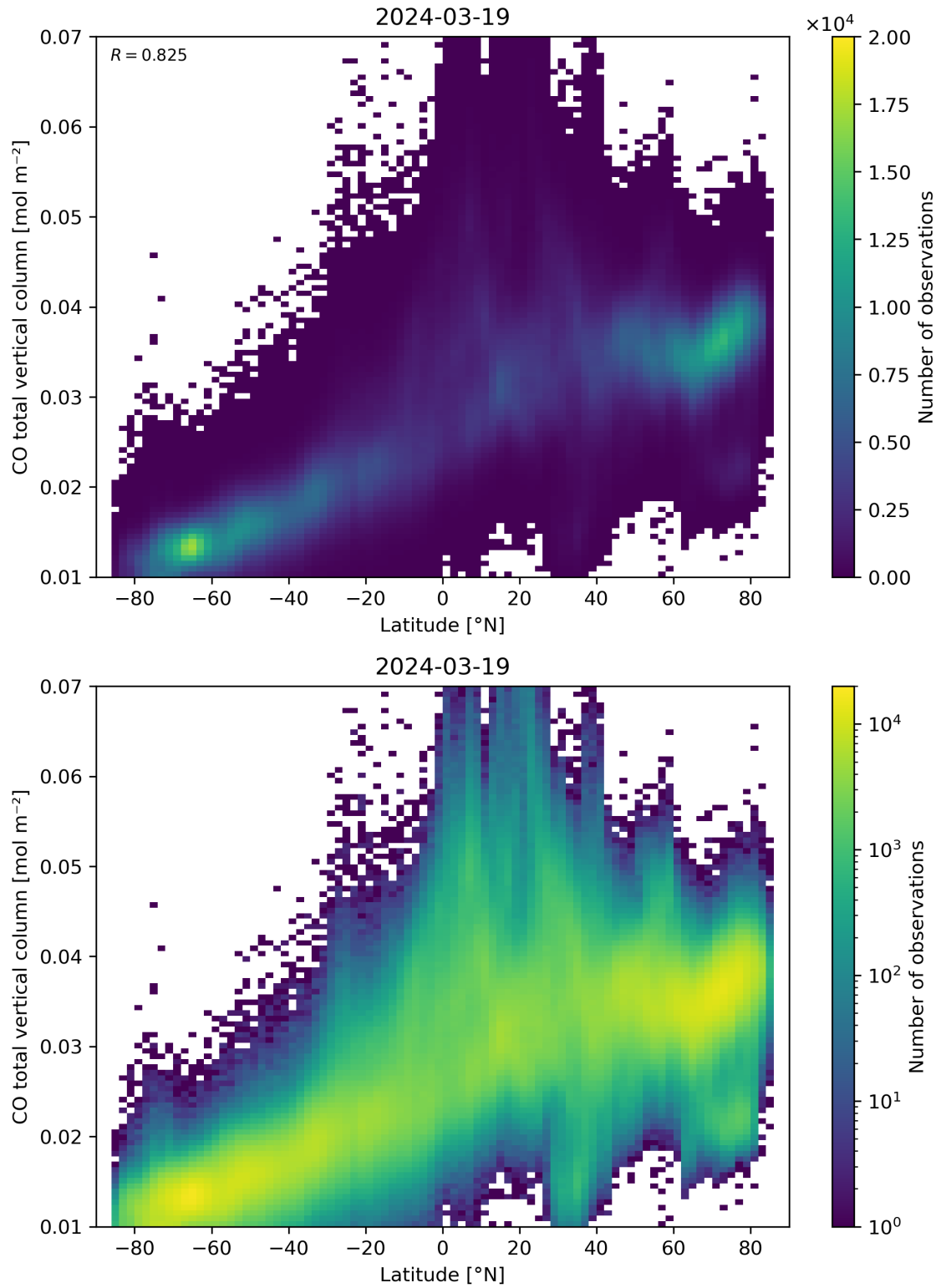
Figure 51: Scatter density plot of “Latitude” against “CO total vertical column” for 2024-03-18 to 2024-03-20.
