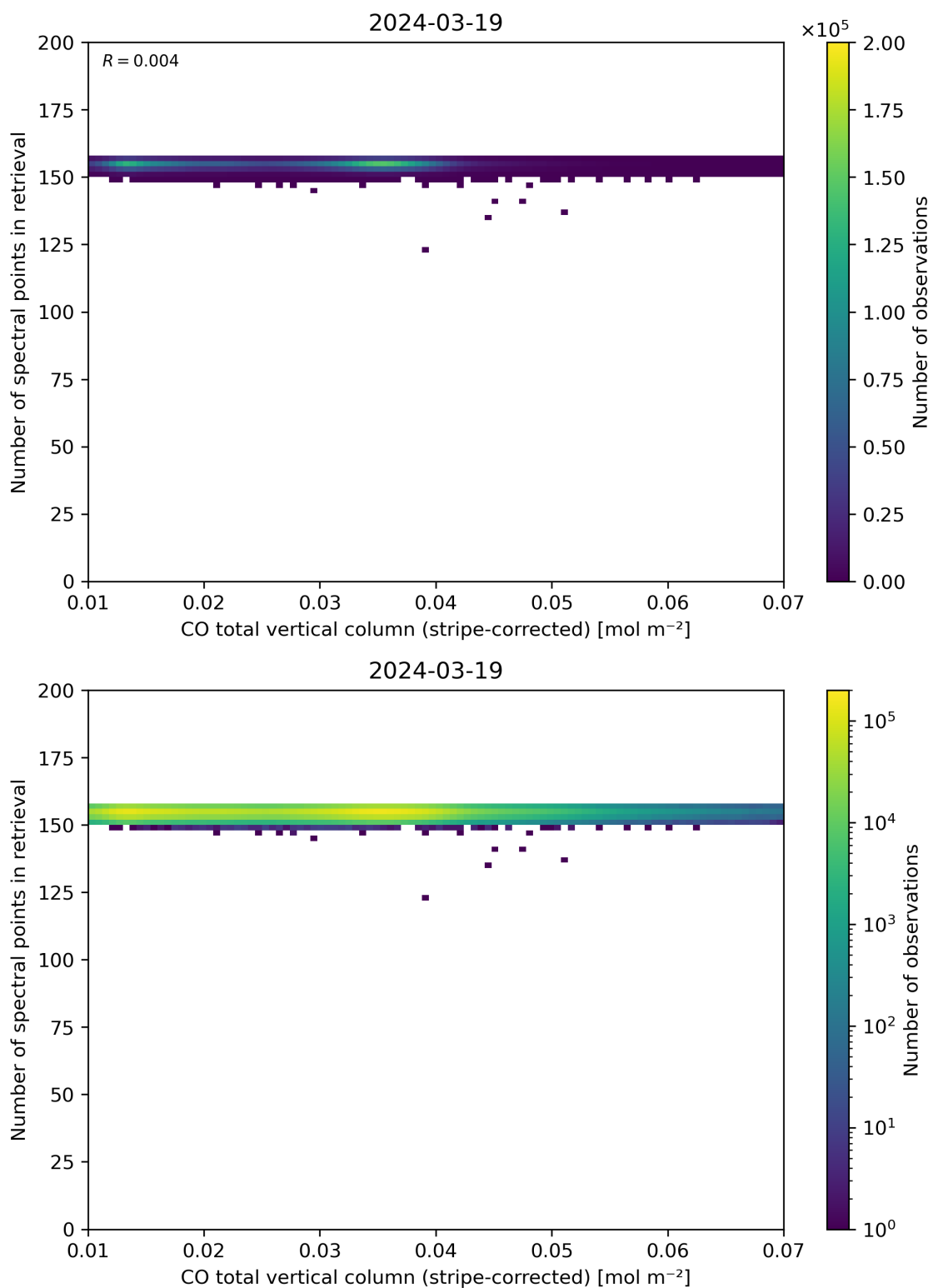
Figure 40: Scatter density plot of “CO total vertical column (stripe-corrected)” against “Number of spectral points in retrieval” for 2024-03-18 to 2024-03-20.
