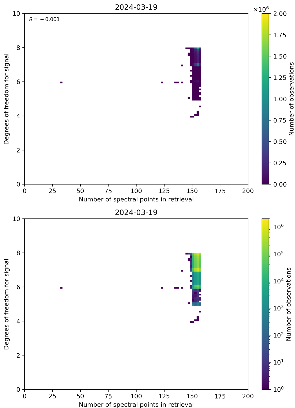
Figure 59: Scatter density plot of “Number of spectral points in retrieval” against “Degrees of freedom for signal” for 2024-03-18 to 2024-03-20.
