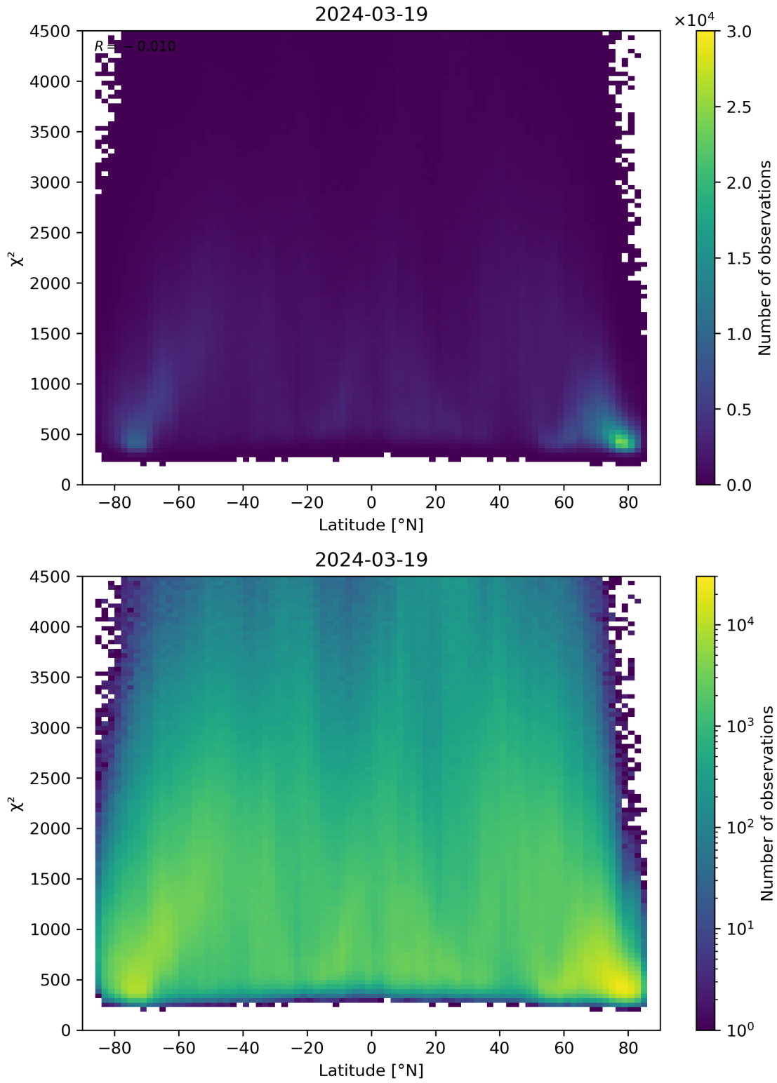
Figure 54: Scatter density plot of “Latitude” against “ \chi^2 ” for 2024-03-18 to 2024-03-20.
