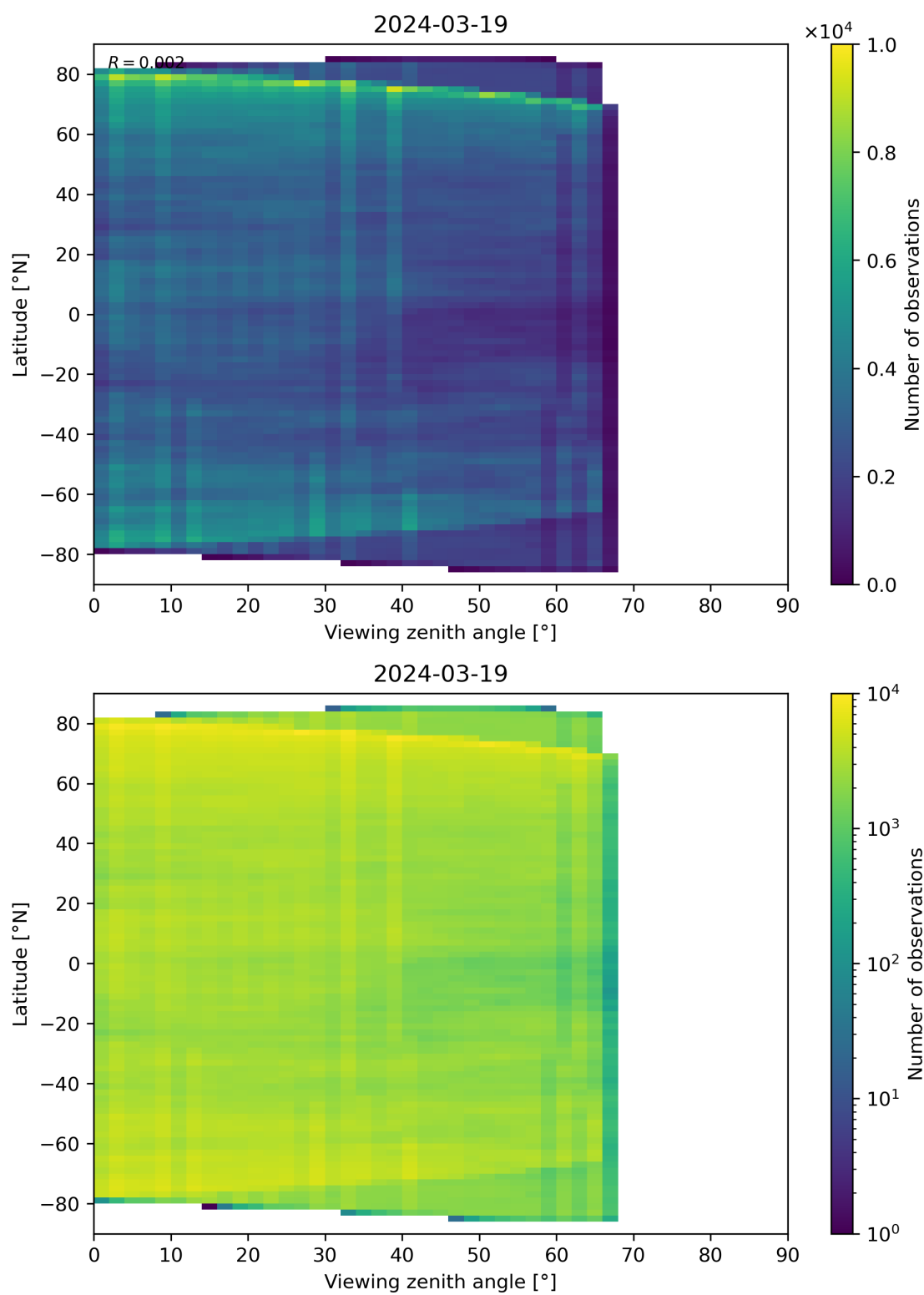
Figure 74: Scatter density plot of “Viewing zenith angle” against “Latitude” for 2024-03-18 to 2024-03-20.
