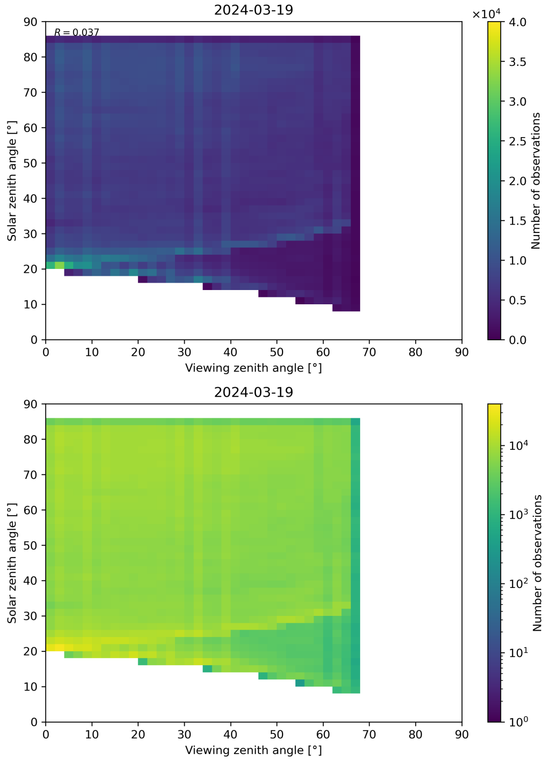
Figure 77: Scatter density plot of “Viewing zenith angle” against “Solar zenith angle” for 2024-03-18 to 2024-03-20.
