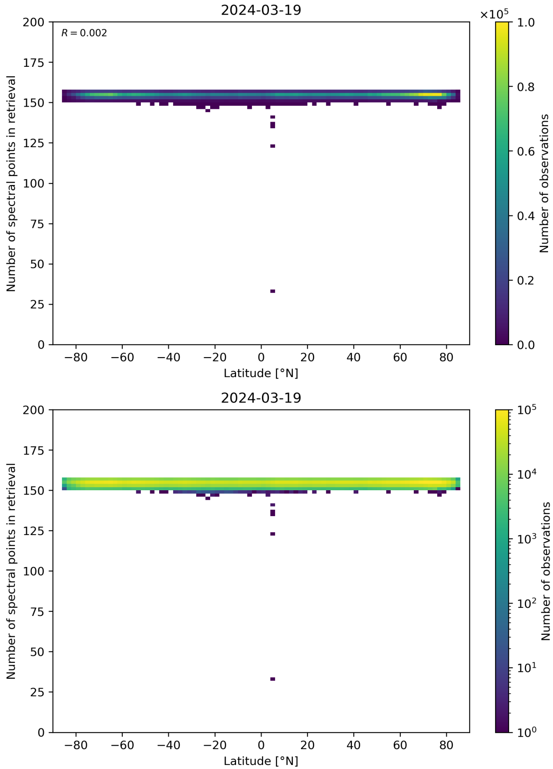
Figure 57: Scatter density plot of “Latitude” against “Number of spectral points in retrieval” for 2024-03-18 to 2024-03-20.
