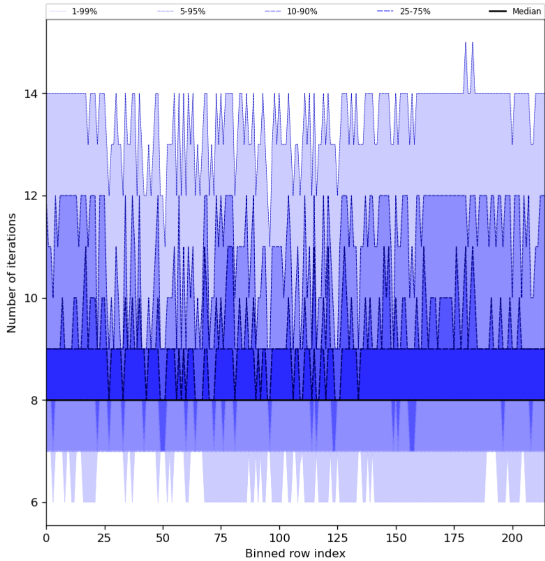
Figure 32: Along track statistics of “Number of iterations” for 2024-03-18 to 2024-03-20
