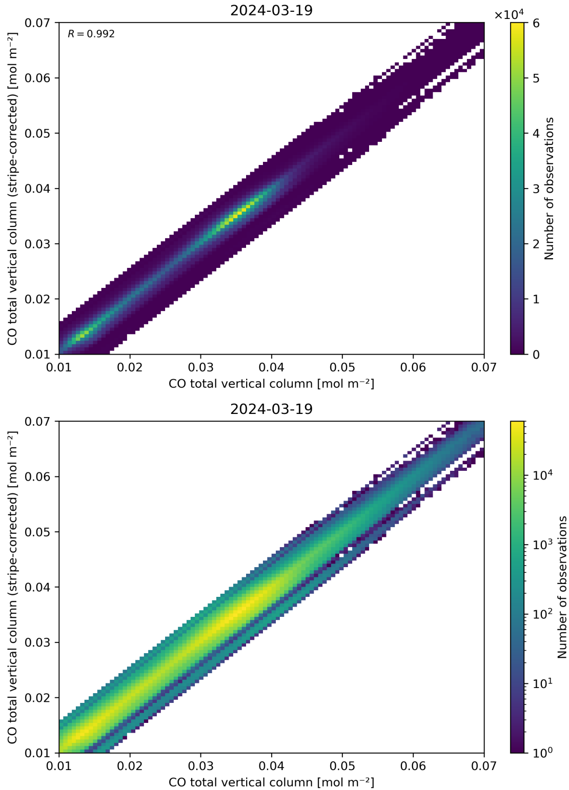
Figure 33: Scatter density plot of “CO total vertical column” against “CO total vertical column (stripe-corrected)” for 2024-03-18 to 2024-03-20.
