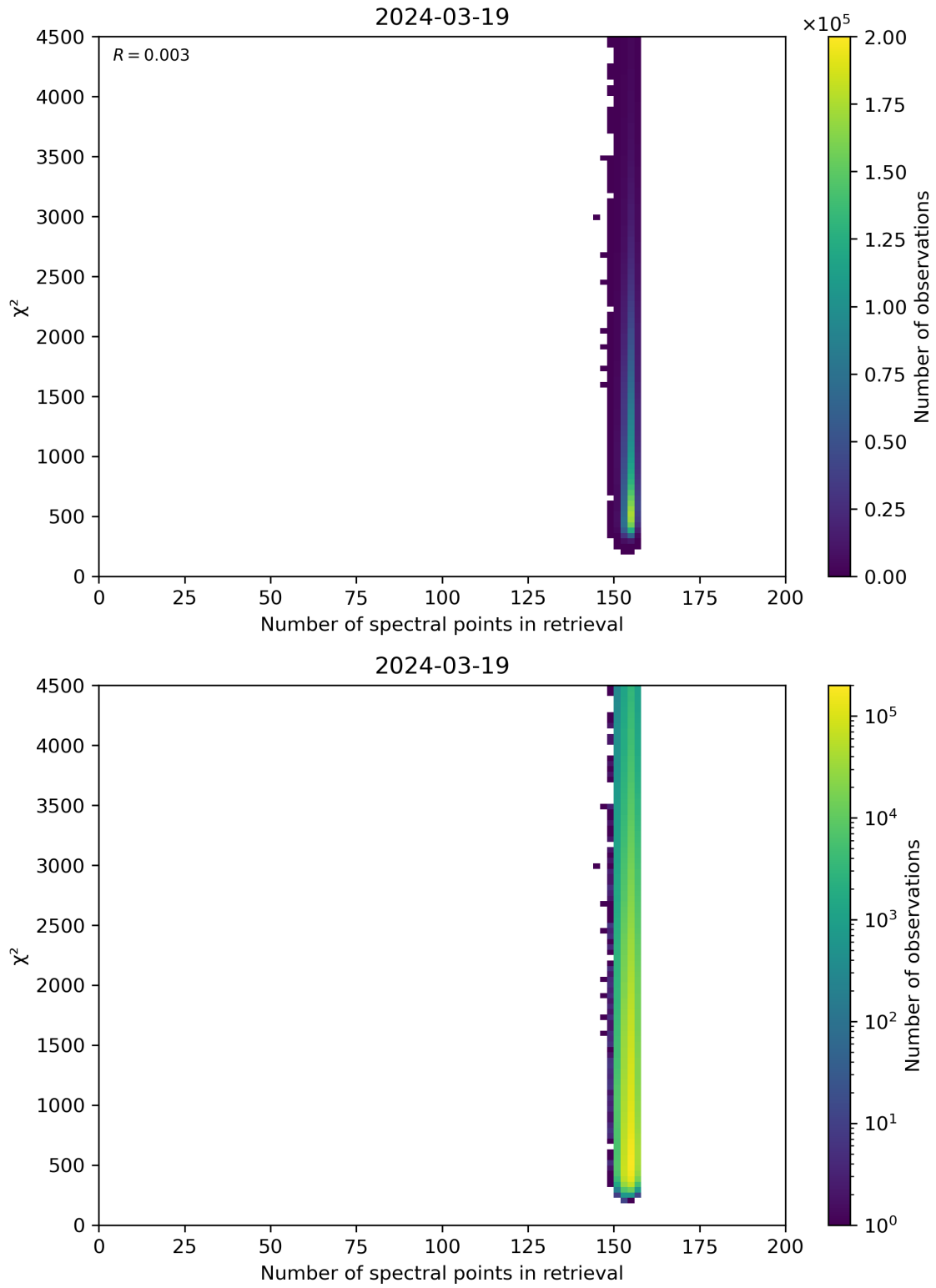
Figure 58: Scatter density plot of “Number of spectral points in retrieval” against “ \chi^2 ” for 2024-03-18 to 2024-03-20.
