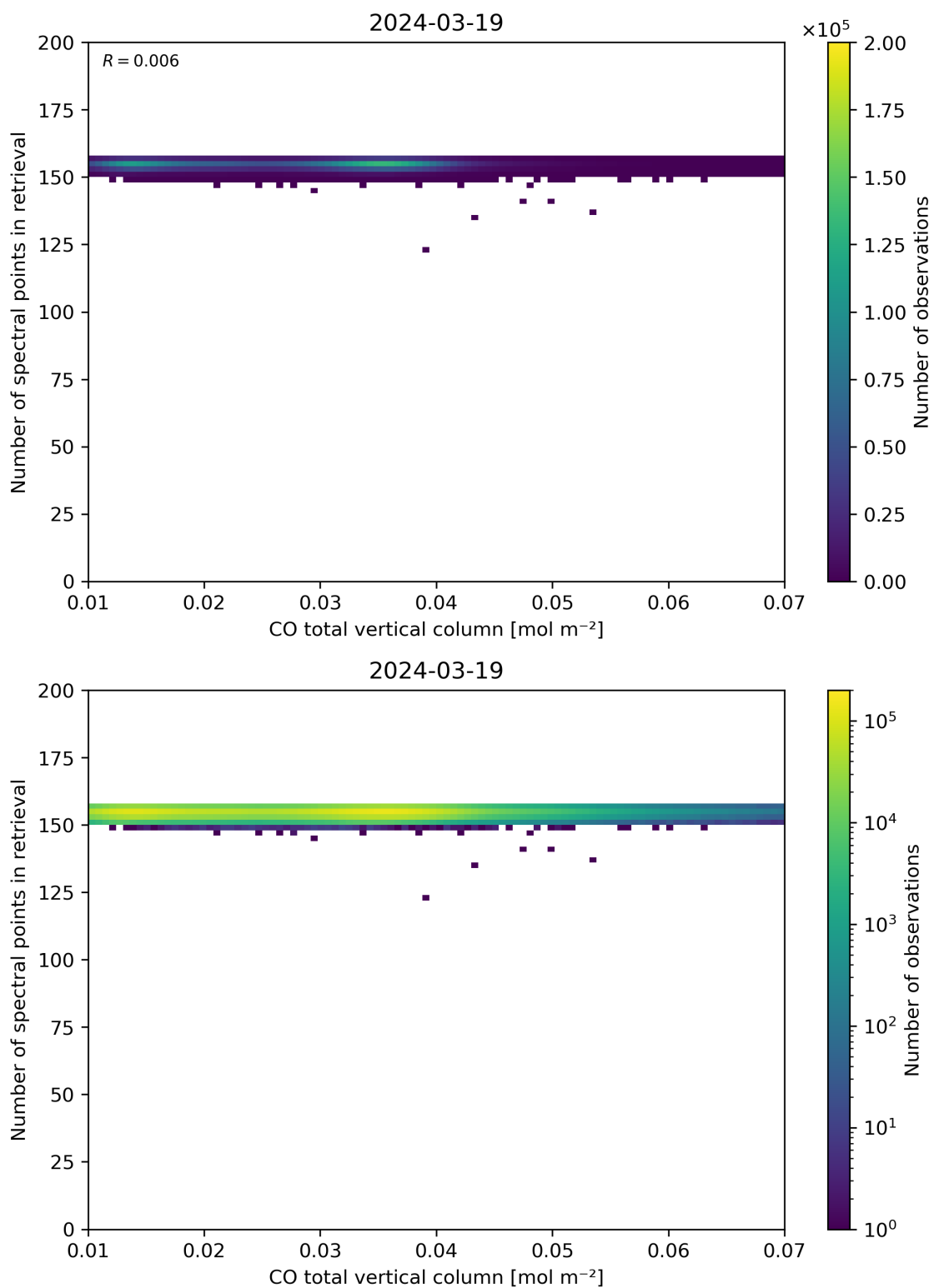
Figure 43: Scatter density plot of “CO total vertical column” against “Number of spectral points in retrieval” for 2024-03-18 to 2024-03-20.
