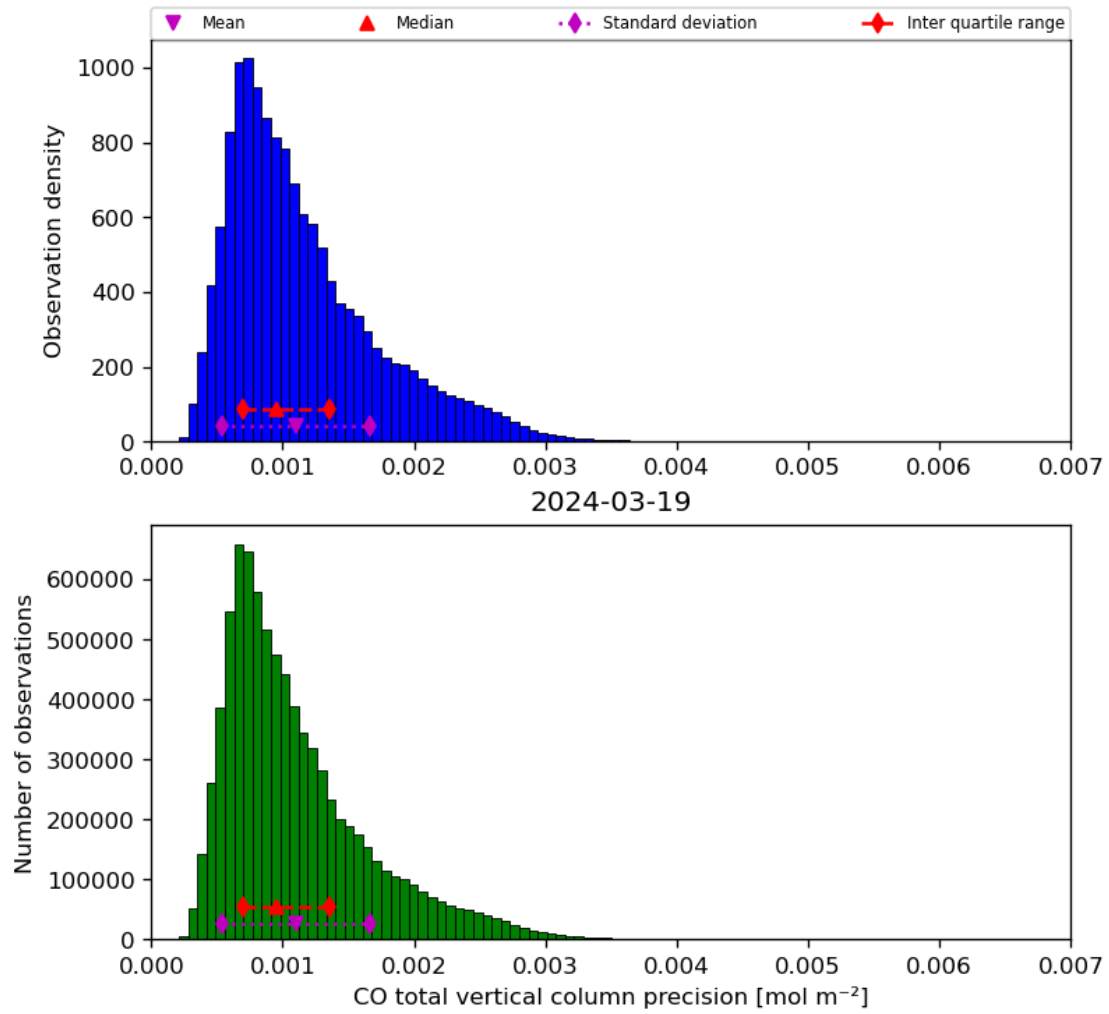
Figure 20: Histogram of “CO total vertical column precision” for 2024-03-18 to 2024-03-20
