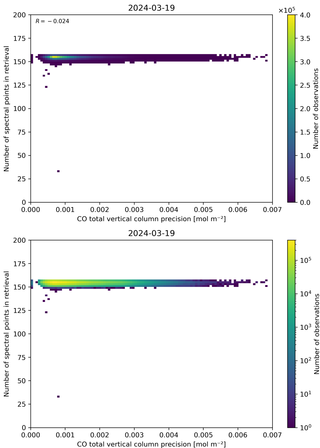
Figure 47: Scatter density plot of “CO total vertical column precision” against “Number of spectral points in retrieval” for 2024-03-18 to 2024-03-20.
