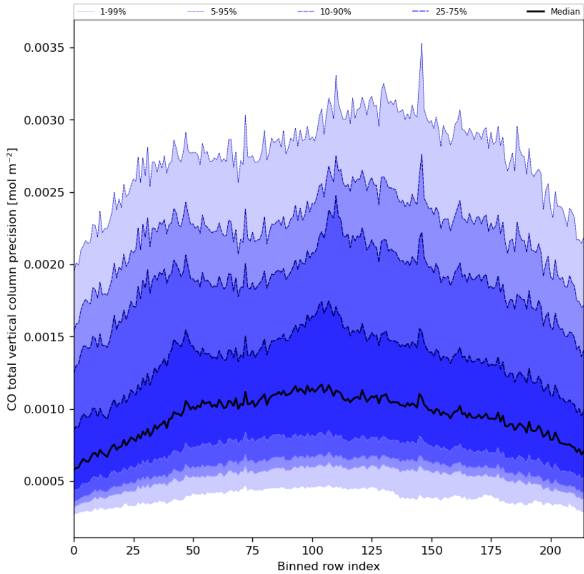
Figure 28: Along track statistics of “CO total vertical column precision” for 2024-03-18 to 2024-03-20
