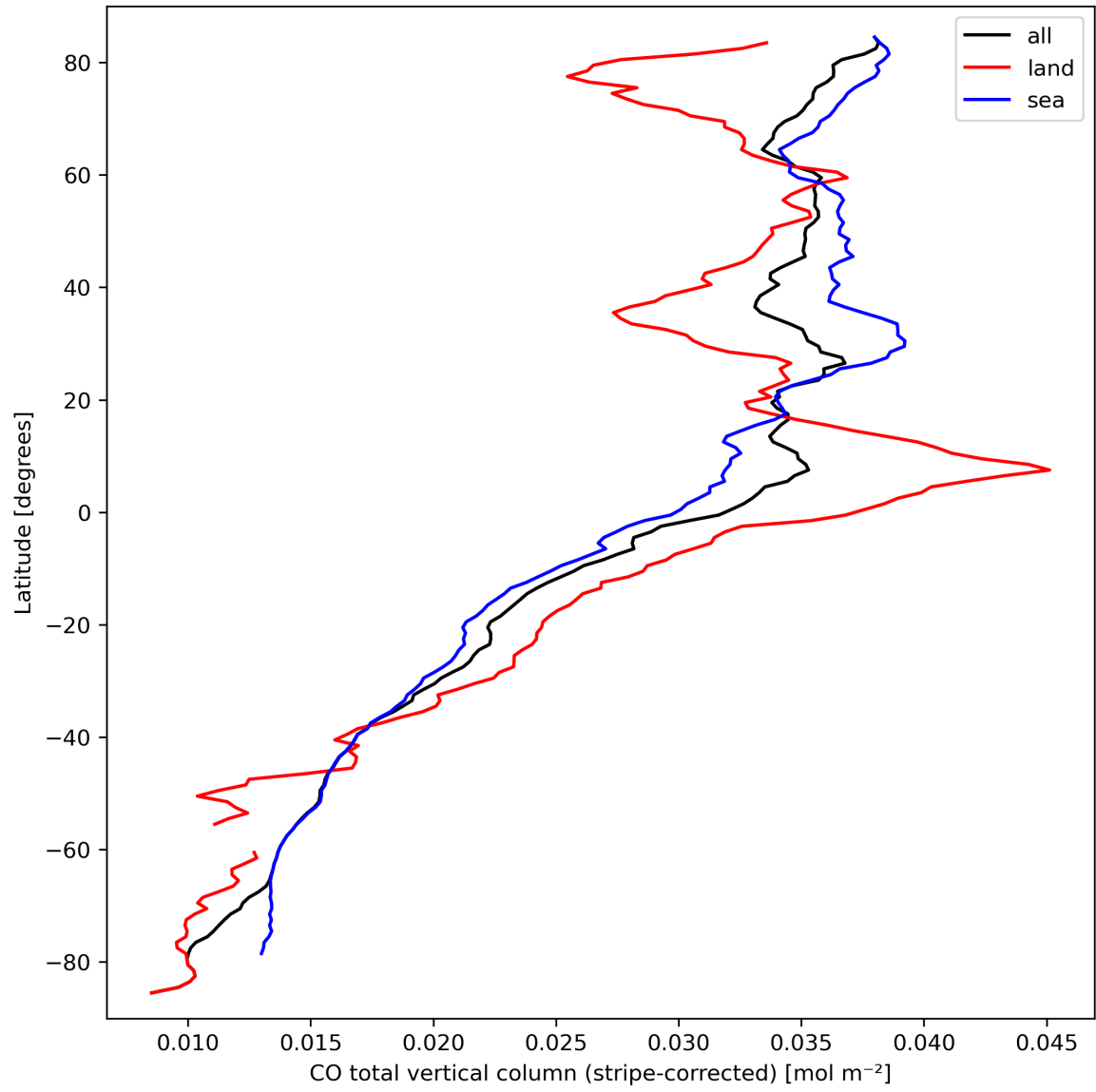
Figure 11: Zonal average of “CO total vertical column (stripe-corrected)” for 2024-03-18 to 2024-03-20.
