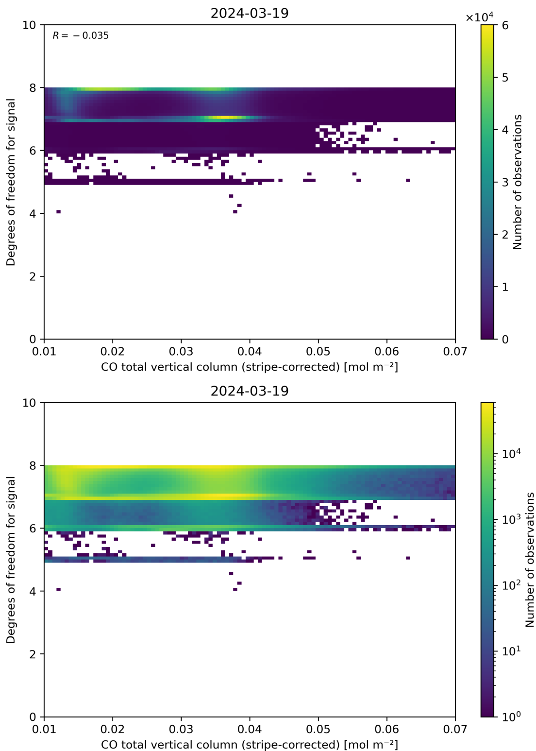
Figure 38: Scatter density plot of “CO total vertical column (stripe-corrected)” against “Degrees of freedom for signal” for 2024-03-18 to 2024-03-20.
