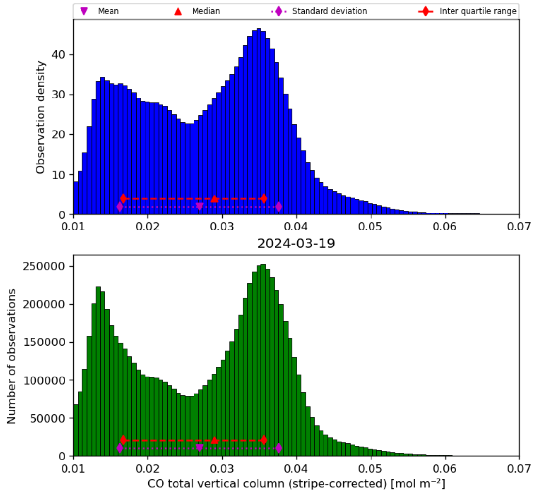
Figure 19: Histogram of “CO total vertical column (stripe-corrected)” for 2024-03-18 to 2024-03-20
