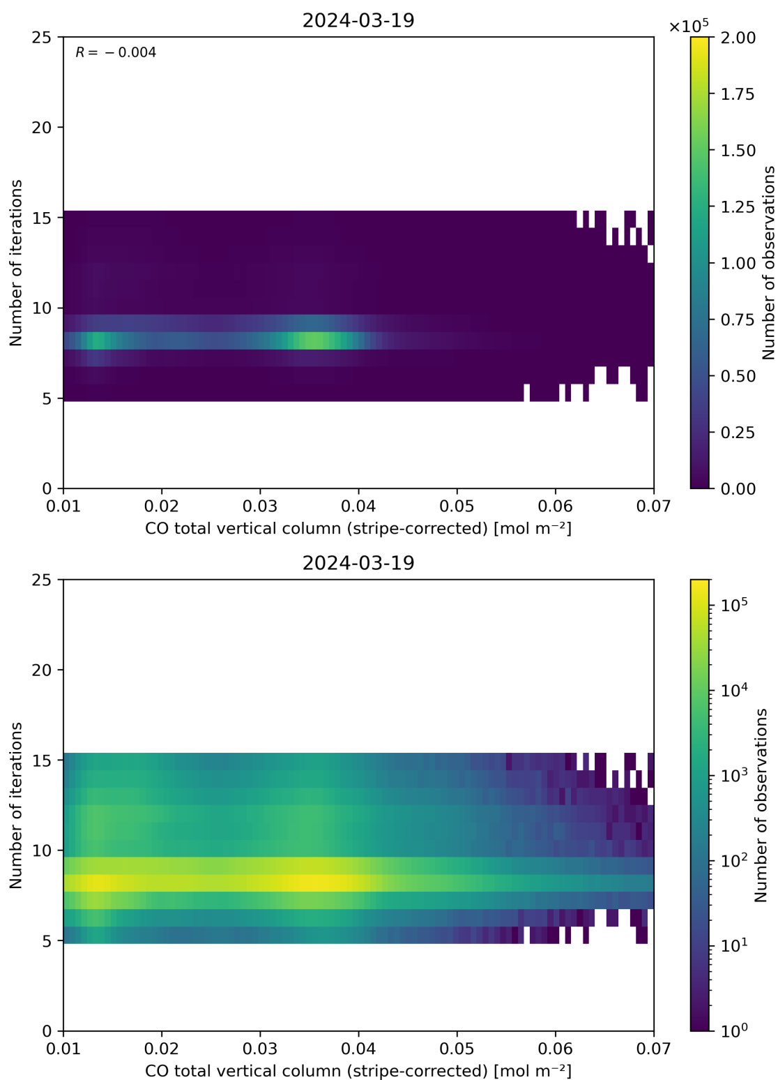
Figure 39: Scatter density plot of “CO total vertical column (stripe-corrected)” against “Number of iterations” for 2024-03-18 to 2024-03-20.
