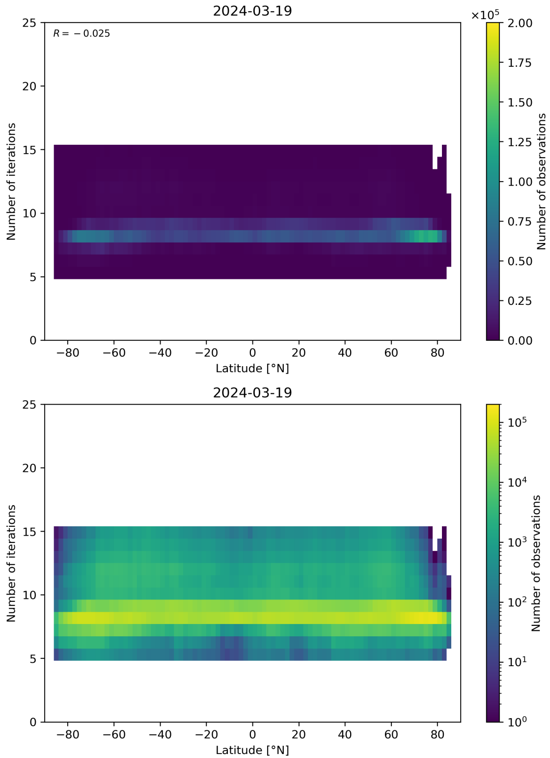
Figure 56: Scatter density plot of “Latitude” against “Number of iterations” for 2024-03-18 to 2024-03-20.
