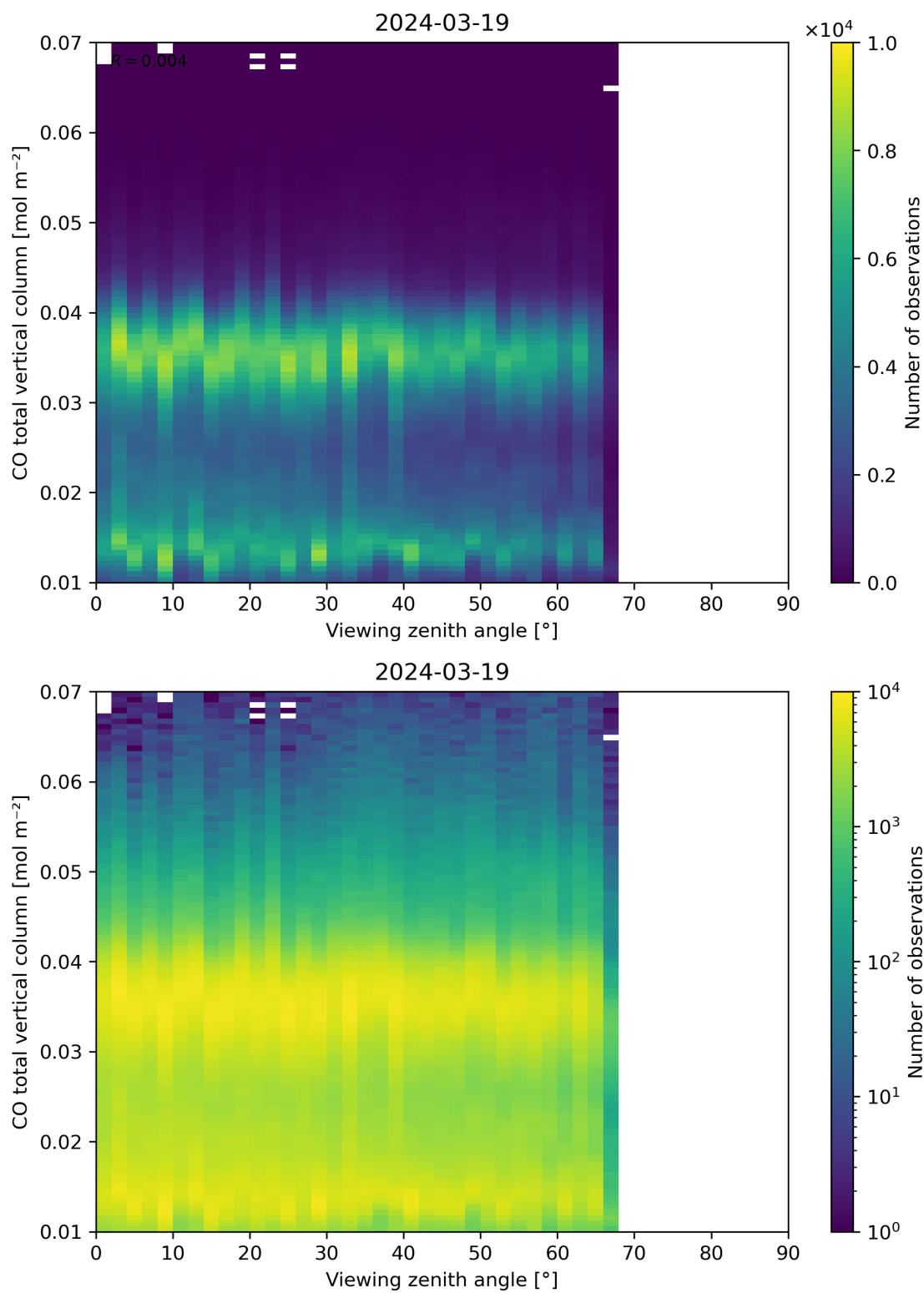
Figure 69: Scatter density plot of “Viewing zenith angle” against “CO total vertical column” for 2024-03-18 to 2024-03-20.
