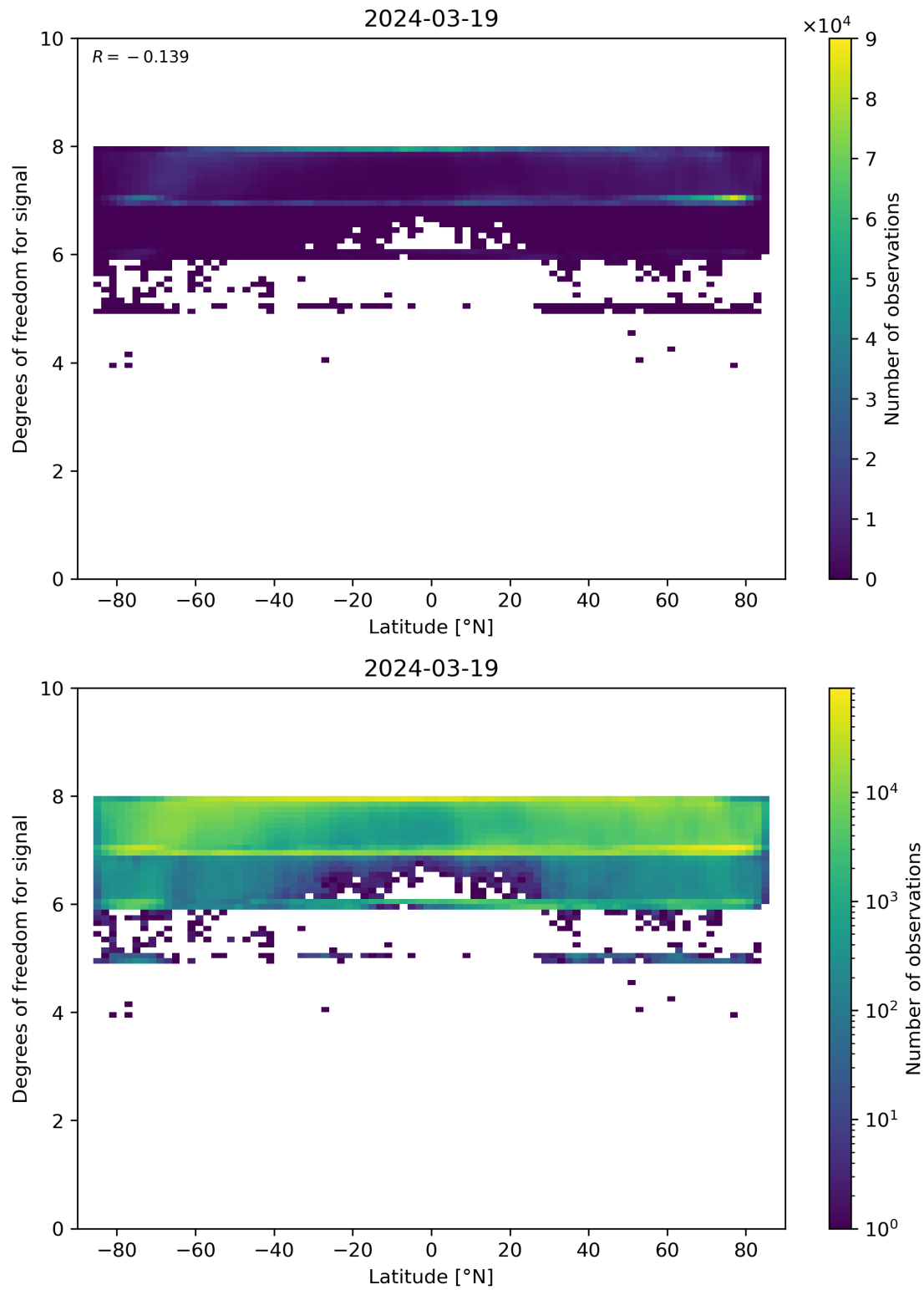
Figure 55: Scatter density plot of “Latitude” against “Degrees of freedom for signal” for 2024-03-18 to 2024-03-20.
