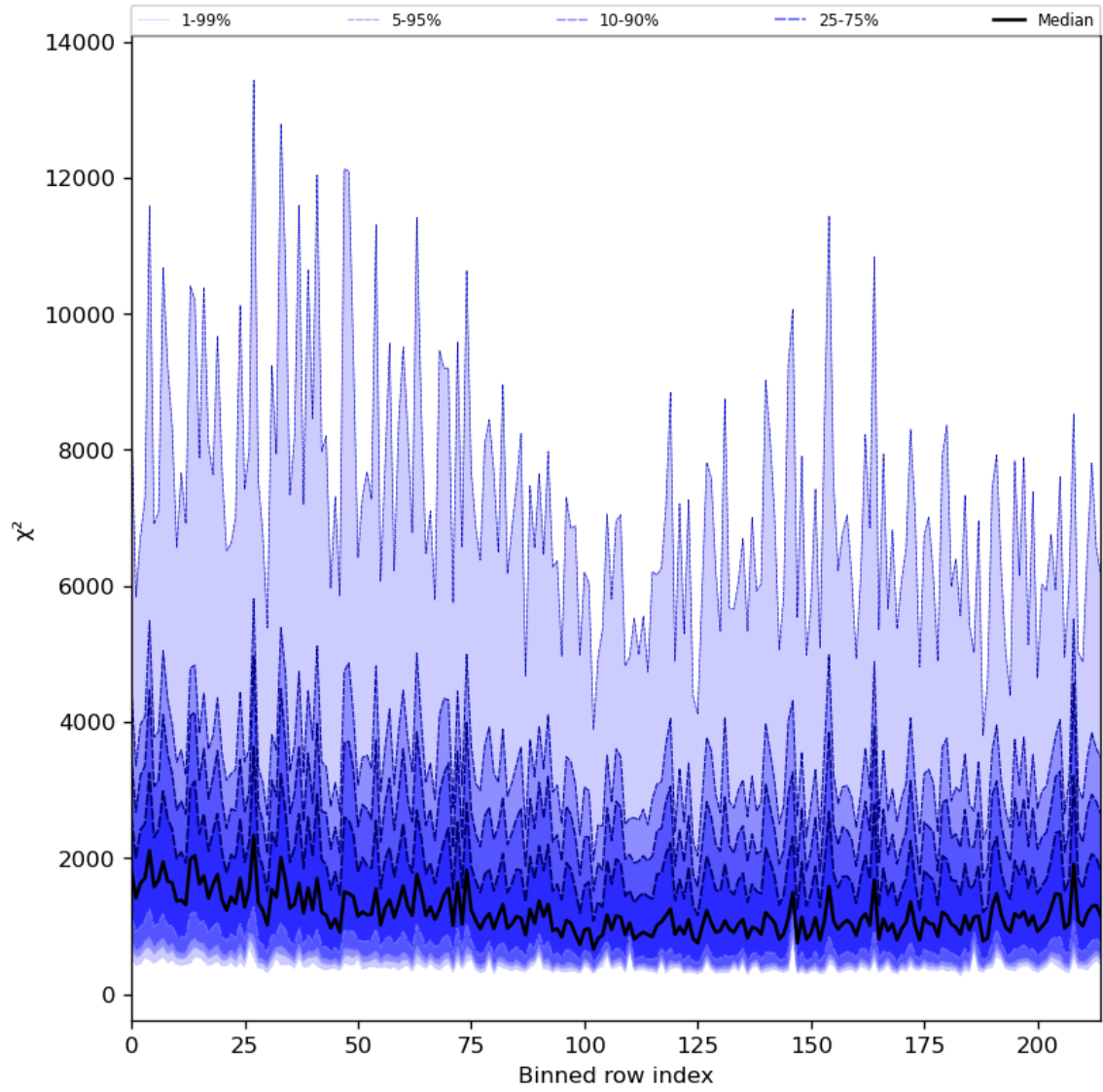
Figure 30: Along track statistics of “ \chi^2 ” for 2024-03-18 to 2024-03-20
