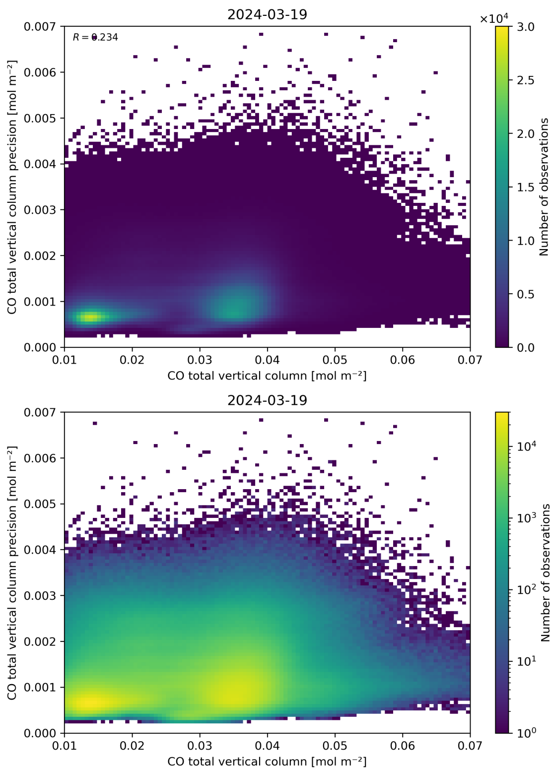
Figure 34: Scatter density plot of “CO total vertical column” against “CO total vertical column precision” for 2024-03-18 to 2024-03-20.
