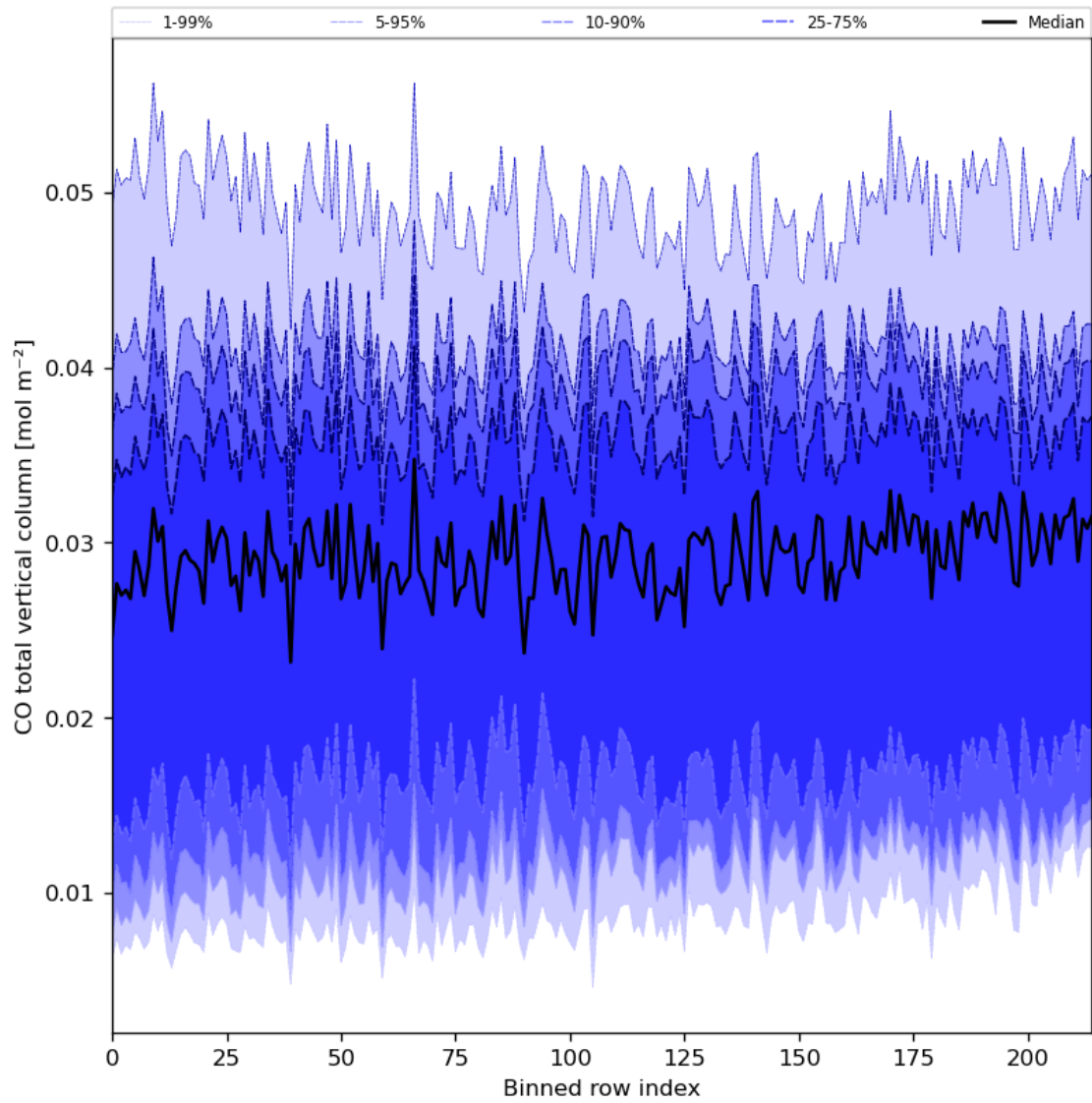
Figure 26: Along track statistics of “CO total vertical column” for 2024-03-18 to 2024-03-20
