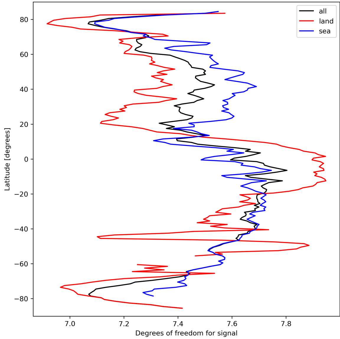
Figure 15: Zonal average of “Degrees of freedom for signal” for 2024-03-18 to 2024-03-20.
