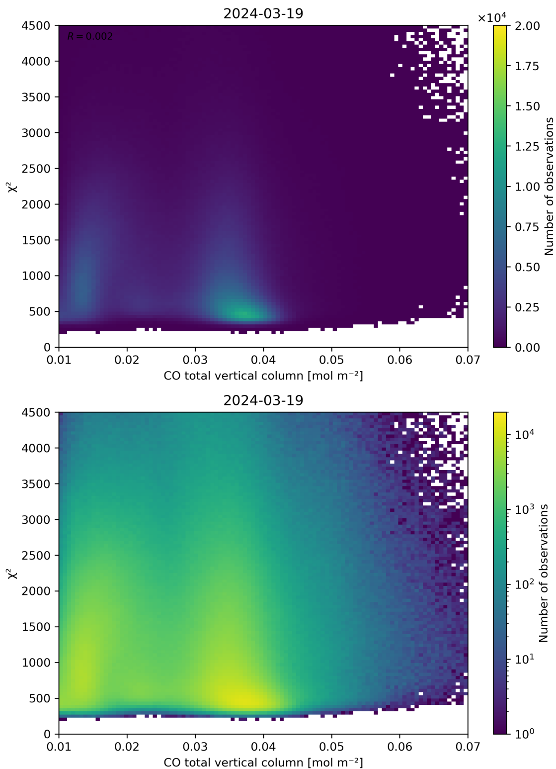
Figure 35: Scatter density plot of “CO total vertical column” against “ \chi^2 ” for 2024-03-18 to 2024-03-20.
