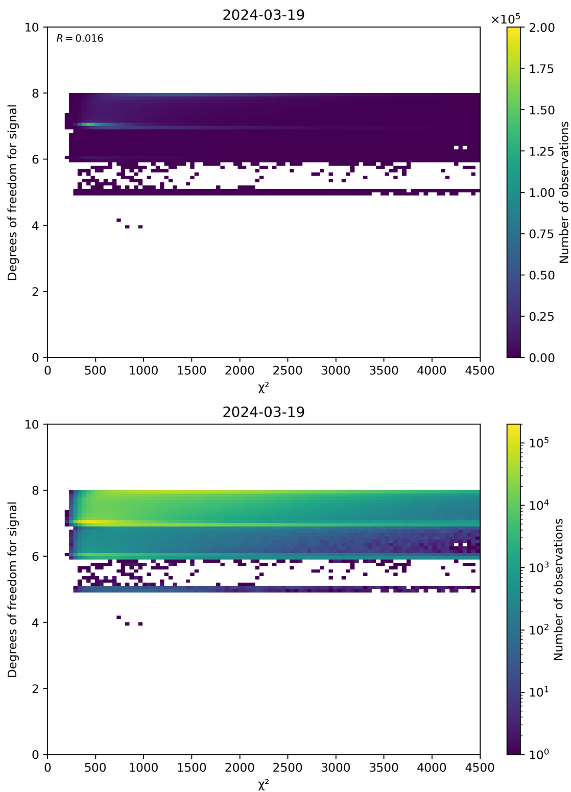
Figure 48: Scatter density plot of “ \chi^2 ” against “Degrees of freedom for signal” for 2024-03-18 to 2024-03-20.
