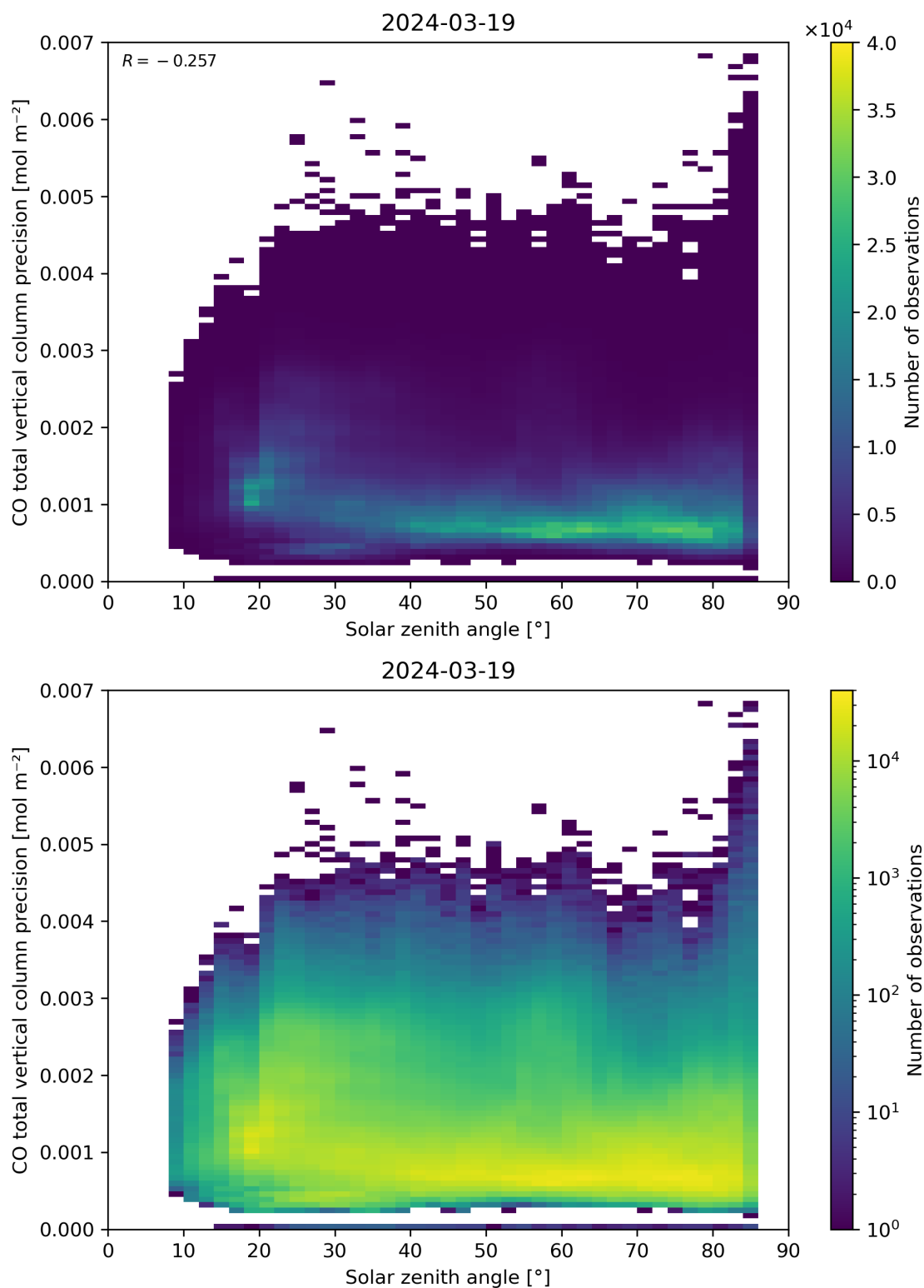
Figure 63: Scatter density plot of “Solar zenith angle” against “CO total vertical column precision” for 2024-03-18 to 2024-03-20.
