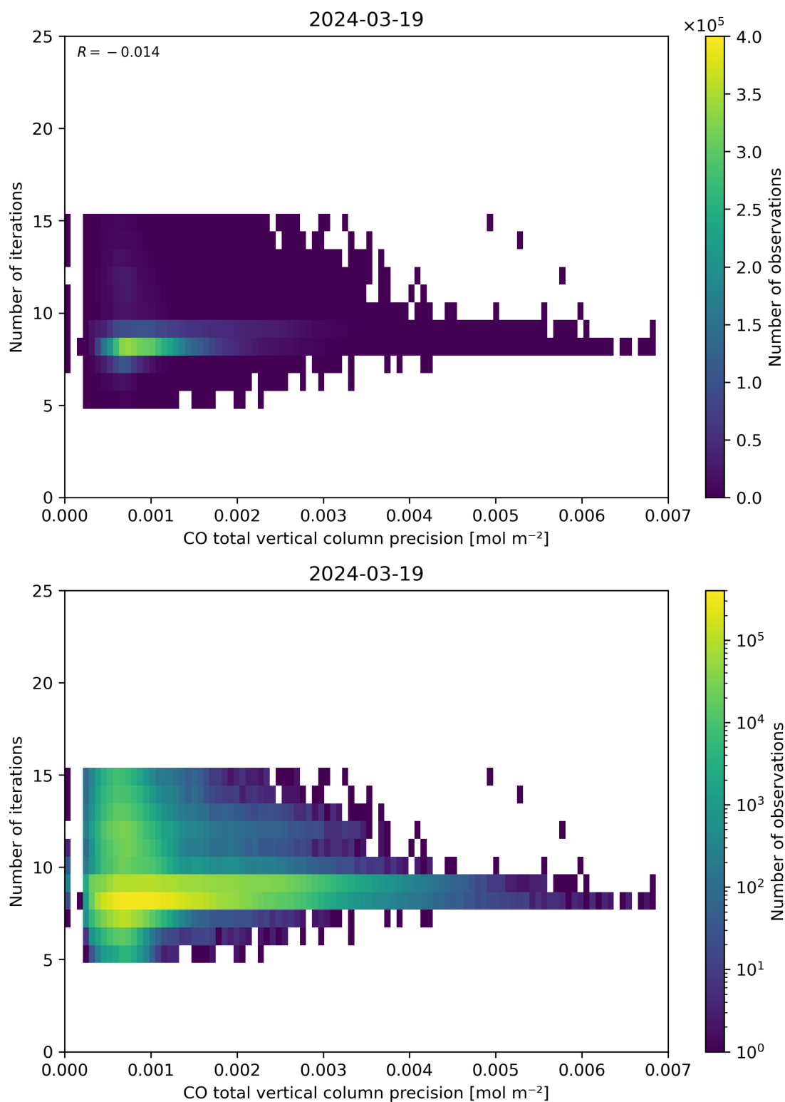
Figure 46: Scatter density plot of “CO total vertical column precision” against “Number of iterations” for 2024-03-18 to 2024-03-20.
