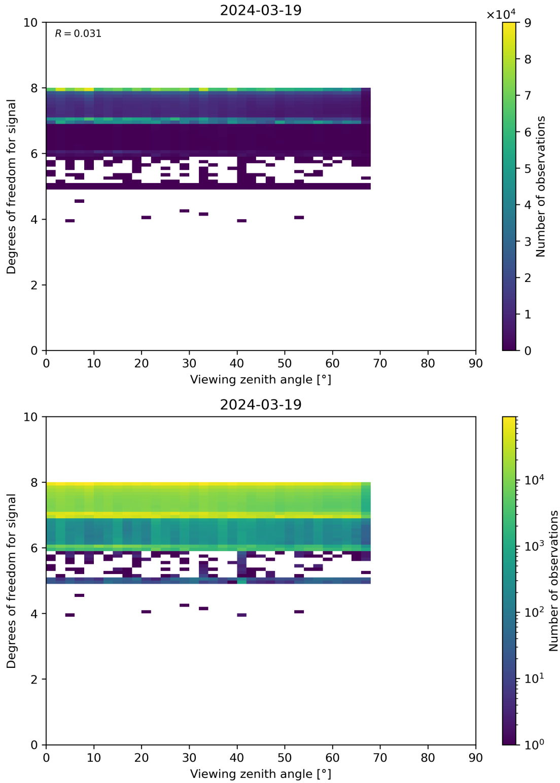
Figure 73: Scatter density plot of “Viewing zenith angle” against “Degrees of freedom for signal” for 2024-03-18 to 2024-03-20.
