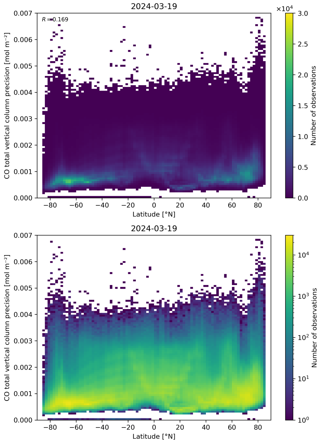
Figure 53: Scatter density plot of “Latitude” against “CO total vertical column precision” for 2024-03-18 to 2024-03-20.
