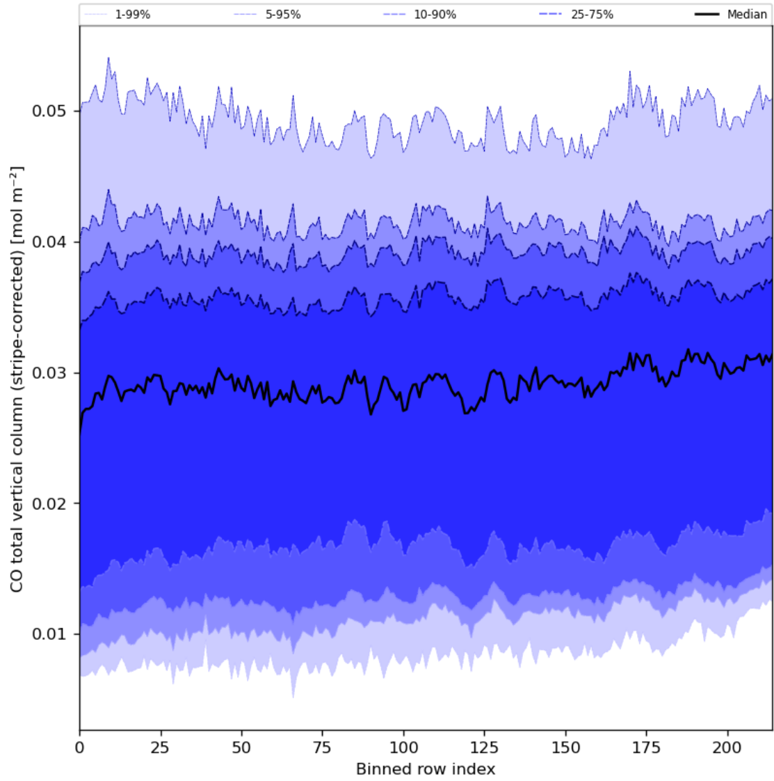
Figure 27: Along track statistics of "CO total vertical column (stripe-corrected)" for 2024-03-18 to 2024-03-20
