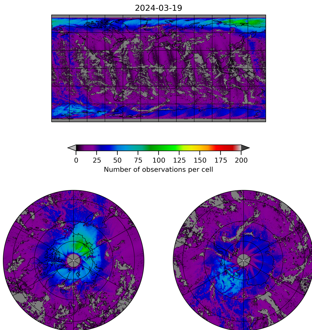
Figure 8: Map of the number of observations for 2024-03-18 to 2024-03-20
