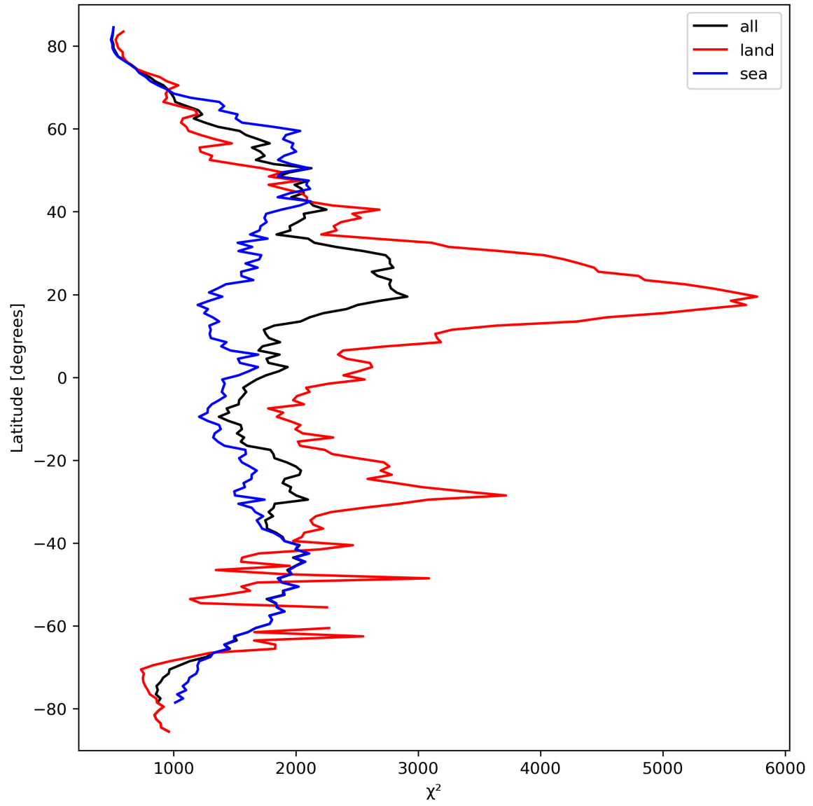
Figure 14: Zonal average of “ \chi^2 ” for 2024-03-18 to 2024-03-20.
