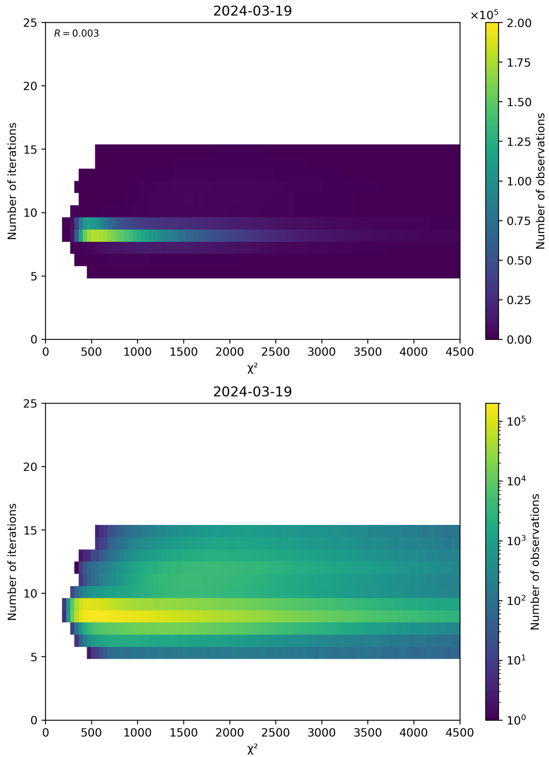
Figure 49: Scatter density plot of “ \chi^2 ” against “Number of iterations” for 2024-03-18 to 2024-03-20.
