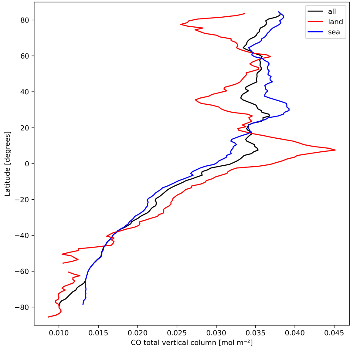
Figure 10: Zonal average of “CO total vertical column” for 2024-03-18 to 2024-03-20.
