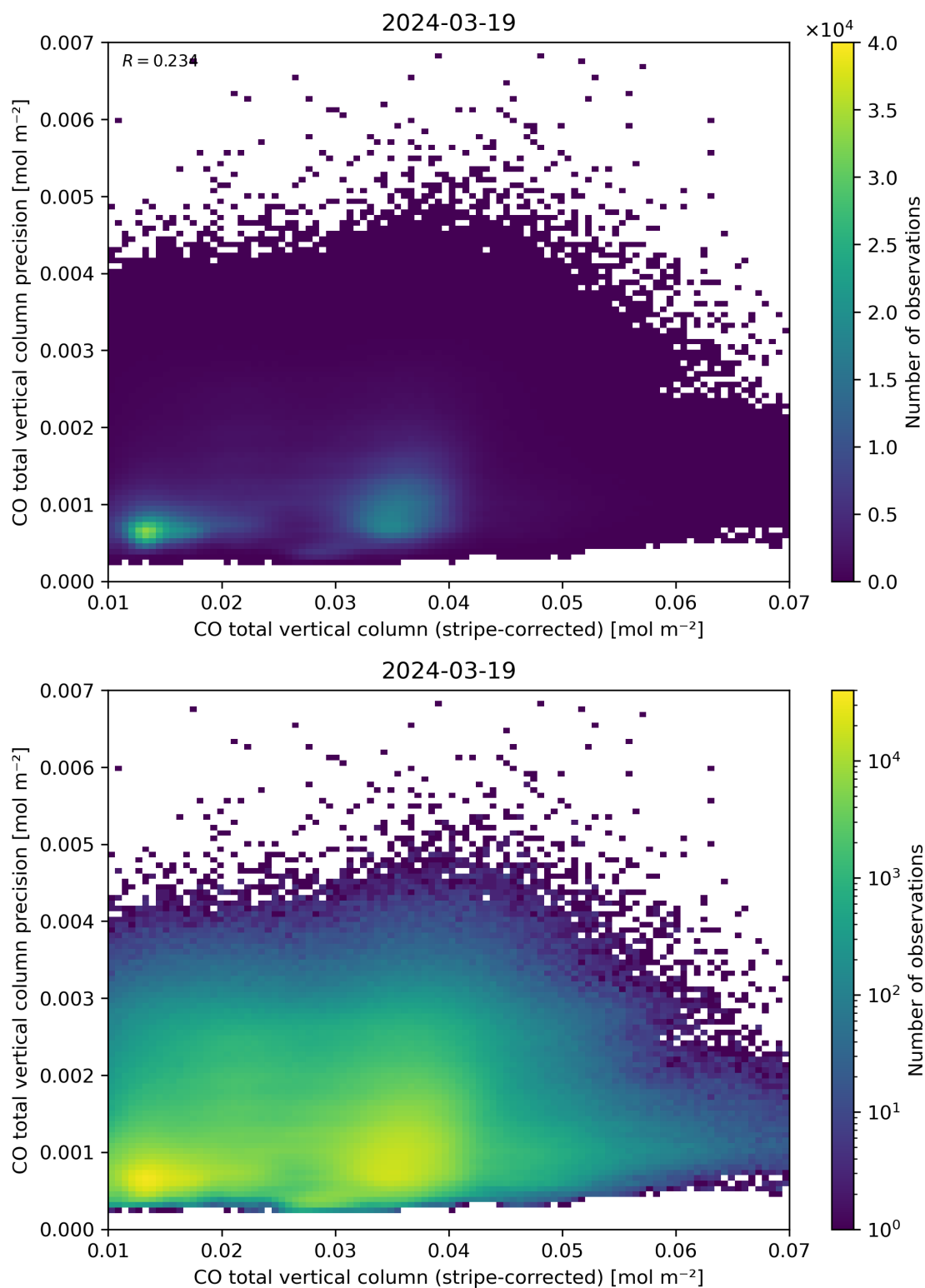
Figure 36: Scatter density plot of “CO total vertical column (stripe-corrected)” against “CO total vertical column precision” for 2024-03-18 to 2024-03-20.
