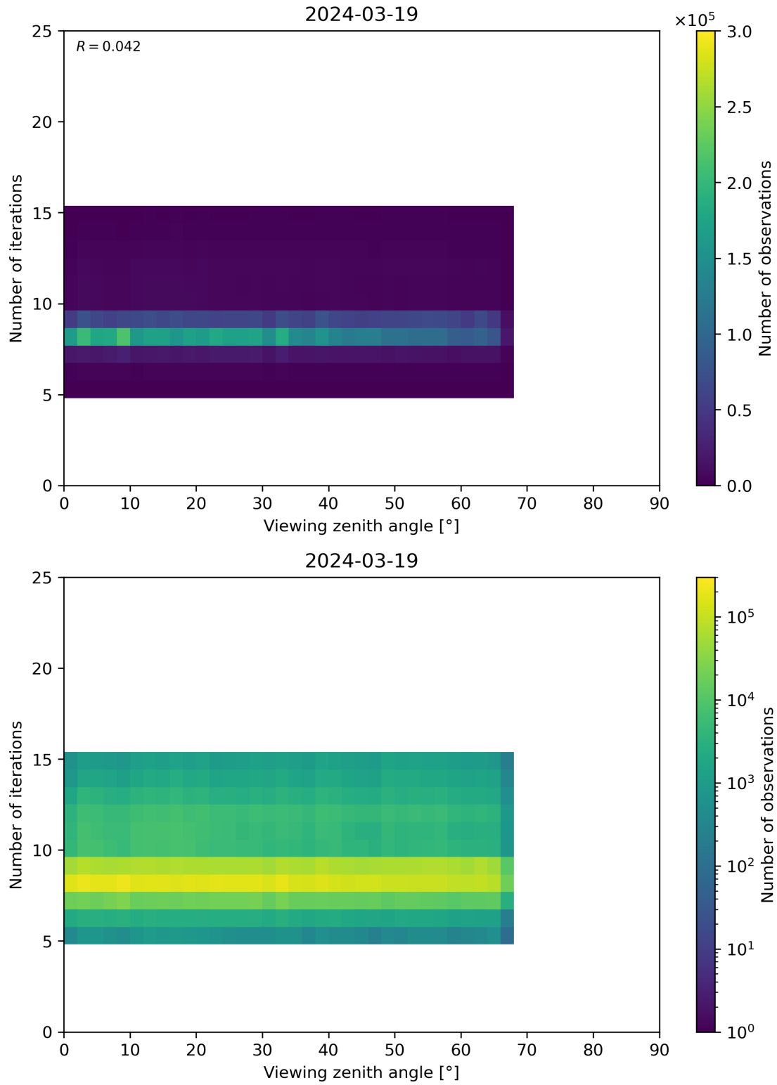
Figure 75: Scatter density plot of “Viewing zenith angle” against “Number of iterations” for 2024-03-18 to 2024-03-20.
