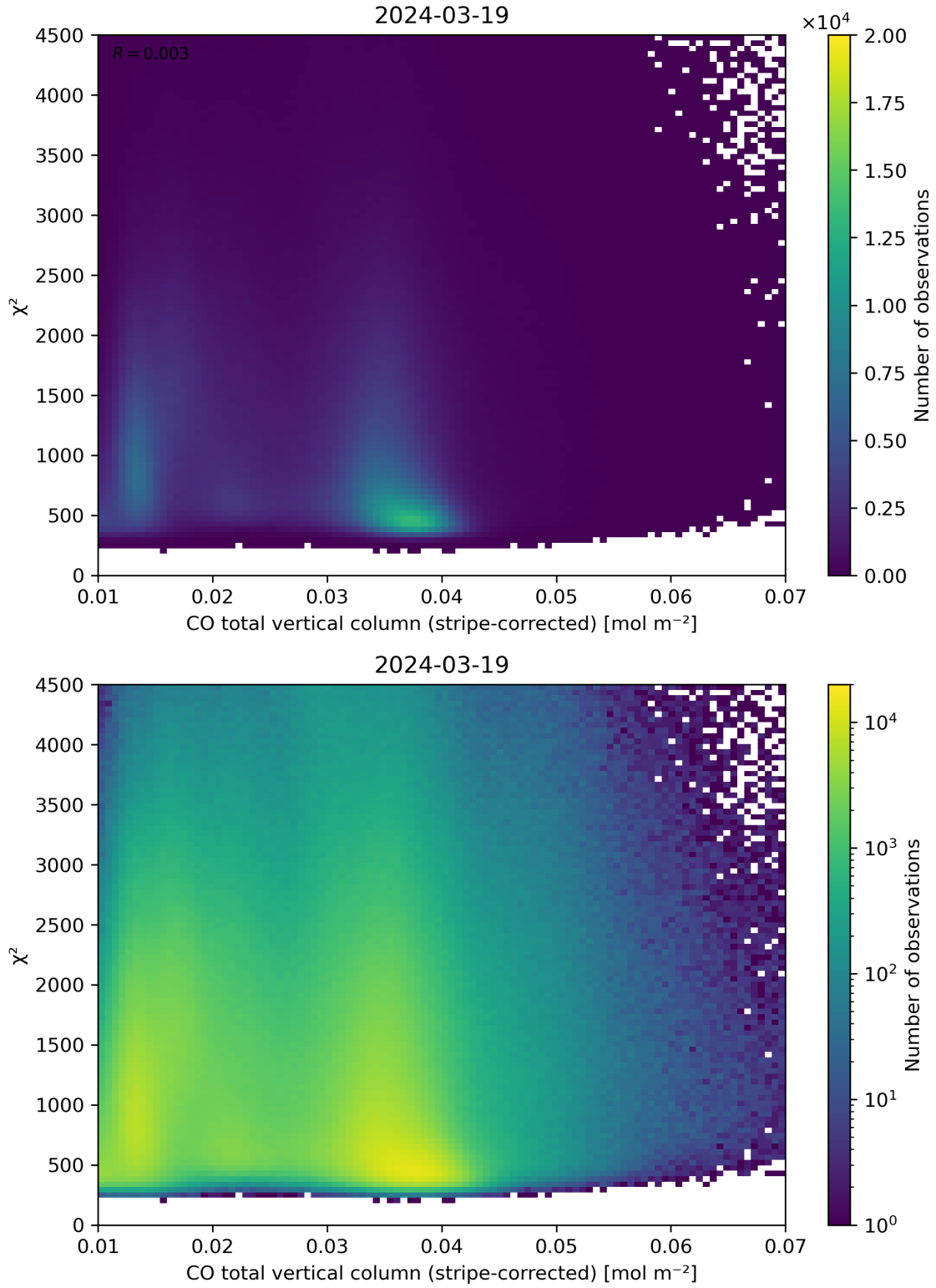
Figure 37: Scatter density plot of “CO total vertical column (stripe-corrected)” against “ \chi^2 ” for 2024-03-18 to 2024-03-20.
