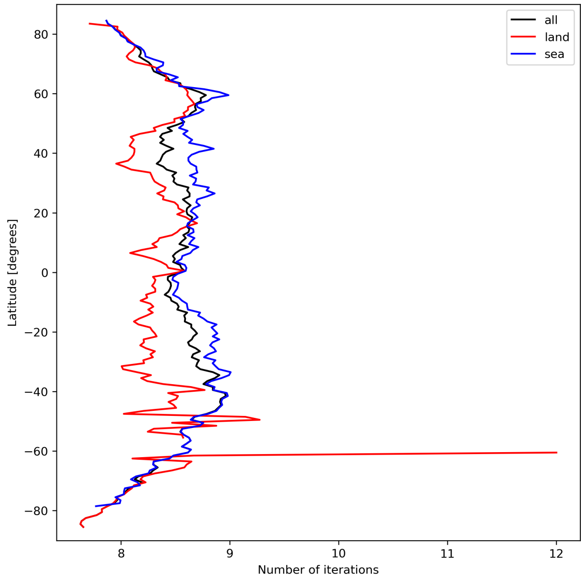
Figure 16: Zonal average of “Number of iterations” for 2024-03-18 to 2024-03-20.
