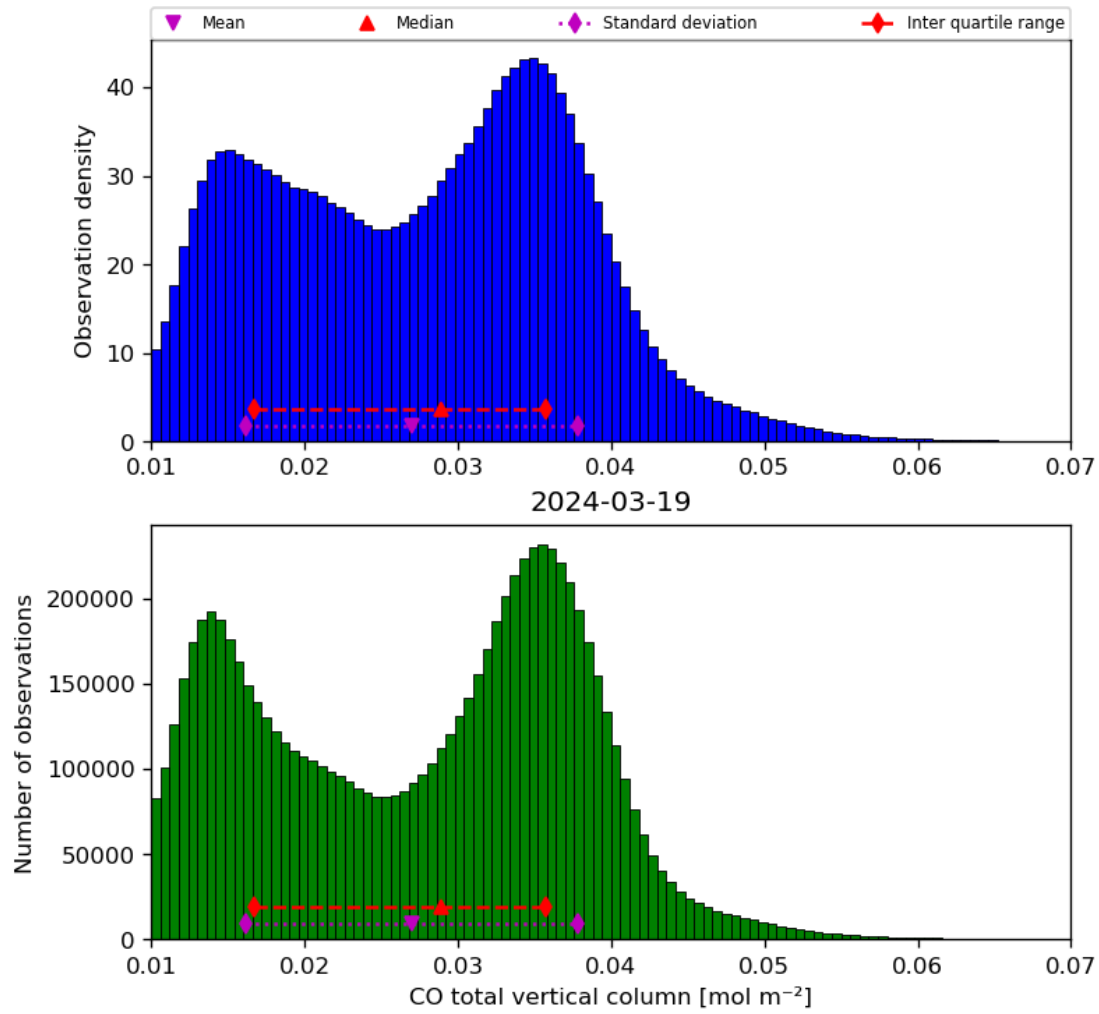
Figure 18: Histogram of “CO total vertical column” for 2024-03-18 to 2024-03-20
