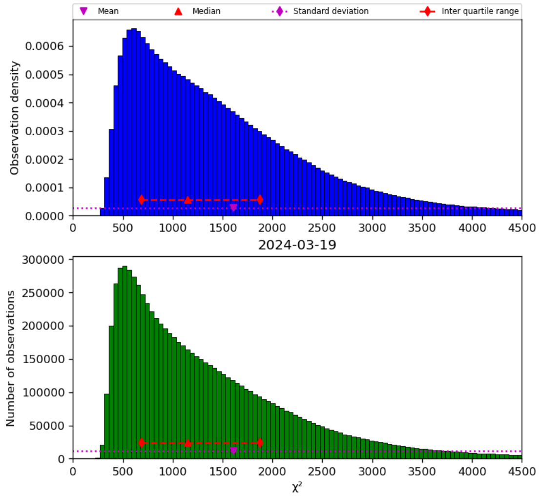
Figure 22: Histogram of “ \chi^2 ” for 2024-03-18 to 2024-03-20
