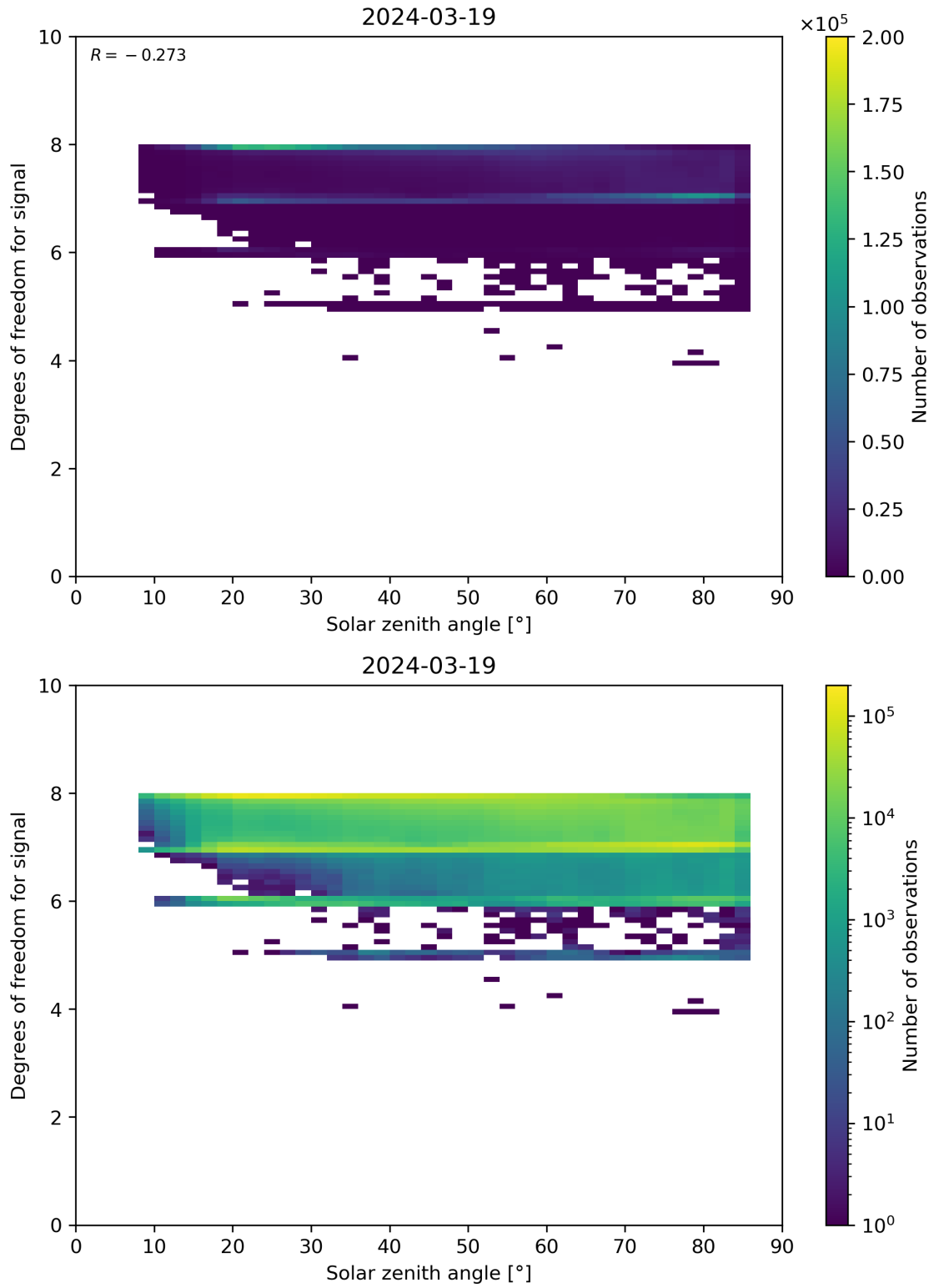
Figure 65: Scatter density plot of “Solar zenith angle” against “Degrees of freedom for signal” for 2024-03-18 to 2024-03-20.
