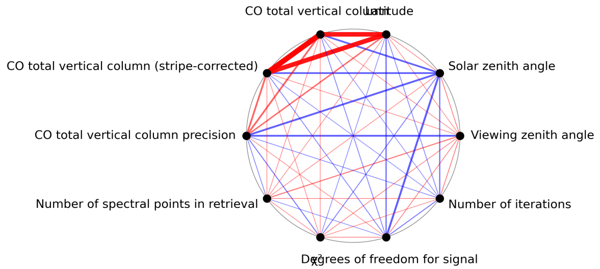
Figure 1: Map of correlation graph for 2024-03-18 to 2024-03-20.
