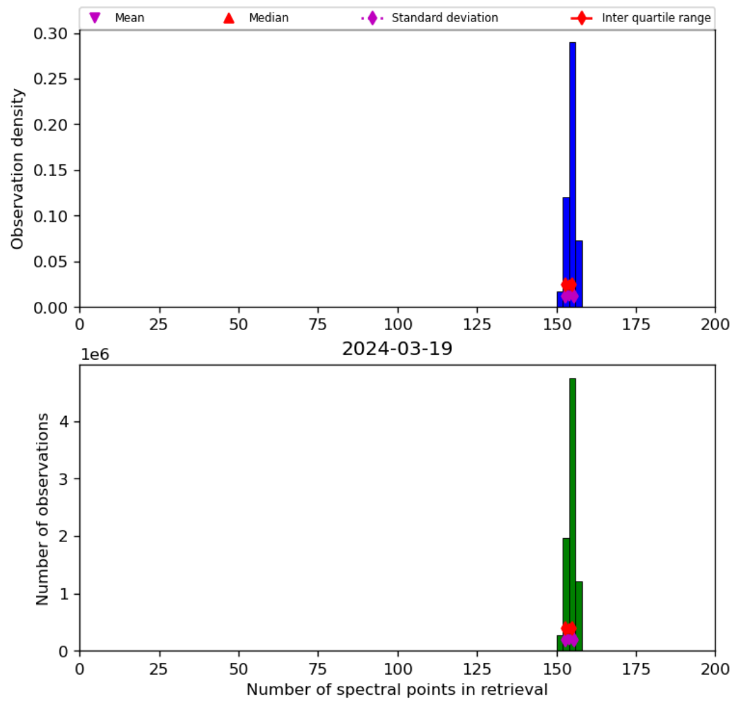
Figure 21: Histogram of “Number of spectral points in retrieval” for 2024-03-18 to 2024-03-20
