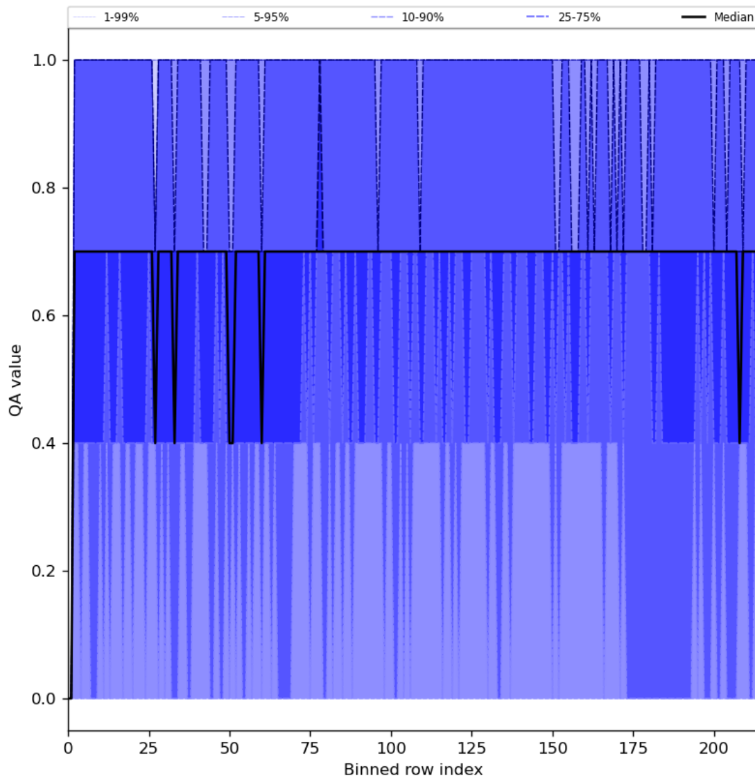
Figure 25: Along track statistics of “QA value” for 2024-03-18 to 2024-03-20
