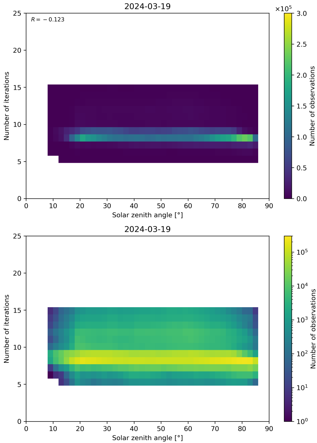
Figure 67: Scatter density plot of “Solar zenith angle” against “Number of iterations” for 2024-03-18 to 2024-03-20.
