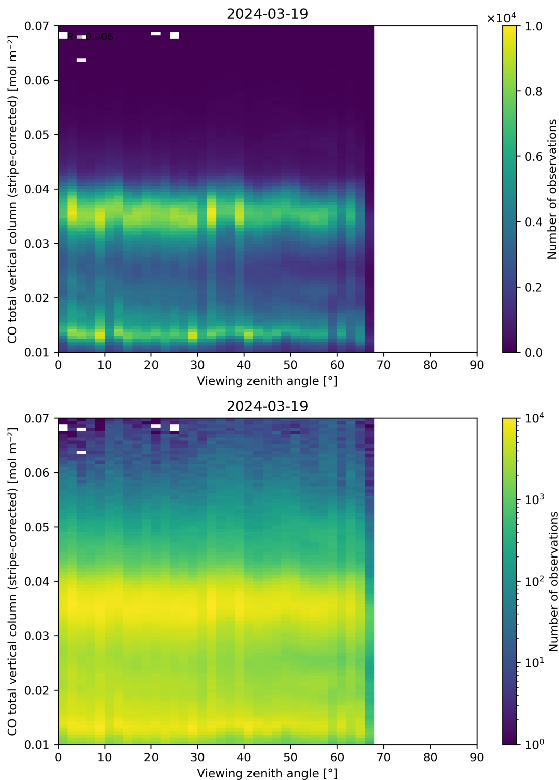
Figure 70: Scatter density plot of “Viewing zenith angle” against “CO total vertical column (stripe-corrected)” for 2024-03-18 to 2024-03-20.
