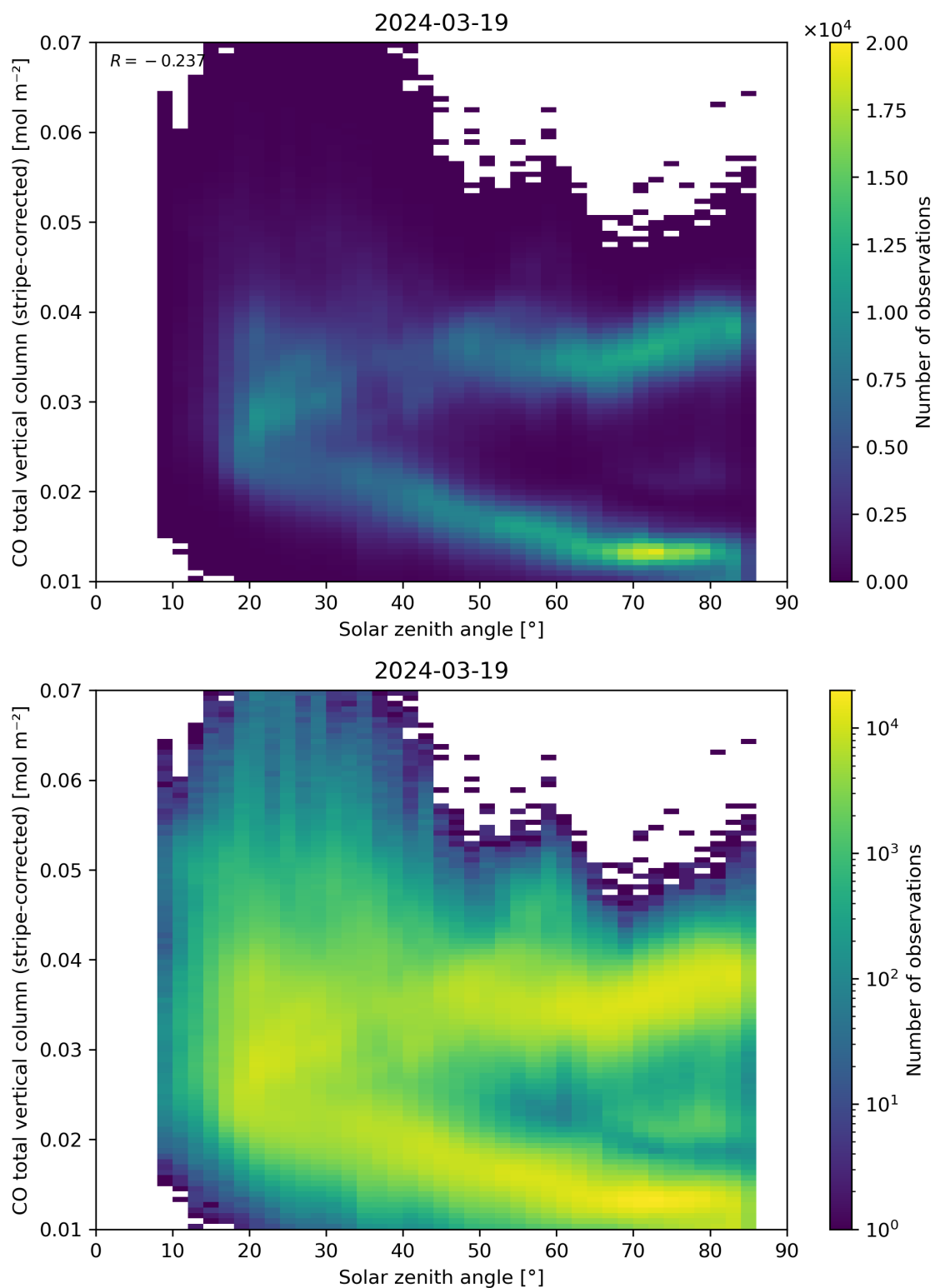
Figure 62: Scatter density plot of “Solar zenith angle” against “CO total vertical column (stripe-corrected)” for 2024-03-18 to 2024-03-20.
