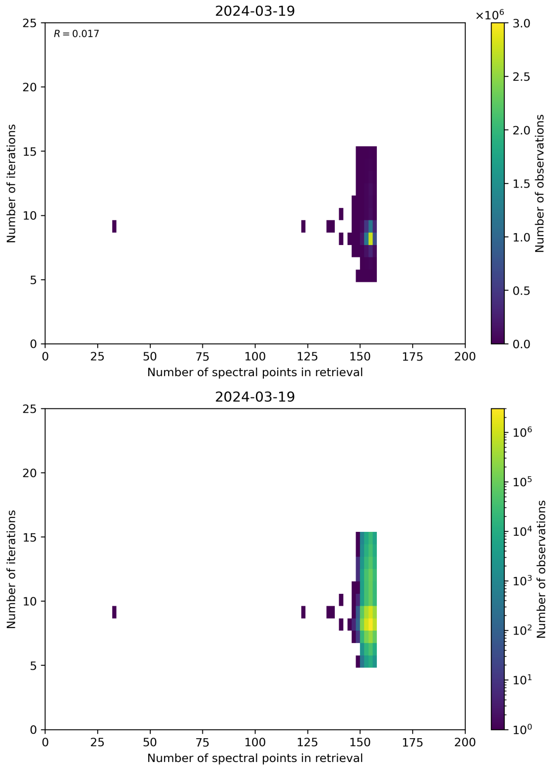
Figure 60: Scatter density plot of “Number of spectral points in retrieval” against “Number of iterations” for 2024-03-18 to 2024-03-20.
