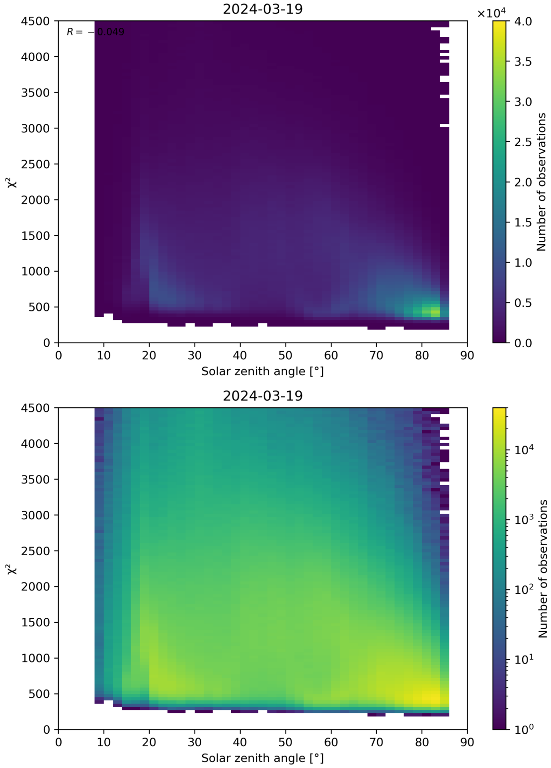
Figure 64: Scatter density plot of “Solar zenith angle” against “ \chi^2 ” for 2024-03-18 to 2024-03-20.
