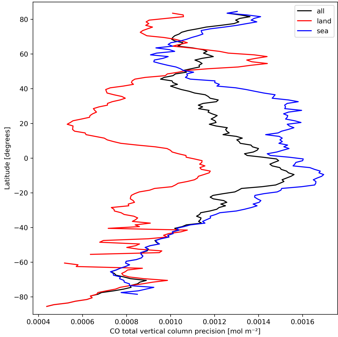
Figure 12: Zonal average of “CO total vertical column precision” for 2024-03-18 to 2024-03-20.
