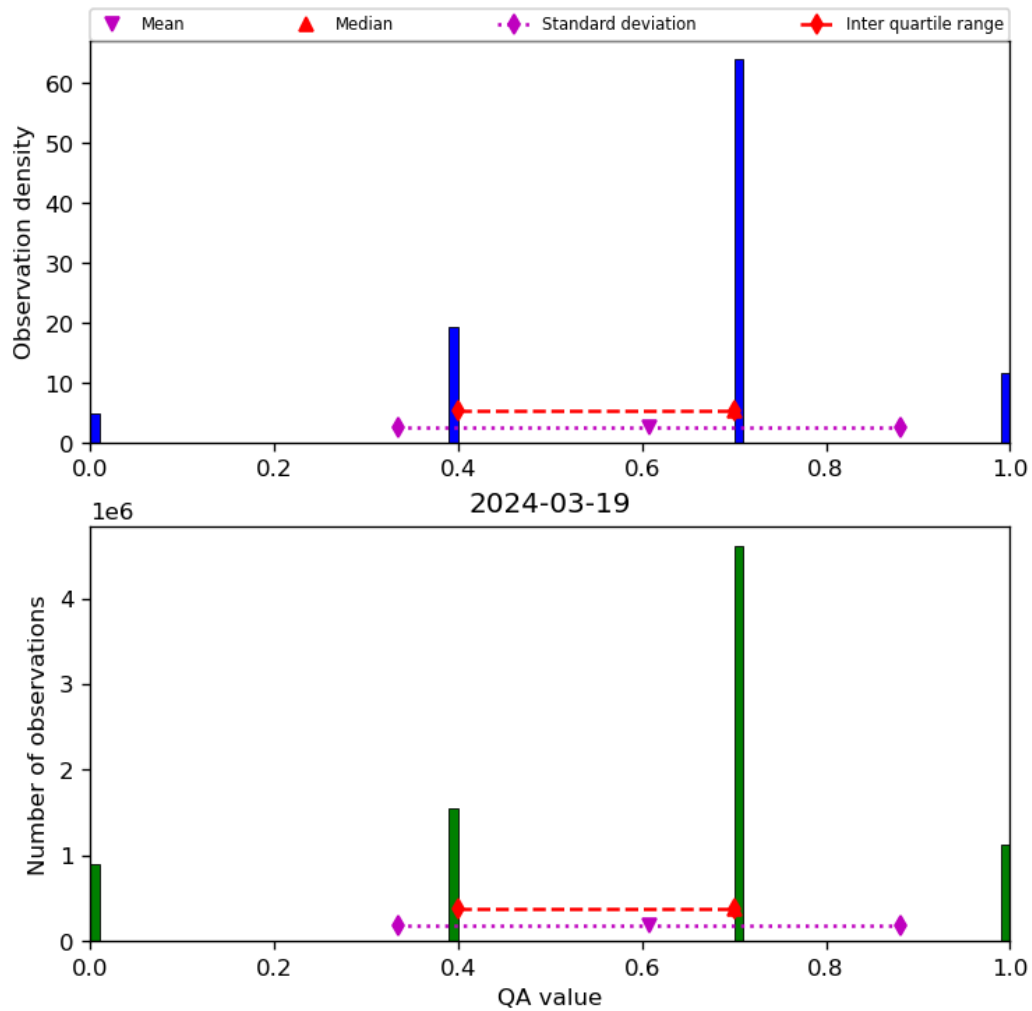
Figure 17: Histogram of “QA value” for 2024-03-18 to 2024-03-20
