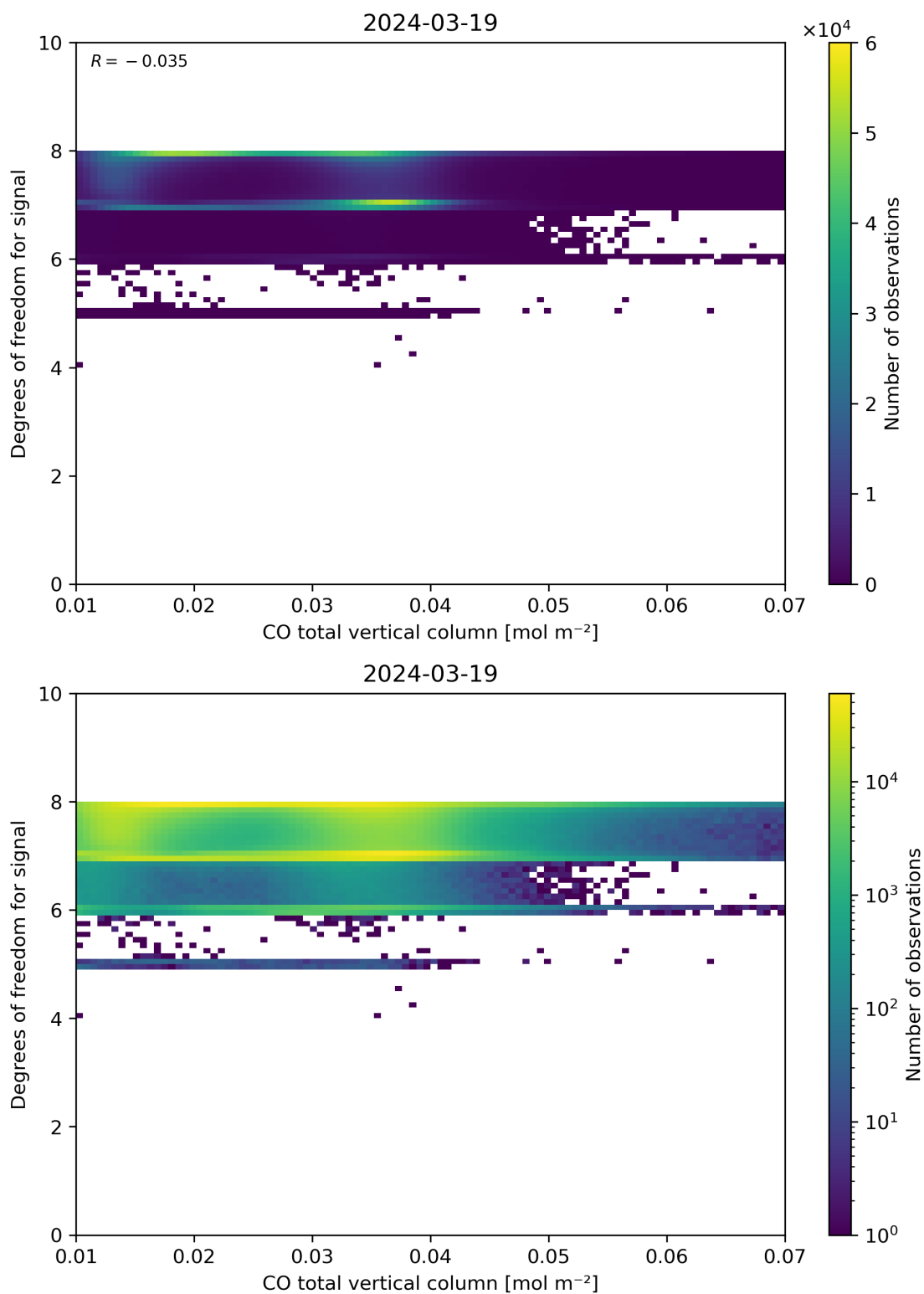
Figure 41: Scatter density plot of “CO total vertical column” against “Degrees of freedom for signal” for 2024-03-18 to 2024-03-20.
