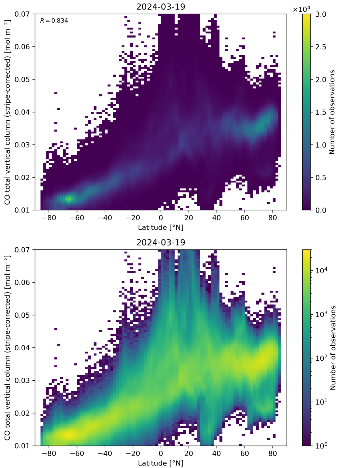
Figure 52: Scatter density plot of “Latitude” against “CO total vertical column (stripe-corrected)” for 2024-03-18 to 2024-03-20.
