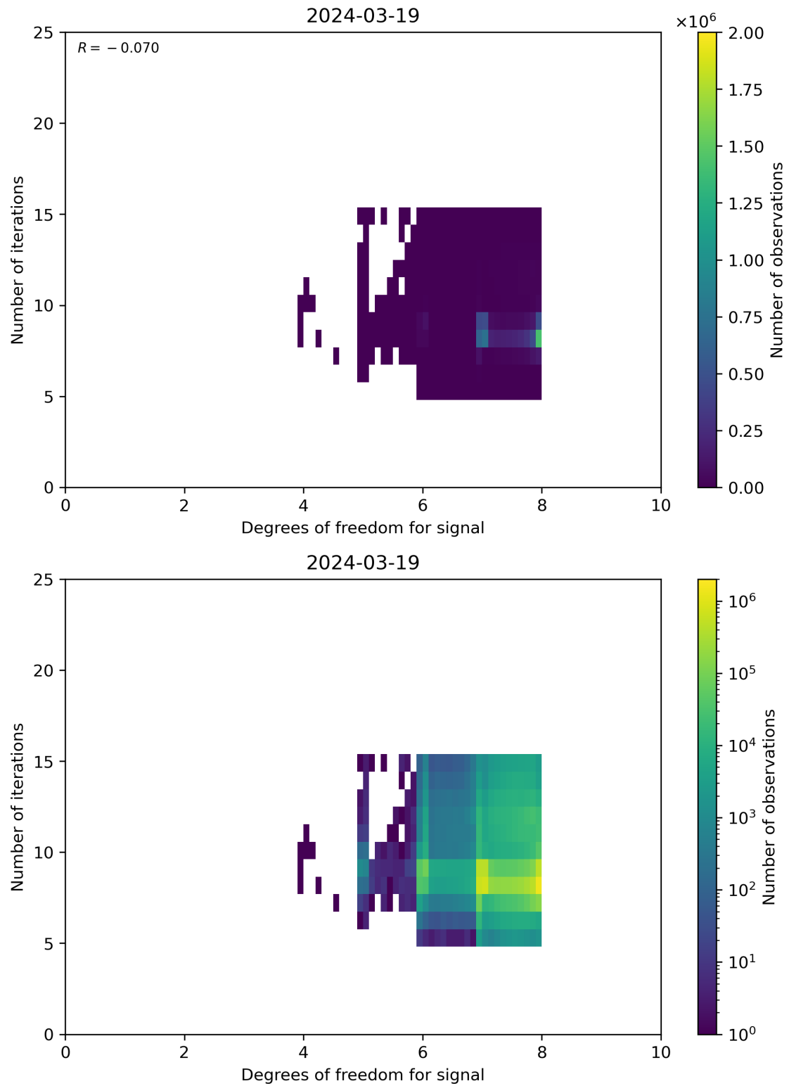
Figure 50: Scatter density plot of “Degrees of freedom for signal” against “Number of iterations” for 2024-03-18 to 2024-03-20.
