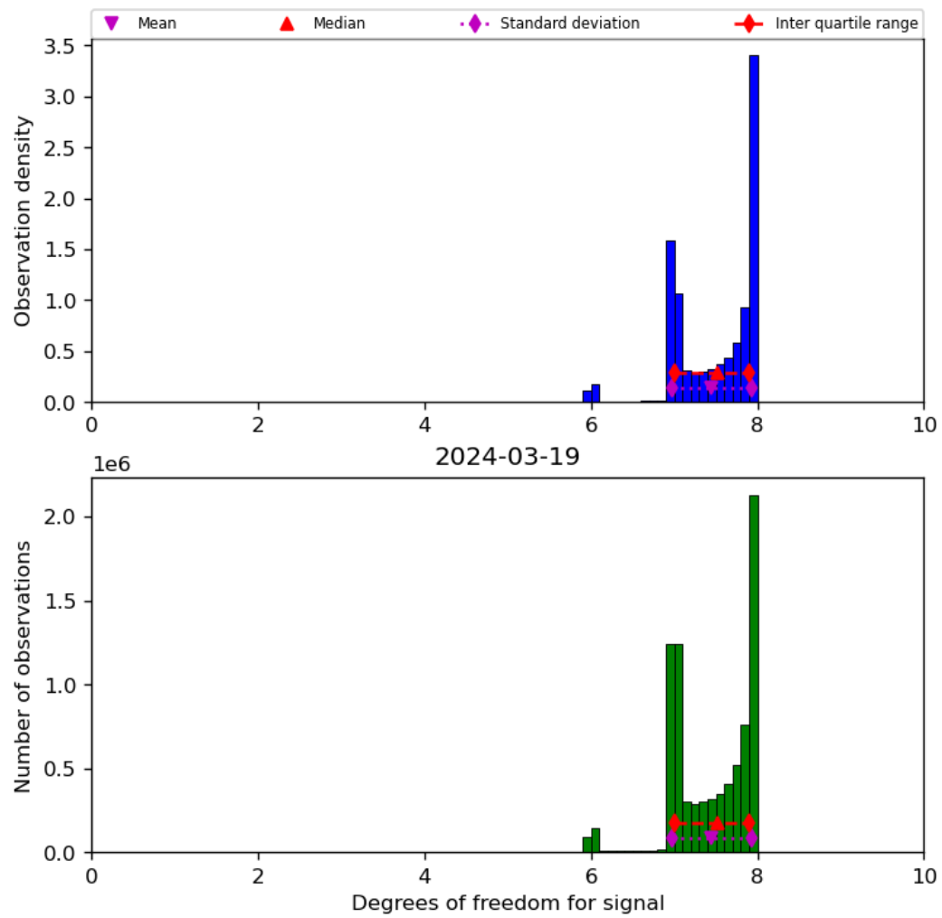
Figure 23: Histogram of “Degrees of freedom for signal” for 2024-03-18 to 2024-03-20
