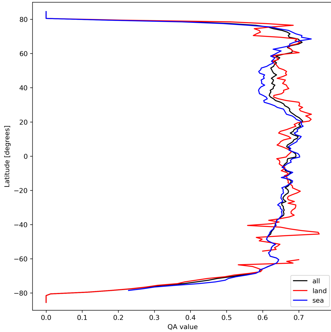
Figure 9: Zonal average of “QA value” for 2024-03-18 to 2024-03-20.
