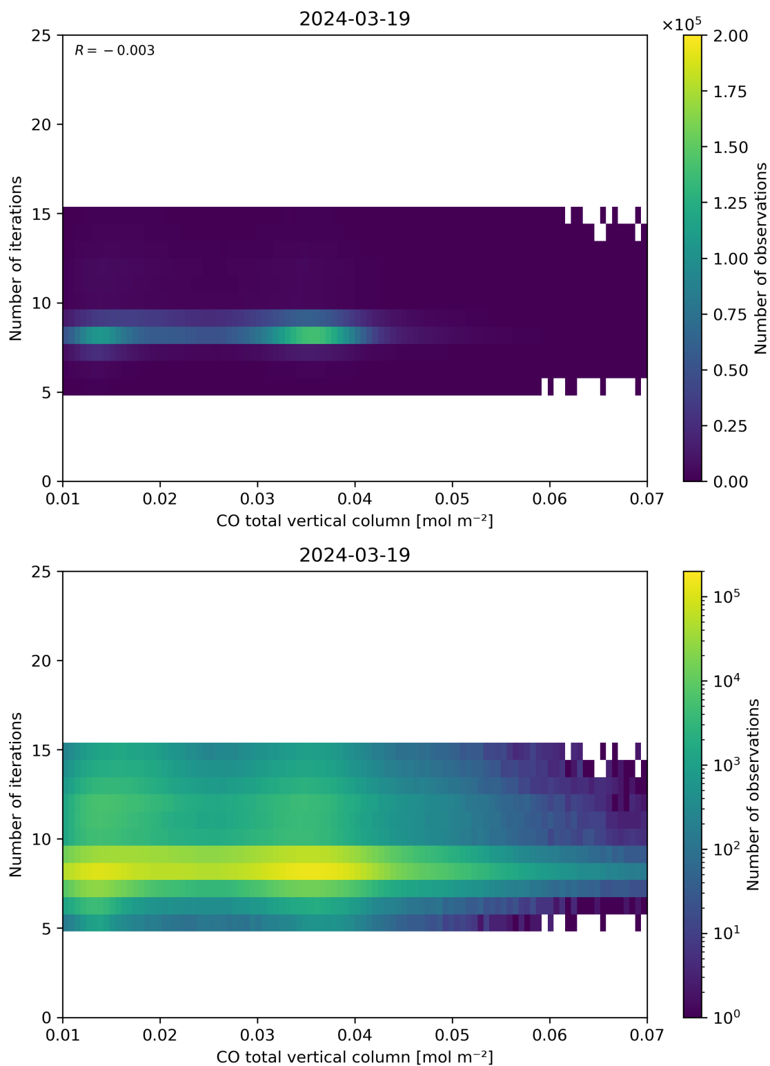
Figure 42: Scatter density plot of “CO total vertical column” against “Number of iterations” for 2024-03-18 to 2024-03-20.
