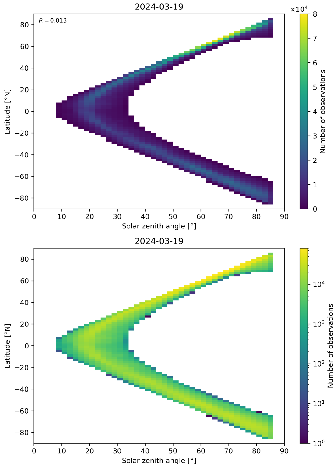
Figure 66: Scatter density plot of “Solar zenith angle” against “Latitude” for 2024-03-18 to 2024-03-20.
