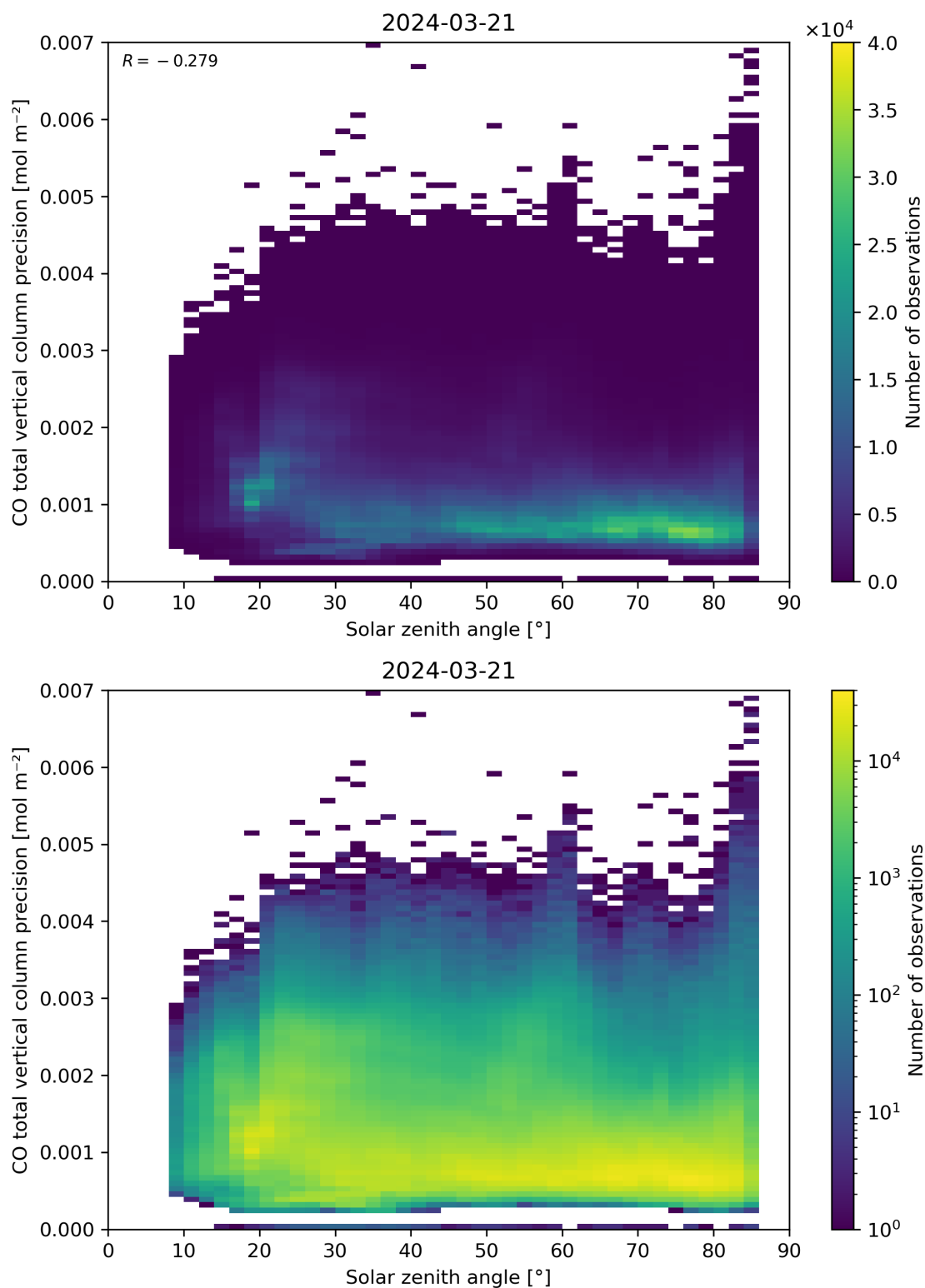
Figure 63: Scatter density plot of “Solar zenith angle” against “CO total vertical column precision” for 2024-03-20 to 2024-03-22.
