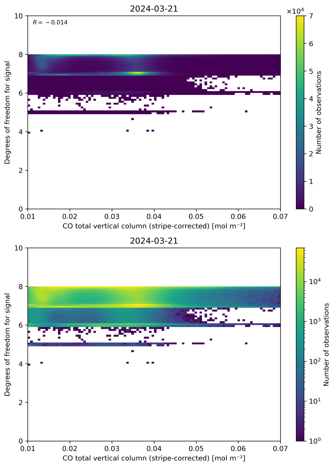
Figure 38: Scatter density plot of “CO total vertical column (stripe-corrected)” against “Degrees of freedom for signal” for 2024-03-20 to 2024-03-22.
