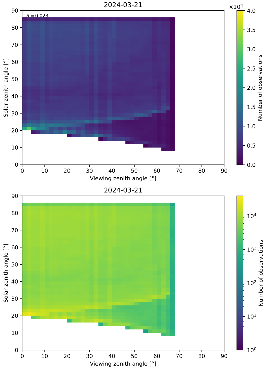
Figure 77: Scatter density plot of “Viewing zenith angle” against “Solar zenith angle” for 2024-03-20 to 2024-03-22.
