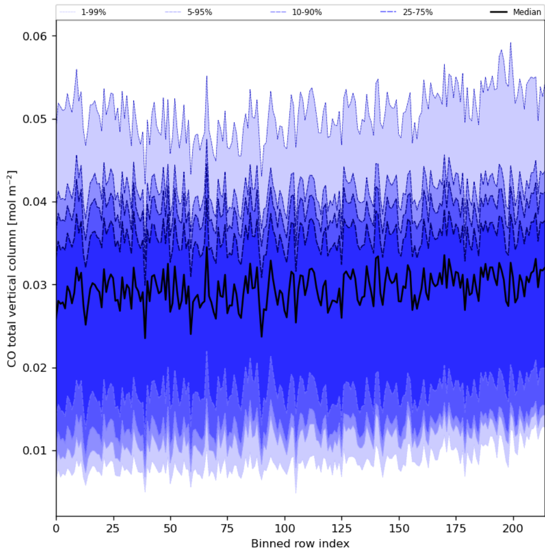
Figure 26: Along track statistics of “CO total vertical column” for 2024-03-20 to 2024-03-22
