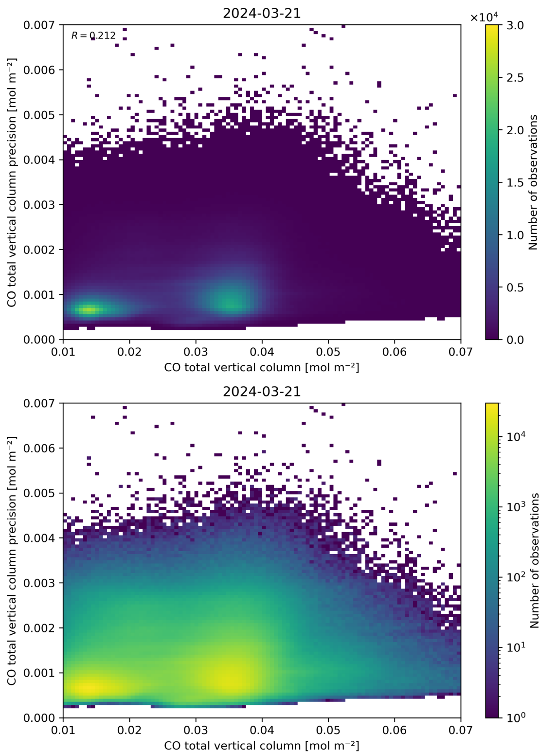
Figure 34: Scatter density plot of “CO total vertical column” against “CO total vertical column precision” for 2024-03-20 to 2024-03-22.
