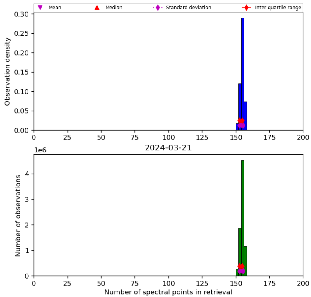
Figure 21: Histogram of “Number of spectral points in retrieval” for 2024-03-20 to 2024-03-22
