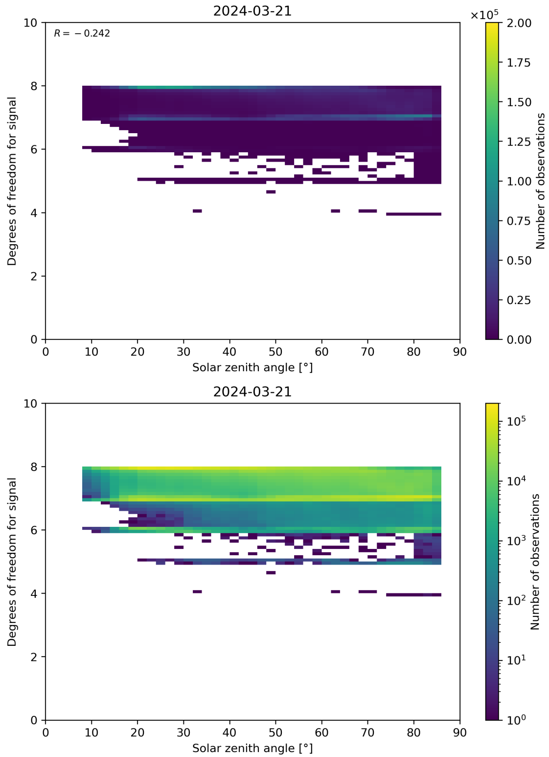
Figure 65: Scatter density plot of “Solar zenith angle” against “Degrees of freedom for signal” for 2024-03-20 to 2024-03-22.
