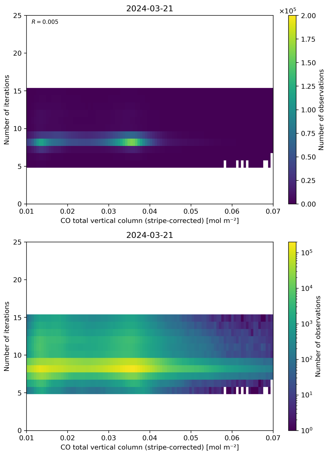
Figure 39: Scatter density plot of “CO total vertical column (stripe-corrected)” against “Number of iterations” for 2024-03-20 to 2024-03-22.
