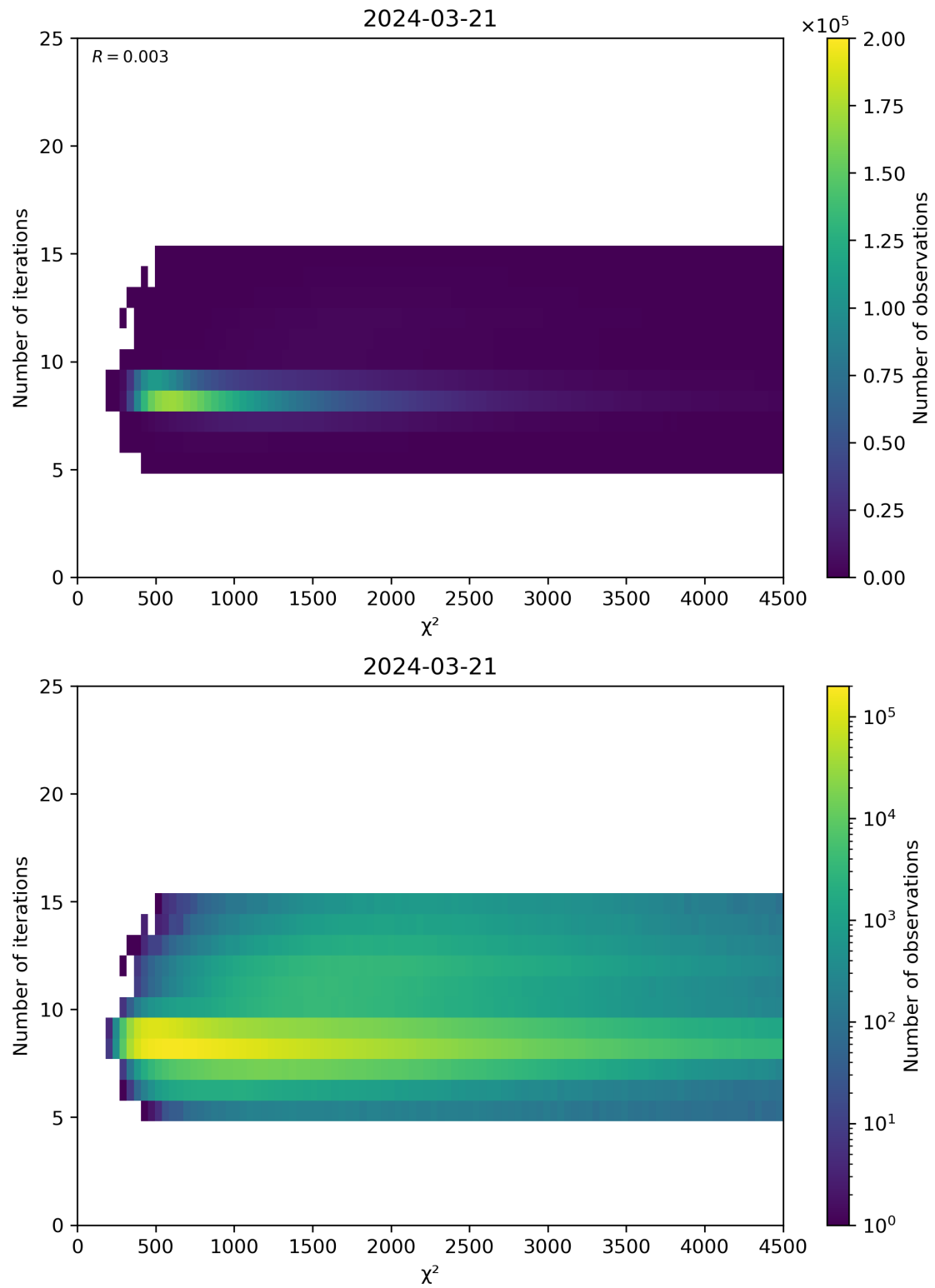
Figure 49: Scatter density plot of “ \chi^2 ” against “Number of iterations” for 2024-03-20 to 2024-03-22.
