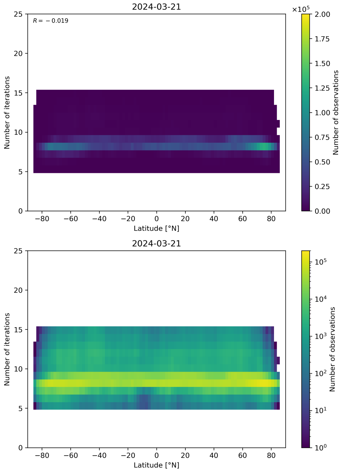
Figure 56: Scatter density plot of “Latitude” against “Number of iterations” for 2024-03-20 to 2024-03-22.
