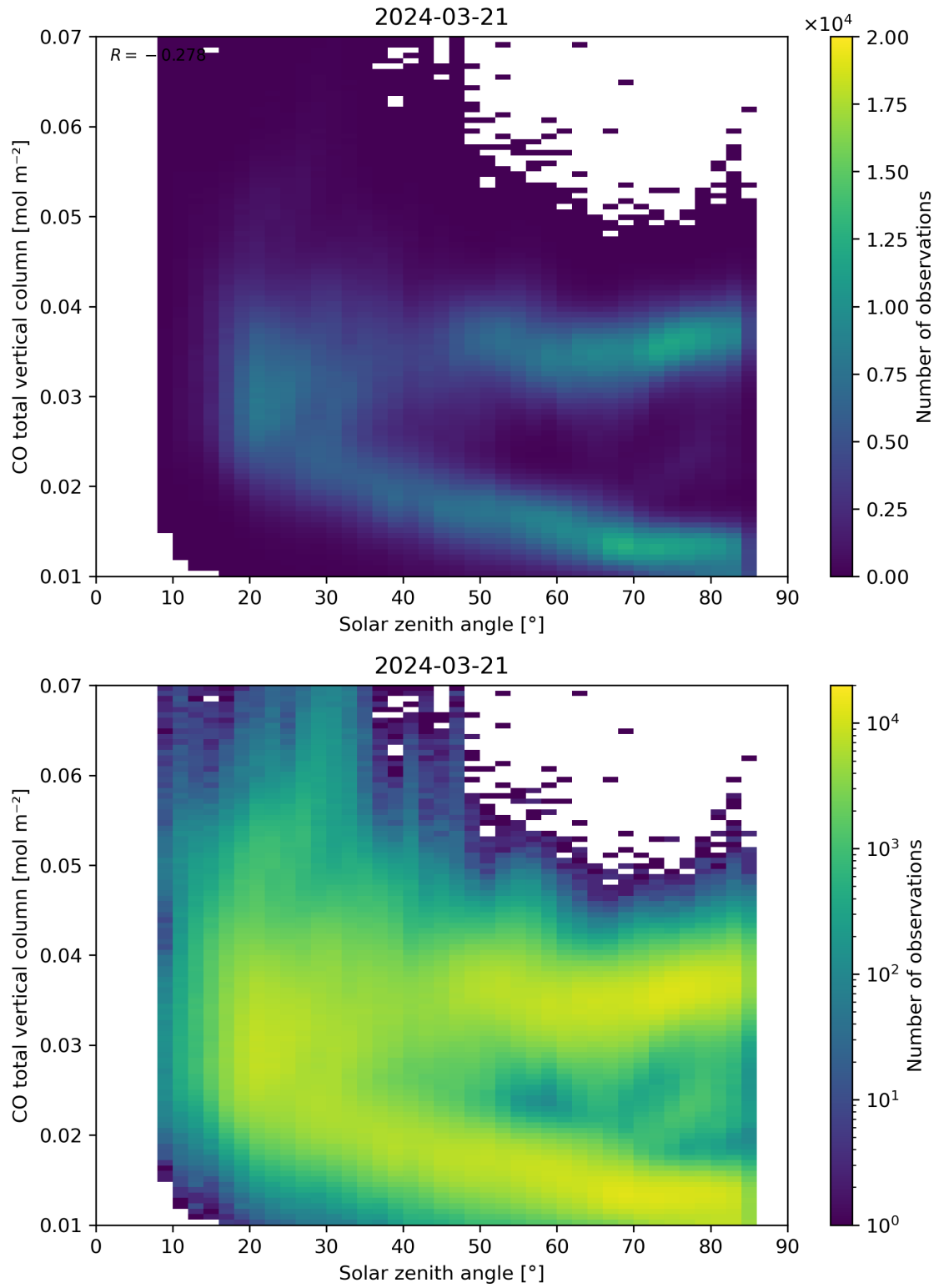
Figure 61: Scatter density plot of “Solar zenith angle” against “CO total vertical column” for 2024-03-20 to 2024-03-22.
