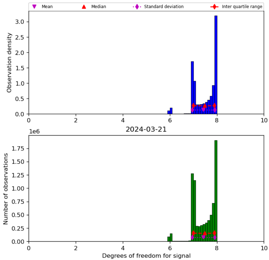
Figure 23: Histogram of “Degrees of freedom for signal” for 2024-03-20 to 2024-03-22
