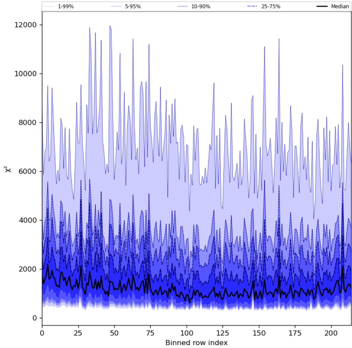
Figure 30: Along track statistics of “ \chi^2 ” for 2024-03-20 to 2024-03-22
