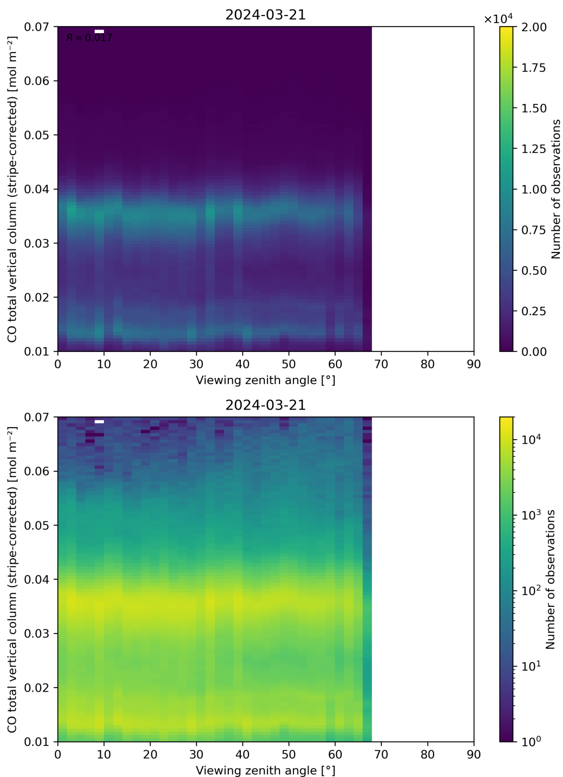
Figure 70: Scatter density plot of “Viewing zenith angle” against “CO total vertical column (stripe-corrected)” for 2024-03-20 to 2024-03-22.
