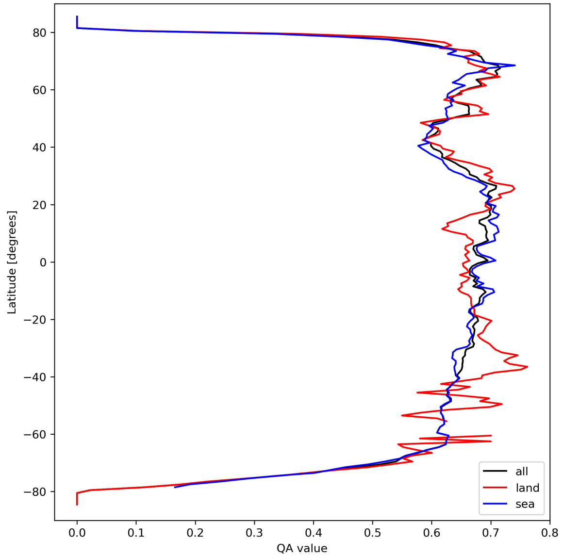
Figure 9: Zonal average of “QA value” for 2024-03-20 to 2024-03-22.
