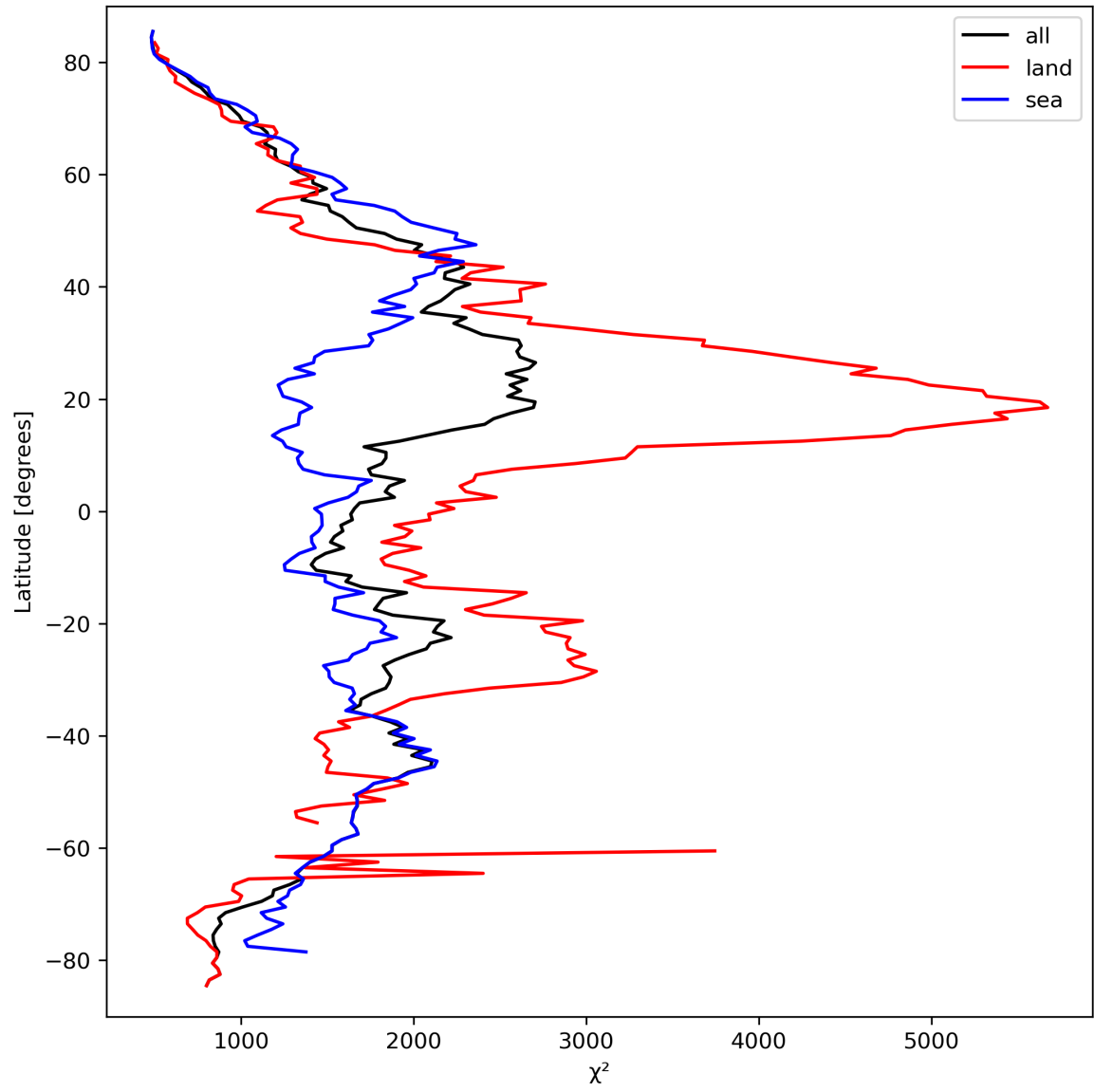
Figure 14: Zonal average of “ \chi^2 ” for 2024-03-20 to 2024-03-22.
