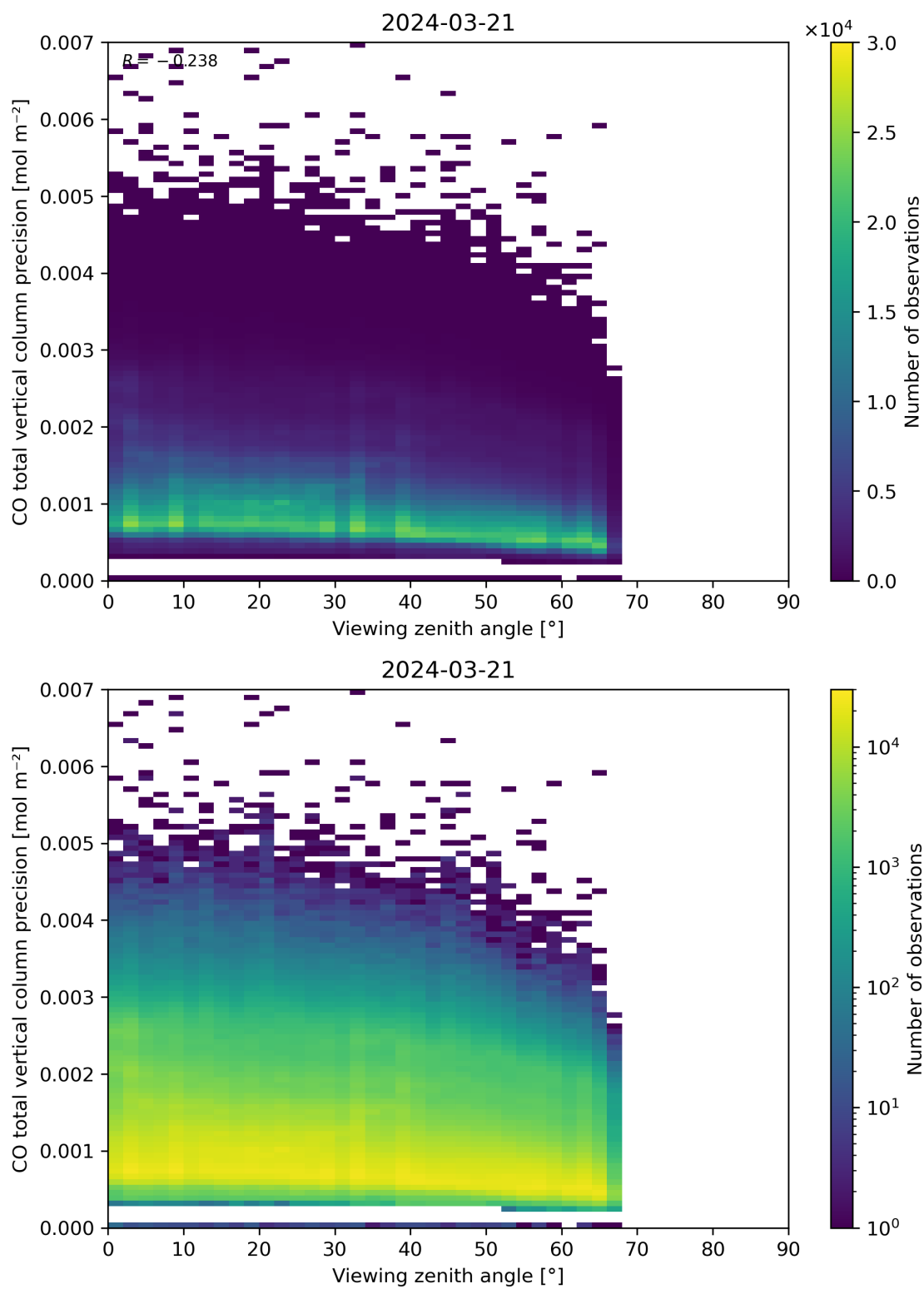
Figure 71: Scatter density plot of “Viewing zenith angle” against “CO total vertical column precision” for 2024-03-20 to 2024-03-22.
