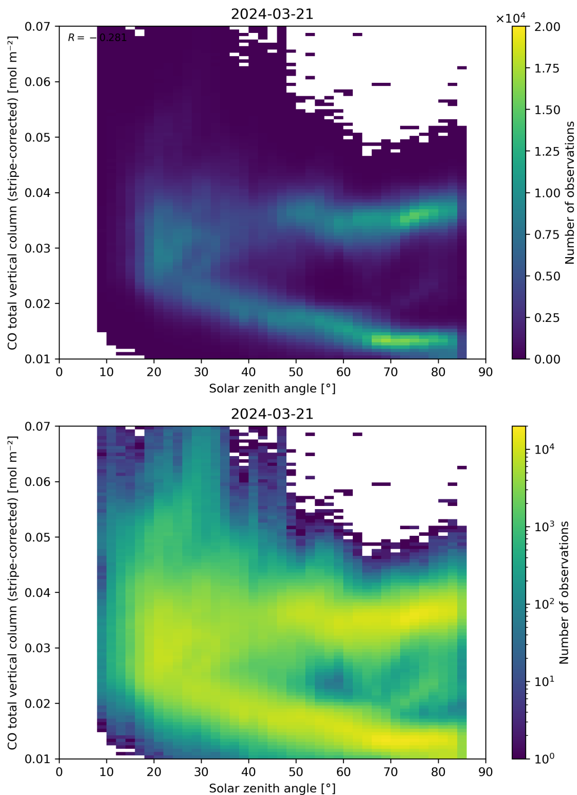
Figure 62: Scatter density plot of “Solar zenith angle” against “CO total vertical column (stripe-corrected)” for 2024-03-20 to 2024-03-22.
