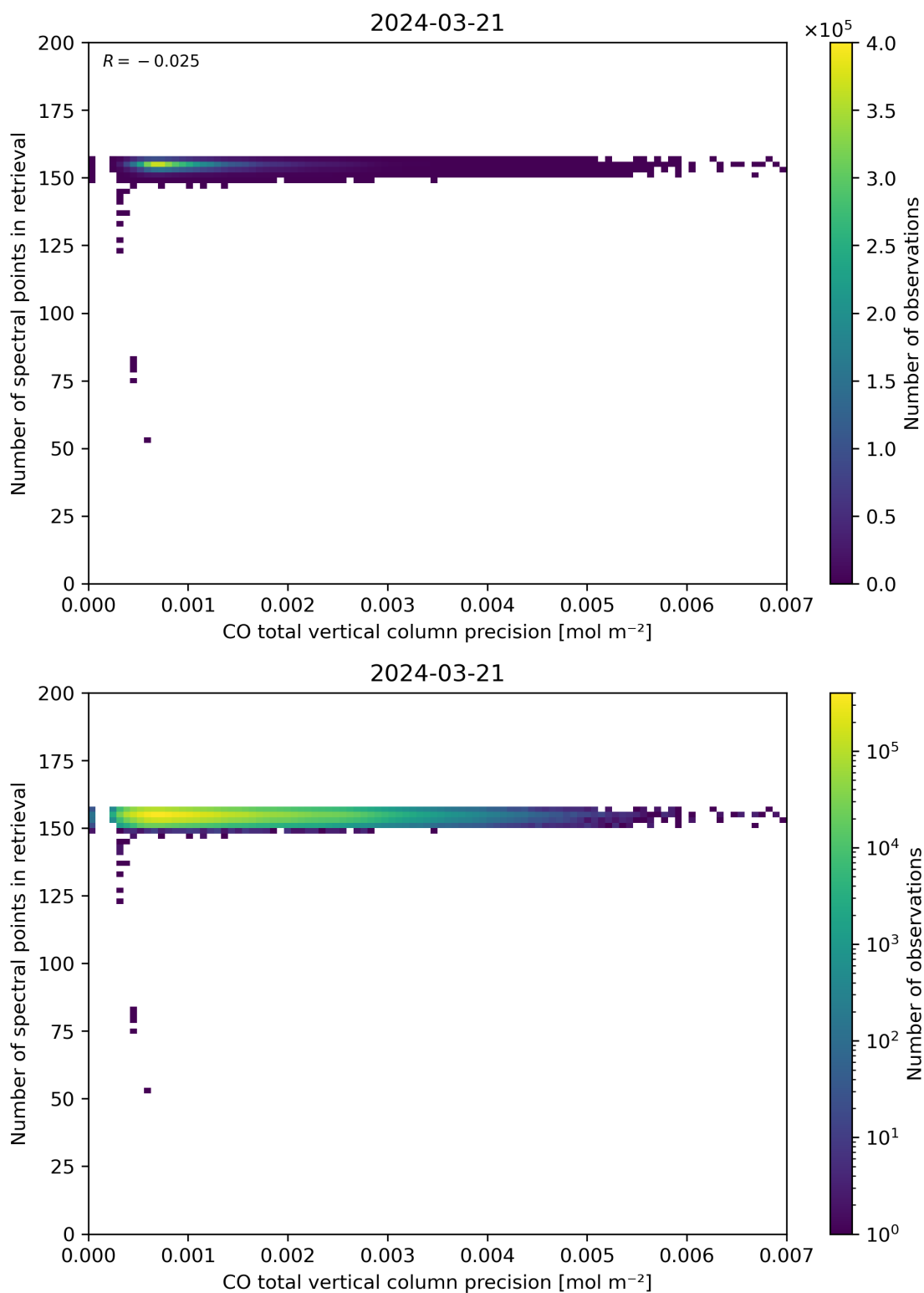
Figure 47: Scatter density plot of “CO total vertical column precision” against “Number of spectral points in retrieval” for 2024-03-20 to 2024-03-22.
