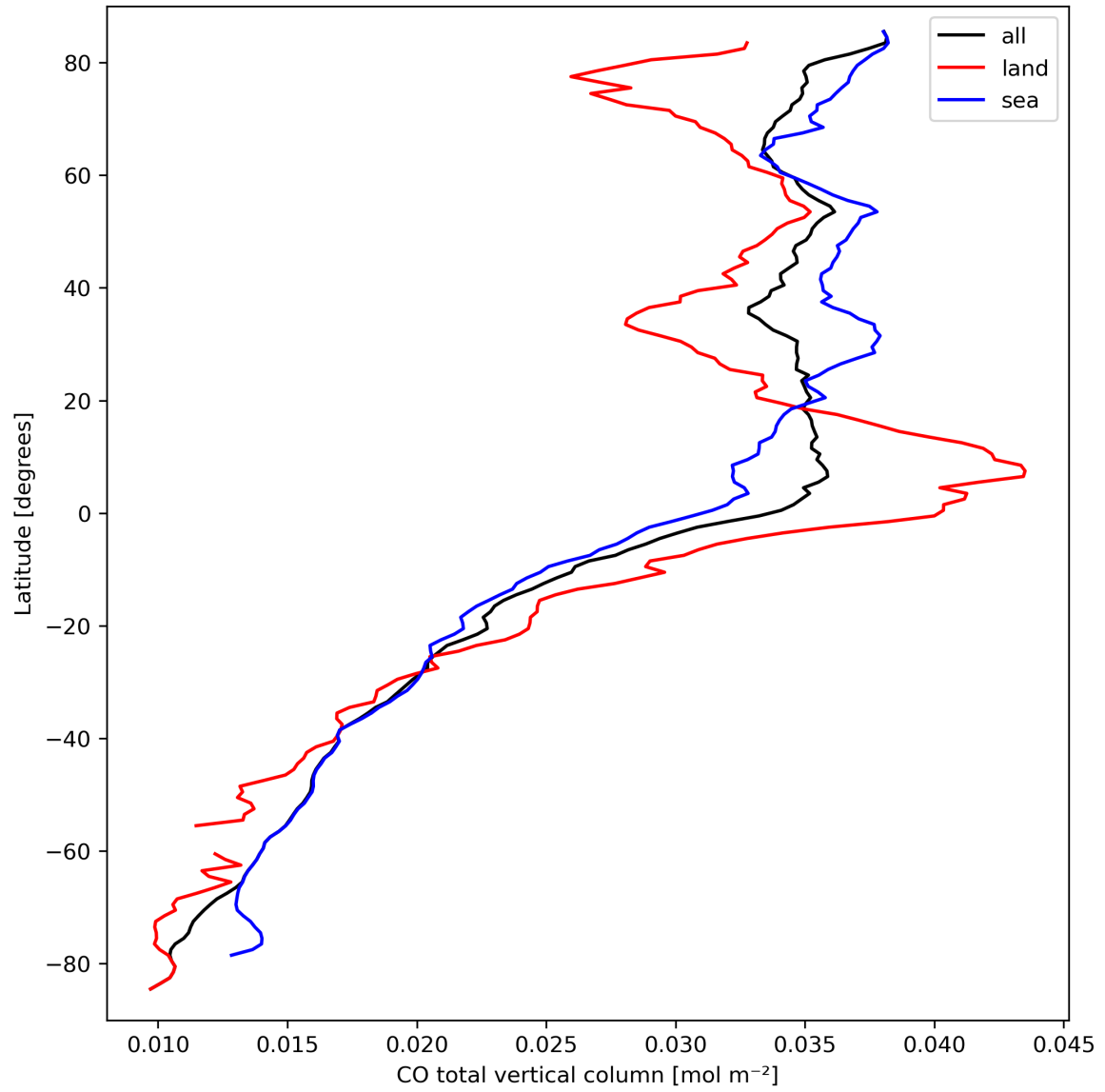
Figure 10: Zonal average of “CO total vertical column” for 2024-03-20 to 2024-03-22.
