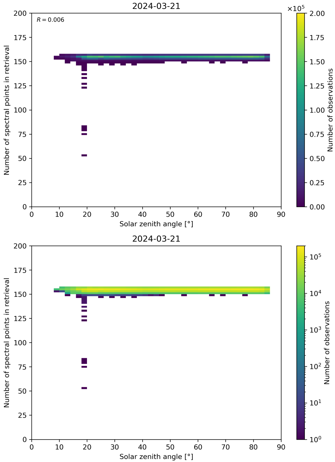
Figure 68: Scatter density plot of “Solar zenith angle” against “Number of spectral points in retrieval” for 2024-03-20 to 2024-03-22.
