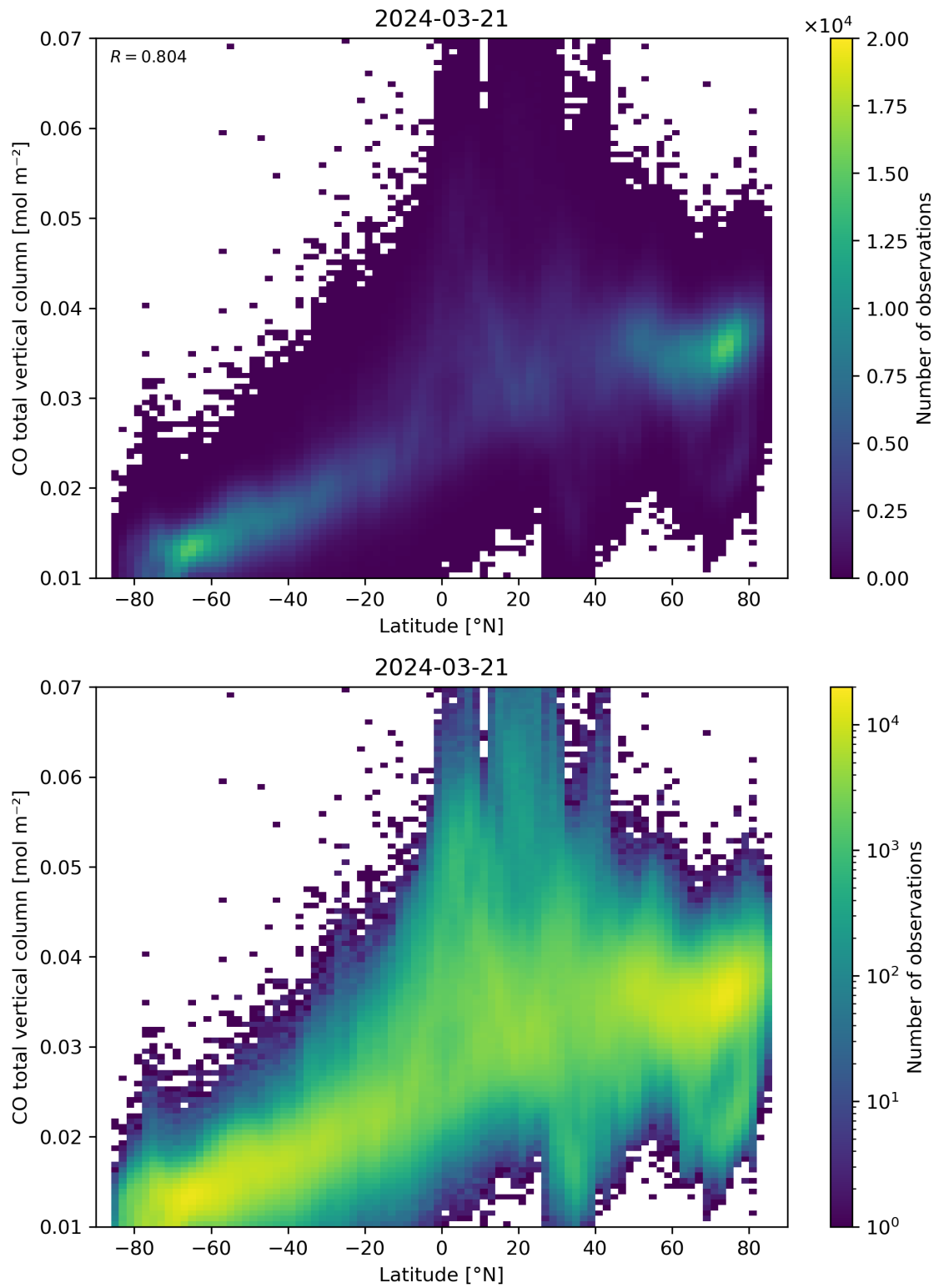
Figure 51: Scatter density plot of “Latitude” against “CO total vertical column” for 2024-03-20 to 2024-03-22.
