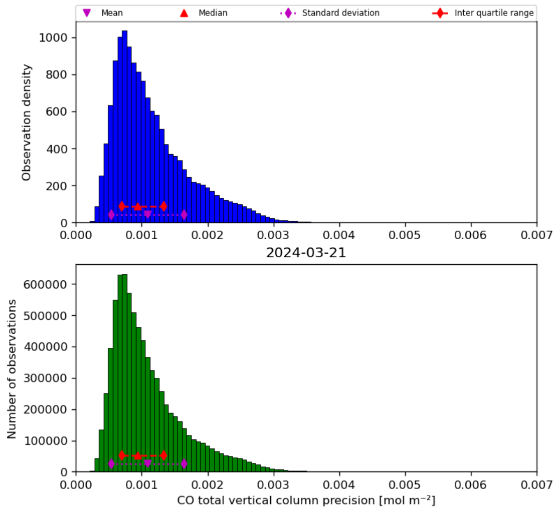
Figure 20: Histogram of “CO total vertical column precision” for 2024-03-20 to 2024-03-22
