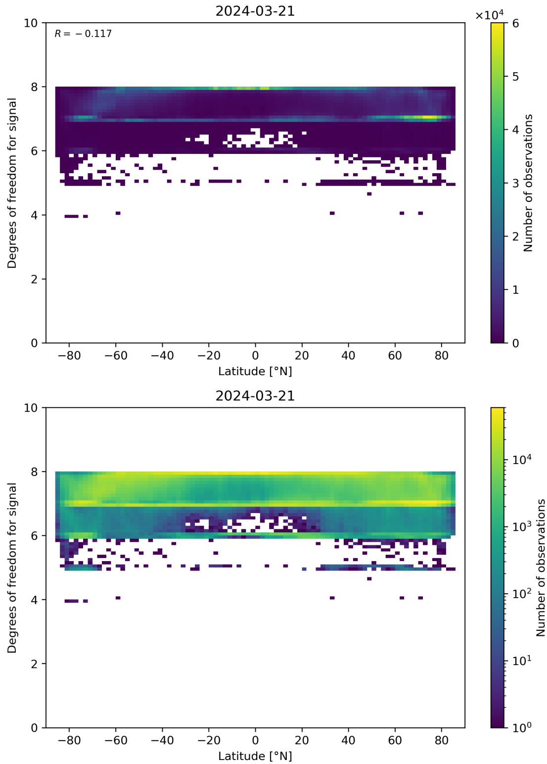
Figure 55: Scatter density plot of “Latitude” against “Degrees of freedom for signal” for 2024-03-20 to 2024-03-22.
