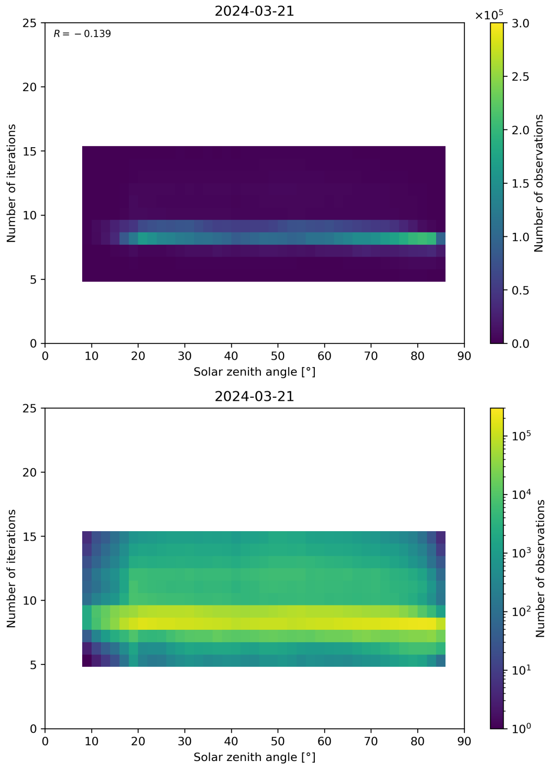
Figure 67: Scatter density plot of “Solar zenith angle” against “Number of iterations” for 2024-03-20 to 2024-03-22.
