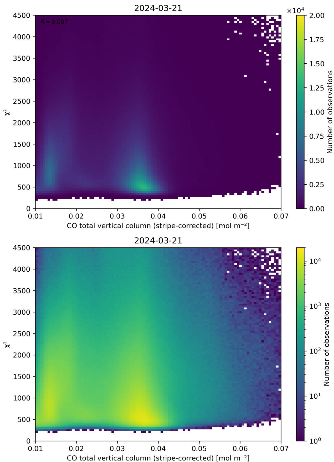
Figure 37: Scatter density plot of “CO total vertical column (stripe-corrected)” against “ \chi^2 ” for 2024-03-20 to 2024-03-22.
