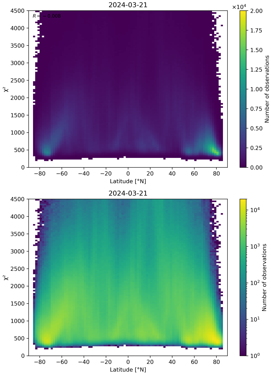
Figure 54: Scatter density plot of “Latitude” against “ \chi^2 ” for 2024-03-20 to 2024-03-22.
