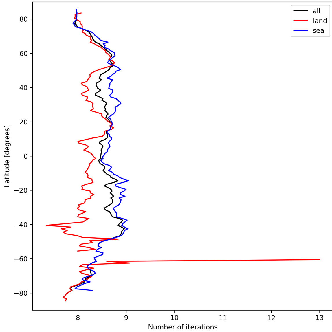
Figure 16: Zonal average of “Number of iterations” for 2024-03-20 to 2024-03-22.
