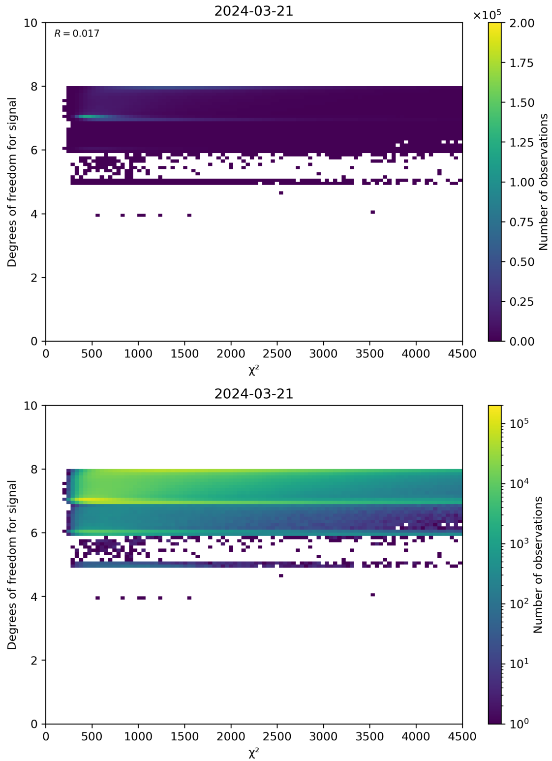
Figure 48: Scatter density plot of “ \chi^2 ” against “Degrees of freedom for signal” for 2024-03-20 to 2024-03-22.
