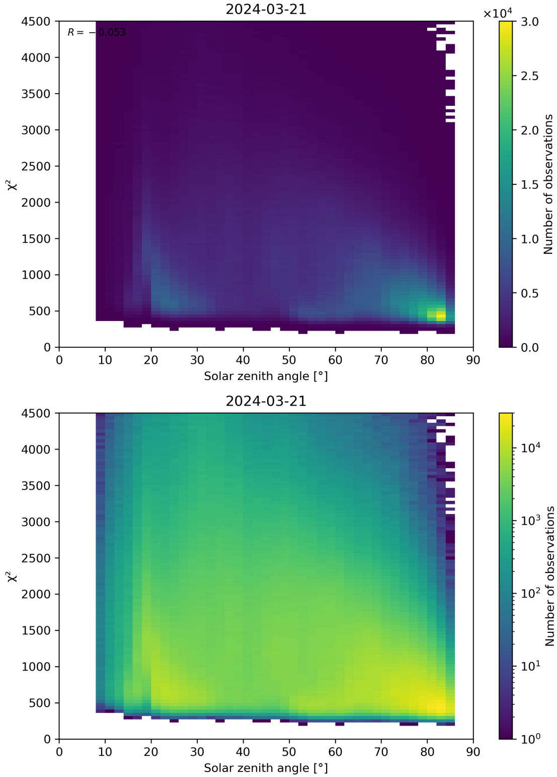
Figure 64: Scatter density plot of “Solar zenith angle” against “ \chi^2 ” for 2024-03-20 to 2024-03-22.
