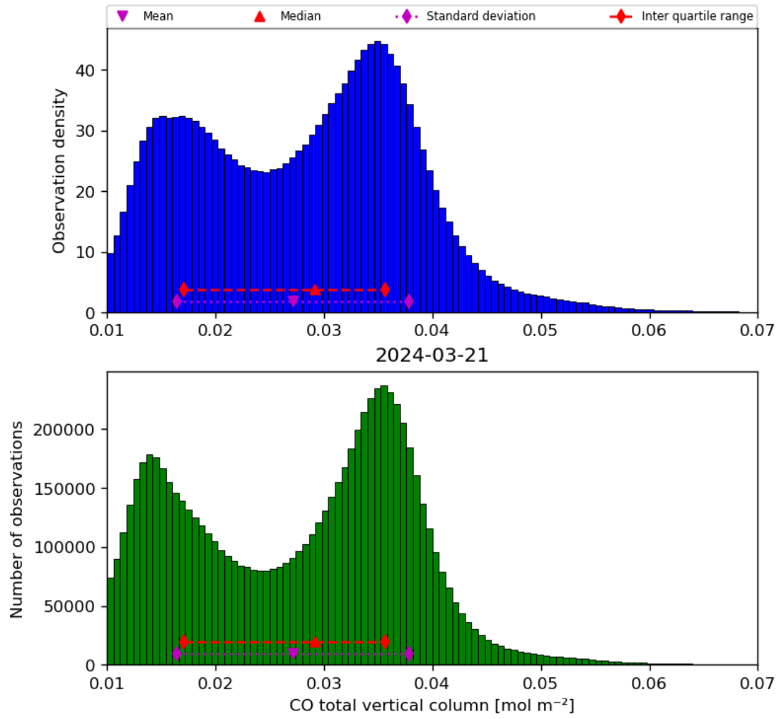
Figure 18: Histogram of “CO total vertical column” for 2024-03-20 to 2024-03-22
