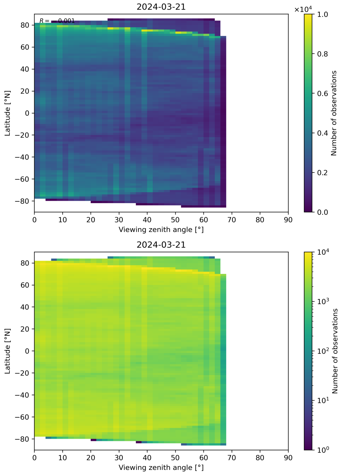
Figure 74: Scatter density plot of “Viewing zenith angle” against “Latitude” for 2024-03-20 to 2024-03-22.
