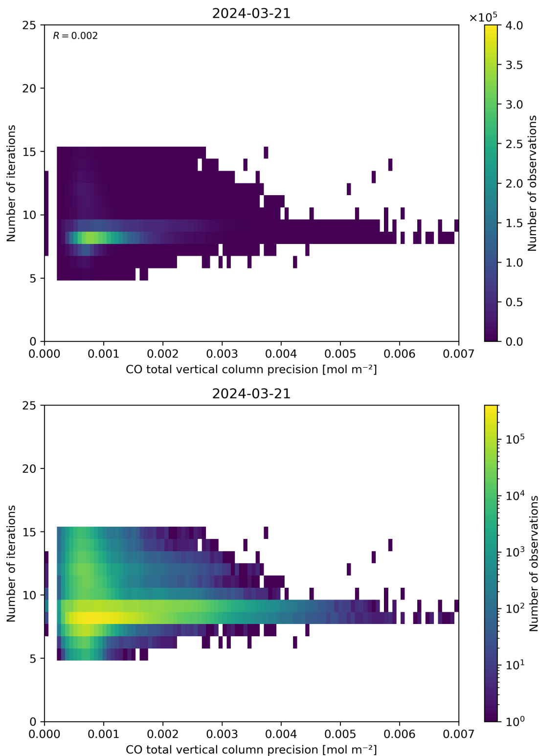
Figure 46: Scatter density plot of “CO total vertical column precision” against “Number of iterations” for 2024-03-20 to 2024-03-22.
