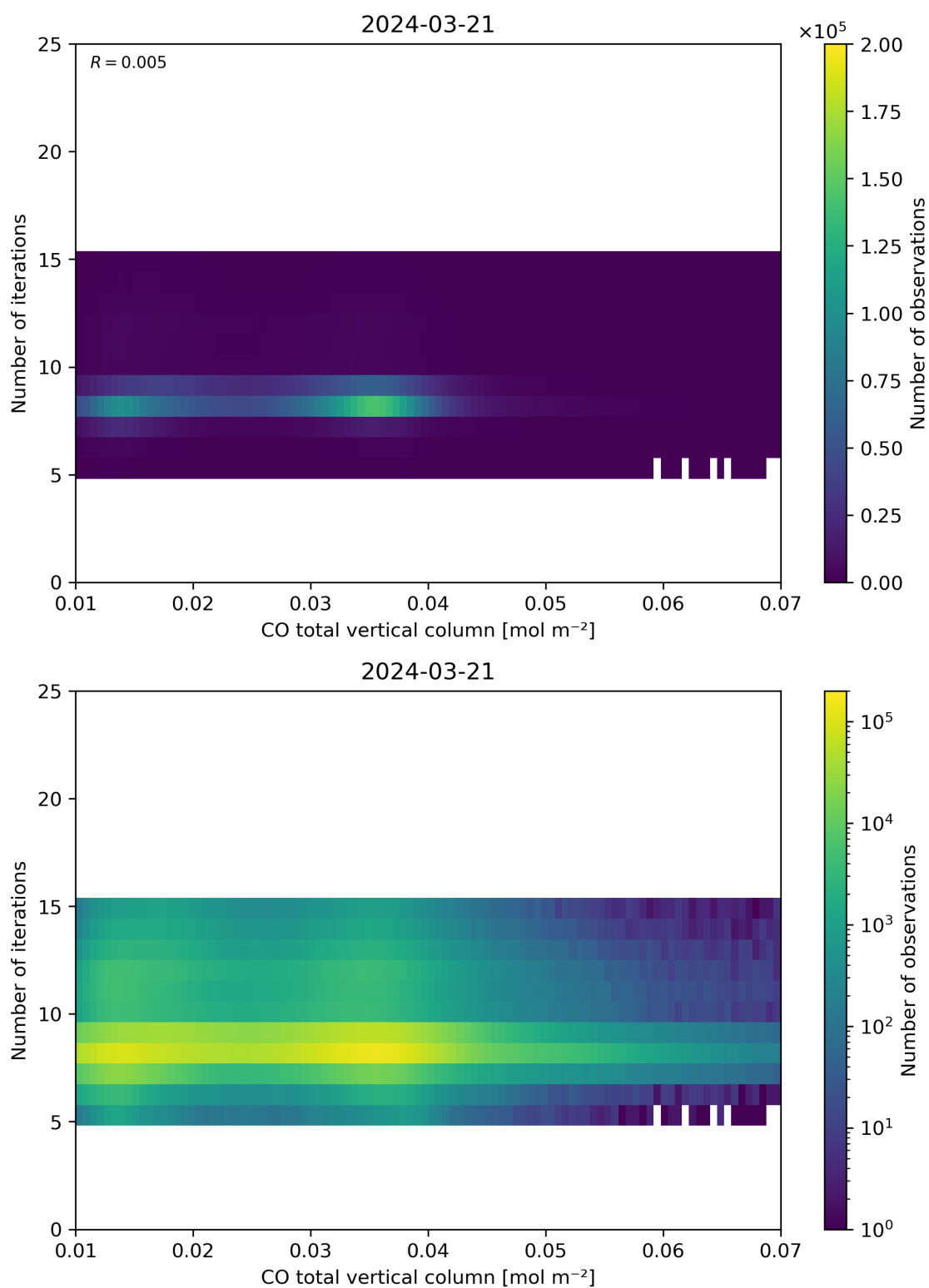
Figure 42: Scatter density plot of “CO total vertical column” against “Number of iterations” for 2024-03-20 to 2024-03-22.
