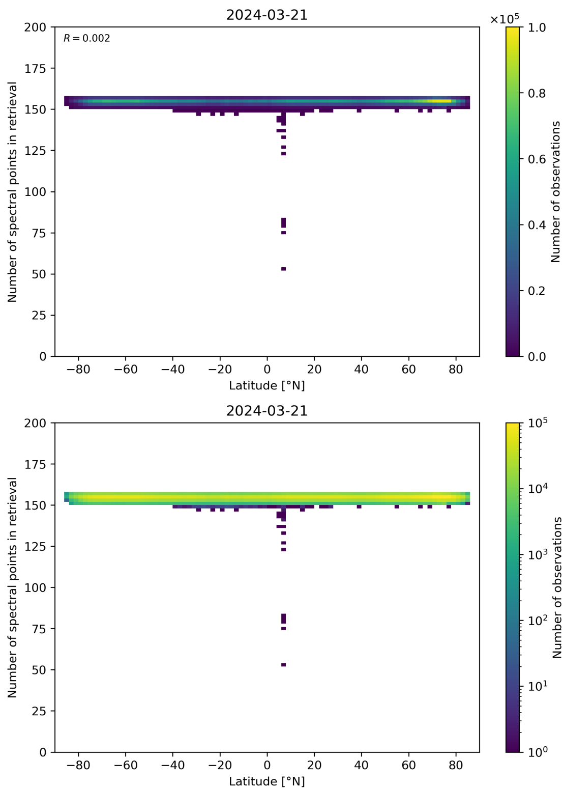
Figure 57: Scatter density plot of “Latitude” against “Number of spectral points in retrieval” for 2024-03-20 to 2024-03-22.
