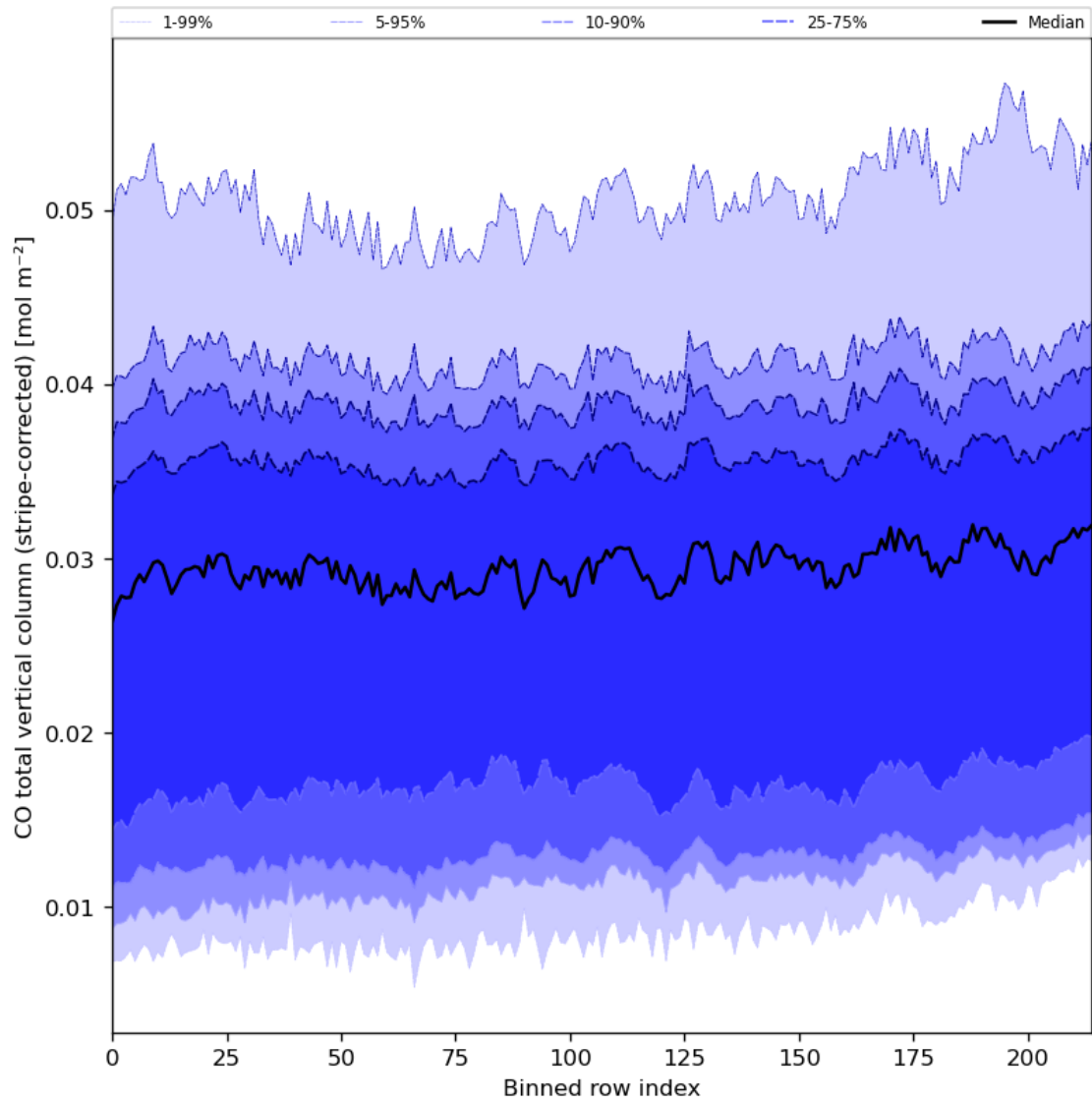
Figure 27: Along track statistics of “CO total vertical column (stripe-corrected)” for 2024-03-20 to 2024-03-22
