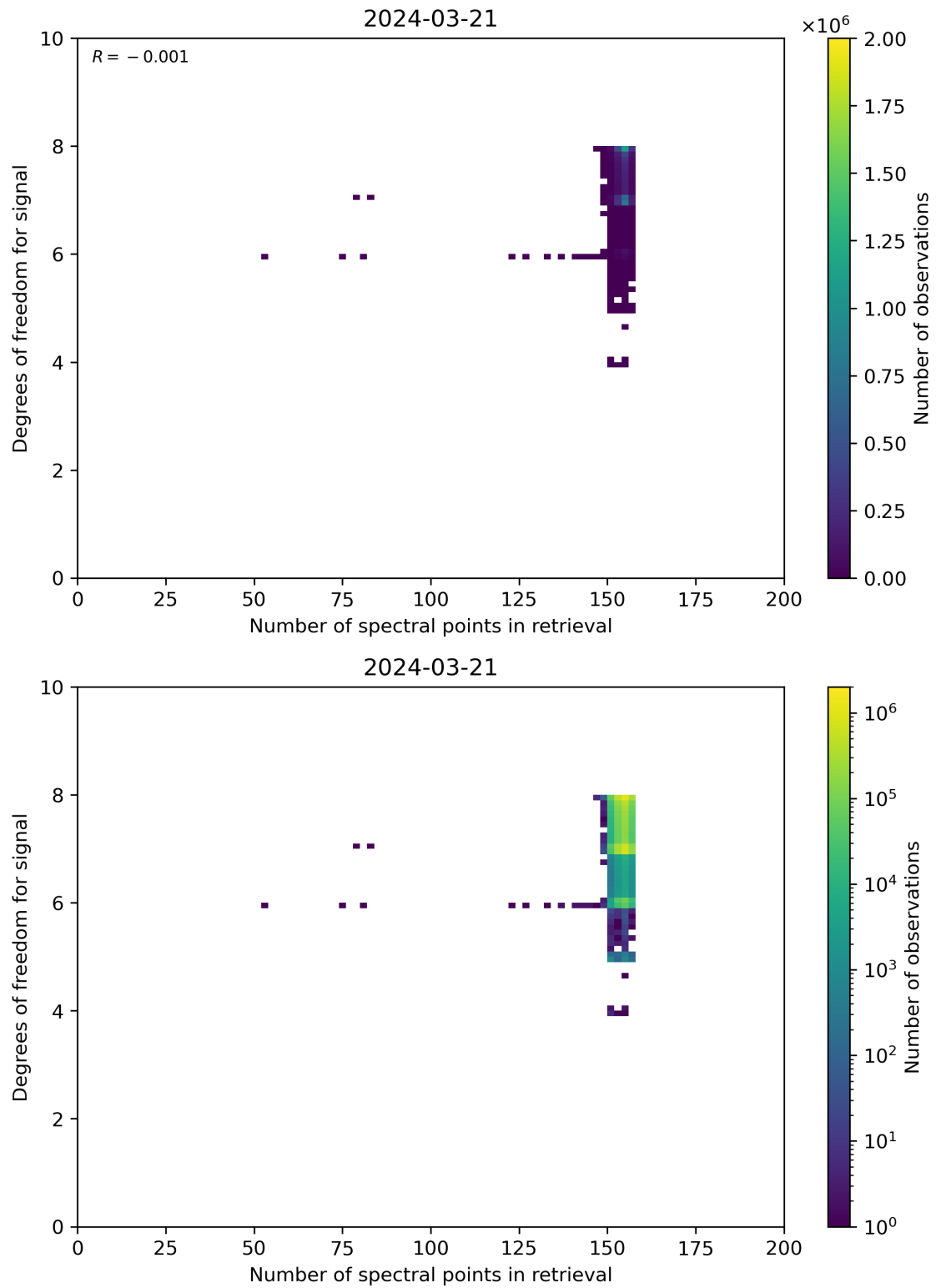
Figure 59: Scatter density plot of “Number of spectral points in retrieval” against “Degrees of freedom for signal” for 2024-03-20 to 2024-03-22.
