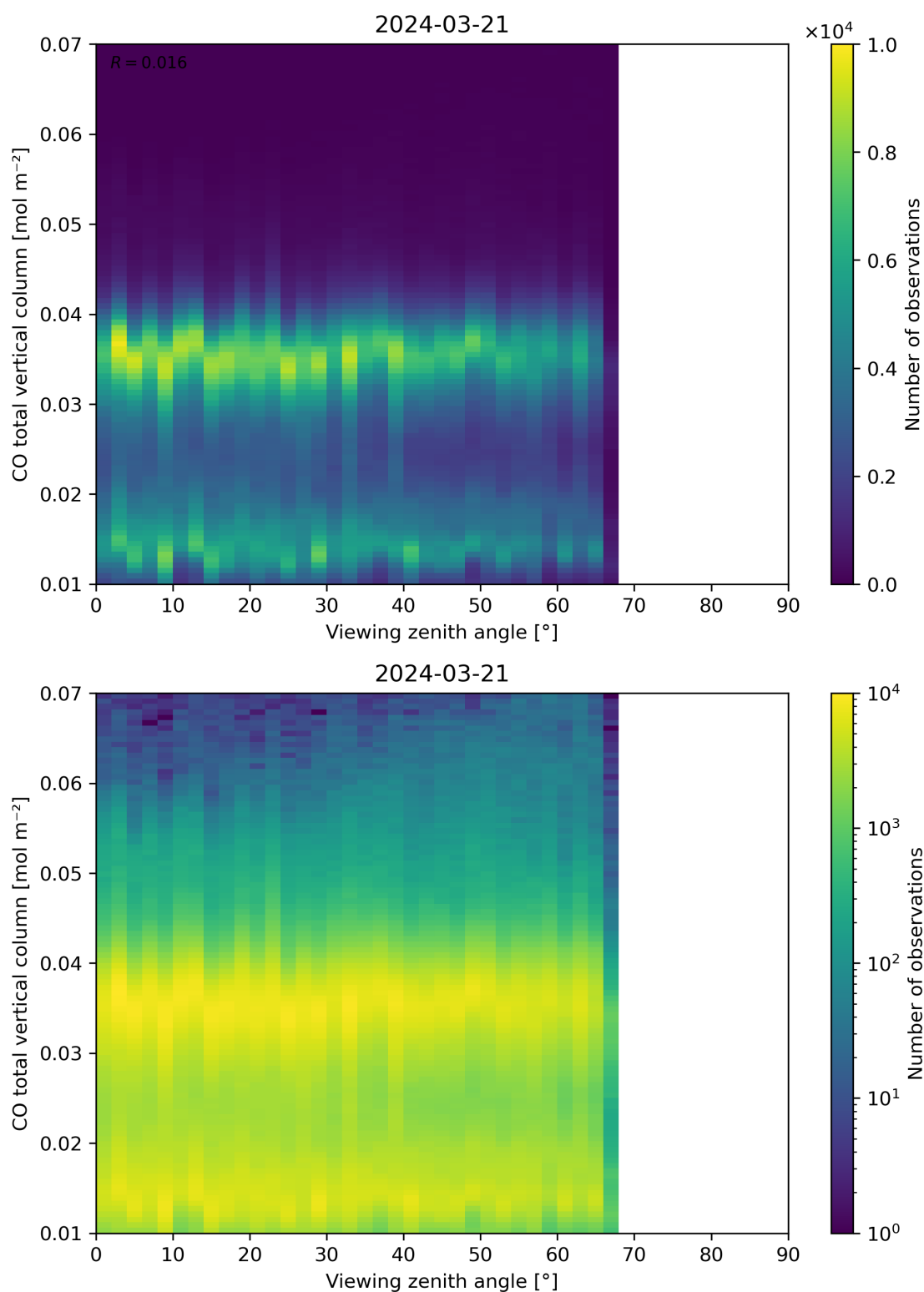
Figure 69: Scatter density plot of “Viewing zenith angle” against “CO total vertical column” for 2024-03-20 to 2024-03-22.
