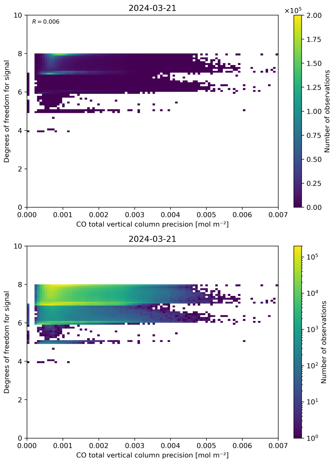
Figure 45: Scatter density plot of “CO total vertical column precision” against “Degrees of freedom for signal” for 2024-03-20 to 2024-03-22.
