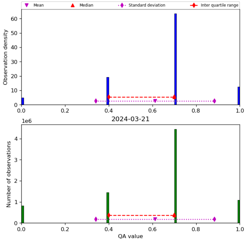
Figure 17: Histogram of “QA value” for 2024-03-20 to 2024-03-22
