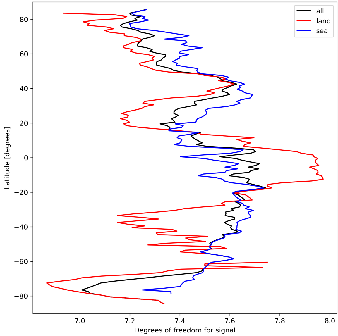
Figure 15: Zonal average of “Degrees of freedom for signal” for 2024-03-20 to 2024-03-22.
