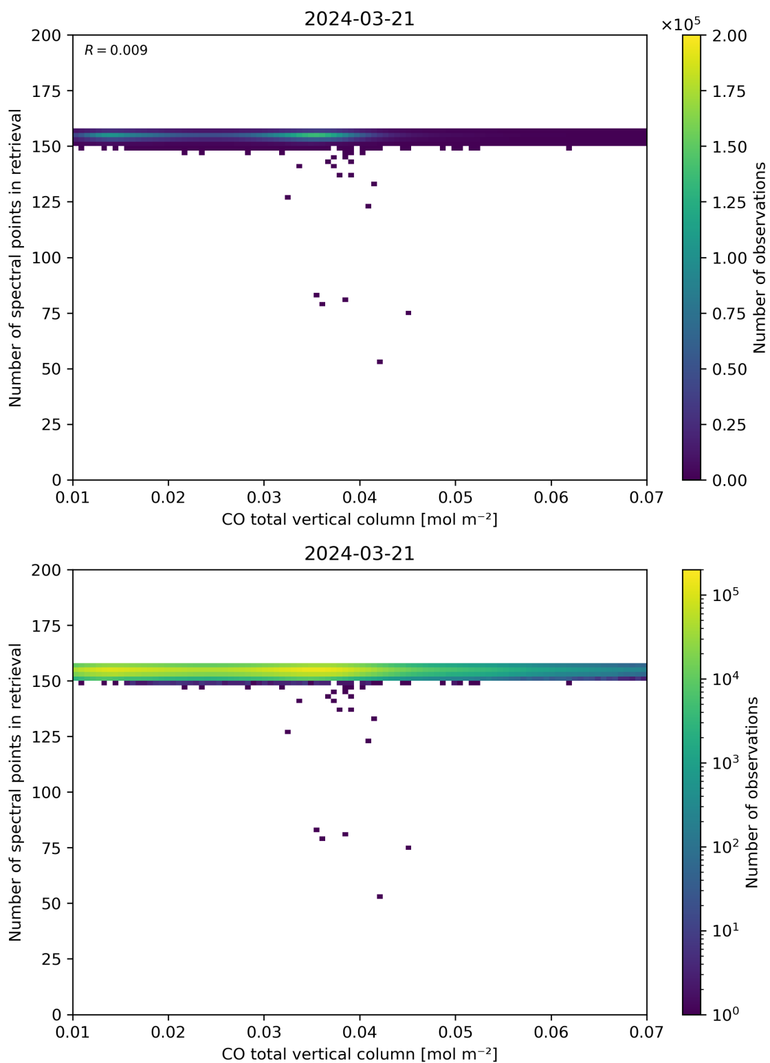
Figure 43: Scatter density plot of “CO total vertical column” against “Number of spectral points in retrieval” for 2024-03-20 to 2024-03-22.
