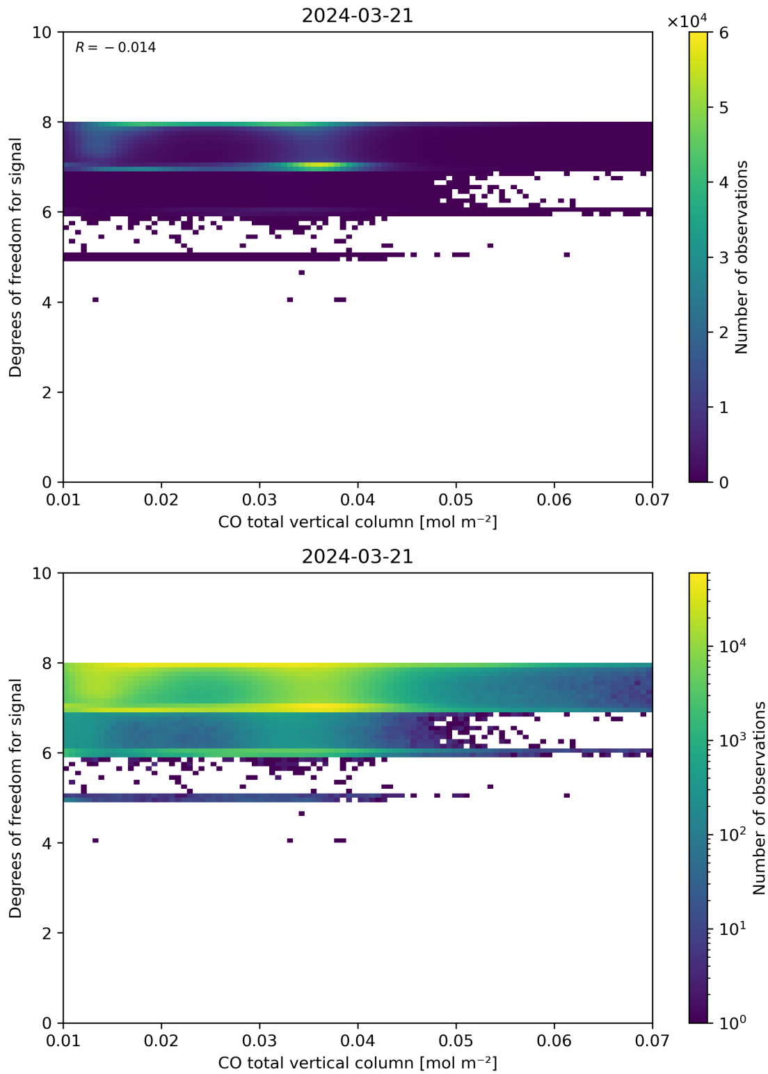
Figure 41: Scatter density plot of “CO total vertical column” against “Degrees of freedom for signal” for 2024-03-20 to 2024-03-22.
