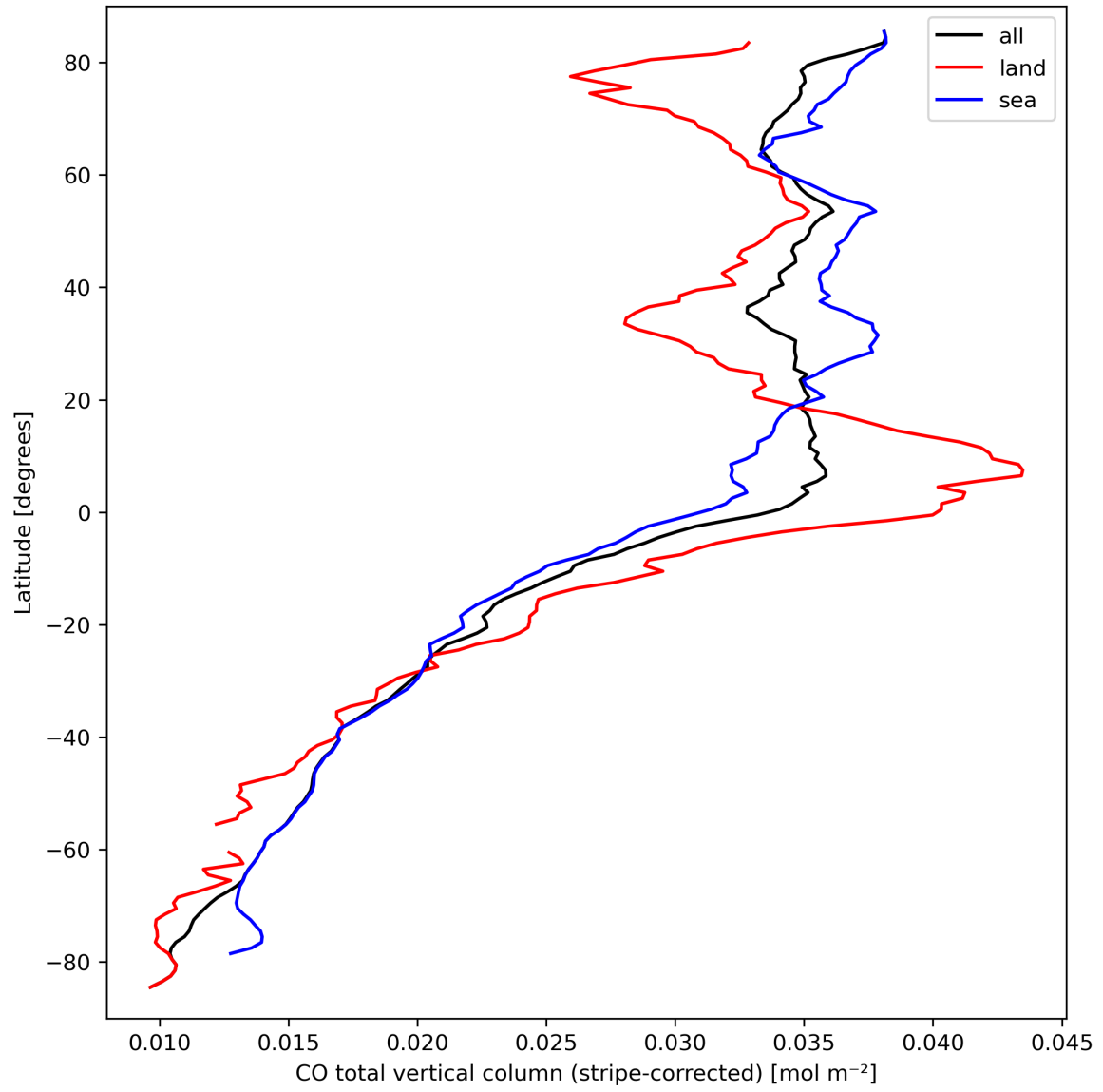
Figure 11: Zonal average of “CO total vertical column (stripe-corrected)” for 2024-03-20 to 2024-03-22.
