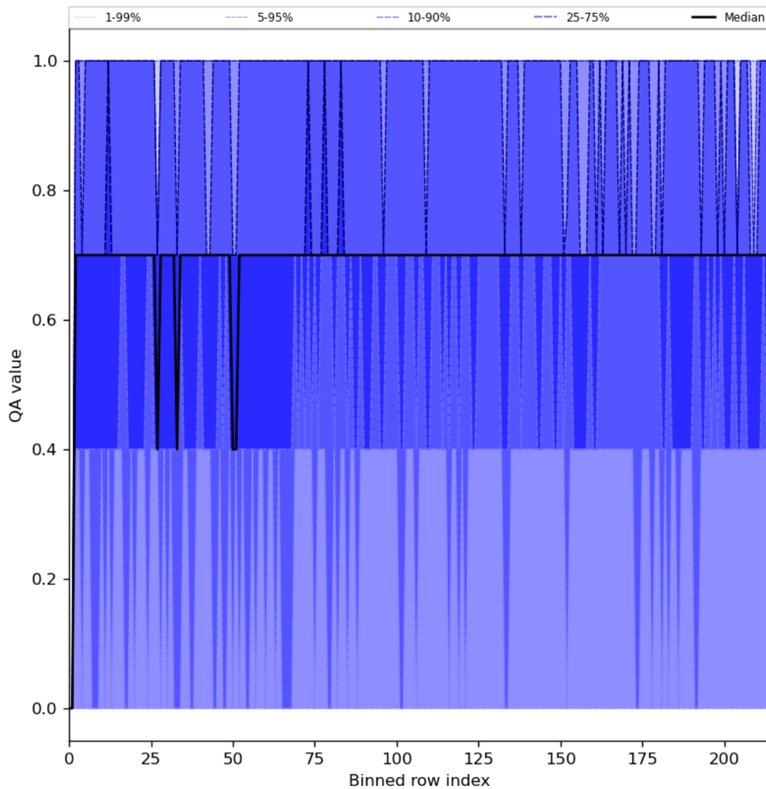
Figure 25: Along track statistics of “QA value” for 2024-03-20 to 2024-03-22
