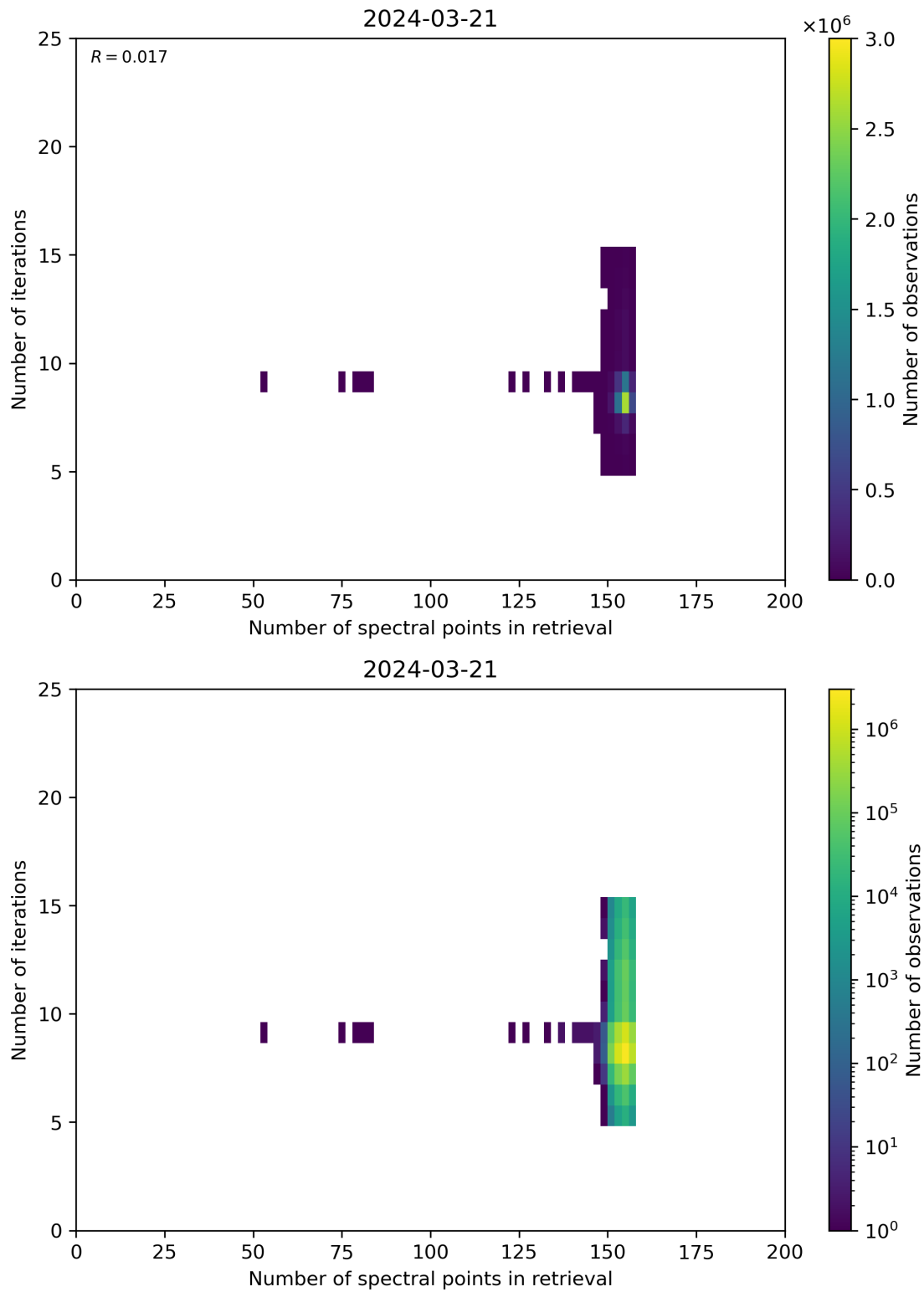
Figure 60: Scatter density plot of “Number of spectral points in retrieval” against “Number of iterations” for 2024-03-20 to 2024-03-22.
