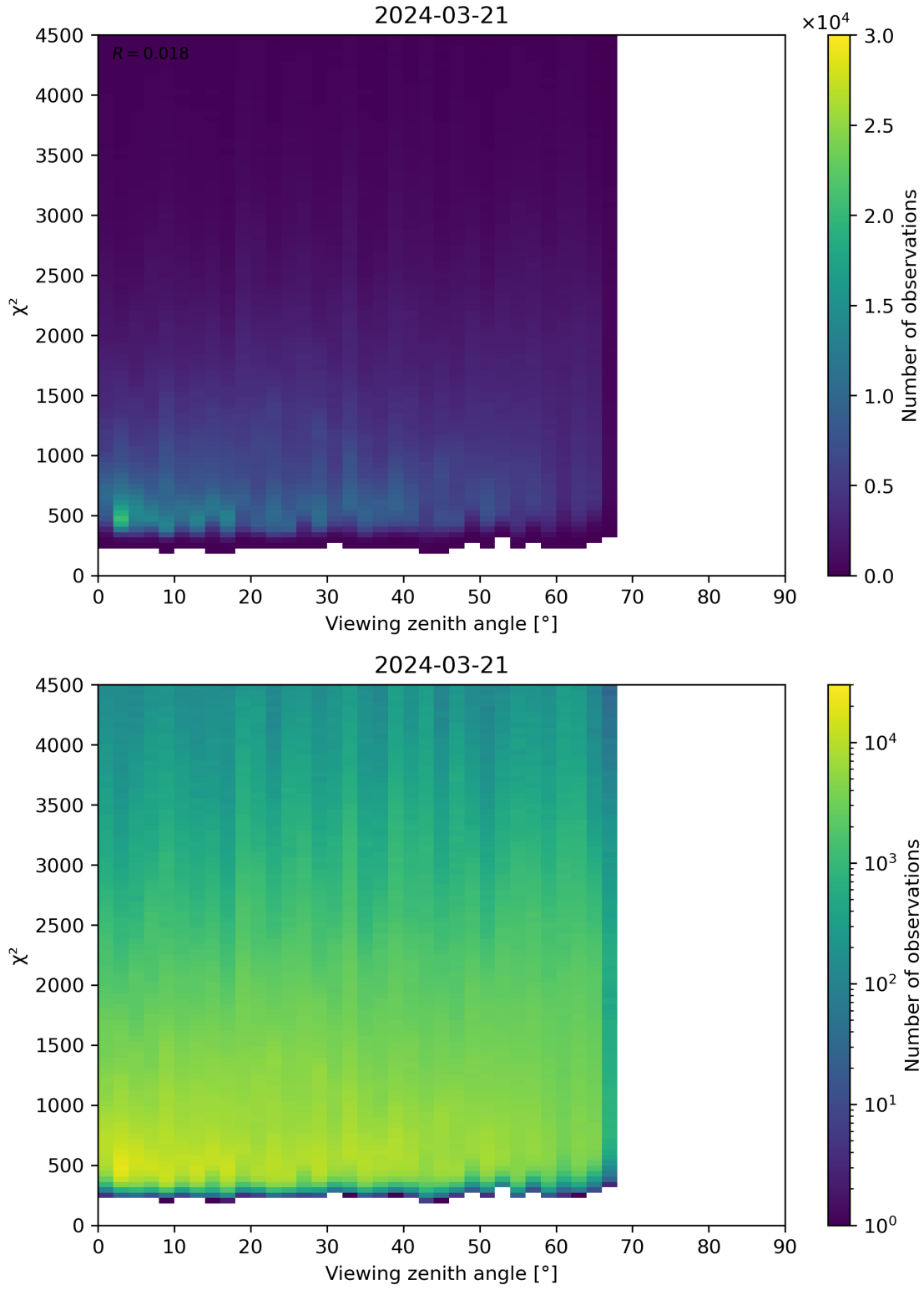
Figure 72: Scatter density plot of “Viewing zenith angle” against “ \chi^2 ” for 2024-03-20 to 2024-03-22.
