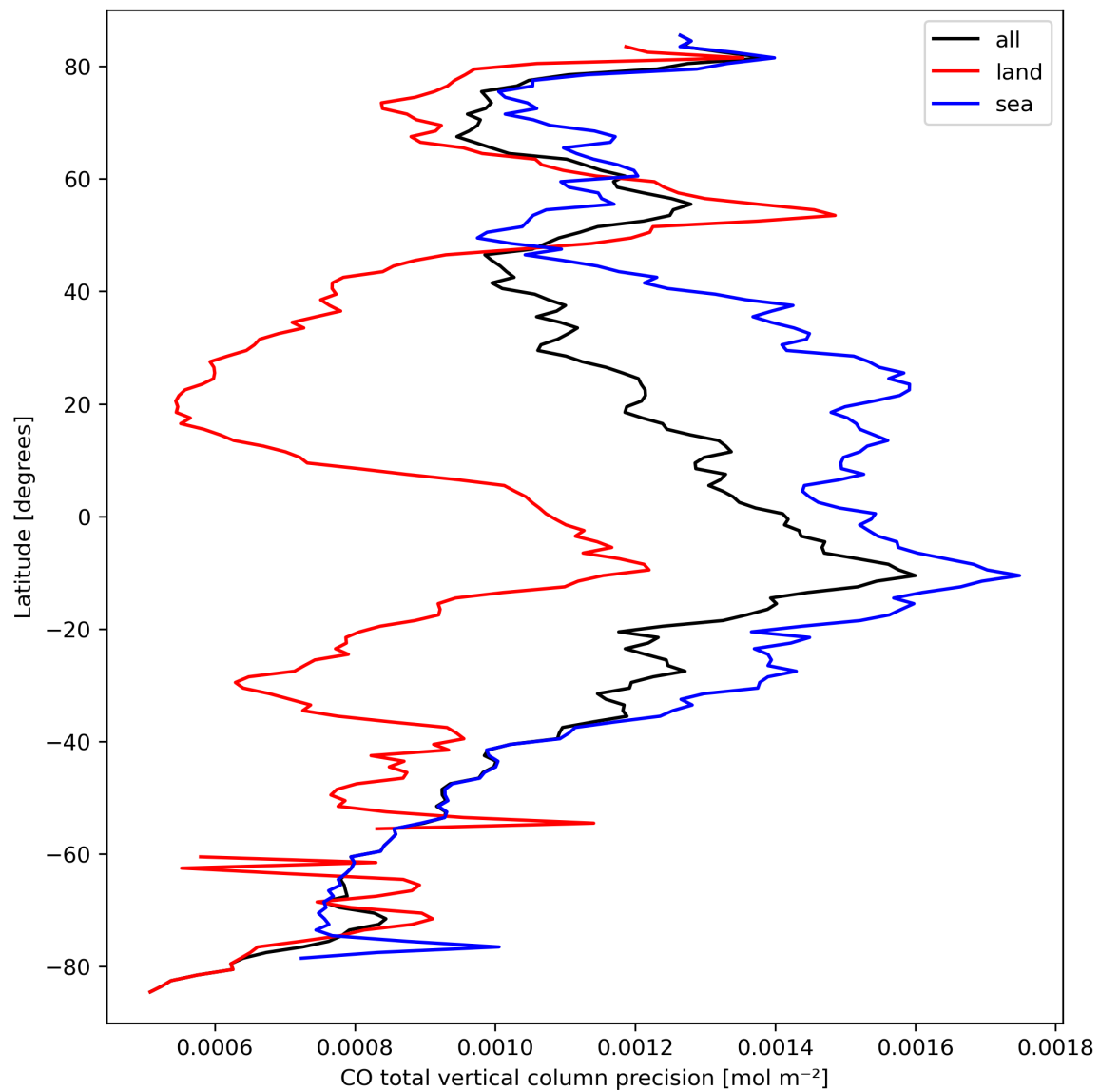
Figure 12: Zonal average of “CO total vertical column precision” for 2024-03-20 to 2024-03-22.
