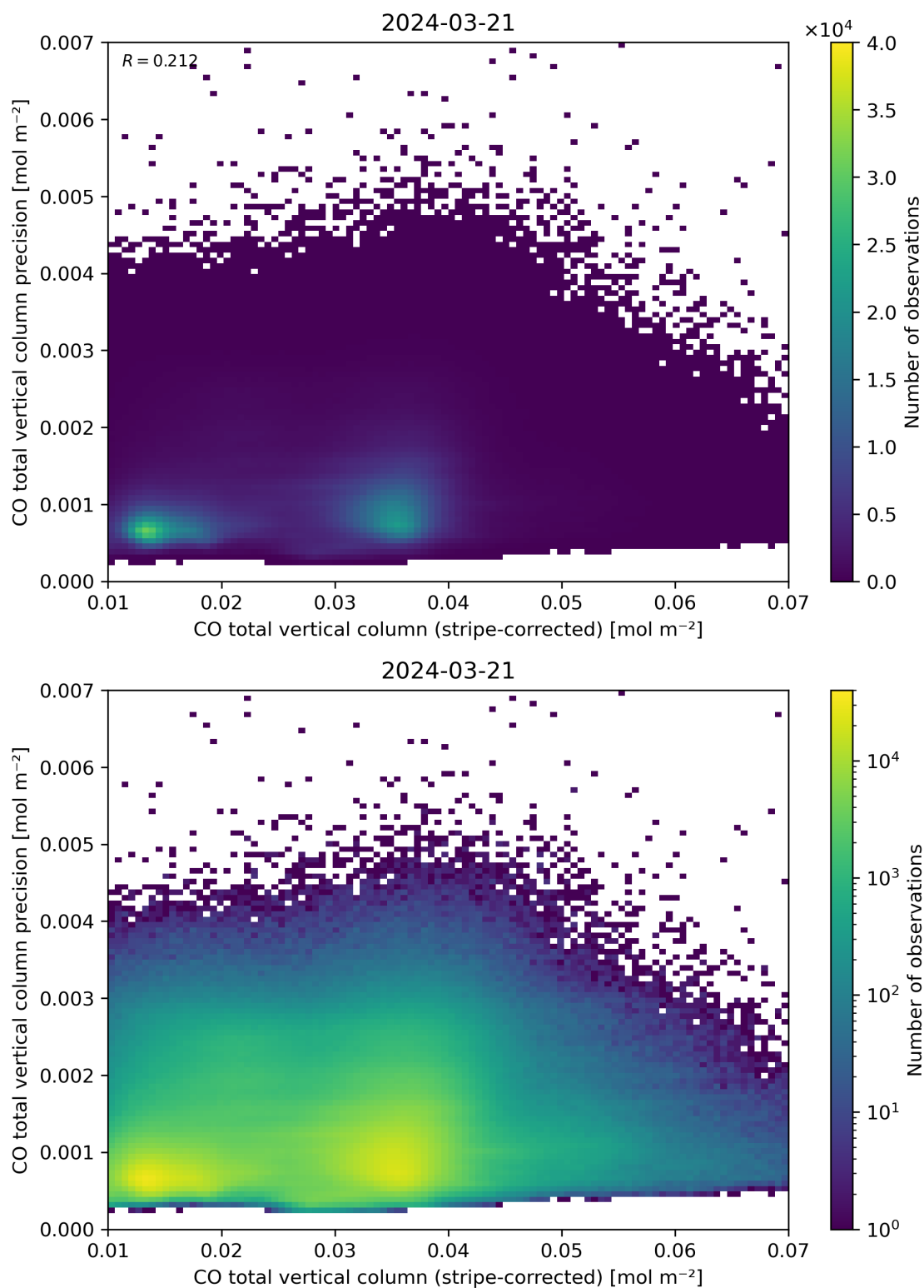
Figure 36: Scatter density plot of “CO total vertical column (stripe-corrected)” against “CO total vertical column precision” for 2024-03-20 to 2024-03-22.
