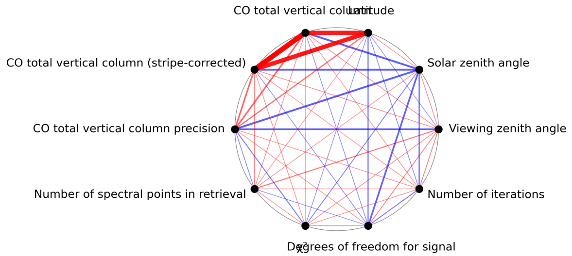
Figure 1: Map of correlation graph for 2024-03-20 to 2024-03-22.
