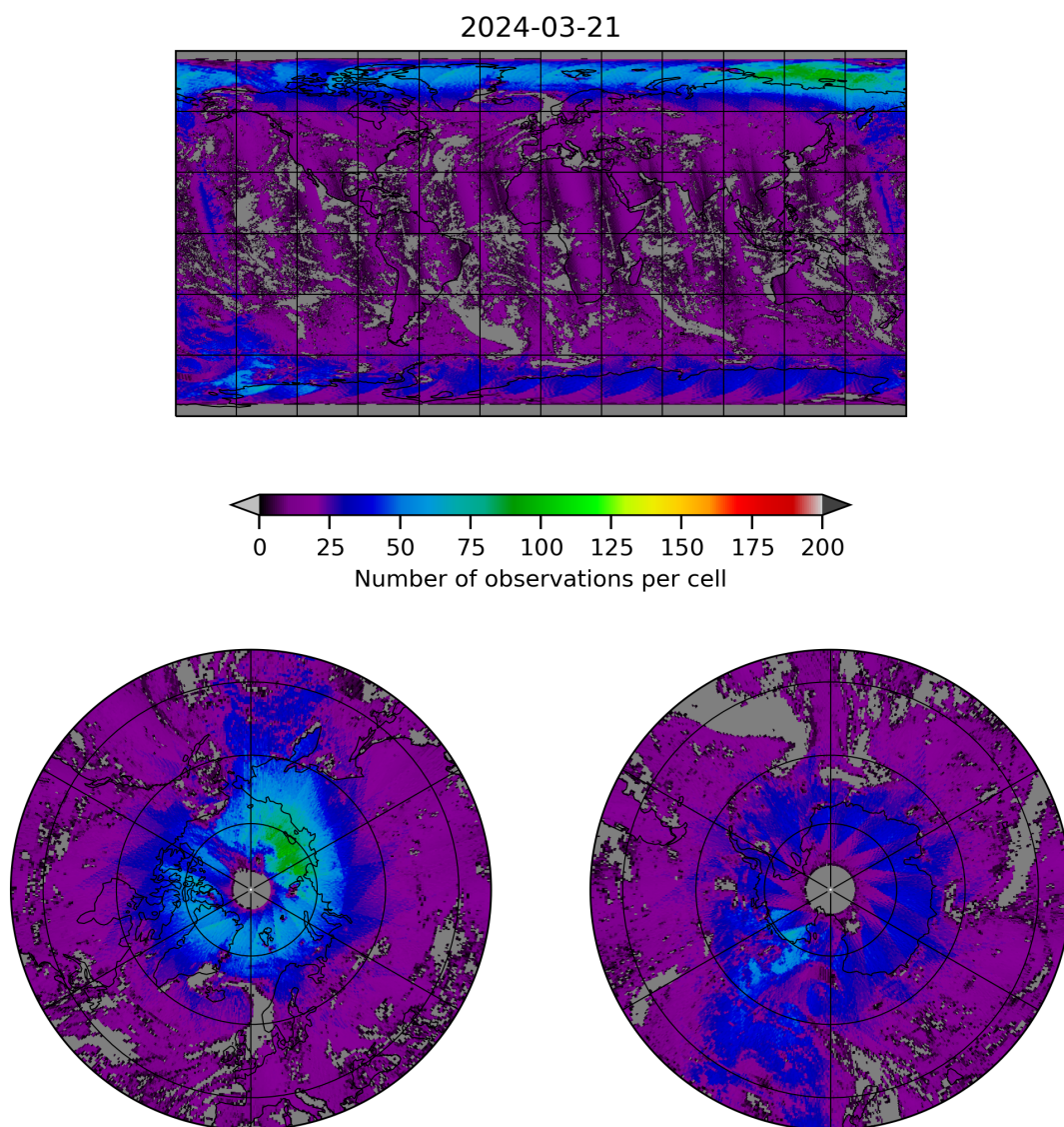
Figure 8: Map of the number of observations for 2024-03-20 to 2024-03-22
