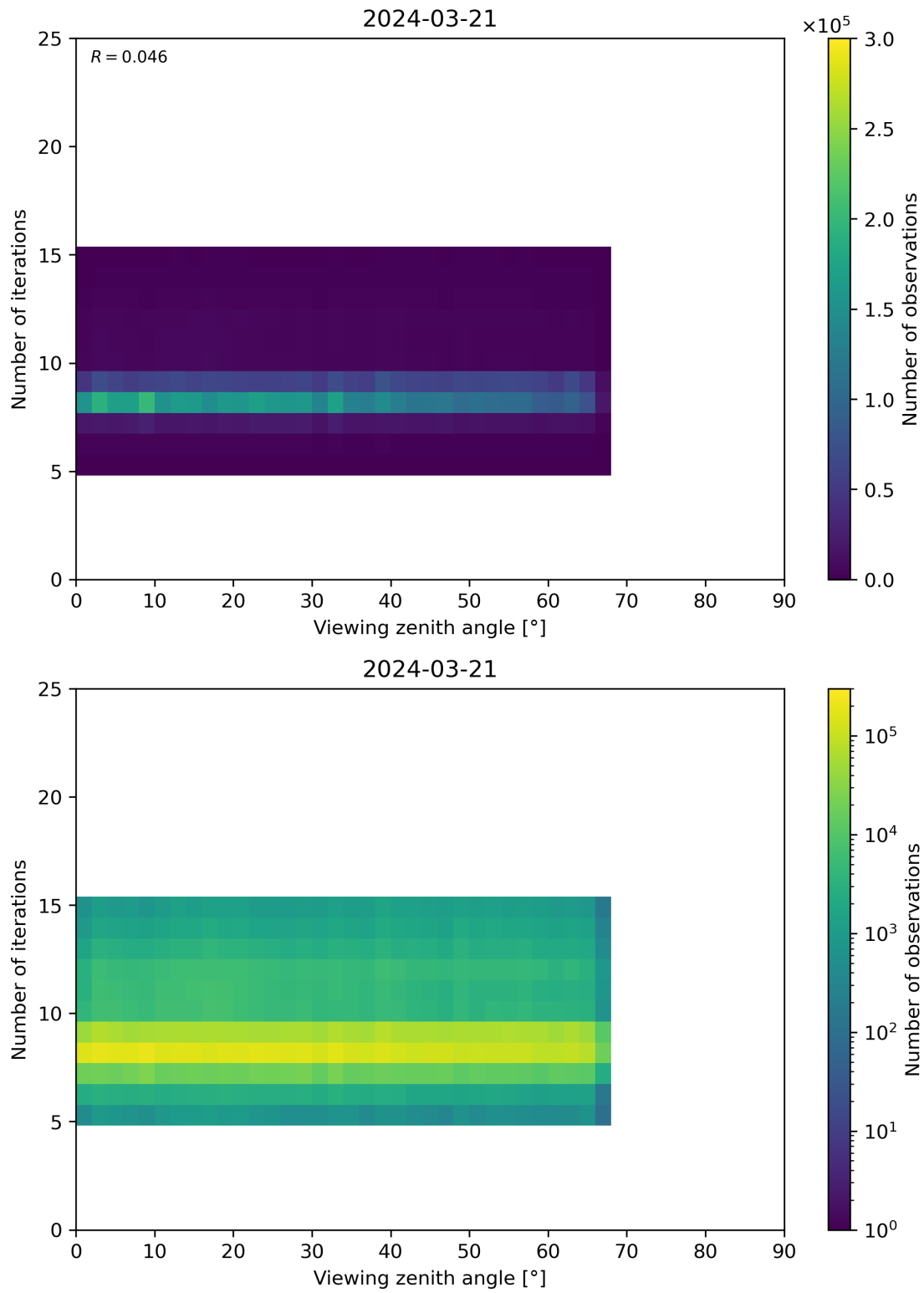
Figure 75: Scatter density plot of “Viewing zenith angle” against “Number of iterations” for 2024-03-20 to 2024-03-22.
