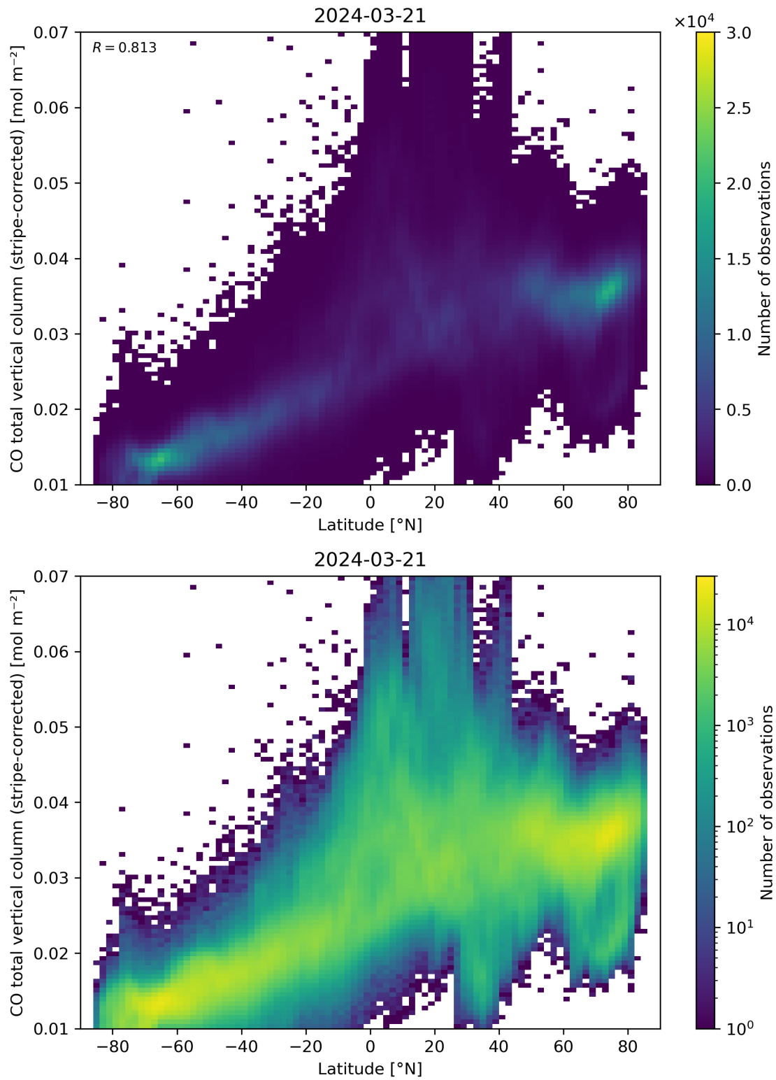
Figure 52: Scatter density plot of “Latitude” against “CO total vertical column (stripe-corrected)” for 2024-03-20 to 2024-03-22.
