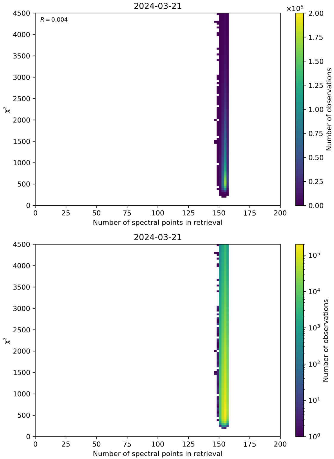
Figure 58: Scatter density plot of “Number of spectral points in retrieval” against “ \chi^2 ” for 2024-03-20 to 2024-03-22.
