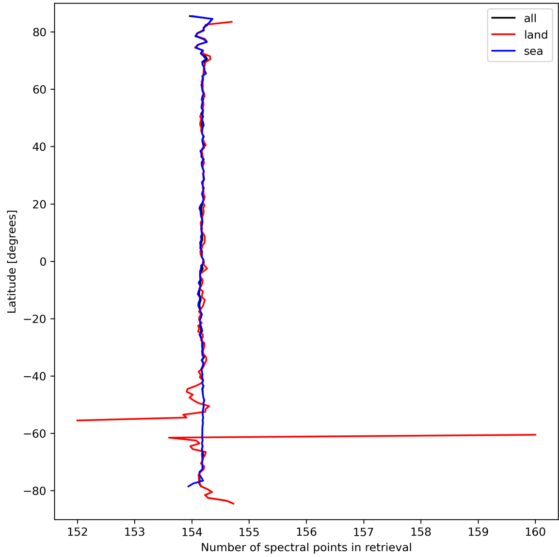
Figure 13: Zonal average of “Number of spectral points in retrieval” for 2024-03-20 to 2024-03-22.
