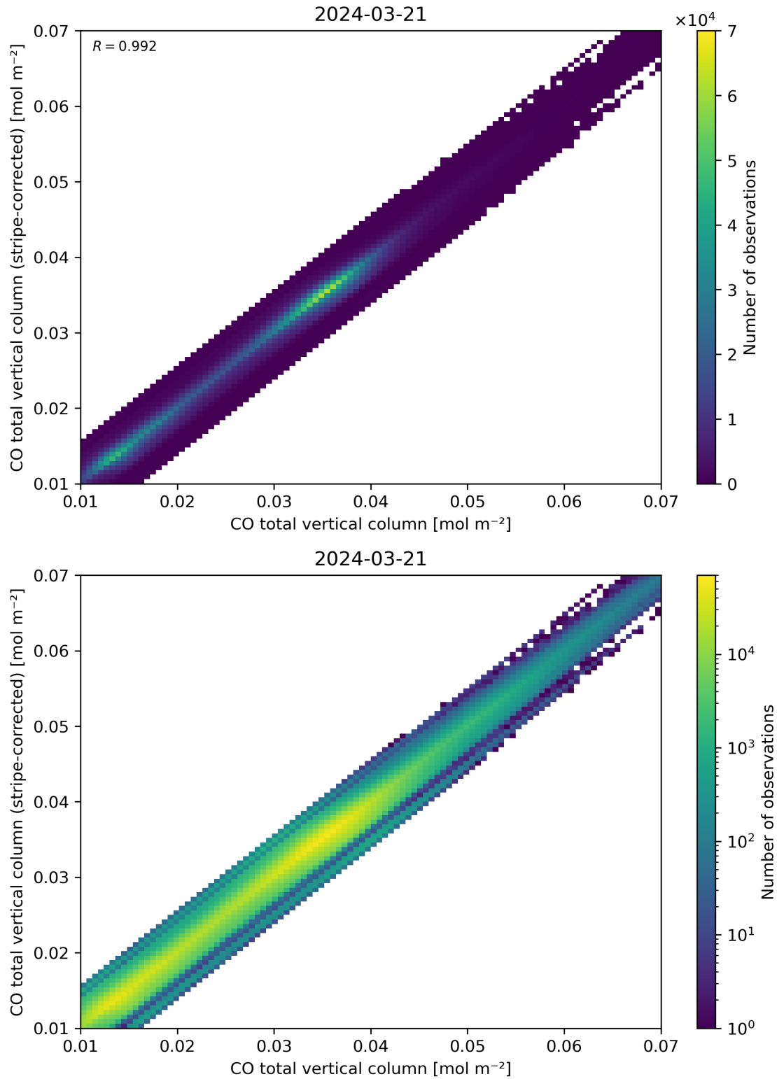
Figure 33: Scatter density plot of “CO total vertical column” against “CO total vertical column (stripe-corrected)” for 2024-03-20 to 2024-03-22.
