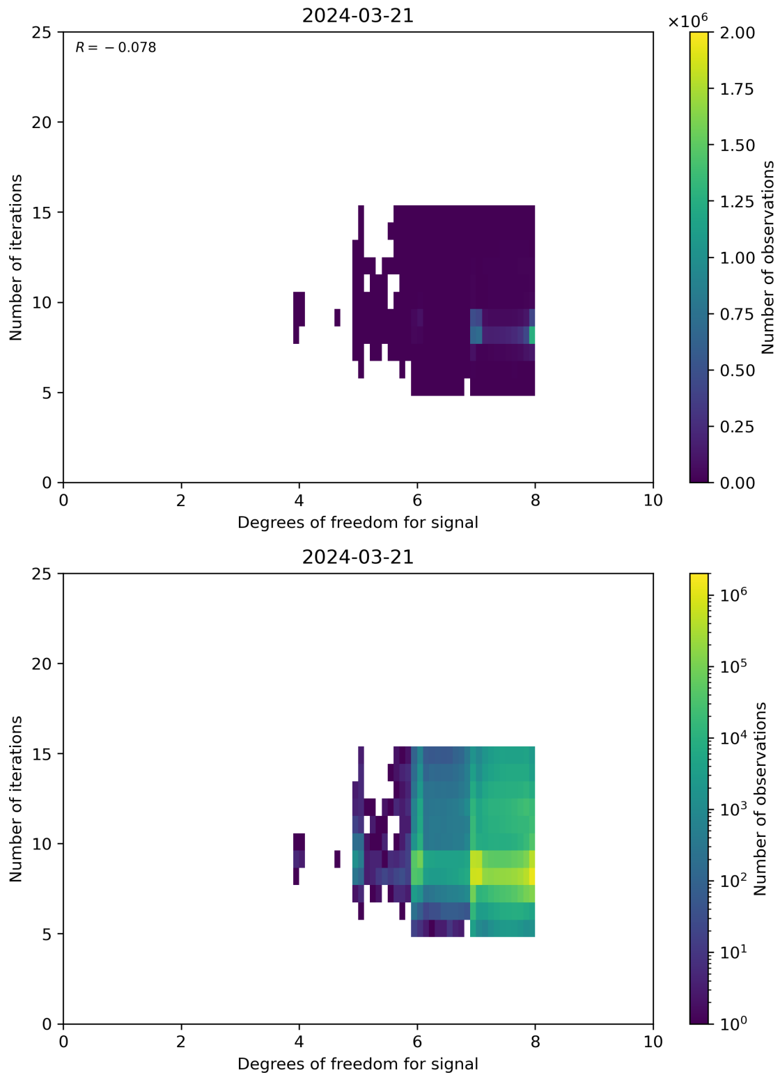
Figure 50: Scatter density plot of “Degrees of freedom for signal” against “Number of iterations” for 2024-03-20 to 2024-03-22.
