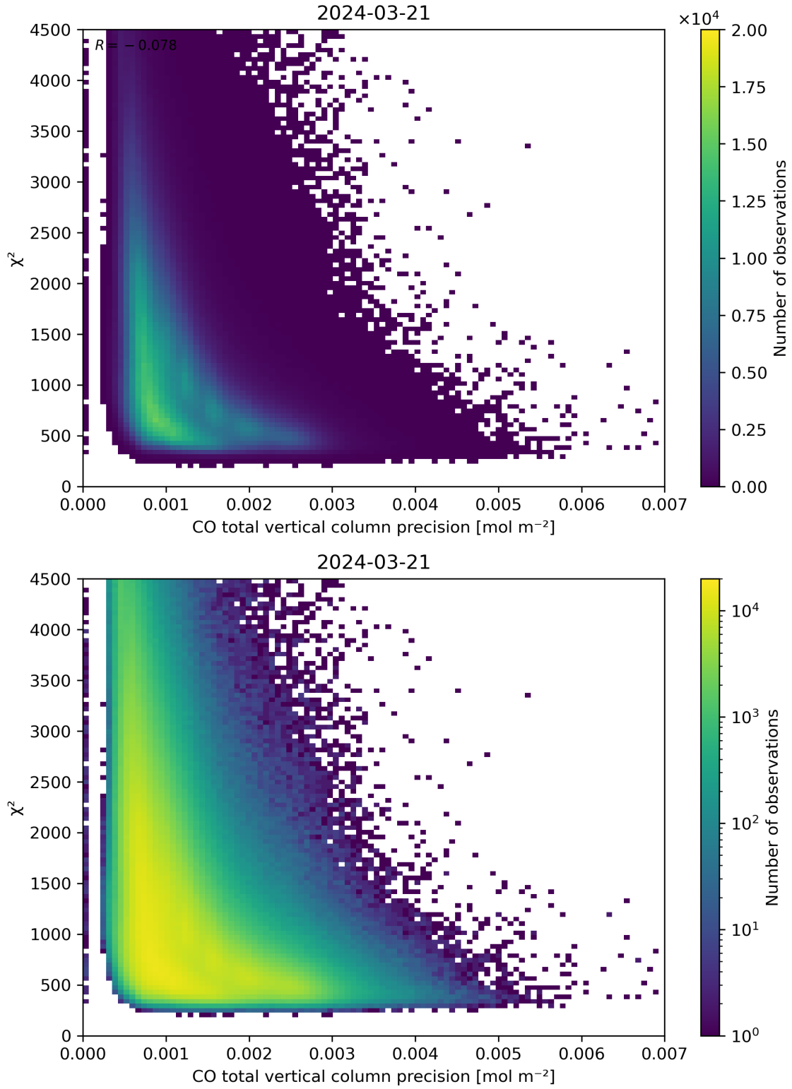
Figure 44: Scatter density plot of “CO total vertical column precision” against “ \chi^2 ” for 2024-03-20 to 2024-03-22.
