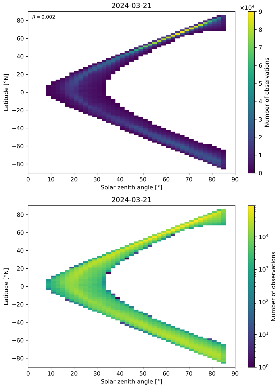
Figure 66: Scatter density plot of “Solar zenith angle” against “Latitude” for 2024-03-20 to 2024-03-22.
