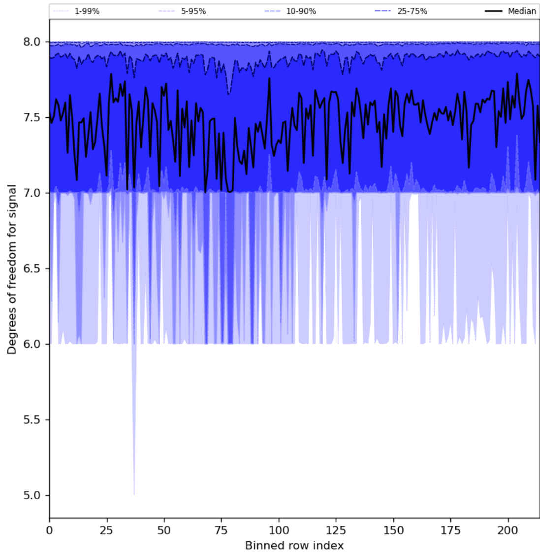
Figure 31: Along track statistics of “Degrees of freedom for signal” for 2024-03-20 to 2024-03-22
