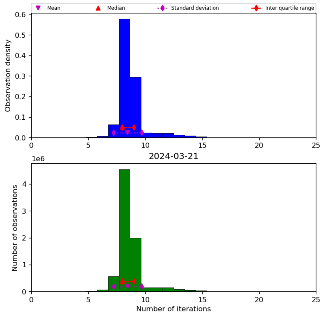
Figure 24: Histogram of “Number of iterations” for 2024-03-20 to 2024-03-22
