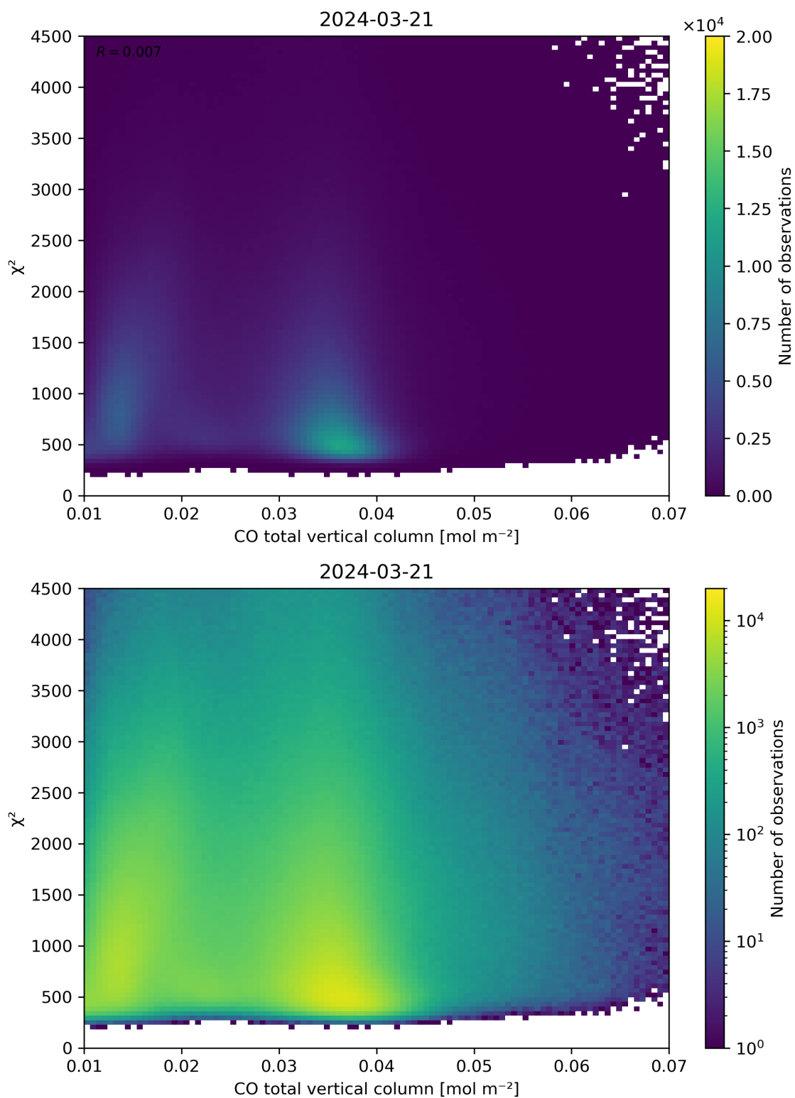
Figure 35: Scatter density plot of “CO total vertical column” against “ \chi^2 ” for 2024-03-20 to 2024-03-22.
