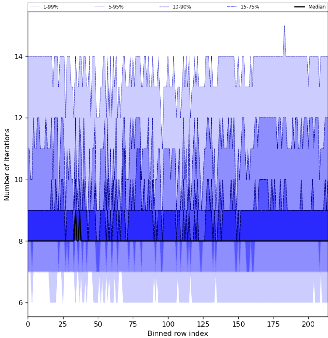
Figure 32: Along track statistics of “Number of iterations” for 2024-03-20 to 2024-03-22
