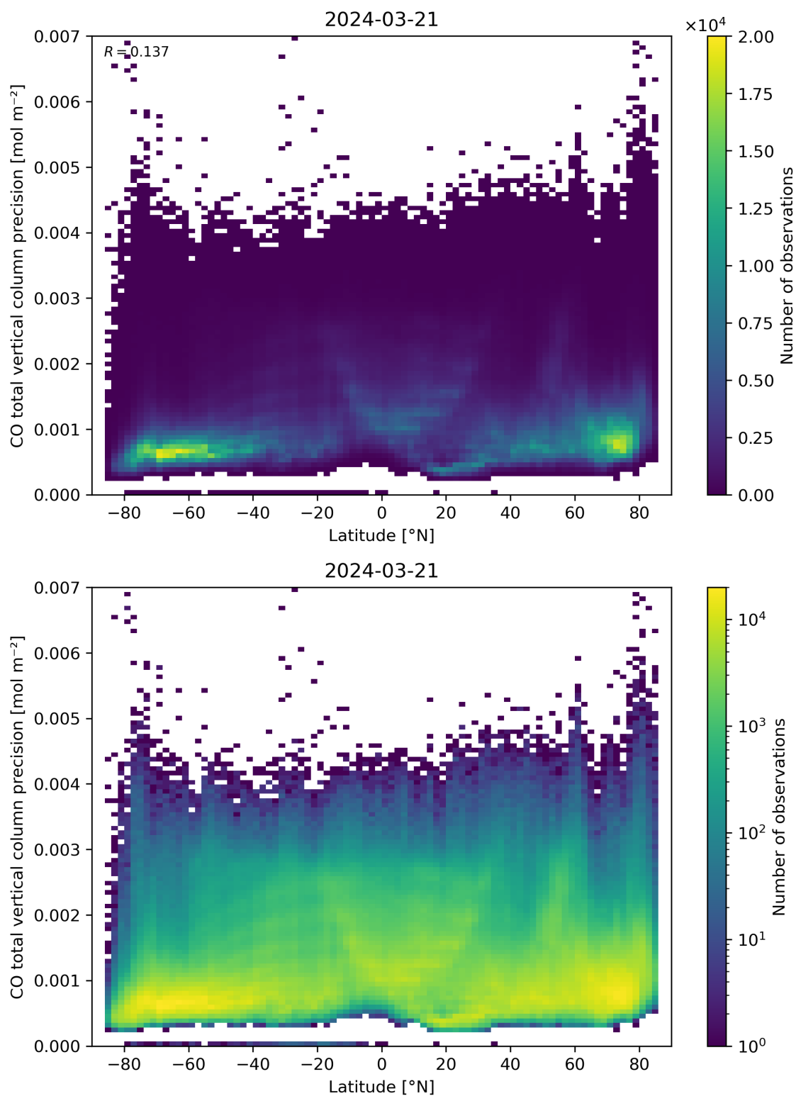
Figure 53: Scatter density plot of “Latitude” against “CO total vertical column precision” for 2024-03-20 to 2024-03-22.
