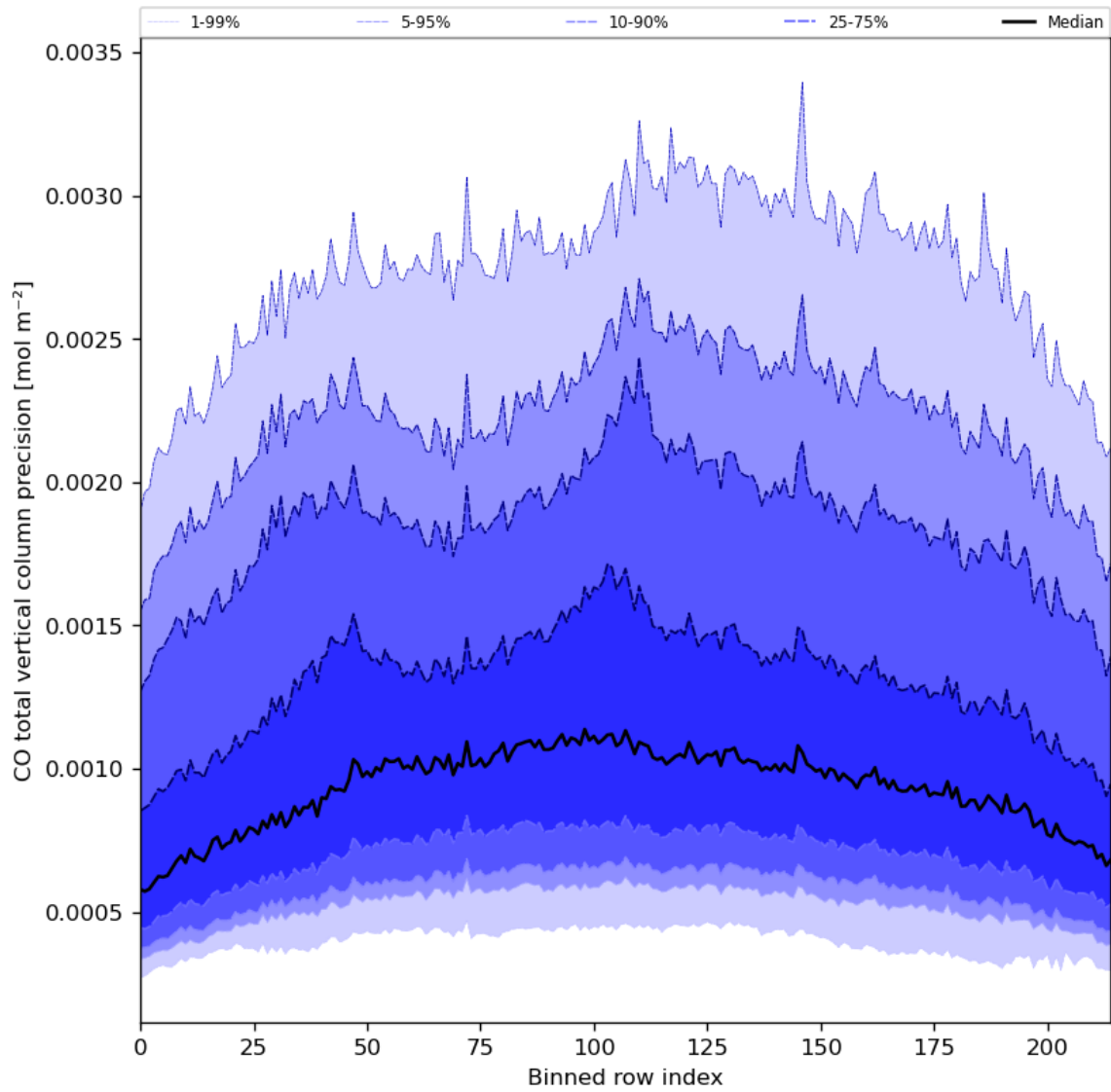
Figure 28: Along track statistics of “CO total vertical column precision” for 2024-03-20 to 2024-03-22
