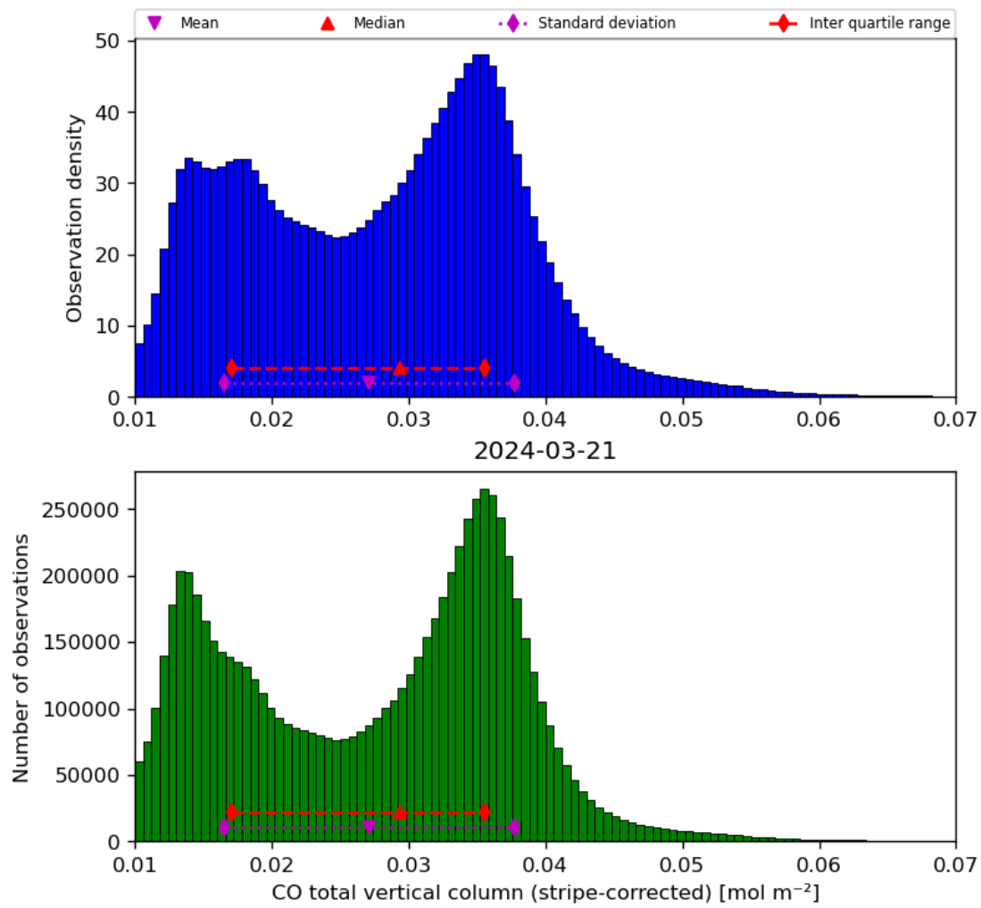
Figure 19: Histogram of “CO total vertical column (stripe-corrected)” for 2024-03-20 to 2024-03-22
