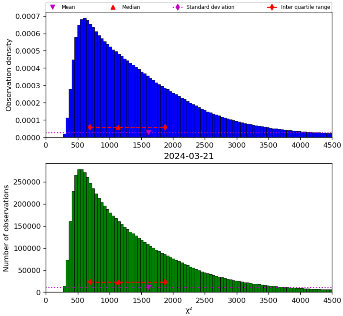
Figure 22: Histogram of “ \chi^2 ” for 2024-03-20 to 2024-03-22
