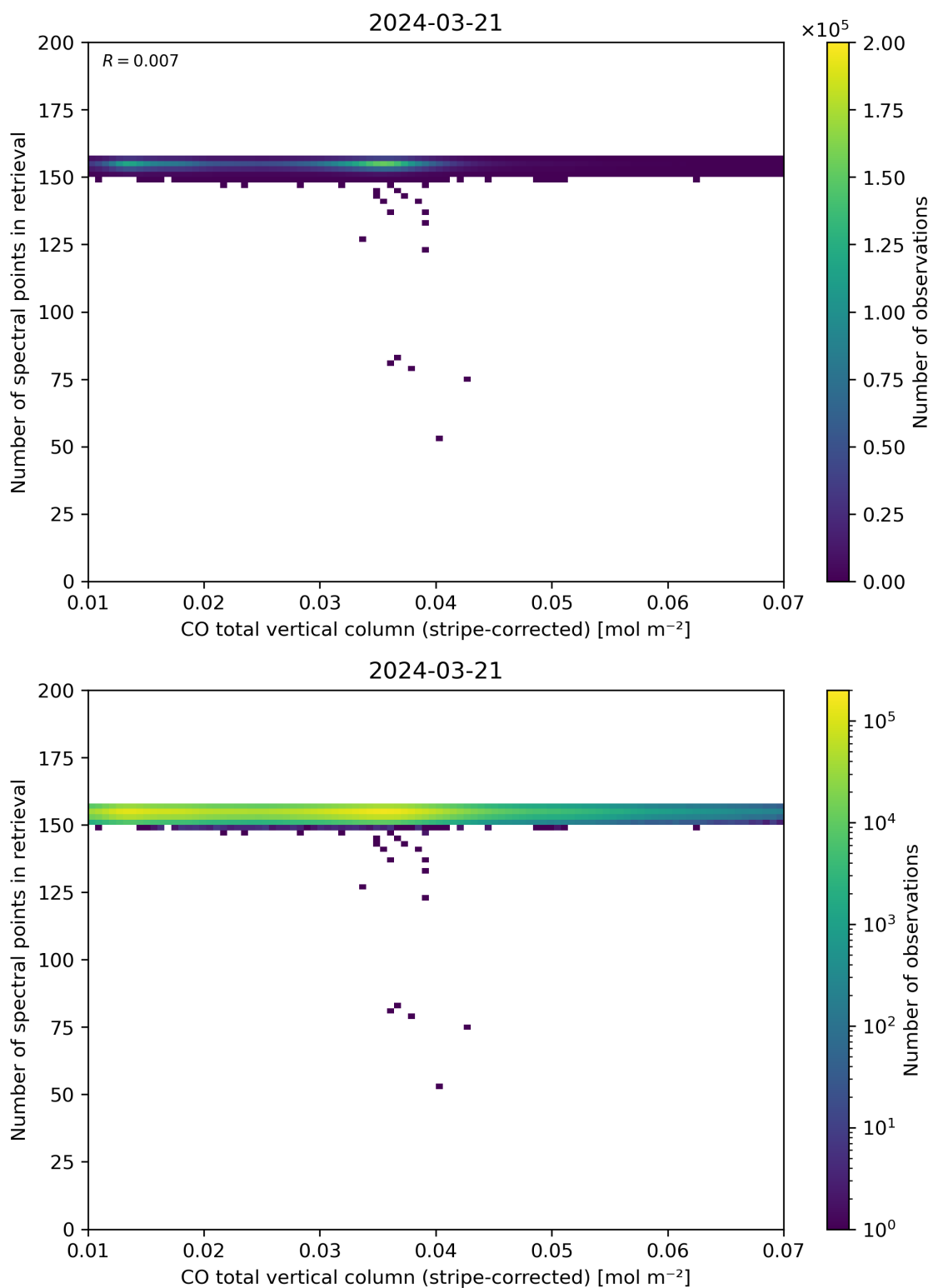
Figure 40: Scatter density plot of “CO total vertical column (stripe-corrected)” against “Number of spectral points in retrieval” for 2024-03-20 to 2024-03-22.
