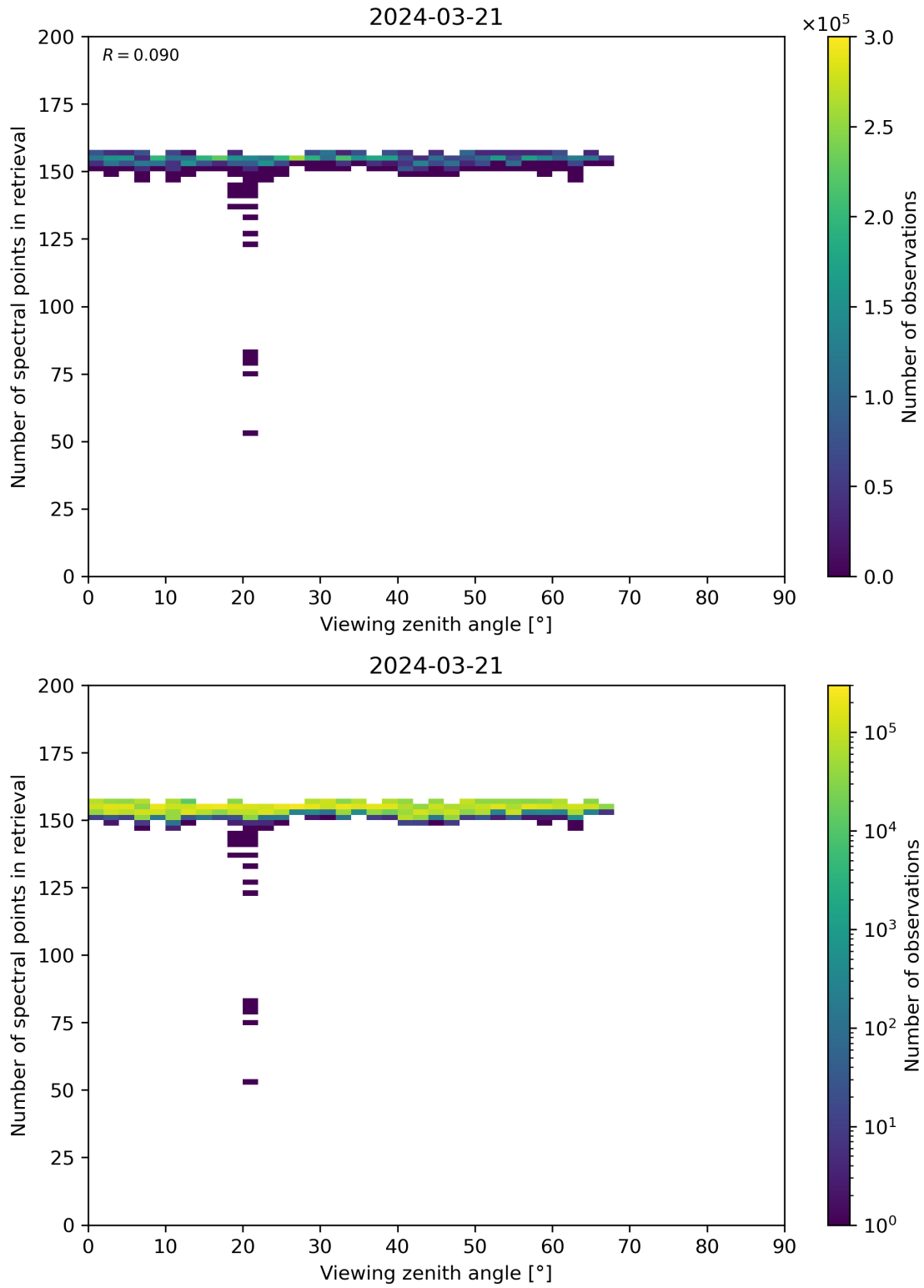
Figure 76: Scatter density plot of “Viewing zenith angle” against “Number of spectral points in retrieval” for 2024-03-20 to 2024-03-22.
