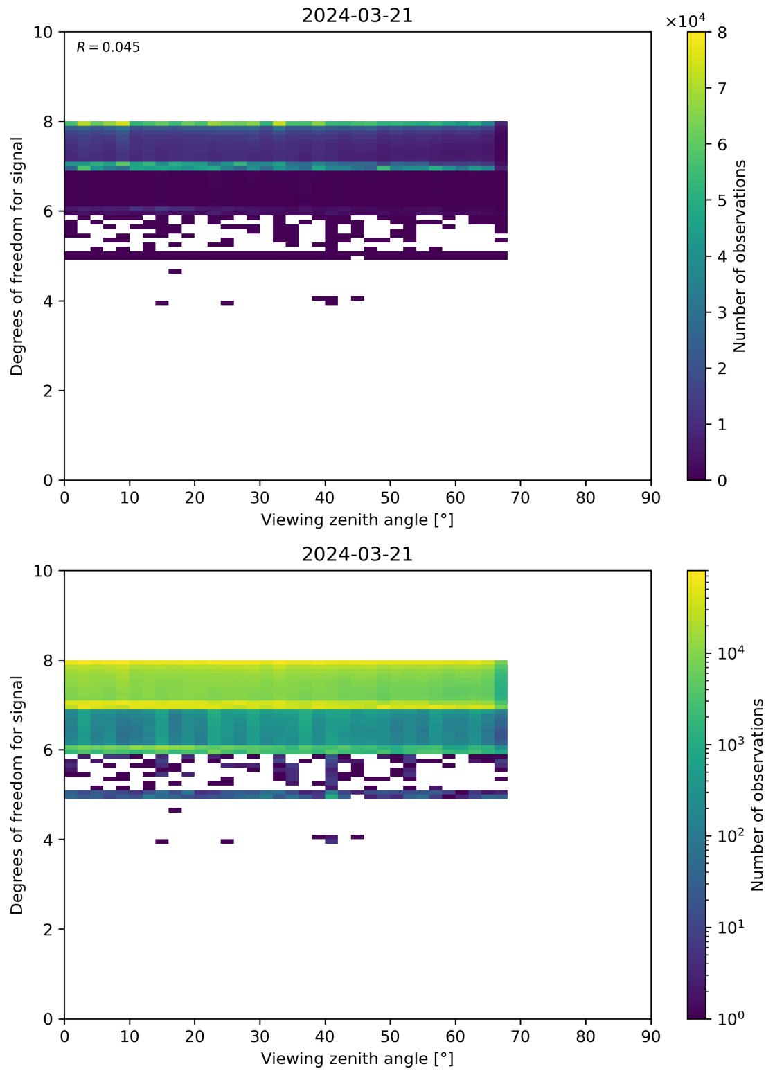
Figure 73: Scatter density plot of “Viewing zenith angle” against “Degrees of freedom for signal” for 2024-03-20 to 2024-03-22.
