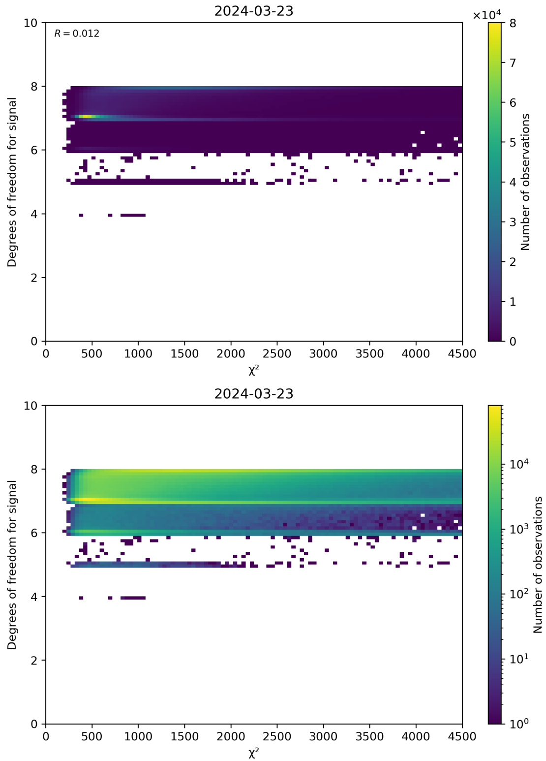
Figure 48: Scatter density plot of “ \chi^2 ” against “Degrees of freedom for signal” for 2024-03-23 to 2024-03-24.
