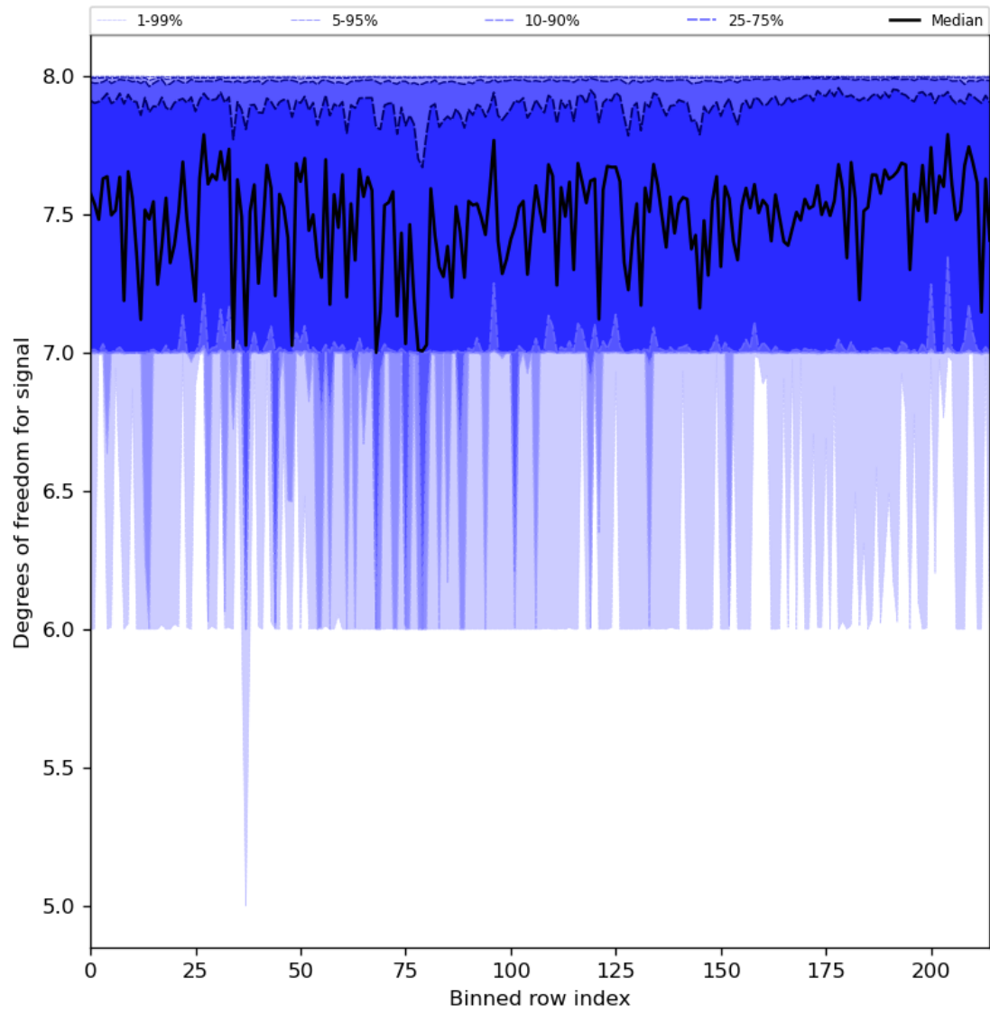
Figure 31: Along track statistics of “Degrees of freedom for signal” for 2024-03-23 to 2024-03-24
