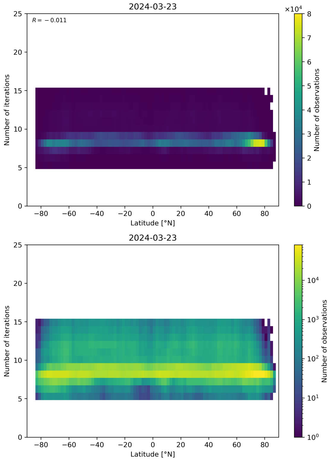
Figure 56: Scatter density plot of “Latitude” against “Number of iterations” for 2024-03-23 to 2024-03-24.
