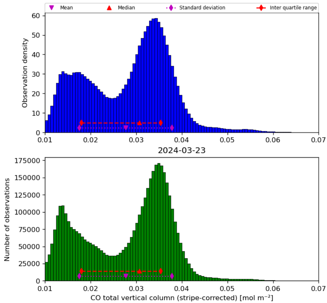
Figure 19: Histogram of “CO total vertical column (stripe-corrected)” for 2024-03-23 to 2024-03-24
