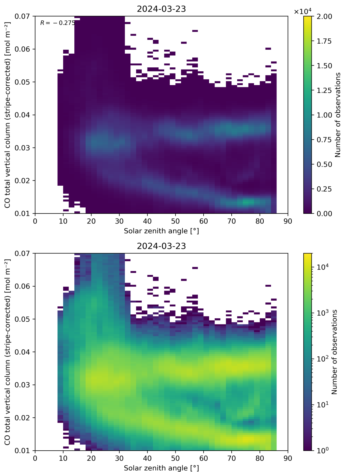
Figure 62: Scatter density plot of “Solar zenith angle” against “CO total vertical column (stripe-corrected)” for 2024-03-23 to 2024-03-24.
