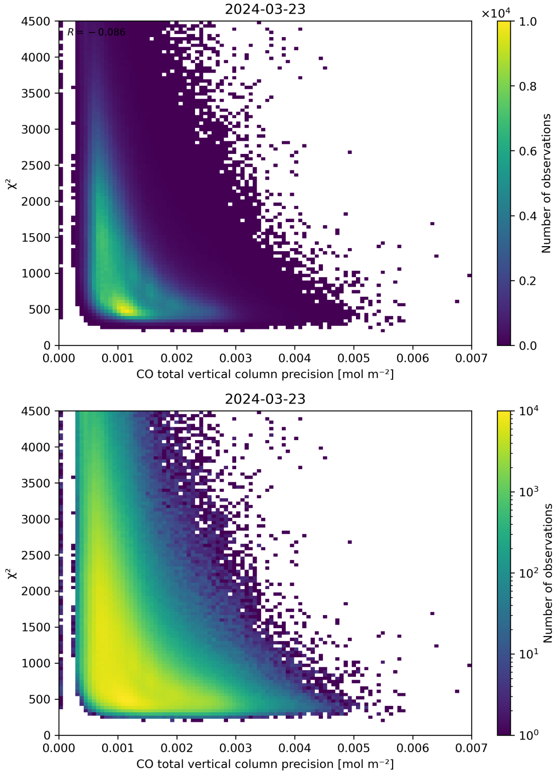
Figure 44: Scatter density plot of “CO total vertical column precision” against “ \chi^2 ” for 2024-03-23 to 2024-03-24.
