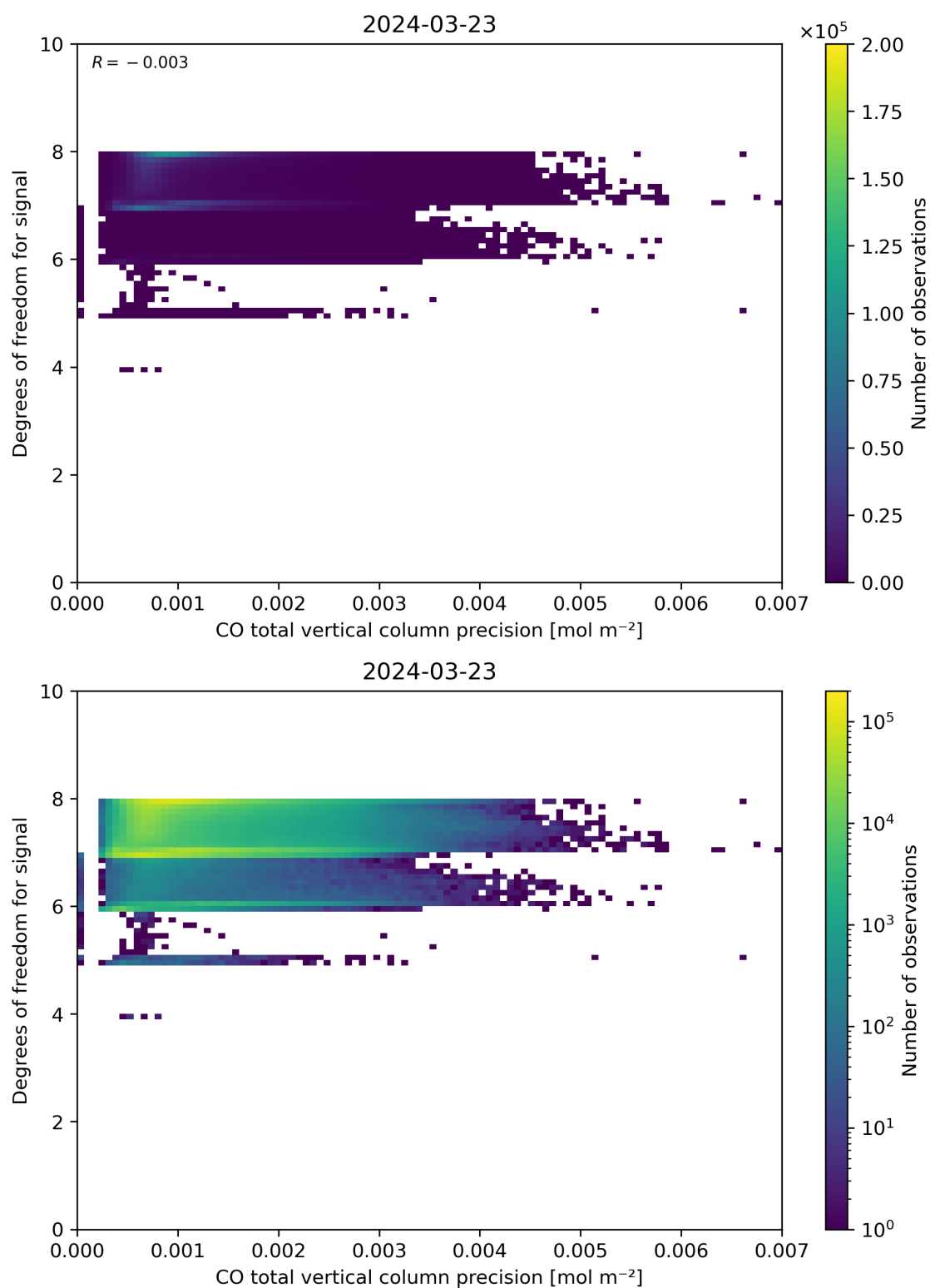
Figure 45: Scatter density plot of “CO total vertical column precision” against “Degrees of freedom for signal” for 2024-03-23 to 2024-03-24.
