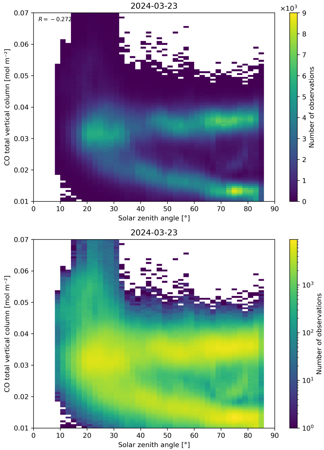
Figure 61: Scatter density plot of “Solar zenith angle” against “CO total vertical column” for 2024-03-23 to 2024-03-24.
