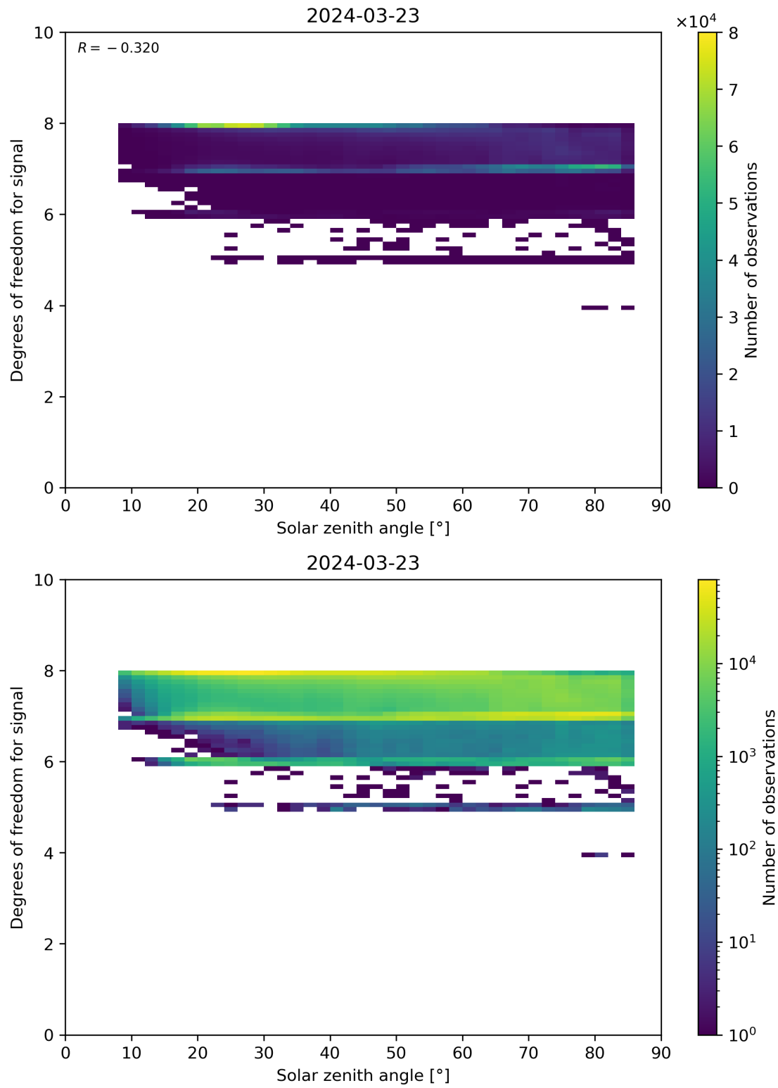
Figure 65: Scatter density plot of “Solar zenith angle” against “Degrees of freedom for signal” for 2024-03-23 to 2024-03-24.
