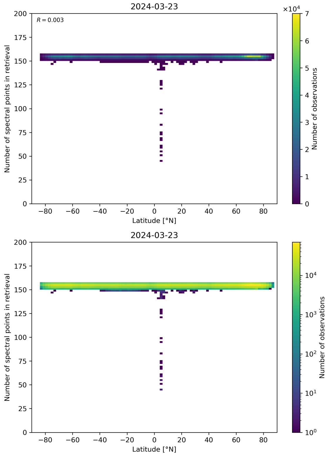
Figure 57: Scatter density plot of “Latitude” against “Number of spectral points in retrieval” for 2024-03-23 to 2024-03-24.
