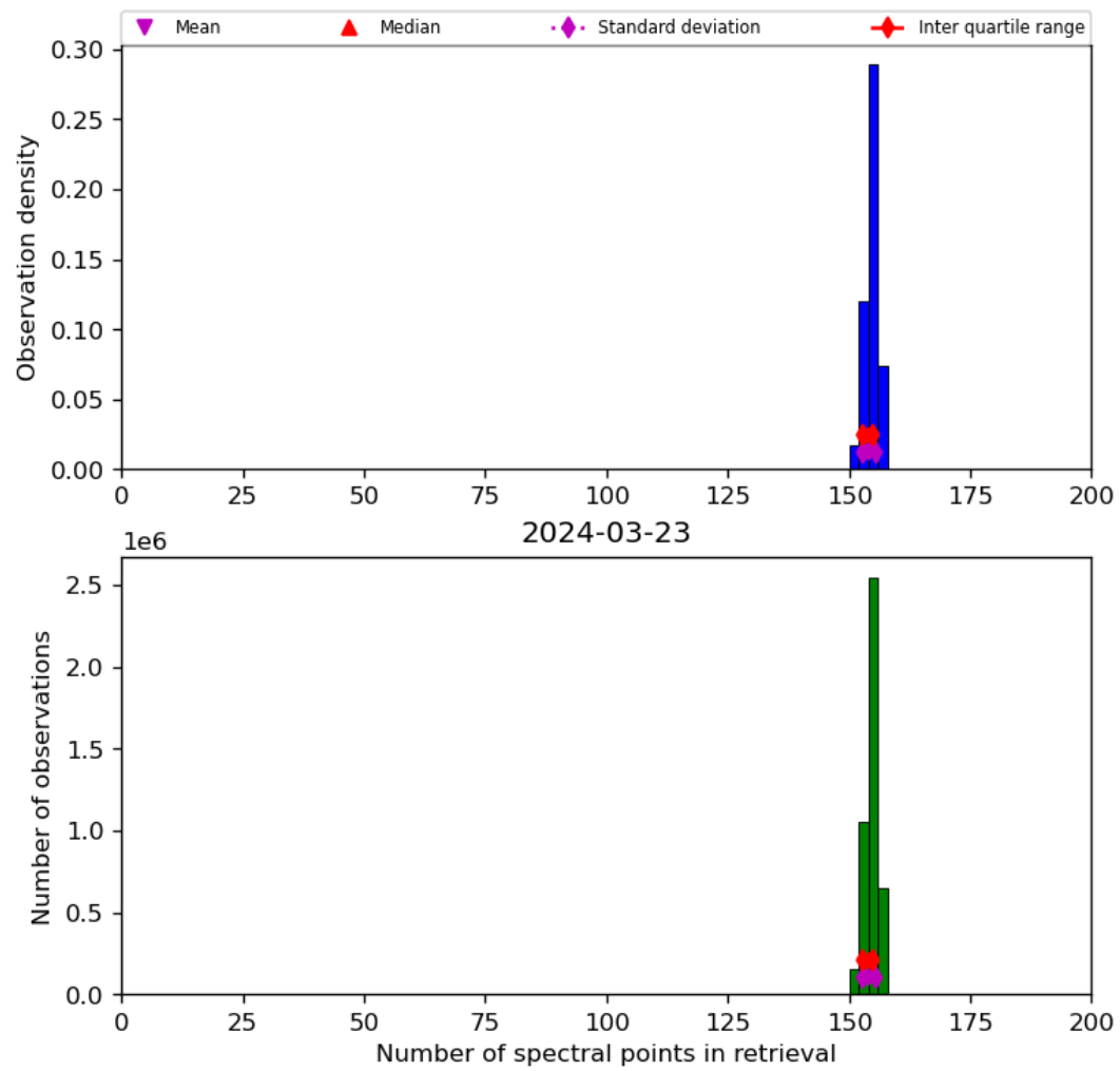
Figure 21: Histogram of “Number of spectral points in retrieval” for 2024-03-23 to 2024-03-24
