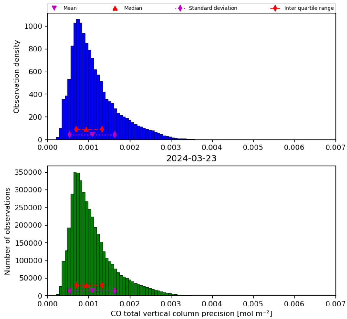
Figure 20: Histogram of “CO total vertical column precision” for 2024-03-23 to 2024-03-24
