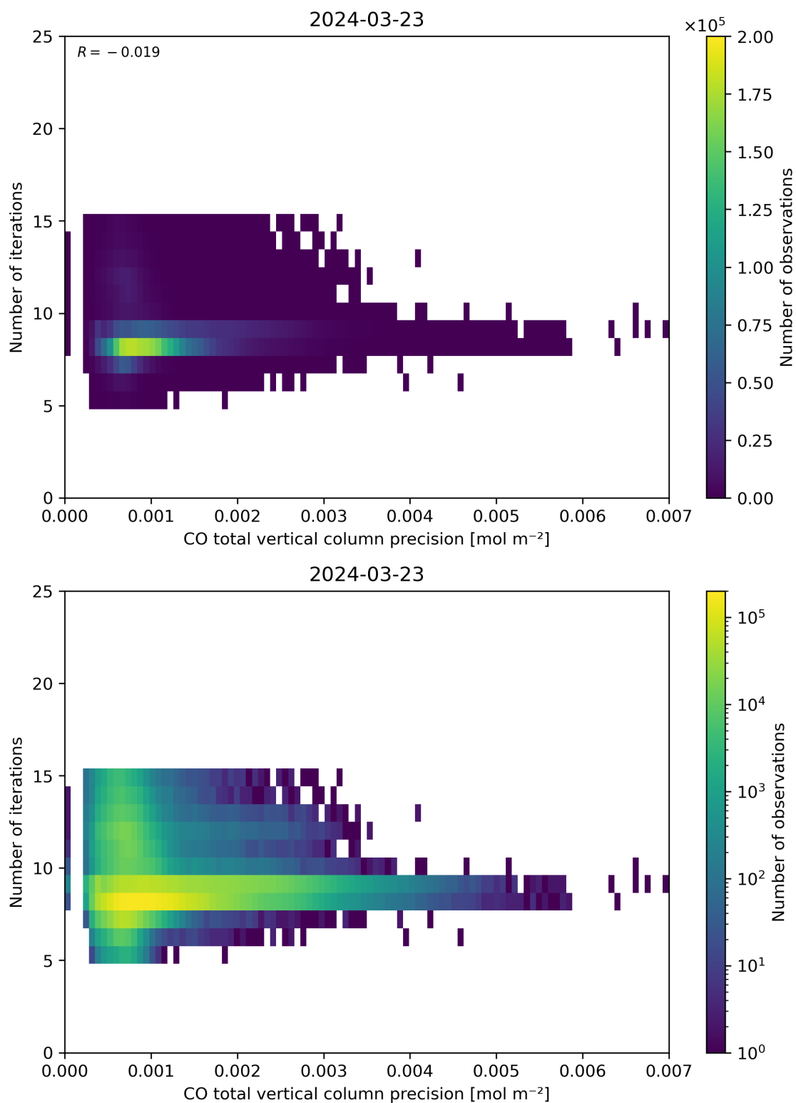
Figure 46: Scatter density plot of “CO total vertical column precision” against “Number of iterations” for 2024-03-23 to 2024-03-24.
