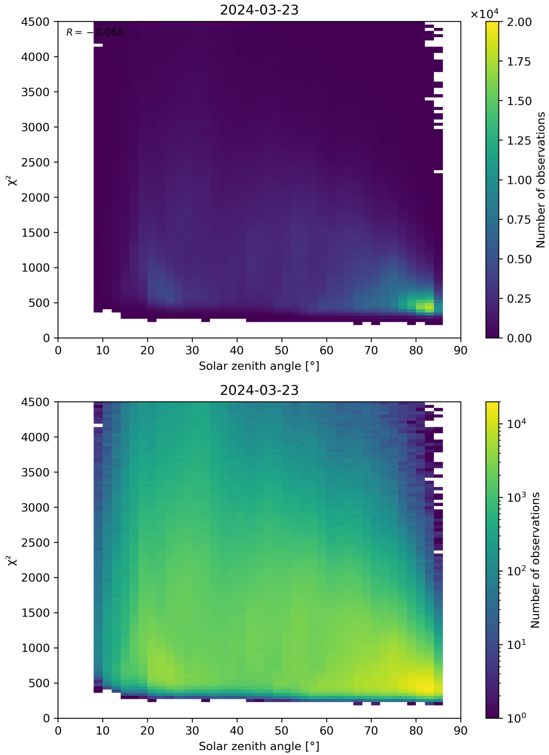
Figure 64: Scatter density plot of “Solar zenith angle” against “ \chi^2 ” for 2024-03-23 to 2024-03-24.
