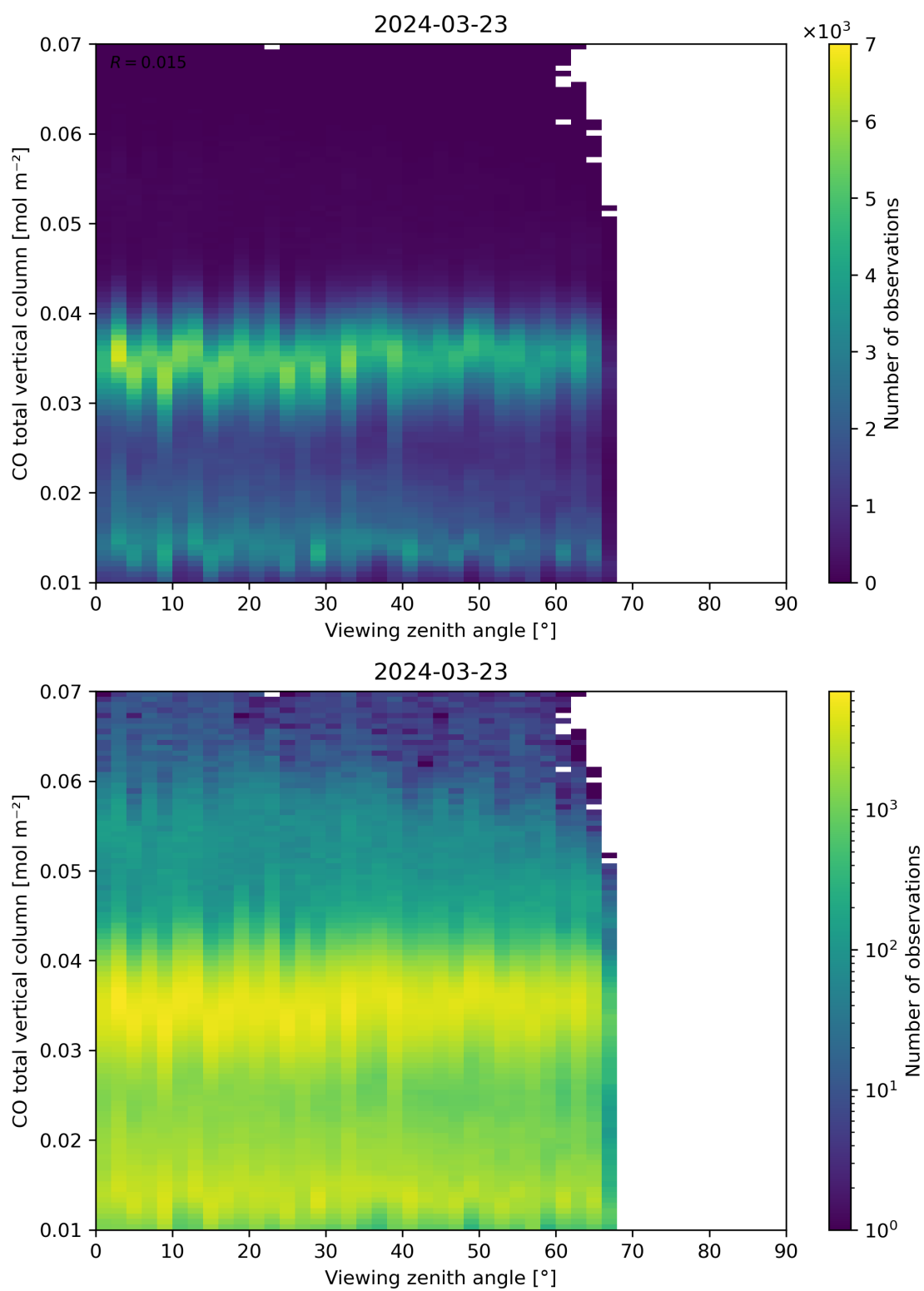
Figure 69: Scatter density plot of “Viewing zenith angle” against “CO total vertical column” for 2024-03-23 to 2024-03-24.
