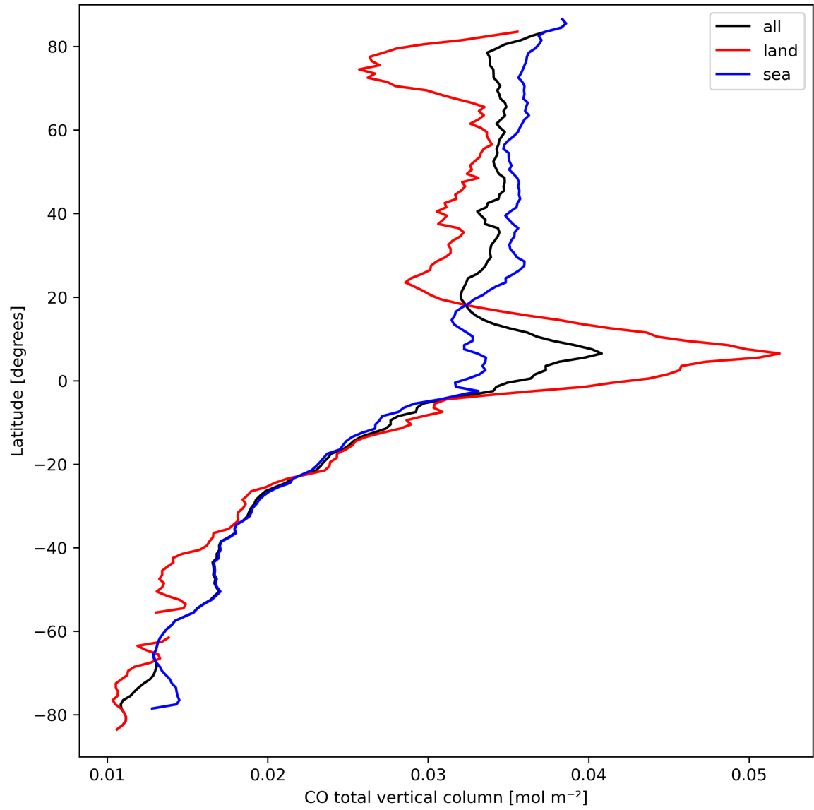
Figure 10: Zonal average of “CO total vertical column” for 2024-03-23 to 2024-03-24.
