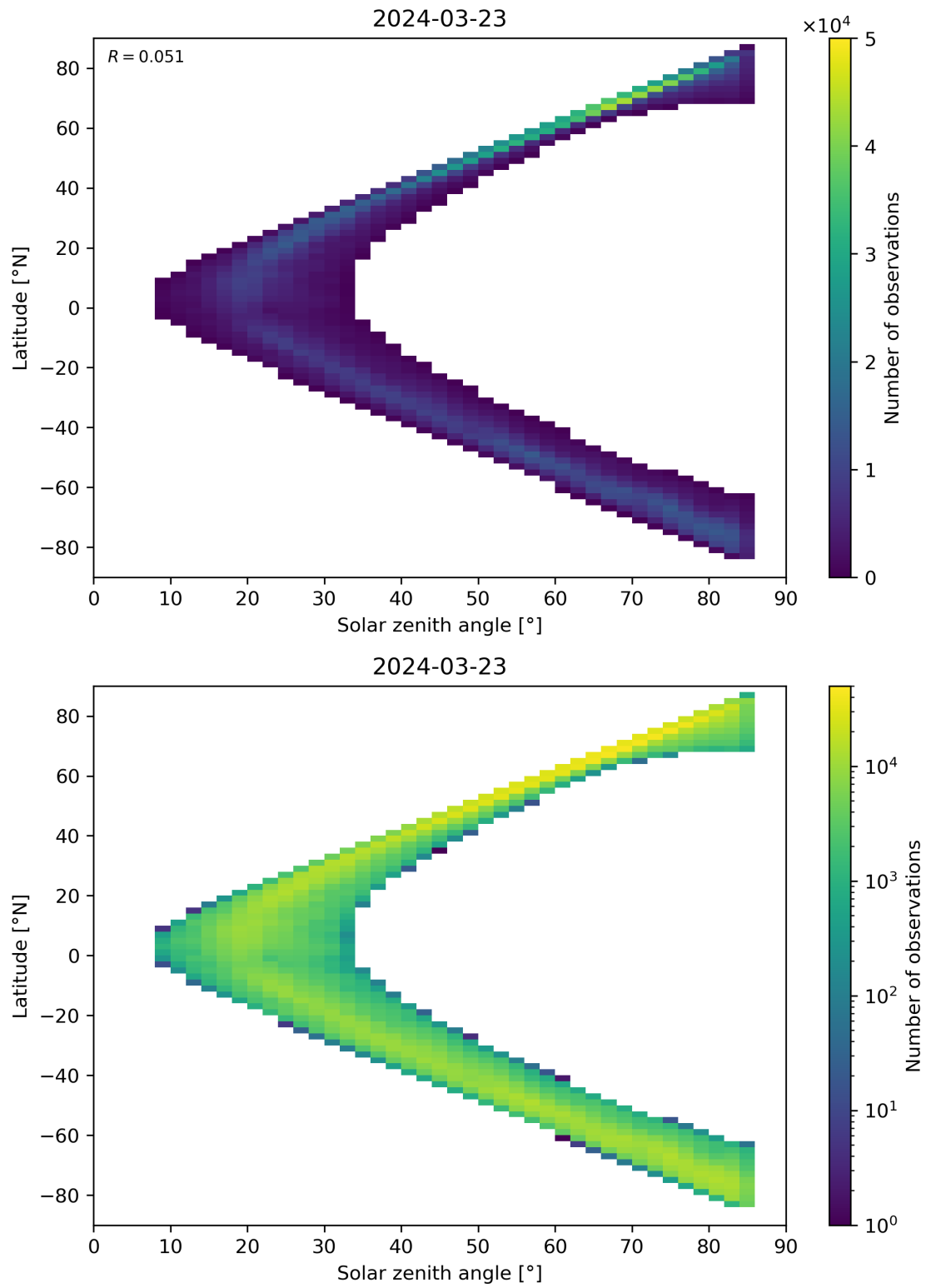
Figure 66: Scatter density plot of “Solar zenith angle” against “Latitude” for 2024-03-23 to 2024-03-24.
