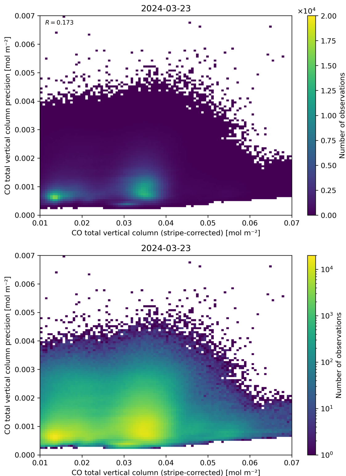
Figure 36: Scatter density plot of “CO total vertical column (stripe-corrected)” against “CO total vertical column precision” for 2024-03-23 to 2024-03-24.
