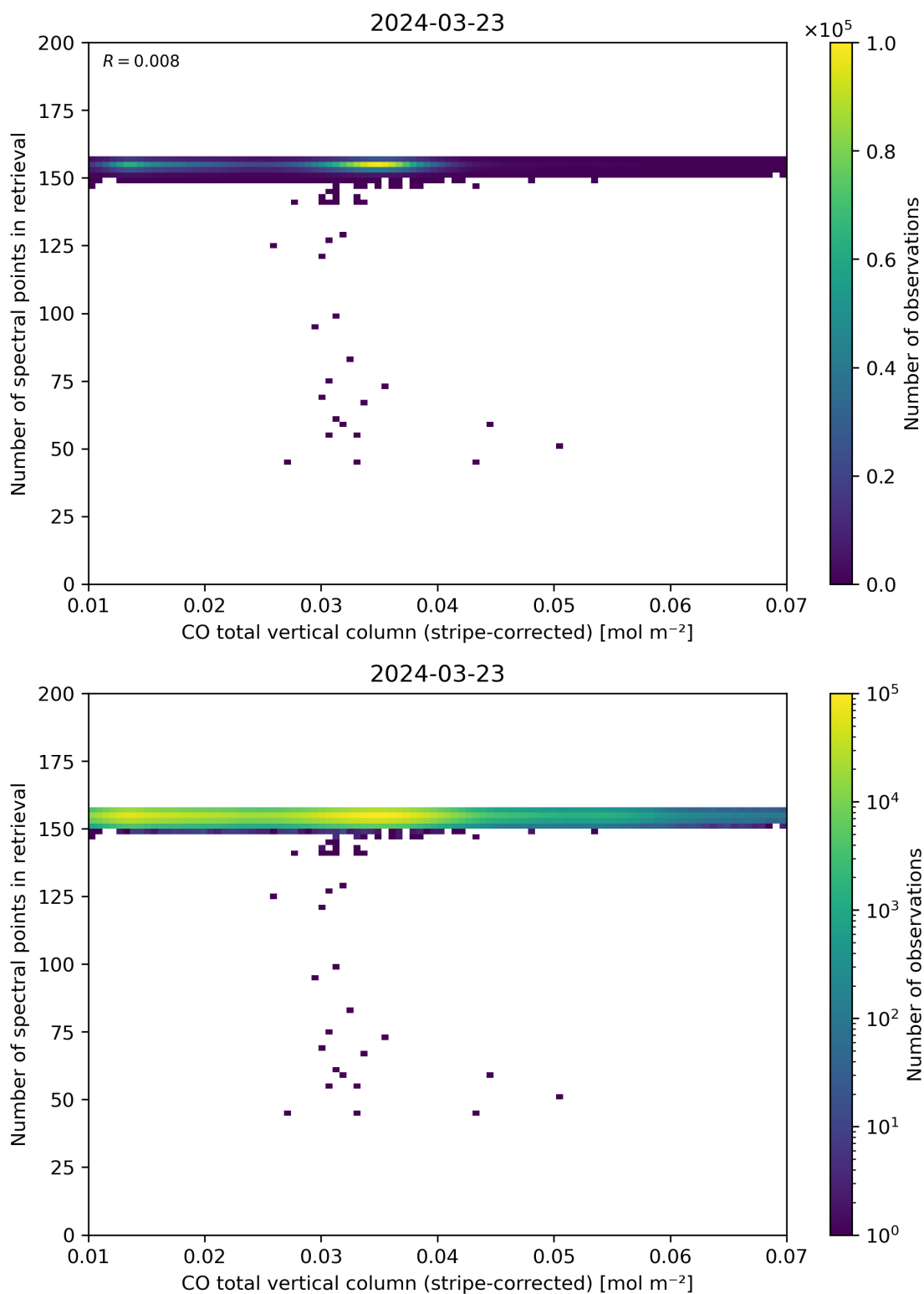
Figure 40: Scatter density plot of “CO total vertical column (stripe-corrected)” against “Number of spectral points in retrieval” for 2024-03-23 to 2024-03-24.
