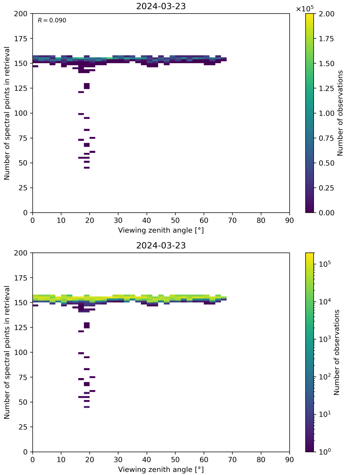
Figure 76: Scatter density plot of “Viewing zenith angle” against “Number of spectral points in retrieval” for 2024-03-23 to 2024-03-24.
