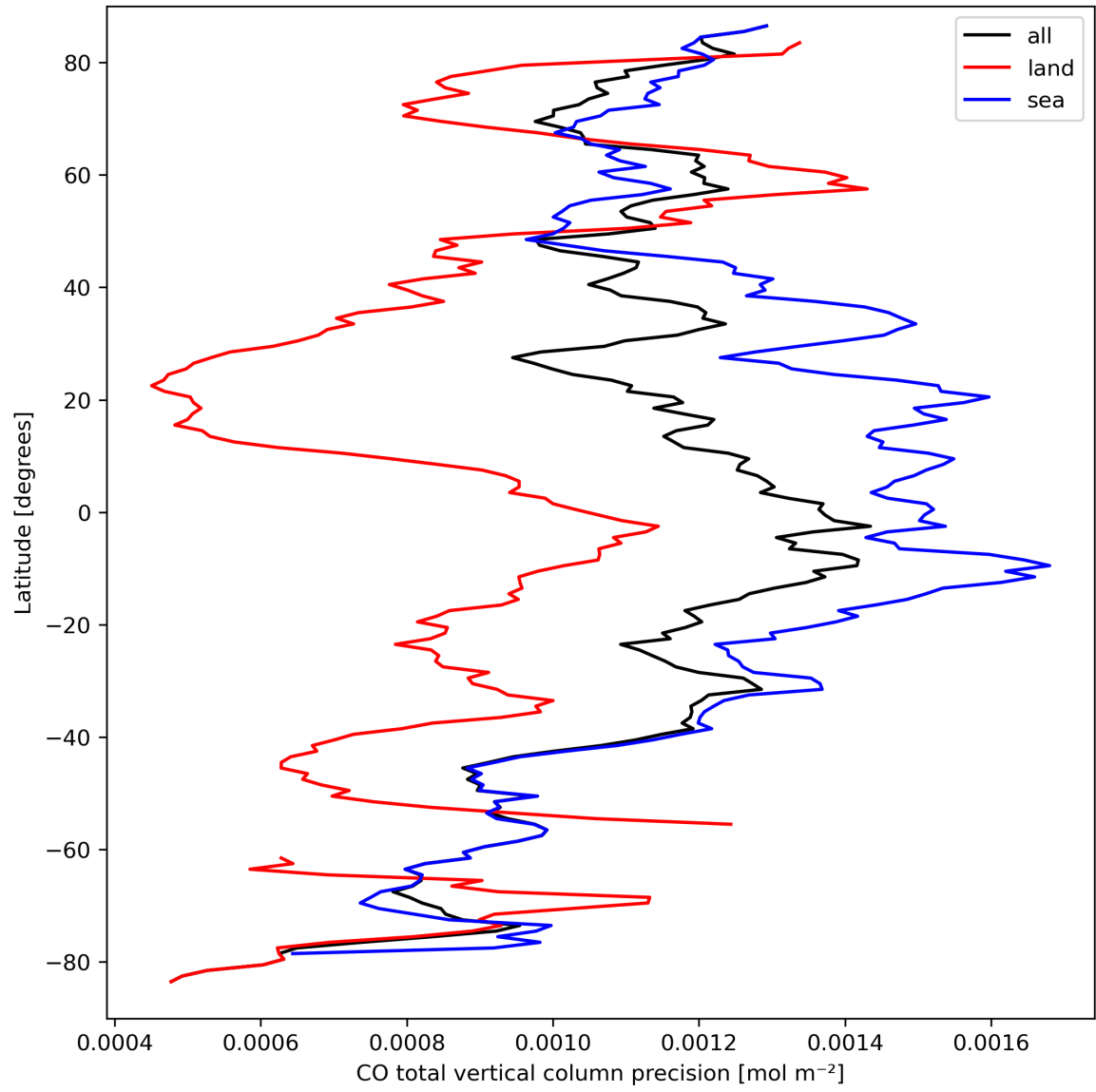
Figure 12: Zonal average of “CO total vertical column precision” for 2024-03-23 to 2024-03-24.
