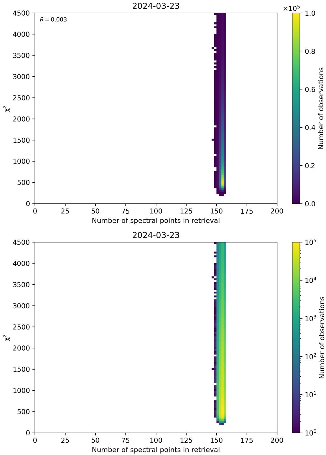
Figure 58: Scatter density plot of “Number of spectral points in retrieval” against “ \chi^2 ” for 2024-03-23 to 2024-03-24.
