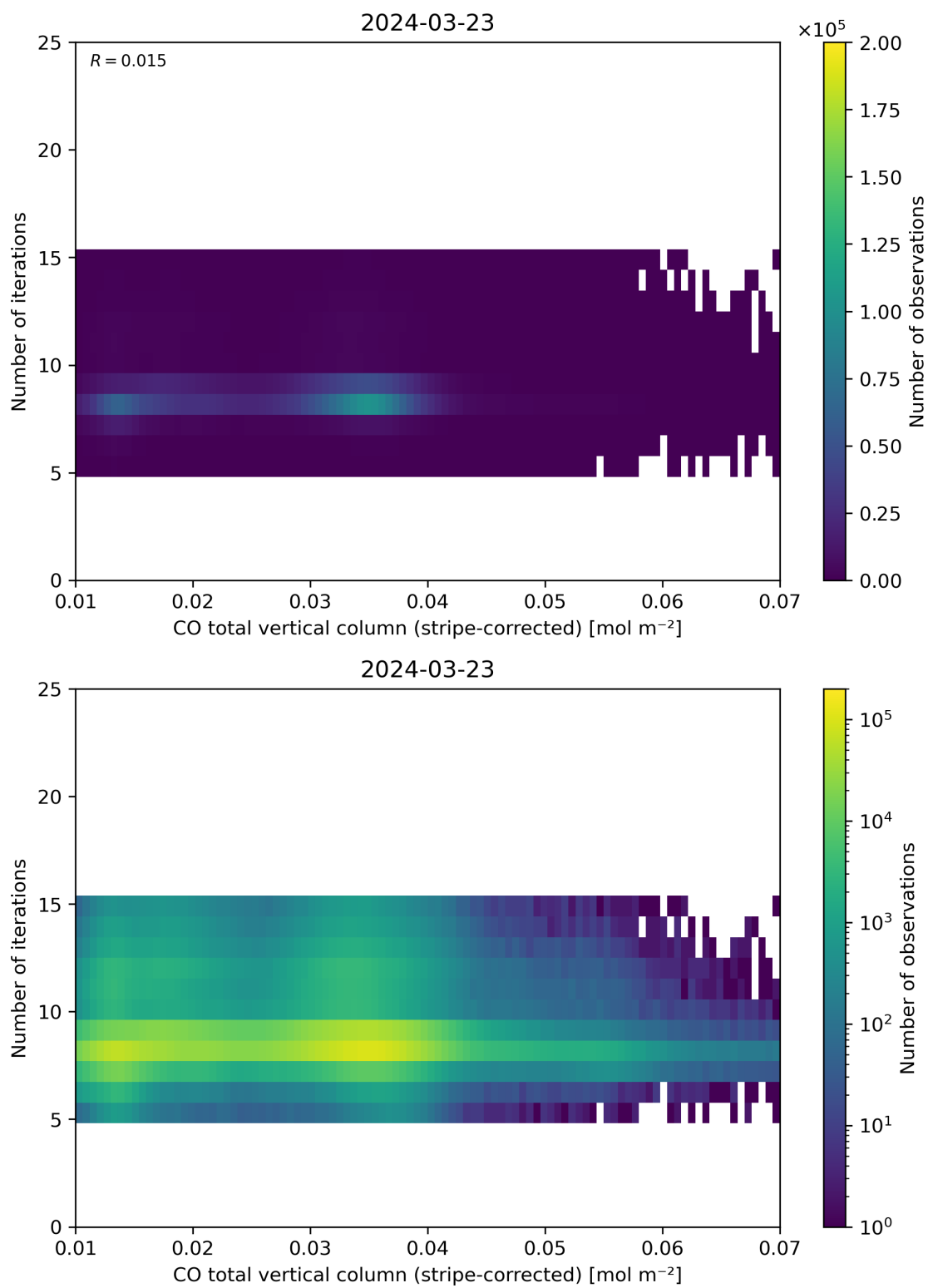
Figure 39: Scatter density plot of “CO total vertical column (stripe-corrected)” against “Number of iterations” for 2024-03-23 to 2024-03-24.
