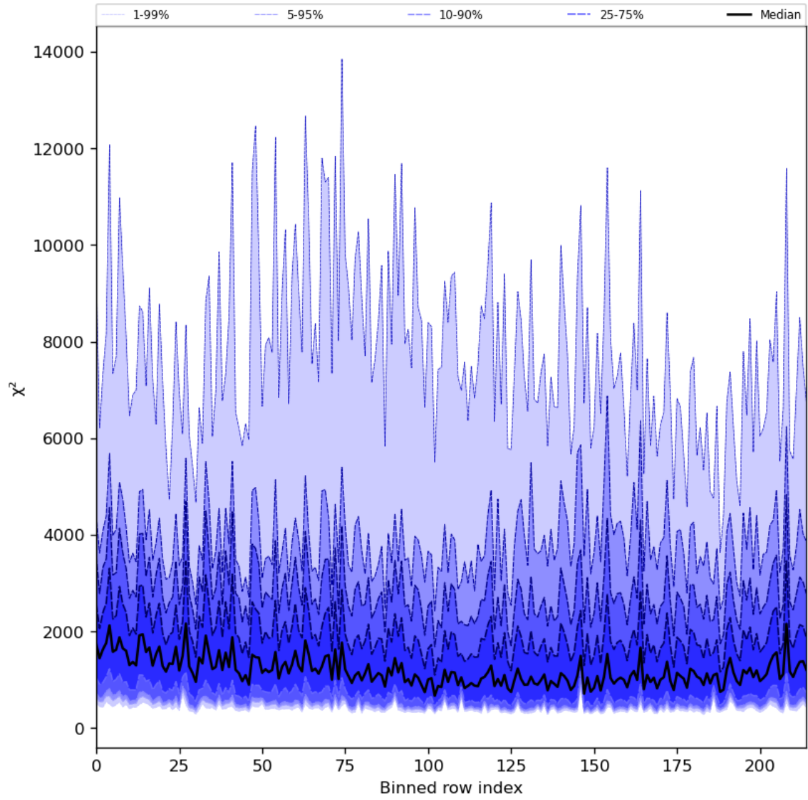
Figure 30: Along track statistics of “ \chi^2 ” for 2024-03-23 to 2024-03-24
