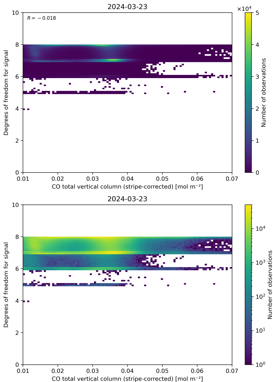
Figure 38: Scatter density plot of “CO total vertical column (stripe-corrected)” against “Degrees of freedom for signal” for 2024-03-23 to 2024-03-24.
