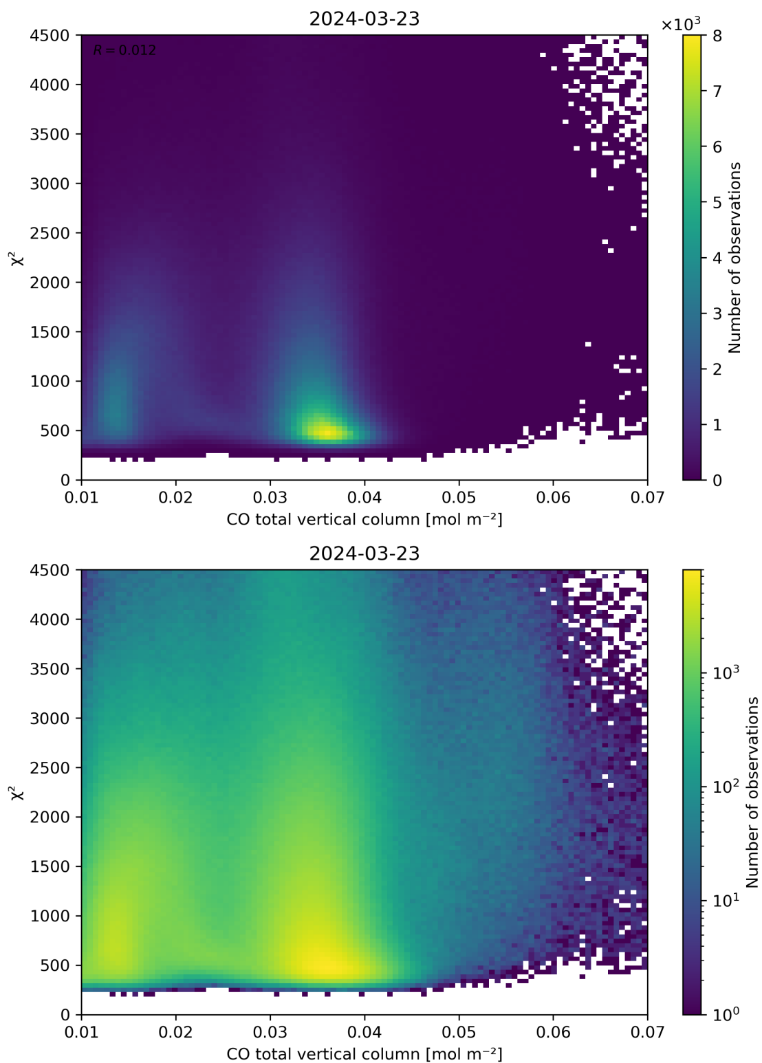
Figure 35: Scatter density plot of “CO total vertical column” against “ \chi^2 ” for 2024-03-23 to 2024-03-24.
