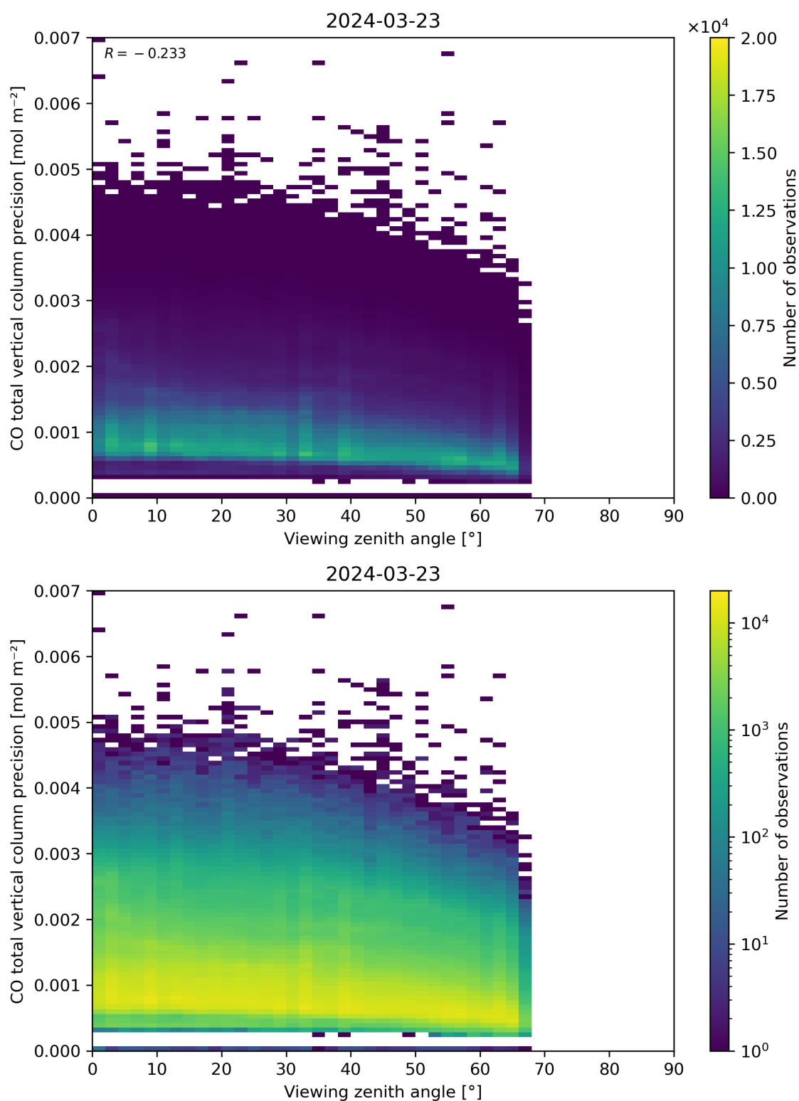
Figure 71: Scatter density plot of “Viewing zenith angle” against “CO total vertical column precision” for 2024-03-23 to 2024-03-24.
