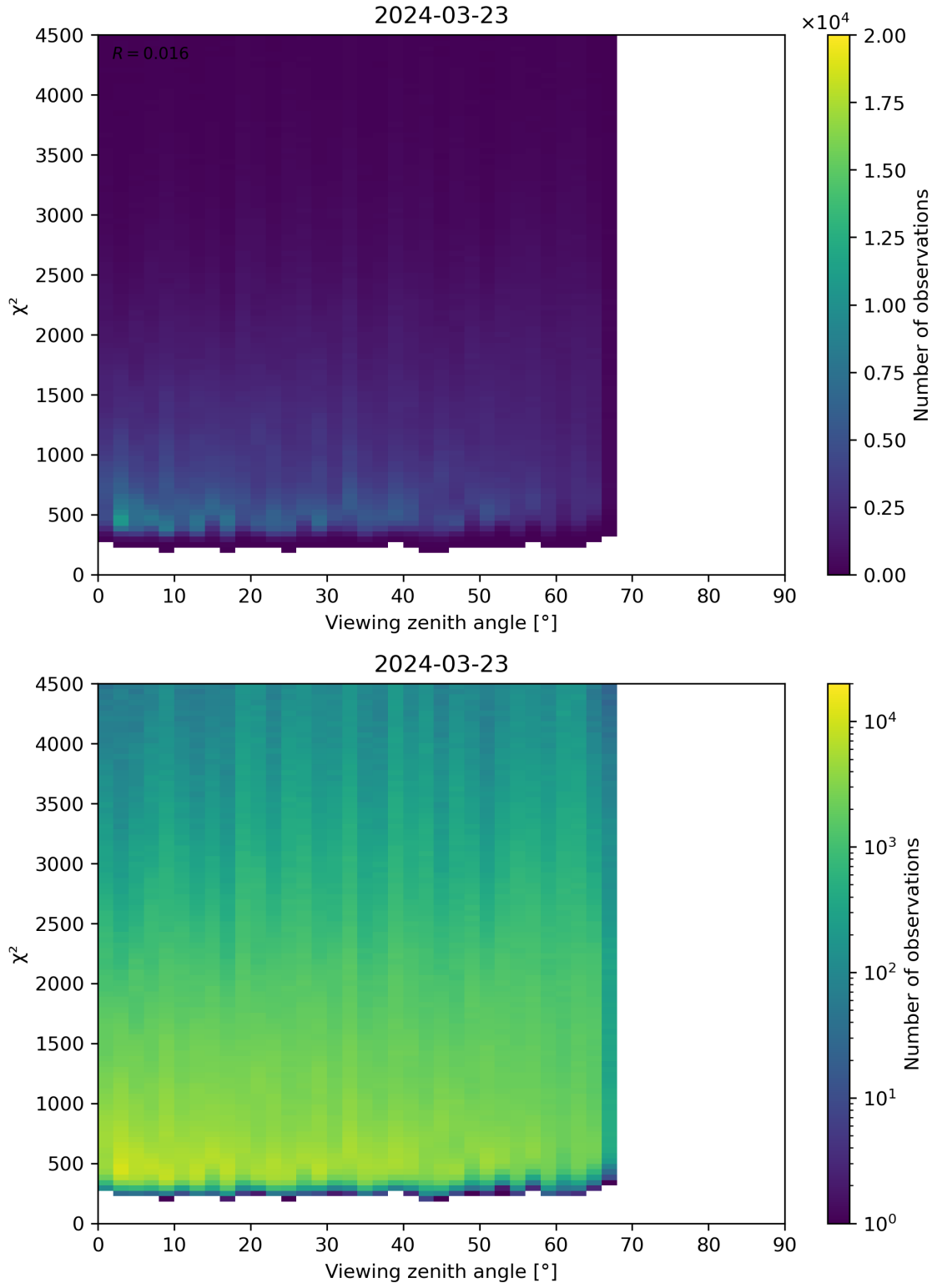
Figure 72: Scatter density plot of “Viewing zenith angle” against “ \chi^2 ” for 2024-03-23 to 2024-03-24.
