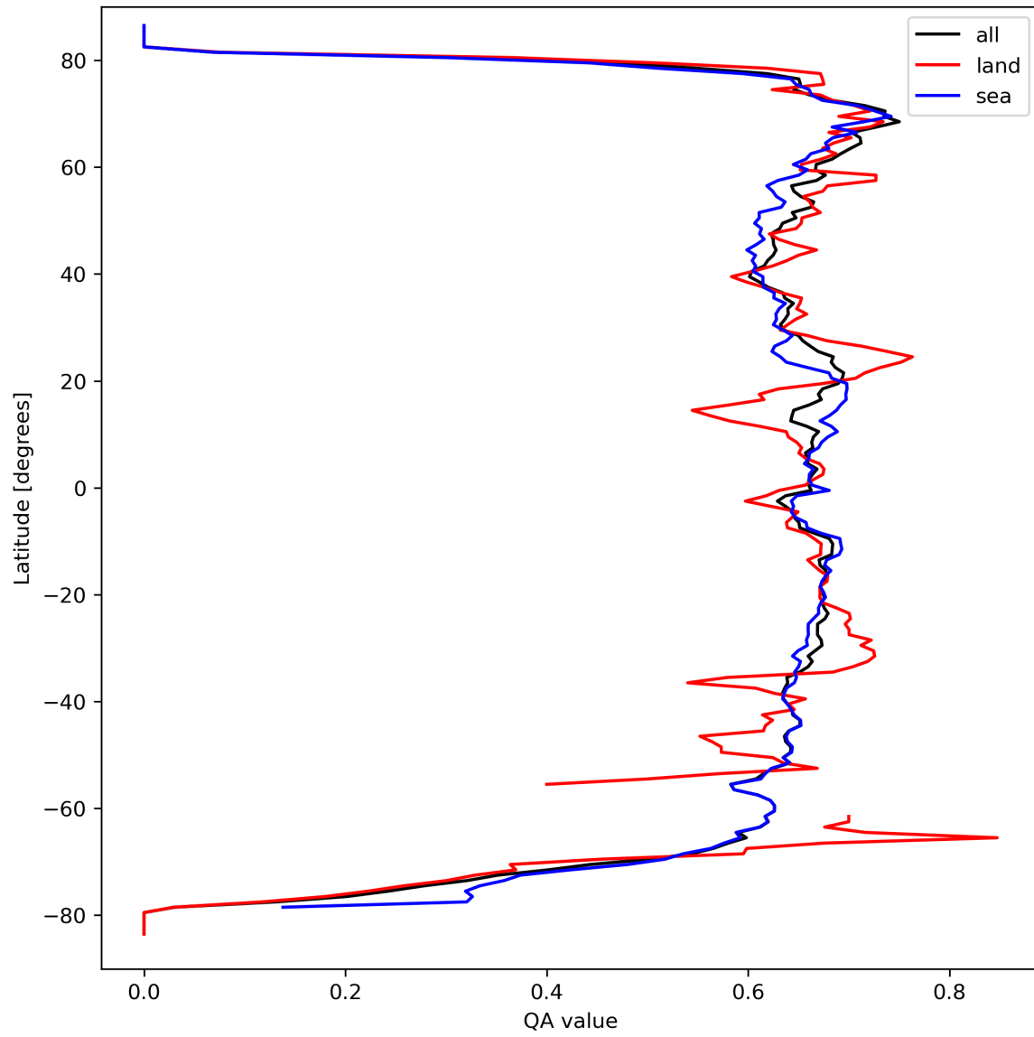
Figure 9: Zonal average of “QA value” for 2024-03-23 to 2024-03-24.
