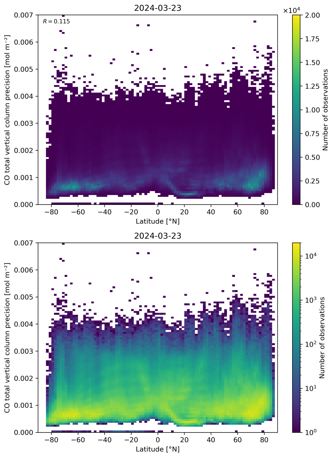
Figure 53: Scatter density plot of “Latitude” against “CO total vertical column precision” for 2024-03-23 to 2024-03-24.
