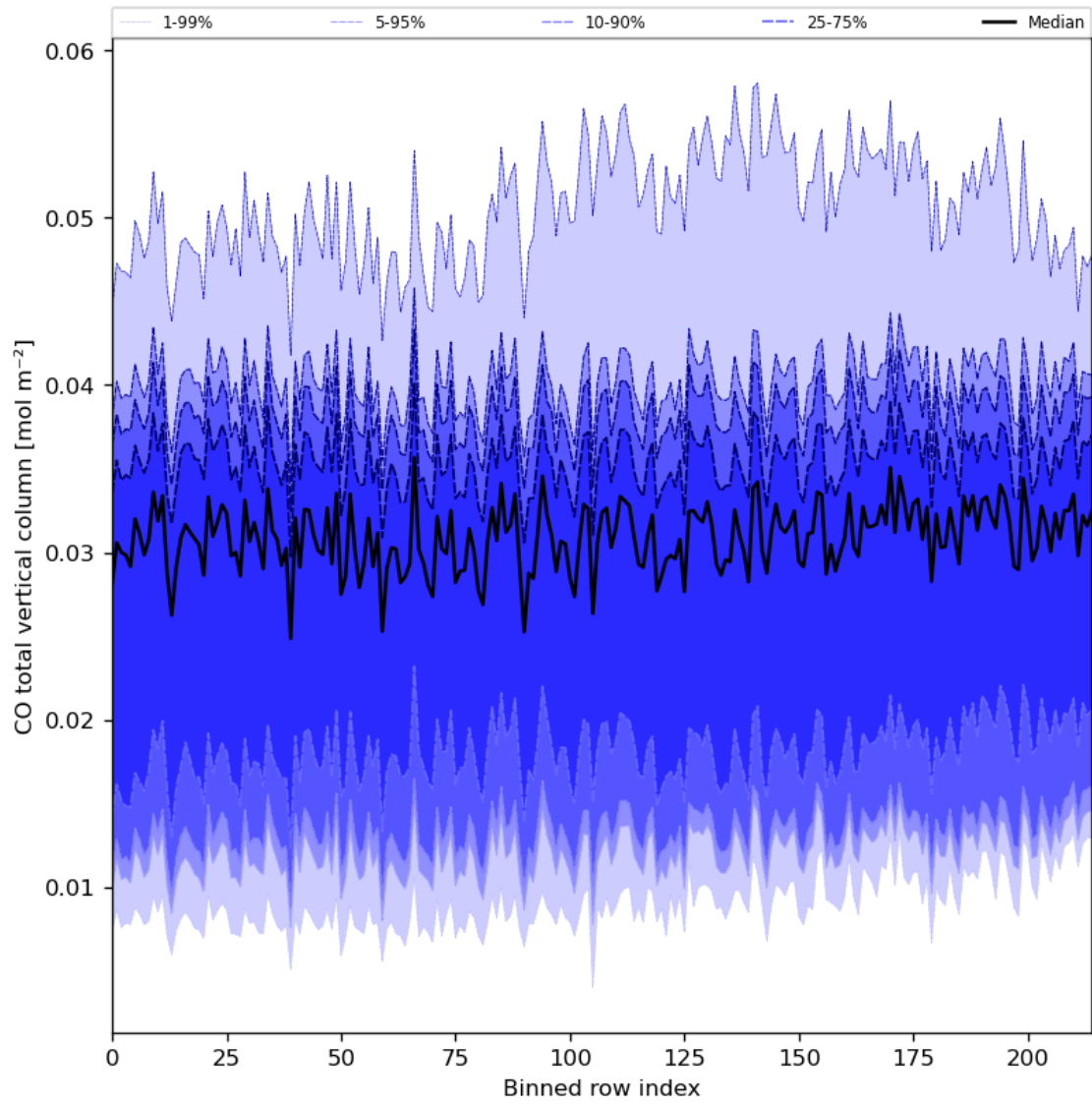
Figure 26: Along track statistics of “CO total vertical column” for 2024-03-23 to 2024-03-24
