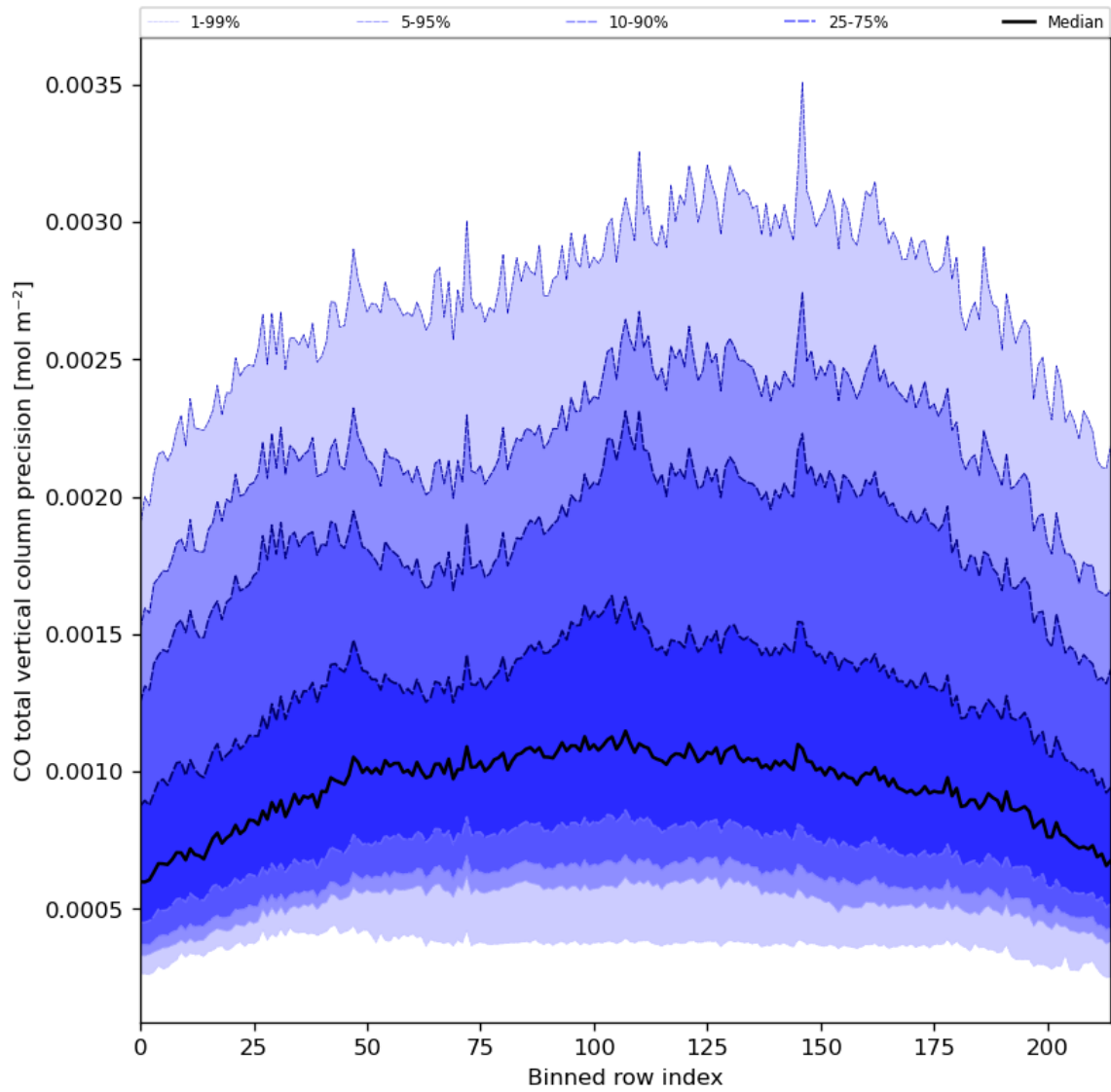
Figure 28: Along track statistics of “CO total vertical column precision” for 2024-03-23 to 2024-03-24
