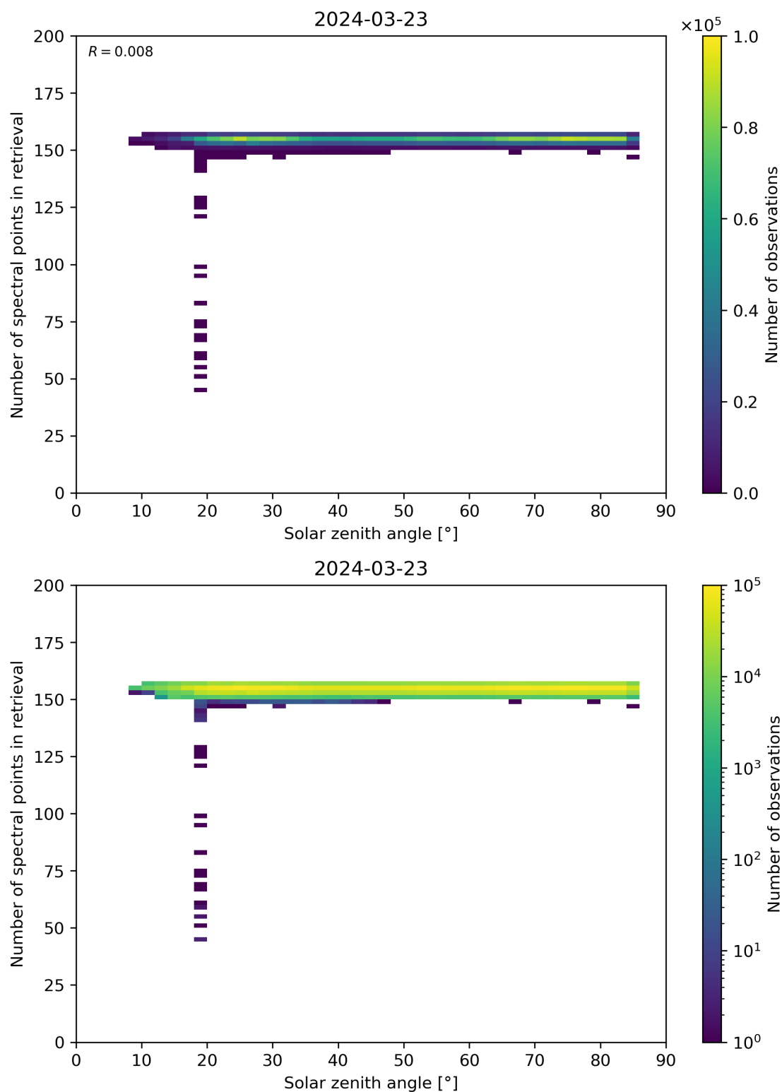
Figure 68: Scatter density plot of “Solar zenith angle” against “Number of spectral points in retrieval” for 2024-03-23 to 2024-03-24.
