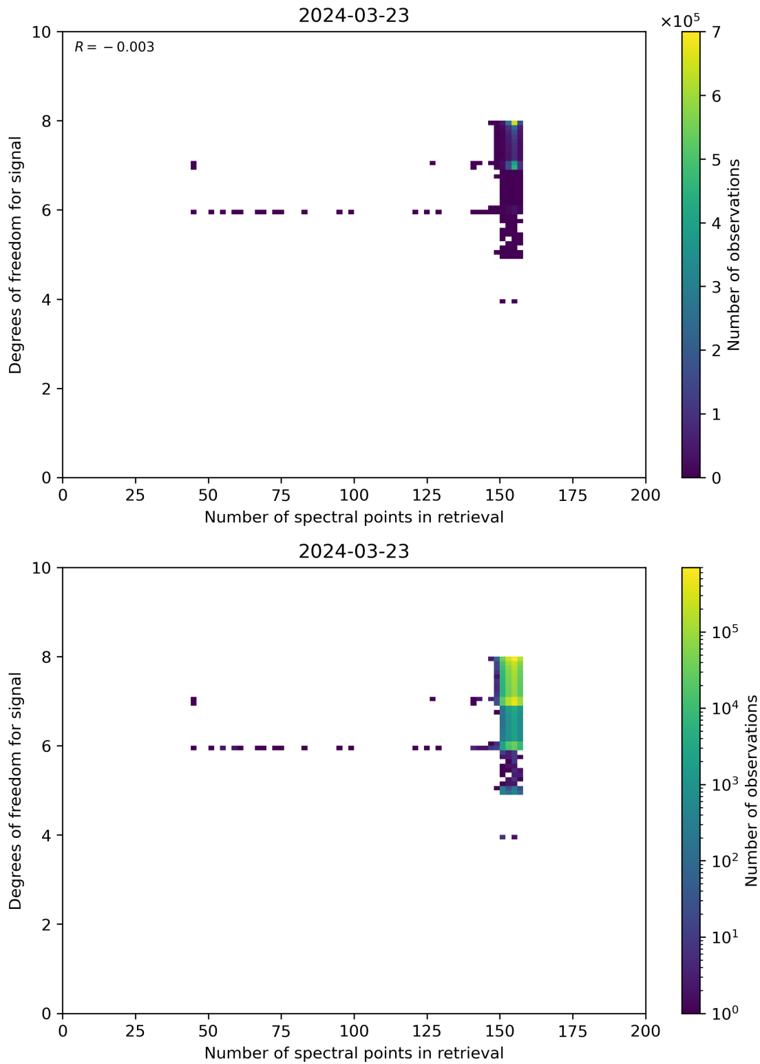
Figure 59: Scatter density plot of “Number of spectral points in retrieval” against “Degrees of freedom for signal” for 2024-03-23 to 2024-03-24.
