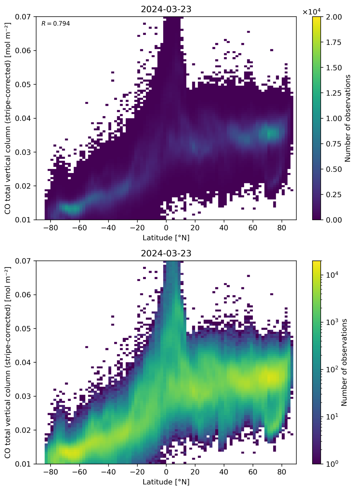
Figure 52: Scatter density plot of “Latitude” against “CO total vertical column (stripe-corrected)” for 2024-03-23 to 2024-03-24.
