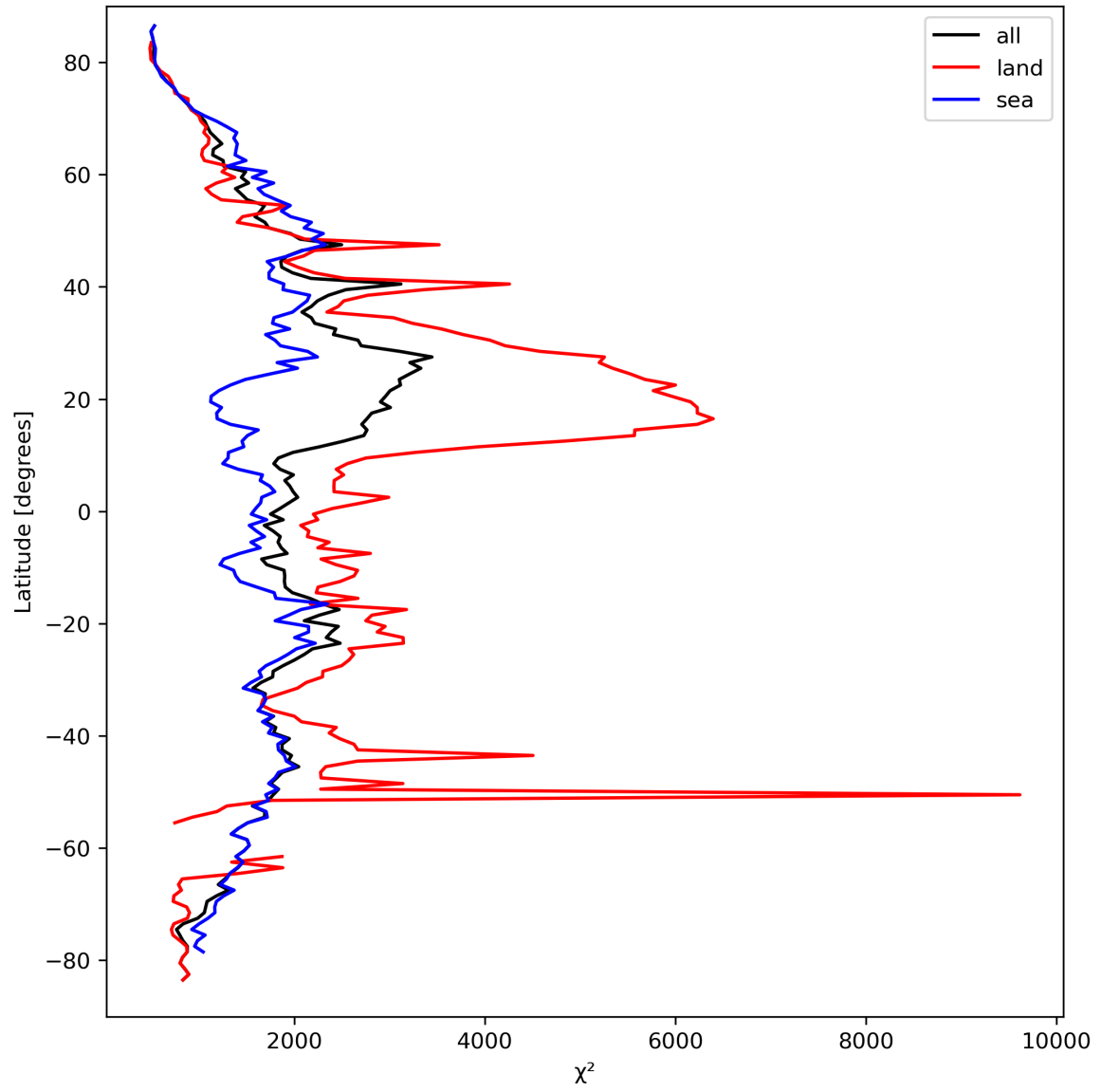
Figure 14: Zonal average of “ \chi^2 ” for 2024-03-23 to 2024-03-24.
