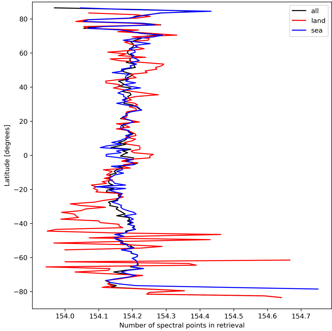
Figure 13: Zonal average of “Number of spectral points in retrieval” for 2024-03-23 to 2024-03-24.
