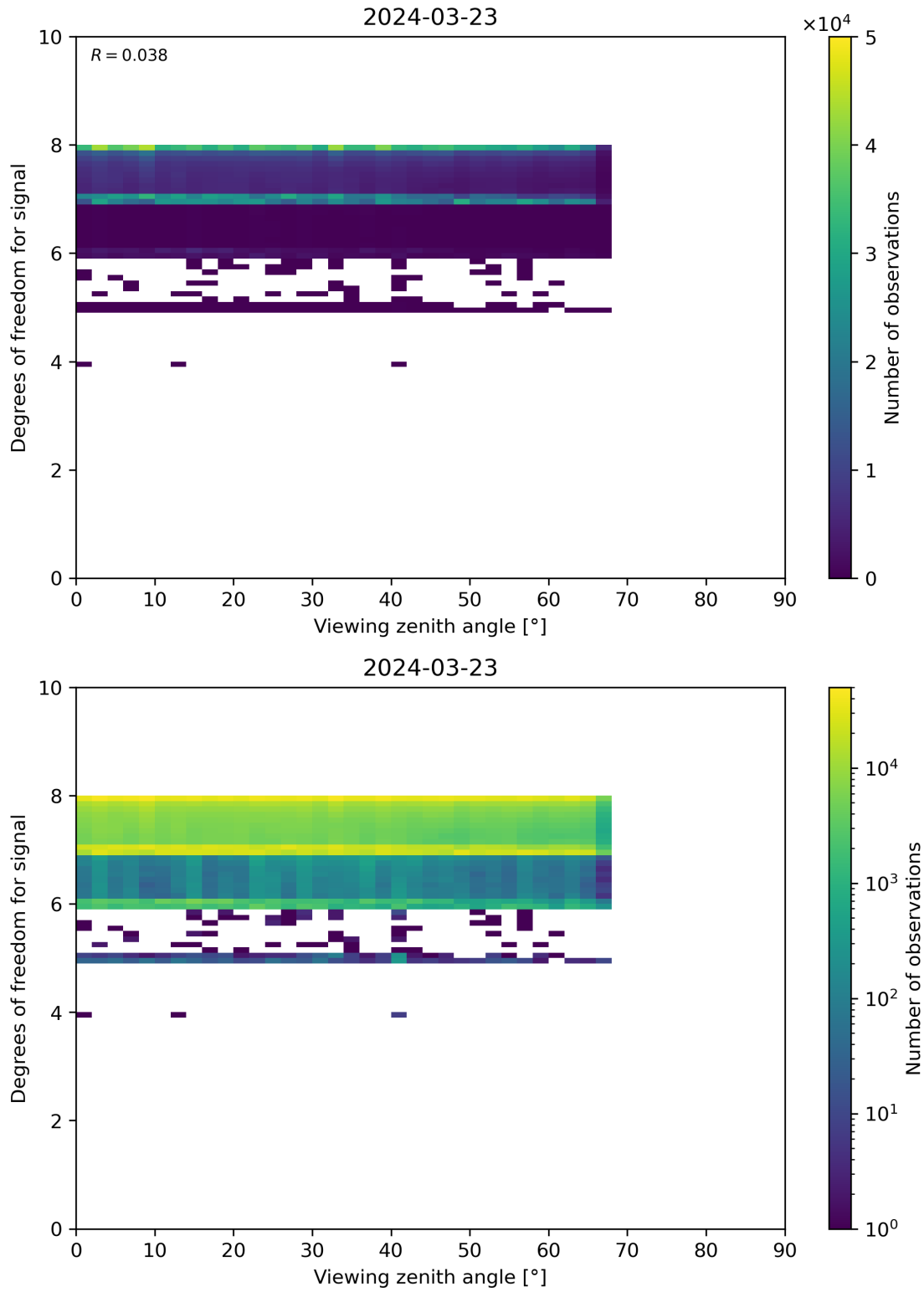
Figure 73: Scatter density plot of “Viewing zenith angle” against “Degrees of freedom for signal” for 2024-03-23 to 2024-03-24.
