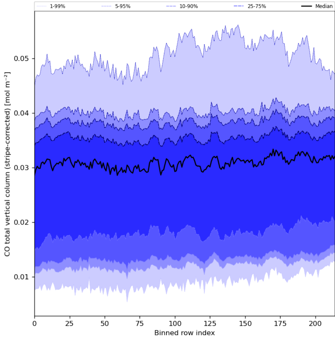
Figure 27: Along track statistics of “CO total vertical column (stripe-corrected)” for 2024-03-23 to 2024-03-24
