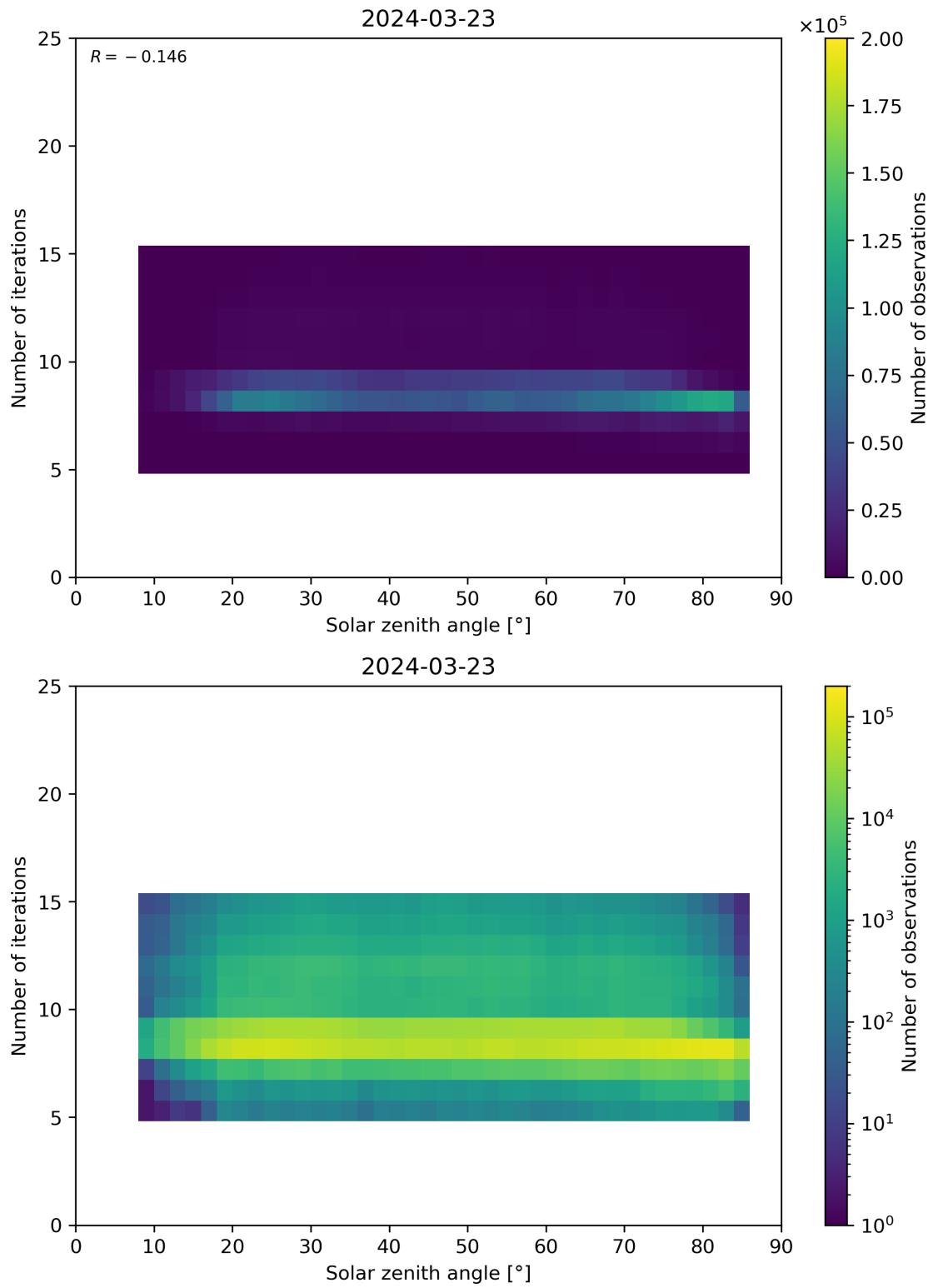
Figure 67: Scatter density plot of “Solar zenith angle” against “Number of iterations” for 2024-03-23 to 2024-03-24.
