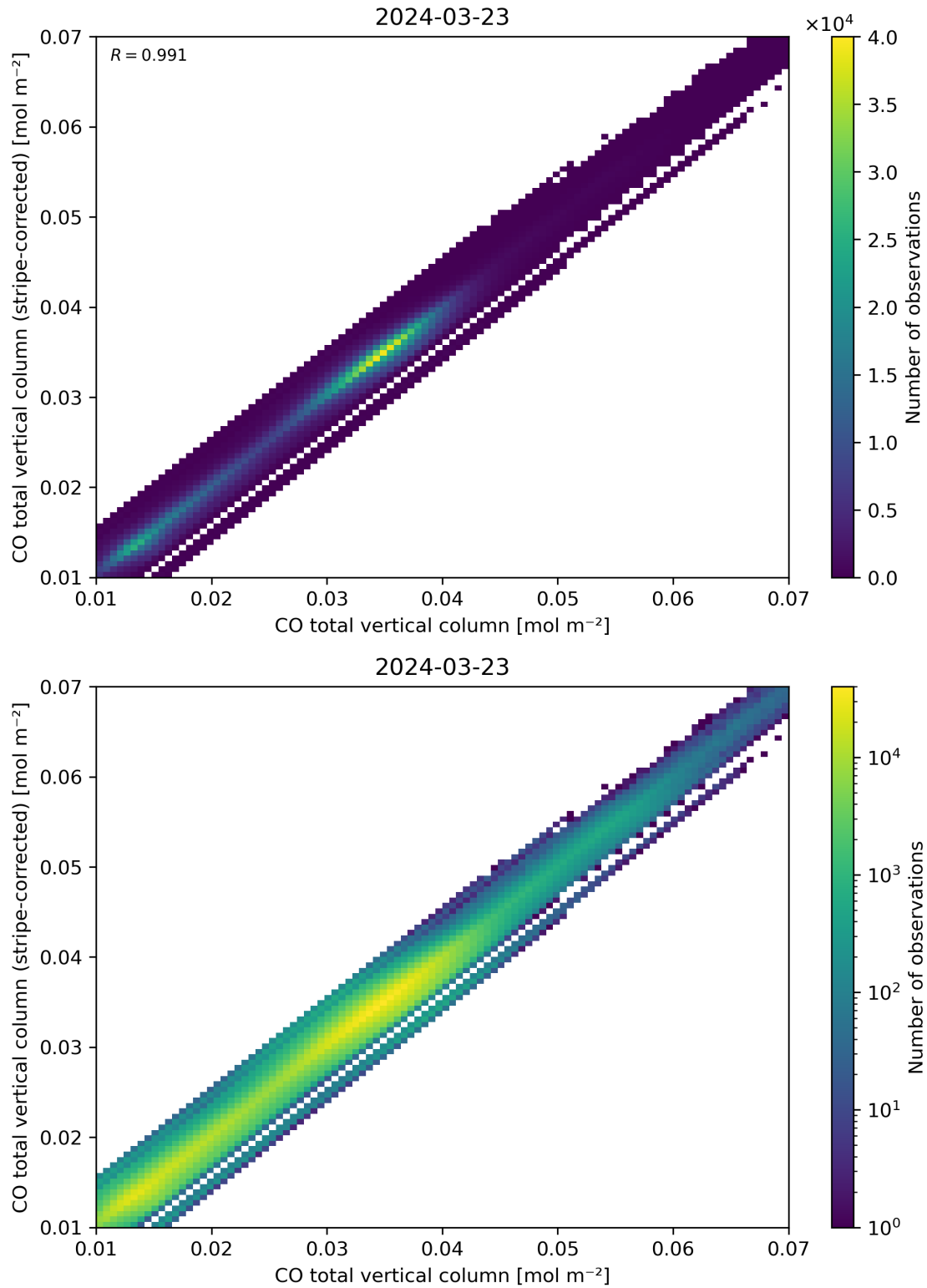
Figure 33: Scatter density plot of “CO total vertical column” against “CO total vertical column (stripe-corrected)” for 2024-03-23 to 2024-03-24.
