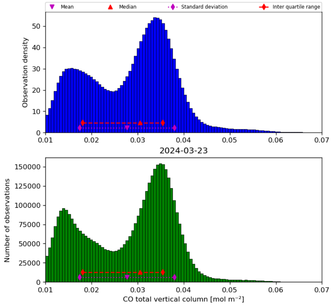
Figure 18: Histogram of “CO total vertical column” for 2024-03-23 to 2024-03-24
