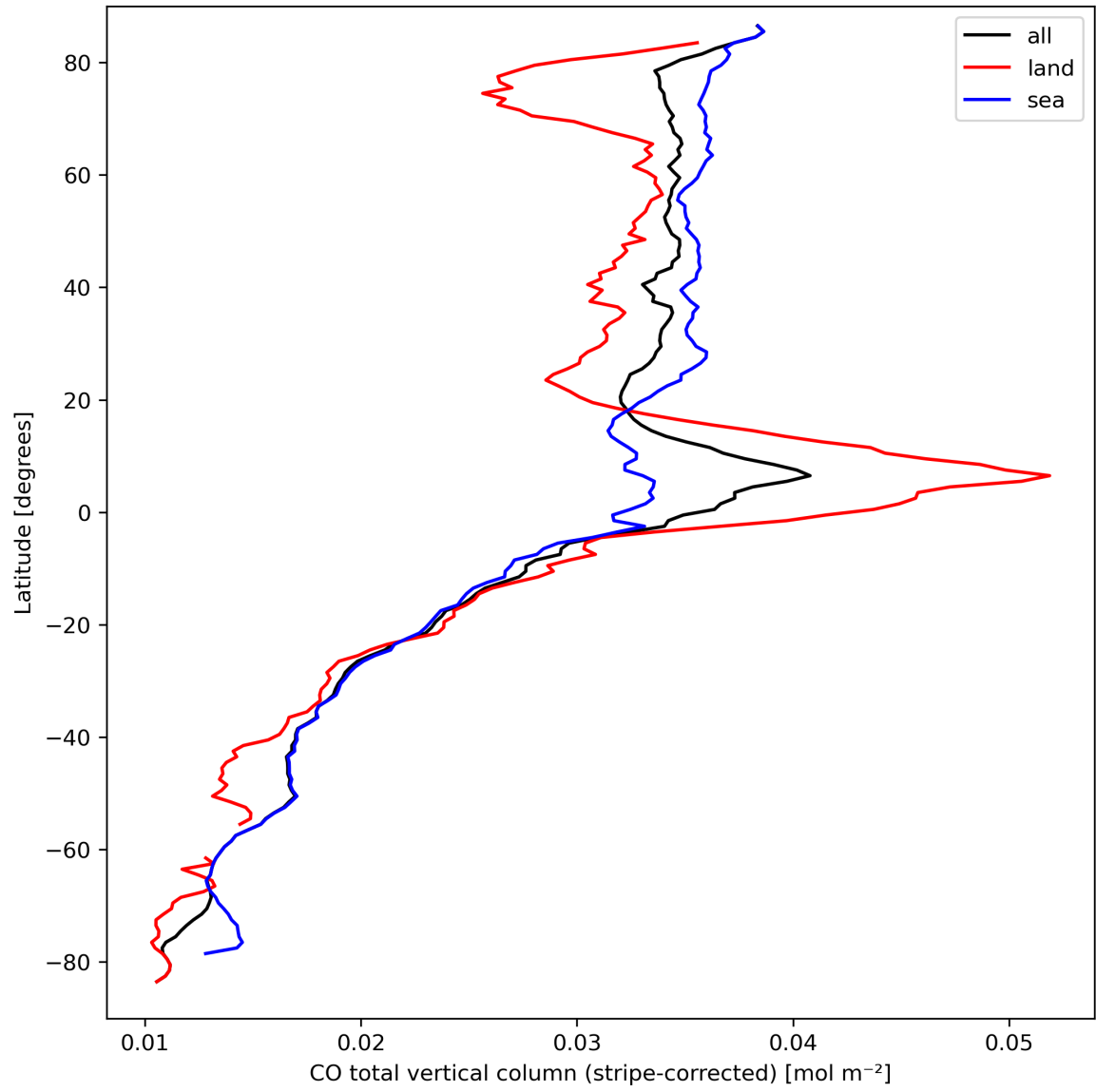
Figure 11: Zonal average of “CO total vertical column (stripe-corrected)” for 2024-03-23 to 2024-03-24.
