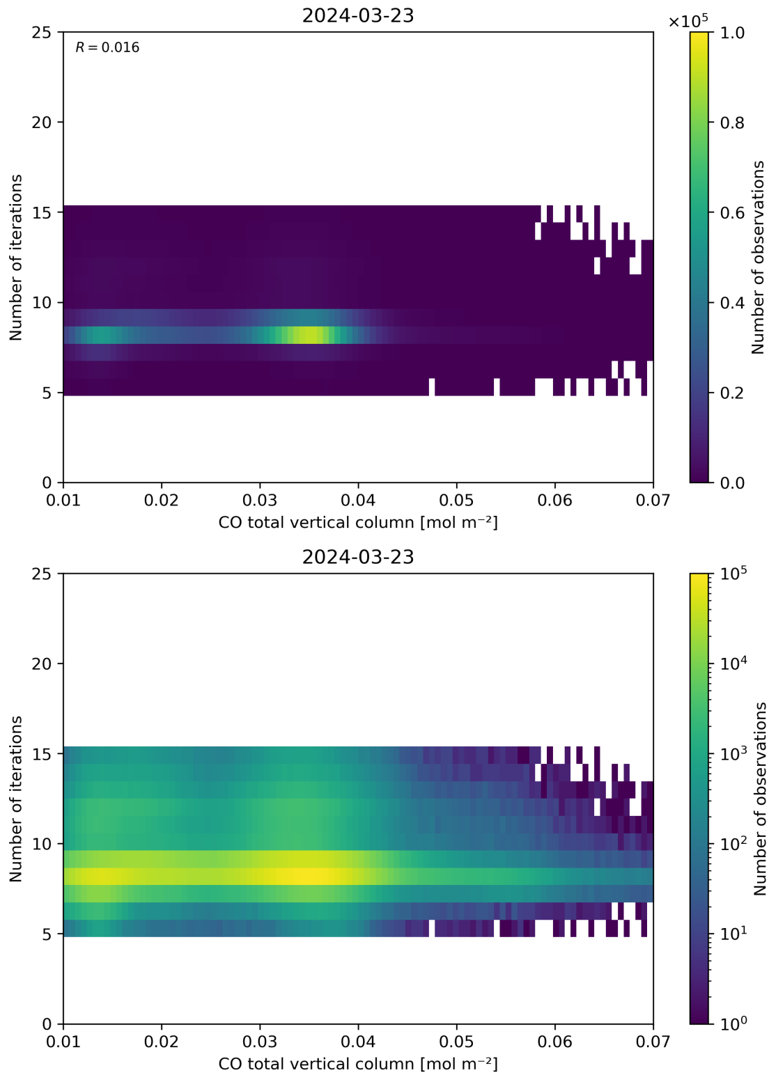
Figure 42: Scatter density plot of “CO total vertical column” against “Number of iterations” for 2024-03-23 to 2024-03-24.
