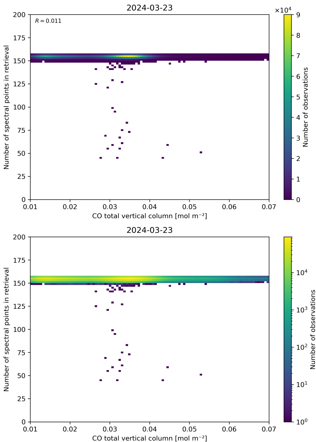
Figure 43: Scatter density plot of “CO total vertical column” against “Number of spectral points in retrieval” for 2024-03-23 to 2024-03-24.
