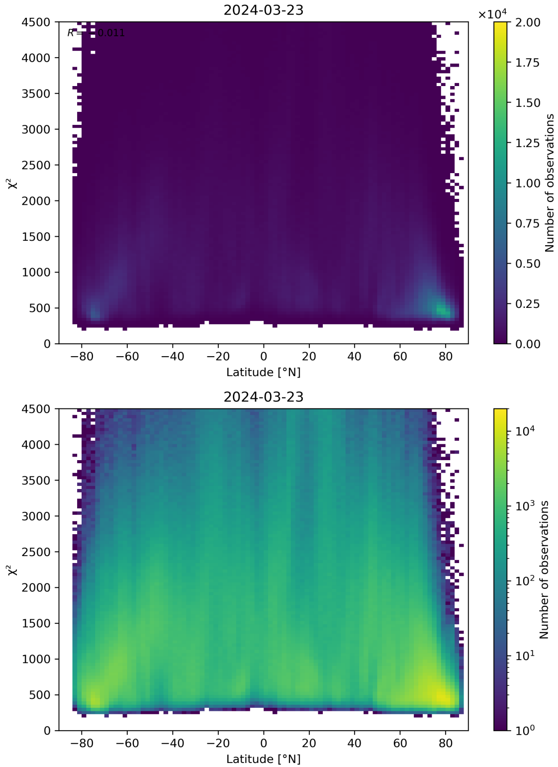
Figure 54: Scatter density plot of “Latitude” against “ \chi^2 ” for 2024-03-23 to 2024-03-24.
