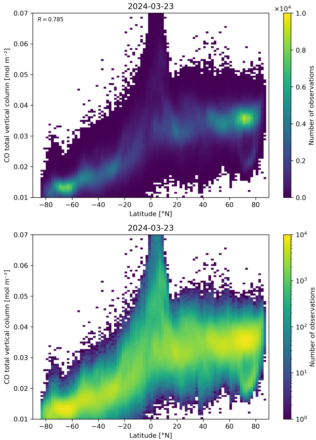
Figure 51: Scatter density plot of “Latitude” against “CO total vertical column” for 2024-03-23 to 2024-03-24.
