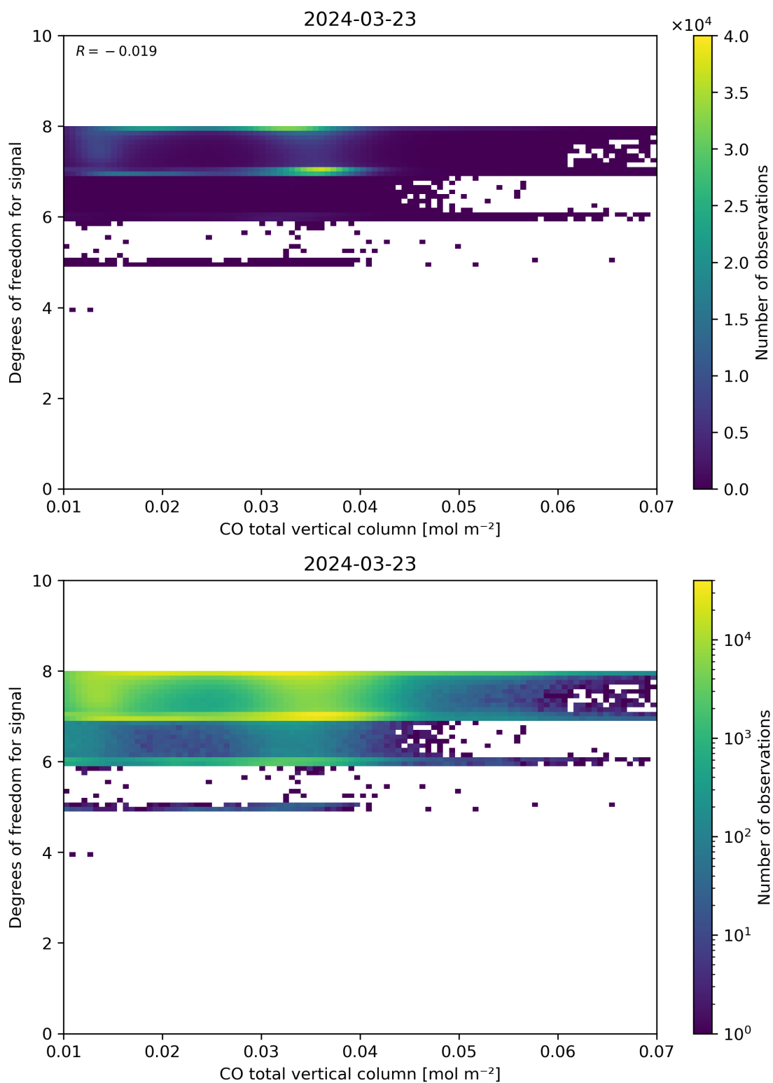
Figure 41: Scatter density plot of “CO total vertical column” against “Degrees of freedom for signal” for 2024-03-23 to 2024-03-24.
