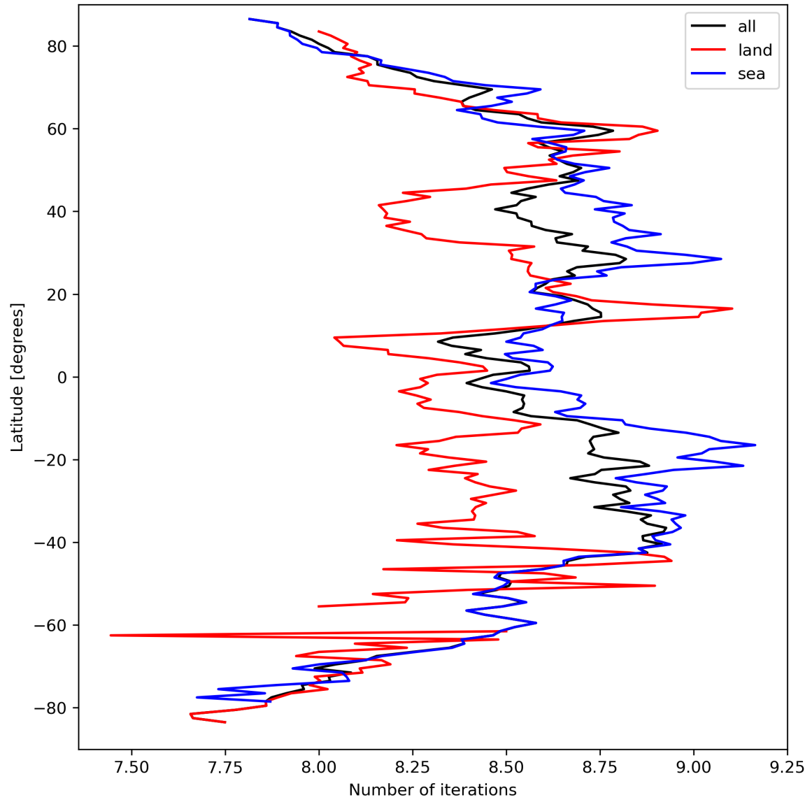
Figure 16: Zonal average of “Number of iterations” for 2024-03-23 to 2024-03-24.
