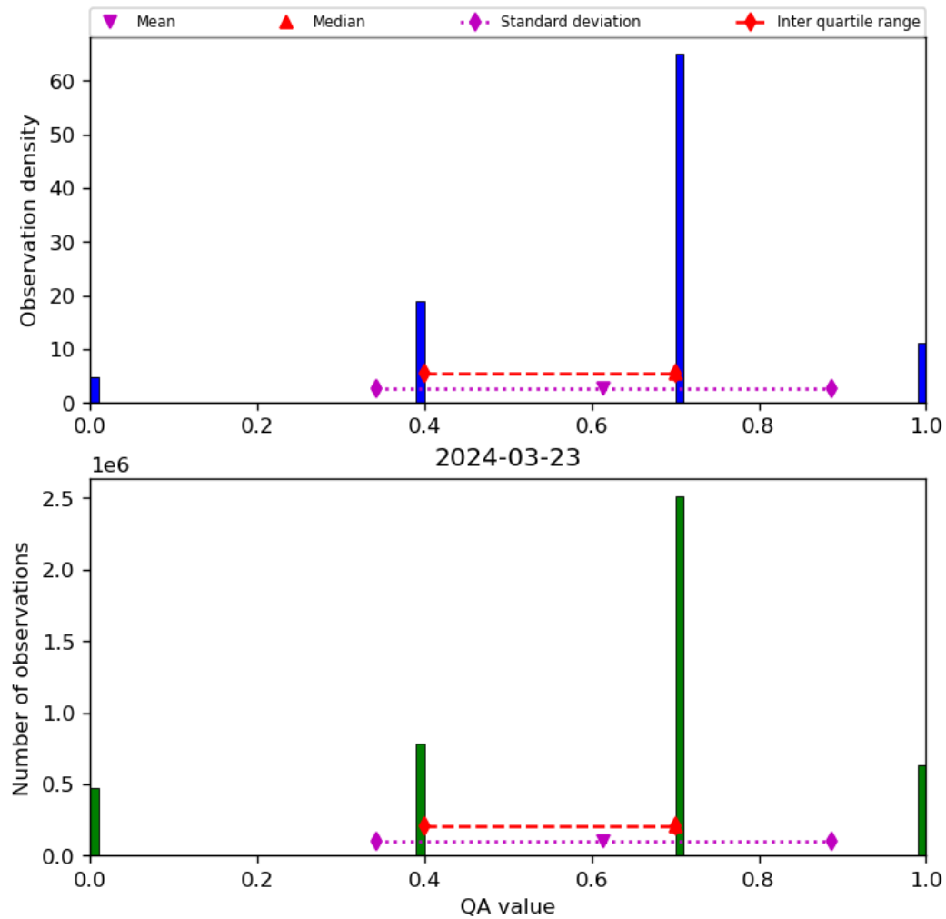
Figure 17: Histogram of “QA value” for 2024-03-23 to 2024-03-24
