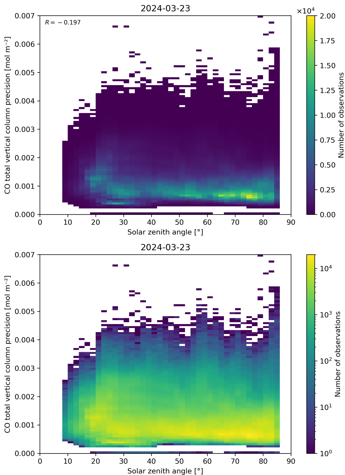
Figure 63: Scatter density plot of “Solar zenith angle” against “CO total vertical column precision” for 2024-03-23 to 2024-03-24.
