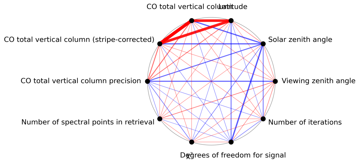
Figure 1: Map of correlation graph for 2024-03-23 to 2024-03-24.
