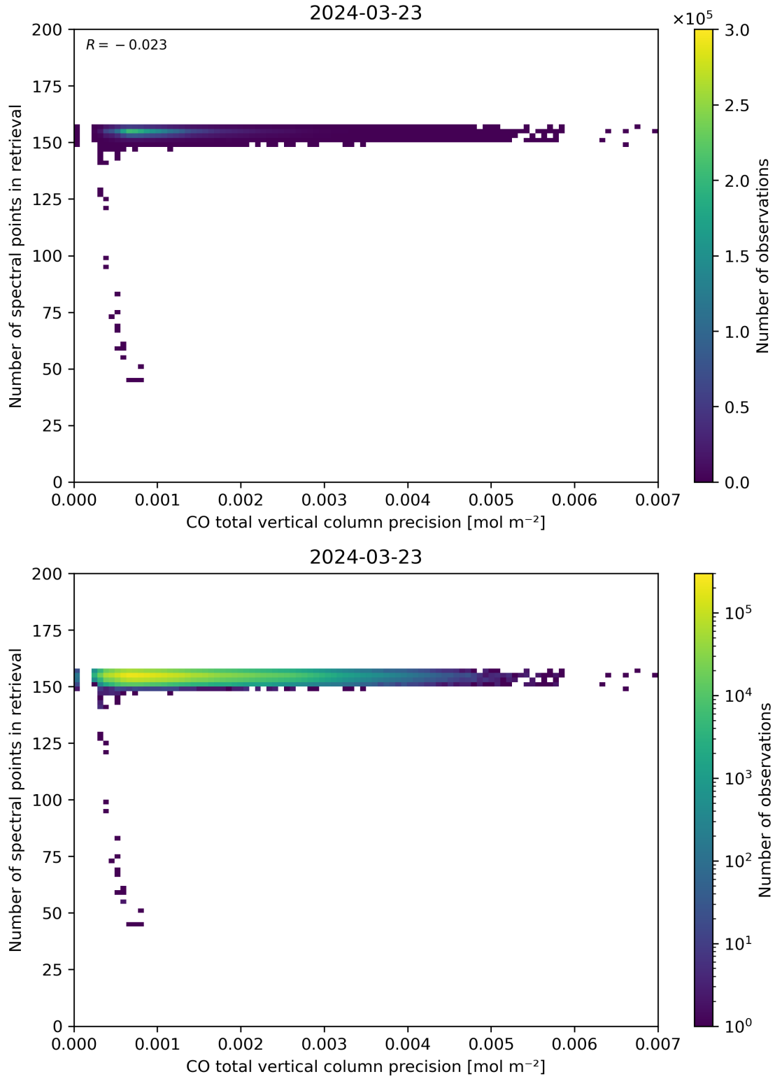
Figure 47: Scatter density plot of “CO total vertical column precision” against “Number of spectral points in retrieval” for 2024-03-23 to 2024-03-24.
