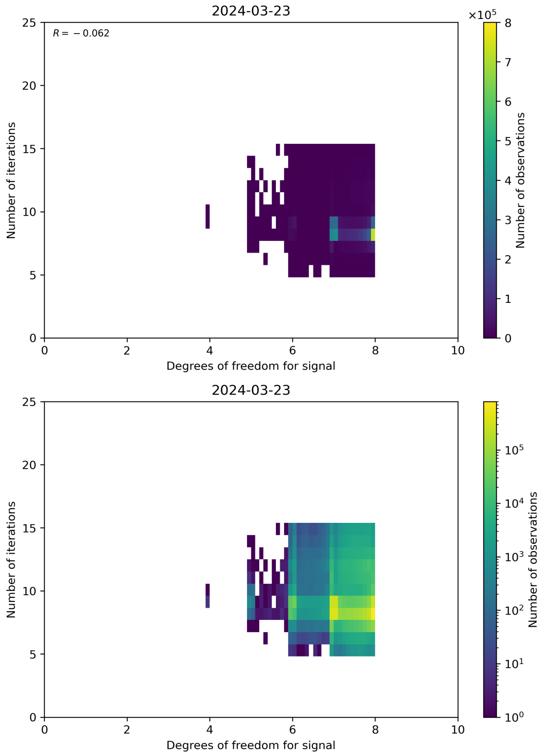
Figure 50: Scatter density plot of “Degrees of freedom for signal” against “Number of iterations” for 2024-03-23 to 2024-03-24.
