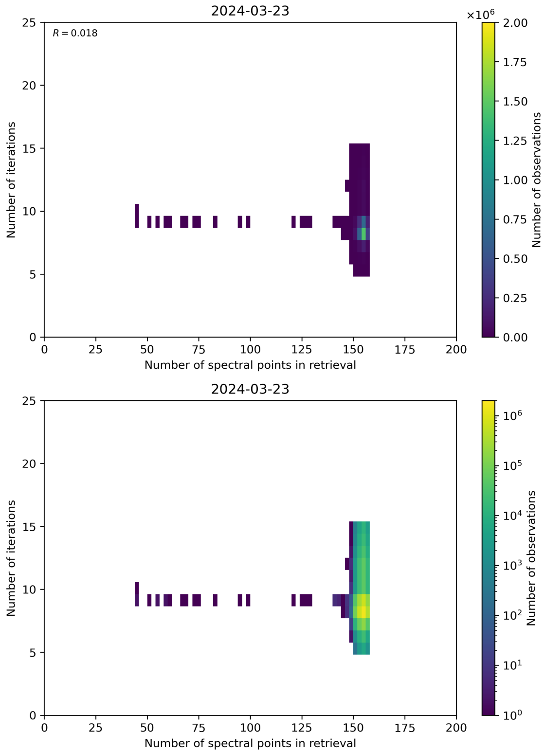
Figure 60: Scatter density plot of “Number of spectral points in retrieval” against “Number of iterations” for 2024-03-23 to 2024-03-24.
