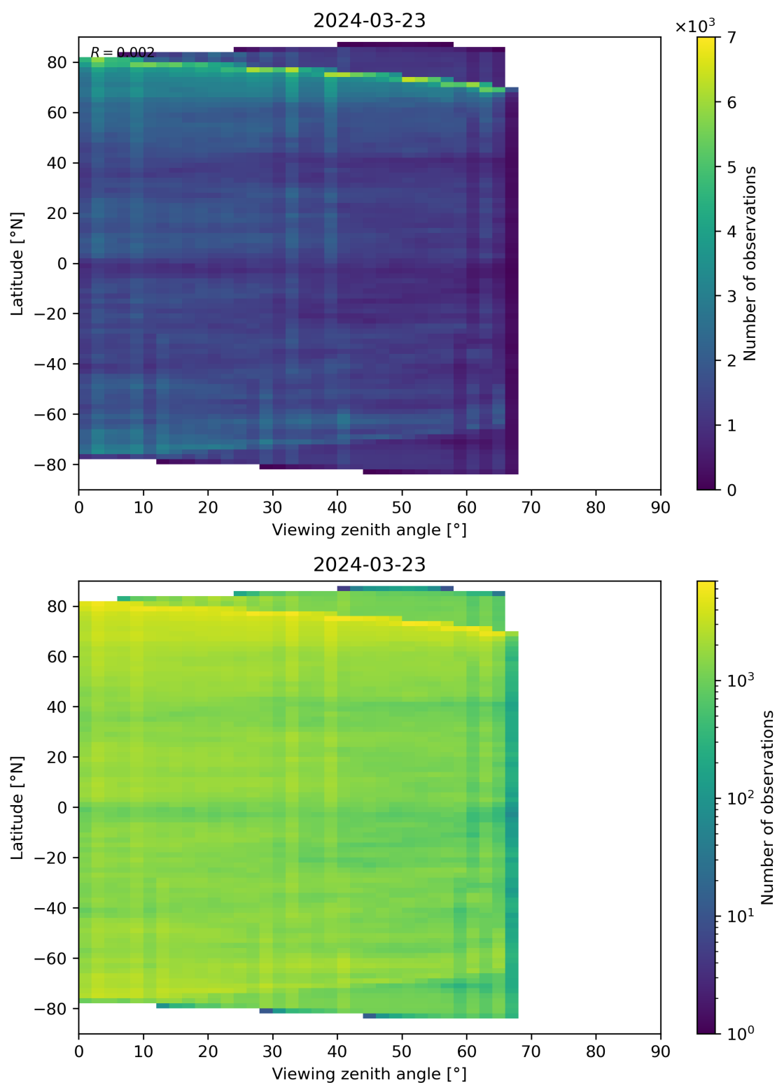
Figure 74: Scatter density plot of “Viewing zenith angle” against “Latitude” for 2024-03-23 to 2024-03-24.
