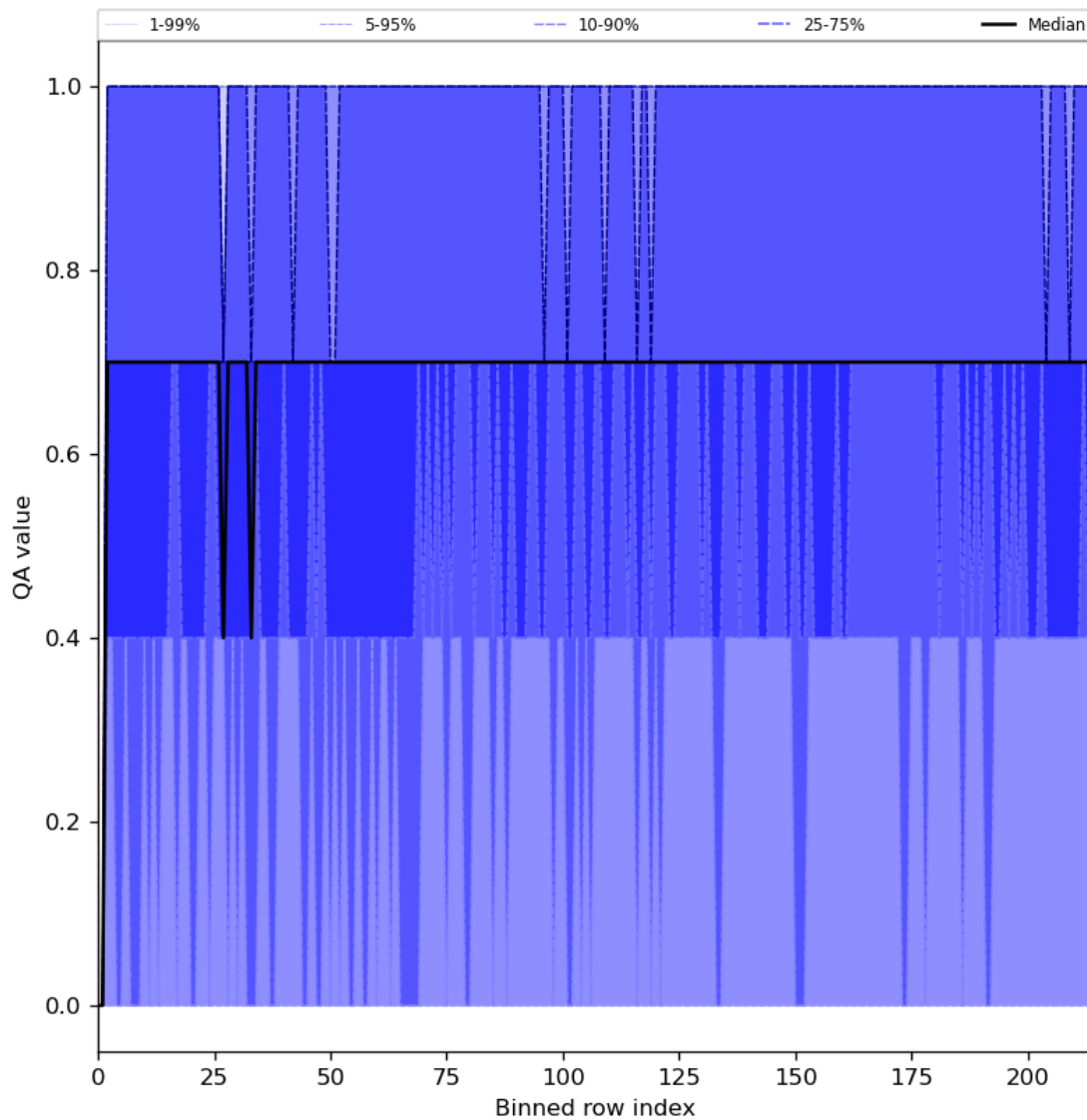
Figure 25: Along track statistics of “QA value” for 2024-03-23 to 2024-03-24
