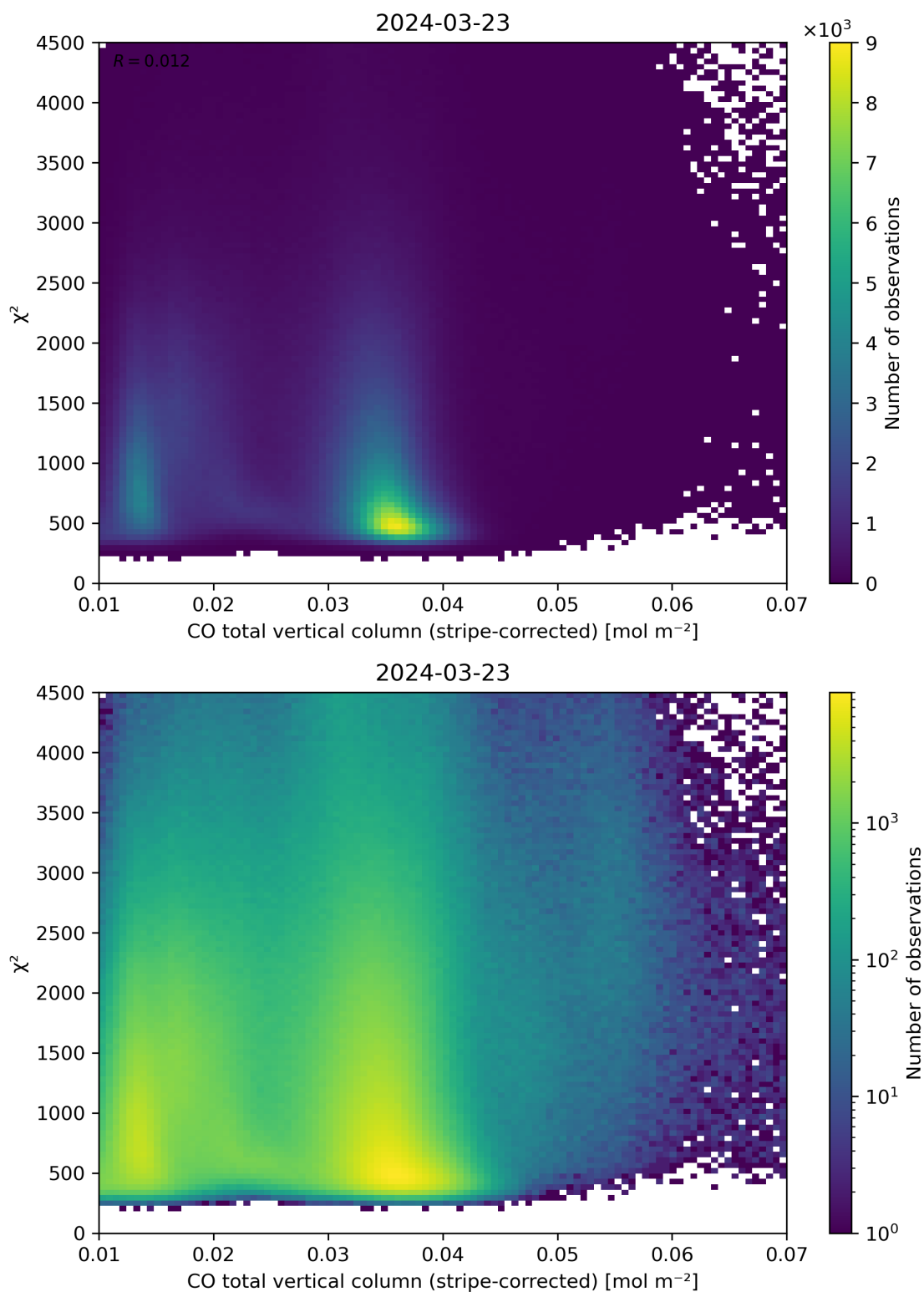
Figure 37: Scatter density plot of “CO total vertical column (stripe-corrected)” against “ \chi^2 ” for 2024-03-23 to 2024-03-24.
