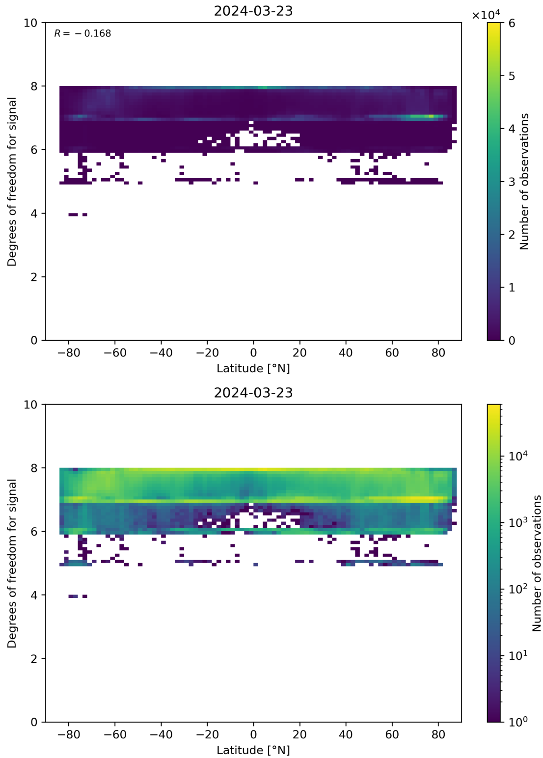
Figure 55: Scatter density plot of “Latitude” against “Degrees of freedom for signal” for 2024-03-23 to 2024-03-24.
