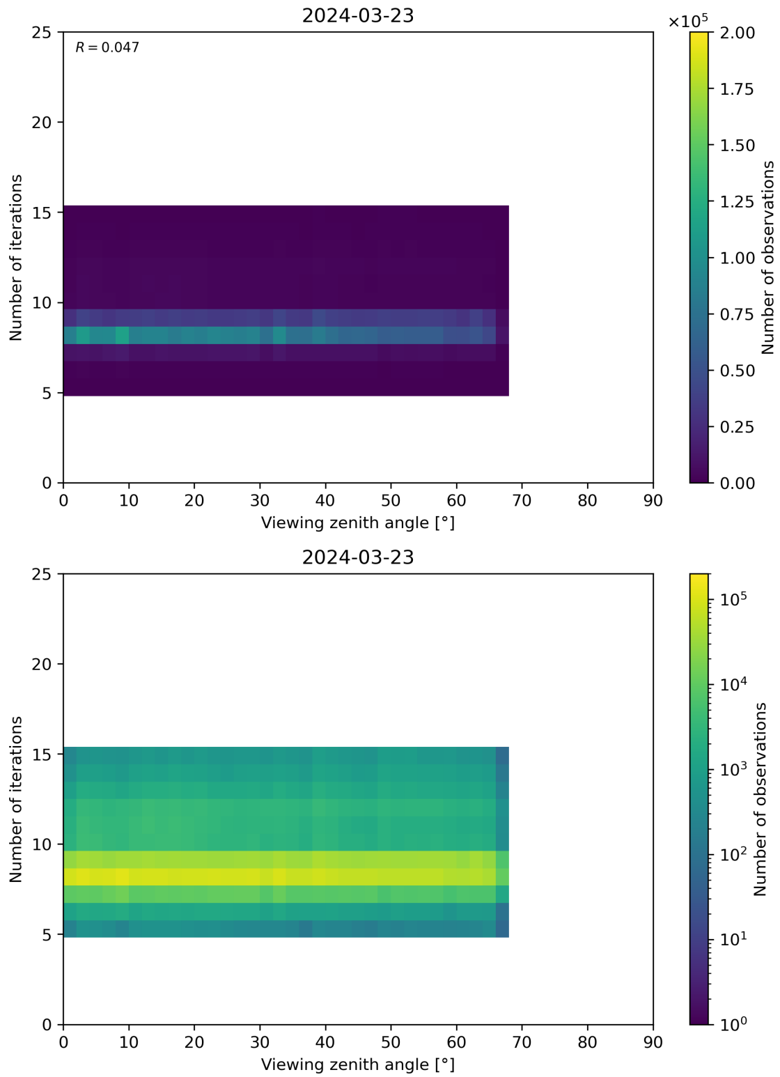
Figure 75: Scatter density plot of “Viewing zenith angle” against “Number of iterations” for 2024-03-23 to 2024-03-24.
