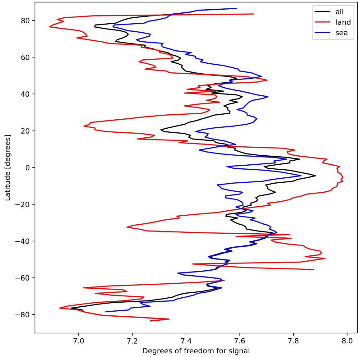
Figure 15: Zonal average of “Degrees of freedom for signal” for 2024-03-23 to 2024-03-24.
