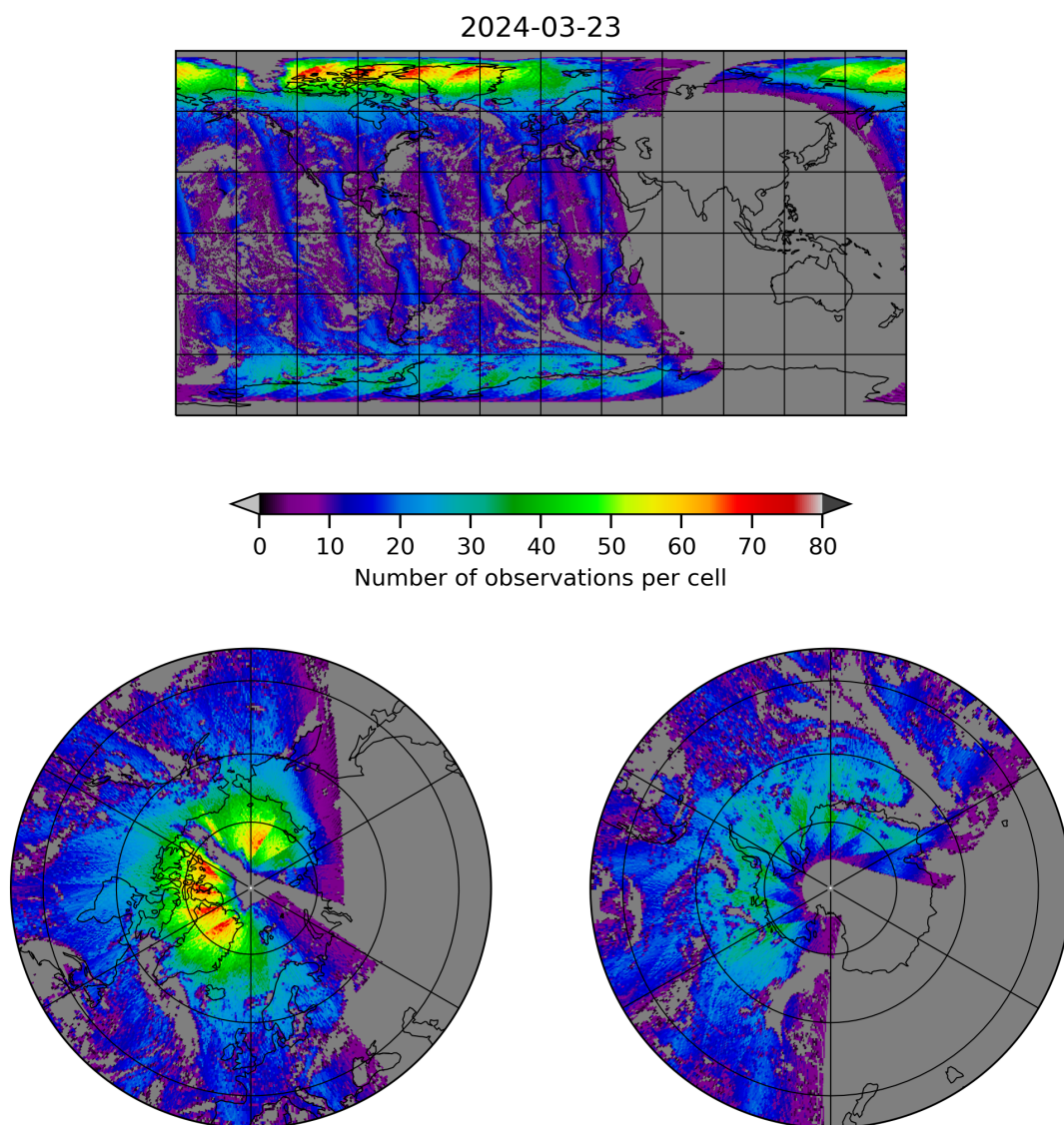
Figure 8: Map of the number of observations for 2024-03-23 to 2024-03-24
