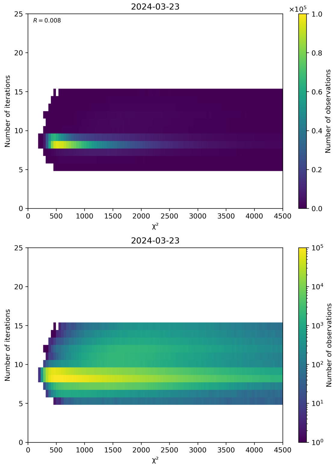
Figure 49: Scatter density plot of “ \chi^2 ” against “Number of iterations” for 2024-03-23 to 2024-03-24.
