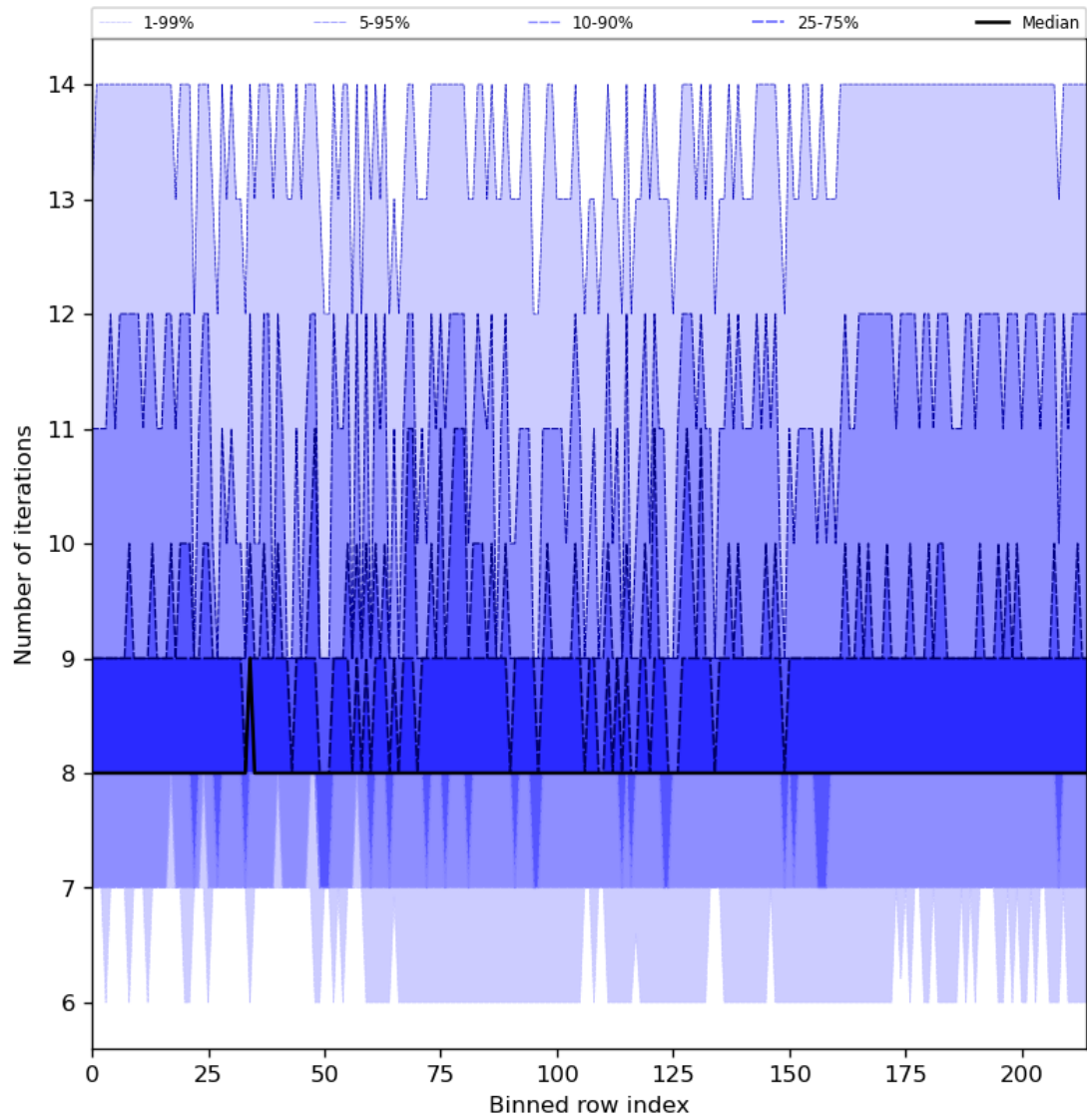
Figure 32: Along track statistics of “Number of iterations” for 2024-03-23 to 2024-03-24
