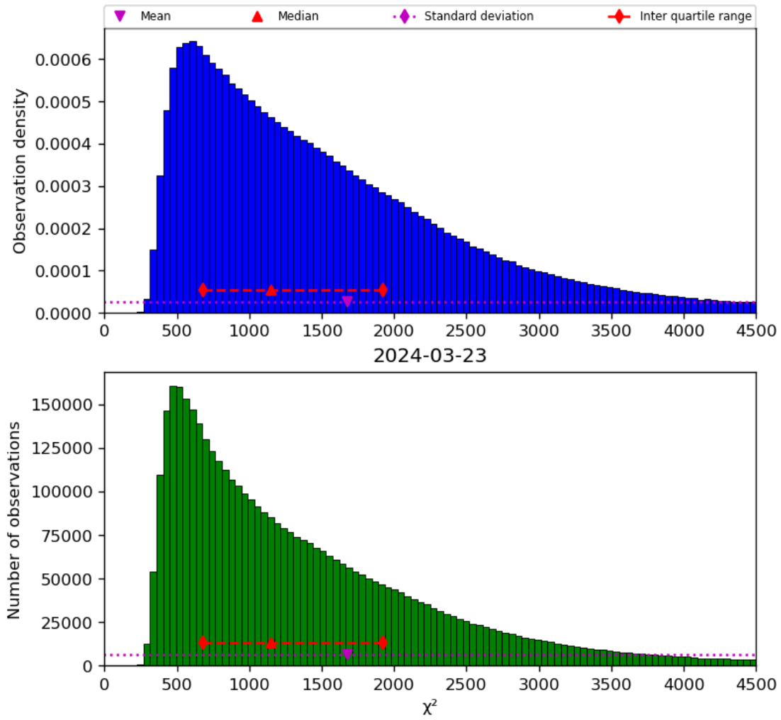
Figure 22: Histogram of “ \chi^2 ” for 2024-03-23 to 2024-03-24
