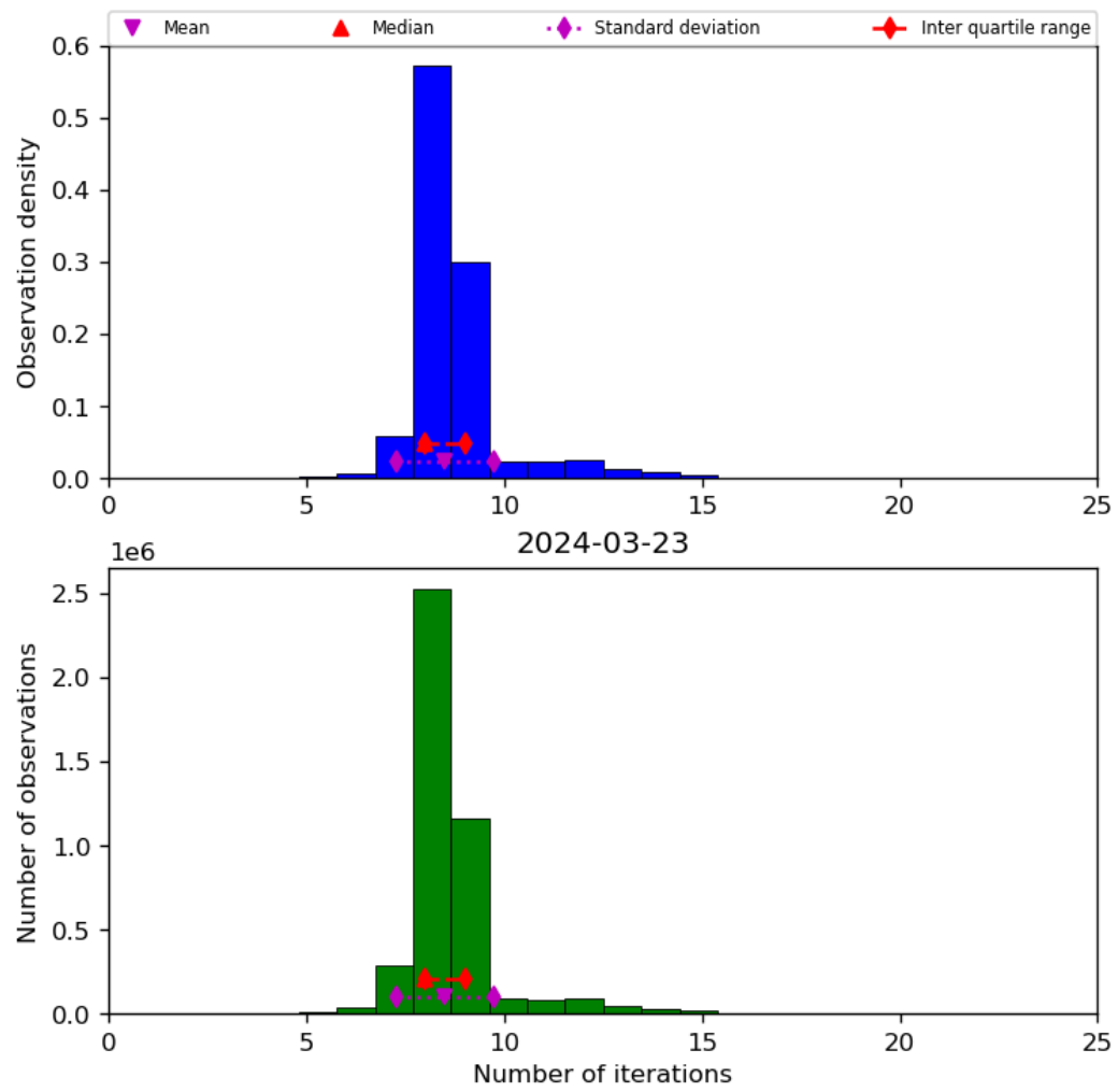
Figure 24: Histogram of “Number of iterations” for 2024-03-23 to 2024-03-24
