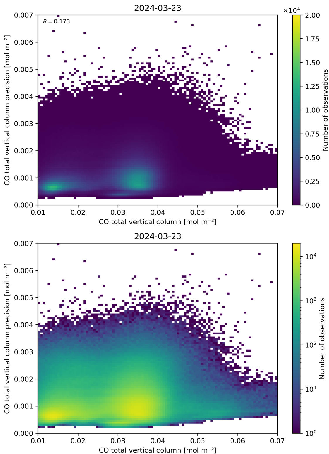
Figure 34: Scatter density plot of “CO total vertical column” against “CO total vertical column precision” for 2024-03-23 to 2024-03-24.
