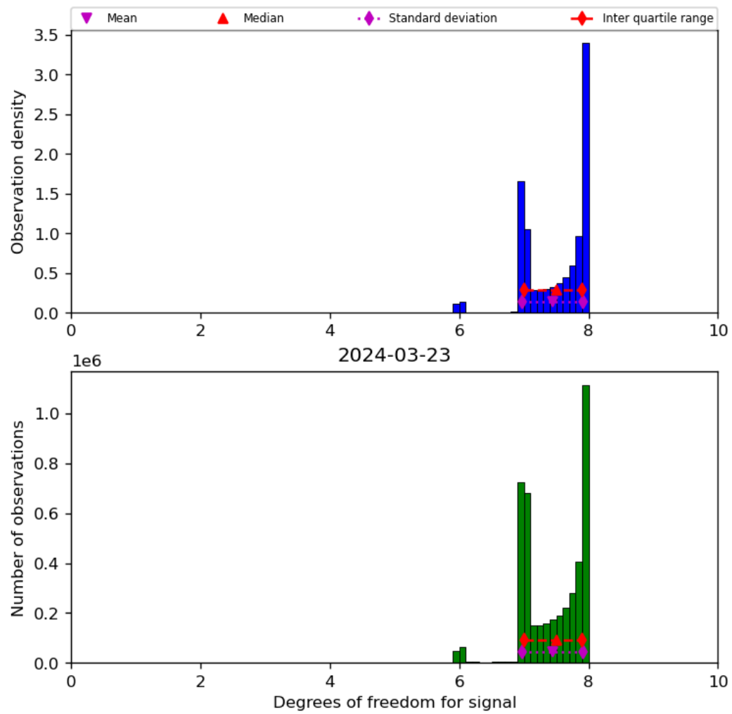
Figure 23: Histogram of “Degrees of freedom for signal” for 2024-03-23 to 2024-03-24
