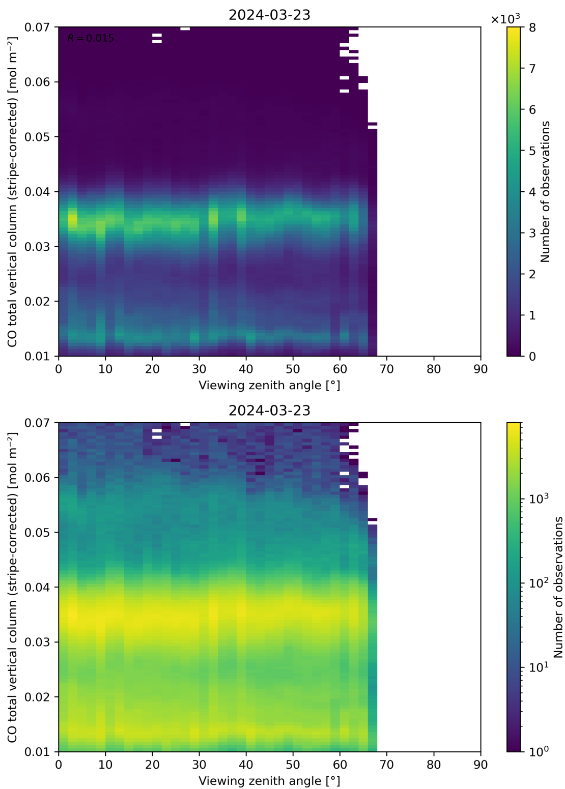
Figure 70: Scatter density plot of “Viewing zenith angle” against “CO total vertical column (stripe-corrected)” for 2024-03-23 to 2024-03-24.
