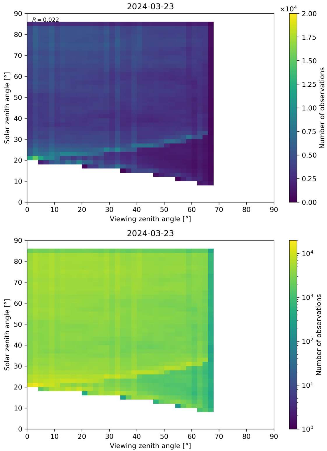
Figure 77: Scatter density plot of “Viewing zenith angle” against “Solar zenith angle” for 2024-03-23 to 2024-03-24.
