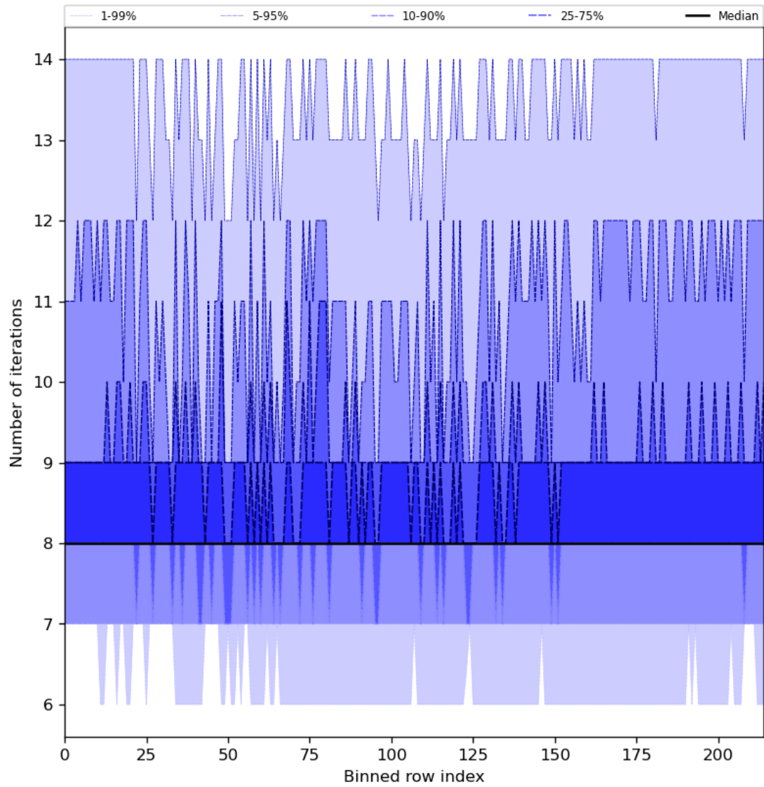
Figure 32: Along track statistics of “Number of iterations” for 2024-03-23 to 2024-03-25
