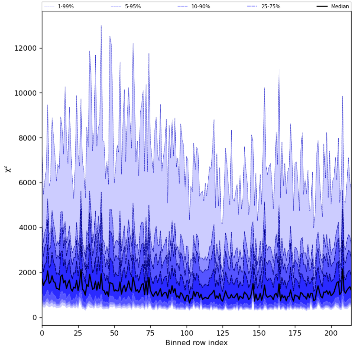
Figure 30: Along track statistics of “ \chi^2 ” for 2024-03-23 to 2024-03-25
