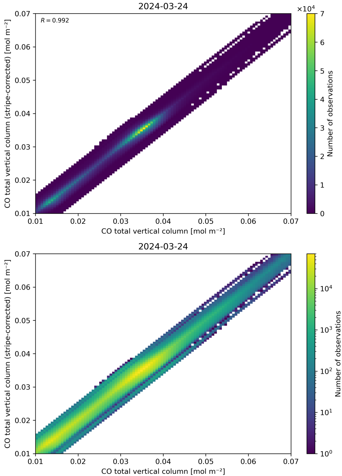
Figure 33: Scatter density plot of “CO total vertical column” against “CO total vertical column (stripe-corrected)” for 2024-03-23 to 2024-03-25.
