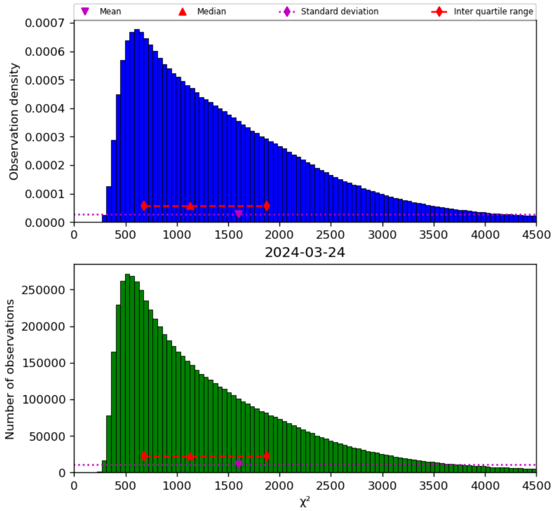
Figure 22: Histogram of “ \chi^2 ” for 2024-03-23 to 2024-03-25
