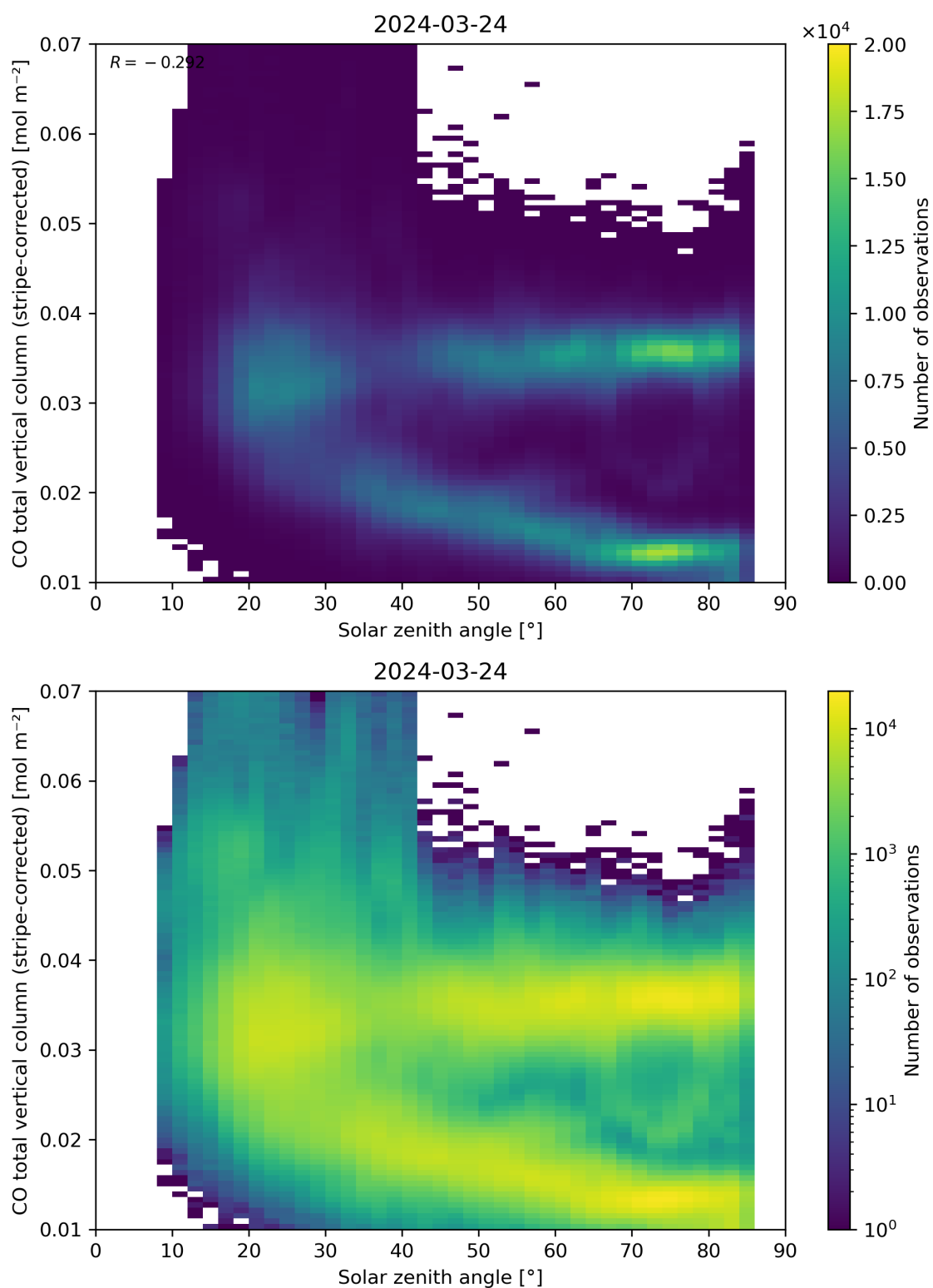
Figure 62: Scatter density plot of “Solar zenith angle” against “CO total vertical column (stripe-corrected)” for 2024-03-23 to 2024-03-25.
