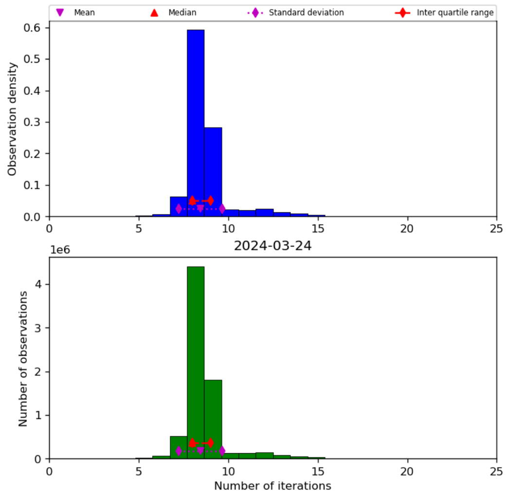
Figure 24: Histogram of “Number of iterations” for 2024-03-23 to 2024-03-25
