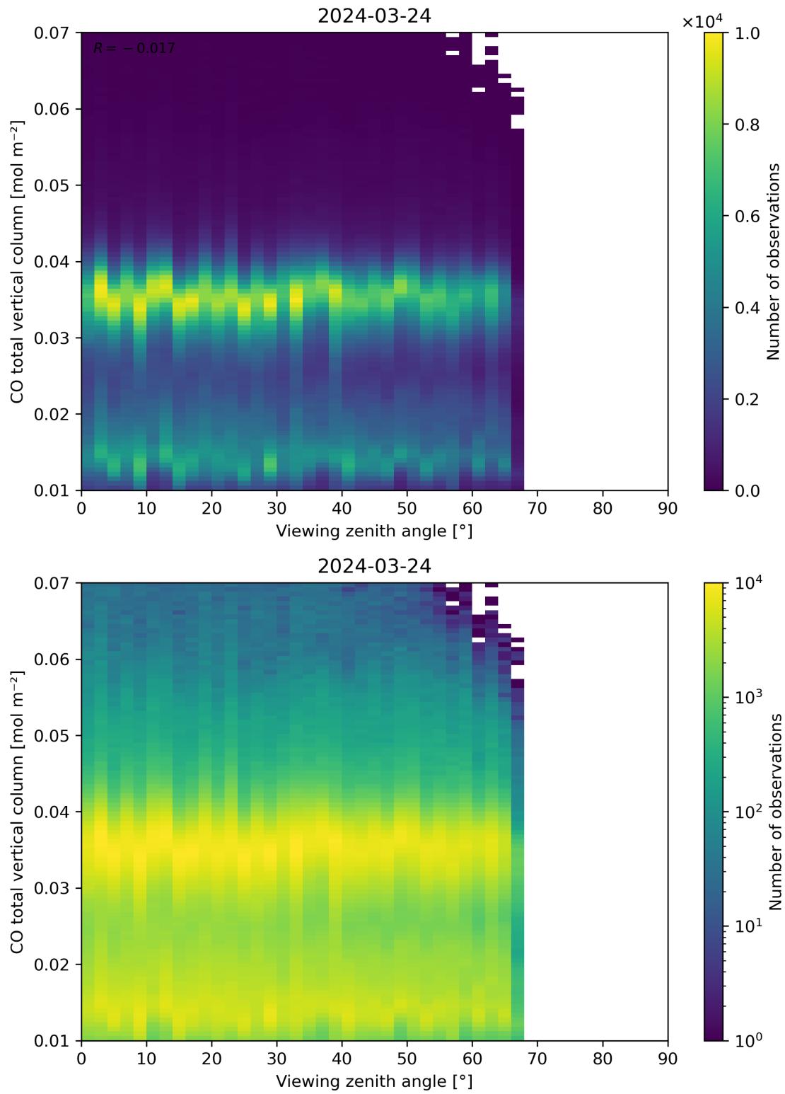
Figure 69: Scatter density plot of “Viewing zenith angle” against “CO total vertical column” for 2024-03-23 to 2024-03-25.
