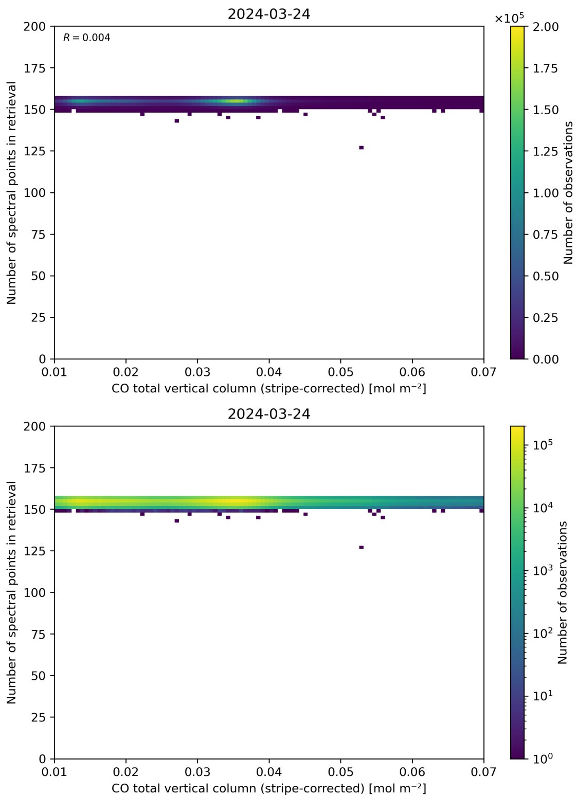
Figure 40: Scatter density plot of “CO total vertical column (stripe-corrected)” against “Number of spectral points in retrieval” for 2024-03-23 to 2024-03-25.
