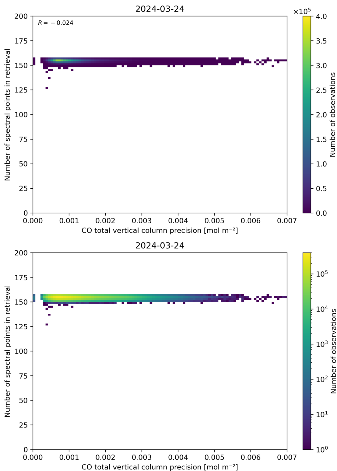
Figure 47: Scatter density plot of “CO total vertical column precision” against “Number of spectral points in retrieval” for 2024-03-23 to 2024-03-25.
