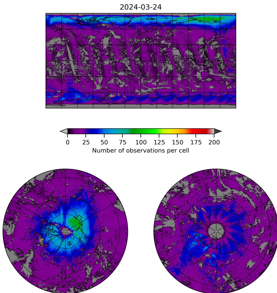
Figure 8: Map of the number of observations for 2024-03-23 to 2024-03-25
