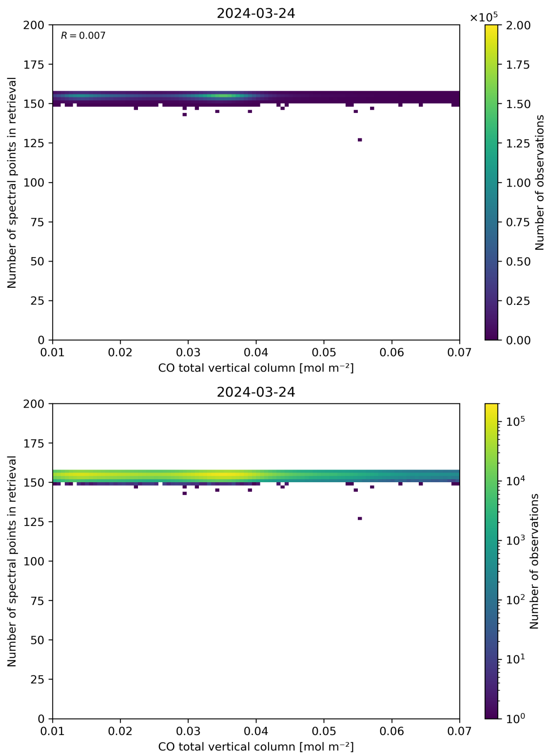
Figure 43: Scatter density plot of “CO total vertical column” against “Number of spectral points in retrieval” for 2024-03-23 to 2024-03-25.
