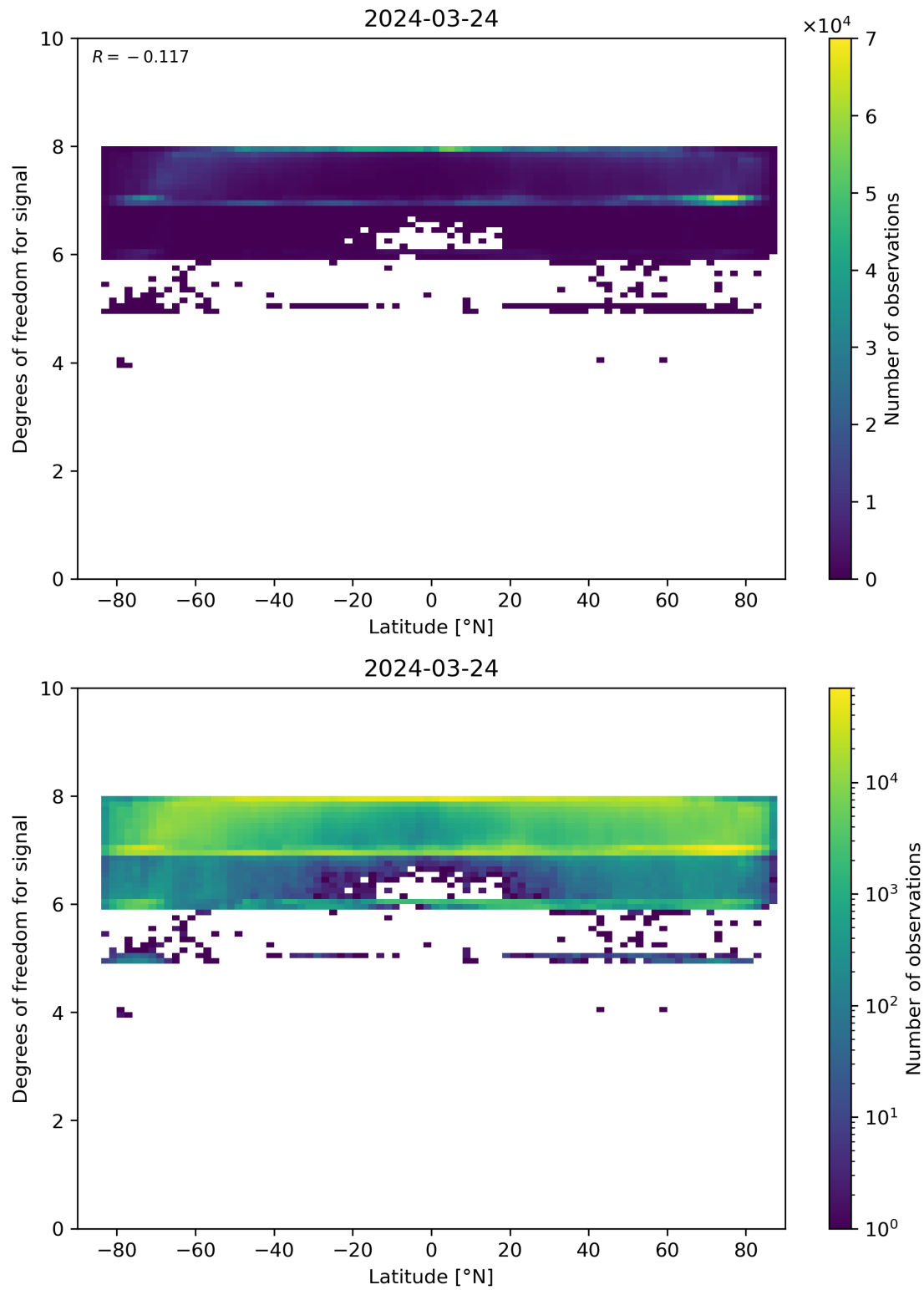
Figure 55: Scatter density plot of “Latitude” against “Degrees of freedom for signal” for 2024-03-23 to 2024-03-25.
