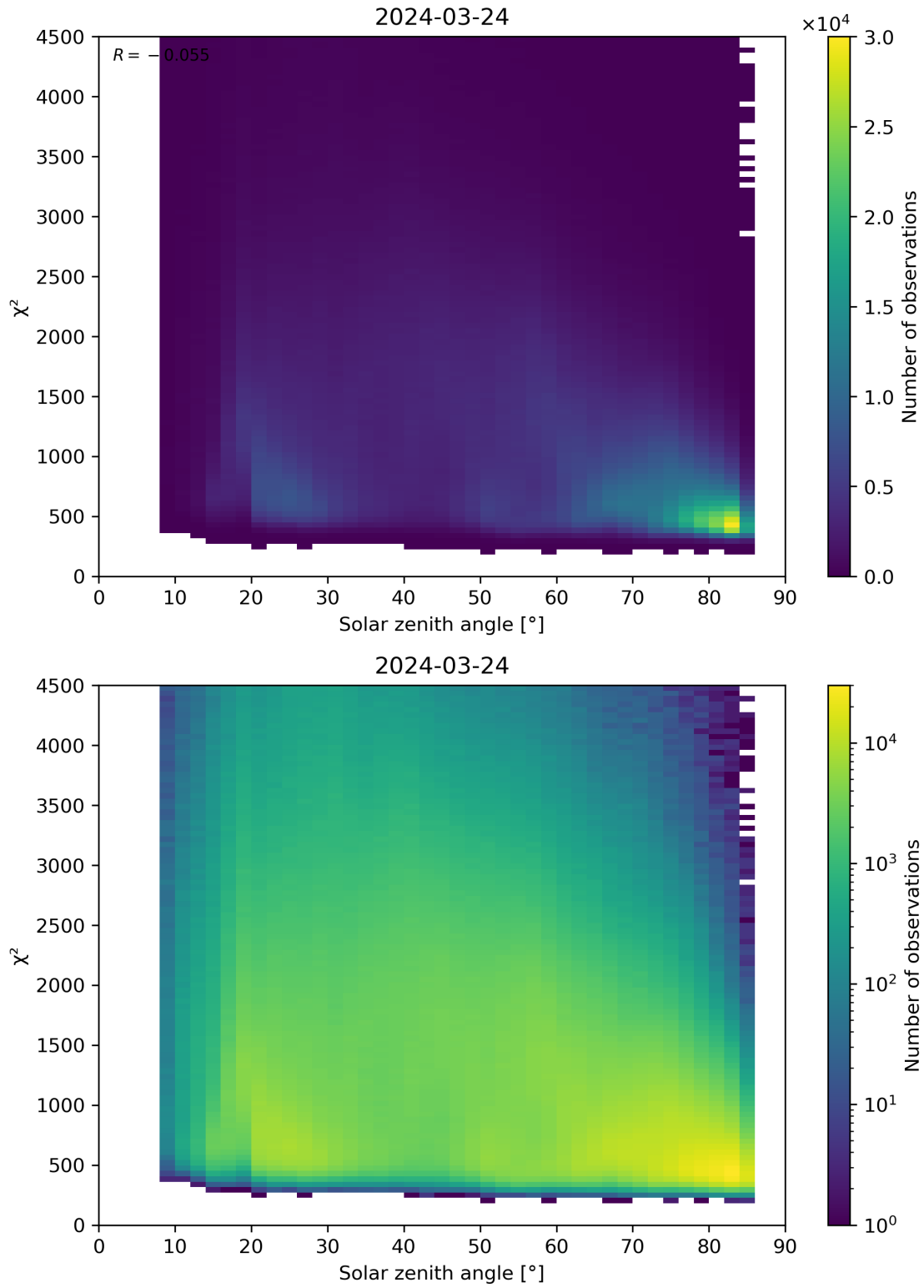
Figure 64: Scatter density plot of “Solar zenith angle” against “ \chi^2 ” for 2024-03-23 to 2024-03-25.
