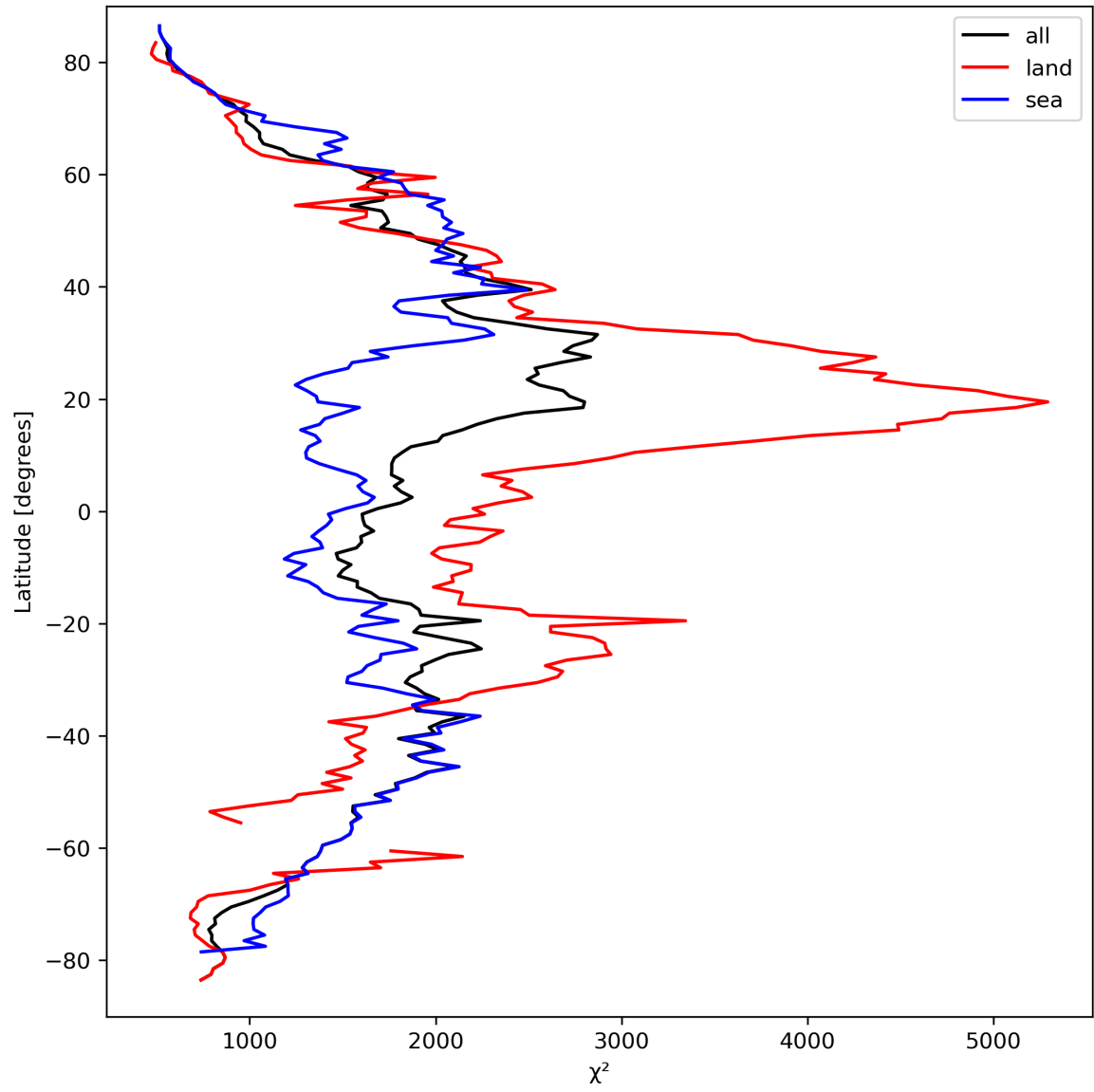
Figure 14: Zonal average of “ \chi^2 ” for 2024-03-23 to 2024-03-25.
