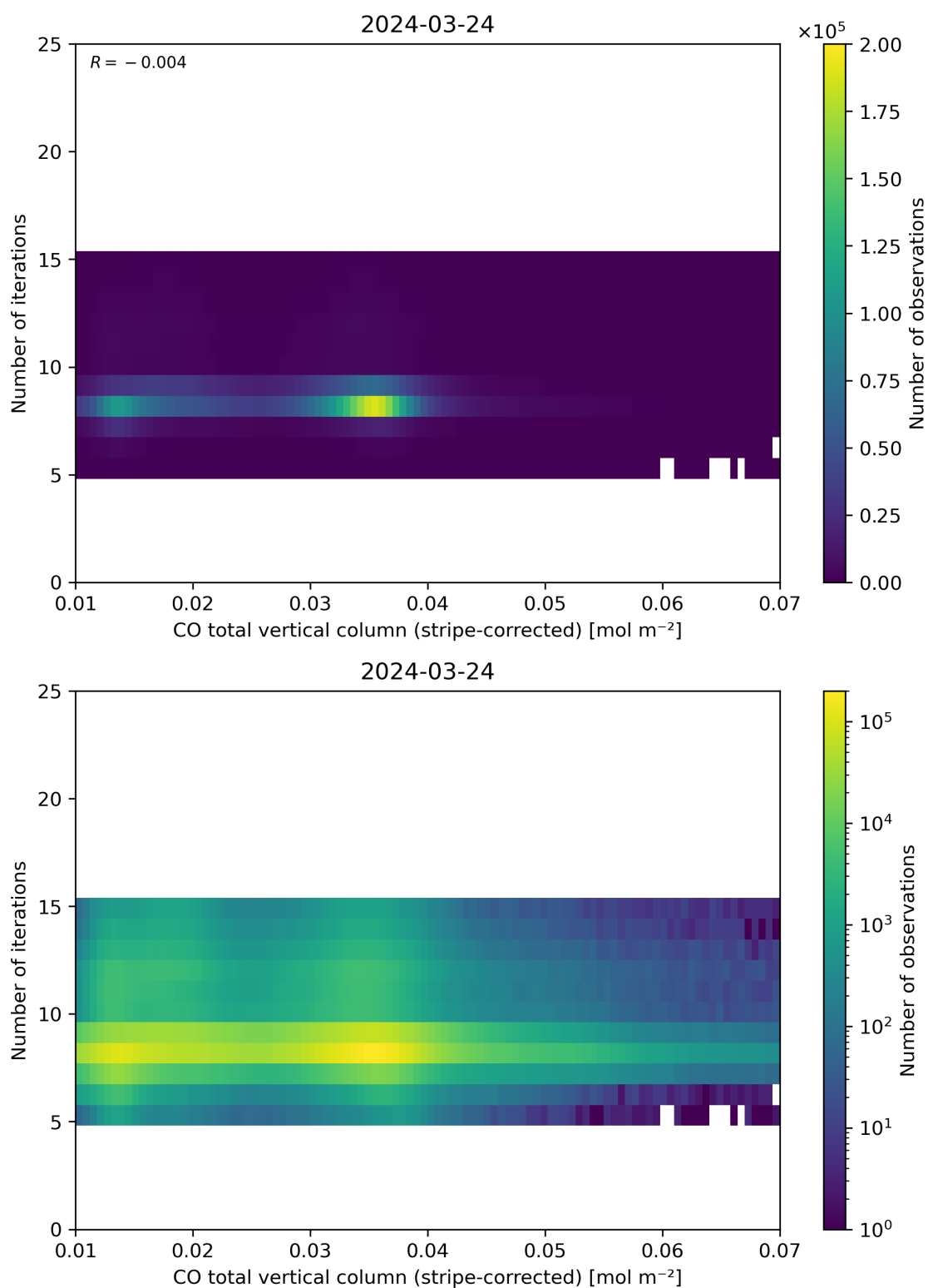
Figure 39: Scatter density plot of “CO total vertical column (stripe-corrected)” against “Number of iterations” for 2024-03-23 to 2024-03-25.
