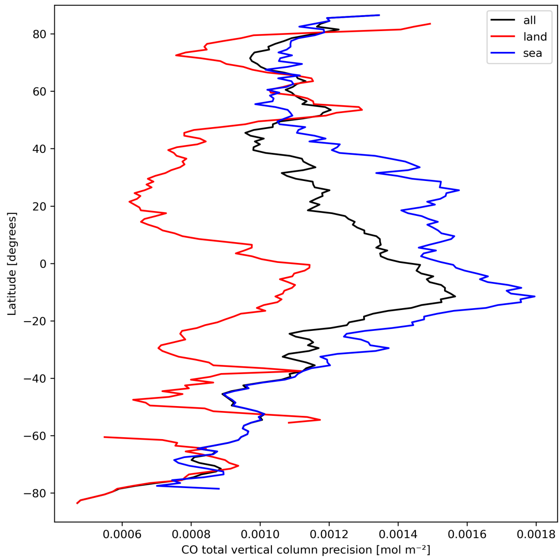
Figure 12: Zonal average of “CO total vertical column precision” for 2024-03-23 to 2024-03-25.
