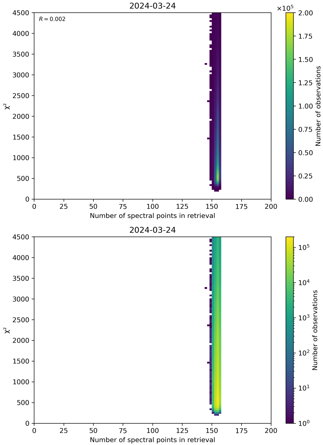
Figure 58: Scatter density plot of “Number of spectral points in retrieval” against “ \chi^2 ” for 2024-03-23 to 2024-03-25.
