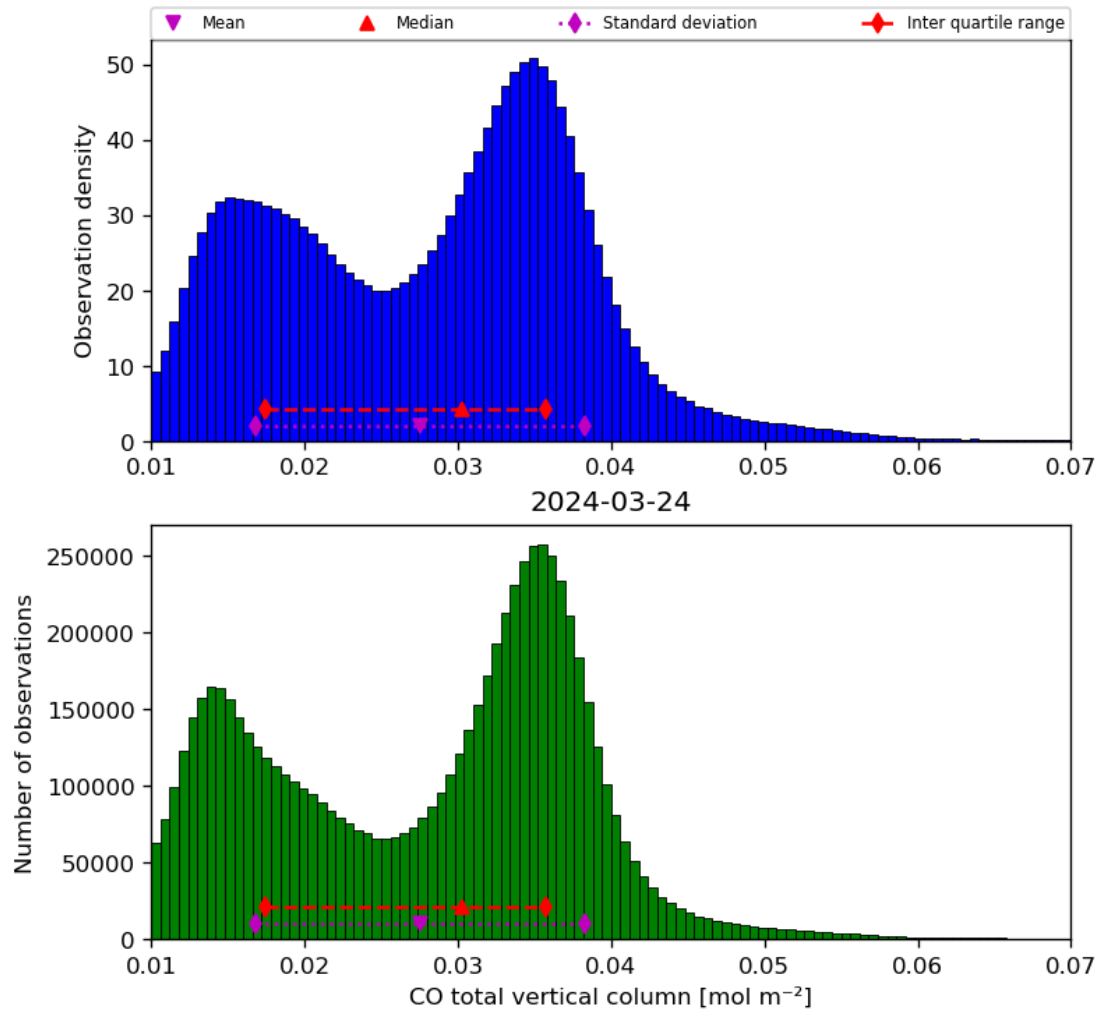
Figure 18: Histogram of “CO total vertical column” for 2024-03-23 to 2024-03-25
