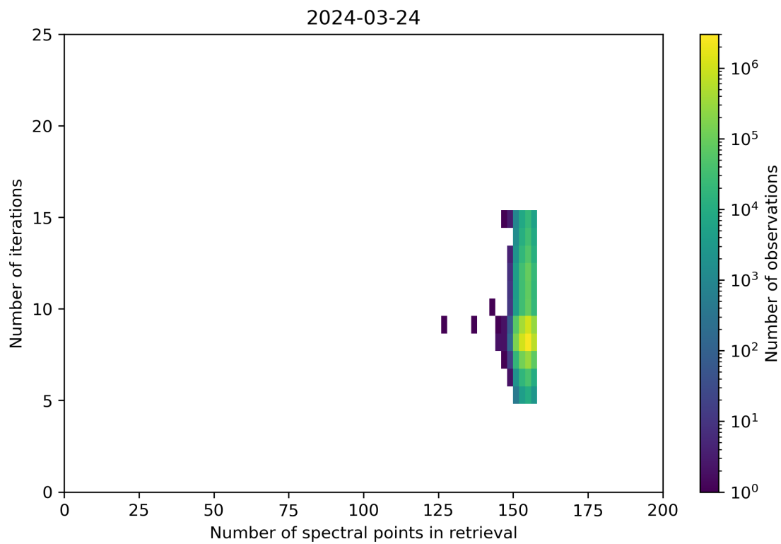
Figure 60: Scatter density plot of “Number of spectral points in retrieval” against “Number of iterations” for 2024-03-23 to 2024-03-25.
