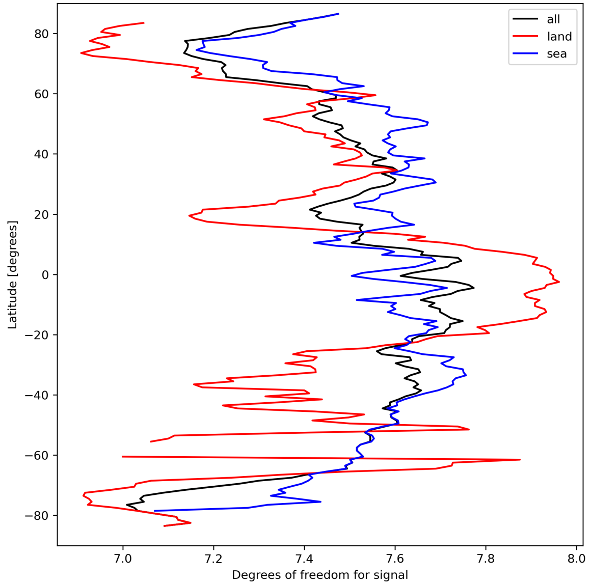
Figure 15: Zonal average of “Degrees of freedom for signal” for 2024-03-23 to 2024-03-25.
