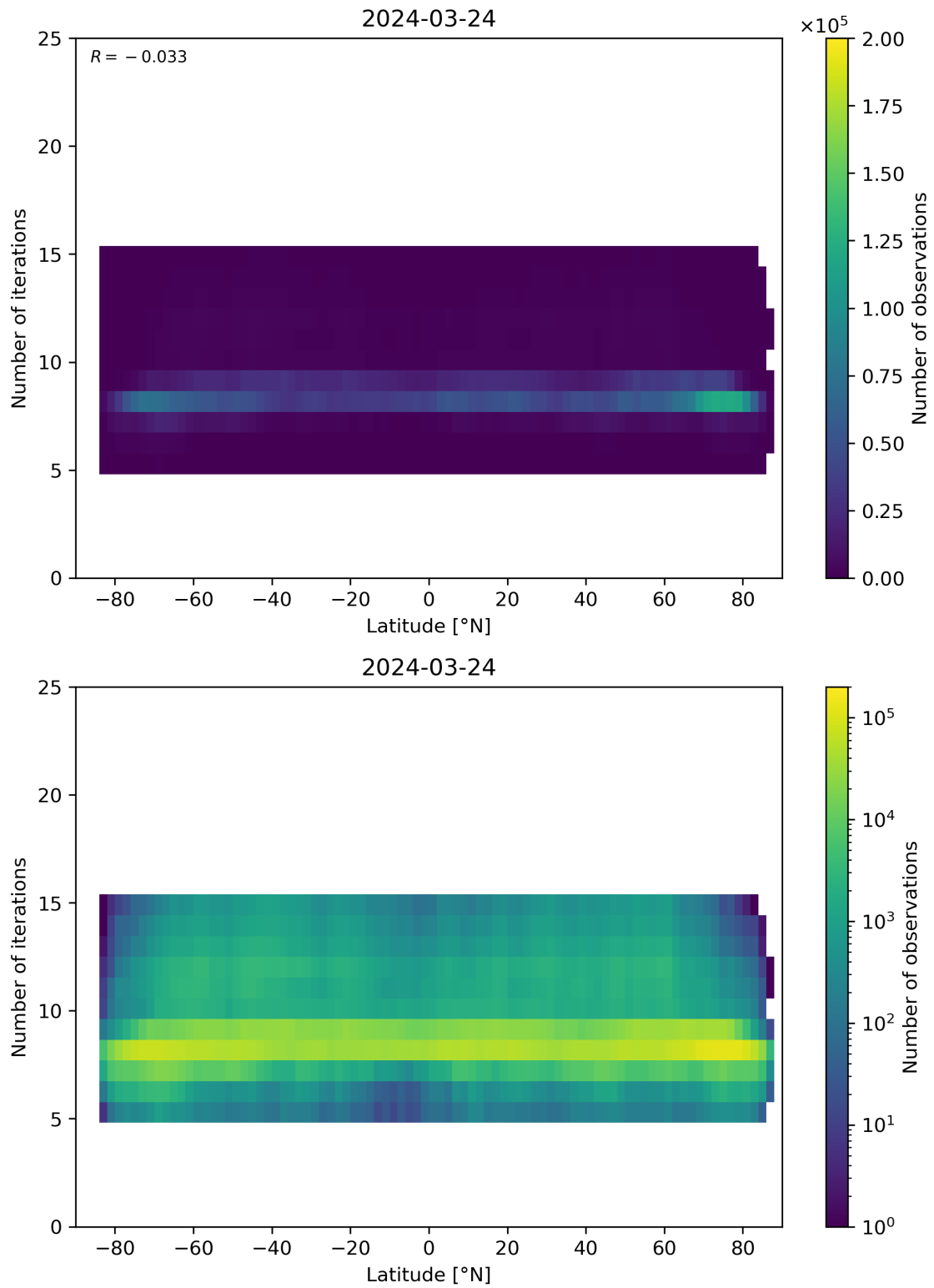
Figure 56: Scatter density plot of “Latitude” against “Number of iterations” for 2024-03-23 to 2024-03-25.
