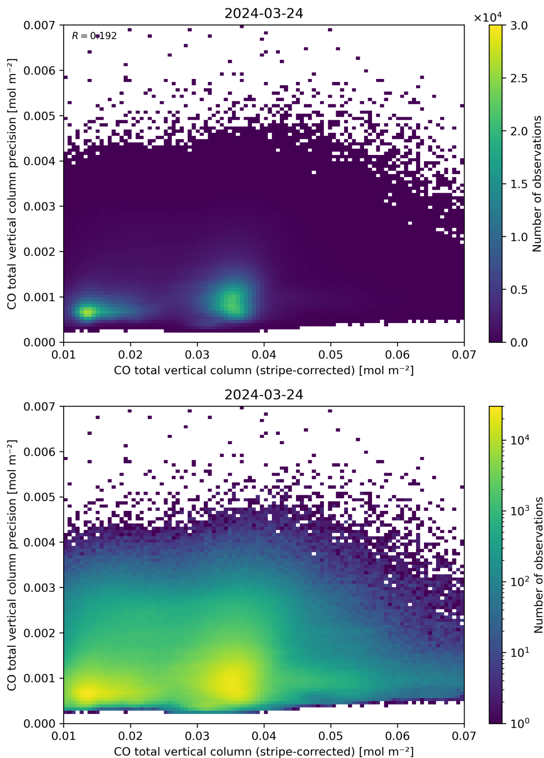
Figure 36: Scatter density plot of “CO total vertical column (stripe-corrected)” against “CO total vertical column precision” for 2024-03-23 to 2024-03-25.
