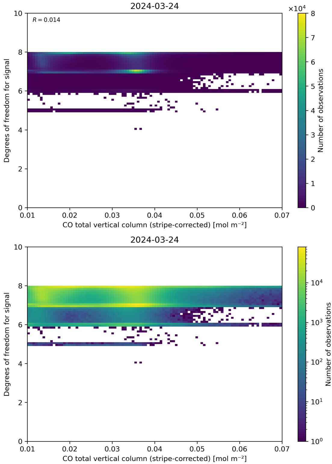
Figure 38: Scatter density plot of “CO total vertical column (stripe-corrected)” against “Degrees of freedom for signal” for 2024-03-23 to 2024-03-25.
