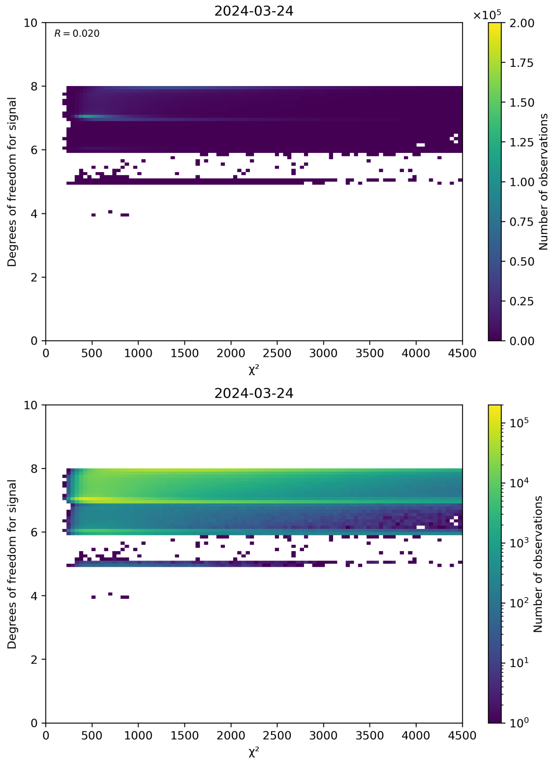
Figure 48: Scatter density plot of “ \chi^2 ” against “Degrees of freedom for signal” for 2024-03-23 to 2024-03-25.
