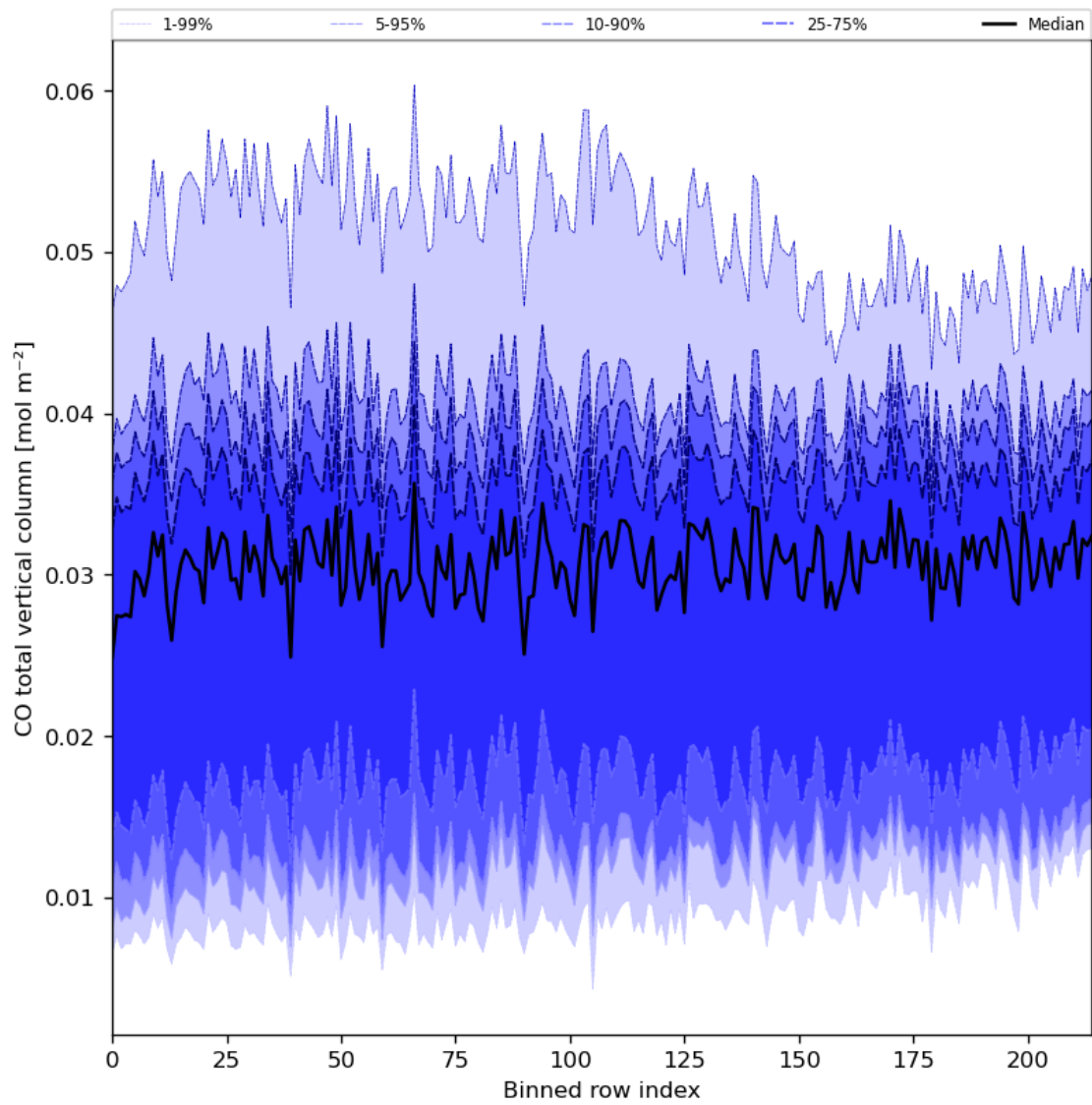
Figure 26: Along track statistics of “CO total vertical column” for 2024-03-23 to 2024-03-25
