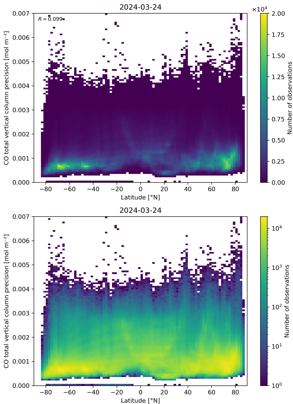
Figure 53: Scatter density plot of “Latitude” against “CO total vertical column precision” for 2024-03-23 to 2024-03-25.
