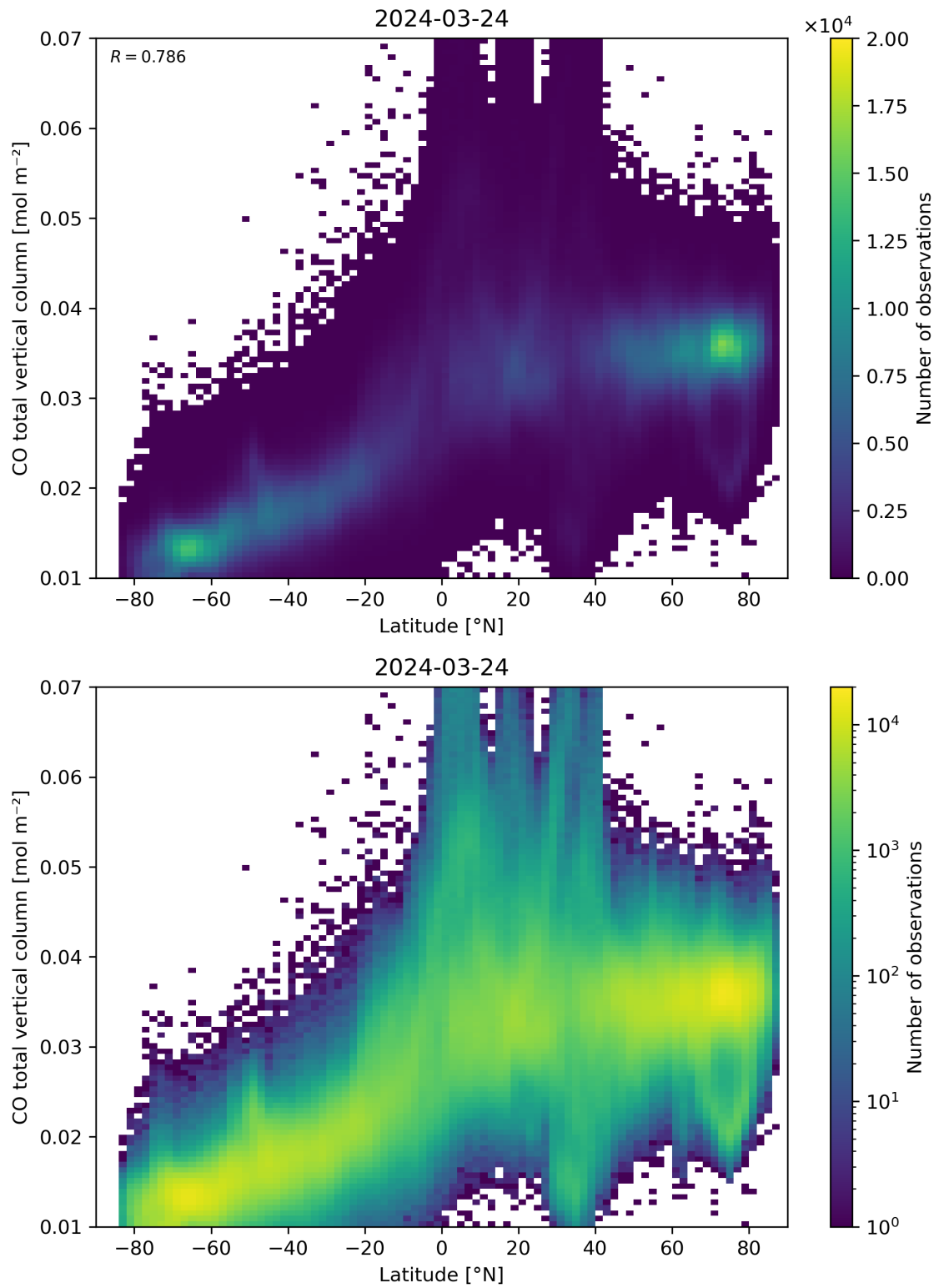
Figure 51: Scatter density plot of “Latitude” against “CO total vertical column” for 2024-03-23 to 2024-03-25.
