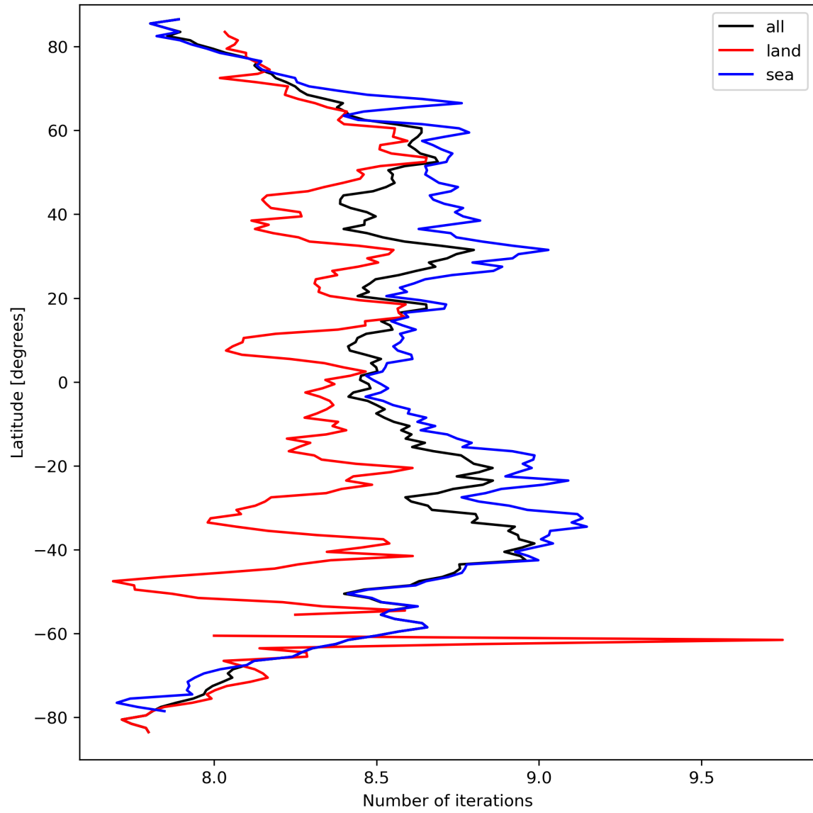
Figure 16: Zonal average of “Number of iterations” for 2024-03-23 to 2024-03-25.
