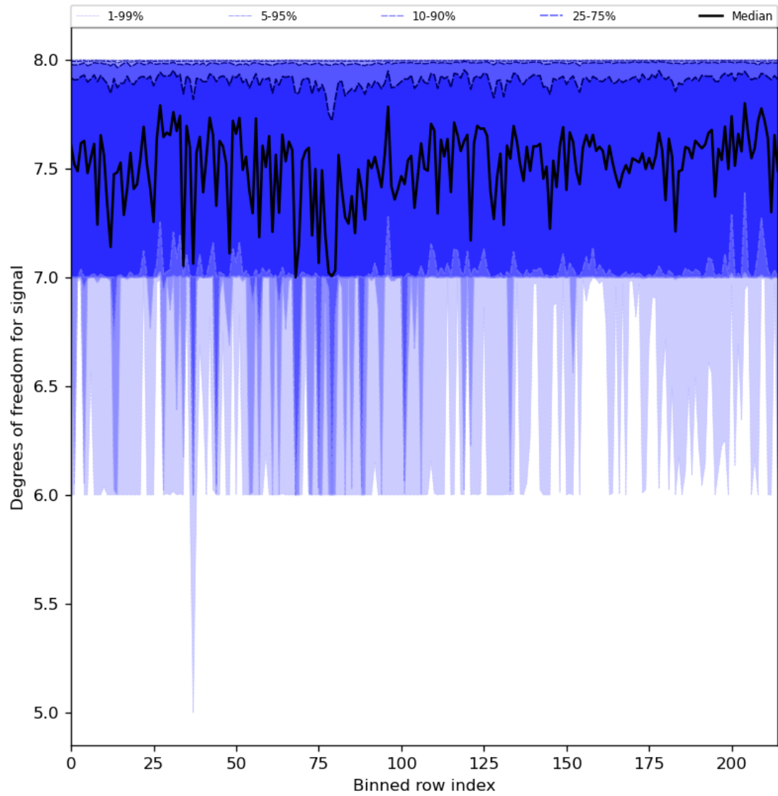
Figure 31: Along track statistics of “Degrees of freedom for signal” for 2024-03-23 to 2024-03-25
