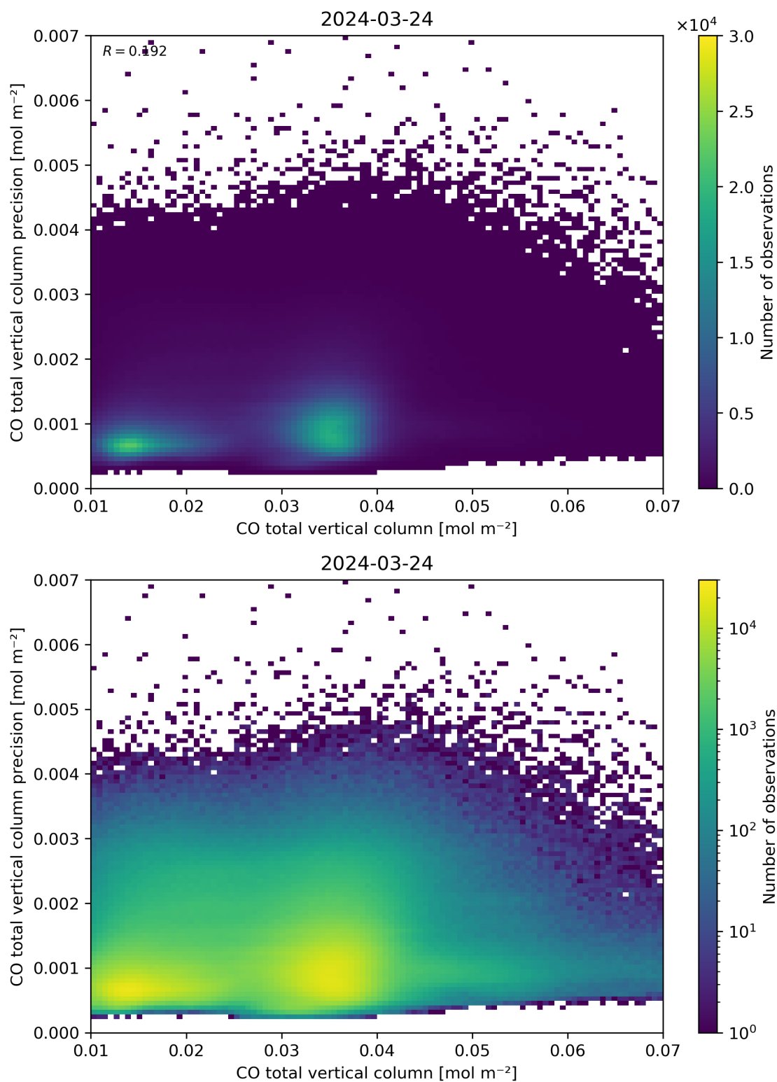
Figure 34: Scatter density plot of “CO total vertical column” against “CO total vertical column precision” for 2024-03-23 to 2024-03-25.
