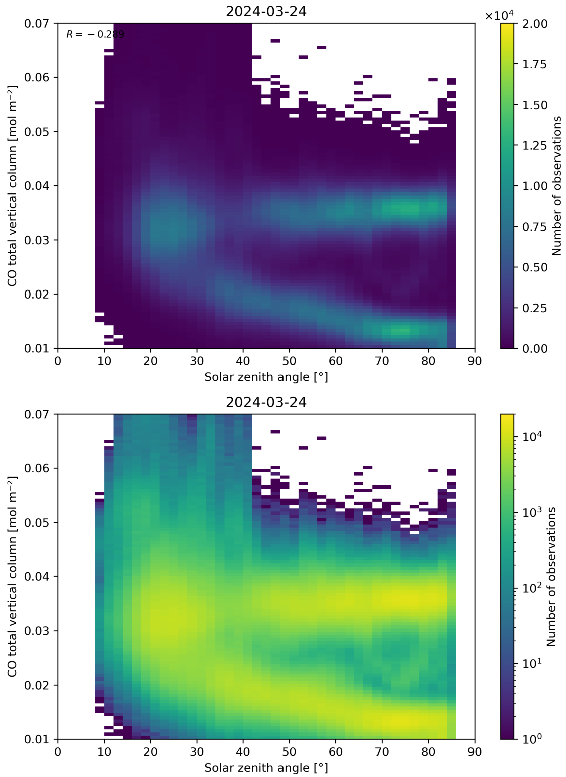
Figure 61: Scatter density plot of “Solar zenith angle” against “CO total vertical column” for 2024-03-23 to 2024-03-25.
