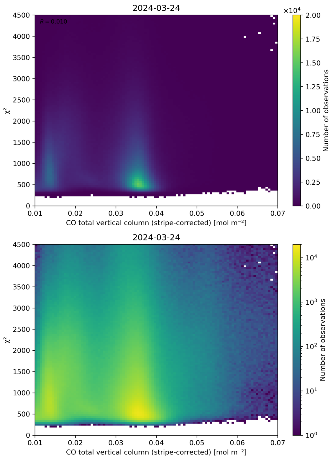
Figure 37: Scatter density plot of “CO total vertical column (stripe-corrected)” against “ \chi^2 ” for 2024-03-23 to 2024-03-25.
