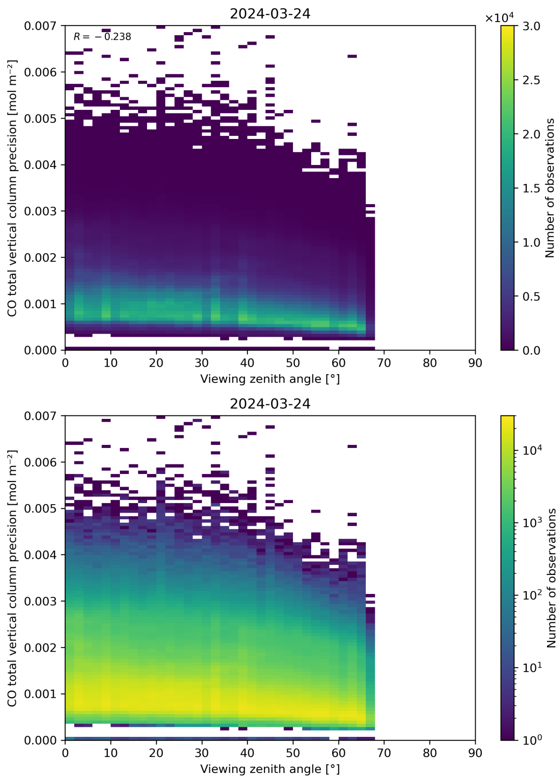
Figure 71: Scatter density plot of “Viewing zenith angle” against “CO total vertical column precision” for 2024-03-23 to 2024-03-25.
