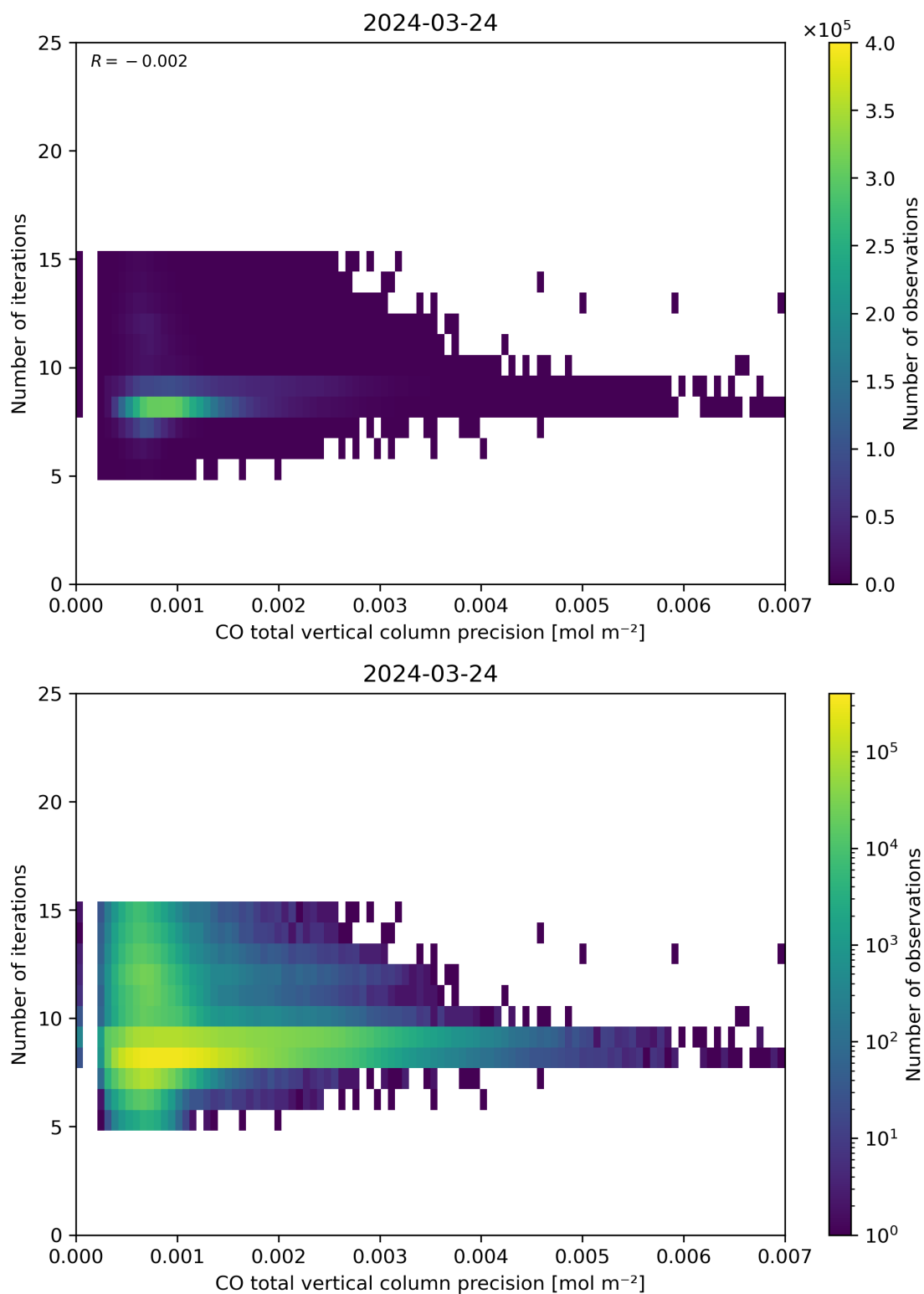
Figure 46: Scatter density plot of “CO total vertical column precision” against “Number of iterations” for 2024-03-23 to 2024-03-25.
