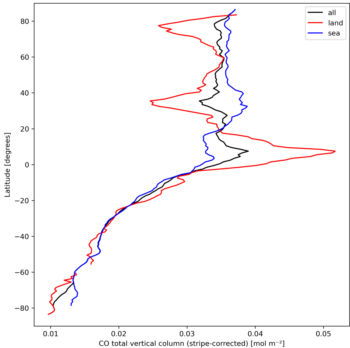
Figure 11: Zonal average of “CO total vertical column (stripe-corrected)” for 2024-03-23 to 2024-03-25.
