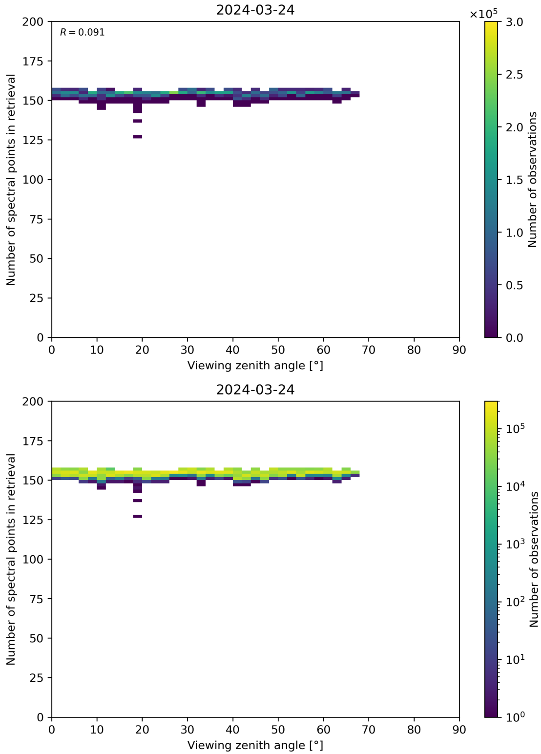
Figure 76: Scatter density plot of “Viewing zenith angle” against “Number of spectral points in retrieval” for 2024-03-23 to 2024-03-25.
