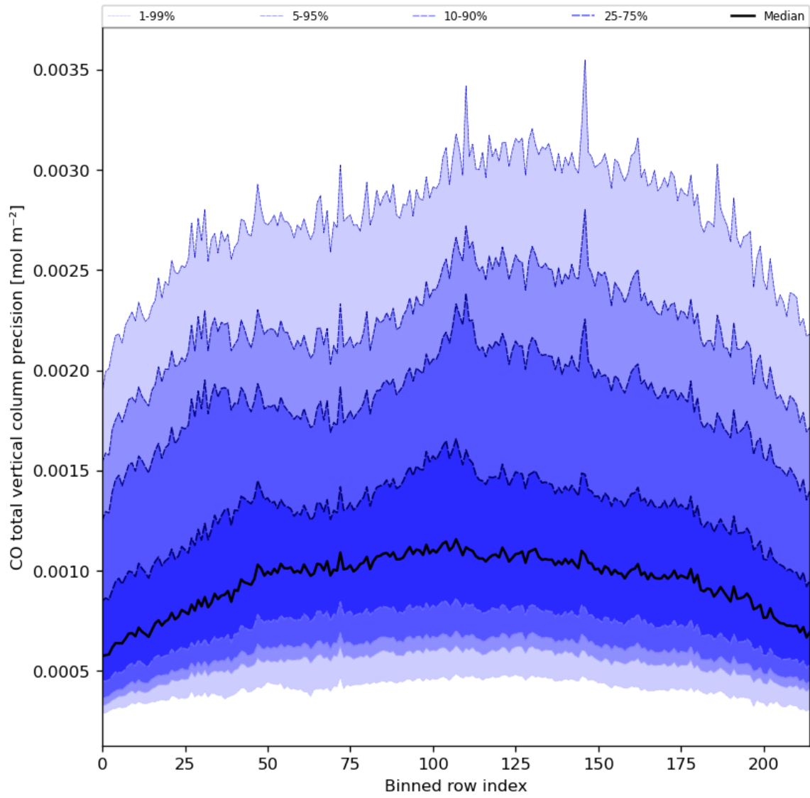
Figure 28: Along track statistics of “CO total vertical column precision” for 2024-03-23 to 2024-03-25
