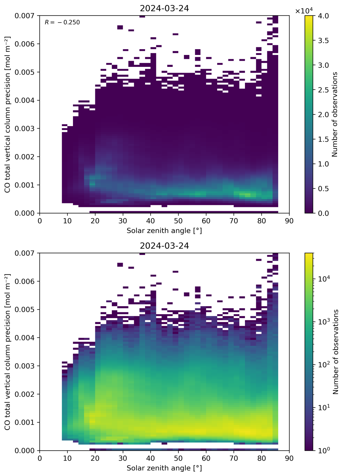
Figure 63: Scatter density plot of “Solar zenith angle” against “CO total vertical column precision” for 2024-03-23 to 2024-03-25.
