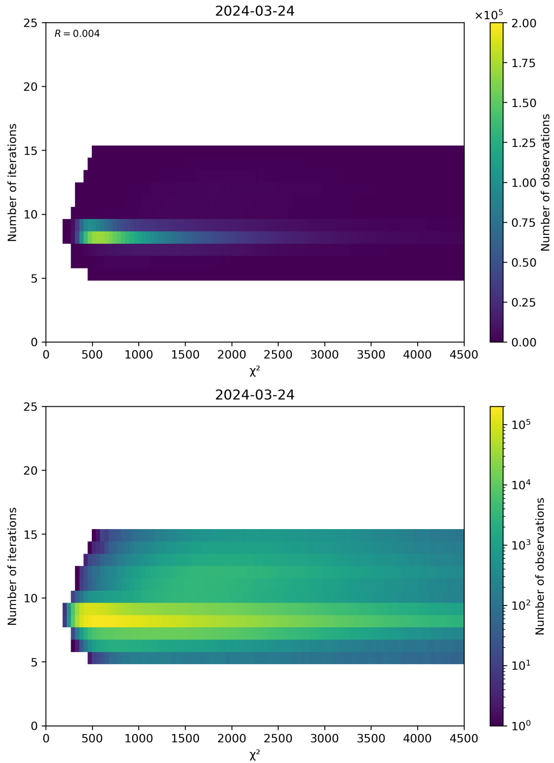
Figure 49: Scatter density plot of “ \chi^2 ” against “Number of iterations” for 2024-03-23 to 2024-03-25.
