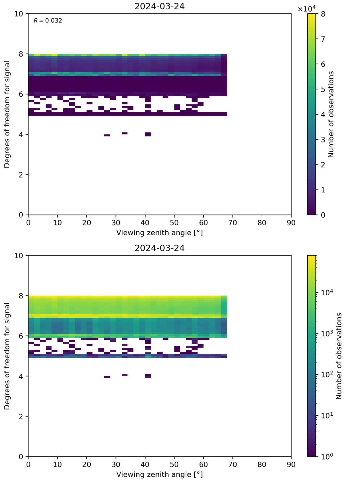
Figure 73: Scatter density plot of “Viewing zenith angle” against “Degrees of freedom for signal” for 2024-03-23 to 2024-03-25.
