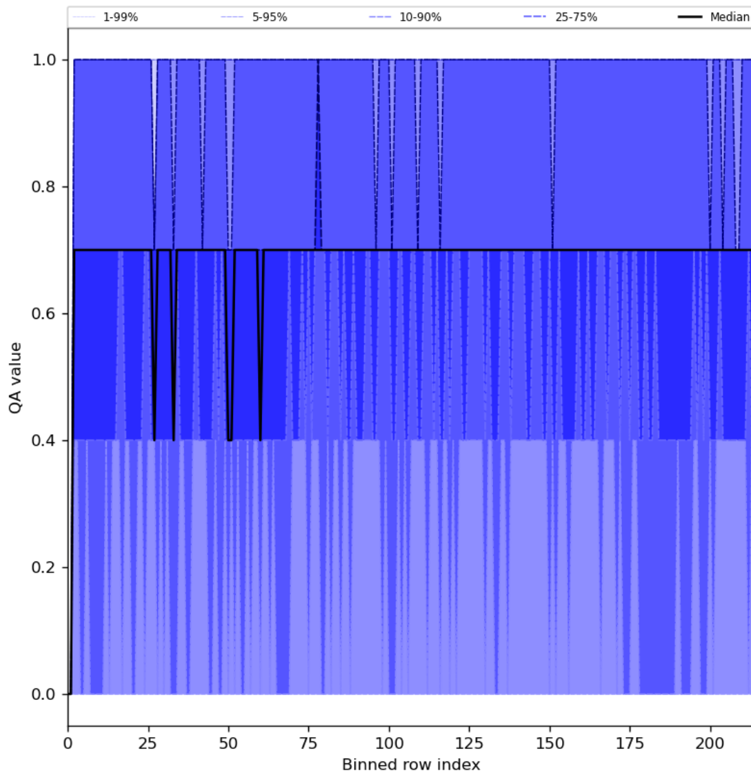
Figure 25: Along track statistics of “QA value” for 2024-03-23 to 2024-03-25
