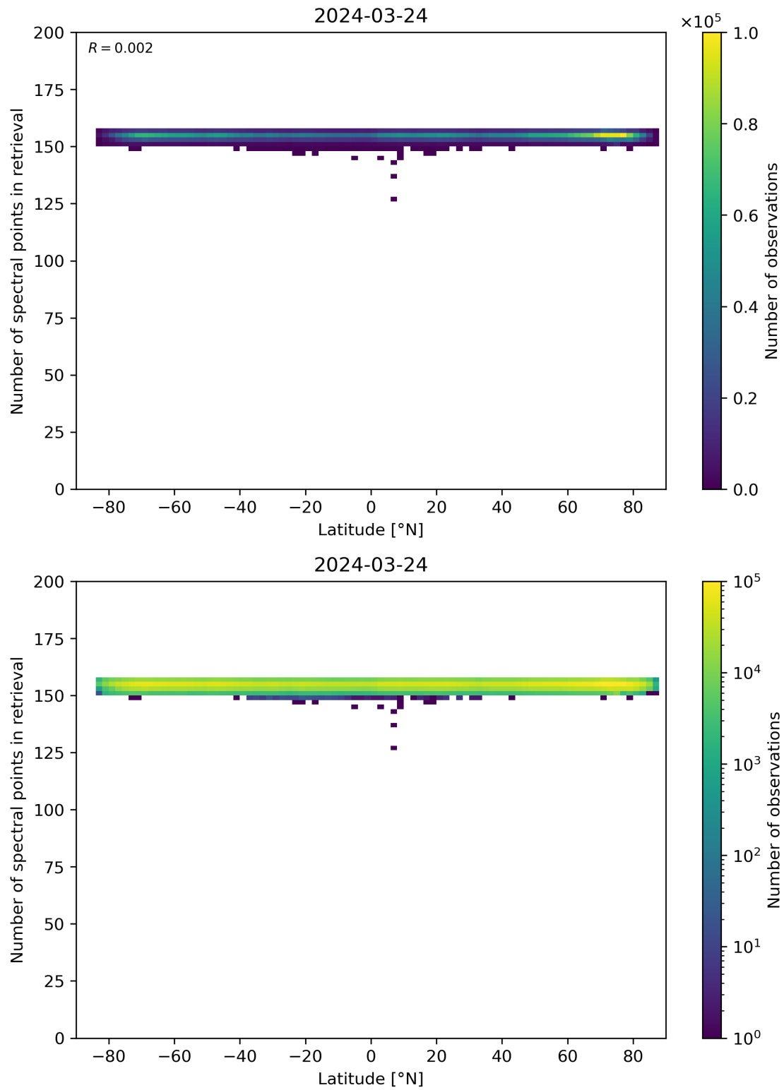
Figure 57: Scatter density plot of “Latitude” against “Number of spectral points in retrieval” for 2024-03-23 to 2024-03-25.
