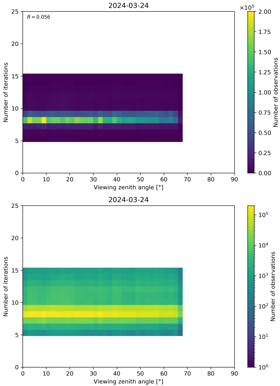
Figure 75: Scatter density plot of “Viewing zenith angle” against “Number of iterations” for 2024-03-23 to 2024-03-25.
