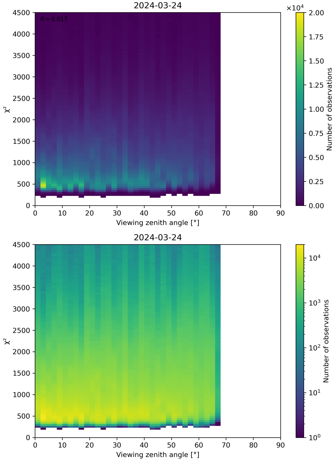
Figure 72: Scatter density plot of “Viewing zenith angle” against “ \chi^2 ” for 2024-03-23 to 2024-03-25.
