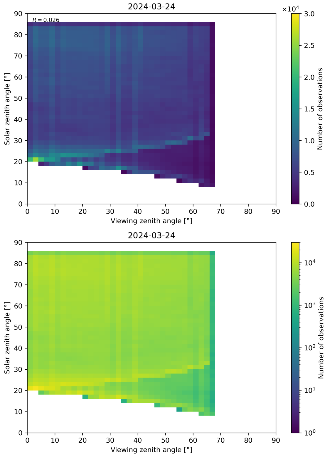
Figure 77: Scatter density plot of “Viewing zenith angle” against “Solar zenith angle” for 2024-03-23 to 2024-03-25.
