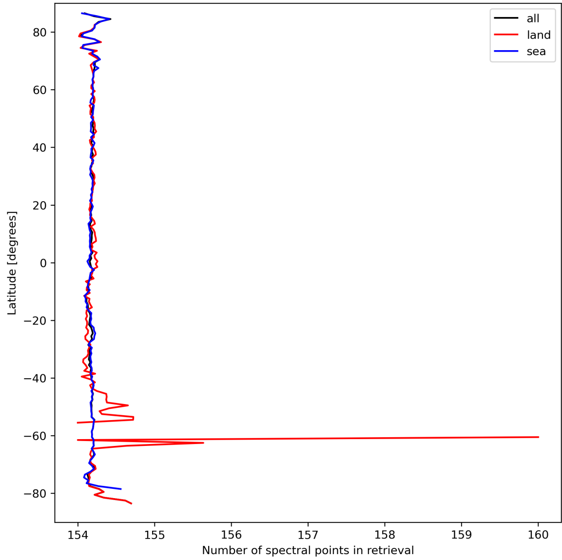
Figure 13: Zonal average of “Number of spectral points in retrieval” for 2024-03-23 to 2024-03-25.
