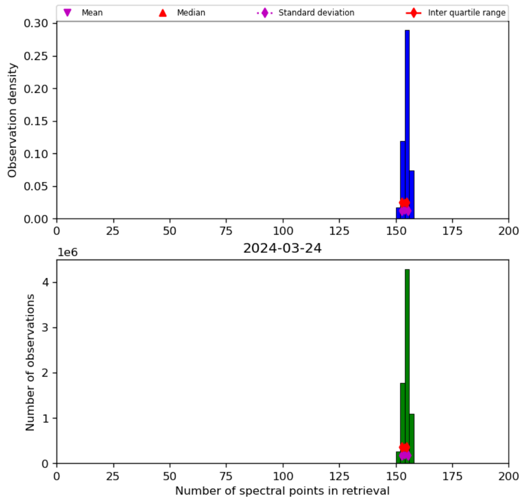
Figure 21: Histogram of “Number of spectral points in retrieval” for 2024-03-23 to 2024-03-25
