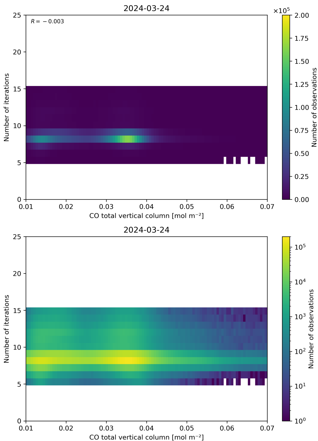
Figure 42: Scatter density plot of “CO total vertical column” against “Number of iterations” for 2024-03-23 to 2024-03-25.
