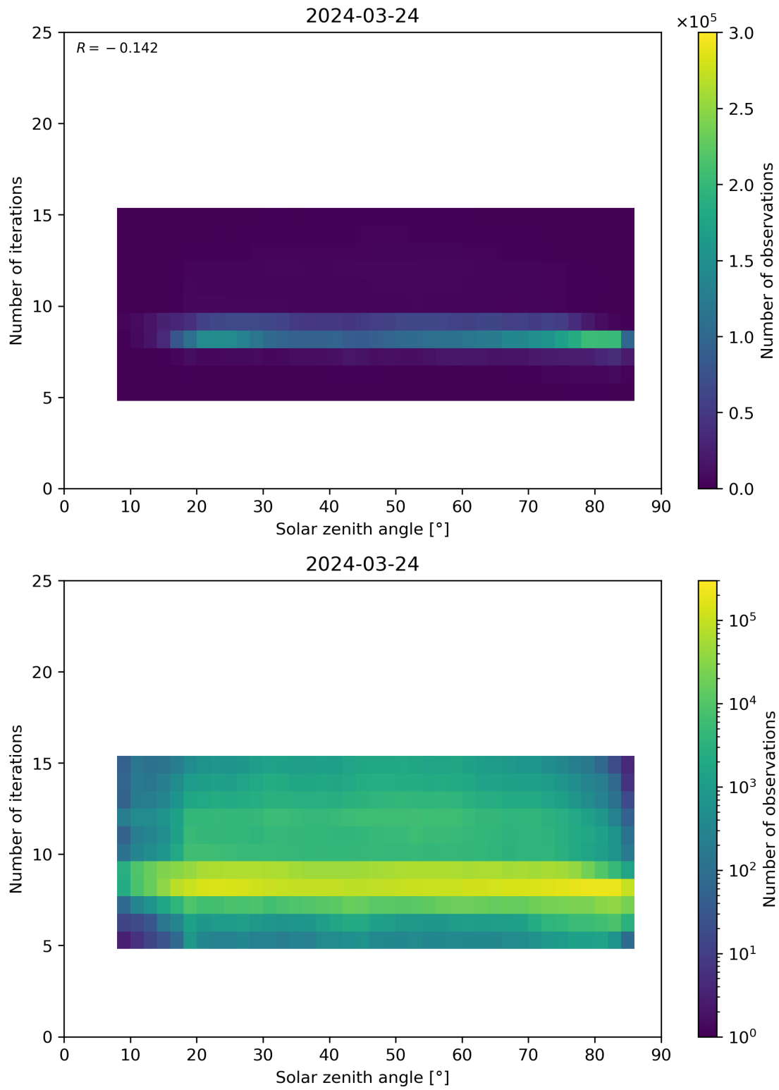
Figure 67: Scatter density plot of “Solar zenith angle” against “Number of iterations” for 2024-03-23 to 2024-03-25.
