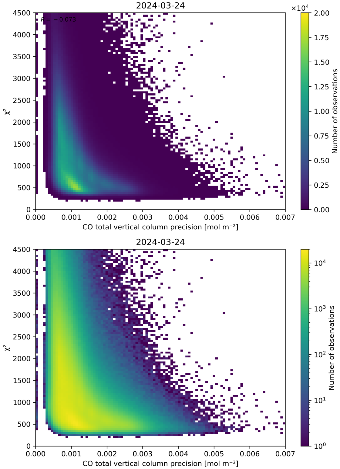
Figure 44: Scatter density plot of “CO total vertical column precision” against “ \chi^2 ” for 2024-03-23 to 2024-03-25.
