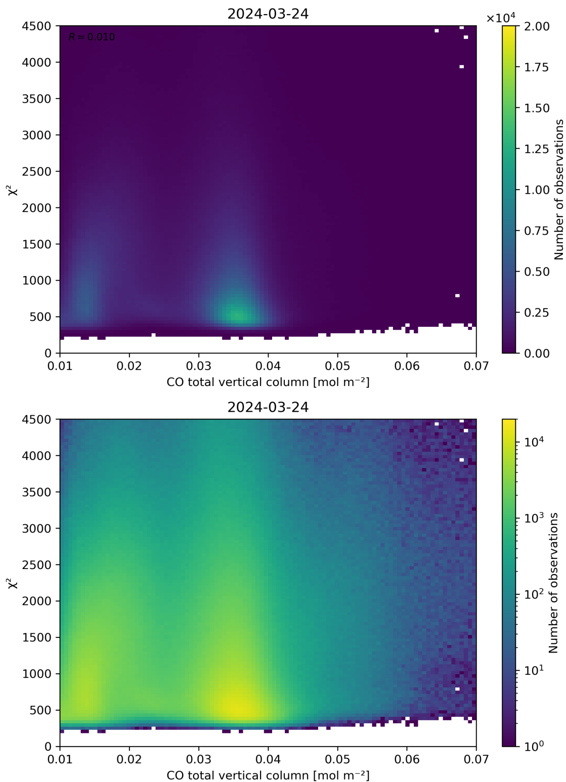
Figure 35: Scatter density plot of “CO total vertical column” against “ \chi^2 ” for 2024-03-23 to 2024-03-25.
