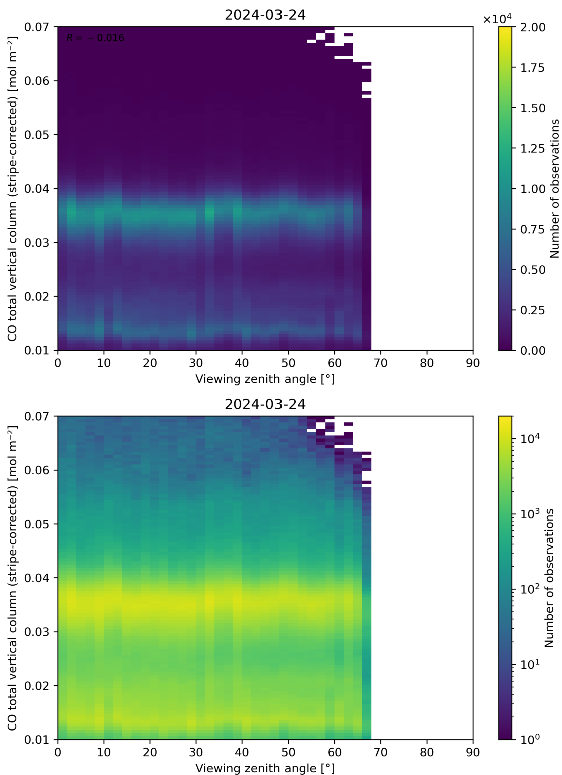
Figure 70: Scatter density plot of “Viewing zenith angle” against “CO total vertical column (stripe-corrected)” for 2024-03-23 to 2024-03-25.
