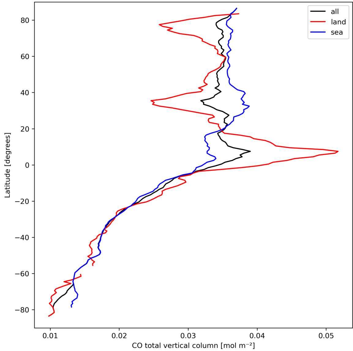
Figure 10: Zonal average of “CO total vertical column” for 2024-03-23 to 2024-03-25.
