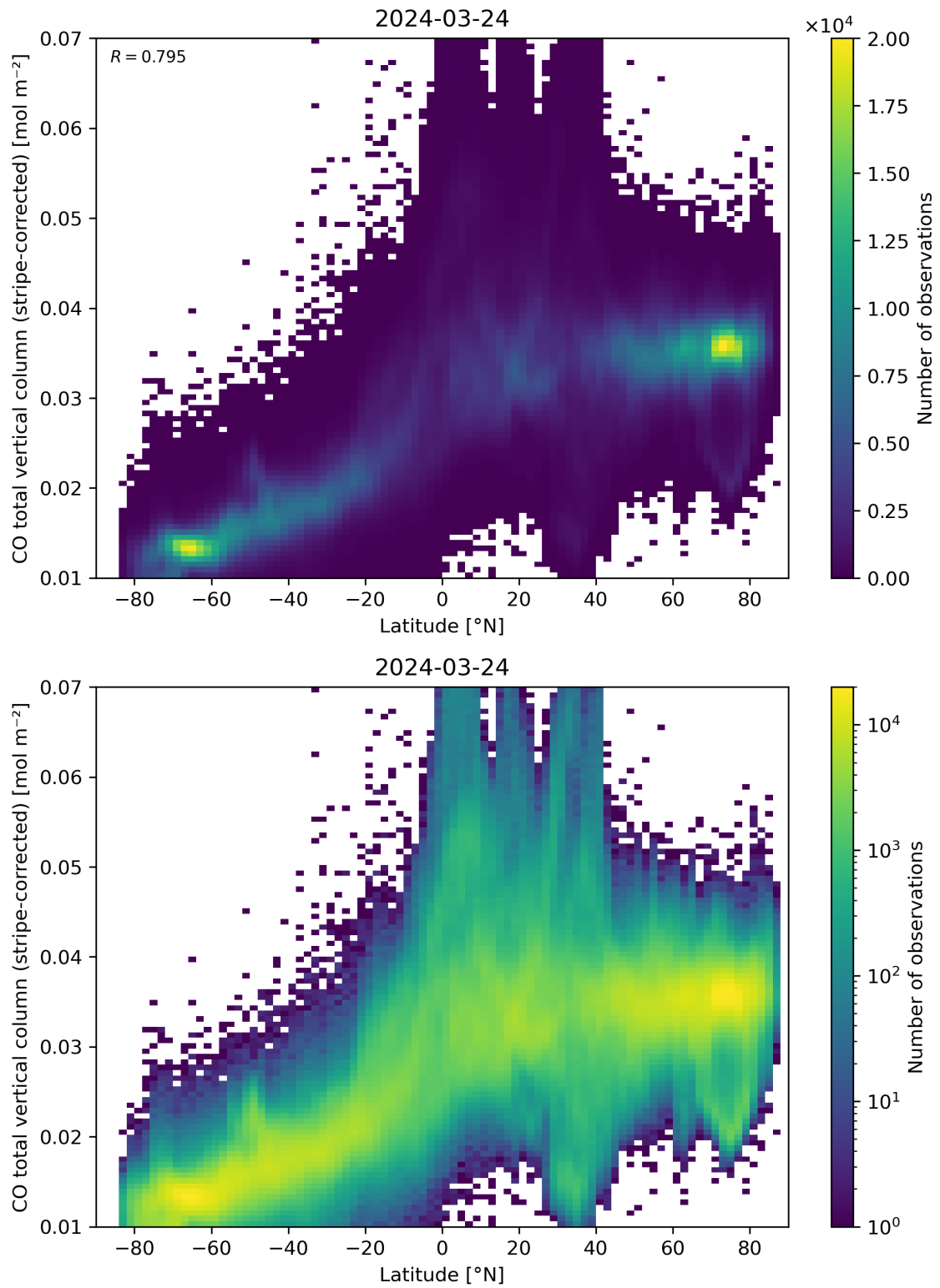
Figure 52: Scatter density plot of “Latitude” against “CO total vertical column (stripe-corrected)” for 2024-03-23 to 2024-03-25.
