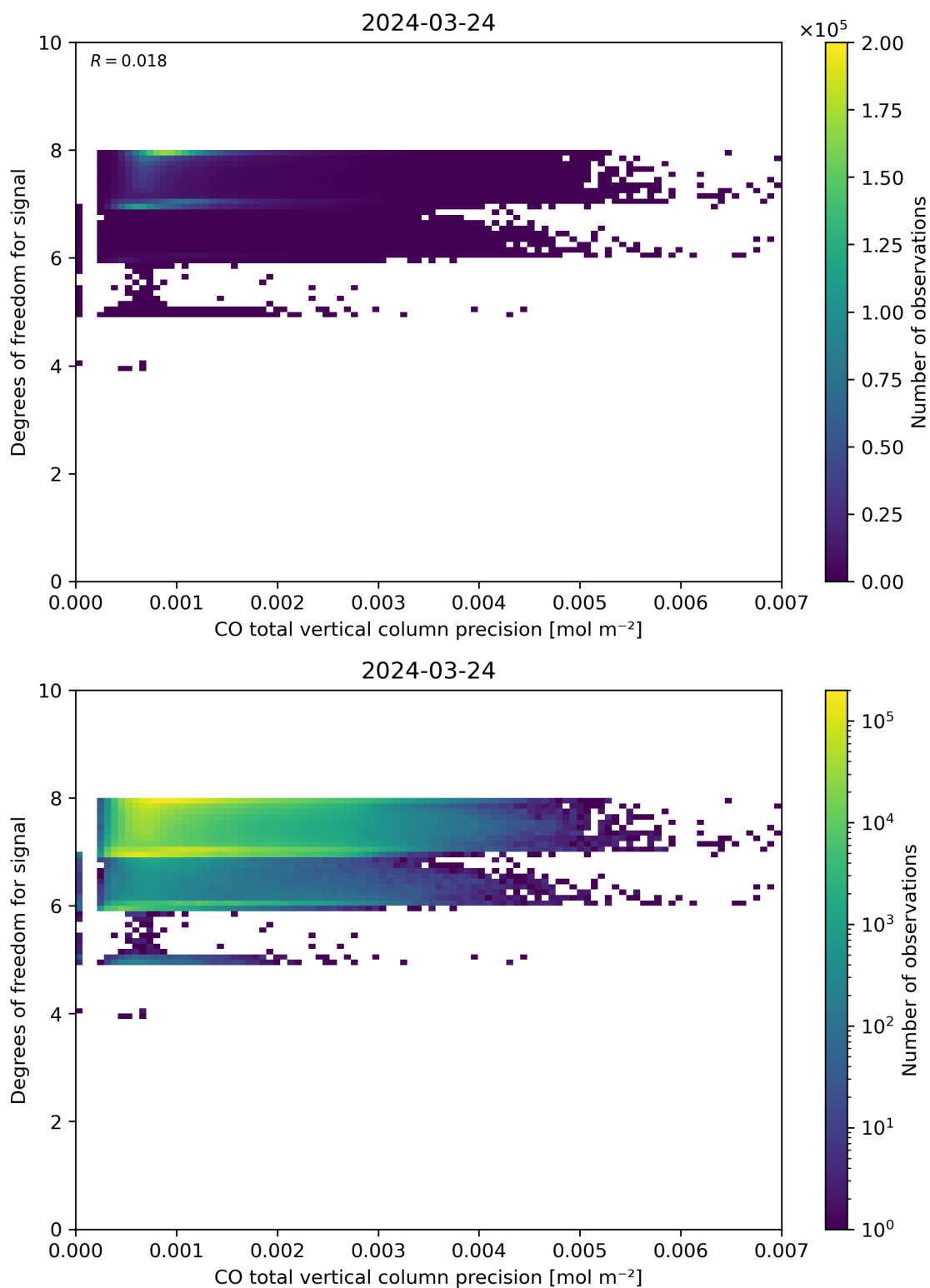
Figure 45: Scatter density plot of “CO total vertical column precision” against “Degrees of freedom for signal” for 2024-03-23 to 2024-03-25.
