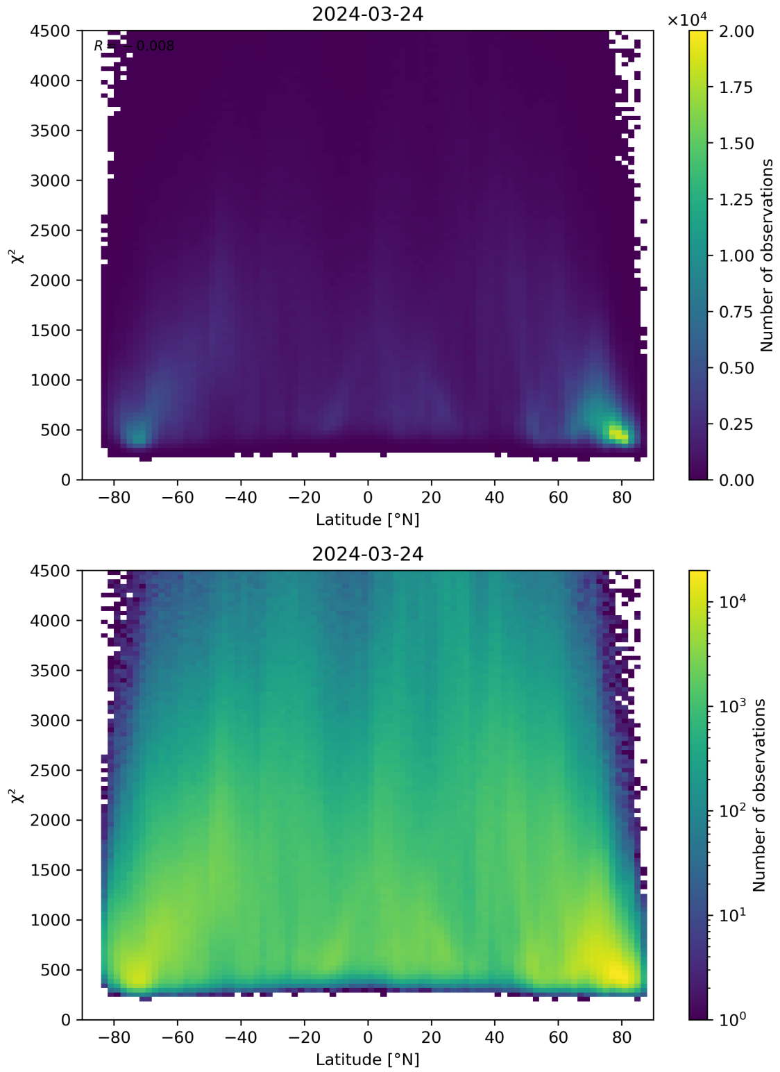
Figure 54: Scatter density plot of “Latitude” against “ \chi^2 ” for 2024-03-23 to 2024-03-25.
