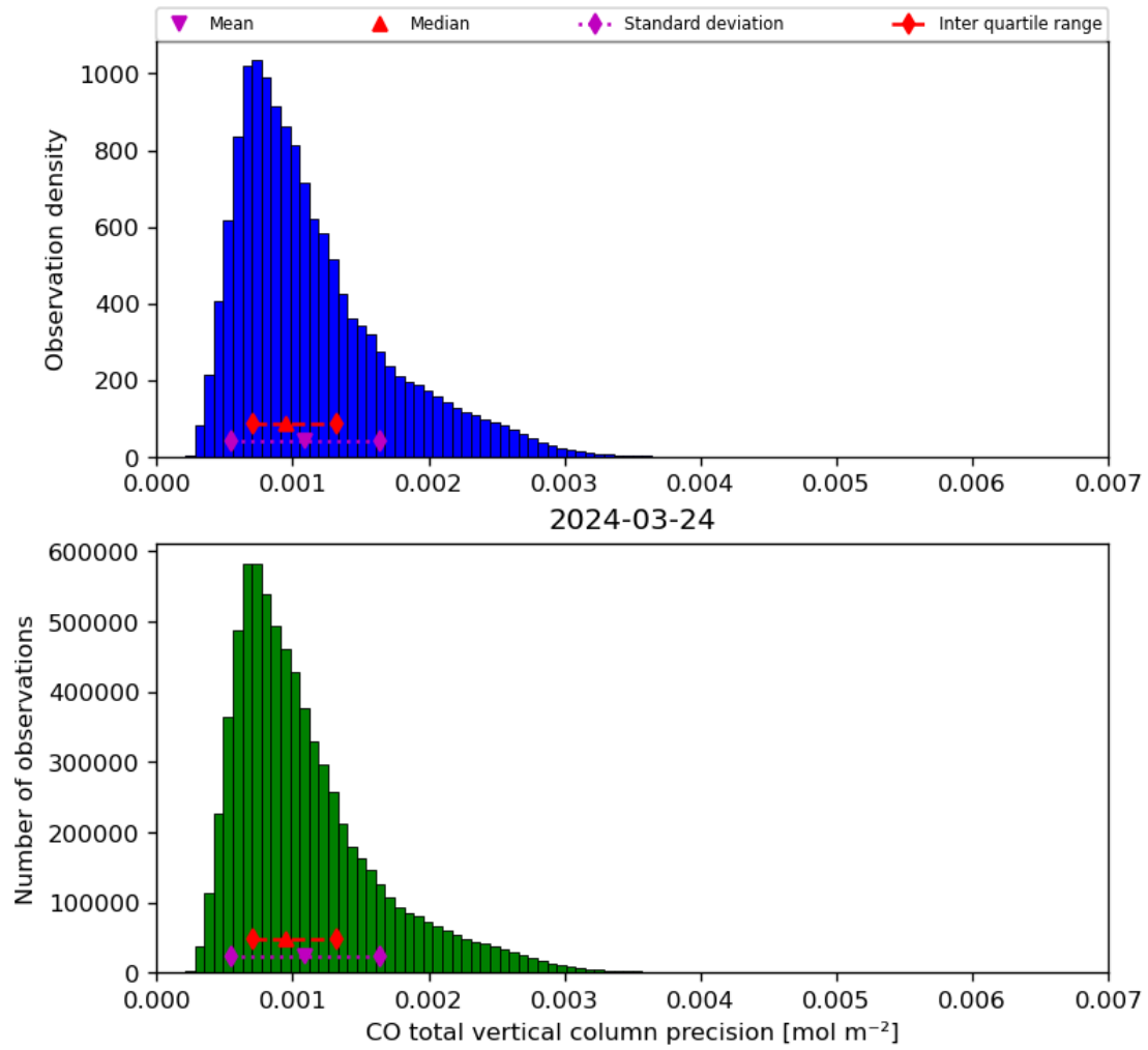
Figure 20: Histogram of “CO total vertical column precision” for 2024-03-23 to 2024-03-25
