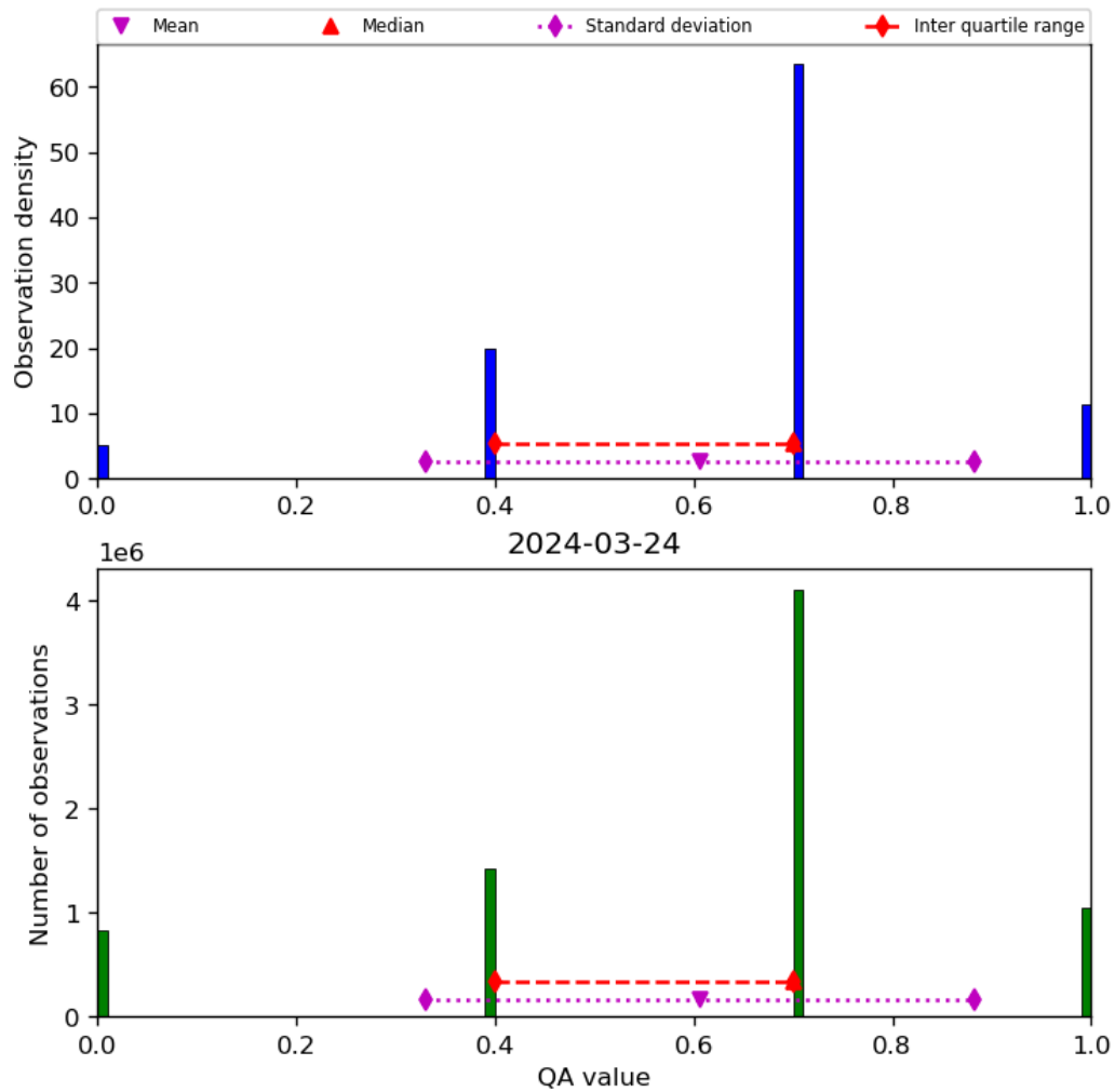
Figure 17: Histogram of “QA value” for 2024-03-23 to 2024-03-25
