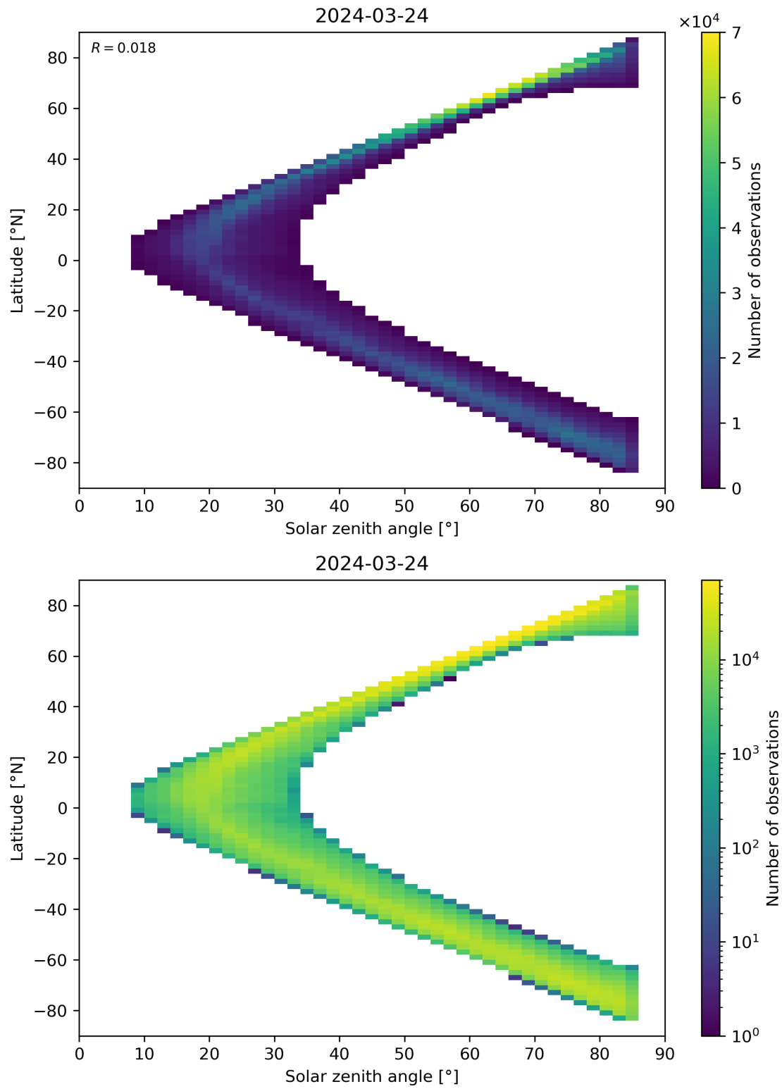
Figure 66: Scatter density plot of “Solar zenith angle” against “Latitude” for 2024-03-23 to 2024-03-25.
