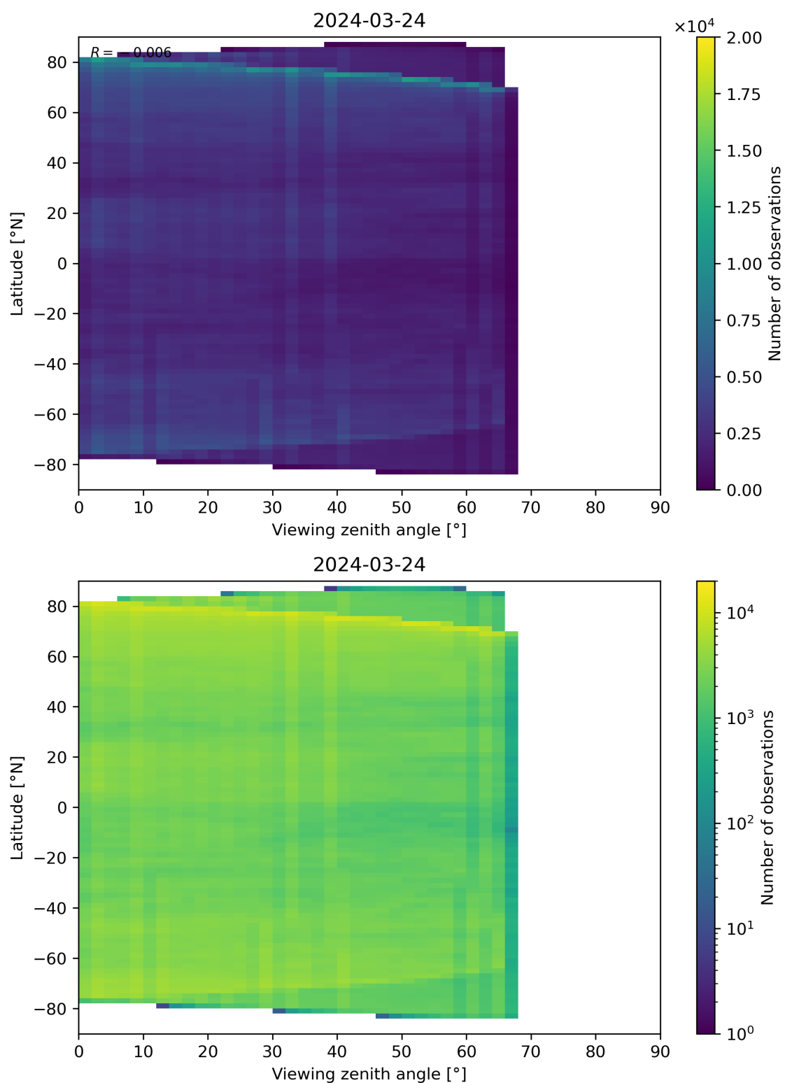
Figure 74: Scatter density plot of “Viewing zenith angle” against “Latitude” for 2024-03-23 to 2024-03-25.
