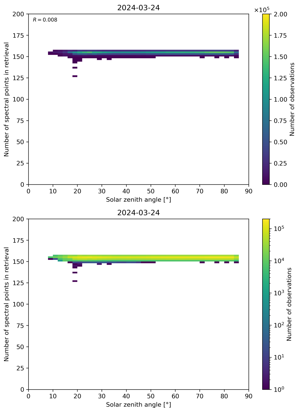
Figure 68: Scatter density plot of “Solar zenith angle” against “Number of spectral points in retrieval” for 2024-03-23 to 2024-03-25.
