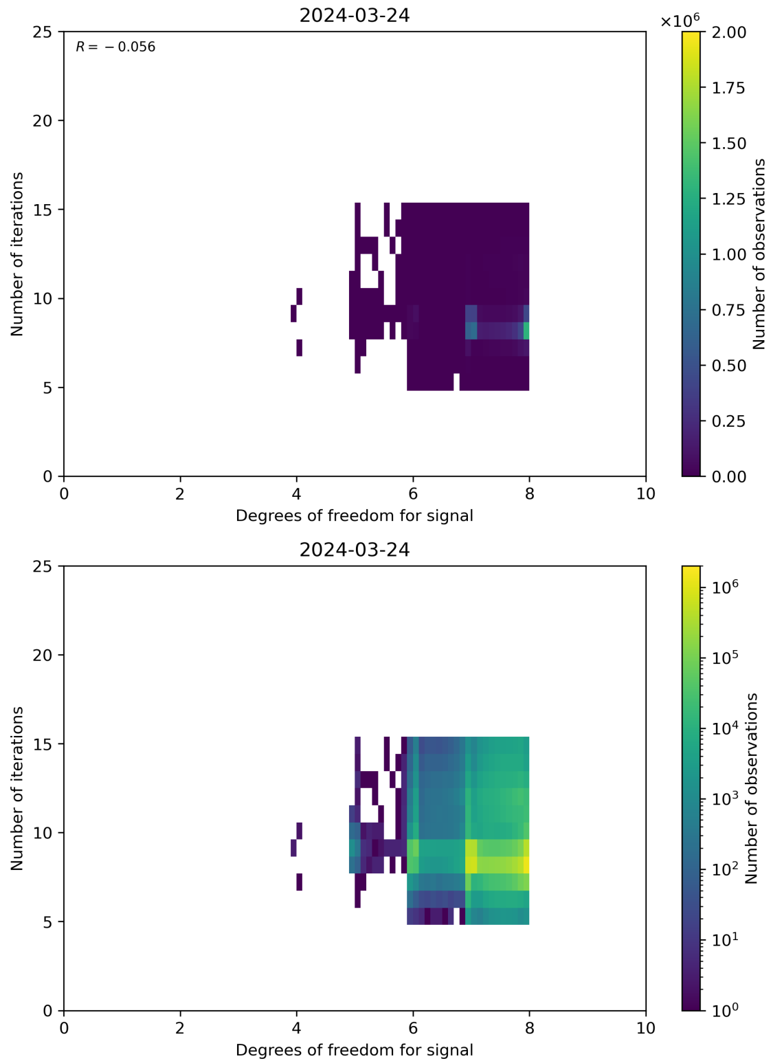
Figure 50: Scatter density plot of “Degrees of freedom for signal” against “Number of iterations” for 2024-03-23 to 2024-03-25.
