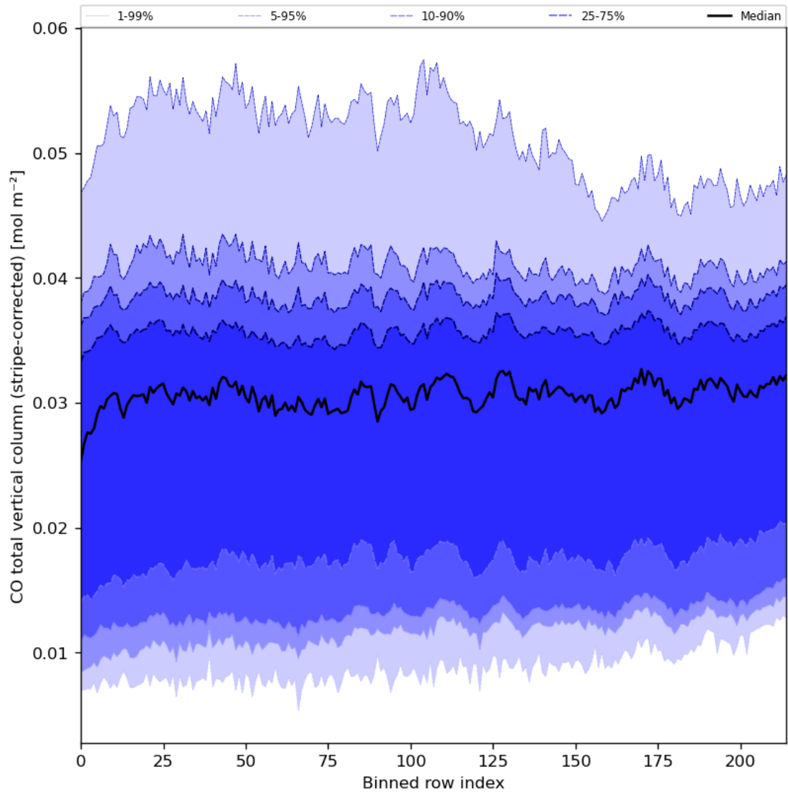
Figure 27: Along track statistics of “CO total vertical column (stripe-corrected)” for 2024-03-23 to 2024-03-25
