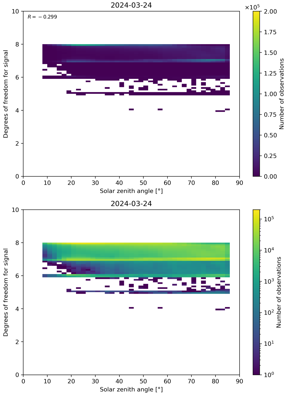
Figure 65: Scatter density plot of “Solar zenith angle” against “Degrees of freedom for signal” for 2024-03-23 to 2024-03-25.
