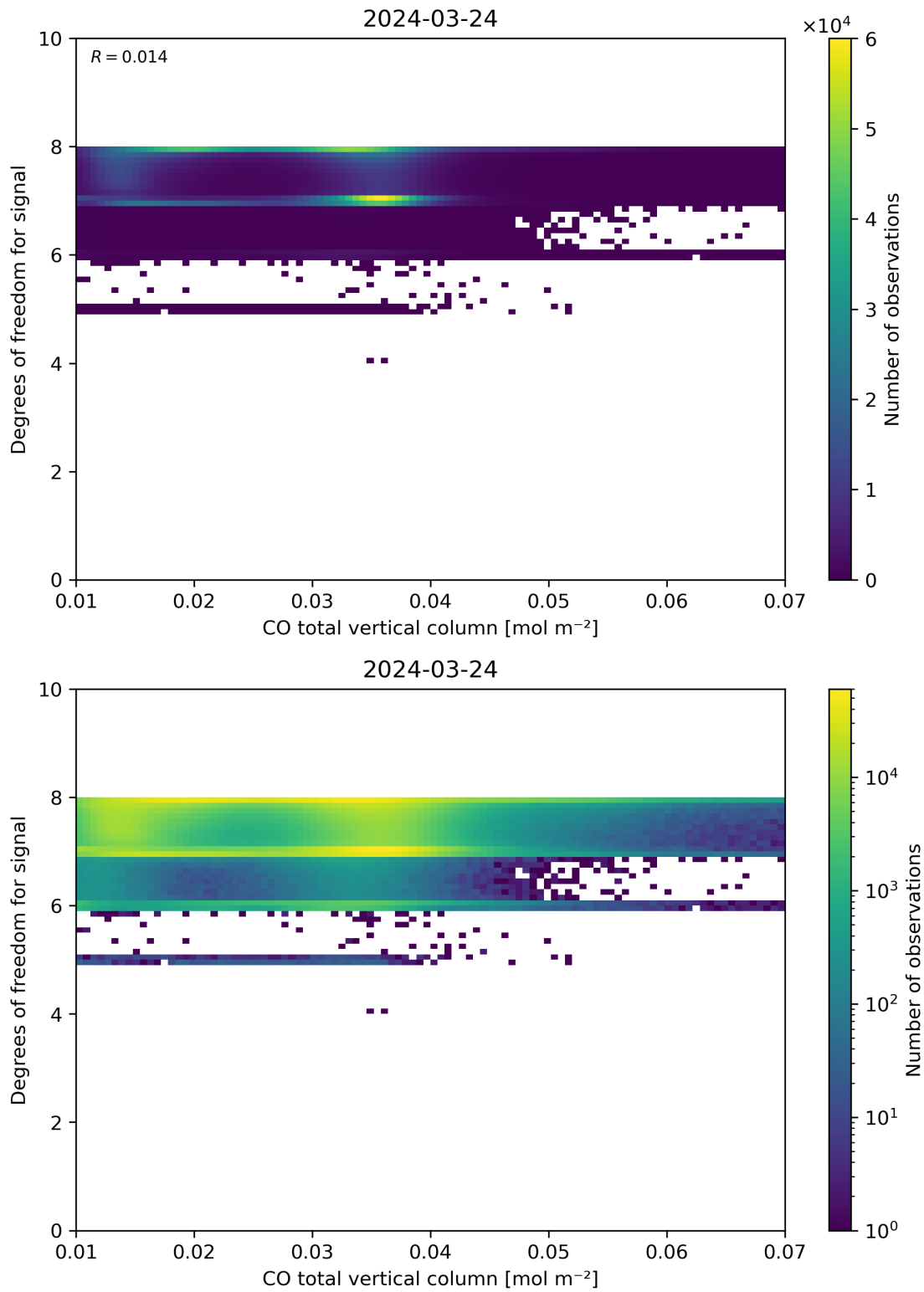
Figure 41: Scatter density plot of “CO total vertical column” against “Degrees of freedom for signal” for 2024-03-23 to 2024-03-25.
