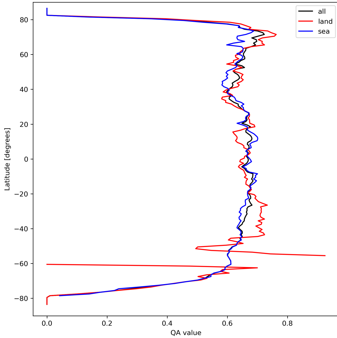
Figure 9: Zonal average of “QA value” for 2024-03-23 to 2024-03-25.
