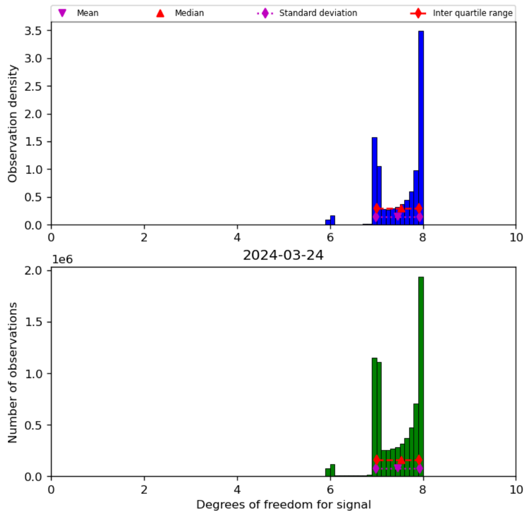
Figure 23: Histogram of “Degrees of freedom for signal” for 2024-03-23 to 2024-03-25
