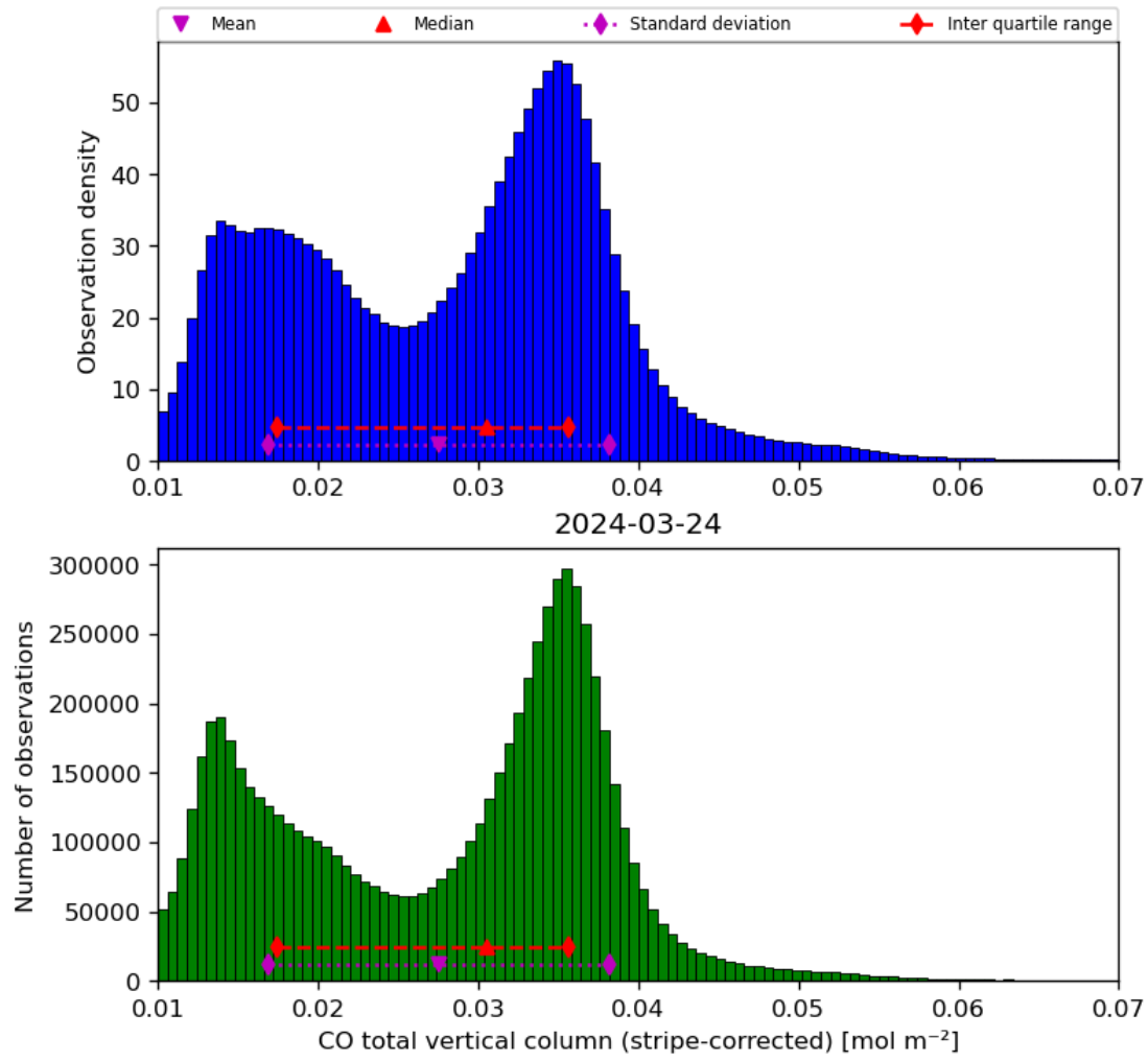
Figure 19: Histogram of “CO total vertical column (stripe-corrected)” for 2024-03-23 to 2024-03-25
