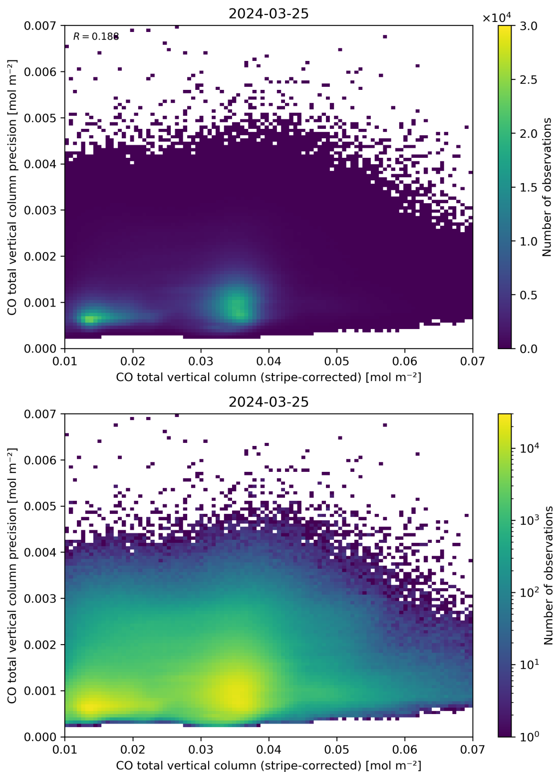
Figure 36: Scatter density plot of “CO total vertical column (stripe-corrected)” against “CO total vertical column precision” for 2024-03-25 to 2024-03-26.
