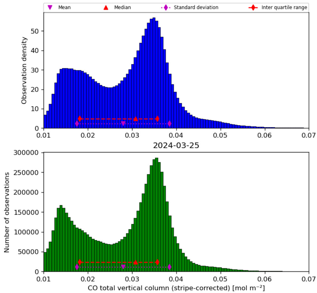
Figure 19: Histogram of “CO total vertical column (stripe-corrected)” for 2024-03-25 to 2024-03-26
