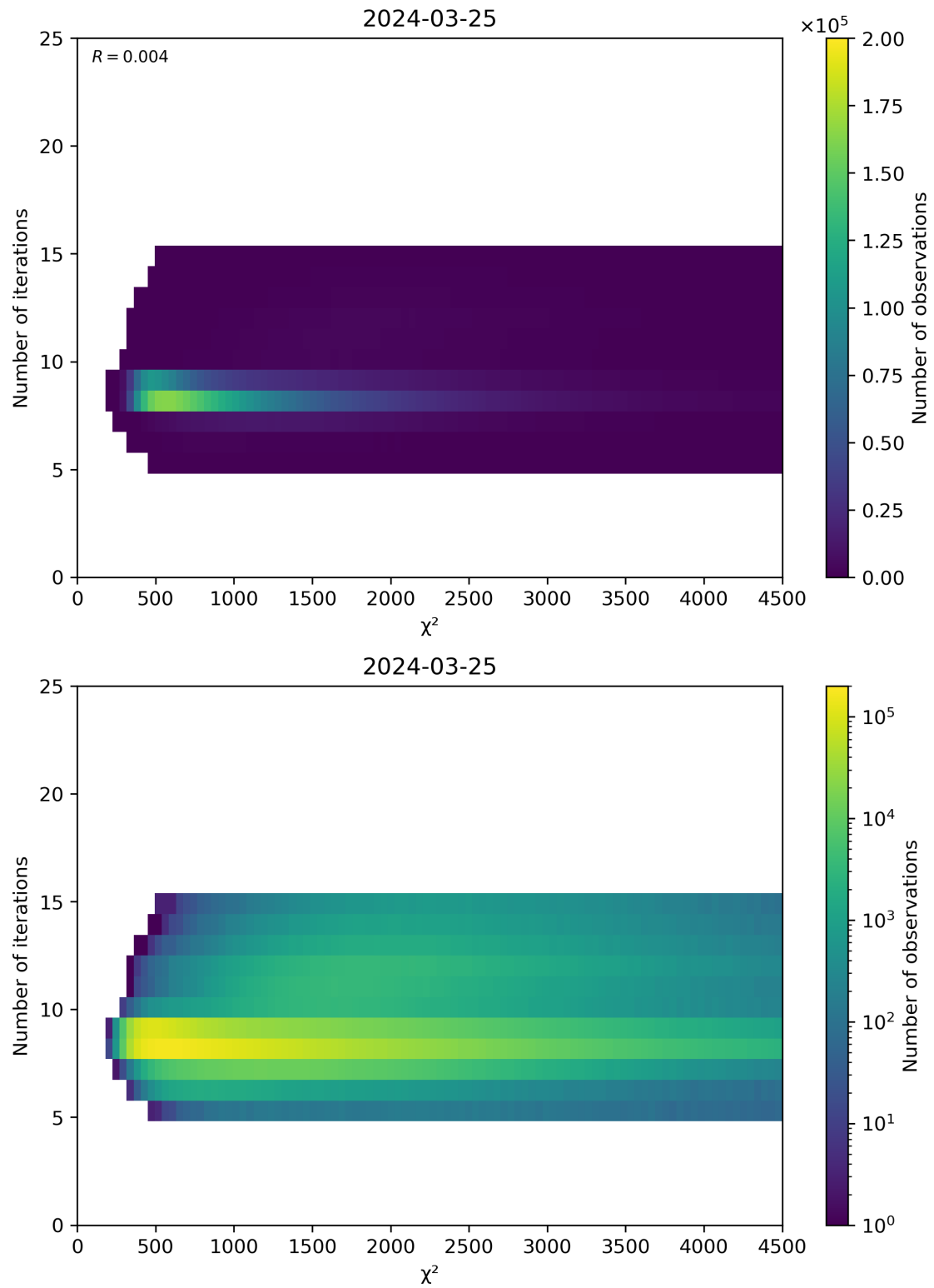
Figure 49: Scatter density plot of “ \chi^2 ” against “Number of iterations” for 2024-03-25 to 2024-03-26.
