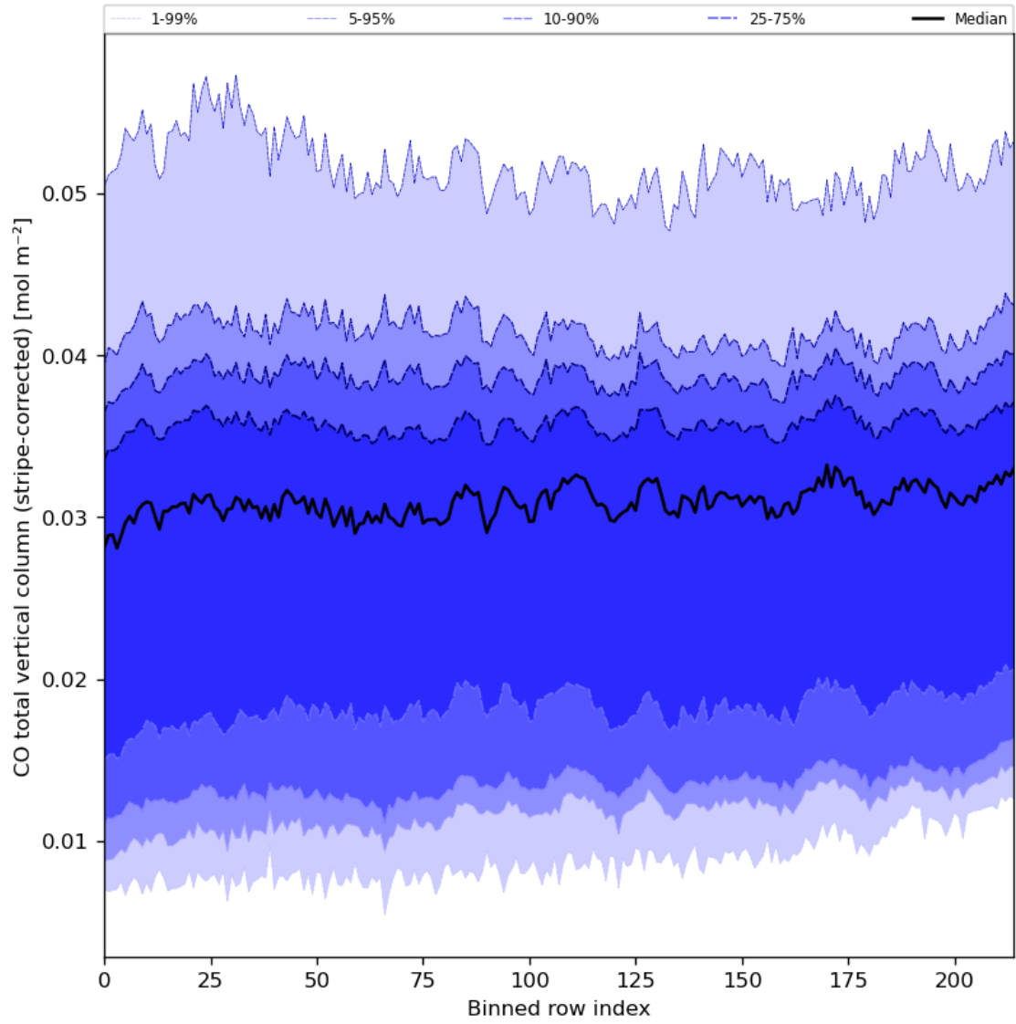
Figure 27: Along track statistics of “CO total vertical column (stripe-corrected)” for 2024-03-25 to 2024-03-26
