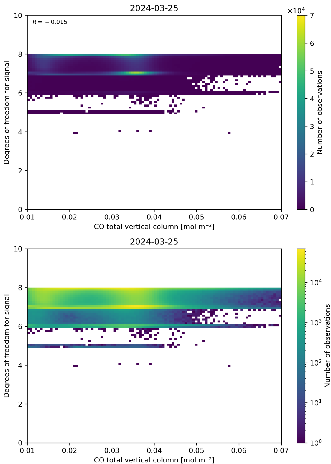
Figure 41: Scatter density plot of “CO total vertical column” against “Degrees of freedom for signal” for 2024-03-25 to 2024-03-26.
