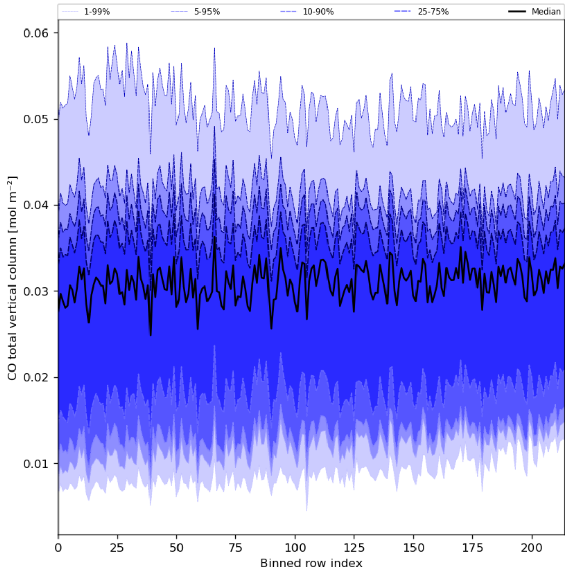
Figure 26: Along track statistics of “CO total vertical column” for 2024-03-25 to 2024-03-26
