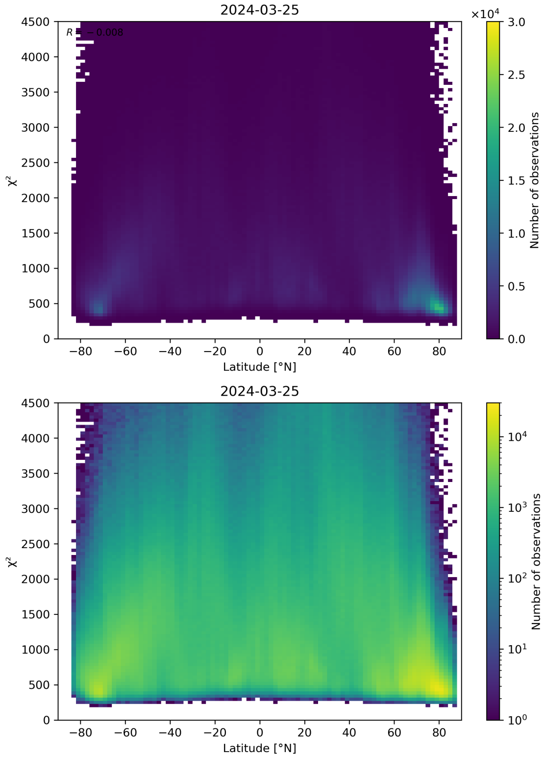
Figure 54: Scatter density plot of “Latitude” against “ \chi^2 ” for 2024-03-25 to 2024-03-26.
