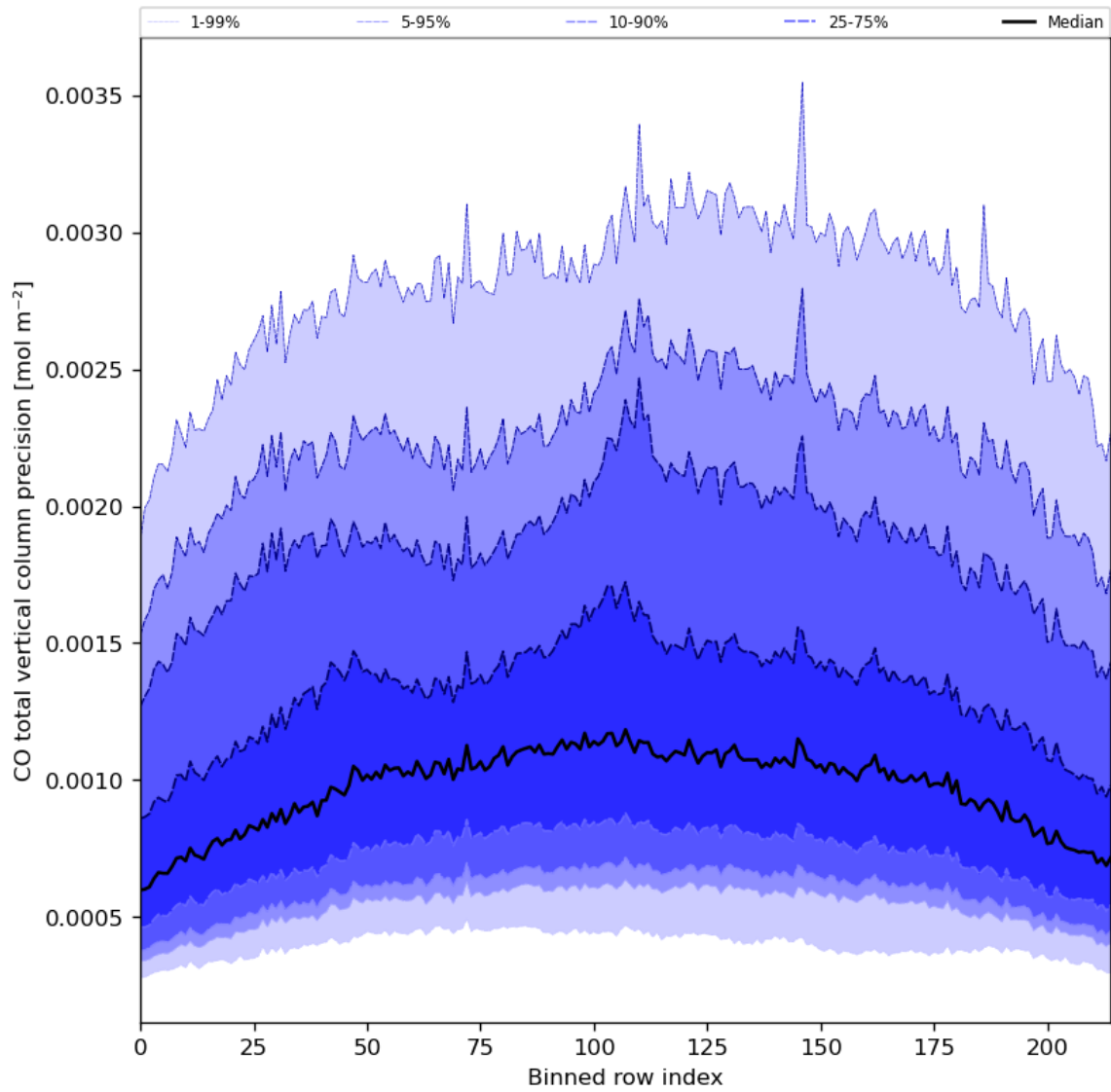
Figure 28: Along track statistics of “CO total vertical column precision” for 2024-03-25 to 2024-03-26
