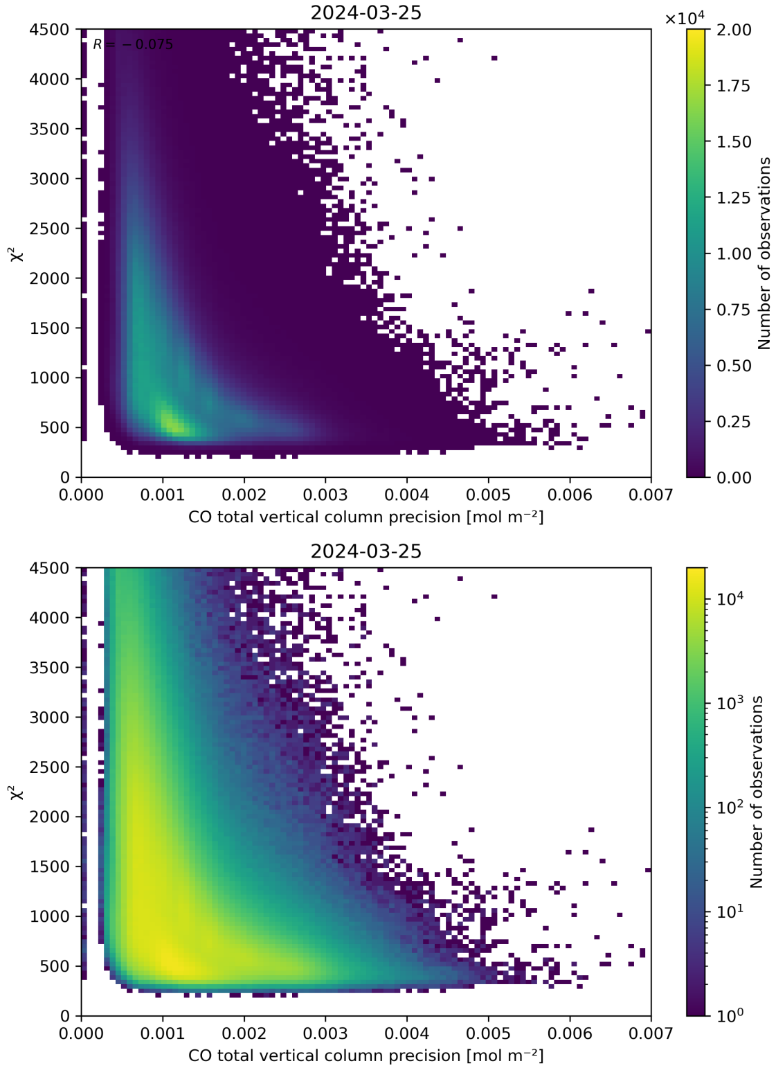
Figure 44: Scatter density plot of “CO total vertical column precision” against “ \chi^2 ” for 2024-03-25 to 2024-03-26.
