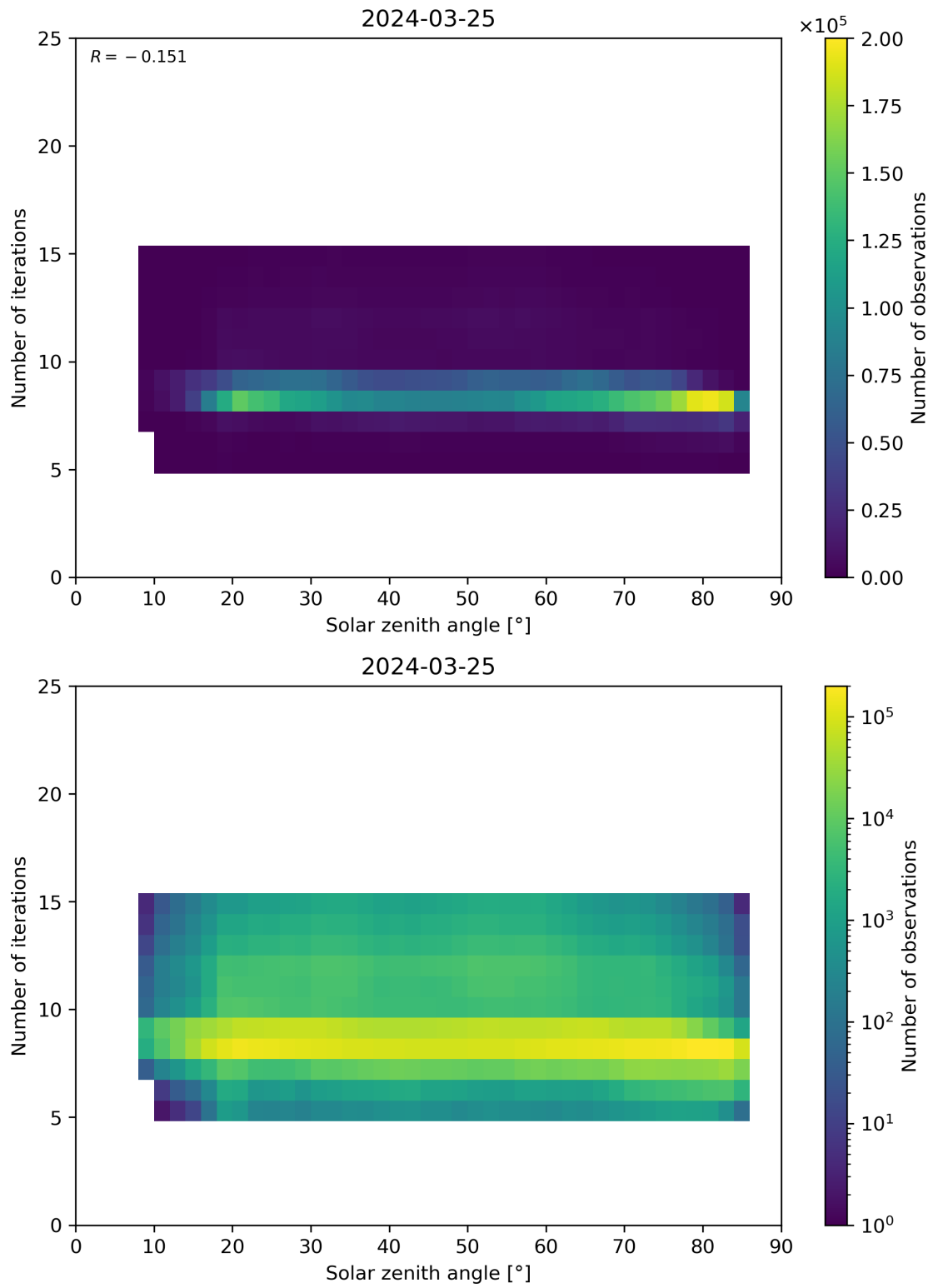
Figure 67: Scatter density plot of “Solar zenith angle” against “Number of iterations” for 2024-03-25 to 2024-03-26.
