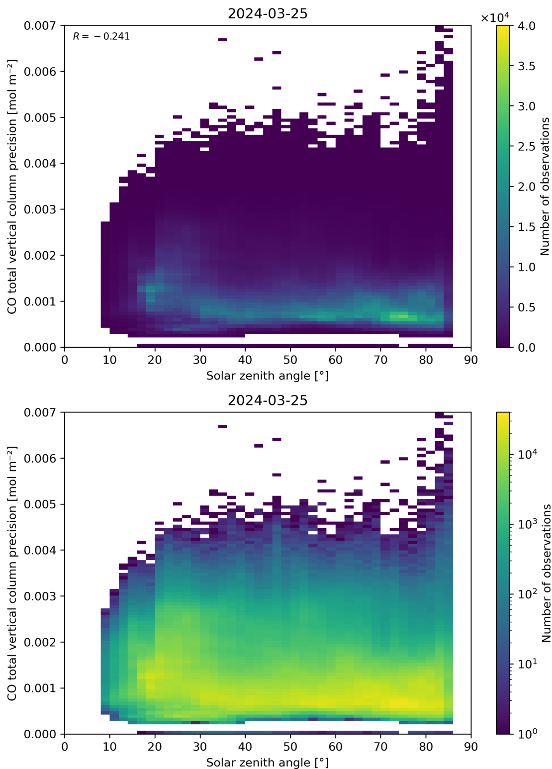
Figure 63: Scatter density plot of “Solar zenith angle” against “CO total vertical column precision” for 2024-03-25 to 2024-03-26.
