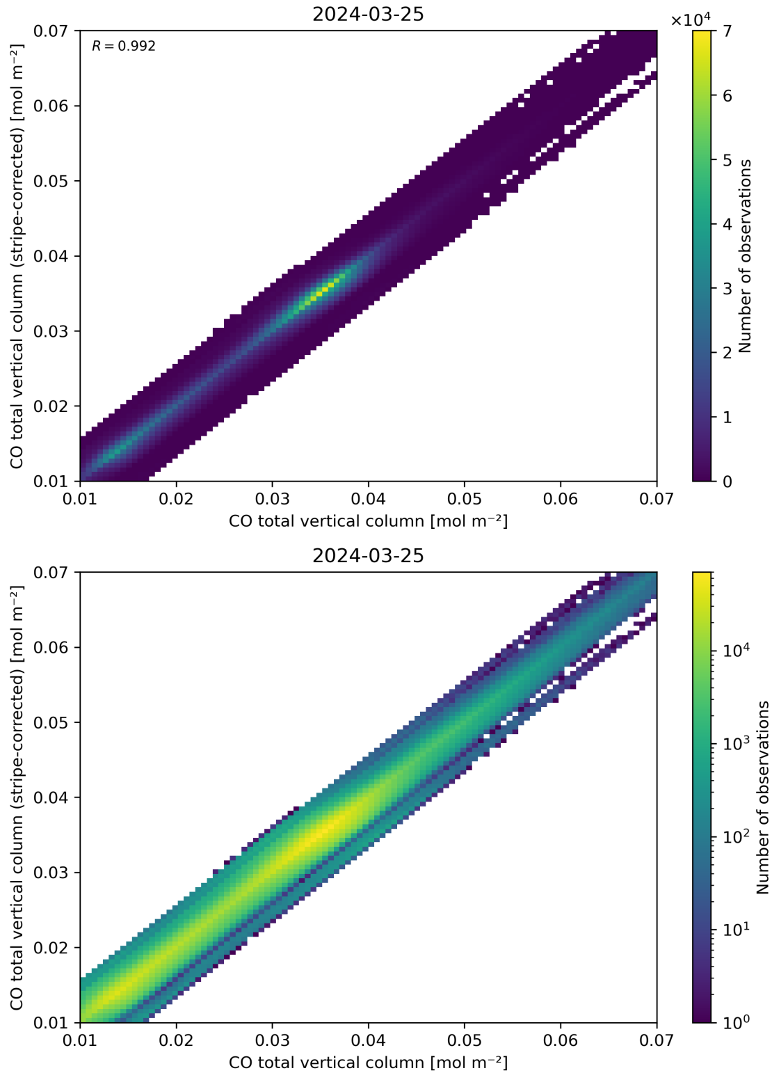
Figure 33: Scatter density plot of “CO total vertical column” against “CO total vertical column (stripe-corrected)” for 2024-03-25 to 2024-03-26.
