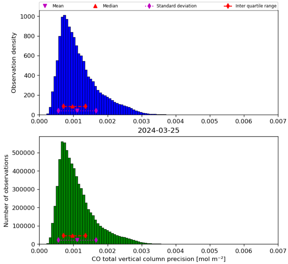
Figure 20: Histogram of “CO total vertical column precision” for 2024-03-25 to 2024-03-26
