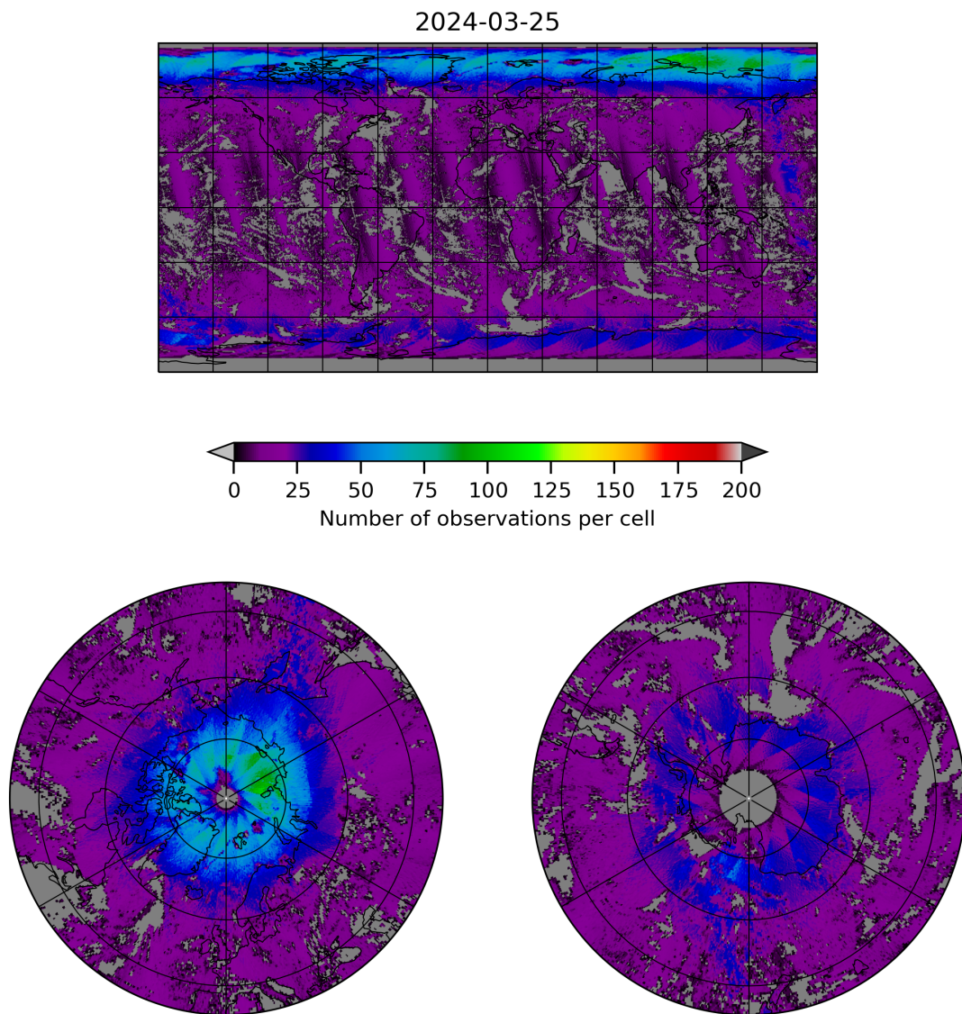
Figure 8: Map of the number of observations for 2024-03-25 to 2024-03-26
