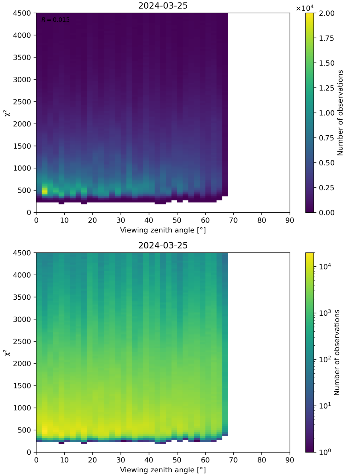
Figure 72: Scatter density plot of “Viewing zenith angle” against “ \chi^2 ” for 2024-03-25 to 2024-03-26.
