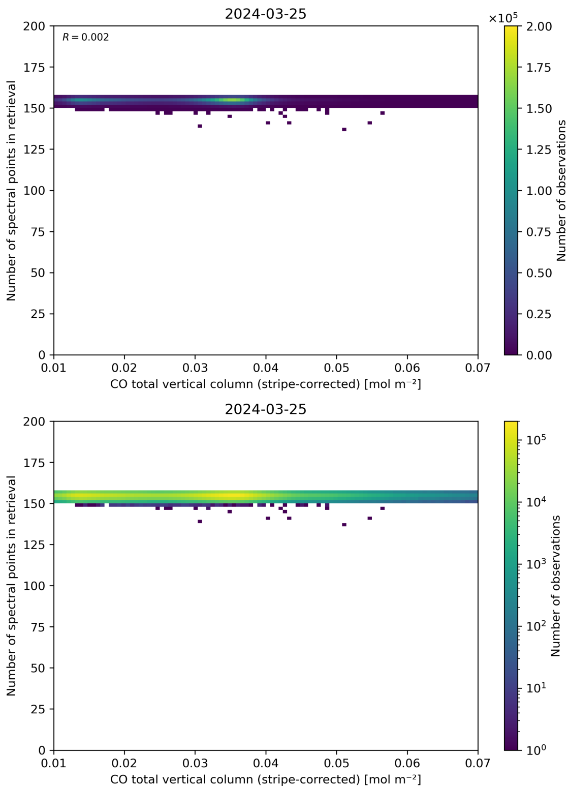
Figure 40: Scatter density plot of “CO total vertical column (stripe-corrected)” against “Number of spectral points in retrieval” for 2024-03-25 to 2024-03-26.
