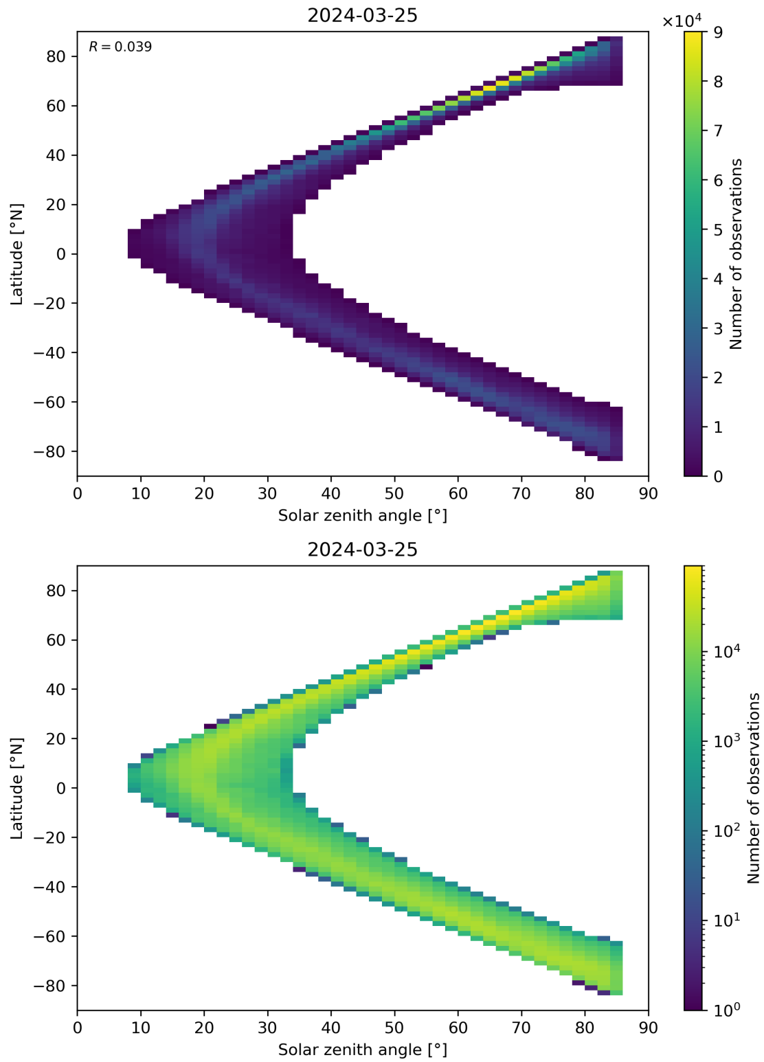
Figure 66: Scatter density plot of “Solar zenith angle” against “Latitude” for 2024-03-25 to 2024-03-26.
