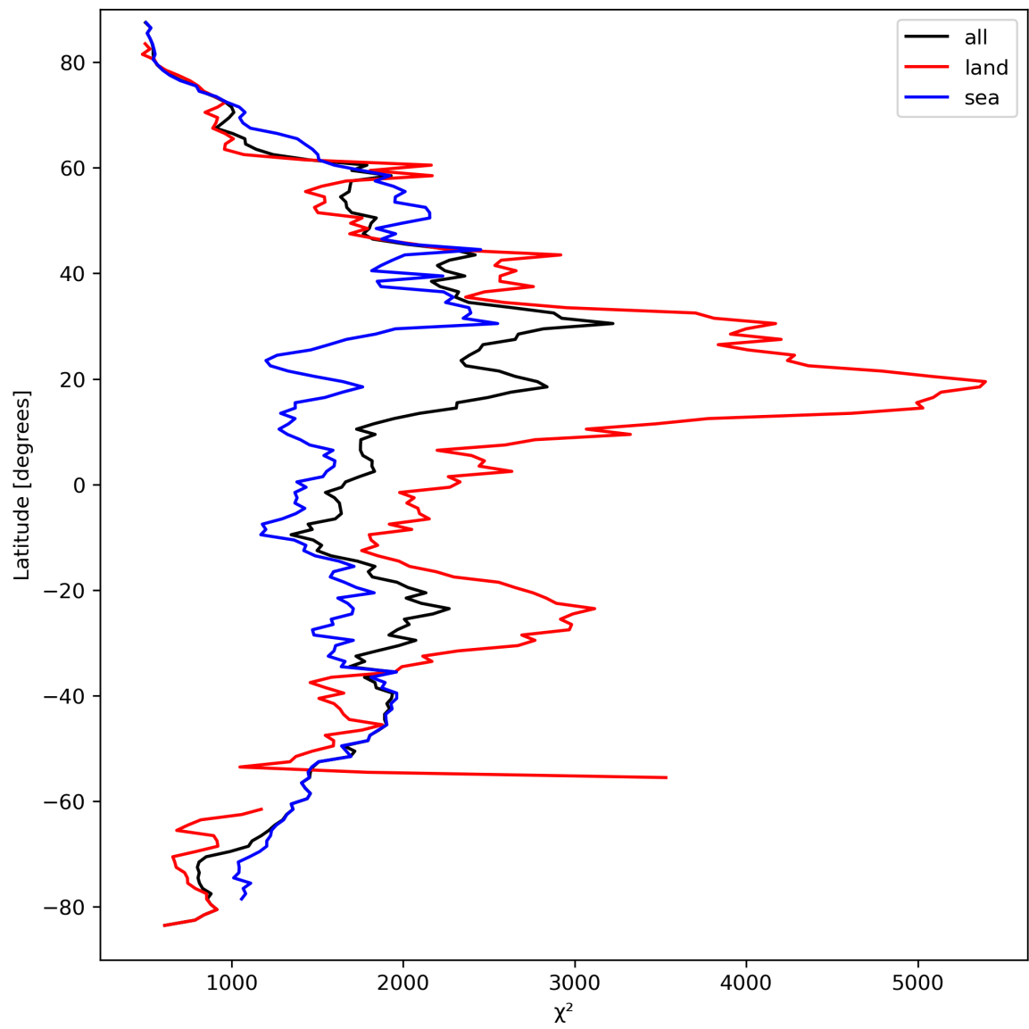
Figure 14: Zonal average of “ \chi^2 ” for 2024-03-25 to 2024-03-26.
