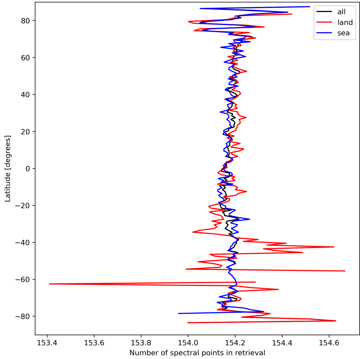
Figure 13: Zonal average of “Number of spectral points in retrieval” for 2024-03-25 to 2024-03-26.
