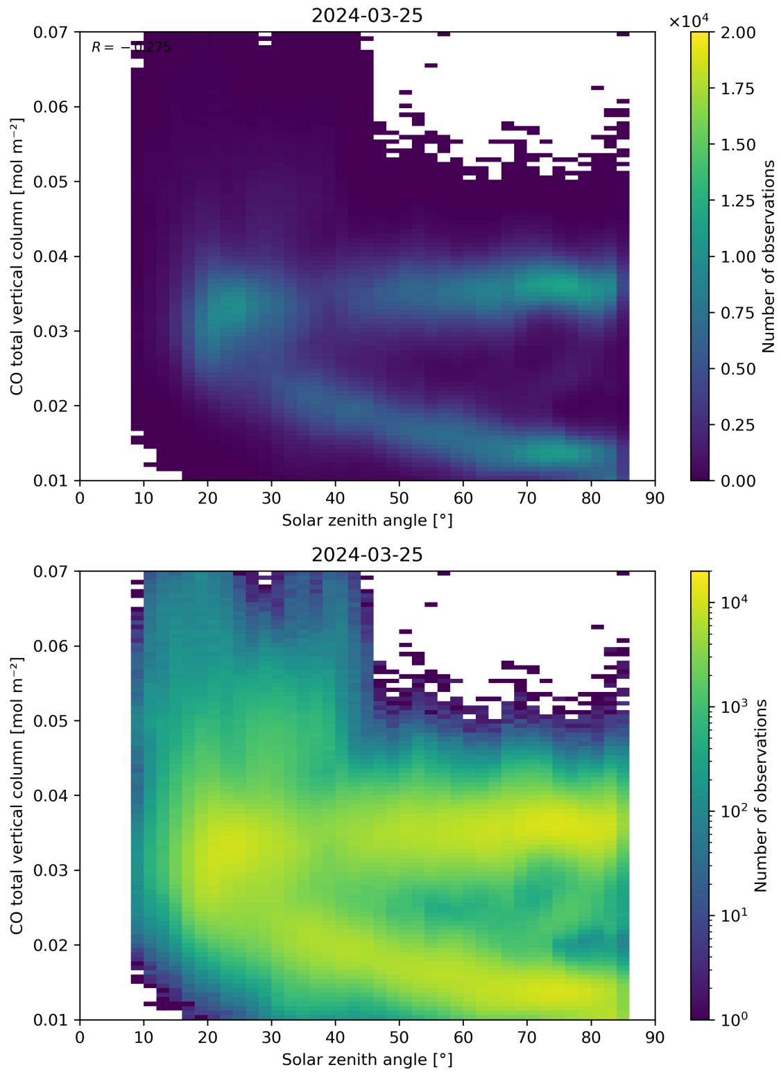
Figure 61: Scatter density plot of “Solar zenith angle” against “CO total vertical column” for 2024-03-25 to 2024-03-26.
