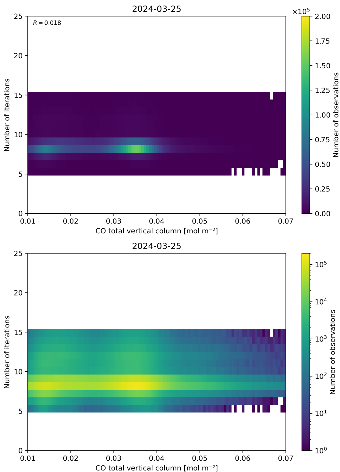
Figure 42: Scatter density plot of “CO total vertical column” against “Number of iterations” for 2024-03-25 to 2024-03-26.
