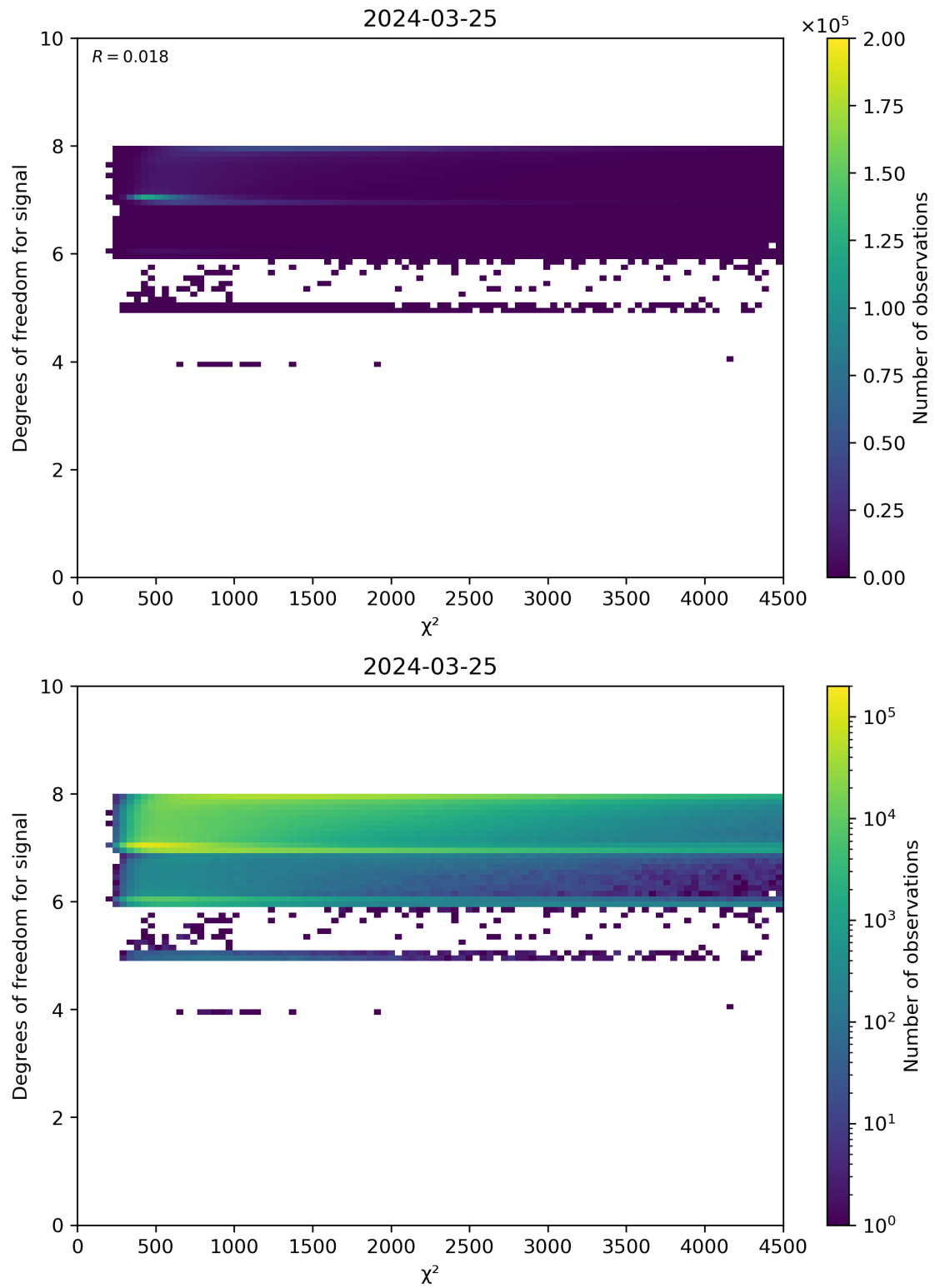
Figure 48: Scatter density plot of “ \chi^2 ” against “Degrees of freedom for signal” for 2024-03-25 to 2024-03-26.
