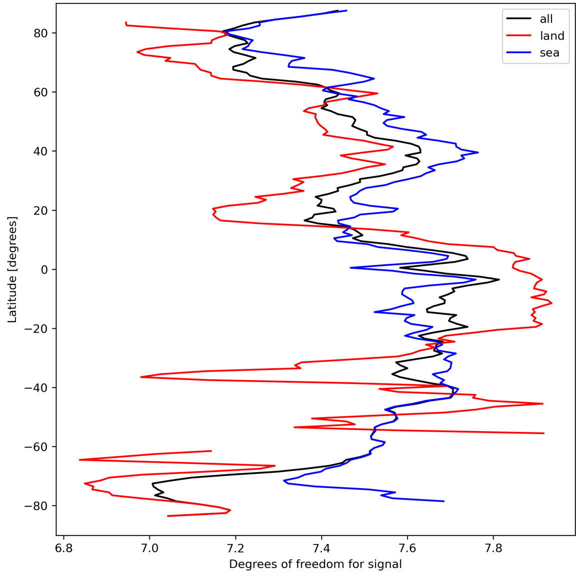
Figure 15: Zonal average of “Degrees of freedom for signal” for 2024-03-25 to 2024-03-26.
