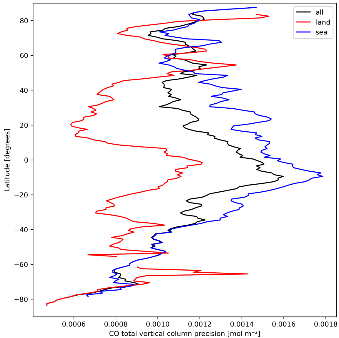
Figure 12: Zonal average of “CO total vertical column precision” for 2024-03-25 to 2024-03-26.
