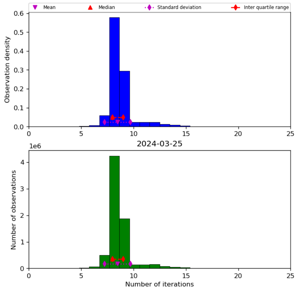
Figure 24: Histogram of “Number of iterations” for 2024-03-25 to 2024-03-26
