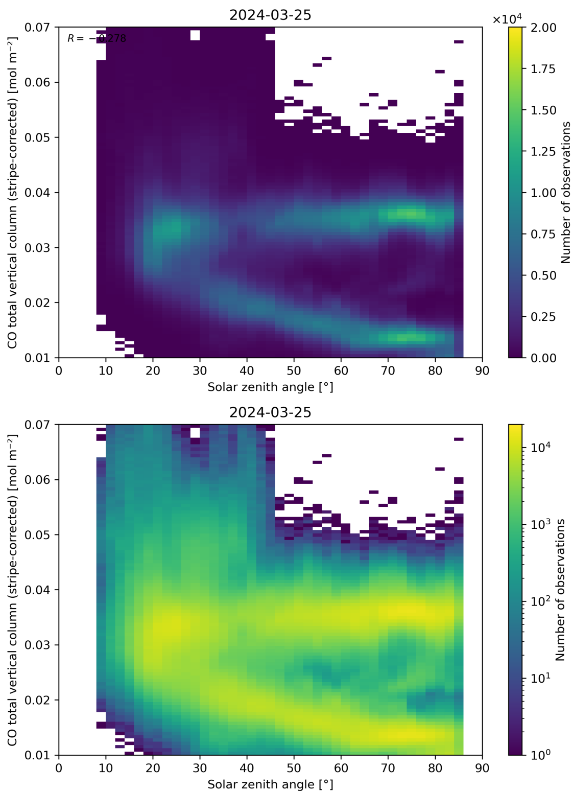
Figure 62: Scatter density plot of “Solar zenith angle” against “CO total vertical column (stripe-corrected)” for 2024-03-25 to 2024-03-26.
