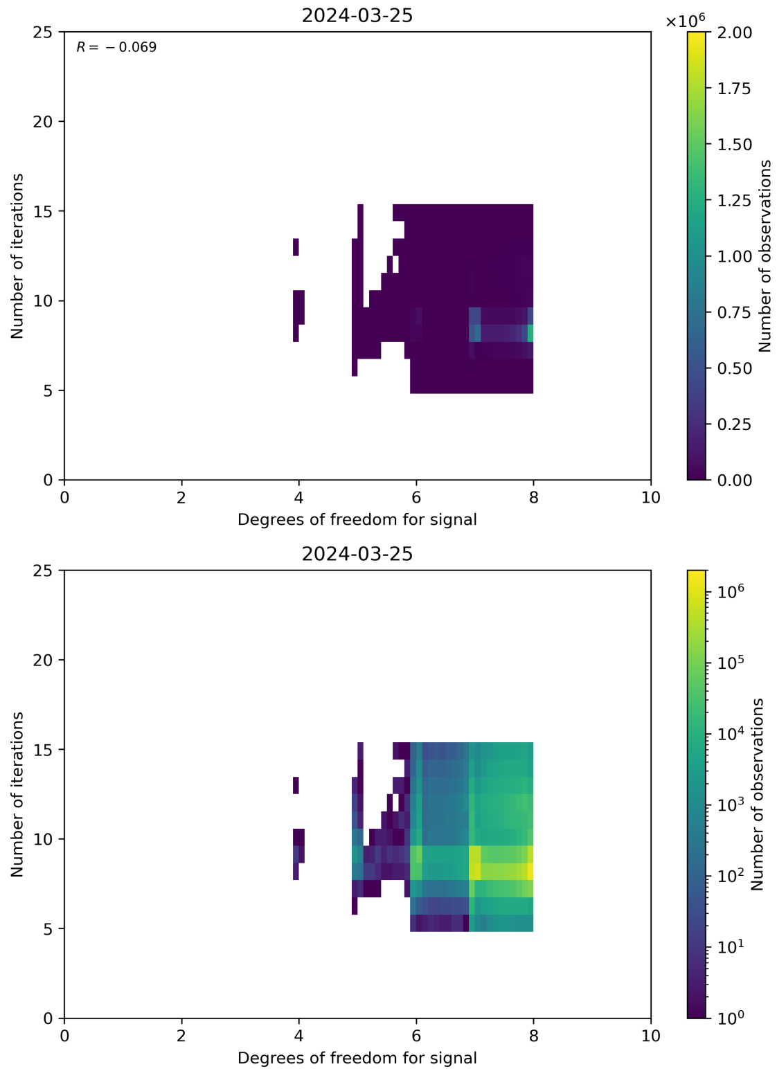
Figure 50: Scatter density plot of “Degrees of freedom for signal” against “Number of iterations” for 2024-03-25 to 2024-03-26.
