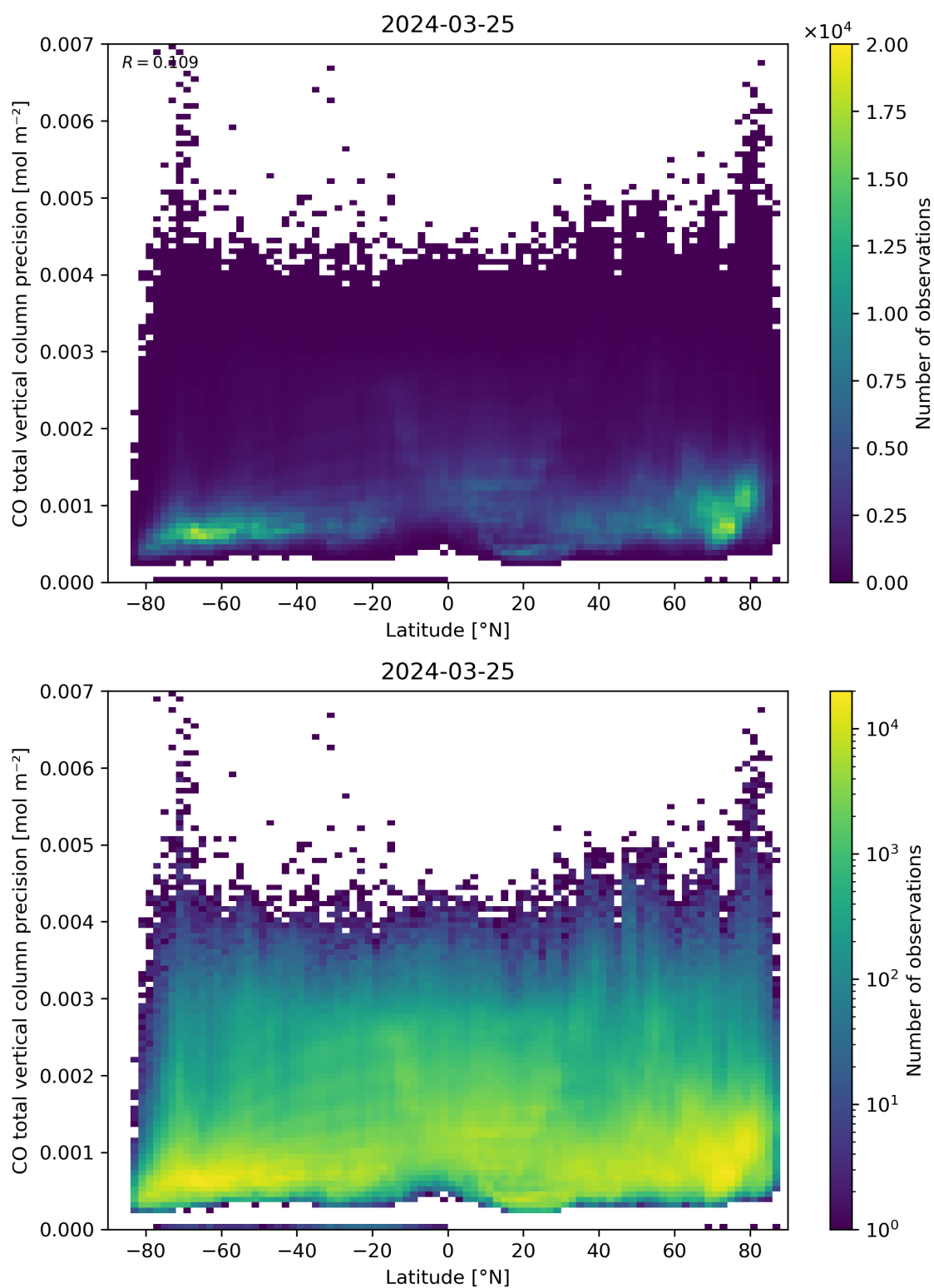
Figure 53: Scatter density plot of “Latitude” against “CO total vertical column precision” for 2024-03-25 to 2024-03-26.
