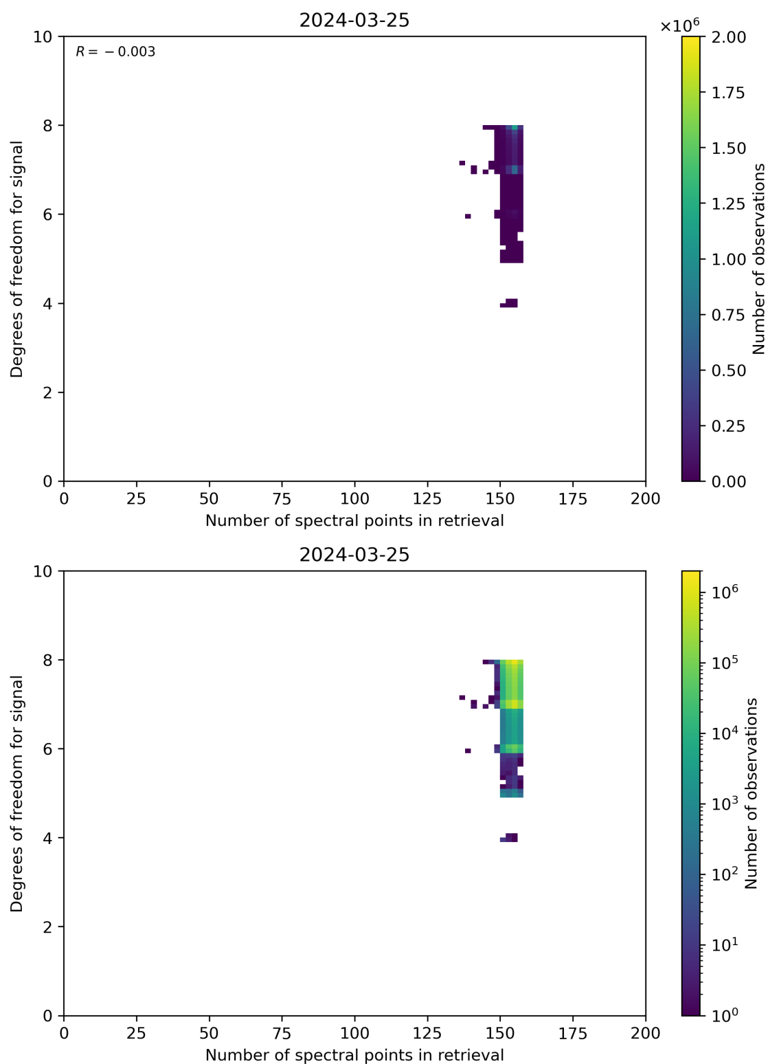
Figure 59: Scatter density plot of “Number of spectral points in retrieval” against “Degrees of freedom for signal” for 2024-03-25 to 2024-03-26.
