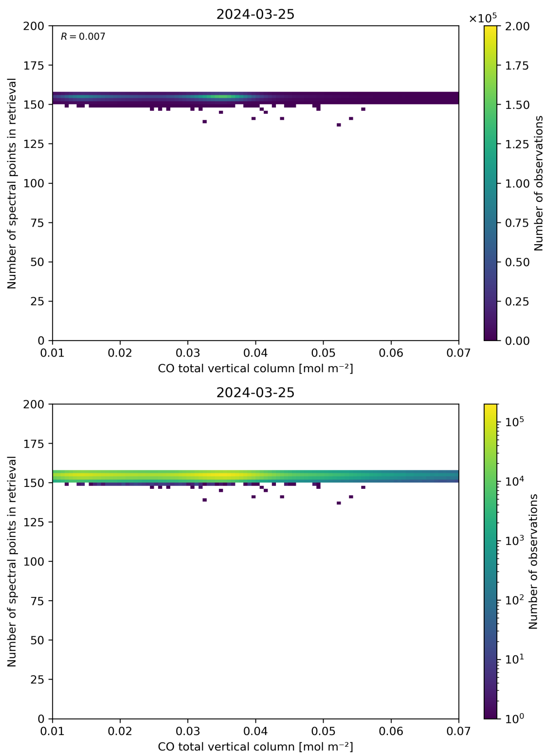
Figure 43: Scatter density plot of “CO total vertical column” against “Number of spectral points in retrieval” for 2024-03-25 to 2024-03-26.
