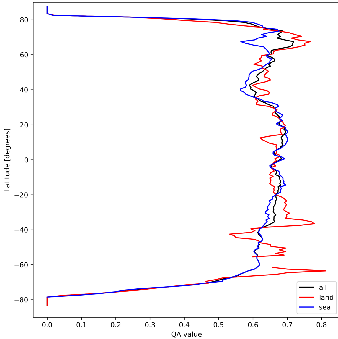
Figure 9: Zonal average of “QA value” for 2024-03-25 to 2024-03-26.
