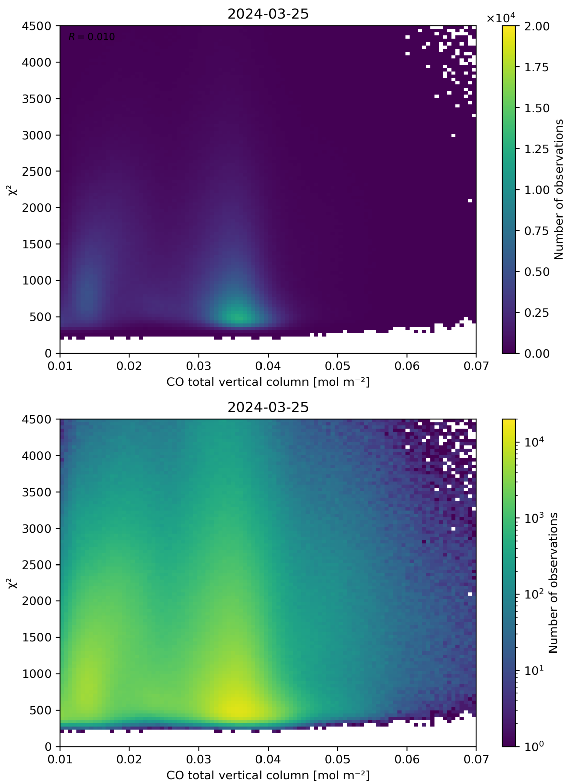
Figure 35: Scatter density plot of “CO total vertical column” against “ \chi^2 ” for 2024-03-25 to 2024-03-26.
