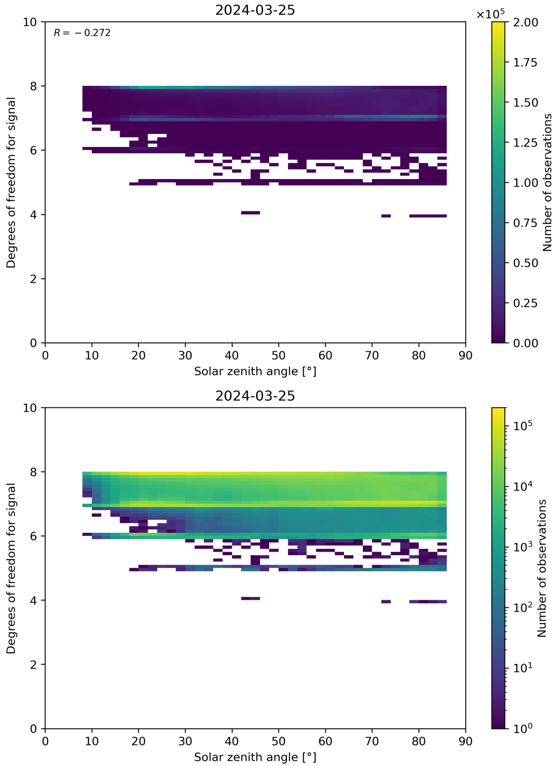
Figure 65: Scatter density plot of “Solar zenith angle” against “Degrees of freedom for signal” for 2024-03-25 to 2024-03-26.
