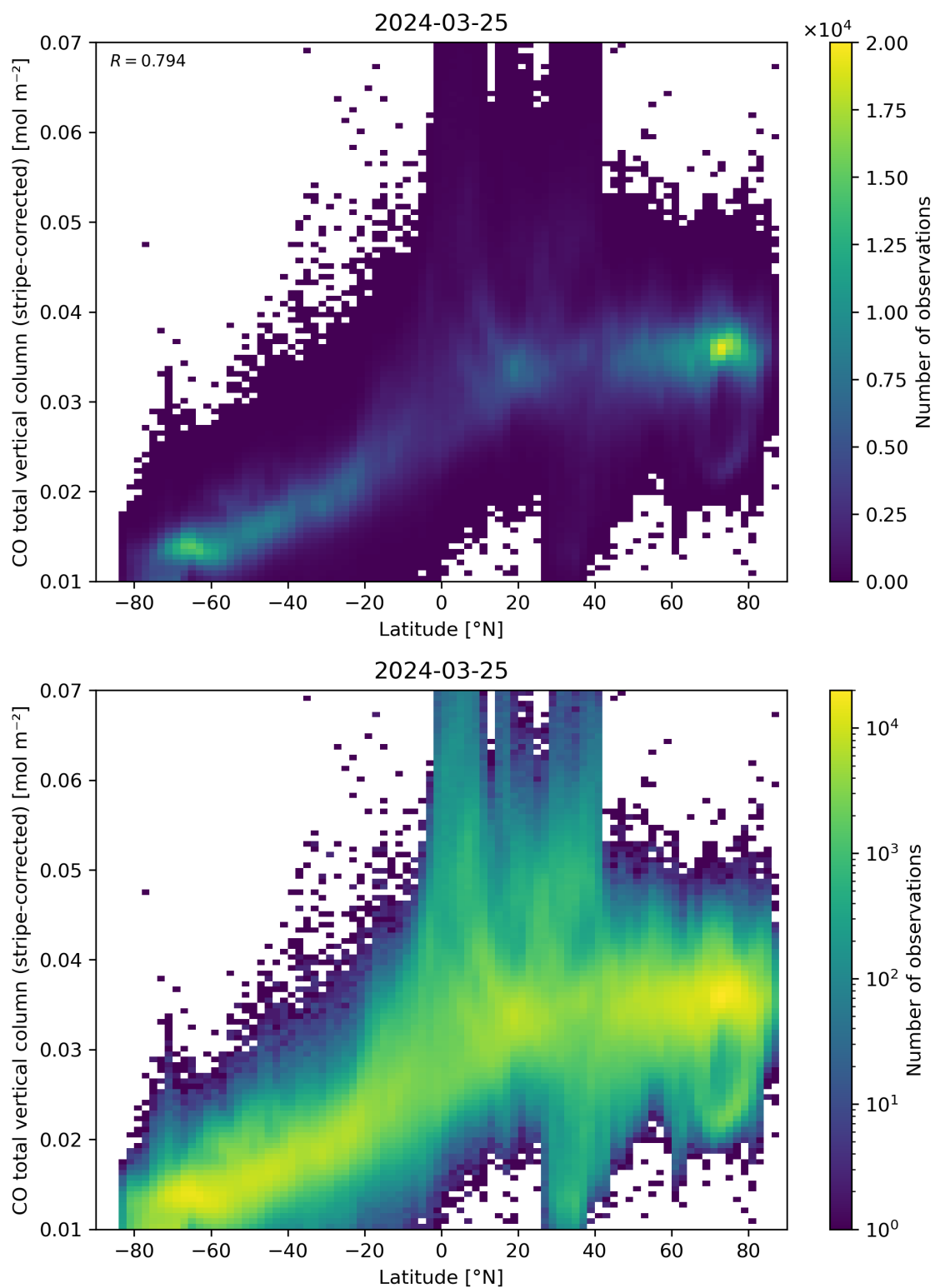
Figure 52: Scatter density plot of “Latitude” against “CO total vertical column (stripe-corrected)” for 2024-03-25 to 2024-03-26.
