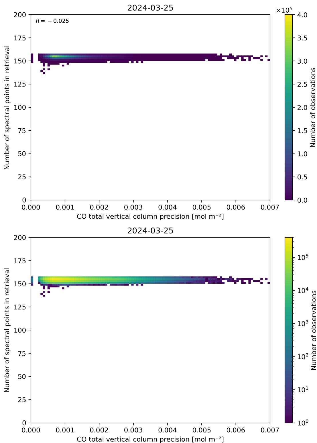
Figure 47: Scatter density plot of “CO total vertical column precision” against “Number of spectral points in retrieval” for 2024-03-25 to 2024-03-26.
