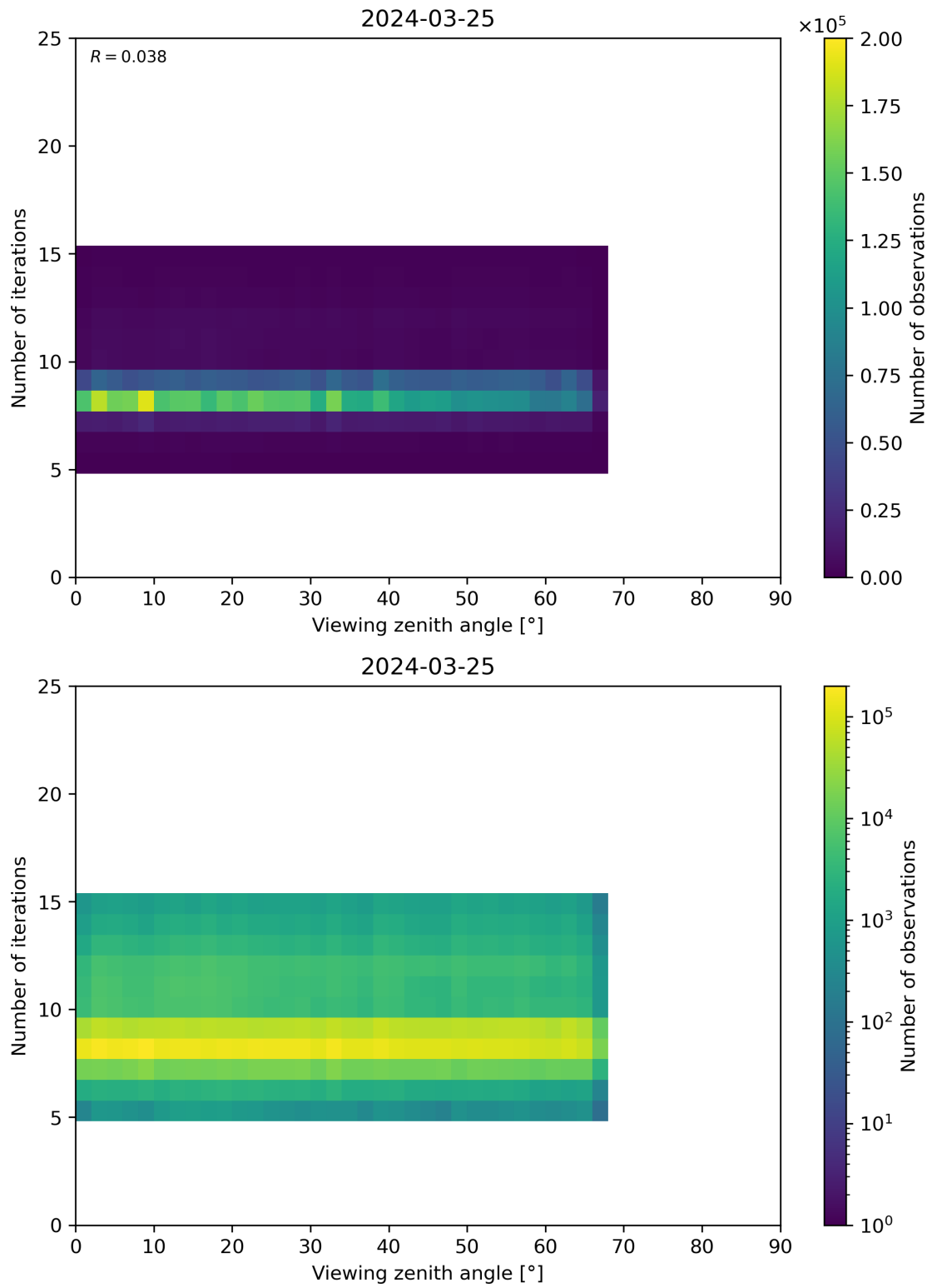
Figure 75: Scatter density plot of “Viewing zenith angle” against “Number of iterations” for 2024-03-25 to 2024-03-26.
