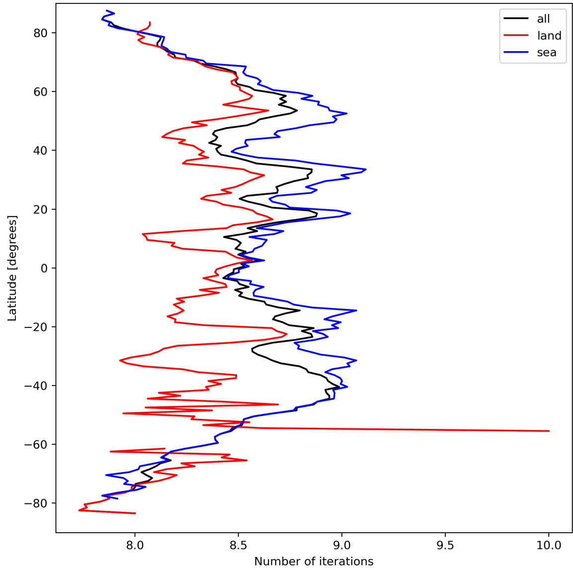
Figure 16: Zonal average of “Number of iterations” for 2024-03-25 to 2024-03-26.
