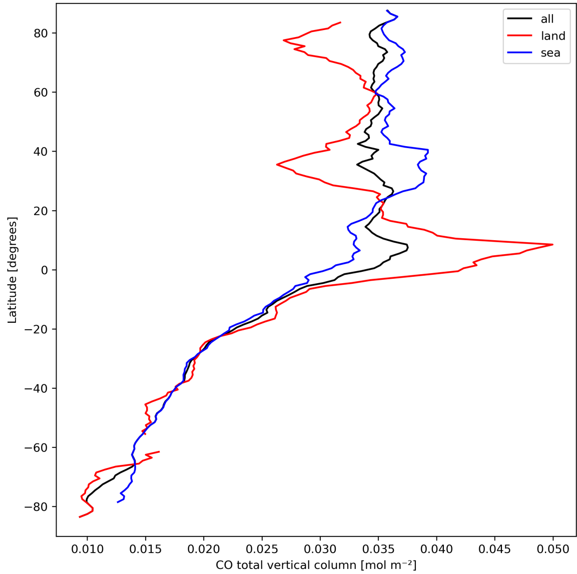
Figure 10: Zonal average of “CO total vertical column” for 2024-03-25 to 2024-03-26.
