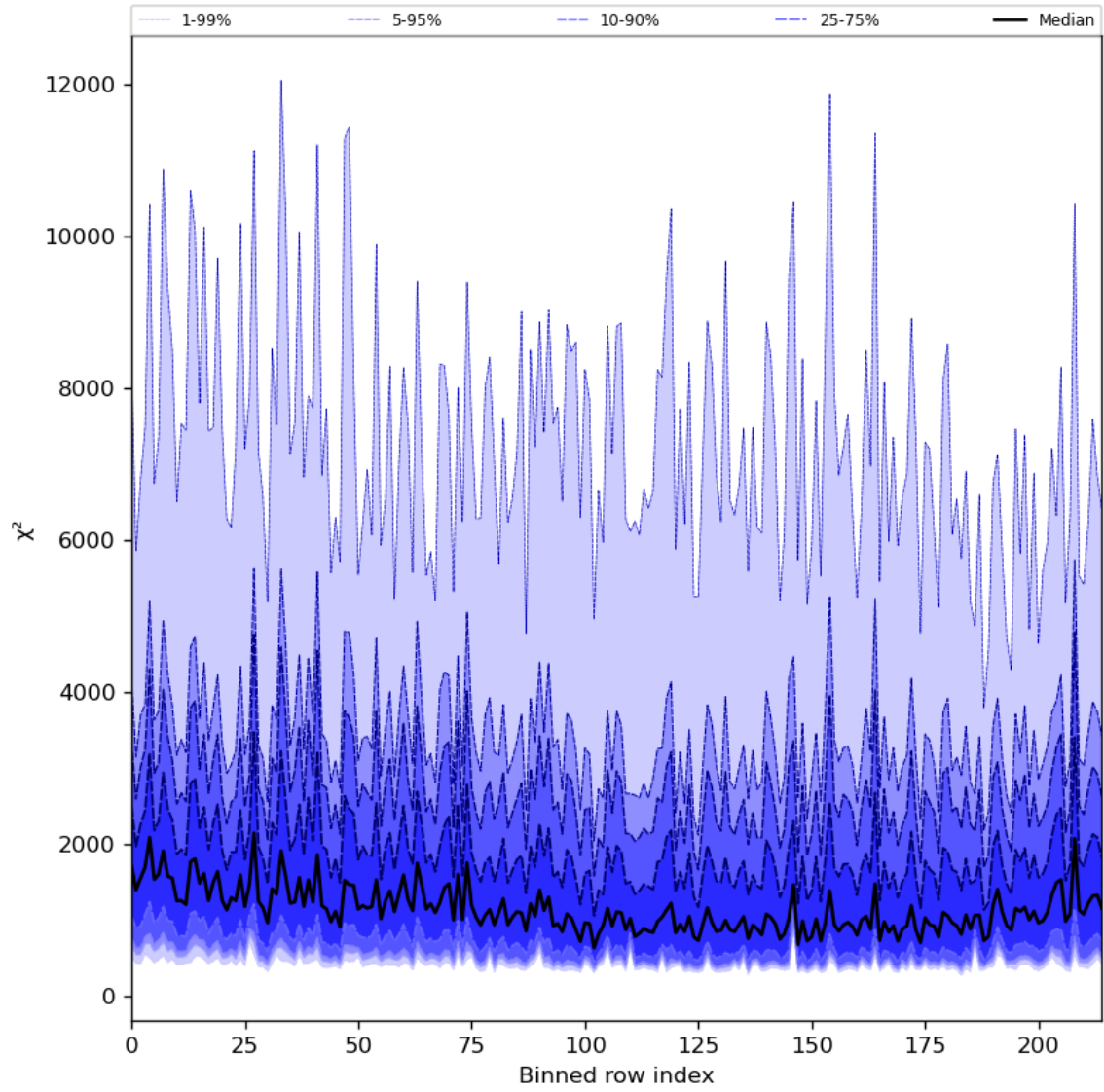
Figure 30: Along track statistics of “ \chi^2 ” for 2024-03-25 to 2024-03-26
