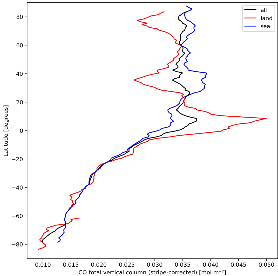
Figure 11: Zonal average of “CO total vertical column (stripe-corrected)” for 2024-03-25 to 2024-03-26.
