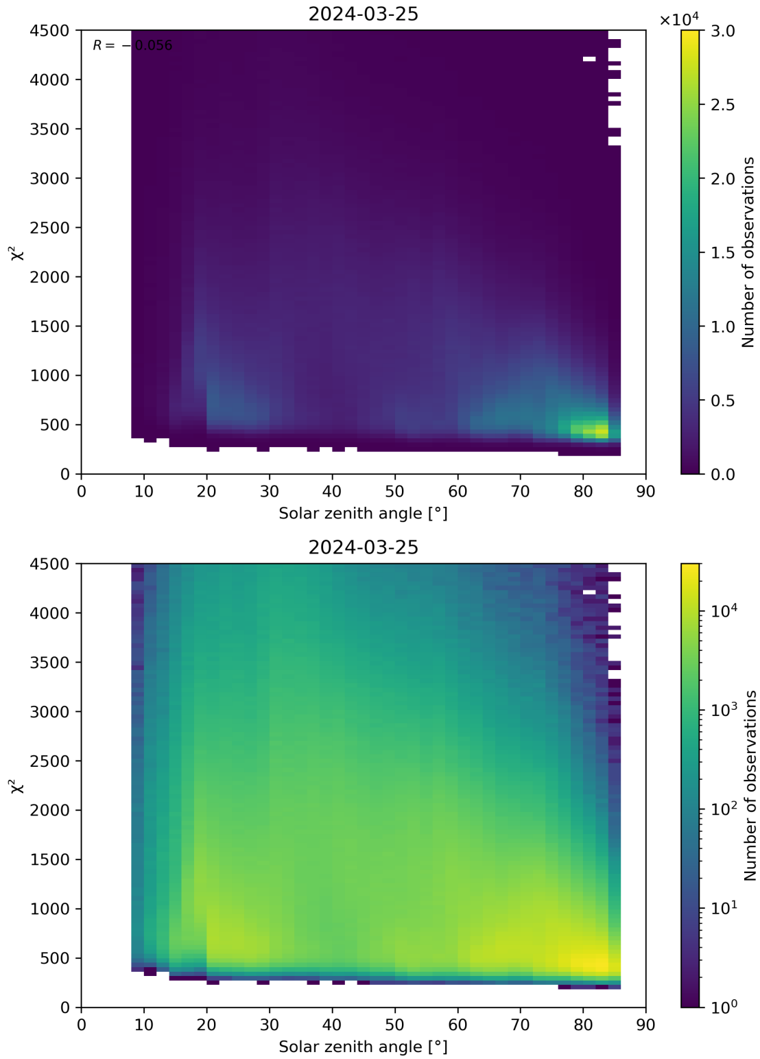
Figure 64: Scatter density plot of “Solar zenith angle” against “ \chi^2 ” for 2024-03-25 to 2024-03-26.
