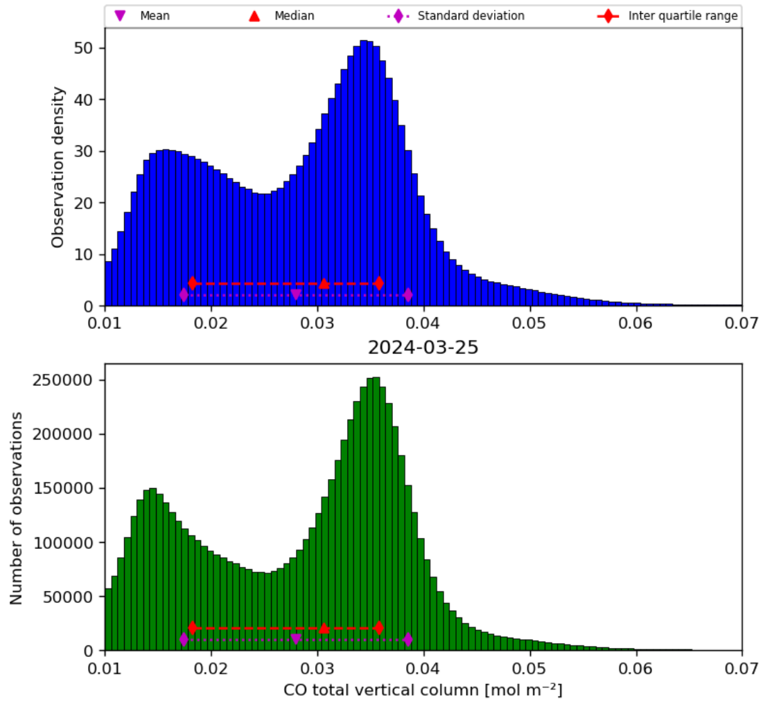
Figure 18: Histogram of “CO total vertical column” for 2024-03-25 to 2024-03-26
