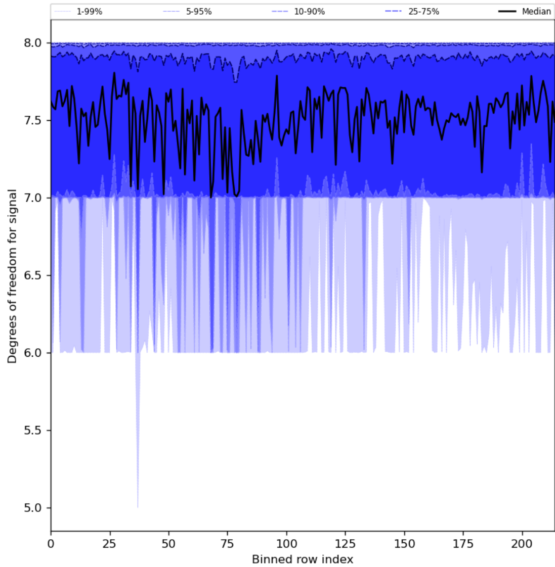
Figure 31: Along track statistics of “Degrees of freedom for signal” for 2024-03-25 to 2024-03-26
