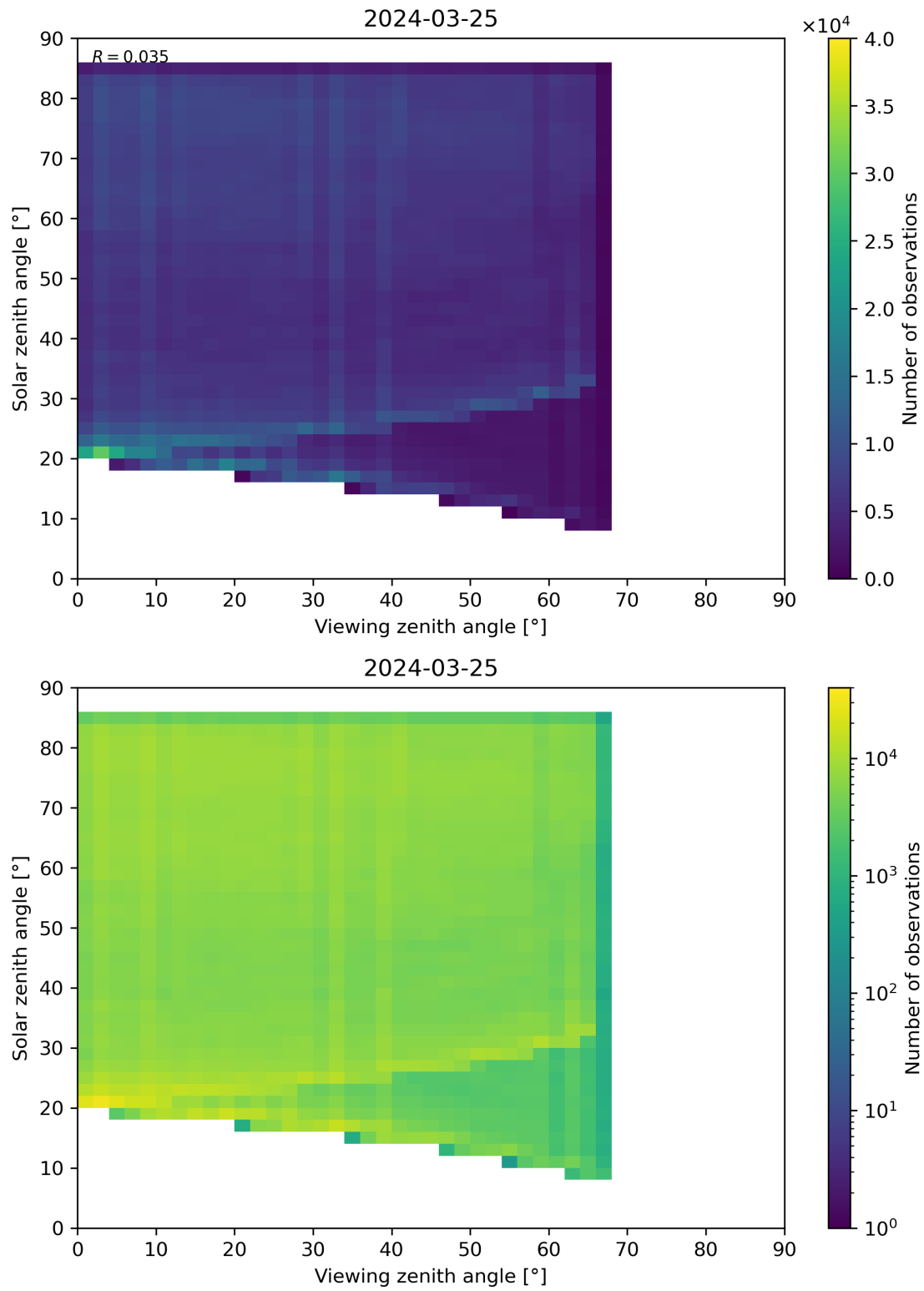
Figure 77: Scatter density plot of “Viewing zenith angle” against “Solar zenith angle” for 2024-03-25 to 2024-03-26.
