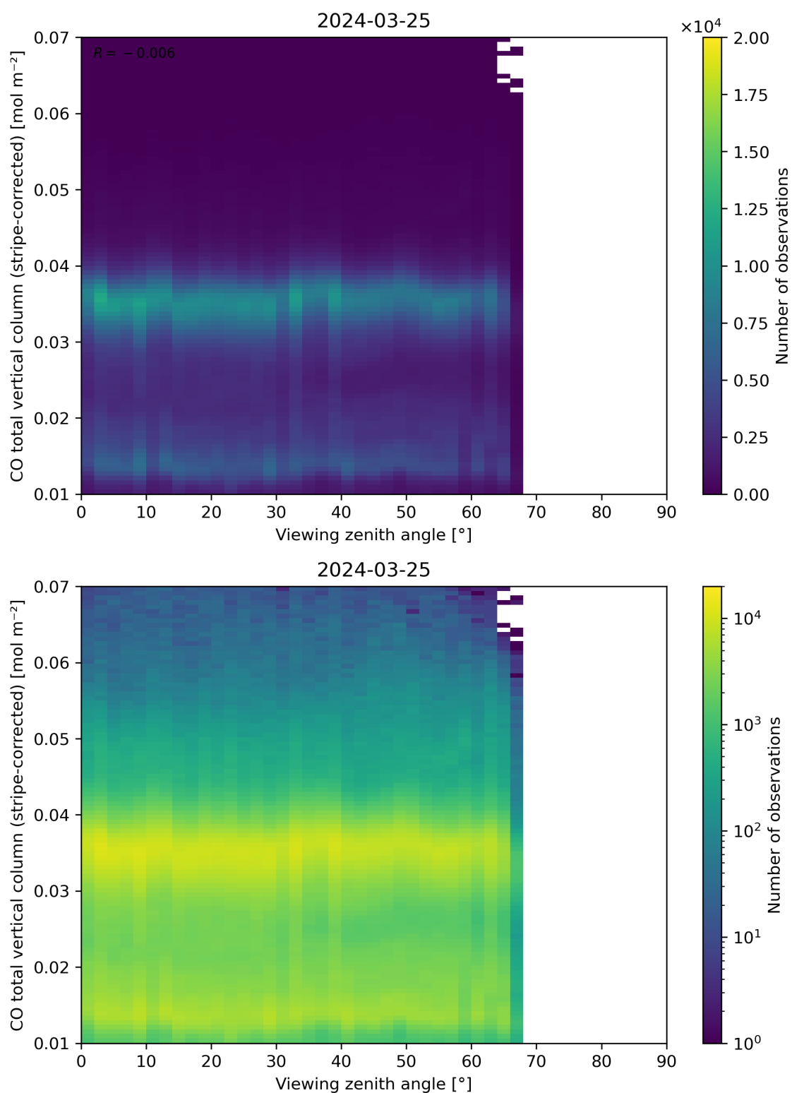
Figure 70: Scatter density plot of “Viewing zenith angle” against “CO total vertical column (stripe-corrected)” for 2024-03-25 to 2024-03-26.
