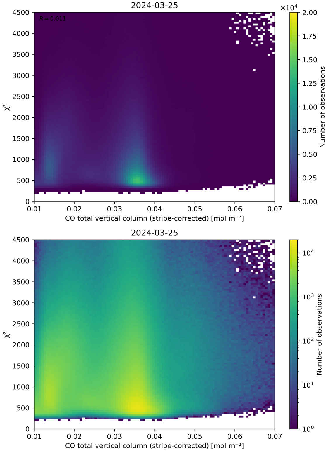
Figure 37: Scatter density plot of “CO total vertical column (stripe-corrected)” against “ \chi^2 ” for 2024-03-25 to 2024-03-26.
