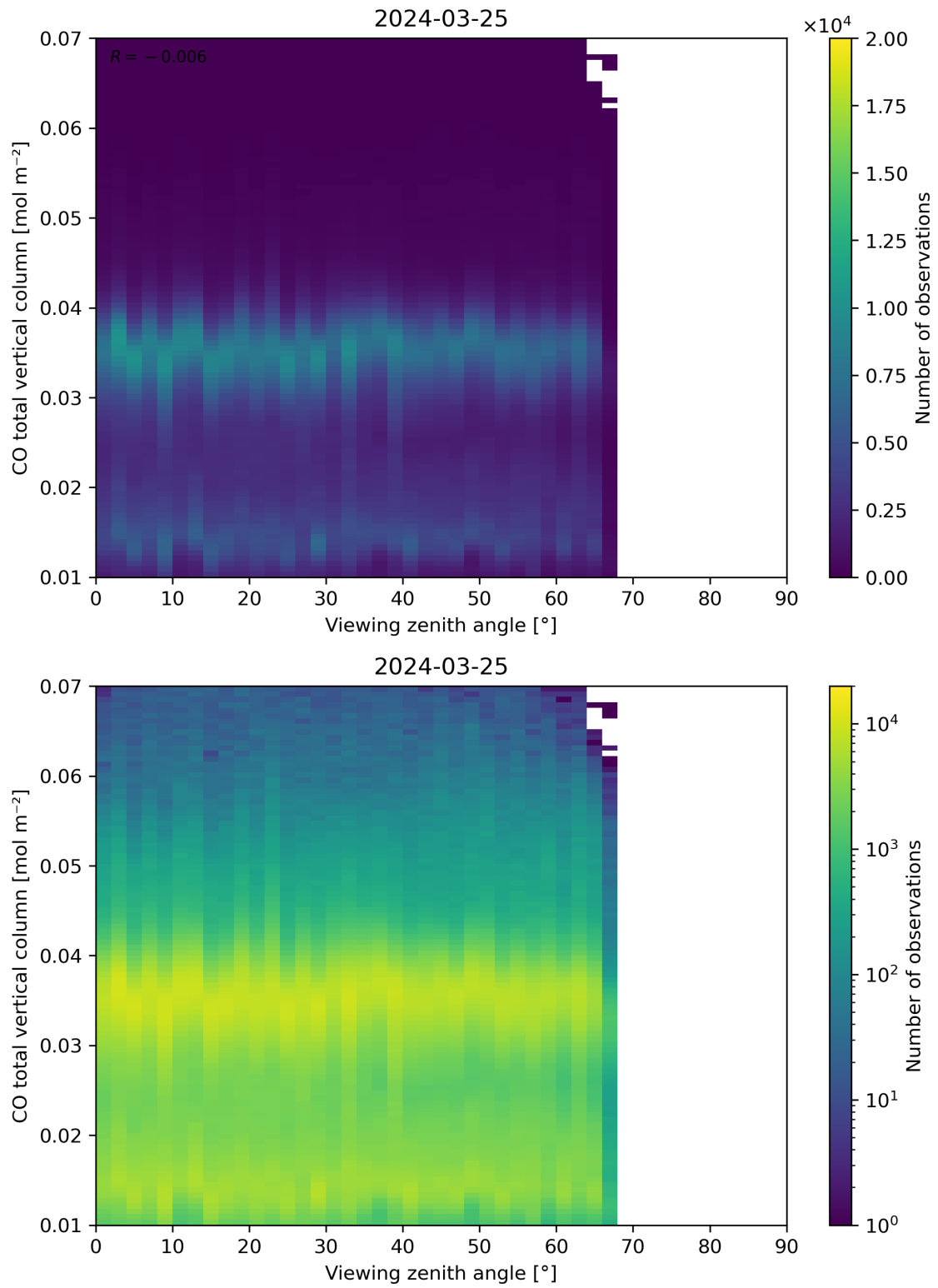
Figure 69: Scatter density plot of “Viewing zenith angle” against “CO total vertical column” for 2024-03-25 to 2024-03-26.
