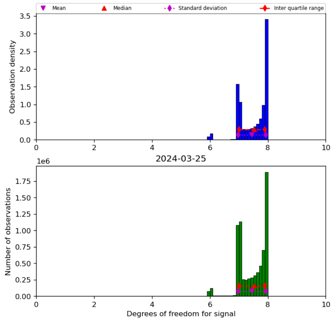
Figure 23: Histogram of “Degrees of freedom for signal” for 2024-03-25 to 2024-03-26
