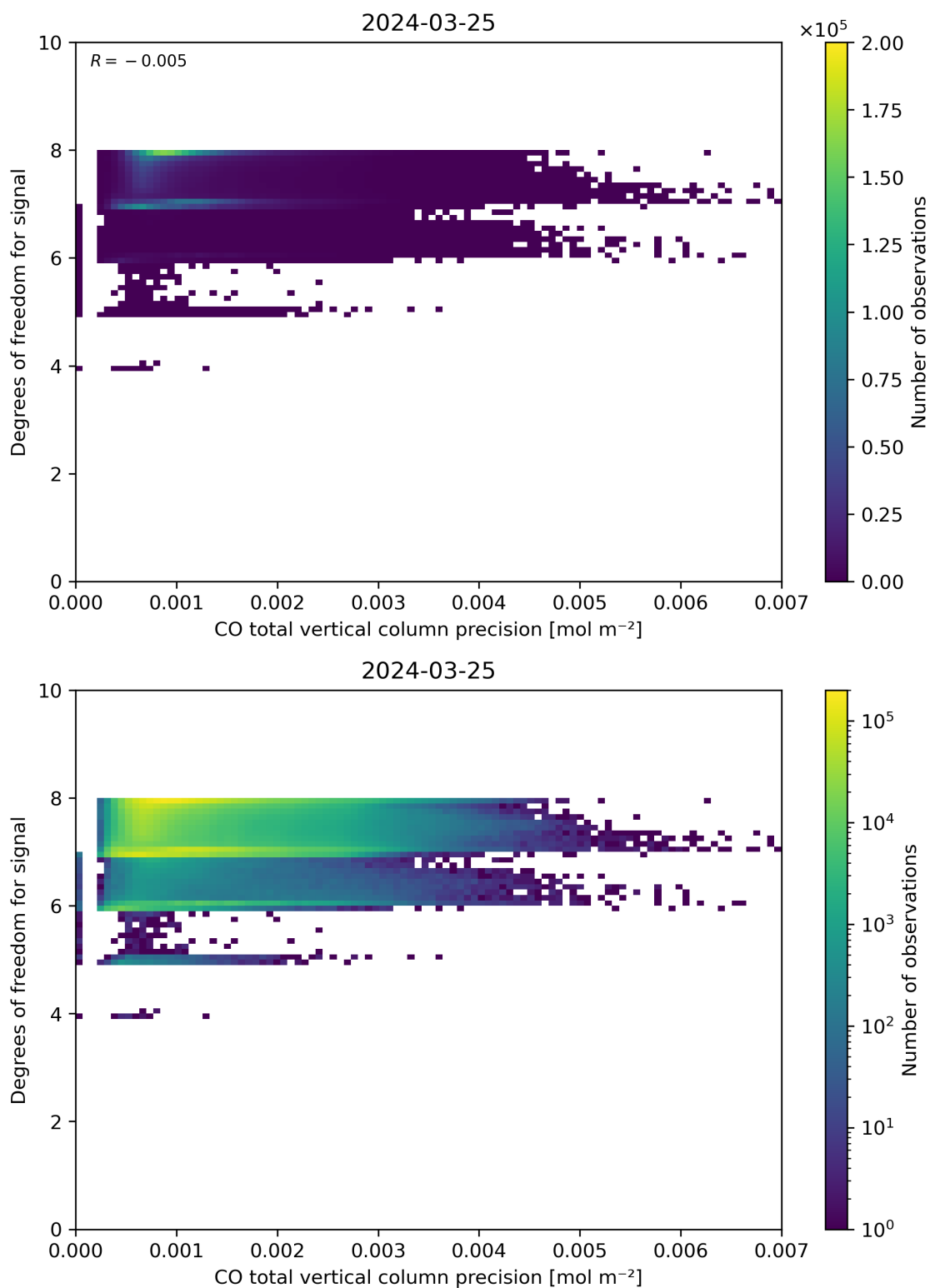
Figure 45: Scatter density plot of “CO total vertical column precision” against “Degrees of freedom for signal” for 2024-03-25 to 2024-03-26.
