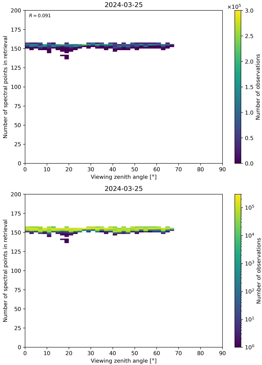
Figure 76: Scatter density plot of “Viewing zenith angle” against “Number of spectral points in retrieval” for 2024-03-25 to 2024-03-26.
