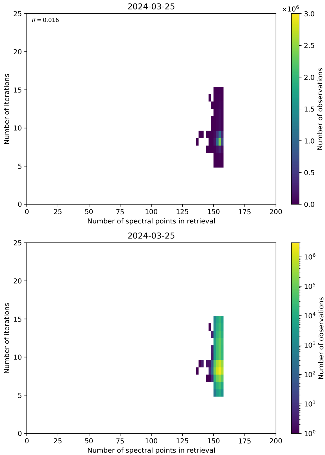
Figure 60: Scatter density plot of “Number of spectral points in retrieval” against “Number of iterations” for 2024-03-25 to 2024-03-26.
