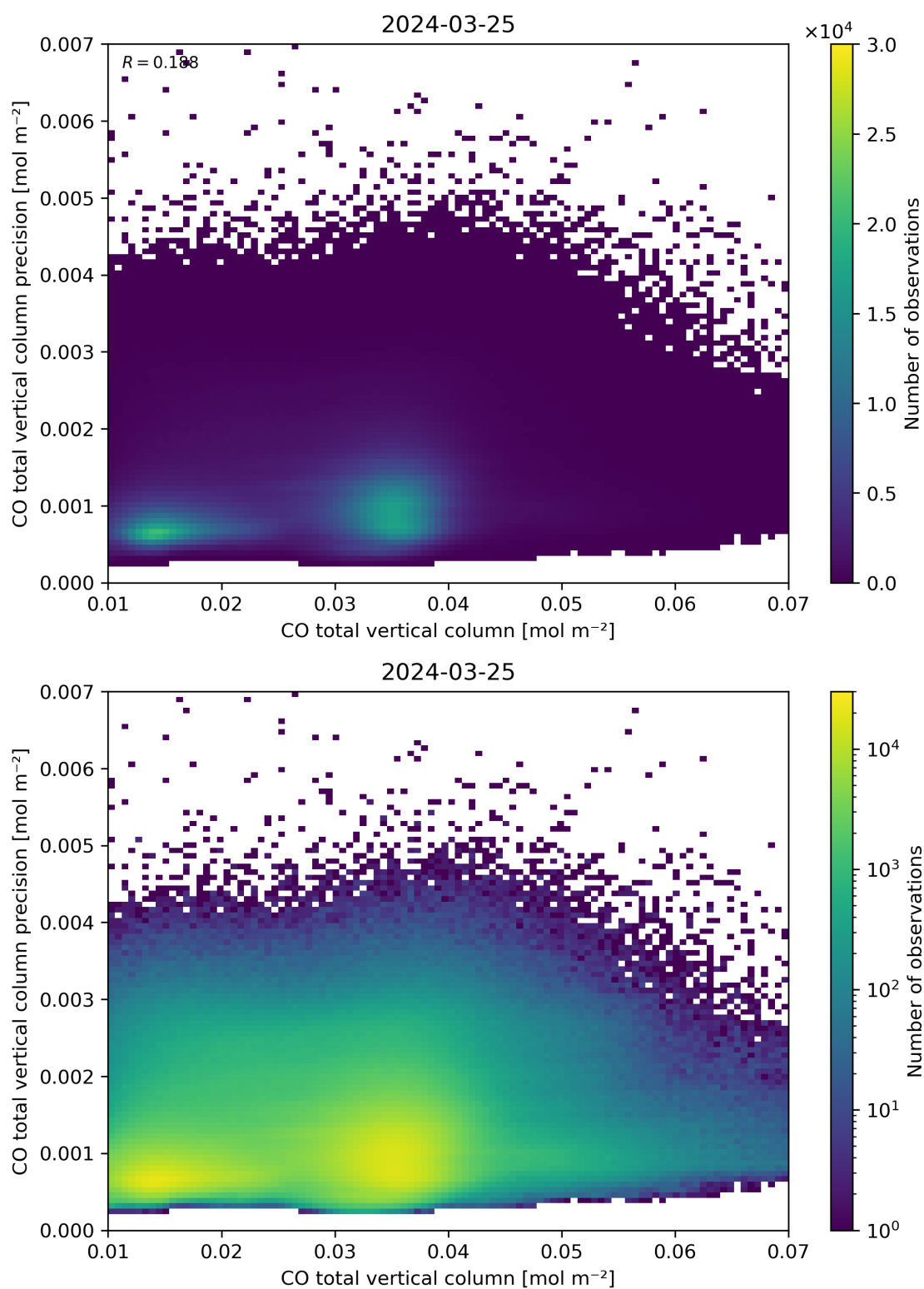
Figure 34: Scatter density plot of “CO total vertical column” against “CO total vertical column precision” for 2024-03-25 to 2024-03-26.
