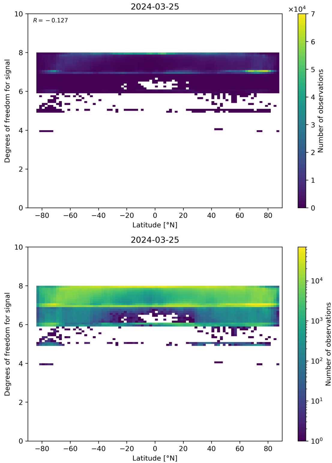
Figure 55: Scatter density plot of “Latitude” against “Degrees of freedom for signal” for 2024-03-25 to 2024-03-26.
