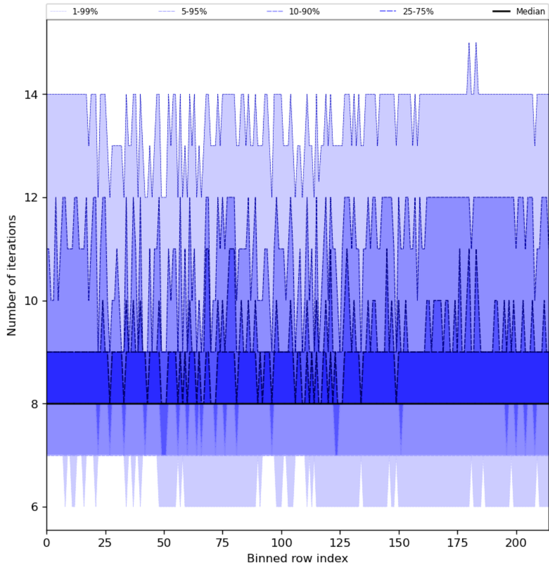
Figure 32: Along track statistics of “Number of iterations” for 2024-03-25 to 2024-03-26
