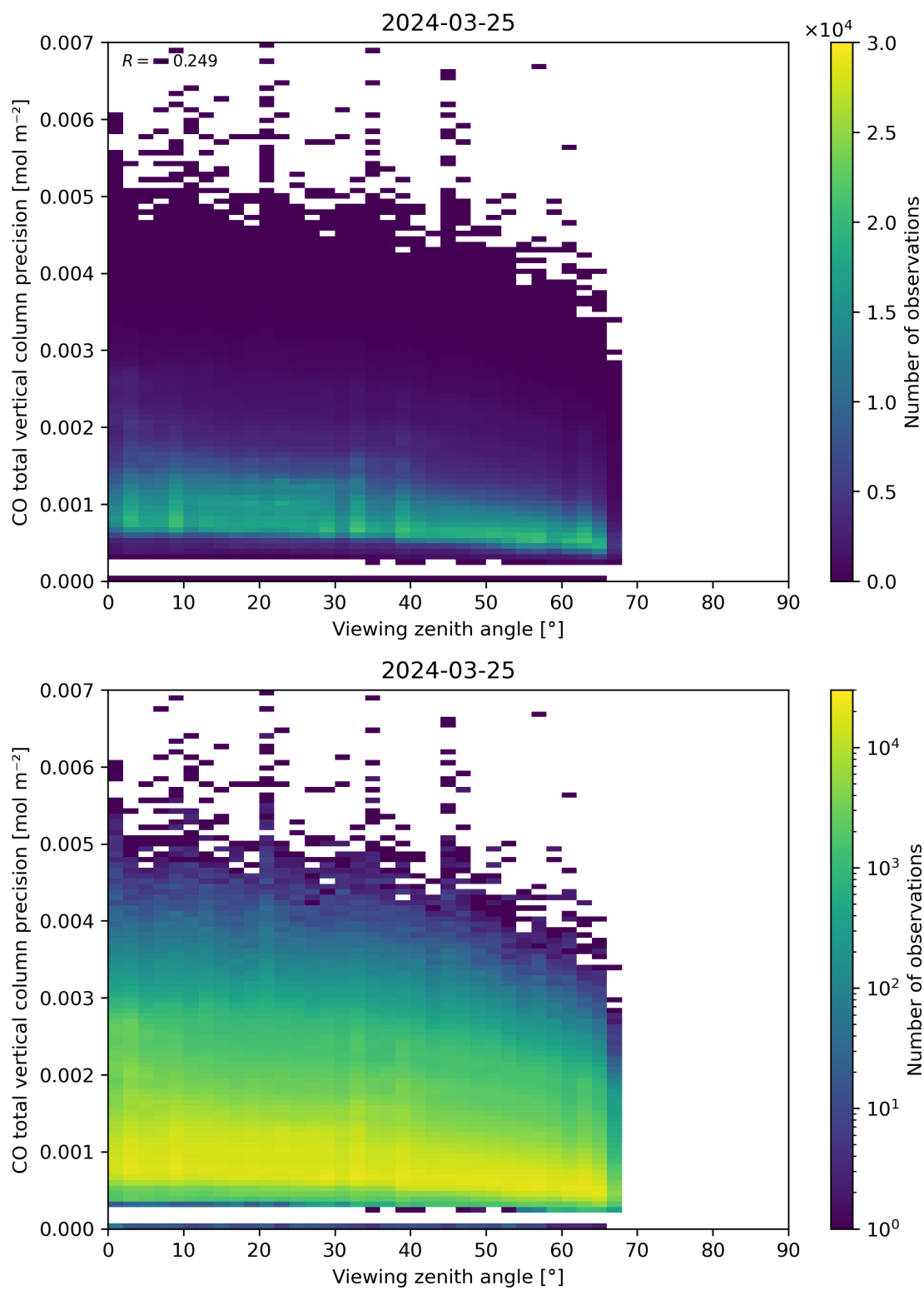
Figure 71: Scatter density plot of “Viewing zenith angle” against “CO total vertical column precision” for 2024-03-25 to 2024-03-26.
