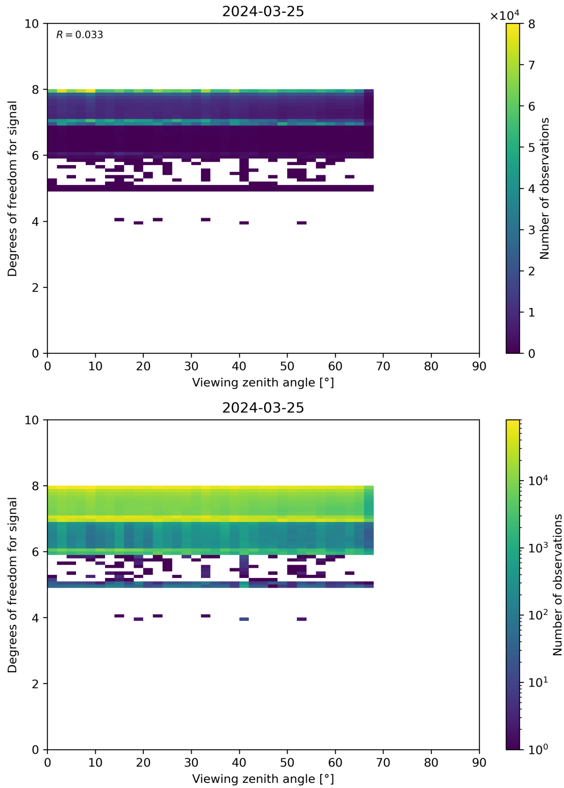
Figure 73: Scatter density plot of “Viewing zenith angle” against “Degrees of freedom for signal” for 2024-03-25 to 2024-03-26.
