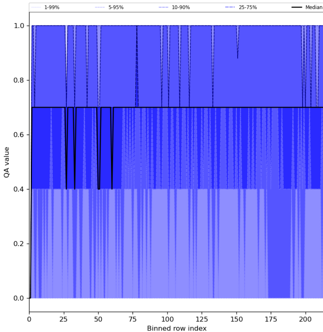
Figure 25: Along track statistics of “QA value” for 2024-03-25 to 2024-03-26
