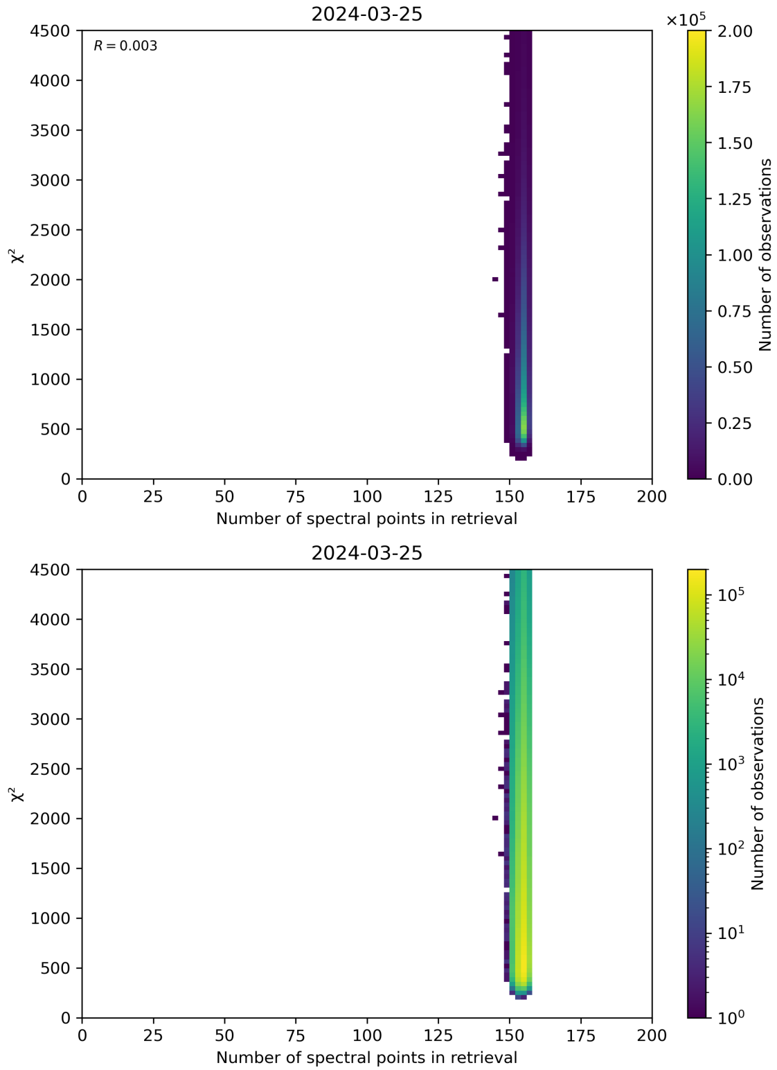
Figure 58: Scatter density plot of “Number of spectral points in retrieval” against “ \chi^2 ” for 2024-03-25 to 2024-03-26.
