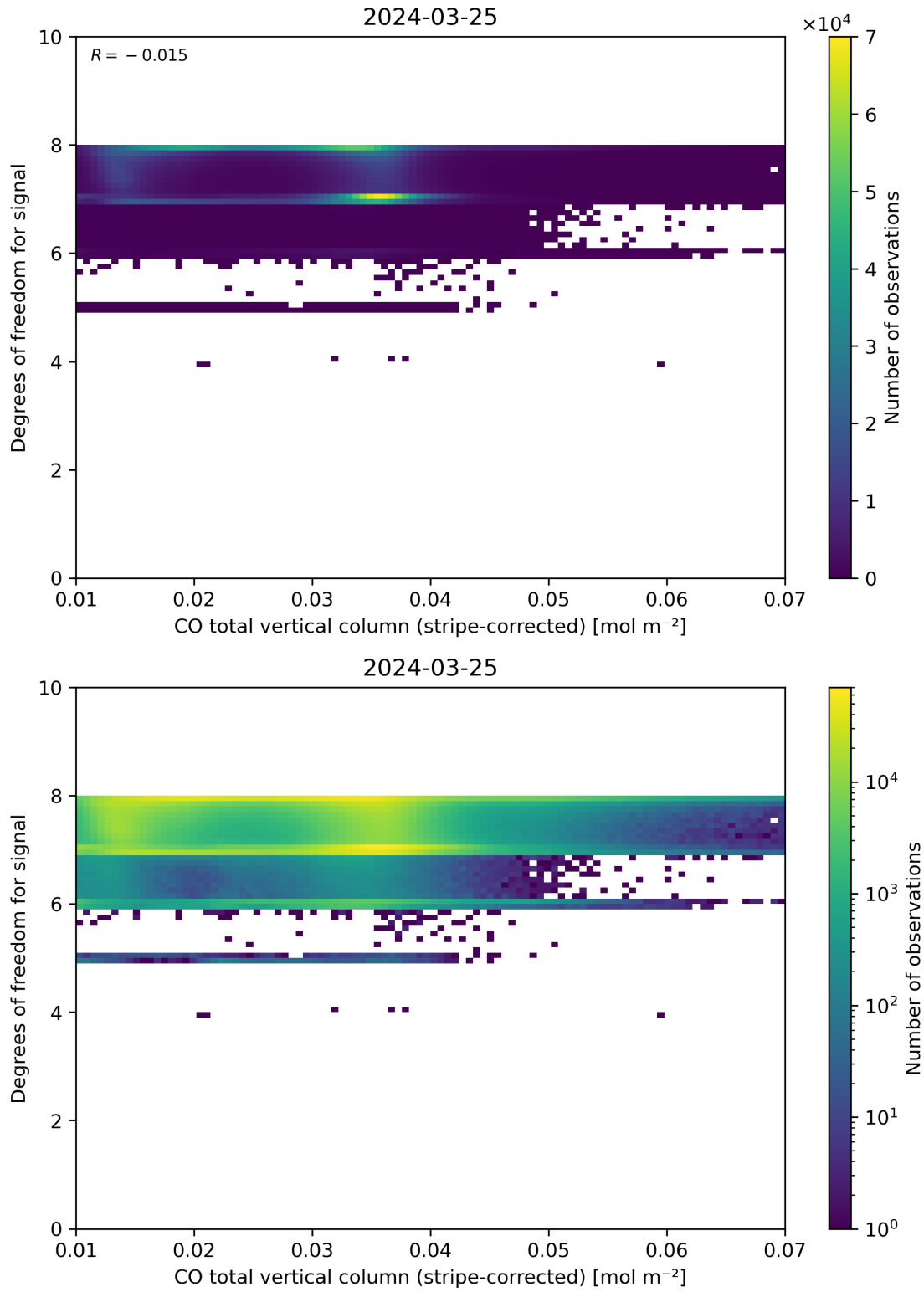
Figure 38: Scatter density plot of “CO total vertical column (stripe-corrected)” against “Degrees of freedom for signal” for 2024-03-25 to 2024-03-26.
