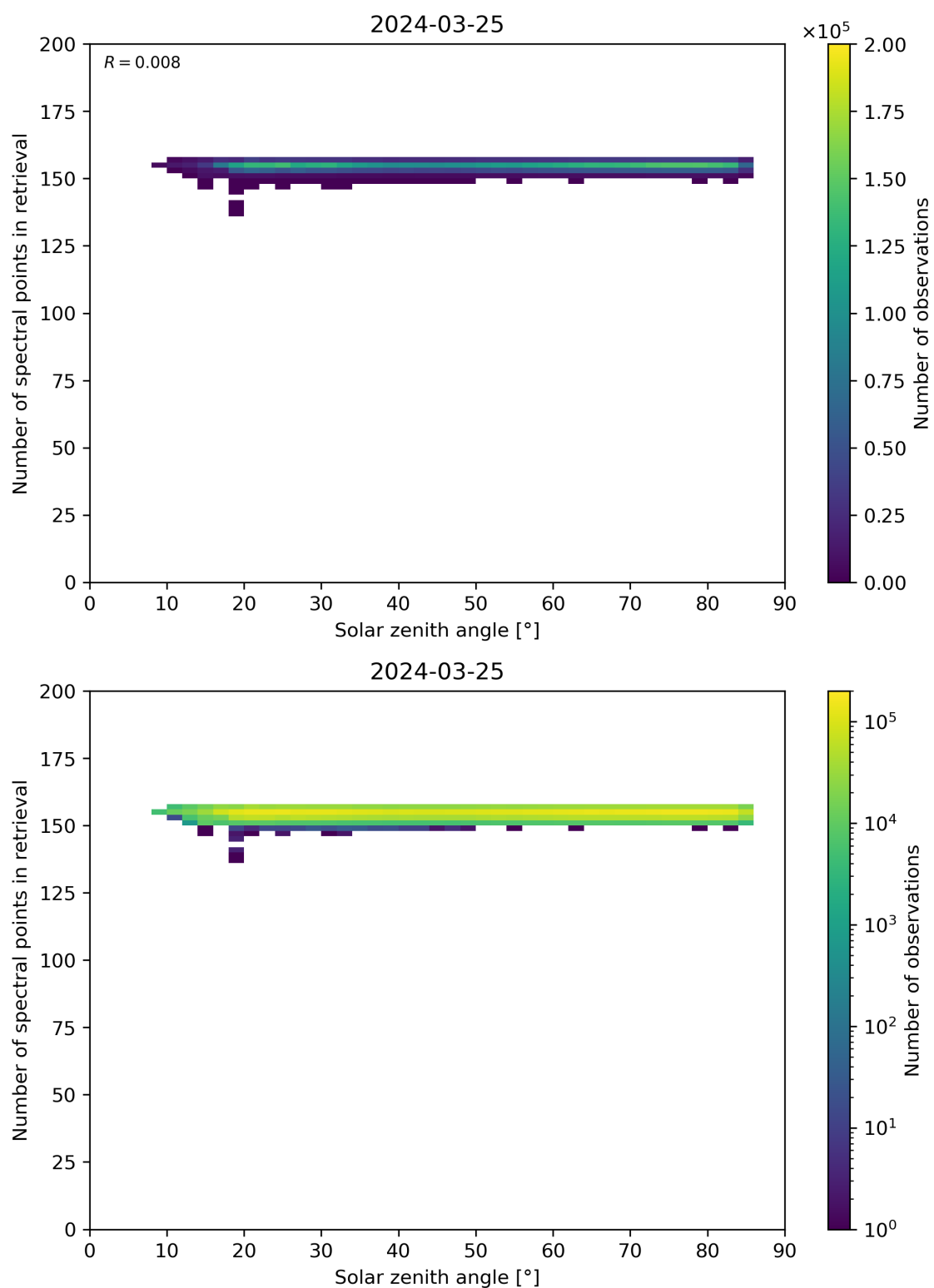
Figure 68: Scatter density plot of “Solar zenith angle” against “Number of spectral points in retrieval” for 2024-03-25 to 2024-03-26.
