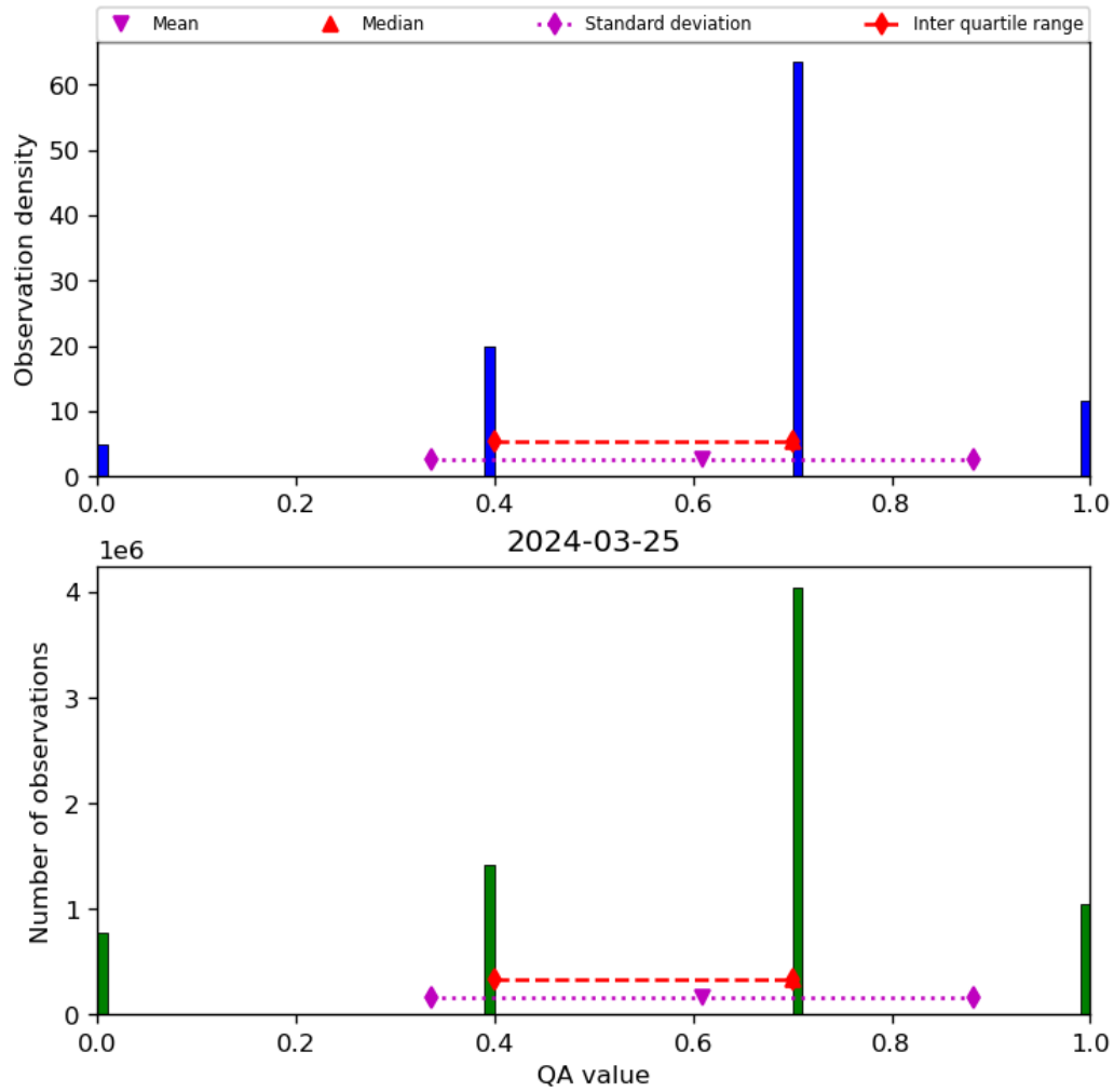
Figure 17: Histogram of “QA value” for 2024-03-25 to 2024-03-26
