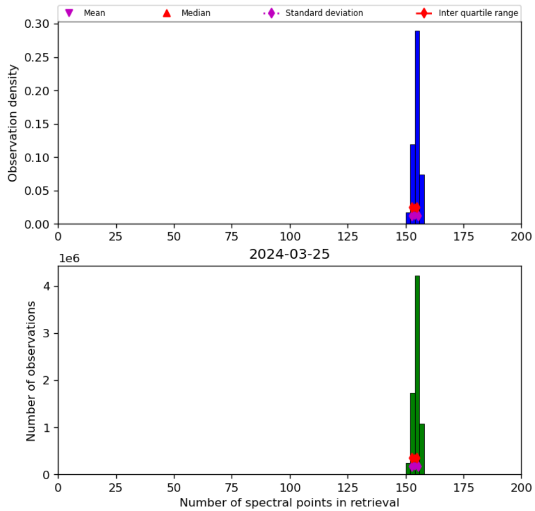
Figure 21: Histogram of “Number of spectral points in retrieval” for 2024-03-25 to 2024-03-26
