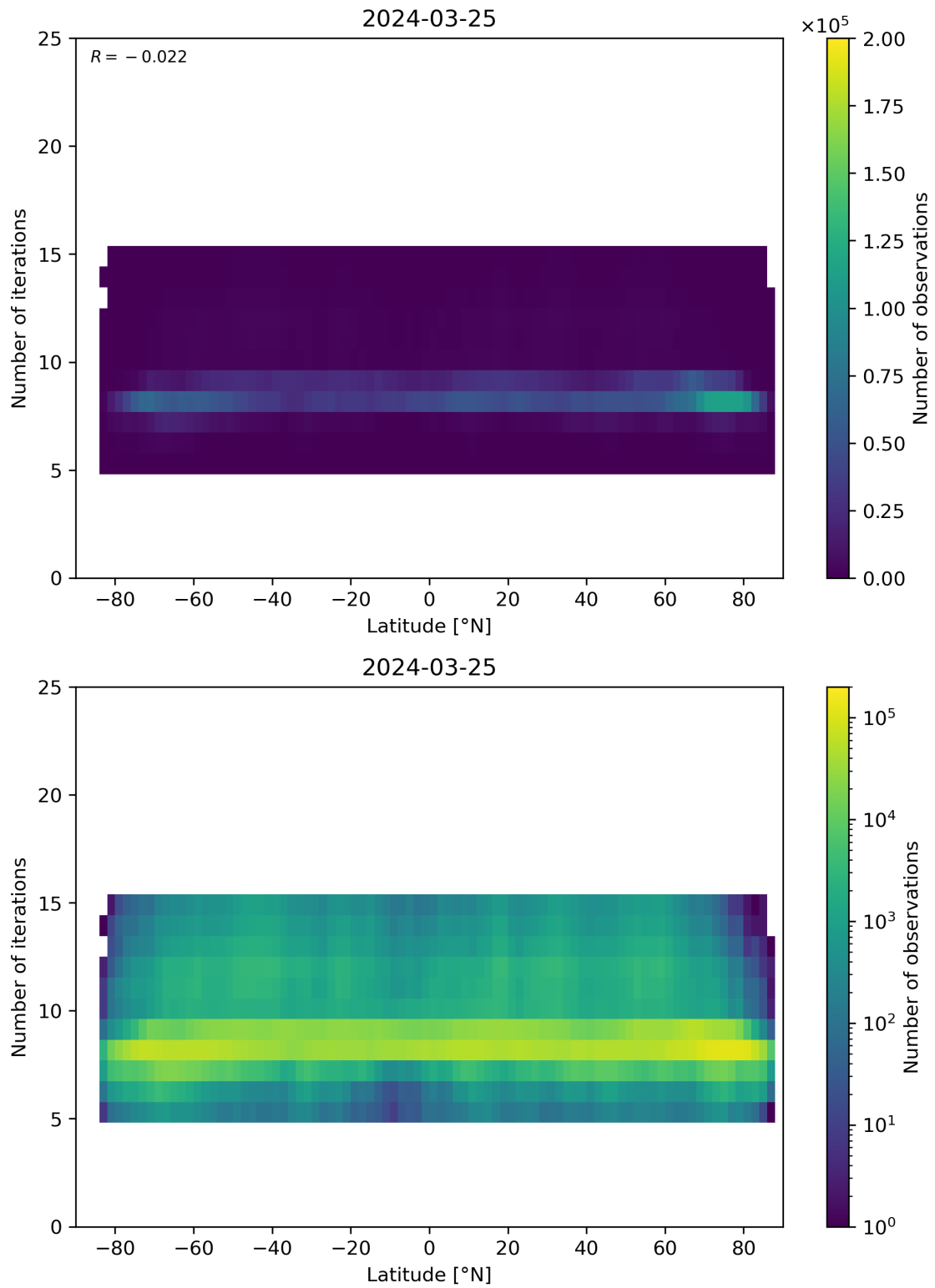
Figure 56: Scatter density plot of “Latitude” against “Number of iterations” for 2024-03-25 to 2024-03-26.
