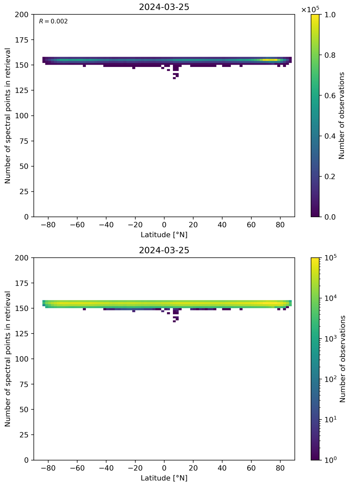
Figure 57: Scatter density plot of “Latitude” against “Number of spectral points in retrieval” for 2024-03-25 to 2024-03-26.
