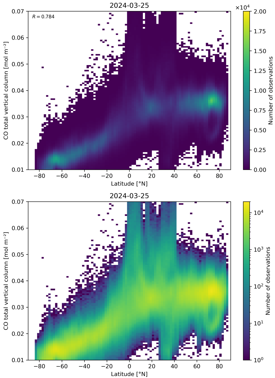
Figure 51: Scatter density plot of “Latitude” against “CO total vertical column” for 2024-03-25 to 2024-03-26.
