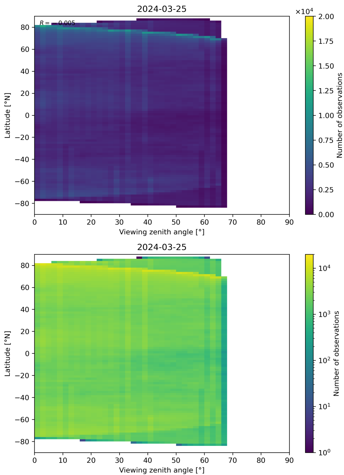
Figure 74: Scatter density plot of “Viewing zenith angle” against “Latitude” for 2024-03-25 to 2024-03-26.
