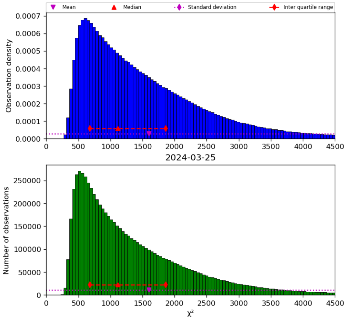
Figure 22: Histogram of “ \chi^2 ” for 2024-03-25 to 2024-03-26
