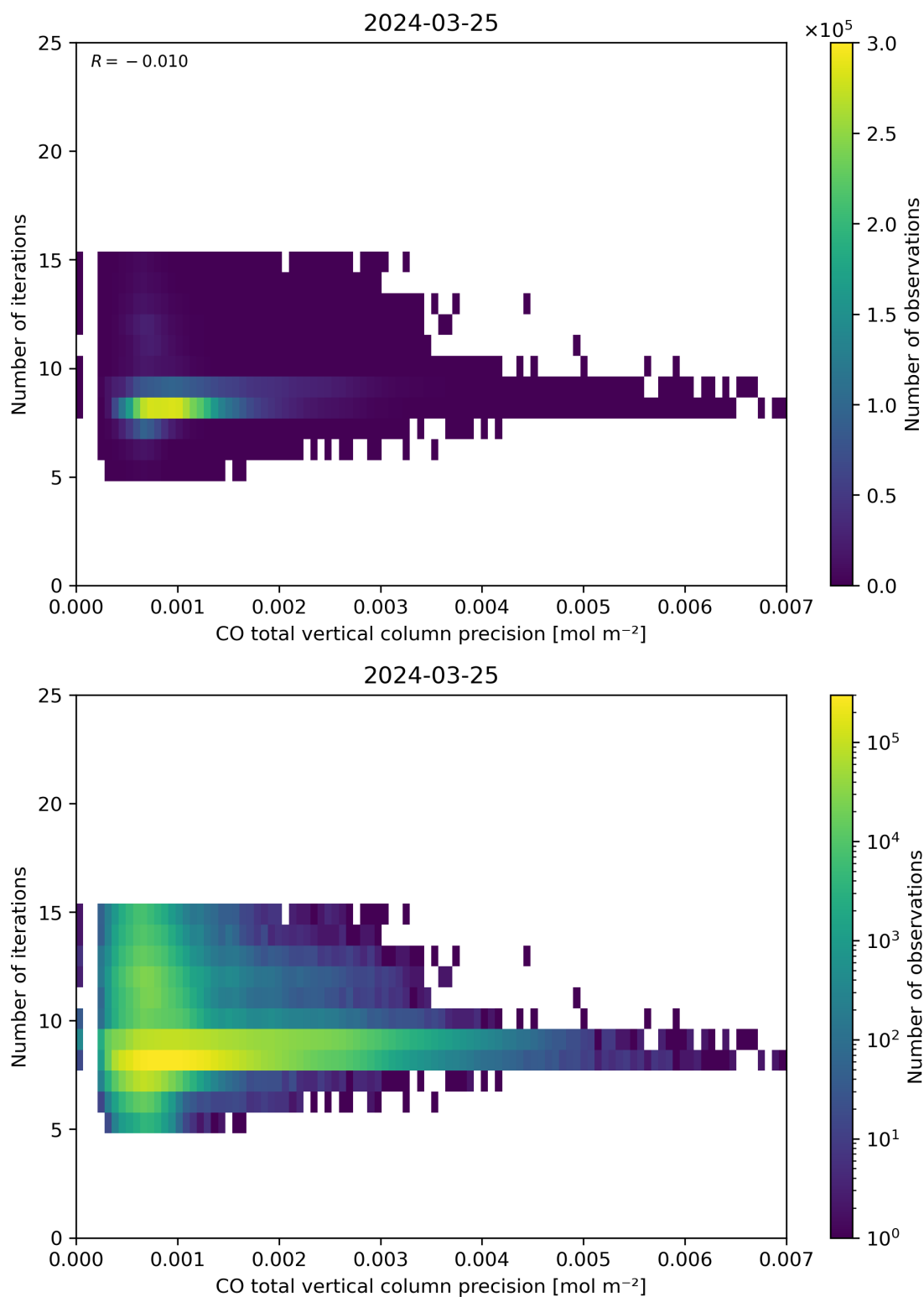
Figure 46: Scatter density plot of “CO total vertical column precision” against “Number of iterations” for 2024-03-25 to 2024-03-26.
