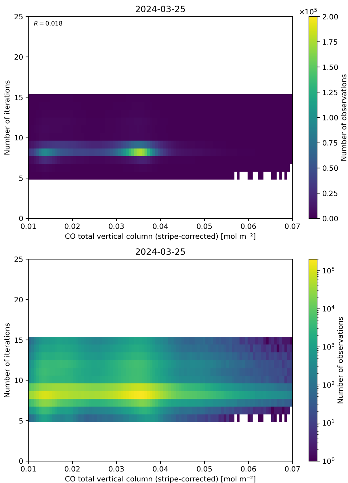
Figure 39: Scatter density plot of “CO total vertical column (stripe-corrected)” against “Number of iterations” for 2024-03-25 to 2024-03-26.
