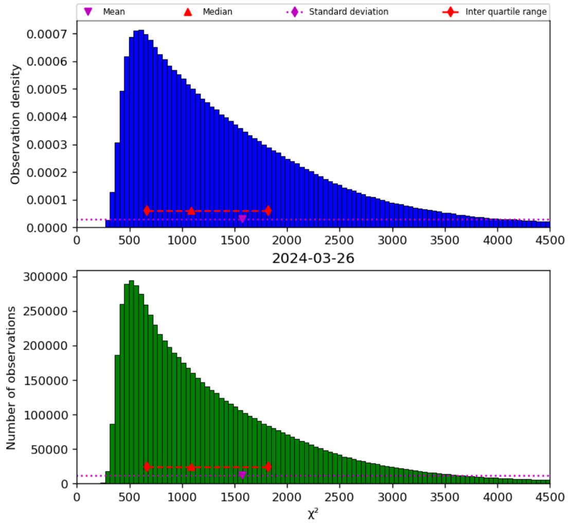
Figure 22: Histogram of “ \chi^2 ” for 2024-03-25 to 2024-03-27
