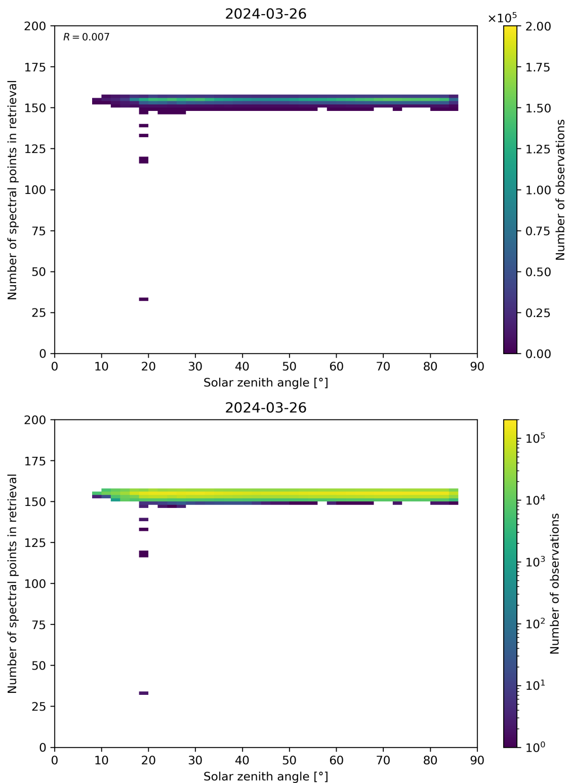
Figure 68: Scatter density plot of “Solar zenith angle” against “Number of spectral points in retrieval” for 2024-03-25 to 2024-03-27.
