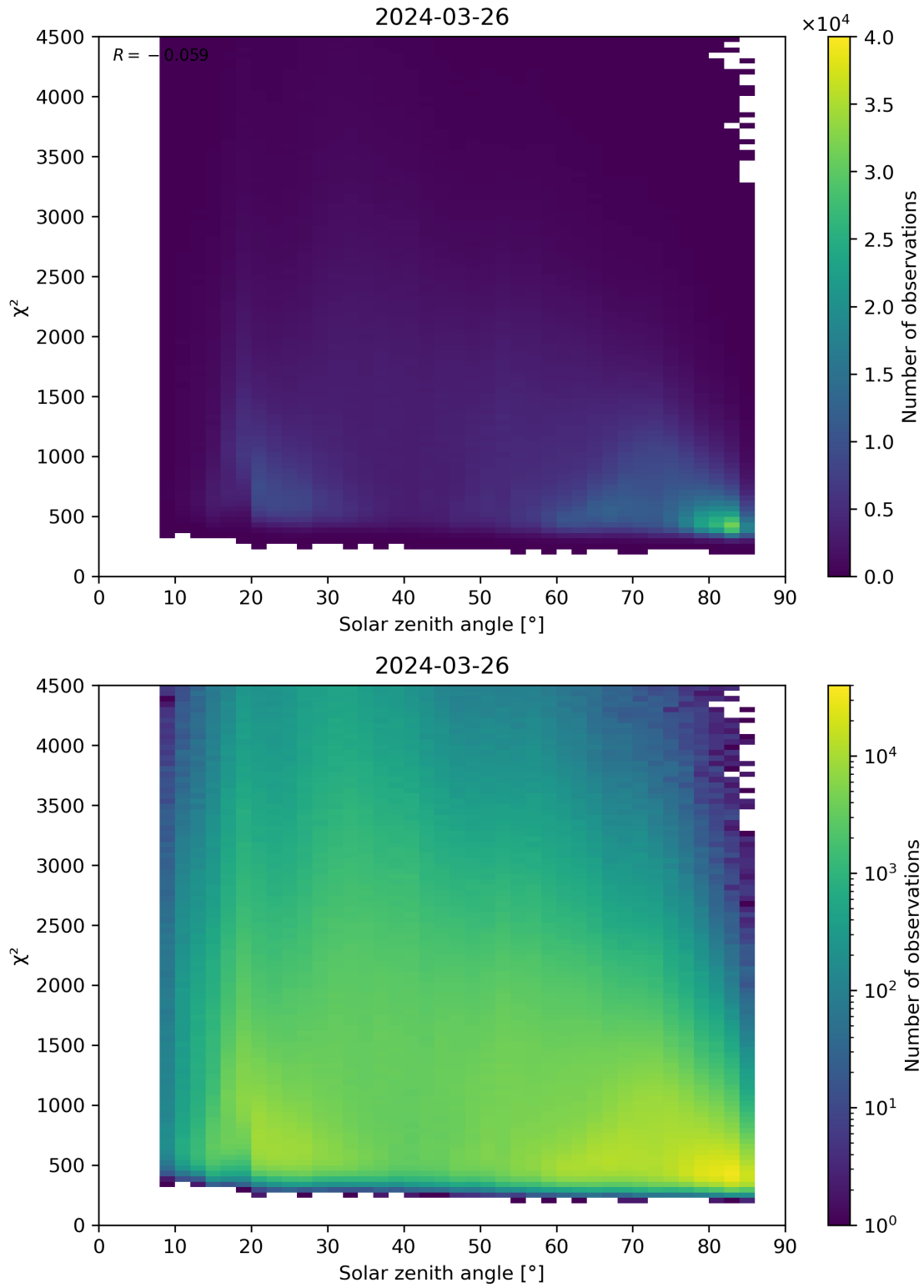
Figure 64: Scatter density plot of “Solar zenith angle” against “ \chi^2 ” for 2024-03-25 to 2024-03-27.
