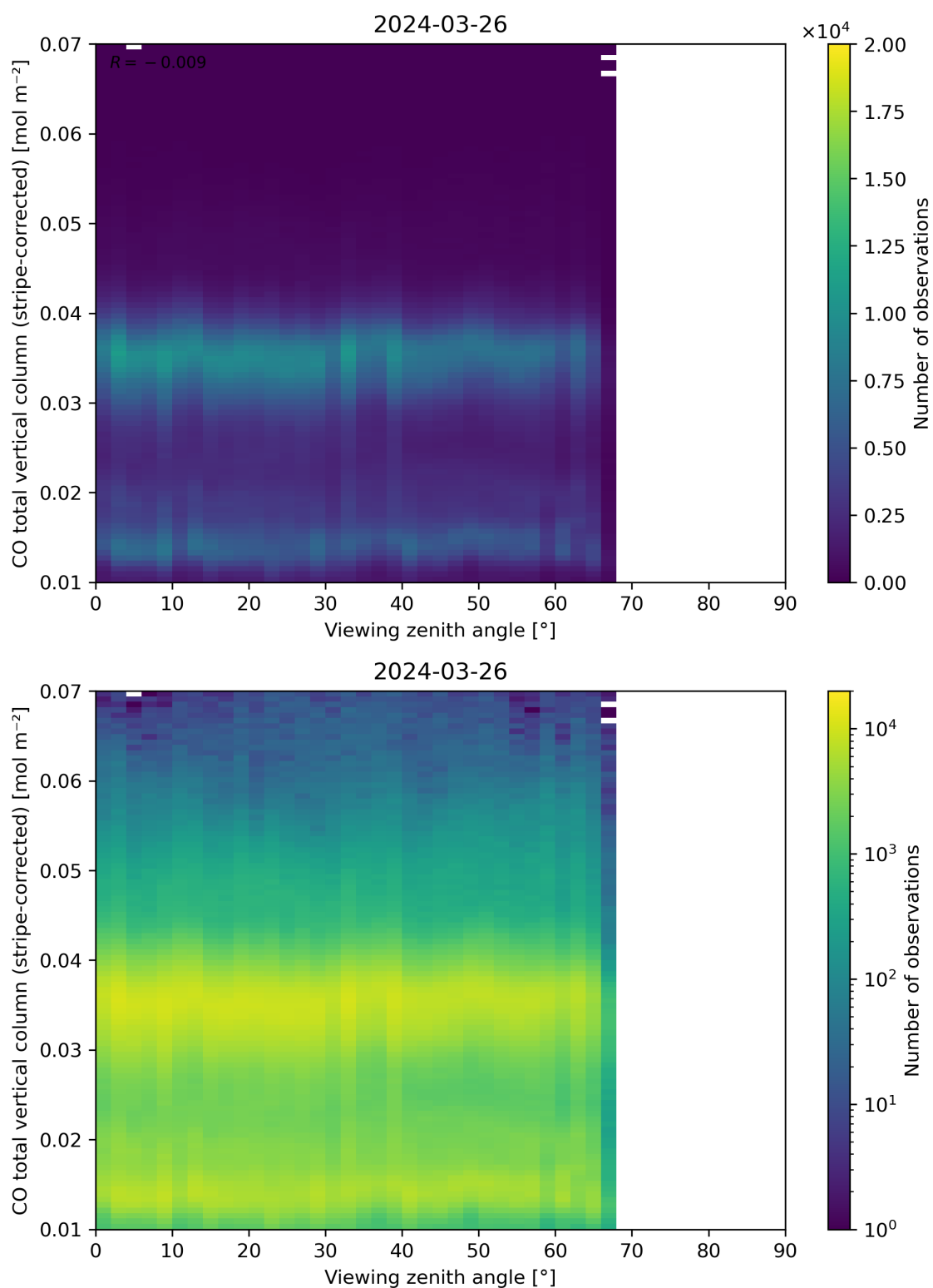
Figure 70: Scatter density plot of “Viewing zenith angle” against “CO total vertical column (stripe-corrected)” for 2024-03-25 to 2024-03-27.
