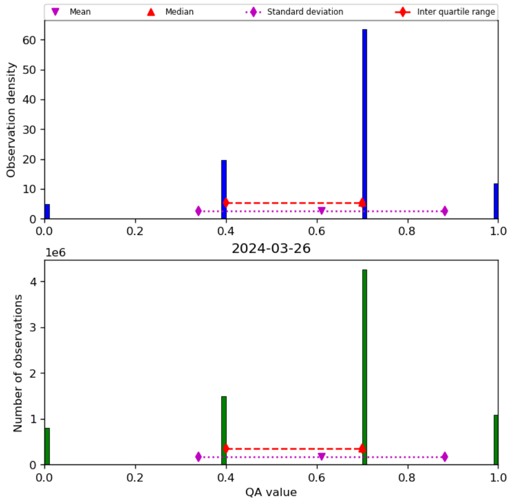
Figure 17: Histogram of “QA value” for 2024-03-25 to 2024-03-27
