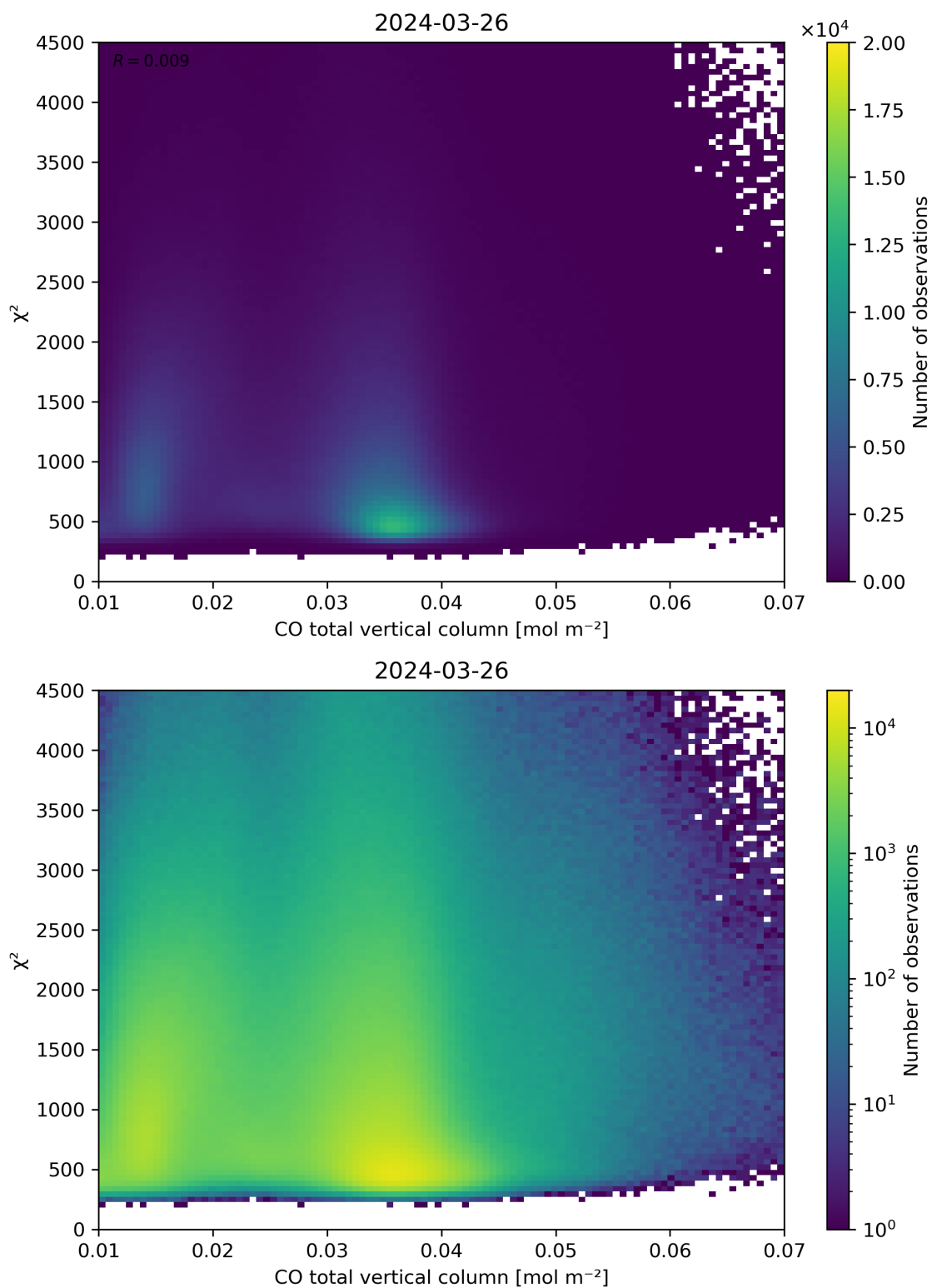
Figure 35: Scatter density plot of “CO total vertical column” against “ \chi^2 ” for 2024-03-25 to 2024-03-27.
