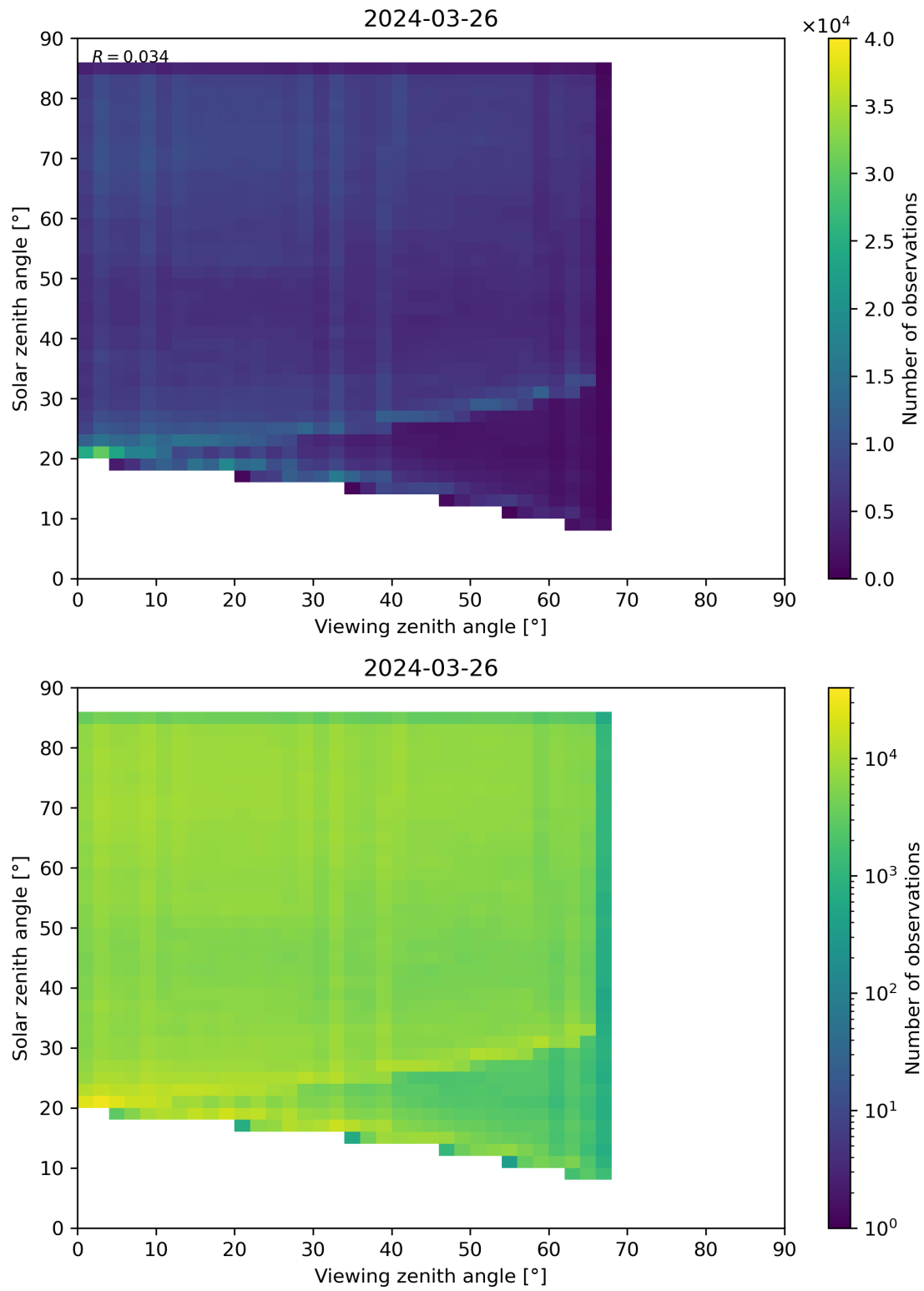
Figure 77: Scatter density plot of “Viewing zenith angle” against “Solar zenith angle” for 2024-03-25 to 2024-03-27.
