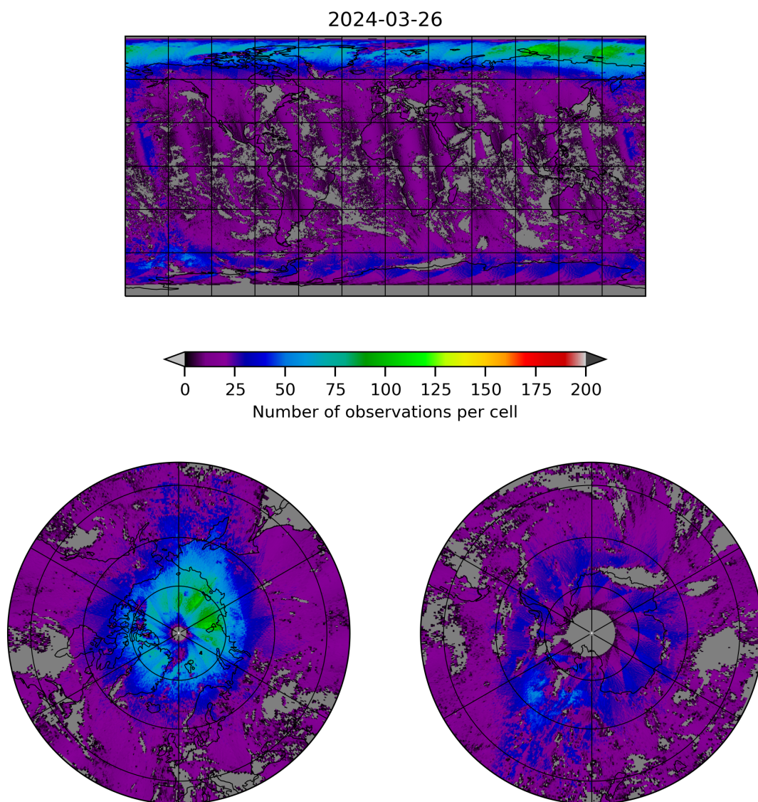
Figure 8: Map of the number of observations for 2024-03-25 to 2024-03-27
