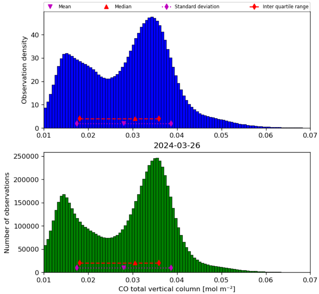
Figure 18: Histogram of “CO total vertical column” for 2024-03-25 to 2024-03-27
