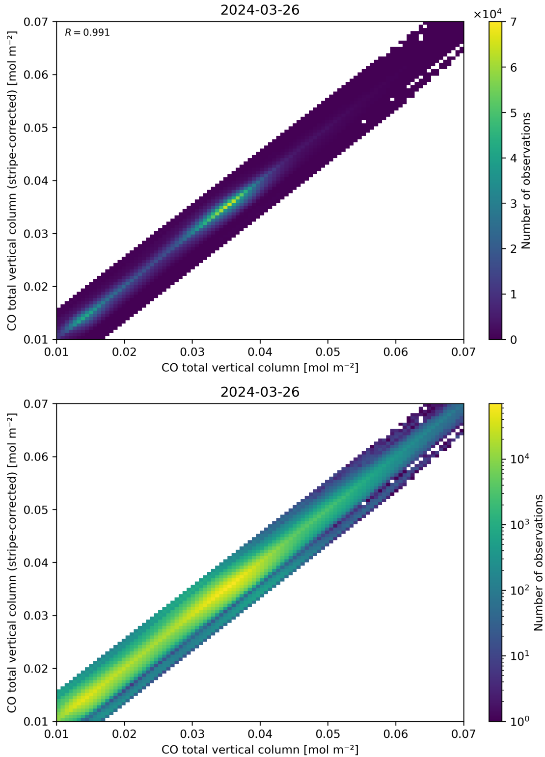
Figure 33: Scatter density plot of “CO total vertical column” against “CO total vertical column (stripe-corrected)” for 2024-03-25 to 2024-03-27.
