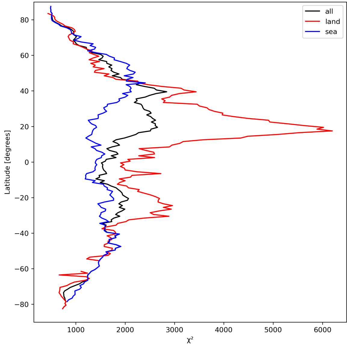
Figure 14: Zonal average of “ \chi^2 ” for 2024-03-25 to 2024-03-27.
