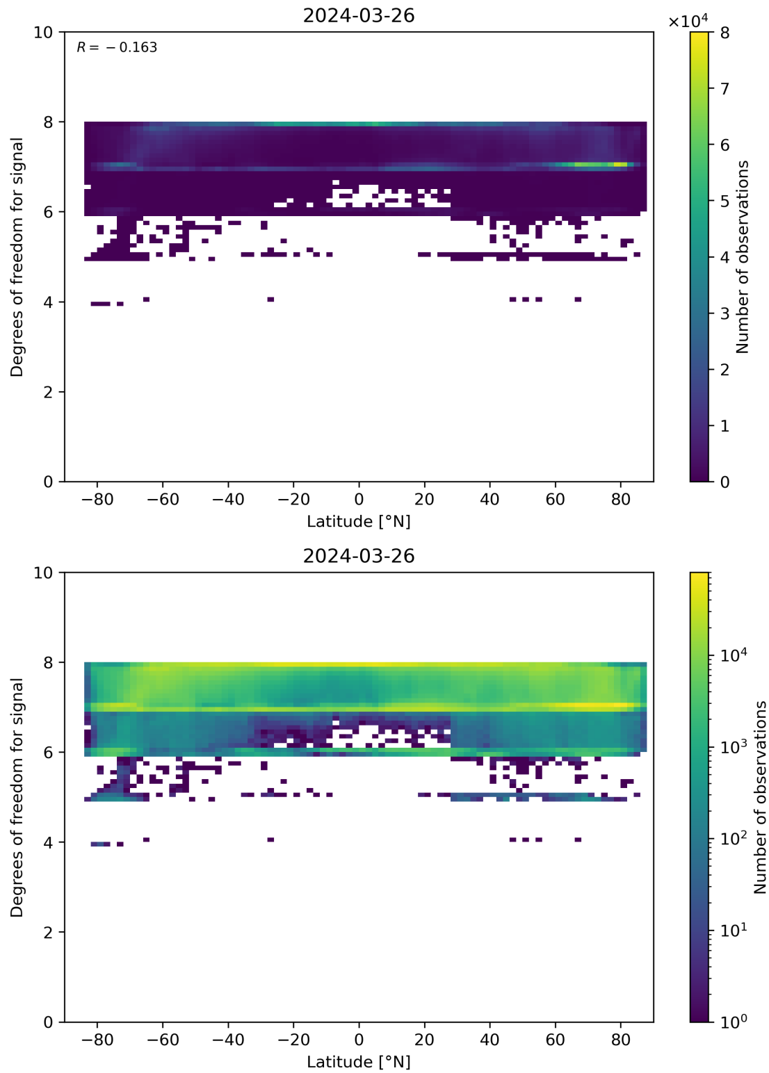
Figure 55: Scatter density plot of “Latitude” against “Degrees of freedom for signal” for 2024-03-25 to 2024-03-27.
