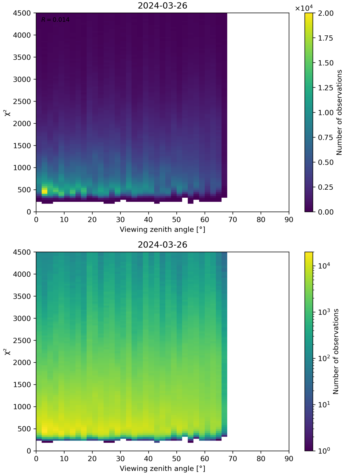
Figure 72: Scatter density plot of “Viewing zenith angle” against “ \chi^2 ” for 2024-03-25 to 2024-03-27.
