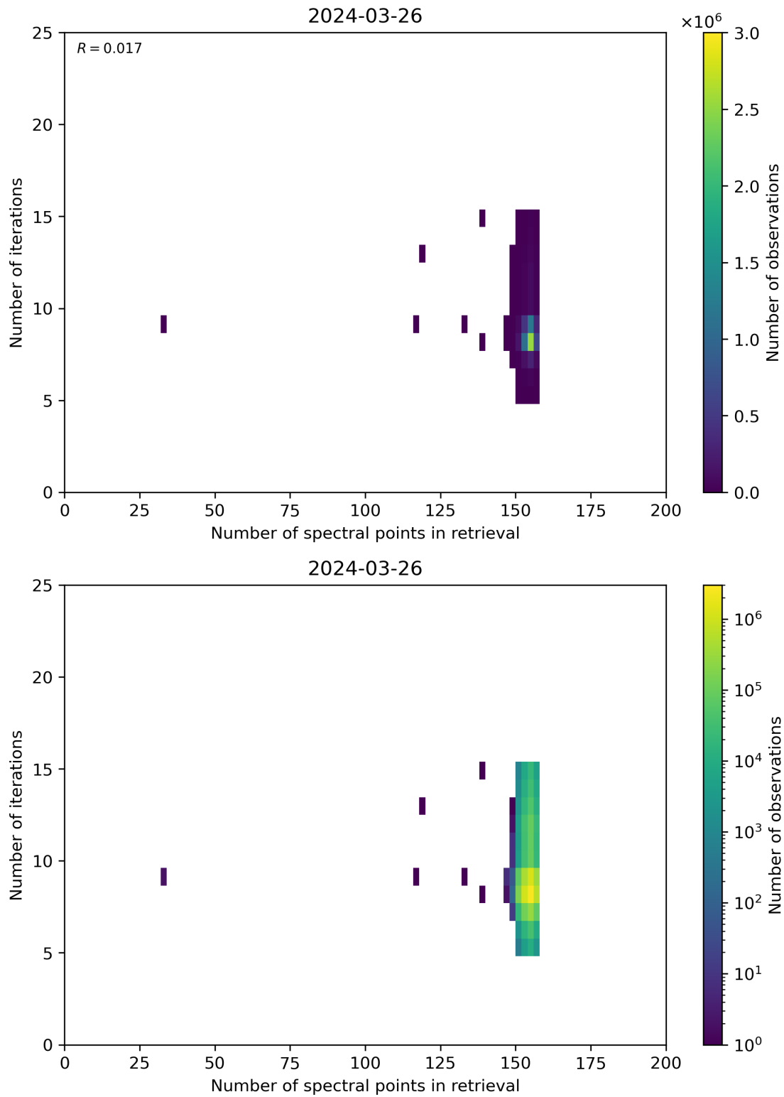
Figure 60: Scatter density plot of “Number of spectral points in retrieval” against “Number of iterations” for 2024-03-25 to 2024-03-27.
