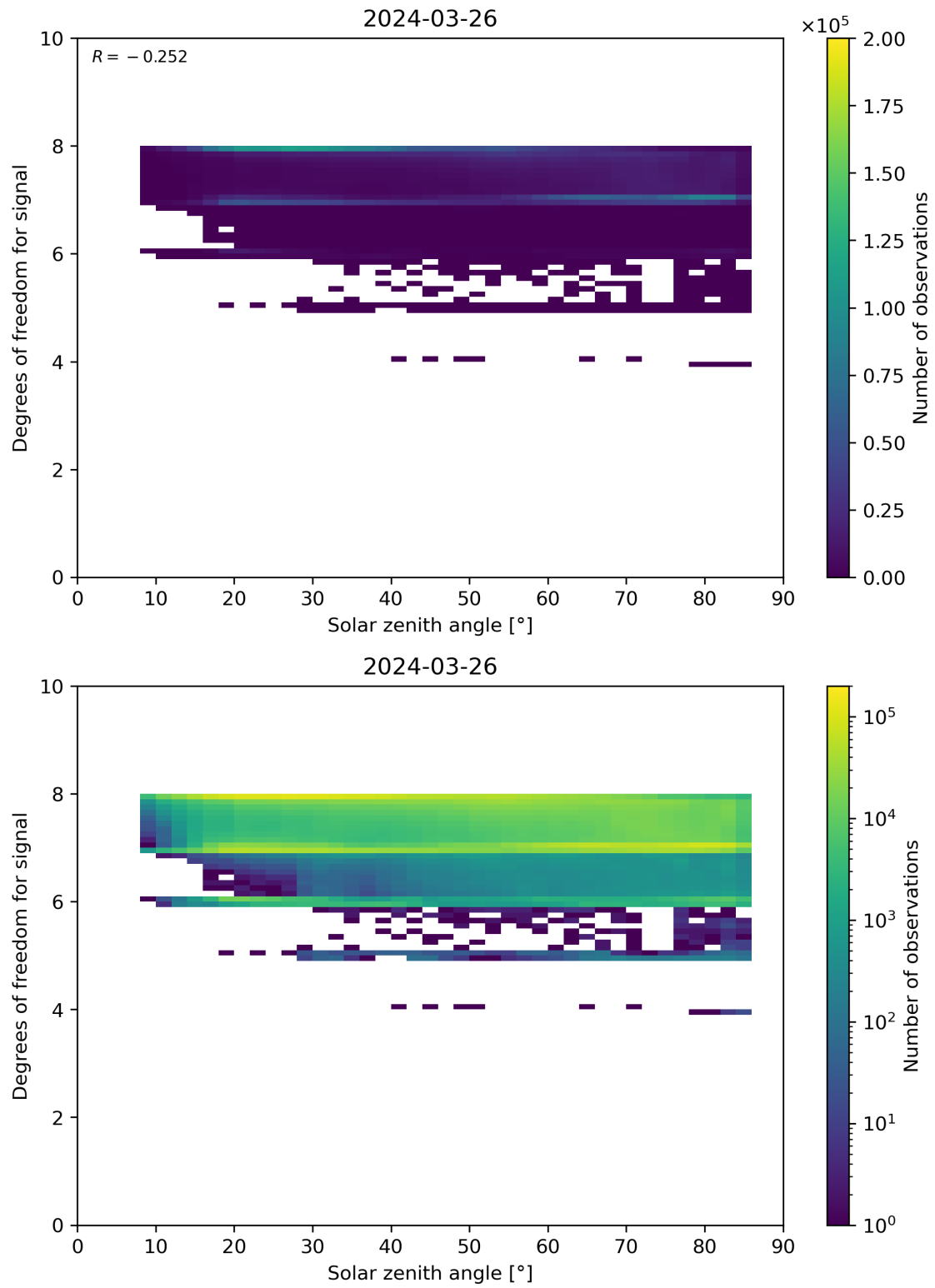
Figure 65: Scatter density plot of “Solar zenith angle” against “Degrees of freedom for signal” for 2024-03-25 to 2024-03-27.
