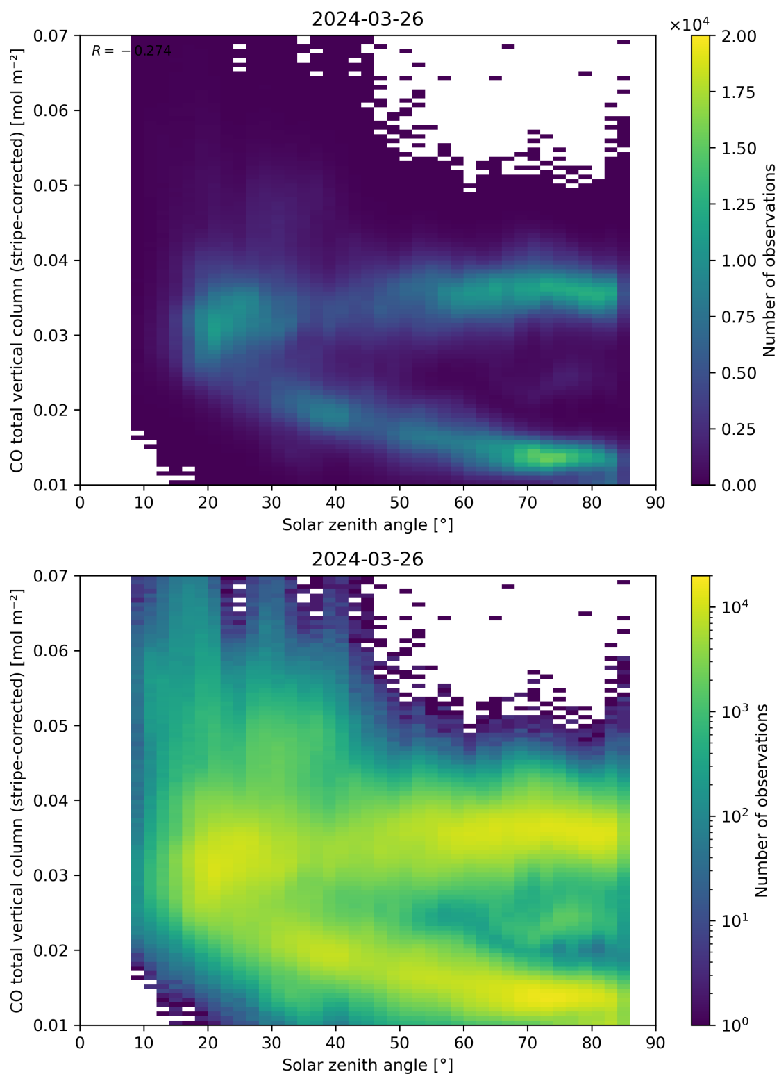
Figure 62: Scatter density plot of “Solar zenith angle” against “CO total vertical column (stripe-corrected)” for 2024-03-25 to 2024-03-27.
