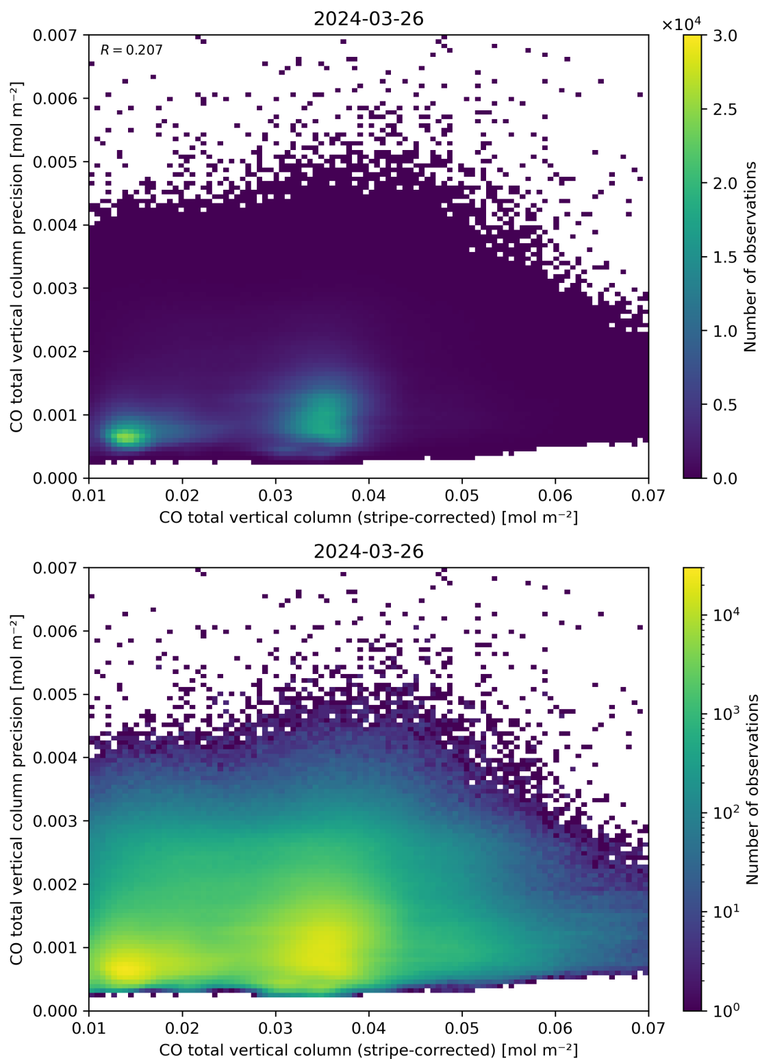
Figure 36: Scatter density plot of “CO total vertical column (stripe-corrected)” against “CO total vertical column precision” for 2024-03-25 to 2024-03-27.
