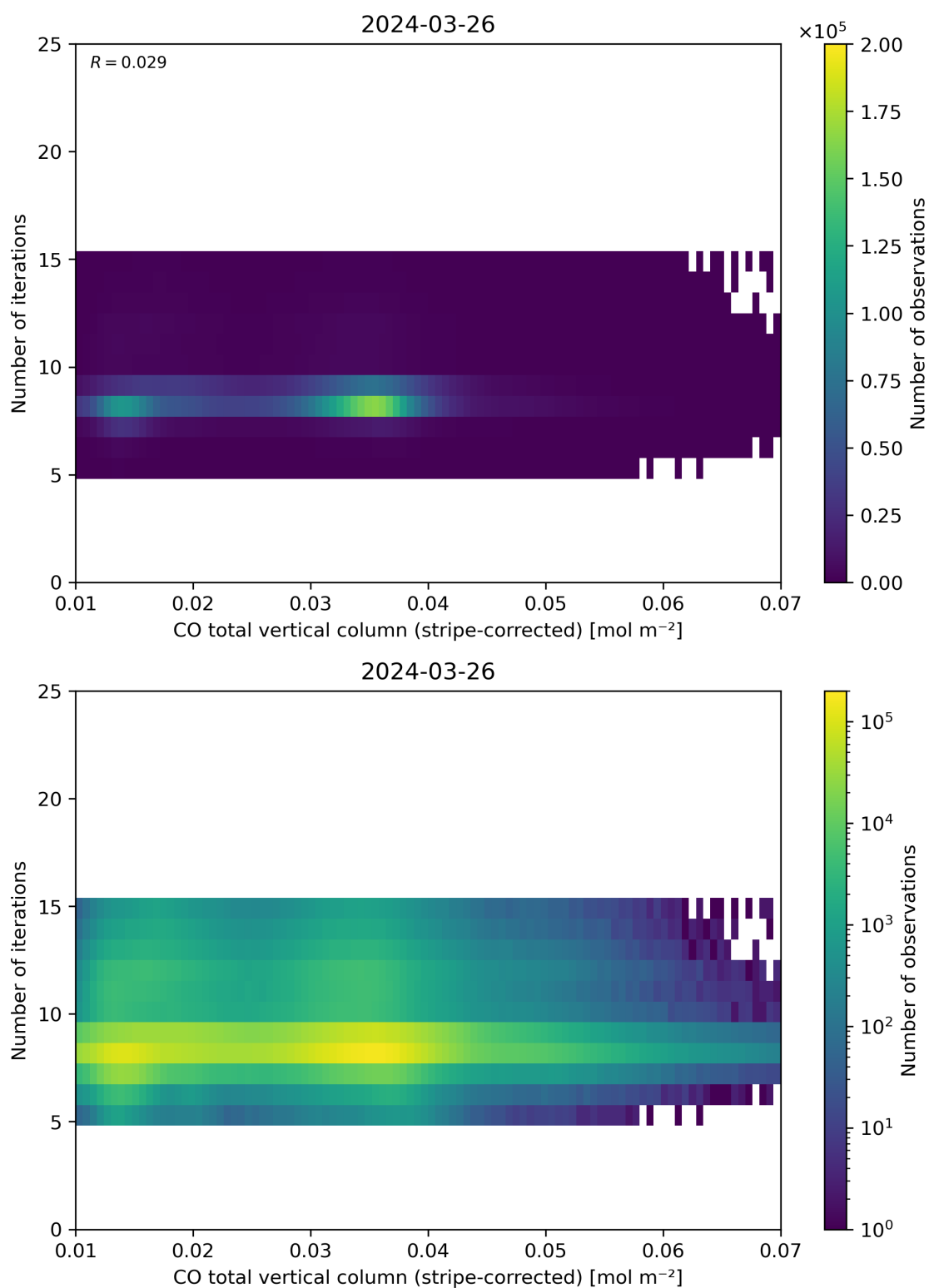
Figure 39: Scatter density plot of “CO total vertical column (stripe-corrected)” against “Number of iterations” for 2024-03-25 to 2024-03-27.
