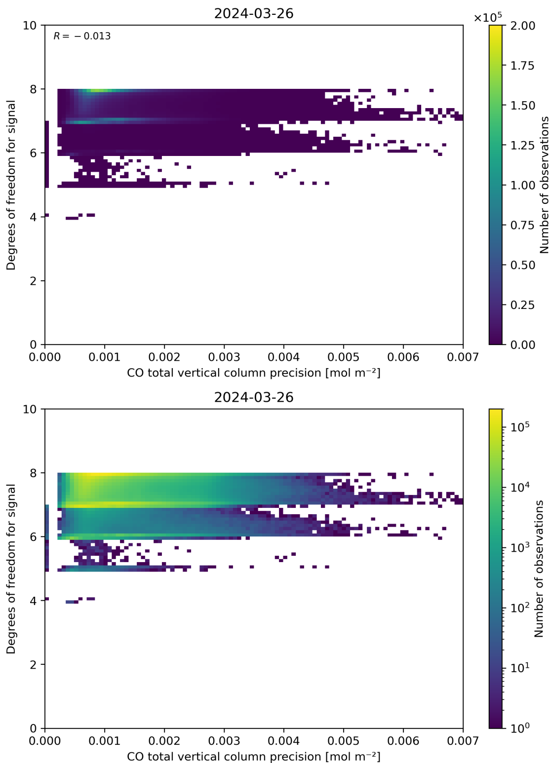
Figure 45: Scatter density plot of “CO total vertical column precision” against “Degrees of freedom for signal” for 2024-03-25 to 2024-03-27.
