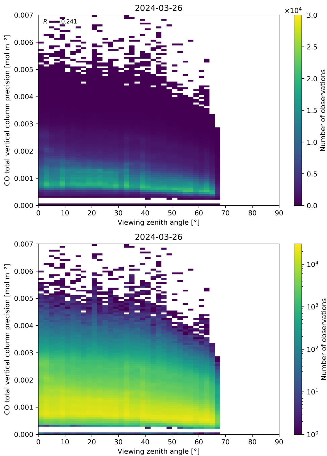
Figure 71: Scatter density plot of “Viewing zenith angle” against “CO total vertical column precision” for 2024-03-25 to 2024-03-27.
