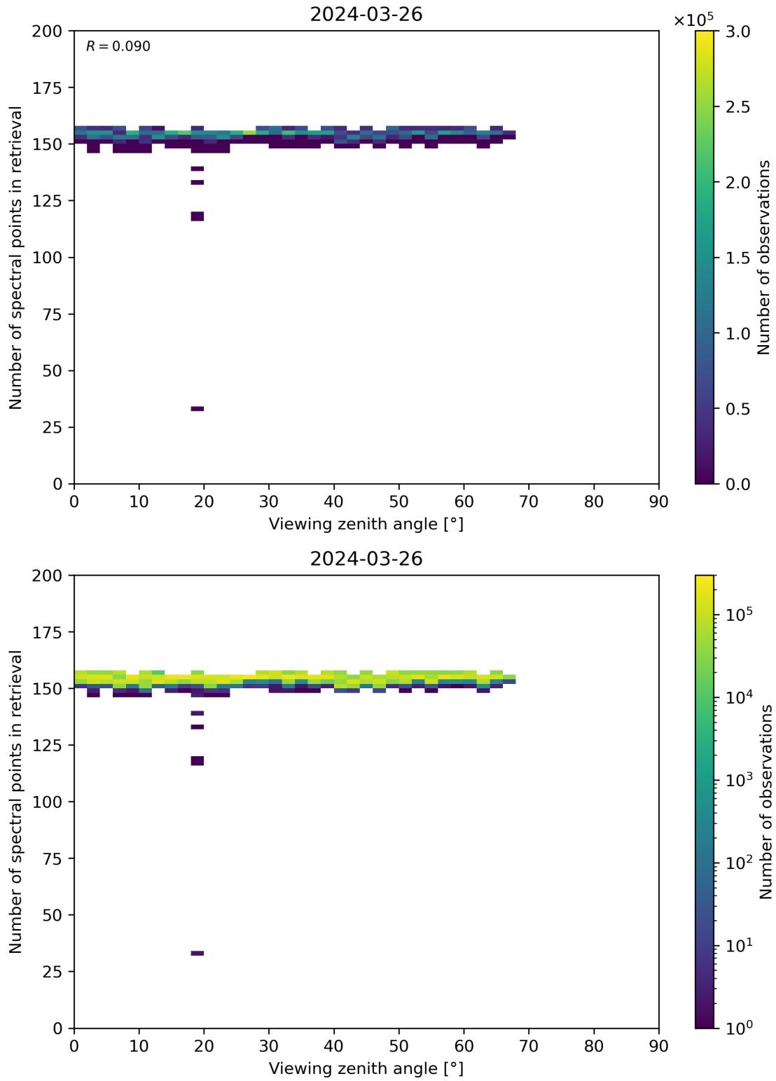
Figure 76: Scatter density plot of “Viewing zenith angle” against “Number of spectral points in retrieval” for 2024-03-25 to 2024-03-27.
