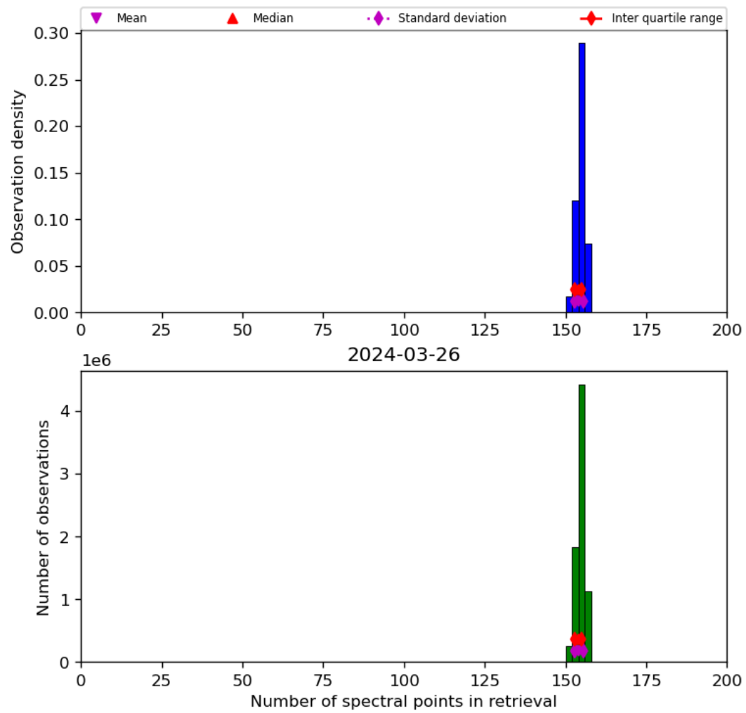
Figure 21: Histogram of “Number of spectral points in retrieval” for 2024-03-25 to 2024-03-27
