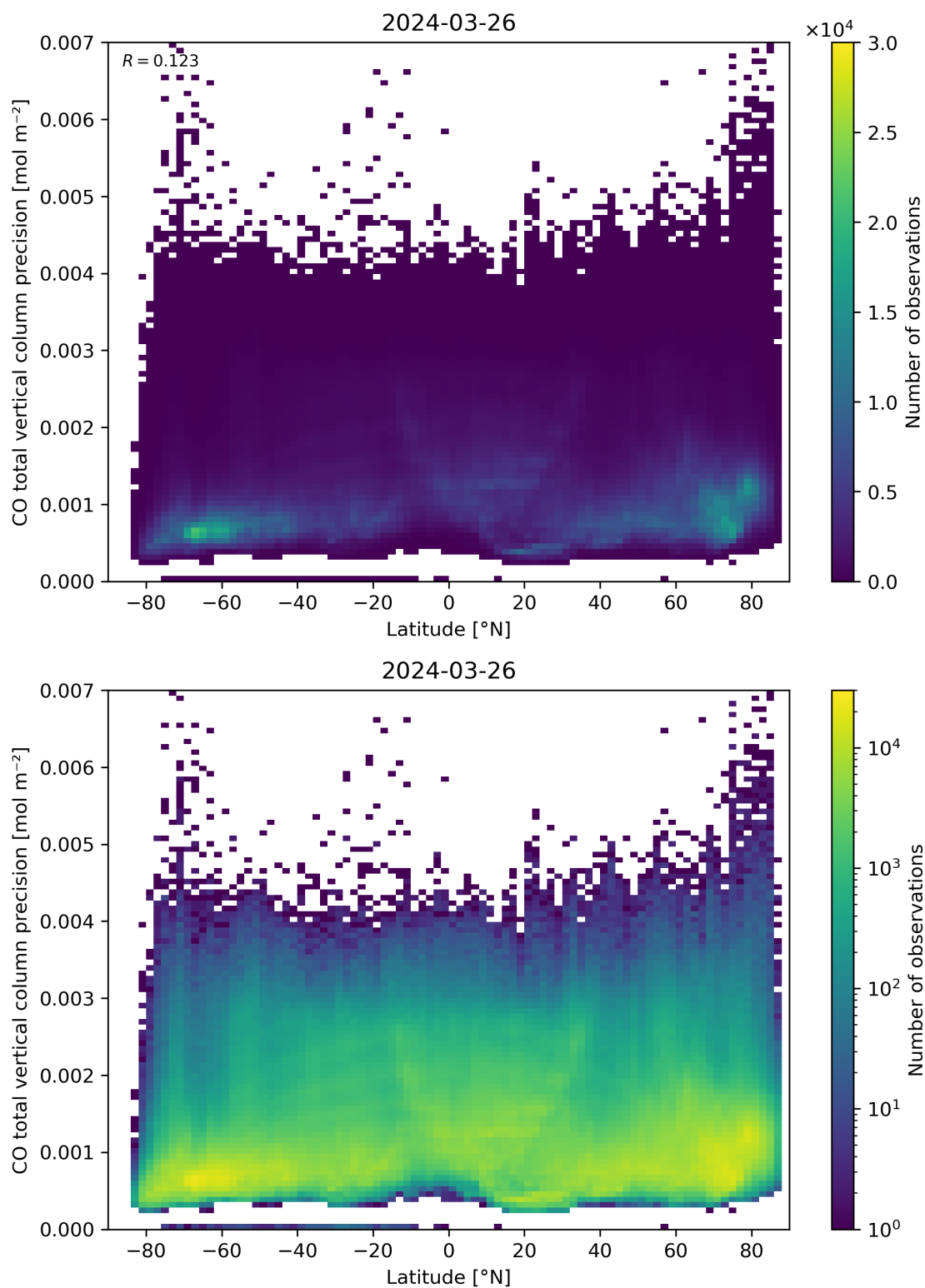
Figure 53: Scatter density plot of “Latitude” against “CO total vertical column precision” for 2024-03-25 to 2024-03-27.
