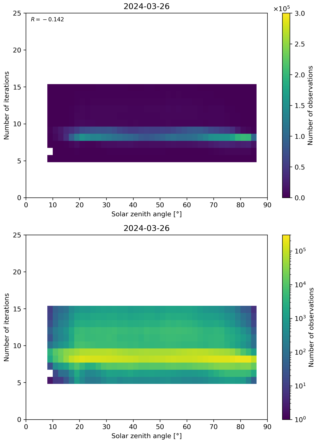
Figure 67: Scatter density plot of “Solar zenith angle” against “Number of iterations” for 2024-03-25 to 2024-03-27.
