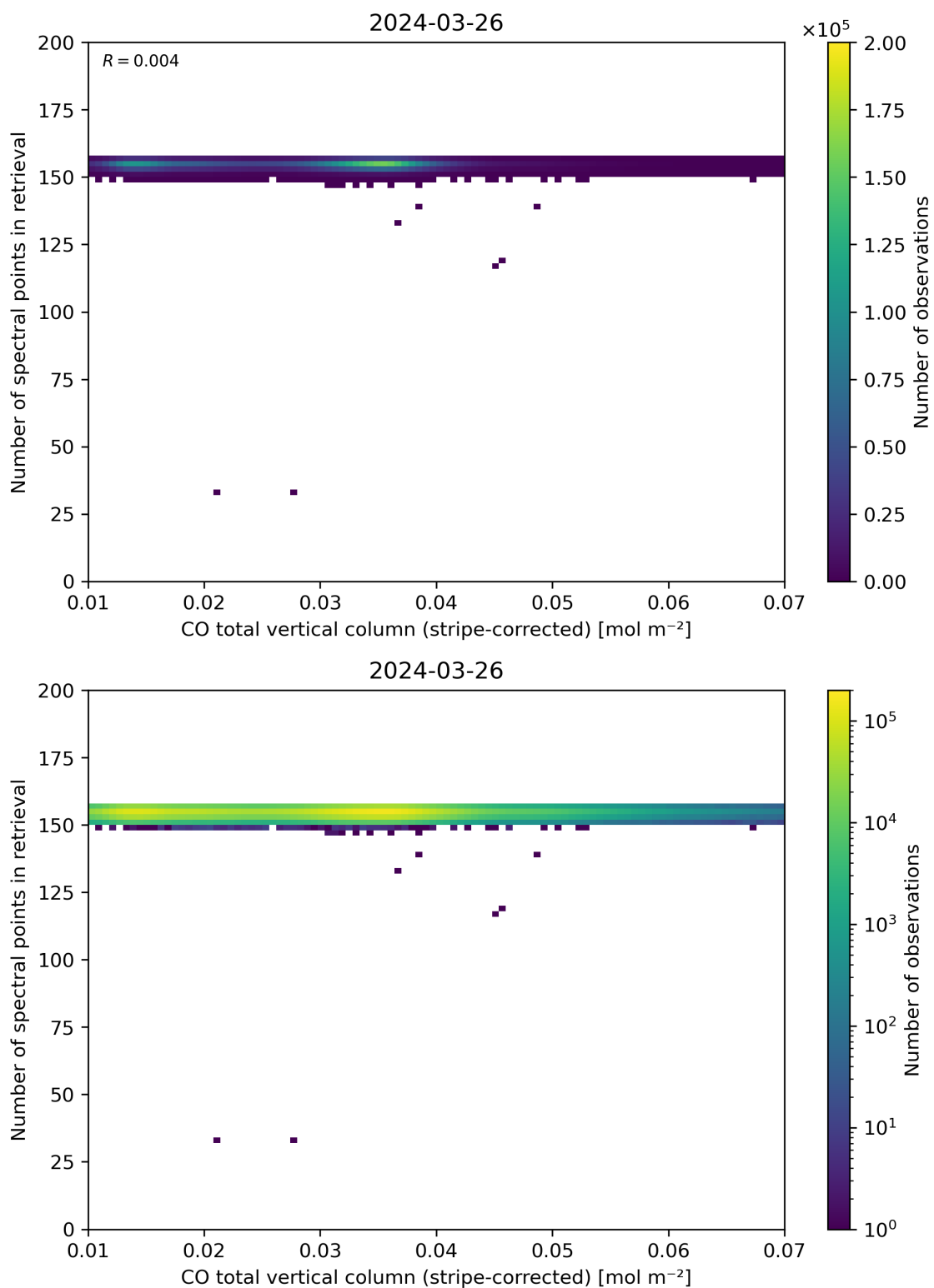
Figure 40: Scatter density plot of “CO total vertical column (stripe-corrected)” against “Number of spectral points in retrieval” for 2024-03-25 to 2024-03-27.
