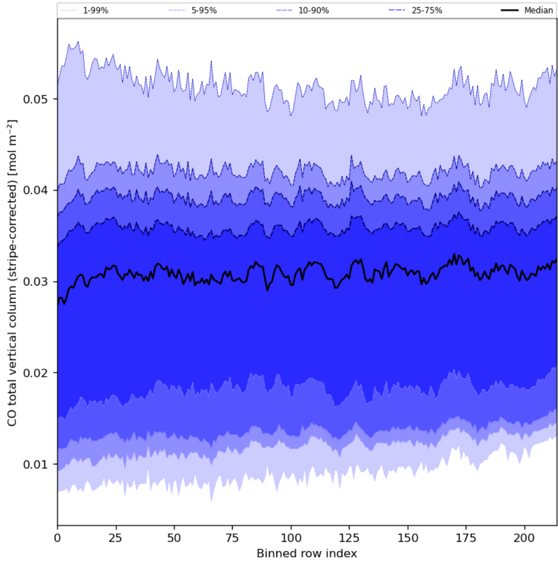
Figure 27: Along track statistics of “CO total vertical column (stripe-corrected)” for 2024-03-25 to 2024-03-27
