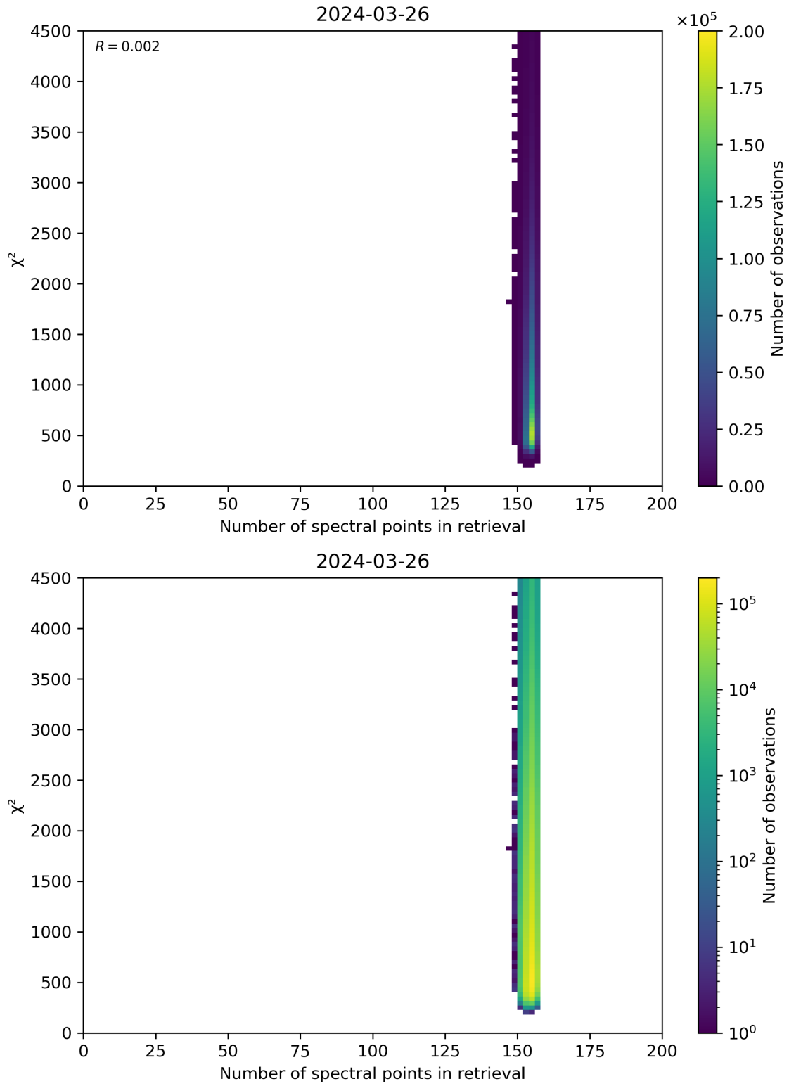
Figure 58: Scatter density plot of “Number of spectral points in retrieval” against “ \chi^2 ” for 2024-03-25 to 2024-03-27.
