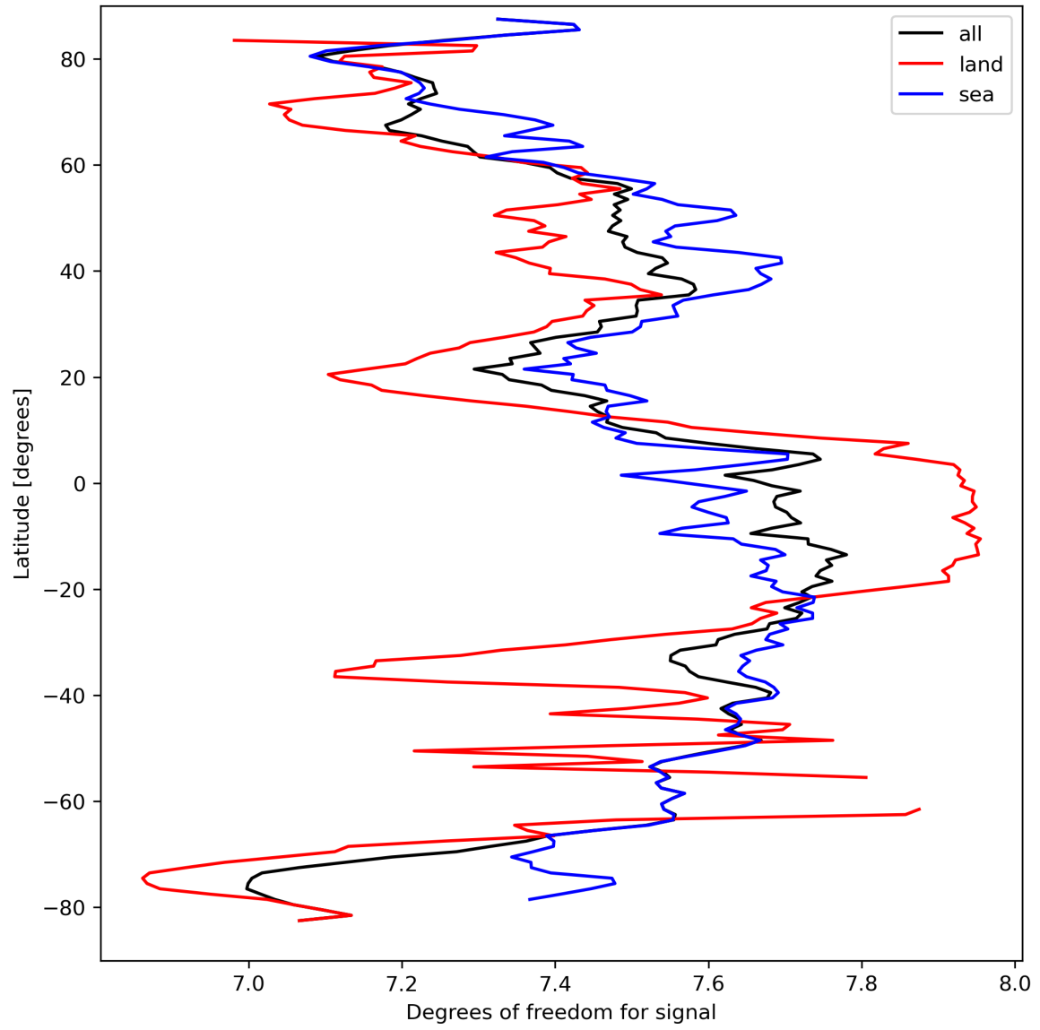
Figure 15: Zonal average of “Degrees of freedom for signal” for 2024-03-25 to 2024-03-27.
