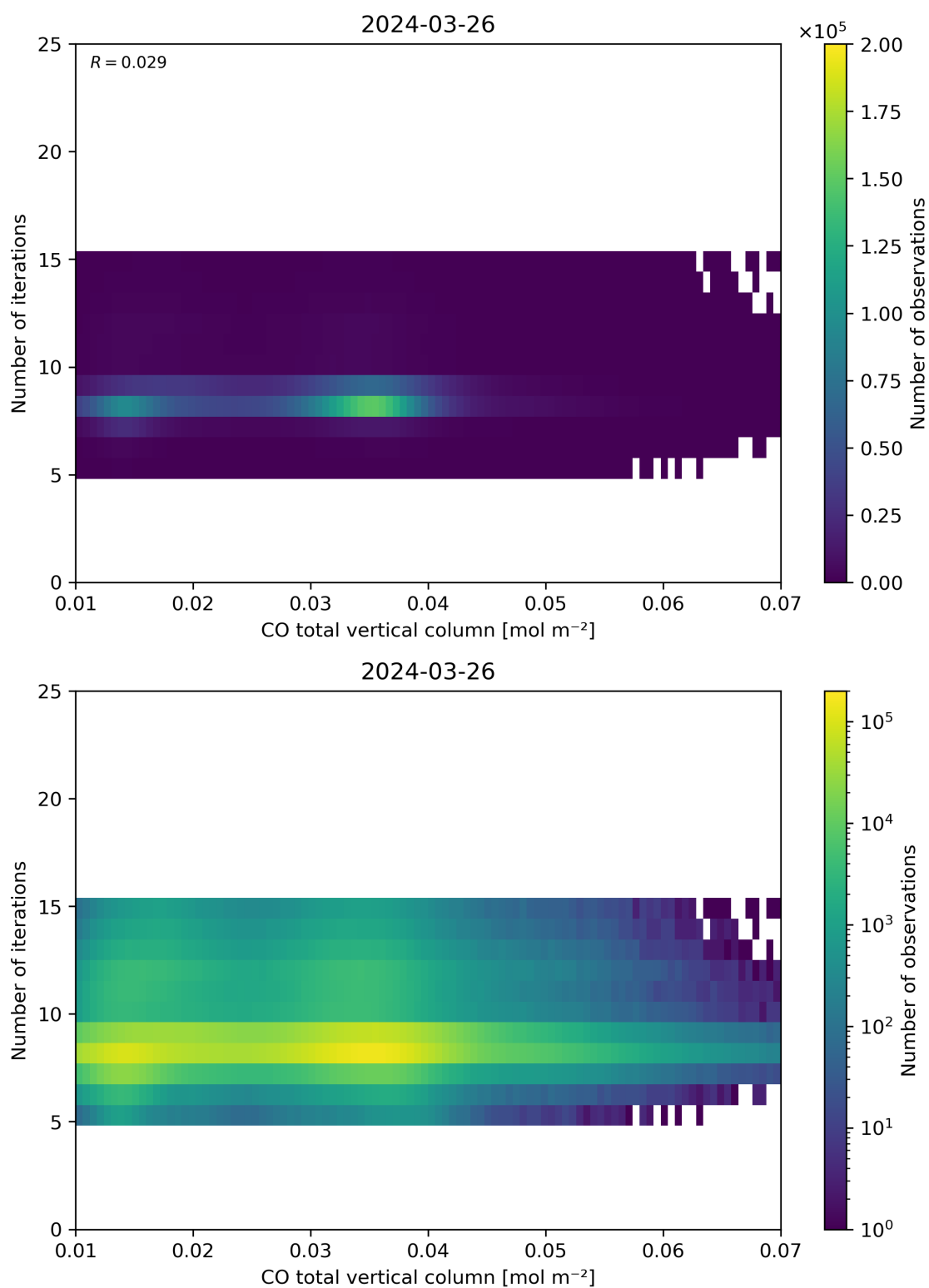
Figure 42: Scatter density plot of “CO total vertical column” against “Number of iterations” for 2024-03-25 to 2024-03-27.
