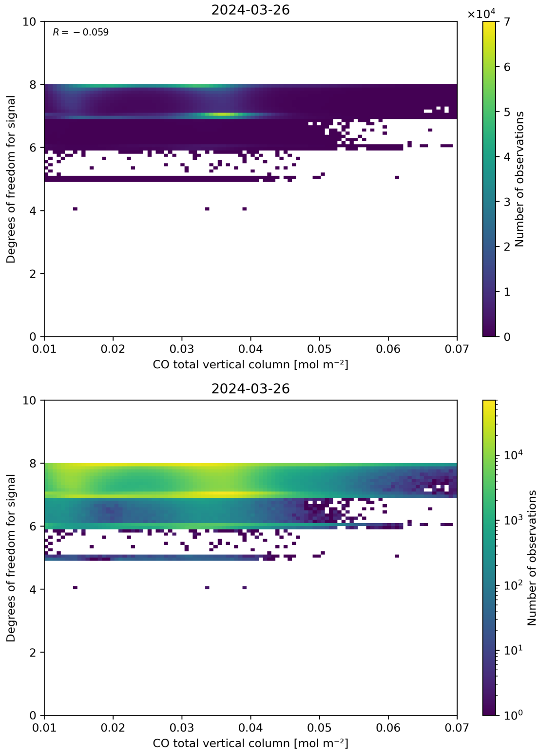
Figure 41: Scatter density plot of “CO total vertical column” against “Degrees of freedom for signal” for 2024-03-25 to 2024-03-27.
