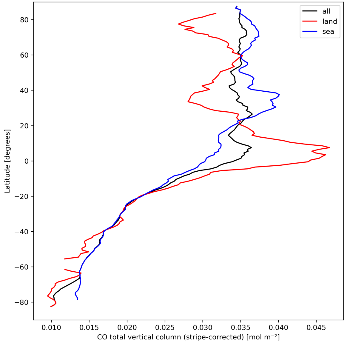
Figure 11: Zonal average of “CO total vertical column (stripe-corrected)” for 2024-03-25 to 2024-03-27.
