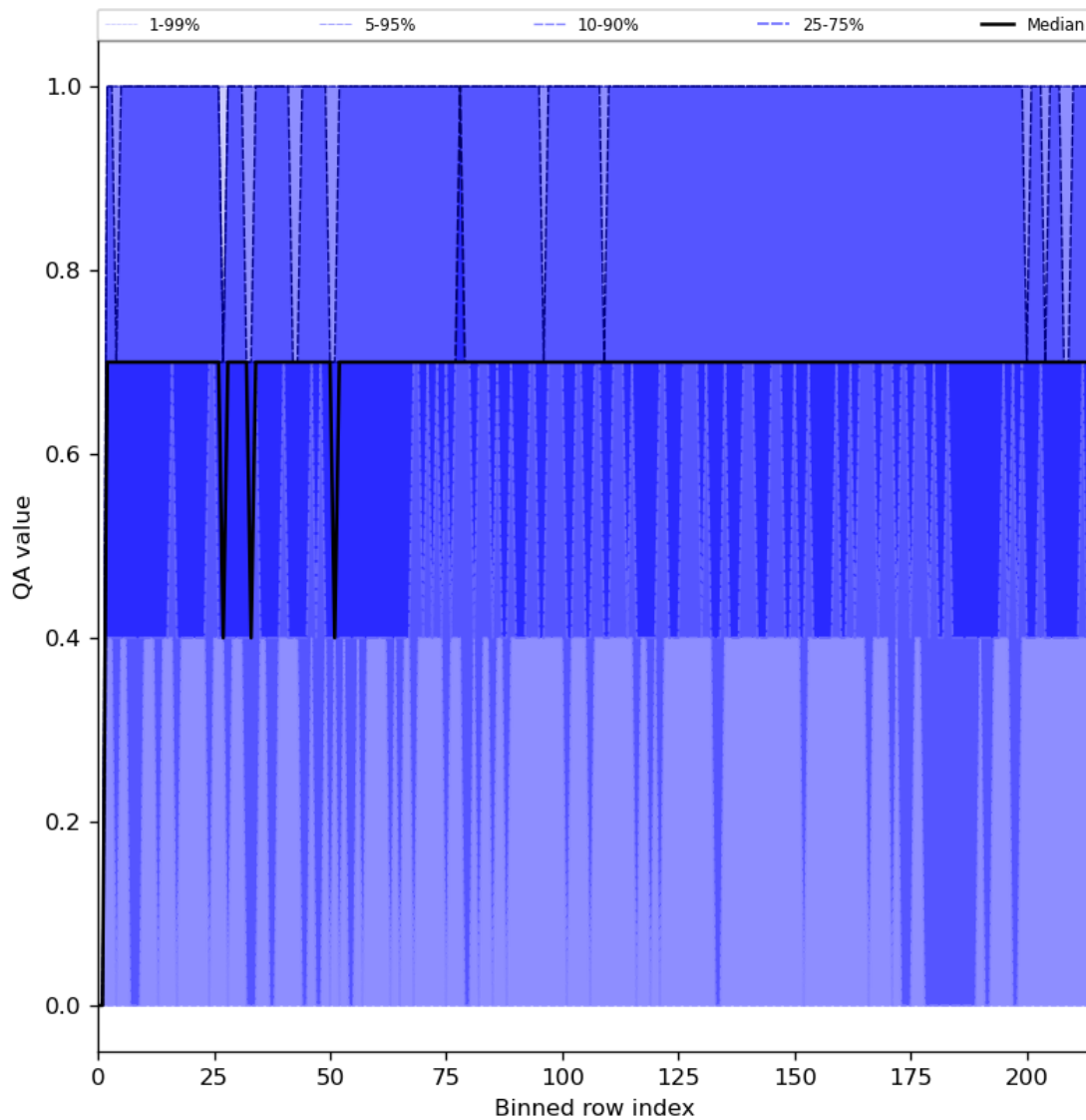
Figure 25: Along track statistics of “QA value” for 2024-03-25 to 2024-03-27
