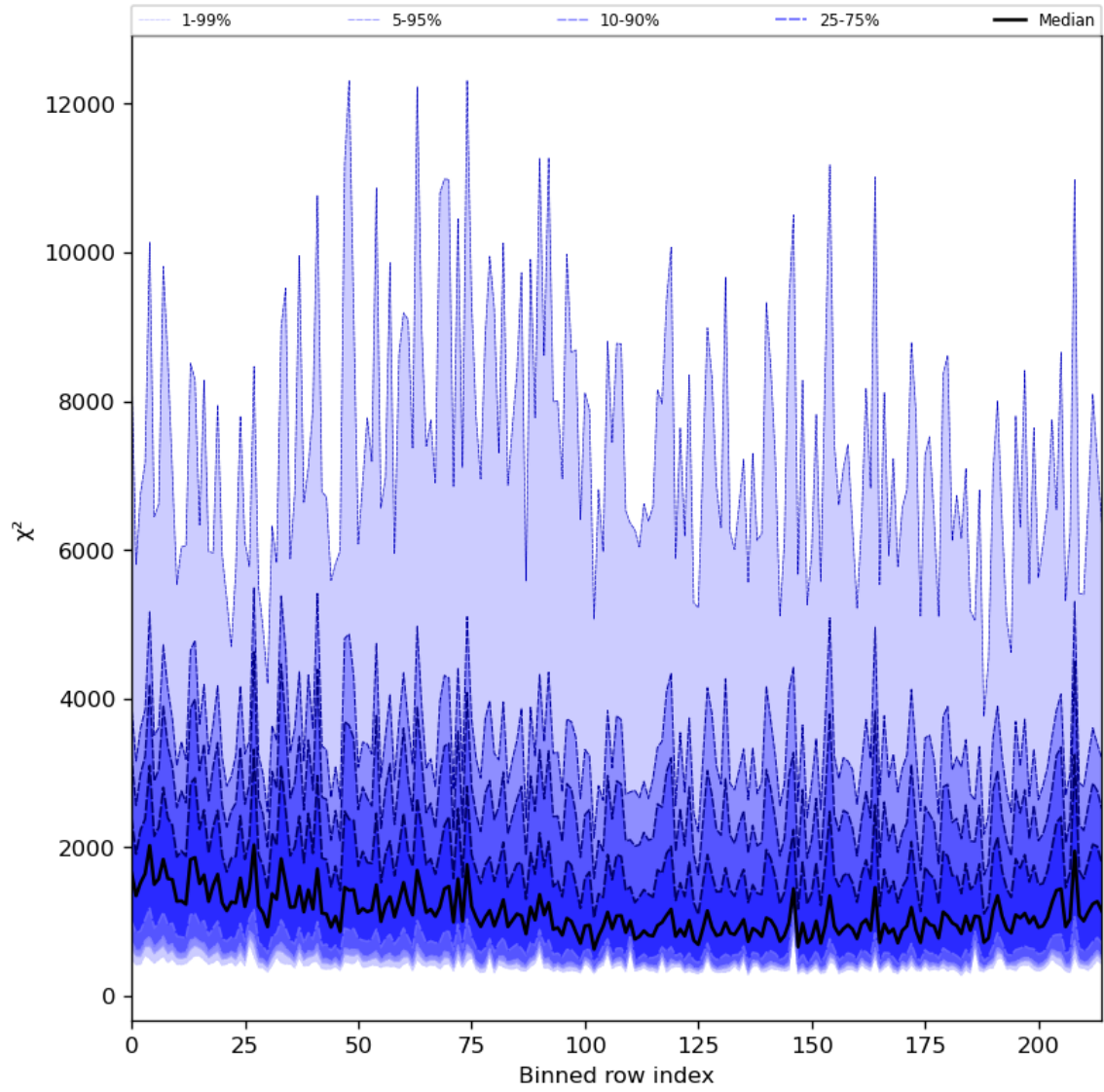
Figure 30: Along track statistics of “ \chi^2 ” for 2024-03-25 to 2024-03-27
