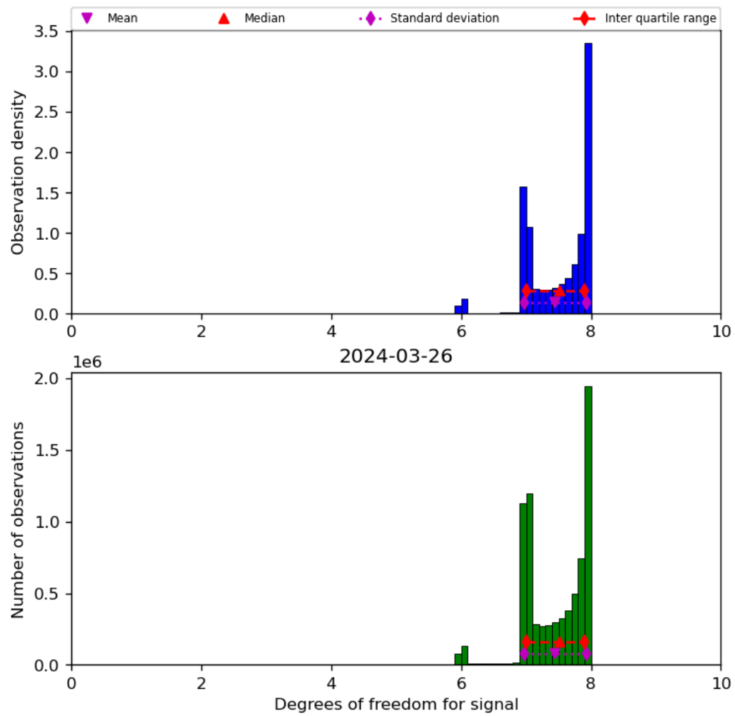
Figure 23: Histogram of “Degrees of freedom for signal” for 2024-03-25 to 2024-03-27
