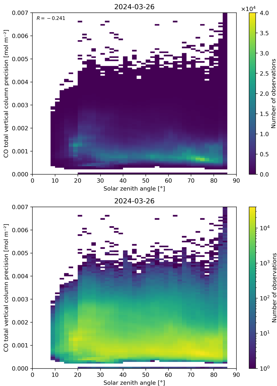
Figure 63: Scatter density plot of “Solar zenith angle” against “CO total vertical column precision” for 2024-03-25 to 2024-03-27.
