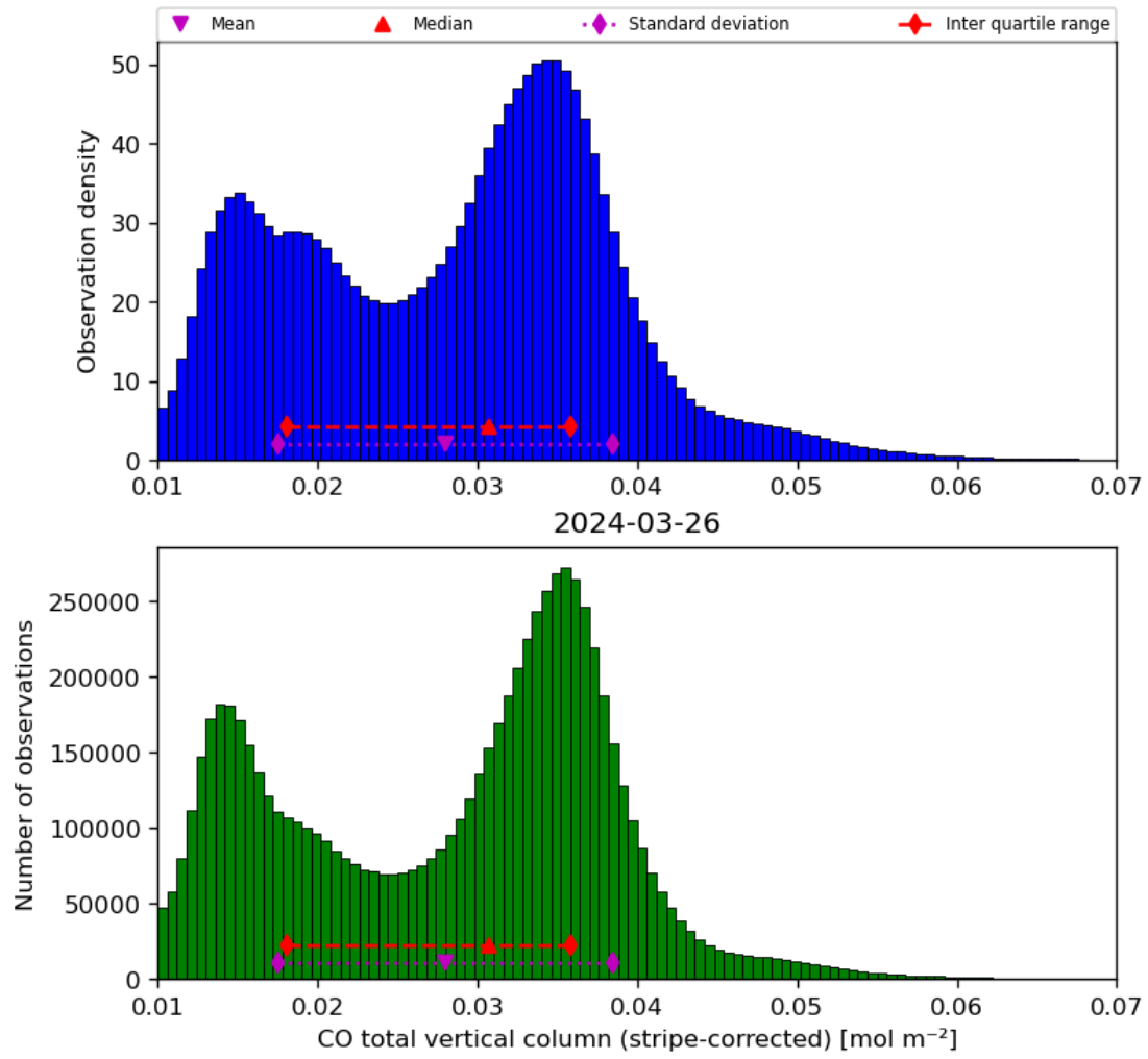
Figure 19: Histogram of “CO total vertical column (stripe-corrected)” for 2024-03-25 to 2024-03-27
