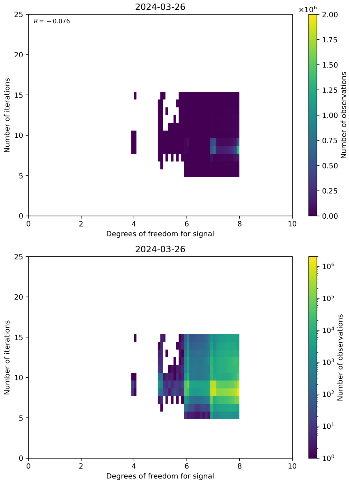
Figure 50: Scatter density plot of “Degrees of freedom for signal” against “Number of iterations” for 2024-03-25 to 2024-03-27.
