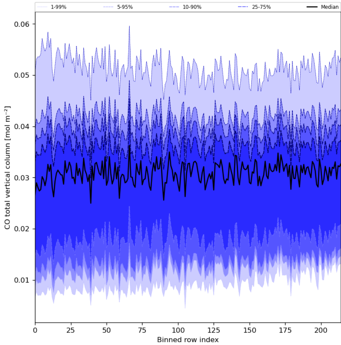
Figure 26: Along track statistics of “CO total vertical column” for 2024-03-25 to 2024-03-27
