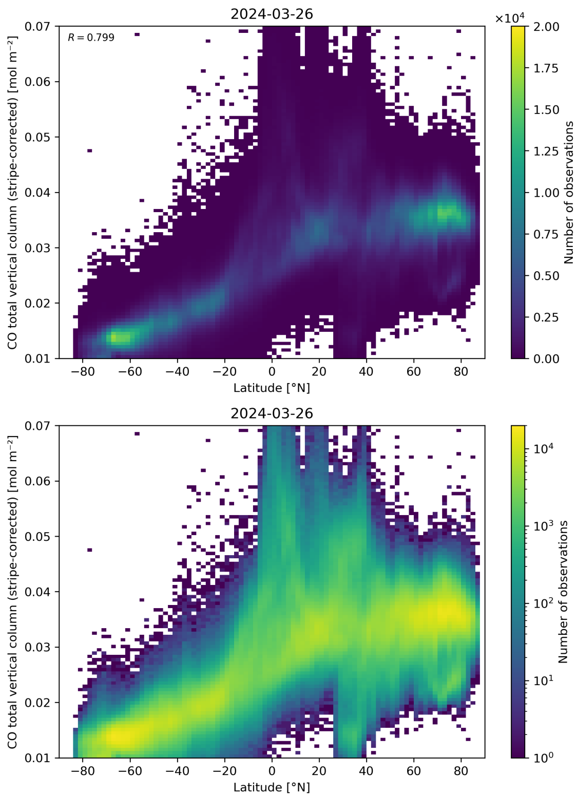
Figure 52: Scatter density plot of “Latitude” against “CO total vertical column (stripe-corrected)” for 2024-03-25 to 2024-03-27.
