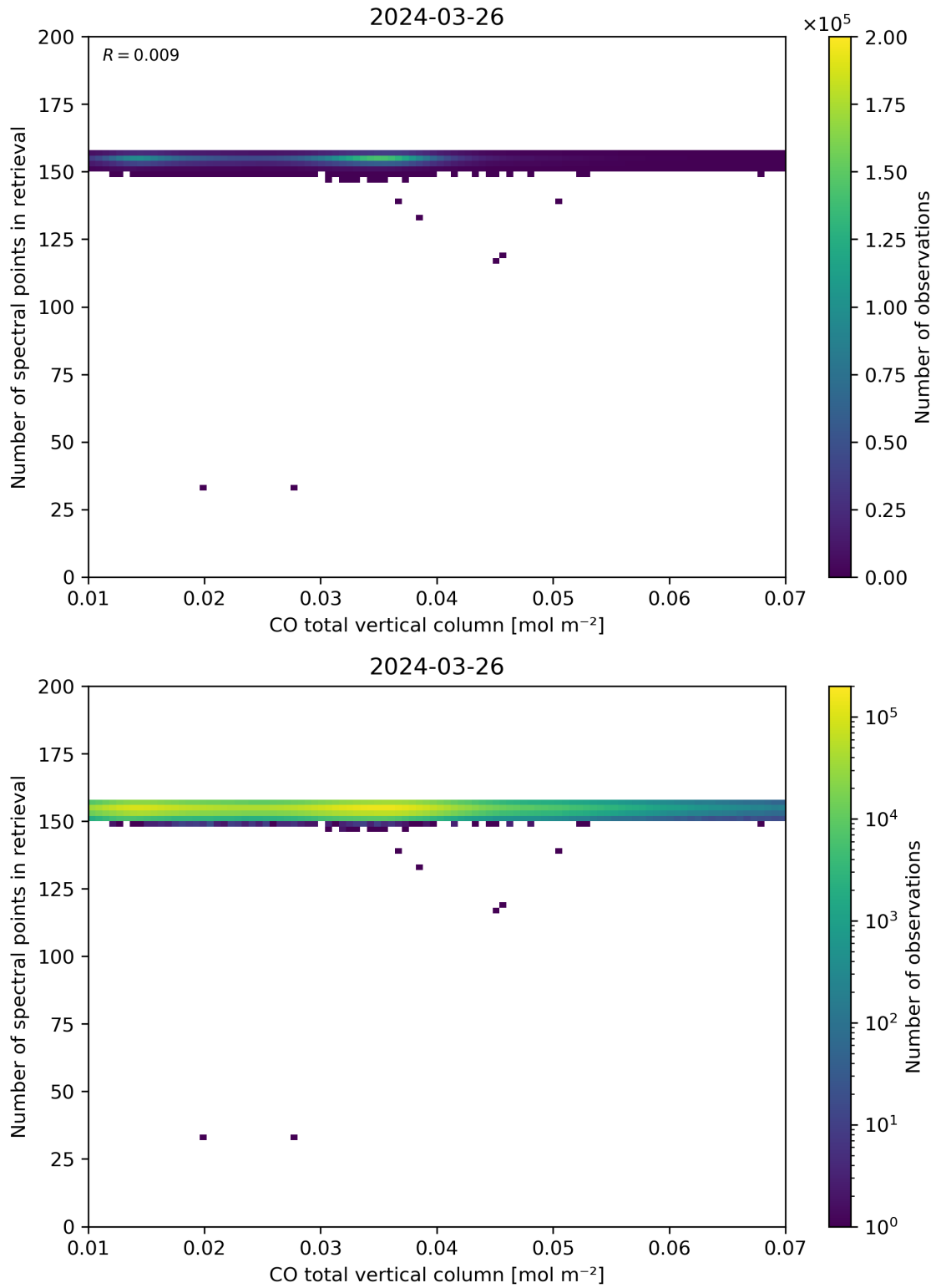
Figure 43: Scatter density plot of “CO total vertical column” against “Number of spectral points in retrieval” for 2024-03-25 to 2024-03-27.
