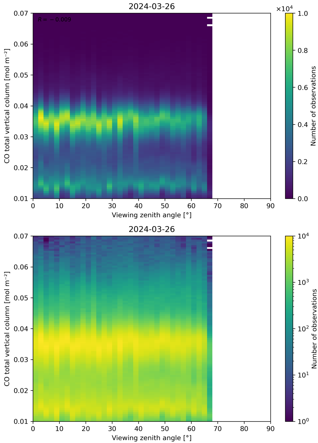
Figure 69: Scatter density plot of “Viewing zenith angle” against “CO total vertical column” for 2024-03-25 to 2024-03-27.
