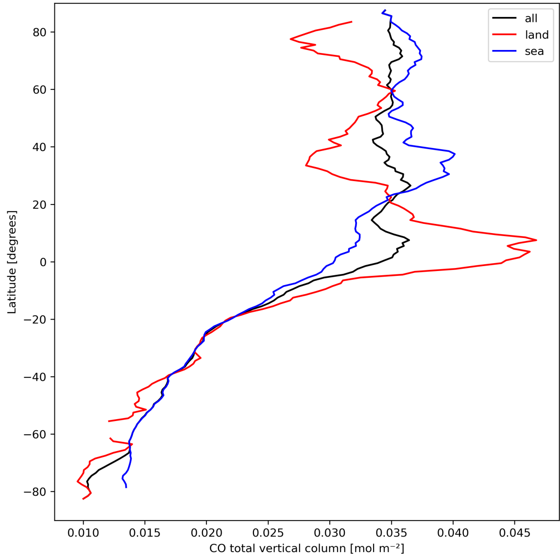
Figure 10: Zonal average of “CO total vertical column” for 2024-03-25 to 2024-03-27.
