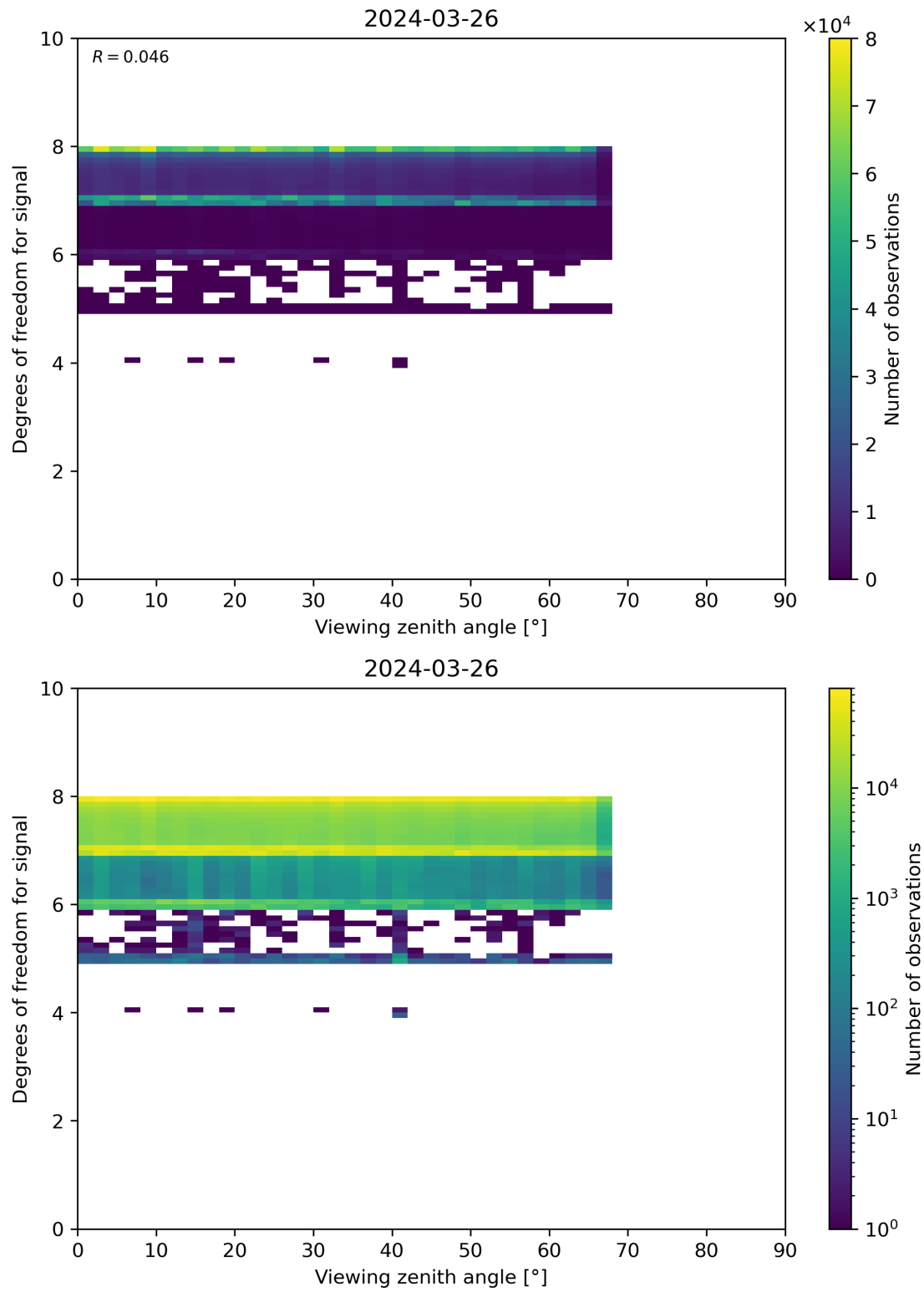
Figure 73: Scatter density plot of “Viewing zenith angle” against “Degrees of freedom for signal” for 2024-03-25 to 2024-03-27.
