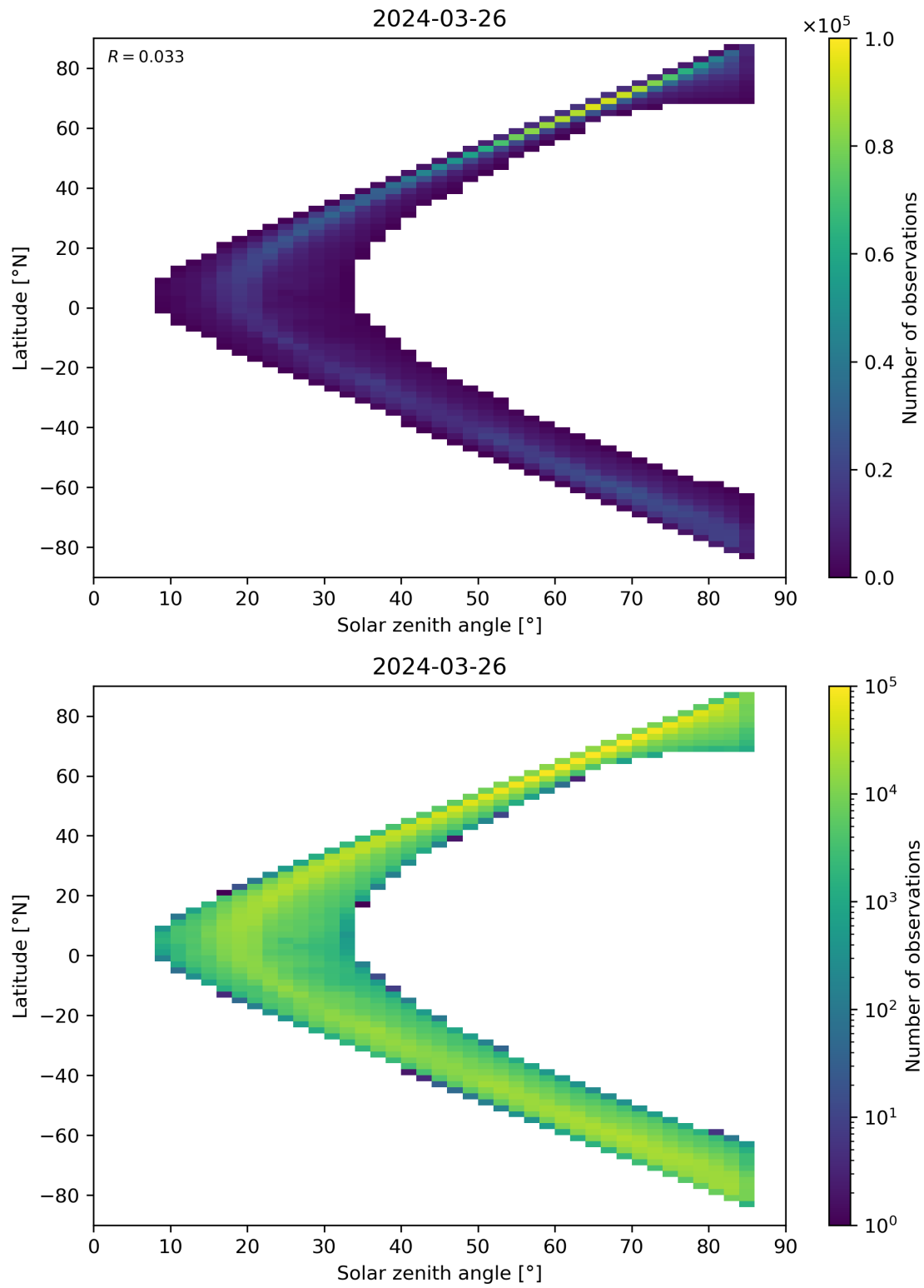
Figure 66: Scatter density plot of “Solar zenith angle” against “Latitude” for 2024-03-25 to 2024-03-27.
