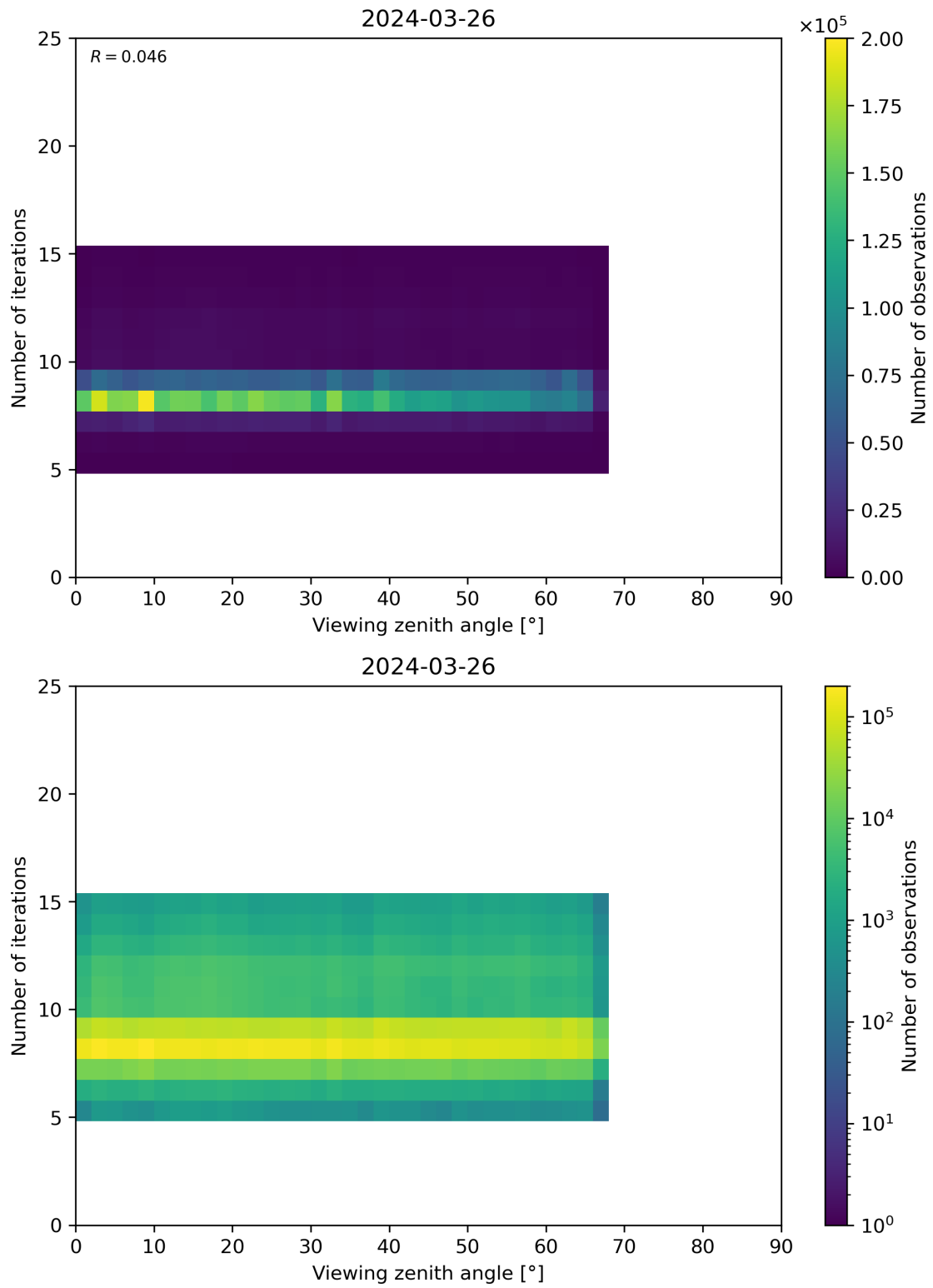
Figure 75: Scatter density plot of “Viewing zenith angle” against “Number of iterations” for 2024-03-25 to 2024-03-27.
