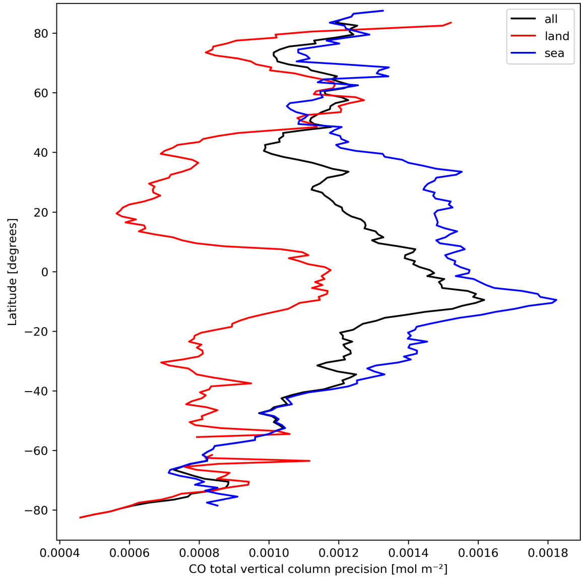
Figure 12: Zonal average of “CO total vertical column precision” for 2024-03-25 to 2024-03-27.
