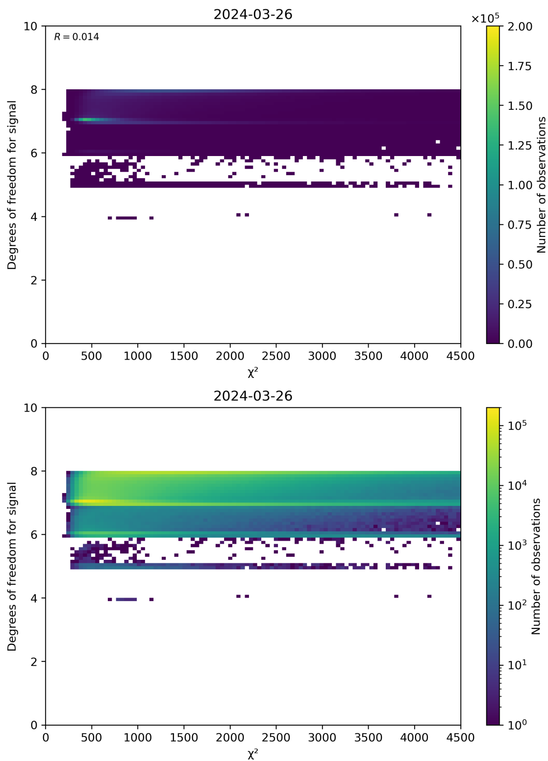
Figure 48: Scatter density plot of “ \chi^2 ” against “Degrees of freedom for signal” for 2024-03-25 to 2024-03-27.
