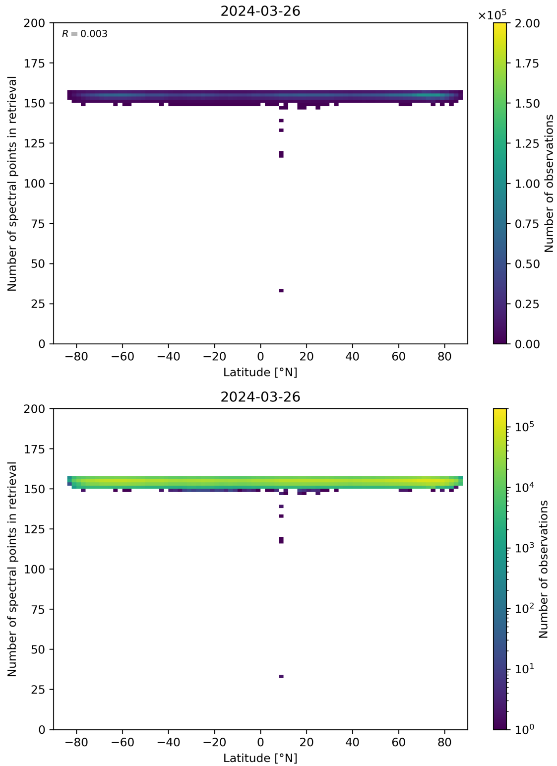
Figure 57: Scatter density plot of “Latitude” against “Number of spectral points in retrieval” for 2024-03-25 to 2024-03-27.
