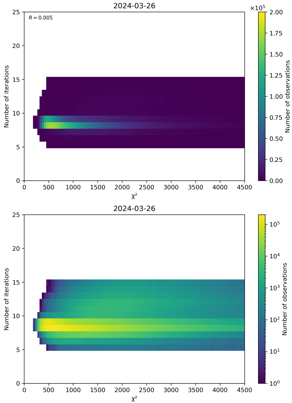
Figure 49: Scatter density plot of “ \chi^2 ” against “Number of iterations” for 2024-03-25 to 2024-03-27.
