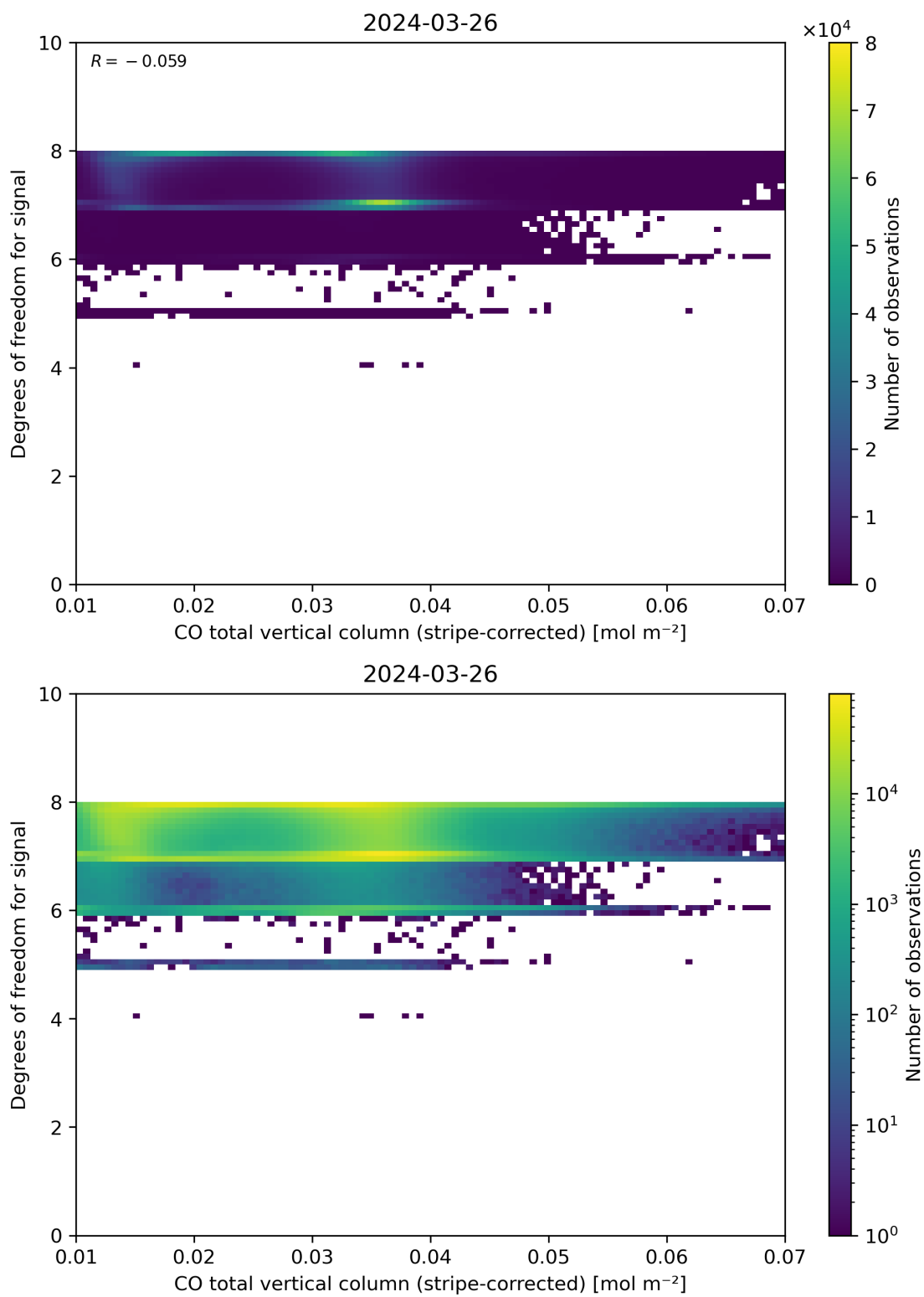
Figure 38: Scatter density plot of “CO total vertical column (stripe-corrected)” against “Degrees of freedom for signal” for 2024-03-25 to 2024-03-27.
