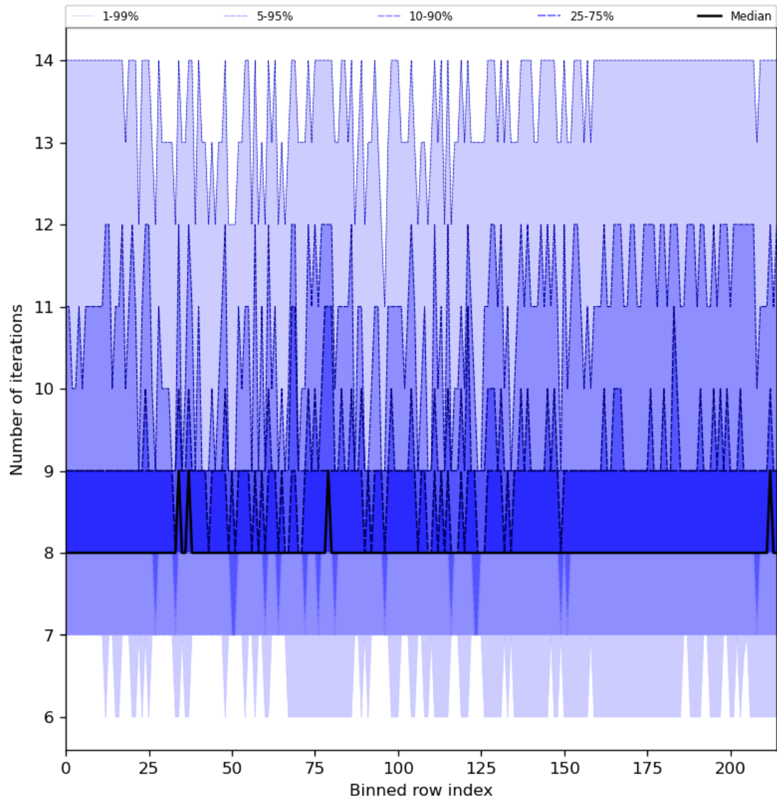
Figure 32: Along track statistics of “Number of iterations” for 2024-03-25 to 2024-03-27
