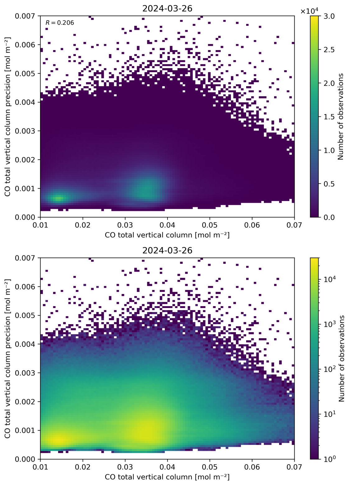
Figure 34: Scatter density plot of “CO total vertical column” against “CO total vertical column precision” for 2024-03-25 to 2024-03-27.
