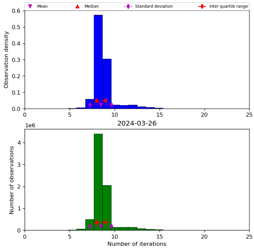
Figure 24: Histogram of “Number of iterations” for 2024-03-25 to 2024-03-27
