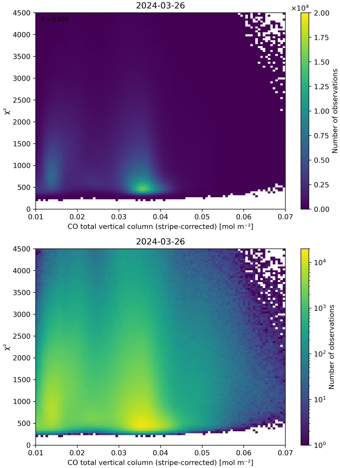
Figure 37: Scatter density plot of “CO total vertical column (stripe-corrected)” against “ \chi^2 ” for 2024-03-25 to 2024-03-27.
