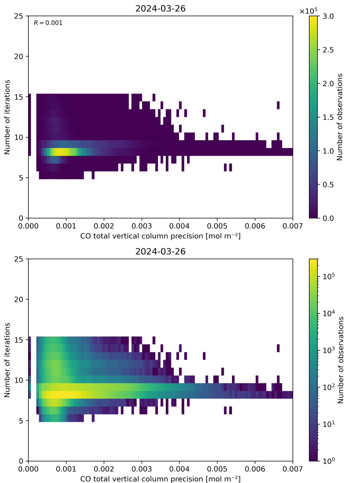
Figure 46: Scatter density plot of “CO total vertical column precision” against “Number of iterations” for 2024-03-25 to 2024-03-27.
