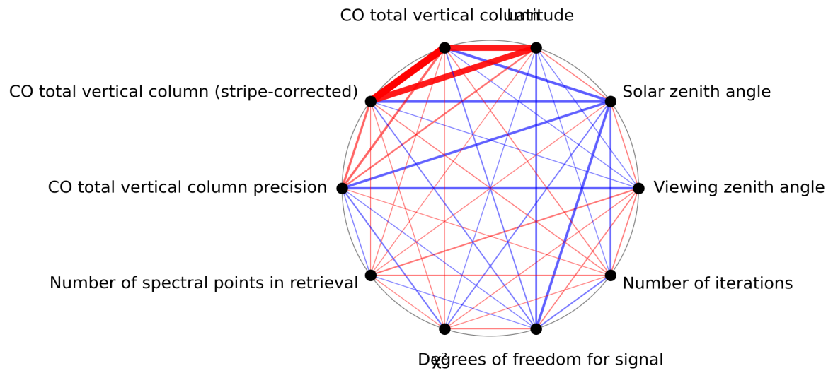
Figure 1: Map of correlation graph for 2024-03-25 to 2024-03-27.
