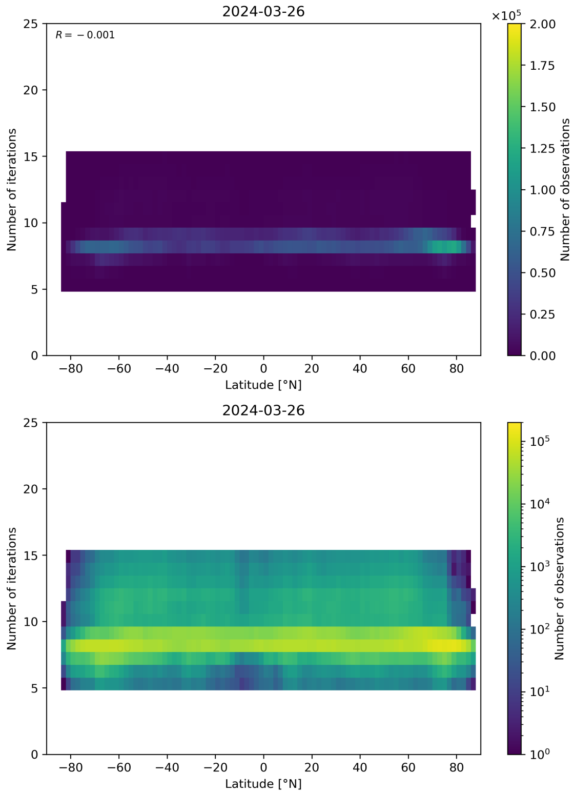
Figure 56: Scatter density plot of “Latitude” against “Number of iterations” for 2024-03-25 to 2024-03-27.
