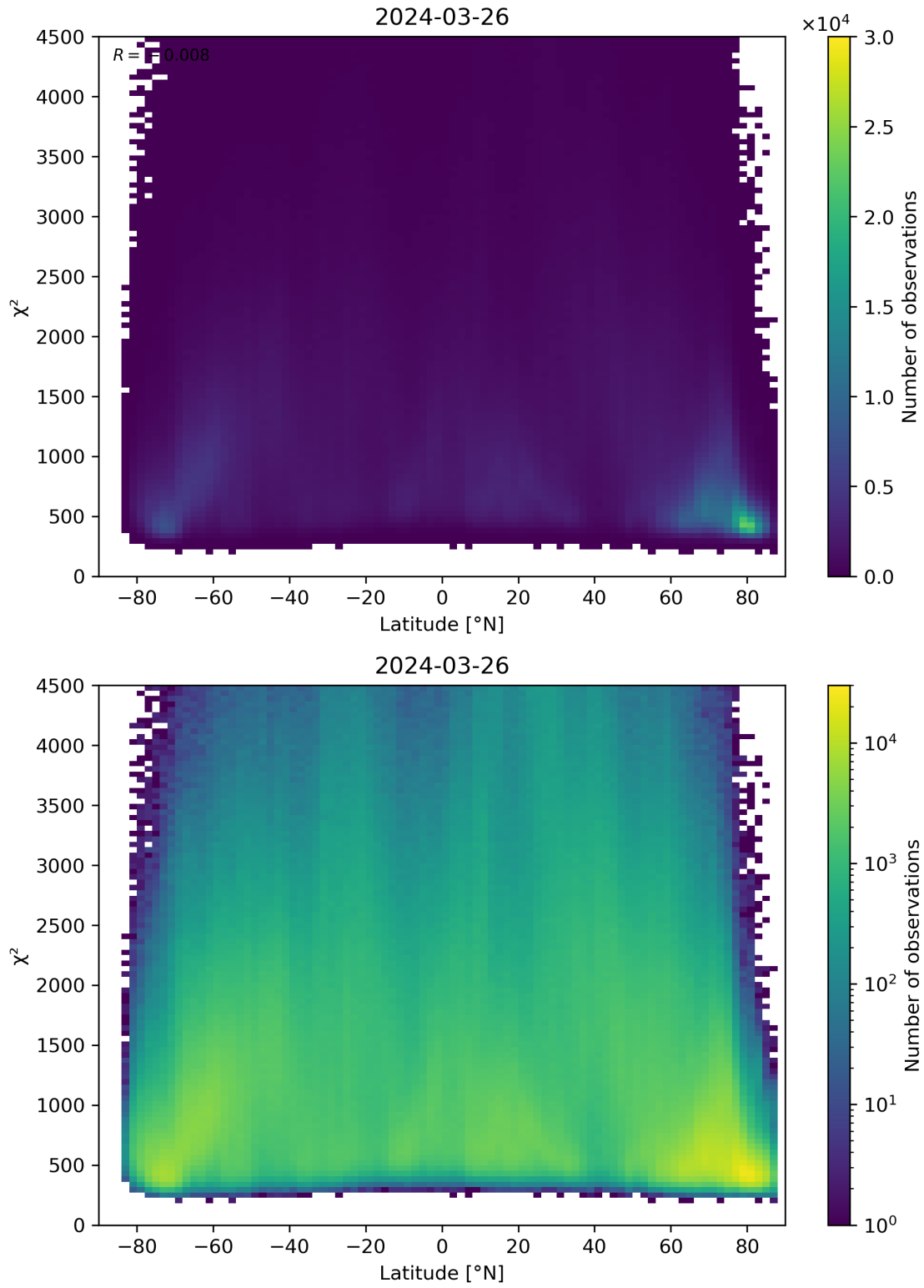
Figure 54: Scatter density plot of “Latitude” against “ \chi^2 ” for 2024-03-25 to 2024-03-27.
