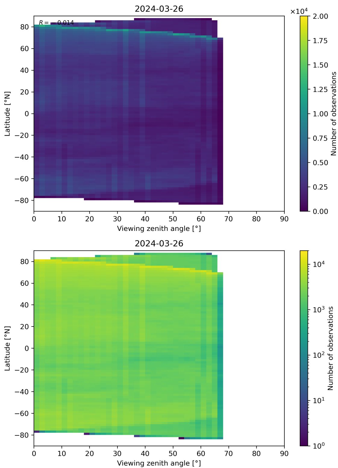
Figure 74: Scatter density plot of “Viewing zenith angle” against “Latitude” for 2024-03-25 to 2024-03-27.
