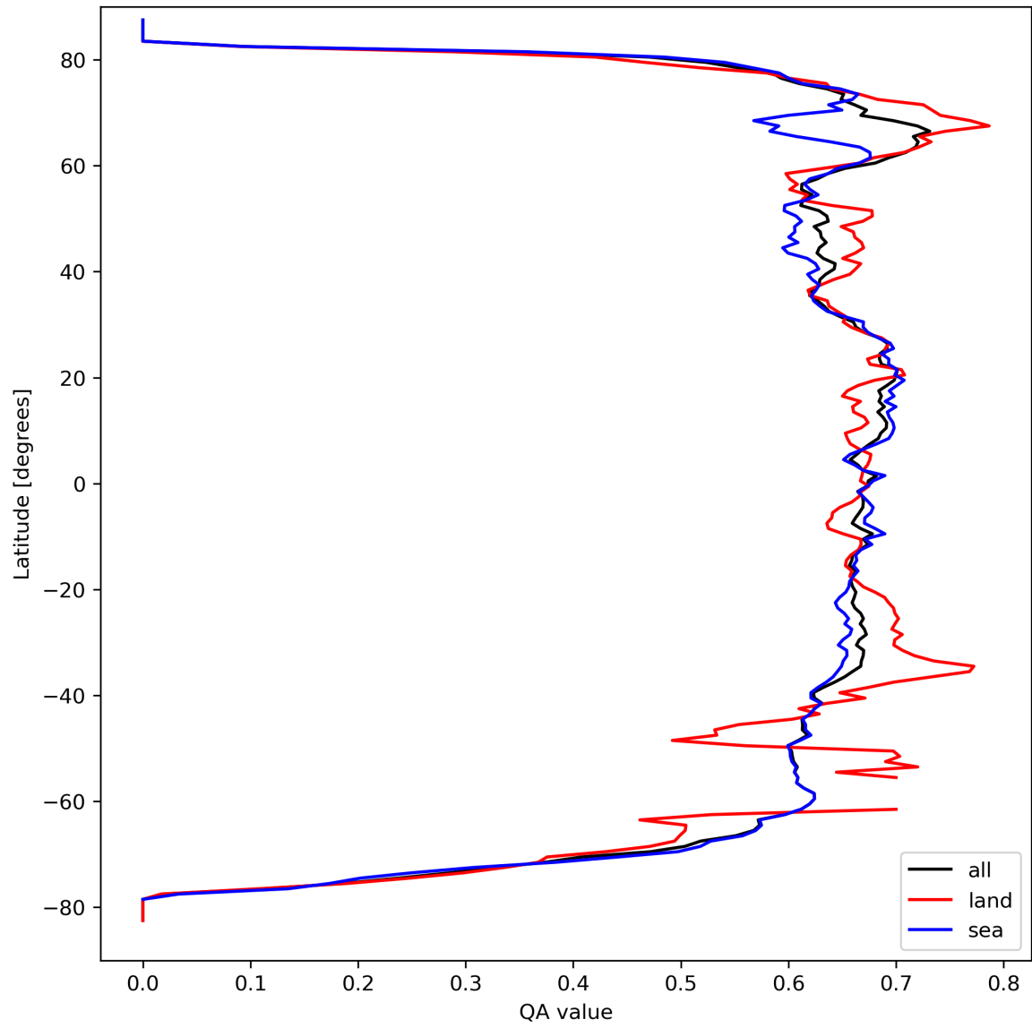
Figure 9: Zonal average of “QA value” for 2024-03-25 to 2024-03-27.
