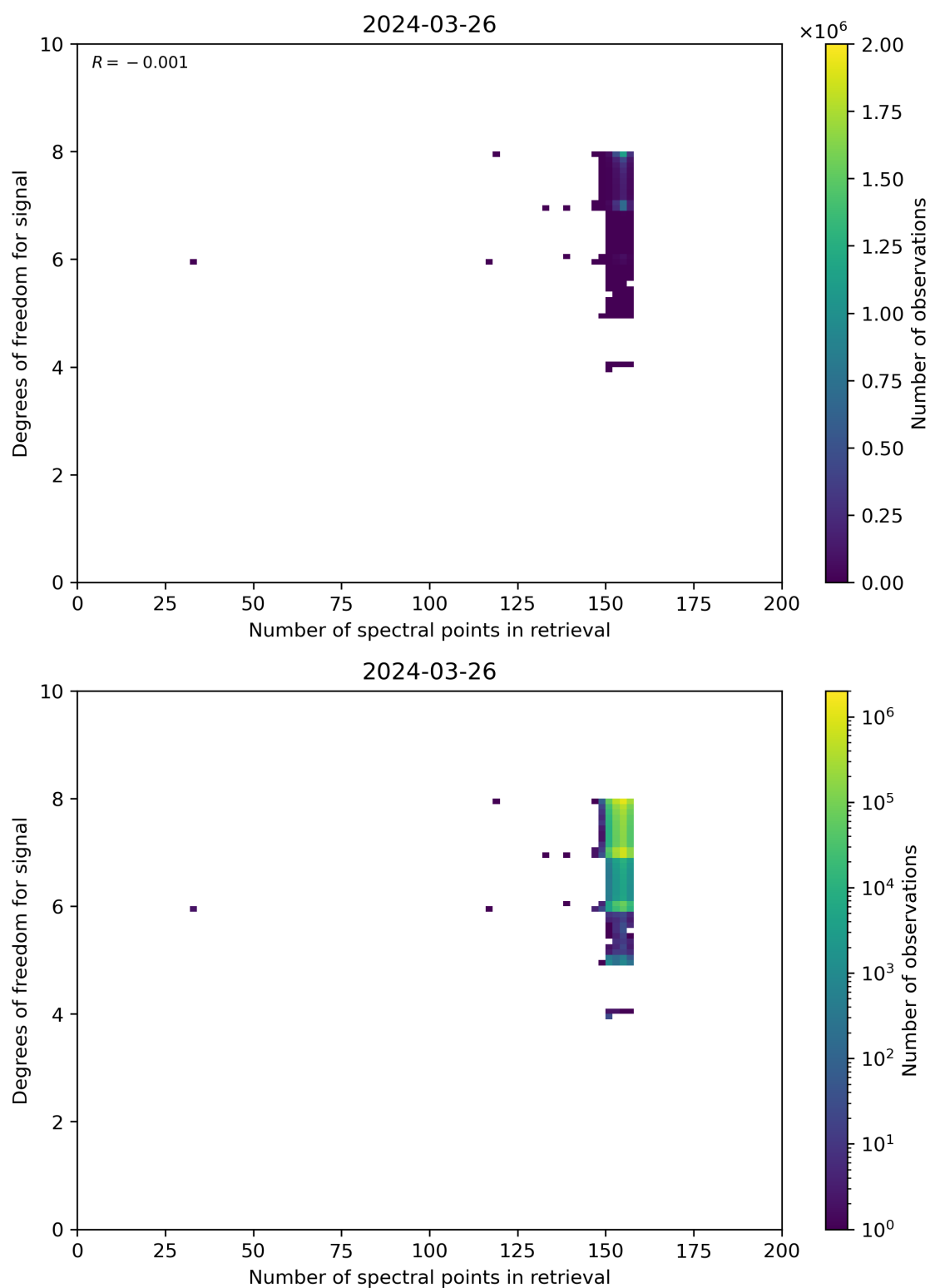
Figure 59: Scatter density plot of “Number of spectral points in retrieval” against “Degrees of freedom for signal” for 2024-03-25 to 2024-03-27.
