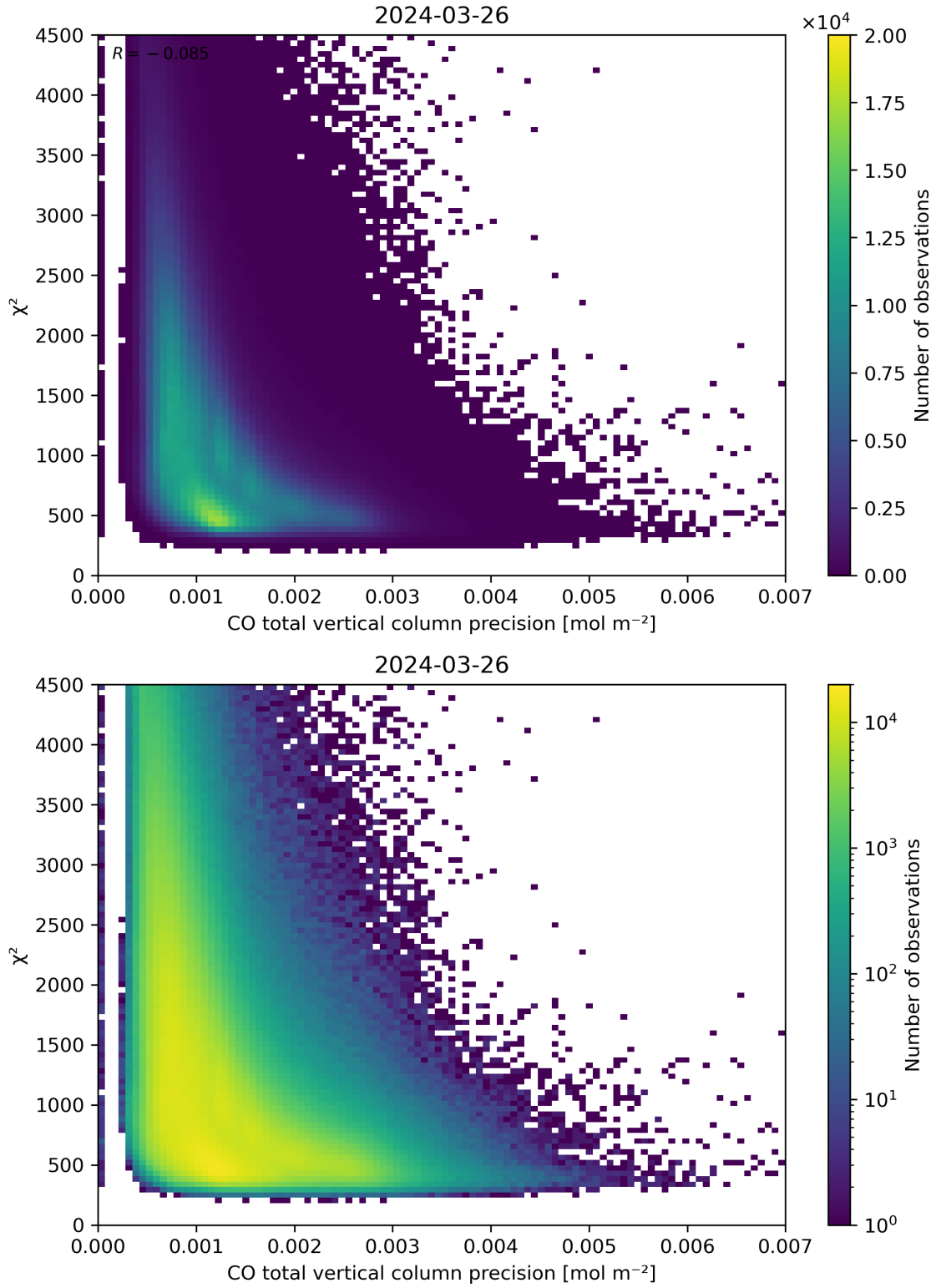
Figure 44: Scatter density plot of “CO total vertical column precision” against “ \chi^2 ” for 2024-03-25 to 2024-03-27.
