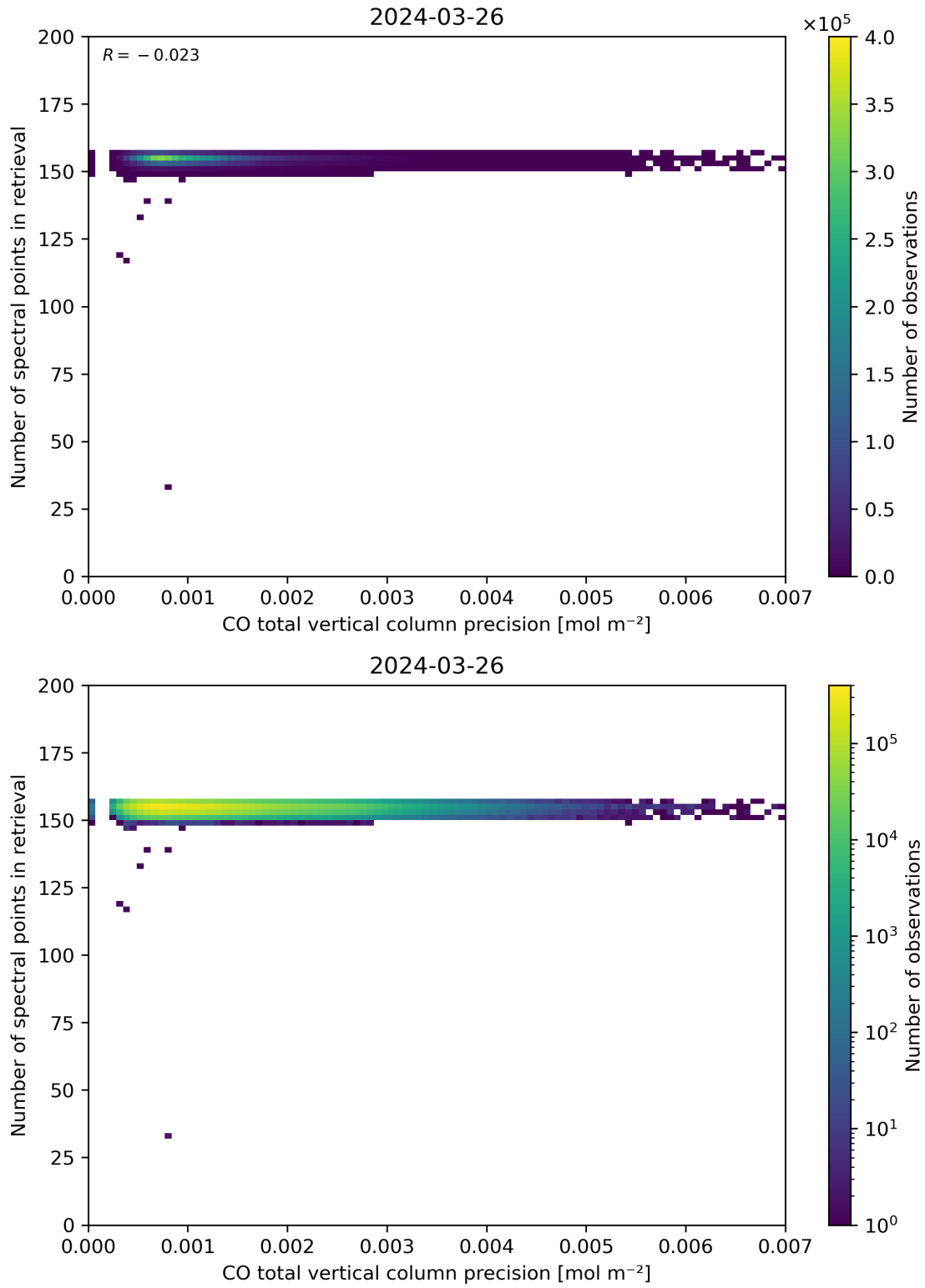
Figure 47: Scatter density plot of “CO total vertical column precision” against “Number of spectral points in retrieval” for 2024-03-25 to 2024-03-27.
