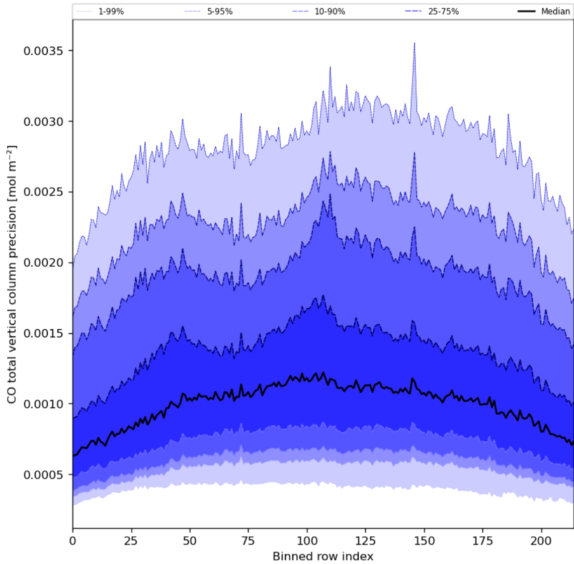
Figure 28: Along track statistics of “CO total vertical column precision” for 2024-03-25 to 2024-03-27
