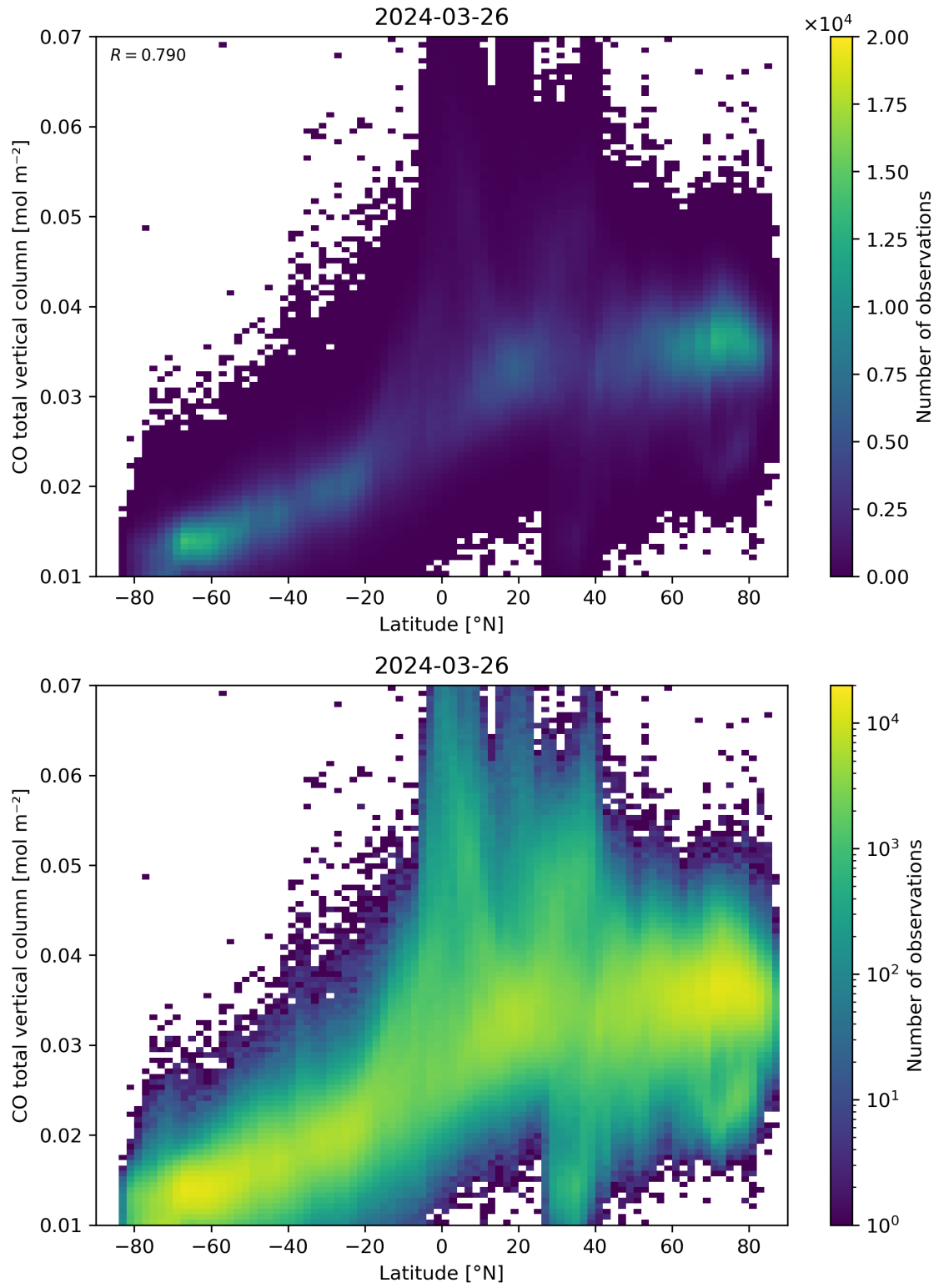
Figure 51: Scatter density plot of “Latitude” against “CO total vertical column” for 2024-03-25 to 2024-03-27.
