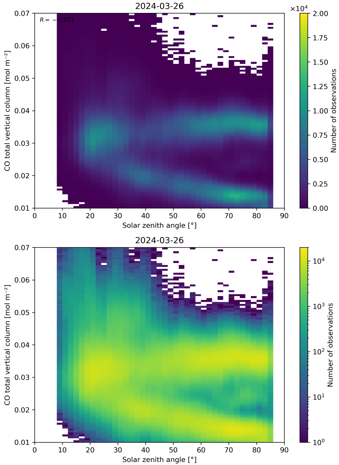
Figure 61: Scatter density plot of “Solar zenith angle” against “CO total vertical column” for 2024-03-25 to 2024-03-27.
