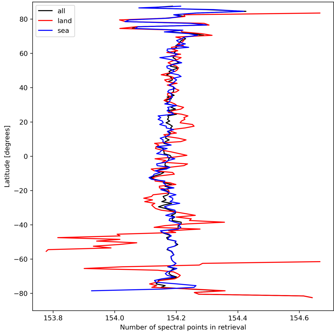
Figure 13: Zonal average of “Number of spectral points in retrieval” for 2024-03-25 to 2024-03-27.
