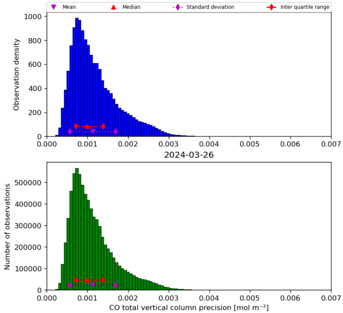
Figure 20: Histogram of “CO total vertical column precision” for 2024-03-25 to 2024-03-27
