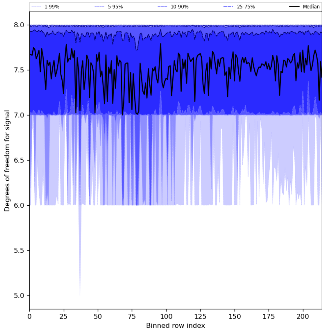
Figure 31: Along track statistics of “Degrees of freedom for signal” for 2024-03-25 to 2024-03-27
