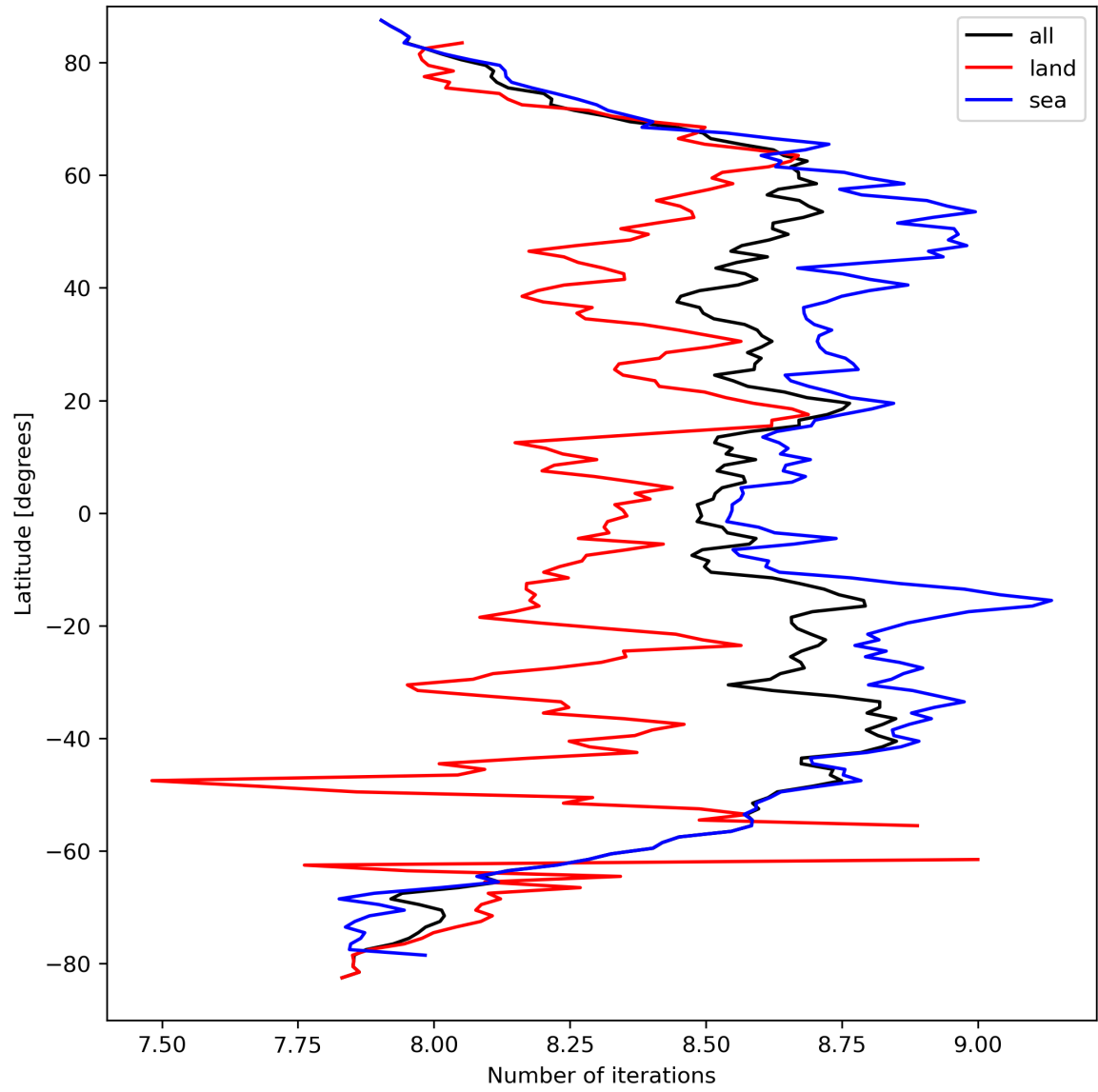
Figure 16: Zonal average of “Number of iterations” for 2024-03-25 to 2024-03-27.
