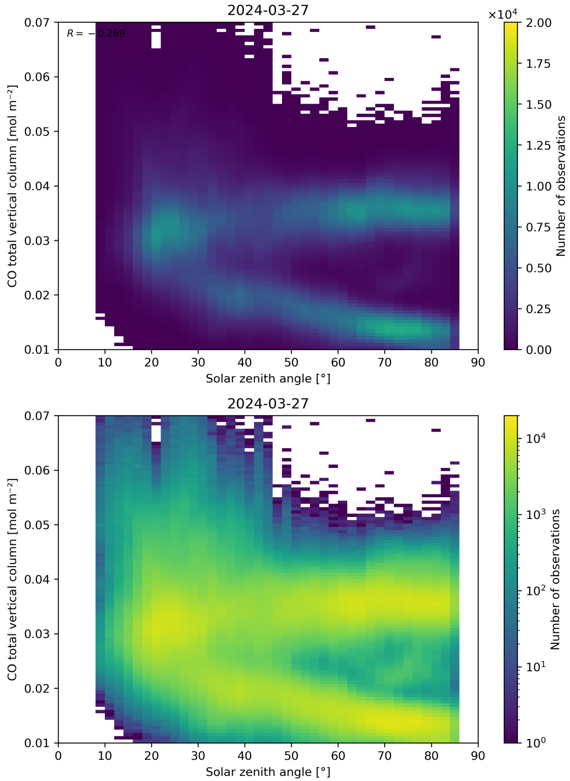
Figure 61: Scatter density plot of “Solar zenith angle” against “CO total vertical column” for 2024-03-26 to 2024-03-28.
