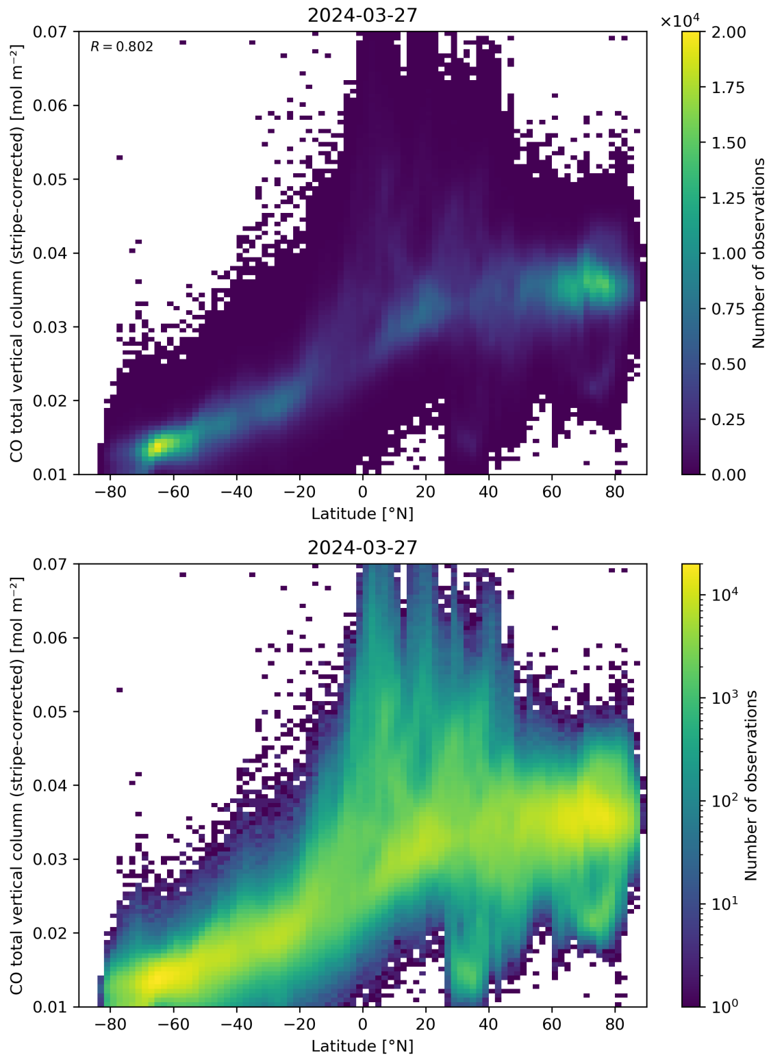
Figure 52: Scatter density plot of “Latitude” against “CO total vertical column (stripe-corrected)” for 2024-03-26 to 2024-03-28.
