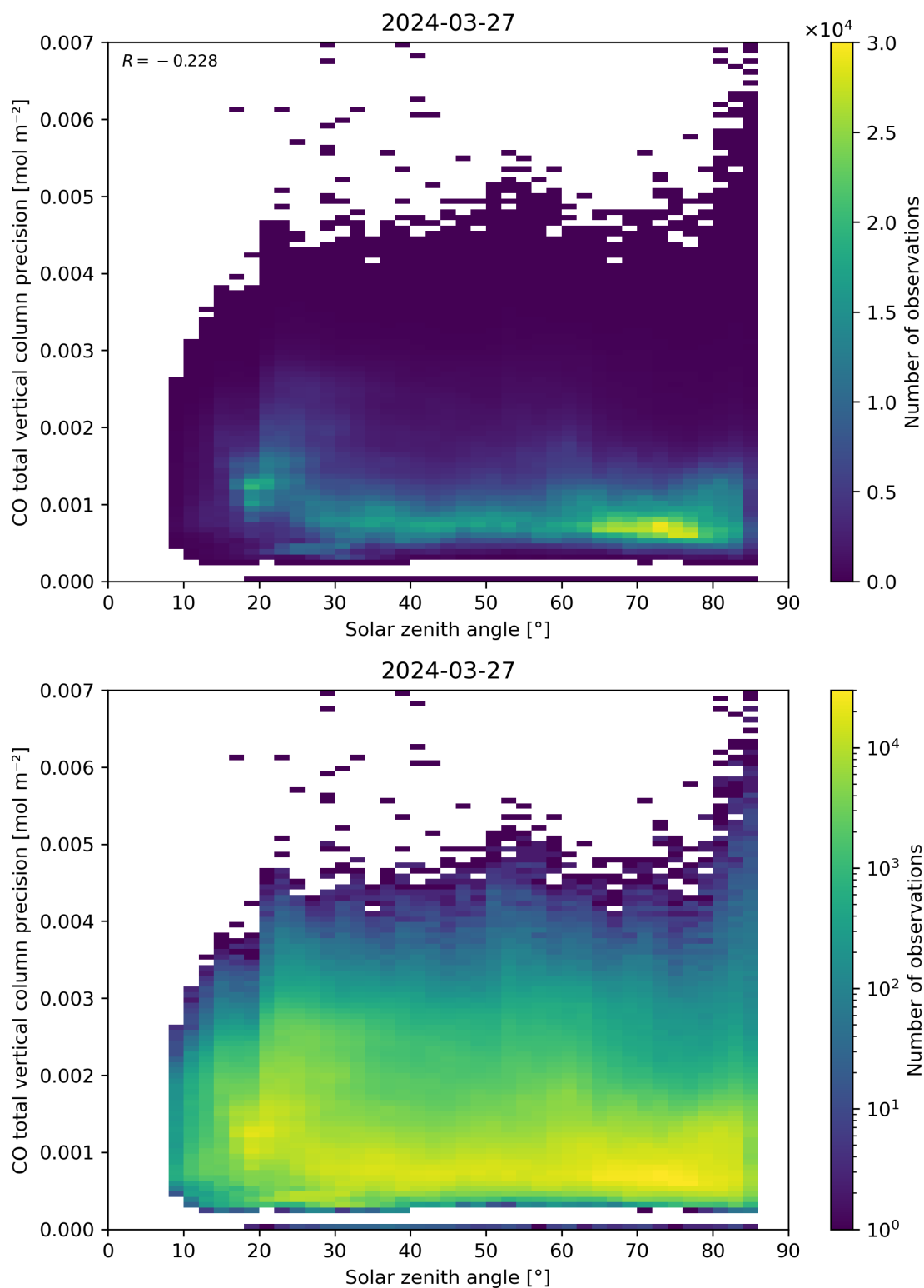
Figure 63: Scatter density plot of “Solar zenith angle” against “CO total vertical column precision” for 2024-03-26 to 2024-03-28.
