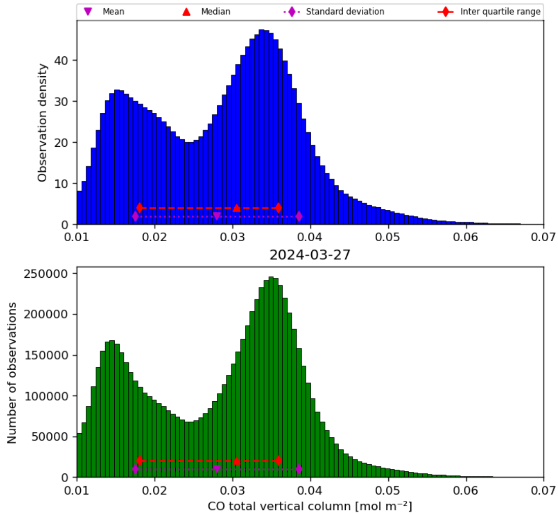
Figure 18: Histogram of “CO total vertical column” for 2024-03-26 to 2024-03-28
