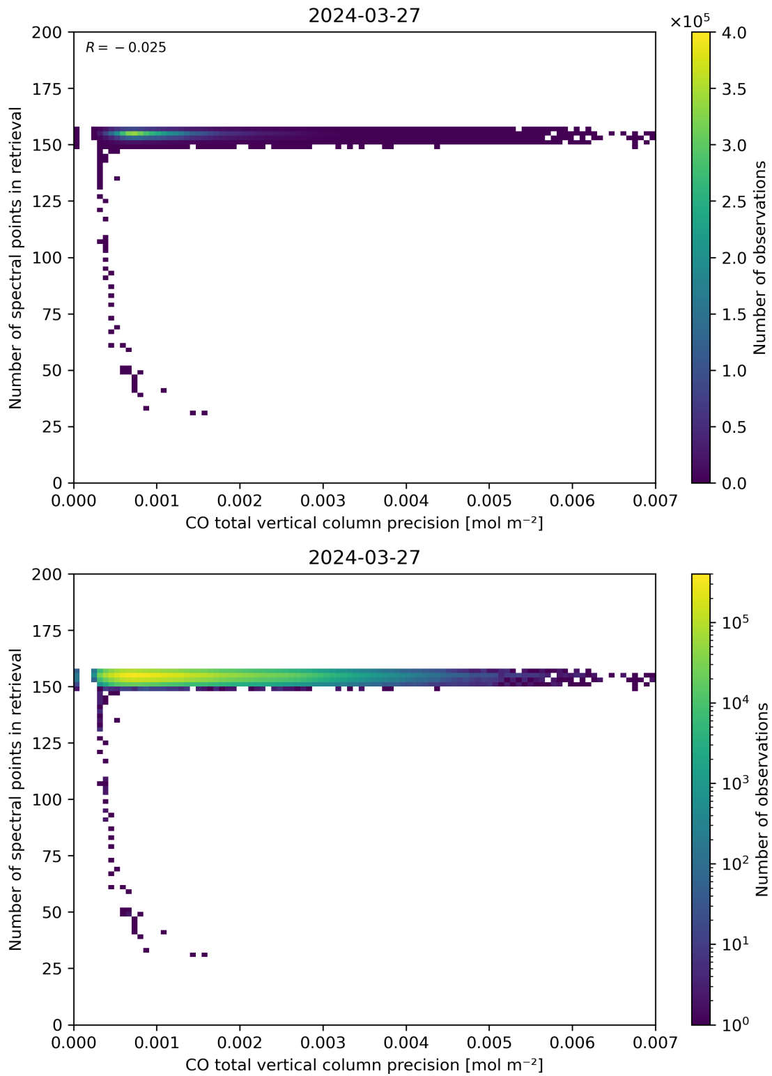
Figure 47: Scatter density plot of “CO total vertical column precision” against “Number of spectral points in retrieval” for 2024-03-26 to 2024-03-28.
