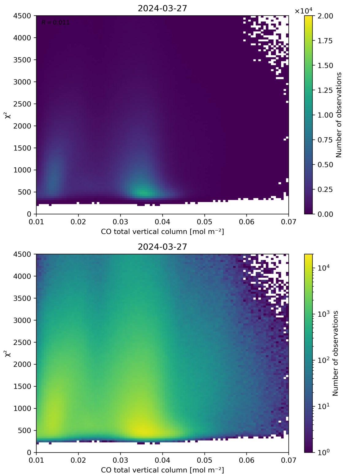
Figure 35: Scatter density plot of “CO total vertical column” against “ \chi^2 ” for 2024-03-26 to 2024-03-28.
