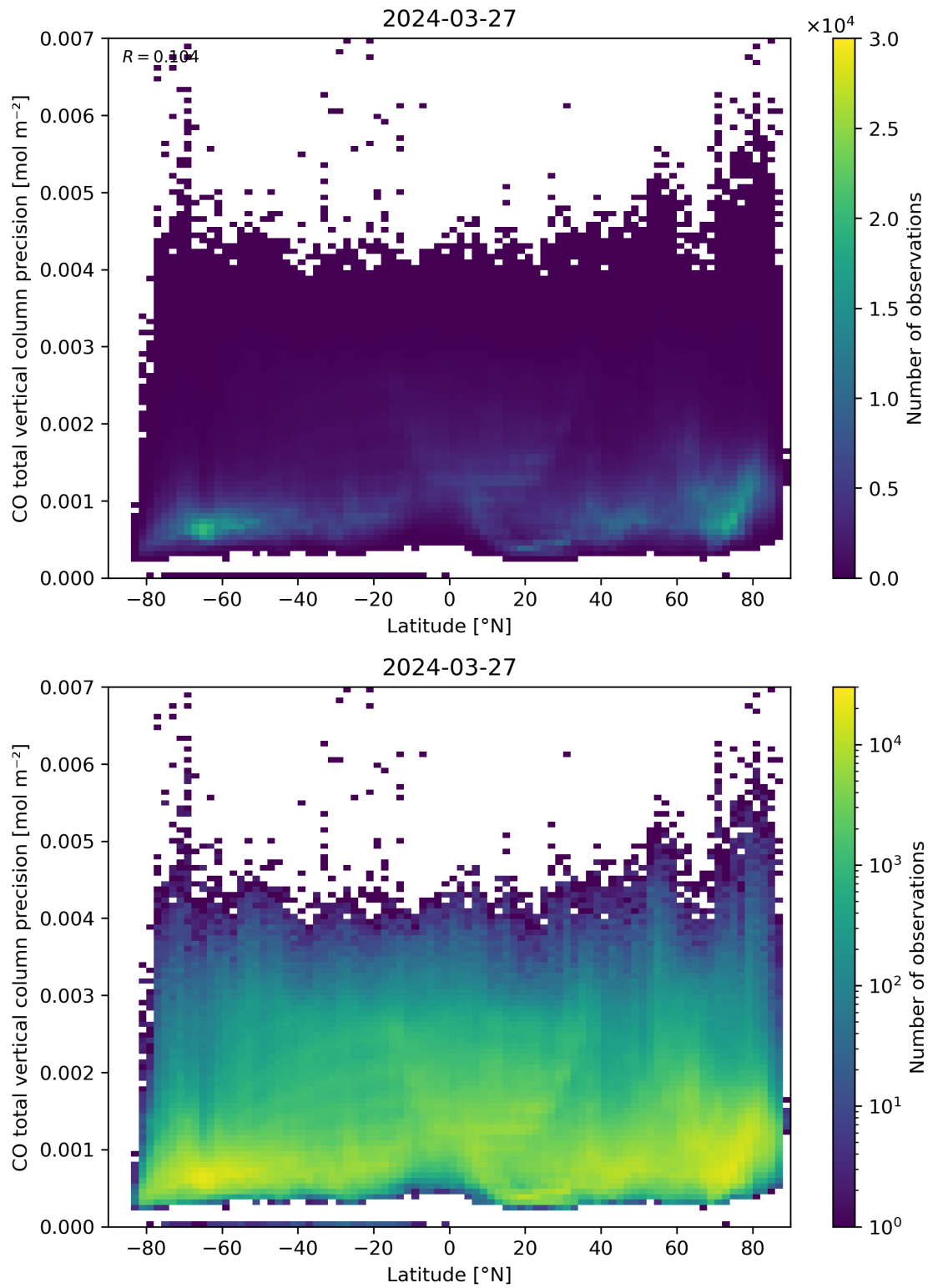
Figure 53: Scatter density plot of “Latitude” against “CO total vertical column precision” for 2024-03-26 to 2024-03-28.
