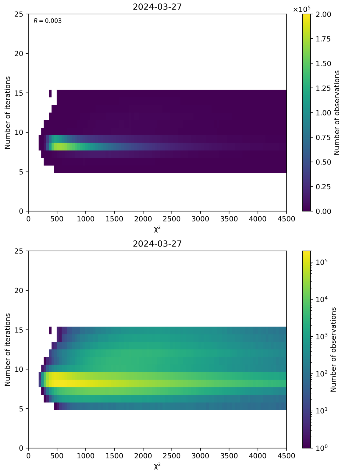
Figure 49: Scatter density plot of “ \chi^2 ” against “Number of iterations” for 2024-03-26 to 2024-03-28.
