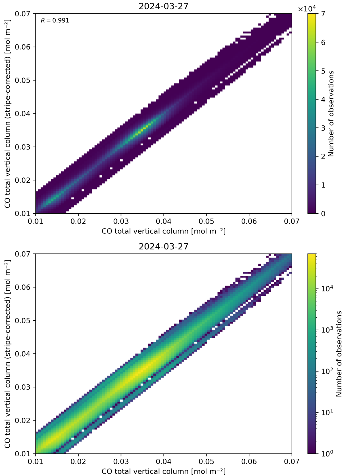
Figure 33: Scatter density plot of “CO total vertical column” against “CO total vertical column (stripe-corrected)” for 2024-03-26 to 2024-03-28.
