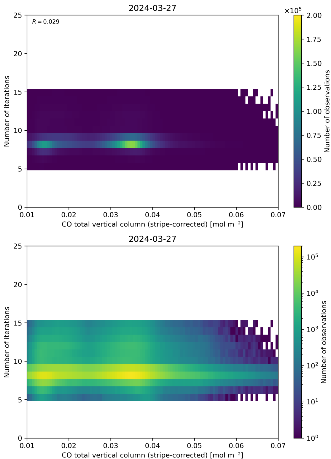
Figure 39: Scatter density plot of “CO total vertical column (stripe-corrected)” against “Number of iterations” for 2024-03-26 to 2024-03-28.
