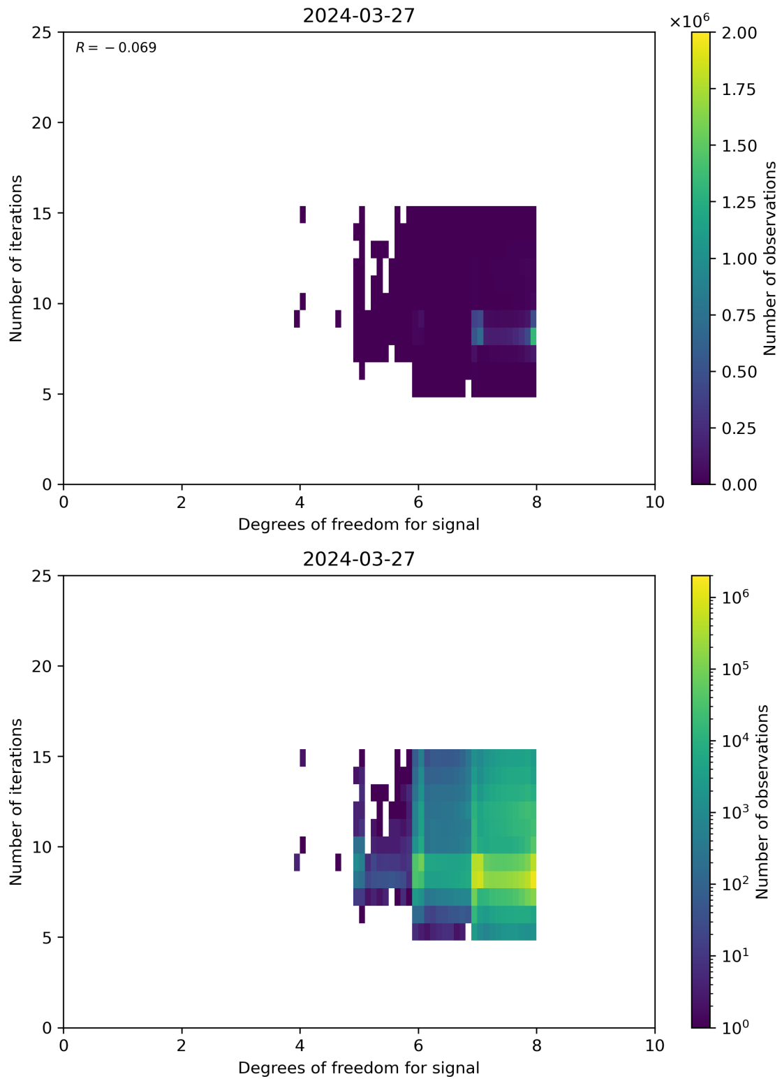
Figure 50: Scatter density plot of “Degrees of freedom for signal” against “Number of iterations” for 2024-03-26 to 2024-03-28.
