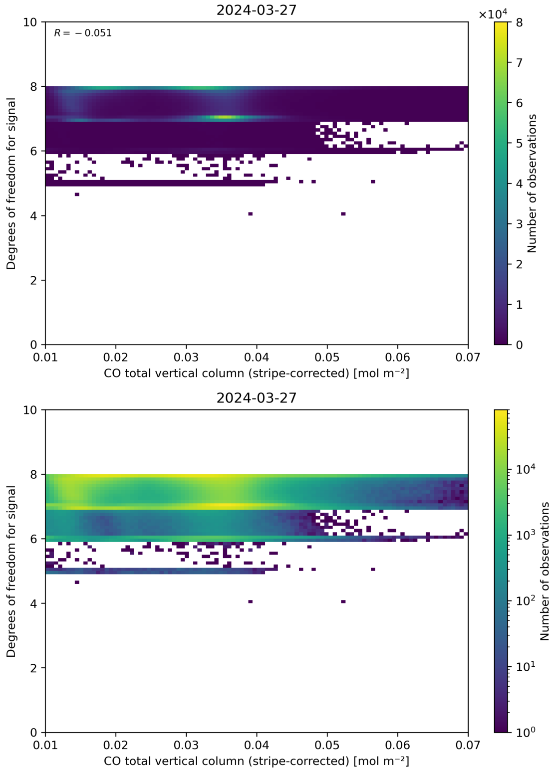
Figure 38: Scatter density plot of “CO total vertical column (stripe-corrected)” against “Degrees of freedom for signal” for 2024-03-26 to 2024-03-28.
