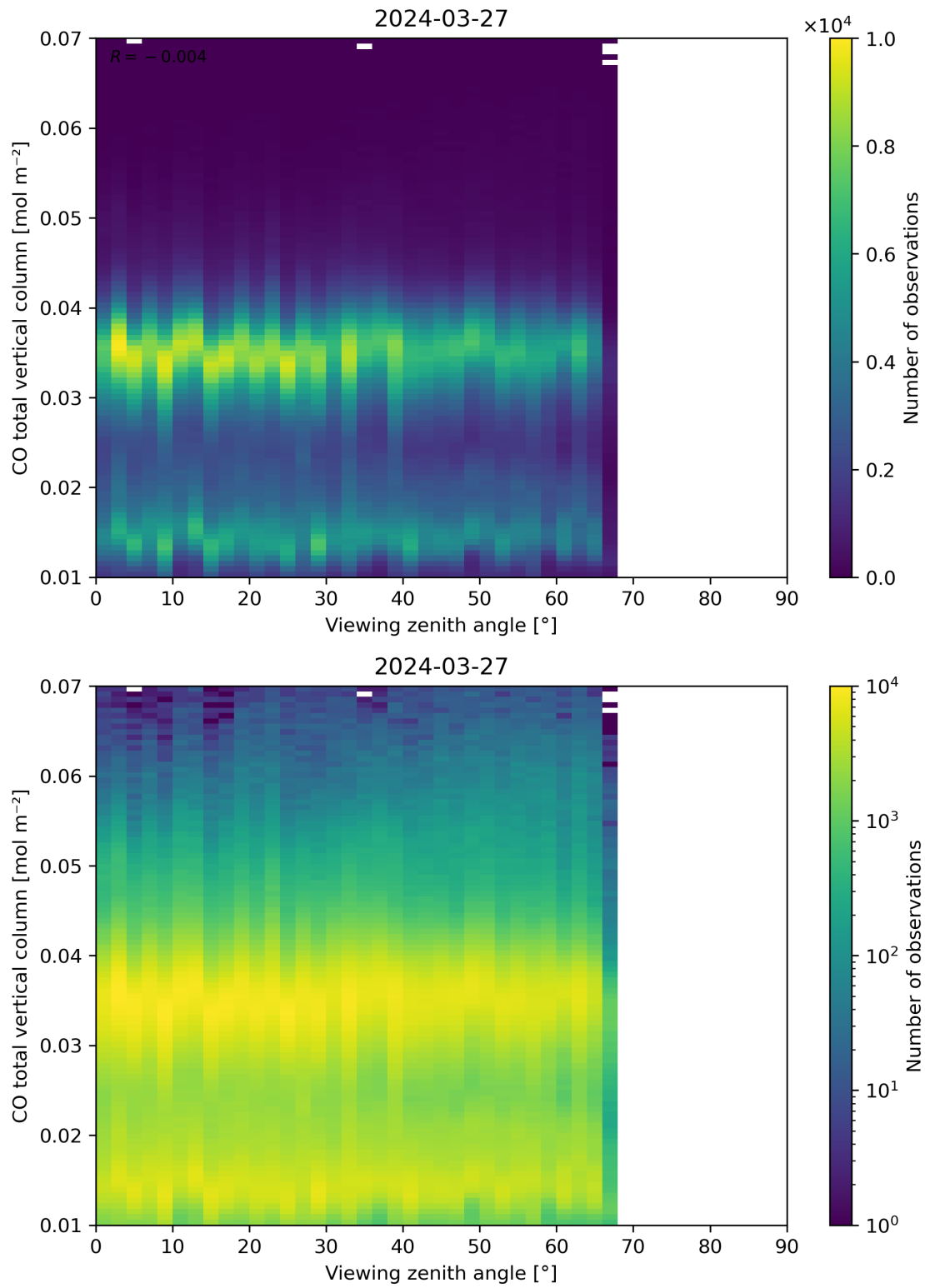
Figure 69: Scatter density plot of “Viewing zenith angle” against “CO total vertical column” for 2024-03-26 to 2024-03-28.
