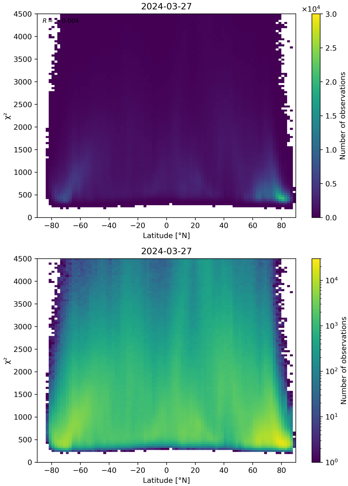
Figure 54: Scatter density plot of “Latitude” against “ \chi^2 ” for 2024-03-26 to 2024-03-28.
