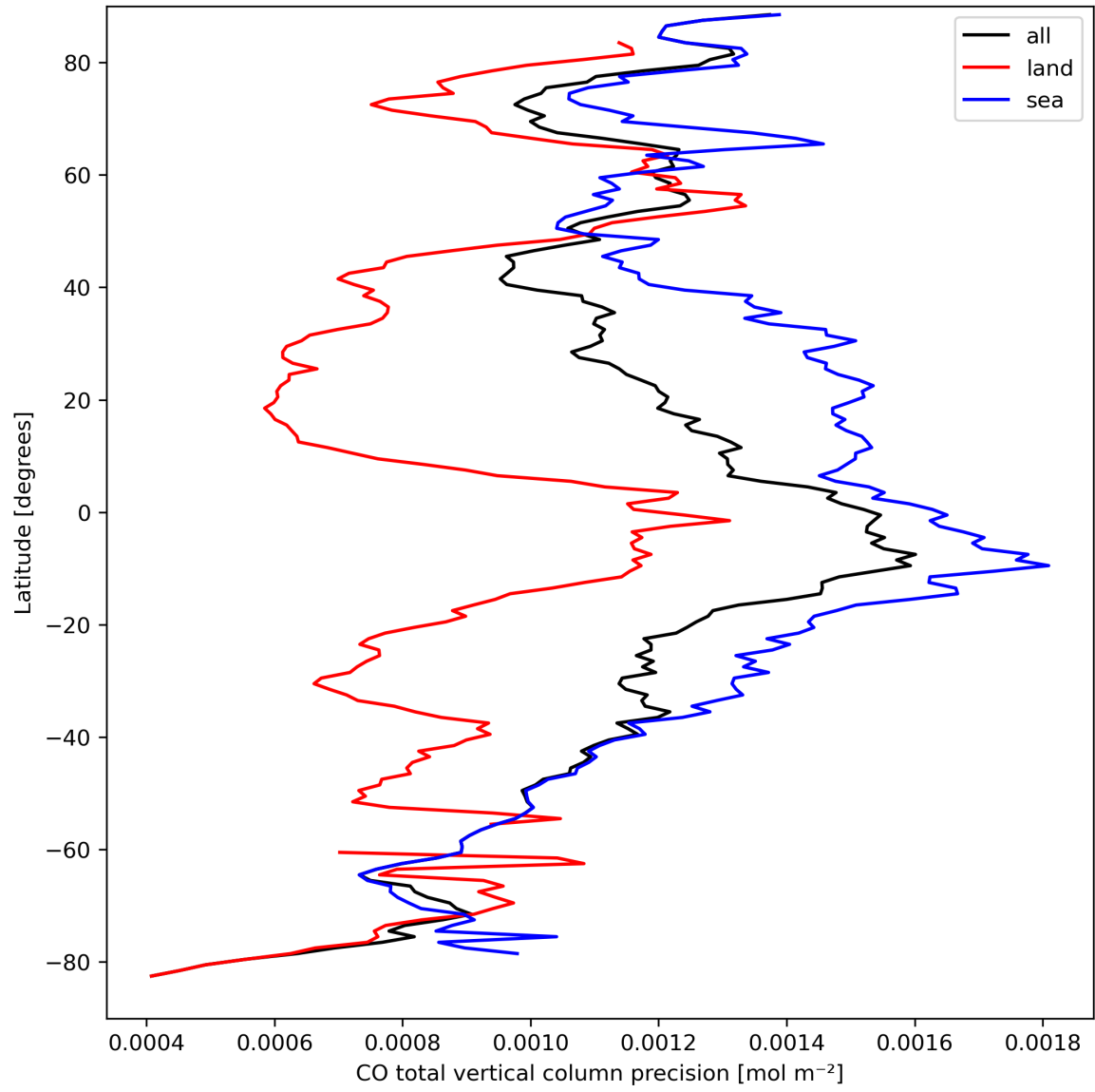
Figure 12: Zonal average of “CO total vertical column precision” for 2024-03-26 to 2024-03-28.
