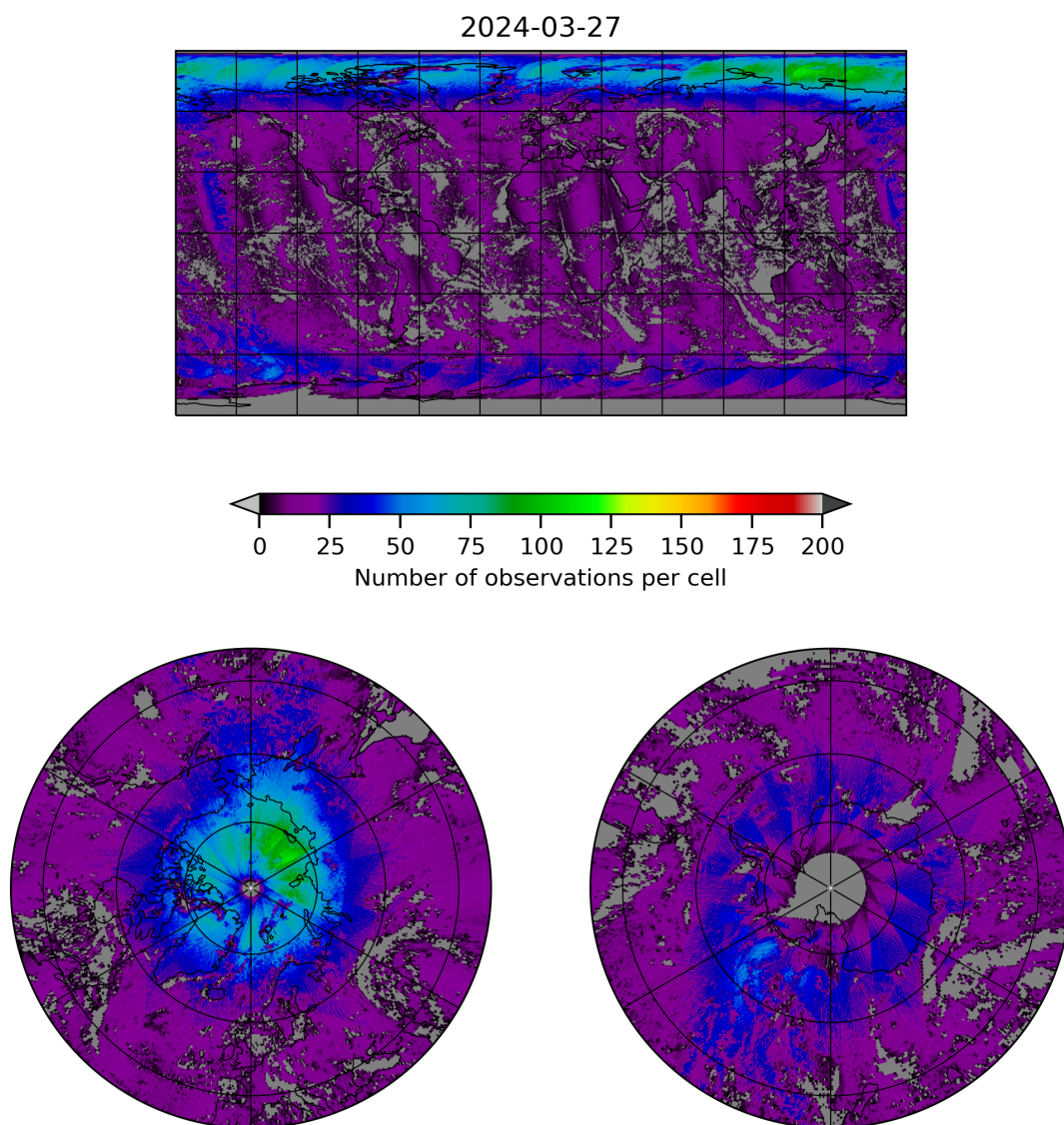
Figure 8: Map of the number of observations for 2024-03-26 to 2024-03-28
