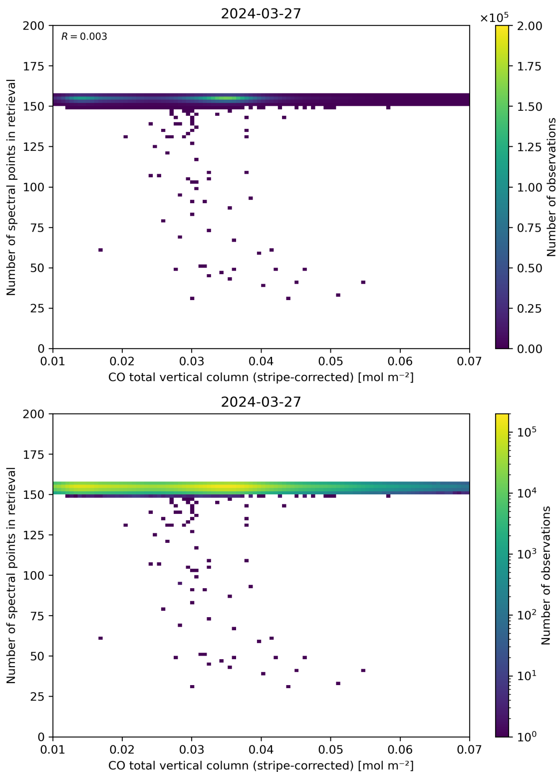
Figure 40: Scatter density plot of “CO total vertical column (stripe-corrected)” against “Number of spectral points in retrieval” for 2024-03-26 to 2024-03-28.
