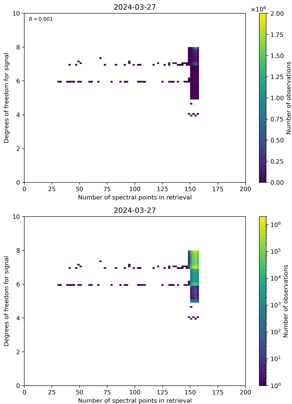
Figure 59: Scatter density plot of “Number of spectral points in retrieval” against “Degrees of freedom for signal” for 2024-03-26 to 2024-03-28.
