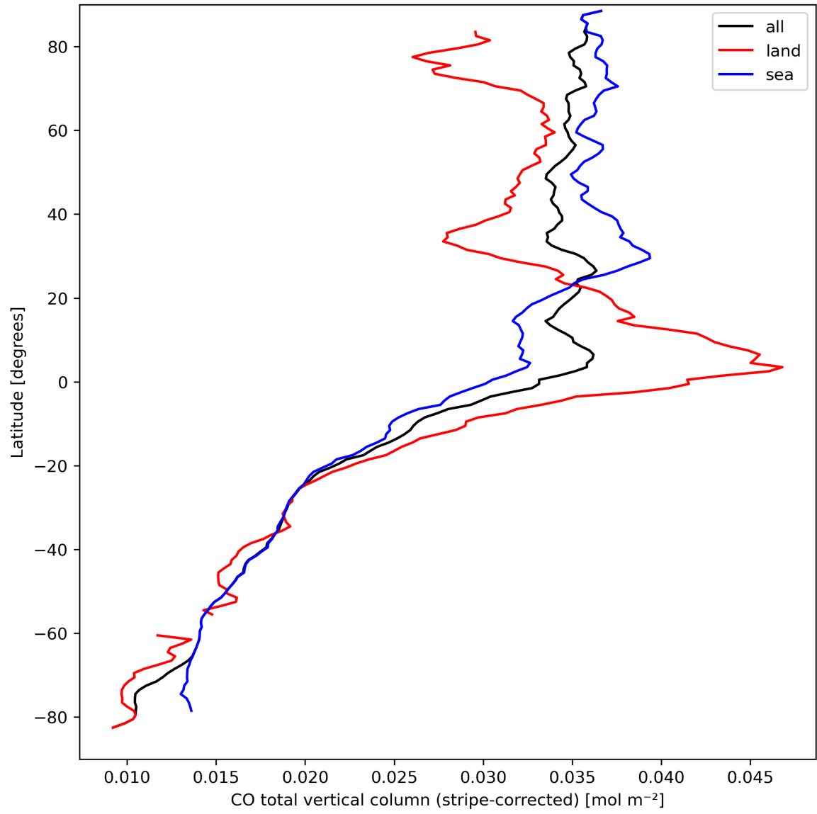
Figure 11: Zonal average of “CO total vertical column (stripe-corrected)” for 2024-03-26 to 2024-03-28.
