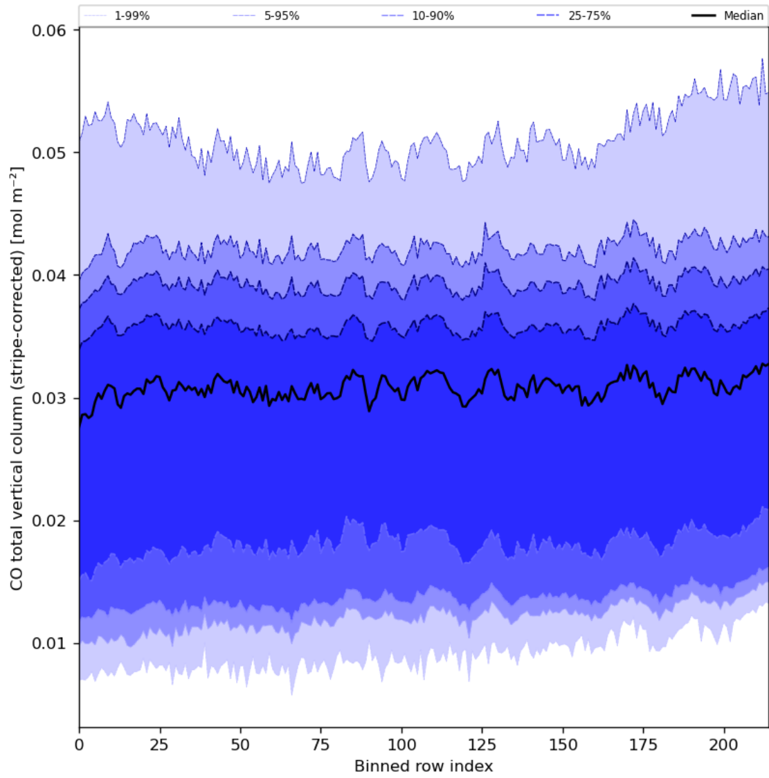
Figure 27: Along track statistics of “CO total vertical column (stripe-corrected)” for 2024-03-26 to 2024-03-28
