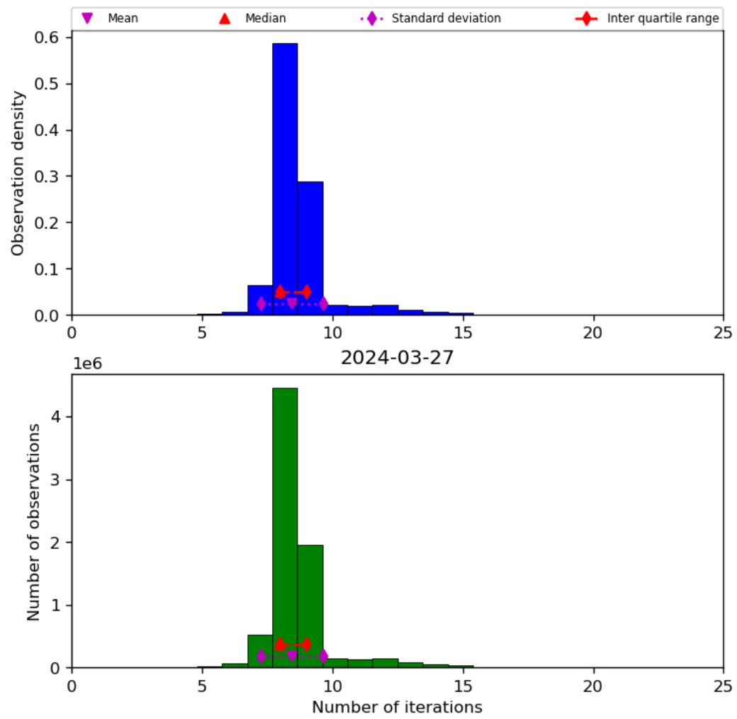
Figure 24: Histogram of “Number of iterations” for 2024-03-26 to 2024-03-28
