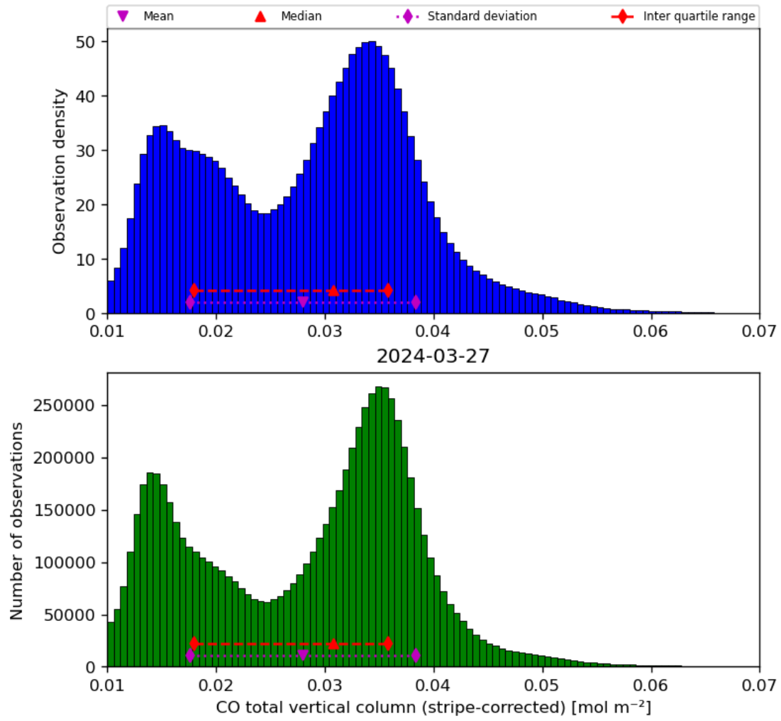
Figure 19: Histogram of “CO total vertical column (stripe-corrected)” for 2024-03-26 to 2024-03-28
