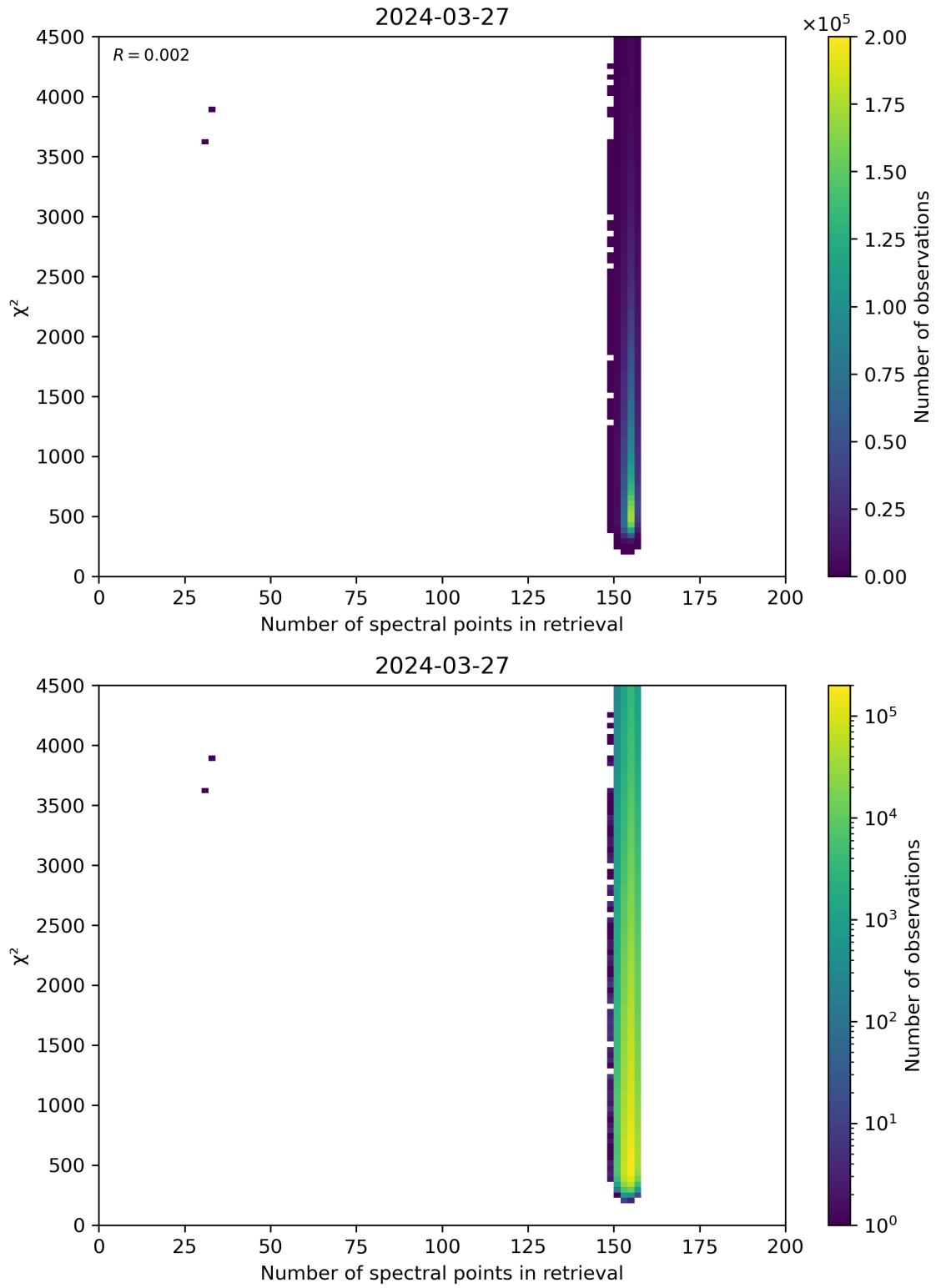
Figure 58: Scatter density plot of “Number of spectral points in retrieval” against “ \chi^2 ” for 2024-03-26 to 2024-03-28.
