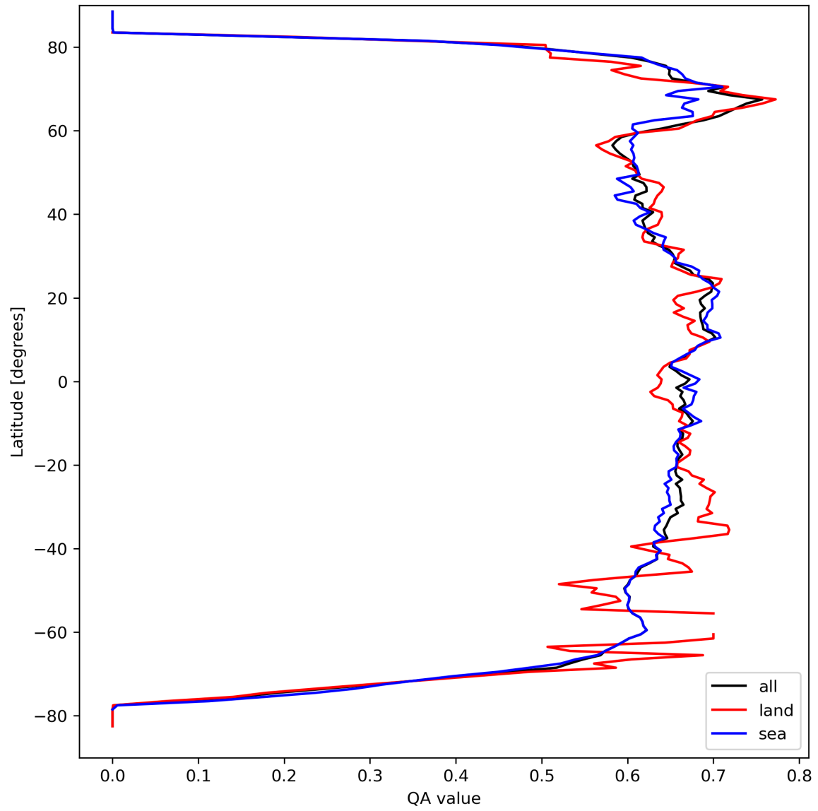
Figure 9: Zonal average of “QA value” for 2024-03-26 to 2024-03-28.
