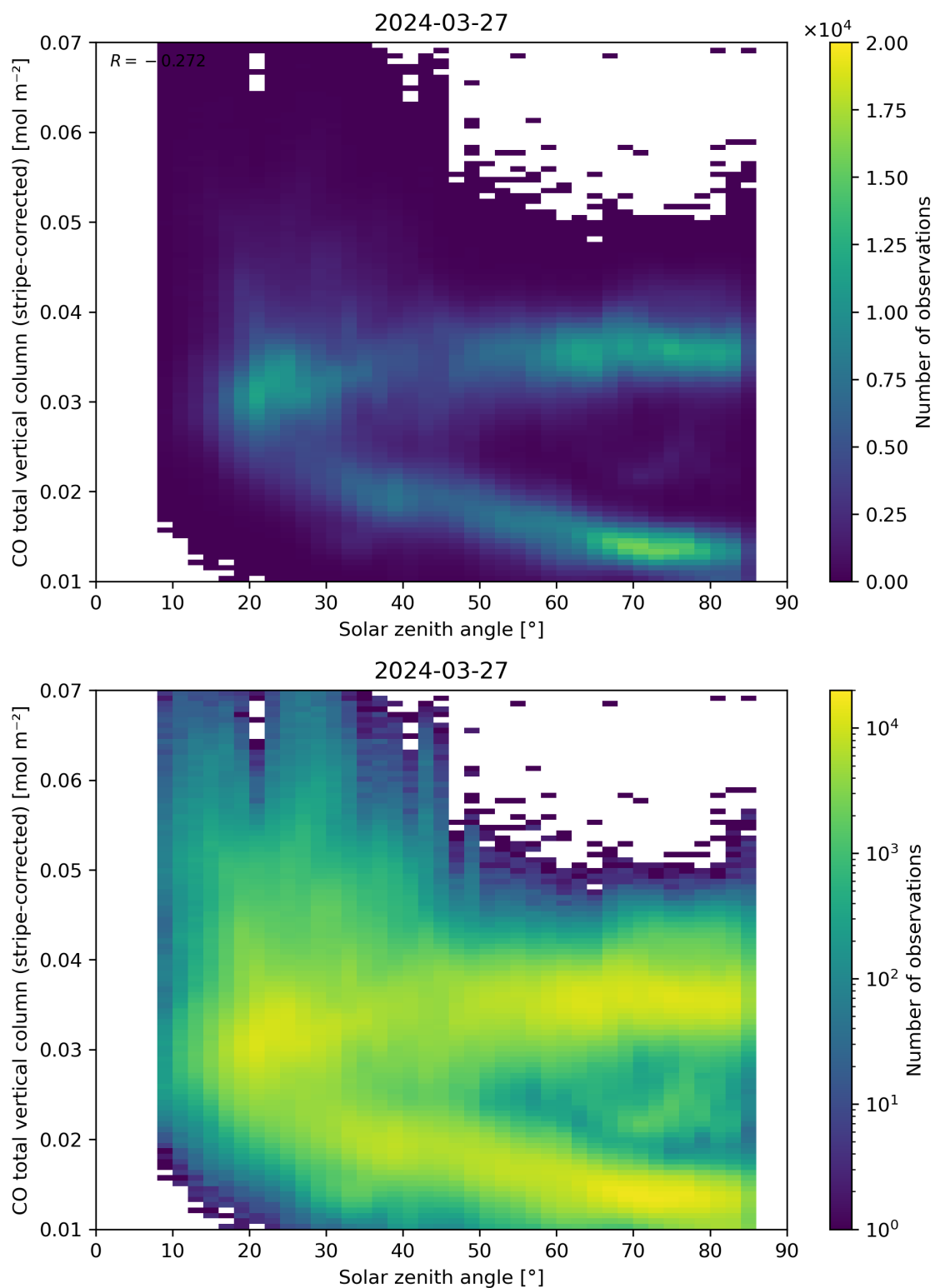
Figure 62: Scatter density plot of “Solar zenith angle” against “CO total vertical column (stripe-corrected)” for 2024-03-26 to 2024-03-28.
