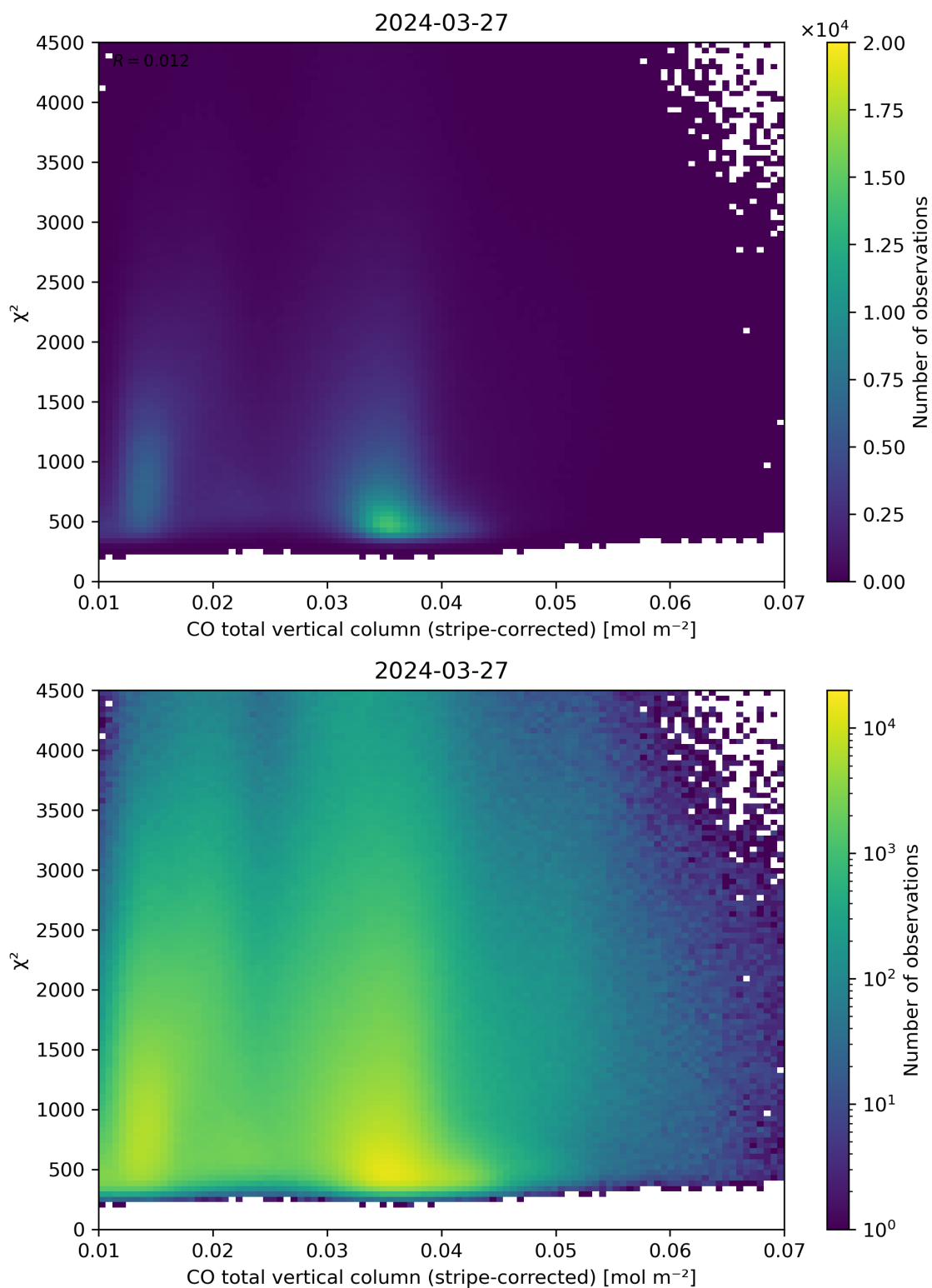
Figure 37: Scatter density plot of “CO total vertical column (stripe-corrected)” against “ \chi^2 ” for 2024-03-26 to 2024-03-28.
