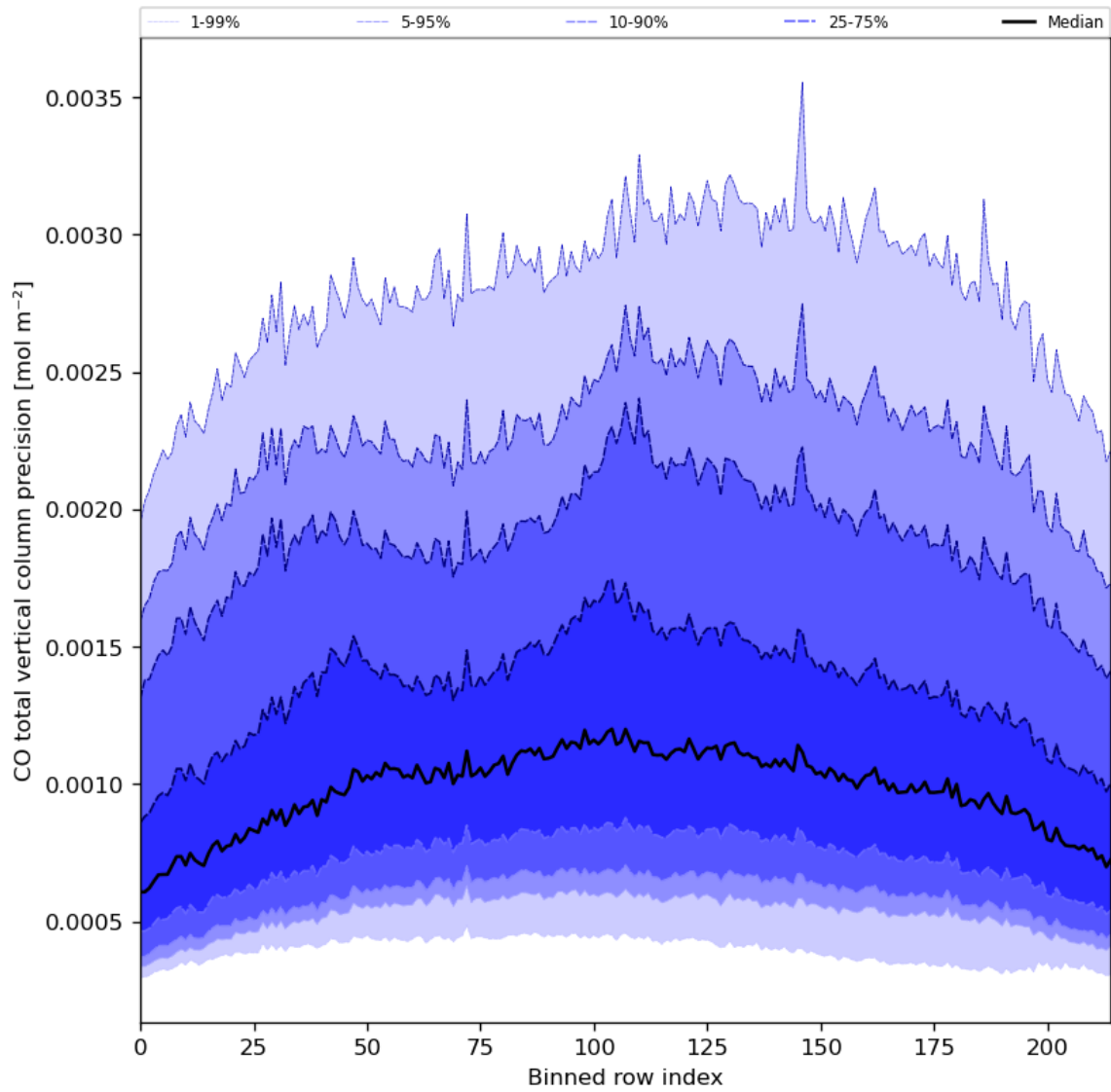
Figure 28: Along track statistics of “CO total vertical column precision” for 2024-03-26 to 2024-03-28
