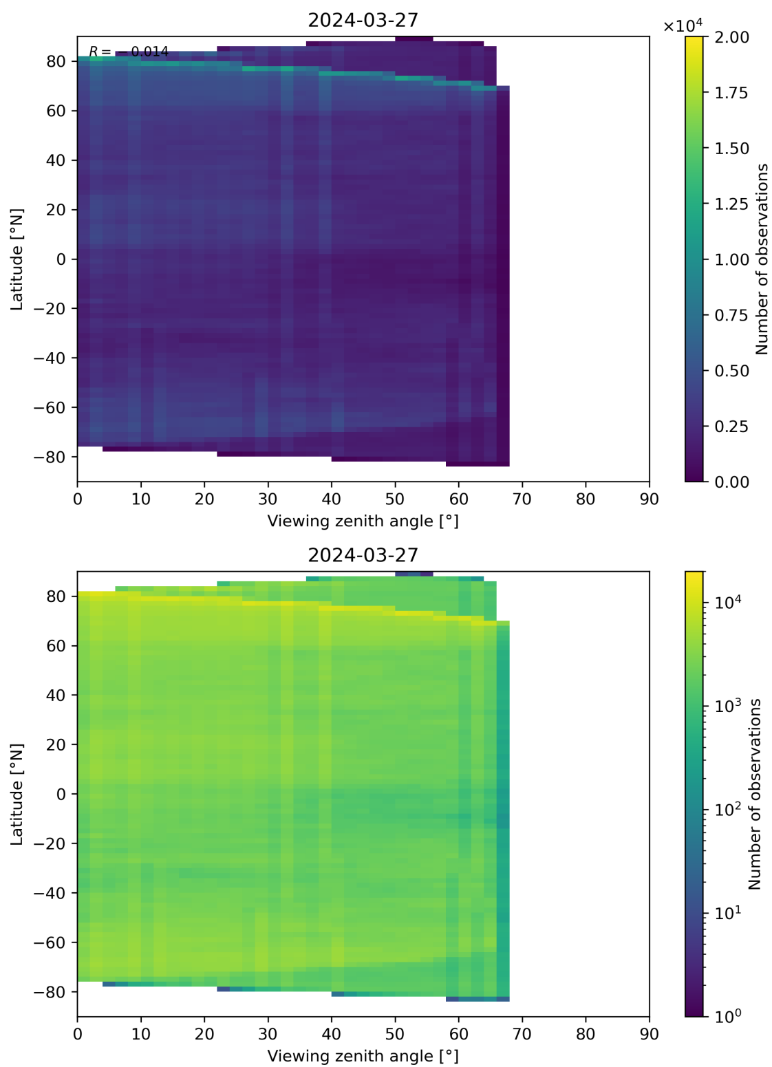
Figure 74: Scatter density plot of “Viewing zenith angle” against “Latitude” for 2024-03-26 to 2024-03-28.
