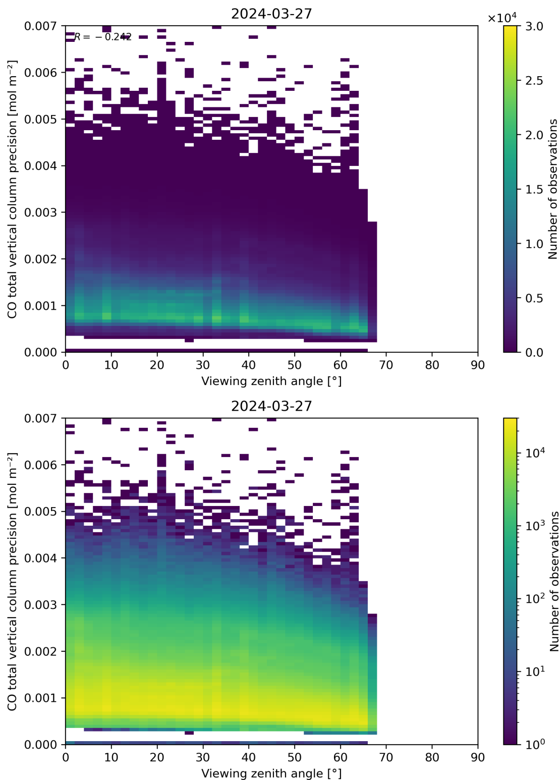
Figure 71: Scatter density plot of “Viewing zenith angle” against “CO total vertical column precision” for 2024-03-26 to 2024-03-28.
