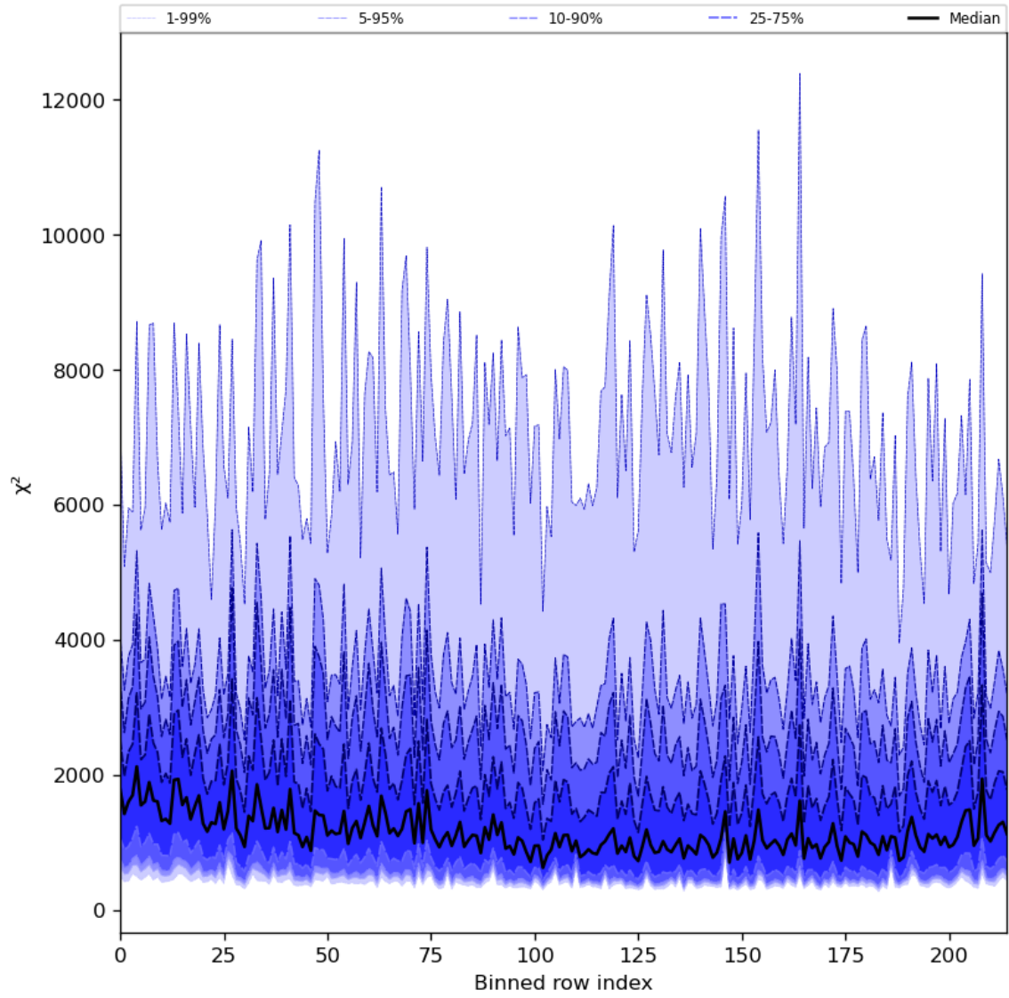
Figure 30: Along track statistics of “ \chi^2 ” for 2024-03-26 to 2024-03-28
