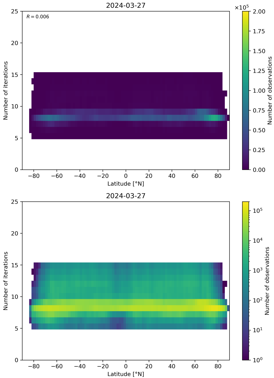
Figure 56: Scatter density plot of “Latitude” against “Number of iterations” for 2024-03-26 to 2024-03-28.
