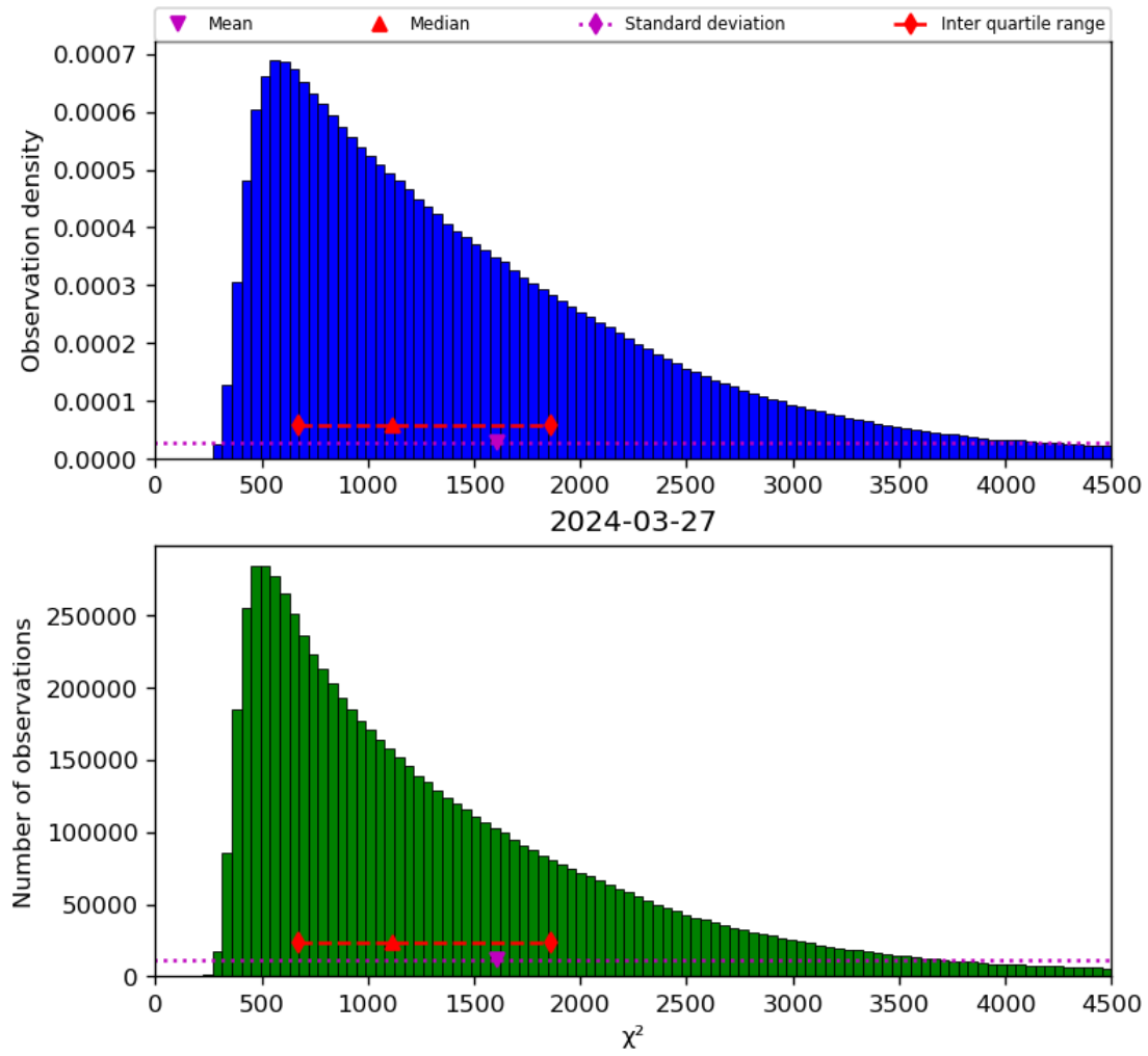
Figure 22: Histogram of " \chi^2 " for 2024-03-26 to 2024-03-28
