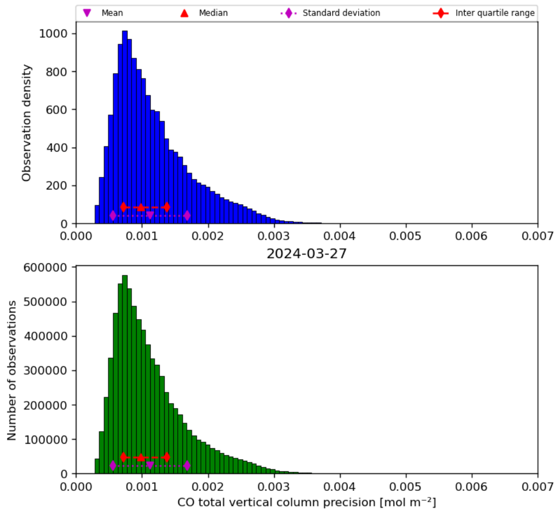
Figure 20: Histogram of “CO total vertical column precision” for 2024-03-26 to 2024-03-28
