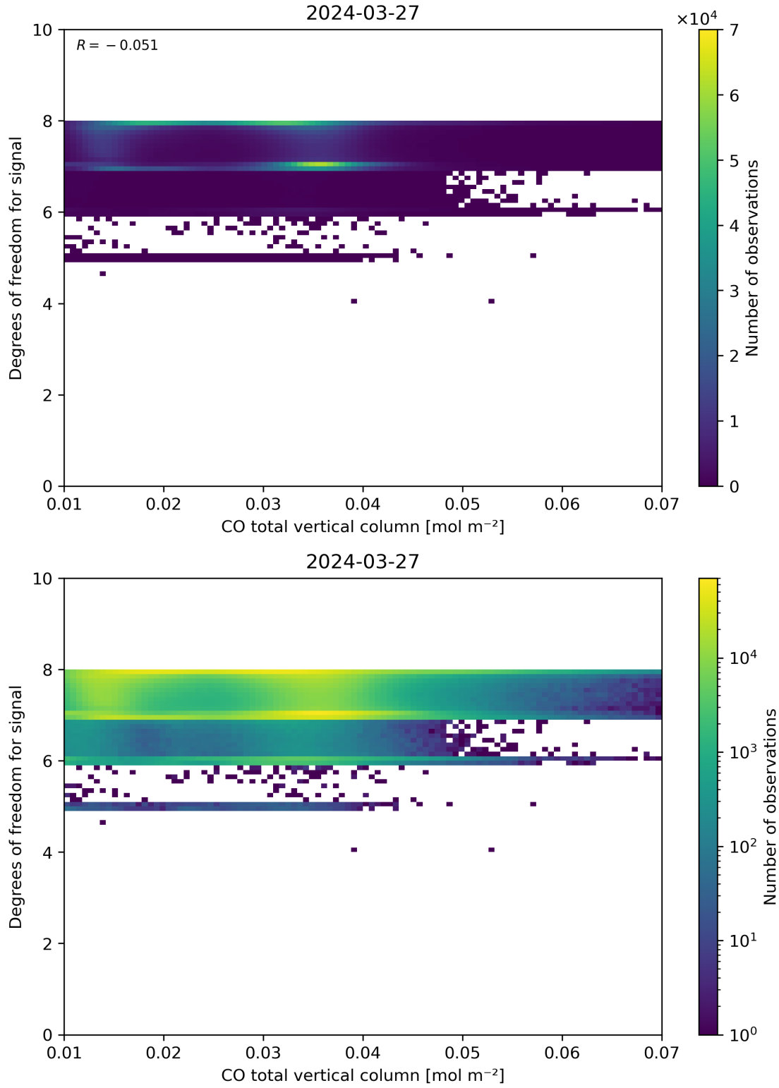
Figure 41: Scatter density plot of “CO total vertical column” against “Degrees of freedom for signal” for 2024-03-26 to 2024-03-28.
