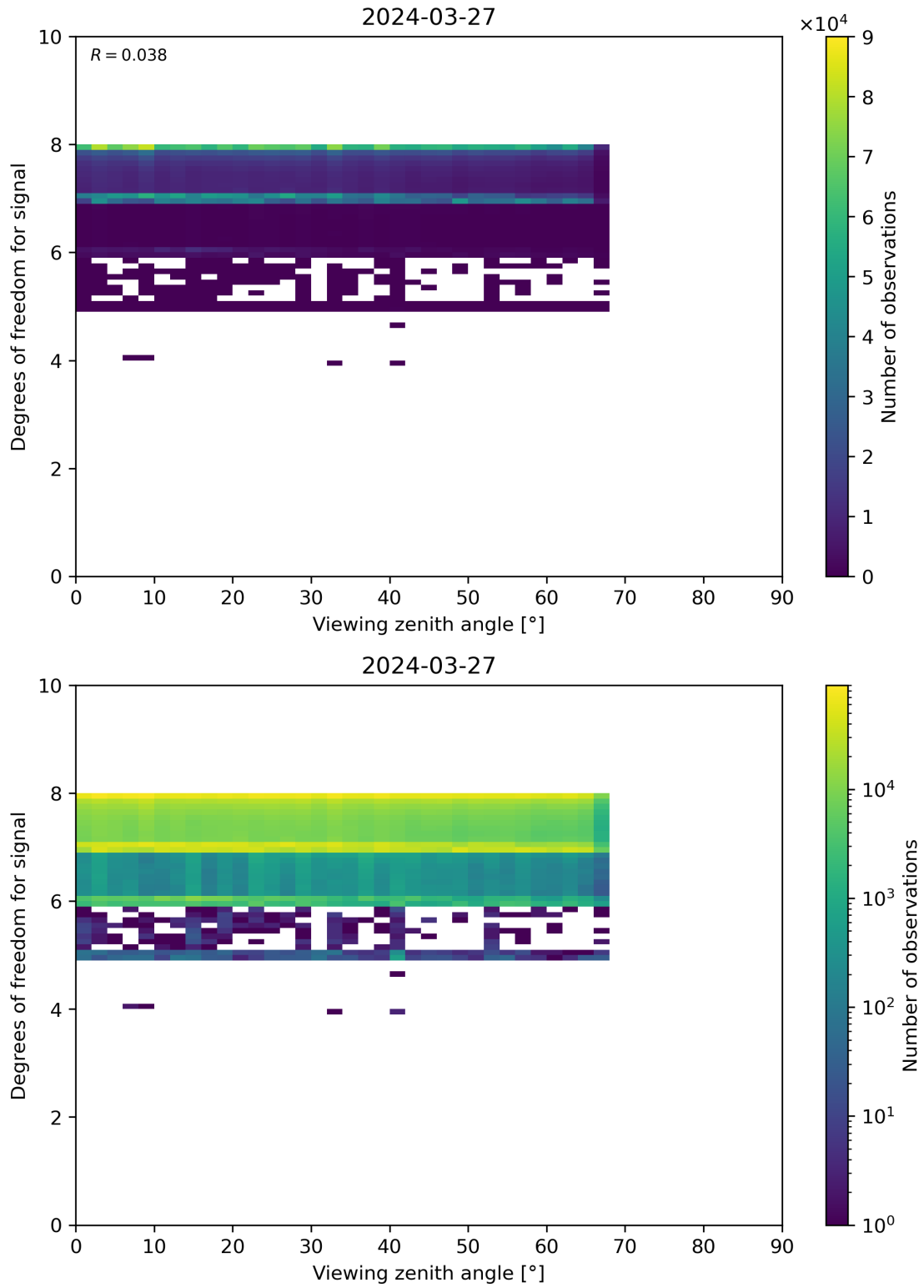
Figure 73: Scatter density plot of “Viewing zenith angle” against “Degrees of freedom for signal” for 2024-03-26 to 2024-03-28.
