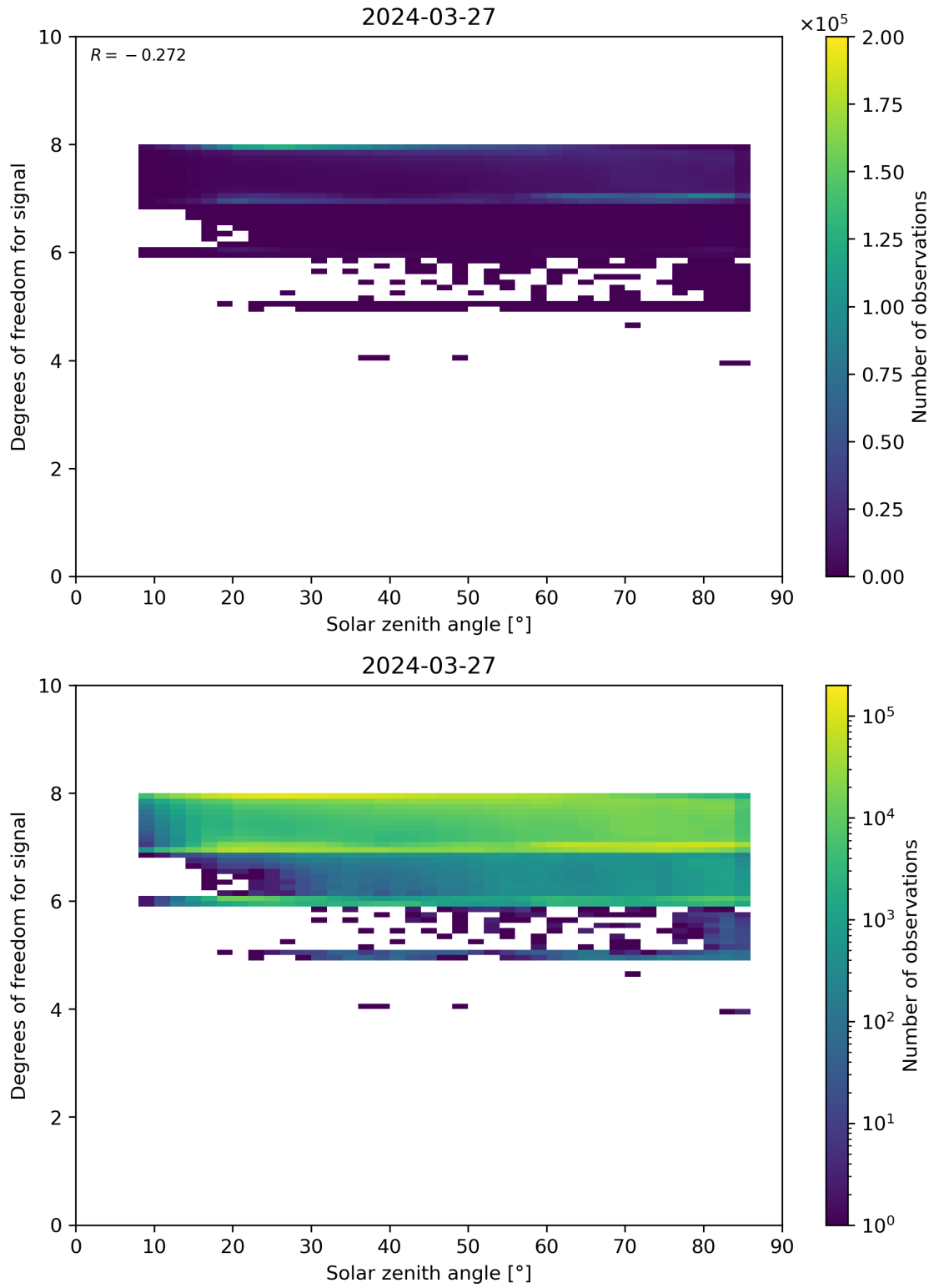
Figure 65: Scatter density plot of “Solar zenith angle” against “Degrees of freedom for signal” for 2024-03-26 to 2024-03-28.
