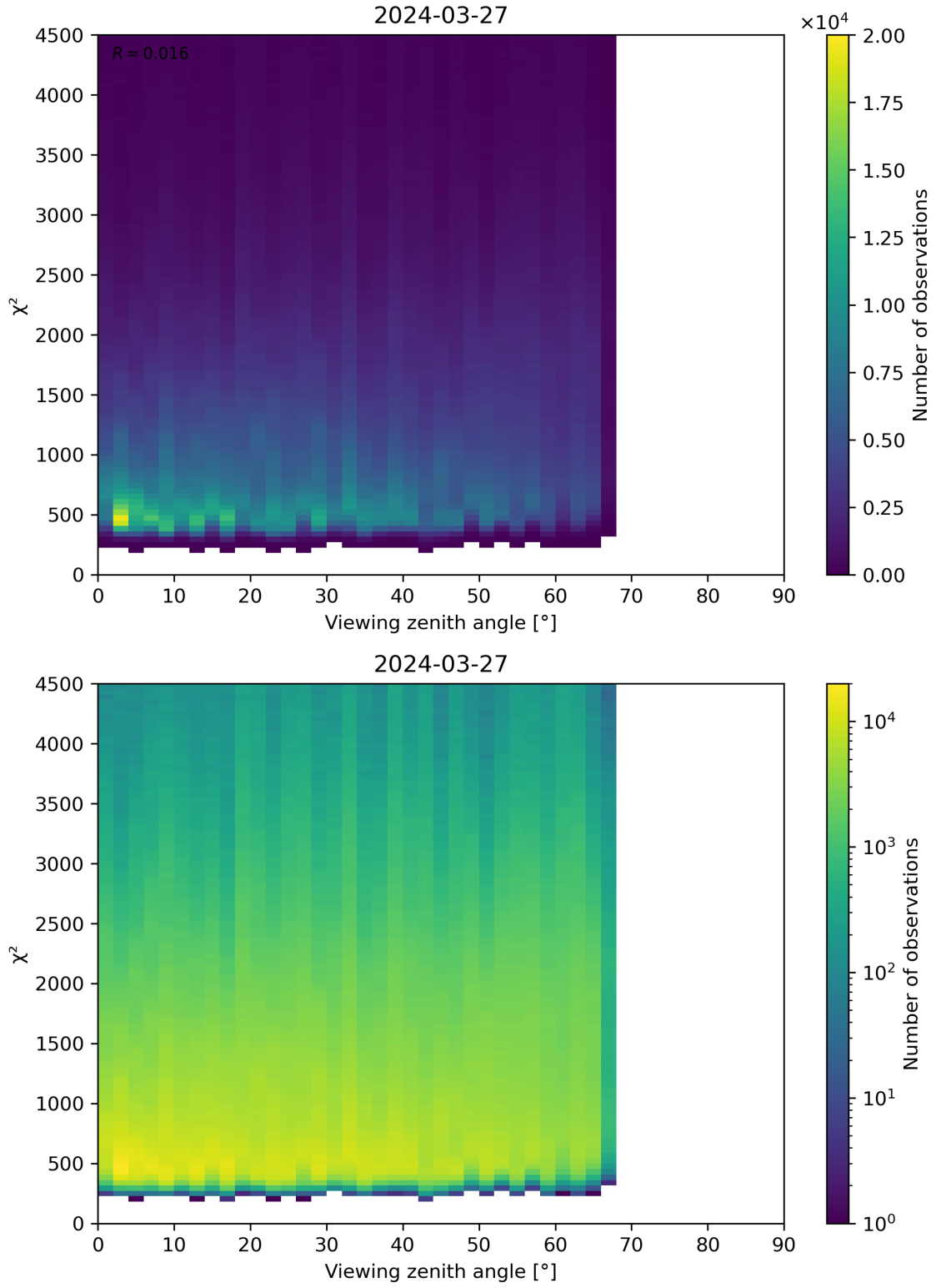
Figure 72: Scatter density plot of “Viewing zenith angle” against “ \chi^2 ” for 2024-03-26 to 2024-03-28.
