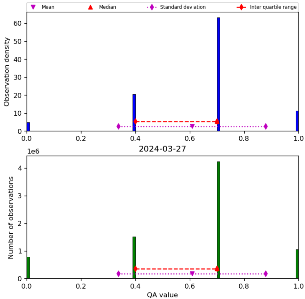
Figure 17: Histogram of “QA value” for 2024-03-26 to 2024-03-28
