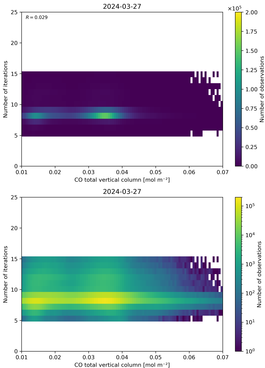
Figure 42: Scatter density plot of “CO total vertical column” against “Number of iterations” for 2024-03-26 to 2024-03-28.
