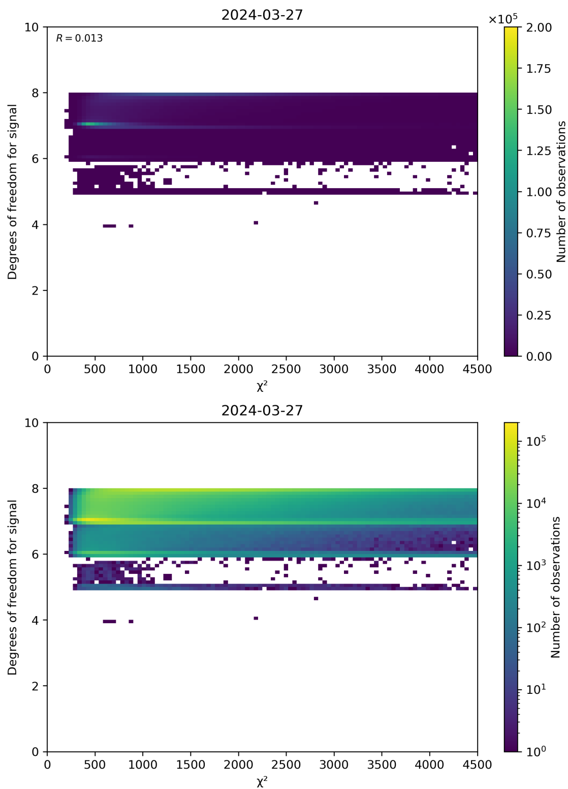
Figure 48: Scatter density plot of “ \chi^2 ” against “Degrees of freedom for signal” for 2024-03-26 to 2024-03-28.
