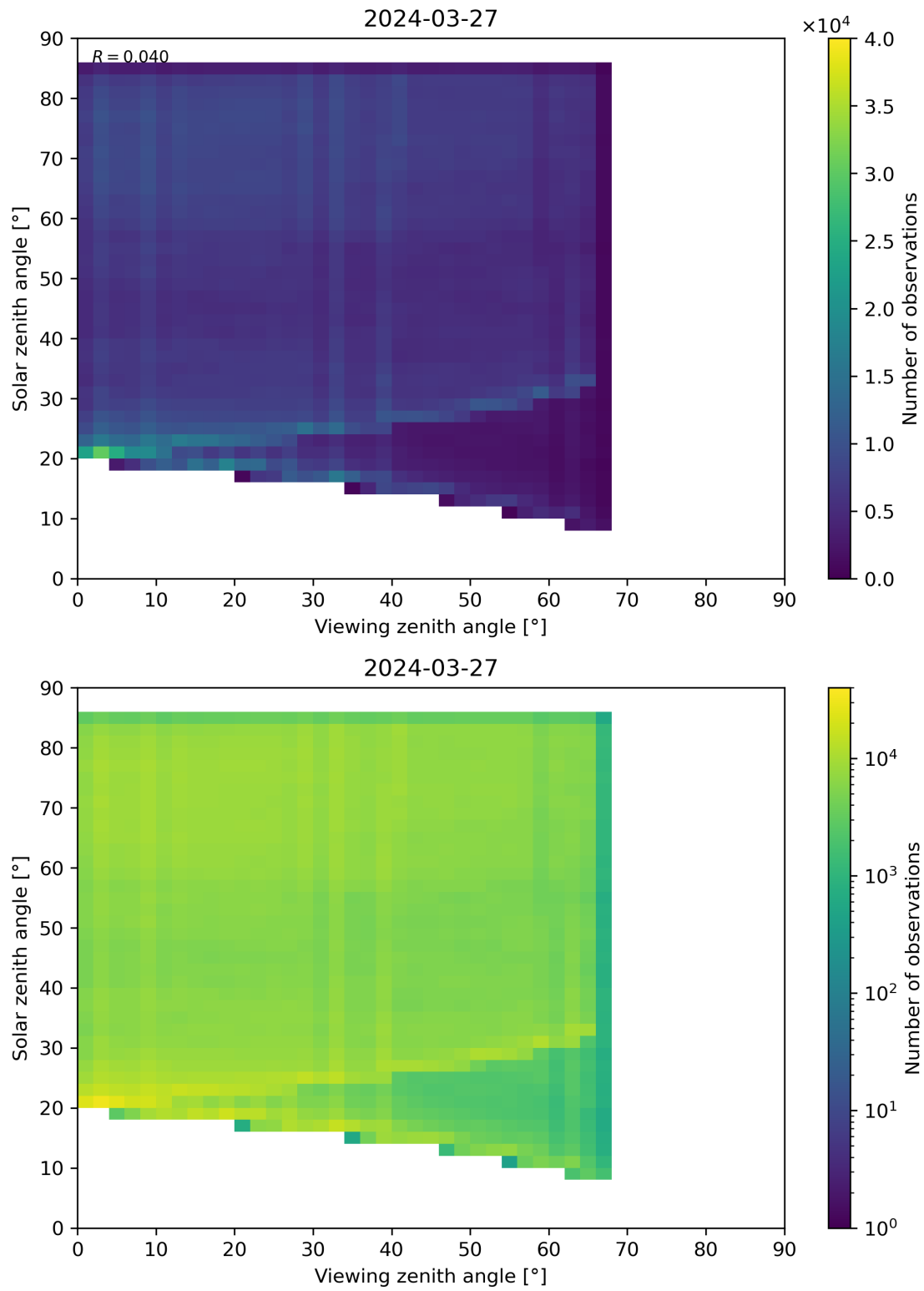
Figure 77: Scatter density plot of “Viewing zenith angle” against “Solar zenith angle” for 2024-03-26 to 2024-03-28.
