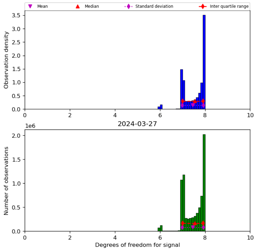
Figure 23: Histogram of “Degrees of freedom for signal” for 2024-03-26 to 2024-03-28
