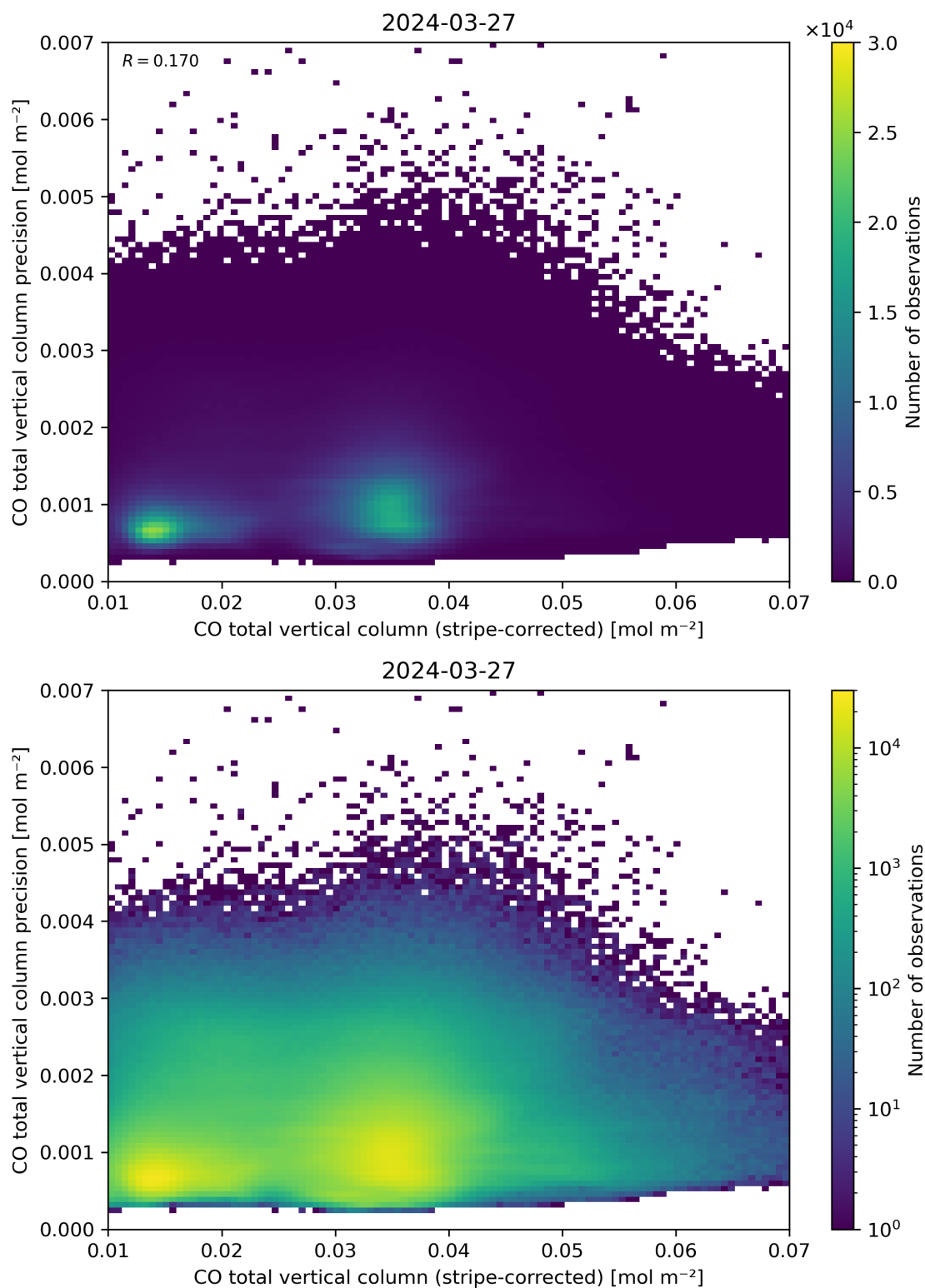
Figure 36: Scatter density plot of “CO total vertical column (stripe-corrected)” against “CO total vertical column precision” for 2024-03-26 to 2024-03-28.
