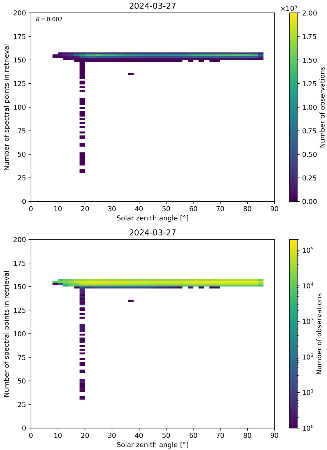
Figure 68: Scatter density plot of “Solar zenith angle” against “Number of spectral points in retrieval” for 2024-03-26 to 2024-03-28.
