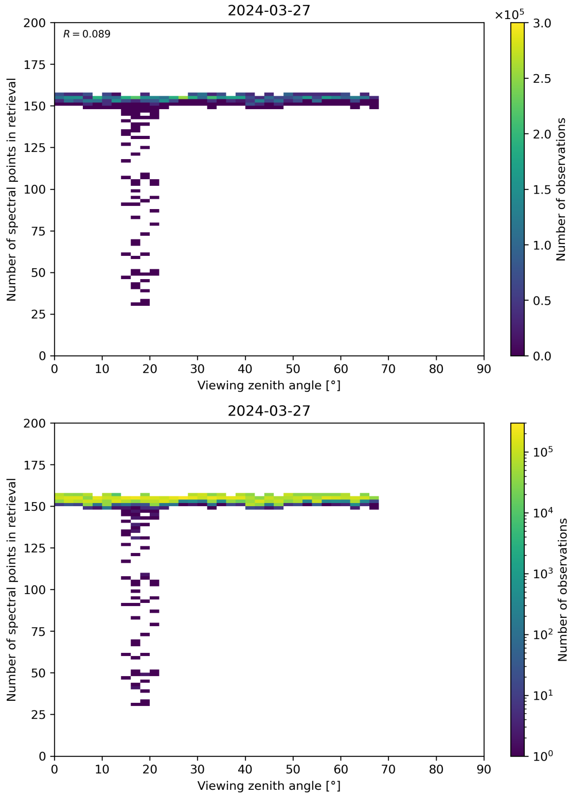
Figure 76: Scatter density plot of “Viewing zenith angle” against “Number of spectral points in retrieval” for 2024-03-26 to 2024-03-28.
