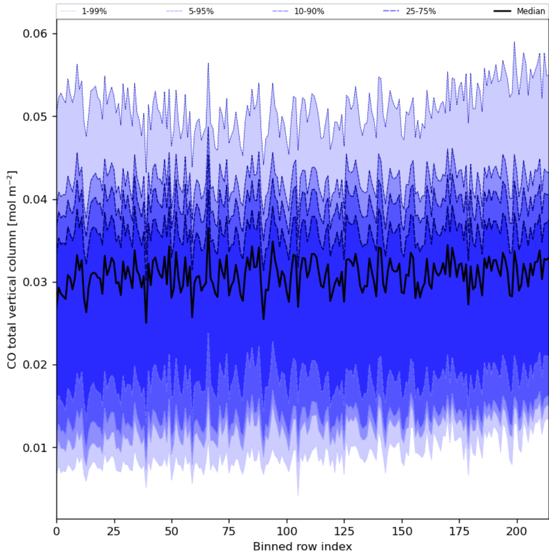
Figure 26: Along track statistics of "CO total vertical column" for 2024-03-26 to 2024-03-28
