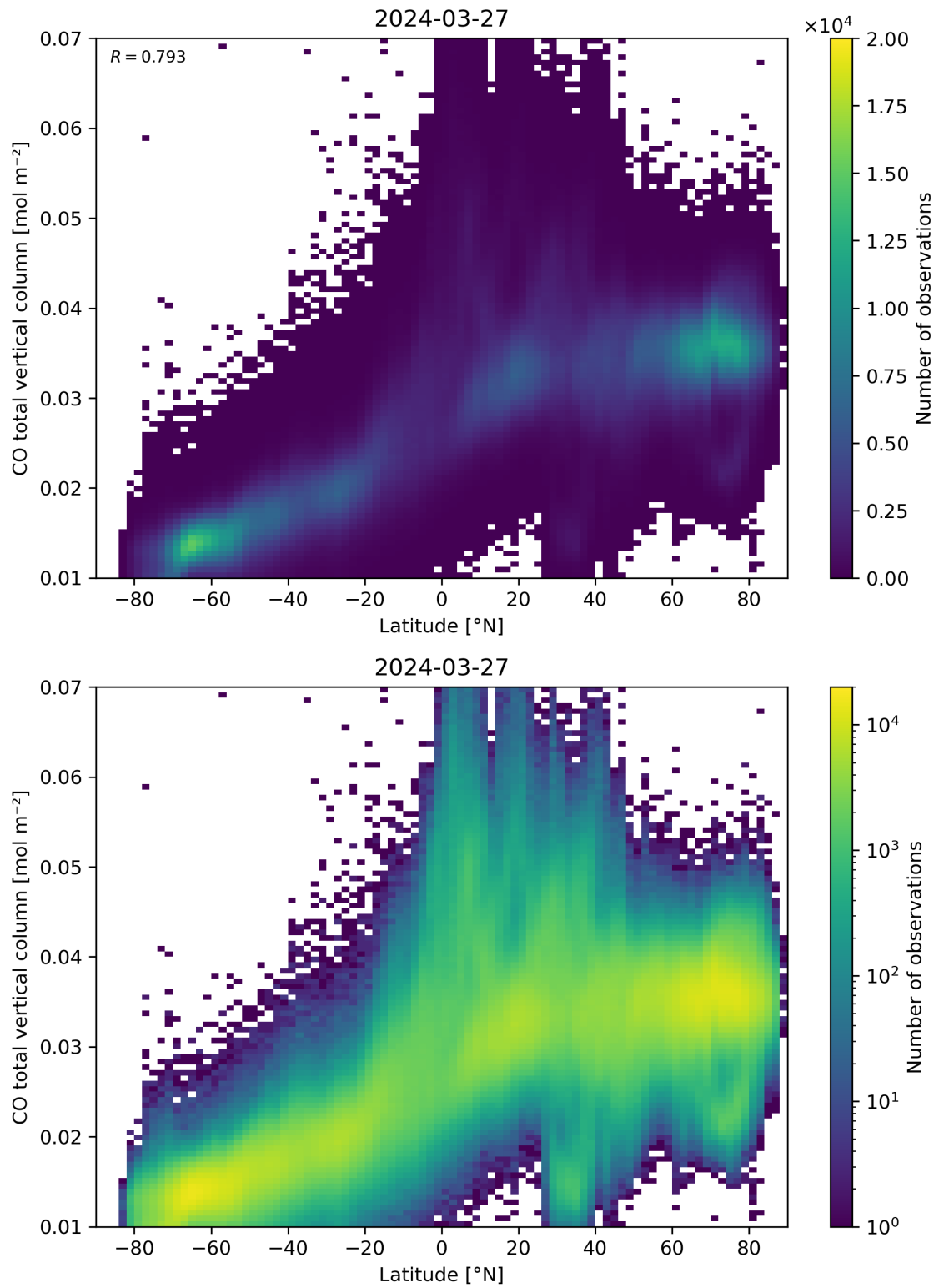
Figure 51: Scatter density plot of “Latitude” against “CO total vertical column” for 2024-03-26 to 2024-03-28.
