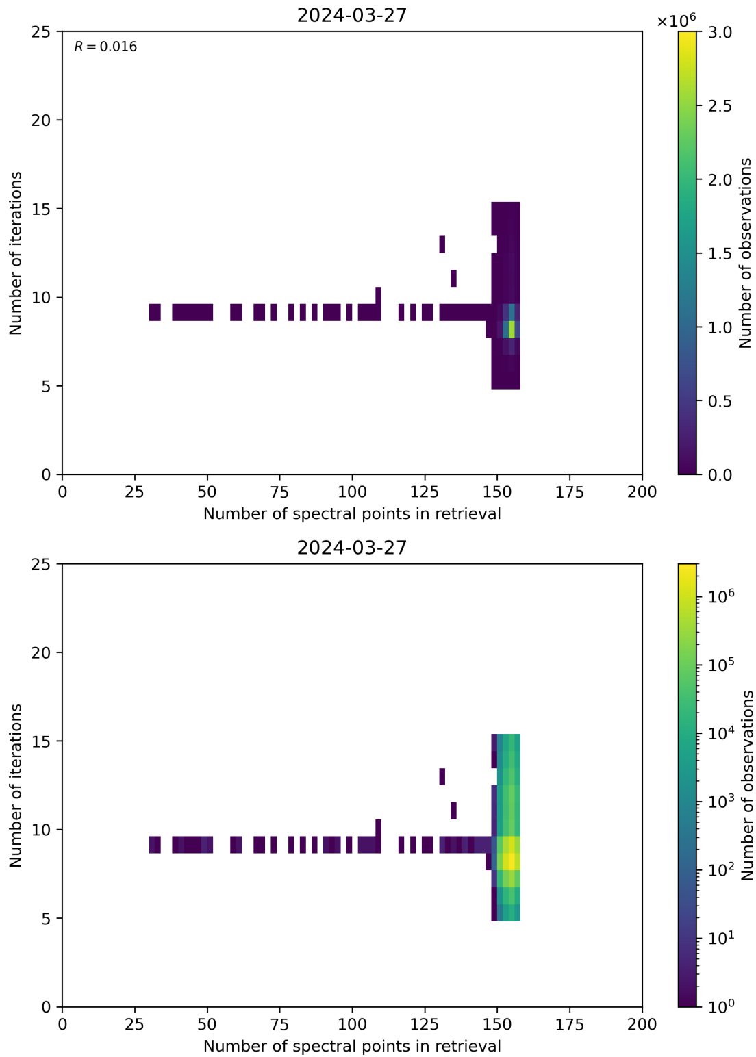
Figure 60: Scatter density plot of “Number of spectral points in retrieval” against “Number of iterations” for 2024-03-26 to 2024-03-28.
