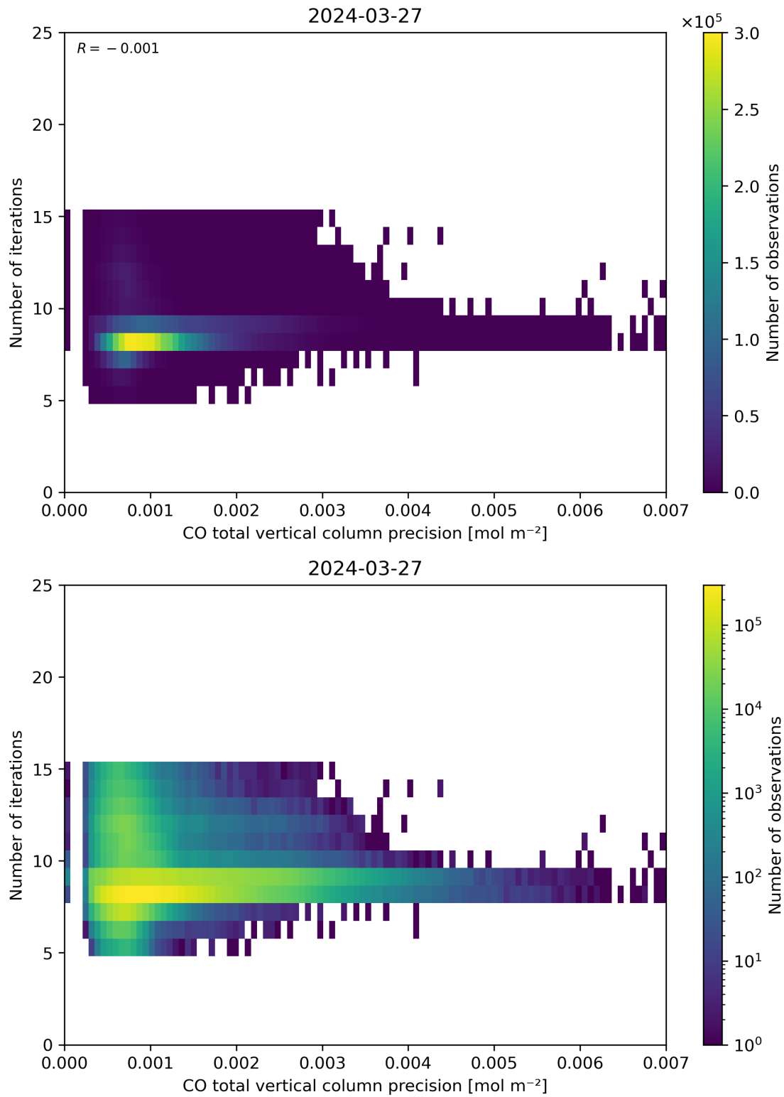
Figure 46: Scatter density plot of “CO total vertical column precision” against “Number of iterations” for 2024-03-26 to 2024-03-28.
