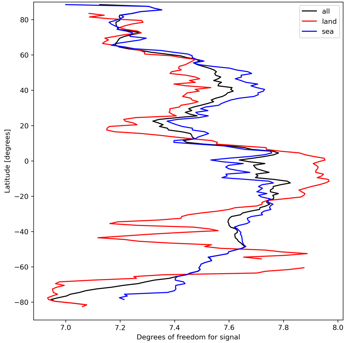
Figure 15: Zonal average of “Degrees of freedom for signal” for 2024-03-26 to 2024-03-28.
