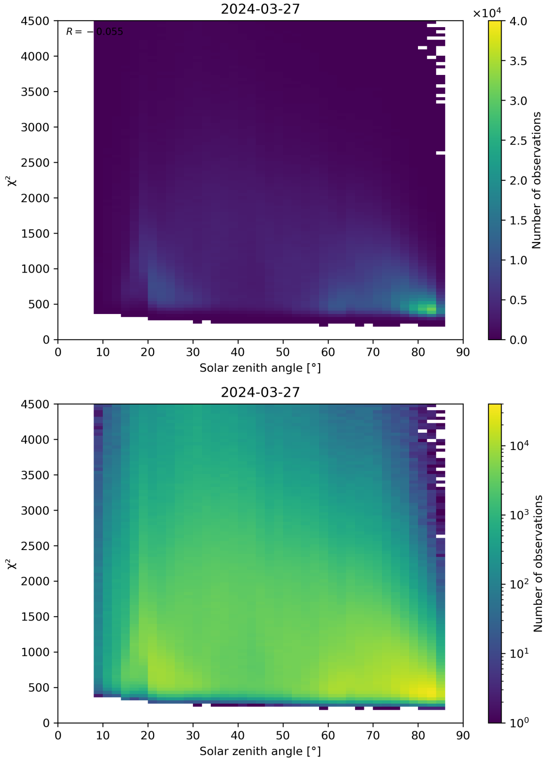
Figure 64: Scatter density plot of “Solar zenith angle” against “ \chi^2 ” for 2024-03-26 to 2024-03-28.
