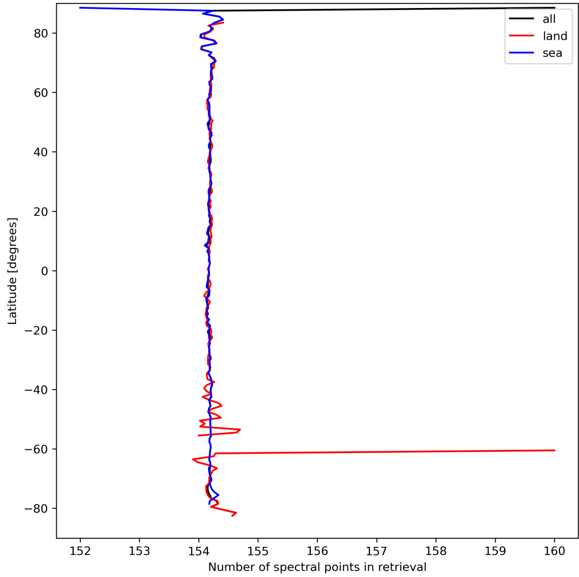
Figure 13: Zonal average of “Number of spectral points in retrieval” for 2024-03-26 to 2024-03-28.
