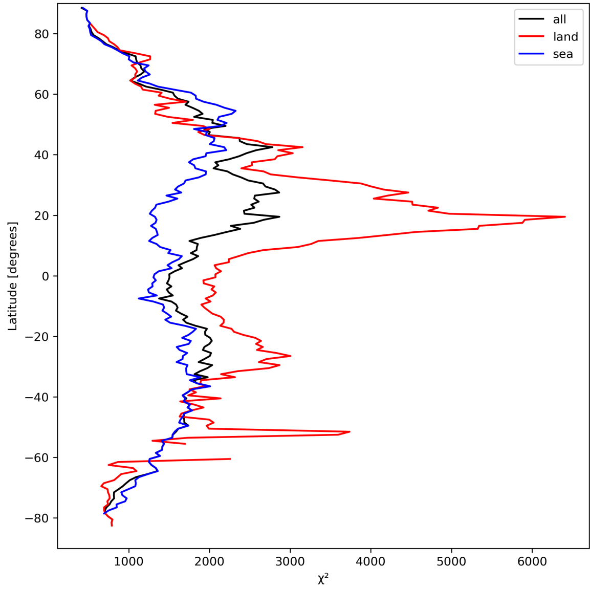
Figure 14: Zonal average of “ \chi^2 ” for 2024-03-26 to 2024-03-28.
