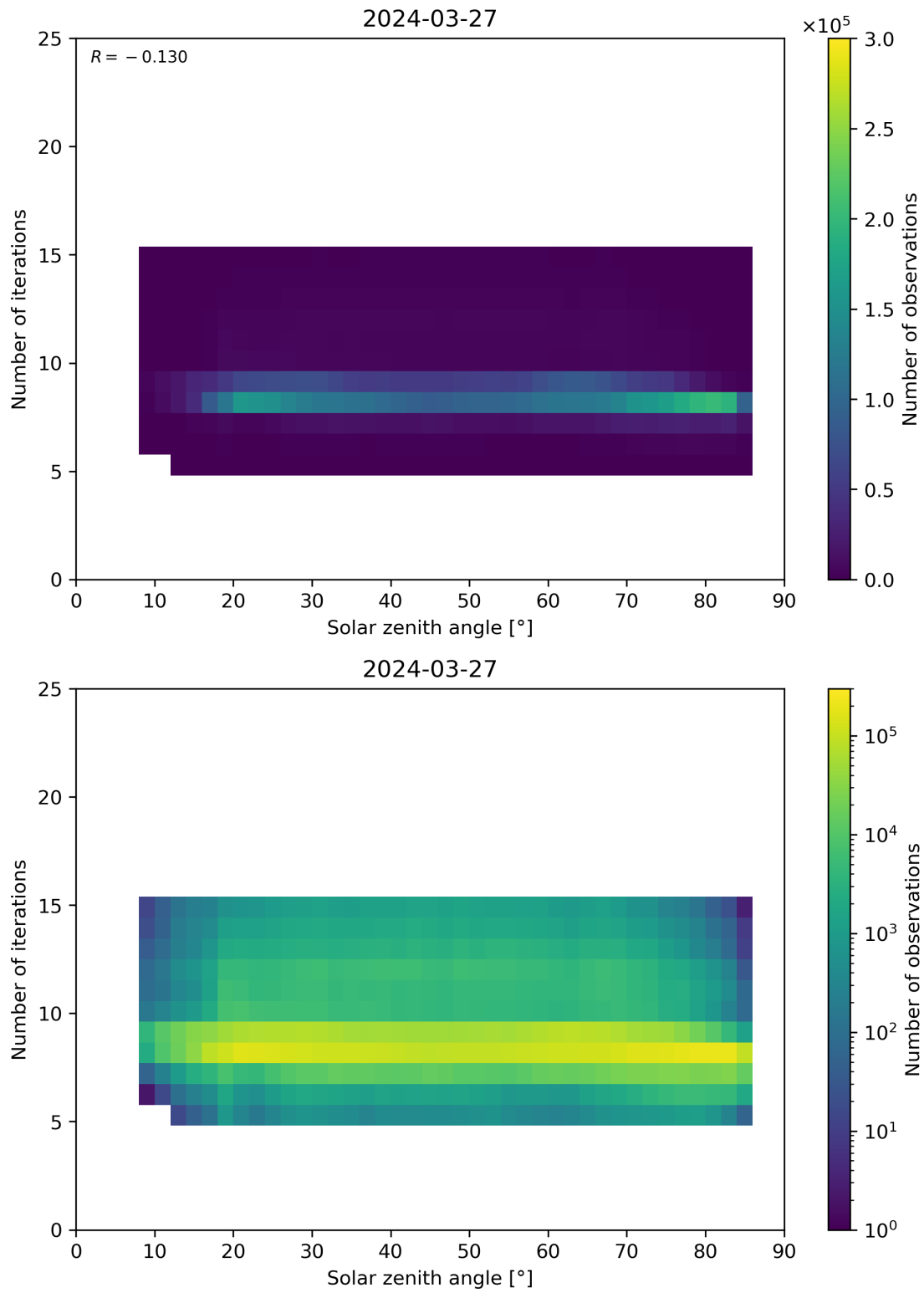
Figure 67: Scatter density plot of “Solar zenith angle” against “Number of iterations” for 2024-03-26 to 2024-03-28.
