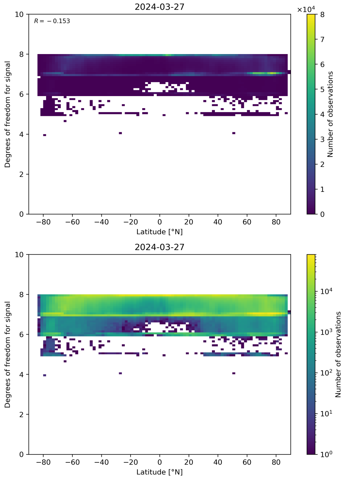
Figure 55: Scatter density plot of “Latitude” against “Degrees of freedom for signal” for 2024-03-26 to 2024-03-28.
