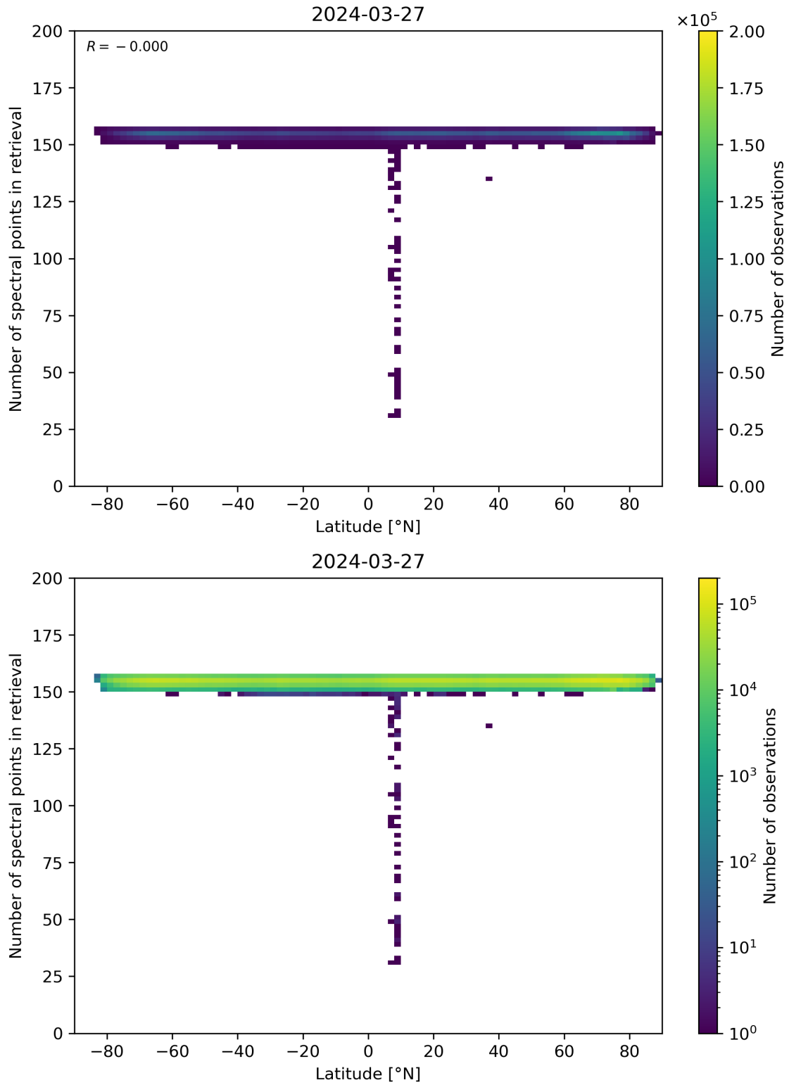
Figure 57: Scatter density plot of “Latitude” against “Number of spectral points in retrieval” for 2024-03-26 to 2024-03-28.
