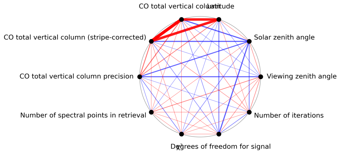
Figure 1: Map of correlation graph for 2024-03-26 to 2024-03-28.
