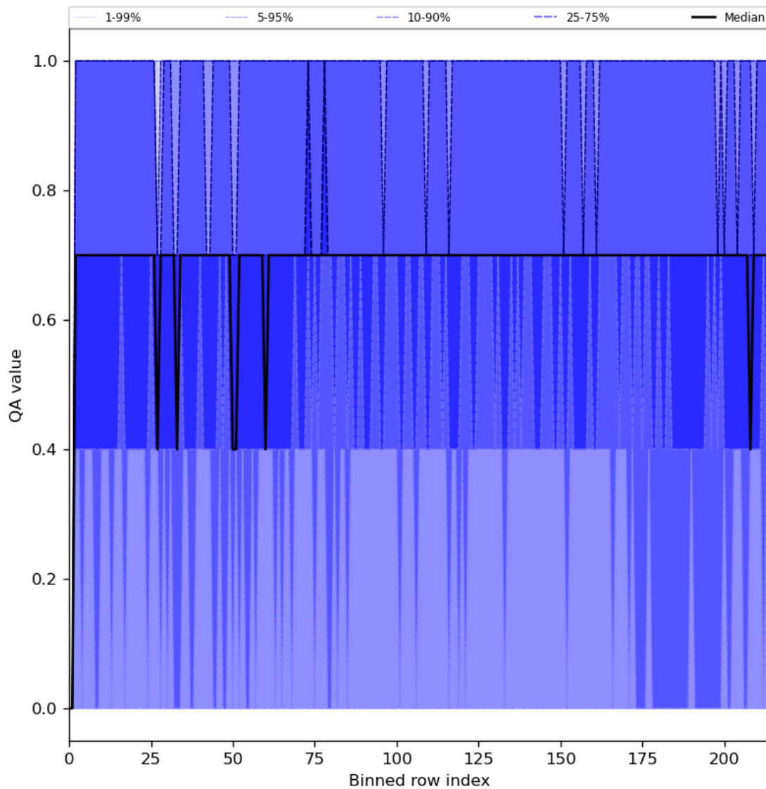
Figure 25: Along track statistics of “QA value” for 2024-03-26 to 2024-03-28
