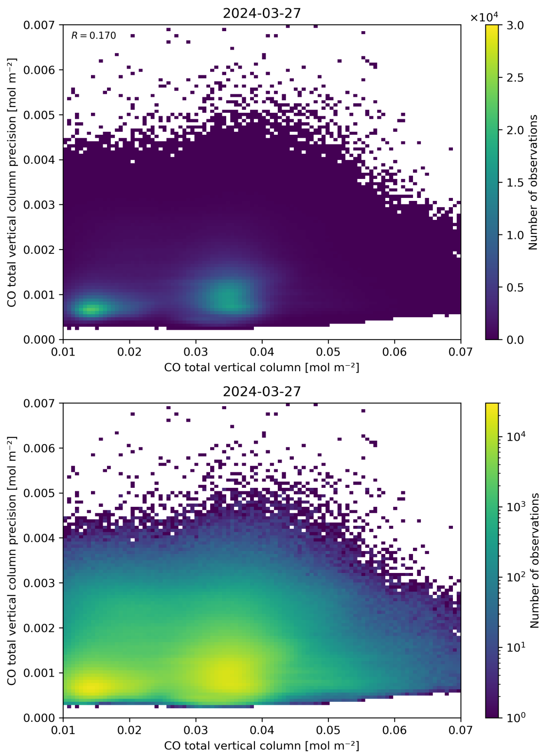
Figure 34: Scatter density plot of “CO total vertical column” against “CO total vertical column precision” for 2024-03-26 to 2024-03-28.
