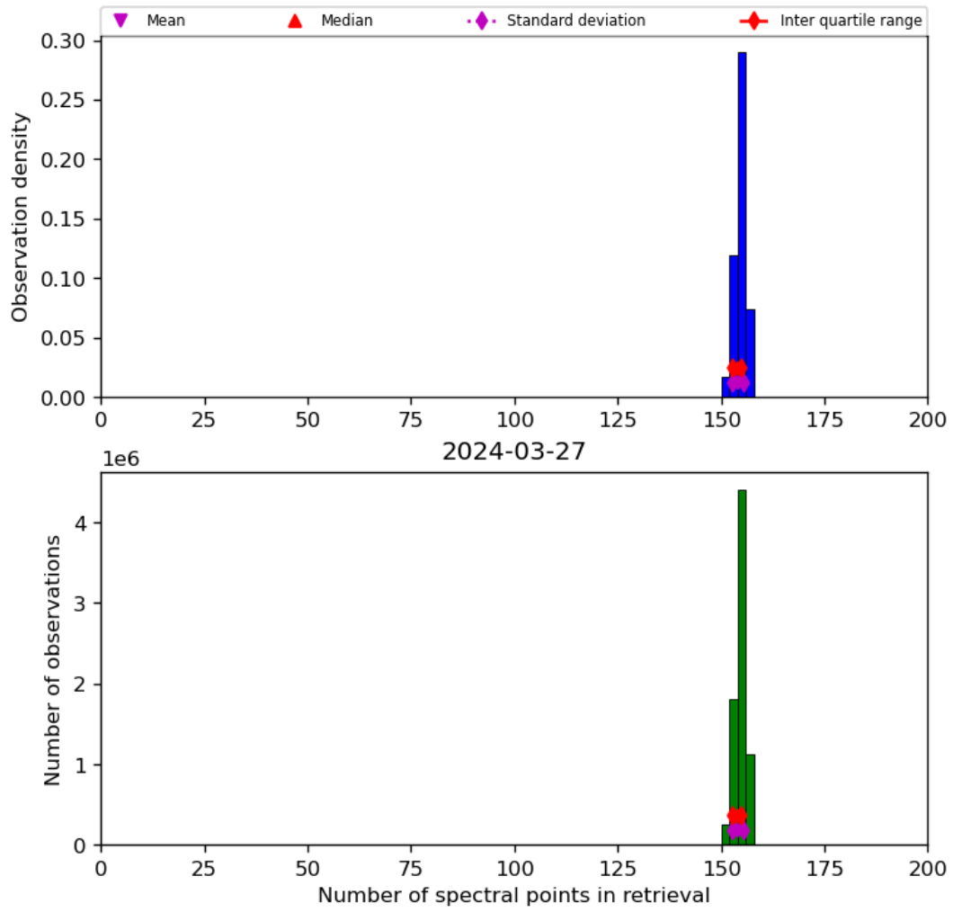
Figure 21: Histogram of “Number of spectral points in retrieval” for 2024-03-26 to 2024-03-28
