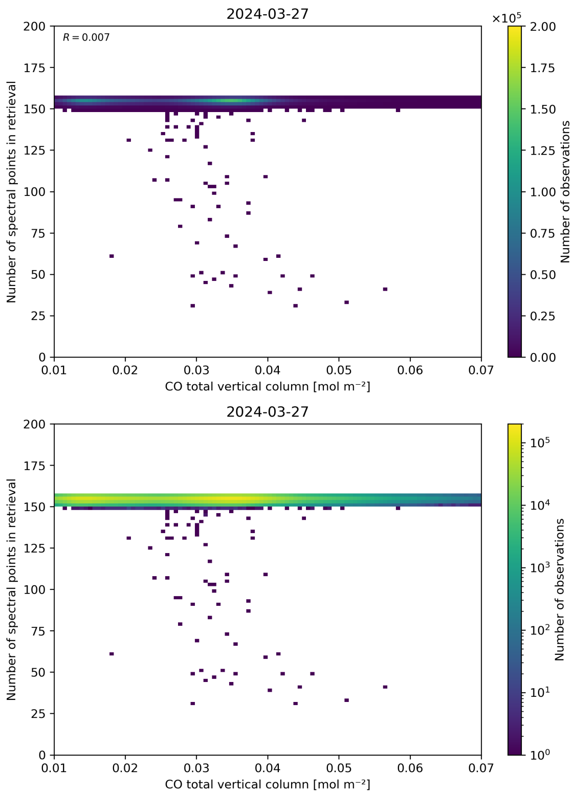
Figure 43: Scatter density plot of “CO total vertical column” against “Number of spectral points in retrieval” for 2024-03-26 to 2024-03-28.
