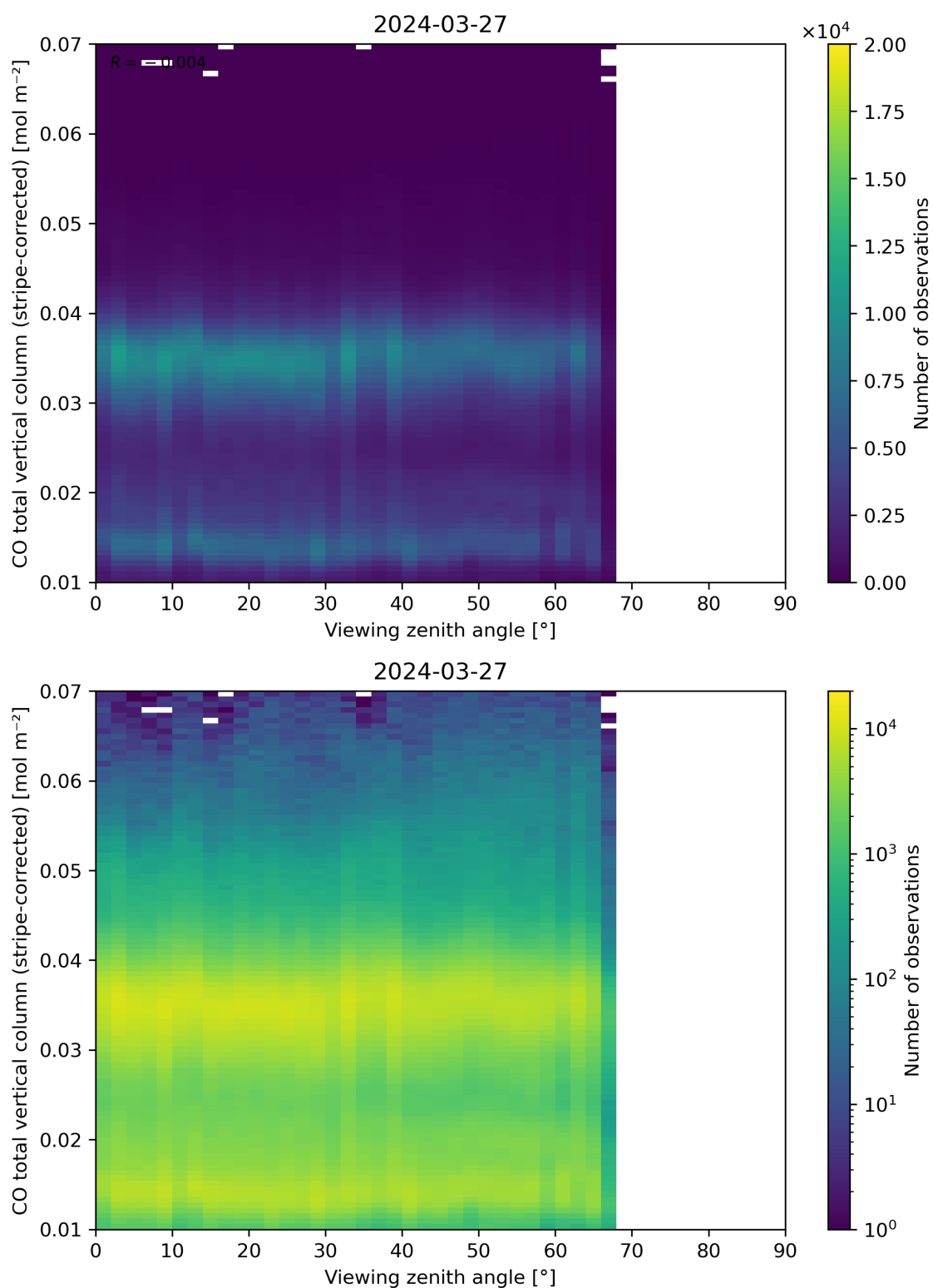
Figure 70: Scatter density plot of “Viewing zenith angle” against “CO total vertical column (stripe-corrected)” for 2024-03-26 to 2024-03-28.
