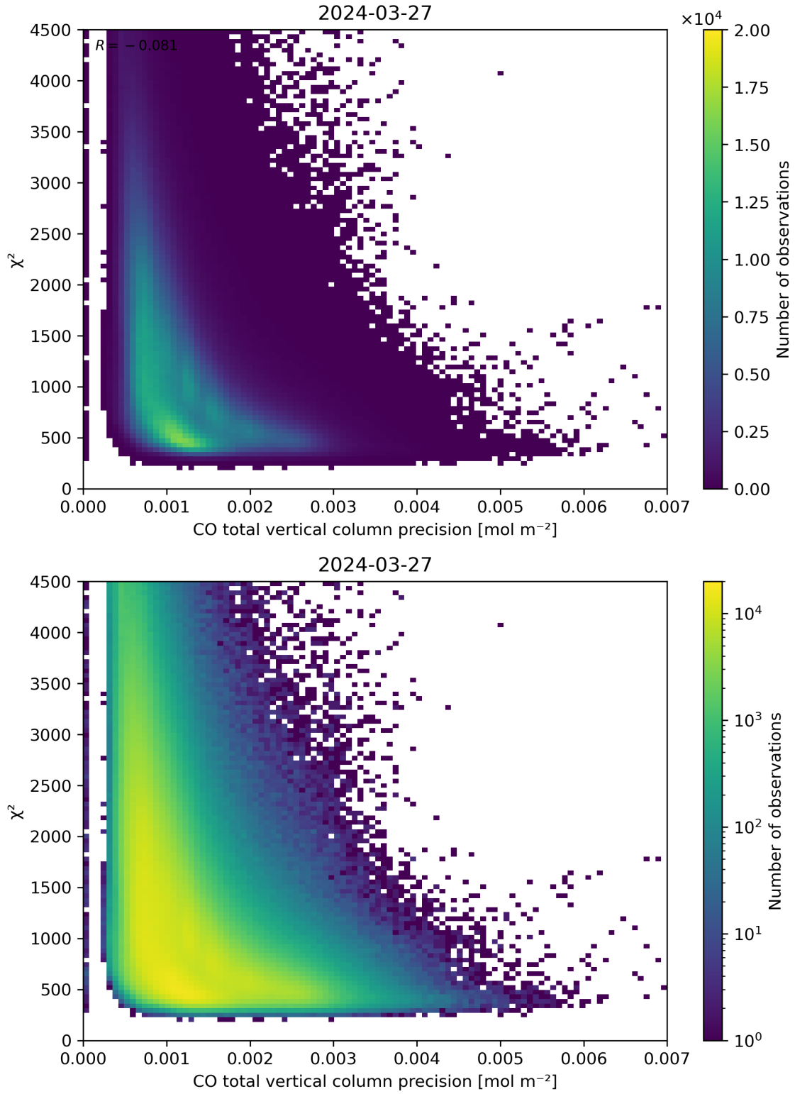
Figure 44: Scatter density plot of “CO total vertical column precision” against “ \chi^2 ” for 2024-03-26 to 2024-03-28.
