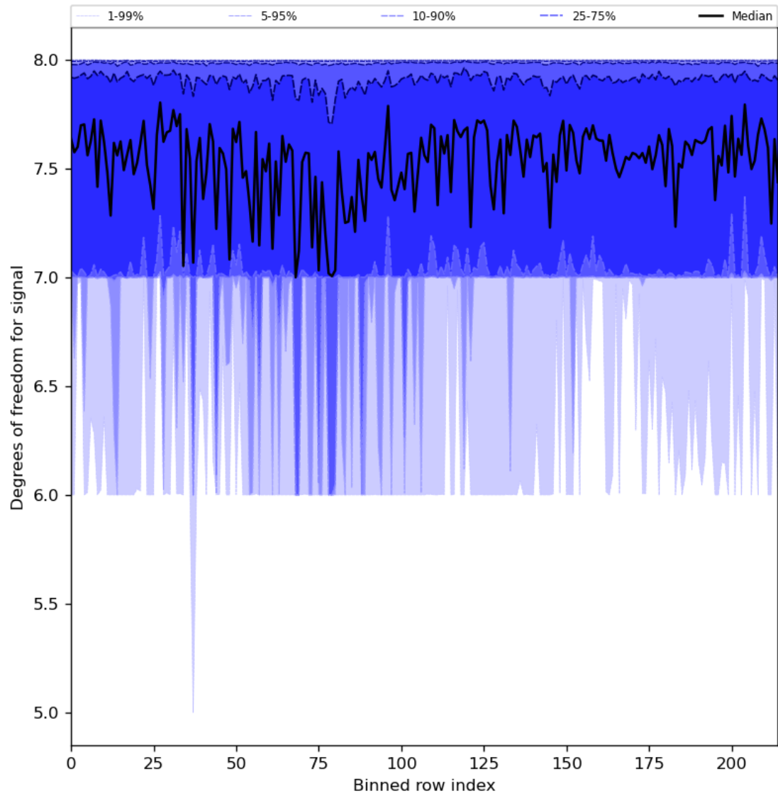
Figure 31: Along track statistics of “Degrees of freedom for signal” for 2024-03-26 to 2024-03-28
