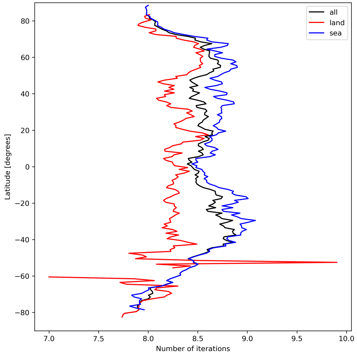
Figure 16: Zonal average of “Number of iterations” for 2024-03-26 to 2024-03-28.
