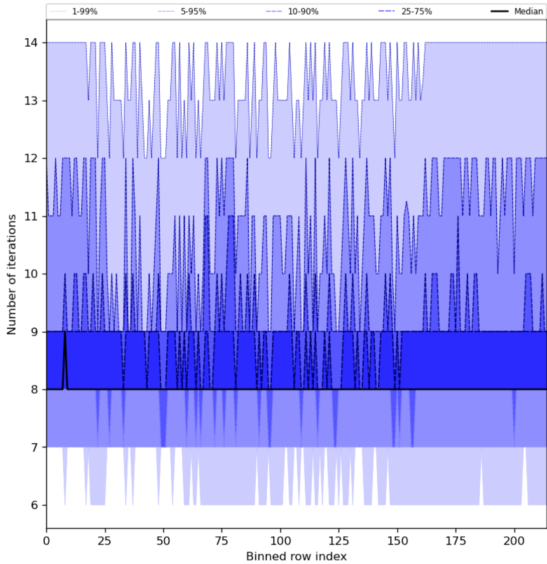
Figure 32: Along track statistics of “Number of iterations” for 2024-03-26 to 2024-03-28
