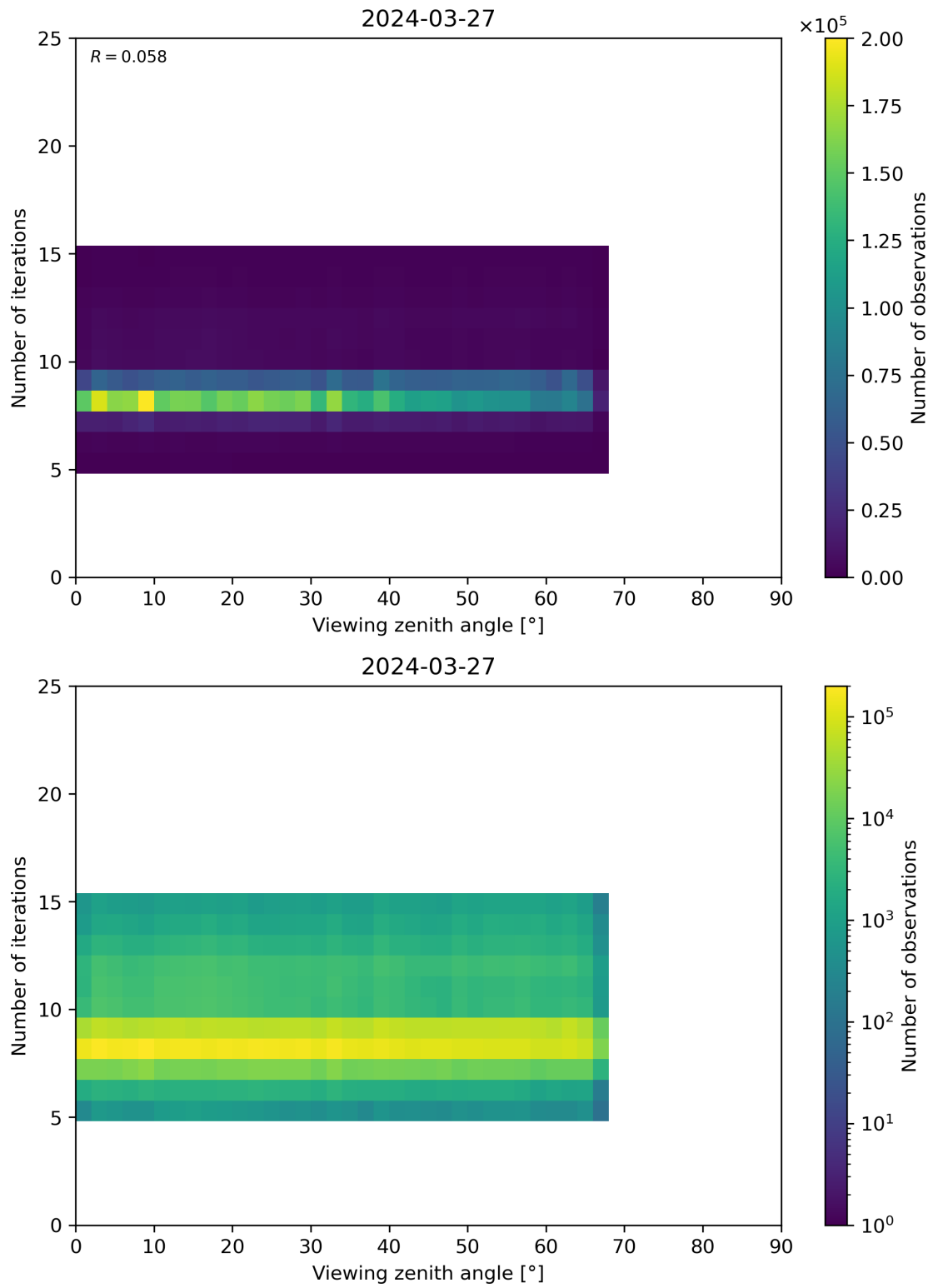
Figure 75: Scatter density plot of “Viewing zenith angle” against “Number of iterations” for 2024-03-26 to 2024-03-28.
