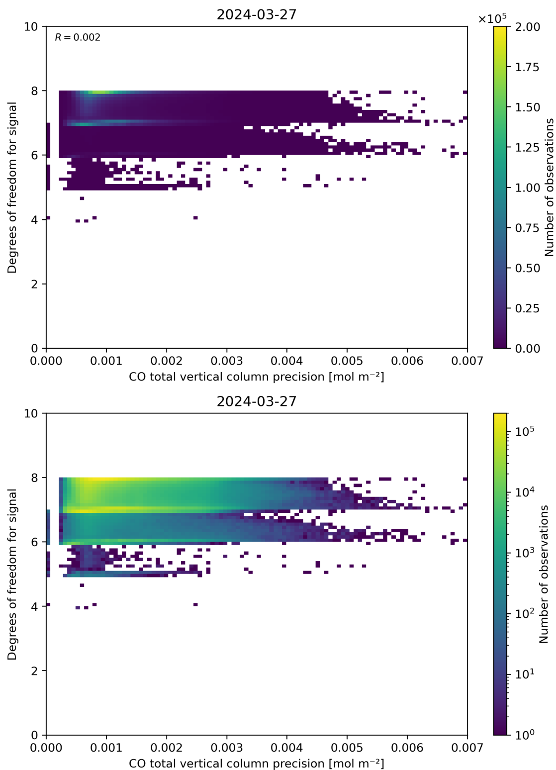
Figure 45: Scatter density plot of “CO total vertical column precision” against “Degrees of freedom for signal” for 2024-03-26 to 2024-03-28.
