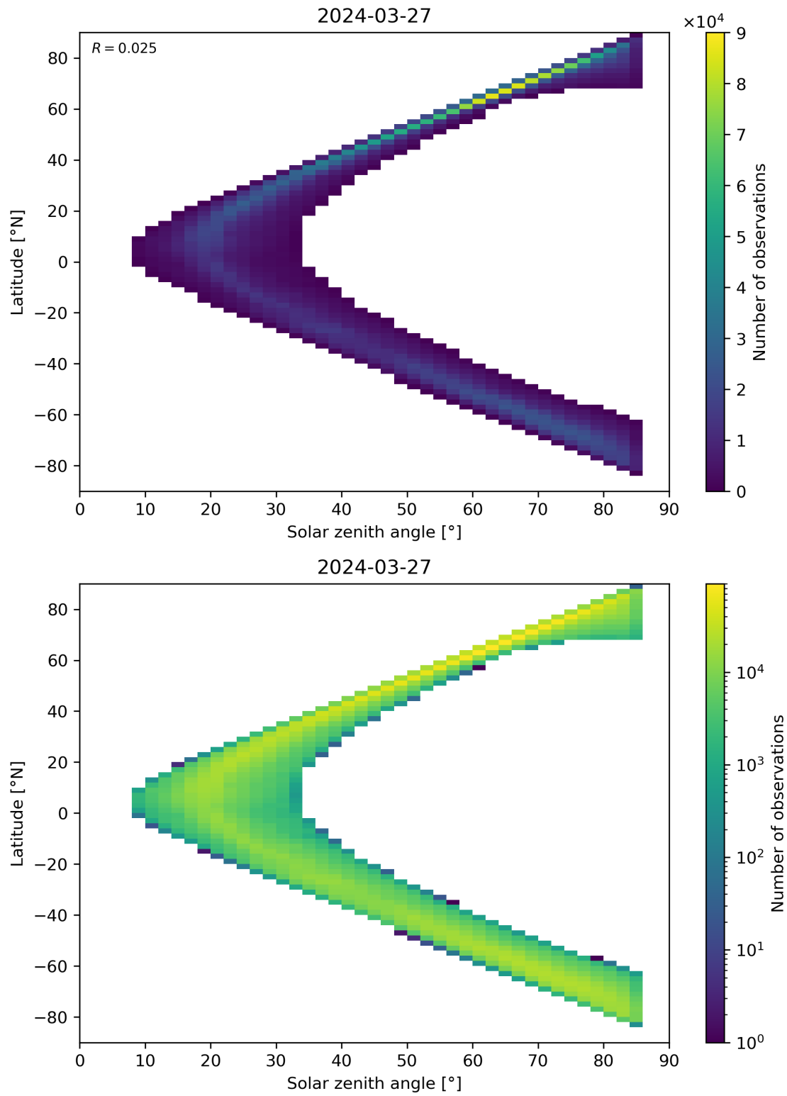
Figure 66: Scatter density plot of “Solar zenith angle” against “Latitude” for 2024-03-26 to 2024-03-28.
