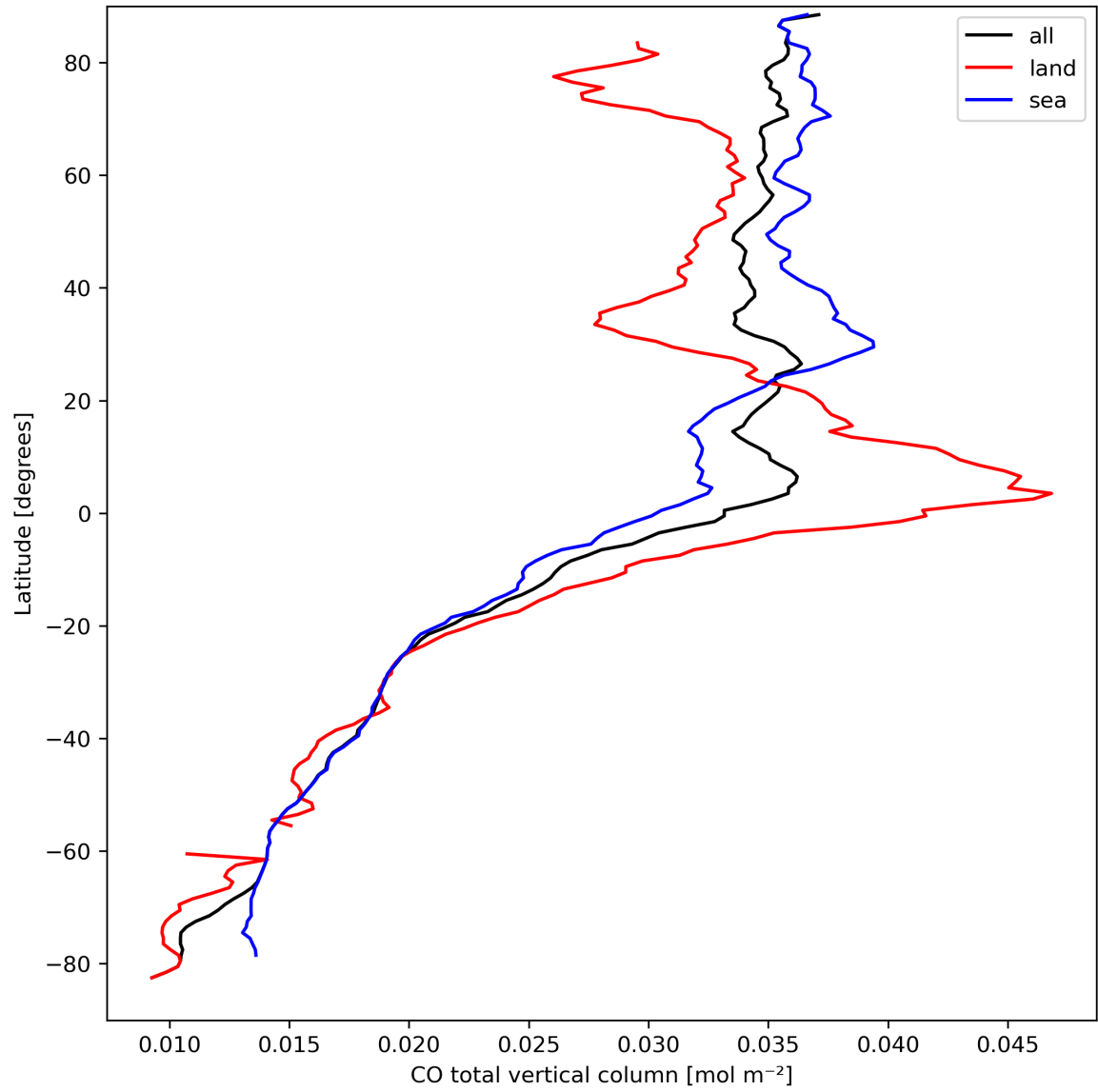
Figure 10: Zonal average of “CO total vertical column” for 2024-03-26 to 2024-03-28.
