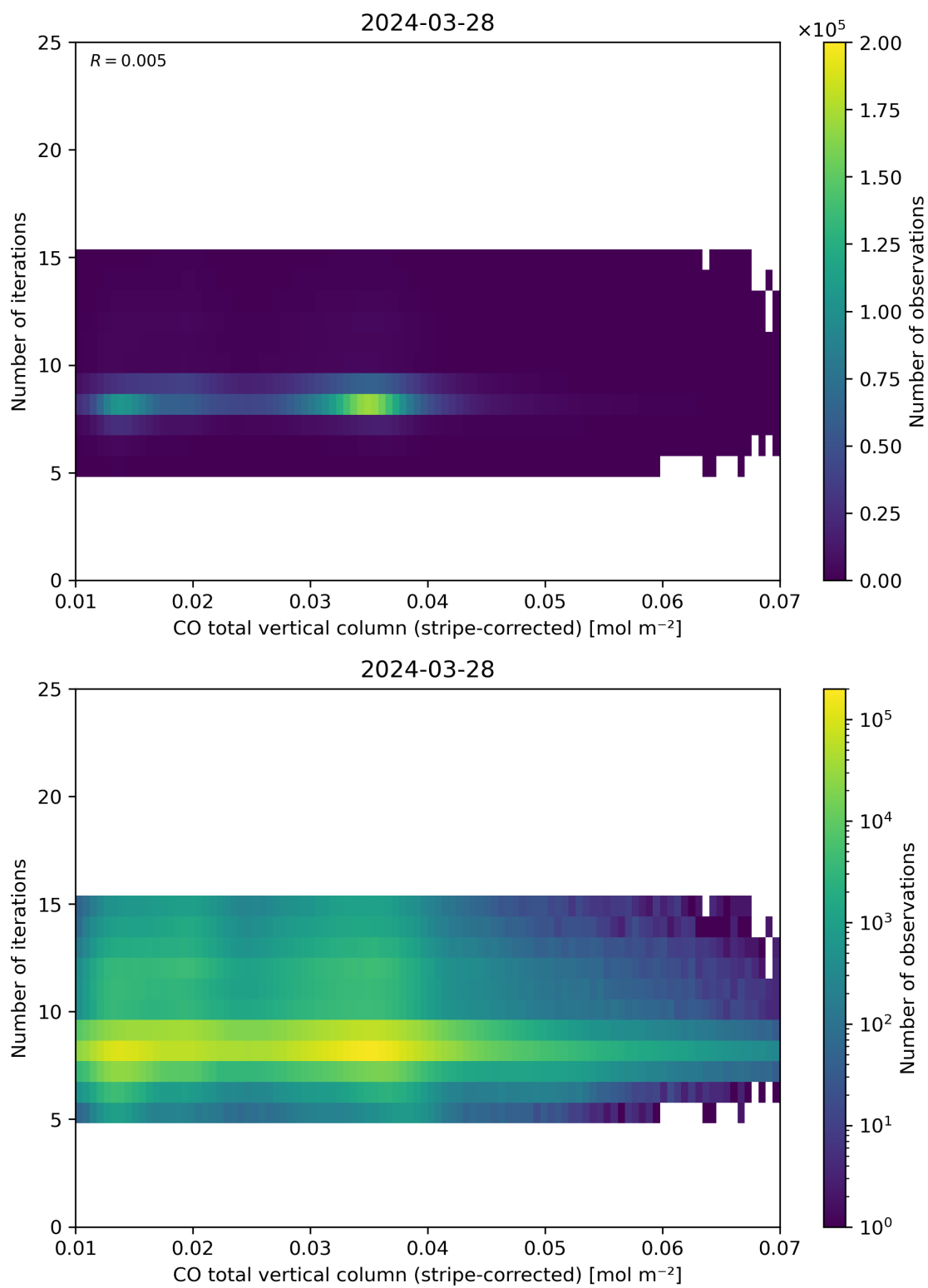
Figure 39: Scatter density plot of “CO total vertical column (stripe-corrected)” against “Number of iterations” for 2024-03-27 to 2024-03-29.
