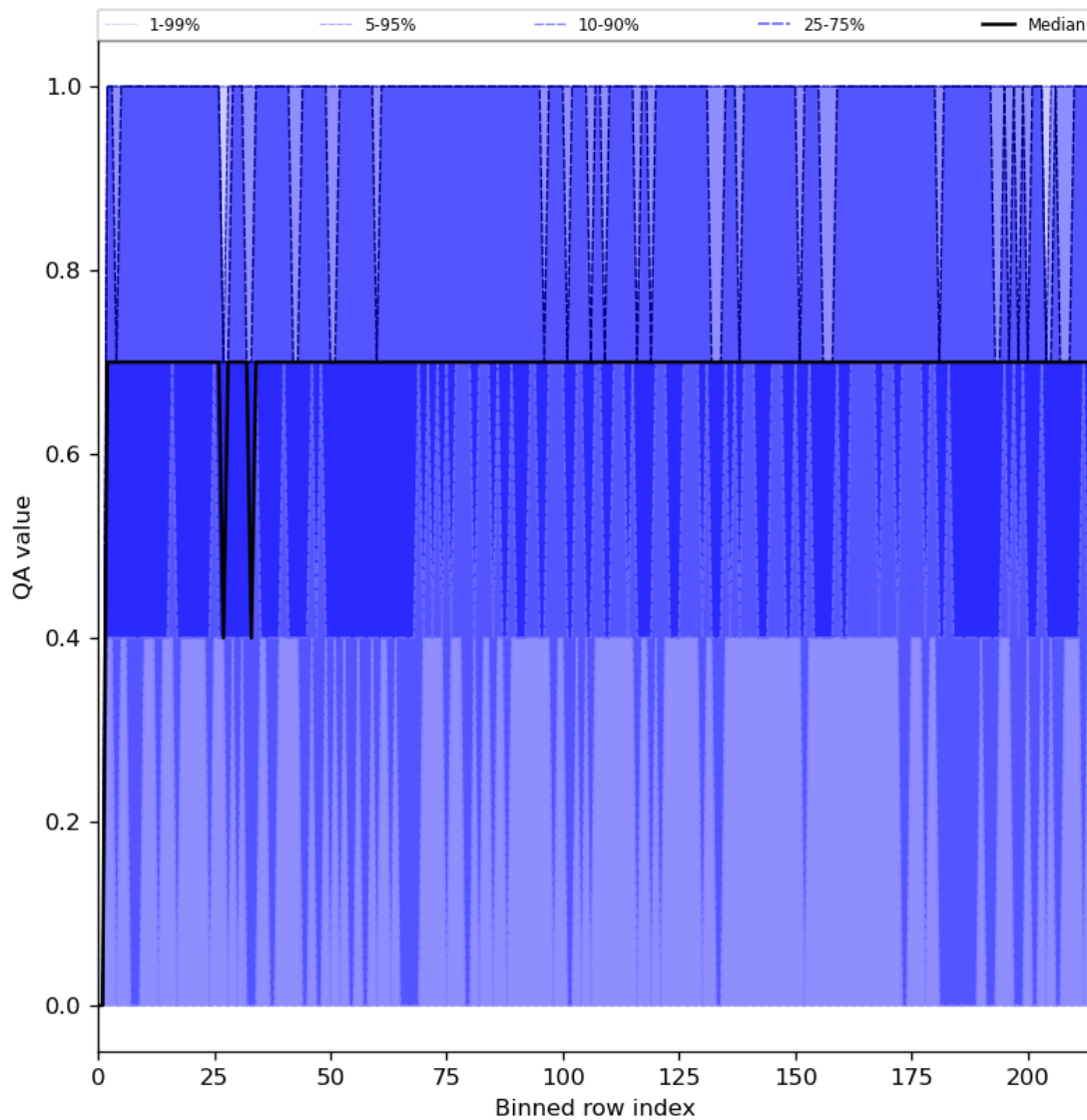
Figure 25: Along track statistics of “QA value” for 2024-03-27 to 2024-03-29
