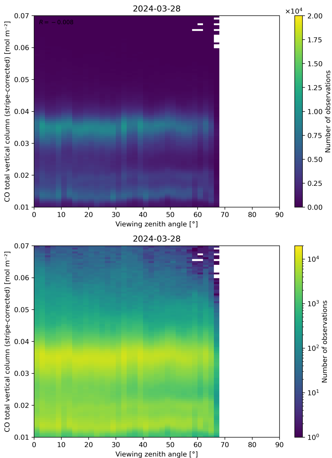
Figure 70: Scatter density plot of “Viewing zenith angle” against “CO total vertical column (stripe-corrected)” for 2024-03-27 to 2024-03-29.
