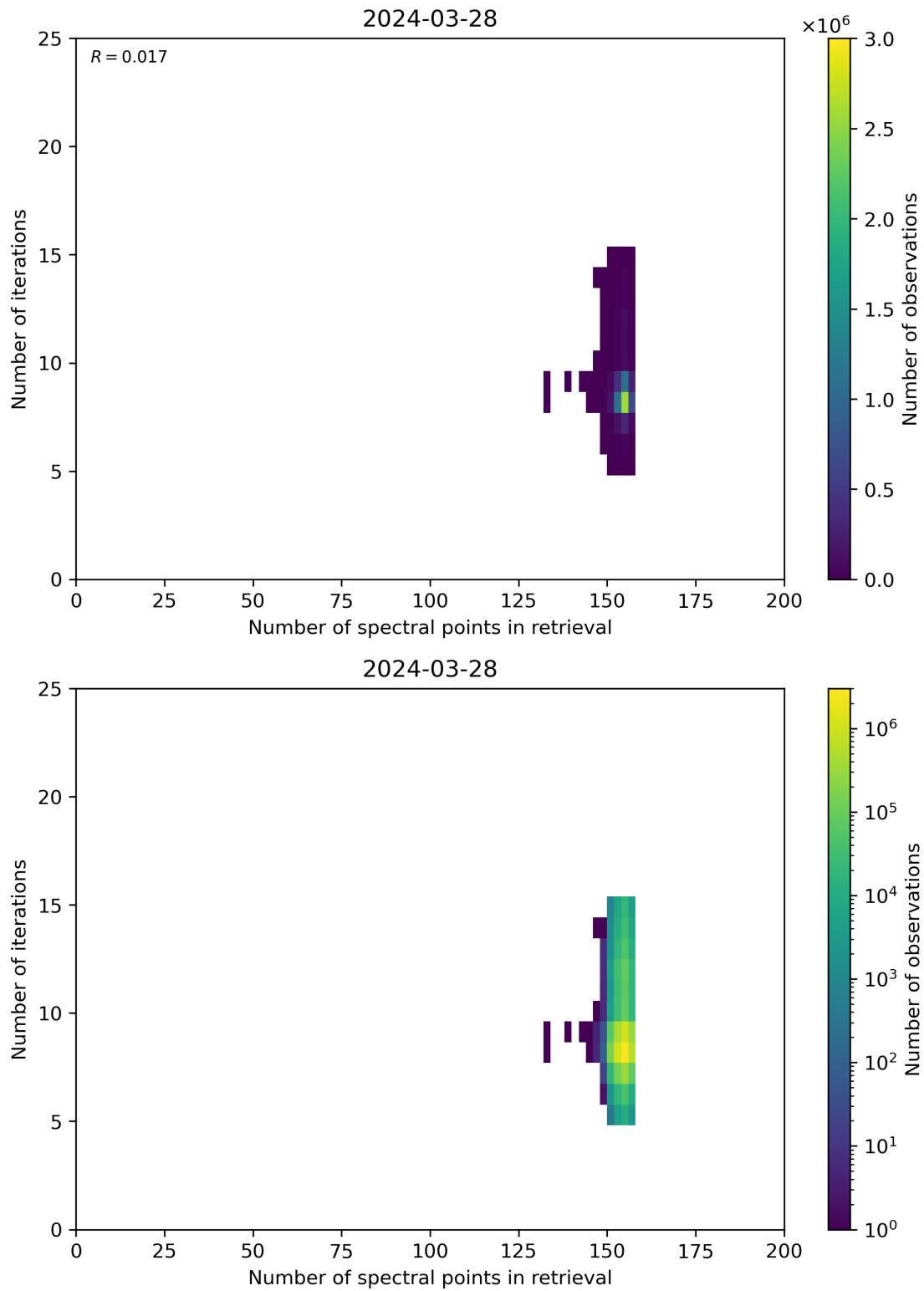
Figure 60: Scatter density plot of “Number of spectral points in retrieval” against “Number of iterations” for 2024-03-27 to 2024-03-29.
