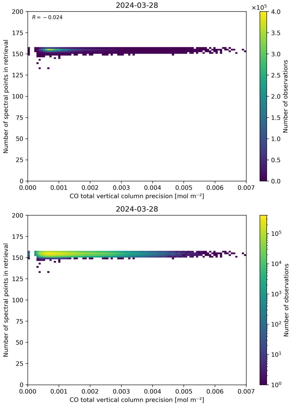
Figure 47: Scatter density plot of “CO total vertical column precision” against “Number of spectral points in retrieval” for 2024-03-27 to 2024-03-29.
