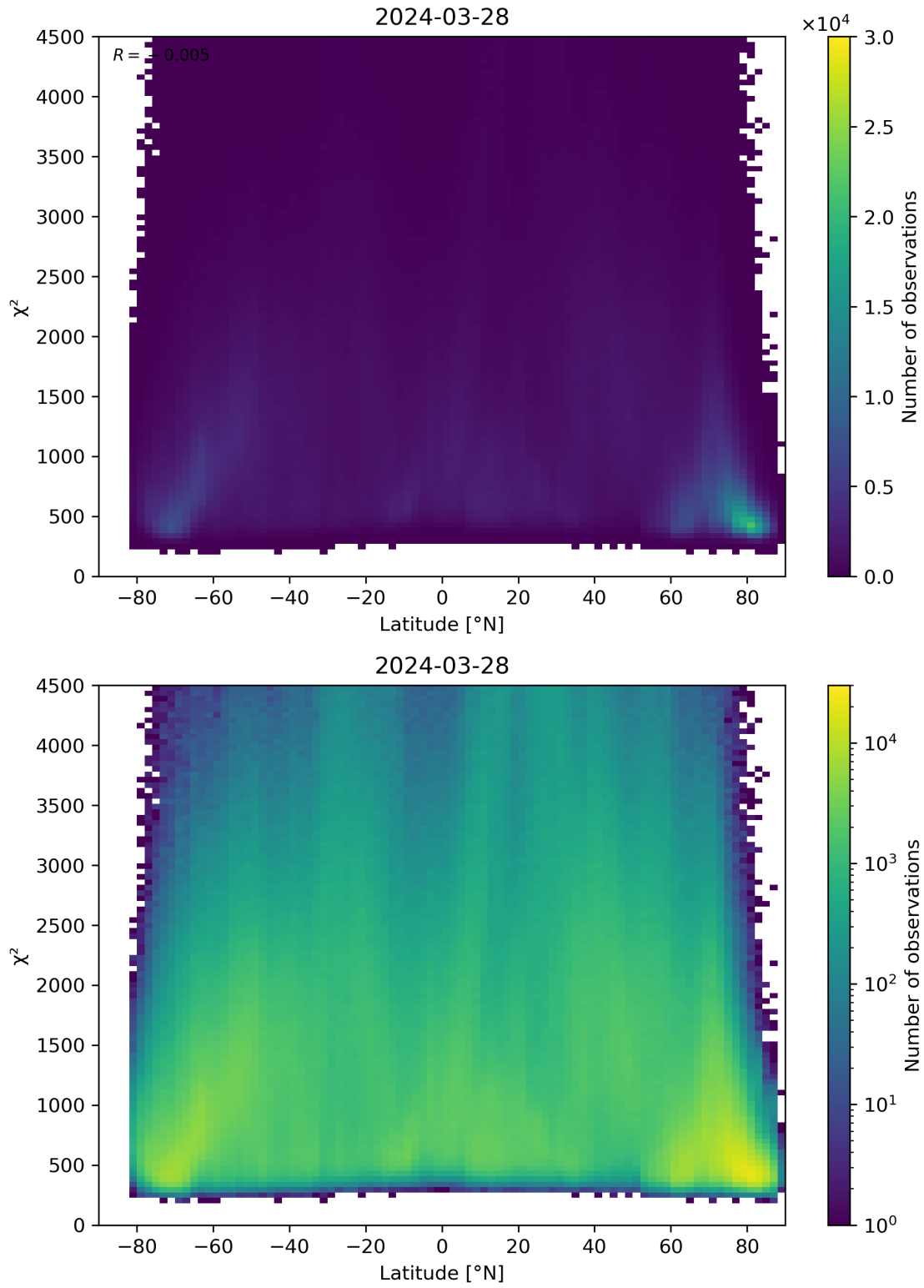
Figure 54: Scatter density plot of “Latitude” against “ \chi^2 ” for 2024-03-27 to 2024-03-29.
