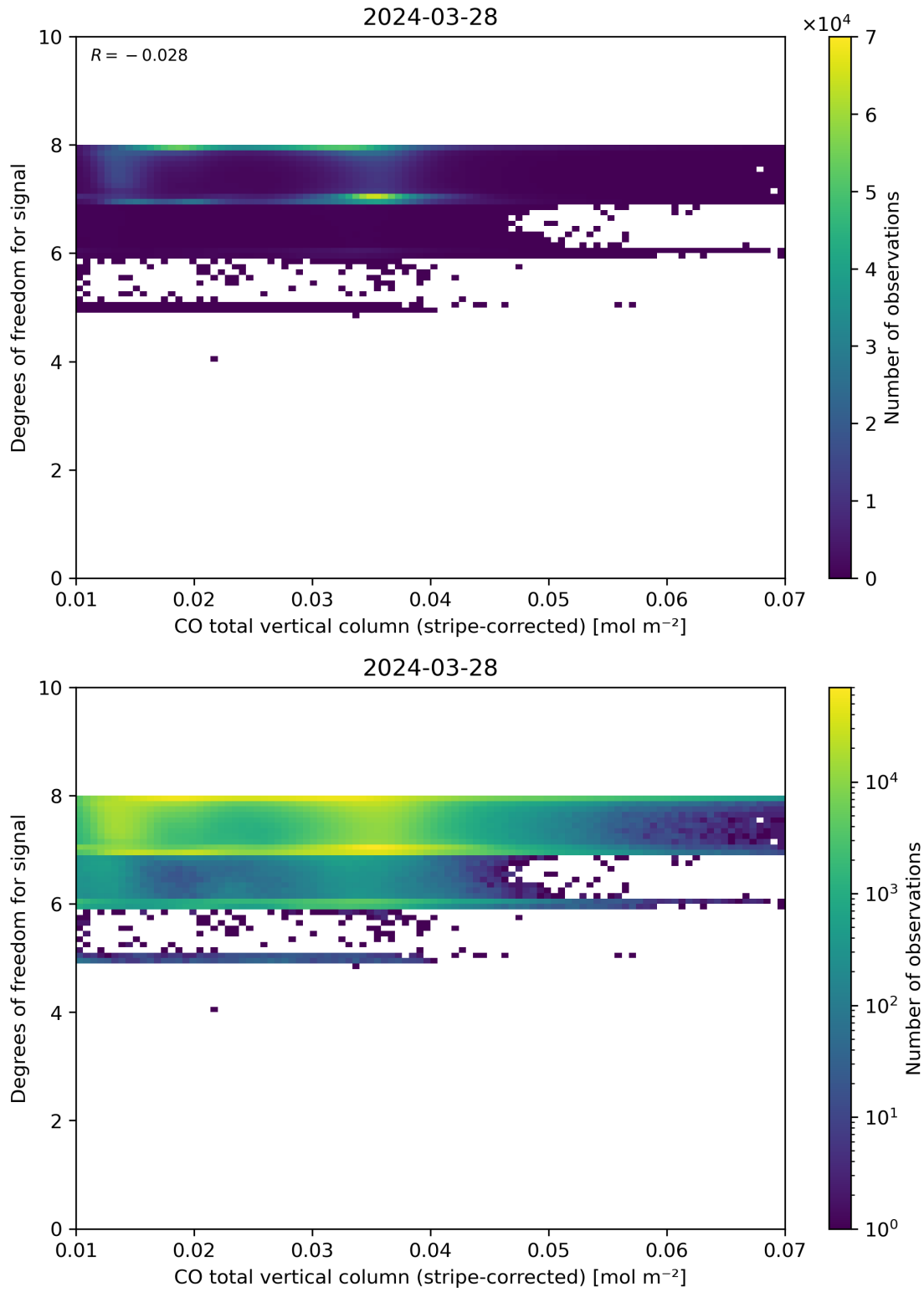
Figure 38: Scatter density plot of “CO total vertical column (stripe-corrected)” against “Degrees of freedom for signal” for 2024-03-27 to 2024-03-29.
