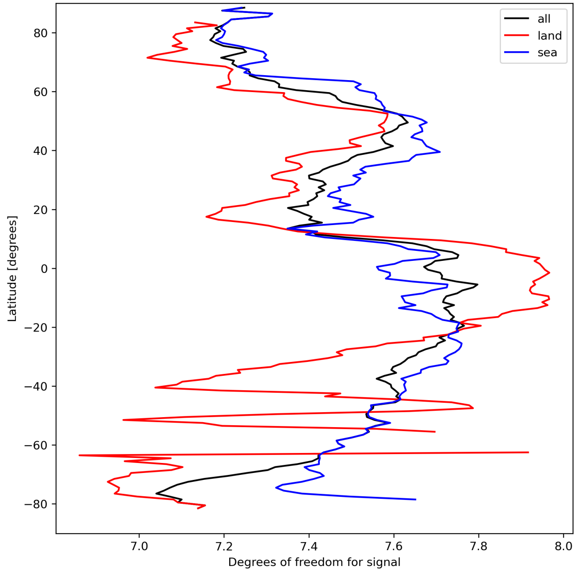
Figure 15: Zonal average of “Degrees of freedom for signal” for 2024-03-27 to 2024-03-29.
