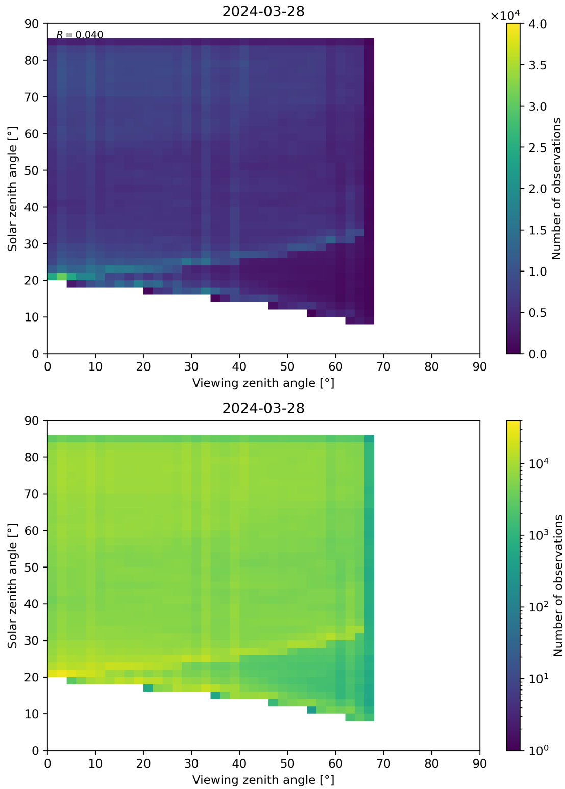
Figure 77: Scatter density plot of “Viewing zenith angle” against “Solar zenith angle” for 2024-03-27 to 2024-03-29.
