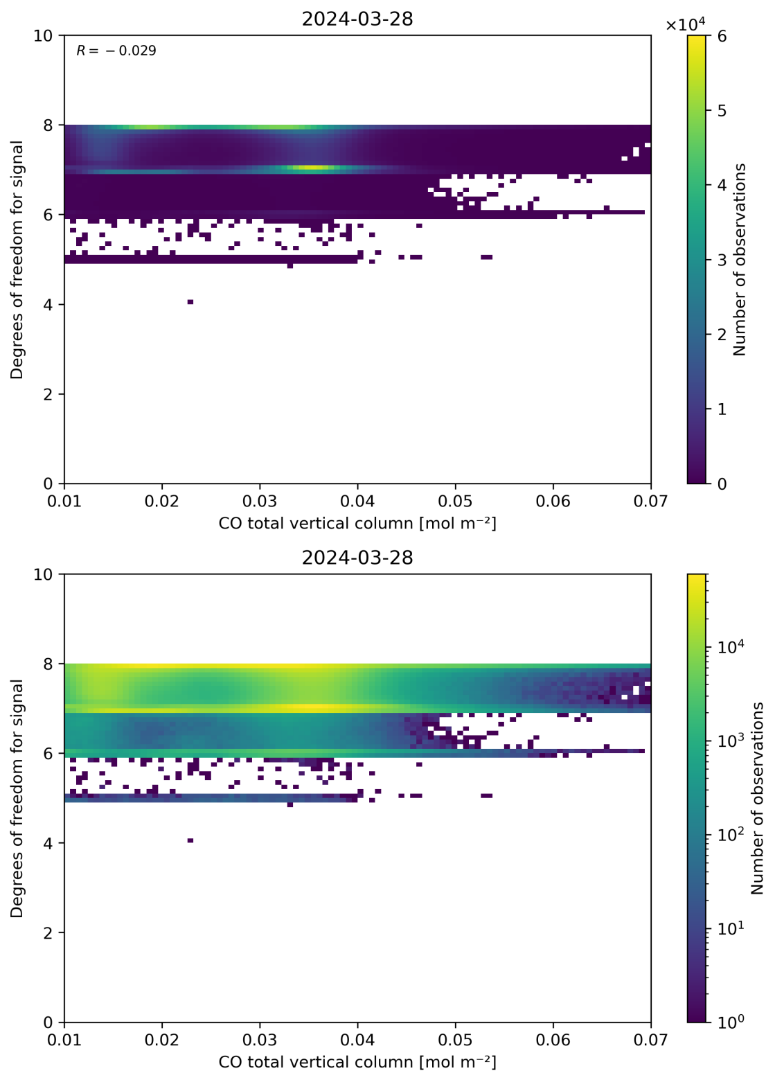
Figure 41: Scatter density plot of “CO total vertical column” against “Degrees of freedom for signal” for 2024-03-27 to 2024-03-29.
