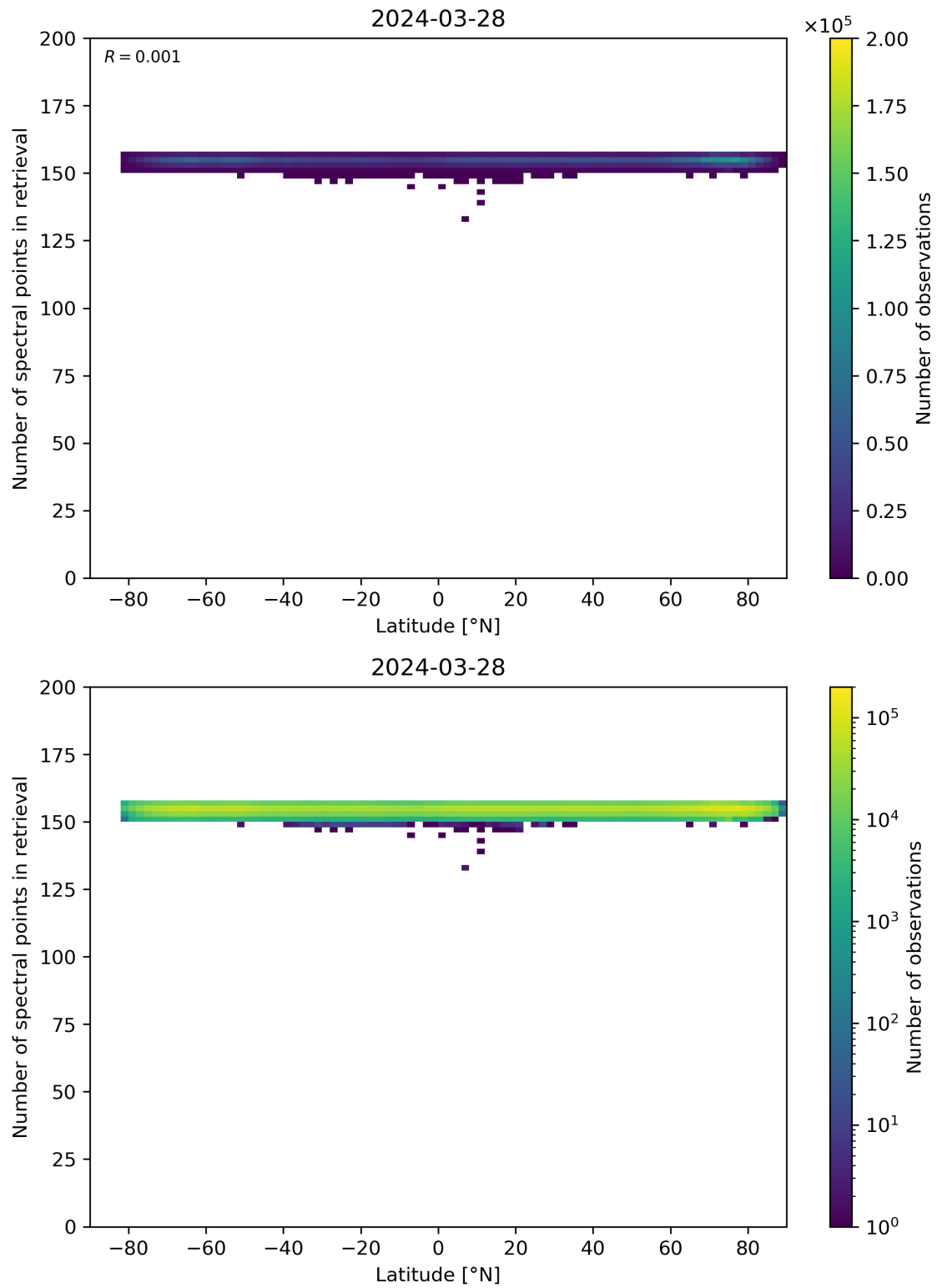
Figure 57: Scatter density plot of “Latitude” against “Number of spectral points in retrieval” for 2024-03-27 to 2024-03-29.
