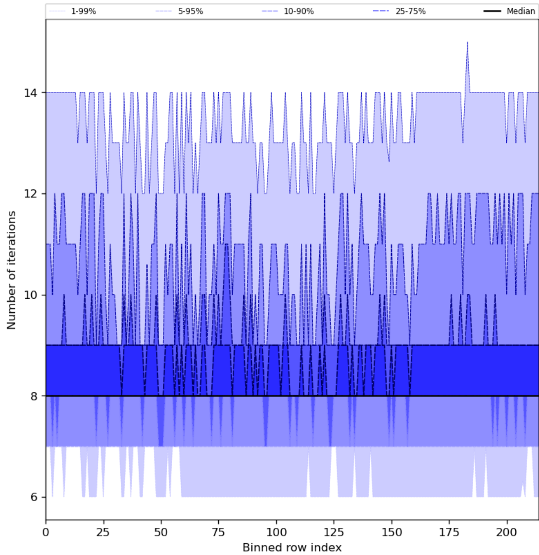
Figure 32: Along track statistics of “Number of iterations” for 2024-03-27 to 2024-03-29
