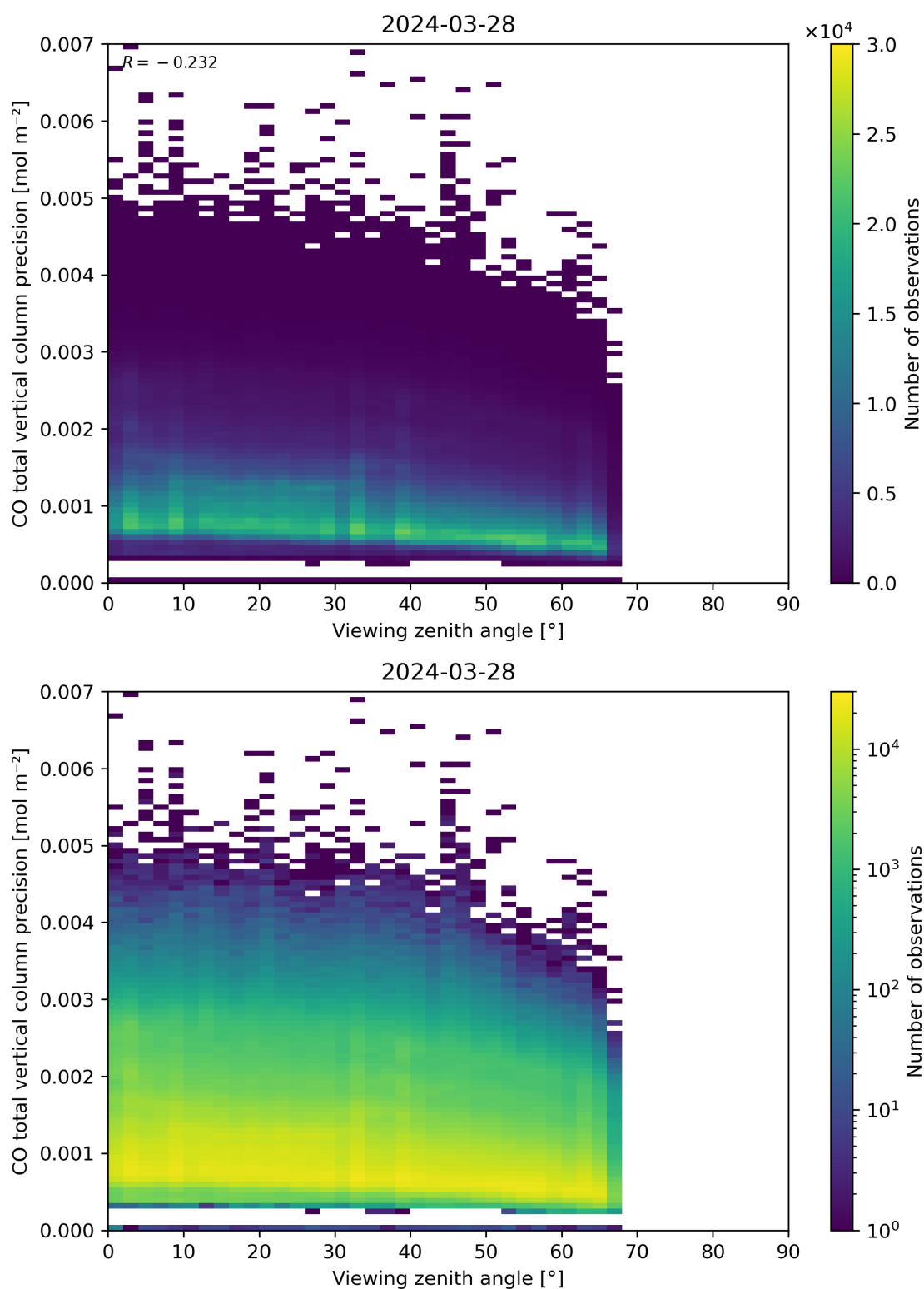
Figure 71: Scatter density plot of “Viewing zenith angle” against “CO total vertical column precision” for 2024-03-27 to 2024-03-29.
