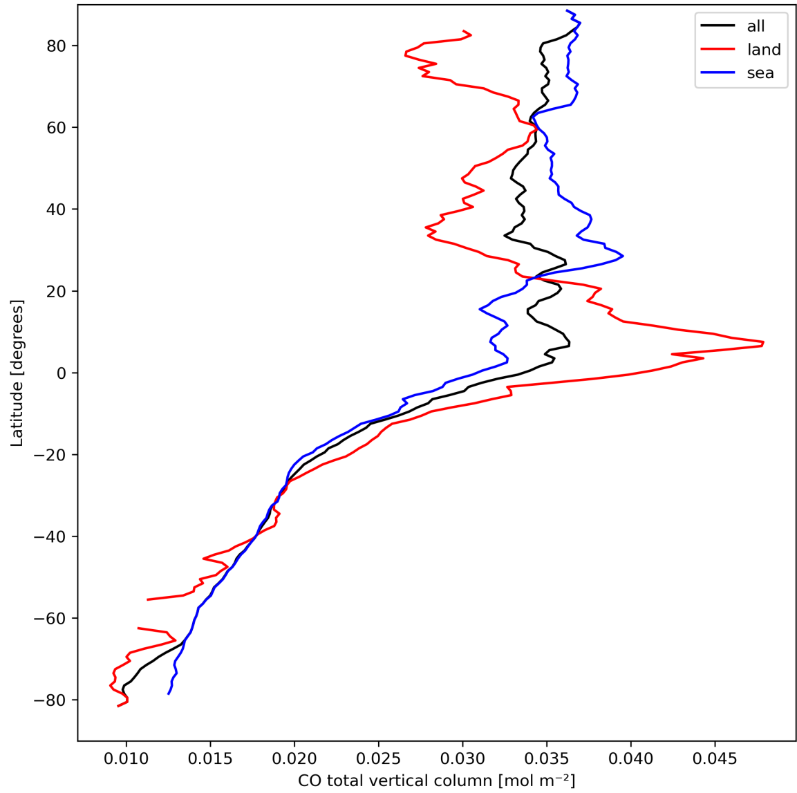
Figure 10: Zonal average of “CO total vertical column” for 2024-03-27 to 2024-03-29.
