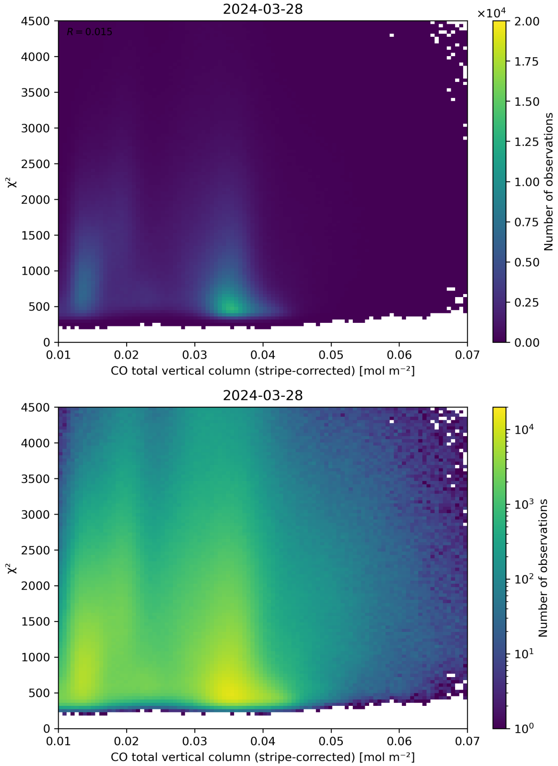
Figure 37: Scatter density plot of “CO total vertical column (stripe-corrected)” against “ \chi^2 ” for 2024-03-27 to 2024-03-29.
