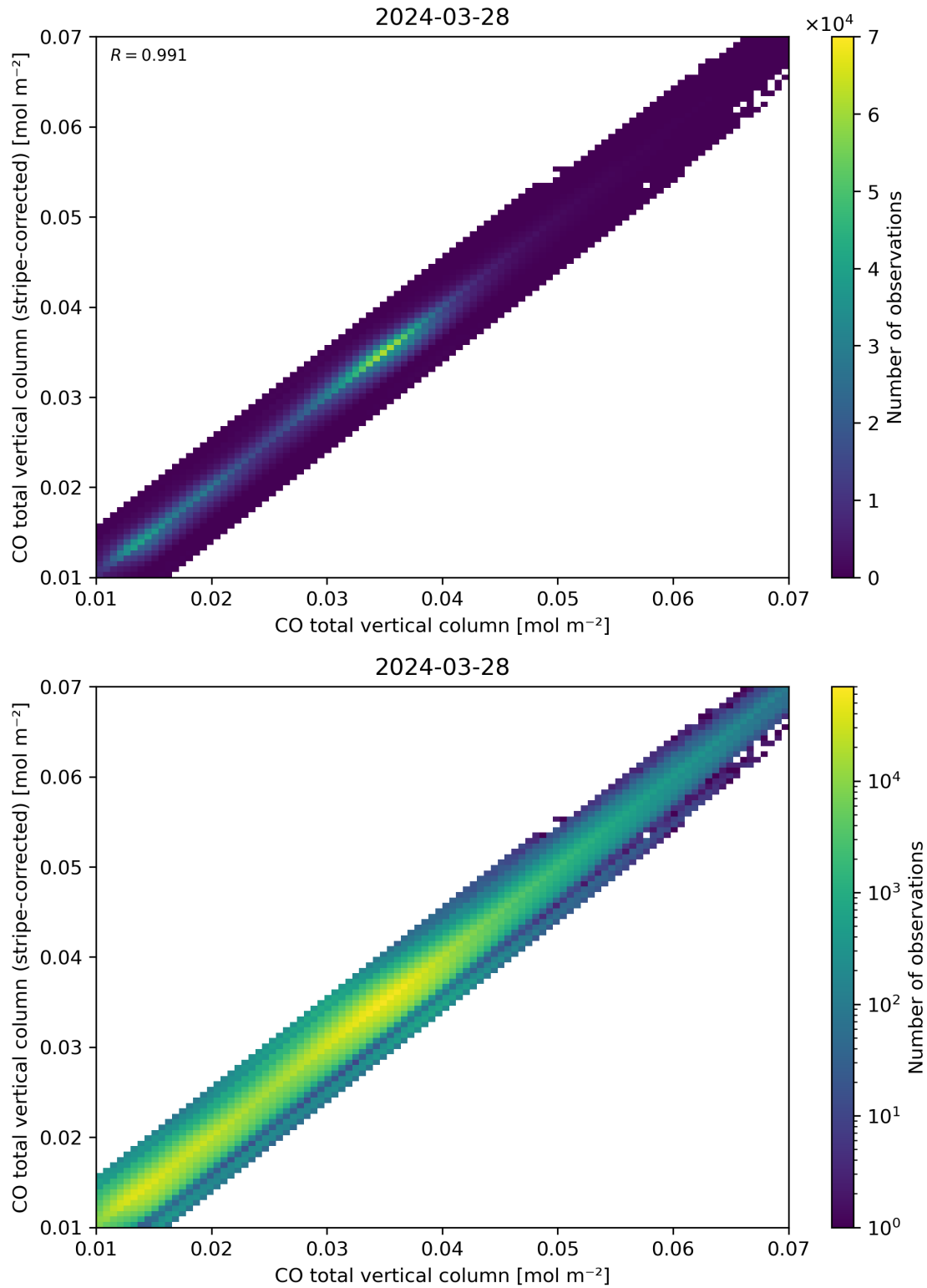
Figure 33: Scatter density plot of “CO total vertical column” against “CO total vertical column (stripe-corrected)” for 2024-03-27 to 2024-03-29.
