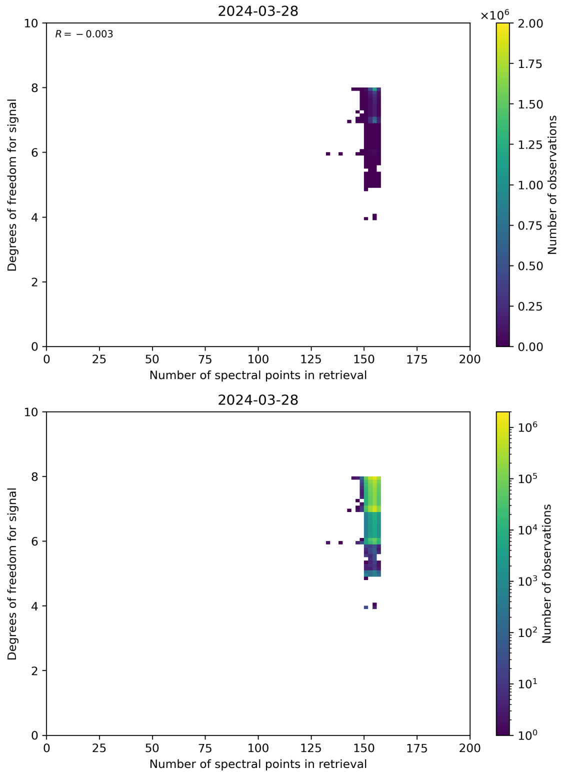
Figure 59: Scatter density plot of “Number of spectral points in retrieval” against “Degrees of freedom for signal” for 2024-03-27 to 2024-03-29.
