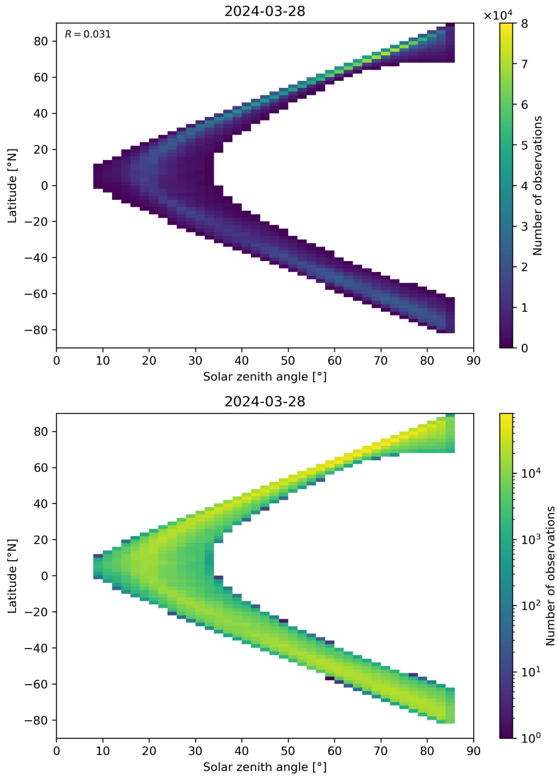
Figure 66: Scatter density plot of “Solar zenith angle” against “Latitude” for 2024-03-27 to 2024-03-29.
