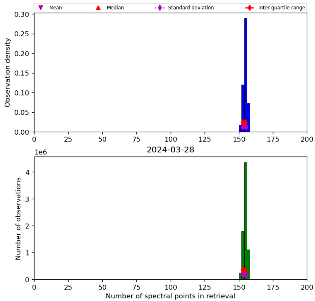
Figure 21: Histogram of “Number of spectral points in retrieval” for 2024-03-27 to 2024-03-29
