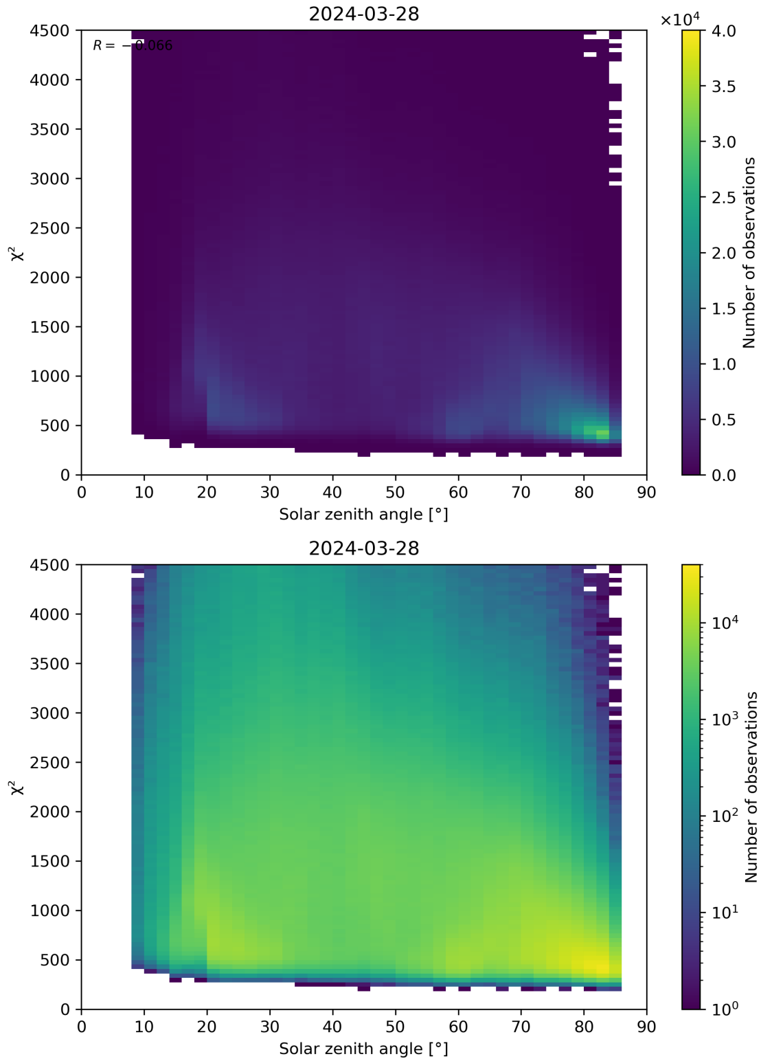
Figure 64: Scatter density plot of “Solar zenith angle” against “ \chi^2 ” for 2024-03-27 to 2024-03-29.
