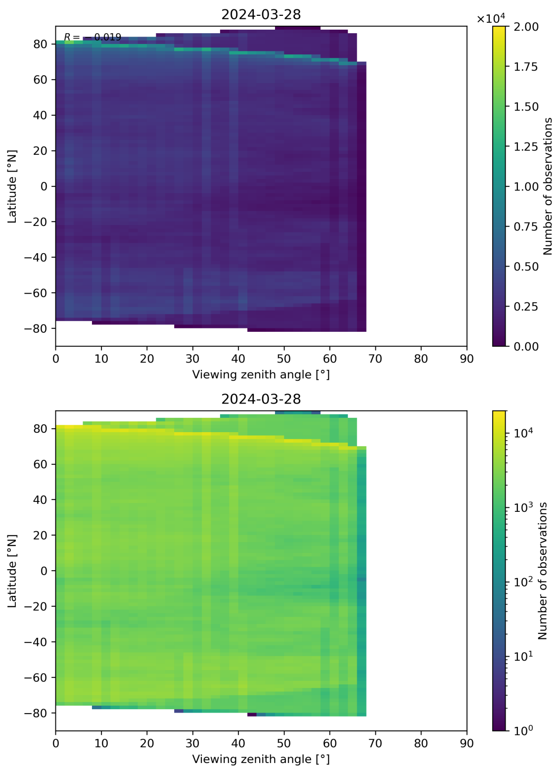
Figure 74: Scatter density plot of “Viewing zenith angle” against “Latitude” for 2024-03-27 to 2024-03-29.
