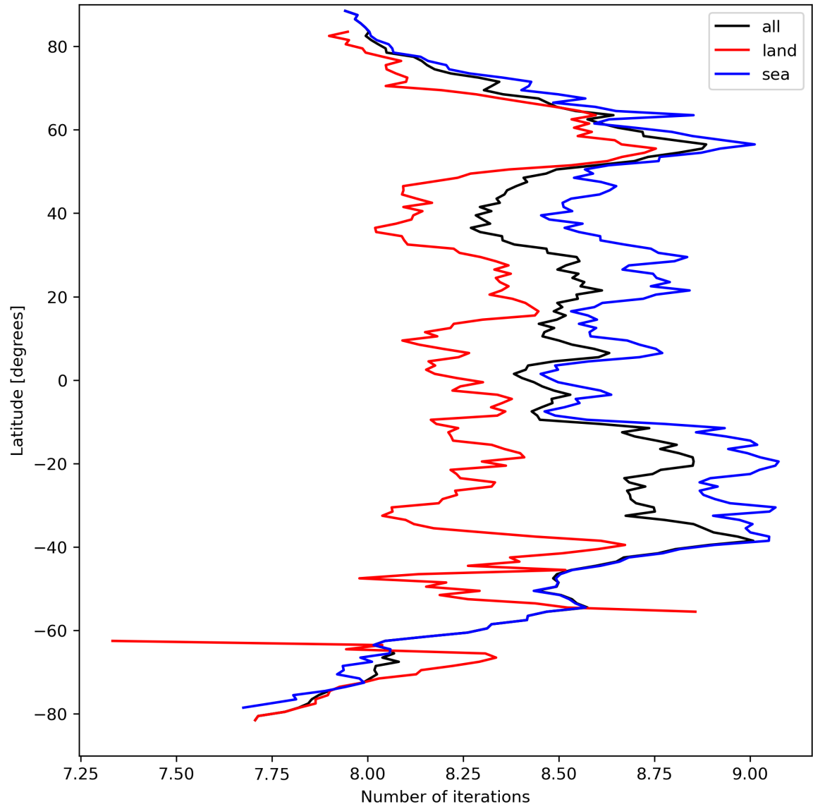
Figure 16: Zonal average of “Number of iterations” for 2024-03-27 to 2024-03-29.
