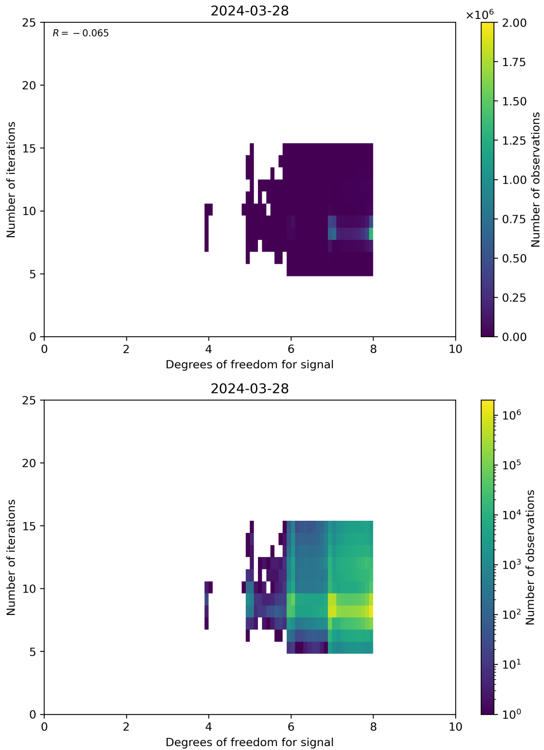
Figure 50: Scatter density plot of “Degrees of freedom for signal” against “Number of iterations” for 2024-03-27 to 2024-03-29.
