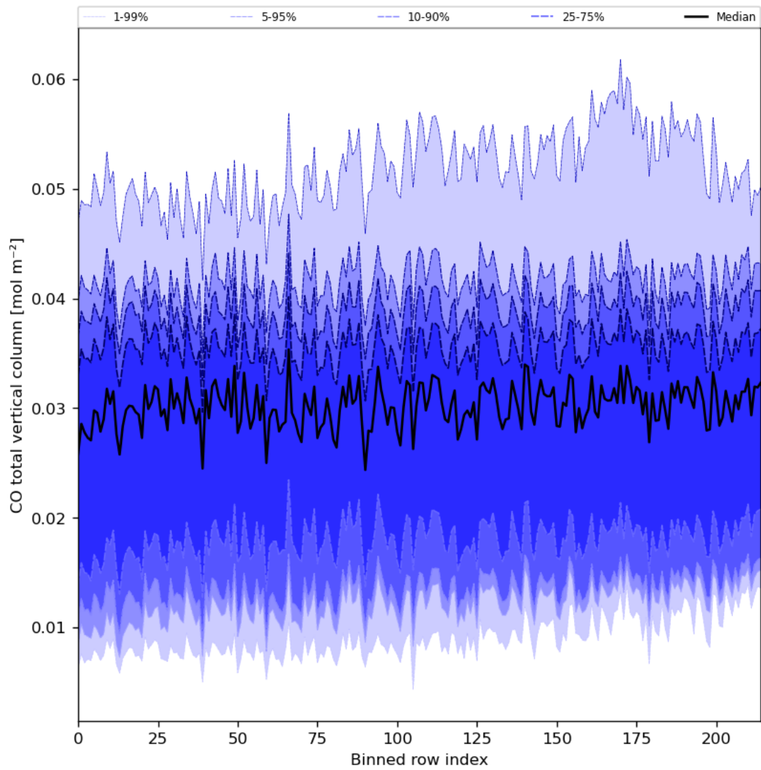
Figure 26: Along track statistics of “CO total vertical column” for 2024-03-27 to 2024-03-29
