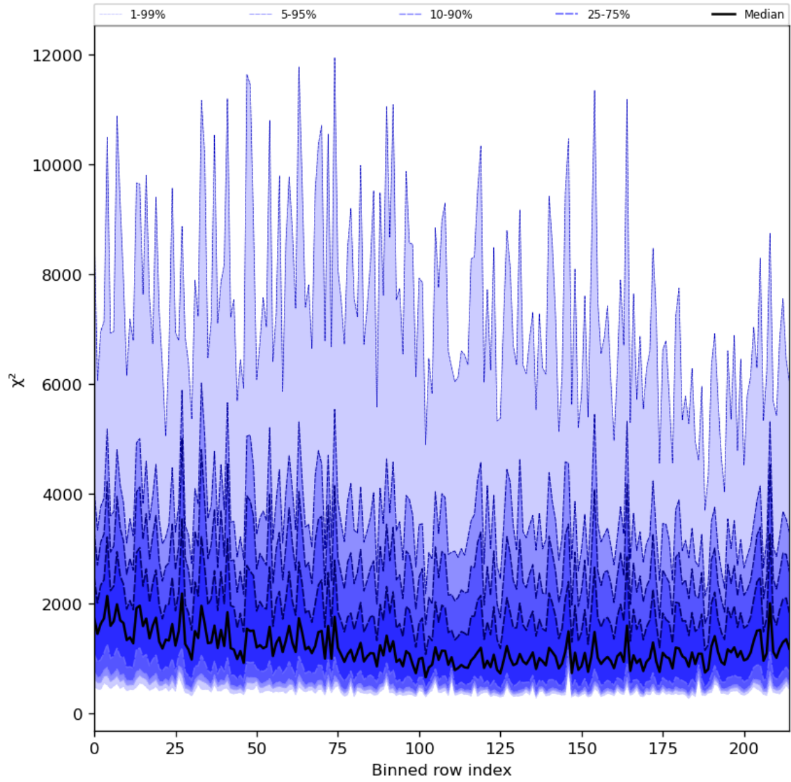
Figure 30: Along track statistics of “ \chi^2 ” for 2024-03-27 to 2024-03-29
