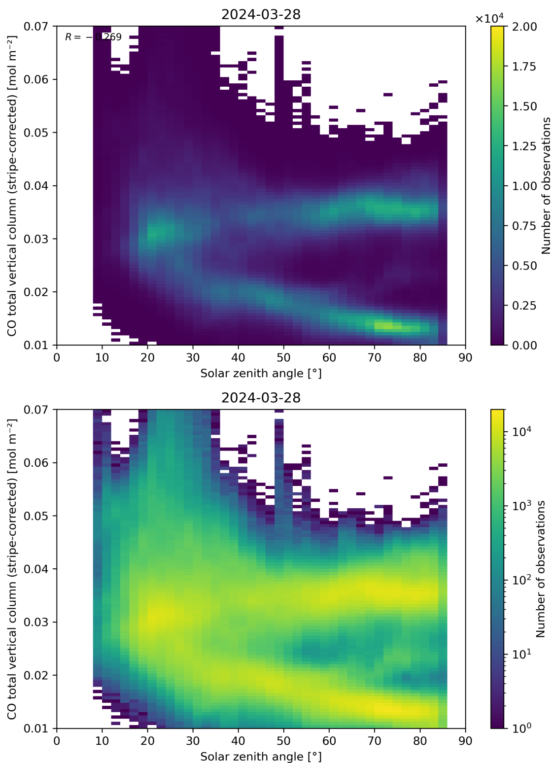
Figure 62: Scatter density plot of “Solar zenith angle” against “CO total vertical column (stripe-corrected)” for 2024-03-27 to 2024-03-29.
