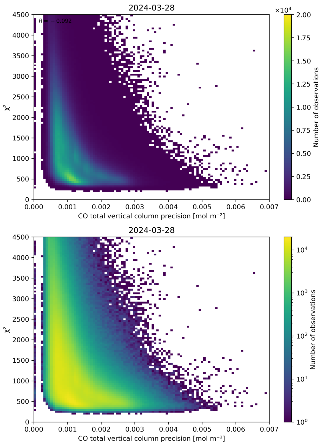
Figure 44: Scatter density plot of “CO total vertical column precision” against “ \chi^2 ” for 2024-03-27 to 2024-03-29.
