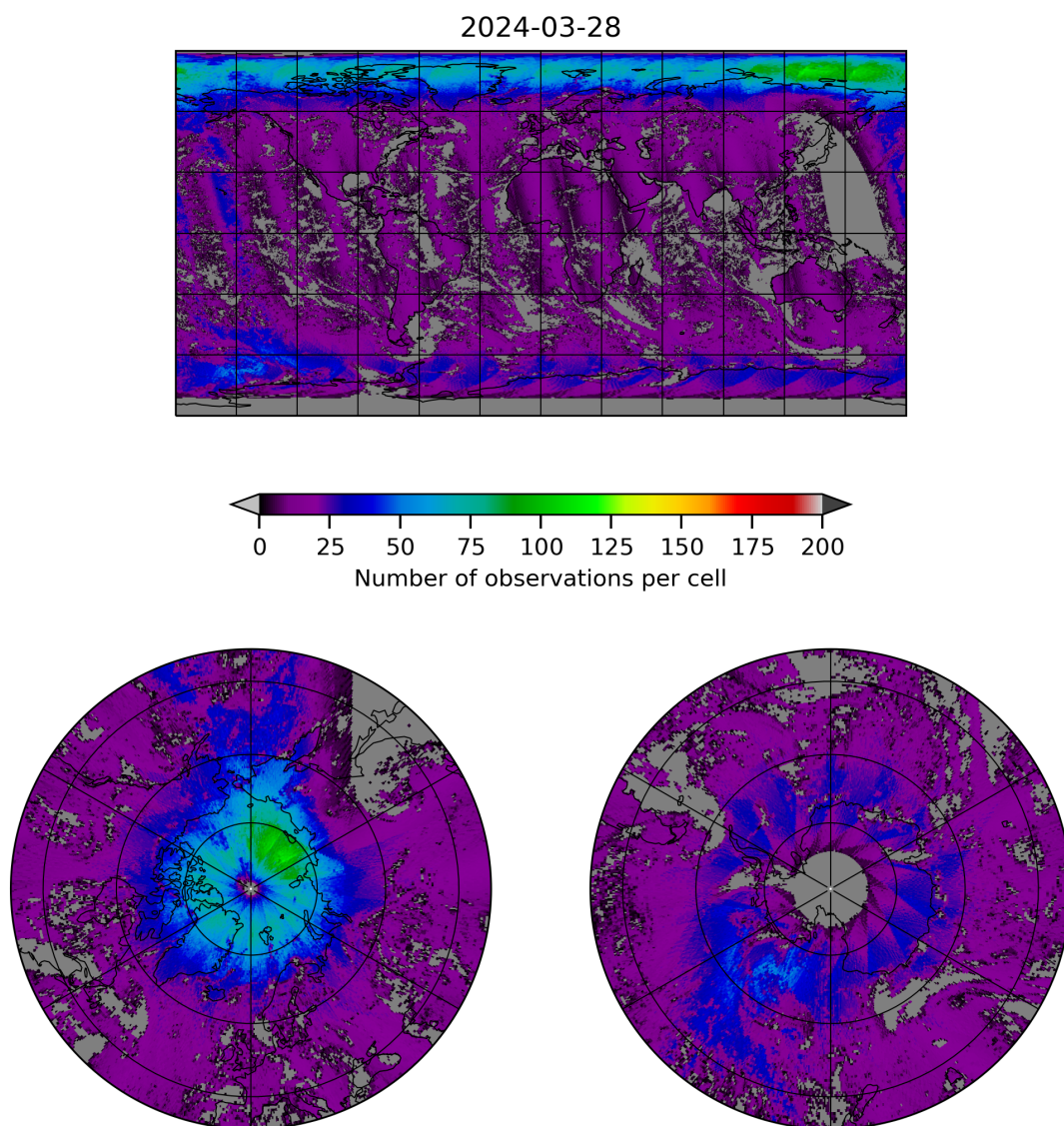
Figure 8: Map of the number of observations for 2024-03-27 to 2024-03-29
