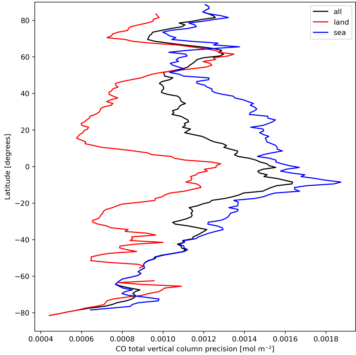
Figure 12: Zonal average of “CO total vertical column precision” for 2024-03-27 to 2024-03-29.
