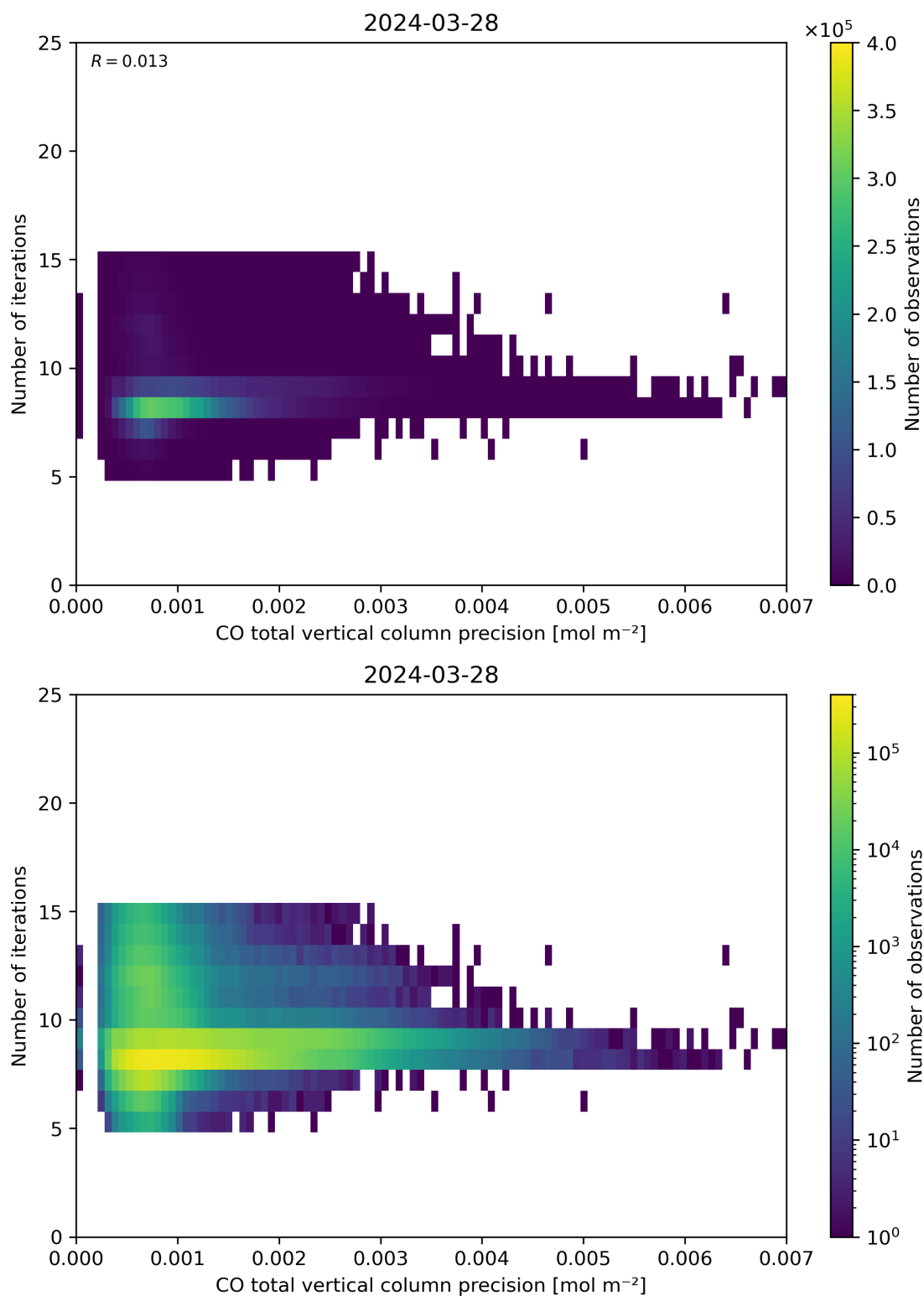
Figure 46: Scatter density plot of “CO total vertical column precision” against “Number of iterations” for 2024-03-27 to 2024-03-29.
