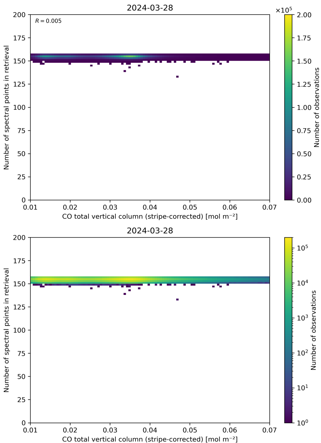
Figure 40: Scatter density plot of “CO total vertical column (stripe-corrected)” against “Number of spectral points in retrieval” for 2024-03-27 to 2024-03-29.
