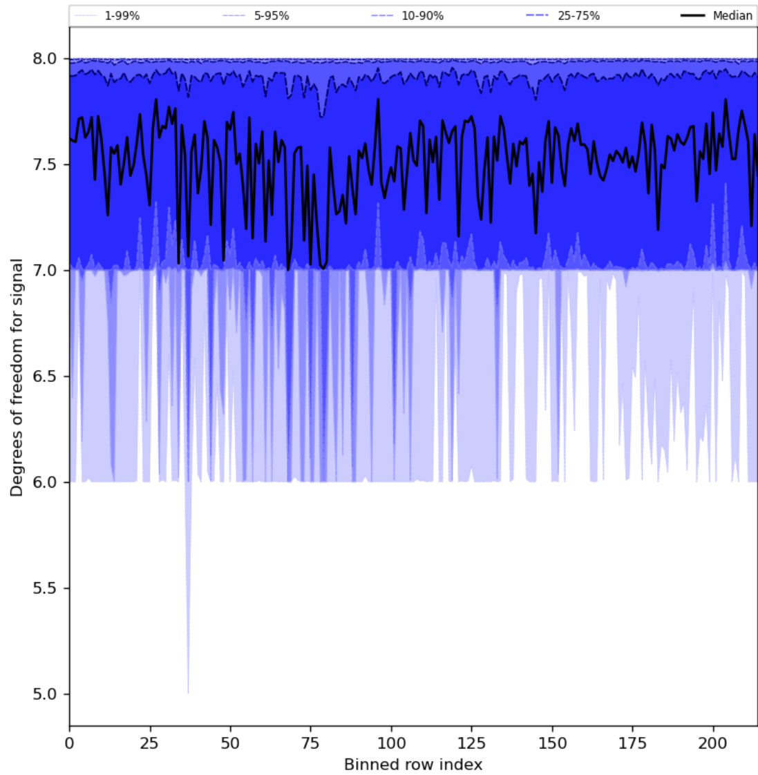
Figure 31: Along track statistics of “Degrees of freedom for signal” for 2024-03-27 to 2024-03-29
