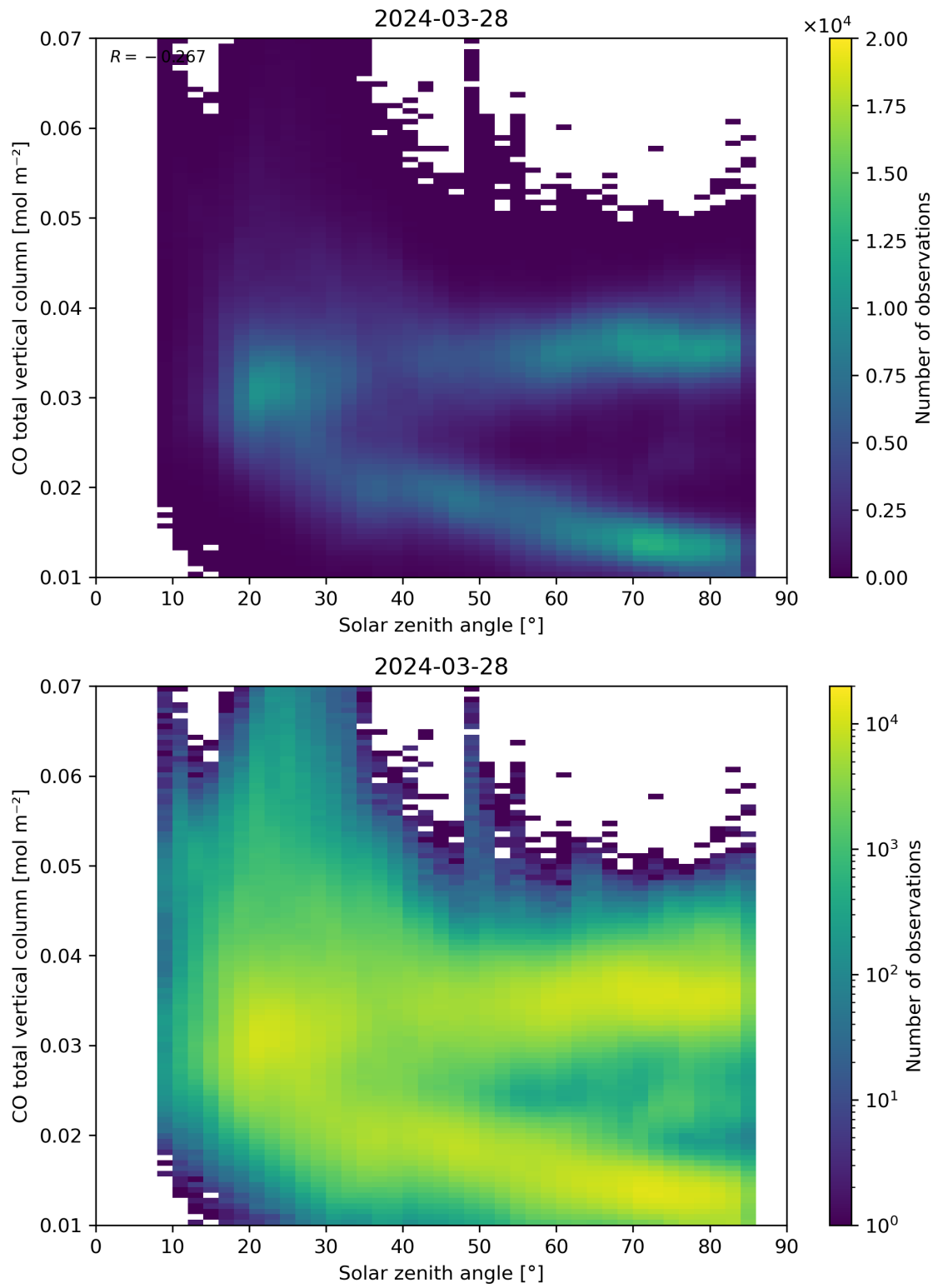
Figure 61: Scatter density plot of “Solar zenith angle” against “CO total vertical column” for 2024-03-27 to 2024-03-29.
