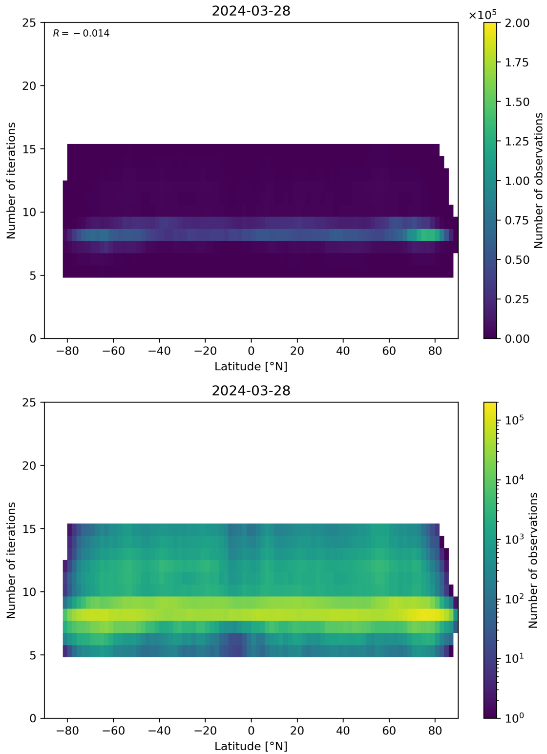
Figure 56: Scatter density plot of “Latitude” against “Number of iterations” for 2024-03-27 to 2024-03-29.
