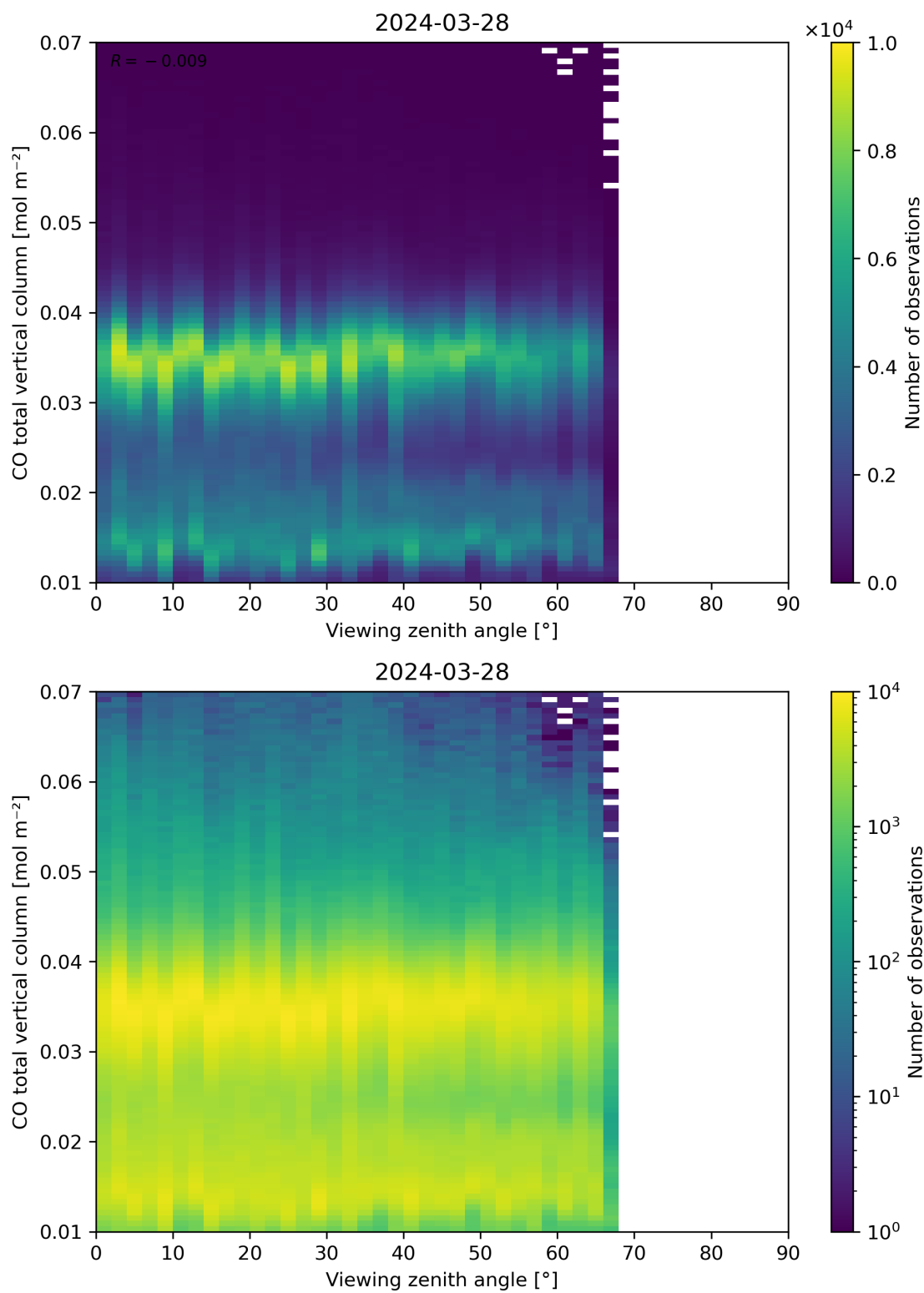
Figure 69: Scatter density plot of “Viewing zenith angle” against “CO total vertical column” for 2024-03-27 to 2024-03-29.
