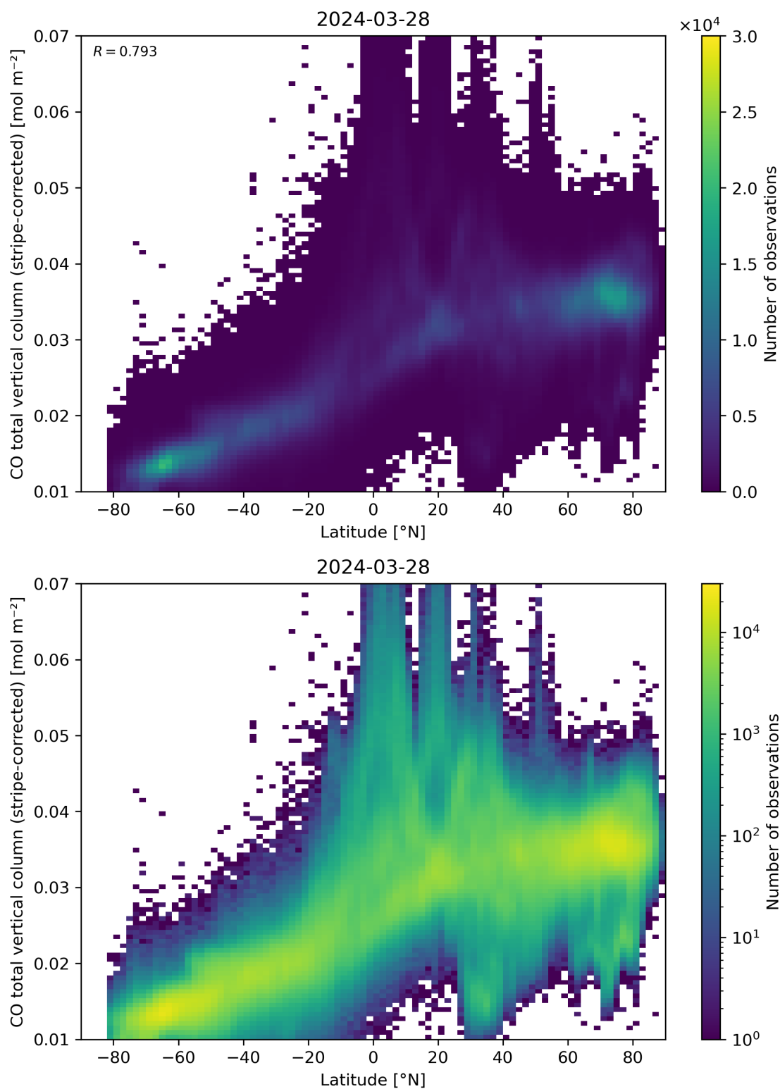
Figure 52: Scatter density plot of “Latitude” against “CO total vertical column (stripe-corrected)” for 2024-03-27 to 2024-03-29.
