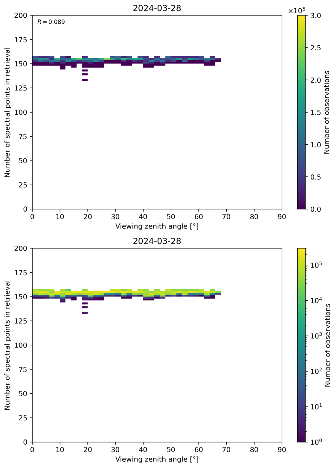
Figure 76: Scatter density plot of “Viewing zenith angle” against “Number of spectral points in retrieval” for 2024-03-27 to 2024-03-29.
