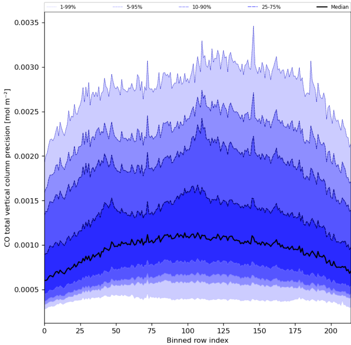
Figure 28: Along track statistics of “CO total vertical column precision” for 2024-03-27 to 2024-03-29
