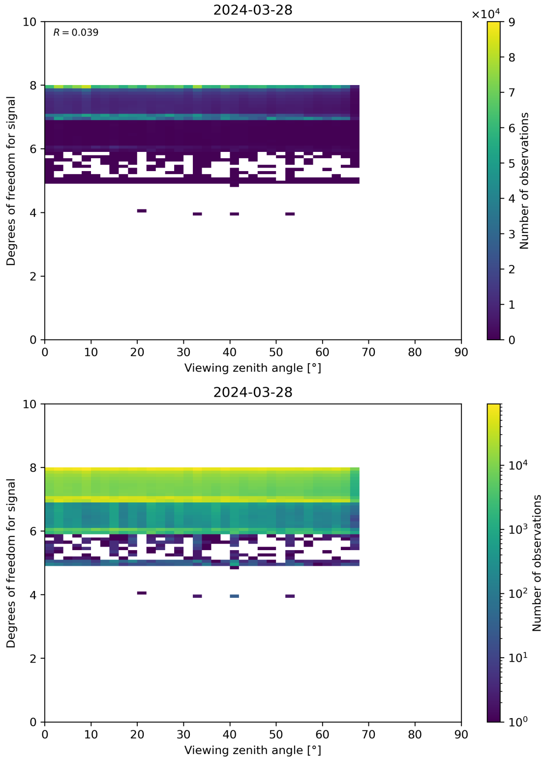
Figure 73: Scatter density plot of “Viewing zenith angle” against “Degrees of freedom for signal” for 2024-03-27 to 2024-03-29.
