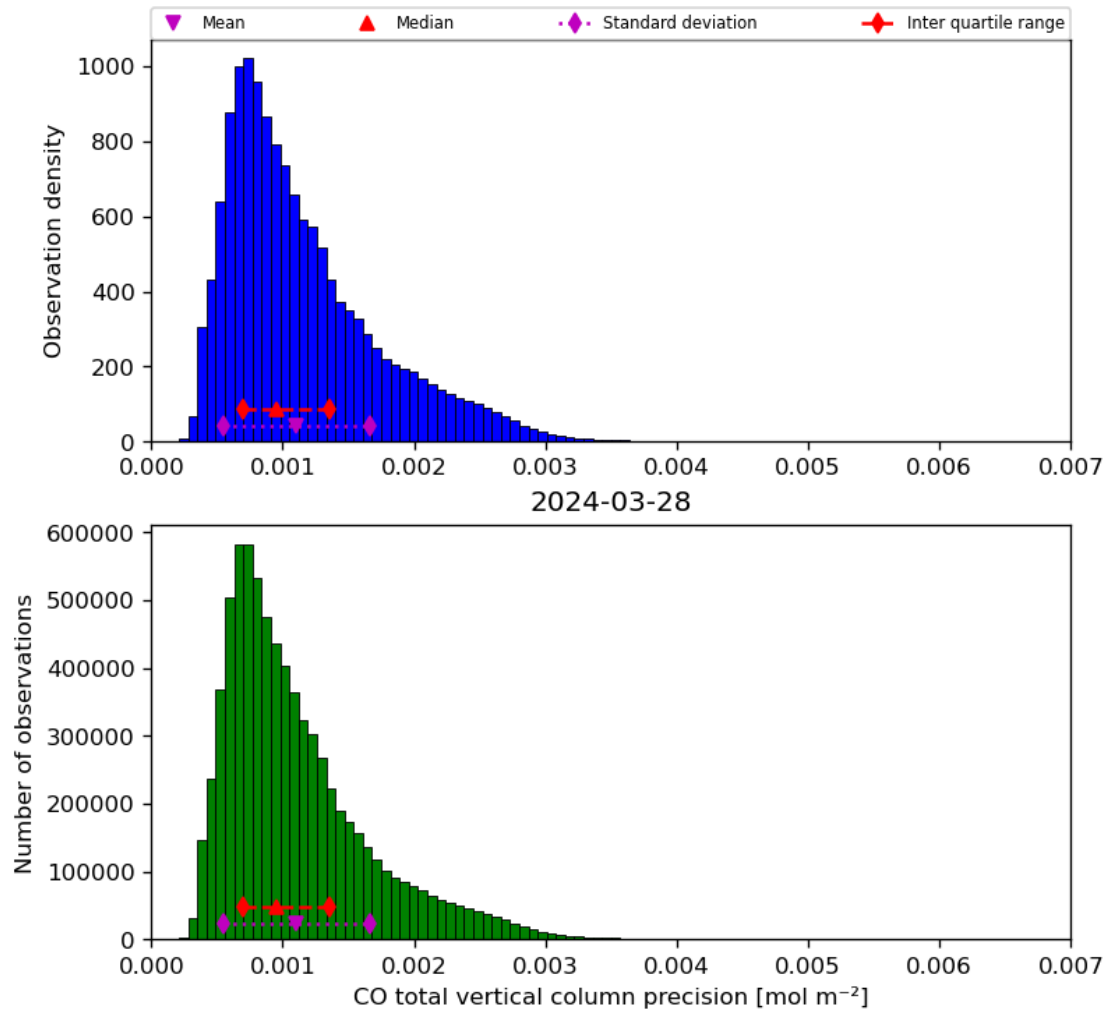
Figure 20: Histogram of “CO total vertical column precision” for 2024-03-27 to 2024-03-29
