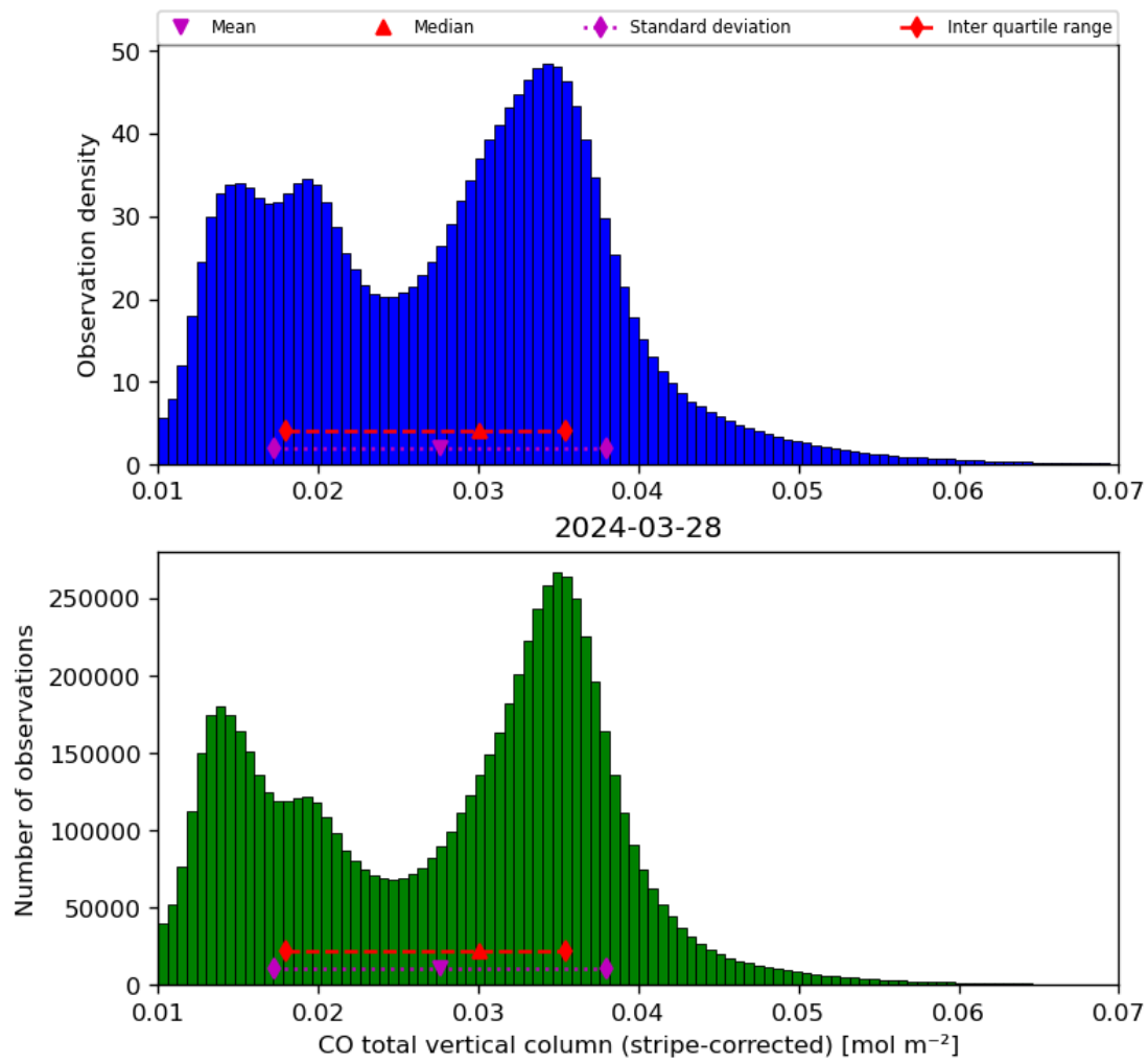
Figure 19: Histogram of “CO total vertical column (stripe-corrected)” for 2024-03-27 to 2024-03-29
