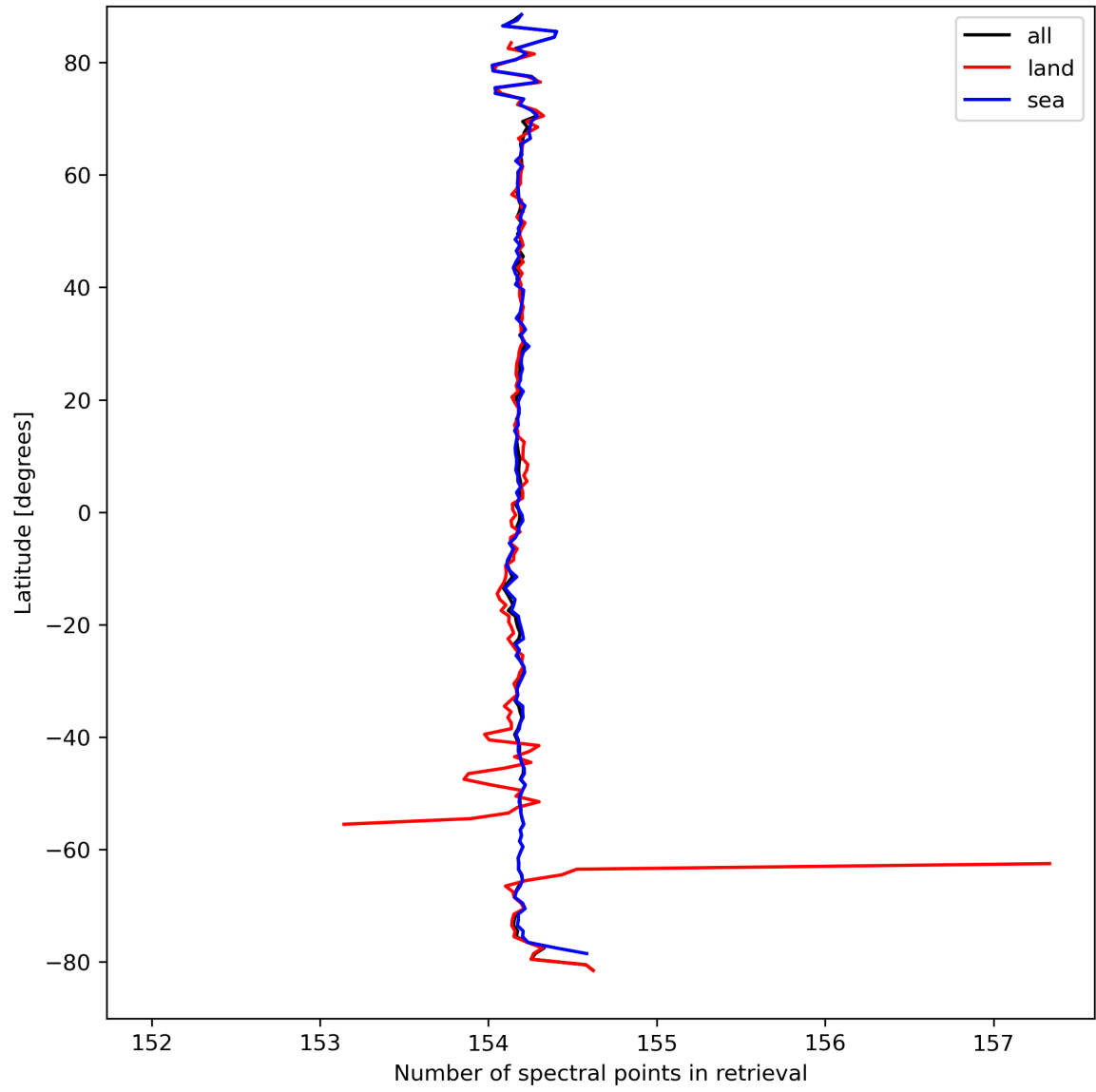
Figure 13: Zonal average of “Number of spectral points in retrieval” for 2024-03-27 to 2024-03-29.
