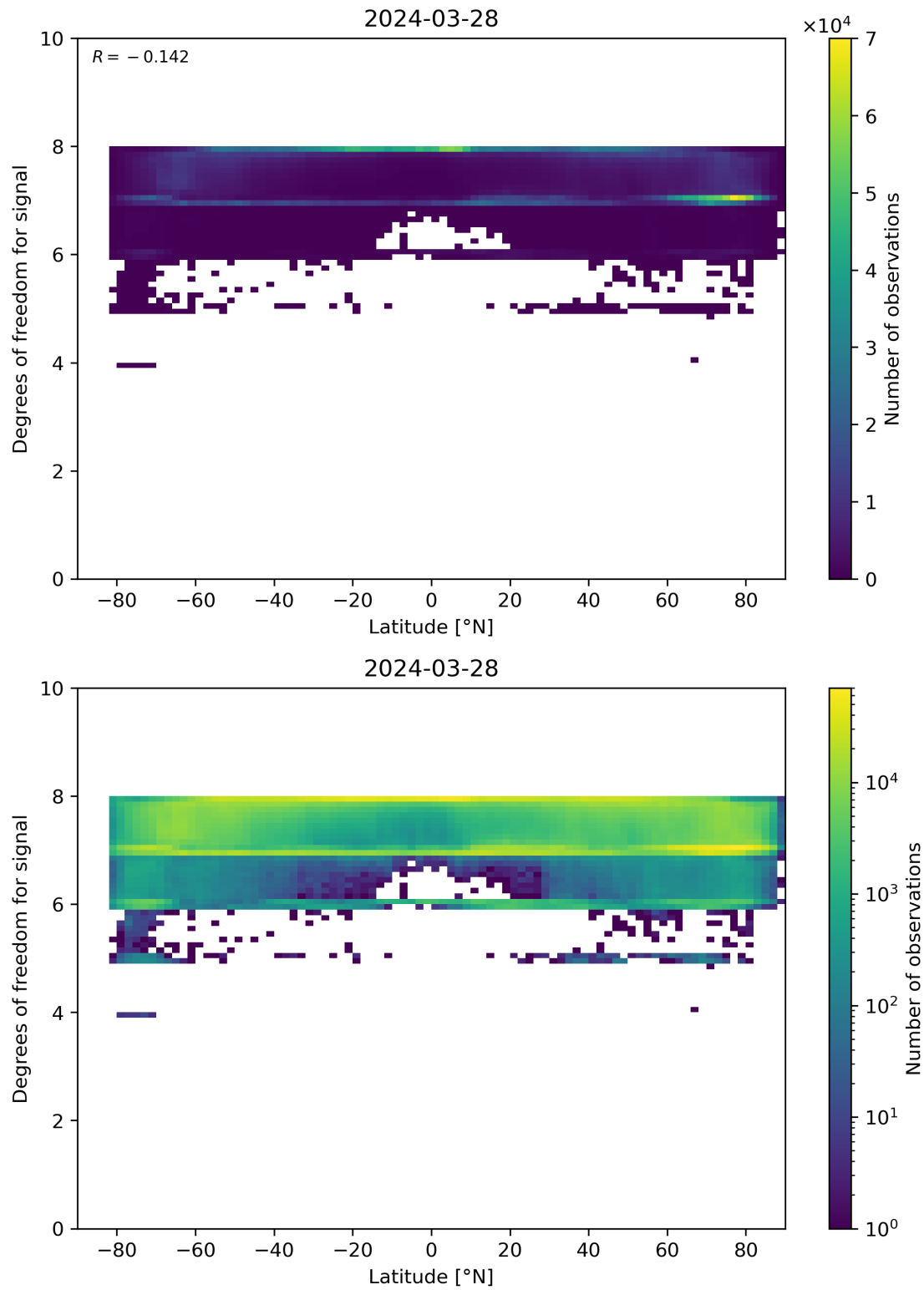
Figure 55: Scatter density plot of “Latitude” against “Degrees of freedom for signal” for 2024-03-27 to 2024-03-29.
