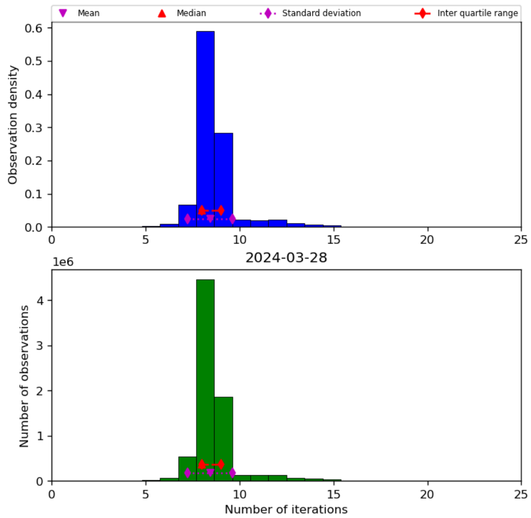
Figure 24: Histogram of “Number of iterations” for 2024-03-27 to 2024-03-29
