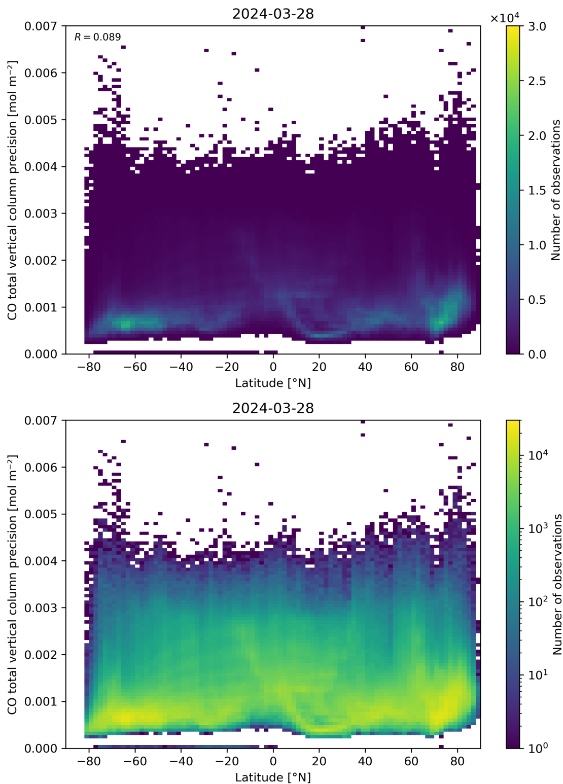
Figure 53: Scatter density plot of “Latitude” against “CO total vertical column precision” for 2024-03-27 to 2024-03-29.
