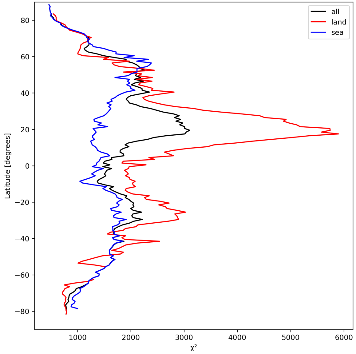
Figure 14: Zonal average of “ \chi^2 ” for 2024-03-27 to 2024-03-29.
