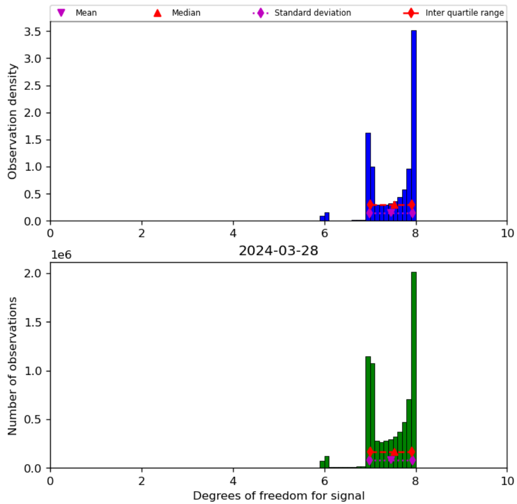
Figure 23: Histogram of “Degrees of freedom for signal” for 2024-03-27 to 2024-03-29
