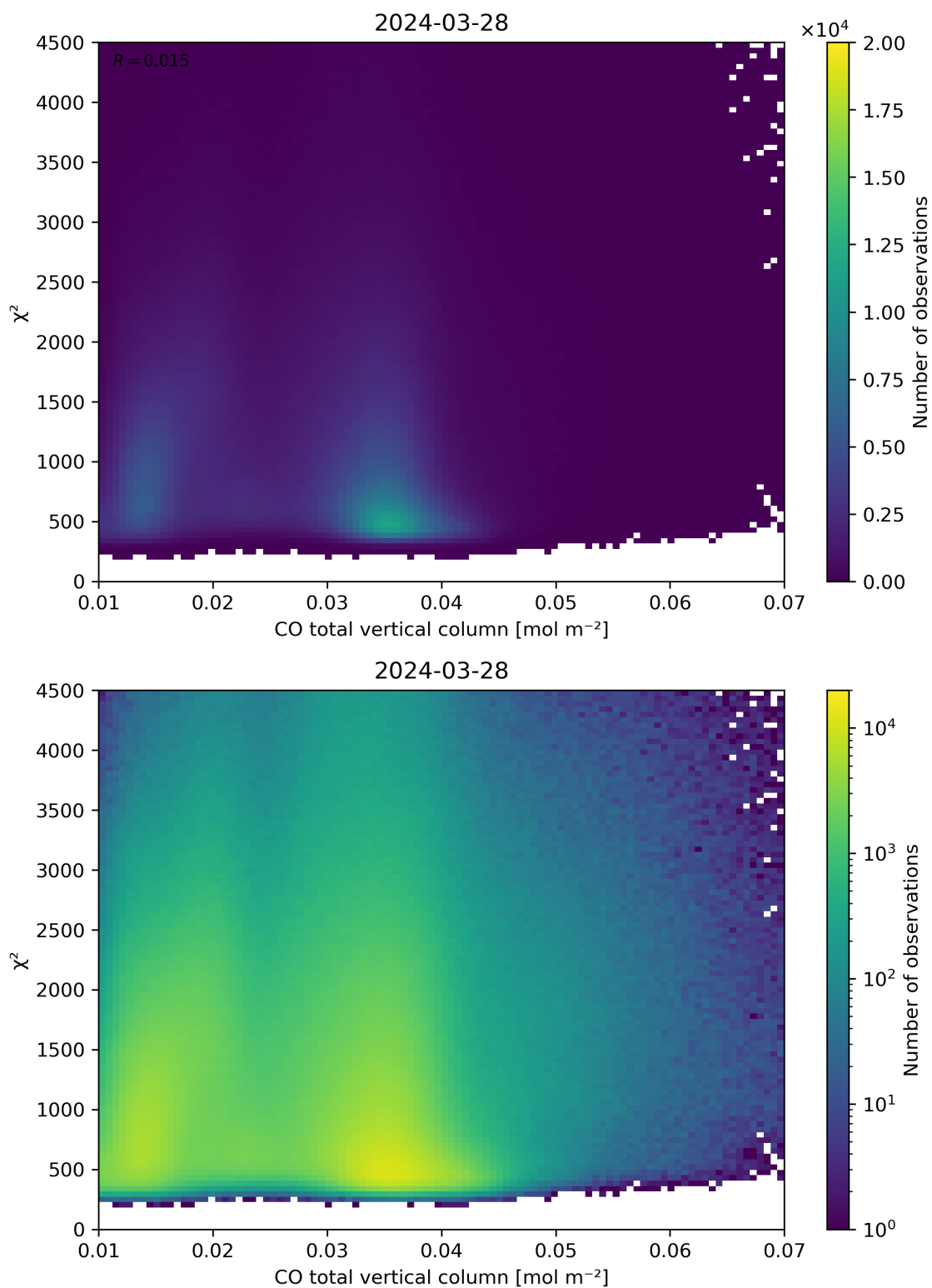
Figure 35: Scatter density plot of “CO total vertical column” against “ \chi^2 ” for 2024-03-27 to 2024-03-29.
