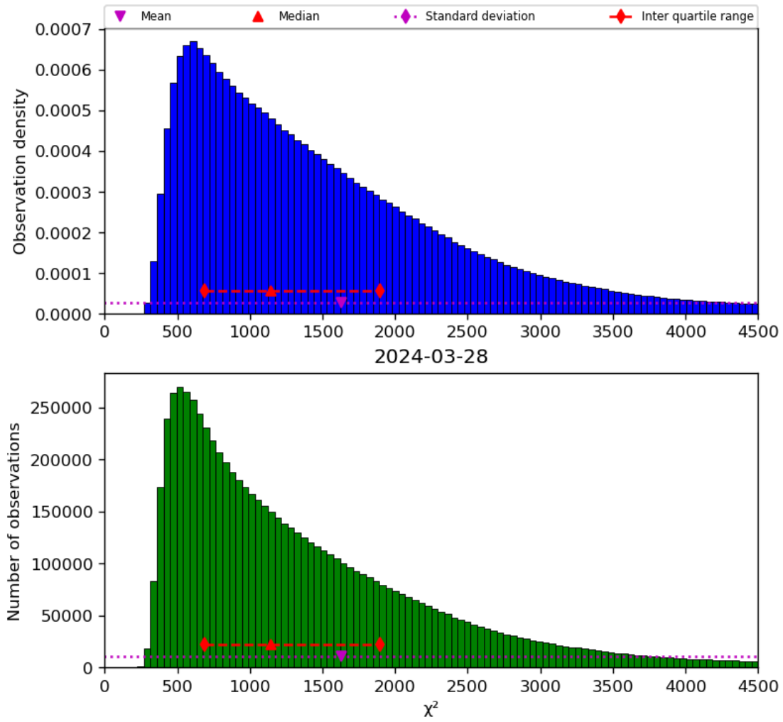
Figure 22: Histogram of “ \chi^2 ” for 2024-03-27 to 2024-03-29
