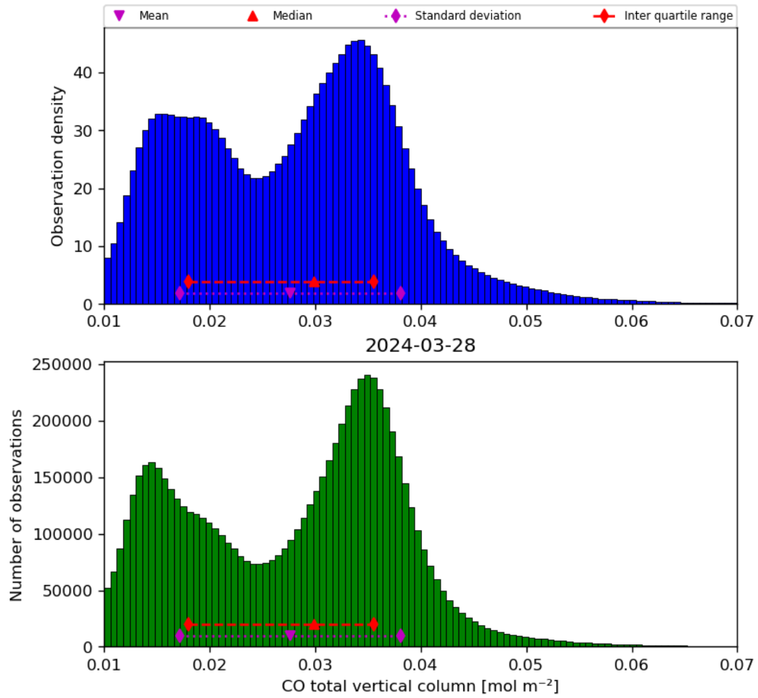
Figure 18: Histogram of “CO total vertical column” for 2024-03-27 to 2024-03-29
