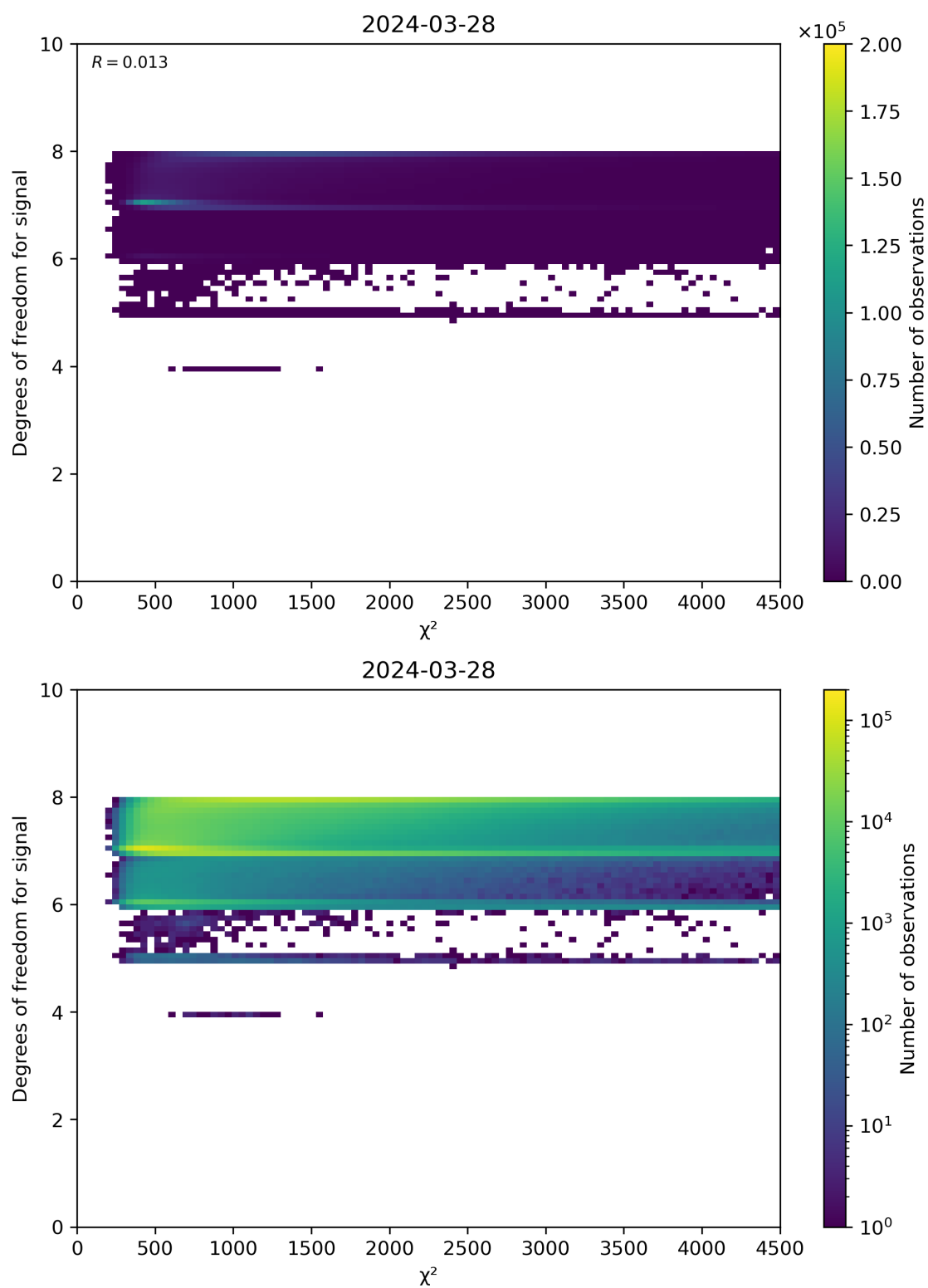
Figure 48: Scatter density plot of “ \chi^2 ” against “Degrees of freedom for signal” for 2024-03-27 to 2024-03-29.
