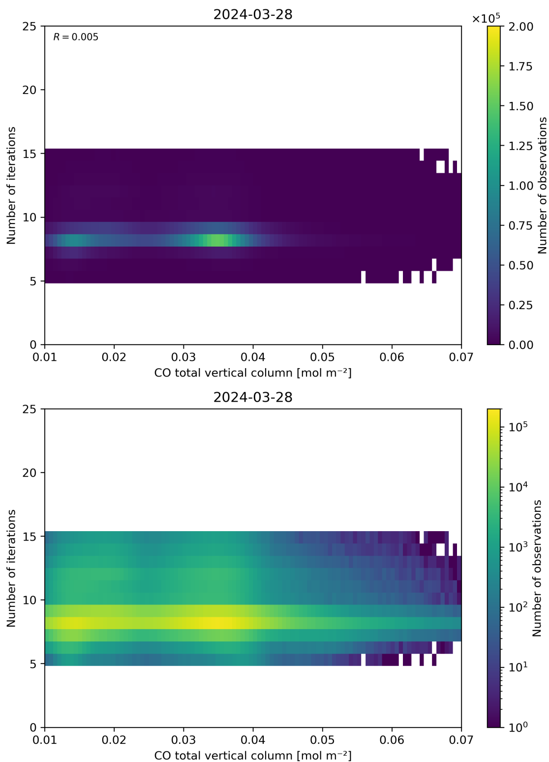
Figure 42: Scatter density plot of “CO total vertical column” against “Number of iterations” for 2024-03-27 to 2024-03-29.
