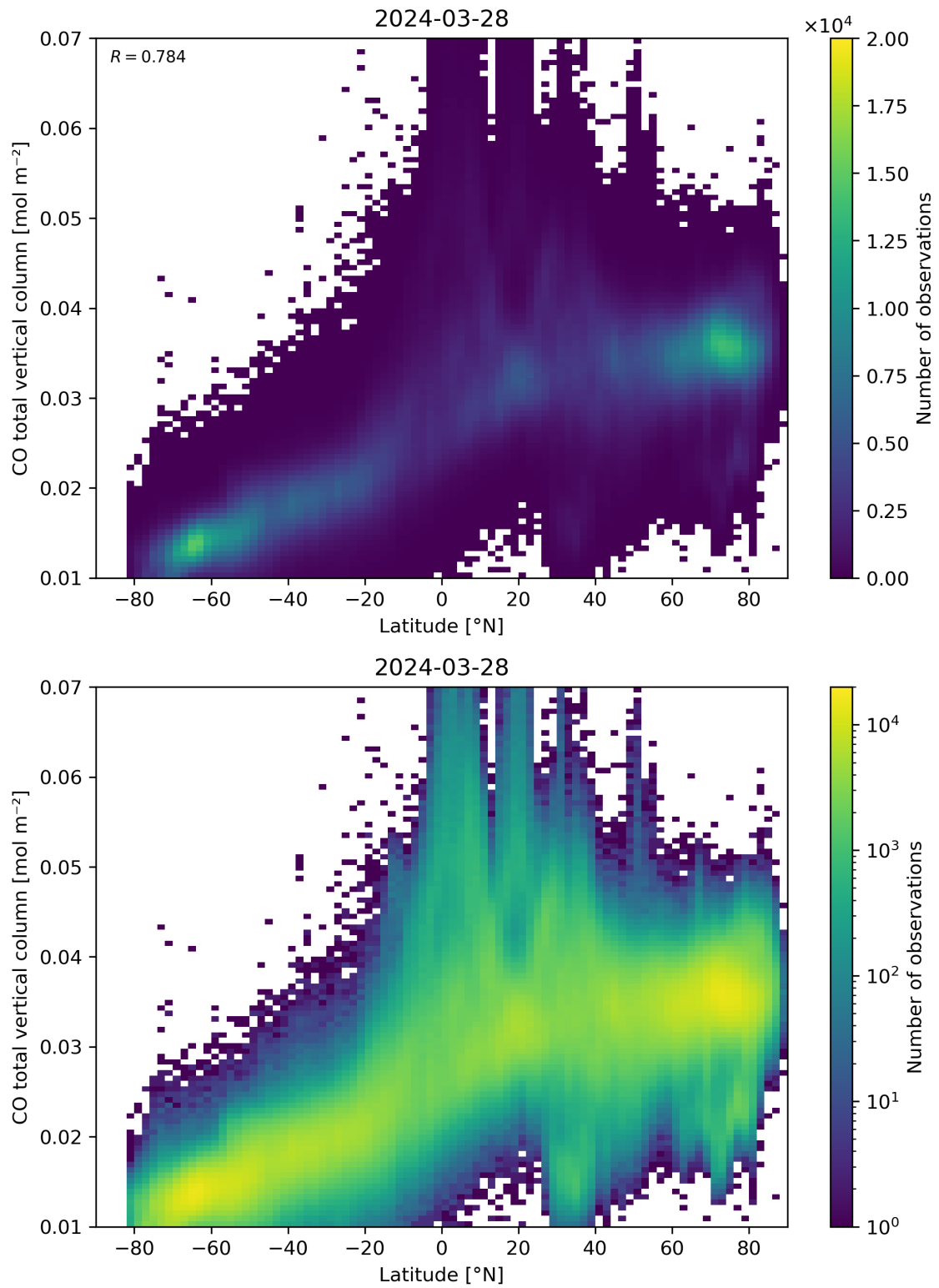
Figure 51: Scatter density plot of “Latitude” against “CO total vertical column” for 2024-03-27 to 2024-03-29.
