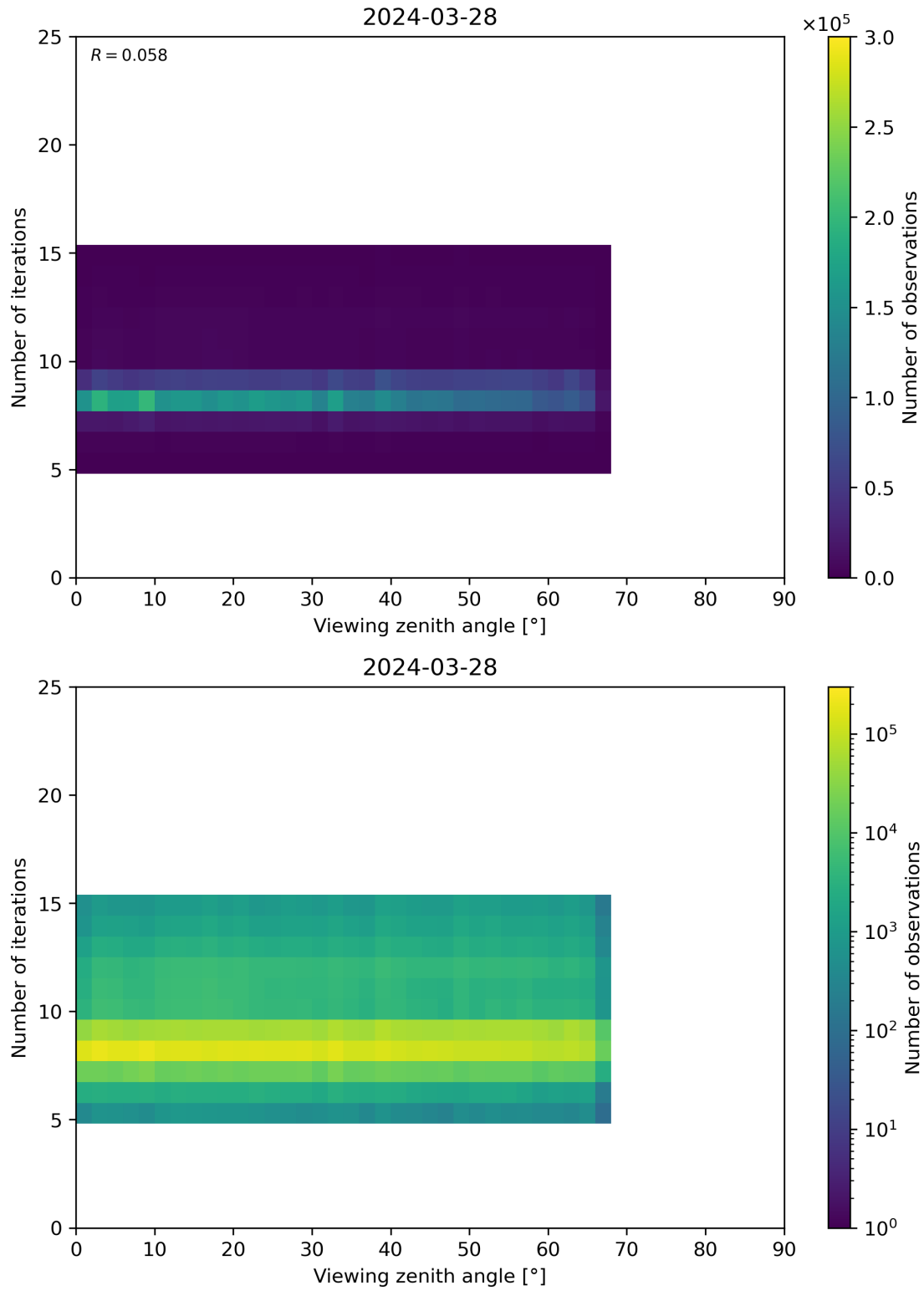
Figure 75: Scatter density plot of “Viewing zenith angle” against “Number of iterations” for 2024-03-27 to 2024-03-29.
