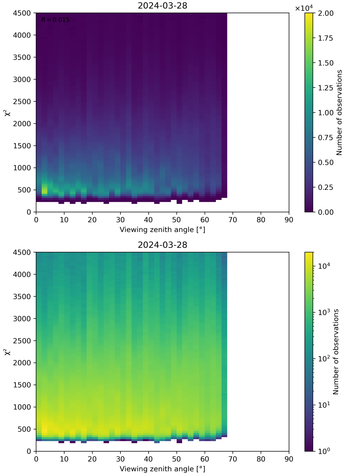
Figure 72: Scatter density plot of “Viewing zenith angle” against “ \chi^2 ” for 2024-03-27 to 2024-03-29.
