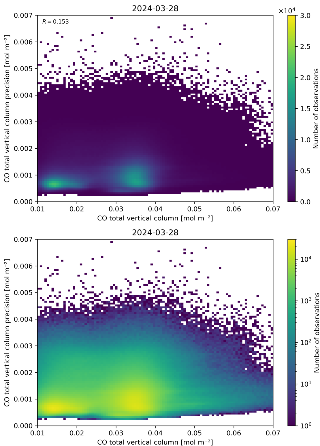
Figure 34: Scatter density plot of “CO total vertical column” against “CO total vertical column precision” for 2024-03-27 to 2024-03-29.
