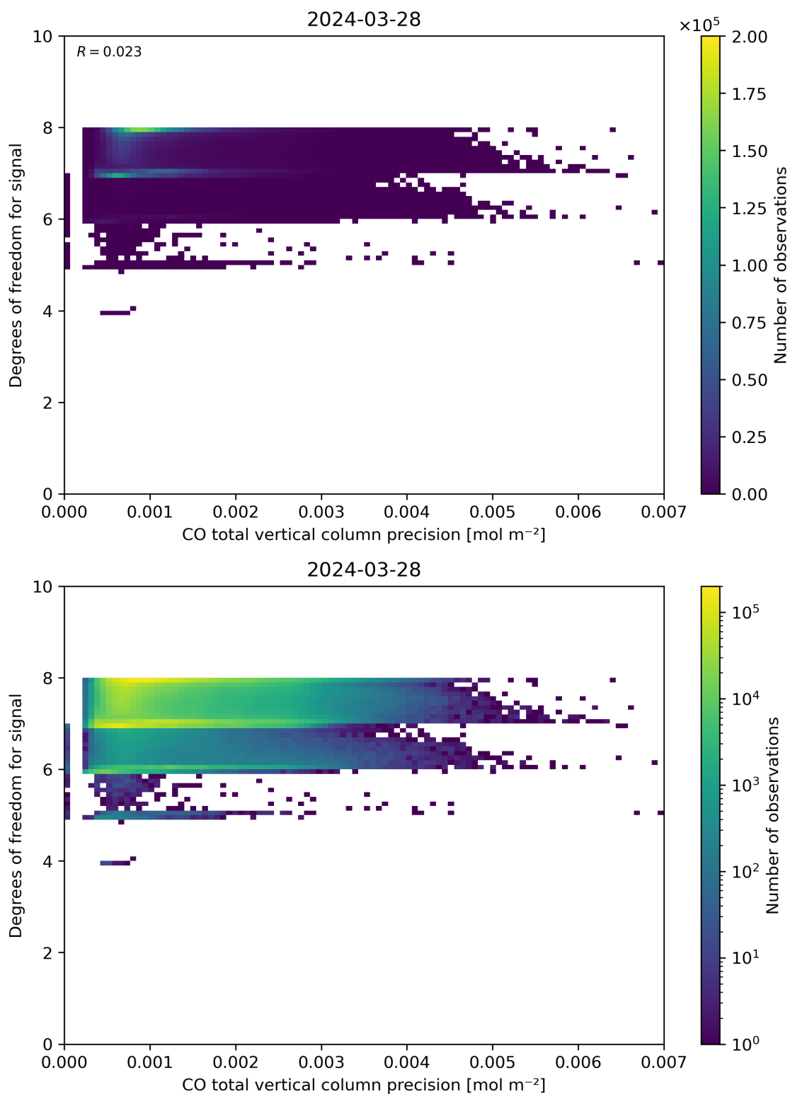
Figure 45: Scatter density plot of “CO total vertical column precision” against “Degrees of freedom for signal” for 2024-03-27 to 2024-03-29.
