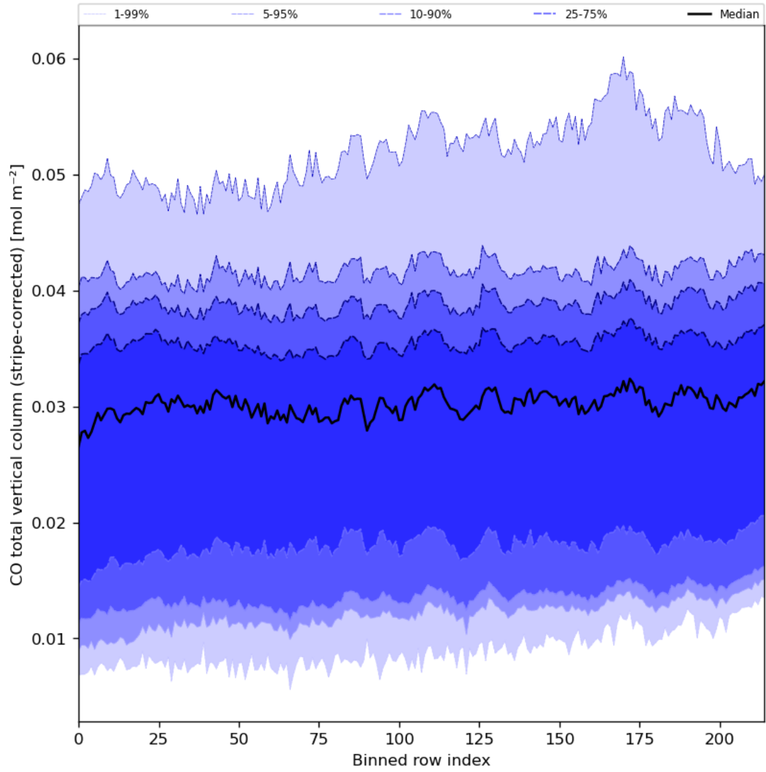
Figure 27: Along track statistics of “CO total vertical column (stripe-corrected)” for 2024-03-27 to 2024-03-29
