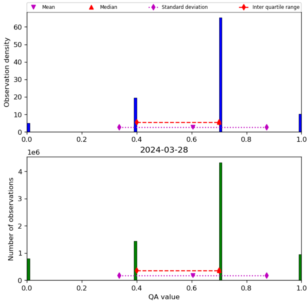
Figure 17: Histogram of “QA value” for 2024-03-27 to 2024-03-29
