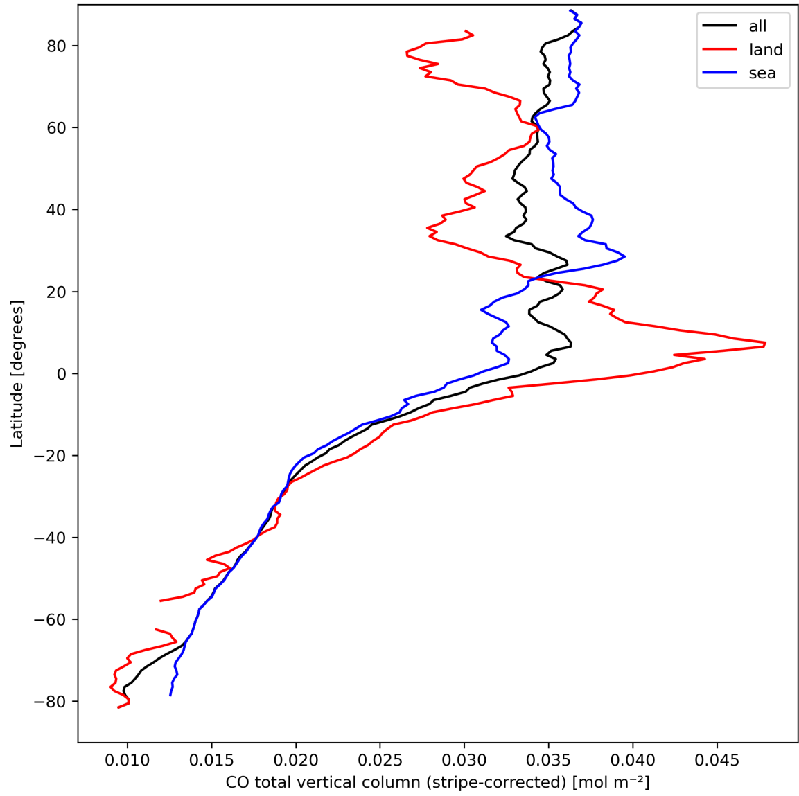
Figure 11: Zonal average of “CO total vertical column (stripe-corrected)” for 2024-03-27 to 2024-03-29.
