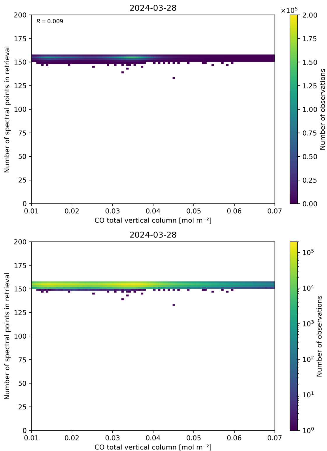
Figure 43: Scatter density plot of “CO total vertical column” against “Number of spectral points in retrieval” for 2024-03-27 to 2024-03-29.
