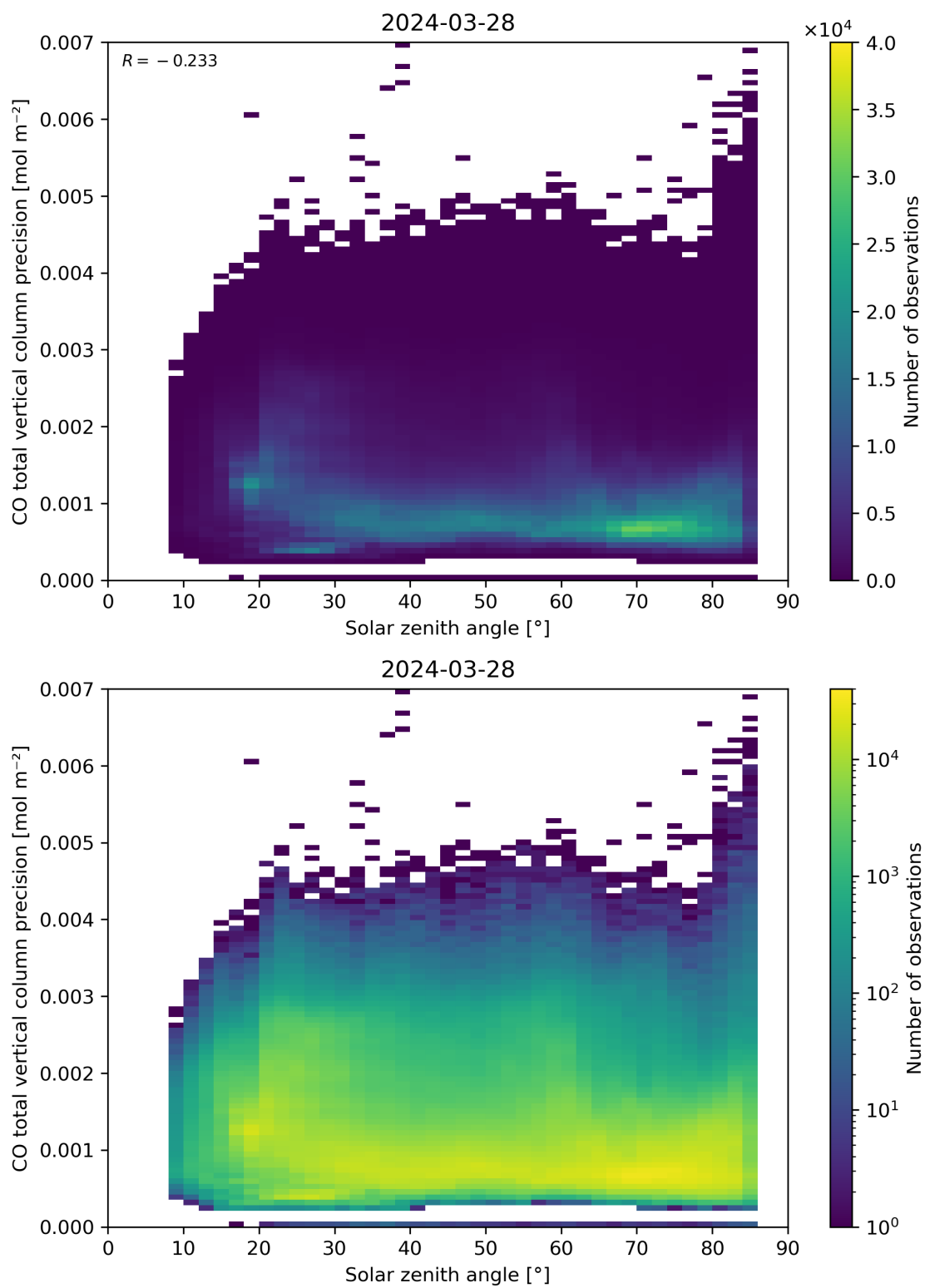
Figure 63: Scatter density plot of “Solar zenith angle” against “CO total vertical column precision” for 2024-03-27 to 2024-03-29.
