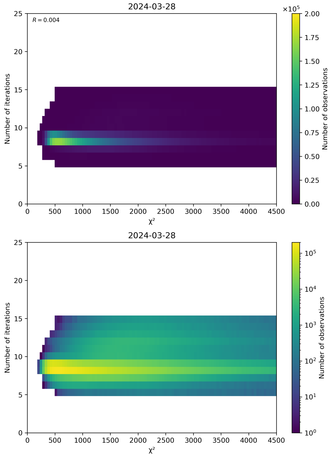
Figure 49: Scatter density plot of “ \chi^2 ” against “Number of iterations” for 2024-03-27 to 2024-03-29.
