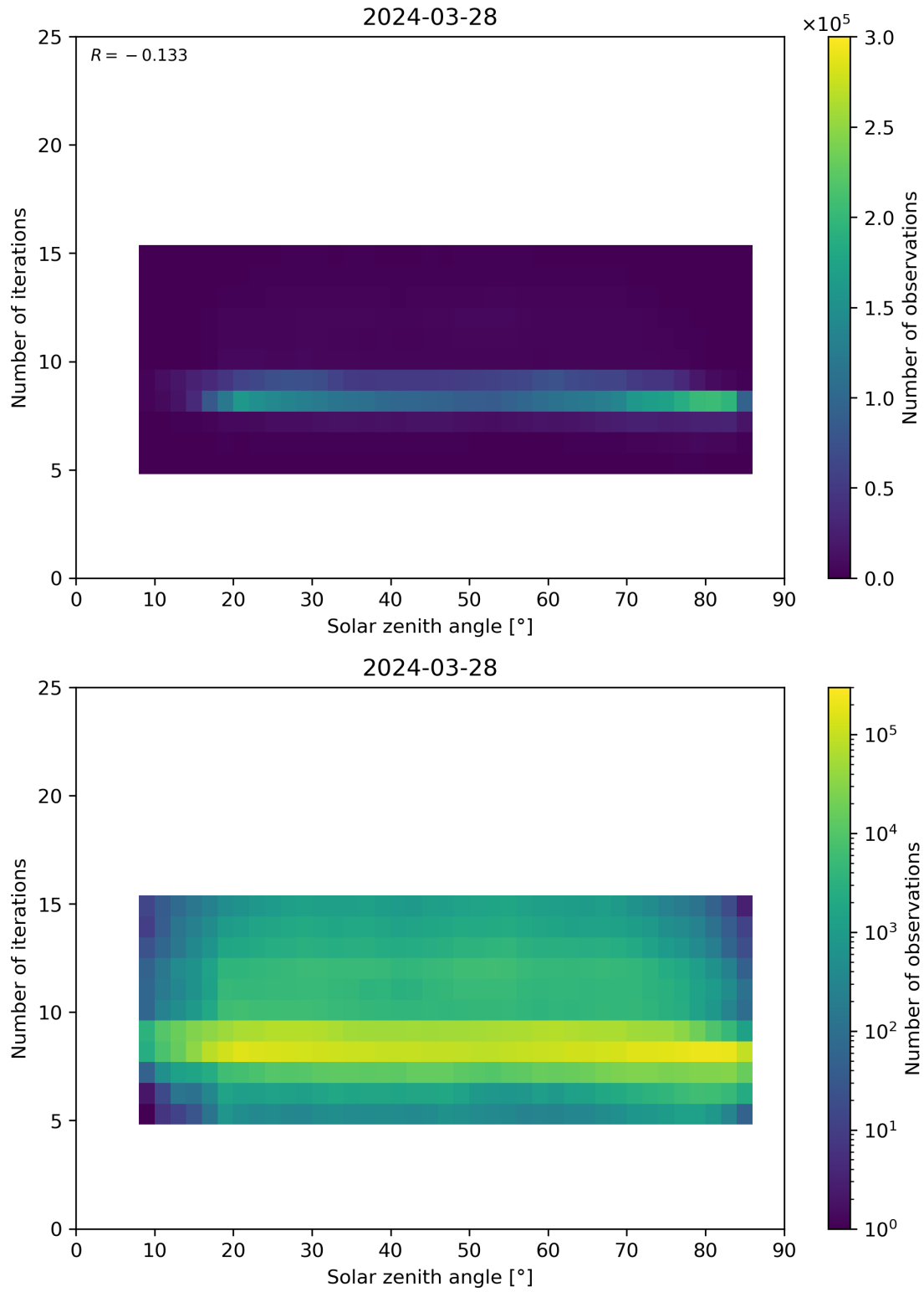
Figure 67: Scatter density plot of “Solar zenith angle” against “Number of iterations” for 2024-03-27 to 2024-03-29.
