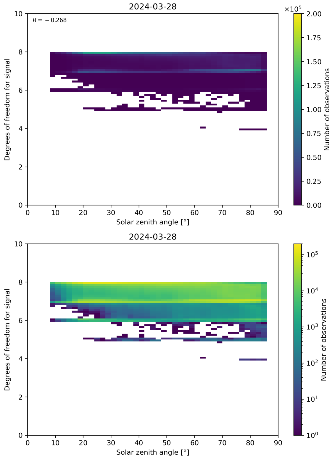
Figure 65: Scatter density plot of “Solar zenith angle” against “Degrees of freedom for signal” for 2024-03-27 to 2024-03-29.
