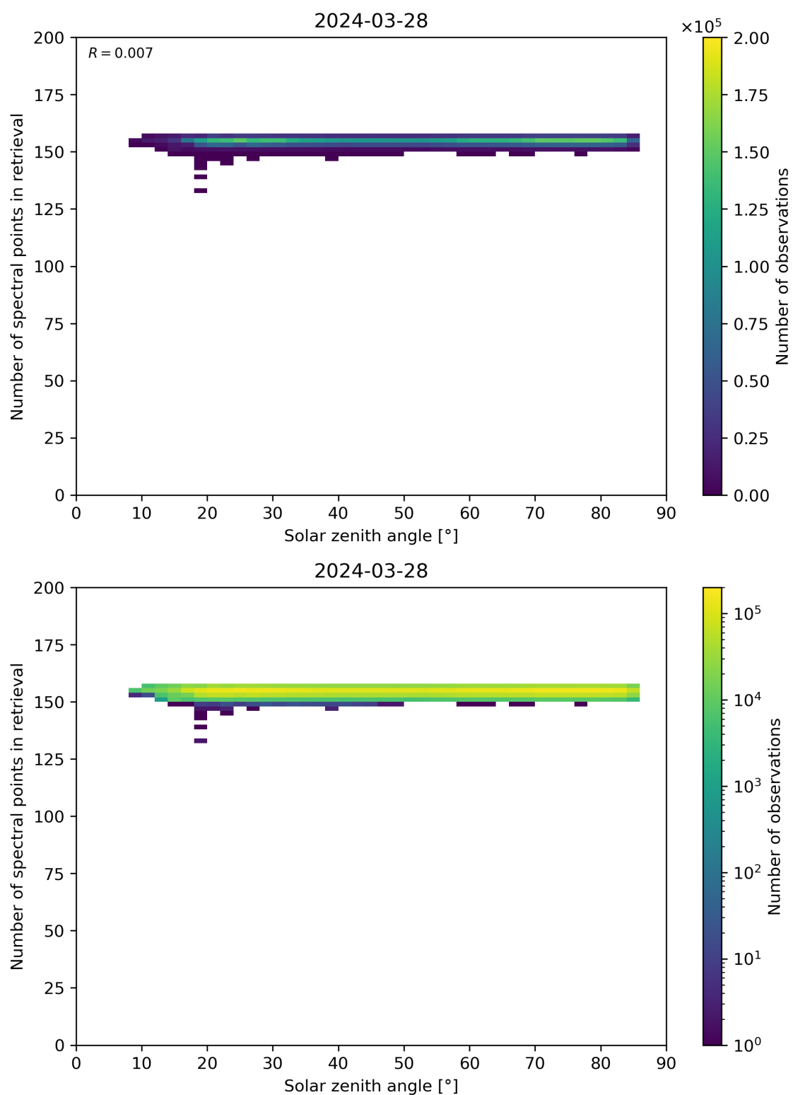
Figure 68: Scatter density plot of “Solar zenith angle” against “Number of spectral points in retrieval” for 2024-03-27 to 2024-03-29.
