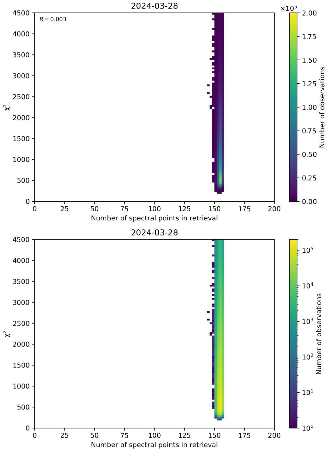
Figure 58: Scatter density plot of “Number of spectral points in retrieval” against “ \chi^2 ” for 2024-03-27 to 2024-03-29.
