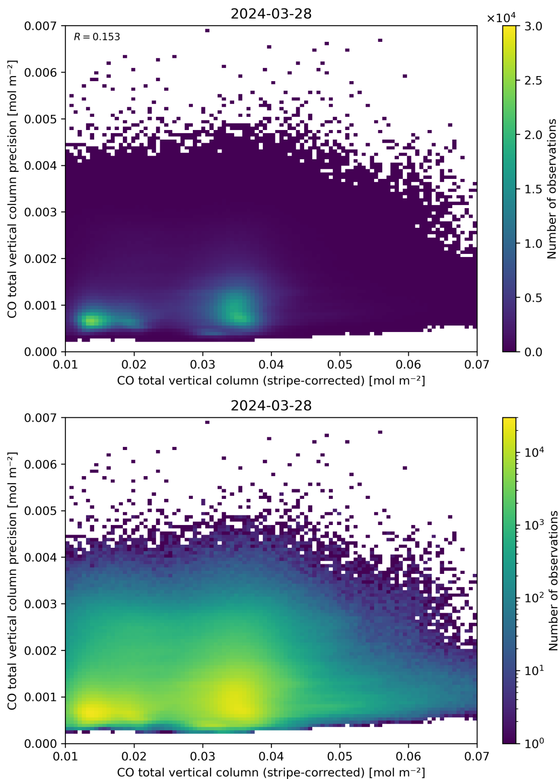
Figure 36: Scatter density plot of “CO total vertical column (stripe-corrected)” against “CO total vertical column precision” for 2024-03-27 to 2024-03-29.
