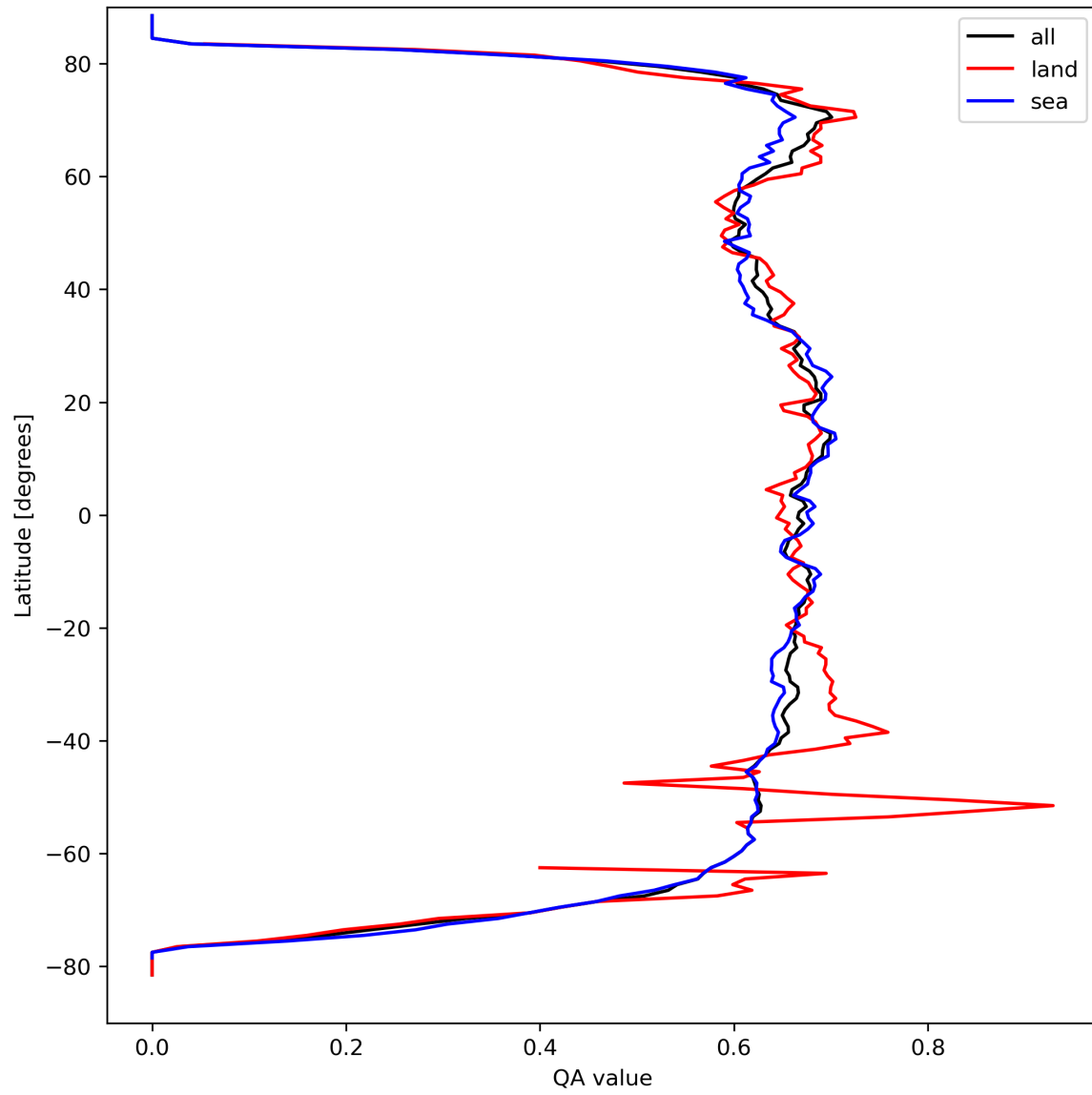
Figure 9: Zonal average of “QA value” for 2024-03-27 to 2024-03-29.
