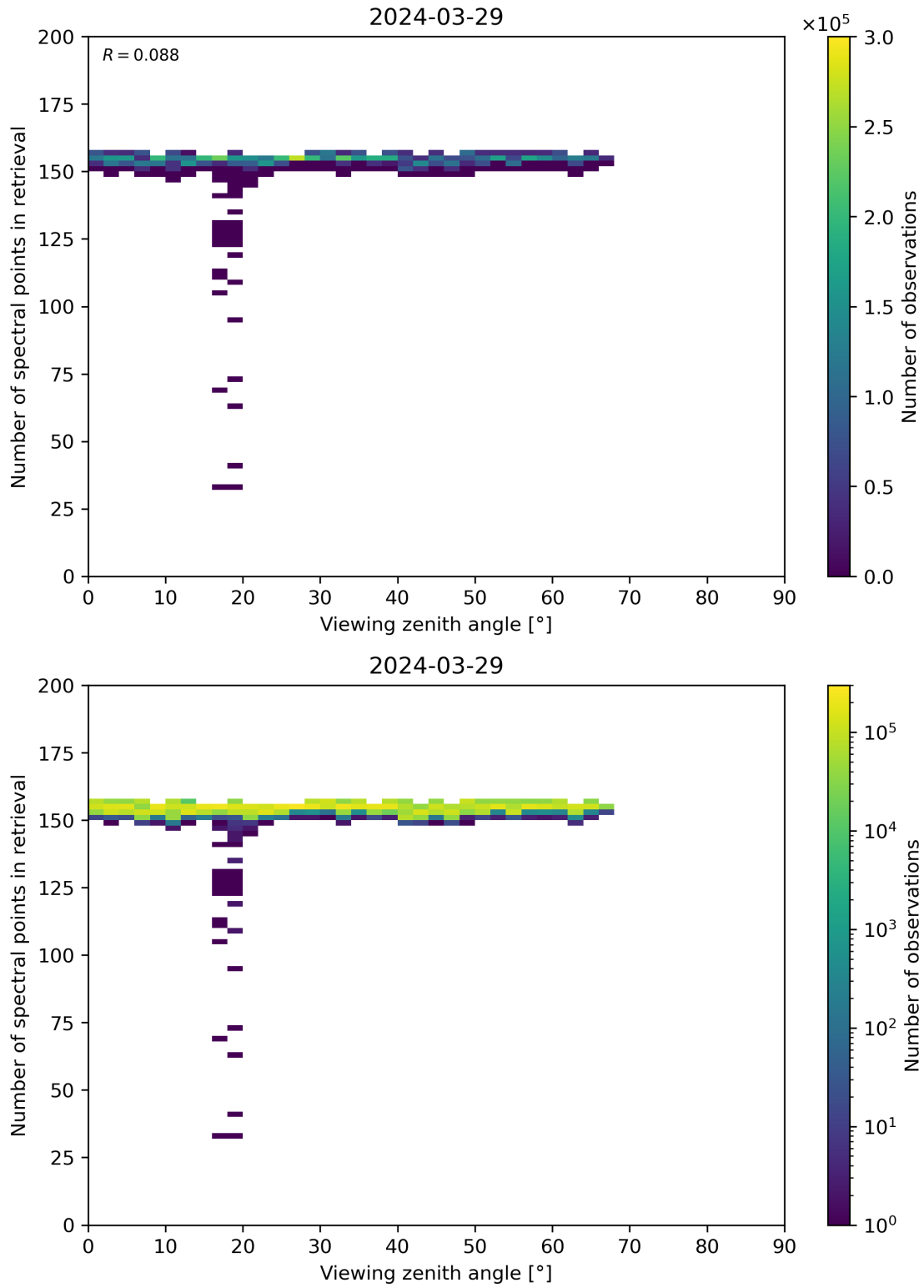
Figure 76: Scatter density plot of “Viewing zenith angle” against “Number of spectral points in retrieval” for 2024-03-28 to 2024-03-30.
