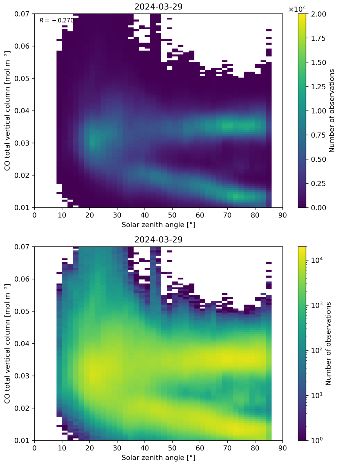
Figure 61: Scatter density plot of “Solar zenith angle” against “CO total vertical column” for 2024-03-28 to 2024-03-30.
