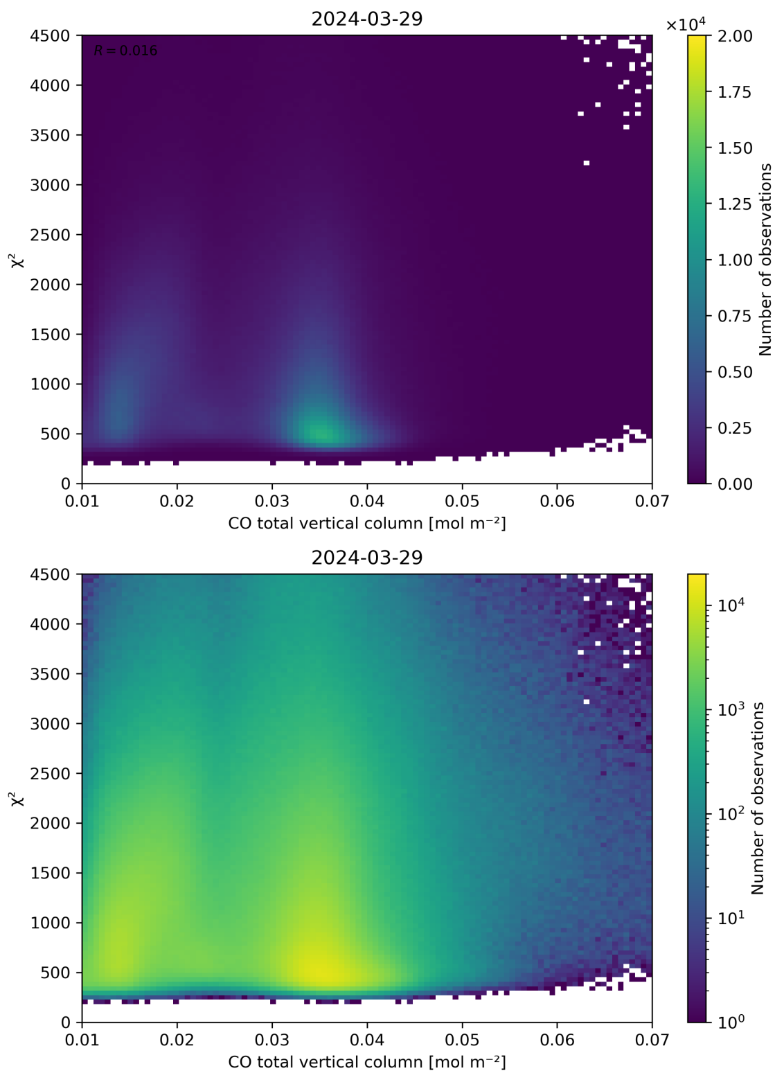
Figure 35: Scatter density plot of “CO total vertical column” against “ \chi^2 ” for 2024-03-28 to 2024-03-30.
