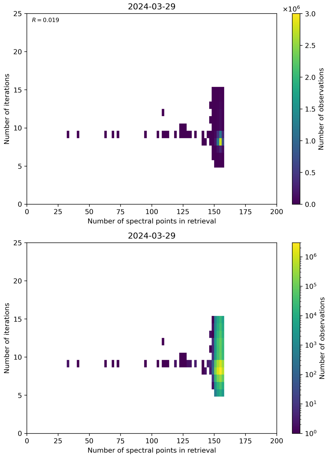
Figure 60: Scatter density plot of “Number of spectral points in retrieval” against “Number of iterations” for 2024-03-28 to 2024-03-30.
