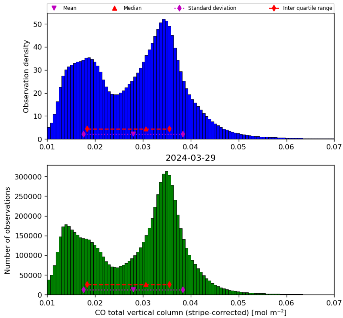
Figure 19: Histogram of “CO total vertical column (stripe-corrected)” for 2024-03-28 to 2024-03-30
