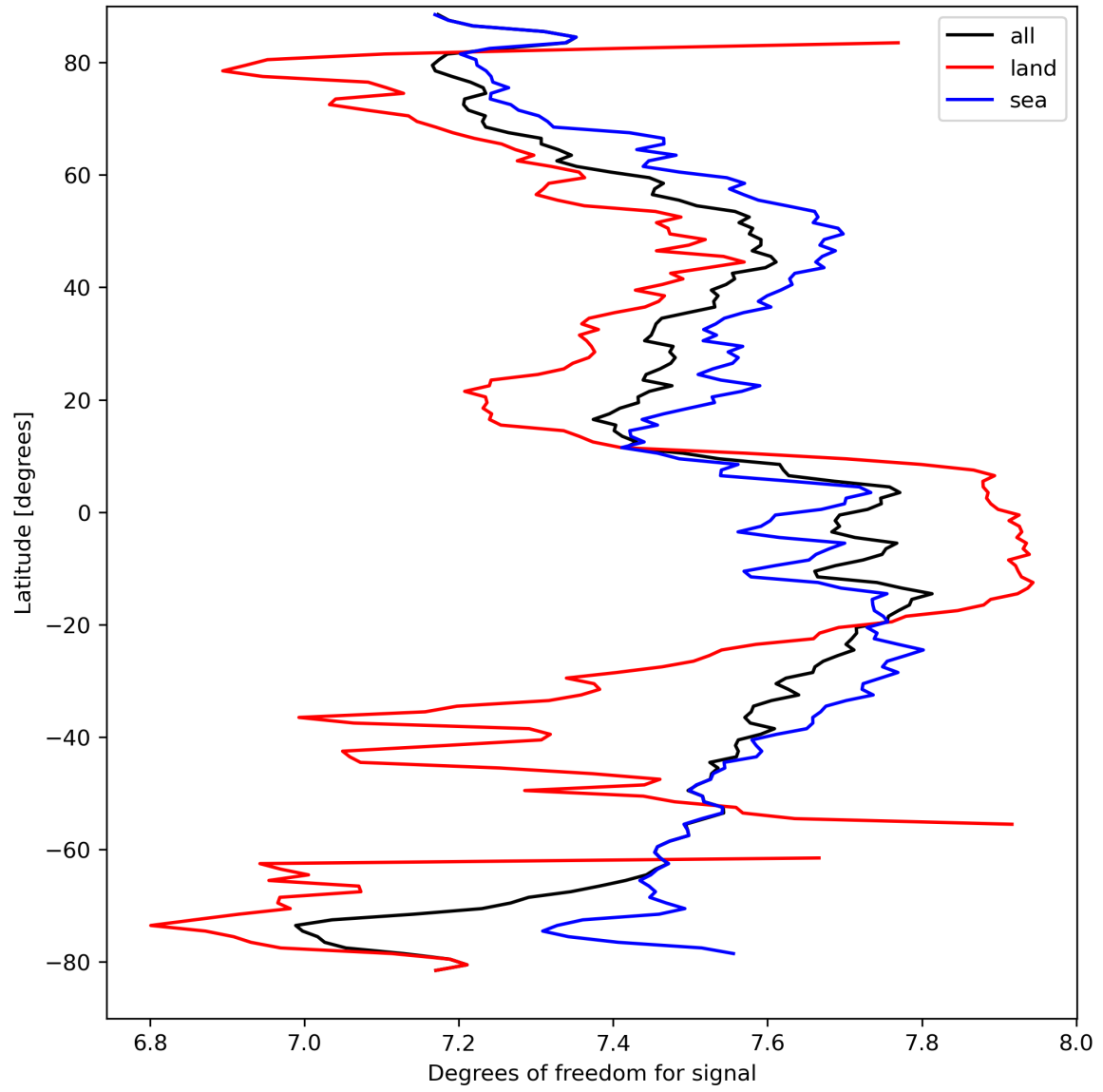
Figure 15: Zonal average of “Degrees of freedom for signal” for 2024-03-28 to 2024-03-30.
