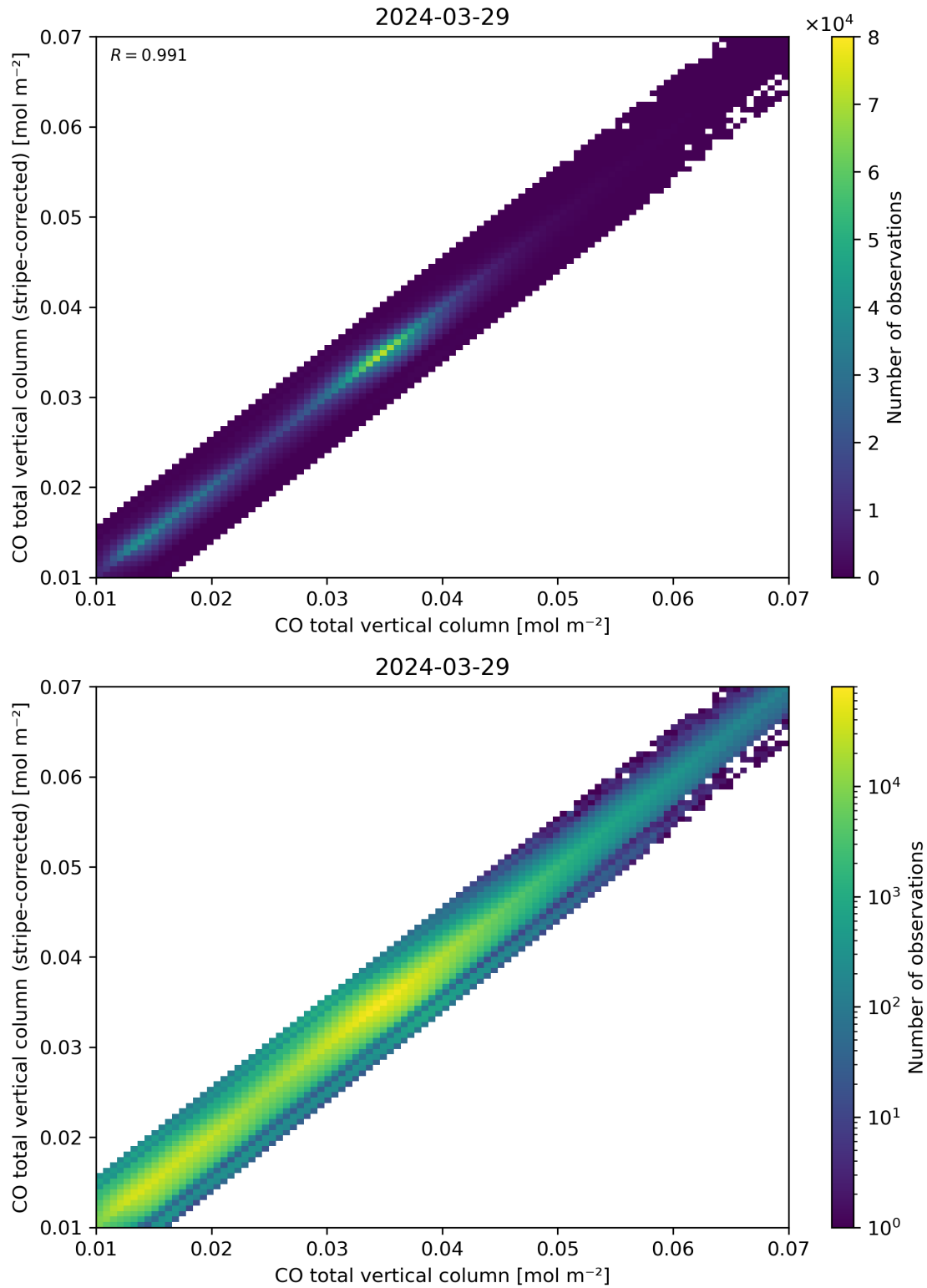
Figure 33: Scatter density plot of “CO total vertical column” against “CO total vertical column (stripe-corrected)” for 2024-03-28 to 2024-03-30.
