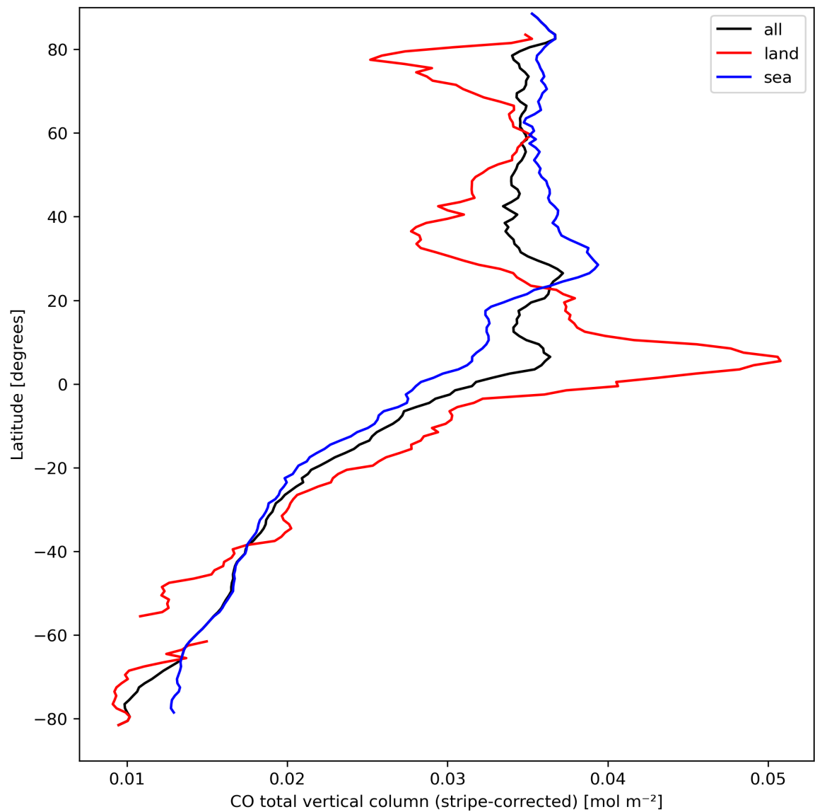
Figure 11: Zonal average of “CO total vertical column (stripe-corrected)” for 2024-03-28 to 2024-03-30.
