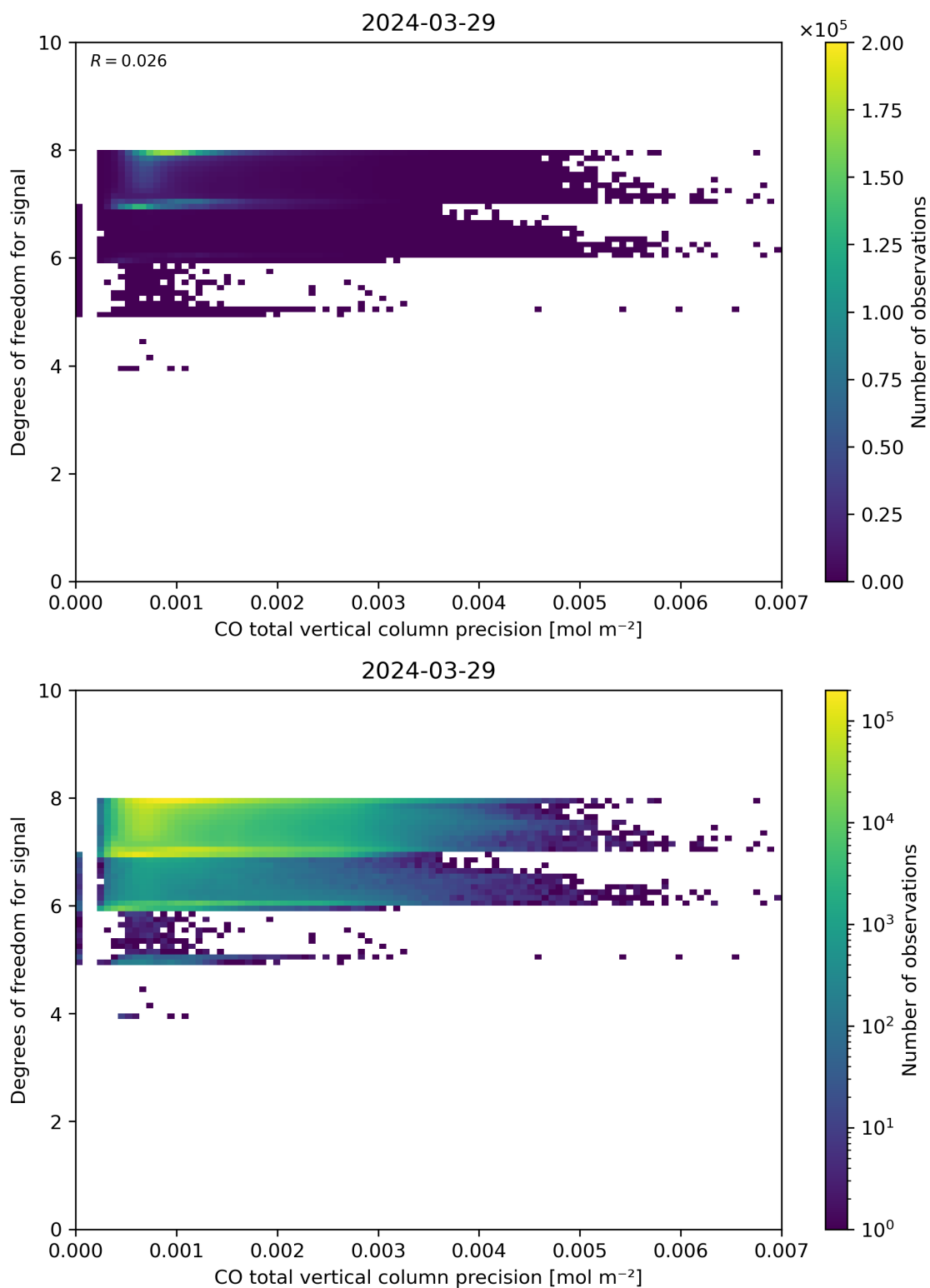
Figure 45: Scatter density plot of “CO total vertical column precision” against “Degrees of freedom for signal” for 2024-03-28 to 2024-03-30.
