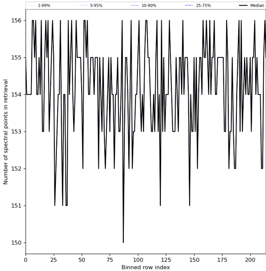
Figure 29: Along track statistics of “Number of spectral points in retrieval” for 2024-03-28 to 2024-03-30
