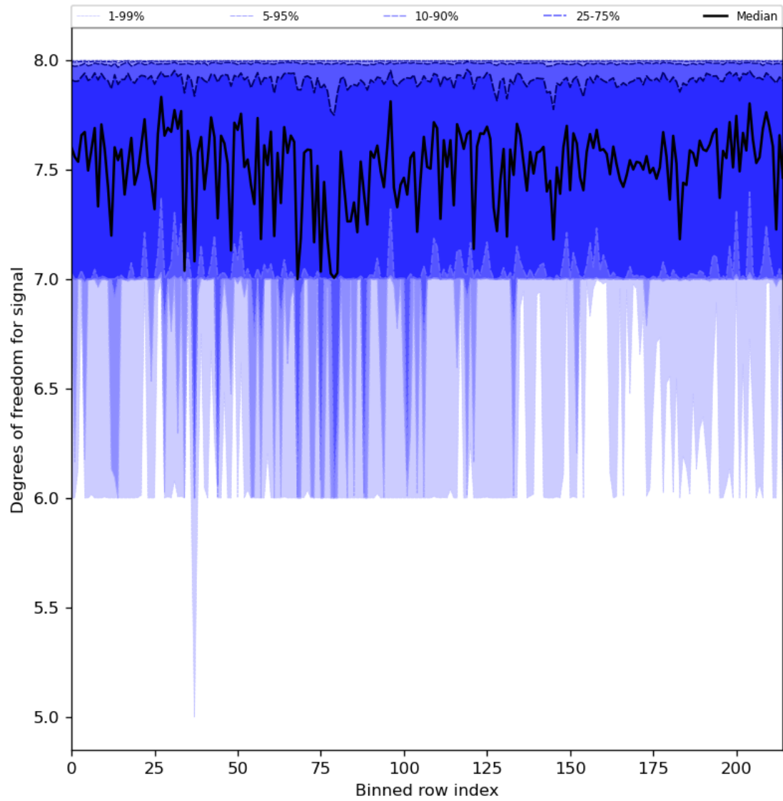
Figure 31: Along track statistics of “Degrees of freedom for signal” for 2024-03-28 to 2024-03-30
