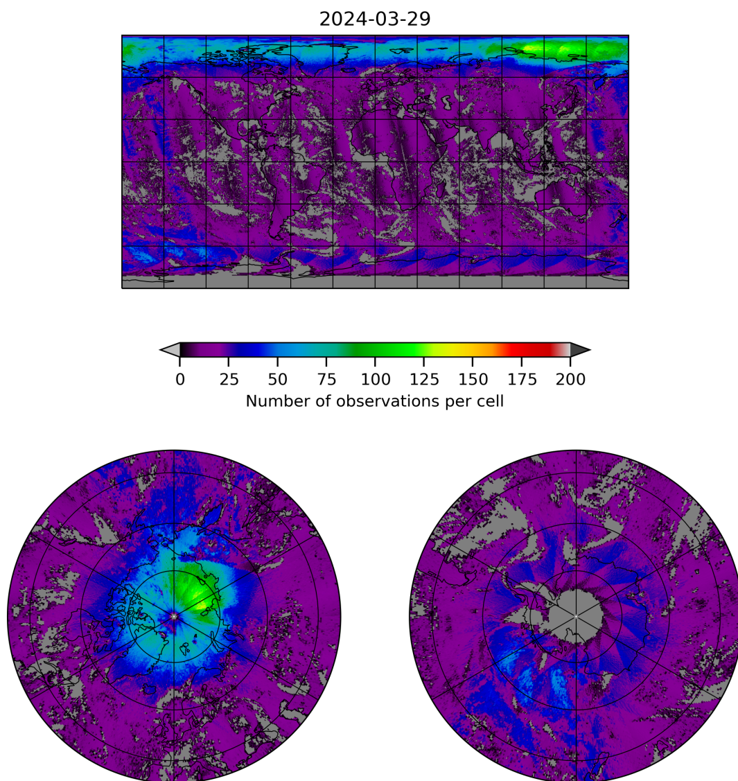
Figure 8: Map of the number of observations for 2024-03-28 to 2024-03-30
