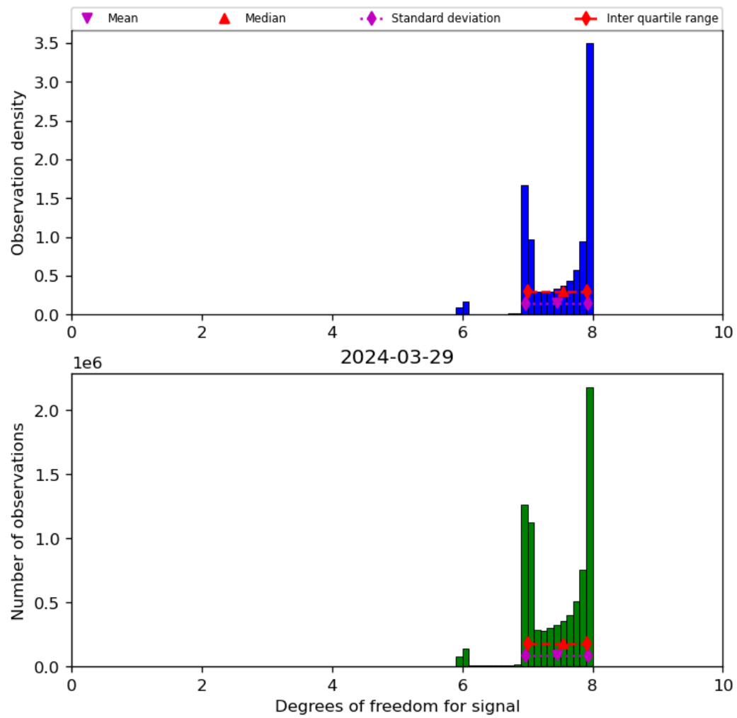
Figure 23: Histogram of “Degrees of freedom for signal” for 2024-03-28 to 2024-03-30
