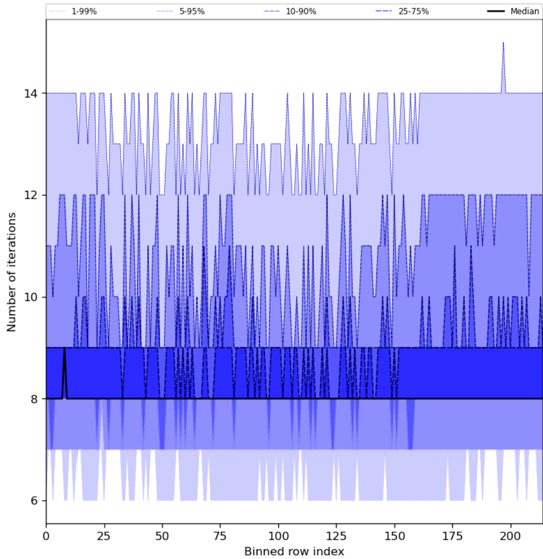
Figure 32: Along track statistics of “Number of iterations” for 2024-03-28 to 2024-03-30
