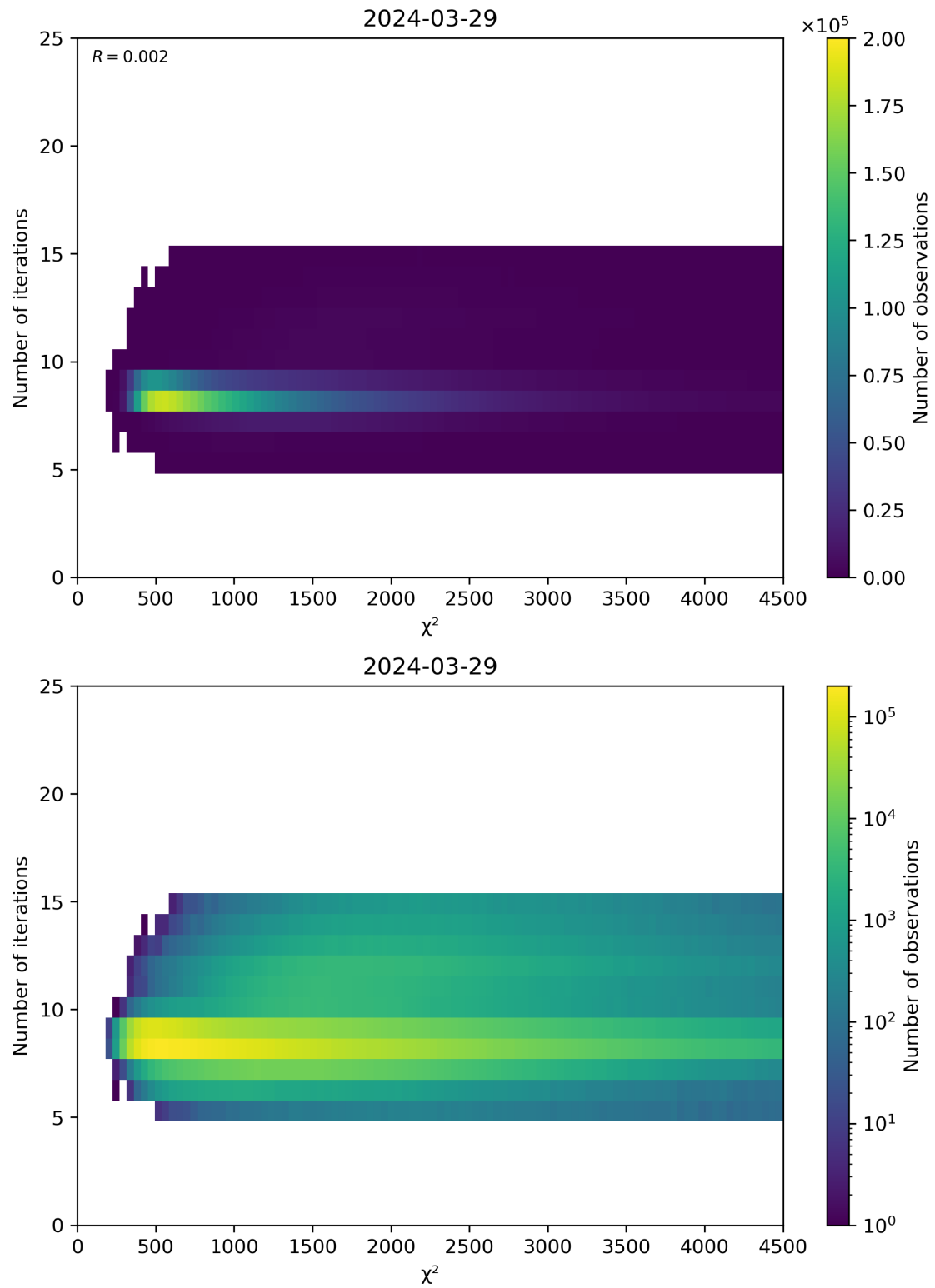
Figure 49: Scatter density plot of “ \chi^2 ” against “Number of iterations” for 2024-03-28 to 2024-03-30.
