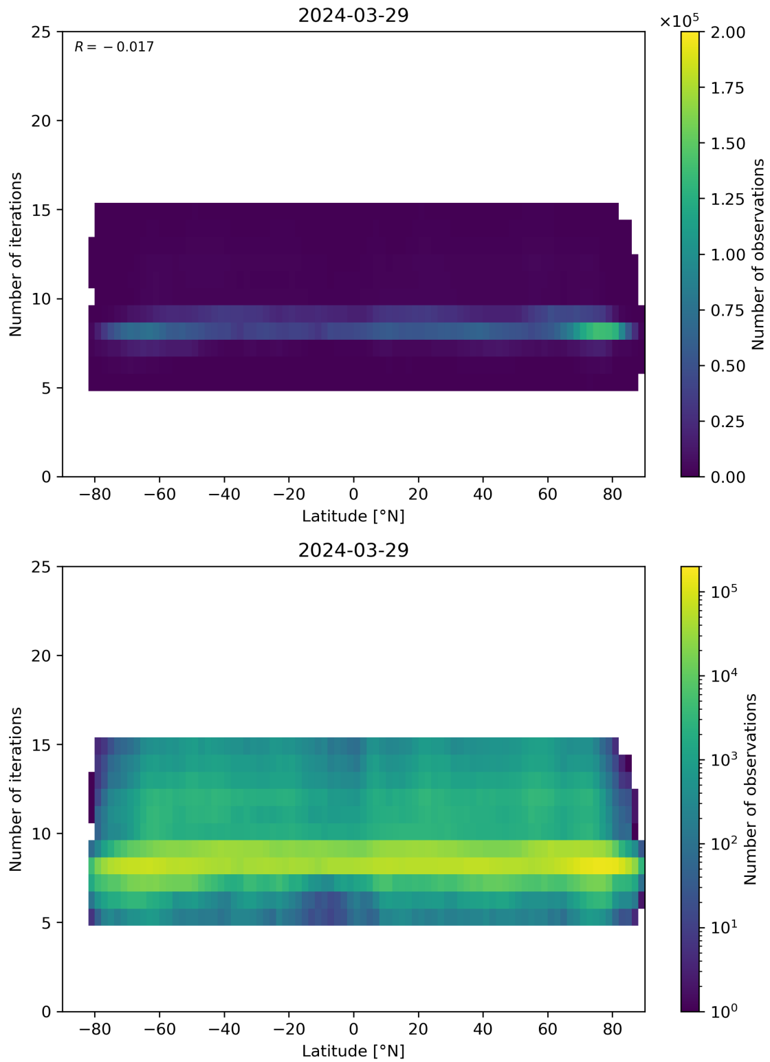
Figure 56: Scatter density plot of “Latitude” against “Number of iterations” for 2024-03-28 to 2024-03-30.
