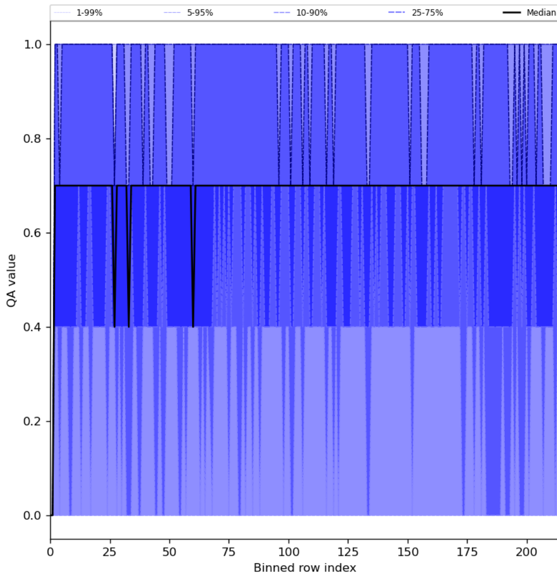
Figure 25: Along track statistics of “QA value” for 2024-03-28 to 2024-03-30
