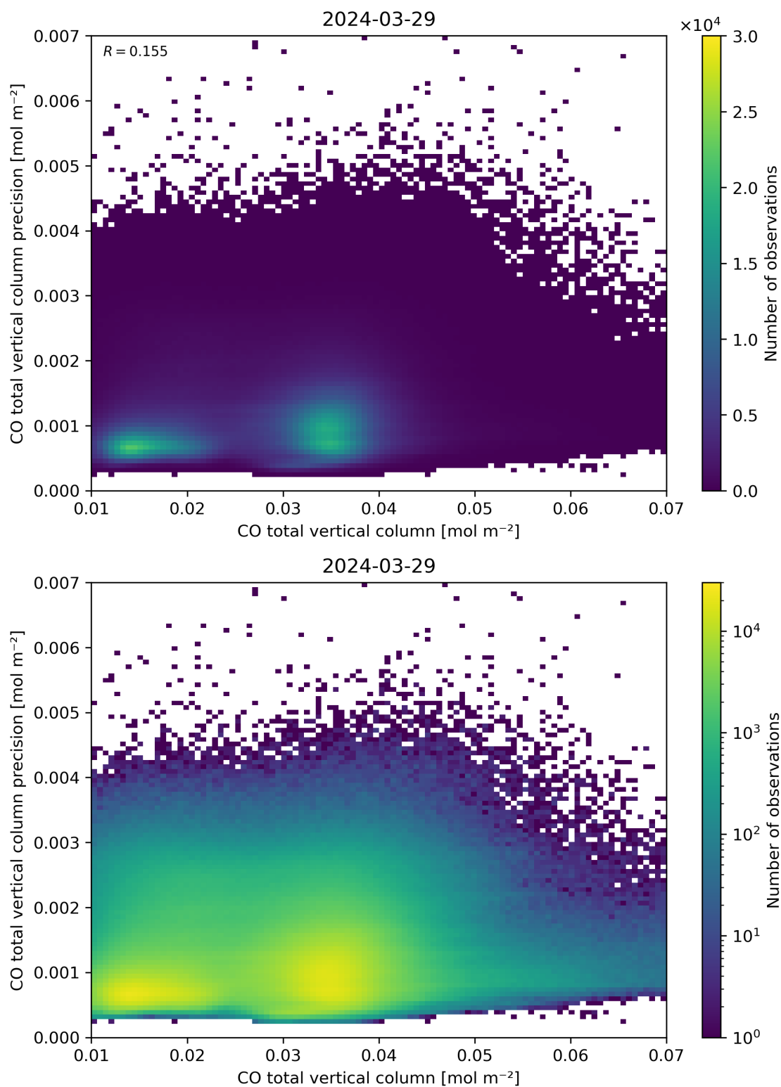
Figure 34: Scatter density plot of “CO total vertical column” against “CO total vertical column precision” for 2024-03-28 to 2024-03-30.
