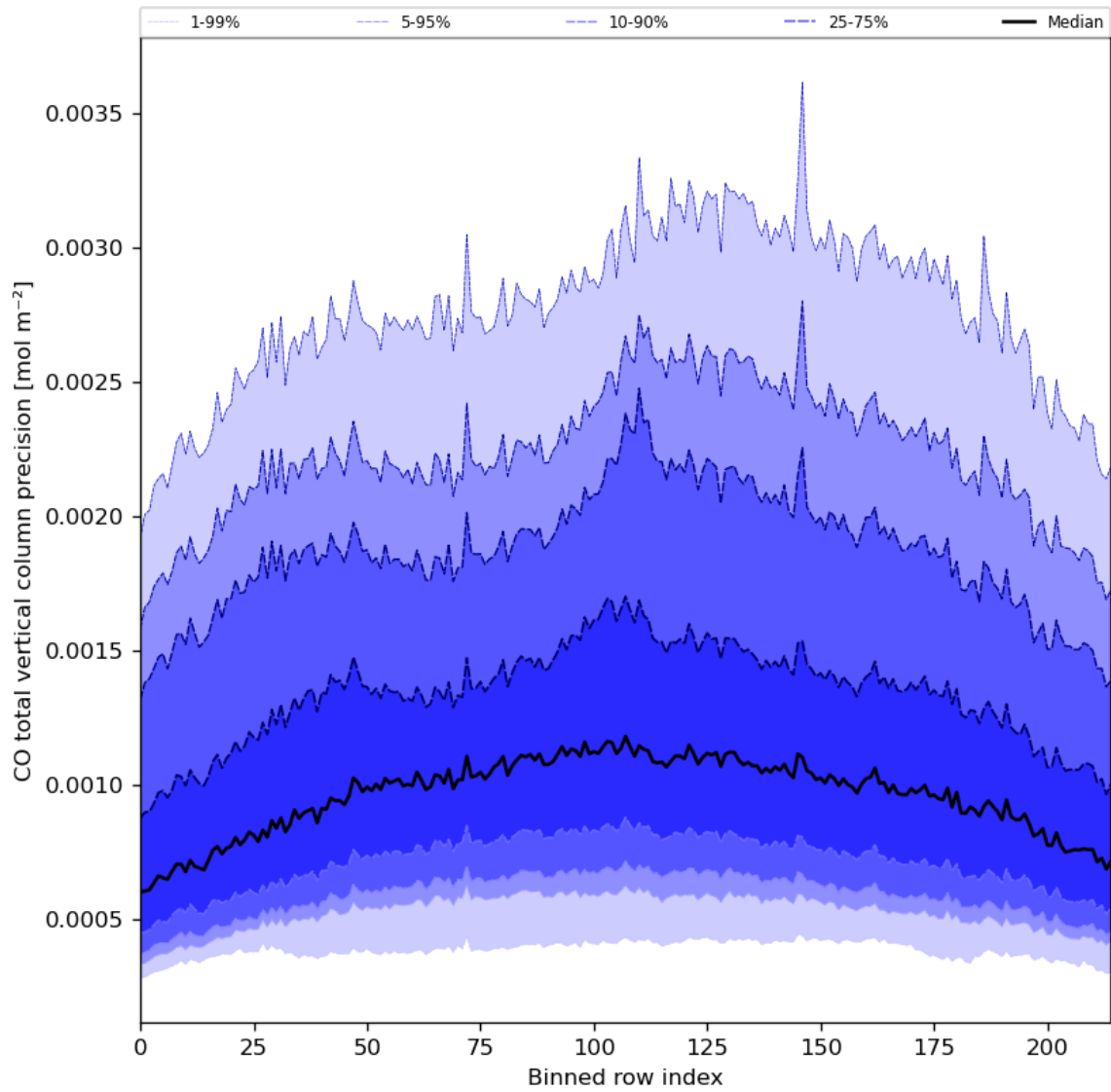
Figure 28: Along track statistics of “CO total vertical column precision” for 2024-03-28 to 2024-03-30
