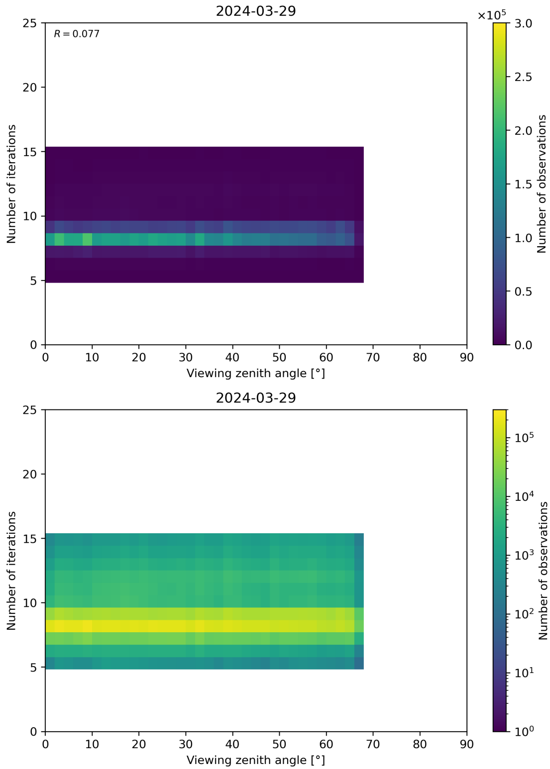
Figure 75: Scatter density plot of “Viewing zenith angle” against “Number of iterations” for 2024-03-28 to 2024-03-30.
