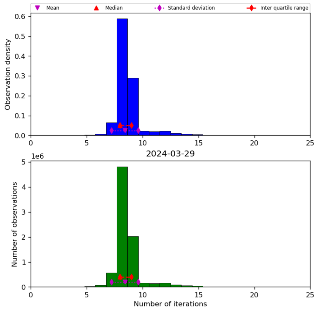
Figure 24: Histogram of “Number of iterations” for 2024-03-28 to 2024-03-30
