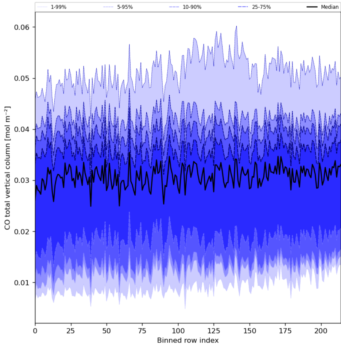
Figure 26: Along track statistics of “CO total vertical column” for 2024-03-28 to 2024-03-30
