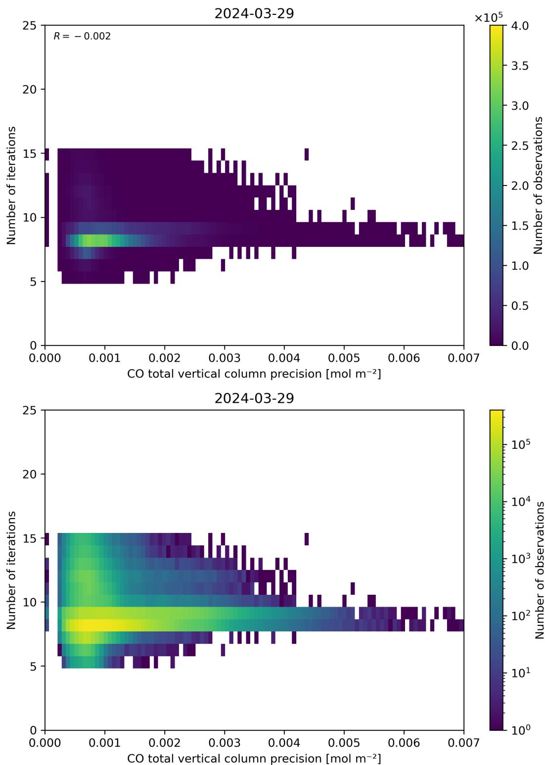
Figure 46: Scatter density plot of “CO total vertical column precision” against “Number of iterations” for 2024-03-28 to 2024-03-30.
