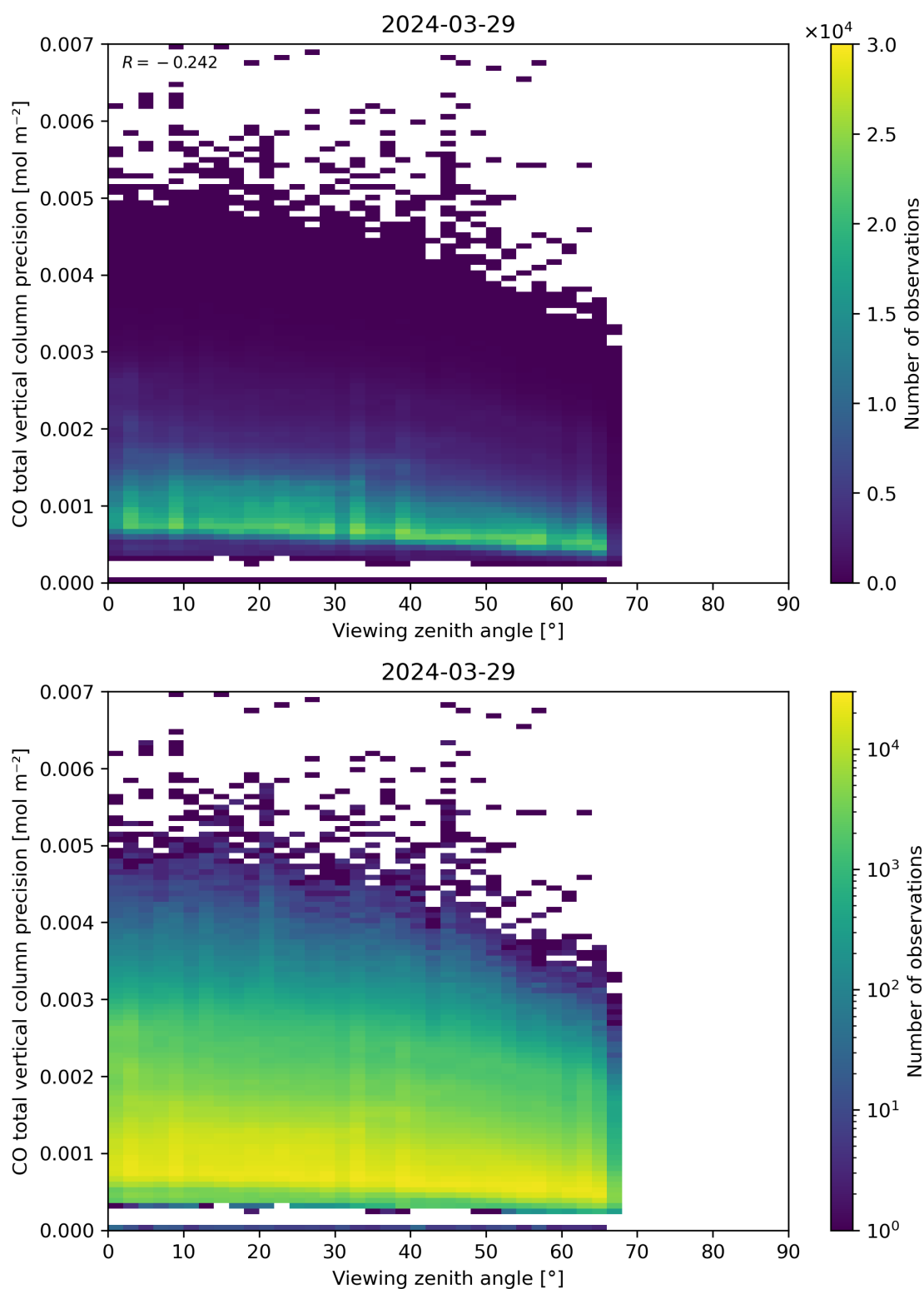
Figure 71: Scatter density plot of “Viewing zenith angle” against “CO total vertical column precision” for 2024-03-28 to 2024-03-30.
