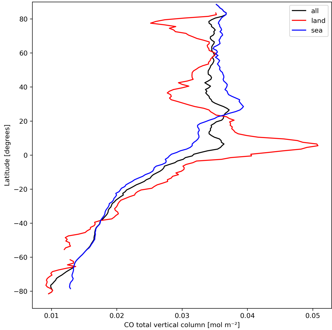
Figure 10: Zonal average of “CO total vertical column” for 2024-03-28 to 2024-03-30.
