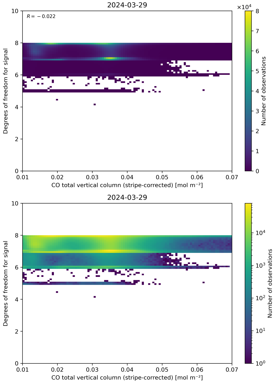
Figure 38: Scatter density plot of “CO total vertical column (stripe-corrected)” against “Degrees of freedom for signal” for 2024-03-28 to 2024-03-30.
