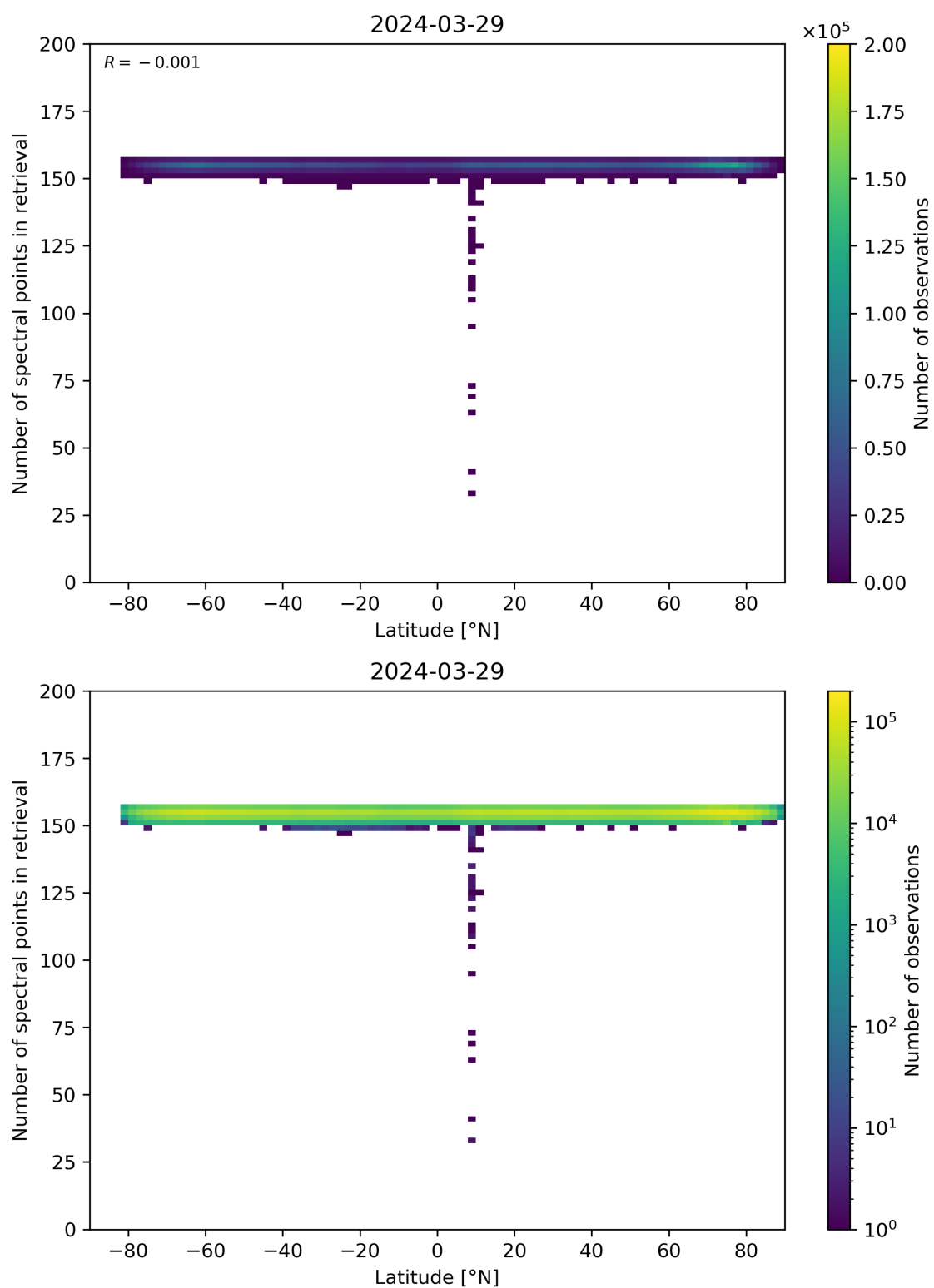
Figure 57: Scatter density plot of “Latitude” against “Number of spectral points in retrieval” for 2024-03-28 to 2024-03-30.
