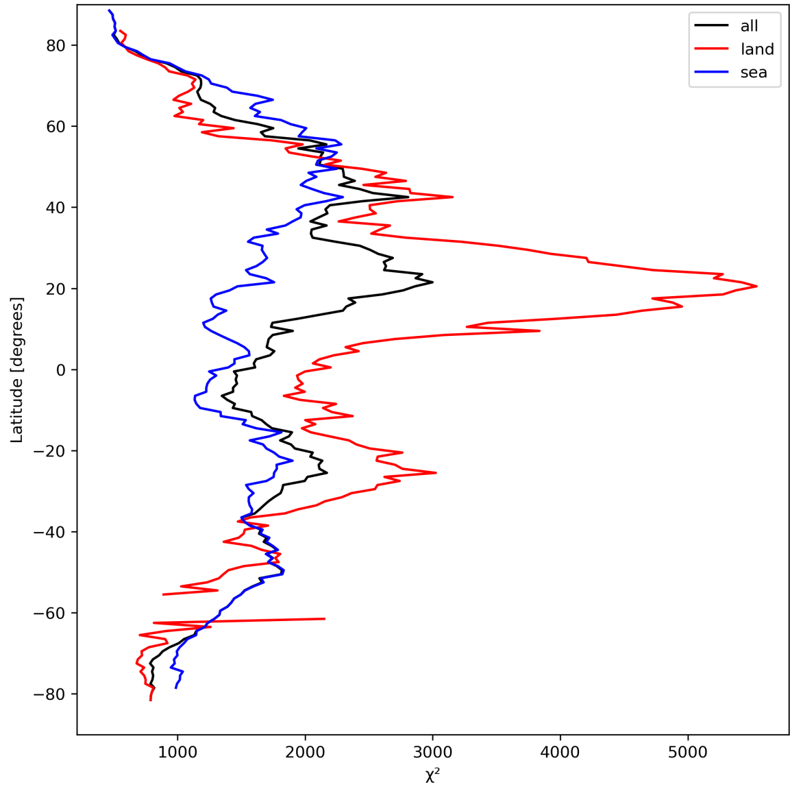
Figure 14: Zonal average of “ \chi^2 ” for 2024-03-28 to 2024-03-30.
