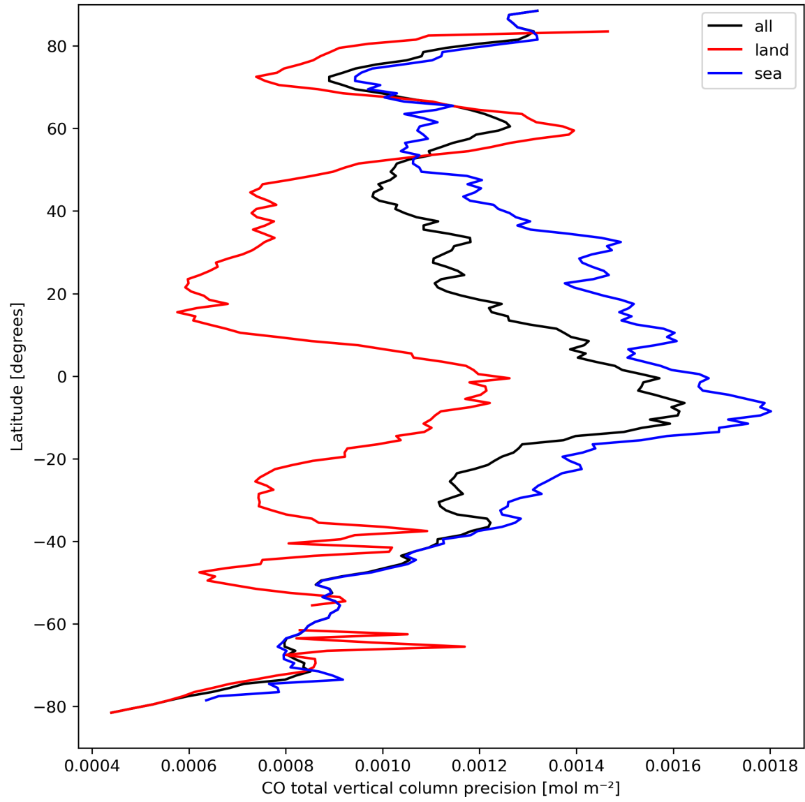
Figure 12: Zonal average of “CO total vertical column precision” for 2024-03-28 to 2024-03-30.
