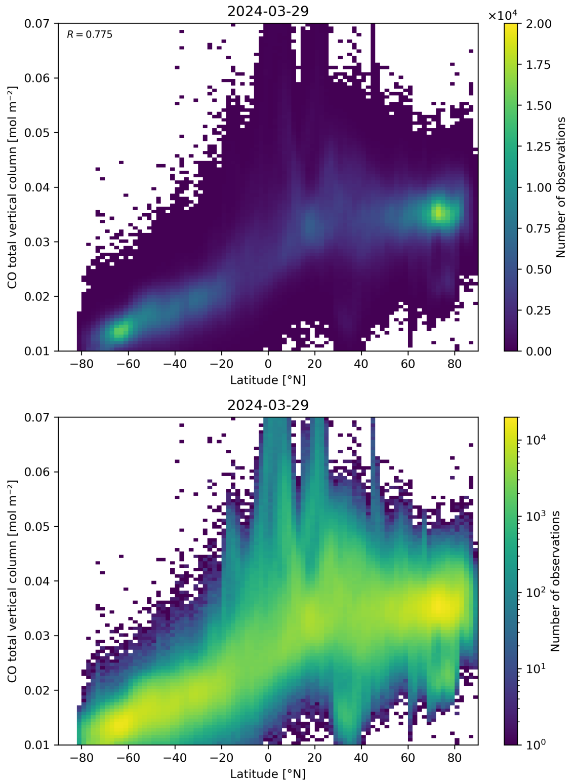
Figure 51: Scatter density plot of “Latitude” against “CO total vertical column” for 2024-03-28 to 2024-03-30.
