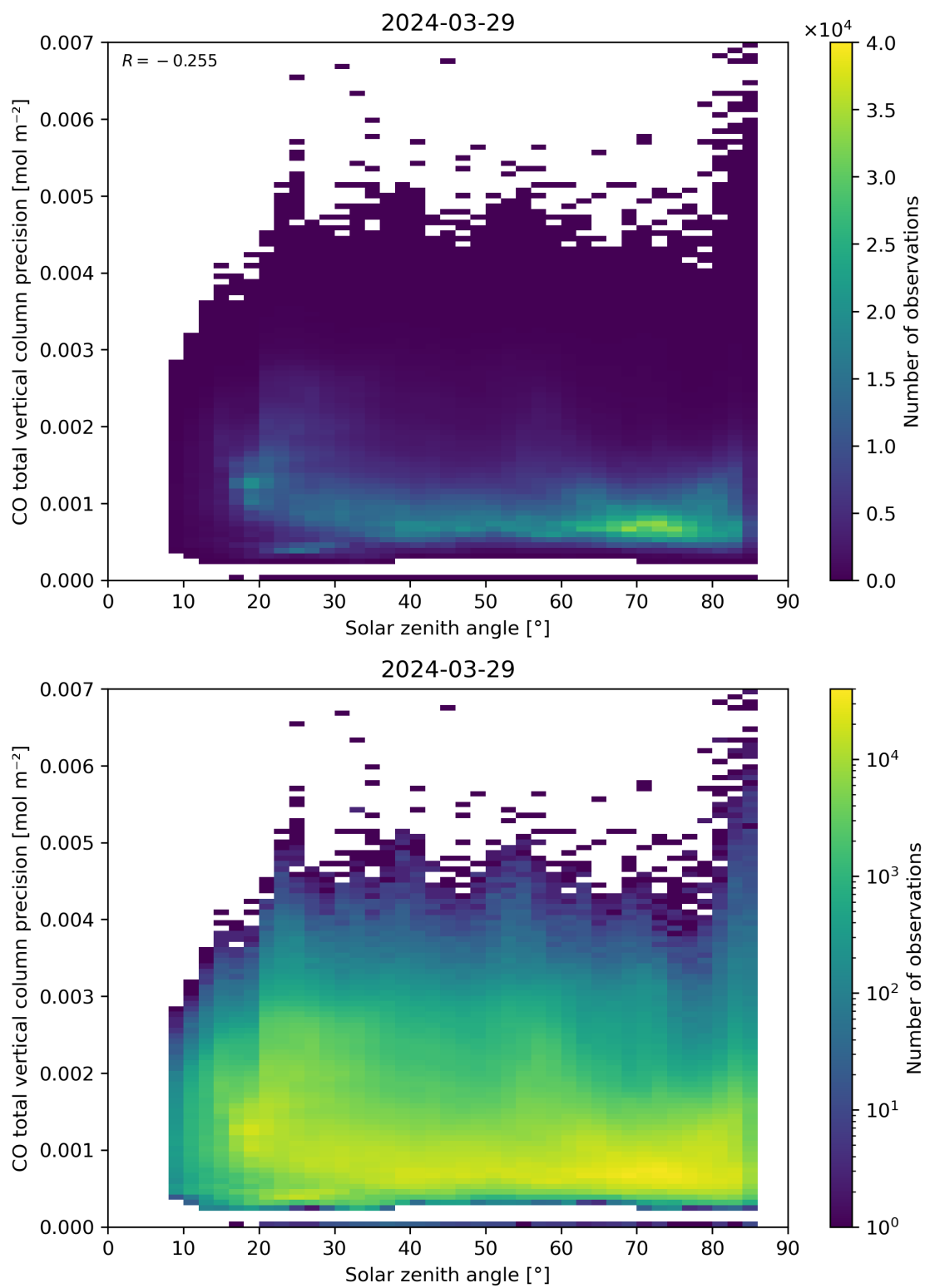
Figure 63: Scatter density plot of “Solar zenith angle” against “CO total vertical column precision” for 2024-03-28 to 2024-03-30.
