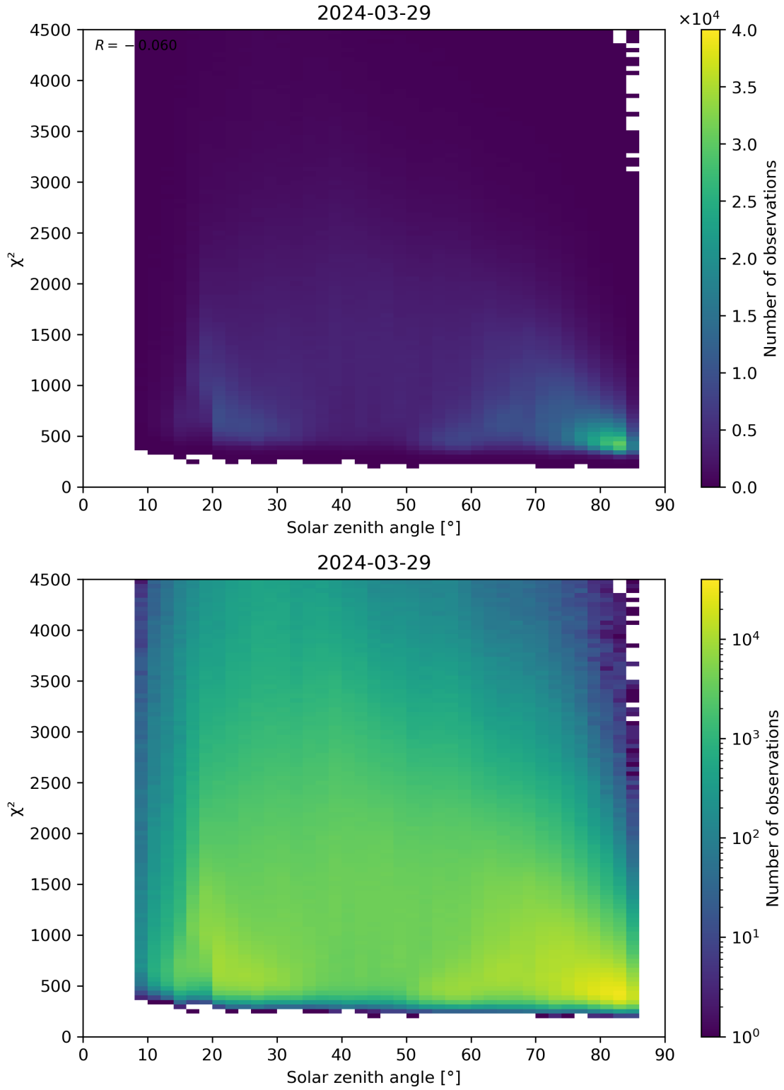
Figure 64: Scatter density plot of “Solar zenith angle” against “ \chi^2 ” for 2024-03-28 to 2024-03-30.
