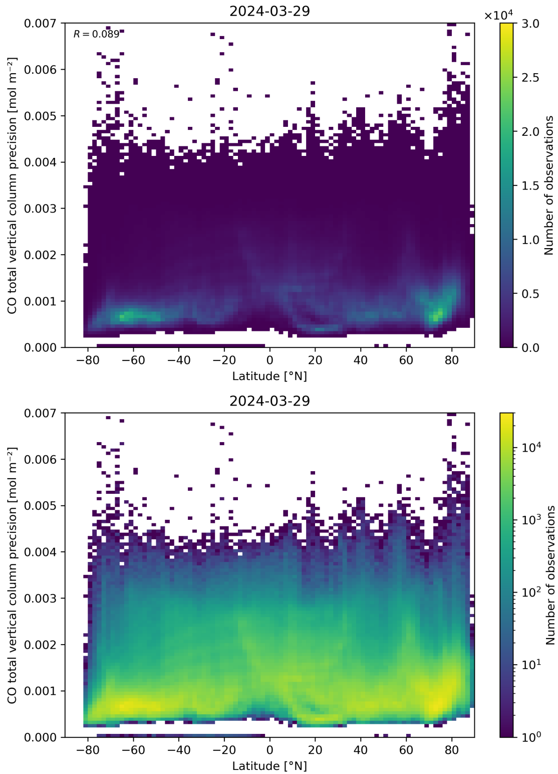
Figure 53: Scatter density plot of “Latitude” against “CO total vertical column precision” for 2024-03-28 to 2024-03-30.
