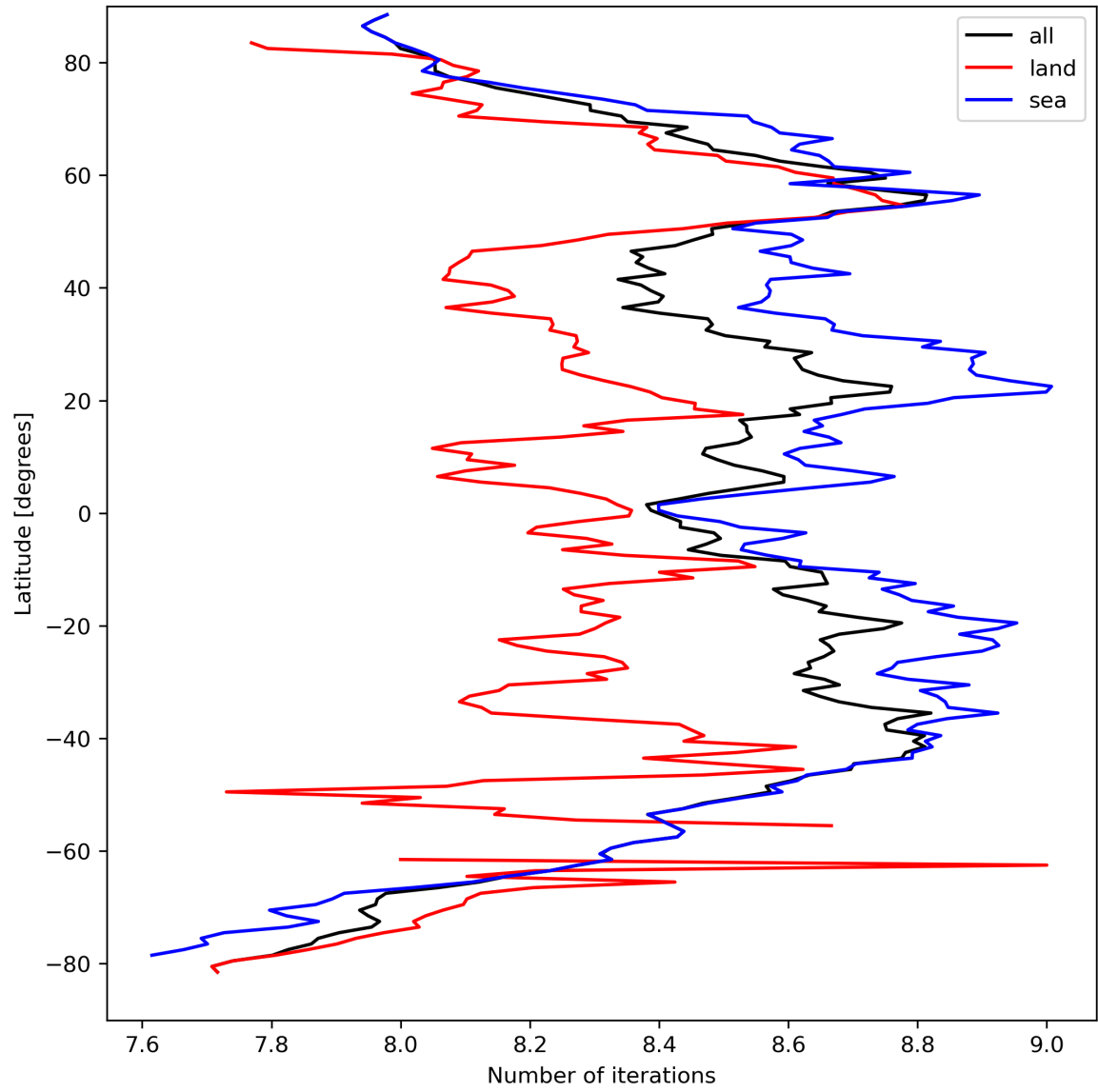
Figure 16: Zonal average of “Number of iterations” for 2024-03-28 to 2024-03-30.
