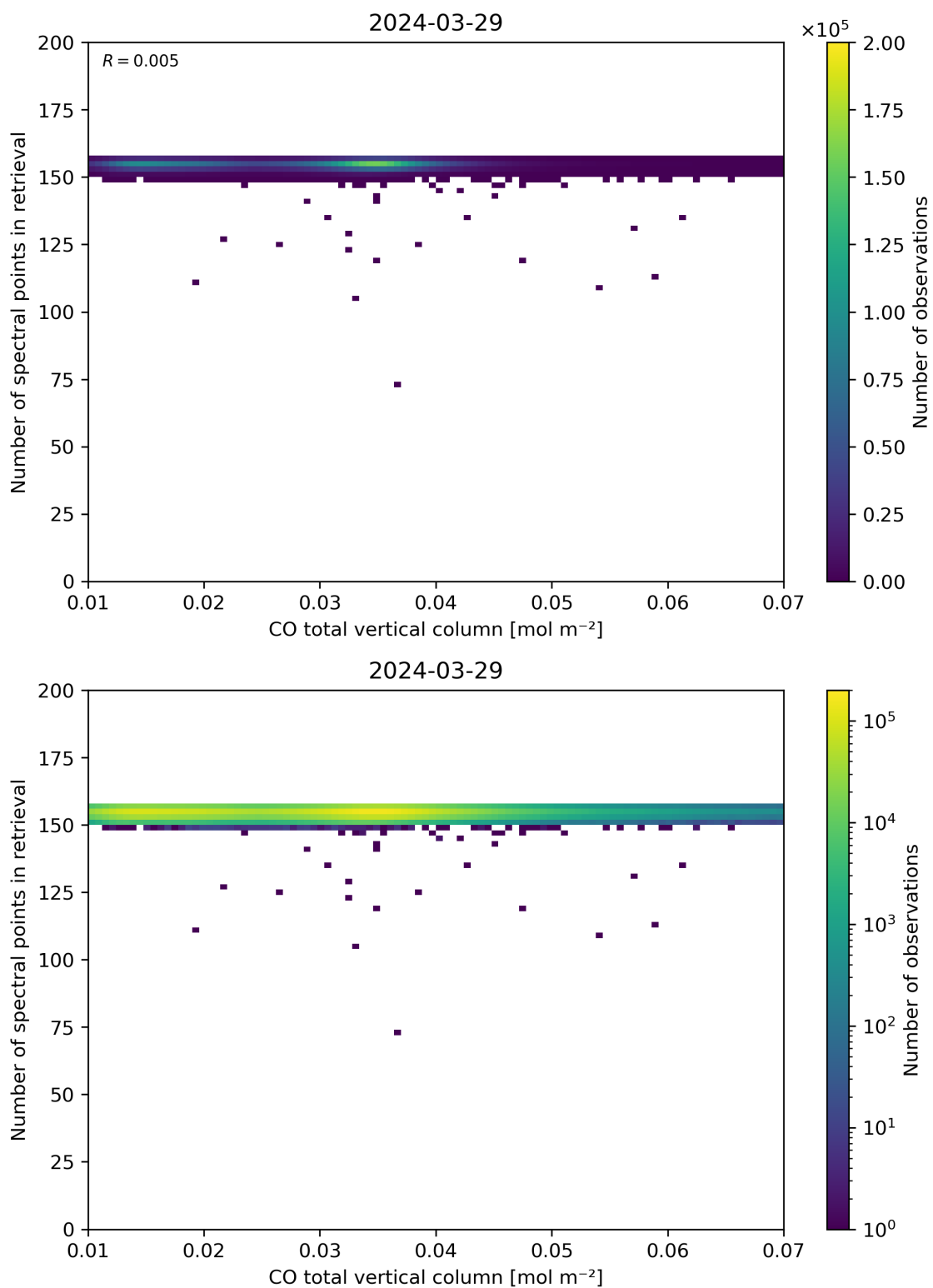
Figure 43: Scatter density plot of “CO total vertical column” against “Number of spectral points in retrieval” for 2024-03-28 to 2024-03-30.
