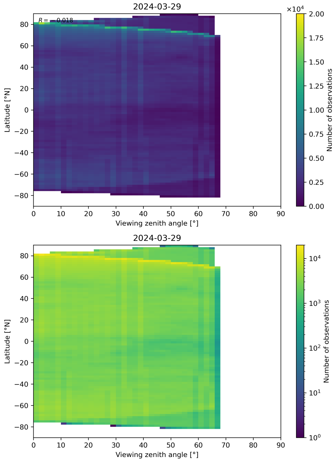
Figure 74: Scatter density plot of “Viewing zenith angle” against “Latitude” for 2024-03-28 to 2024-03-30.
