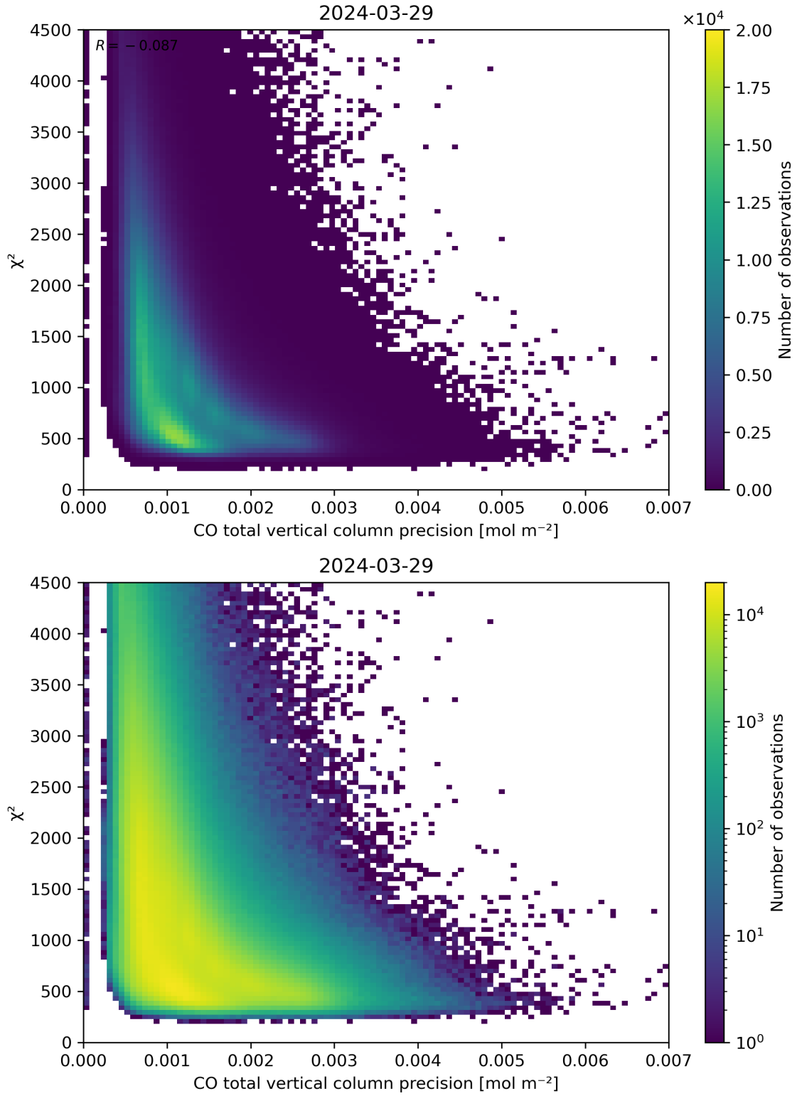
Figure 44: Scatter density plot of “CO total vertical column precision” against “ \chi^2 ” for 2024-03-28 to 2024-03-30.
