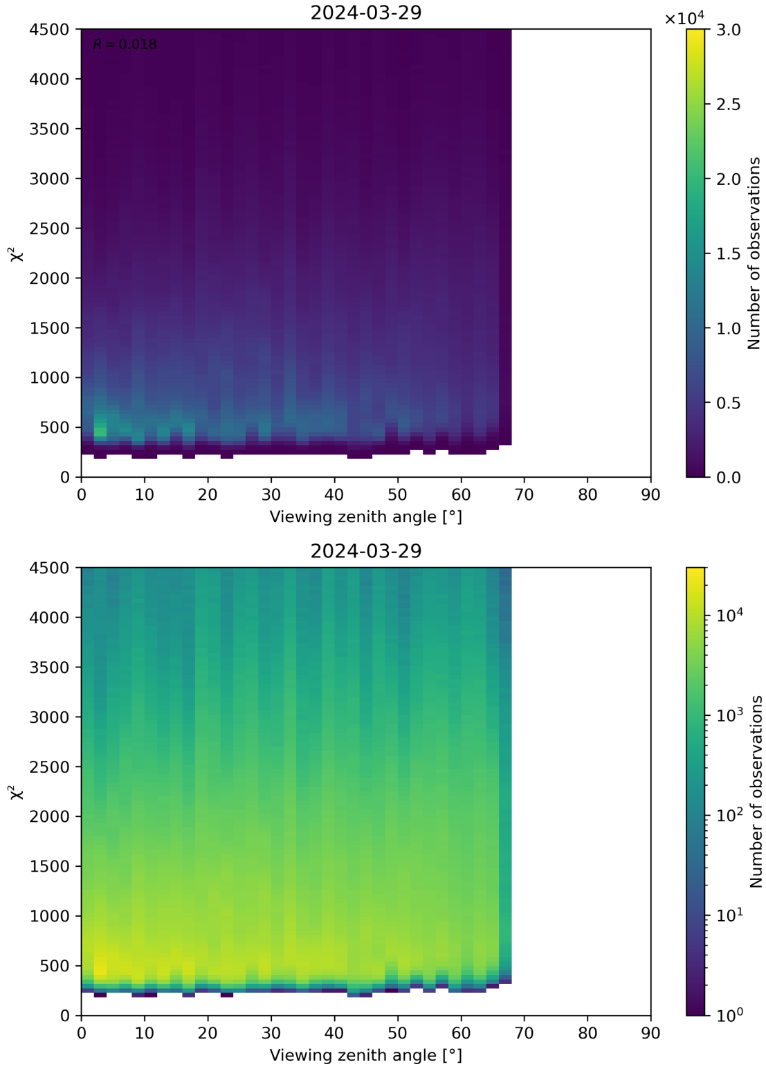
Figure 72: Scatter density plot of “Viewing zenith angle” against “ \chi^2 ” for 2024-03-28 to 2024-03-30.
