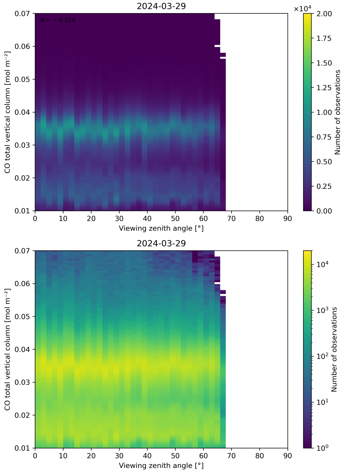
Figure 69: Scatter density plot of “Viewing zenith angle” against “CO total vertical column” for 2024-03-28 to 2024-03-30.
