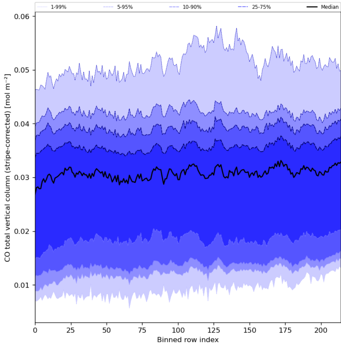
Figure 27: Along track statistics of “CO total vertical column (stripe-corrected)” for 2024-03-28 to 2024-03-30
