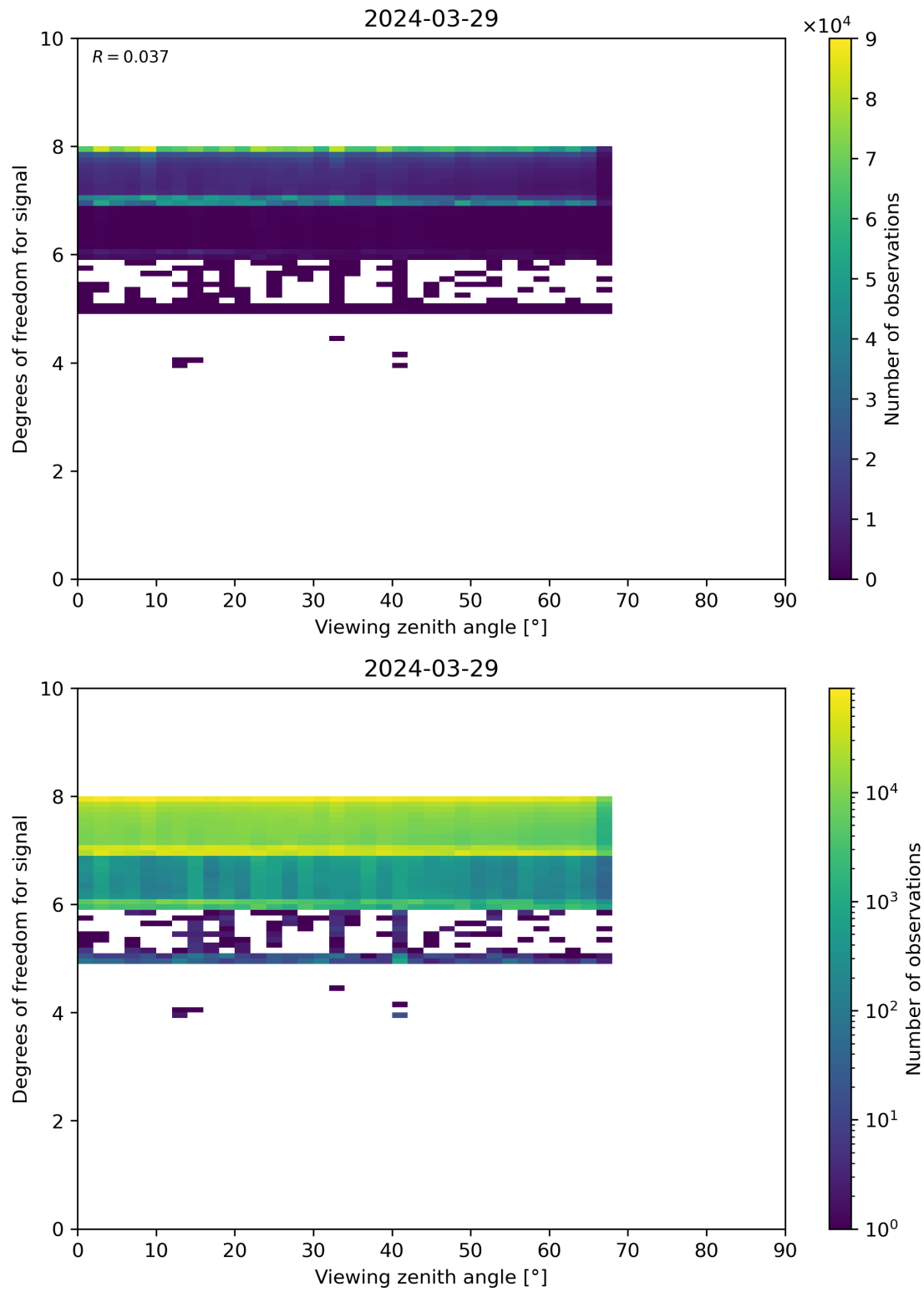
Figure 73: Scatter density plot of “Viewing zenith angle” against “Degrees of freedom for signal” for 2024-03-28 to 2024-03-30.
