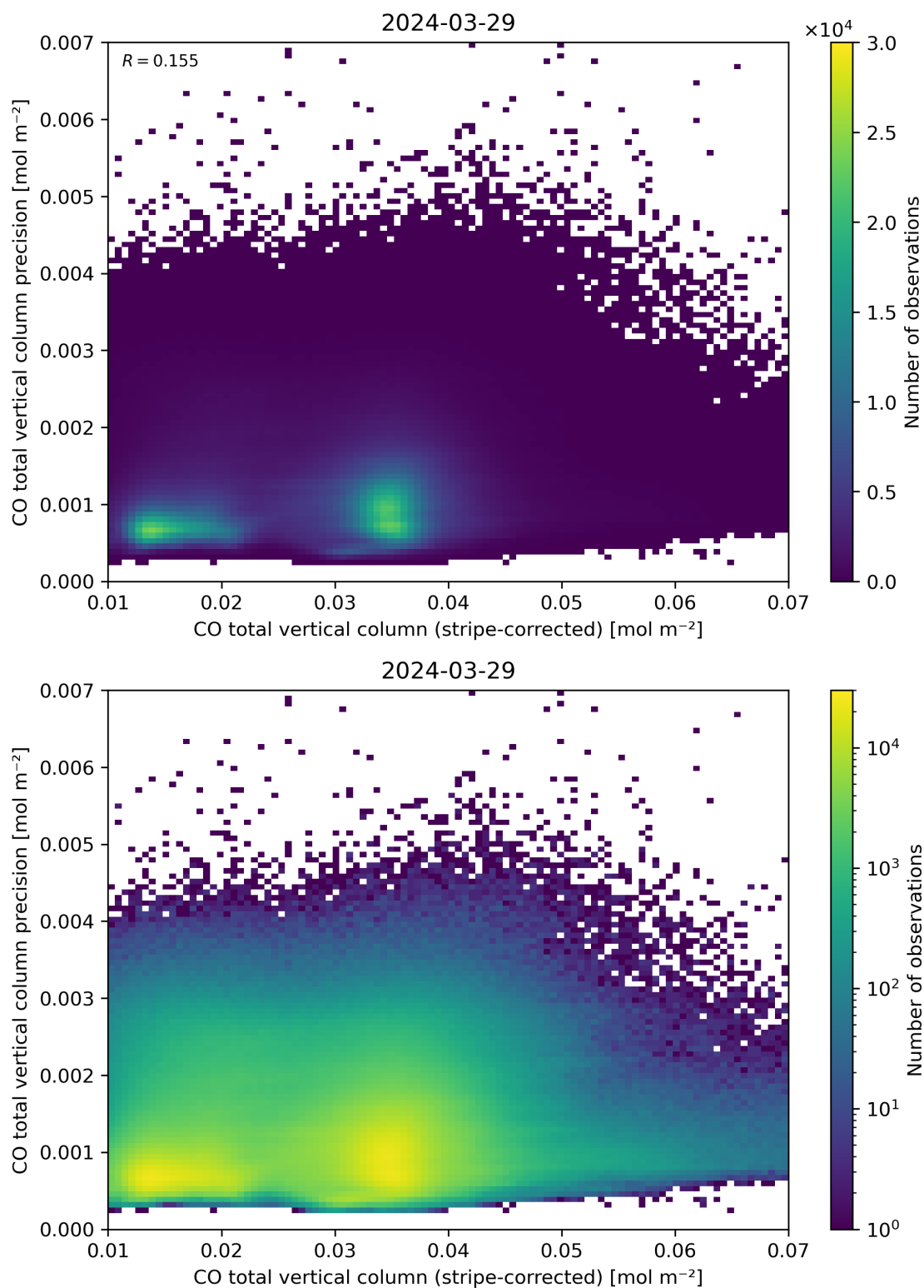
Figure 36: Scatter density plot of “CO total vertical column (stripe-corrected)” against “CO total vertical column precision” for 2024-03-28 to 2024-03-30.
