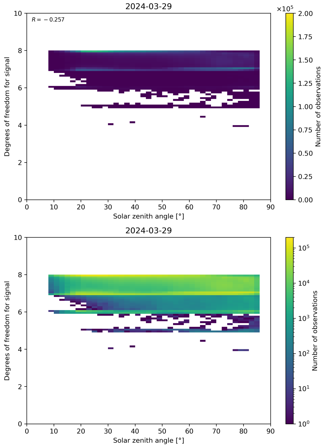
Figure 65: Scatter density plot of “Solar zenith angle” against “Degrees of freedom for signal” for 2024-03-28 to 2024-03-30.
