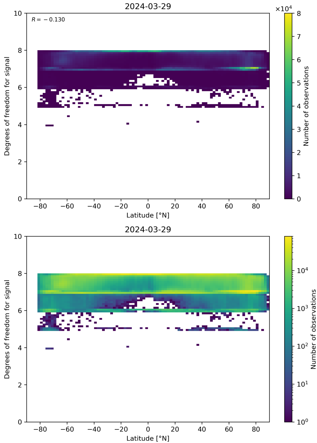
Figure 55: Scatter density plot of “Latitude” against “Degrees of freedom for signal” for 2024-03-28 to 2024-03-30.
