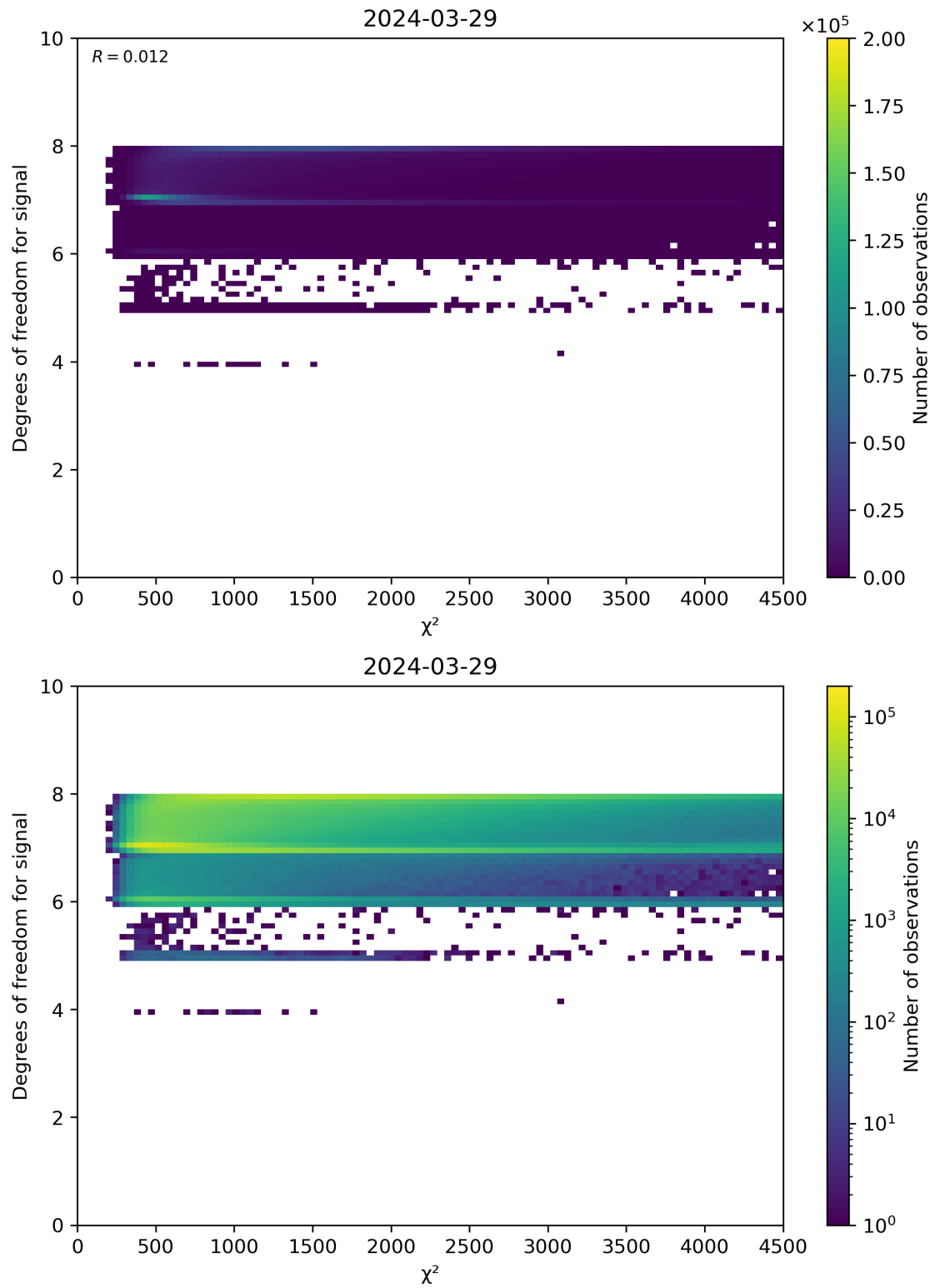
Figure 48: Scatter density plot of “ \chi^2 ” against “Degrees of freedom for signal” for 2024-03-28 to 2024-03-30.
