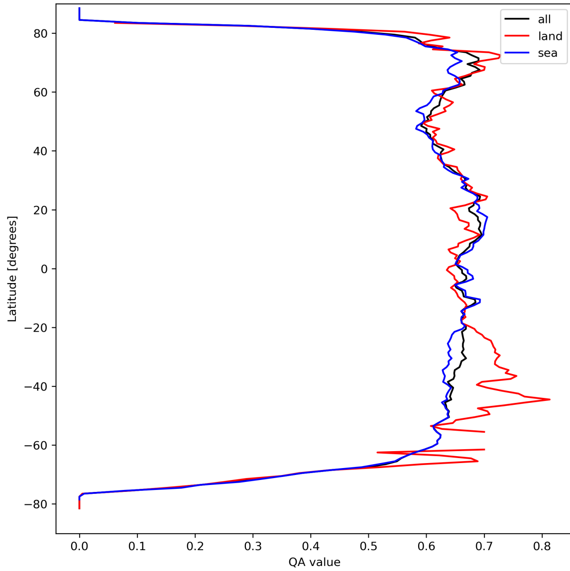
Figure 9: Zonal average of “QA value” for 2024-03-28 to 2024-03-30.
