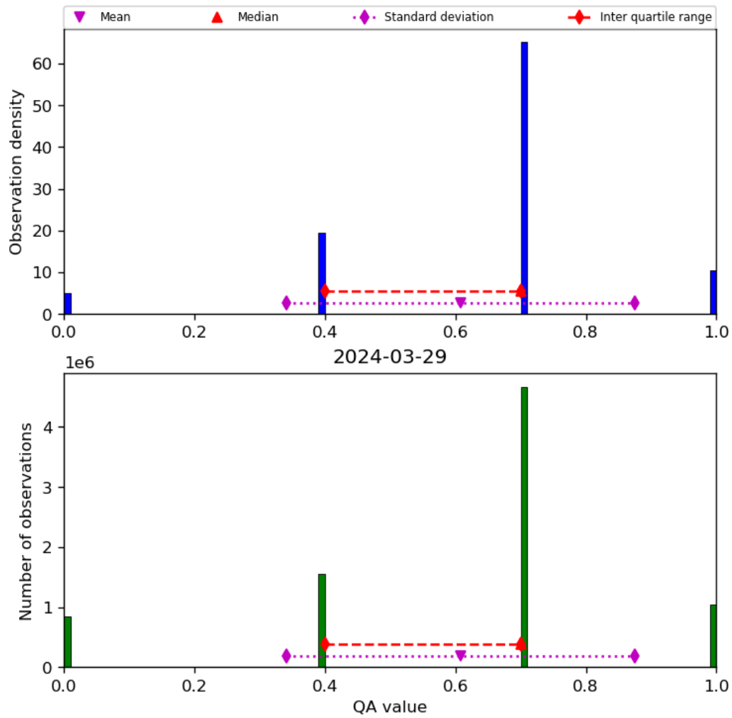
Figure 17: Histogram of “QA value” for 2024-03-28 to 2024-03-30
