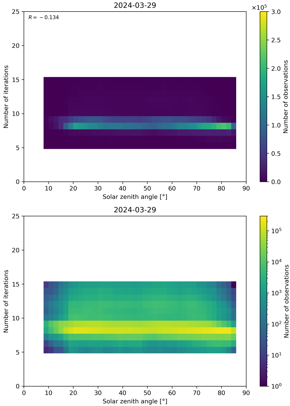
Figure 67: Scatter density plot of “Solar zenith angle” against “Number of iterations” for 2024-03-28 to 2024-03-30.
