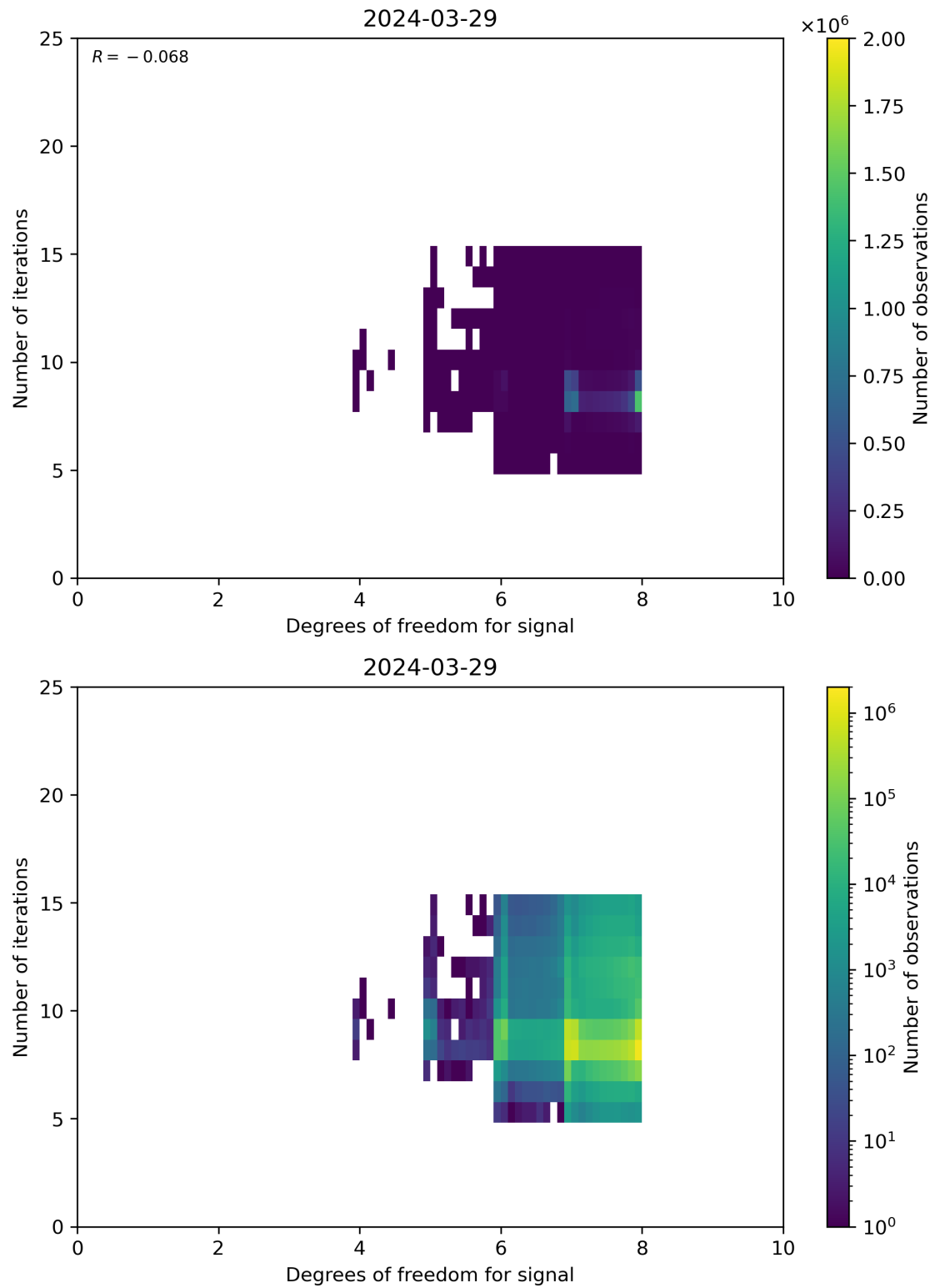
Figure 50: Scatter density plot of “Degrees of freedom for signal” against “Number of iterations” for 2024-03-28 to 2024-03-30.
