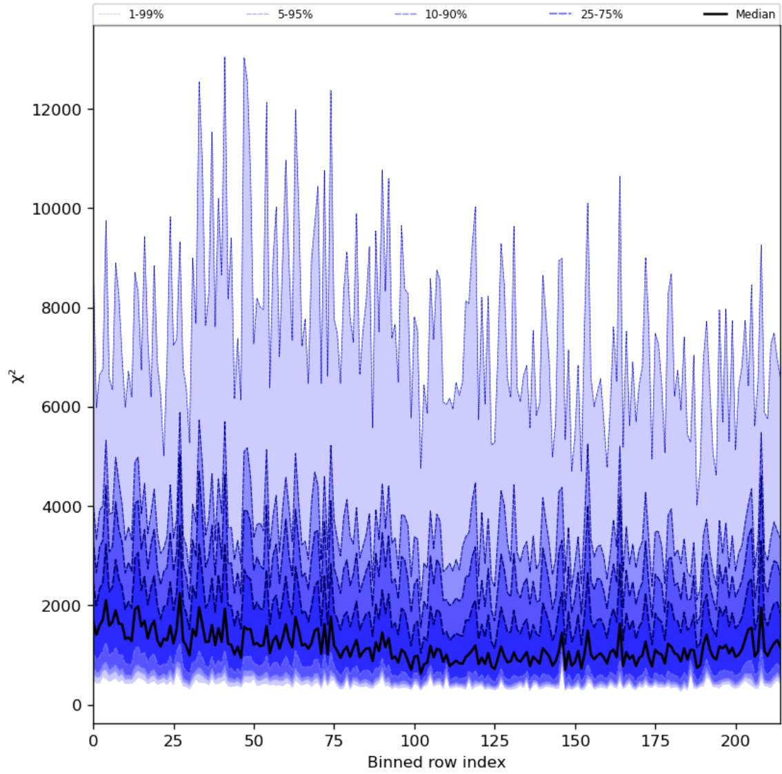
Figure 30: Along track statistics of “ \chi^2 ” for 2024-03-28 to 2024-03-30
