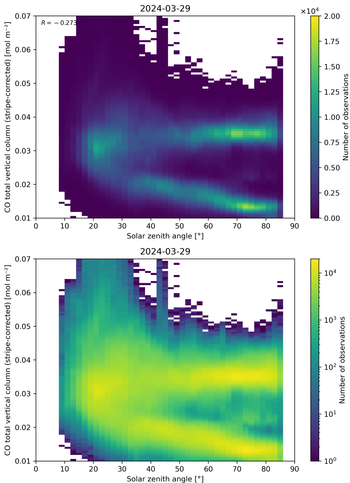
Figure 62: Scatter density plot of “Solar zenith angle” against “CO total vertical column (stripe-corrected)” for 2024-03-28 to 2024-03-30.
