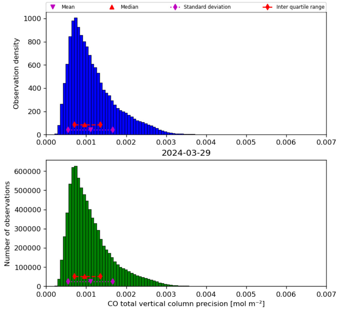
Figure 20: Histogram of “CO total vertical column precision” for 2024-03-28 to 2024-03-30
