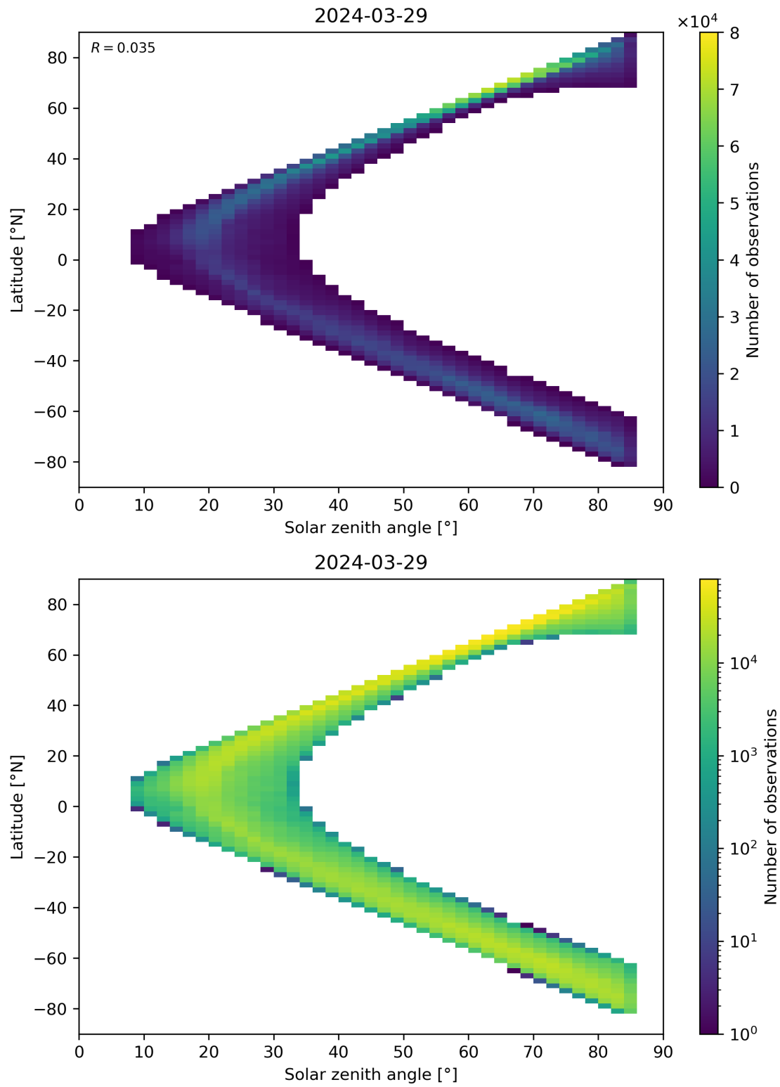
Figure 66: Scatter density plot of “Solar zenith angle” against “Latitude” for 2024-03-28 to 2024-03-30.
