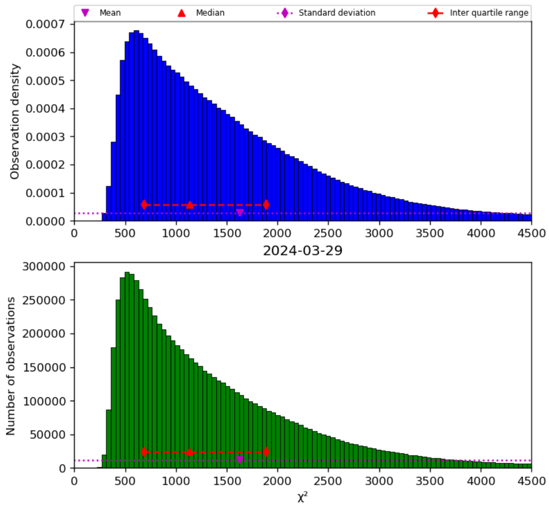
Figure 22: Histogram of “ \chi^2 ” for 2024-03-28 to 2024-03-30
