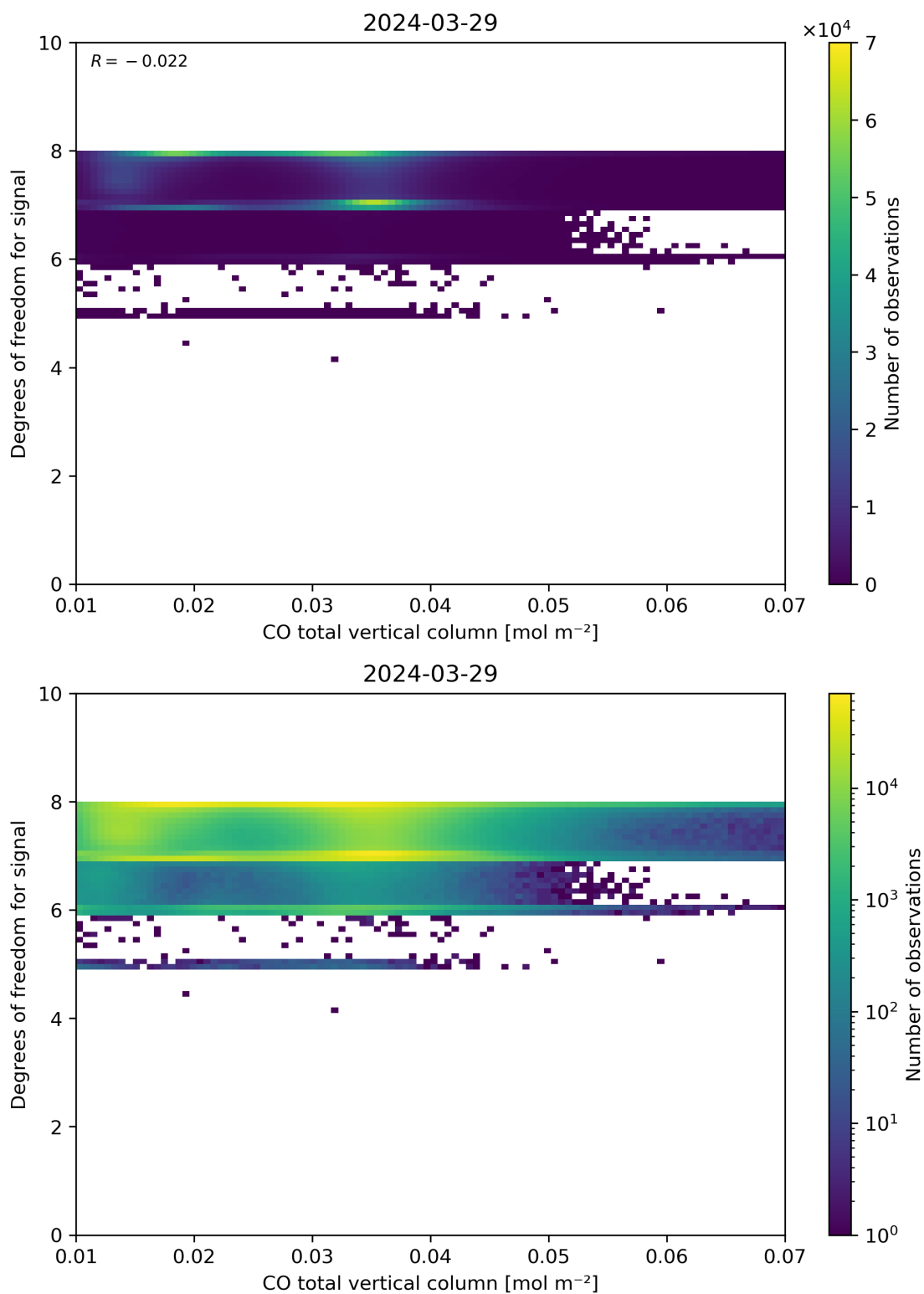
Figure 41: Scatter density plot of “CO total vertical column” against “Degrees of freedom for signal” for 2024-03-28 to 2024-03-30.
