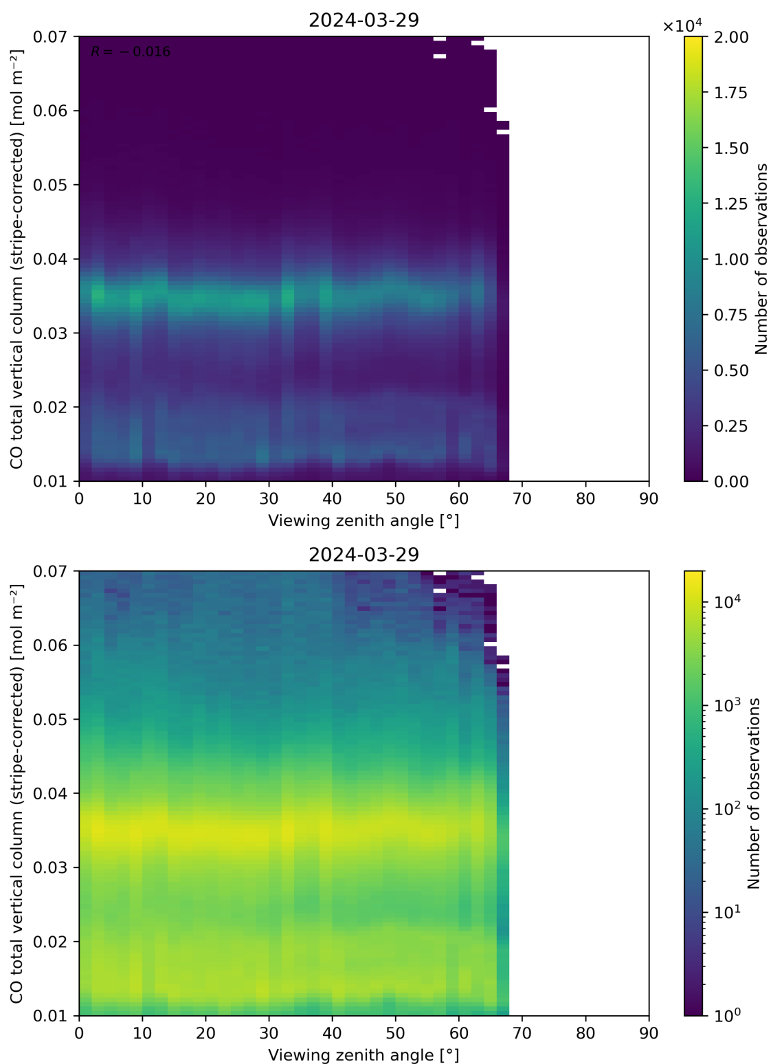
Figure 70: Scatter density plot of “Viewing zenith angle” against “CO total vertical column (stripe-corrected)” for 2024-03-28 to 2024-03-30.
