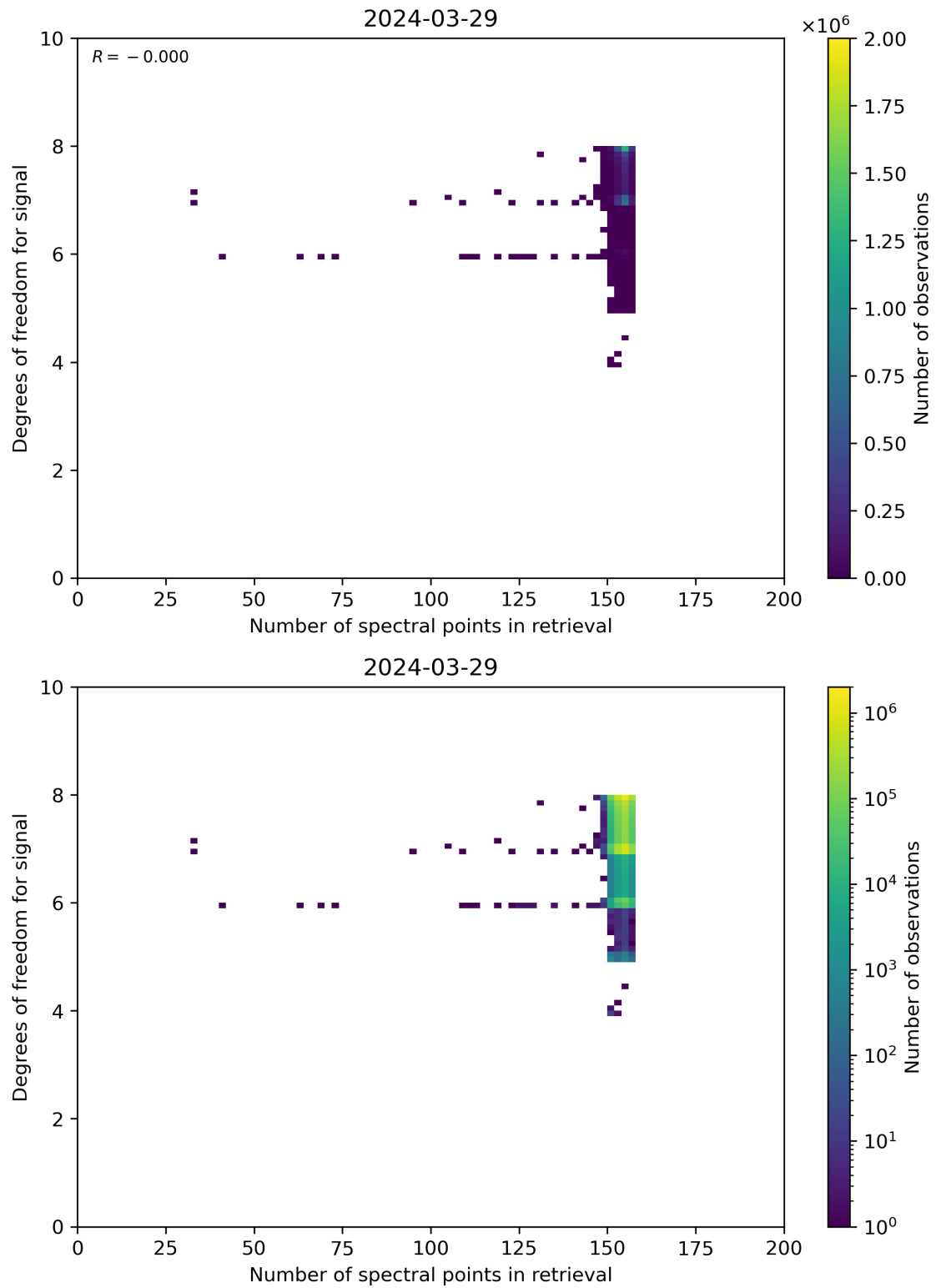
Figure 59: Scatter density plot of “Number of spectral points in retrieval” against “Degrees of freedom for signal” for 2024-03-28 to 2024-03-30.
