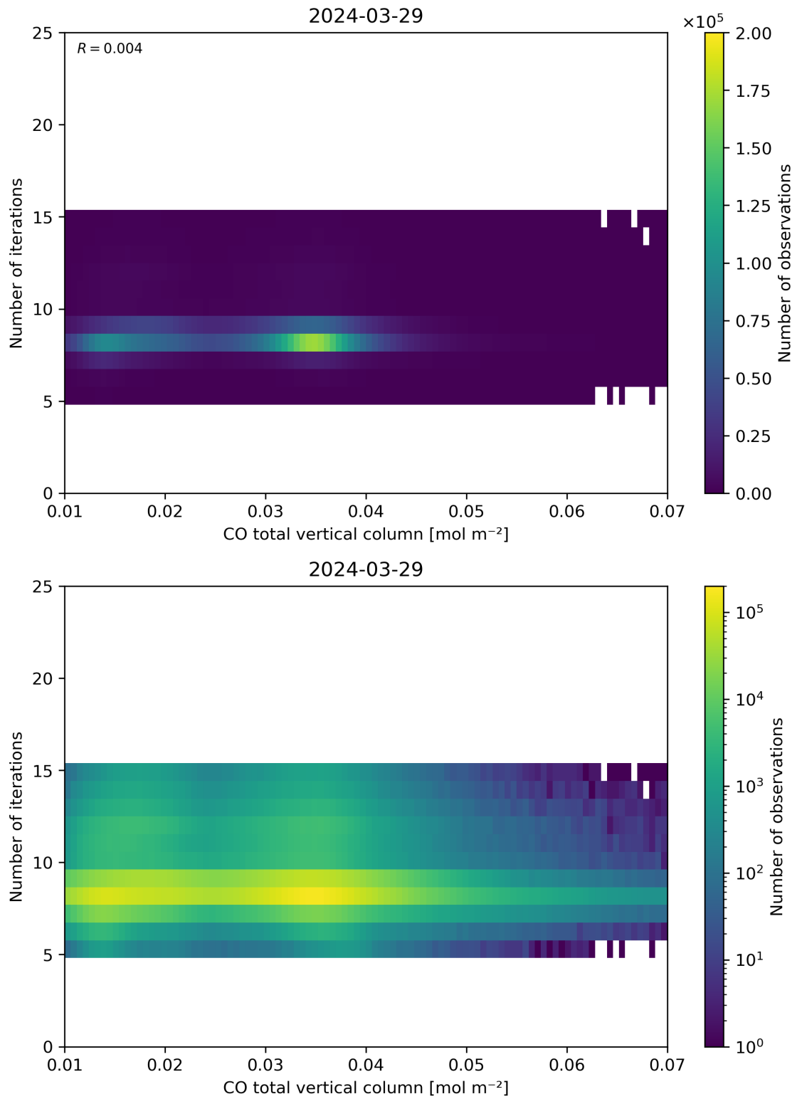
Figure 42: Scatter density plot of “CO total vertical column” against “Number of iterations” for 2024-03-28 to 2024-03-30.
