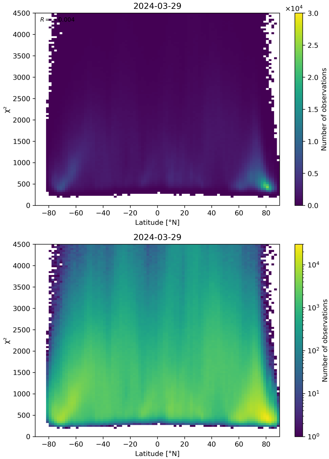
Figure 54: Scatter density plot of “Latitude” against “ \chi^2 ” for 2024-03-28 to 2024-03-30.
