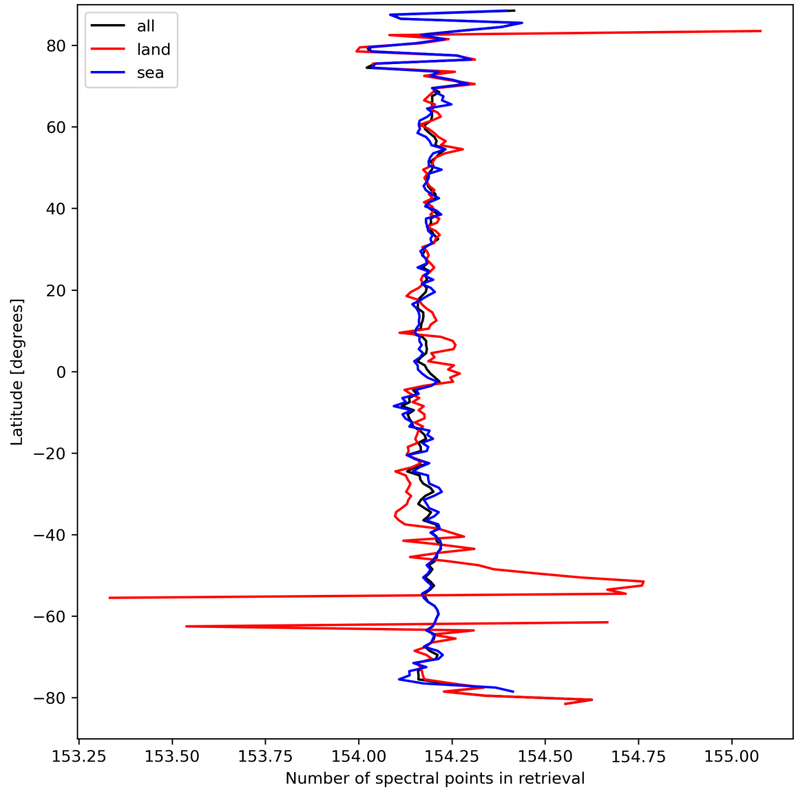
Figure 13: Zonal average of “Number of spectral points in retrieval” for 2024-03-28 to 2024-03-30.
