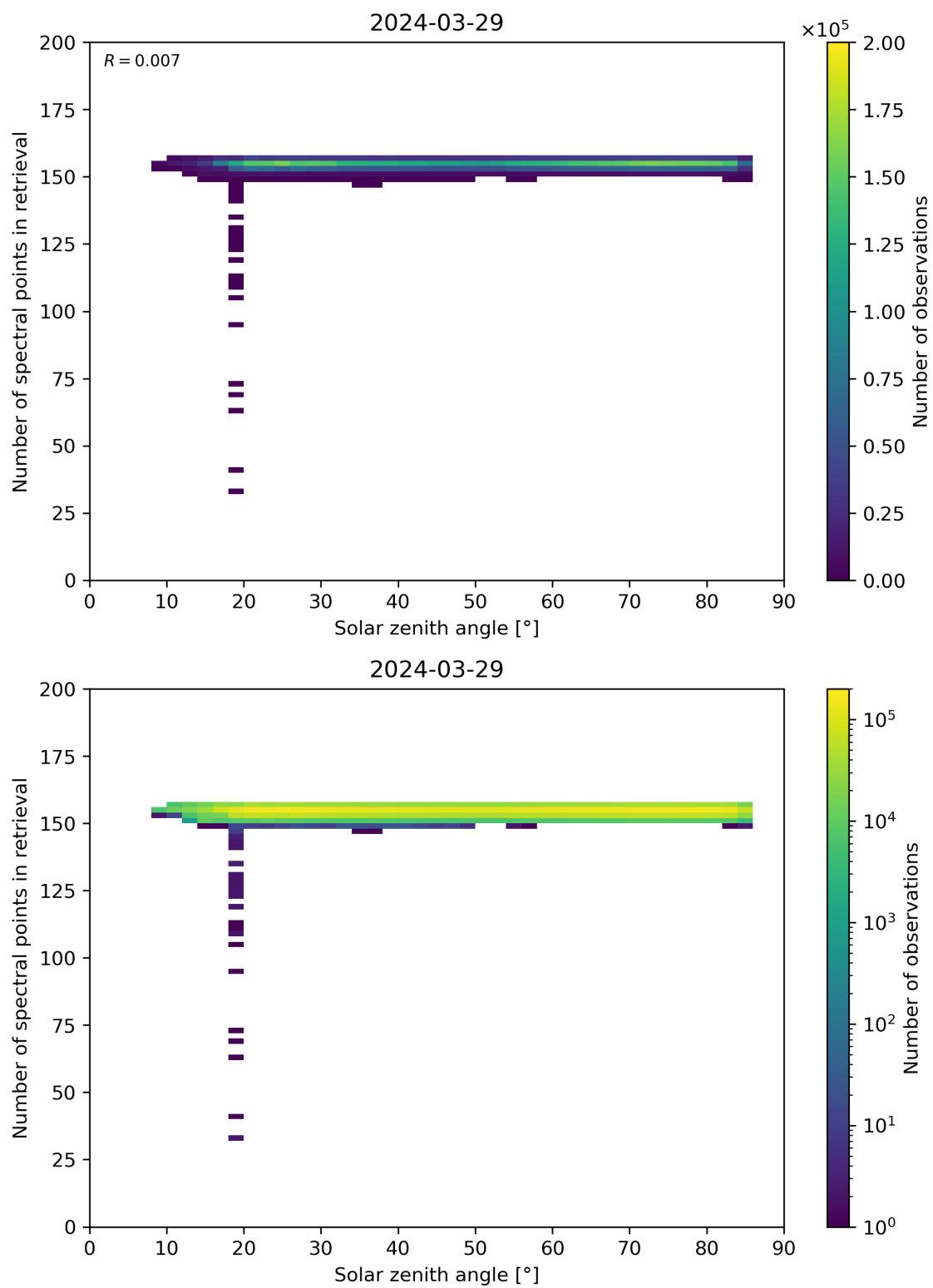
Figure 68: Scatter density plot of “Solar zenith angle” against “Number of spectral points in retrieval” for 2024-03-28 to 2024-03-30.
