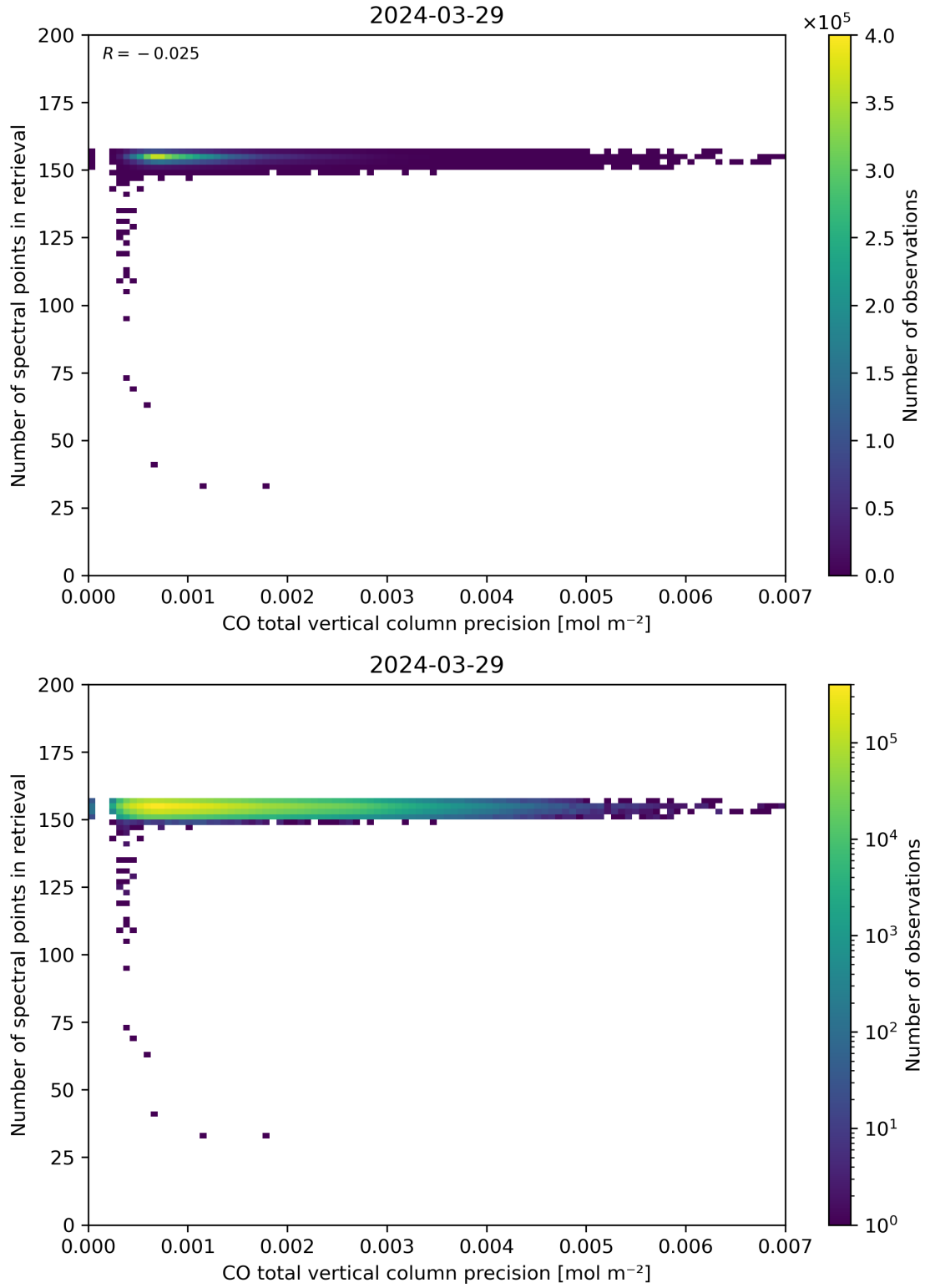
Figure 47: Scatter density plot of “CO total vertical column precision” against “Number of spectral points in retrieval” for 2024-03-28 to 2024-03-30.
