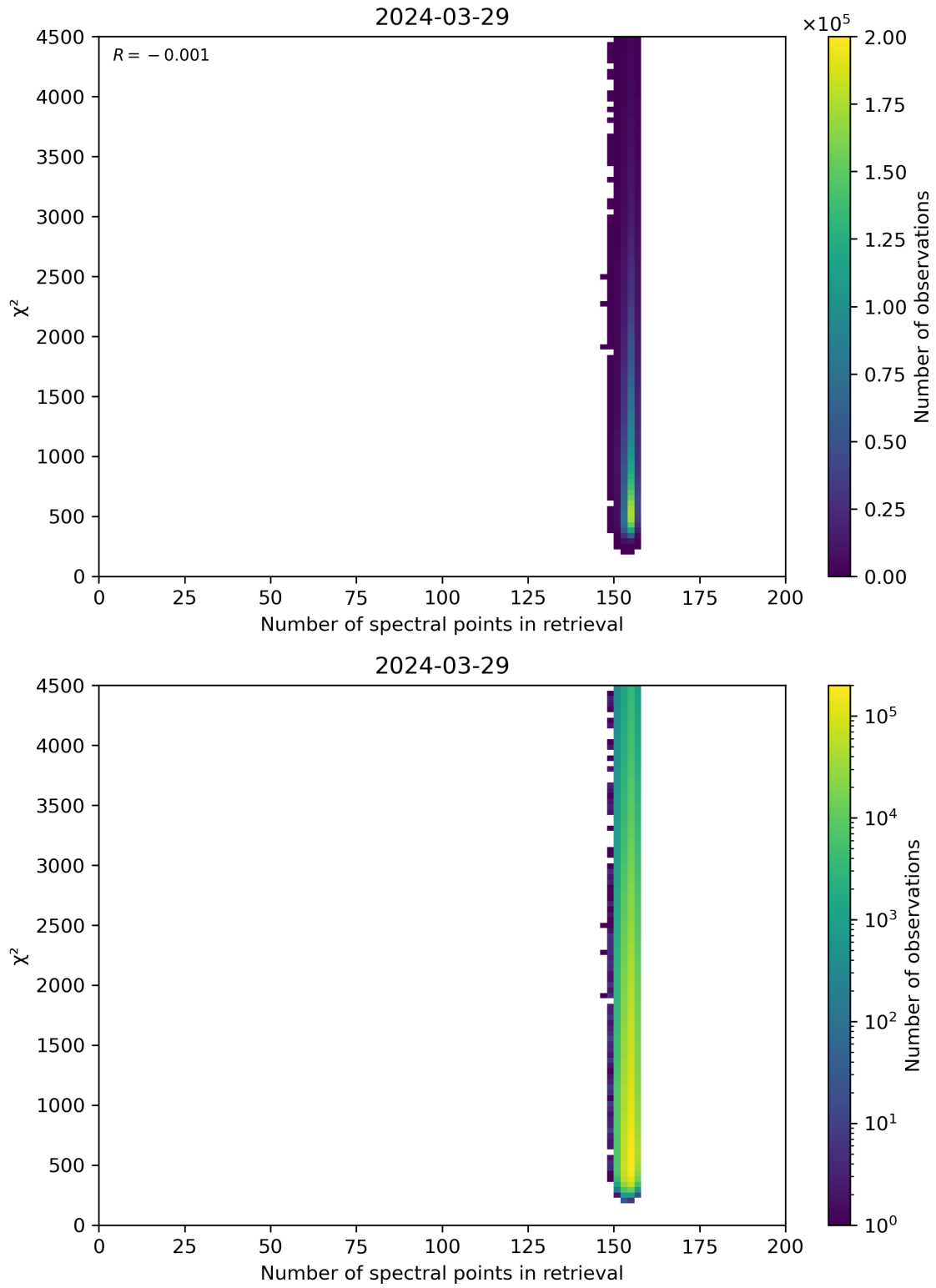
Figure 58: Scatter density plot of “Number of spectral points in retrieval” against “ \chi^2 ” for 2024-03-28 to 2024-03-30.
