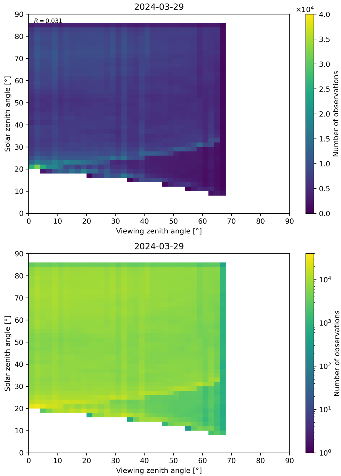
Figure 77: Scatter density plot of “Viewing zenith angle” against “Solar zenith angle” for 2024-03-28 to 2024-03-30.
