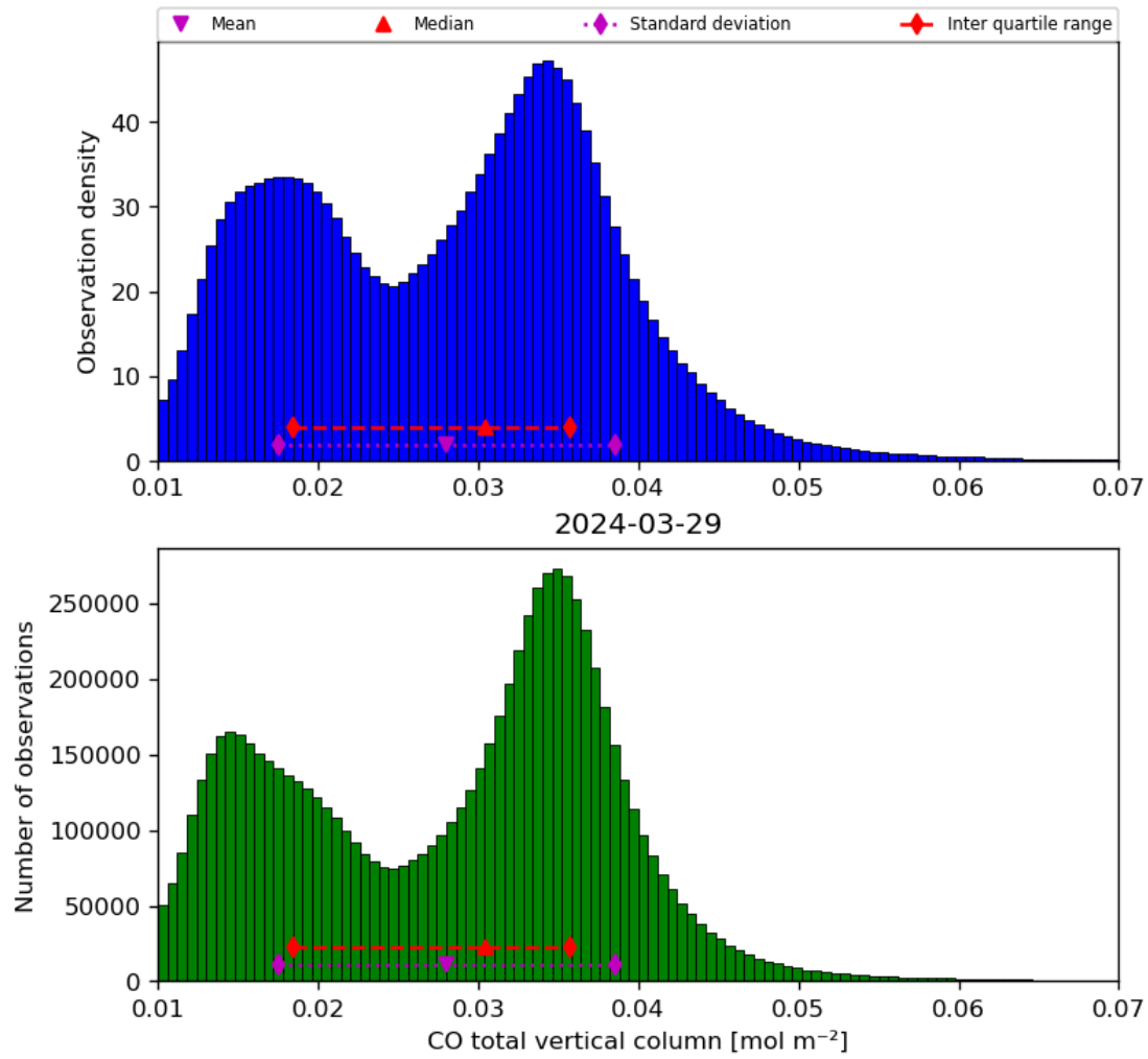
Figure 18: Histogram of “CO total vertical column” for 2024-03-28 to 2024-03-30
