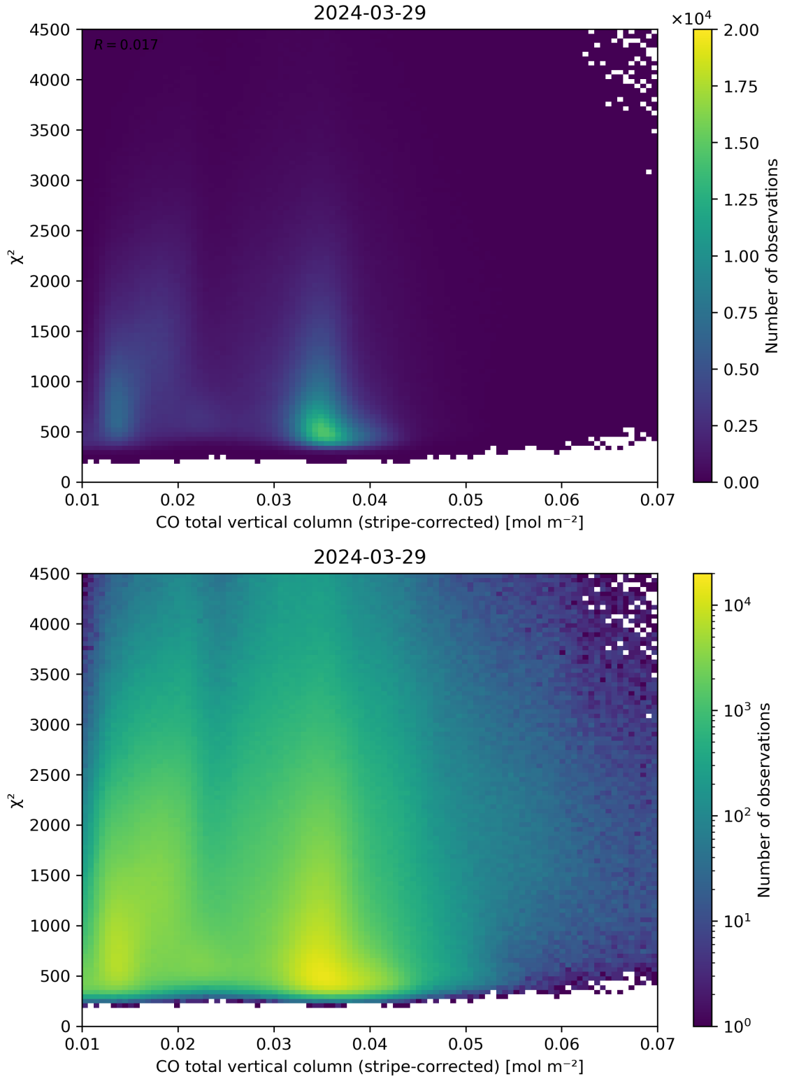
Figure 37: Scatter density plot of “CO total vertical column (stripe-corrected)” against “ \chi^2 ” for 2024-03-28 to 2024-03-30.
