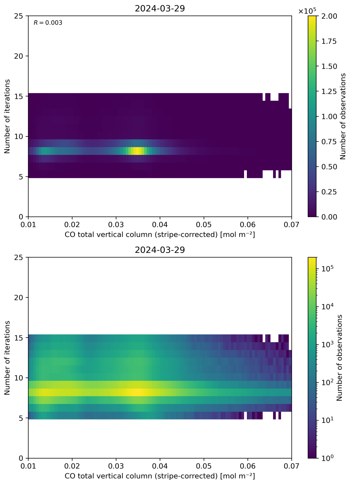
Figure 39: Scatter density plot of “CO total vertical column (stripe-corrected)” against “Number of iterations” for 2024-03-28 to 2024-03-30.
