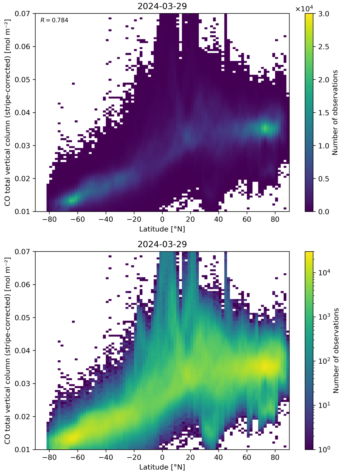
Figure 52: Scatter density plot of “Latitude” against “CO total vertical column (stripe-corrected)” for 2024-03-28 to 2024-03-30.
