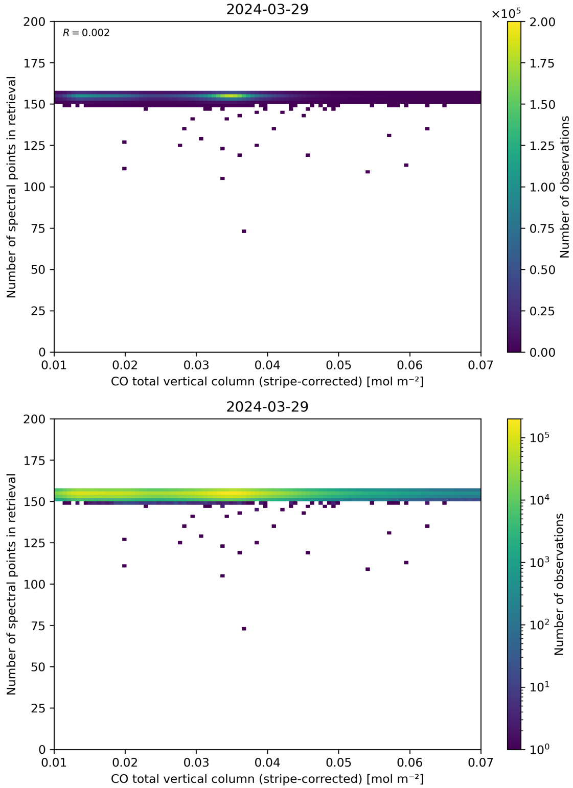
Figure 40: Scatter density plot of “CO total vertical column (stripe-corrected)” against “Number of spectral points in retrieval” for 2024-03-28 to 2024-03-30.
