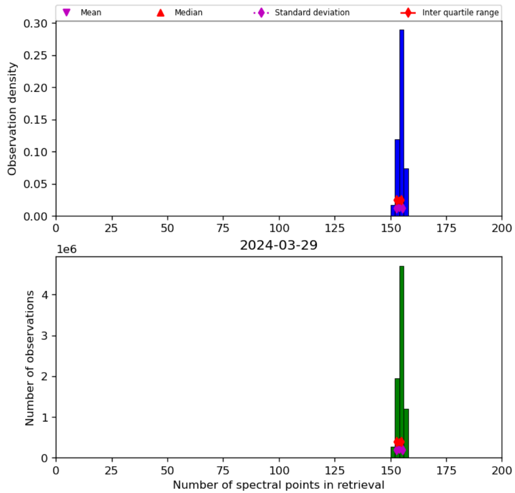
Figure 21: Histogram of “Number of spectral points in retrieval” for 2024-03-28 to 2024-03-30
