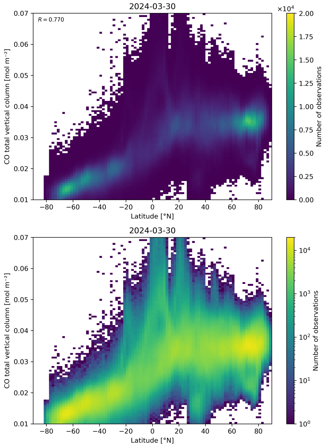
Figure 51: Scatter density plot of “Latitude” against “CO total vertical column” for 2024-03-30 to 2024-03-31.
