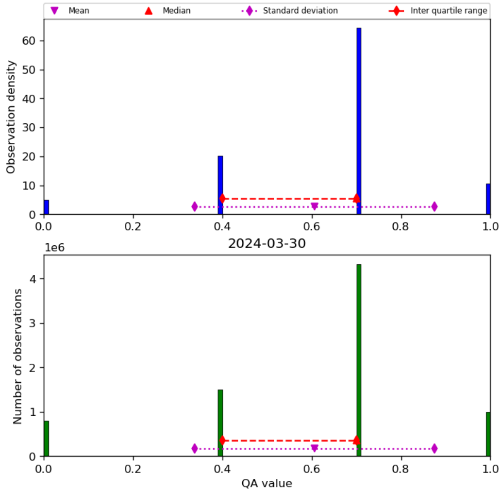
Figure 17: Histogram of “QA value” for 2024-03-30 to 2024-03-31
