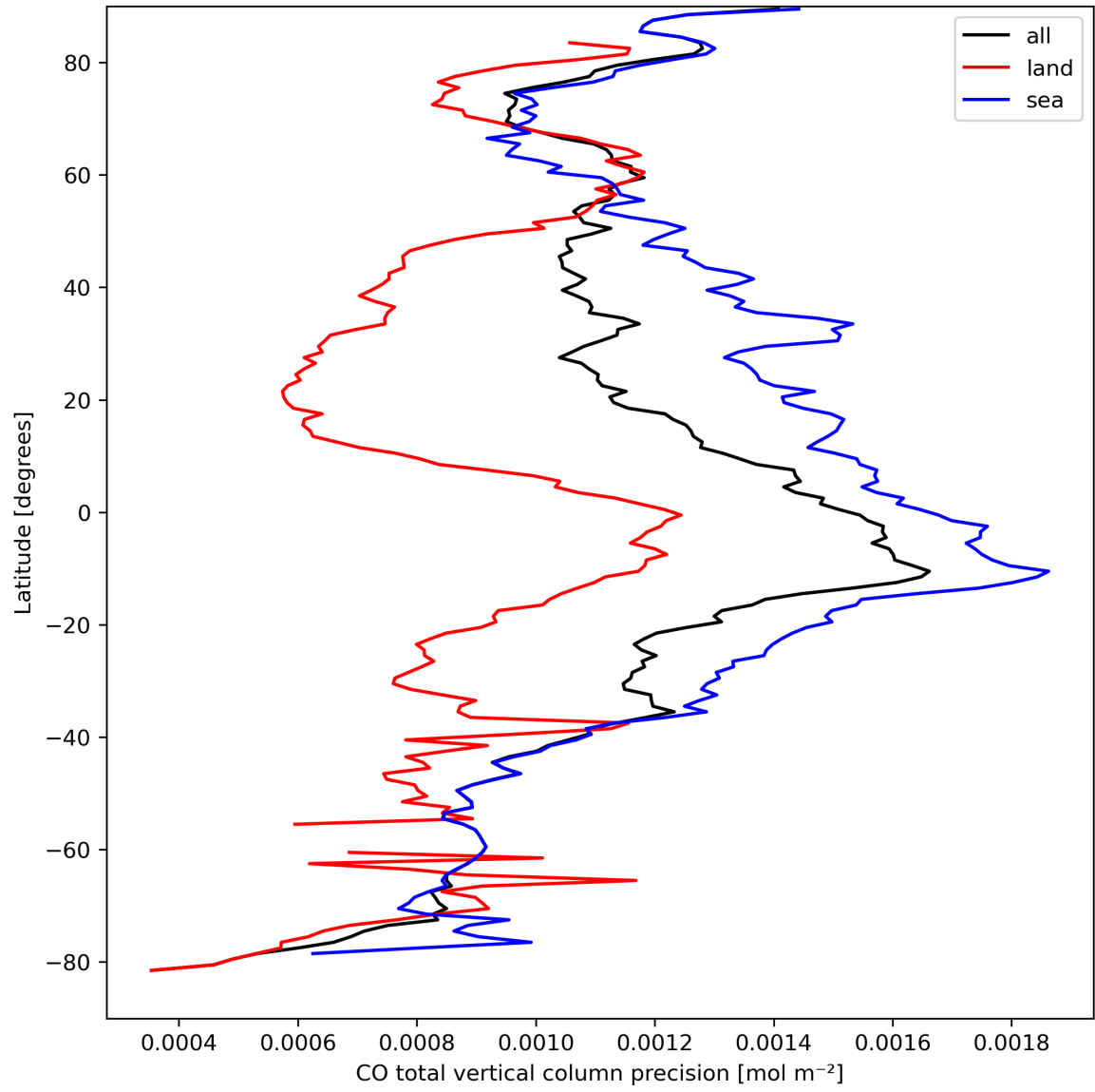
Figure 12: Zonal average of “CO total vertical column precision” for 2024-03-30 to 2024-03-31.
