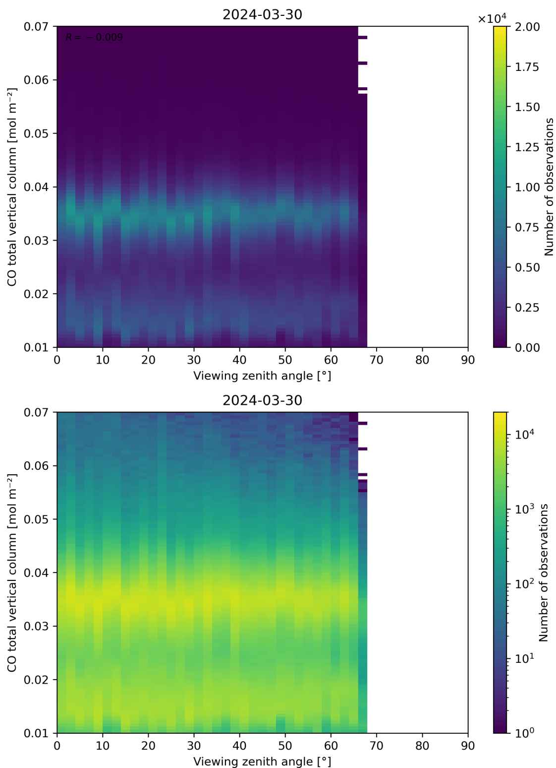
Figure 69: Scatter density plot of “Viewing zenith angle” against “CO total vertical column” for 2024-03-30 to 2024-03-31.
