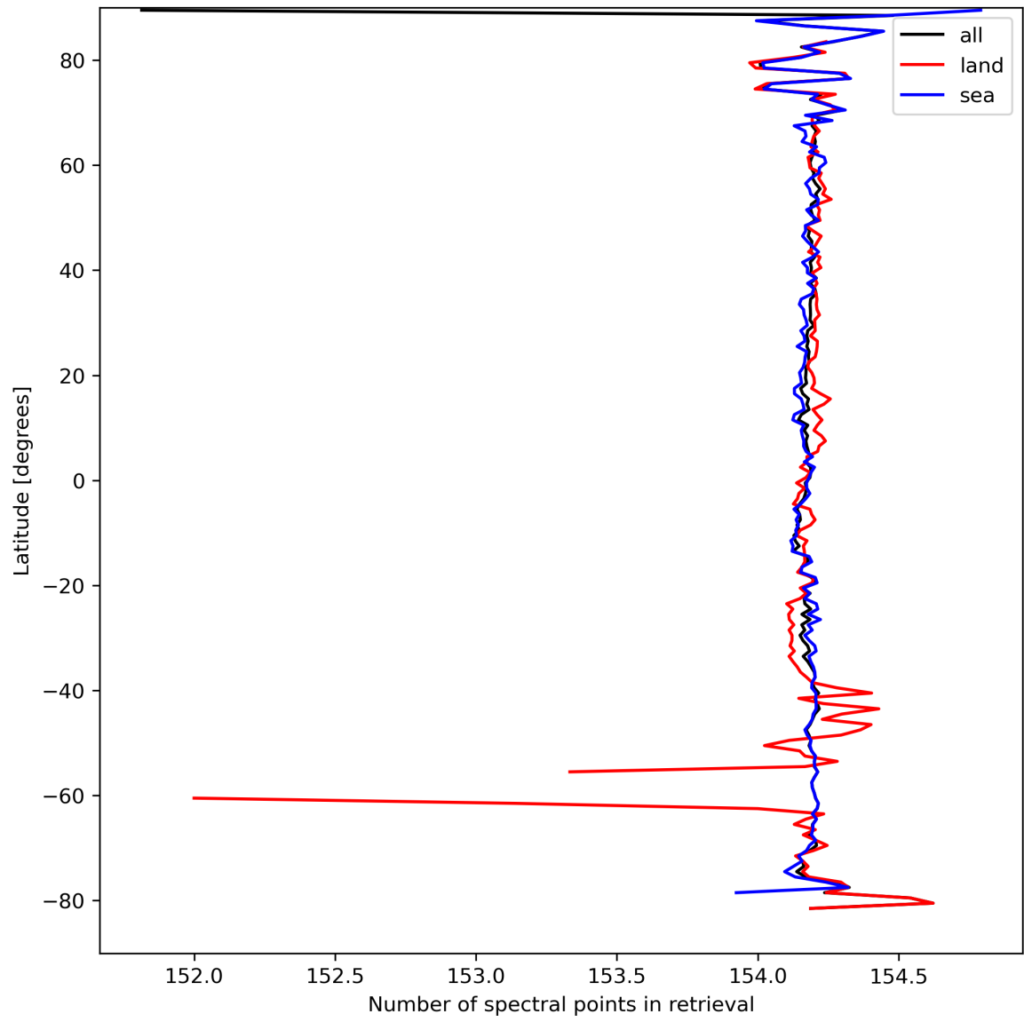
Figure 13: Zonal average of “Number of spectral points in retrieval” for 2024-03-30 to 2024-03-31.
