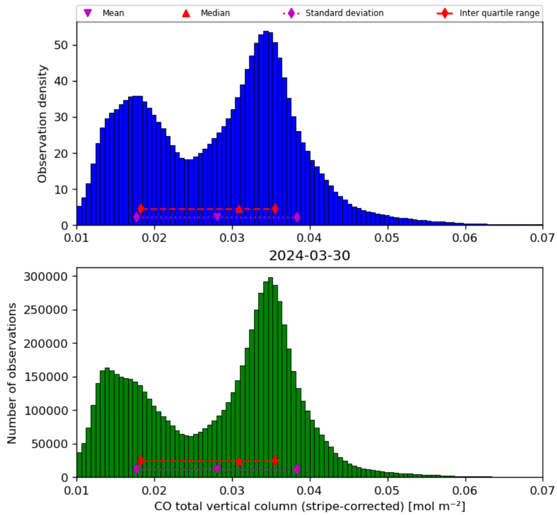
Figure 19: Histogram of “CO total vertical column (stripe-corrected)” for 2024-03-30 to 2024-03-31
