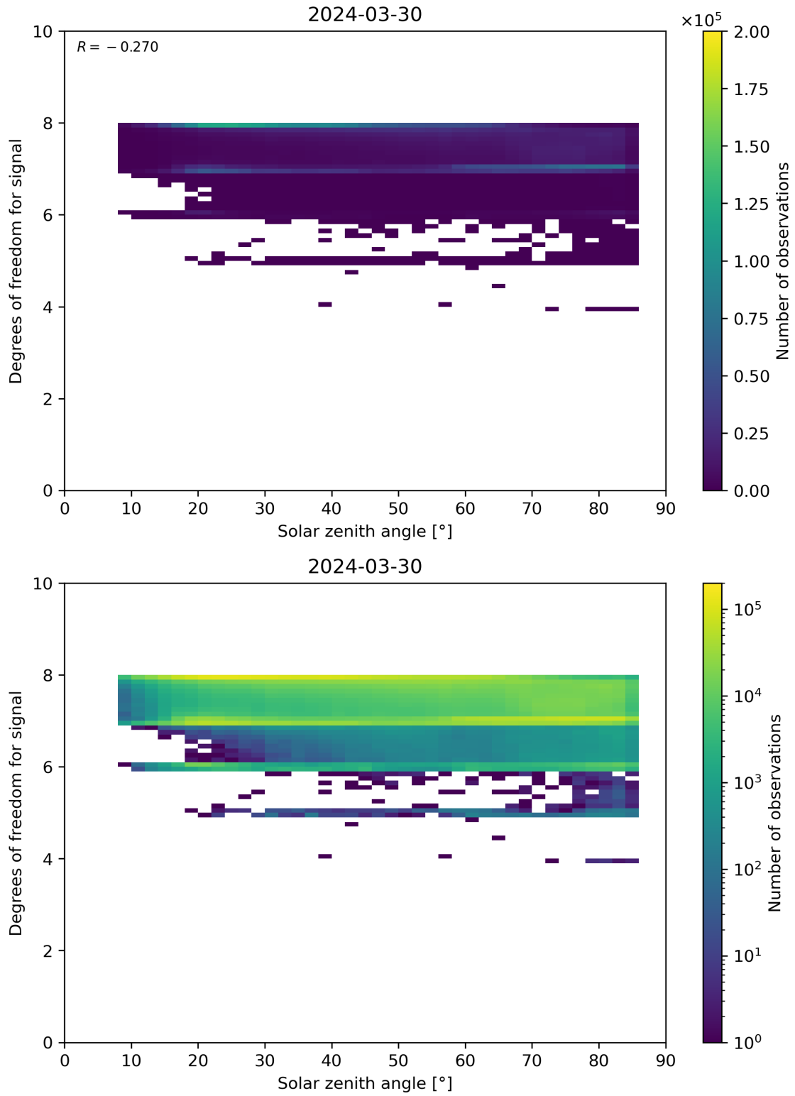
Figure 65: Scatter density plot of “Solar zenith angle” against “Degrees of freedom for signal” for 2024-03-30 to 2024-03-31.
