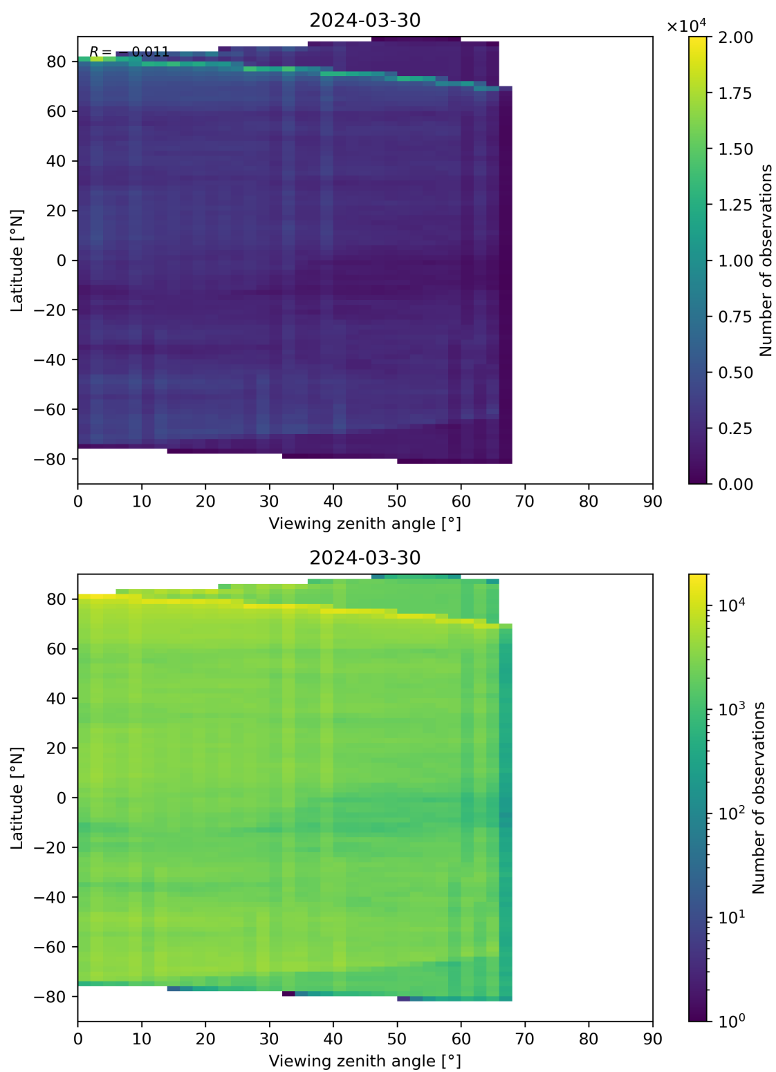
Figure 74: Scatter density plot of “Viewing zenith angle” against “Latitude” for 2024-03-30 to 2024-03-31.
