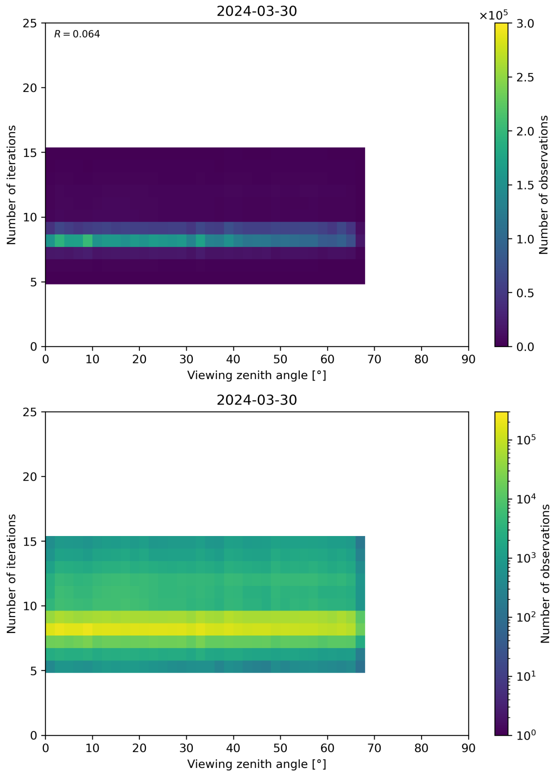
Figure 75: Scatter density plot of “Viewing zenith angle” against “Number of iterations” for 2024-03-30 to 2024-03-31.
