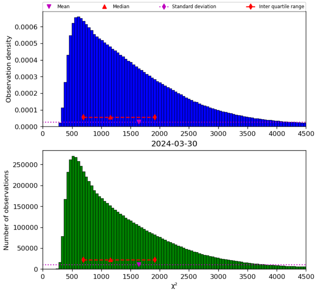
Figure 22: Histogram of “ \chi^2 ” for 2024-03-30 to 2024-03-31
