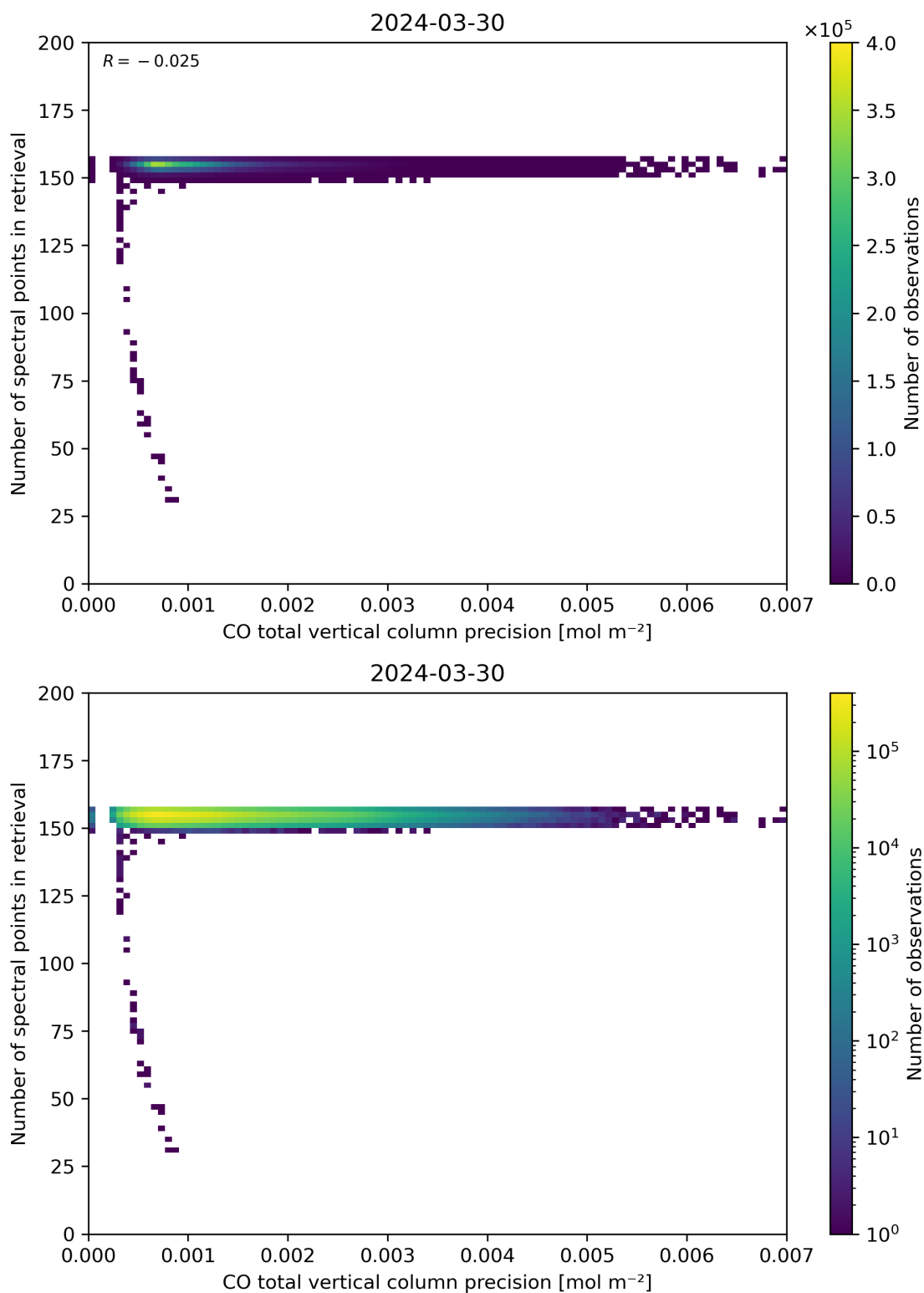
Figure 47: Scatter density plot of “CO total vertical column precision” against “Number of spectral points in retrieval” for 2024-03-30 to 2024-03-31.
