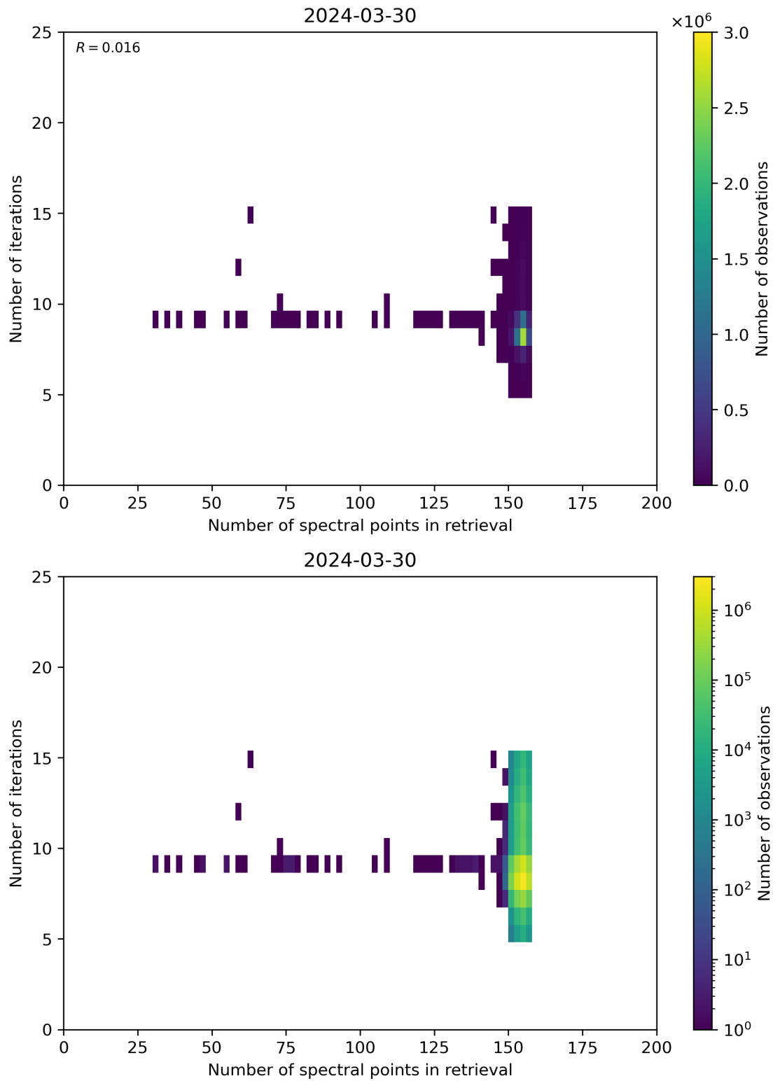
Figure 60: Scatter density plot of “Number of spectral points in retrieval” against “Number of iterations” for 2024-03-30 to 2024-03-31.
