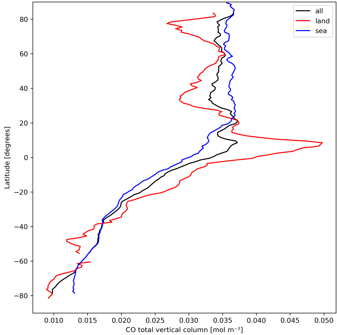
Figure 10: Zonal average of “CO total vertical column” for 2024-03-30 to 2024-03-31.
