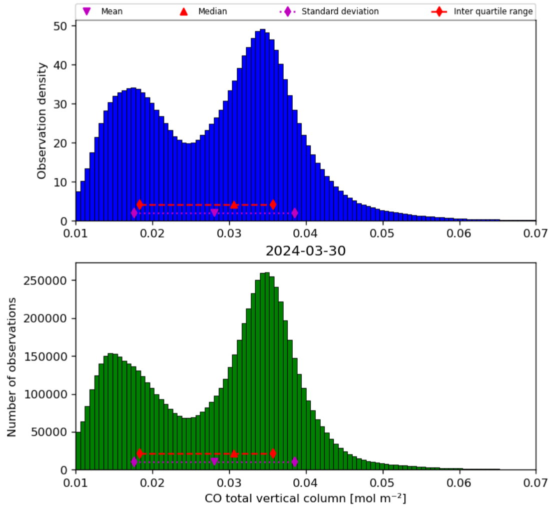
Figure 18: Histogram of “CO total vertical column” for 2024-03-30 to 2024-03-31
