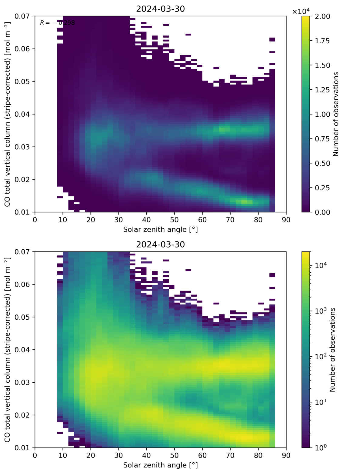
Figure 62: Scatter density plot of “Solar zenith angle” against “CO total vertical column (stripe-corrected)” for 2024-03-30 to 2024-03-31.
