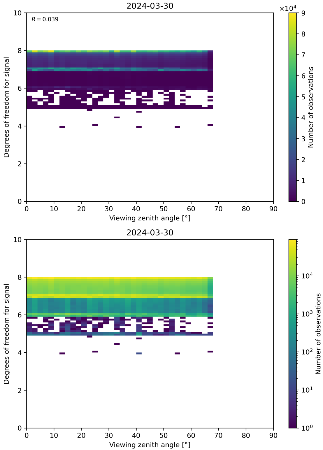
Figure 73: Scatter density plot of “Viewing zenith angle” against “Degrees of freedom for signal” for 2024-03-30 to 2024-03-31.
