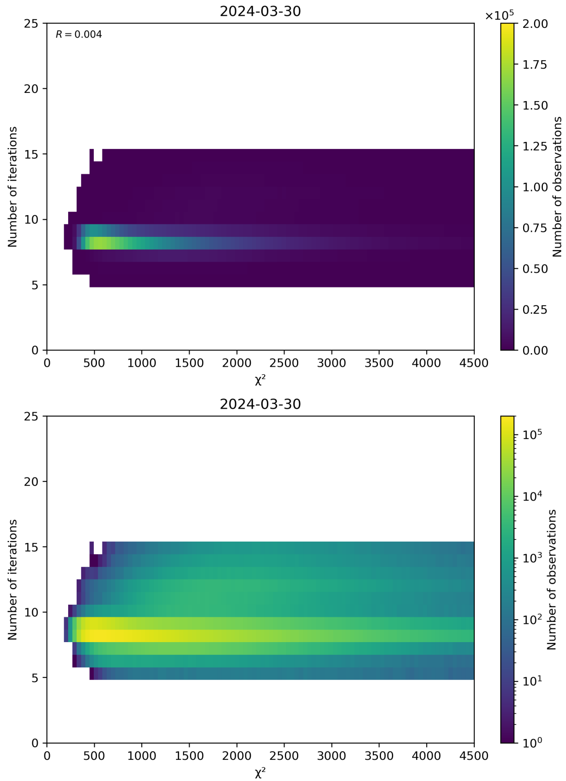
Figure 49: Scatter density plot of “ \chi^2 ” against “Number of iterations” for 2024-03-30 to 2024-03-31.
