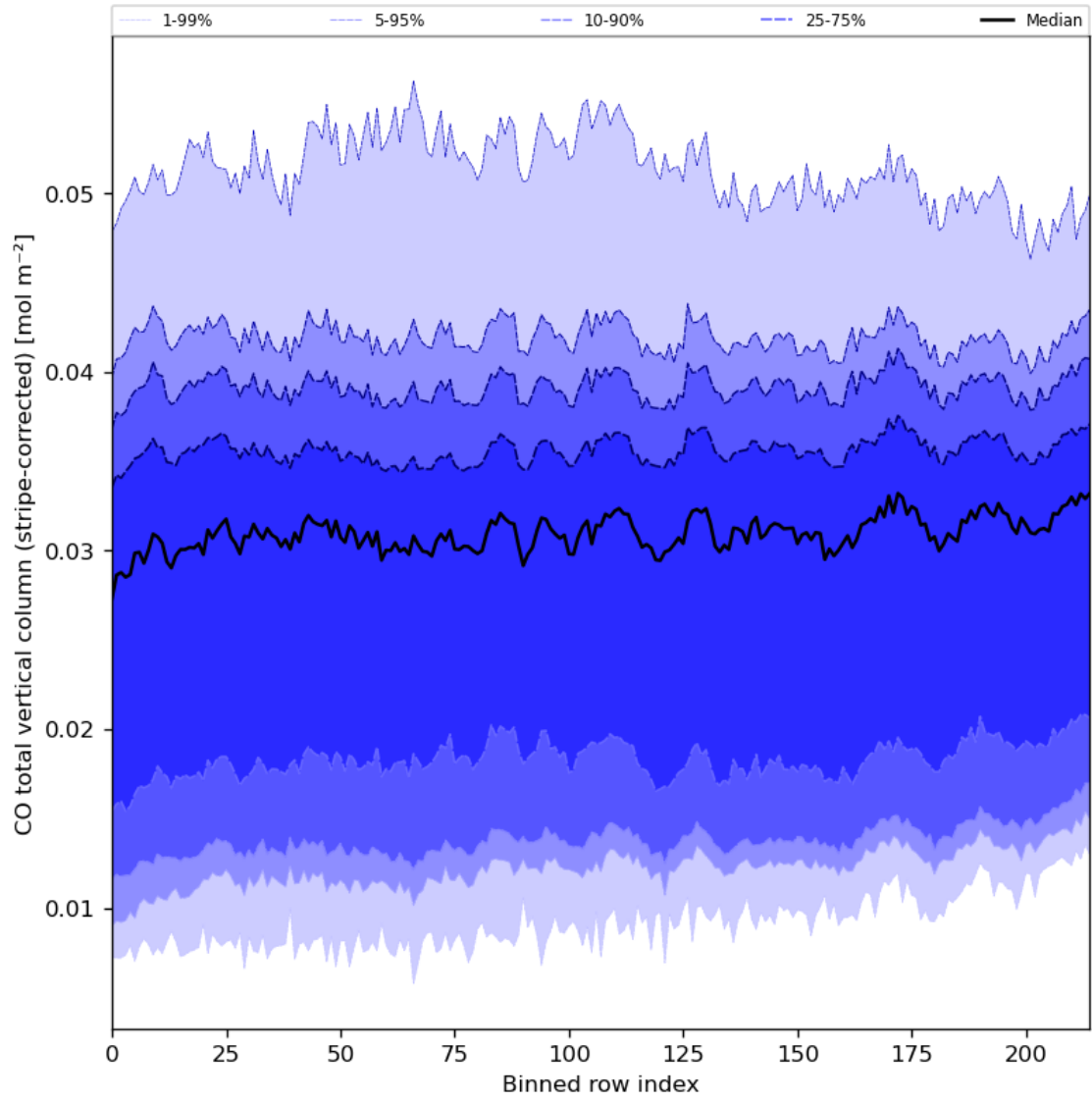
Figure 27: Along track statistics of “CO total vertical column (stripe-corrected)” for 2024-03-30 to 2024-03-31
