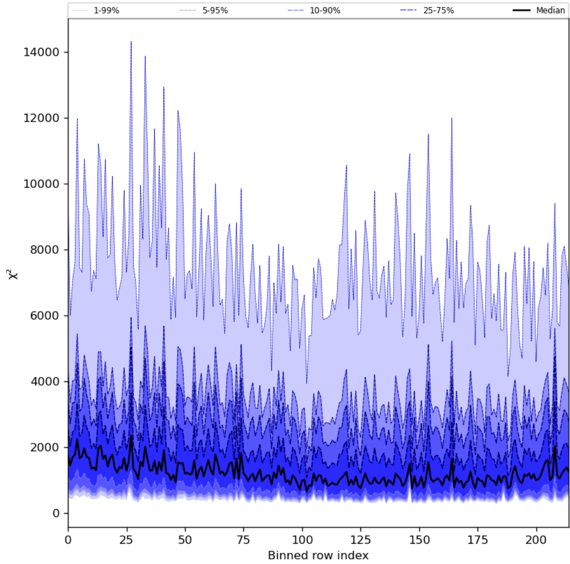
Figure 30: Along track statistics of “ \chi^2 ” for 2024-03-30 to 2024-03-31
