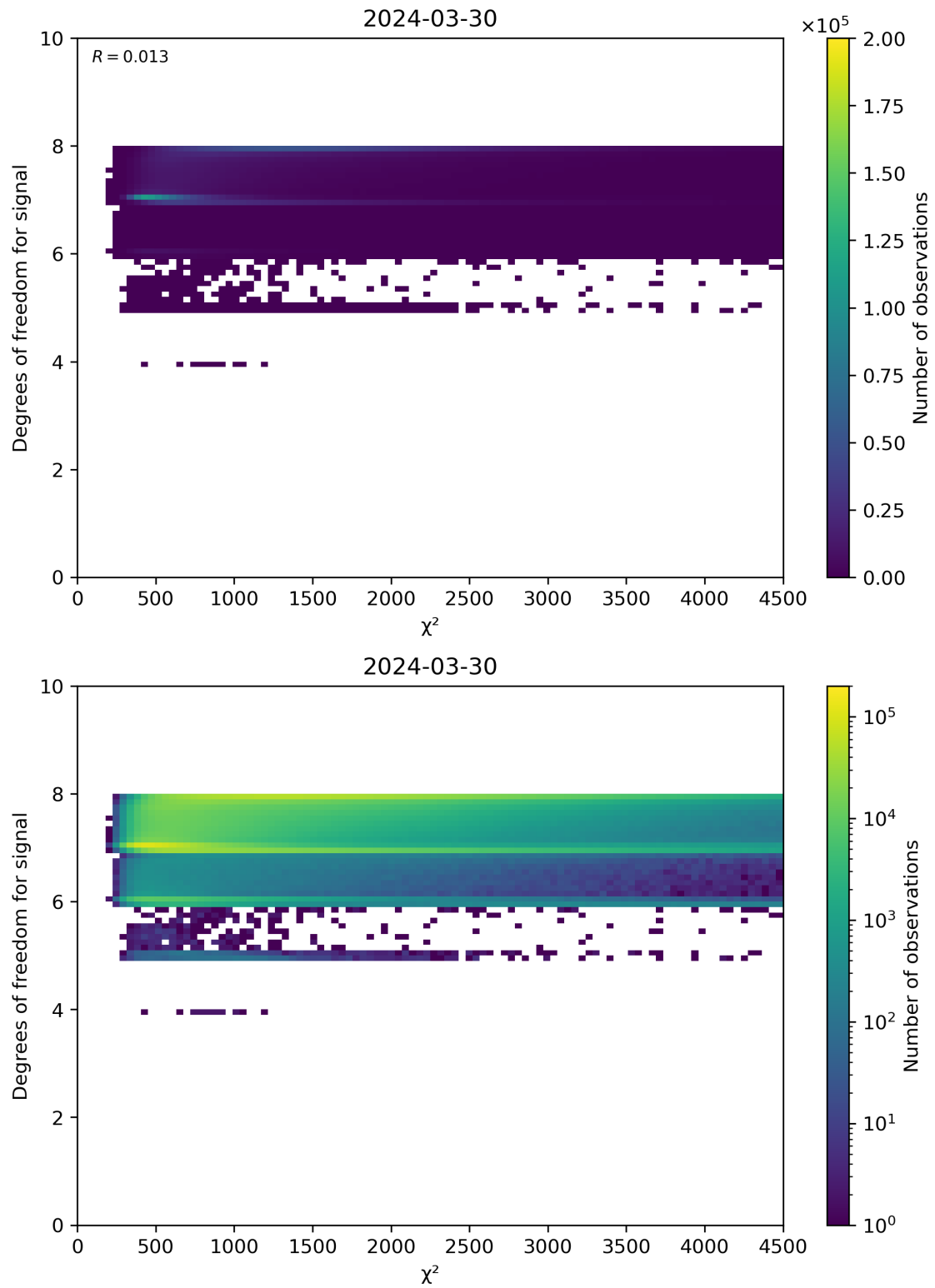
Figure 48: Scatter density plot of “ \chi^2 ” against “Degrees of freedom for signal” for 2024-03-30 to 2024-03-31.
