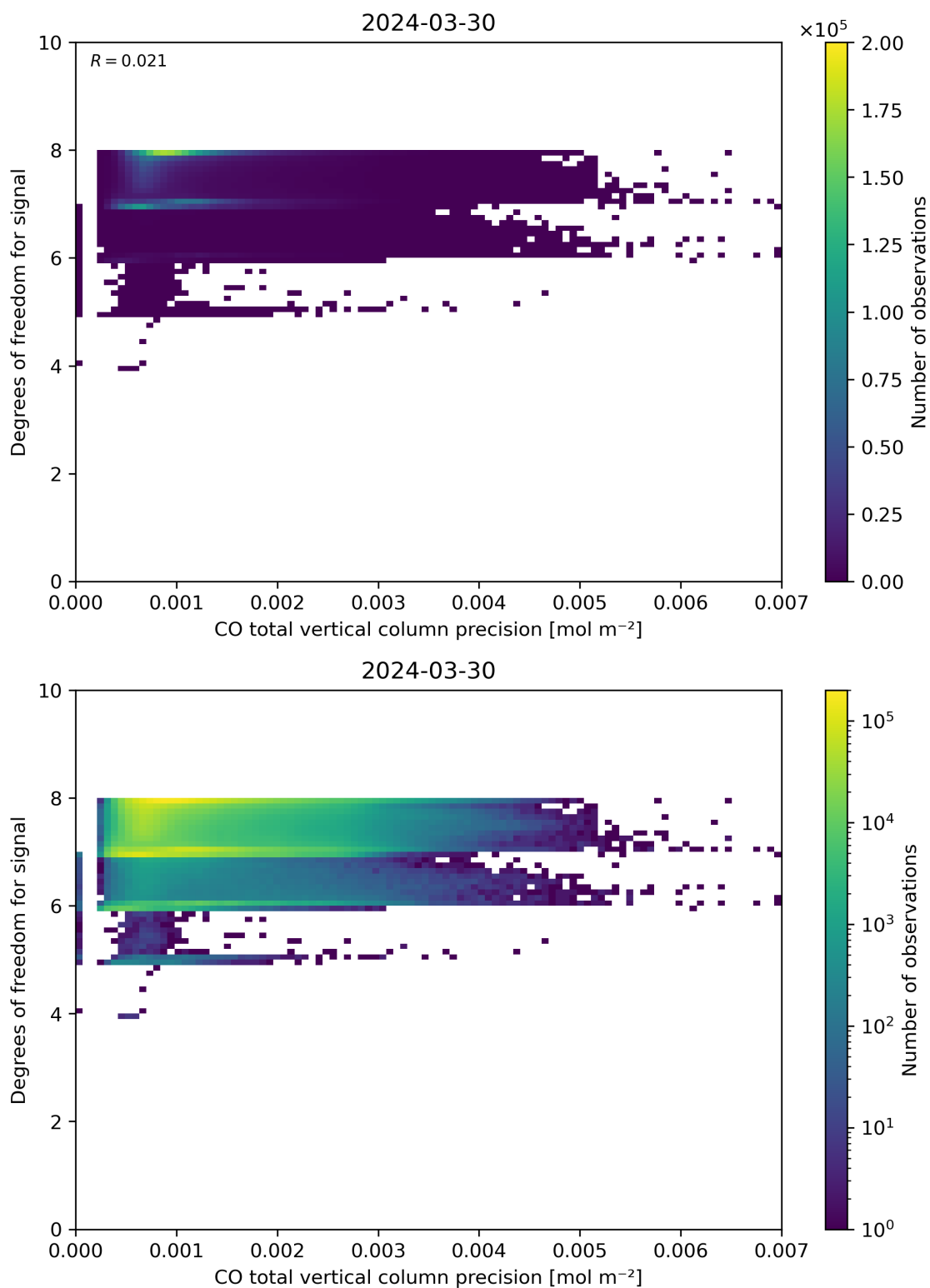
Figure 45: Scatter density plot of “CO total vertical column precision” against “Degrees of freedom for signal” for 2024-03-30 to 2024-03-31.
