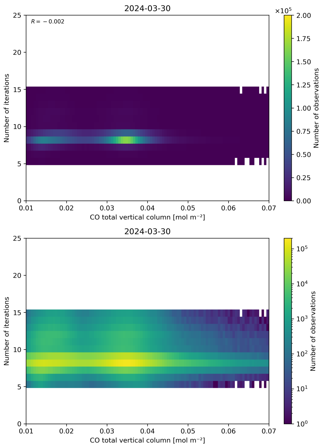
Figure 42: Scatter density plot of “CO total vertical column” against “Number of iterations” for 2024-03-30 to 2024-03-31.
