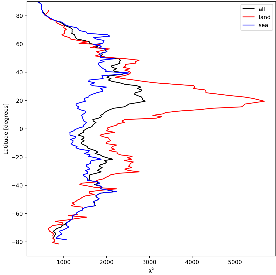
Figure 14: Zonal average of “ \chi^2 ” for 2024-03-30 to 2024-03-31.
