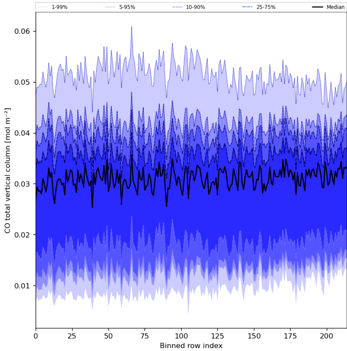
Figure 26: Along track statistics of “CO total vertical column” for 2024-03-30 to 2024-03-31
