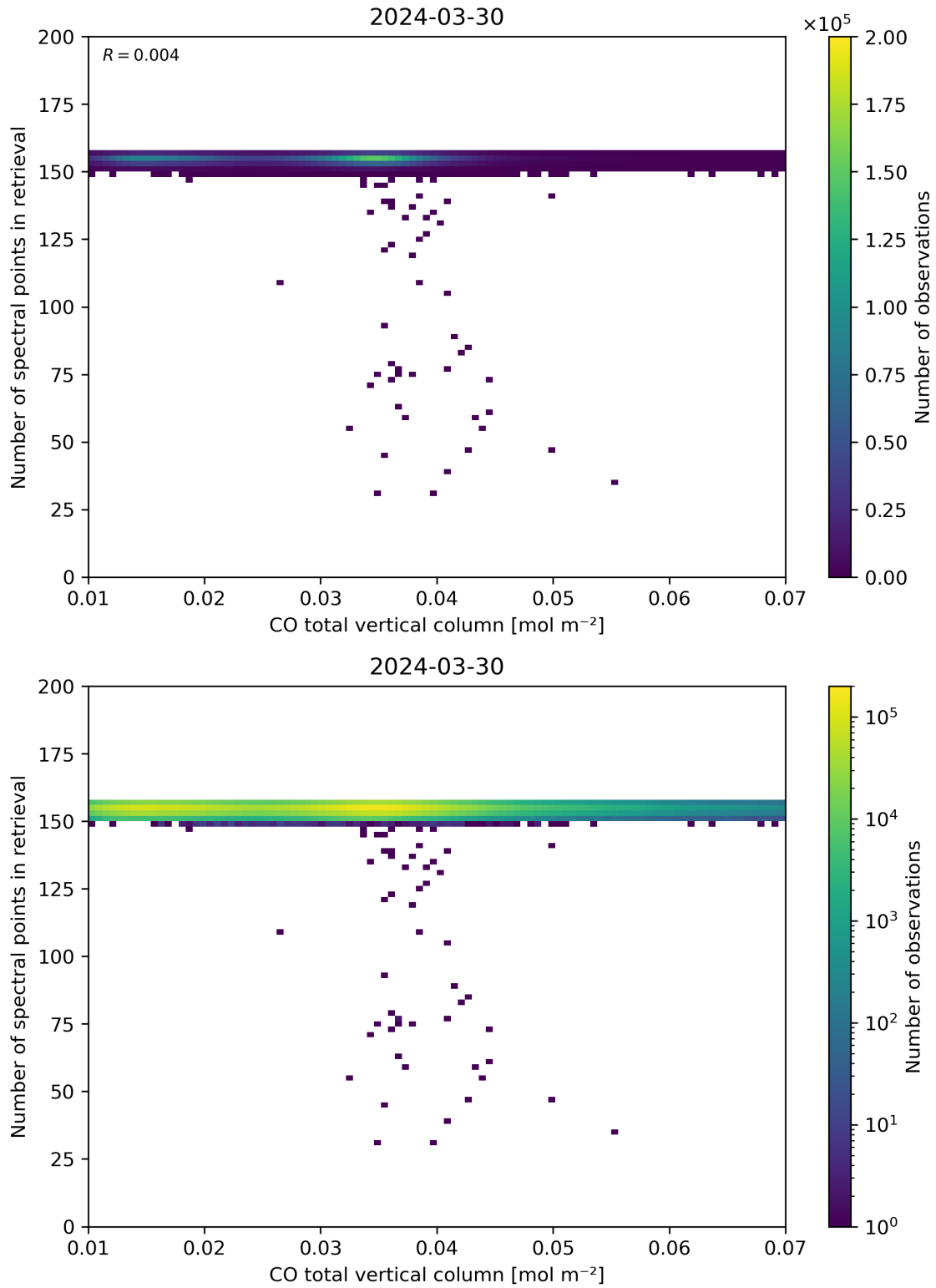
Figure 43: Scatter density plot of “CO total vertical column” against “Number of spectral points in retrieval” for 2024-03-30 to 2024-03-31.
