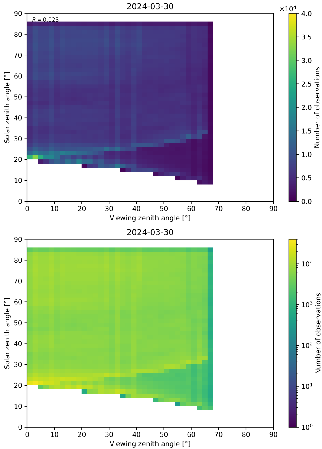
Figure 77: Scatter density plot of “Viewing zenith angle” against “Solar zenith angle” for 2024-03-30 to 2024-03-31.
