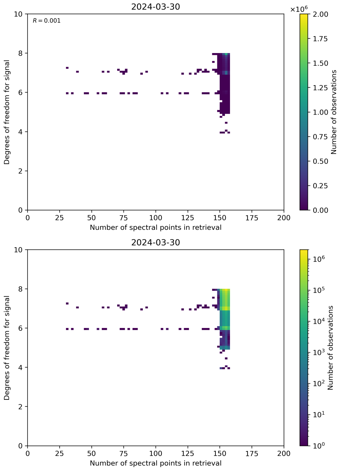
Figure 59: Scatter density plot of “Number of spectral points in retrieval” against “Degrees of freedom for signal” for 2024-03-30 to 2024-03-31.
