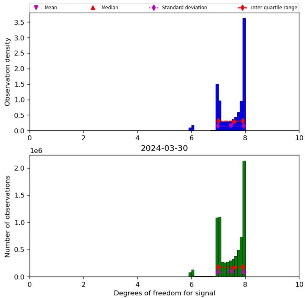
Figure 23: Histogram of “Degrees of freedom for signal” for 2024-03-30 to 2024-03-31
