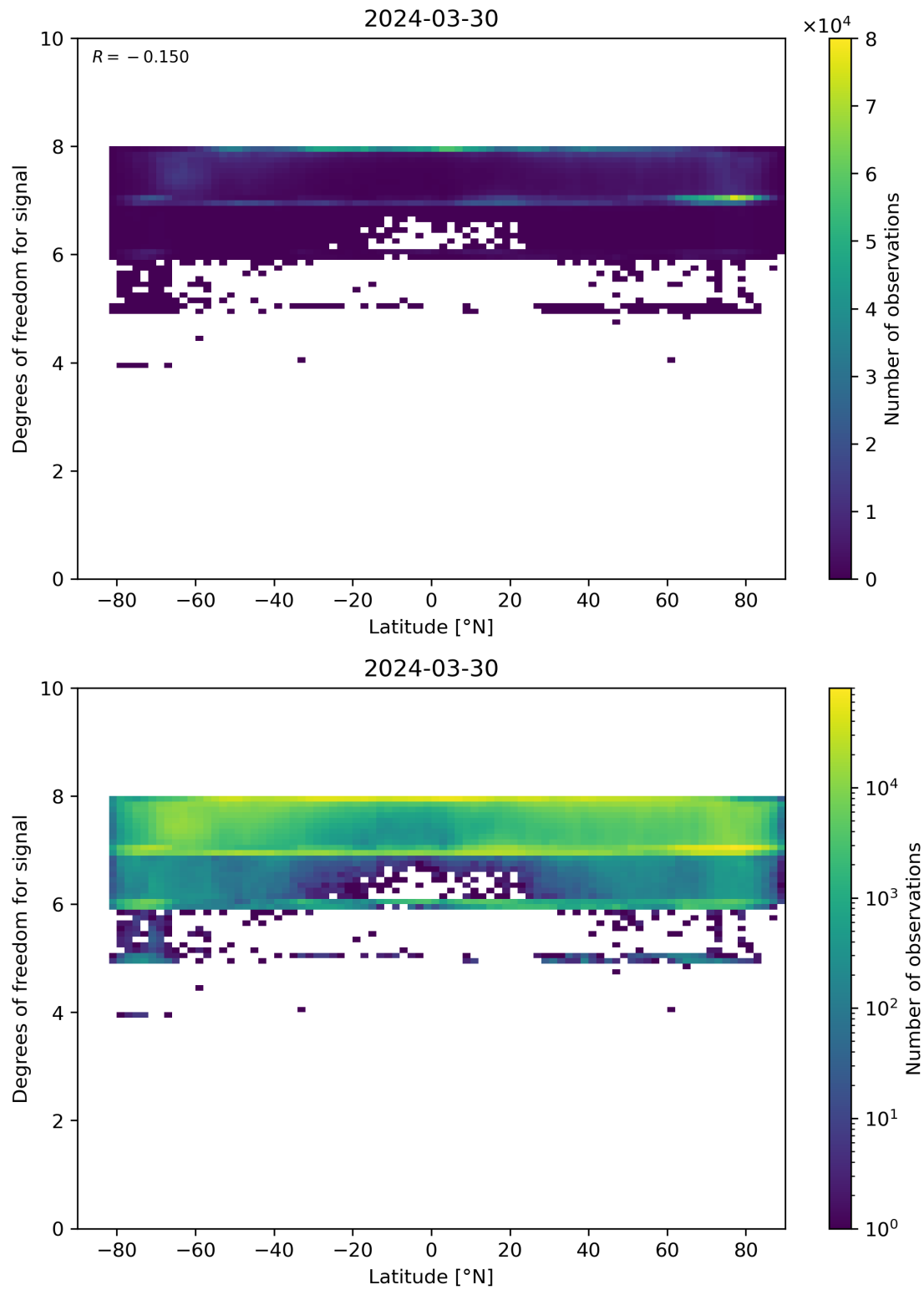
Figure 55: Scatter density plot of “Latitude” against “Degrees of freedom for signal” for 2024-03-30 to 2024-03-31.
