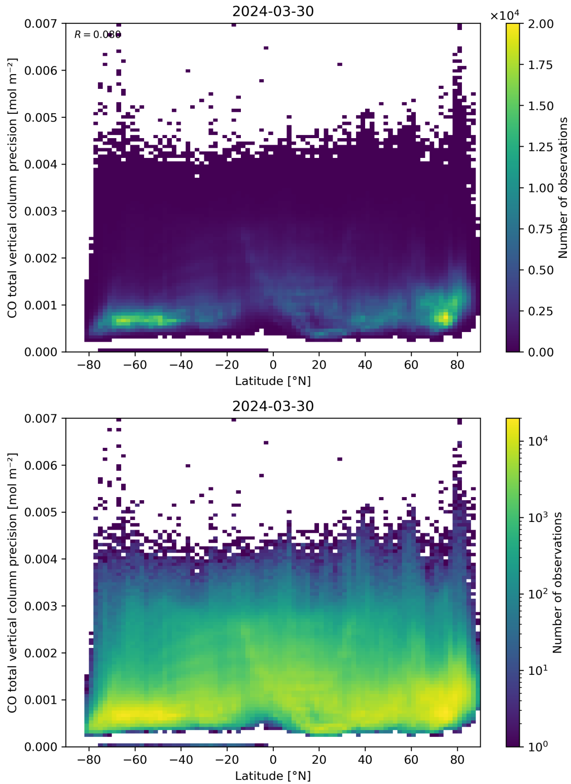
Figure 53: Scatter density plot of “Latitude” against “CO total vertical column precision” for 2024-03-30 to 2024-03-31.
