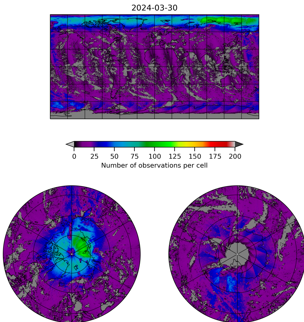
Figure 8: Map of the number of observations for 2024-03-30 to 2024-03-31
