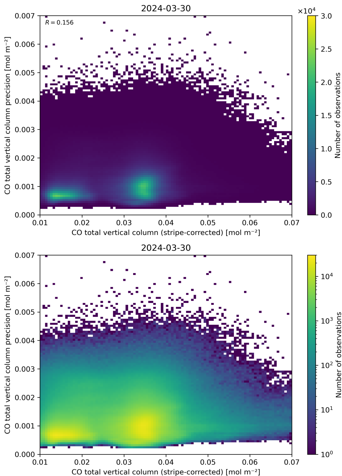
Figure 36: Scatter density plot of “CO total vertical column (stripe-corrected)” against “CO total vertical column precision” for 2024-03-30 to 2024-03-31.
