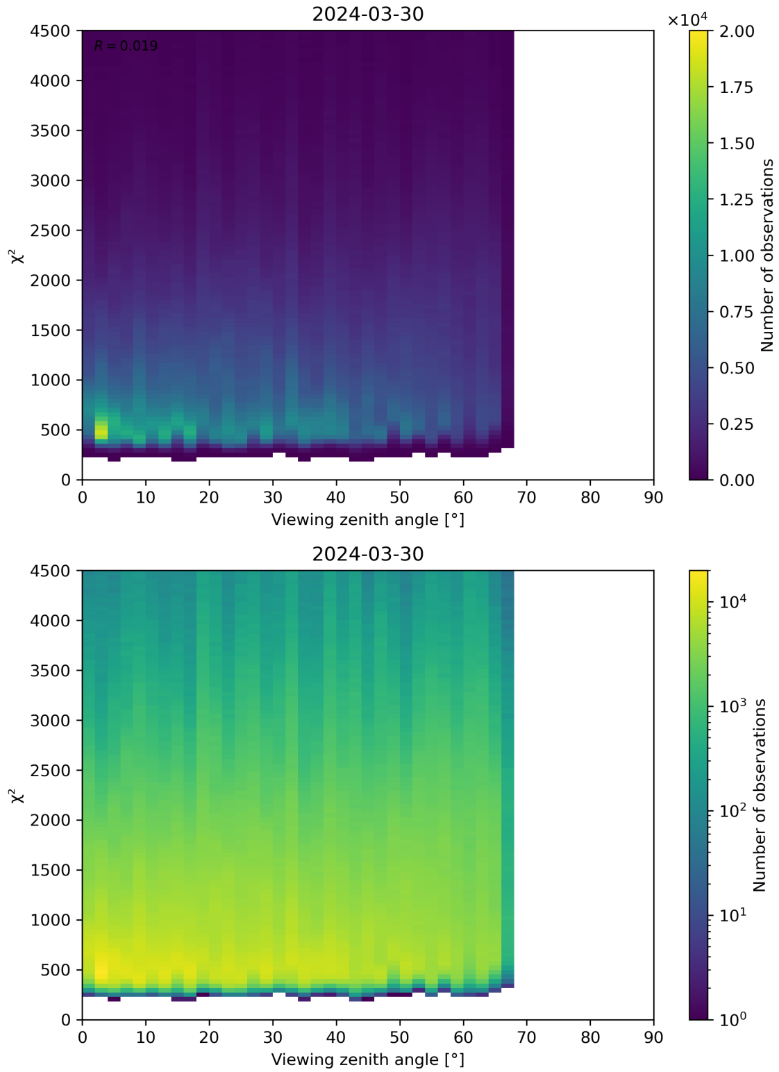
Figure 72: Scatter density plot of “Viewing zenith angle” against “ \chi^2 ” for 2024-03-30 to 2024-03-31.
