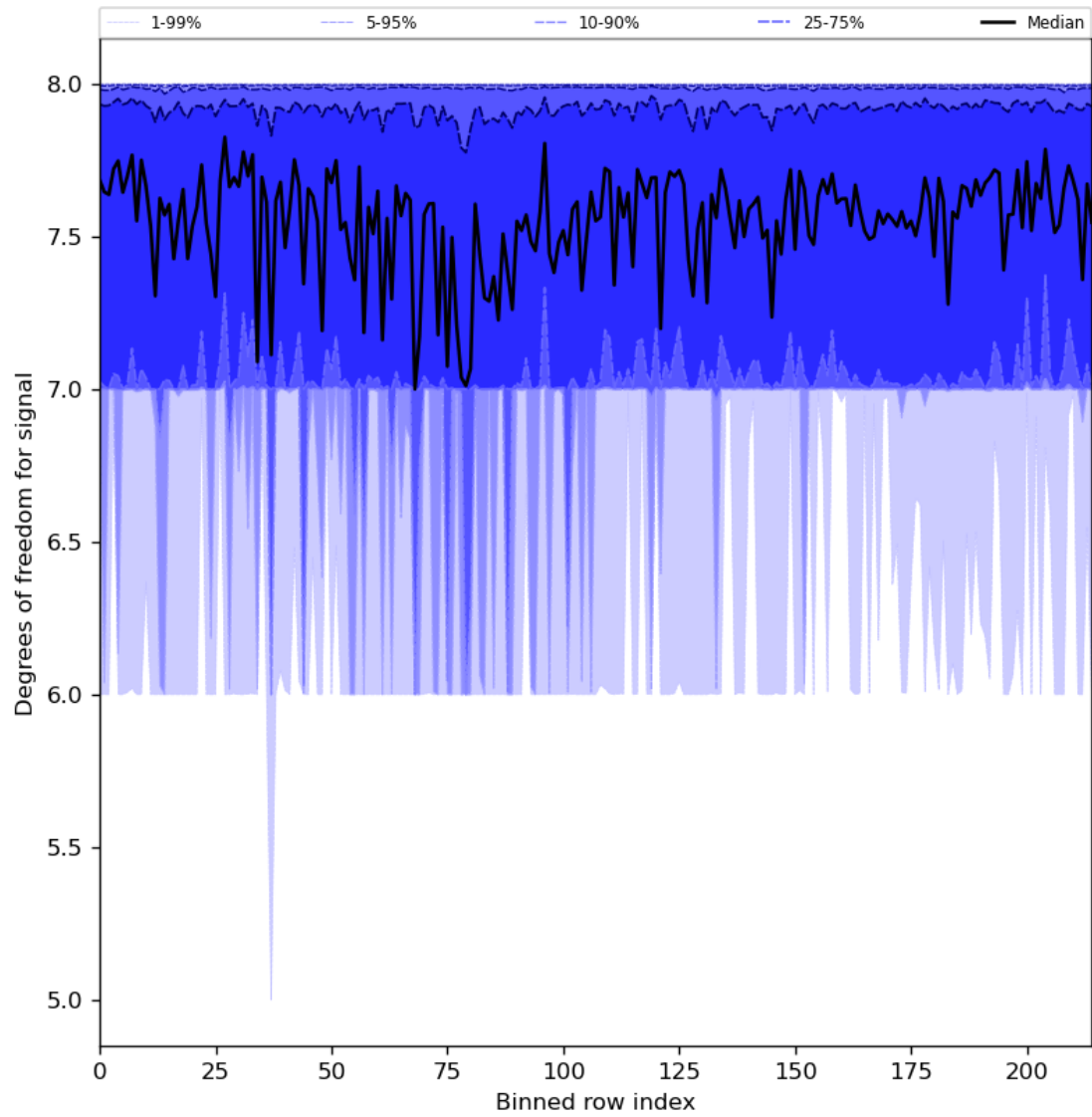
Figure 31: Along track statistics of “Degrees of freedom for signal” for 2024-03-30 to 2024-03-31
