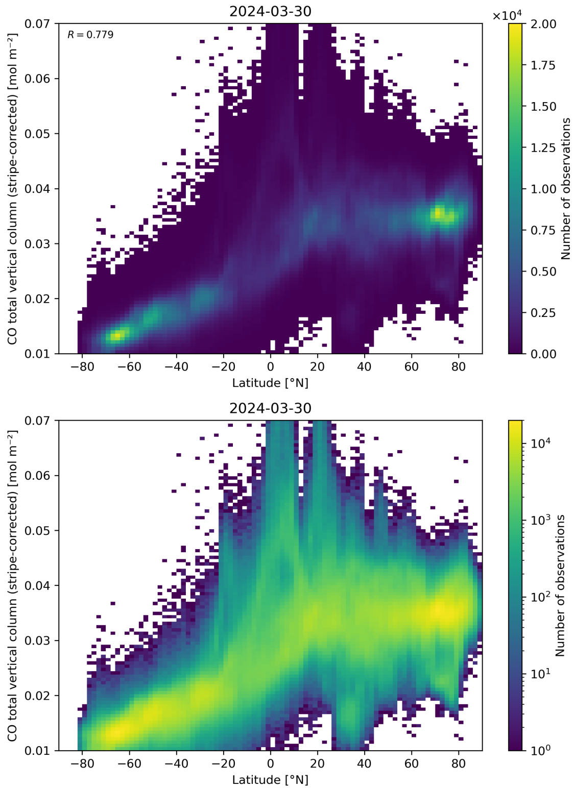
Figure 52: Scatter density plot of “Latitude” against “CO total vertical column (stripe-corrected)” for 2024-03-30 to 2024-03-31.
