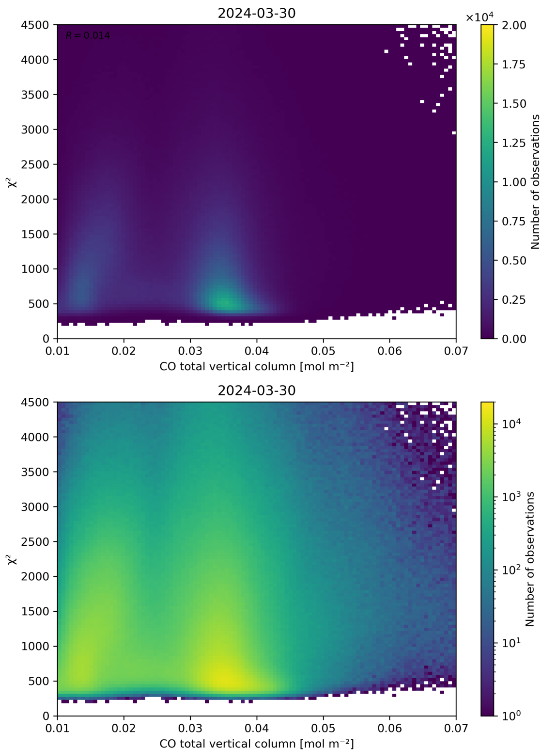
Figure 35: Scatter density plot of “CO total vertical column” against “ \chi^2 ” for 2024-03-30 to 2024-03-31.
