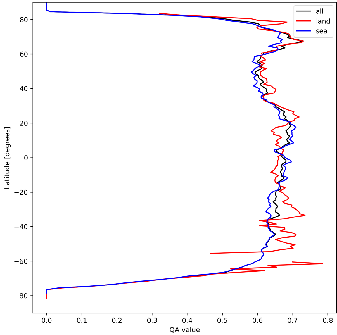
Figure 9: Zonal average of “QA value” for 2024-03-30 to 2024-03-31.
