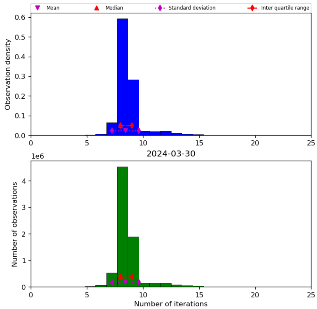
Figure 24: Histogram of “Number of iterations” for 2024-03-30 to 2024-03-31
