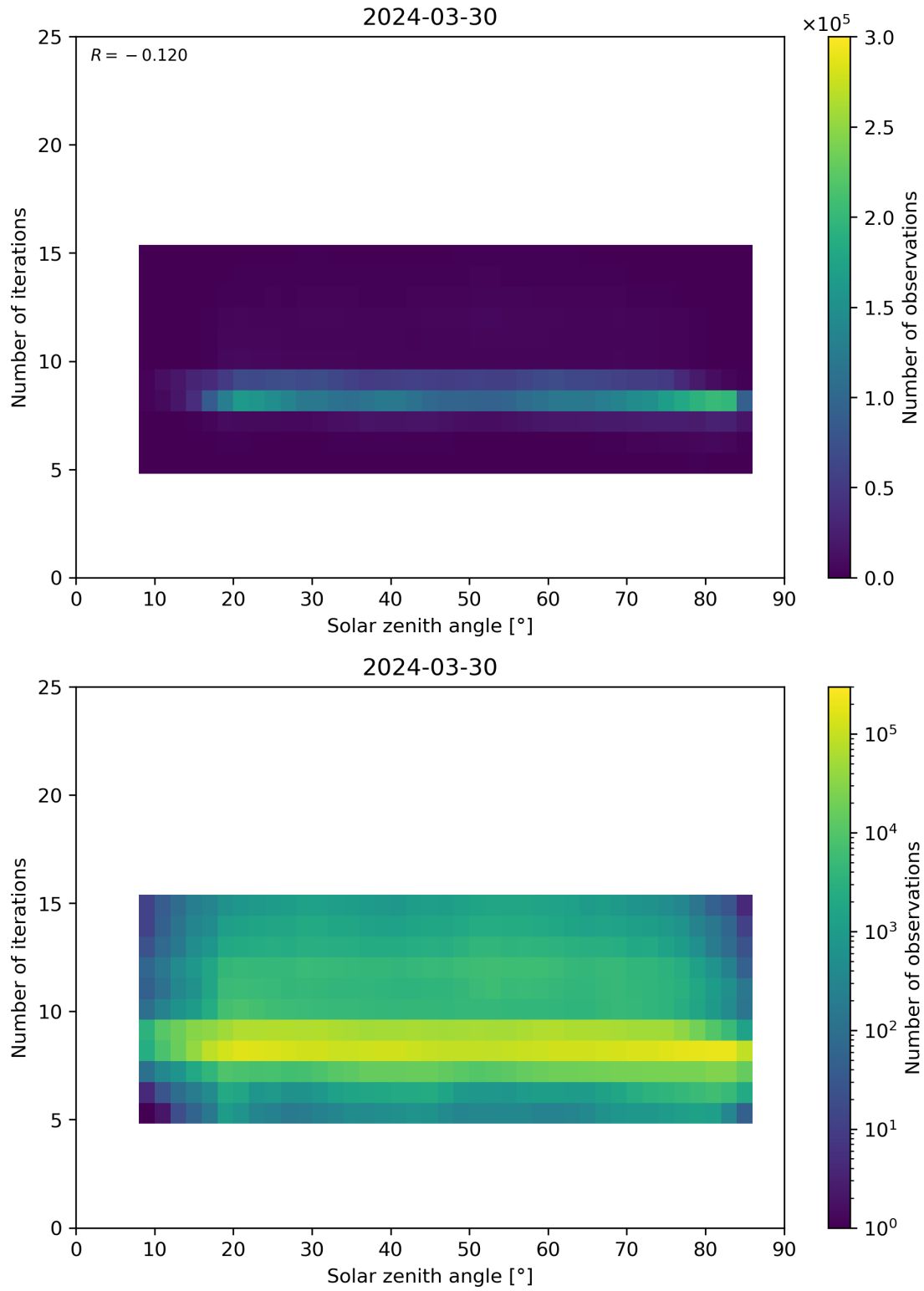
Figure 67: Scatter density plot of “Solar zenith angle” against “Number of iterations” for 2024-03-30 to 2024-03-31.
