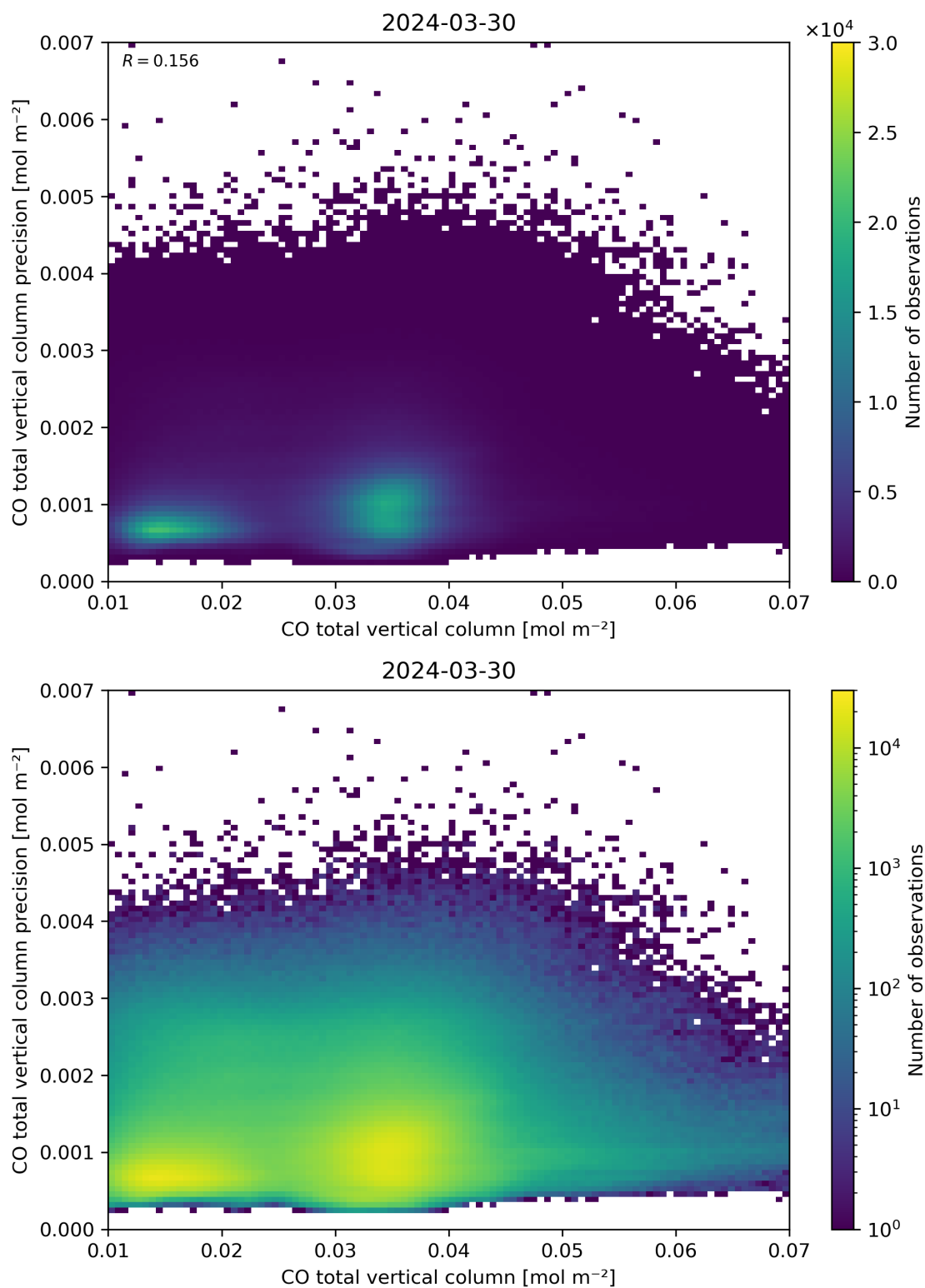
Figure 34: Scatter density plot of “CO total vertical column” against “CO total vertical column precision” for 2024-03-30 to 2024-03-31.
