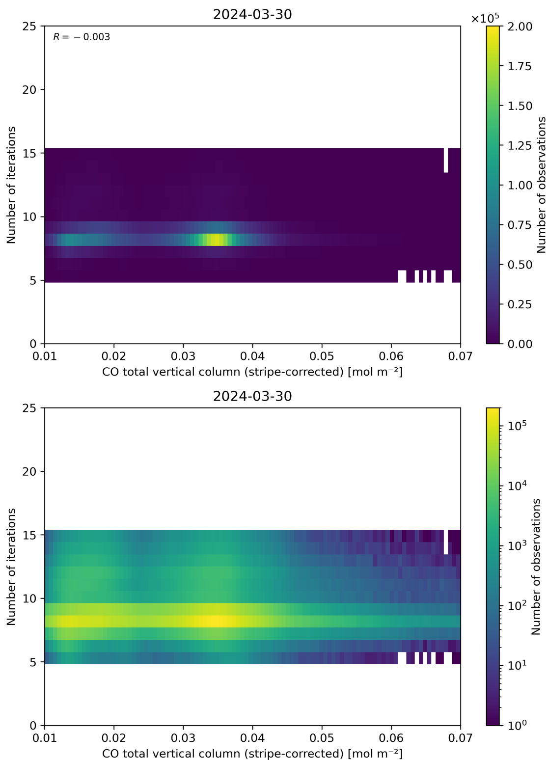
Figure 39: Scatter density plot of “CO total vertical column (stripe-corrected)” against “Number of iterations” for 2024-03-30 to 2024-03-31.
