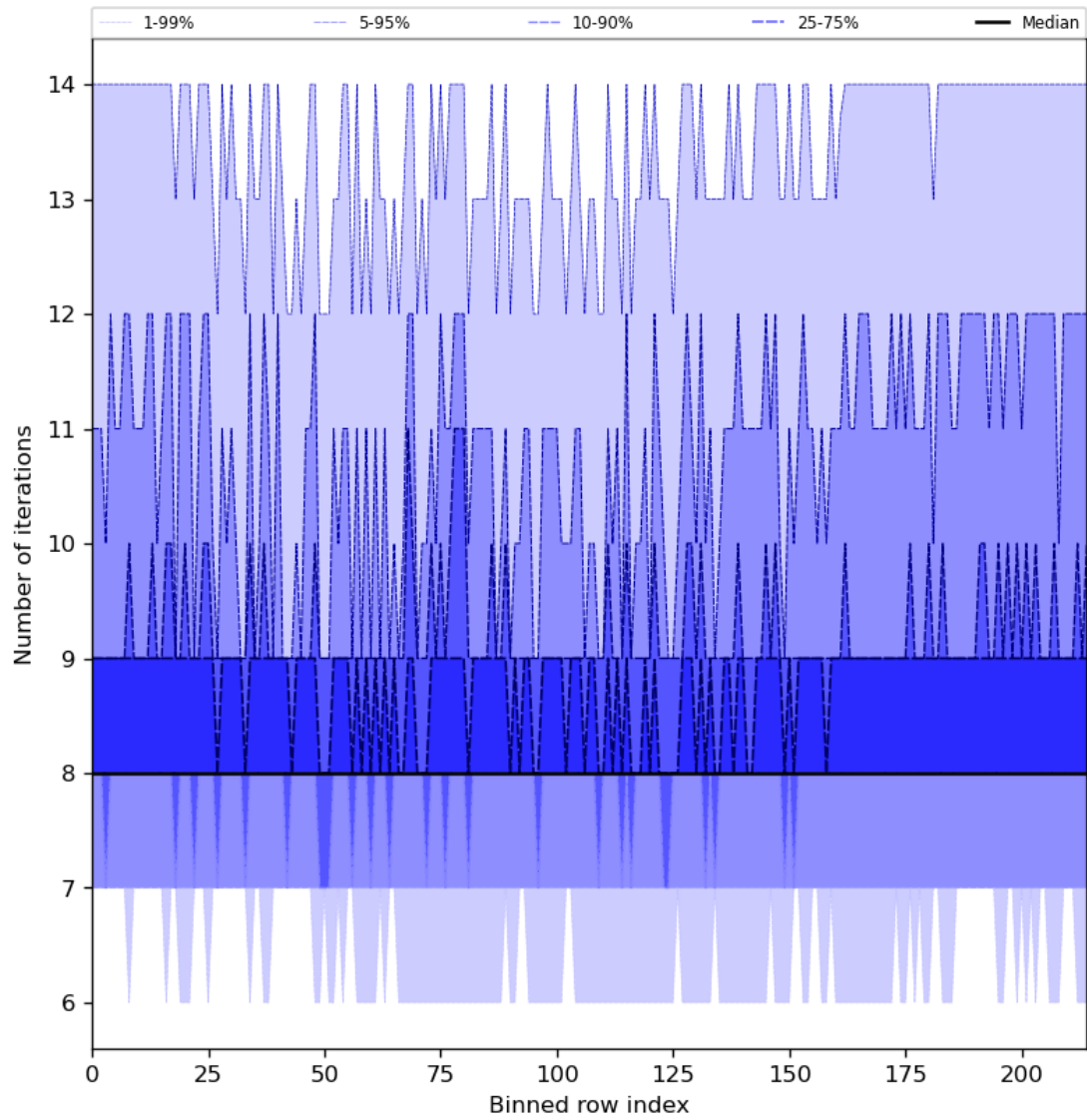
Figure 32: Along track statistics of “Number of iterations” for 2024-03-30 to 2024-03-31
