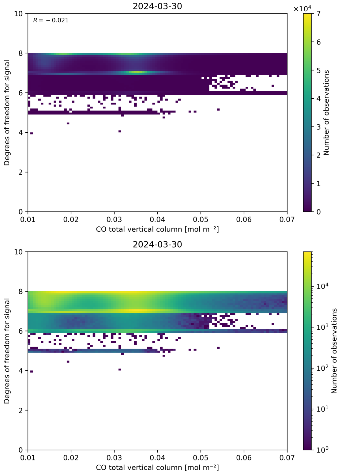
Figure 41: Scatter density plot of “CO total vertical column” against “Degrees of freedom for signal” for 2024-03-30 to 2024-03-31.
