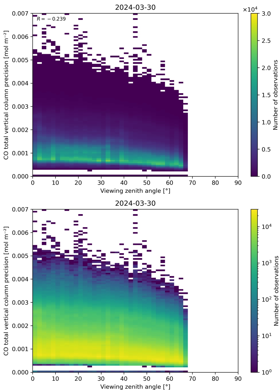
Figure 71: Scatter density plot of “Viewing zenith angle” against “CO total vertical column precision” for 2024-03-30 to 2024-03-31.
