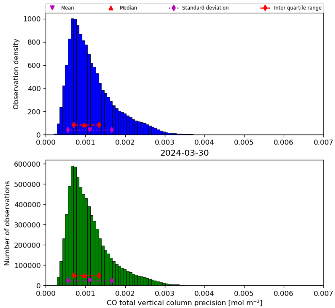
Figure 20: Histogram of “CO total vertical column precision” for 2024-03-30 to 2024-03-31
