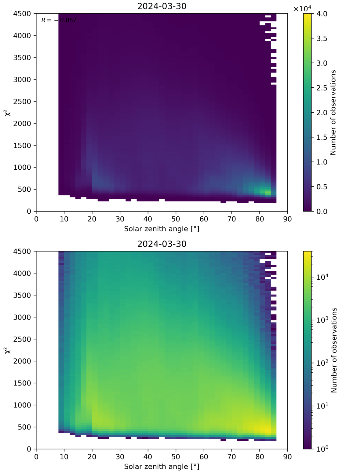
Figure 64: Scatter density plot of “Solar zenith angle” against “ \chi^2 ” for 2024-03-30 to 2024-03-31.
