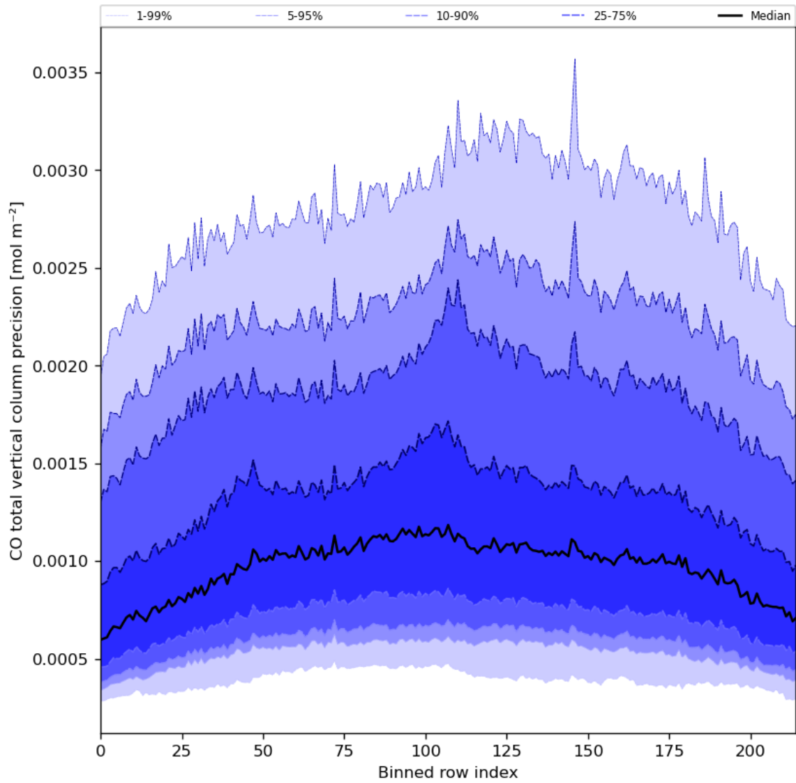
Figure 28: Along track statistics of “CO total vertical column precision” for 2024-03-30 to 2024-03-31
