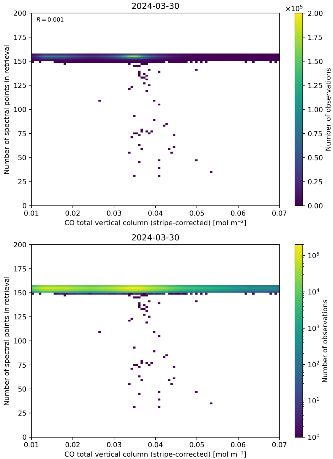
Figure 40: Scatter density plot of “CO total vertical column (stripe-corrected)” against “Number of spectral points in retrieval” for 2024-03-30 to 2024-03-31.
