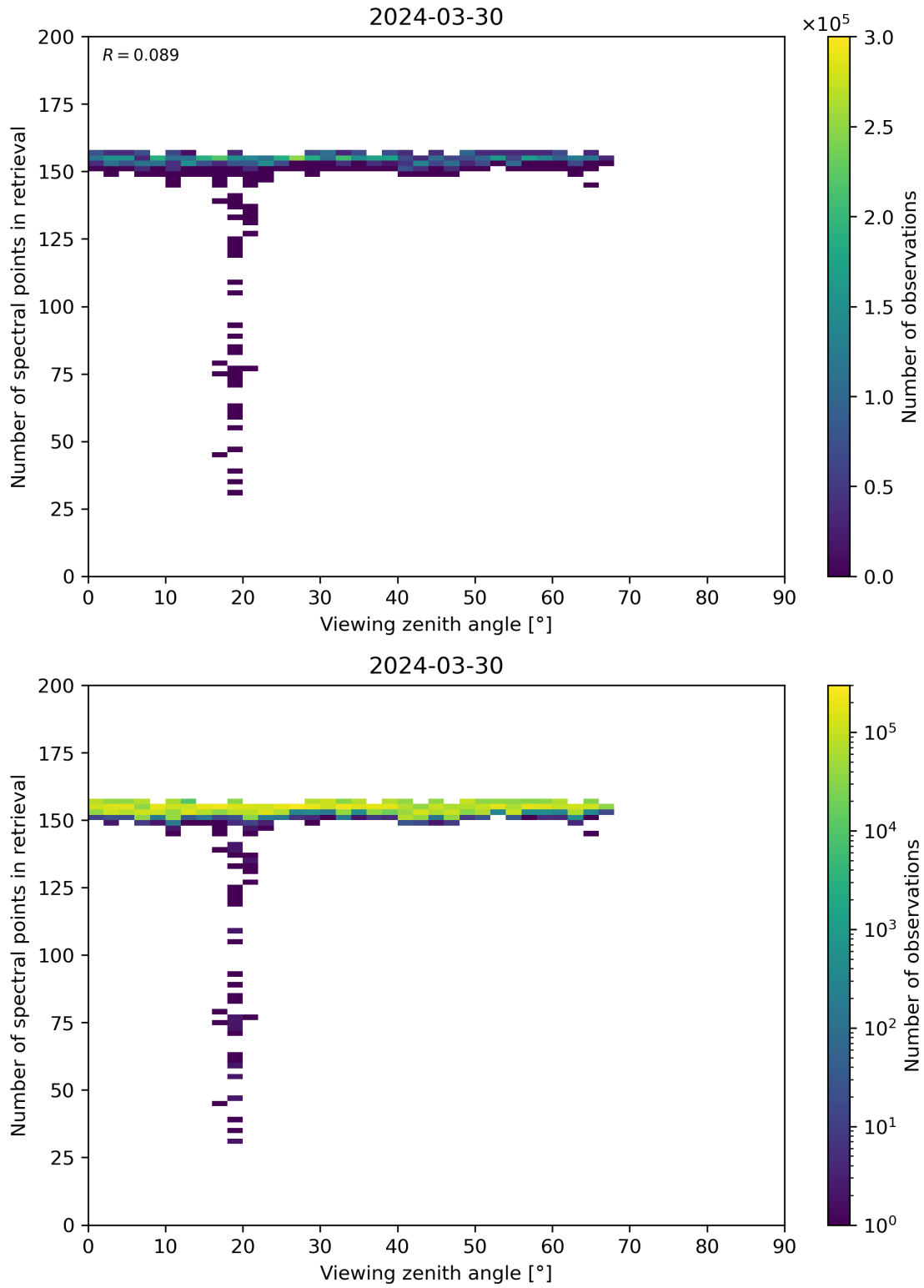
Figure 76: Scatter density plot of “Viewing zenith angle” against “Number of spectral points in retrieval” for 2024-03-30 to 2024-03-31.
