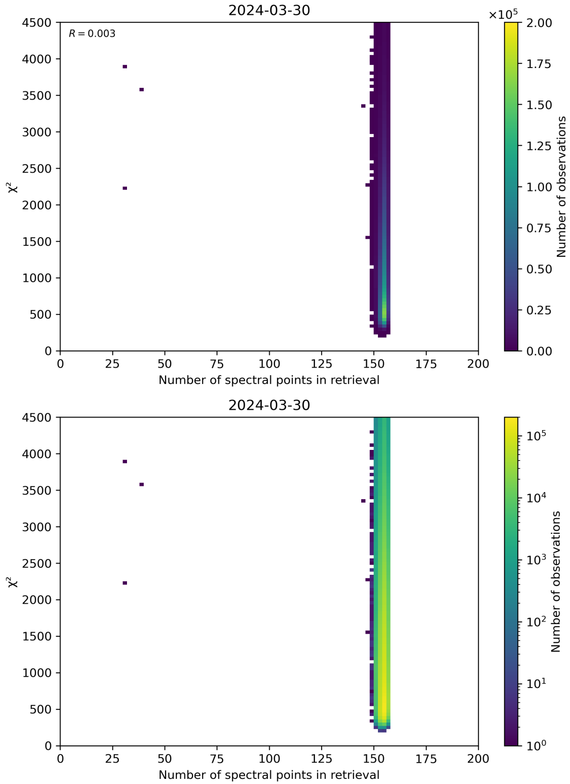
Figure 58: Scatter density plot of “Number of spectral points in retrieval” against “ \chi^2 ” for 2024-03-30 to 2024-03-31.
