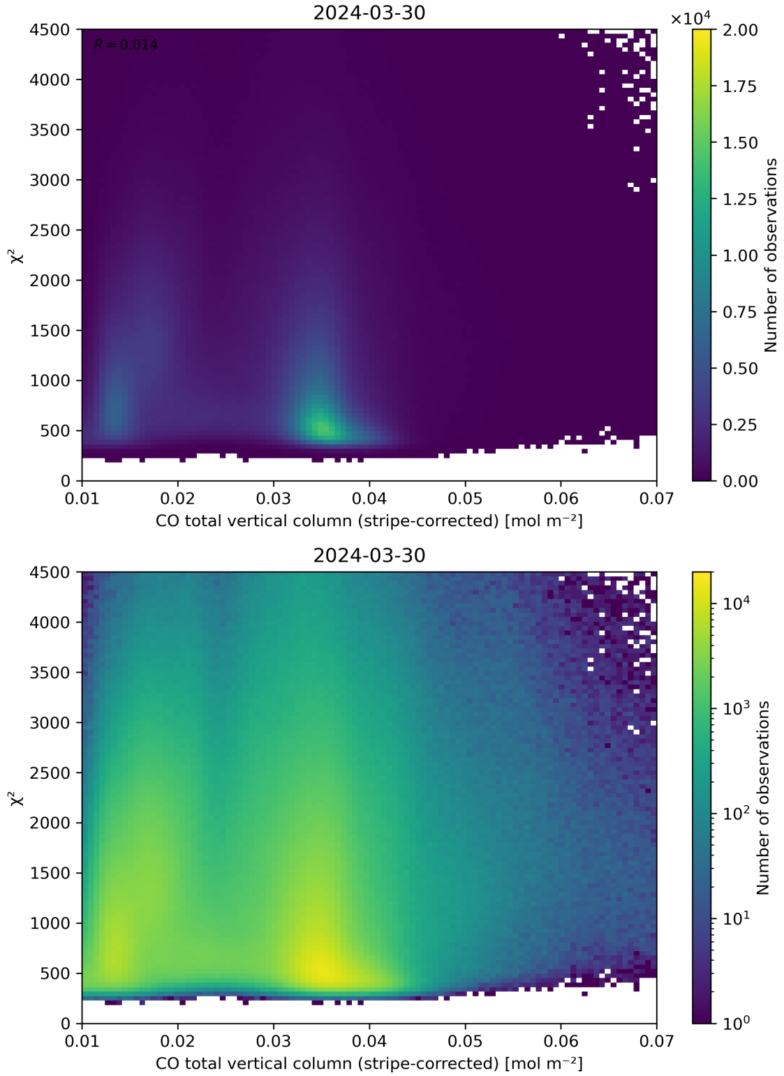
Figure 37: Scatter density plot of “CO total vertical column (stripe-corrected)” against “ \chi^2 ” for 2024-03-30 to 2024-03-31.
