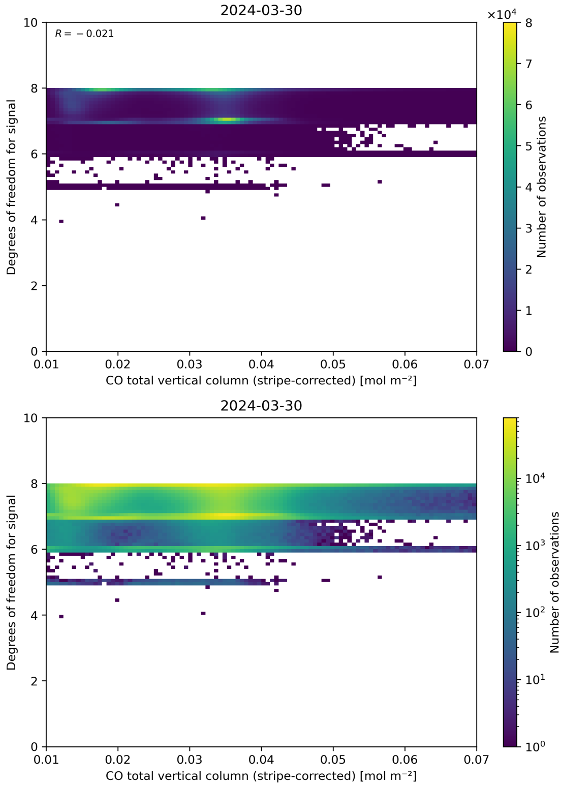
Figure 38: Scatter density plot of “CO total vertical column (stripe-corrected)” against “Degrees of freedom for signal” for 2024-03-30 to 2024-03-31.
