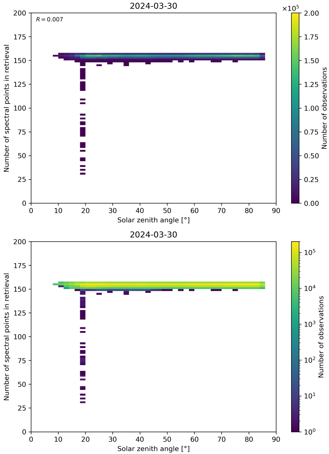
Figure 68: Scatter density plot of “Solar zenith angle” against “Number of spectral points in retrieval” for 2024-03-30 to 2024-03-31.
