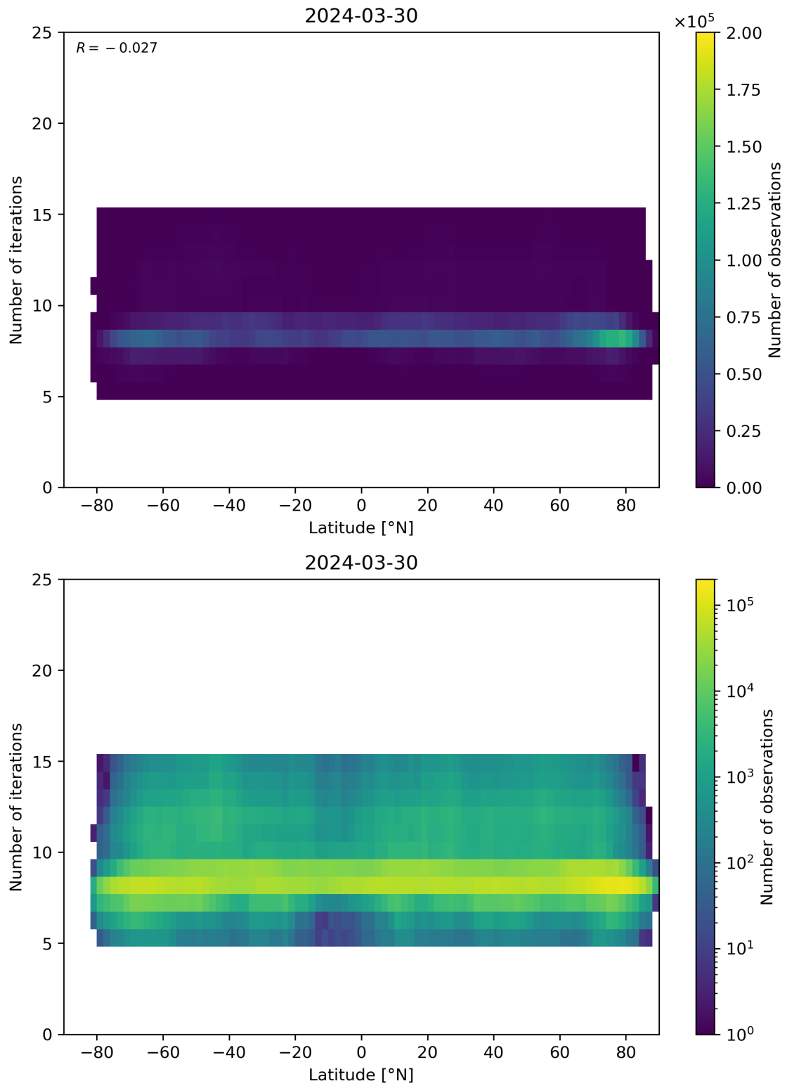
Figure 56: Scatter density plot of “Latitude” against “Number of iterations” for 2024-03-30 to 2024-03-31.
