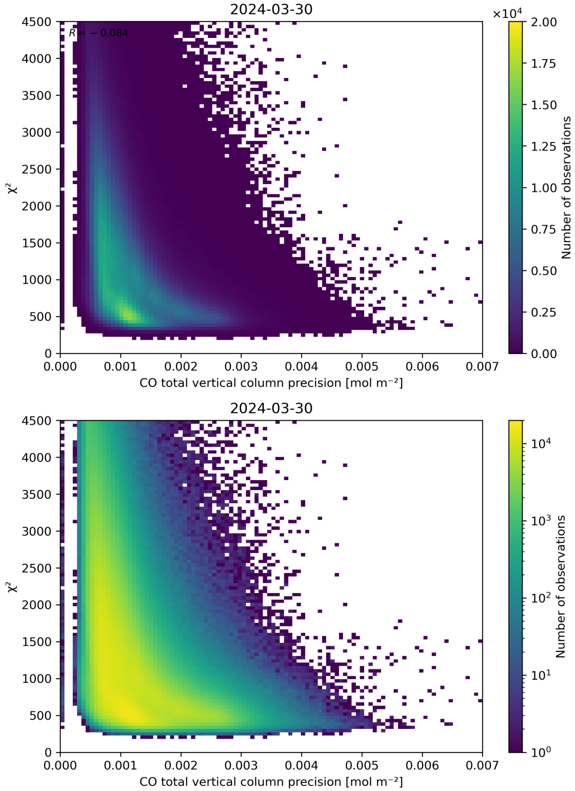
Figure 44: Scatter density plot of “CO total vertical column precision” against “ \chi^2 ” for 2024-03-30 to 2024-03-31.
