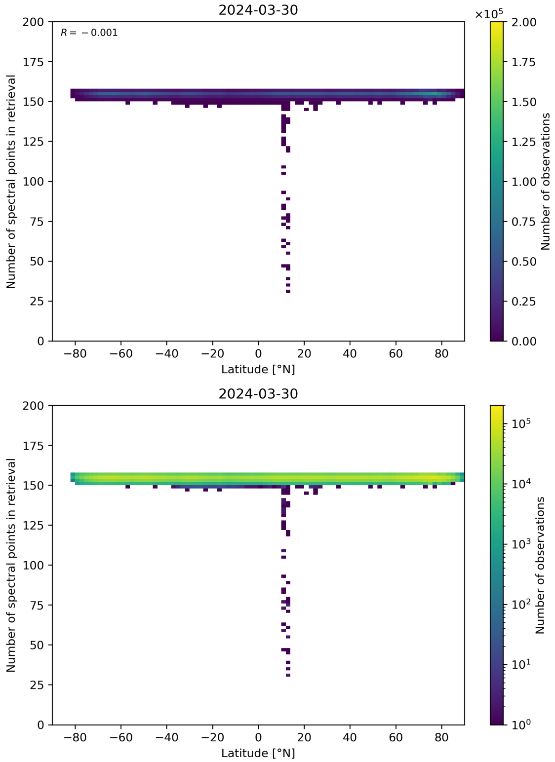
Figure 57: Scatter density plot of “Latitude” against “Number of spectral points in retrieval” for 2024-03-30 to 2024-03-31.
