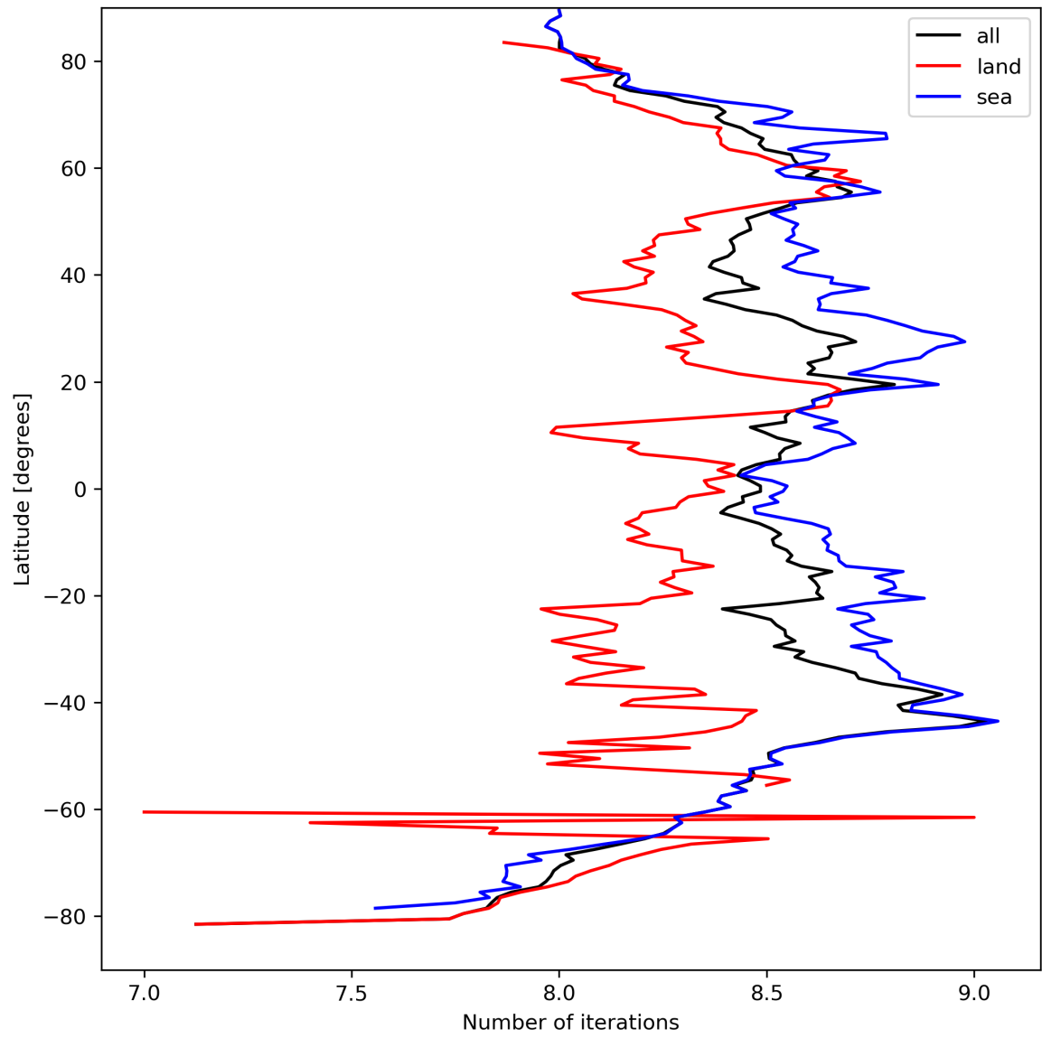
Figure 16: Zonal average of “Number of iterations” for 2024-03-30 to 2024-03-31.
