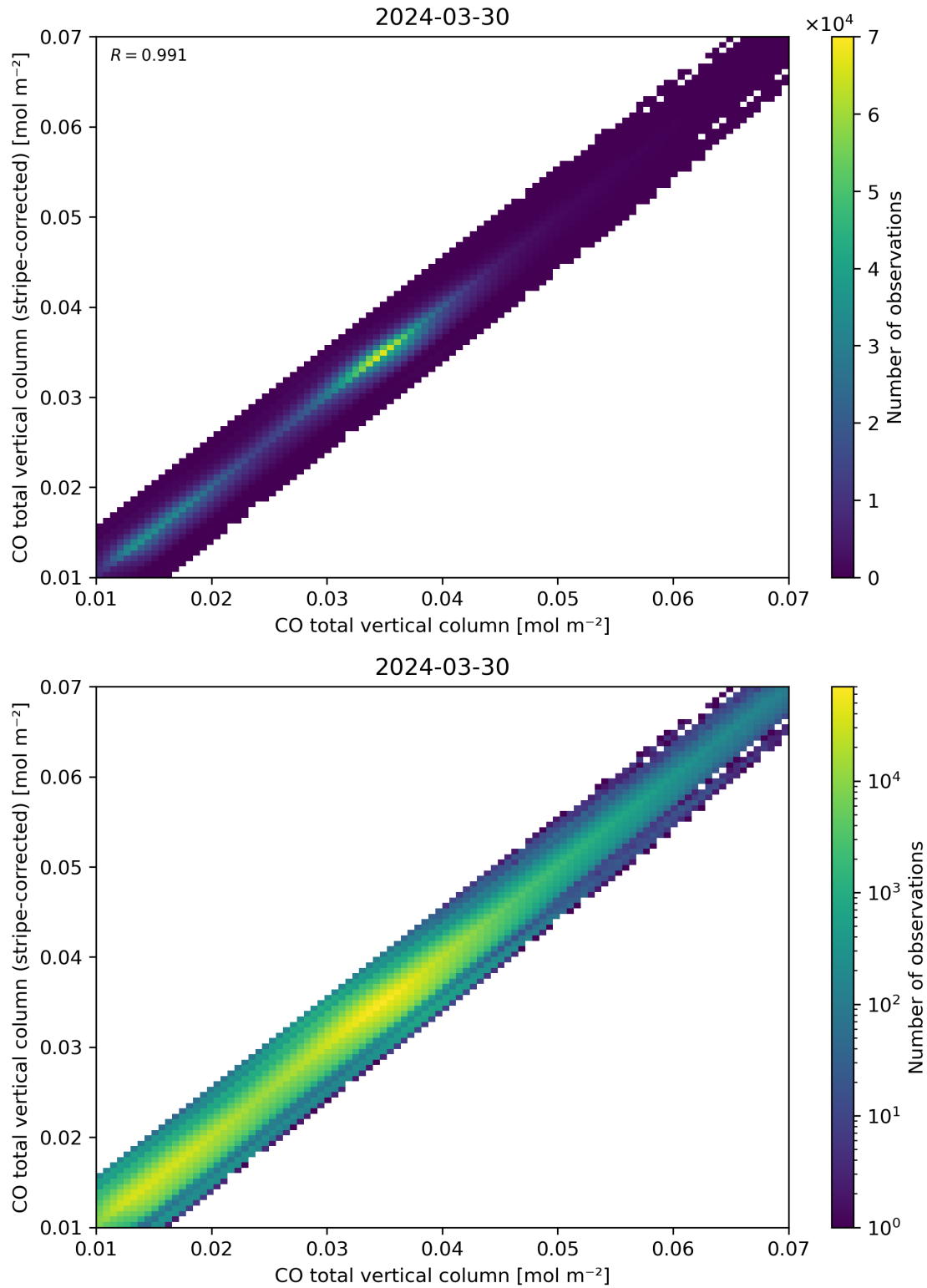
Figure 33: Scatter density plot of “CO total vertical column” against “CO total vertical column (stripe-corrected)” for 2024-03-30 to 2024-03-31.
