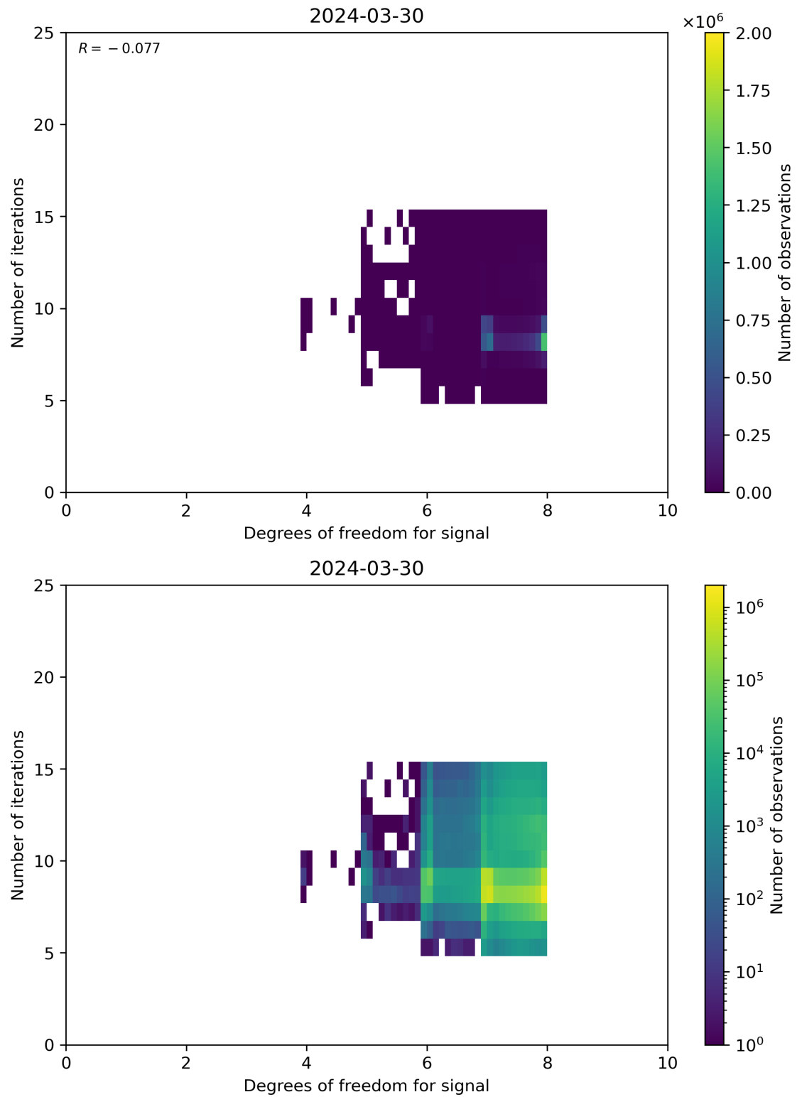
Figure 50: Scatter density plot of “Degrees of freedom for signal” against “Number of iterations” for 2024-03-30 to 2024-03-31.
