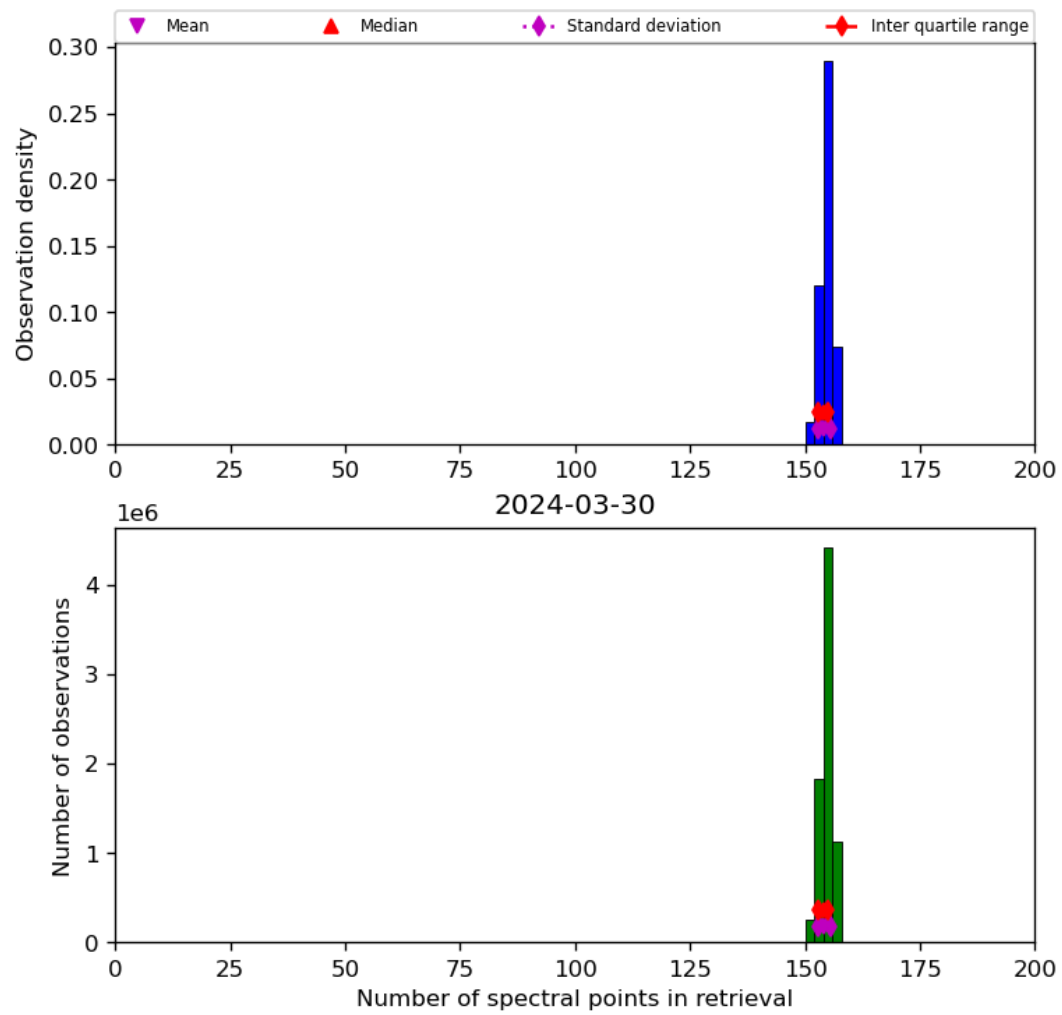
Figure 21: Histogram of “Number of spectral points in retrieval” for 2024-03-30 to 2024-03-31
