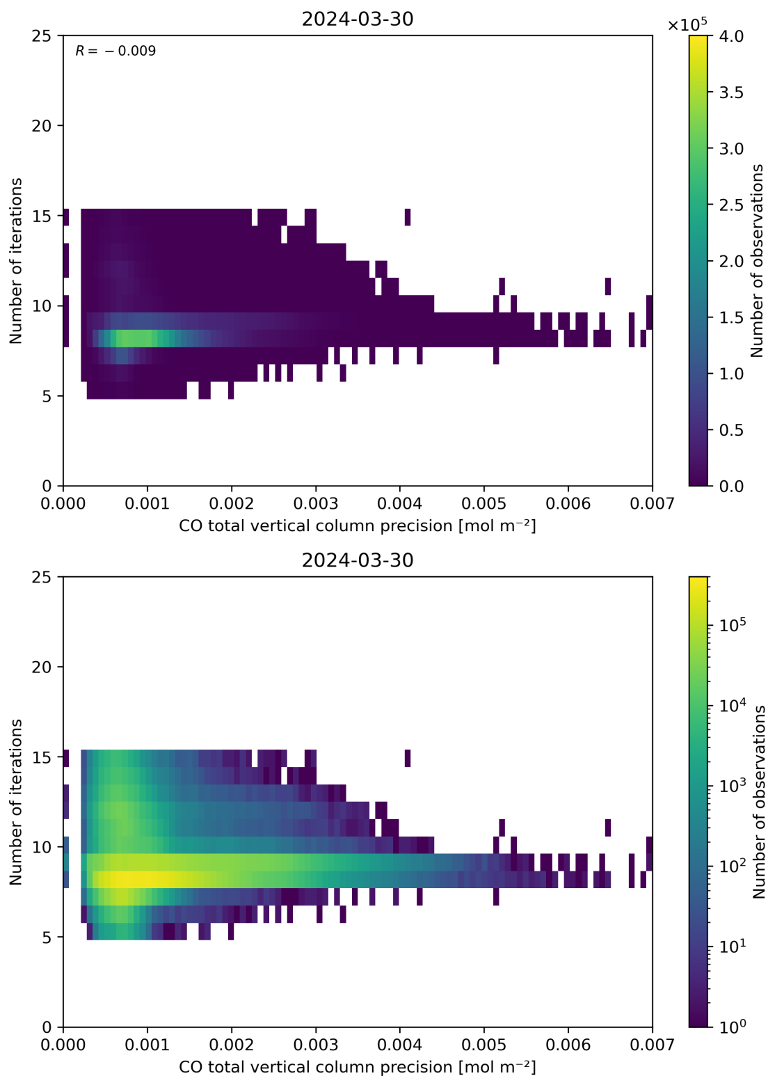
Figure 46: Scatter density plot of “CO total vertical column precision” against “Number of iterations” for 2024-03-30 to 2024-03-31.
