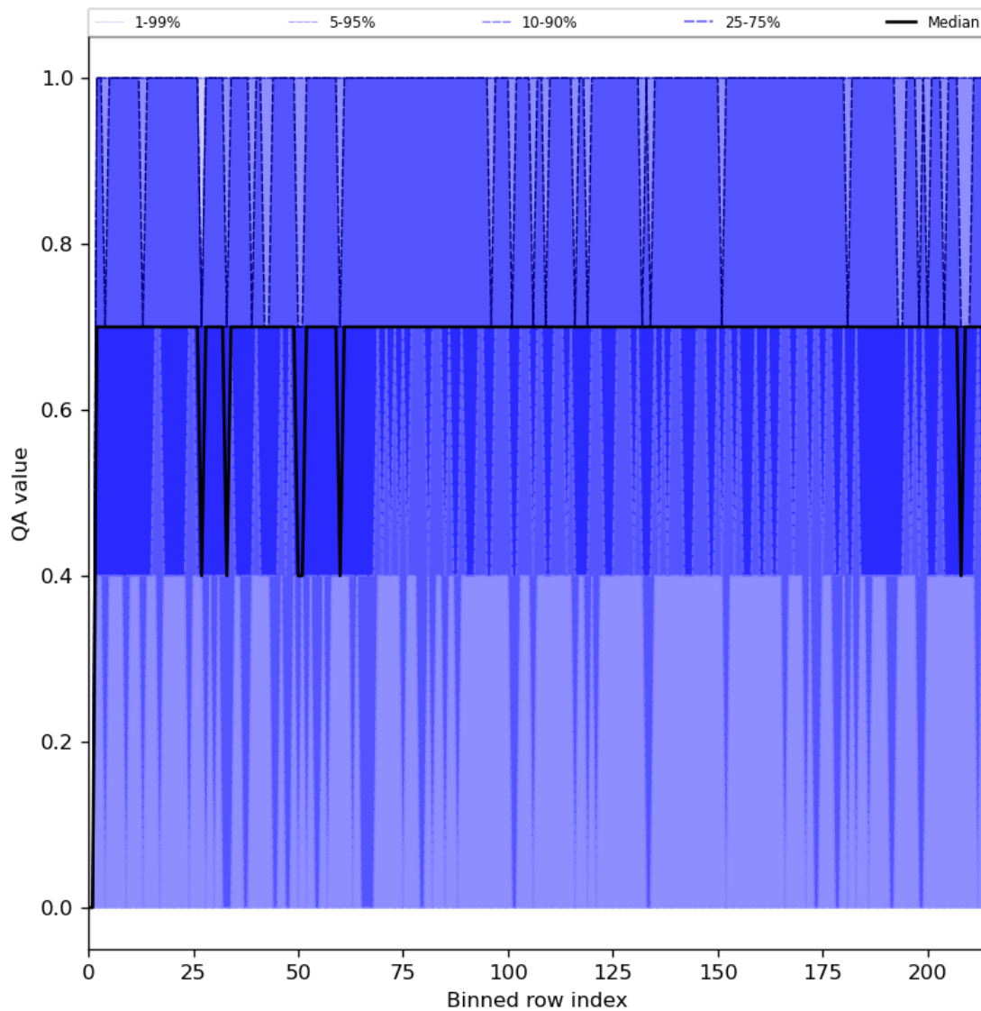
Figure 25: Along track statistics of “QA value” for 2024-03-30 to 2024-03-31
