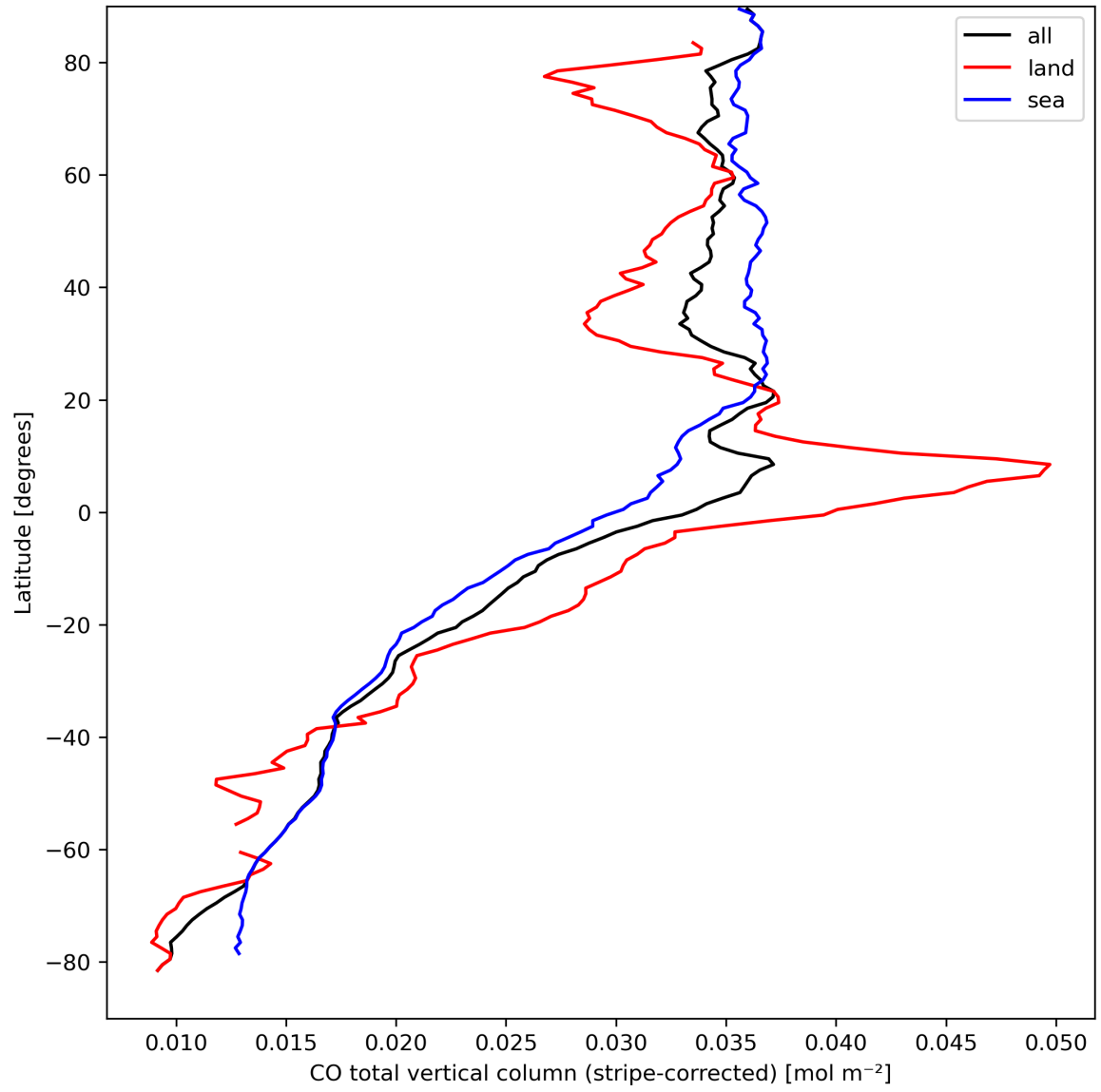
Figure 11: Zonal average of “CO total vertical column (stripe-corrected)” for 2024-03-30 to 2024-03-31.
