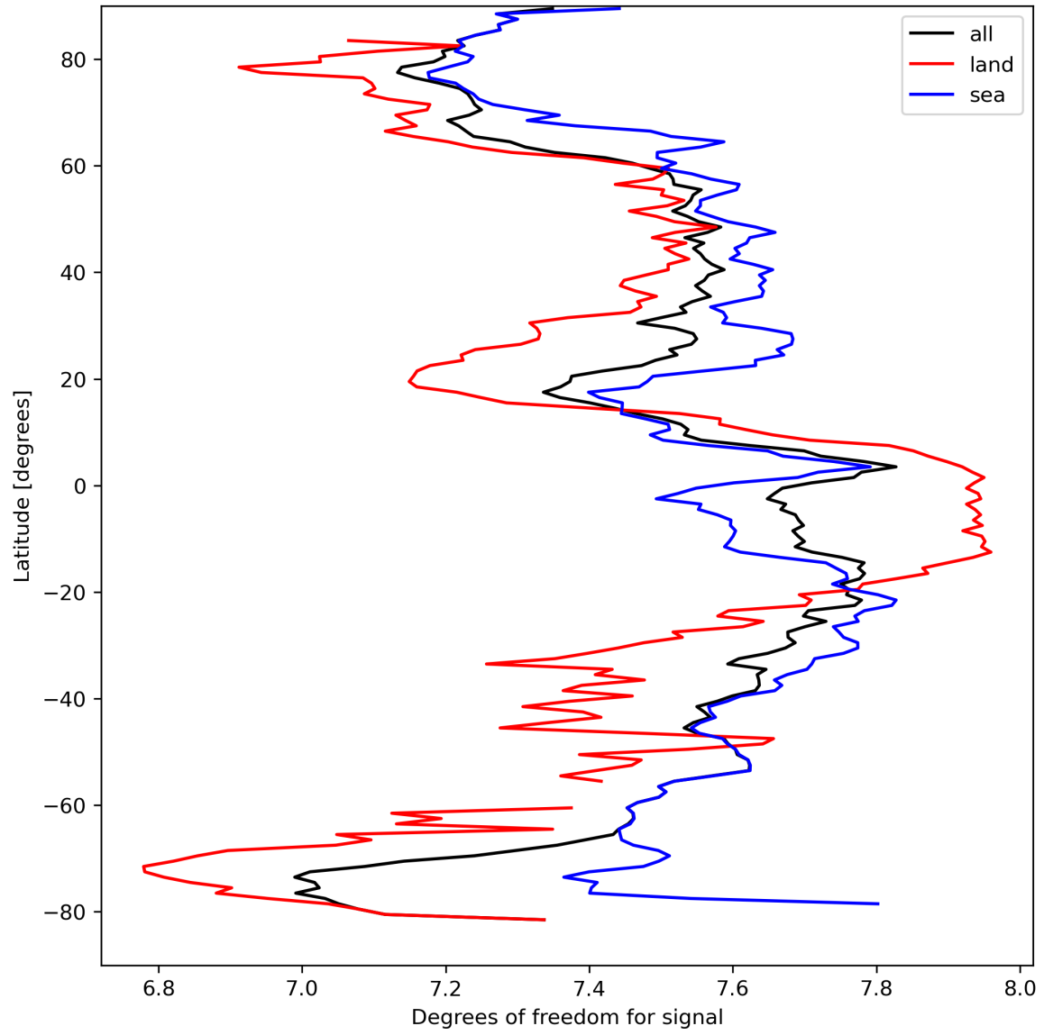
Figure 15: Zonal average of “Degrees of freedom for signal” for 2024-03-30 to 2024-03-31.
