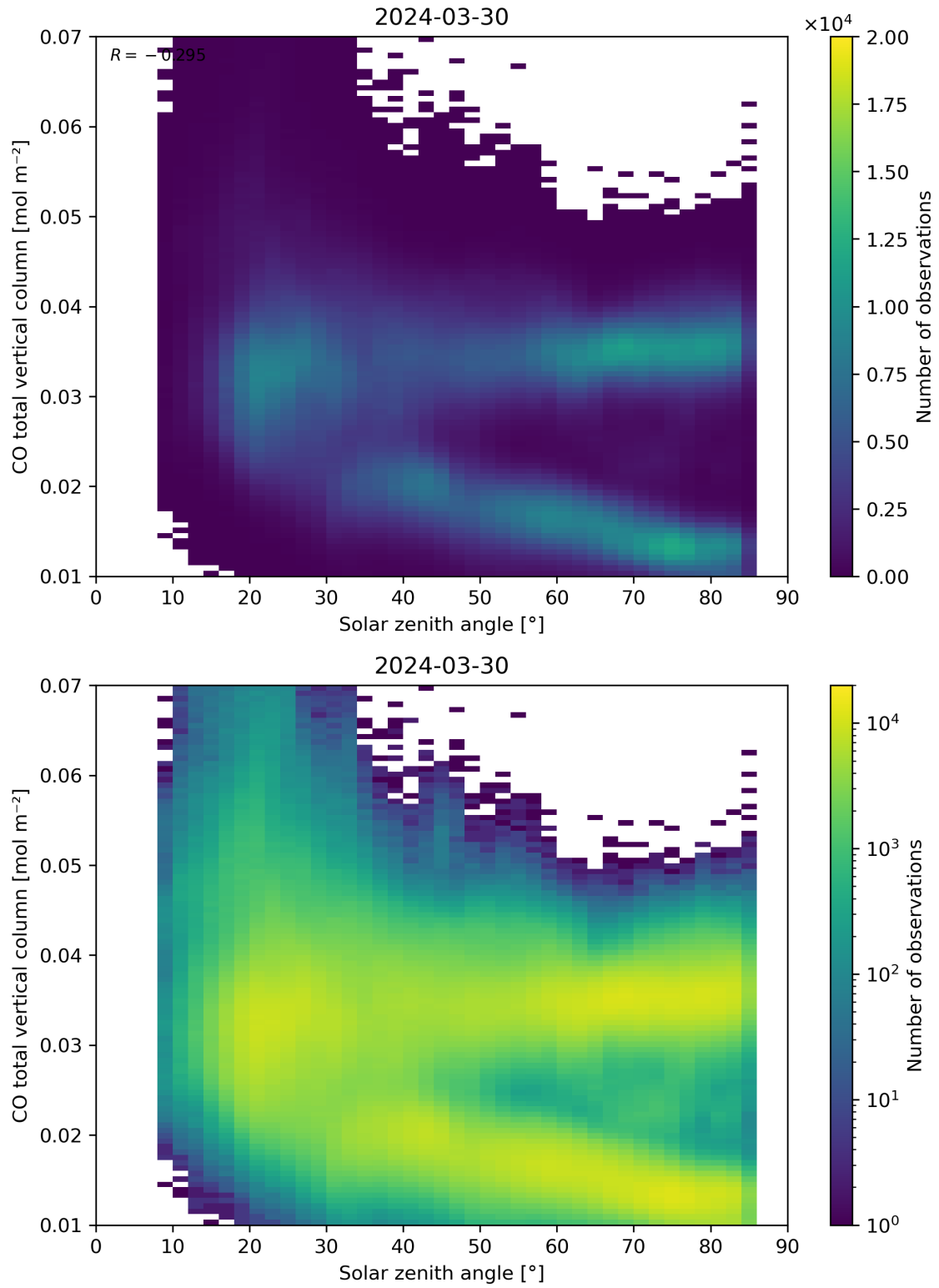
Figure 61: Scatter density plot of “Solar zenith angle” against “CO total vertical column” for 2024-03-30 to 2024-03-31.
