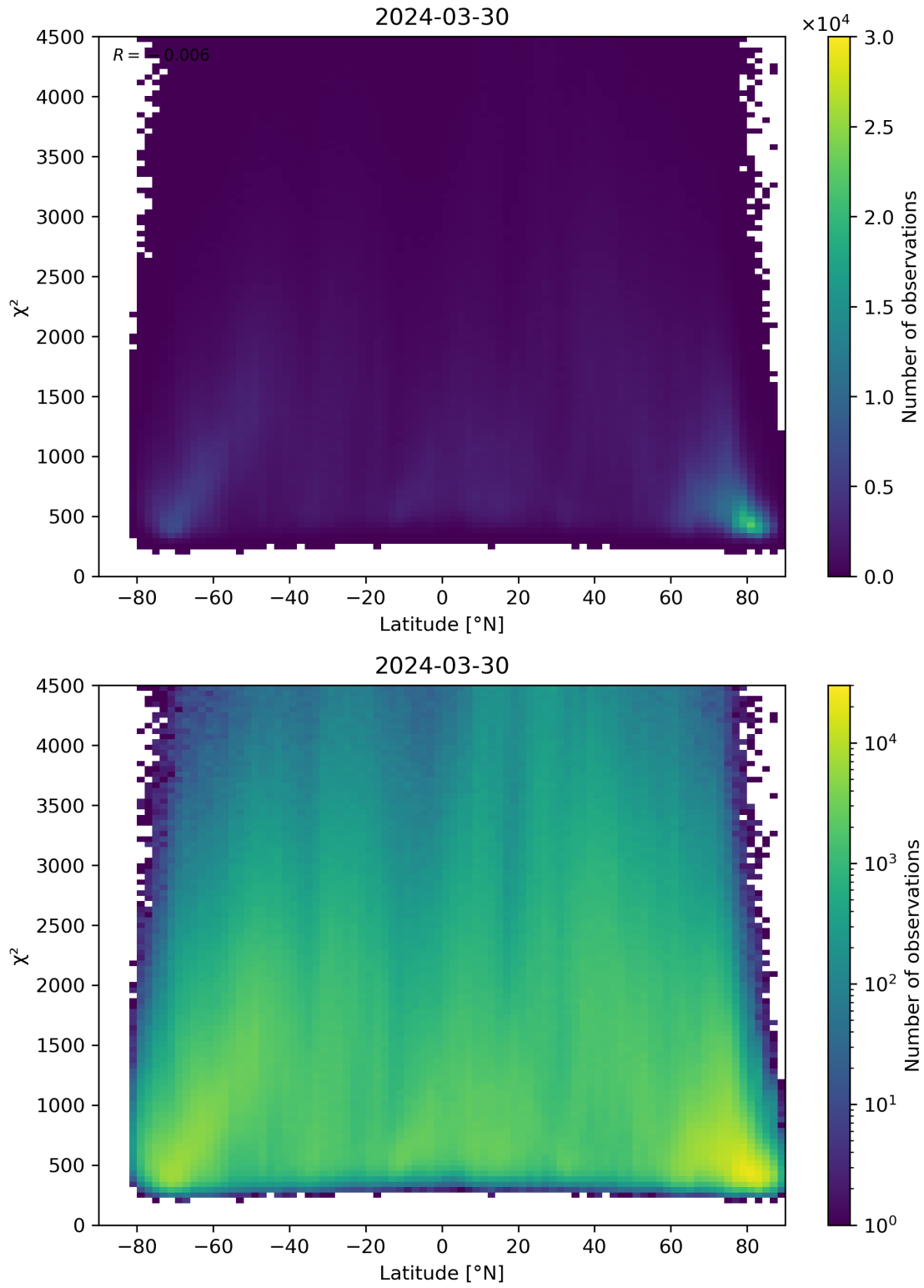
Figure 54: Scatter density plot of “Latitude” against “ \chi^2 ” for 2024-03-30 to 2024-03-31.
