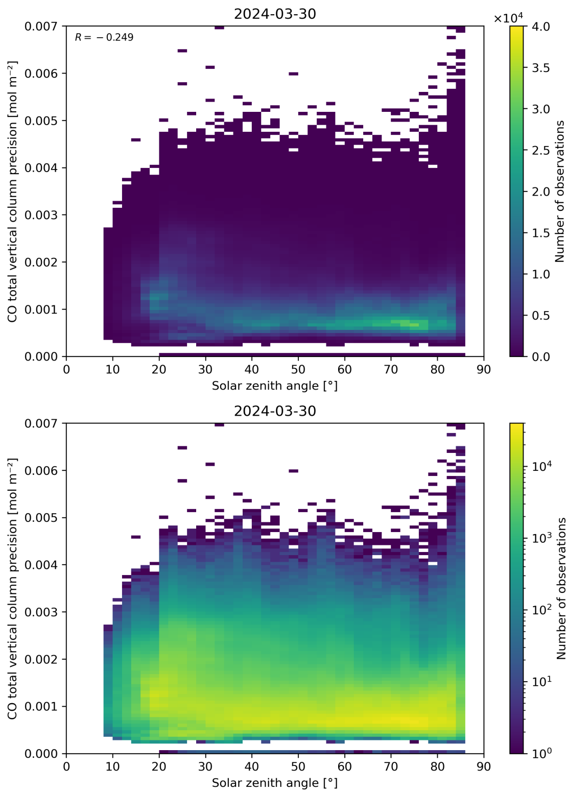
Figure 63: Scatter density plot of “Solar zenith angle” against “CO total vertical column precision” for 2024-03-30 to 2024-03-31.
