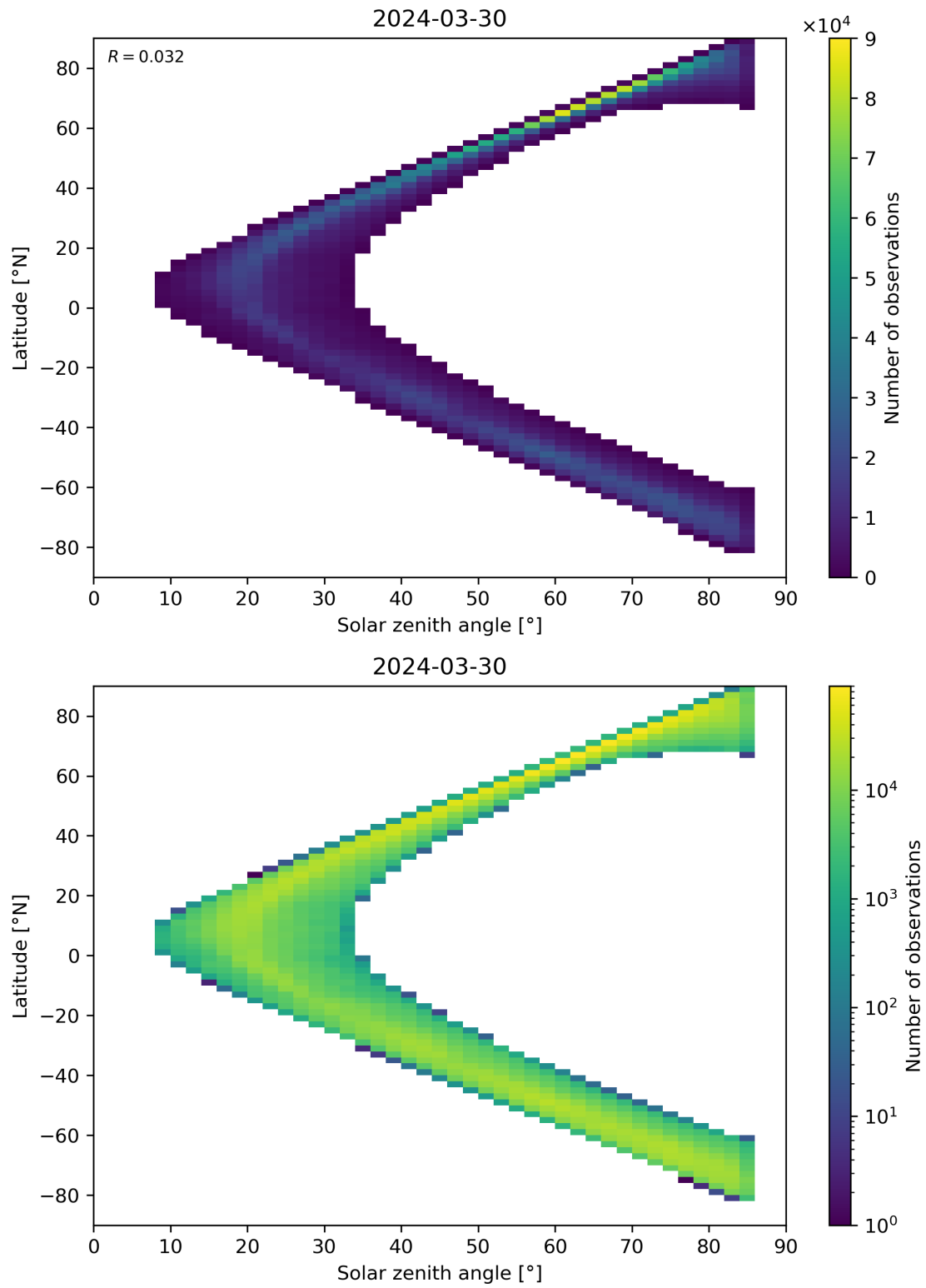
Figure 66: Scatter density plot of “Solar zenith angle” against “Latitude” for 2024-03-30 to 2024-03-31.
