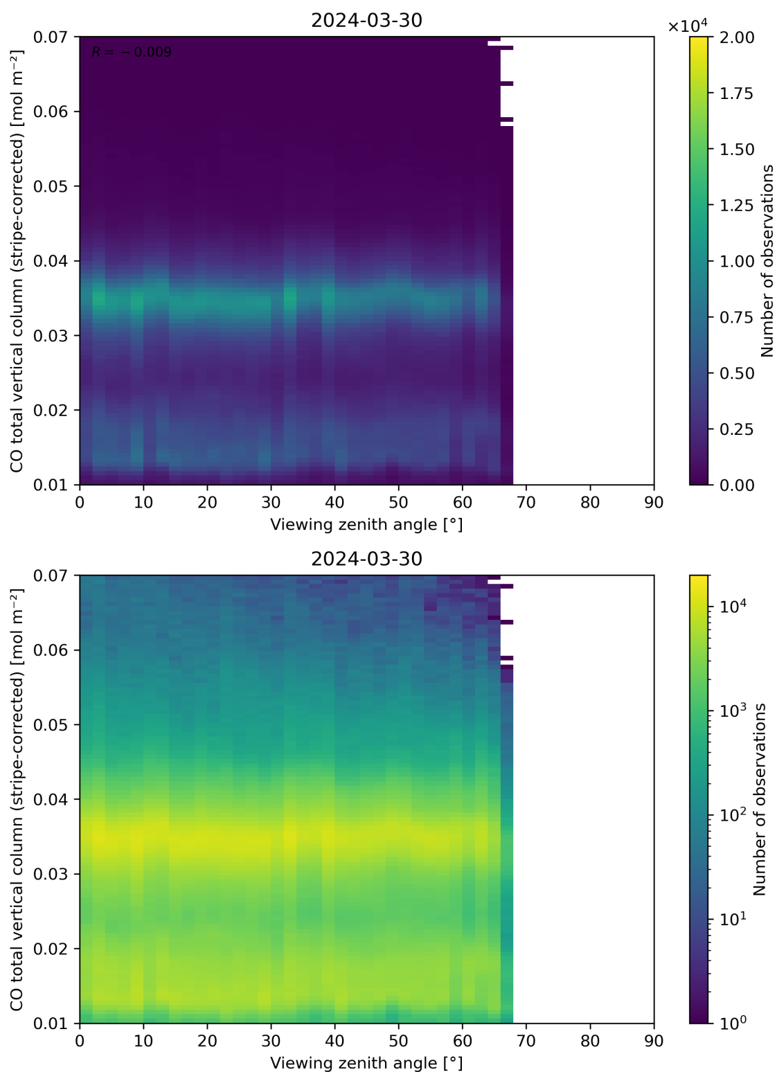
Figure 70: Scatter density plot of “Viewing zenith angle” against “CO total vertical column (stripe-corrected)” for 2024-03-30 to 2024-03-31.
