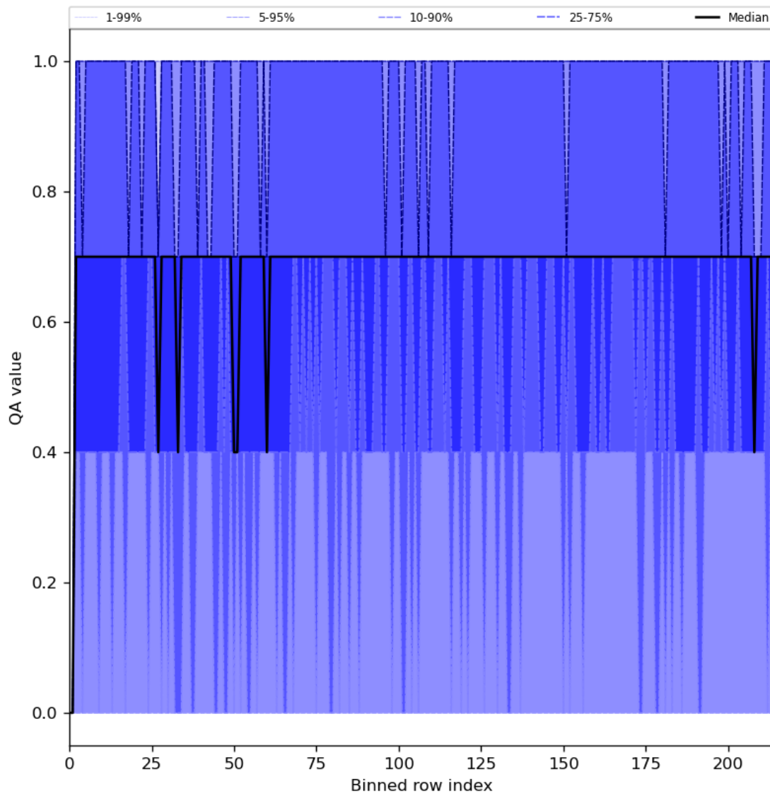
Figure 25: Along track statistics of “QA value” for 2024-03-31 to 2024-04-01
