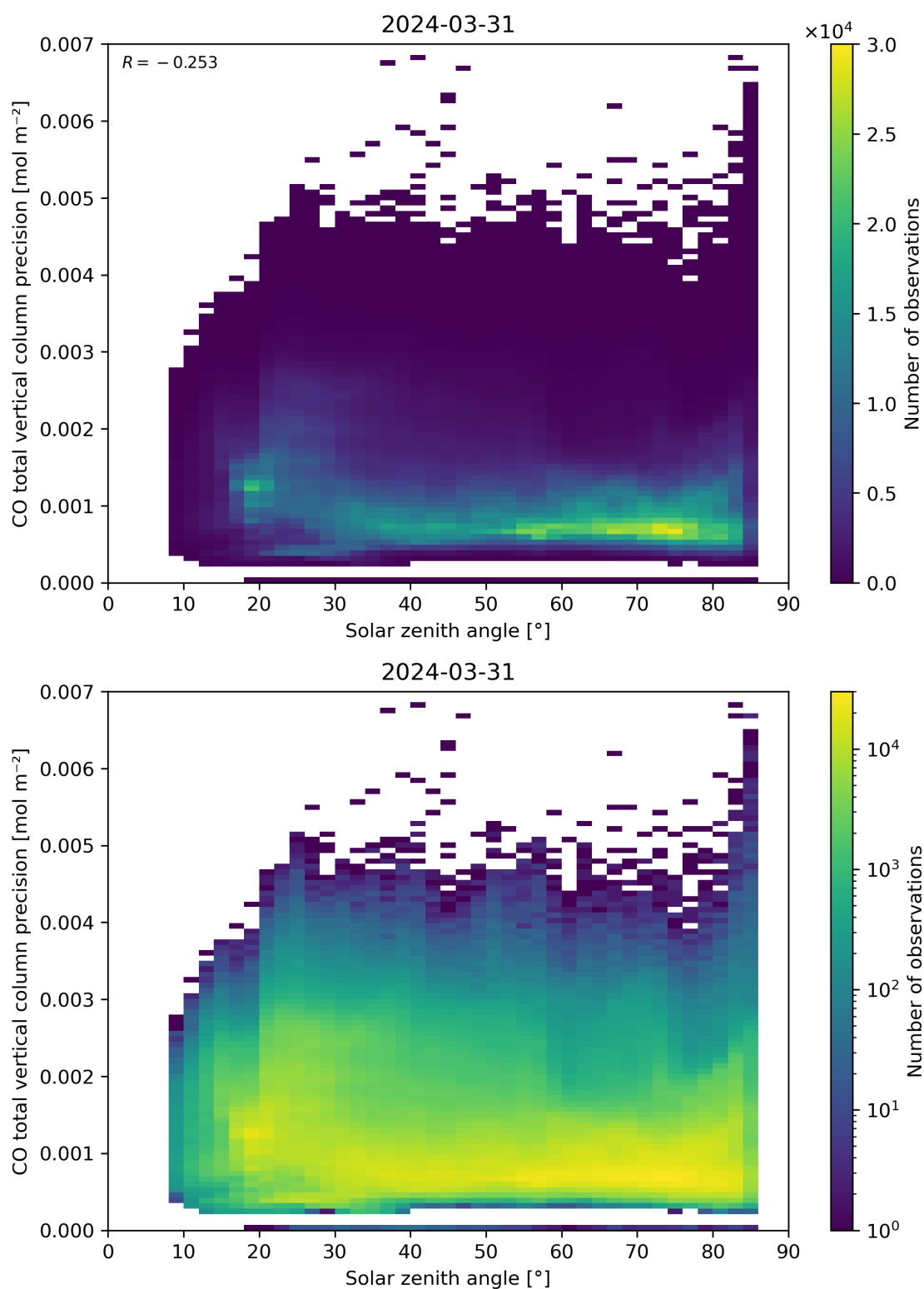
Figure 63: Scatter density plot of “Solar zenith angle” against “CO total vertical column precision” for 2024-03-31 to 2024-04-01.
