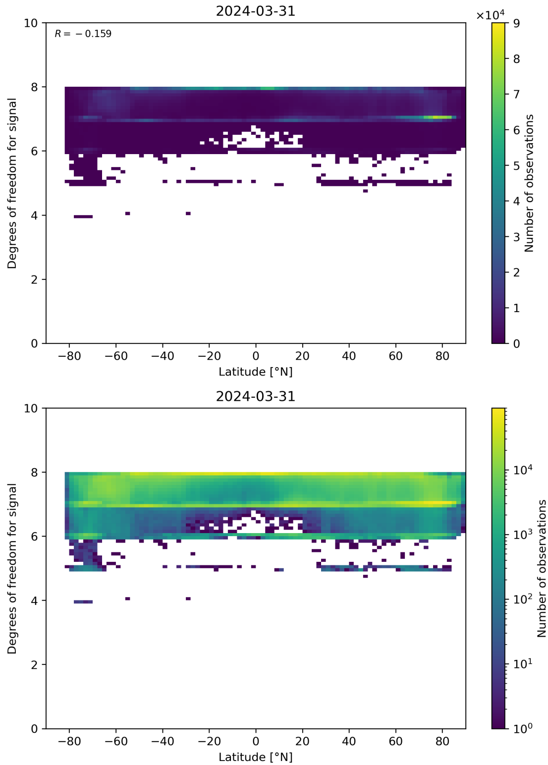
Figure 55: Scatter density plot of “Latitude” against “Degrees of freedom for signal” for 2024-03-31 to 2024-04-01.
