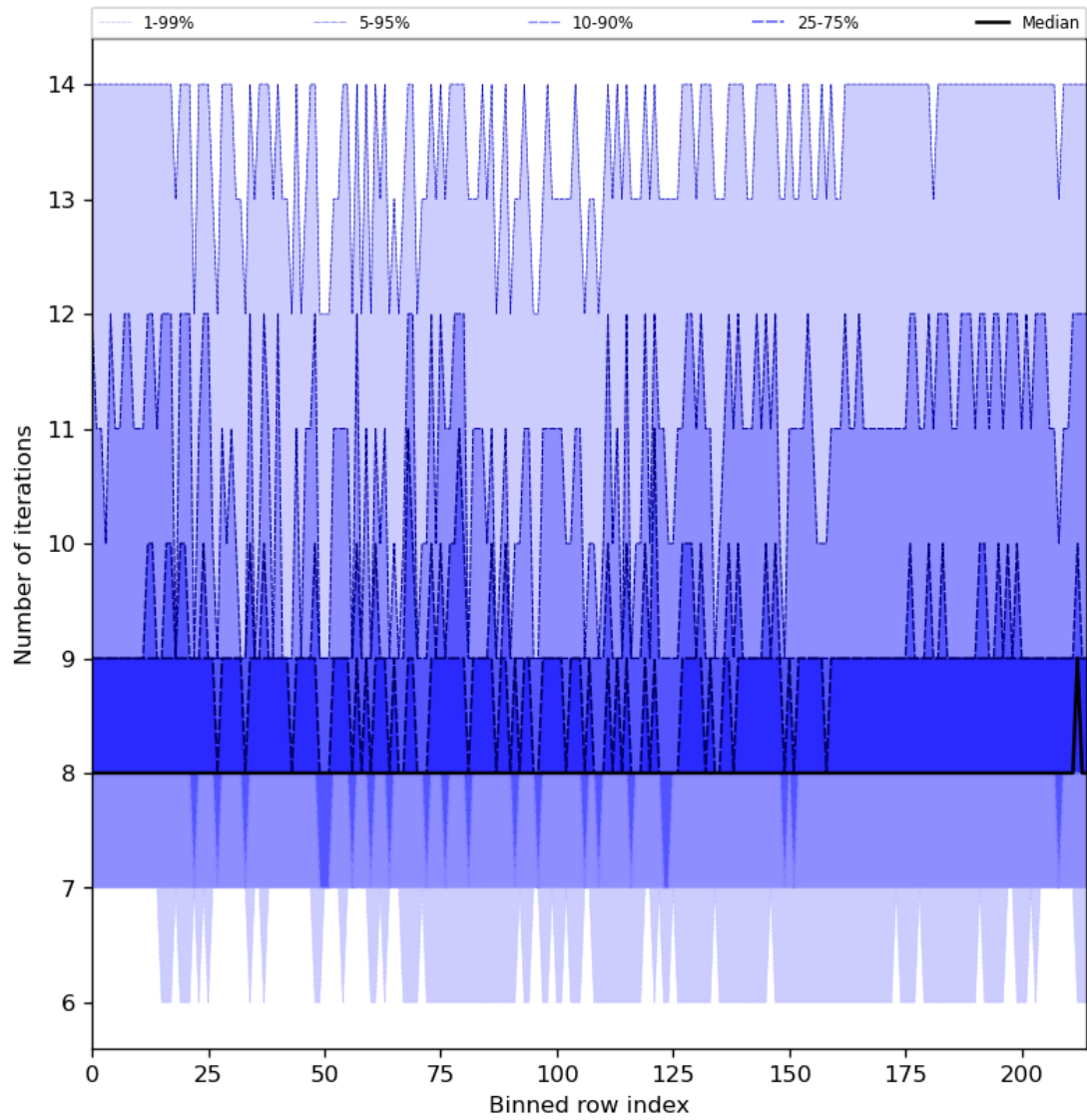
Figure 32: Along track statistics of “Number of iterations” for 2024-03-31 to 2024-04-01
