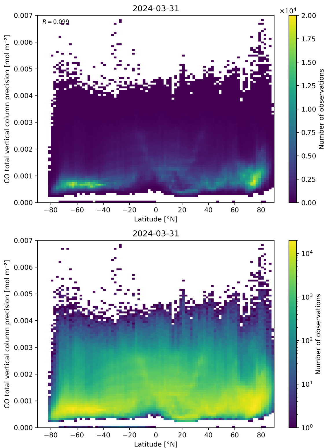
Figure 53: Scatter density plot of “Latitude” against “CO total vertical column precision” for 2024-03-31 to 2024-04-01.
