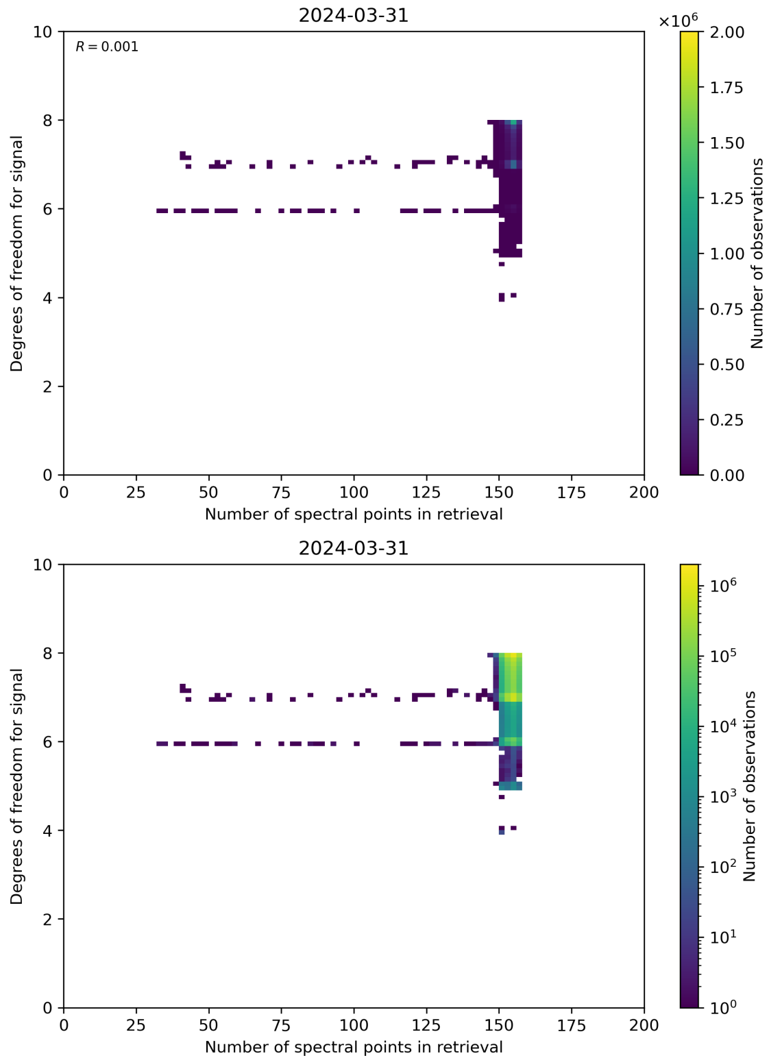
Figure 59: Scatter density plot of “Number of spectral points in retrieval” against “Degrees of freedom for signal” for 2024-03-31 to 2024-04-01.
