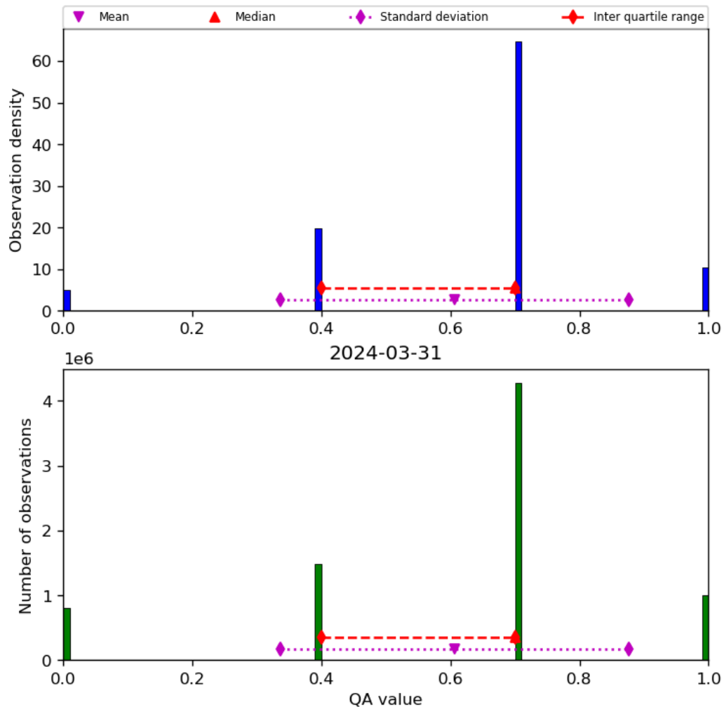
Figure 17: Histogram of “QA value” for 2024-03-31 to 2024-04-01
