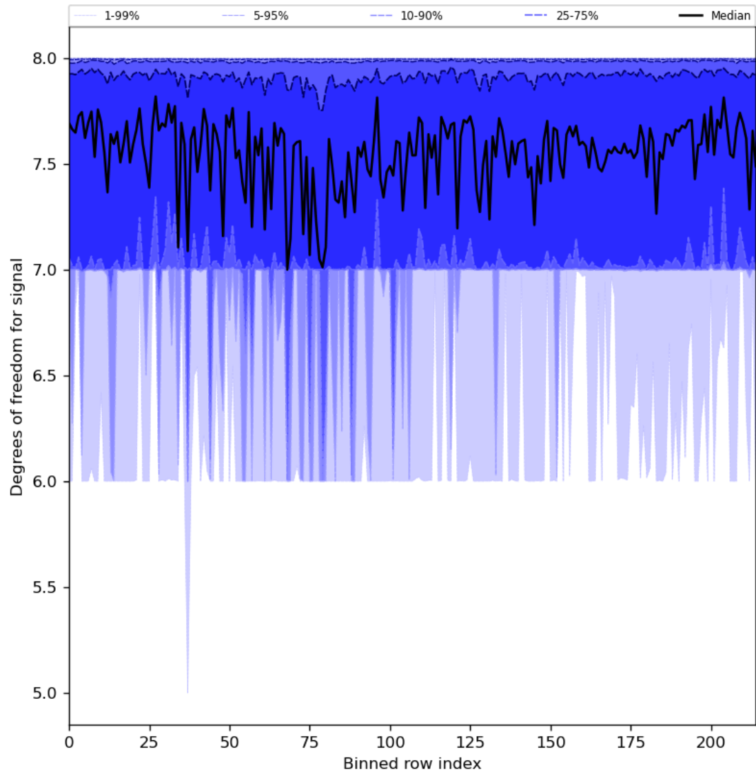
Figure 31: Along track statistics of “Degrees of freedom for signal” for 2024-03-31 to 2024-04-01
