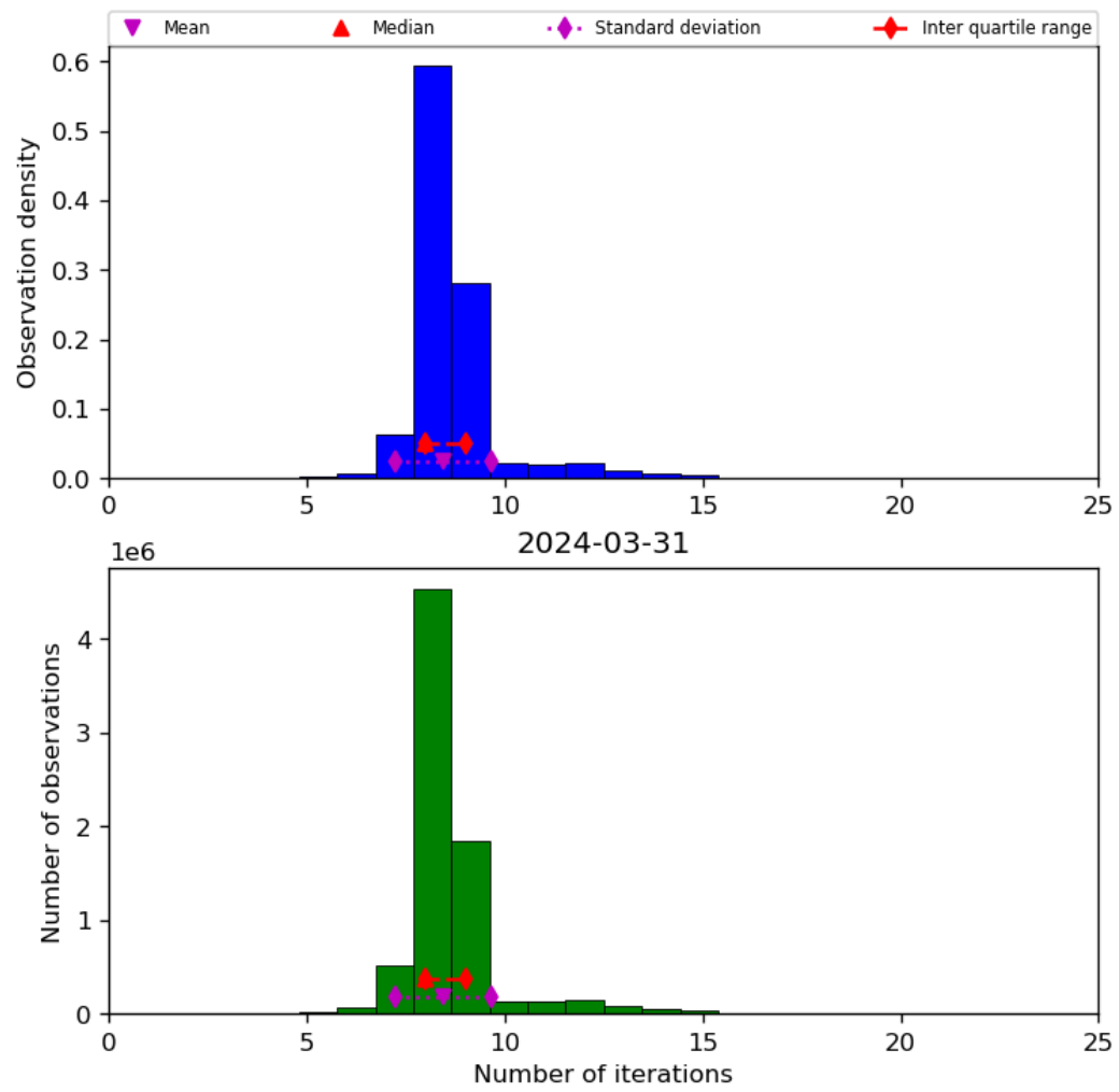
Figure 24: Histogram of “Number of iterations” for 2024-03-31 to 2024-04-01
