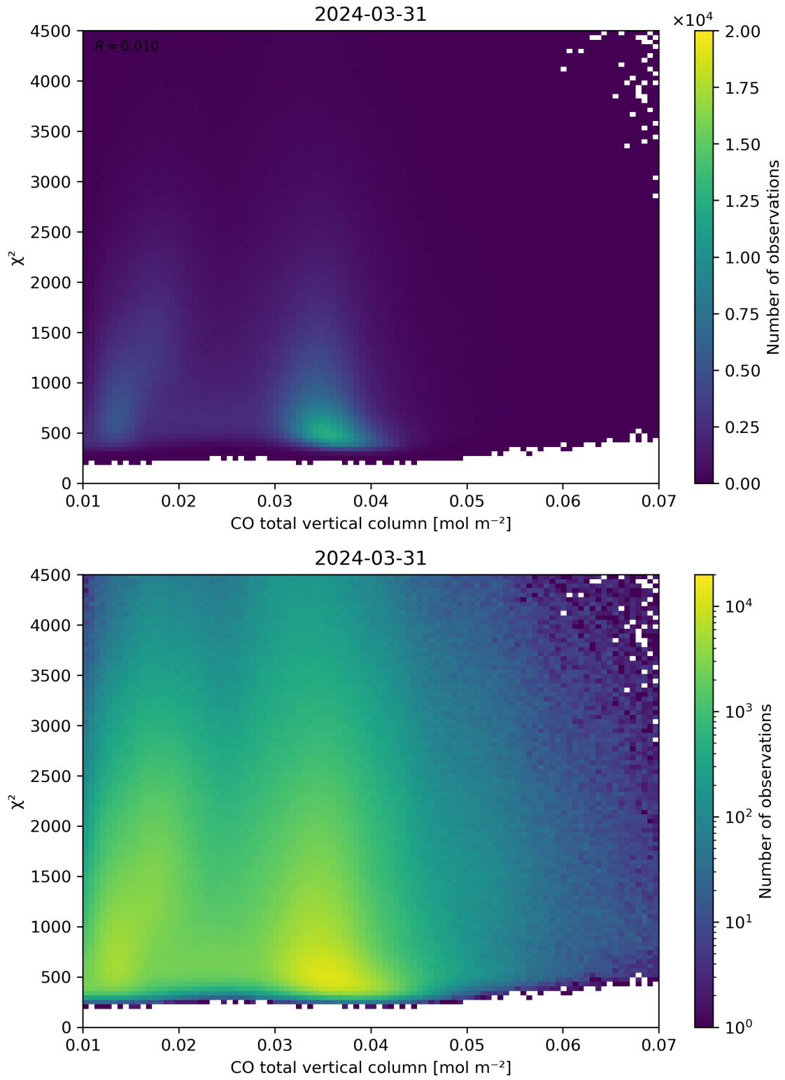
Figure 35: Scatter density plot of “CO total vertical column” against “ \chi^2 ” for 2024-03-31 to 2024-04-01.
