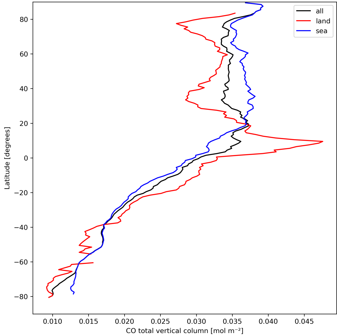
Figure 10: Zonal average of “CO total vertical column” for 2024-03-31 to 2024-04-01.
