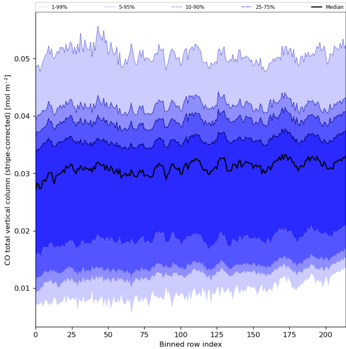
Figure 27: Along track statistics of “CO total vertical column (stripe-corrected)” for 2024-03-31 to 2024-04-01
