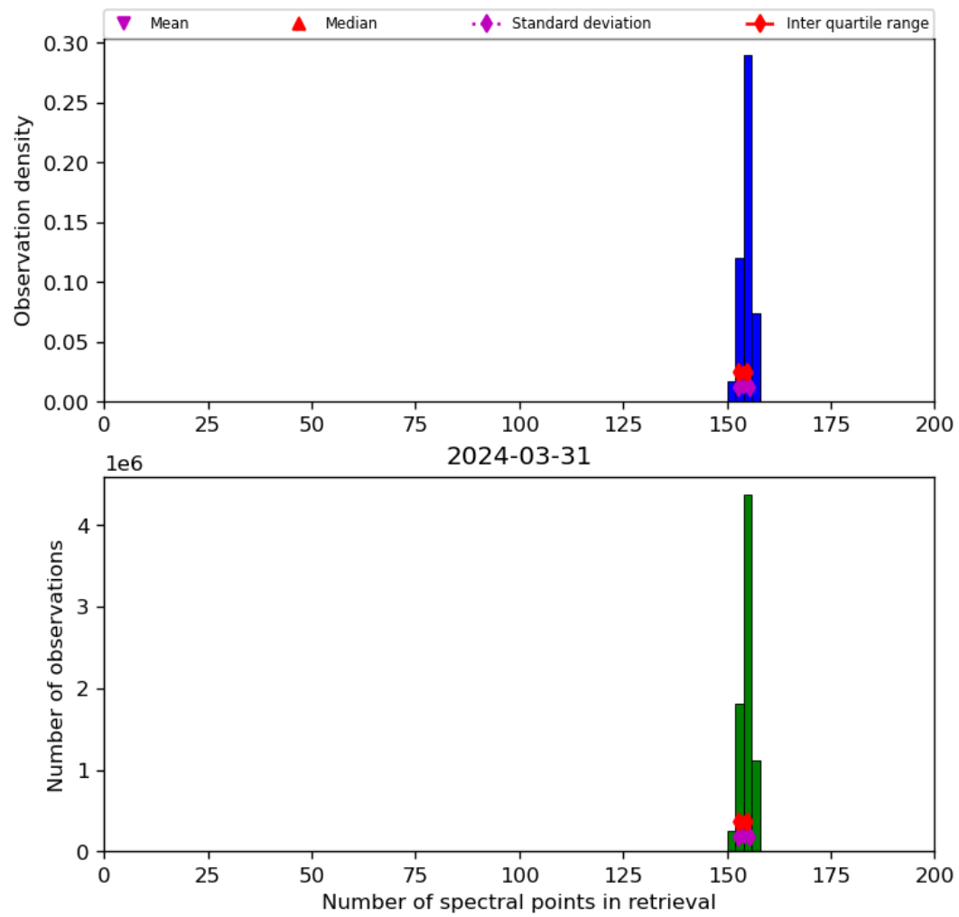
Figure 21: Histogram of “Number of spectral points in retrieval” for 2024-03-31 to 2024-04-01
