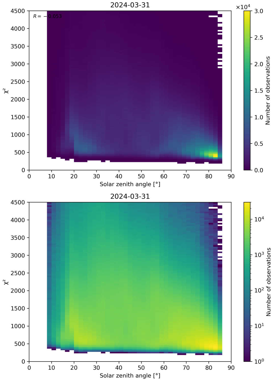
Figure 64: Scatter density plot of “Solar zenith angle” against “ \chi^2 ” for 2024-03-31 to 2024-04-01.
