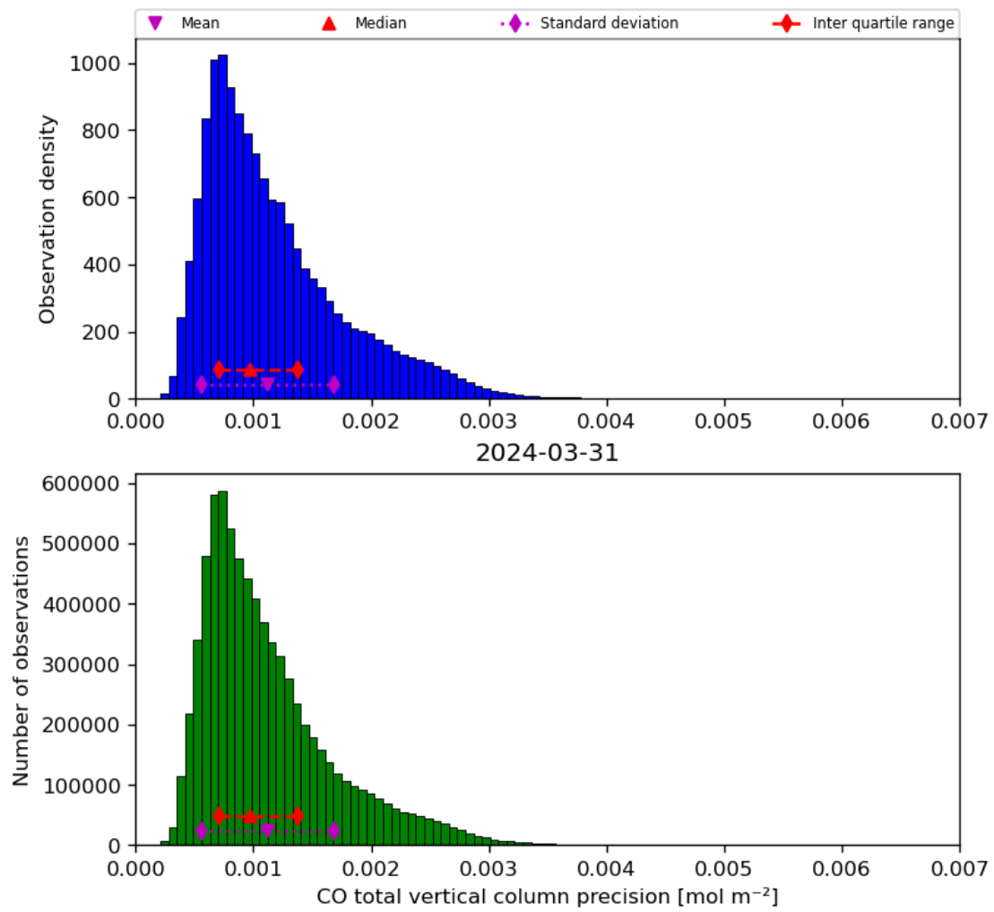
Figure 20: Histogram of “CO total vertical column precision” for 2024-03-31 to 2024-04-01
