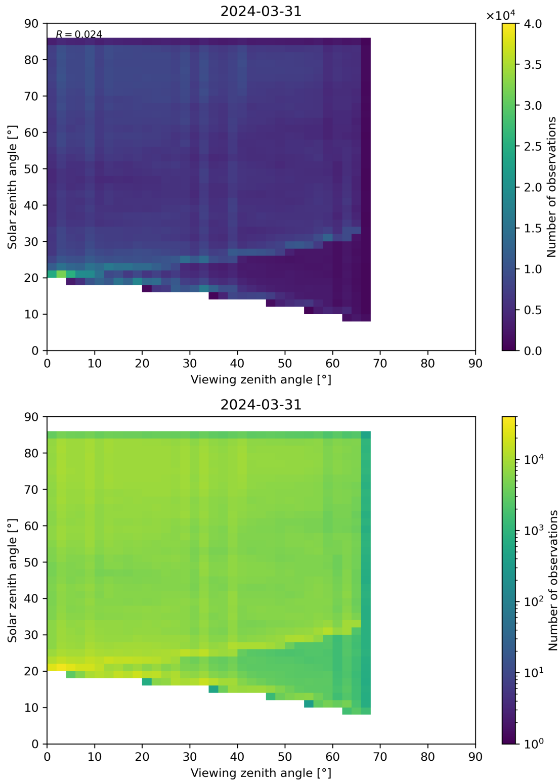
Figure 77: Scatter density plot of “Viewing zenith angle” against “Solar zenith angle” for 2024-03-31 to 2024-04-01.
