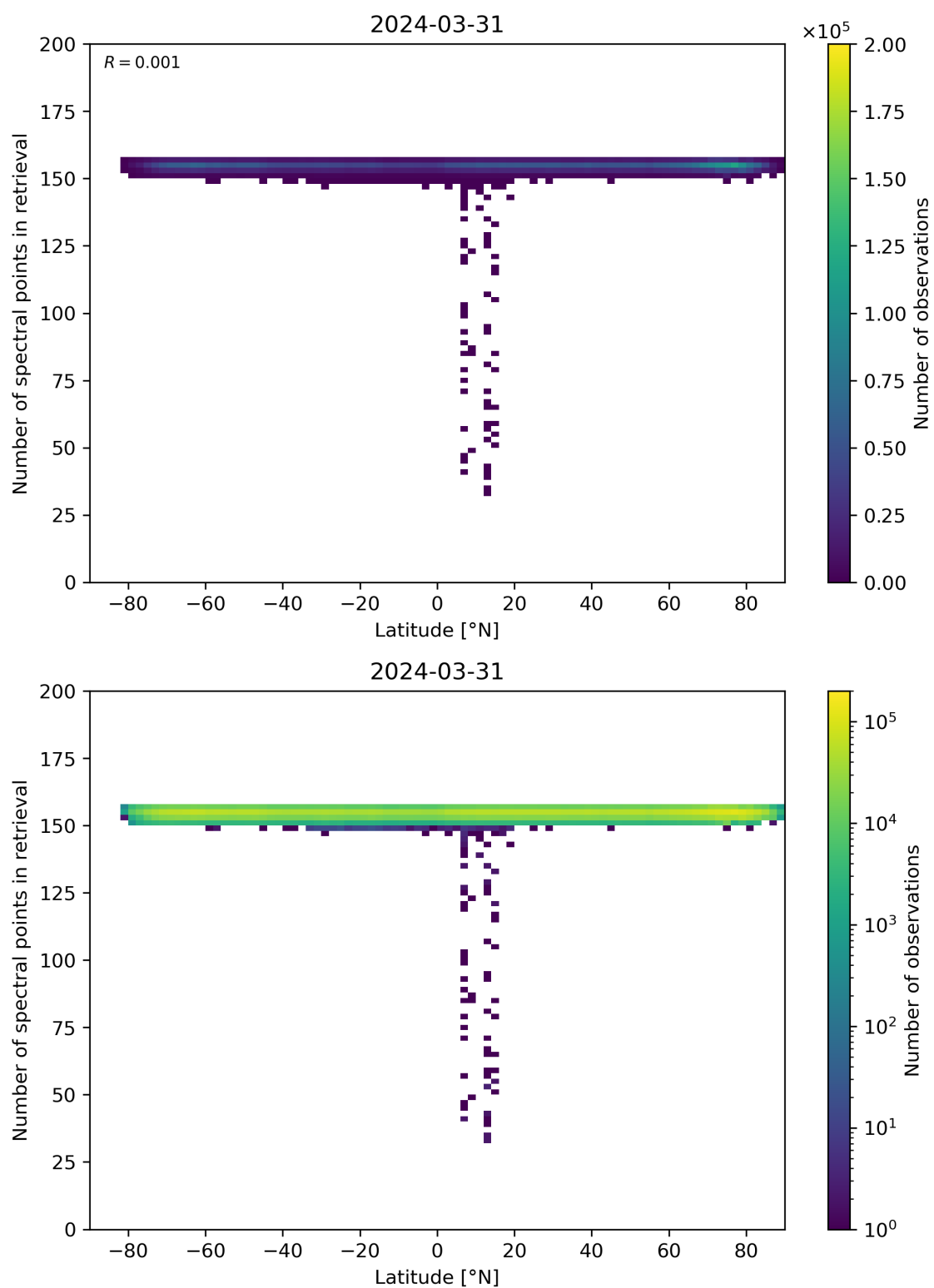
Figure 57: Scatter density plot of “Latitude” against “Number of spectral points in retrieval” for 2024-03-31 to 2024-04-01.
