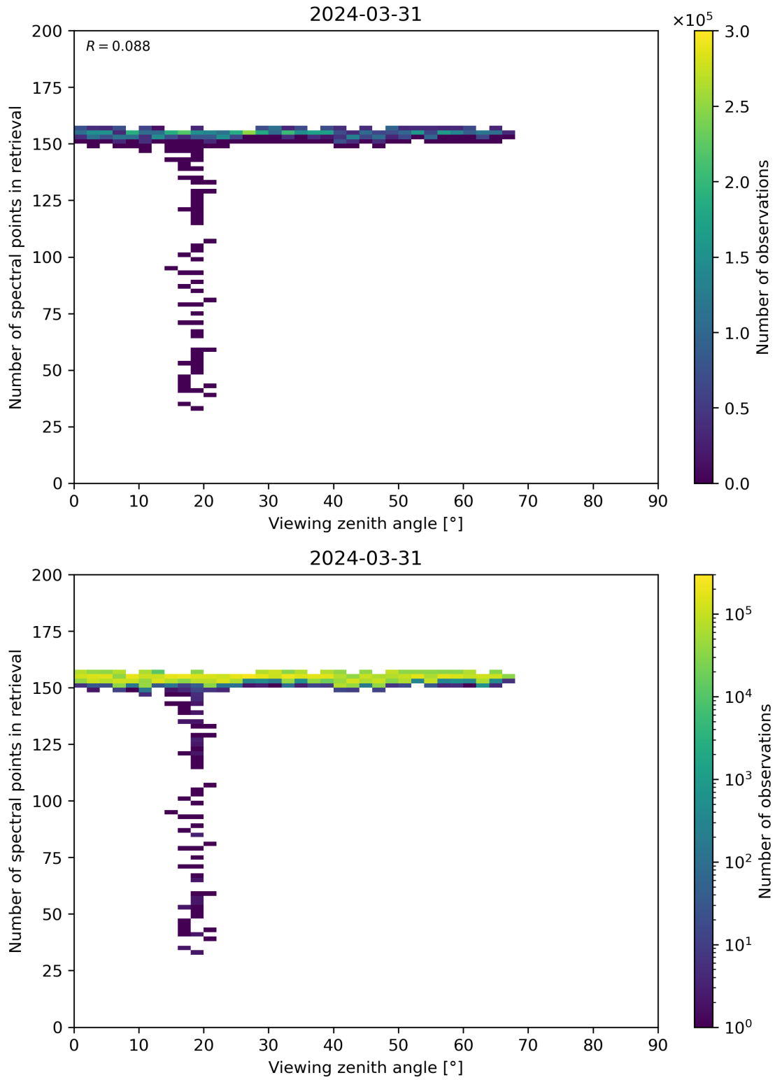
Figure 76: Scatter density plot of “Viewing zenith angle” against “Number of spectral points in retrieval” for 2024-03-31 to 2024-04-01.
