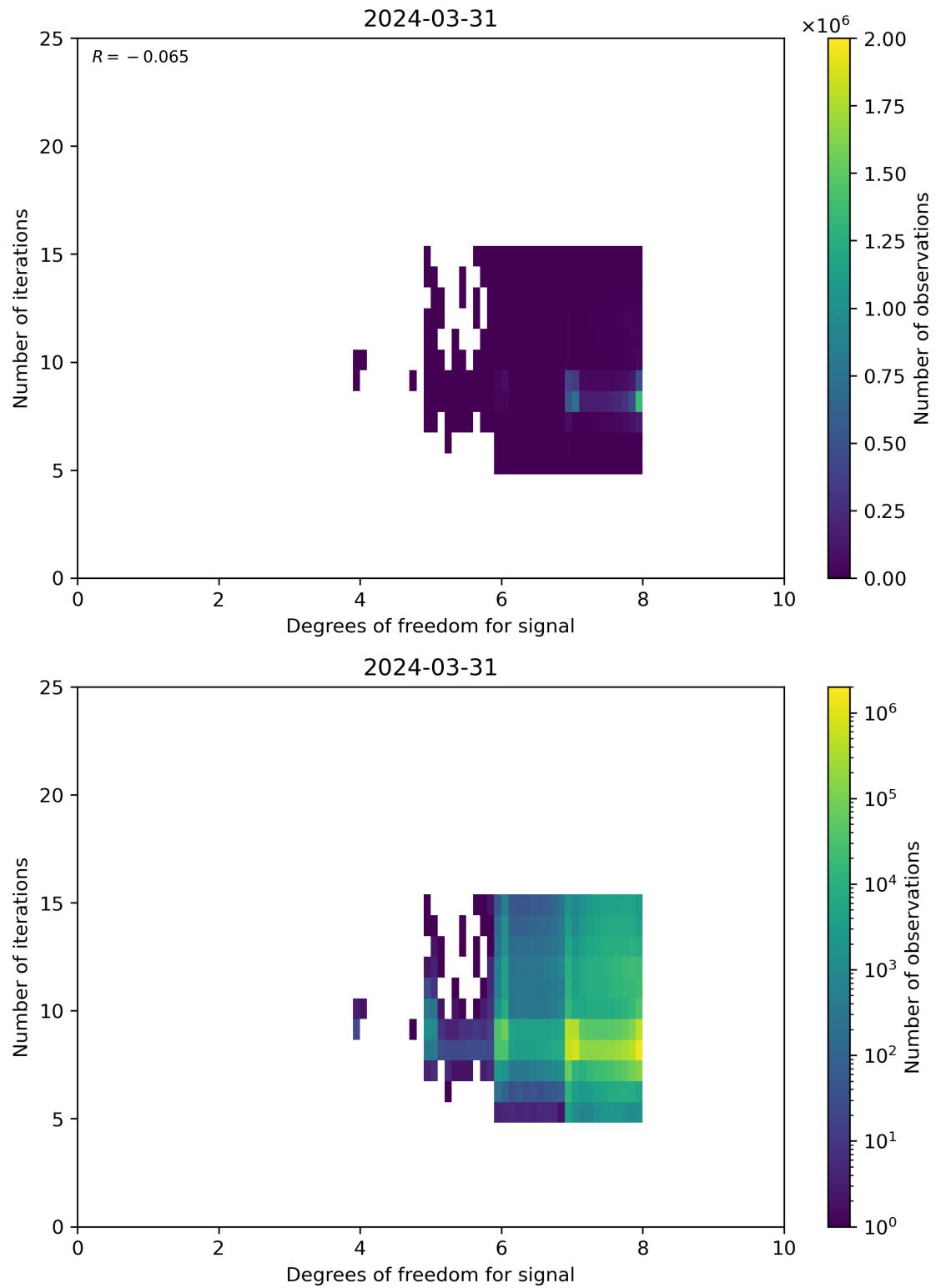
Figure 50: Scatter density plot of “Degrees of freedom for signal” against “Number of iterations” for 2024-03-31 to 2024-04-01.
