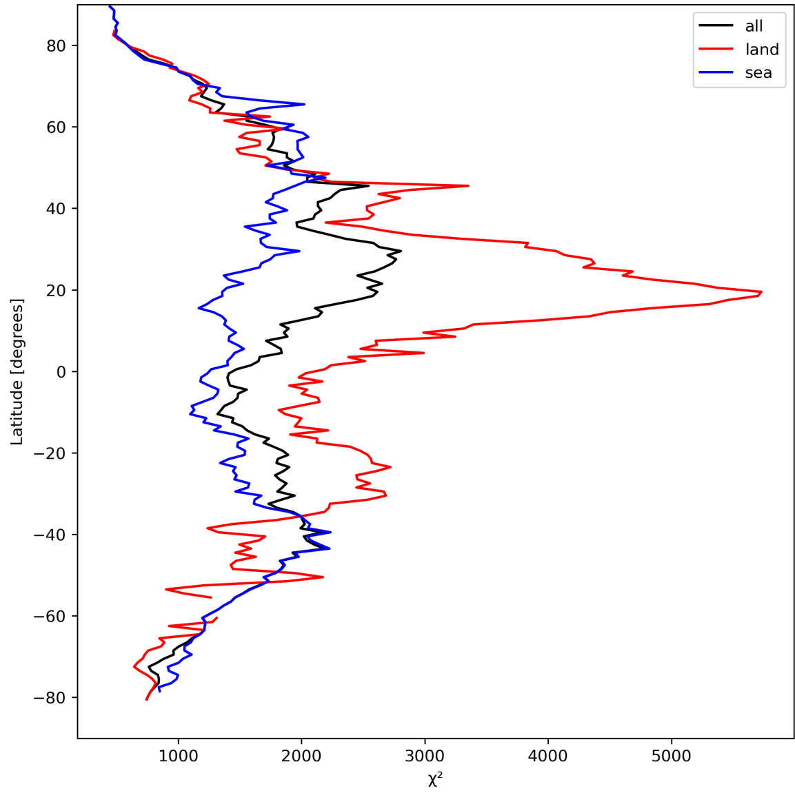
Figure 14: Zonal average of “ \chi^2 ” for 2024-03-31 to 2024-04-01.
