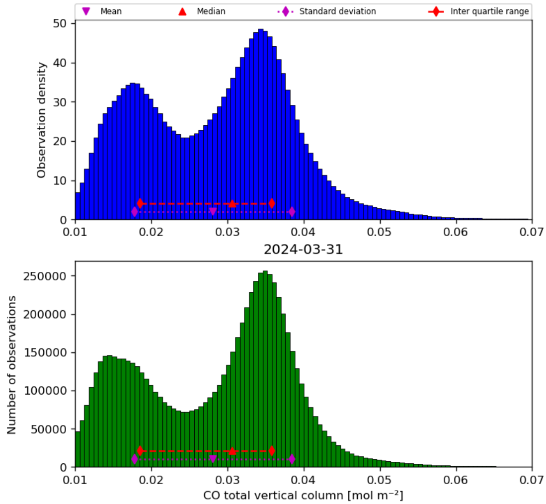
Figure 18: Histogram of “CO total vertical column” for 2024-03-31 to 2024-04-01
