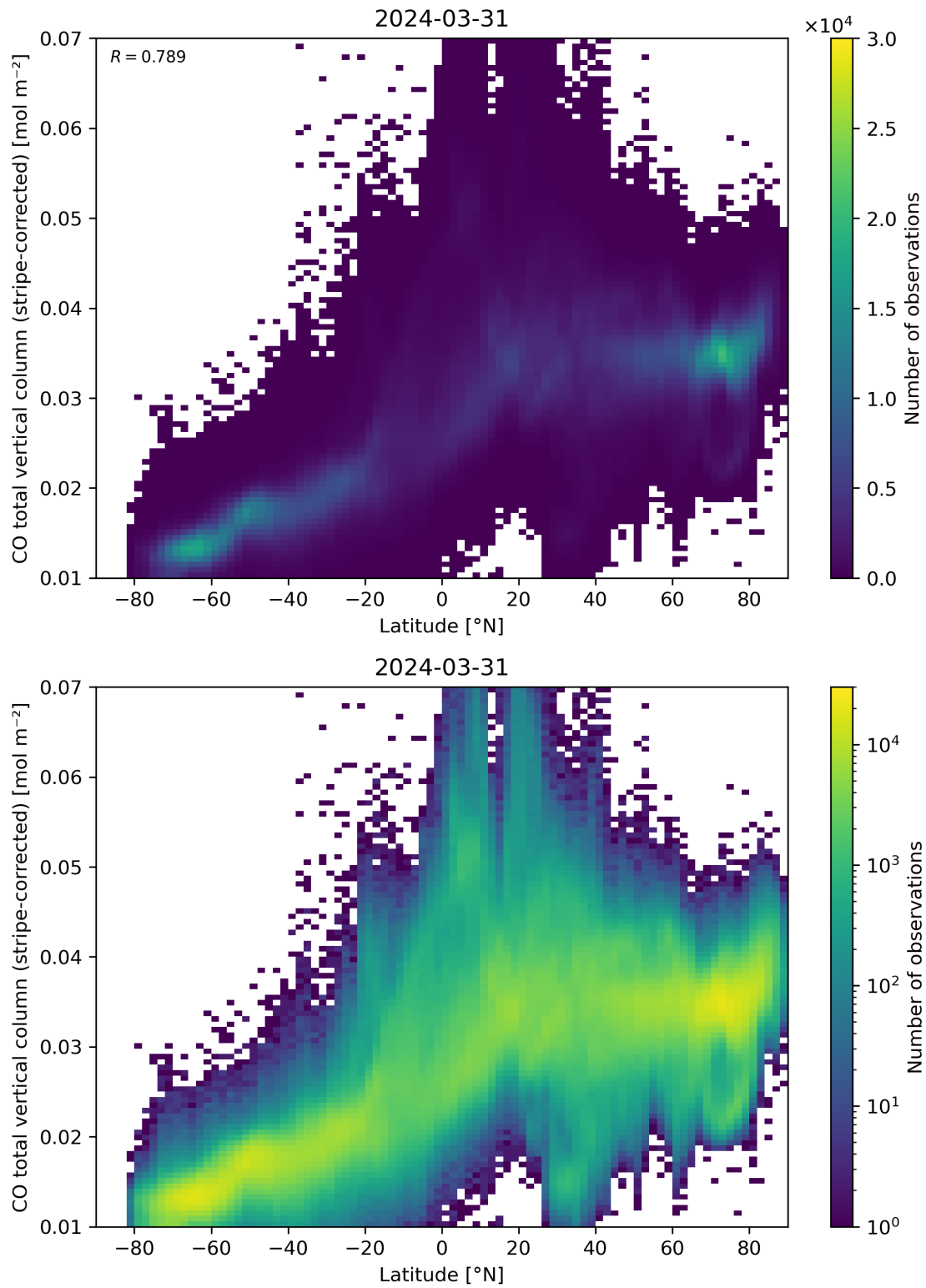
Figure 52: Scatter density plot of “Latitude” against “CO total vertical column (stripe-corrected)” for 2024-03-31 to 2024-04-01.
