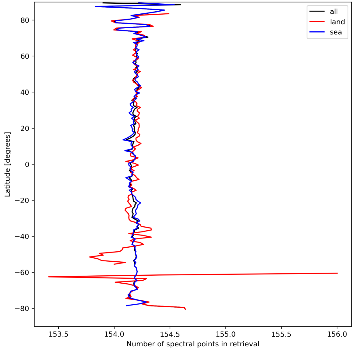
Figure 13: Zonal average of “Number of spectral points in retrieval” for 2024-03-31 to 2024-04-01.
