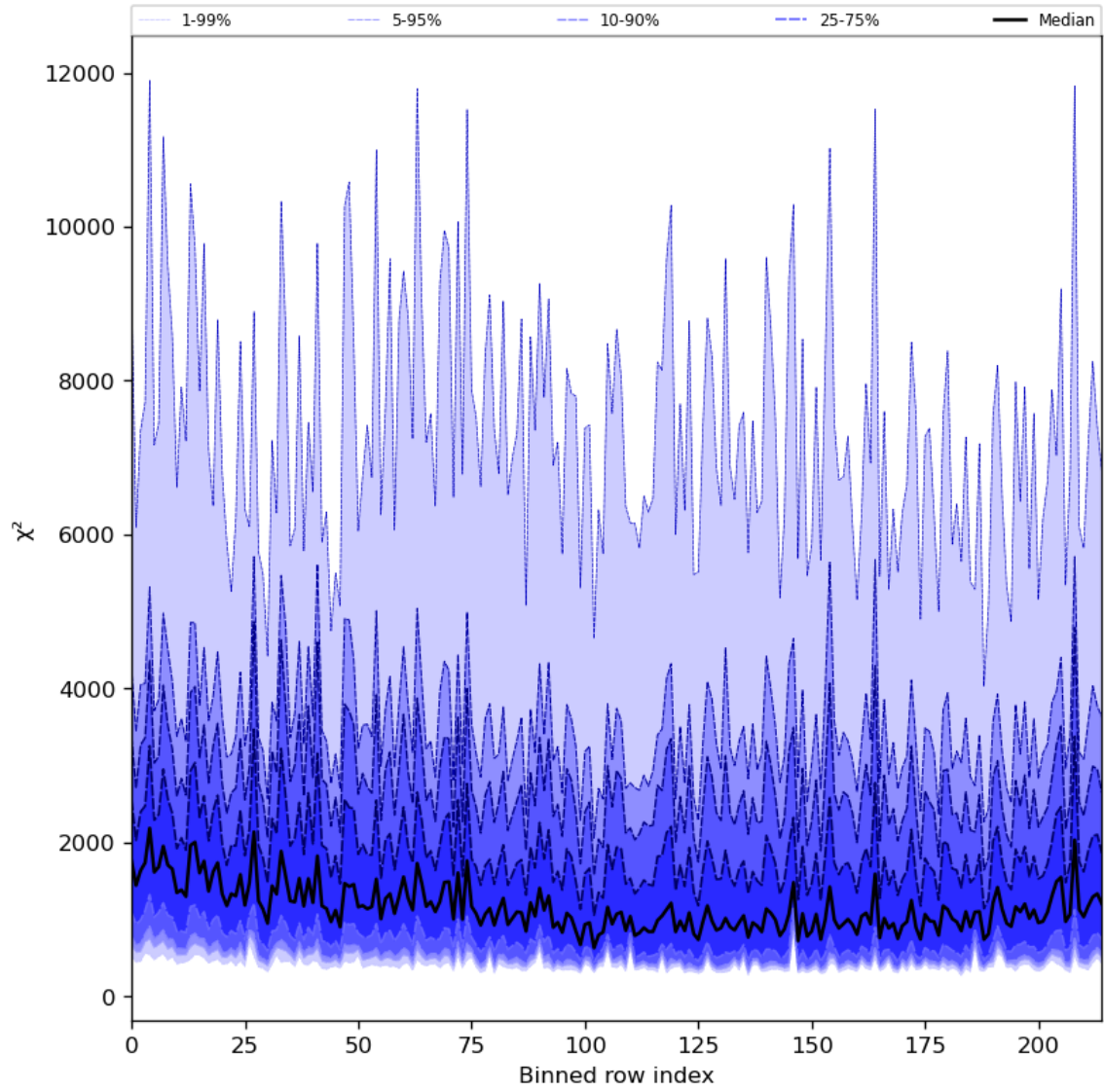
Figure 30: Along track statistics of “ \chi^2 ” for 2024-03-31 to 2024-04-01
