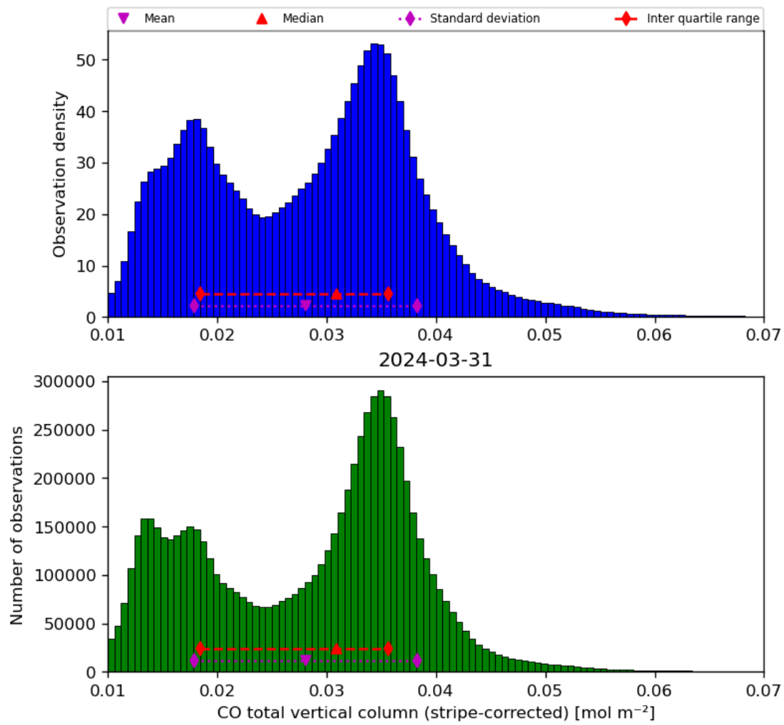
Figure 19: Histogram of “CO total vertical column (stripe-corrected)” for 2024-03-31 to 2024-04-01
