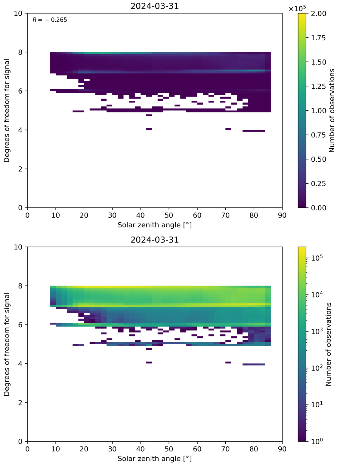
Figure 65: Scatter density plot of “Solar zenith angle” against “Degrees of freedom for signal” for 2024-03-31 to 2024-04-01.
