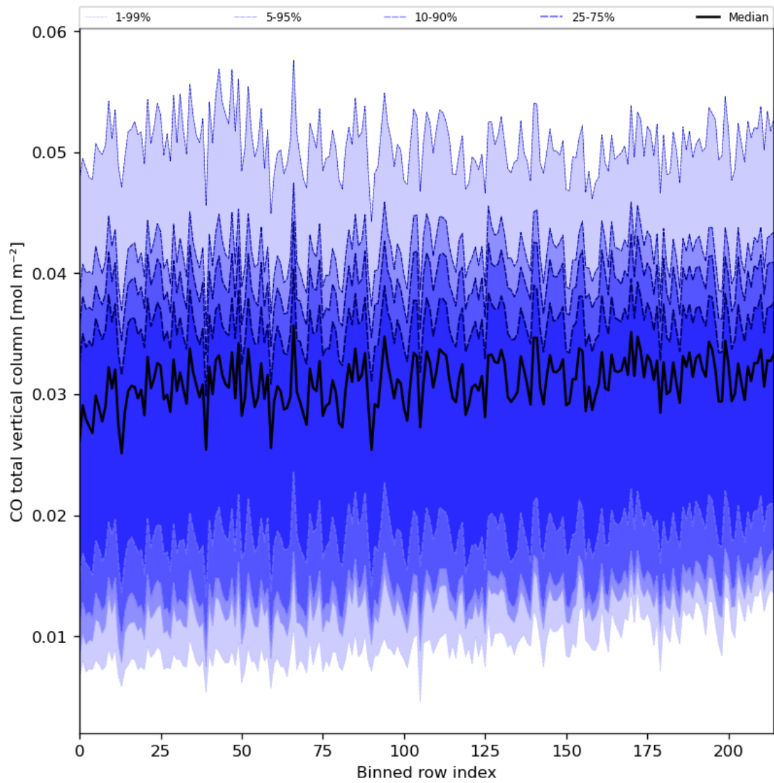
Figure 26: Along track statistics of “CO total vertical column” for 2024-03-31 to 2024-04-01
