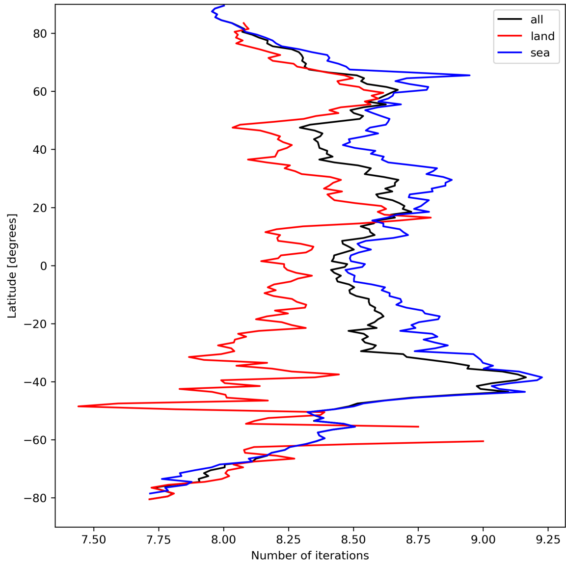
Figure 16: Zonal average of “Number of iterations” for 2024-03-31 to 2024-04-01.
