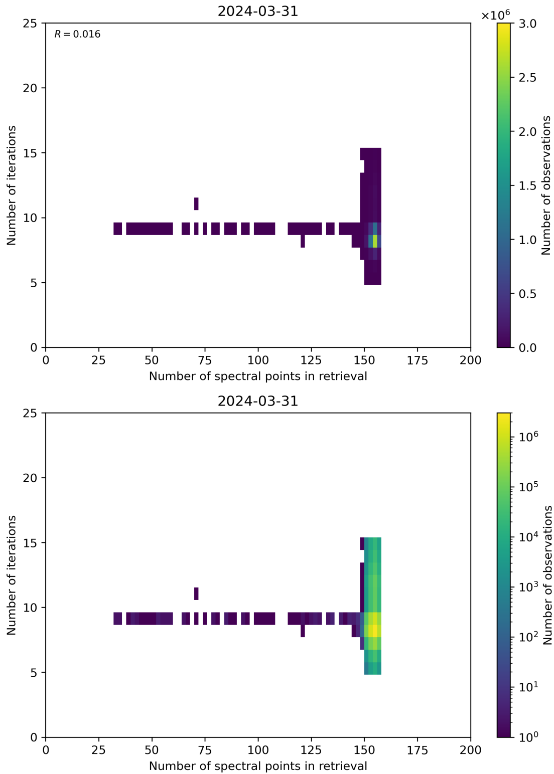
Figure 60: Scatter density plot of “Number of spectral points in retrieval” against “Number of iterations” for 2024-03-31 to 2024-04-01.
