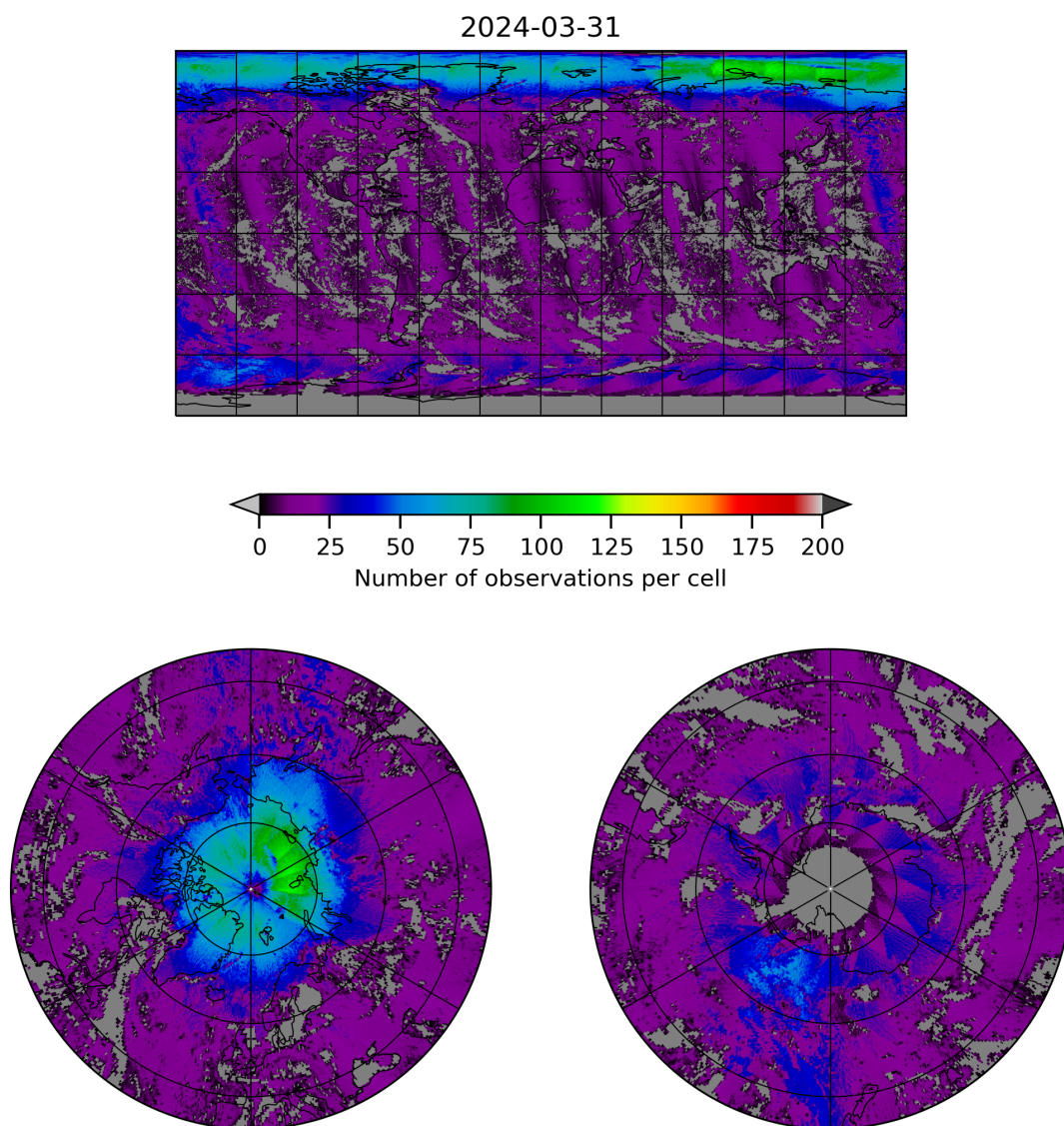
Figure 8: Map of the number of observations for 2024-03-31 to 2024-04-01
