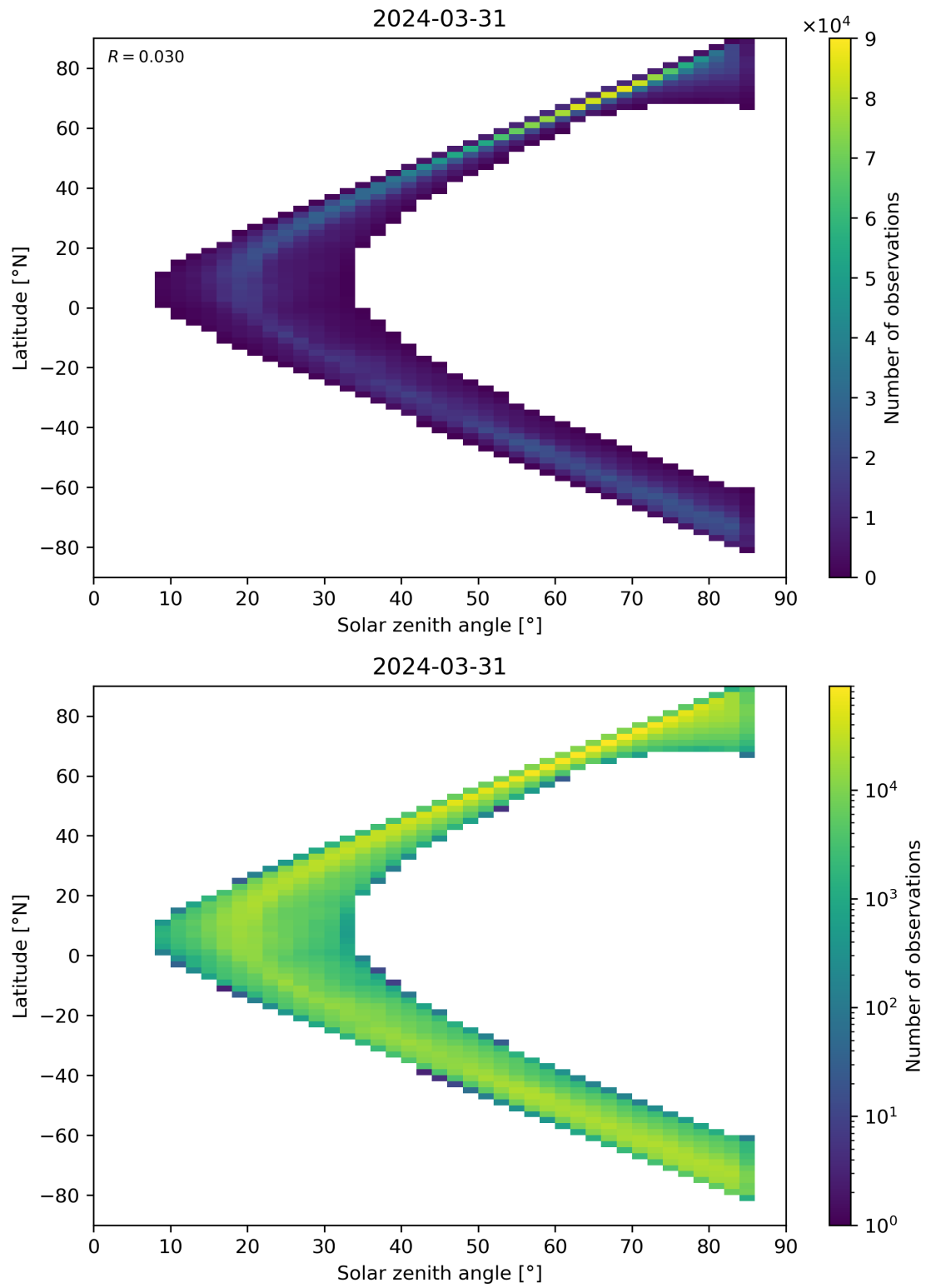
Figure 66: Scatter density plot of “Solar zenith angle” against “Latitude” for 2024-03-31 to 2024-04-01.
