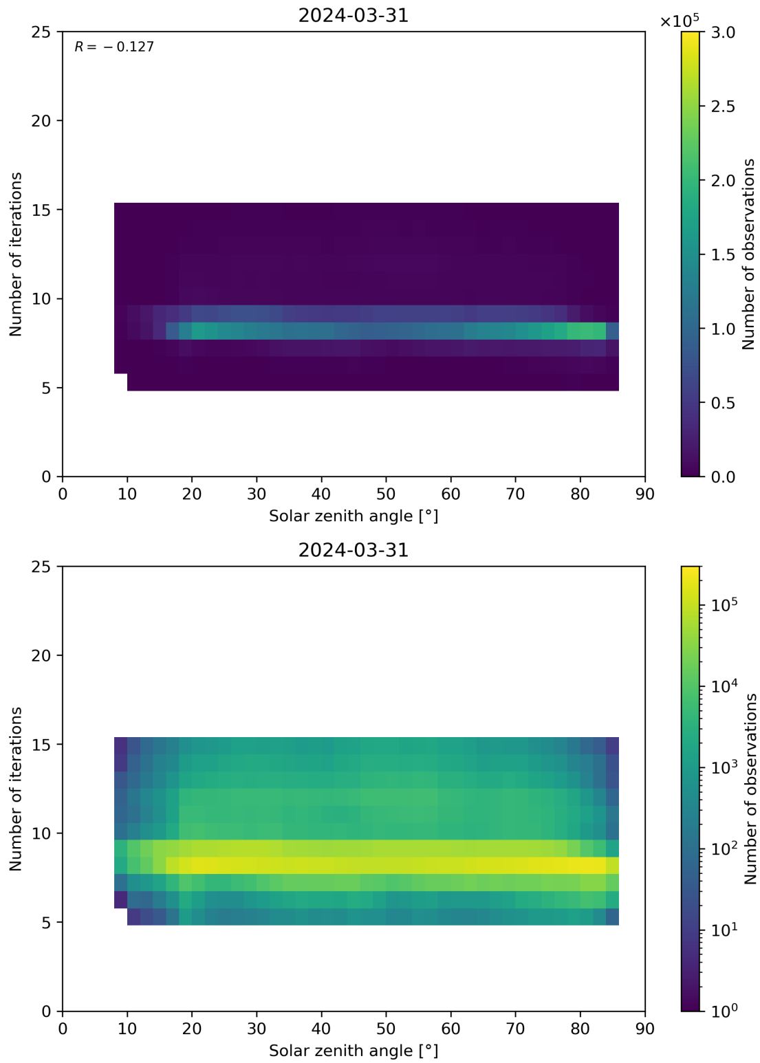
Figure 67: Scatter density plot of “Solar zenith angle” against “Number of iterations” for 2024-03-31 to 2024-04-01.
