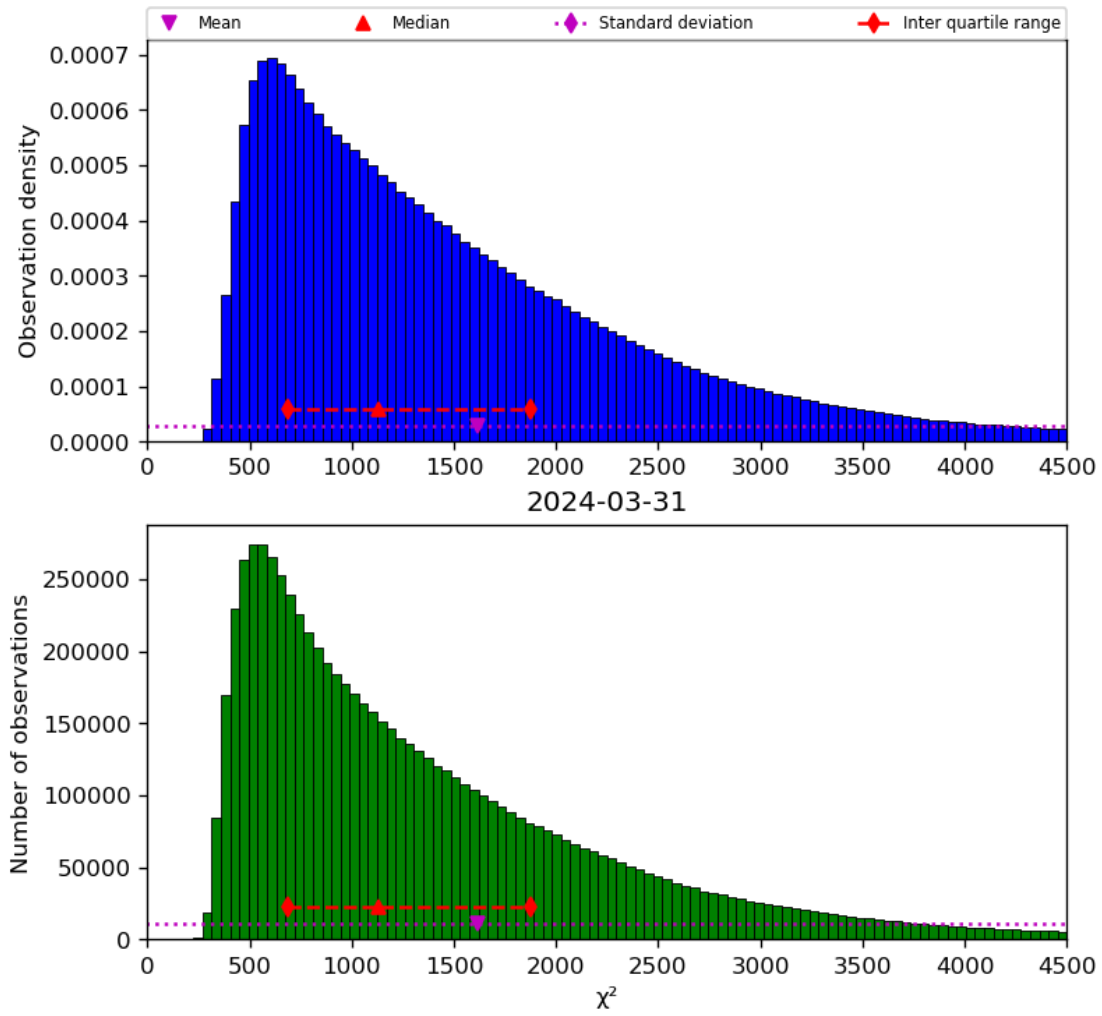
Figure 22: Histogram of " \chi^2 " for 2024-03-31 to 2024-04-01
