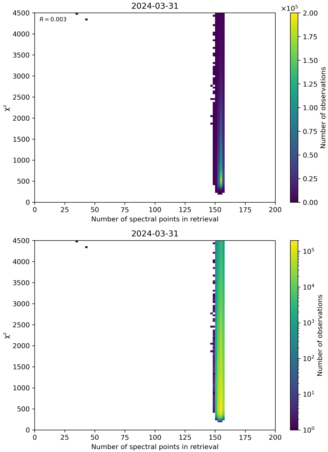
Figure 58: Scatter density plot of “Number of spectral points in retrieval” against “ \chi^2 ” for 2024-03-31 to 2024-04-01.
