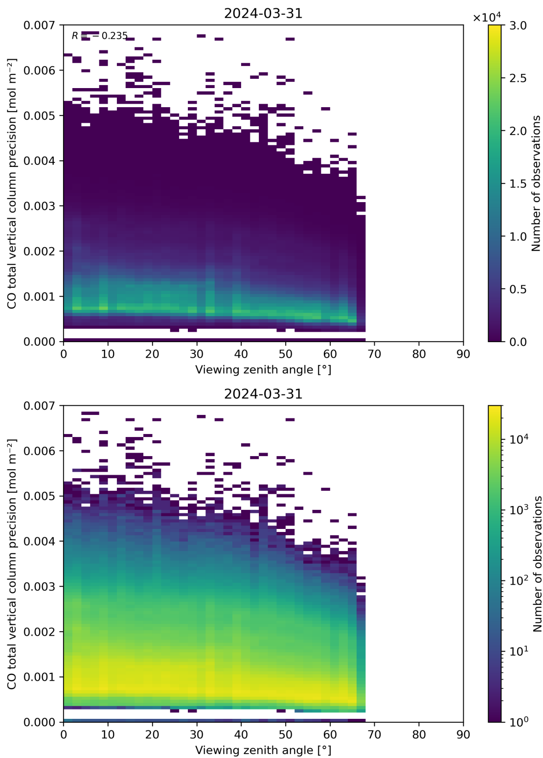
Figure 71: Scatter density plot of “Viewing zenith angle” against “CO total vertical column precision” for 2024-03-31 to 2024-04-01.
