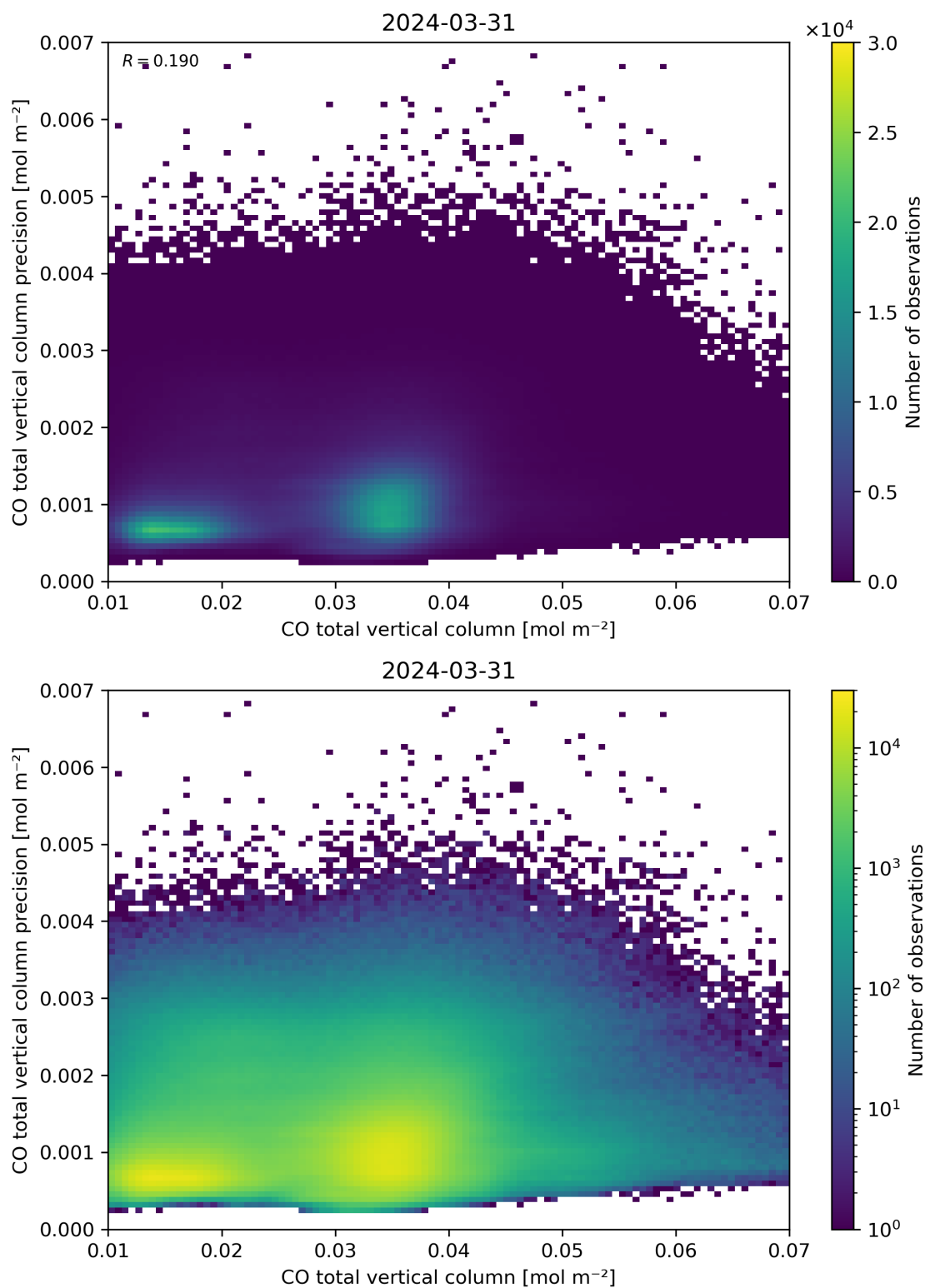
Figure 34: Scatter density plot of “CO total vertical column” against “CO total vertical column precision” for 2024-03-31 to 2024-04-01.
