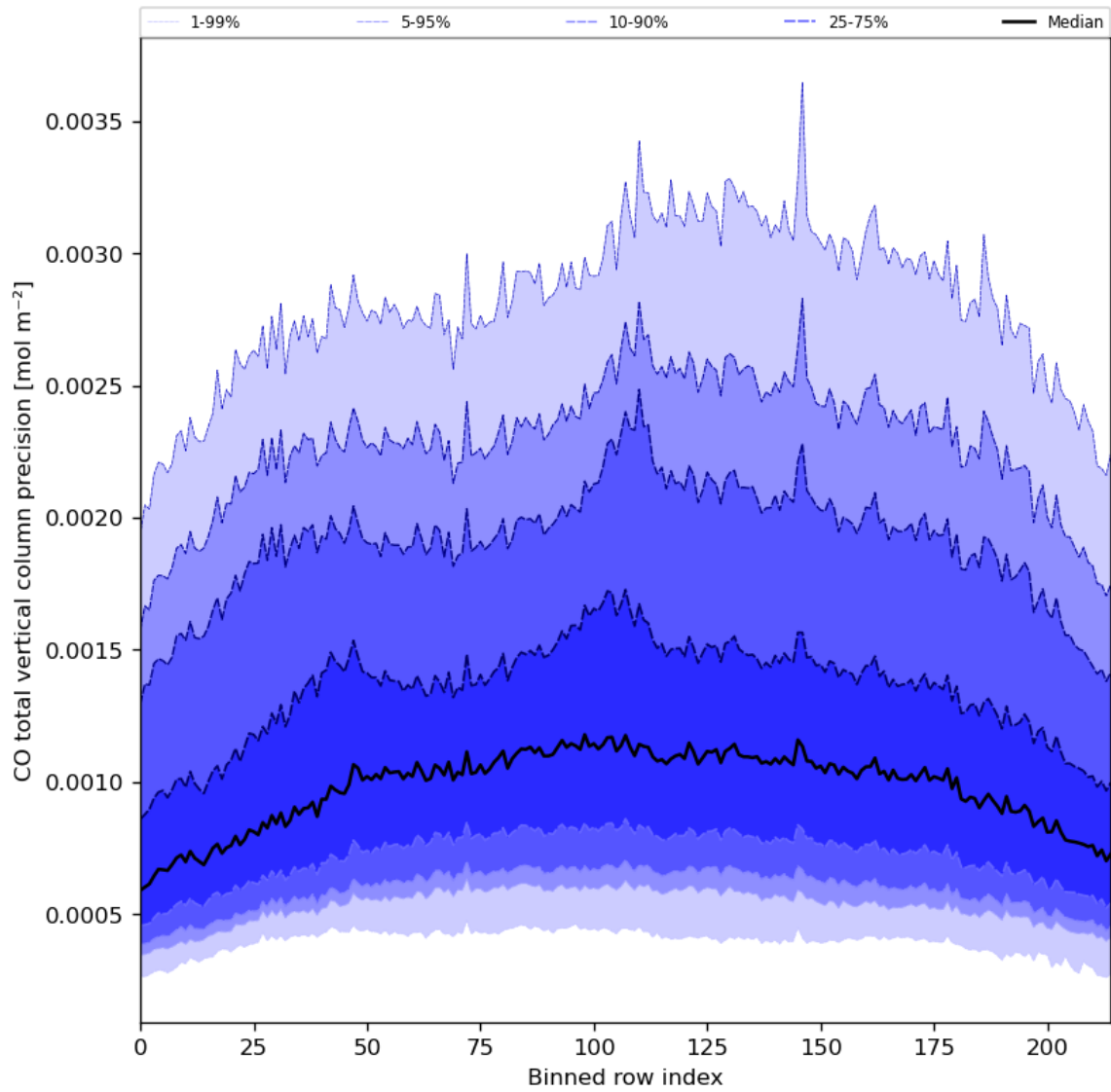
Figure 28: Along track statistics of “CO total vertical column precision” for 2024-03-31 to 2024-04-01
