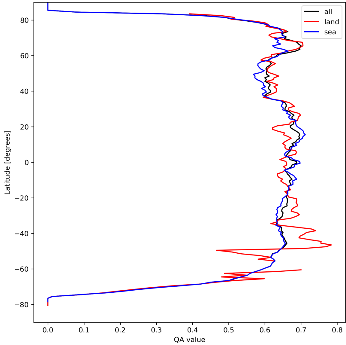
Figure 9: Zonal average of “QA value” for 2024-03-31 to 2024-04-01.
