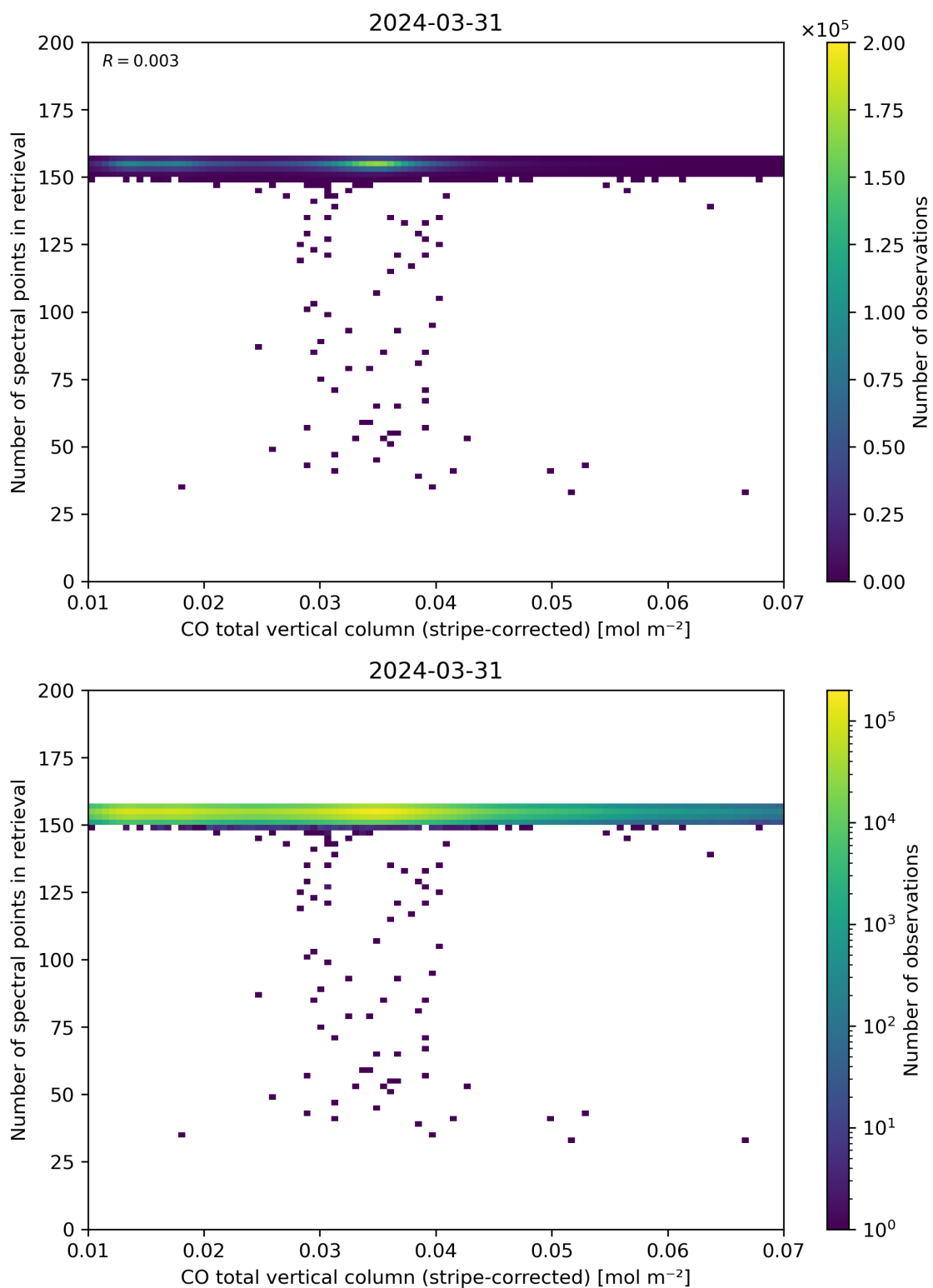
Figure 40: Scatter density plot of “CO total vertical column (stripe-corrected)” against “Number of spectral points in retrieval” for 2024-03-31 to 2024-04-01.
