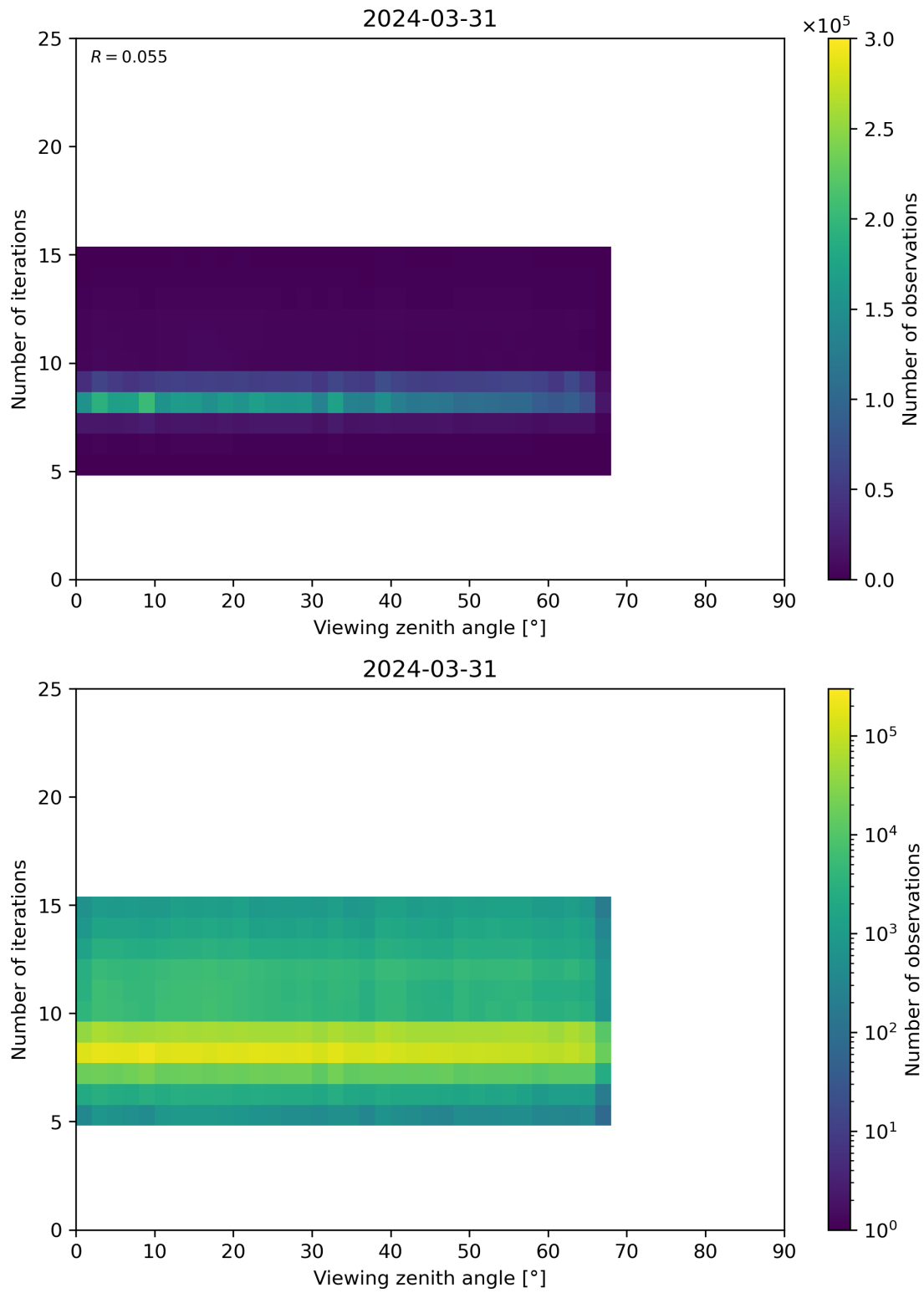
Figure 75: Scatter density plot of “Viewing zenith angle” against “Number of iterations” for 2024-03-31 to 2024-04-01.
