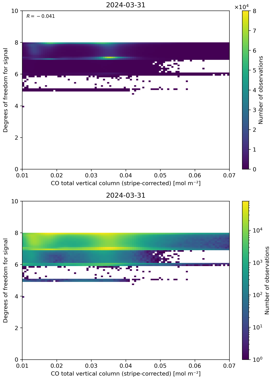
Figure 38: Scatter density plot of “CO total vertical column (stripe-corrected)” against “Degrees of freedom for signal” for 2024-03-31 to 2024-04-01.
