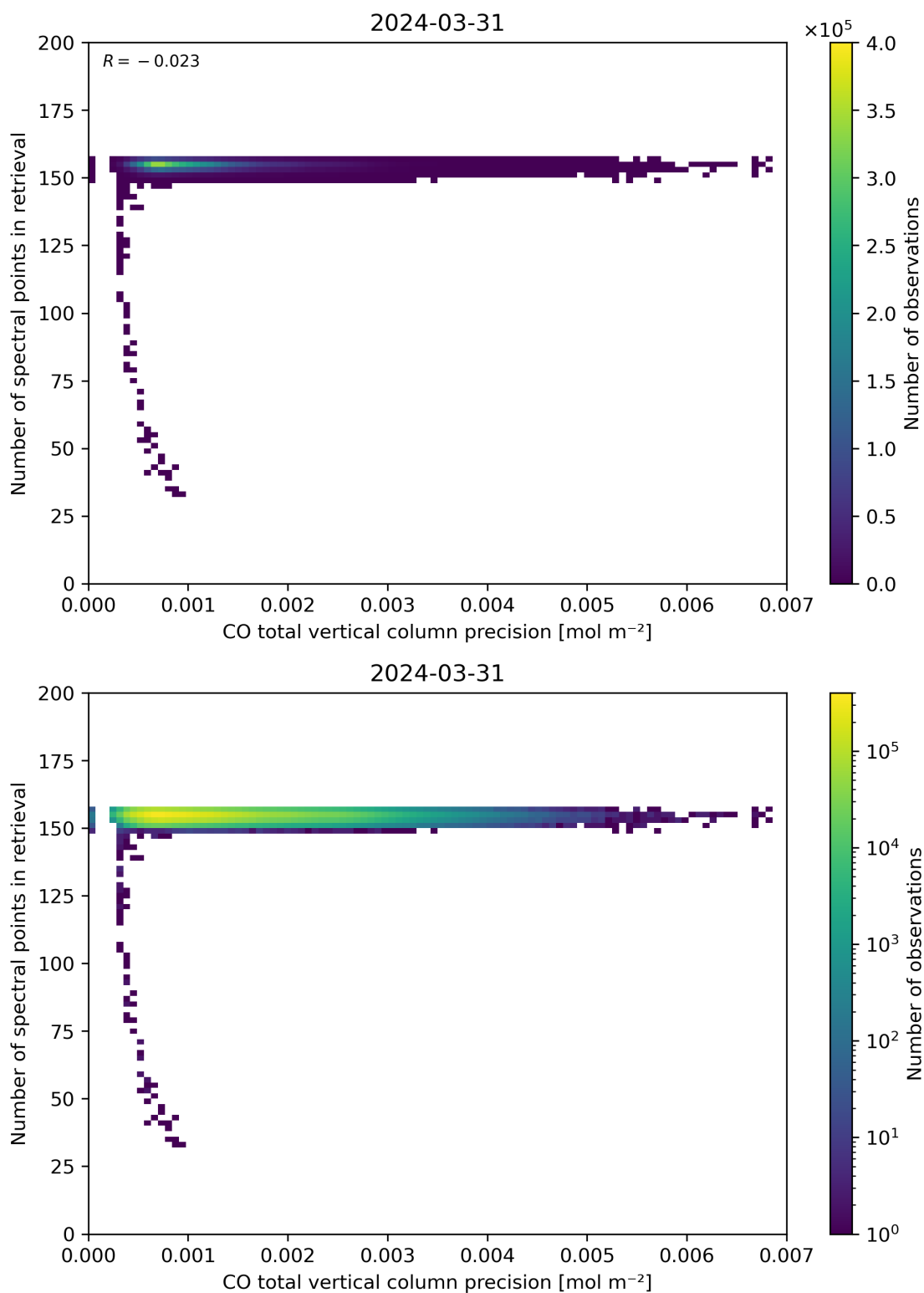
Figure 47: Scatter density plot of “CO total vertical column precision” against “Number of spectral points in retrieval” for 2024-03-31 to 2024-04-01.
