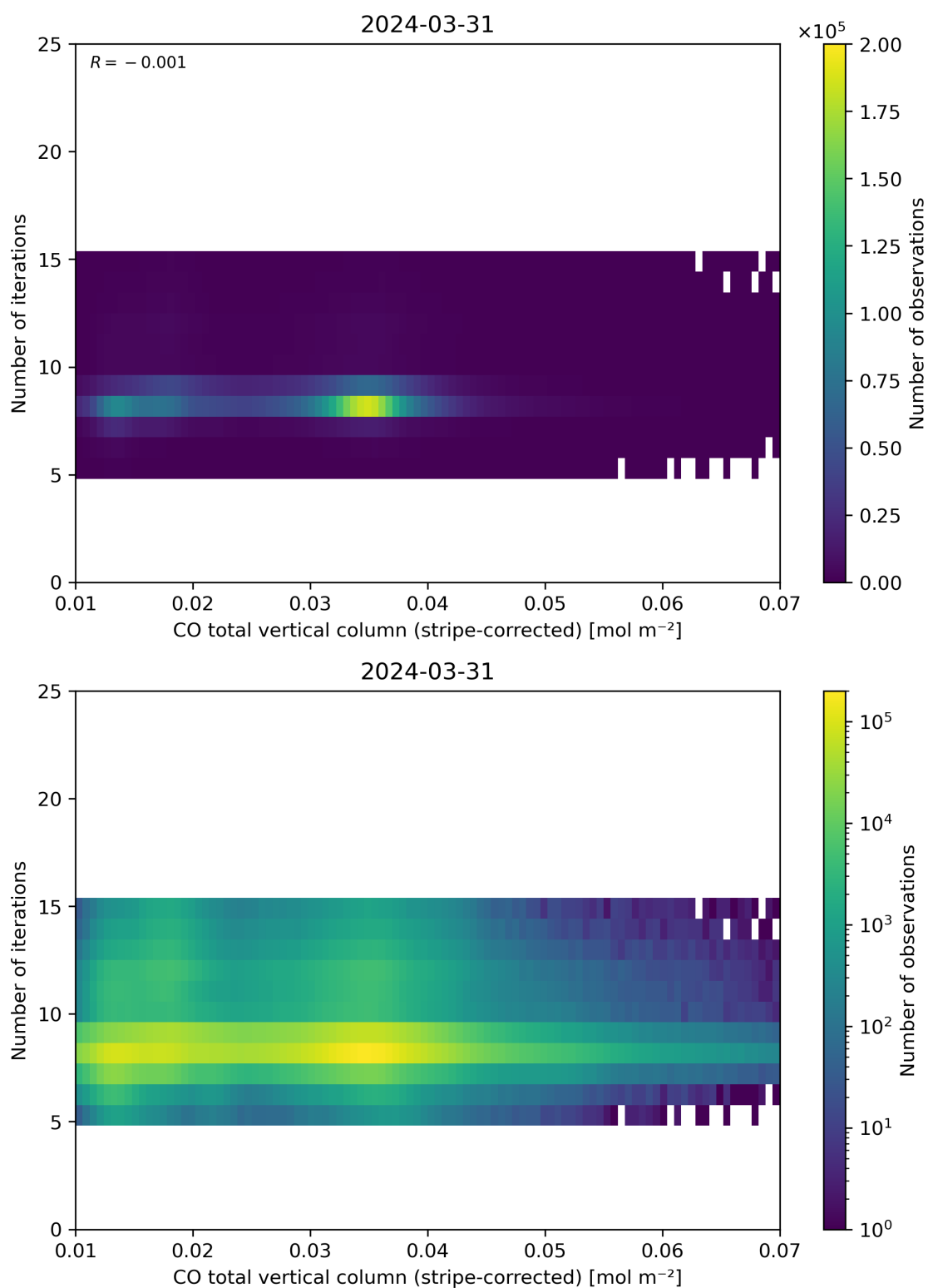
Figure 39: Scatter density plot of “CO total vertical column (stripe-corrected)” against “Number of iterations” for 2024-03-31 to 2024-04-01.
