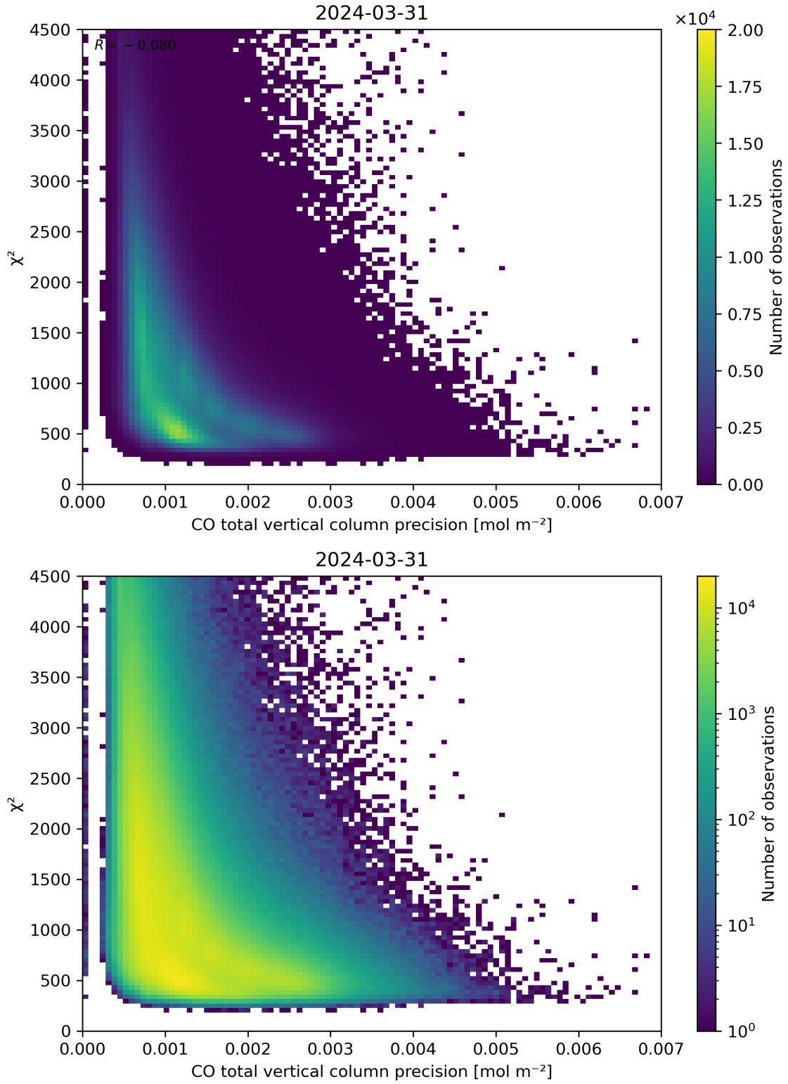
Figure 44: Scatter density plot of “CO total vertical column precision” against “ \chi^2 ” for 2024-03-31 to 2024-04-01.
