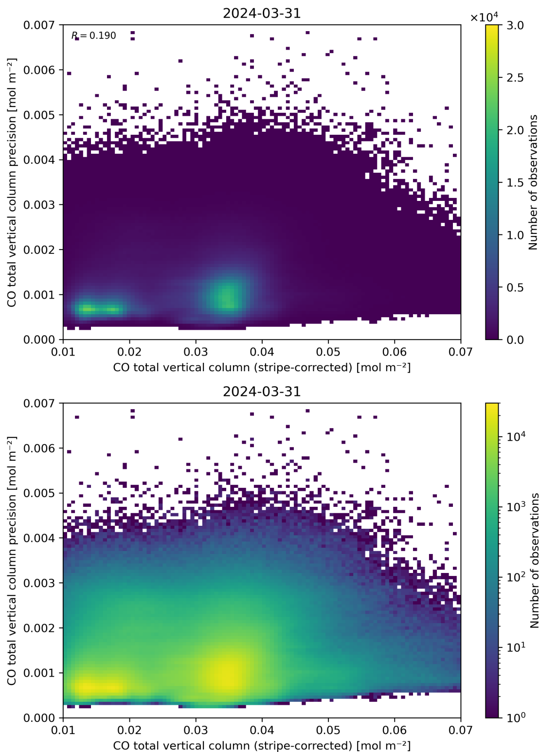
Figure 36: Scatter density plot of “CO total vertical column (stripe-corrected)” against “CO total vertical column precision” for 2024-03-31 to 2024-04-01.
