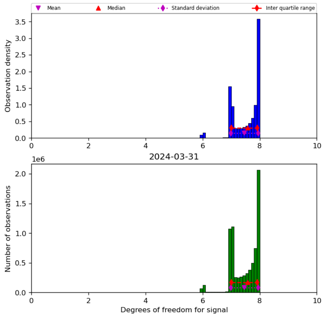
Figure 23: Histogram of “Degrees of freedom for signal” for 2024-03-31 to 2024-04-01
