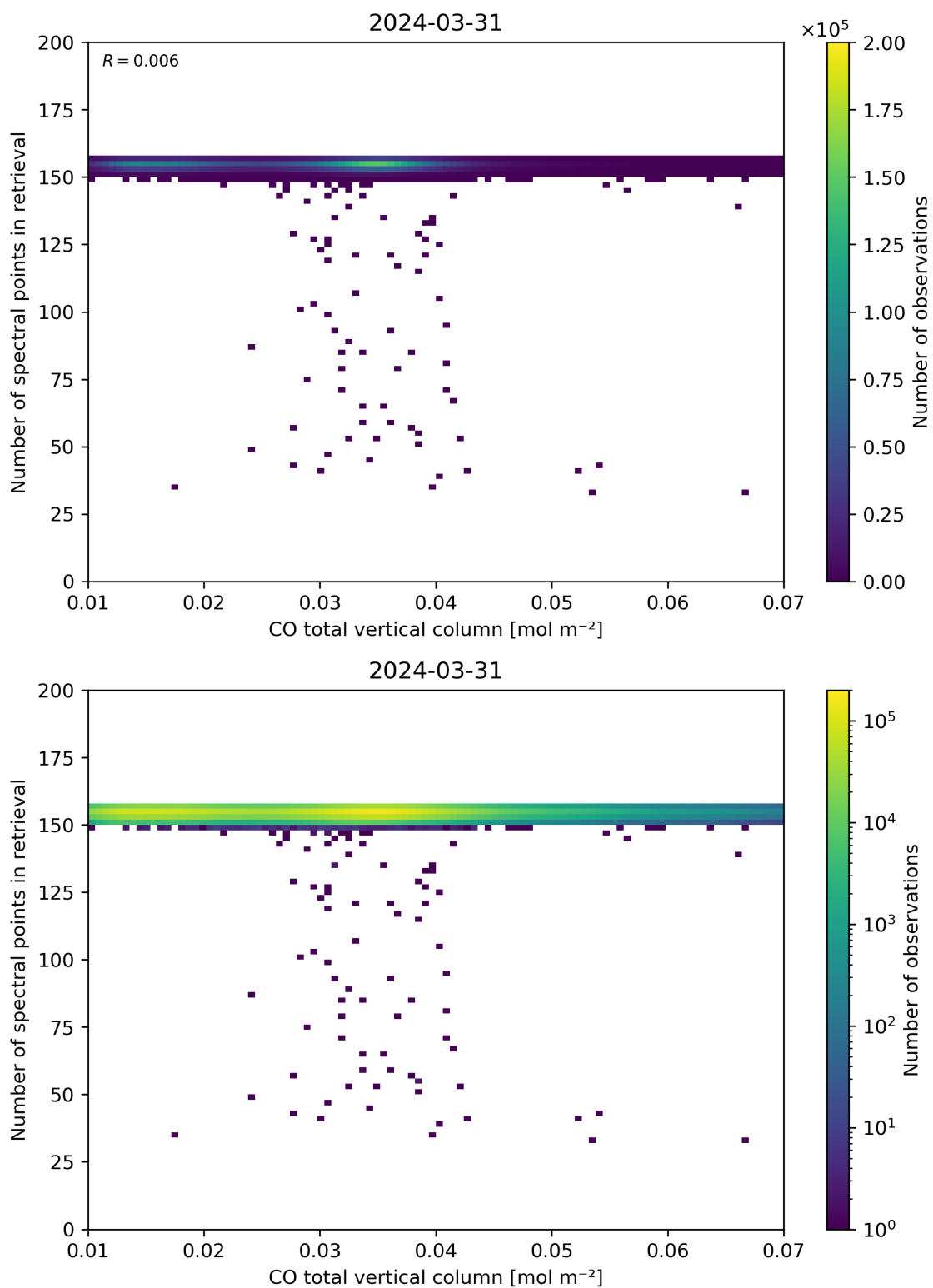
Figure 43: Scatter density plot of “CO total vertical column” against “Number of spectral points in retrieval” for 2024-03-31 to 2024-04-01.
