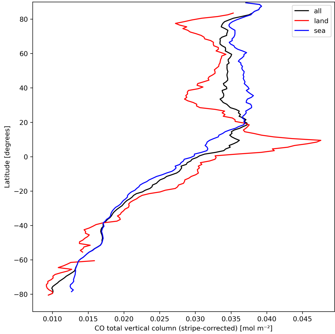
Figure 11: Zonal average of “CO total vertical column (stripe-corrected)” for 2024-03-31 to 2024-04-01.
