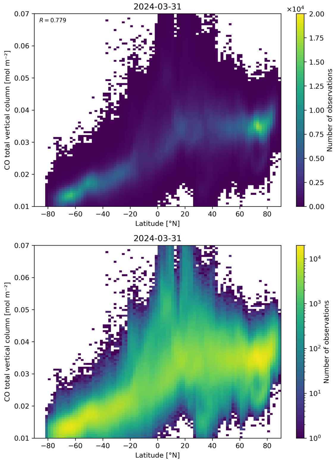
Figure 51: Scatter density plot of “Latitude” against “CO total vertical column” for 2024-03-31 to 2024-04-01.
