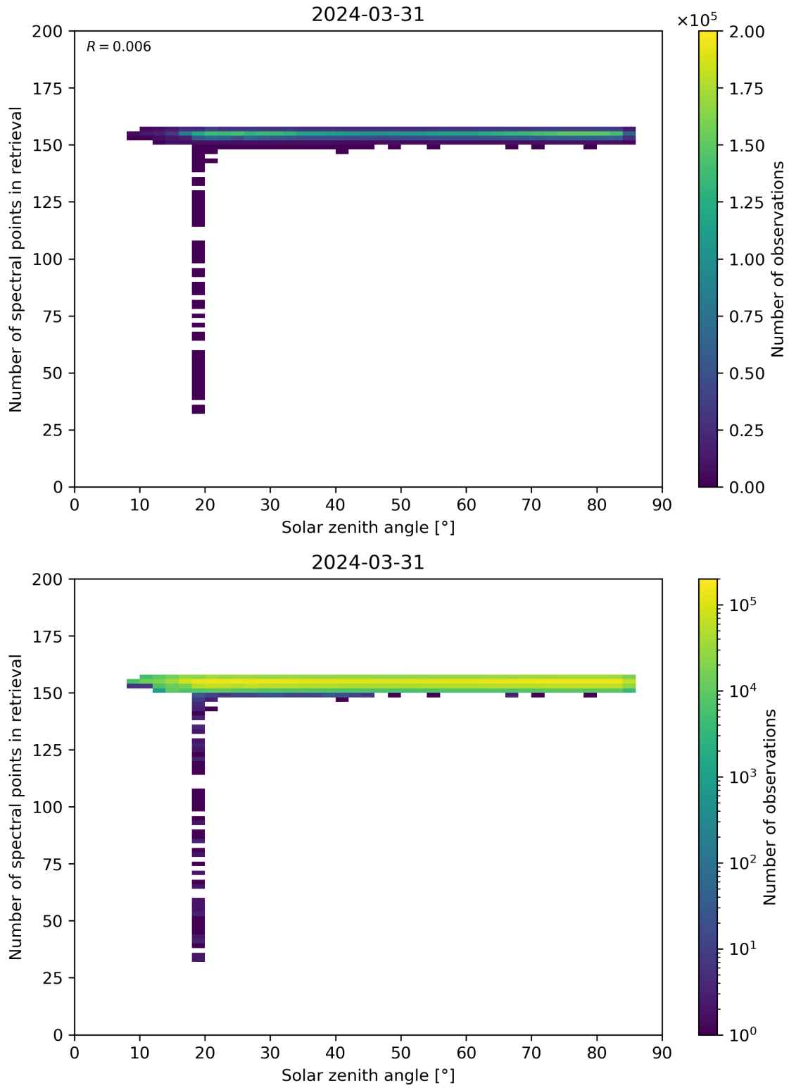
Figure 68: Scatter density plot of “Solar zenith angle” against “Number of spectral points in retrieval” for 2024-03-31 to 2024-04-01.
