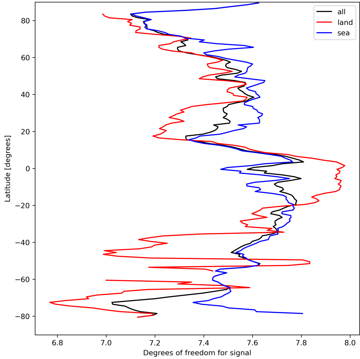
Figure 15: Zonal average of “Degrees of freedom for signal” for 2024-03-31 to 2024-04-01.
