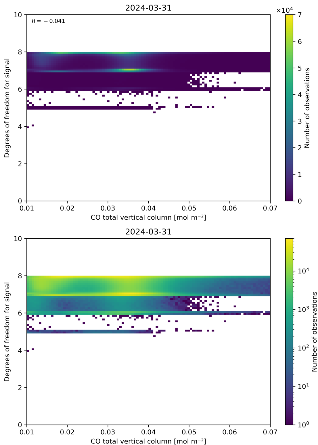
Figure 41: Scatter density plot of “CO total vertical column” against “Degrees of freedom for signal” for 2024-03-31 to 2024-04-01.
