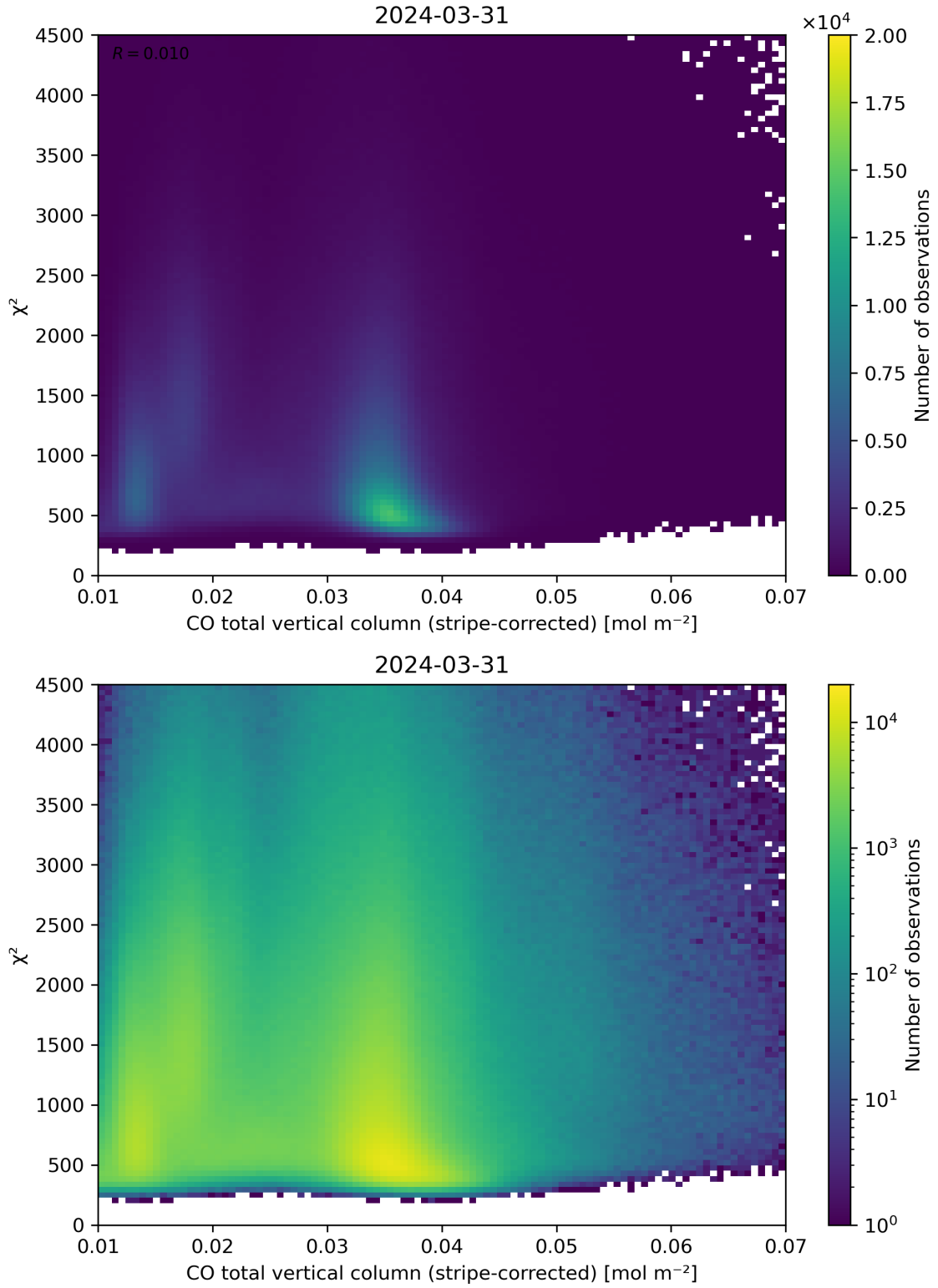
Figure 37: Scatter density plot of “CO total vertical column (stripe-corrected)” against “ \chi^2 ” for 2024-03-31 to 2024-04-01.
