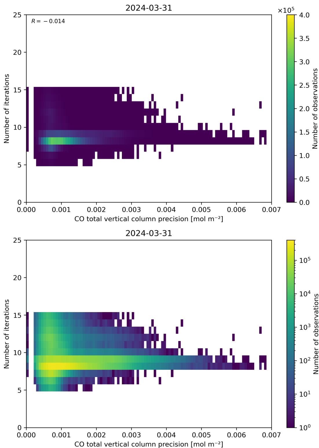
Figure 46: Scatter density plot of “CO total vertical column precision” against “Number of iterations” for 2024-03-31 to 2024-04-01.
