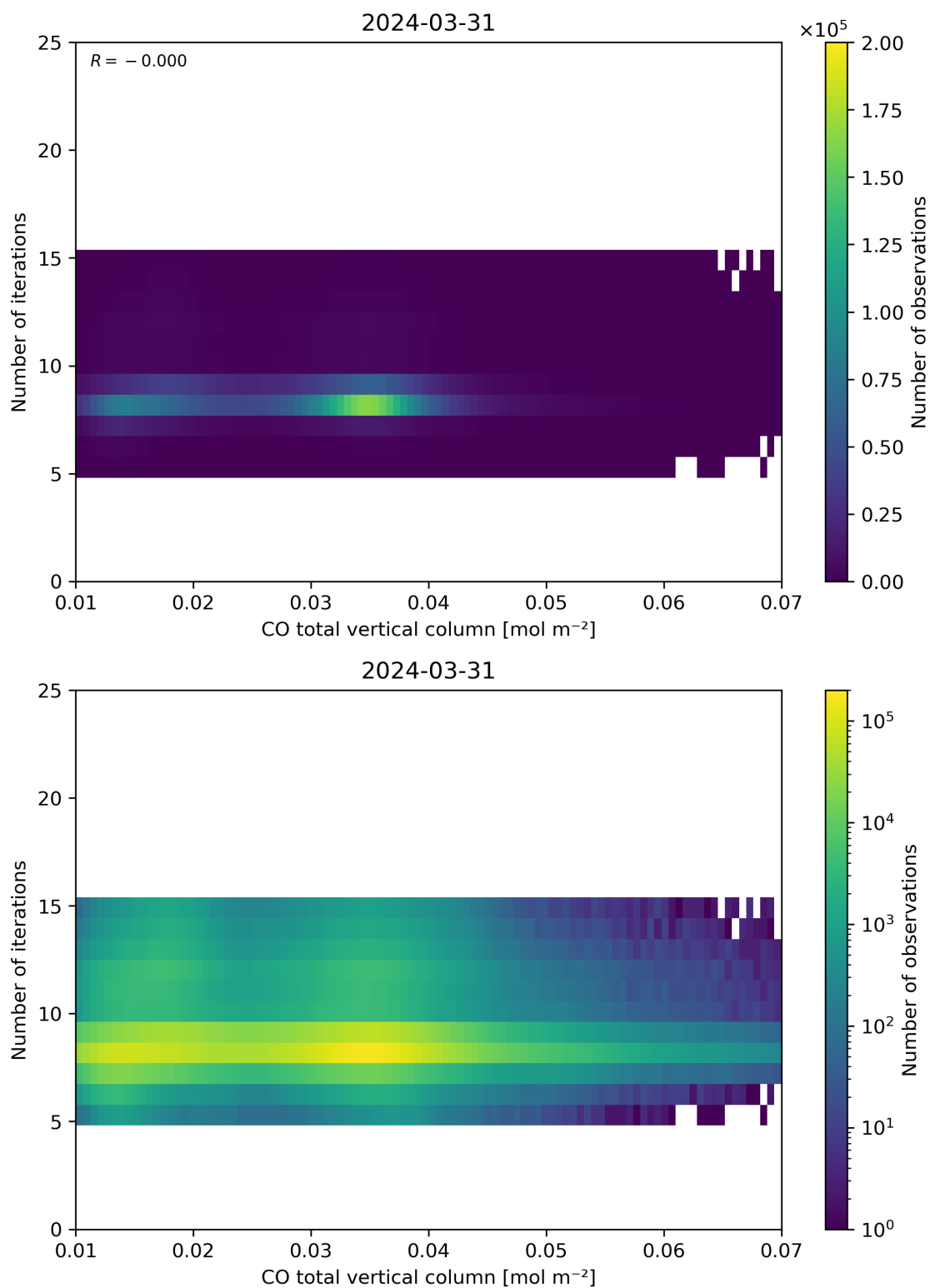
Figure 42: Scatter density plot of “CO total vertical column” against “Number of iterations” for 2024-03-31 to 2024-04-01.
