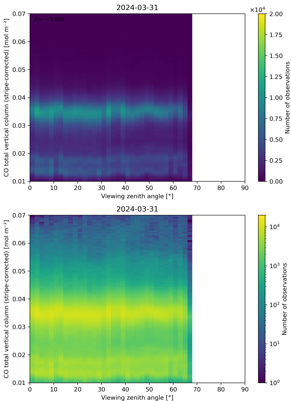
Figure 70: Scatter density plot of “Viewing zenith angle” against “CO total vertical column (stripe-corrected)” for 2024-03-31 to 2024-04-01.
