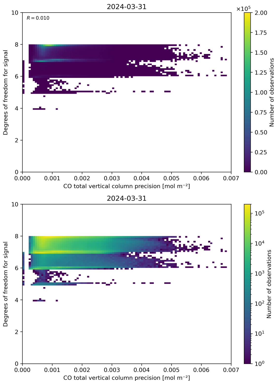
Figure 45: Scatter density plot of “CO total vertical column precision” against “Degrees of freedom for signal” for 2024-03-31 to 2024-04-01.
