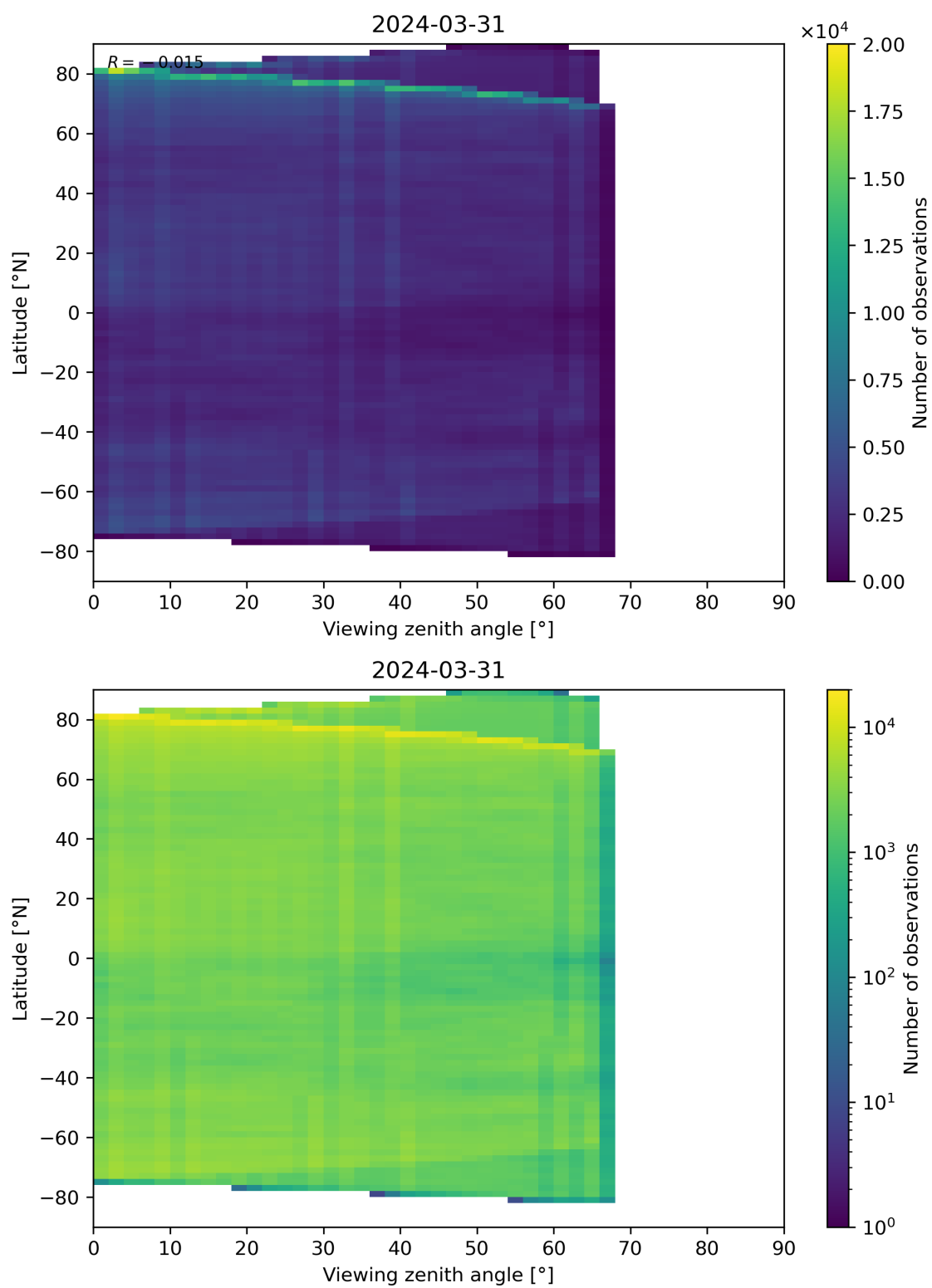
Figure 74: Scatter density plot of “Viewing zenith angle” against “Latitude” for 2024-03-31 to 2024-04-01.
