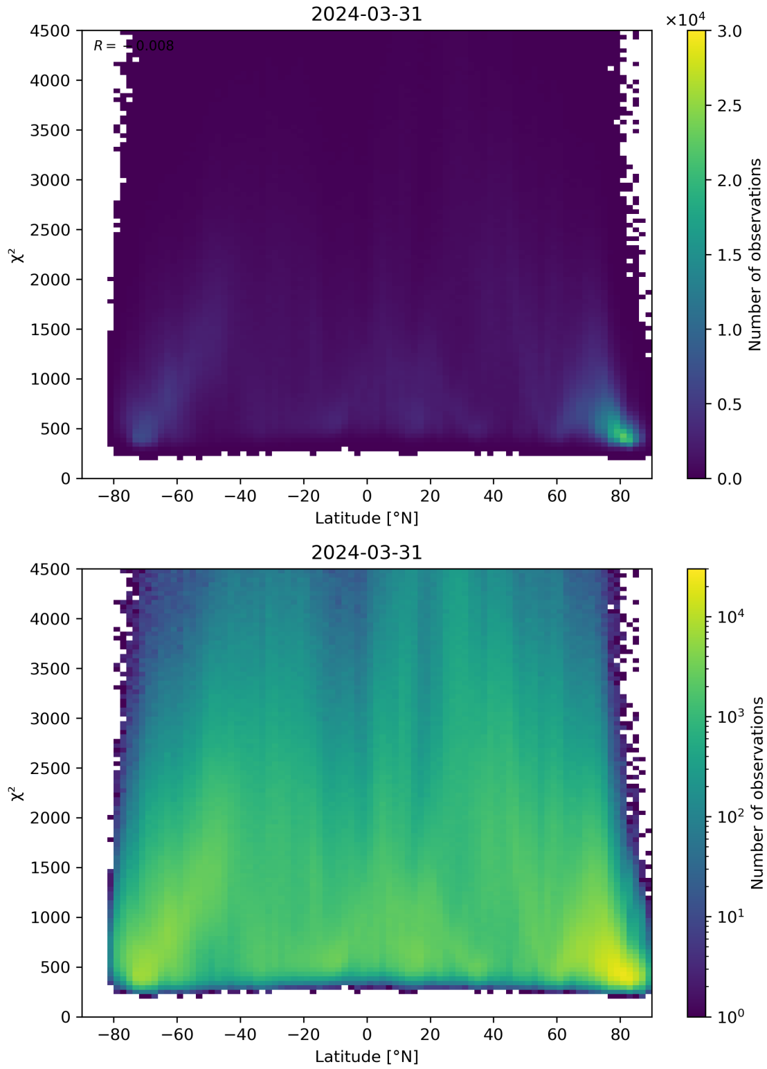
Figure 54: Scatter density plot of “Latitude” against “ \chi^2 ” for 2024-03-31 to 2024-04-01.
