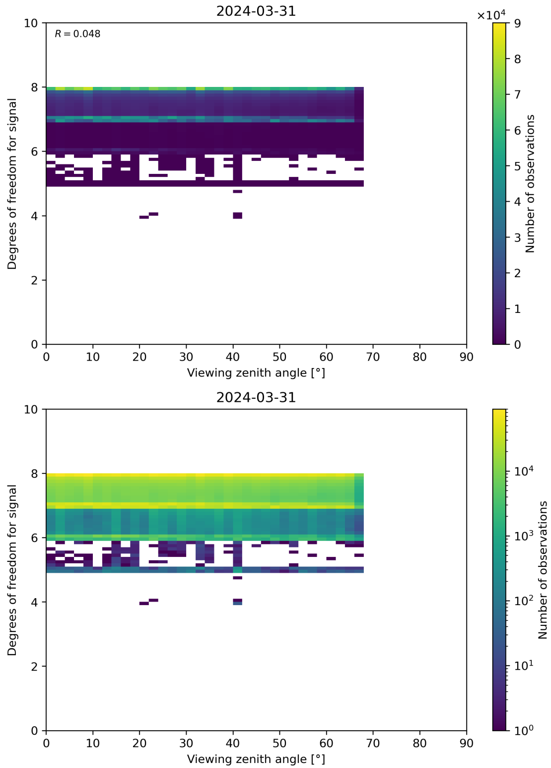
Figure 73: Scatter density plot of “Viewing zenith angle” against “Degrees of freedom for signal” for 2024-03-31 to 2024-04-01.
