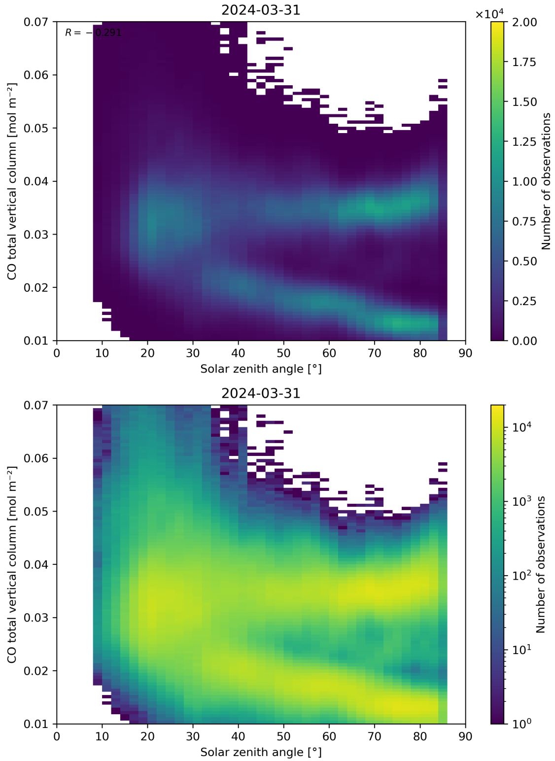
Figure 61: Scatter density plot of “Solar zenith angle” against “CO total vertical column” for 2024-03-31 to 2024-04-01.
