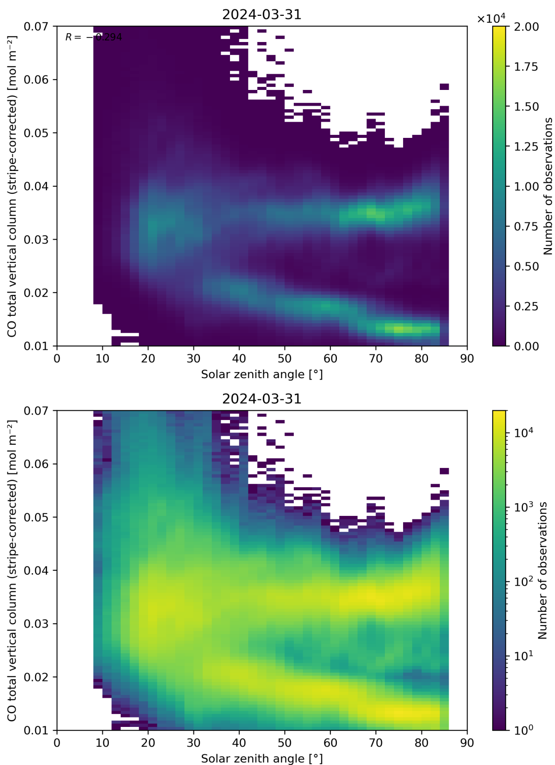
Figure 62: Scatter density plot of “Solar zenith angle” against “CO total vertical column (stripe-corrected)” for 2024-03-31 to 2024-04-01.
