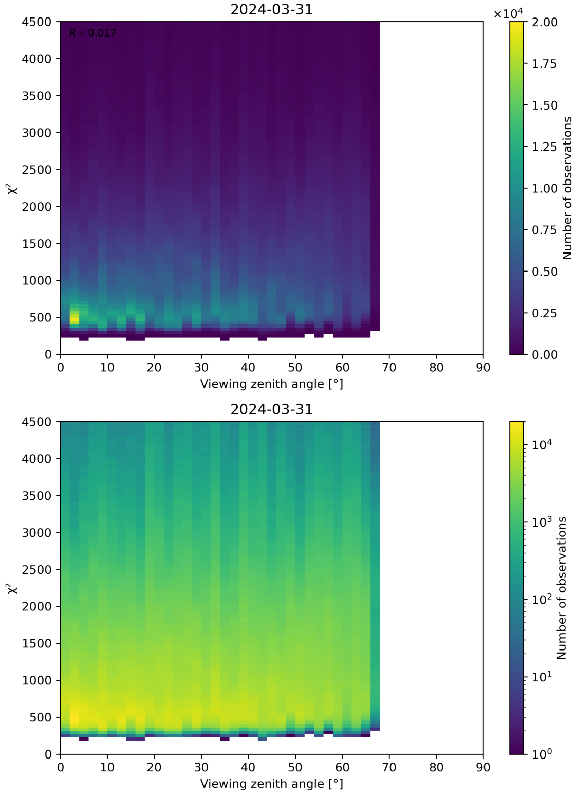
Figure 72: Scatter density plot of “Viewing zenith angle” against “ \chi^2 ” for 2024-03-31 to 2024-04-01.
