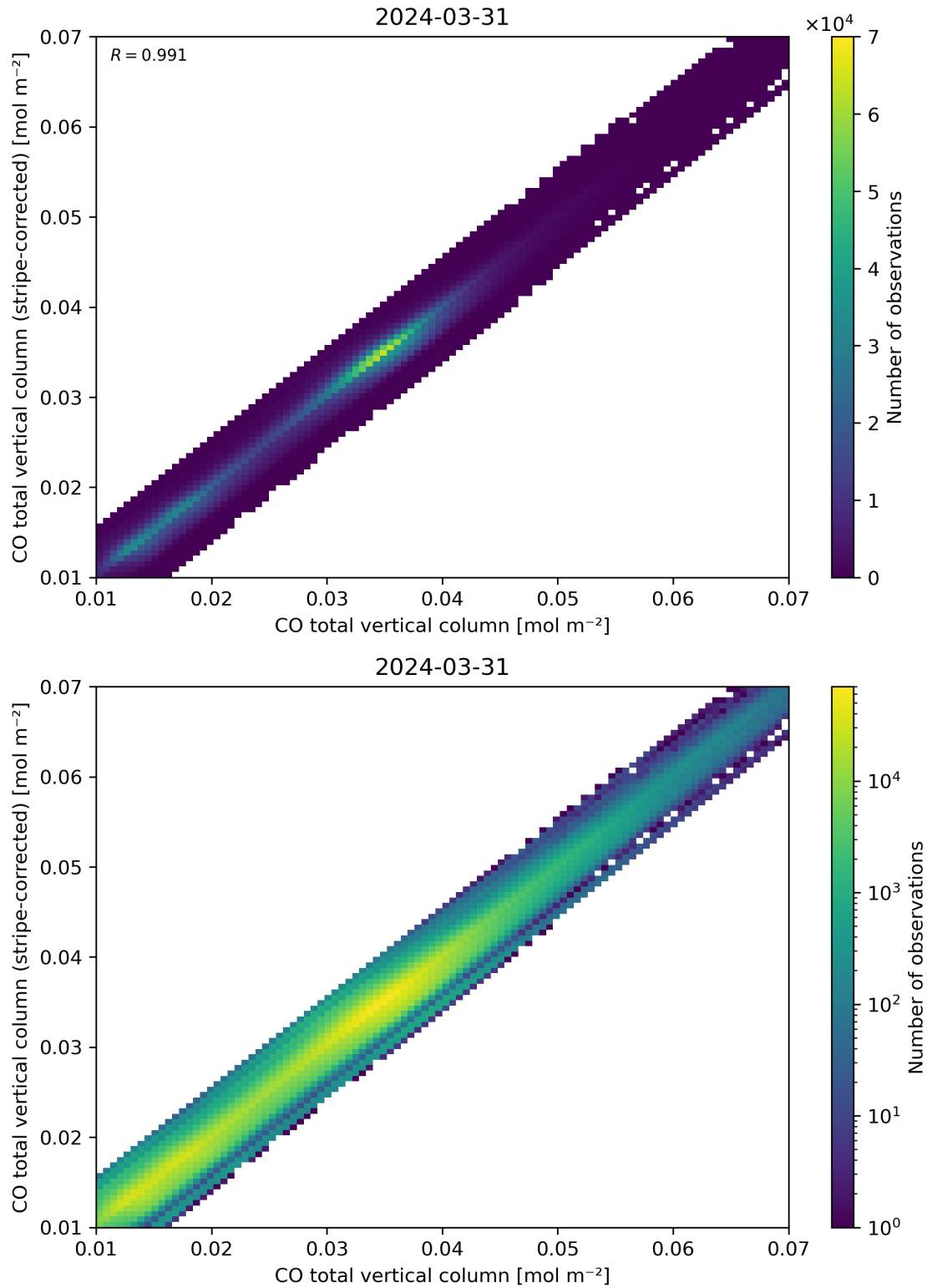
Figure 33: Scatter density plot of “CO total vertical column” against “CO total vertical column (stripe-corrected)” for 2024-03-31 to 2024-04-01.
