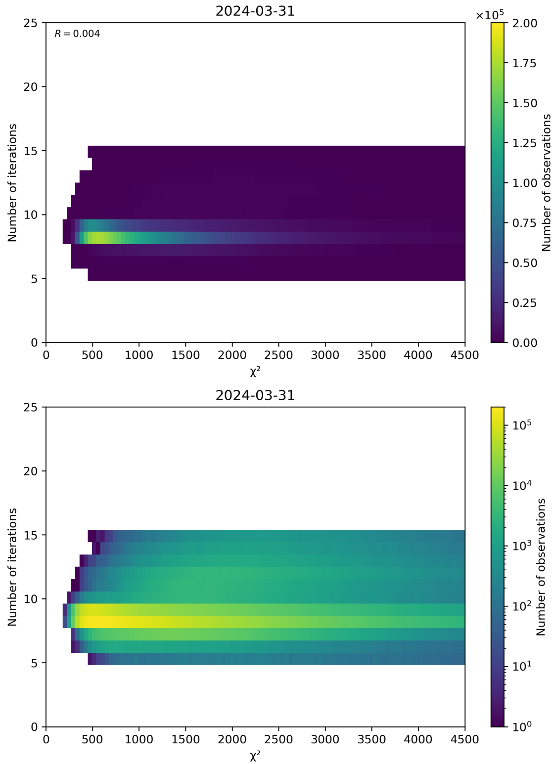
Figure 49: Scatter density plot of “ \chi^2 ” against “Number of iterations” for 2024-03-31 to 2024-04-01.
