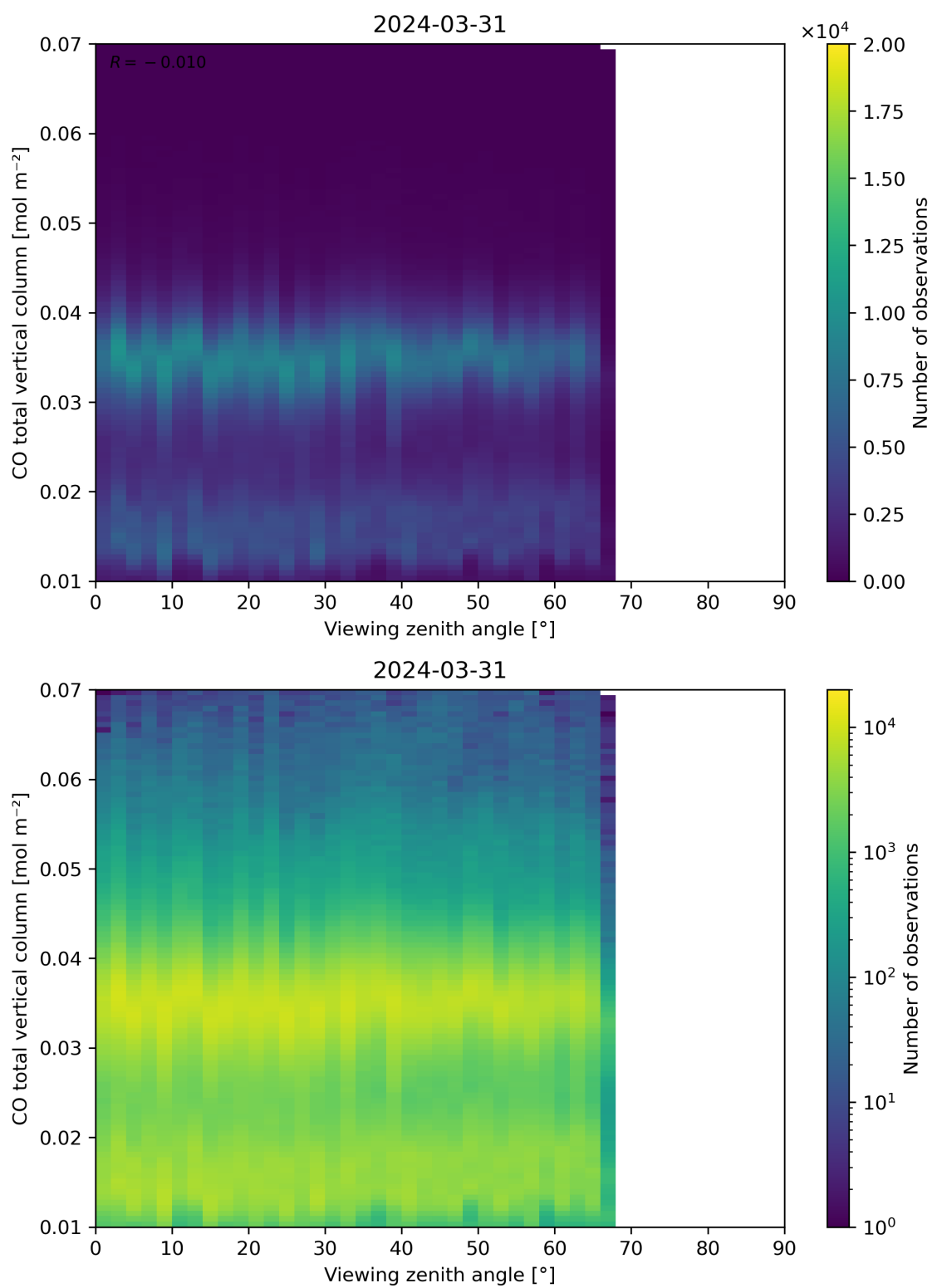
Figure 69: Scatter density plot of “Viewing zenith angle” against “CO total vertical column” for 2024-03-31 to 2024-04-01.
