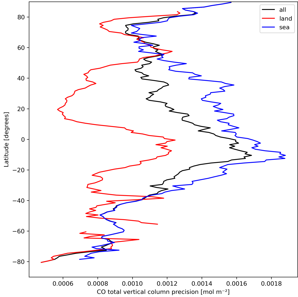
Figure 12: Zonal average of "CO total vertical column precision" for 2024-03-31 to 2024-04-01.
