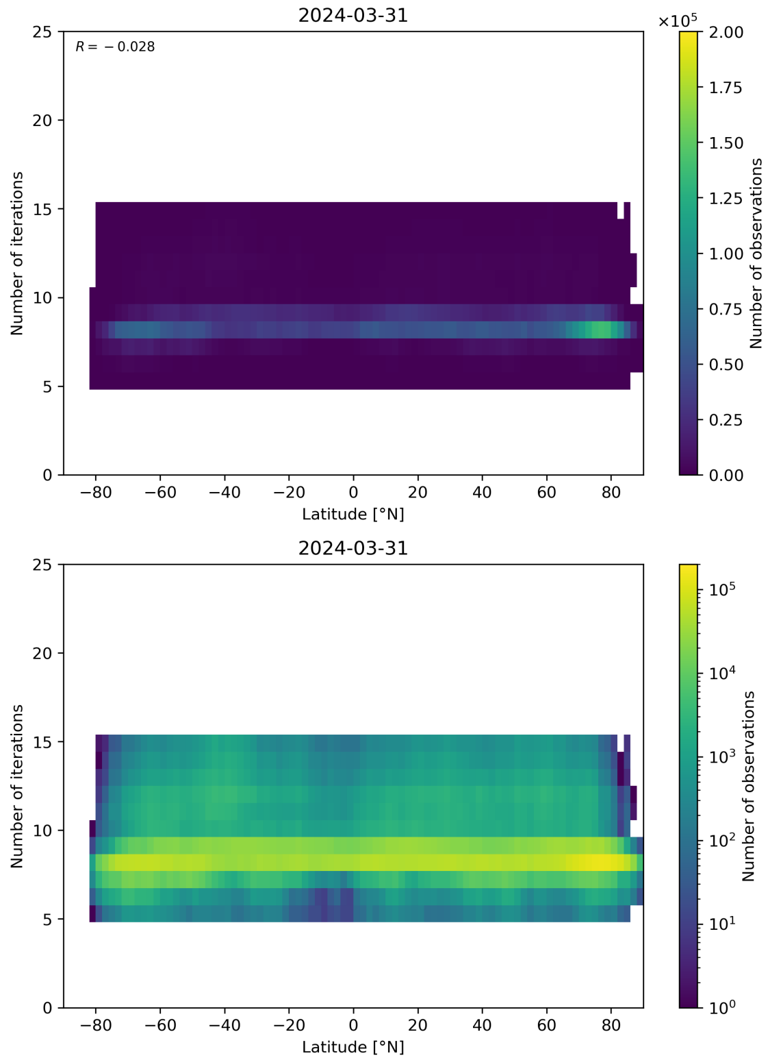
Figure 56: Scatter density plot of “Latitude” against “Number of iterations” for 2024-03-31 to 2024-04-01.
