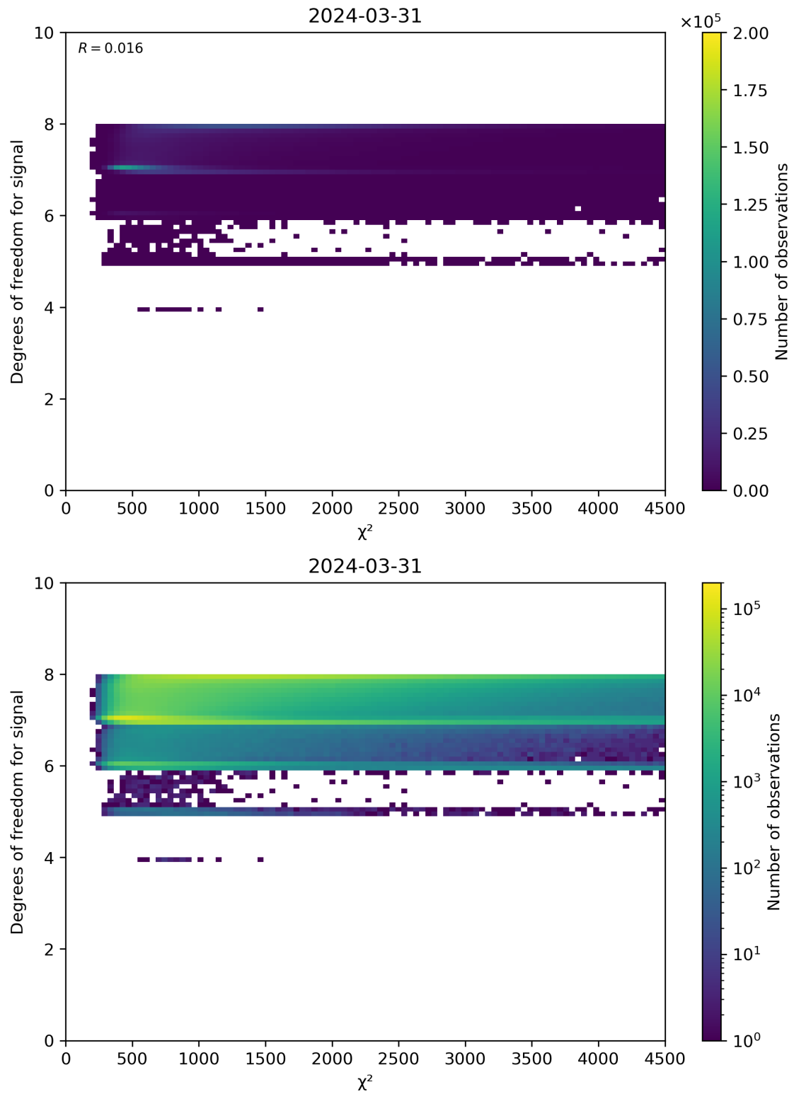
Figure 48: Scatter density plot of “ \chi^2 ” against “Degrees of freedom for signal” for 2024-03-31 to 2024-04-01.
