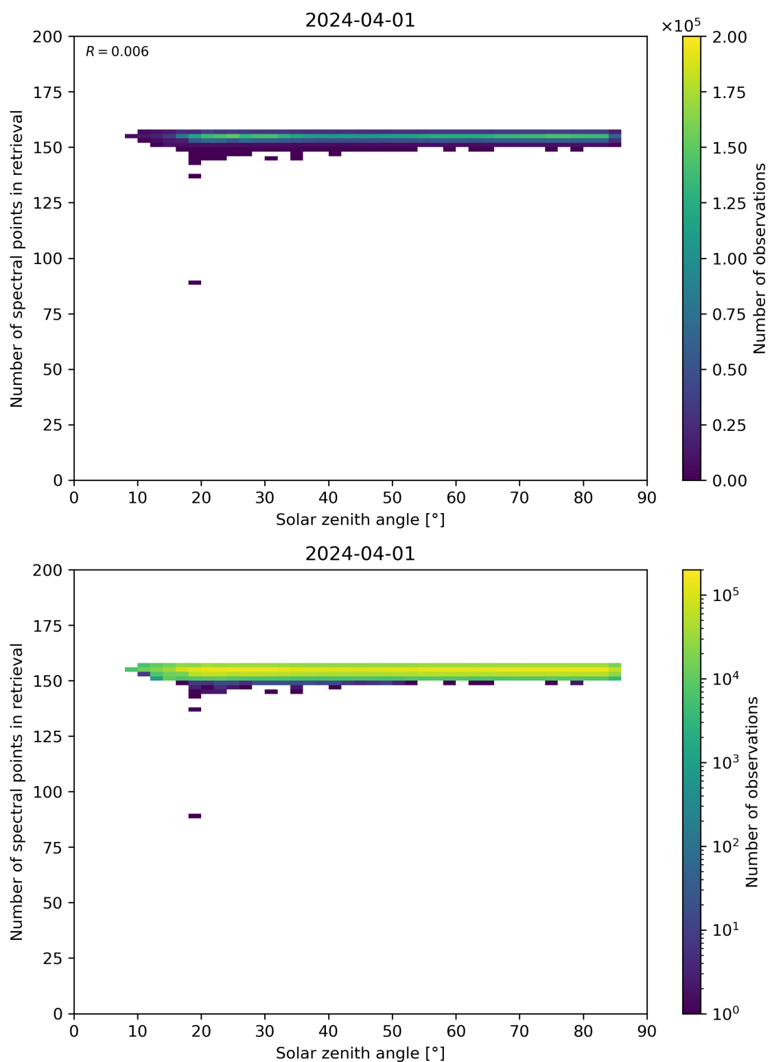
Figure 68: Scatter density plot of “Solar zenith angle” against “Number of spectral points in retrieval” for 2024-03-31 to 2024-04-02.
