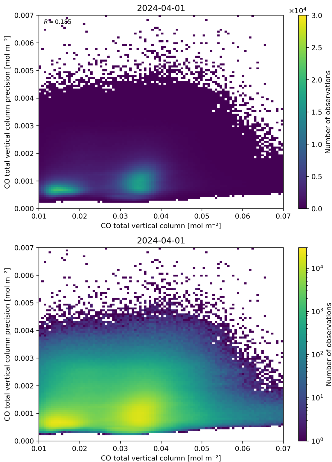
Figure 34: Scatter density plot of “CO total vertical column” against “CO total vertical column precision” for 2024-03-31 to 2024-04-02.
