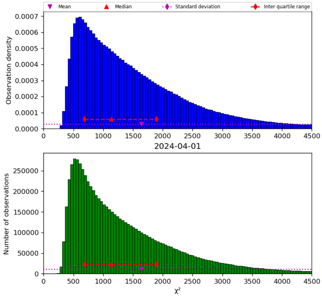
Figure 22: Histogram of “ \chi^2 ” for 2024-03-31 to 2024-04-02
