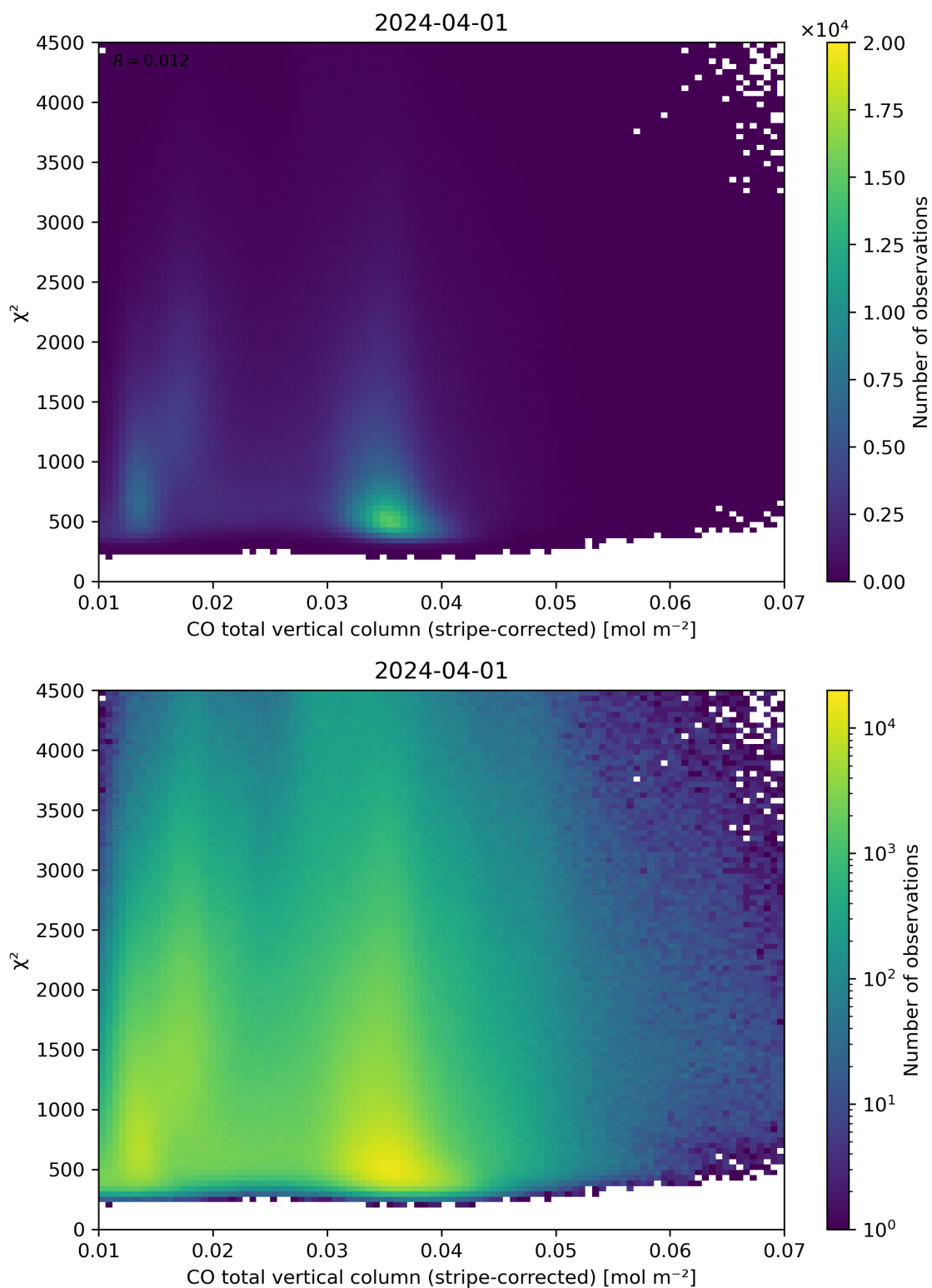
Figure 37: Scatter density plot of “CO total vertical column (stripe-corrected)” against “ \chi^2 ” for 2024-03-31 to 2024-04-02.
