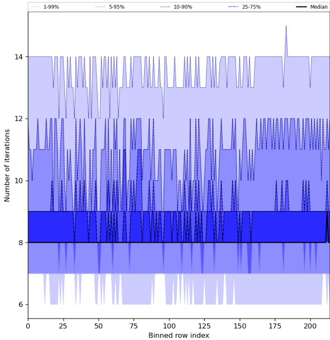
Figure 32: Along track statistics of “Number of iterations” for 2024-03-31 to 2024-04-02
