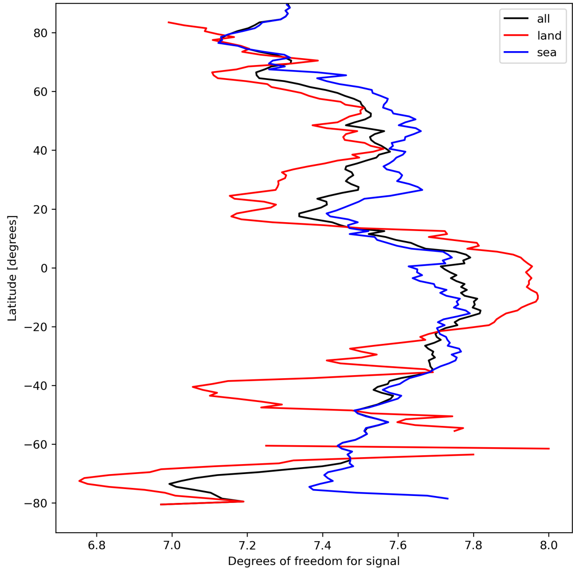
Figure 15: Zonal average of “Degrees of freedom for signal” for 2024-03-31 to 2024-04-02.
