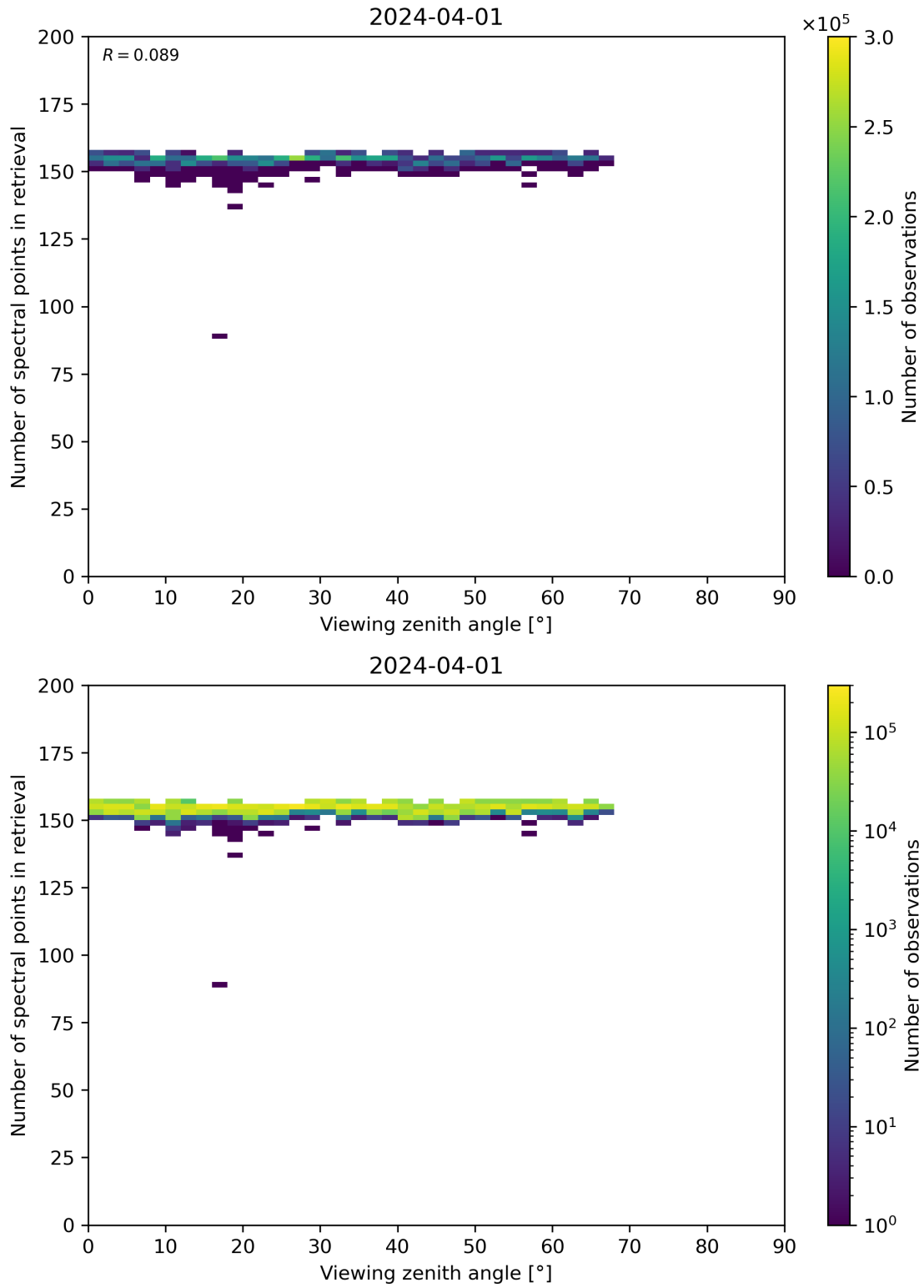
Figure 76: Scatter density plot of “Viewing zenith angle” against “Number of spectral points in retrieval” for 2024-03-31 to 2024-04-02.
