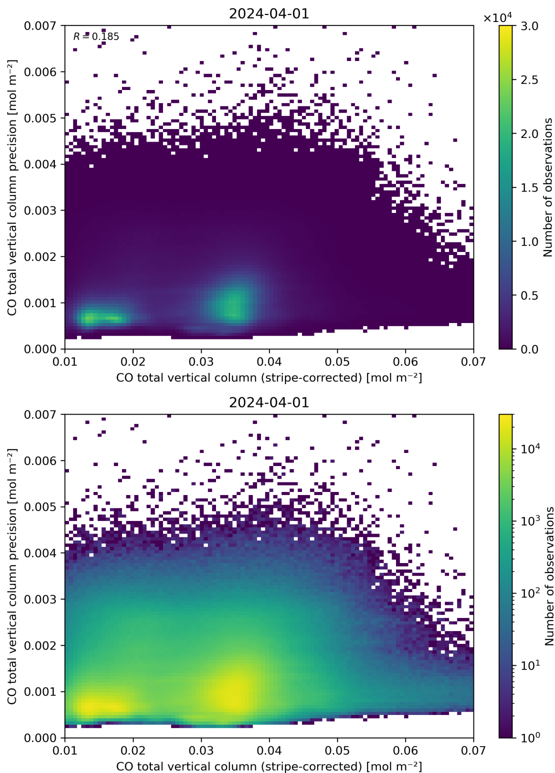
Figure 36: Scatter density plot of “CO total vertical column (stripe-corrected)” against “CO total vertical column precision” for 2024-03-31 to 2024-04-02.
