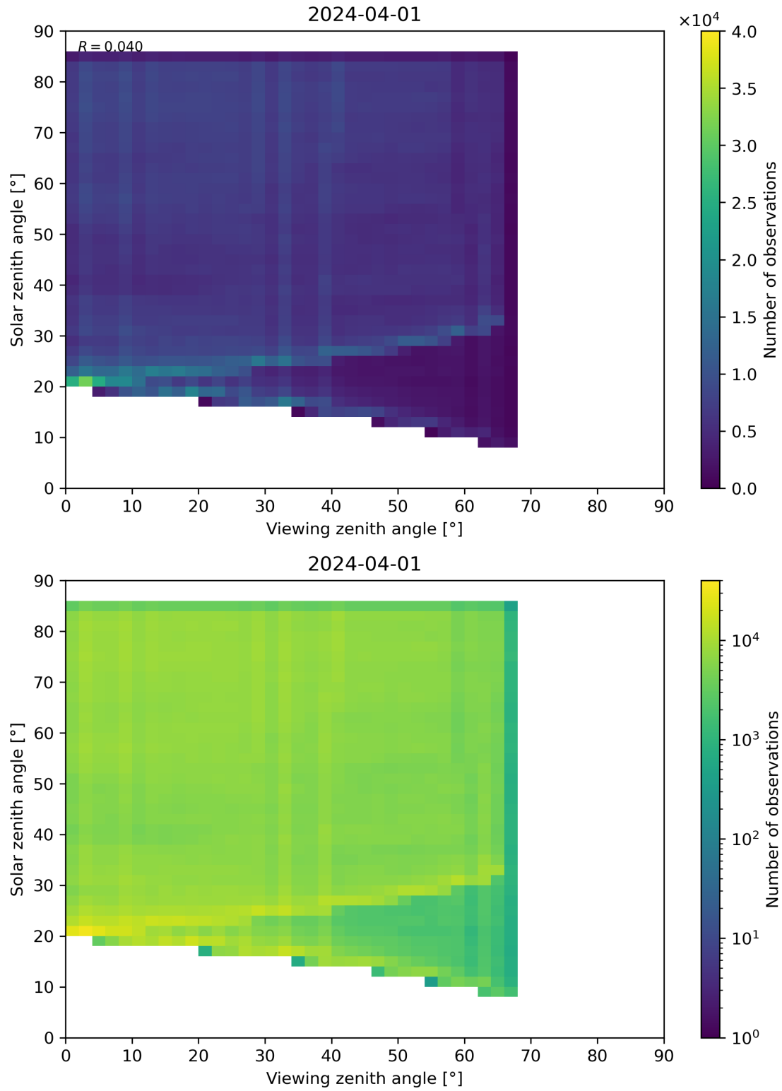
Figure 77: Scatter density plot of “Viewing zenith angle” against “Solar zenith angle” for 2024-03-31 to 2024-04-02.
