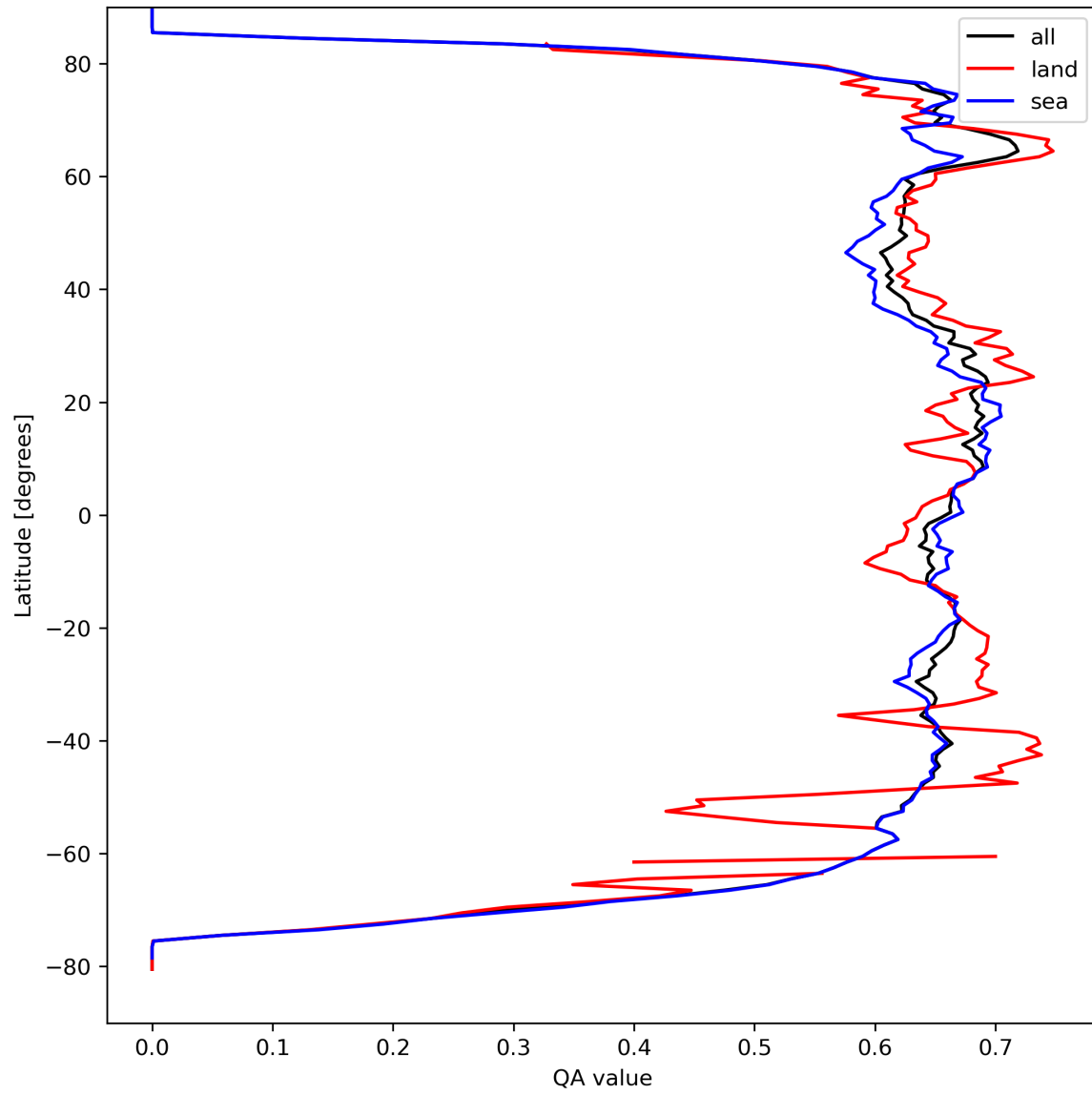
Figure 9: Zonal average of “QA value” for 2024-03-31 to 2024-04-02.
