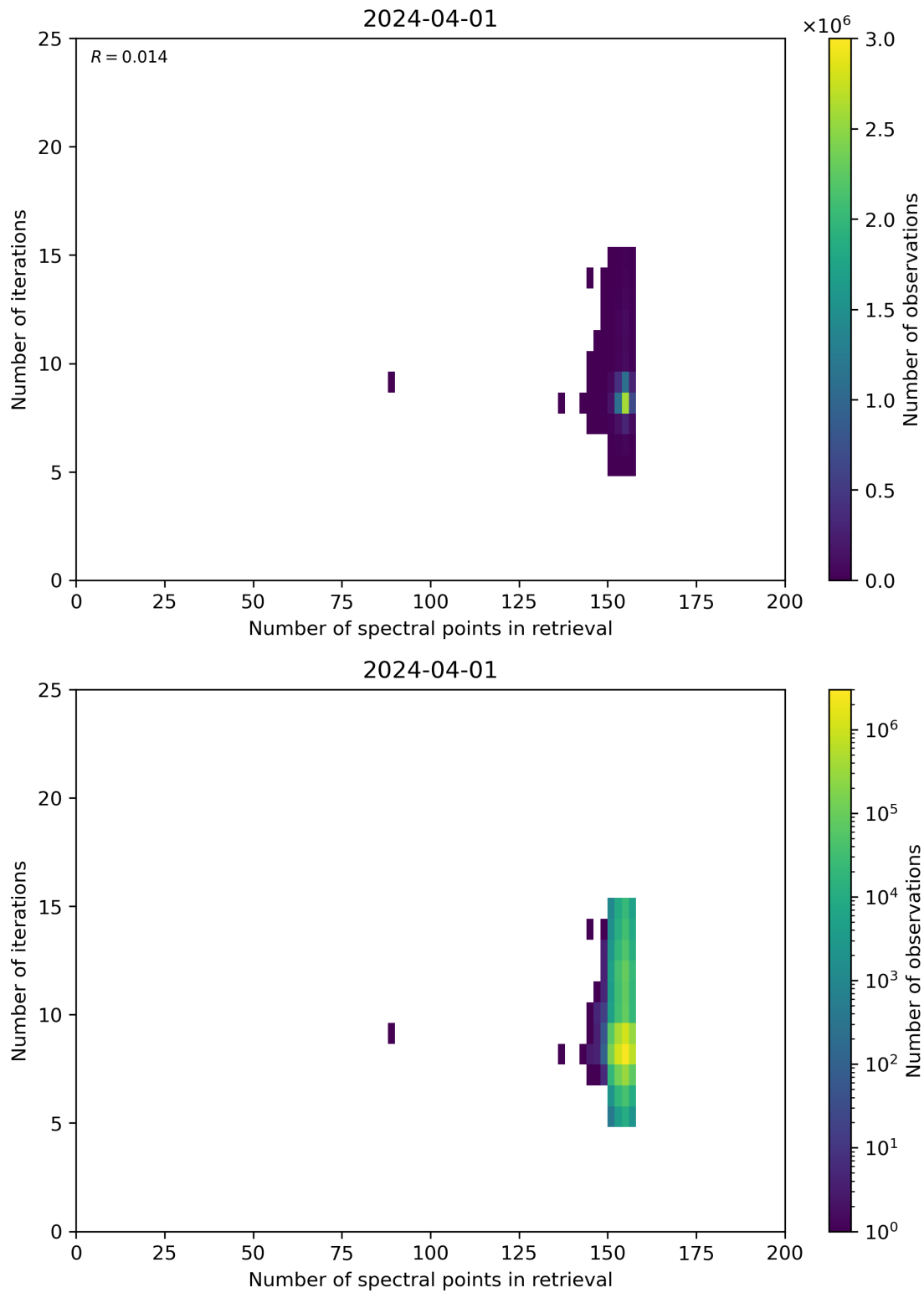
Figure 60: Scatter density plot of “Number of spectral points in retrieval” against “Number of iterations” for 2024-03-31 to 2024-04-02.
