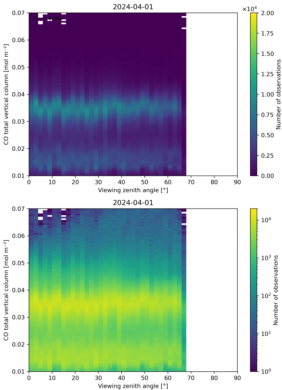
Figure 69: Scatter density plot of “Viewing zenith angle” against “CO total vertical column” for 2024-03-31 to 2024-04-02.
