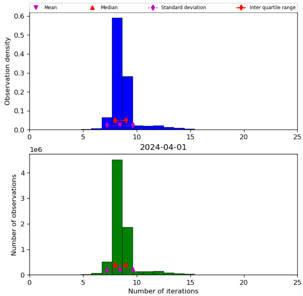
Figure 24: Histogram of “Number of iterations” for 2024-03-31 to 2024-04-02
