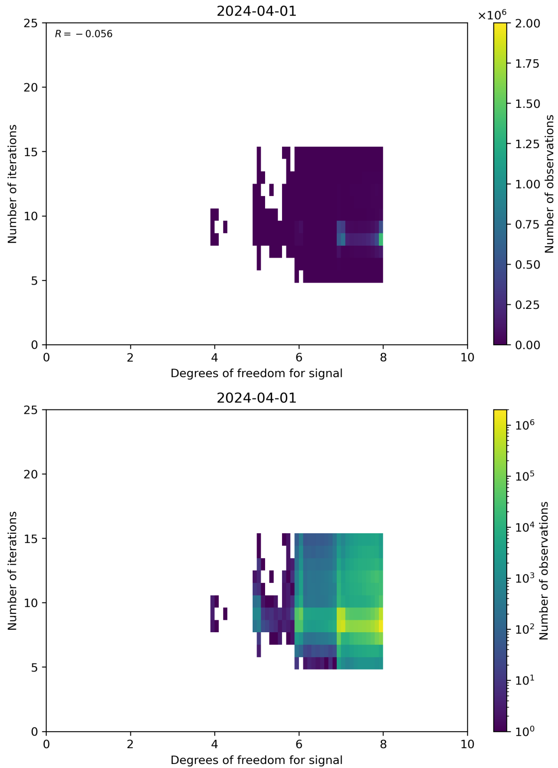
Figure 50: Scatter density plot of “Degrees of freedom for signal” against “Number of iterations” for 2024-03-31 to 2024-04-02.
