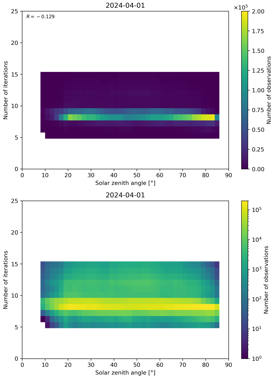
Figure 67: Scatter density plot of “Solar zenith angle” against “Number of iterations” for 2024-03-31 to 2024-04-02.
