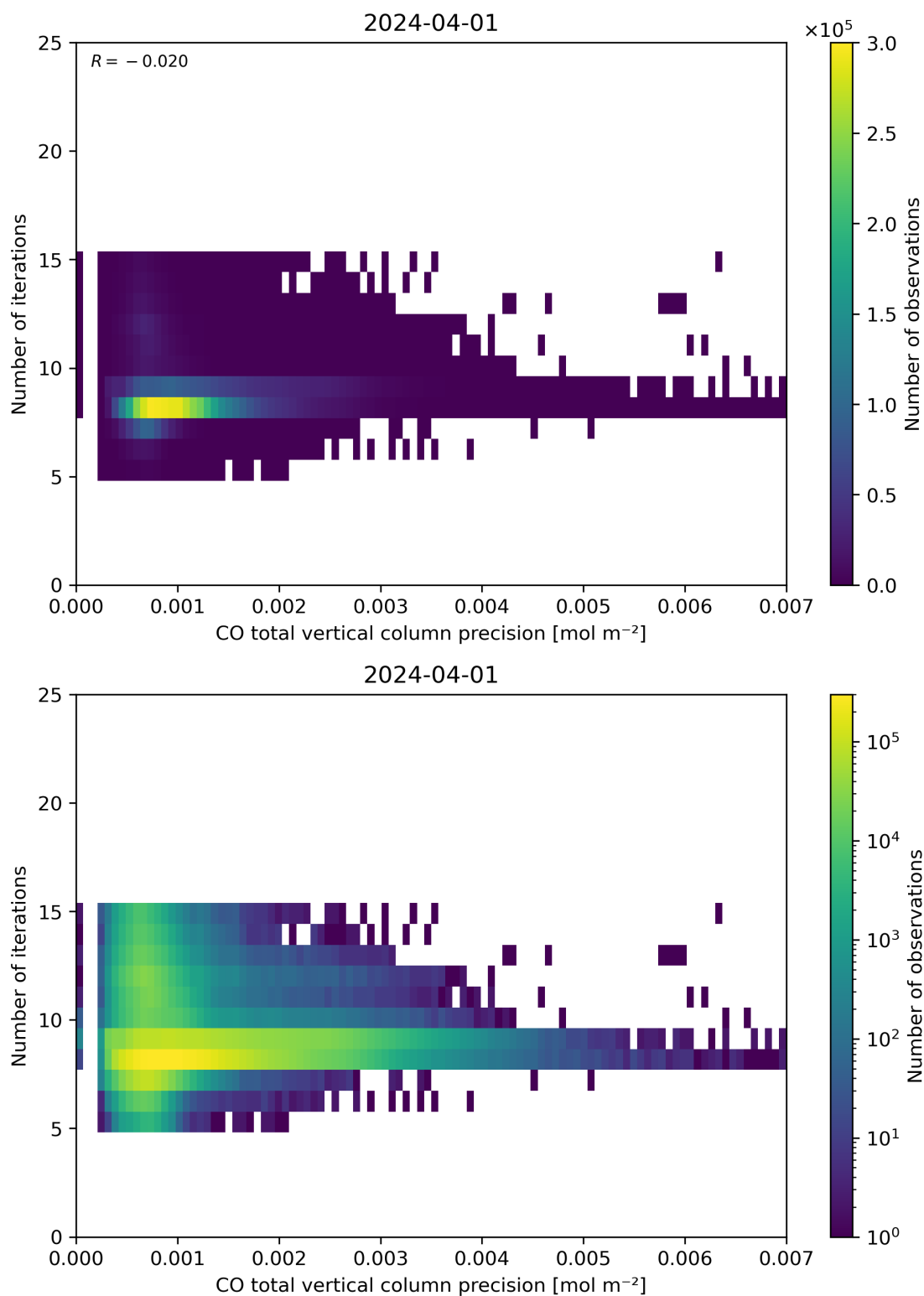
Figure 46: Scatter density plot of “CO total vertical column precision” against “Number of iterations” for 2024-03-31 to 2024-04-02.
