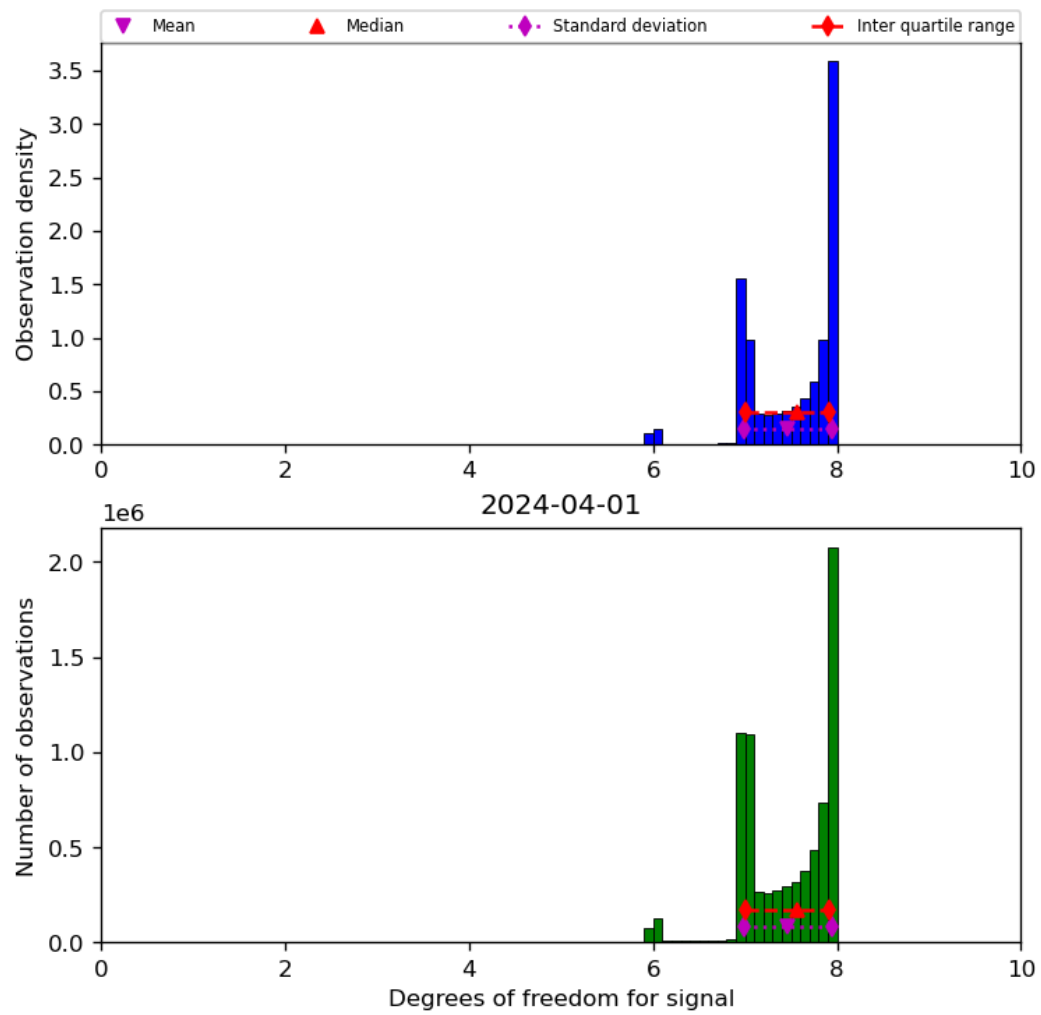
Figure 23: Histogram of “Degrees of freedom for signal” for 2024-03-31 to 2024-04-02
