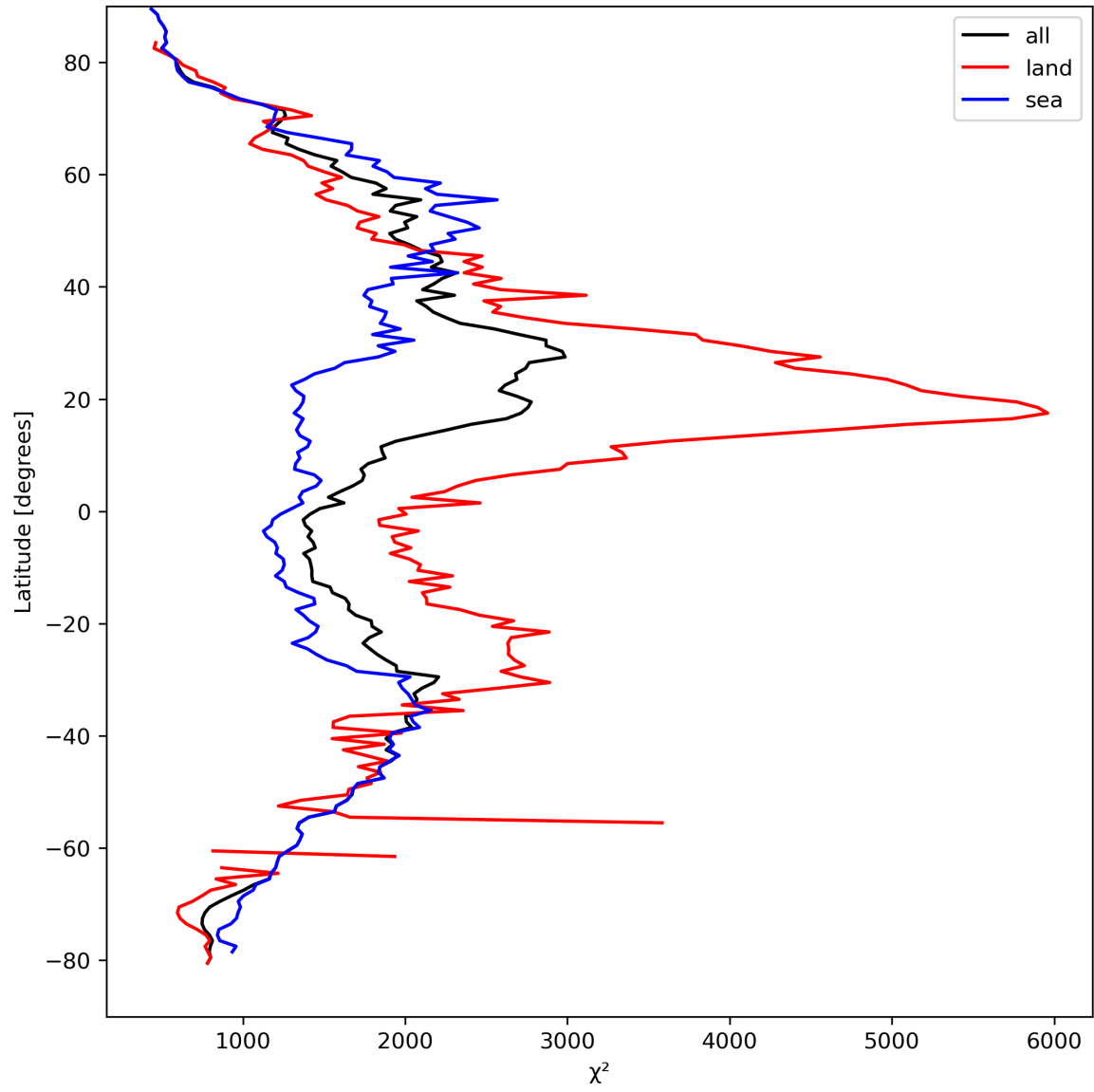
Figure 14: Zonal average of “ \chi^2 ” for 2024-03-31 to 2024-04-02.
