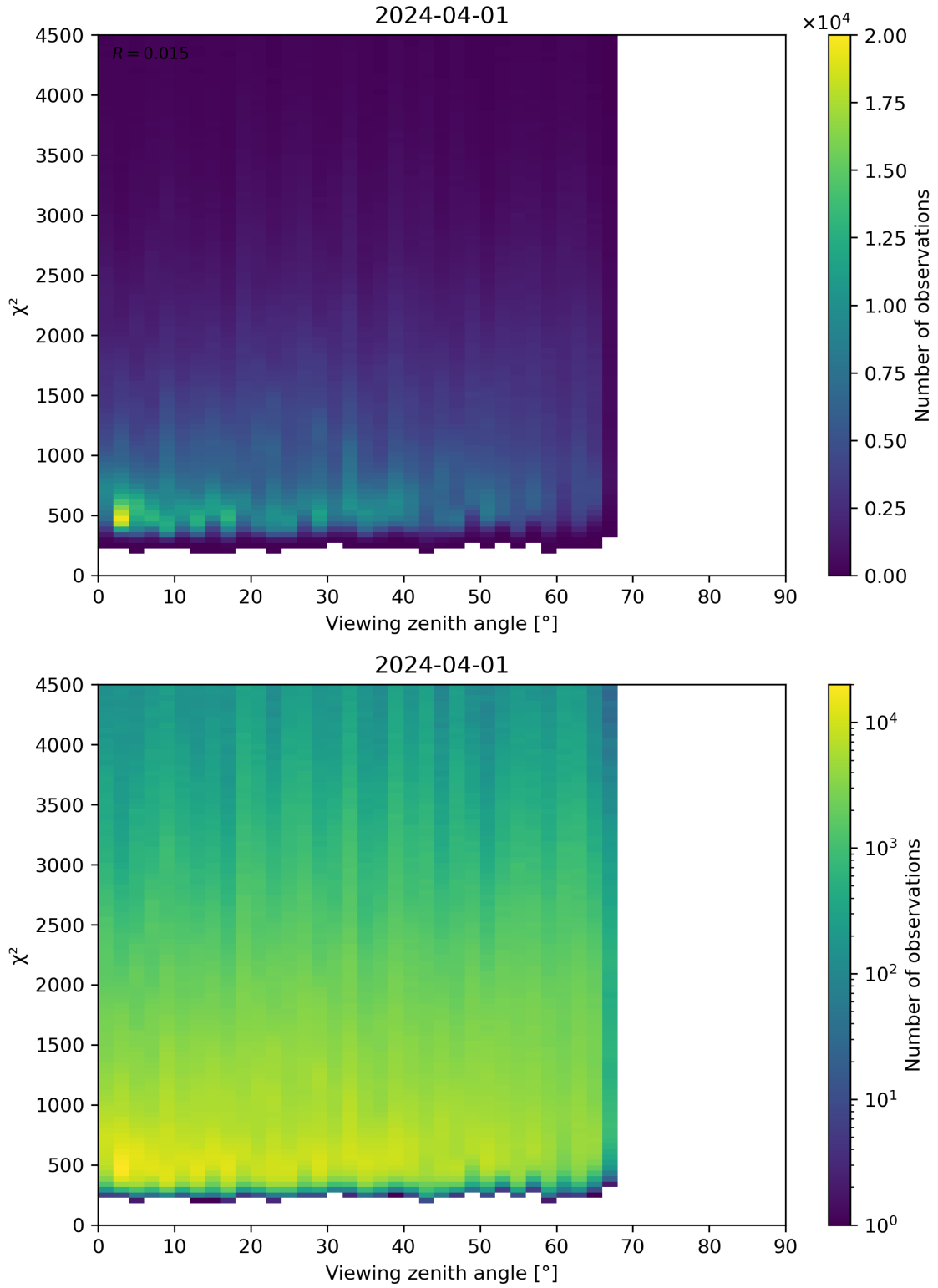
Figure 72: Scatter density plot of “Viewing zenith angle” against “ \chi^2 ” for 2024-03-31 to 2024-04-02.
