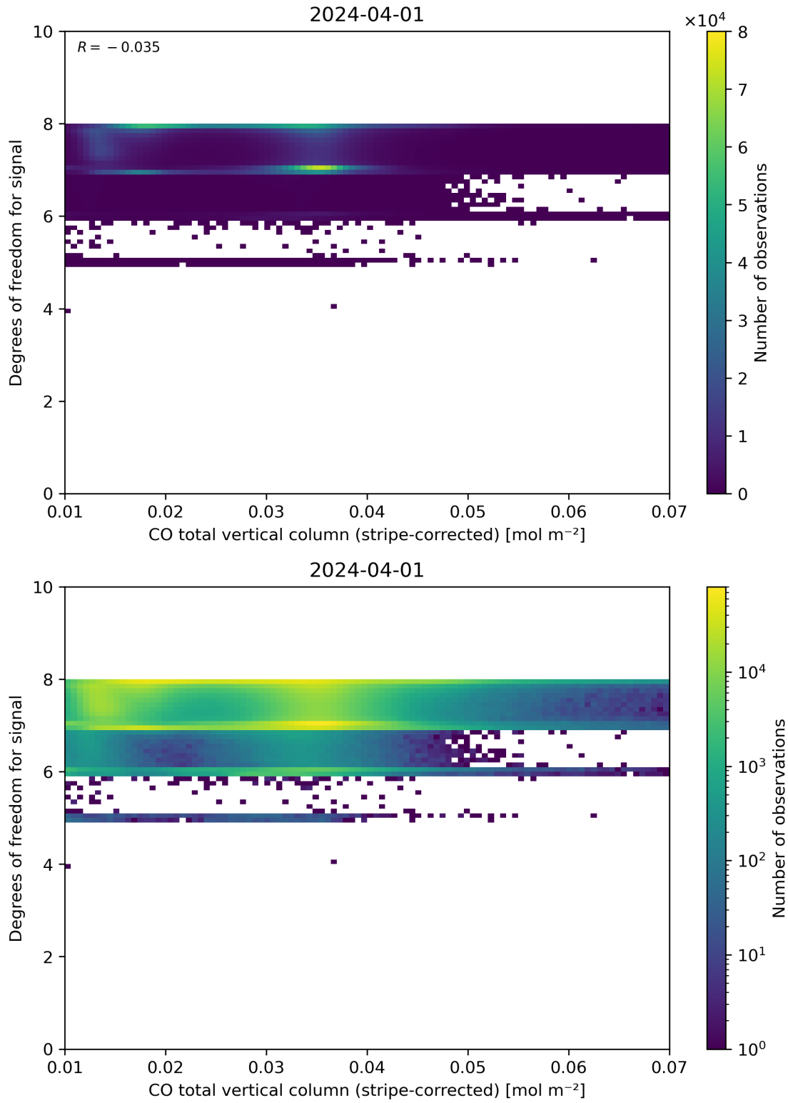
Figure 38: Scatter density plot of “CO total vertical column (stripe-corrected)” against “Degrees of freedom for signal” for 2024-03-31 to 2024-04-02.
