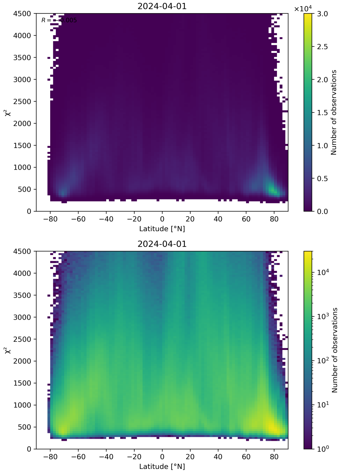
Figure 54: Scatter density plot of “Latitude” against “ \chi^2 ” for 2024-03-31 to 2024-04-02.
