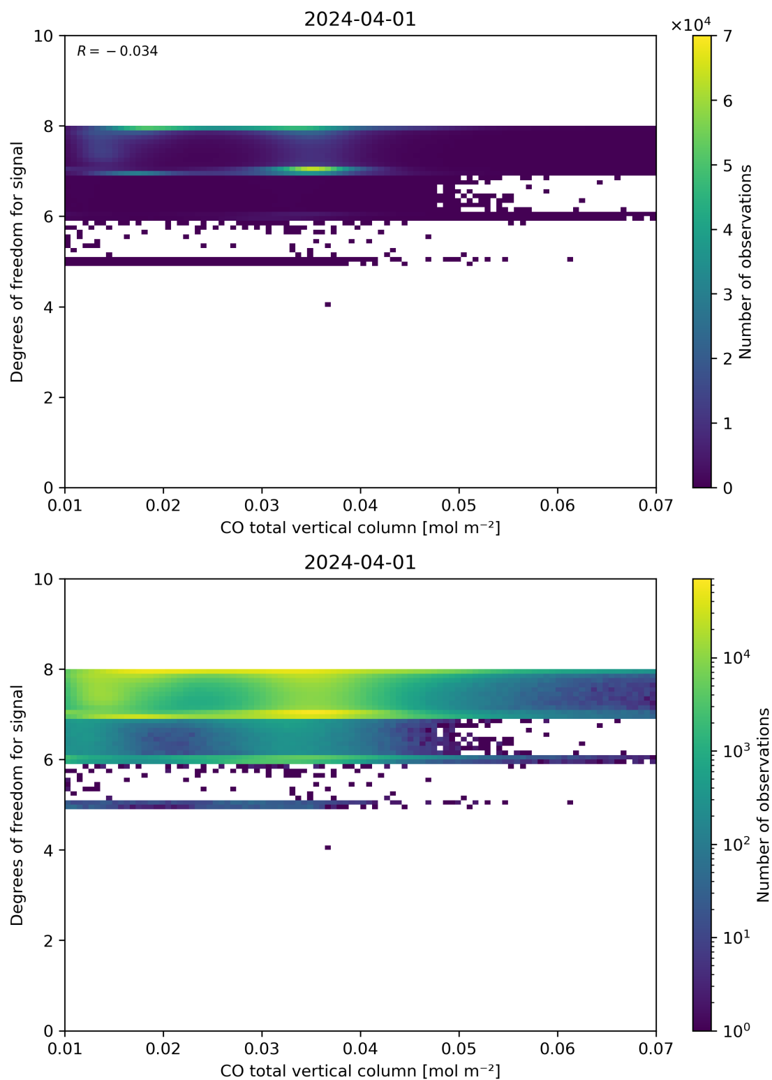
Figure 41: Scatter density plot of “CO total vertical column” against “Degrees of freedom for signal” for 2024-03-31 to 2024-04-02.
