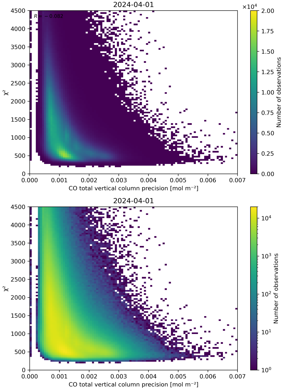
Figure 44: Scatter density plot of “CO total vertical column precision” against “ \chi^2 ” for 2024-03-31 to 2024-04-02.
