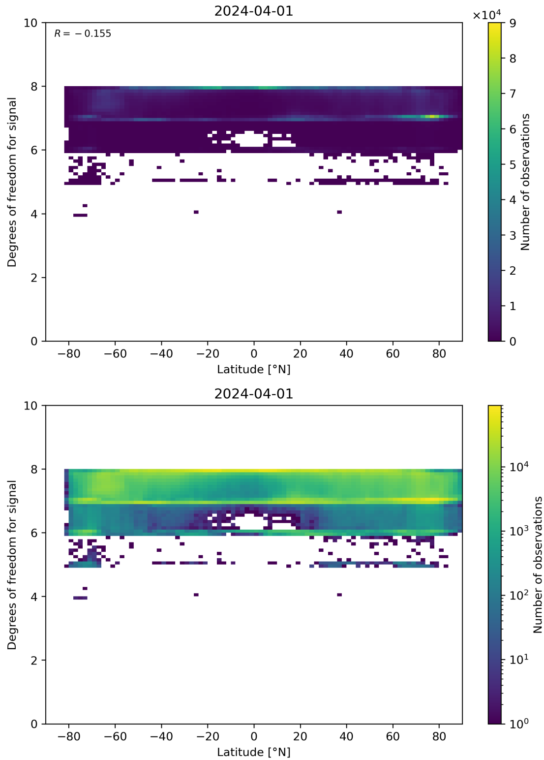
Figure 55: Scatter density plot of “Latitude” against “Degrees of freedom for signal” for 2024-03-31 to 2024-04-02.
