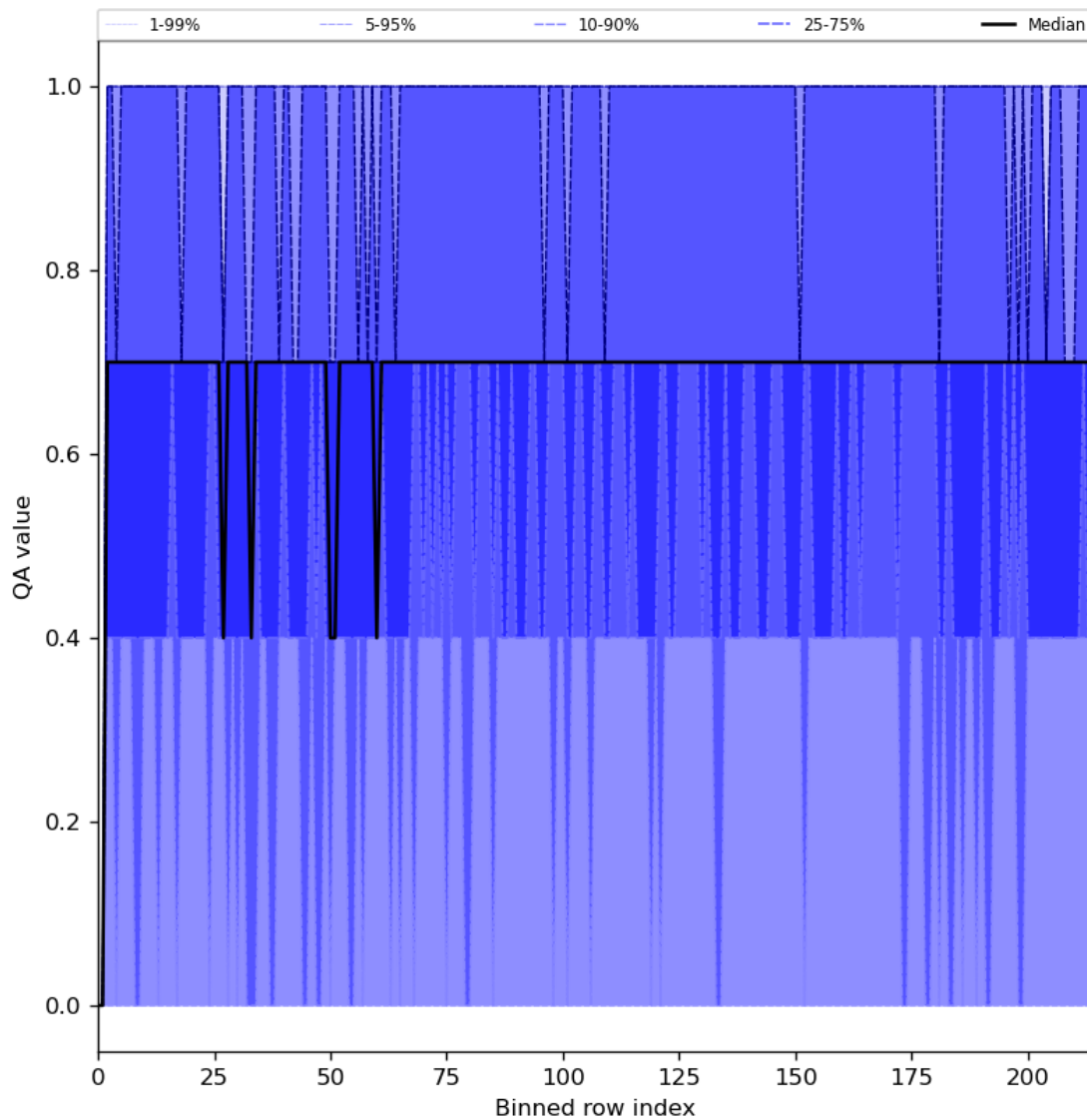
Figure 25: Along track statistics of “QA value” for 2024-03-31 to 2024-04-02
