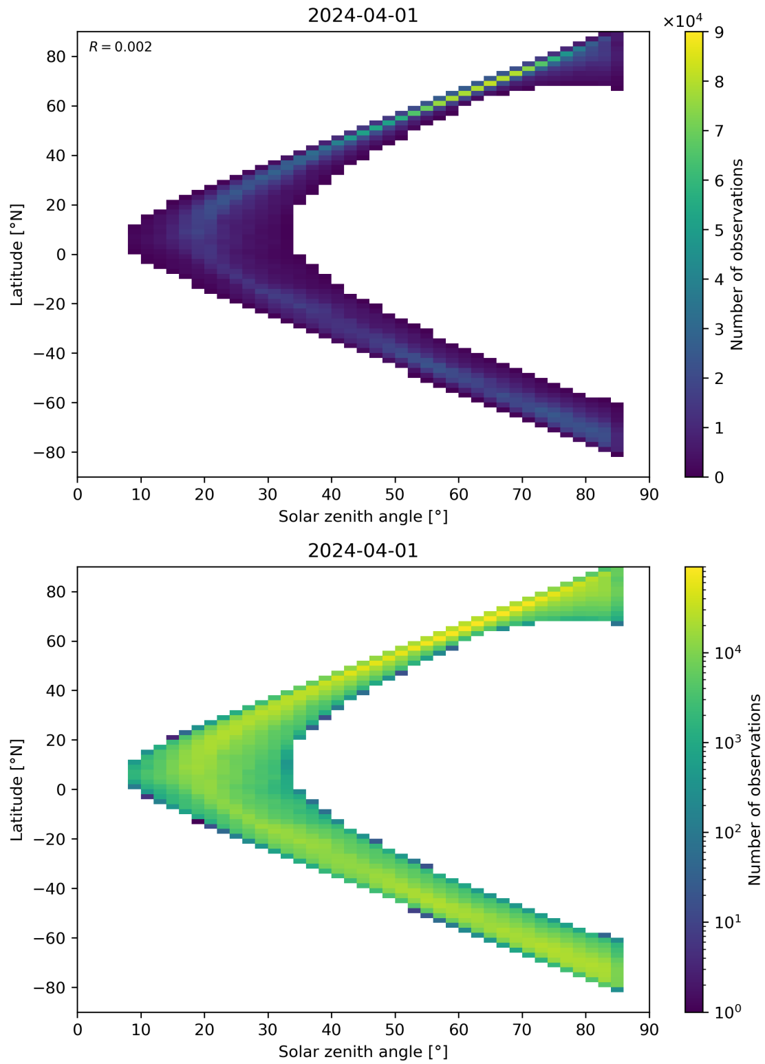
Figure 66: Scatter density plot of “Solar zenith angle” against “Latitude” for 2024-03-31 to 2024-04-02.
