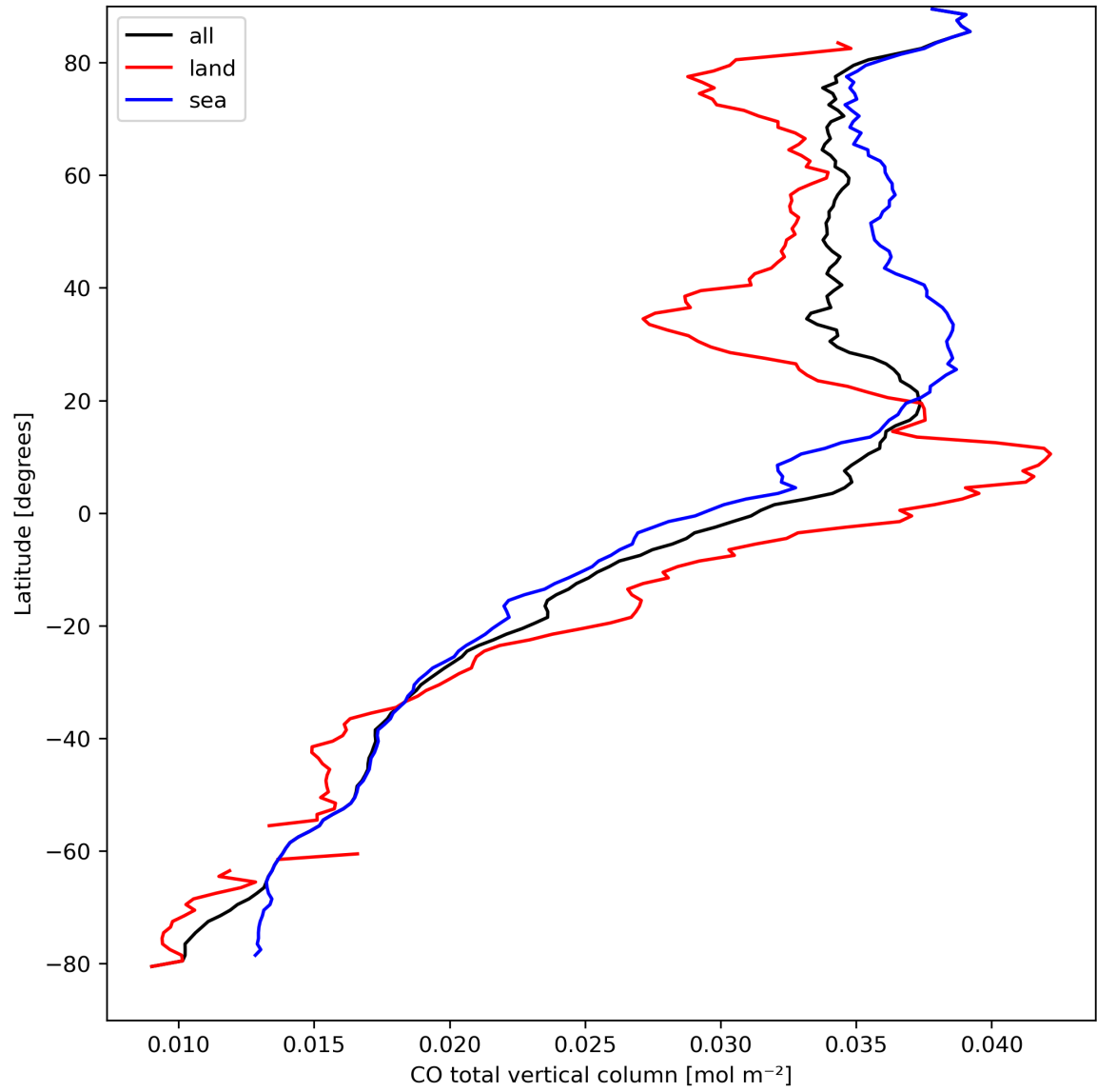
Figure 10: Zonal average of “CO total vertical column” for 2024-03-31 to 2024-04-02.
