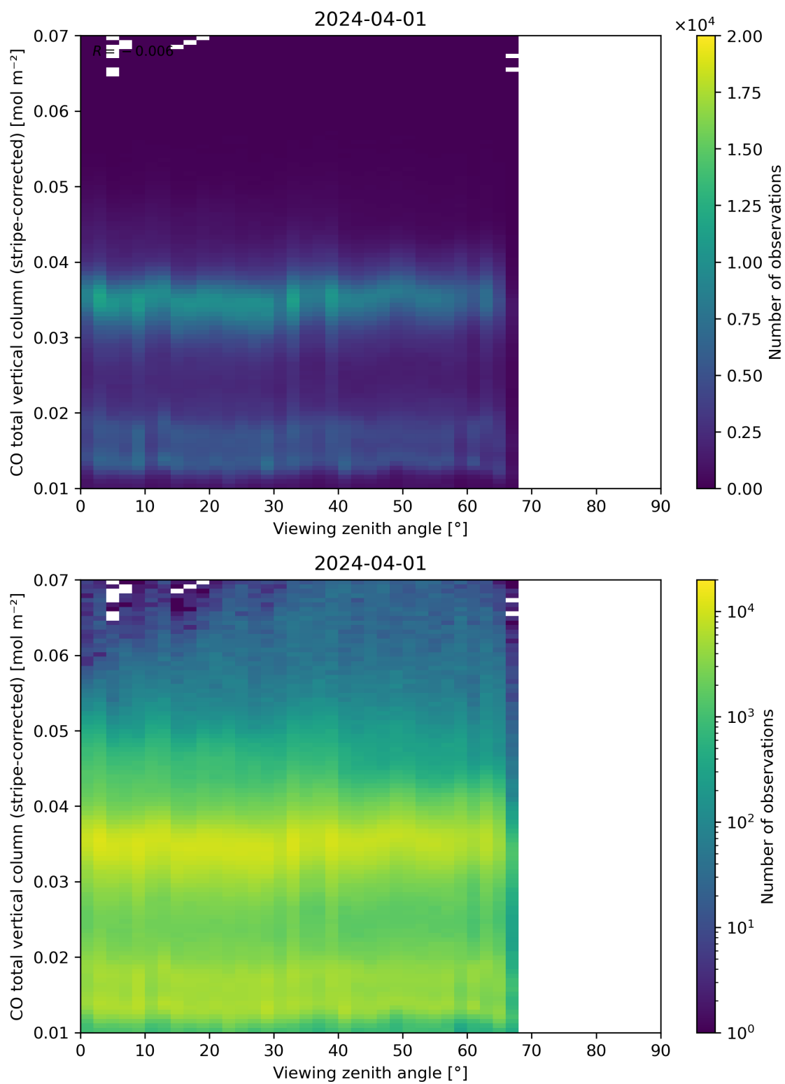
Figure 70: Scatter density plot of “Viewing zenith angle” against “CO total vertical column (stripe-corrected)” for 2024-03-31 to 2024-04-02.
