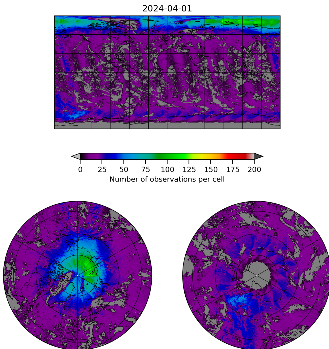
Figure 8: Map of the number of observations for 2024-03-31 to 2024-04-02
