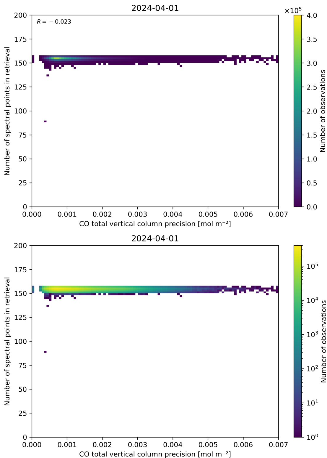
Figure 47: Scatter density plot of “CO total vertical column precision” against “Number of spectral points in retrieval” for 2024-03-31 to 2024-04-02.
