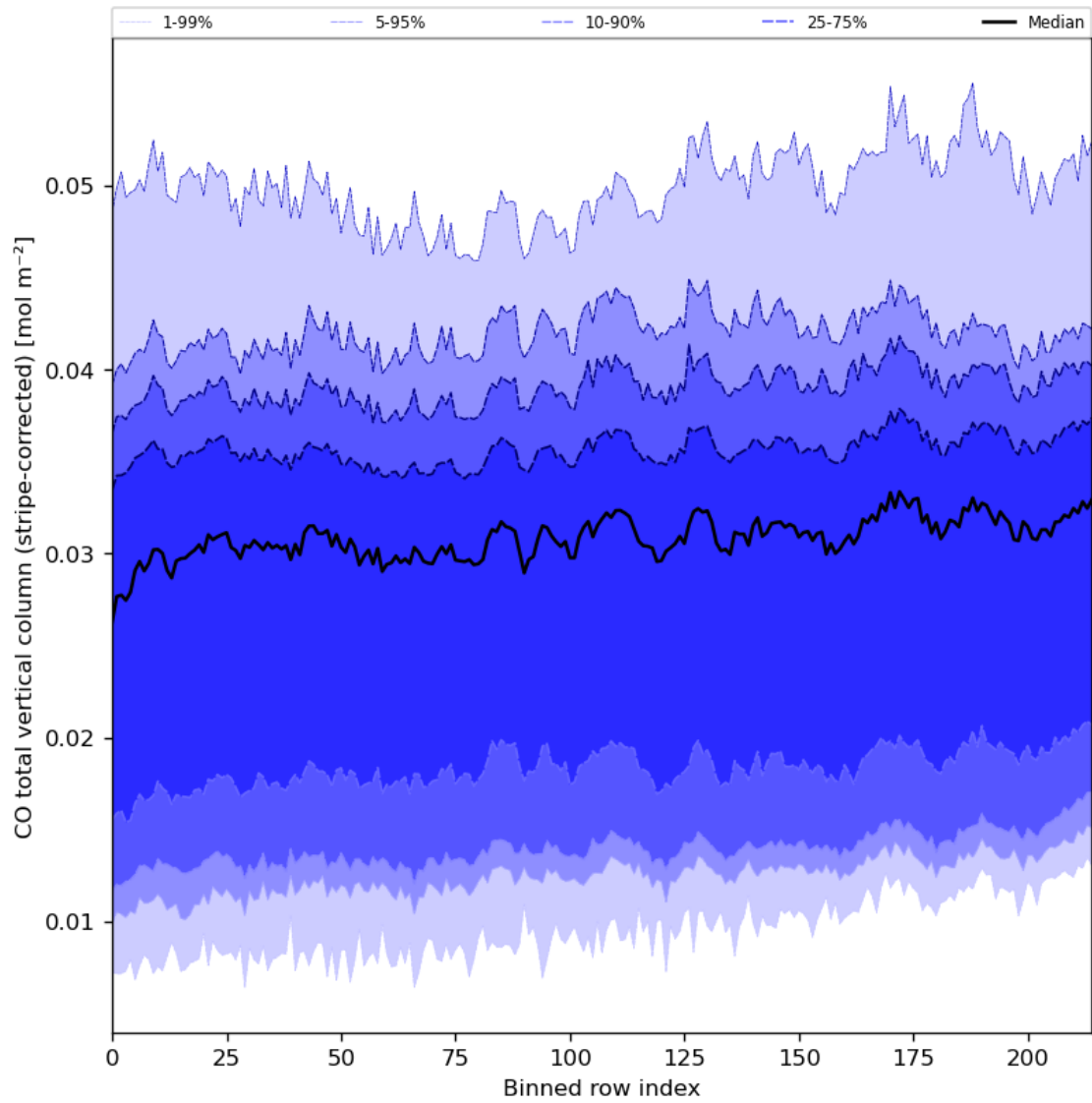
Figure 27: Along track statistics of “CO total vertical column (stripe-corrected)” for 2024-03-31 to 2024-04-02
