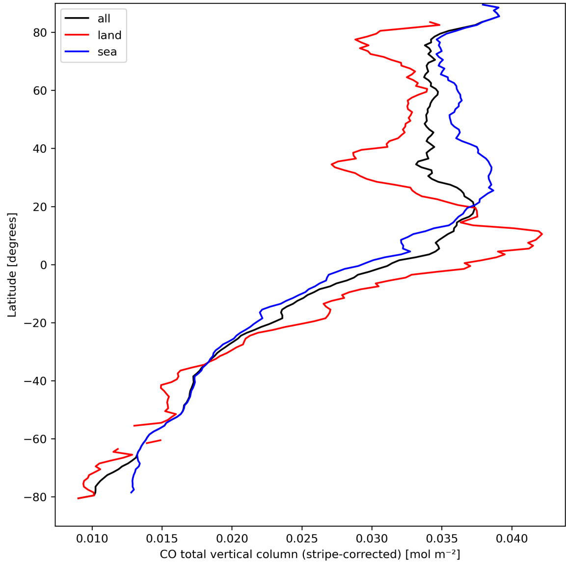
Figure 11: Zonal average of “CO total vertical column (stripe-corrected)” for 2024-03-31 to 2024-04-02.
