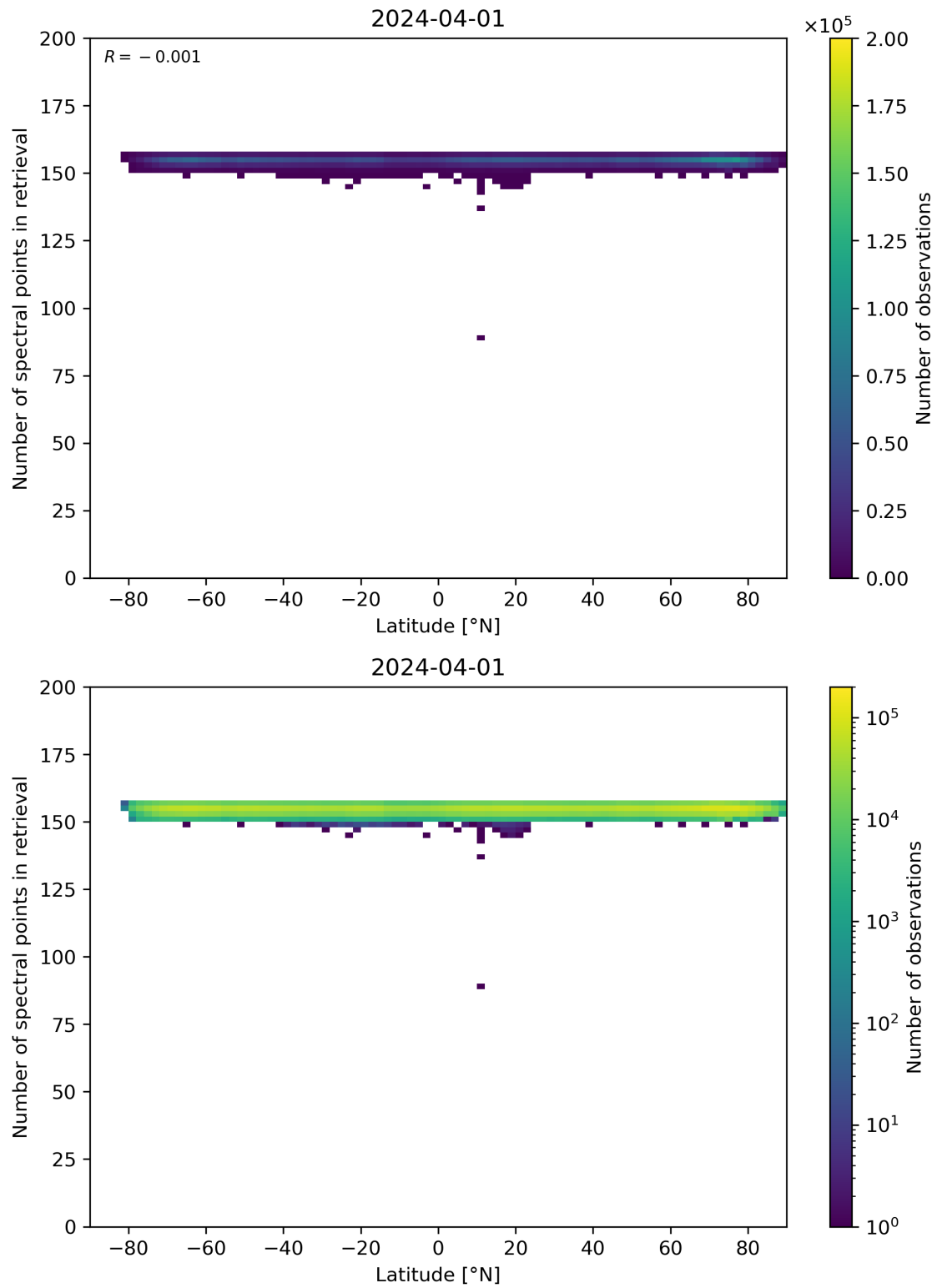
Figure 57: Scatter density plot of “Latitude” against “Number of spectral points in retrieval” for 2024-03-31 to 2024-04-02.
