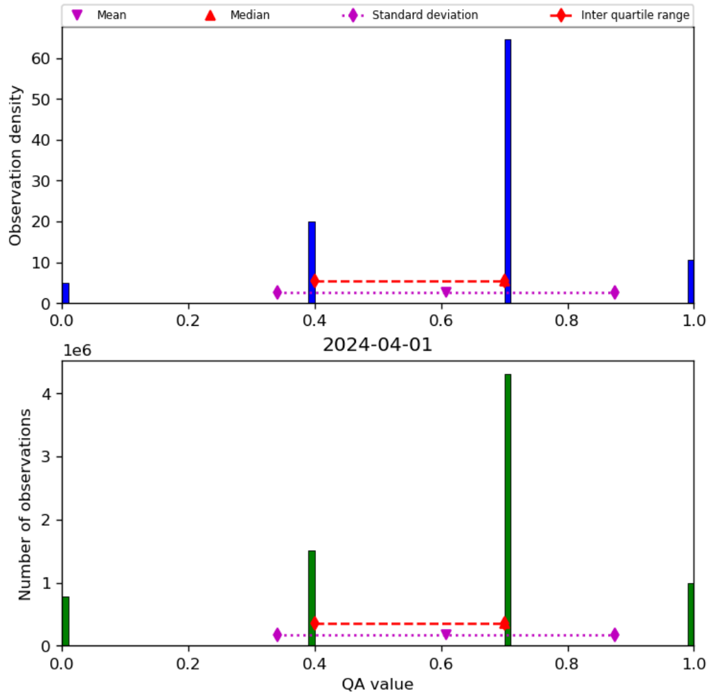
Figure 17: Histogram of “QA value” for 2024-03-31 to 2024-04-02
