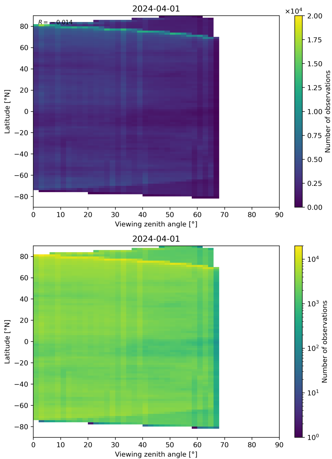
Figure 74: Scatter density plot of “Viewing zenith angle” against “Latitude” for 2024-03-31 to 2024-04-02.
