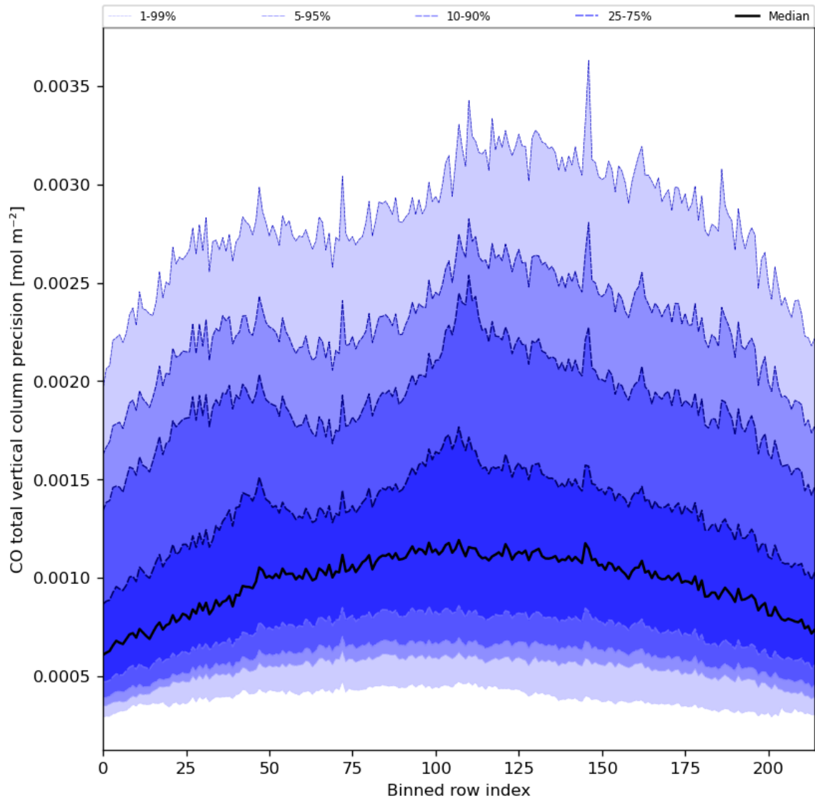
Figure 28: Along track statistics of “CO total vertical column precision” for 2024-03-31 to 2024-04-02
