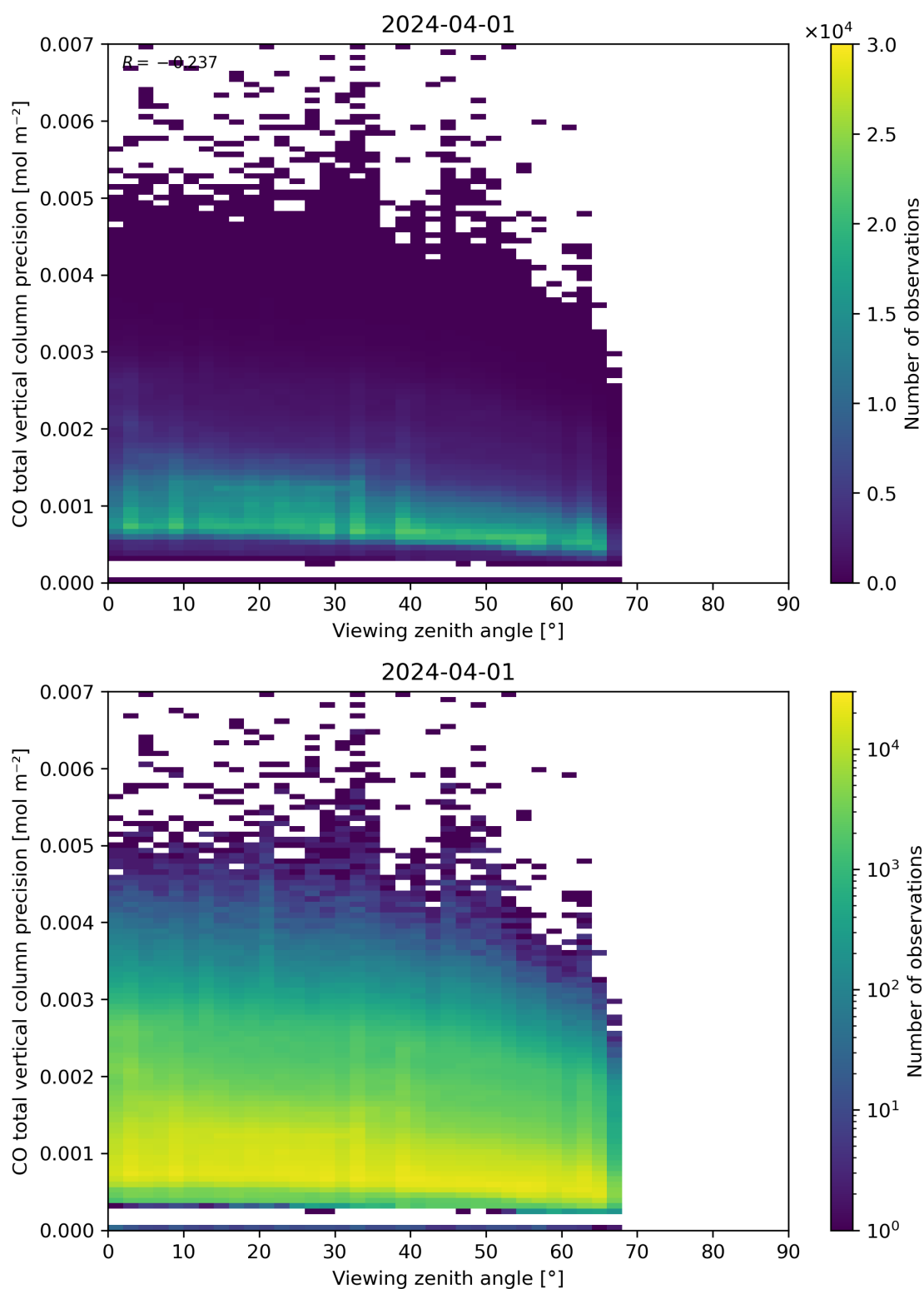
Figure 71: Scatter density plot of “Viewing zenith angle” against “CO total vertical column precision” for 2024-03-31 to 2024-04-02.
