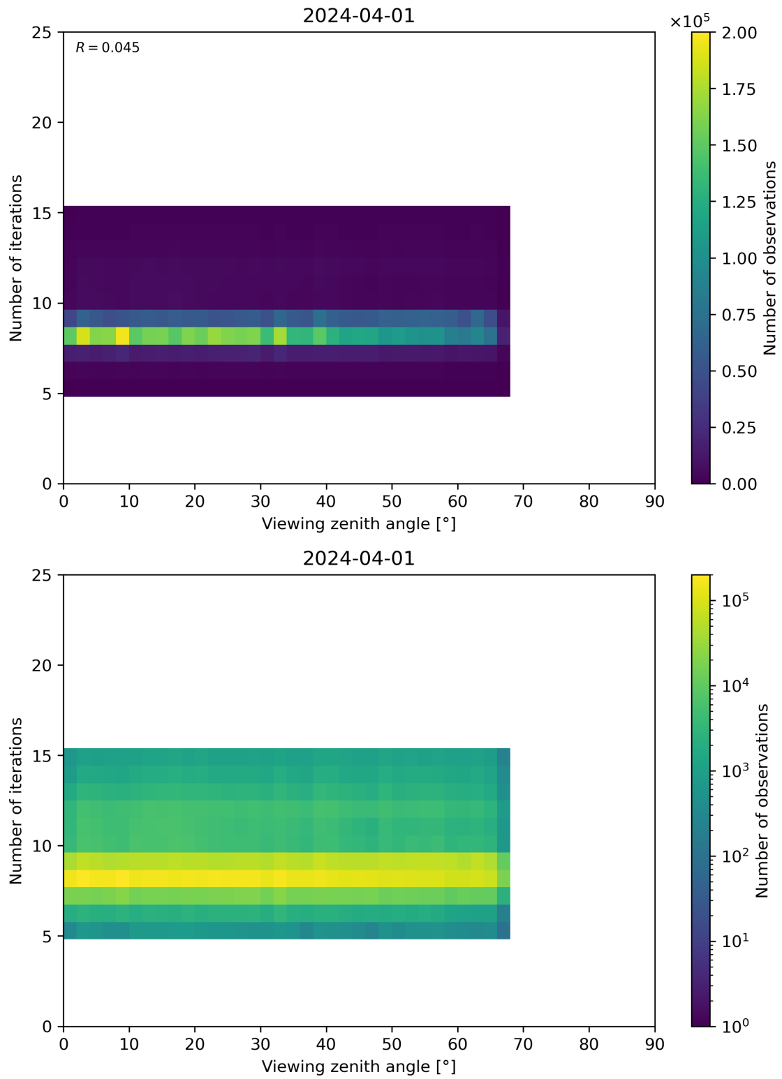
Figure 75: Scatter density plot of “Viewing zenith angle” against “Number of iterations” for 2024-03-31 to 2024-04-02.
