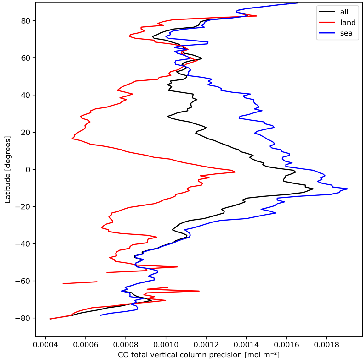
Figure 12: Zonal average of “CO total vertical column precision” for 2024-03-31 to 2024-04-02.
