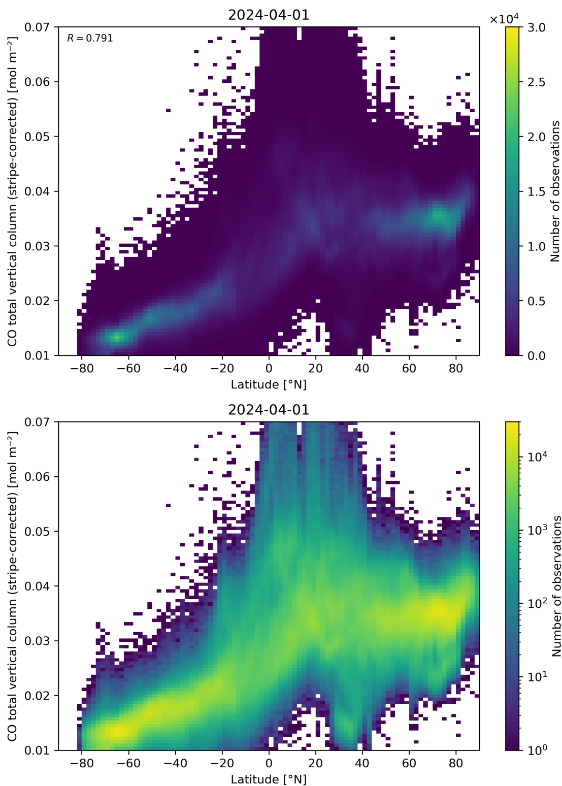
Figure 52: Scatter density plot of “Latitude” against “CO total vertical column (stripe-corrected)” for 2024-03-31 to 2024-04-02.
