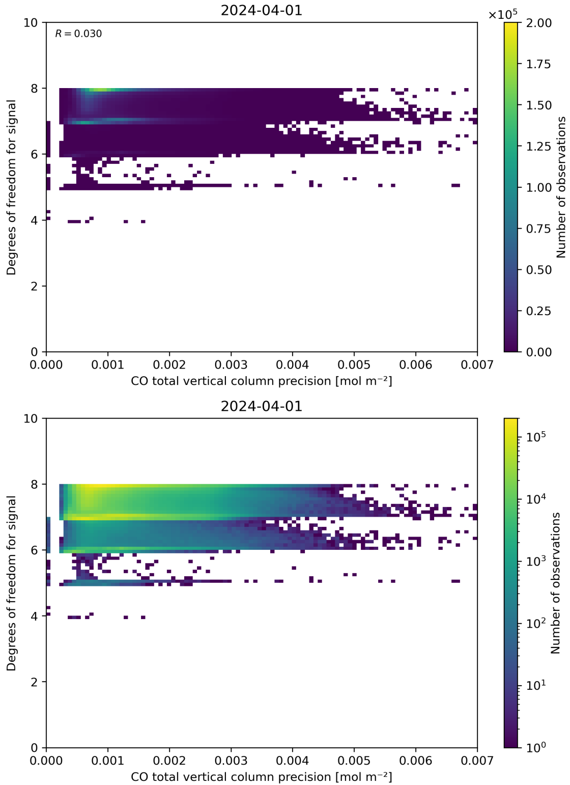
Figure 45: Scatter density plot of “CO total vertical column precision” against “Degrees of freedom for signal” for 2024-03-31 to 2024-04-02.
