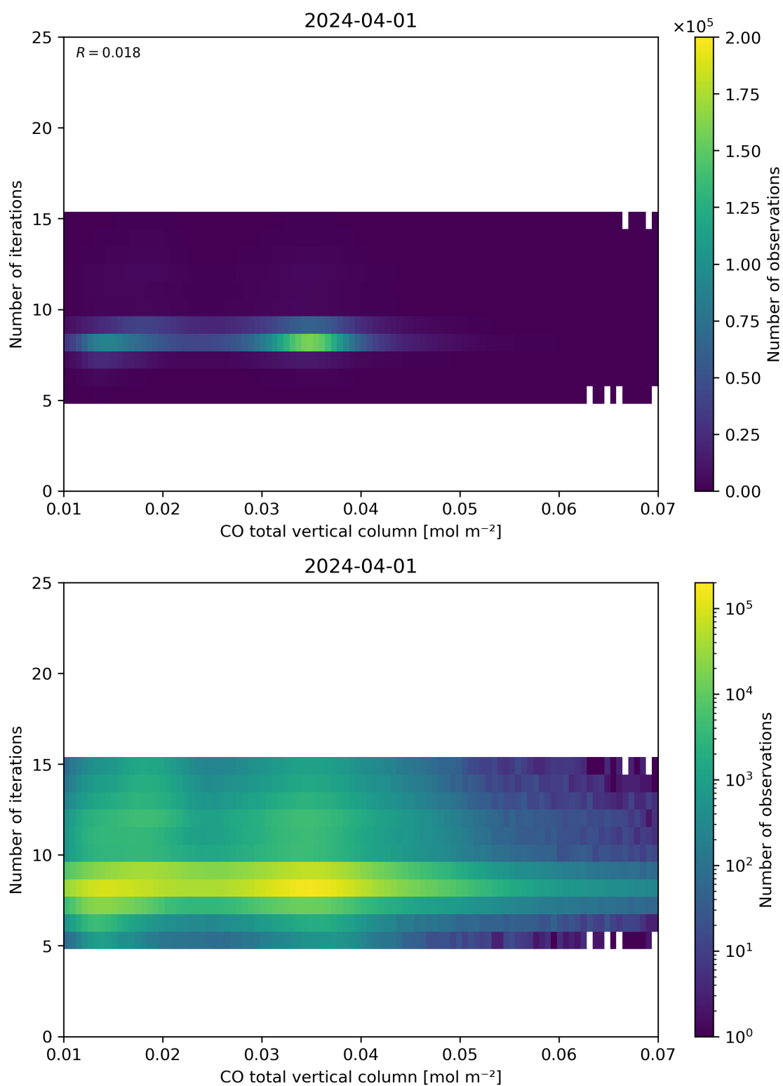
Figure 42: Scatter density plot of “CO total vertical column” against “Number of iterations” for 2024-03-31 to 2024-04-02.
