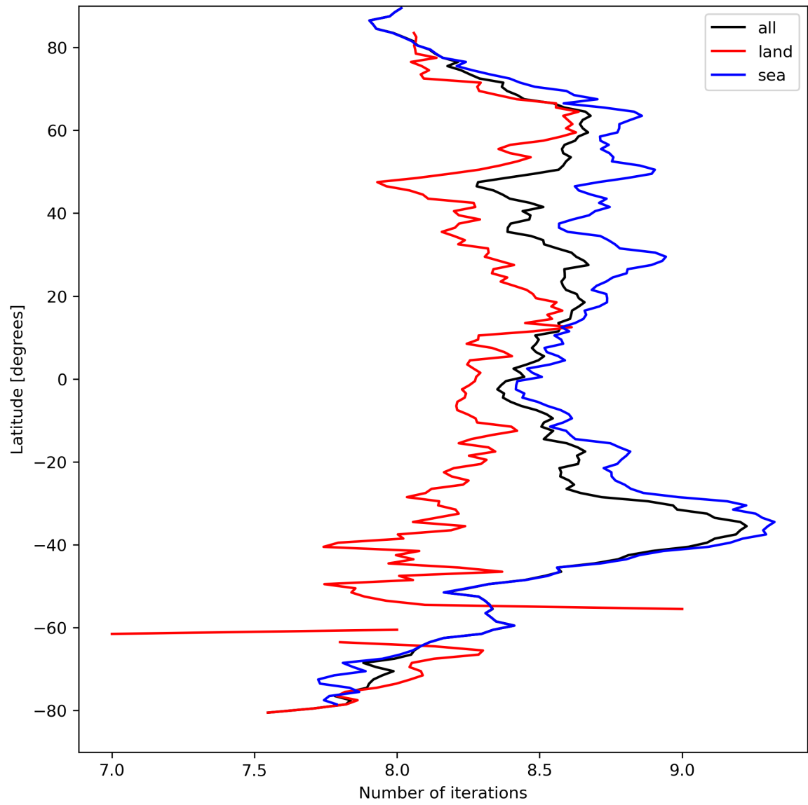
Figure 16: Zonal average of “Number of iterations” for 2024-03-31 to 2024-04-02.
