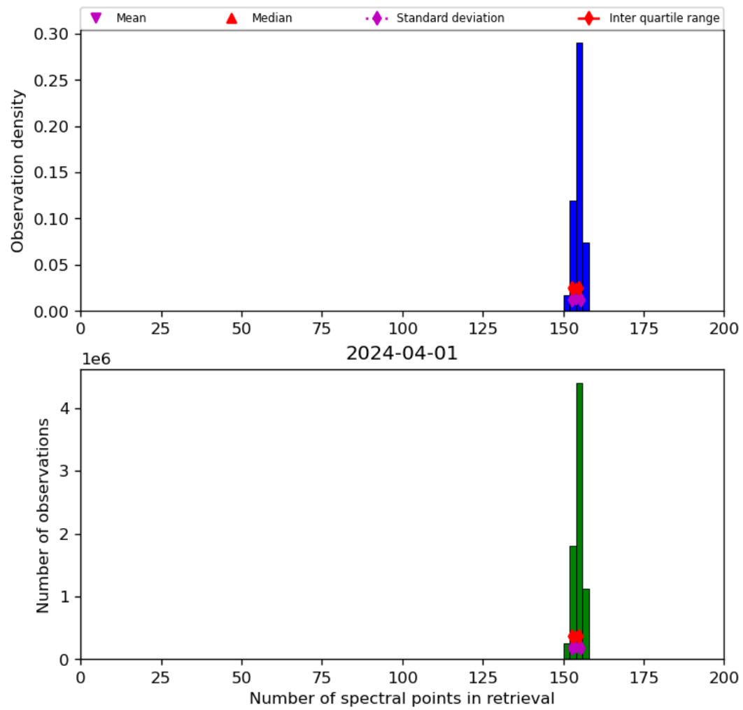
Figure 21: Histogram of “Number of spectral points in retrieval” for 2024-03-31 to 2024-04-02
