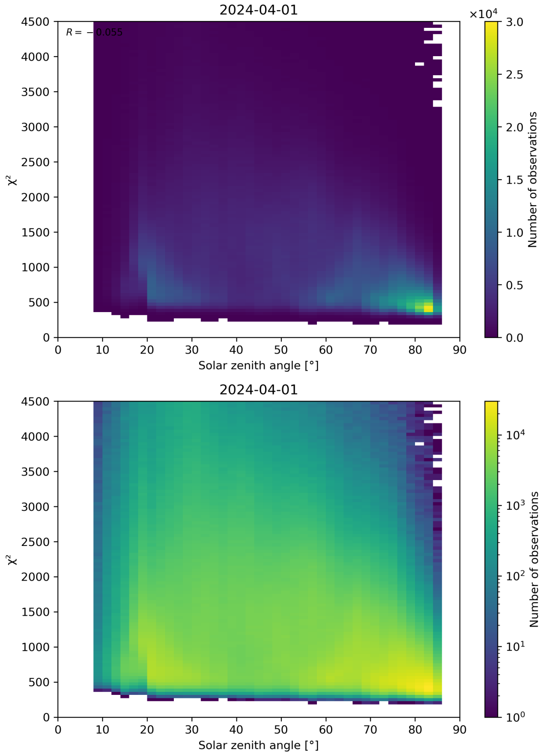
Figure 64: Scatter density plot of “Solar zenith angle” against “ \chi^2 ” for 2024-03-31 to 2024-04-02.
