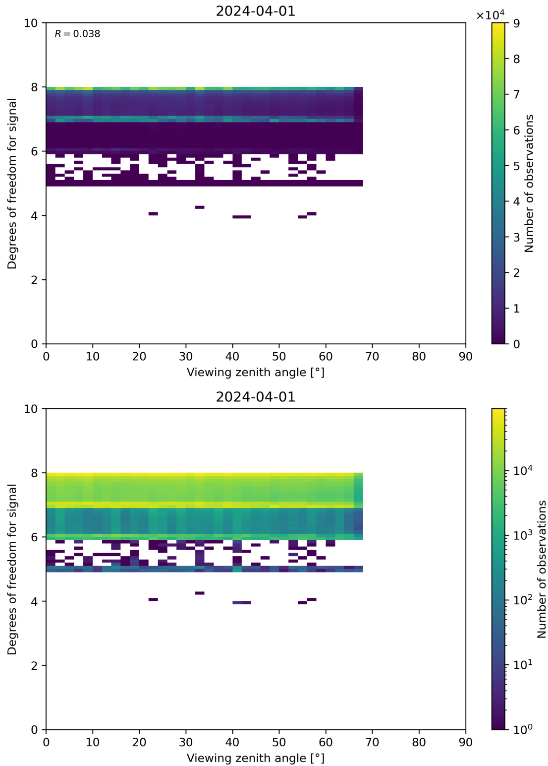
Figure 73: Scatter density plot of “Viewing zenith angle” against “Degrees of freedom for signal” for 2024-03-31 to 2024-04-02.
