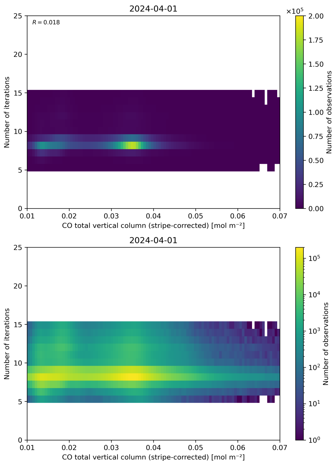
Figure 39: Scatter density plot of “CO total vertical column (stripe-corrected)” against “Number of iterations” for 2024-03-31 to 2024-04-02.
