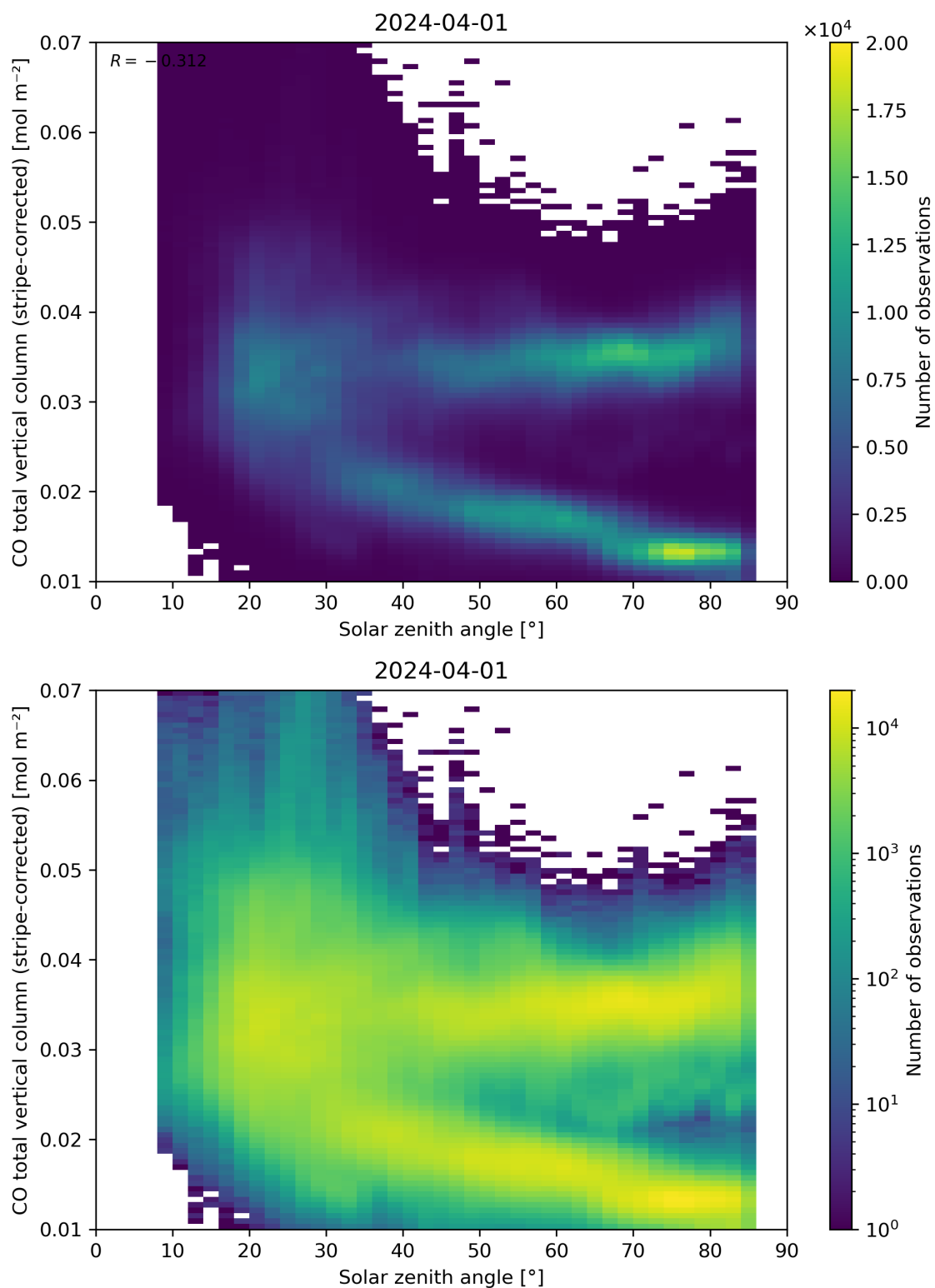
Figure 62: Scatter density plot of “Solar zenith angle” against “CO total vertical column (stripe-corrected)” for 2024-03-31 to 2024-04-02.
