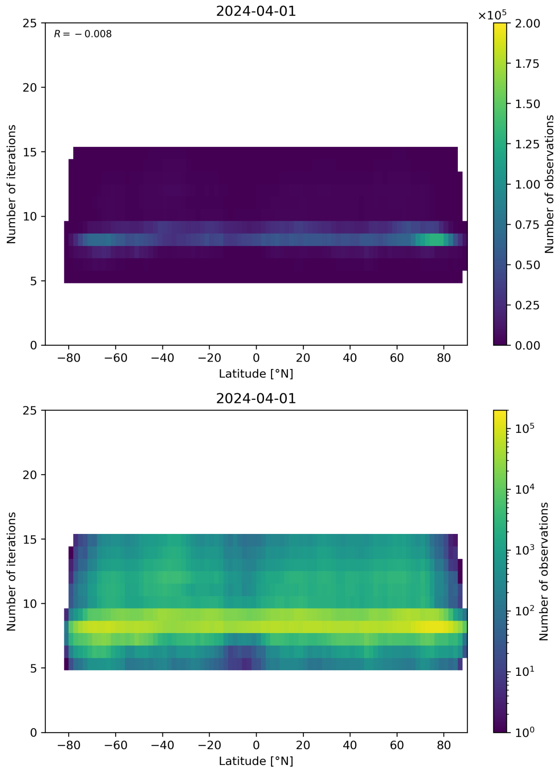
Figure 56: Scatter density plot of “Latitude” against “Number of iterations” for 2024-03-31 to 2024-04-02.
