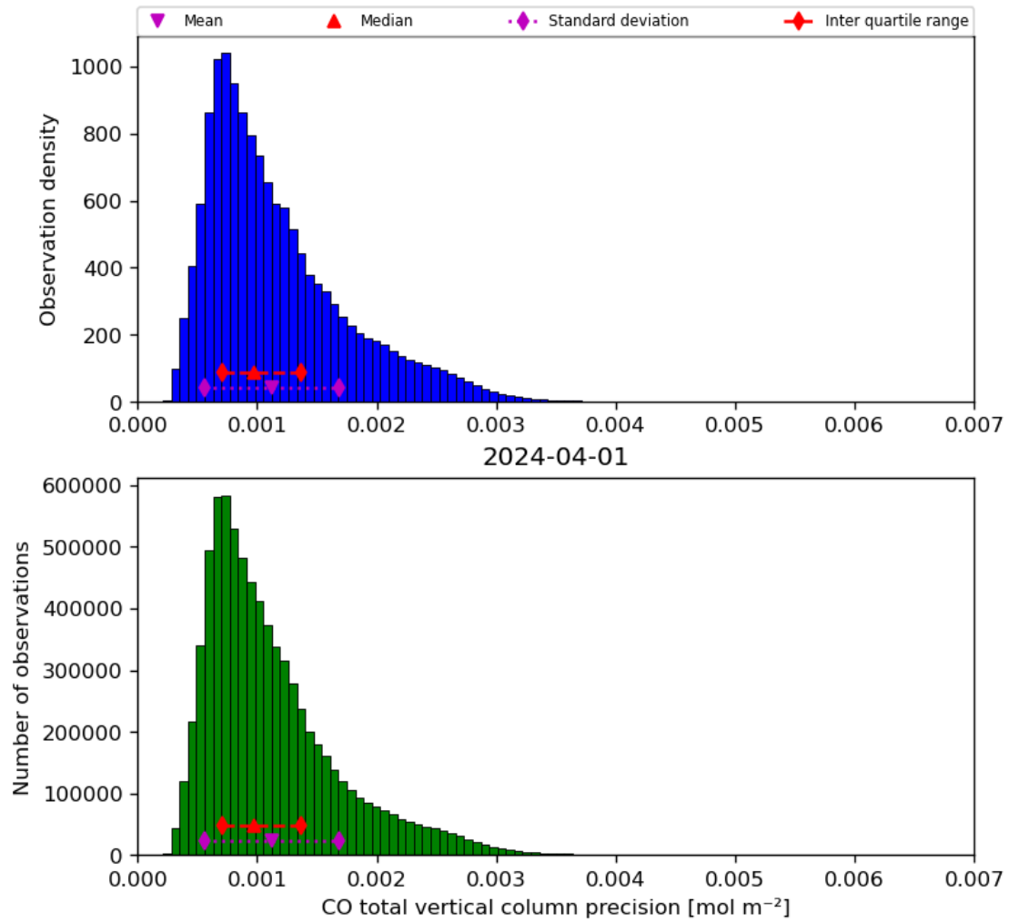
Figure 20: Histogram of “CO total vertical column precision” for 2024-03-31 to 2024-04-02
