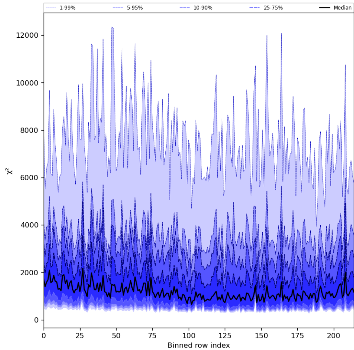
Figure 30: Along track statistics of “ \chi^2 ” for 2024-03-31 to 2024-04-02
