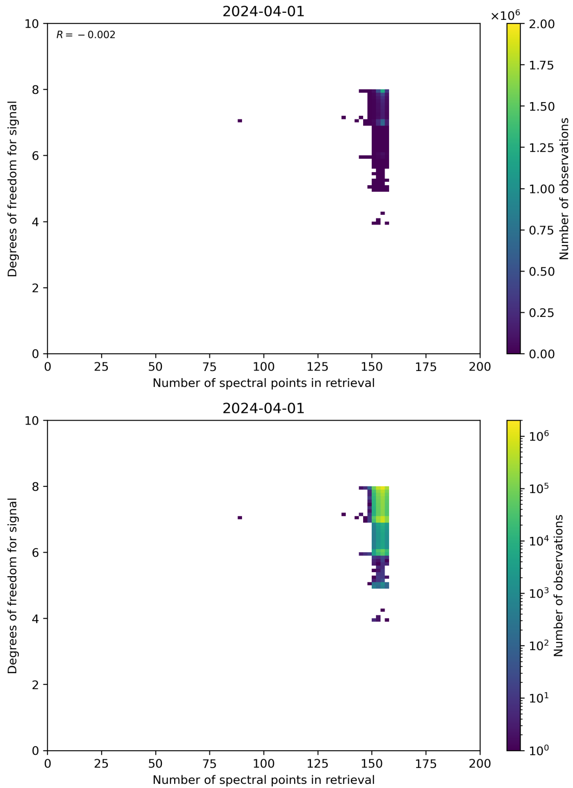
Figure 59: Scatter density plot of “Number of spectral points in retrieval” against “Degrees of freedom for signal” for 2024-03-31 to 2024-04-02.
