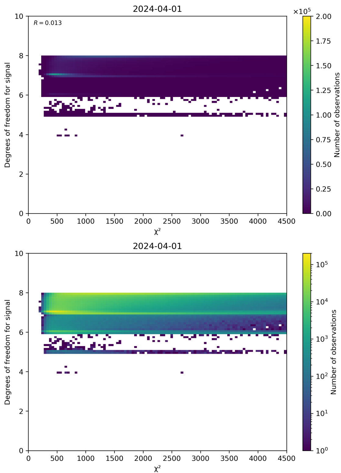
Figure 48: Scatter density plot of “ \chi^2 ” against “Degrees of freedom for signal” for 2024-03-31 to 2024-04-02.
