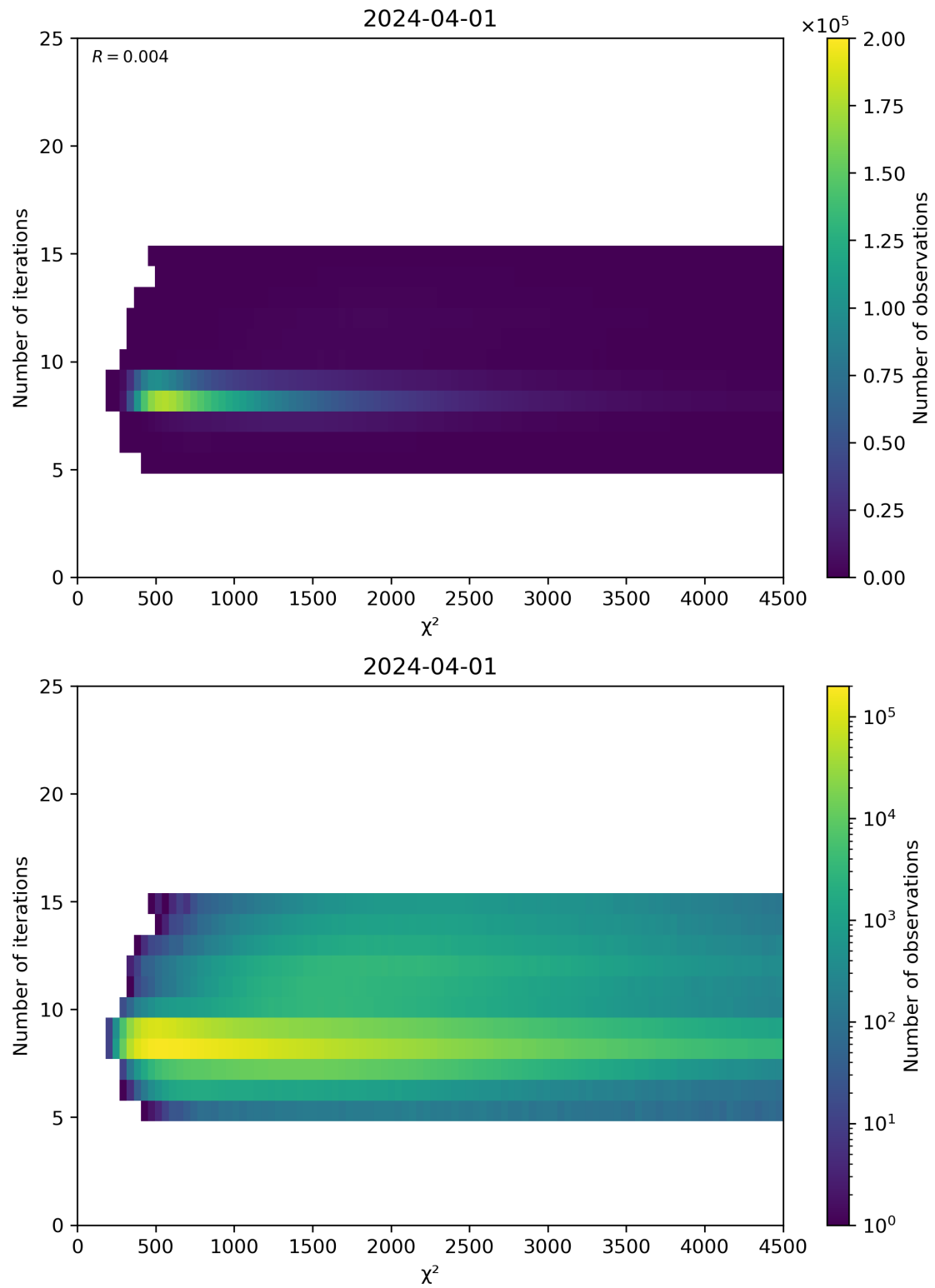
Figure 49: Scatter density plot of “ \chi^2 ” against “Number of iterations” for 2024-03-31 to 2024-04-02.
