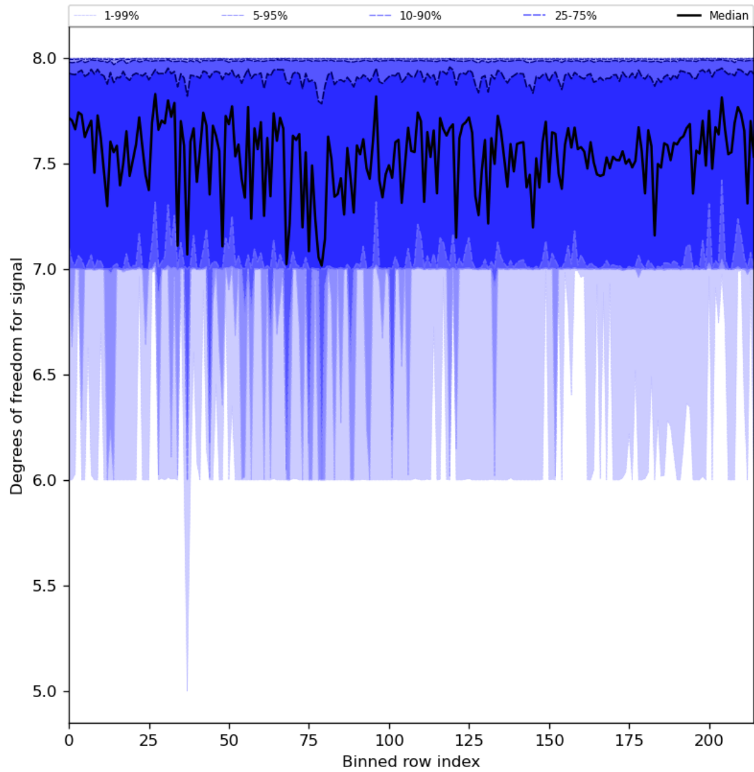
Figure 31: Along track statistics of “Degrees of freedom for signal” for 2024-03-31 to 2024-04-02
