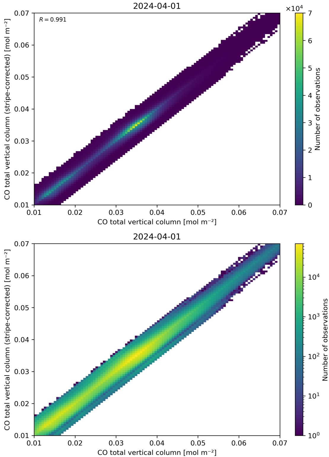
Figure 33: Scatter density plot of “CO total vertical column” against “CO total vertical column (stripe-corrected)” for 2024-03-31 to 2024-04-02.
