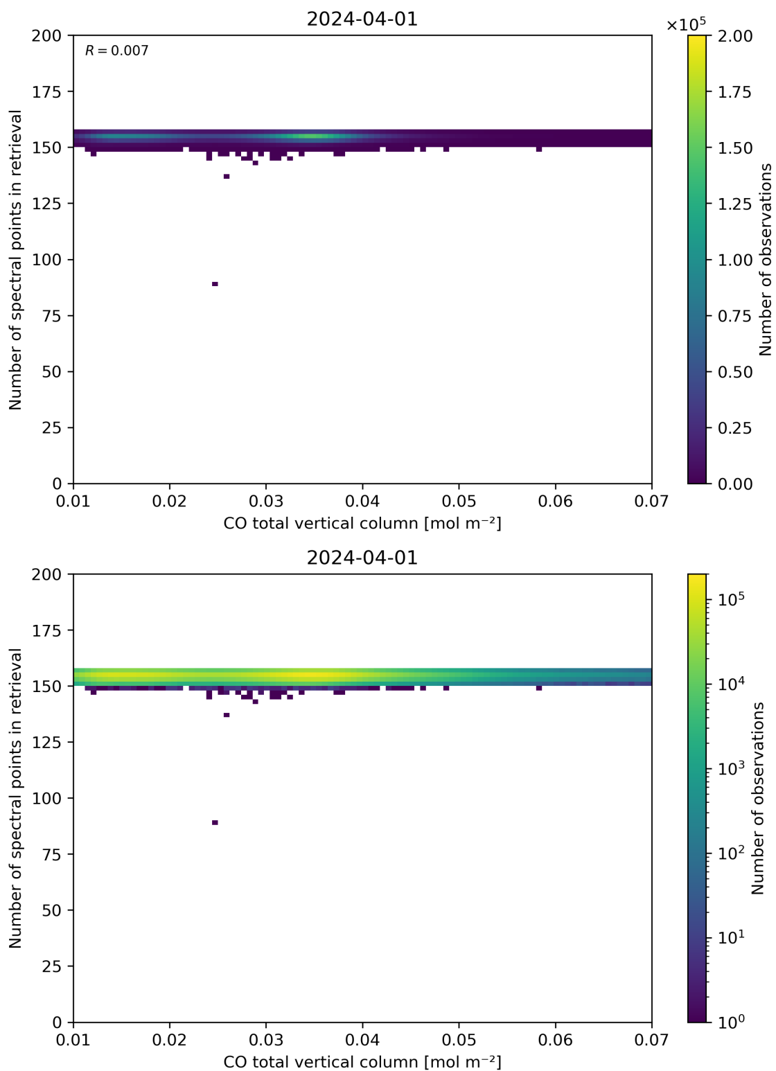
Figure 43: Scatter density plot of “CO total vertical column” against “Number of spectral points in retrieval” for 2024-03-31 to 2024-04-02.
