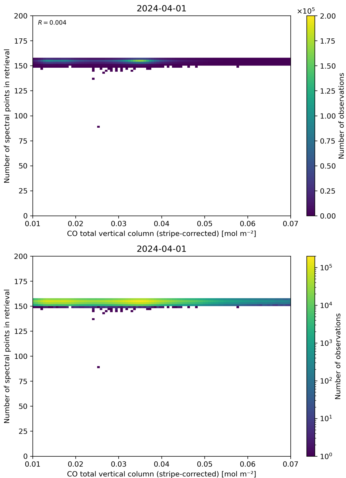
Figure 40: Scatter density plot of “CO total vertical column (stripe-corrected)” against “Number of spectral points in retrieval” for 2024-03-31 to 2024-04-02.
