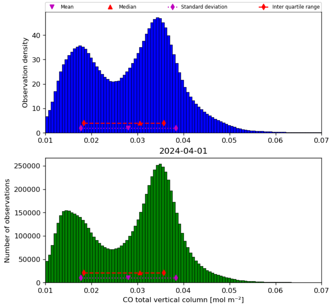
Figure 18: Histogram of “CO total vertical column” for 2024-03-31 to 2024-04-02
