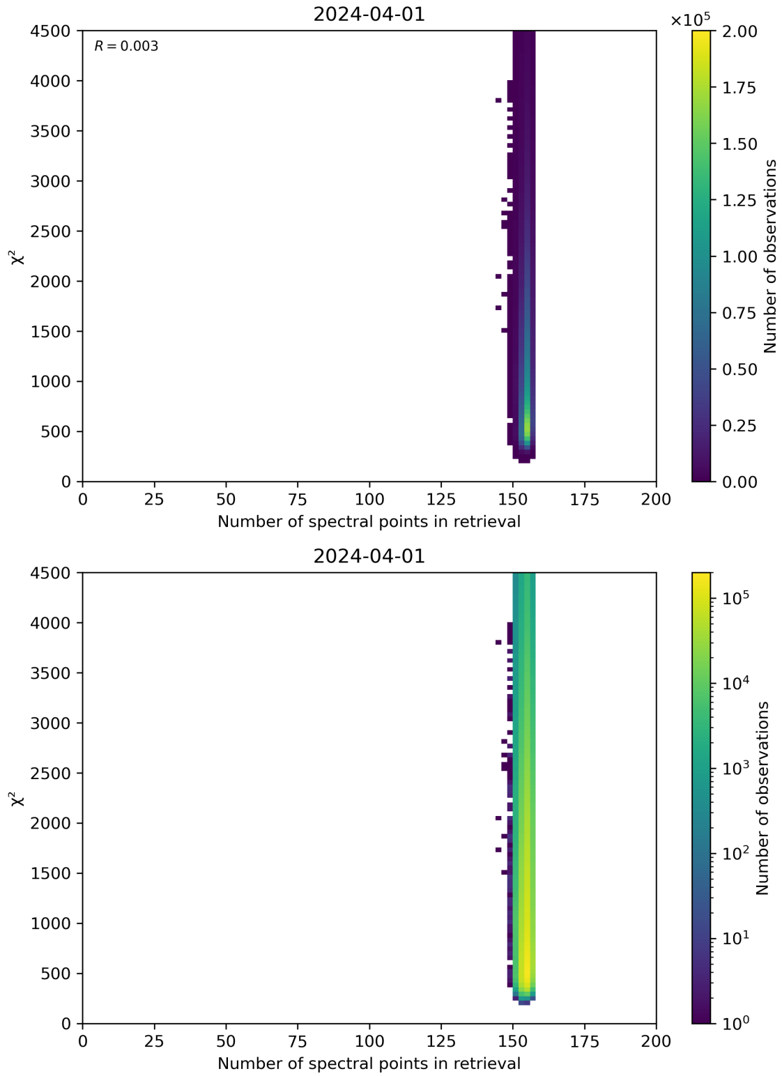
Figure 58: Scatter density plot of “Number of spectral points in retrieval” against “ \chi^2 ” for 2024-03-31 to 2024-04-02.
