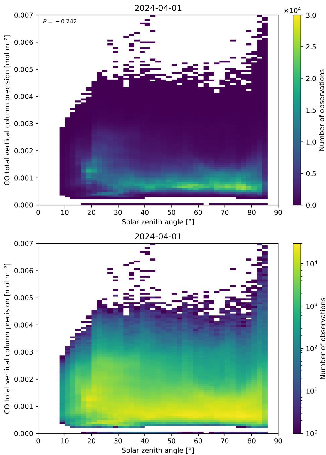
Figure 63: Scatter density plot of “Solar zenith angle” against “CO total vertical column precision” for 2024-03-31 to 2024-04-02.
