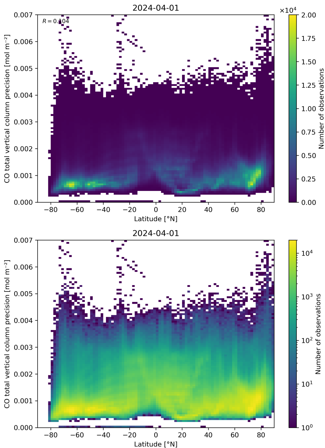
Figure 53: Scatter density plot of “Latitude” against “CO total vertical column precision” for 2024-03-31 to 2024-04-02.
