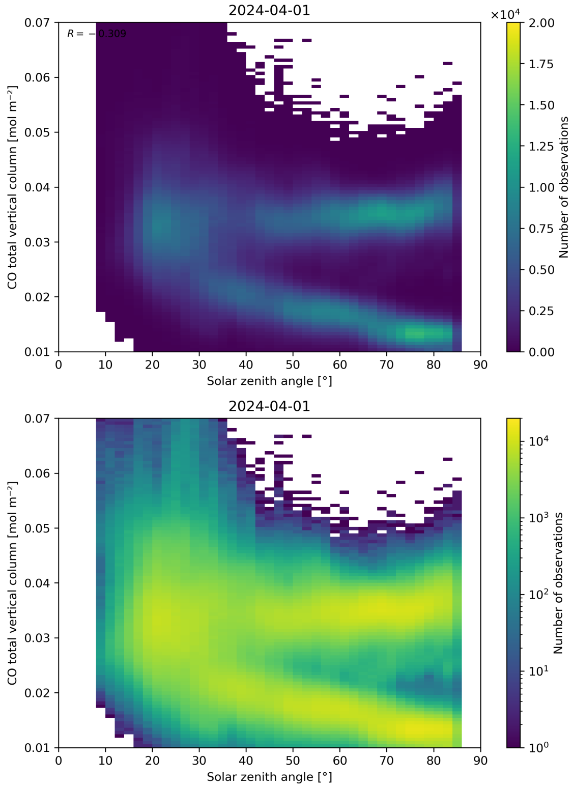
Figure 61: Scatter density plot of “Solar zenith angle” against “CO total vertical column” for 2024-03-31 to 2024-04-02.
