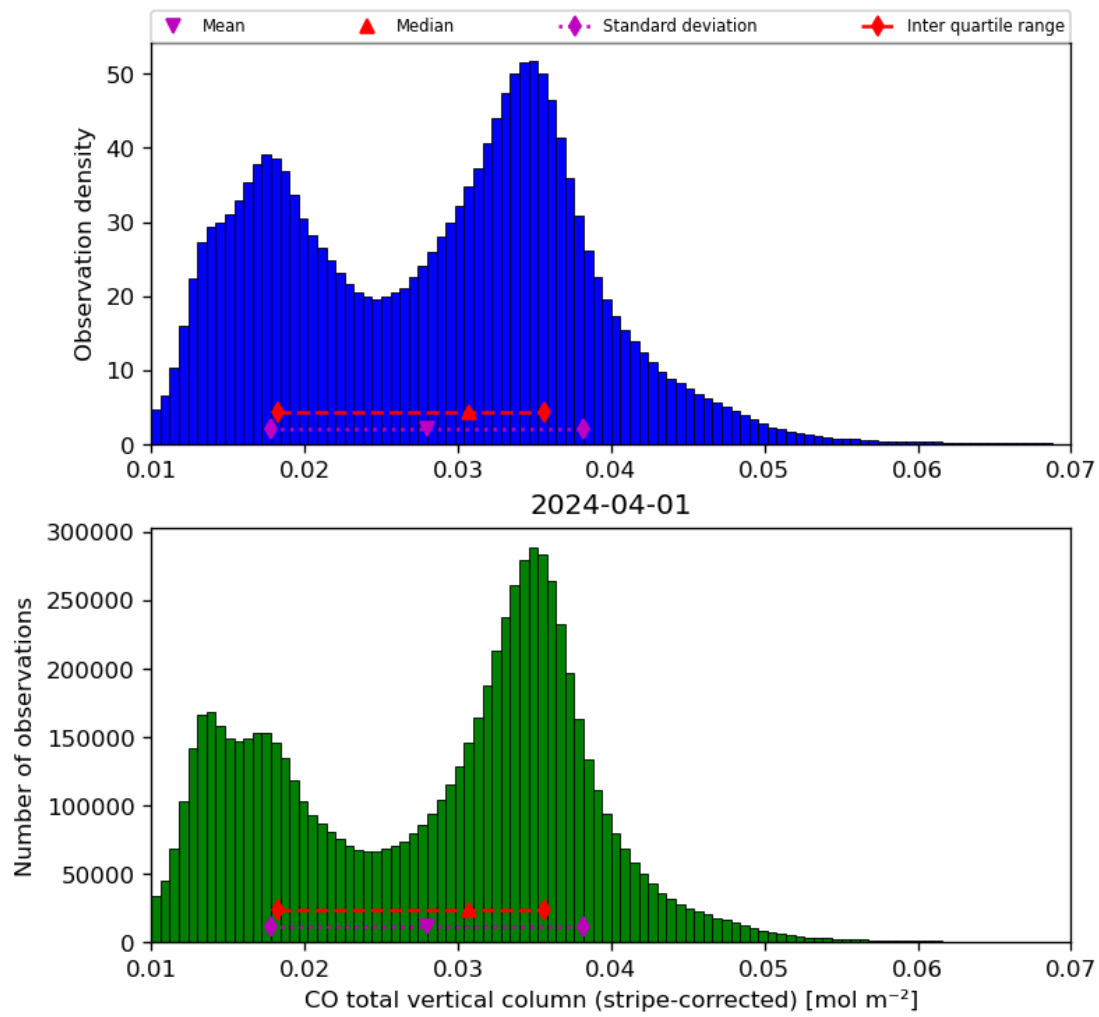
Figure 19: Histogram of “CO total vertical column (stripe-corrected)” for 2024-03-31 to 2024-04-02
