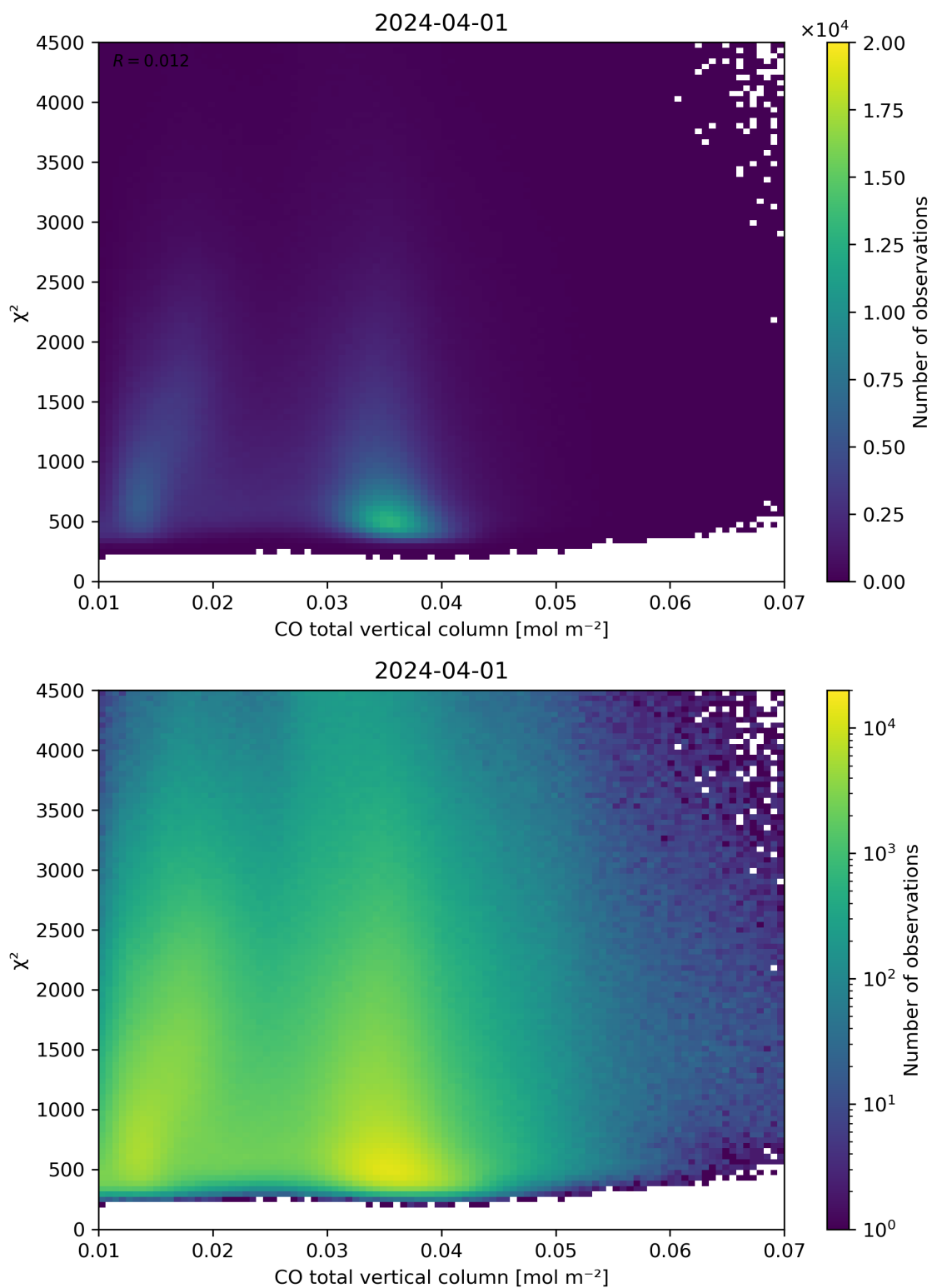
Figure 35: Scatter density plot of “CO total vertical column” against “ \chi^2 ” for 2024-03-31 to 2024-04-02.
