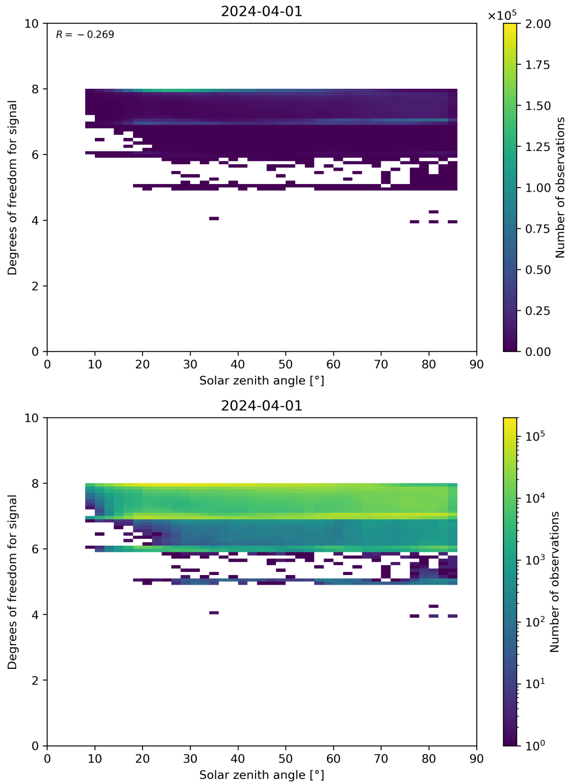
Figure 65: Scatter density plot of “Solar zenith angle” against “Degrees of freedom for signal” for 2024-03-31 to 2024-04-02.
