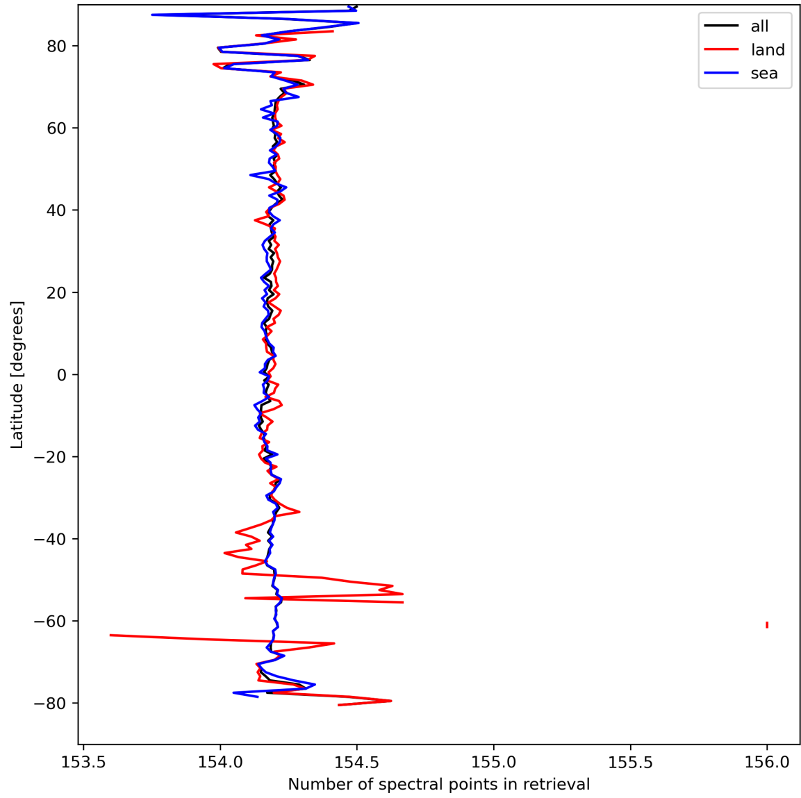
Figure 13: Zonal average of “Number of spectral points in retrieval” for 2024-03-31 to 2024-04-02.
