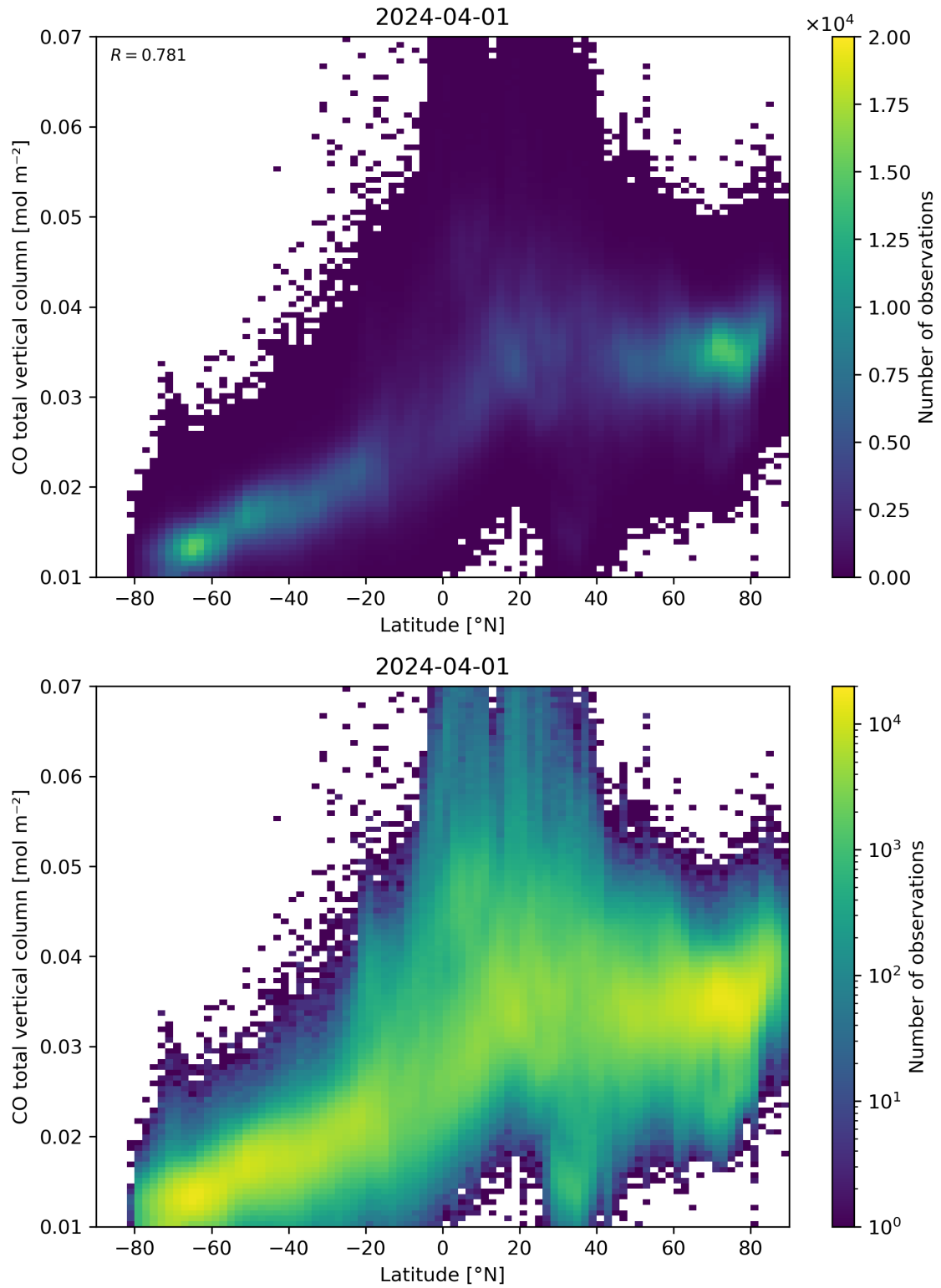
Figure 51: Scatter density plot of “Latitude” against “CO total vertical column” for 2024-03-31 to 2024-04-02.
