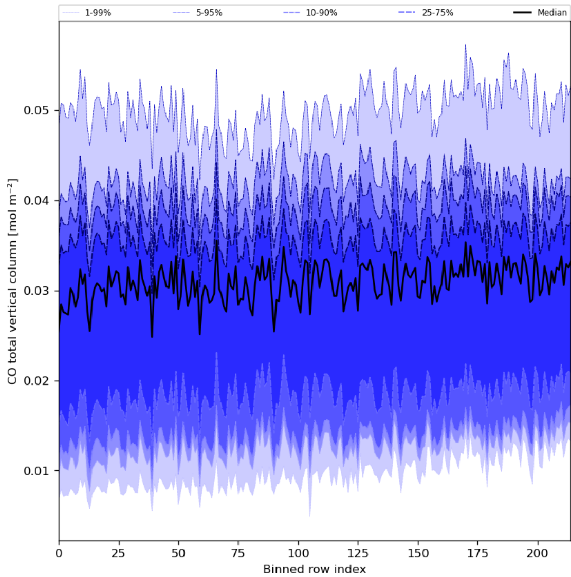
Figure 26: Along track statistics of “CO total vertical column” for 2024-03-31 to 2024-04-02
