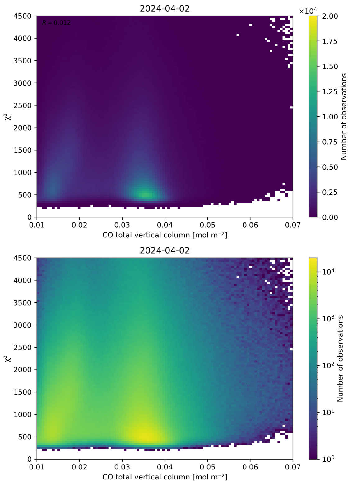
Figure 35: Scatter density plot of “CO total vertical column” against “ \chi^2 ” for 2024-04-01 to 2024-04-03.
