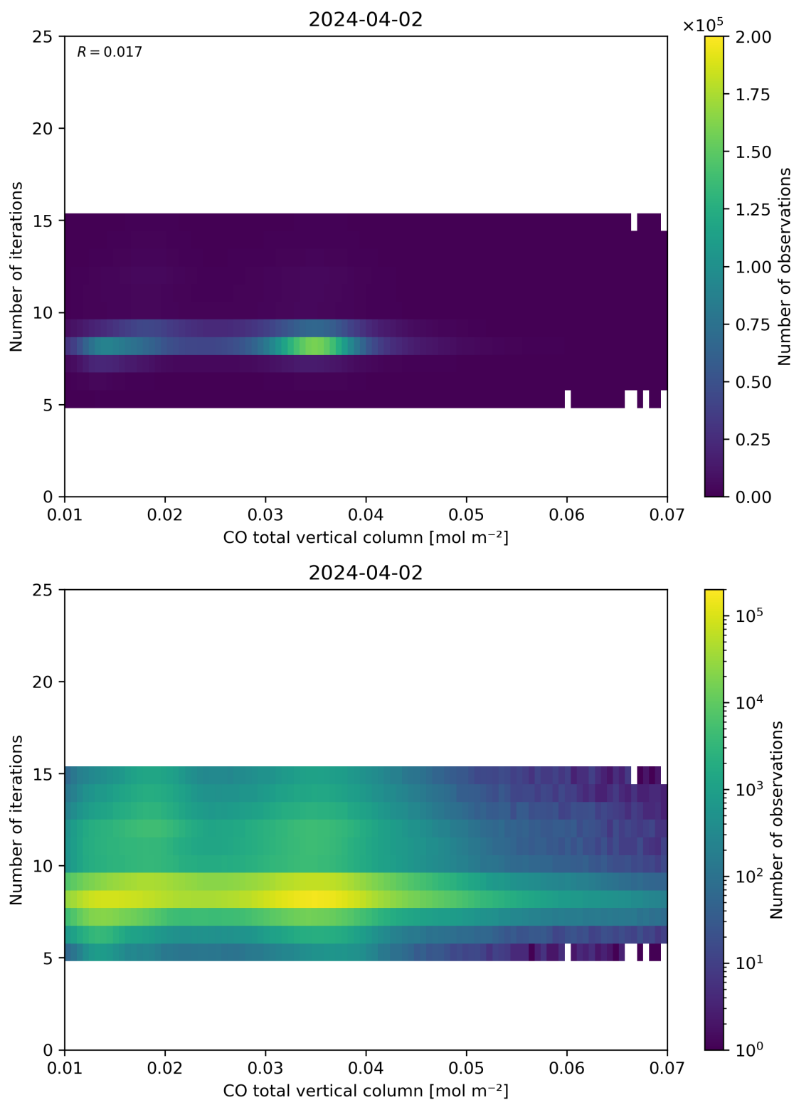
Figure 42: Scatter density plot of “CO total vertical column” against “Number of iterations” for 2024-04-01 to 2024-04-03.
