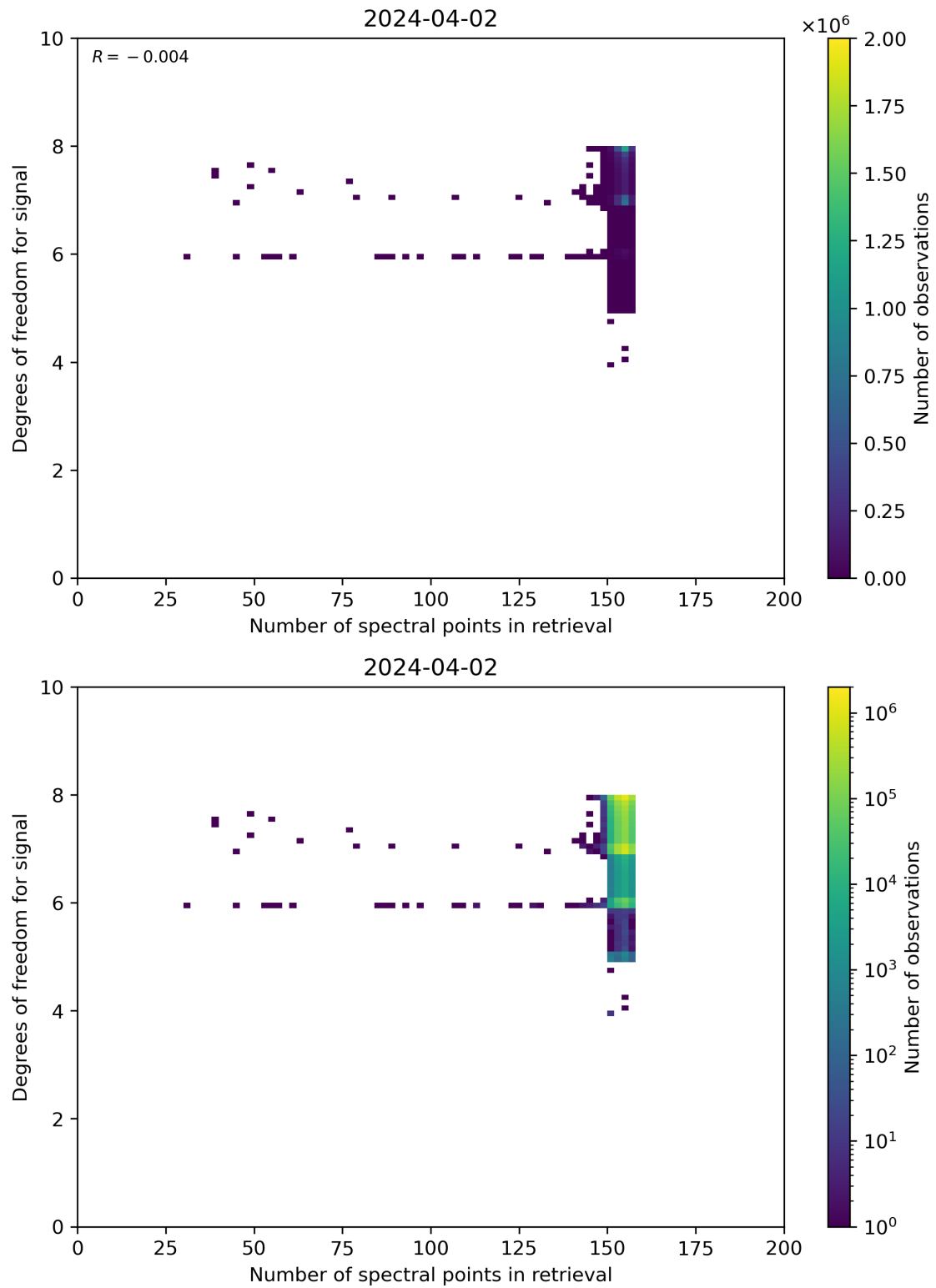
Figure 59: Scatter density plot of “Number of spectral points in retrieval” against “Degrees of freedom for signal” for 2024-04-01 to 2024-04-03.
