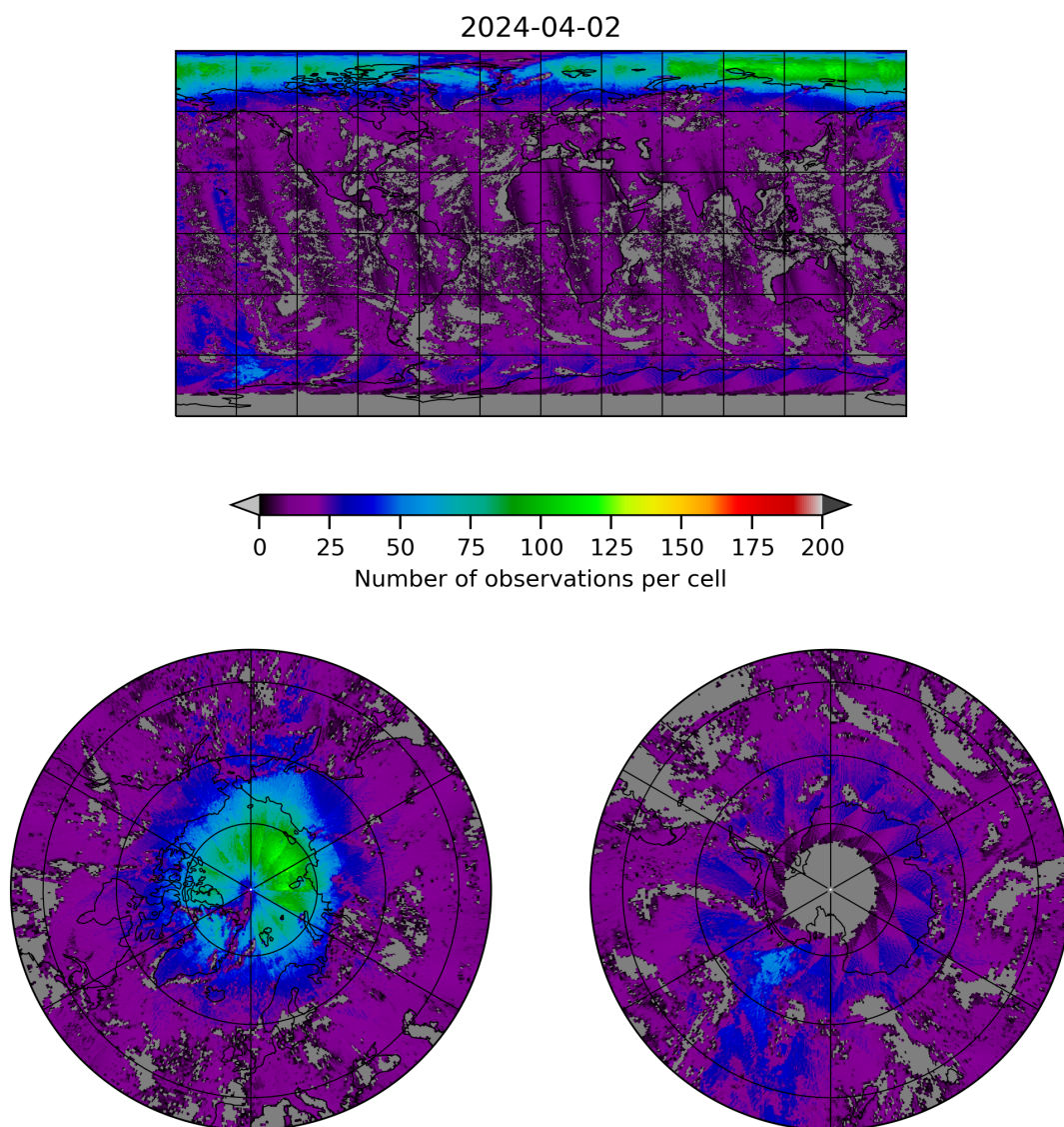
Figure 8: Map of the number of observations for 2024-04-01 to 2024-04-03
