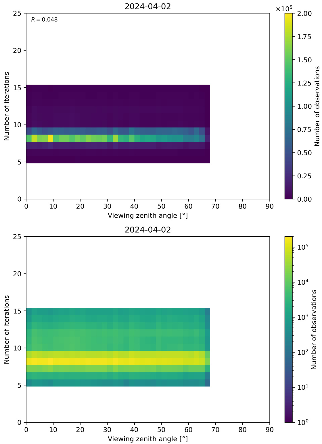
Figure 75: Scatter density plot of “Viewing zenith angle” against “Number of iterations” for 2024-04-01 to 2024-04-03.
