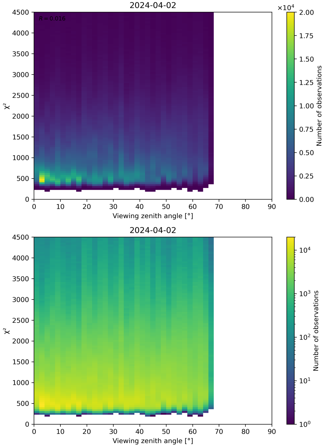
Figure 72: Scatter density plot of “Viewing zenith angle” against “ \chi^2 ” for 2024-04-01 to 2024-04-03.
