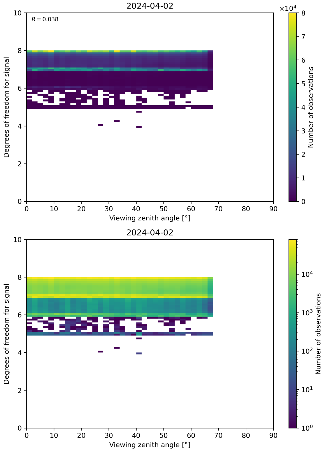
Figure 73: Scatter density plot of “Viewing zenith angle” against “Degrees of freedom for signal” for 2024-04-01 to 2024-04-03.
