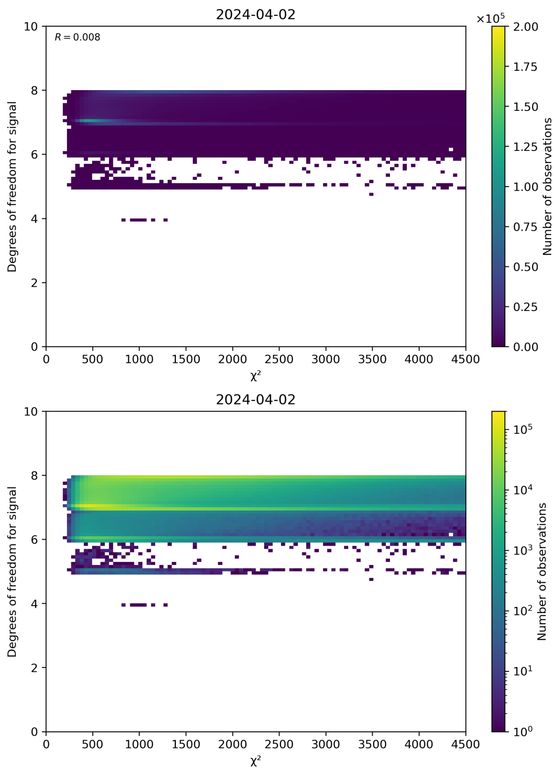
Figure 48: Scatter density plot of “ \chi^2 ” against “Degrees of freedom for signal” for 2024-04-01 to 2024-04-03.
