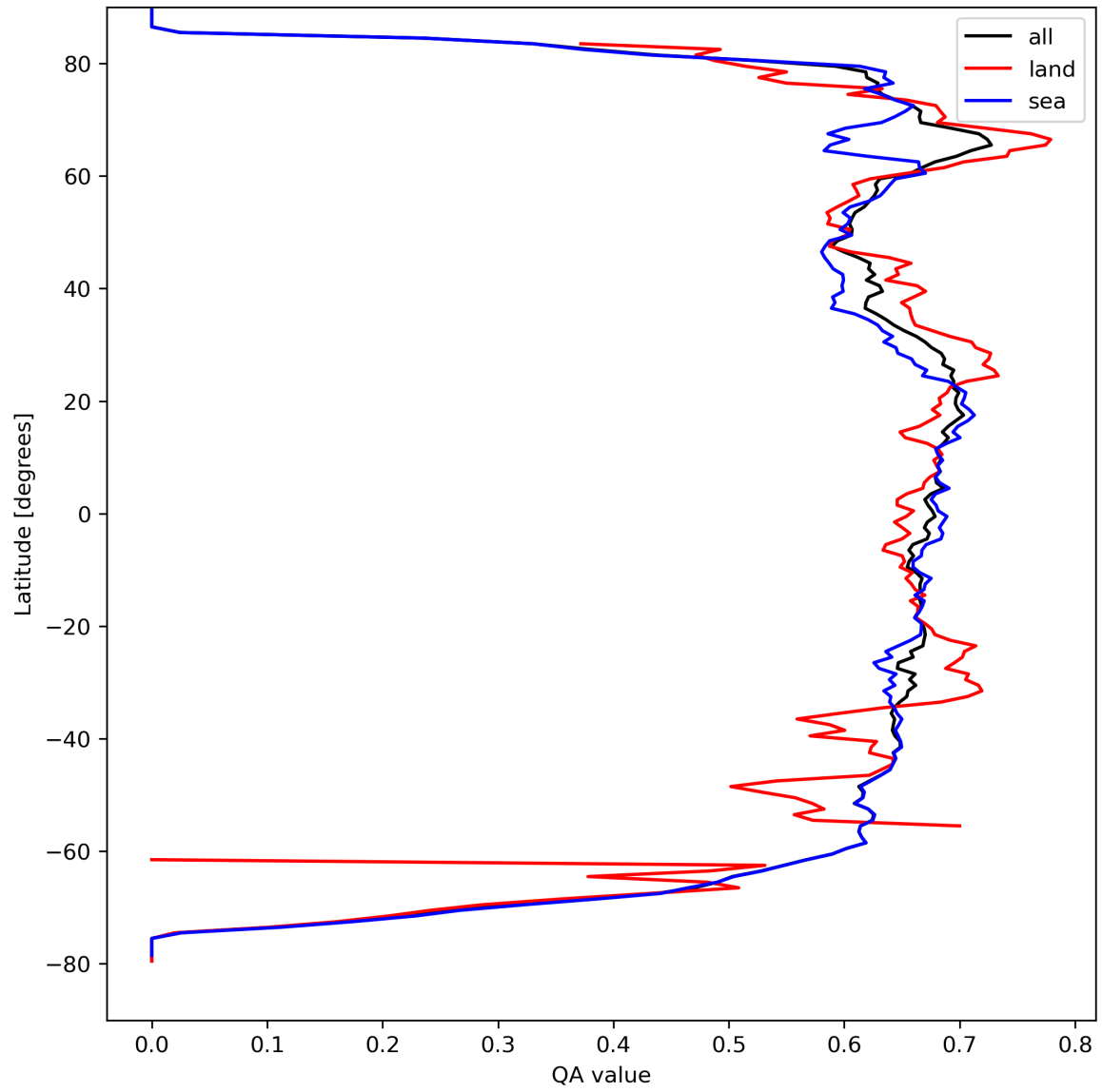
Figure 9: Zonal average of “QA value” for 2024-04-01 to 2024-04-03.
