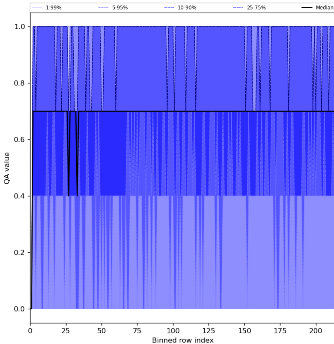
Figure 25: Along track statistics of “QA value” for 2024-04-01 to 2024-04-03
