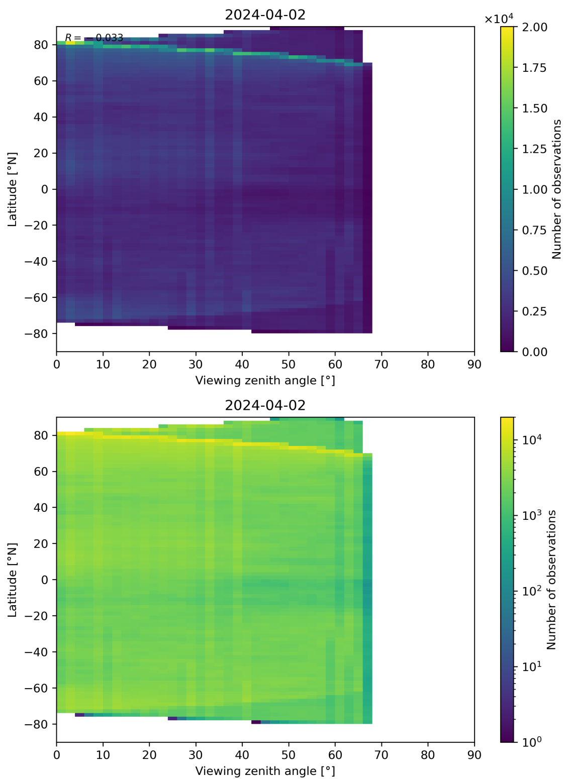
Figure 74: Scatter density plot of “Viewing zenith angle” against “Latitude” for 2024-04-01 to 2024-04-03.
