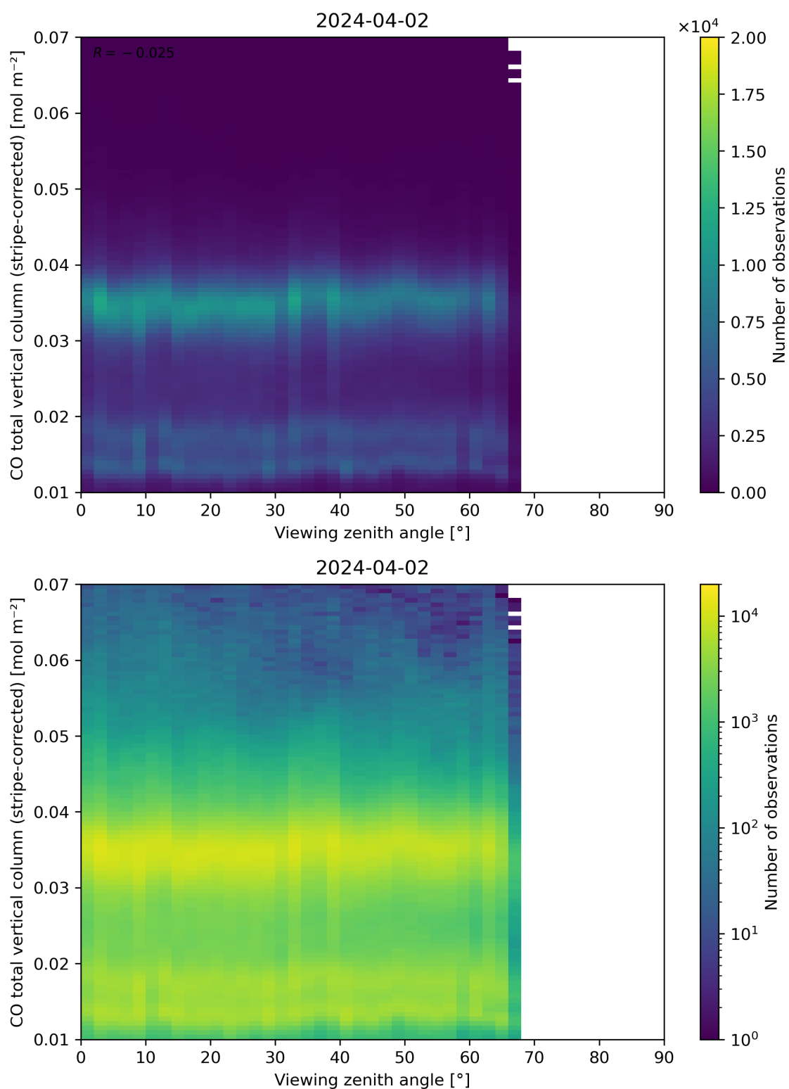
Figure 70: Scatter density plot of “Viewing zenith angle” against “CO total vertical column (stripe-corrected)” for 2024-04-01 to 2024-04-03.
