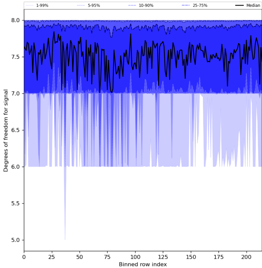
Figure 31: Along track statistics of “Degrees of freedom for signal” for 2024-04-01 to 2024-04-03
