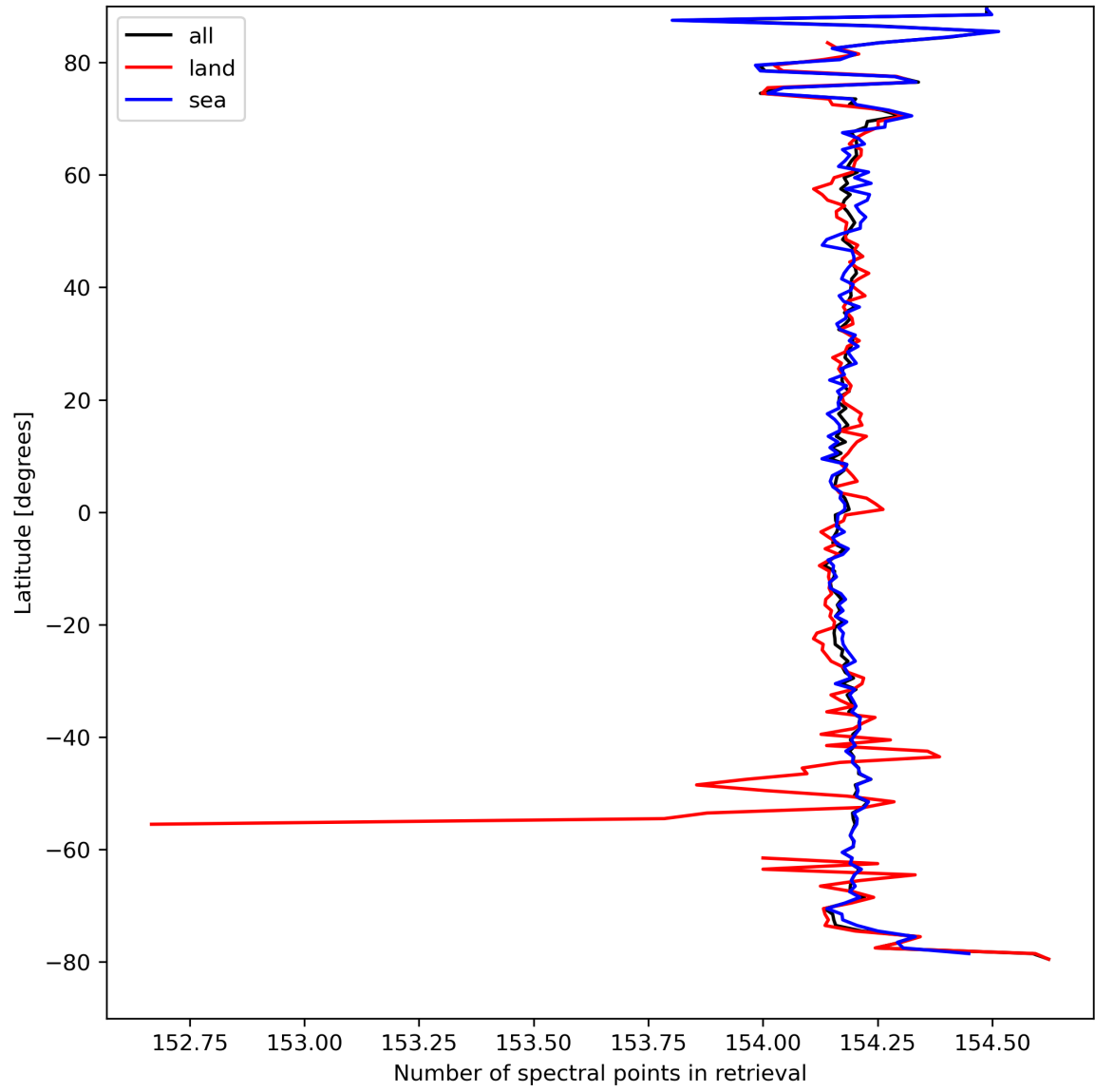
Figure 13: Zonal average of “Number of spectral points in retrieval” for 2024-04-01 to 2024-04-03.
