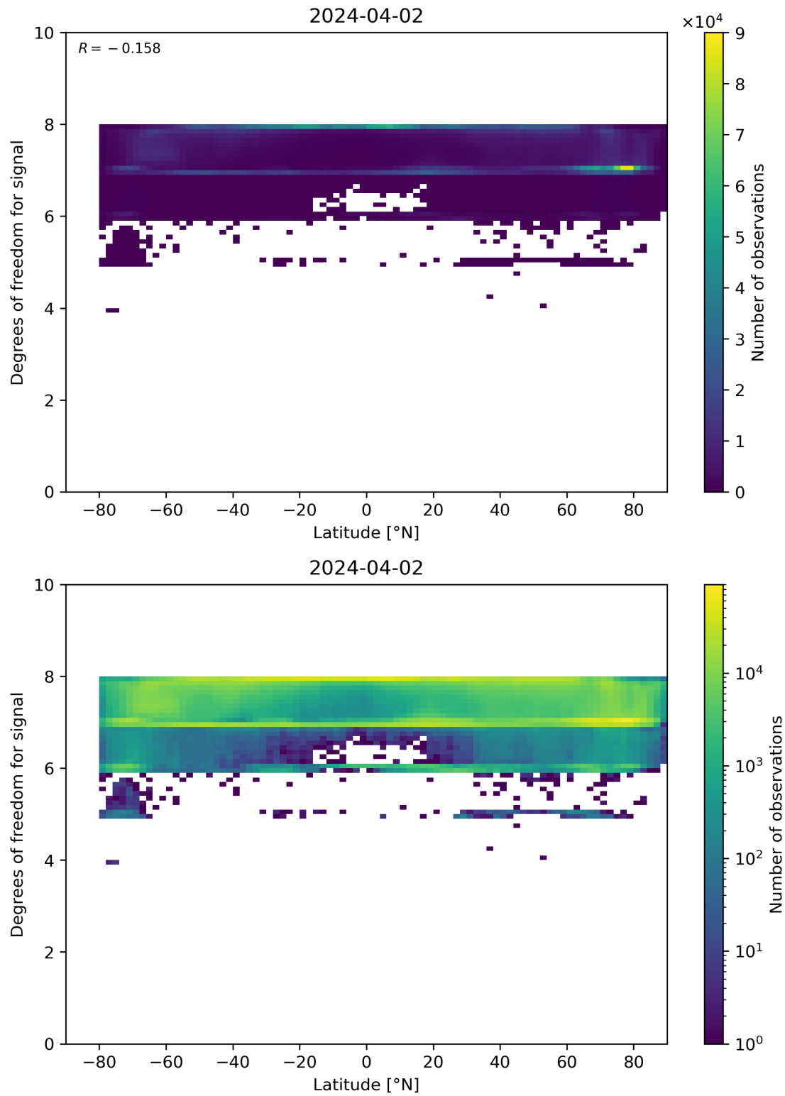
Figure 55: Scatter density plot of “Latitude” against “Degrees of freedom for signal” for 2024-04-01 to 2024-04-03.
