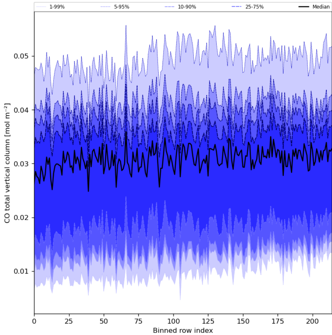
Figure 26: Along track statistics of “CO total vertical column” for 2024-04-01 to 2024-04-03
