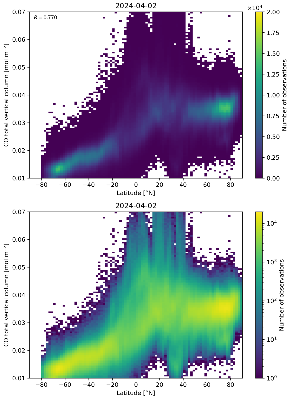
Figure 51: Scatter density plot of “Latitude” against “CO total vertical column” for 2024-04-01 to 2024-04-03.
