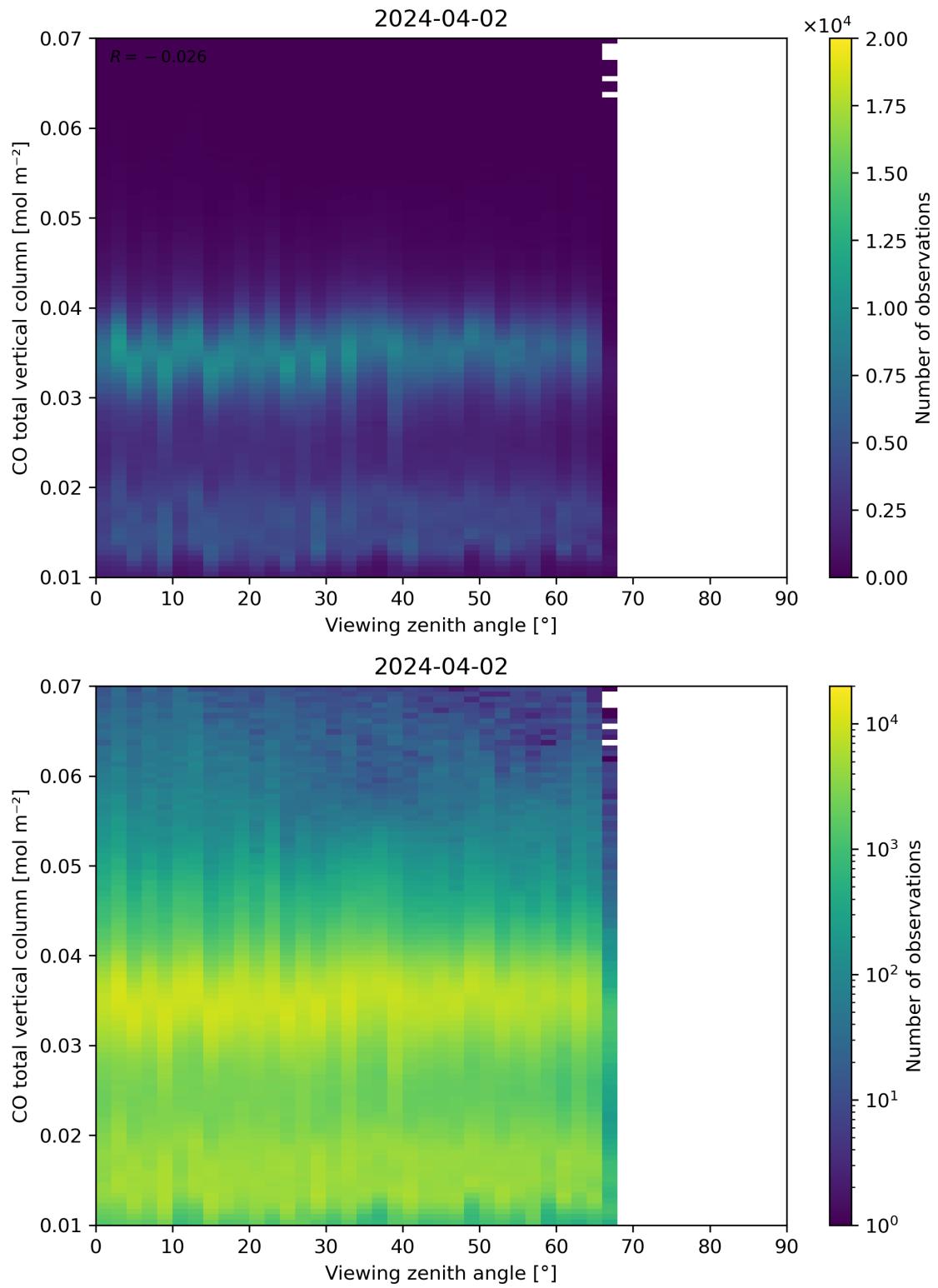
Figure 69: Scatter density plot of “Viewing zenith angle” against “CO total vertical column” for 2024-04-01 to 2024-04-03.
