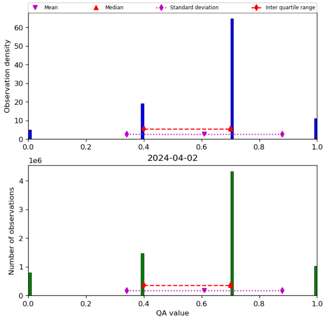
Figure 17: Histogram of “QA value” for 2024-04-01 to 2024-04-03
