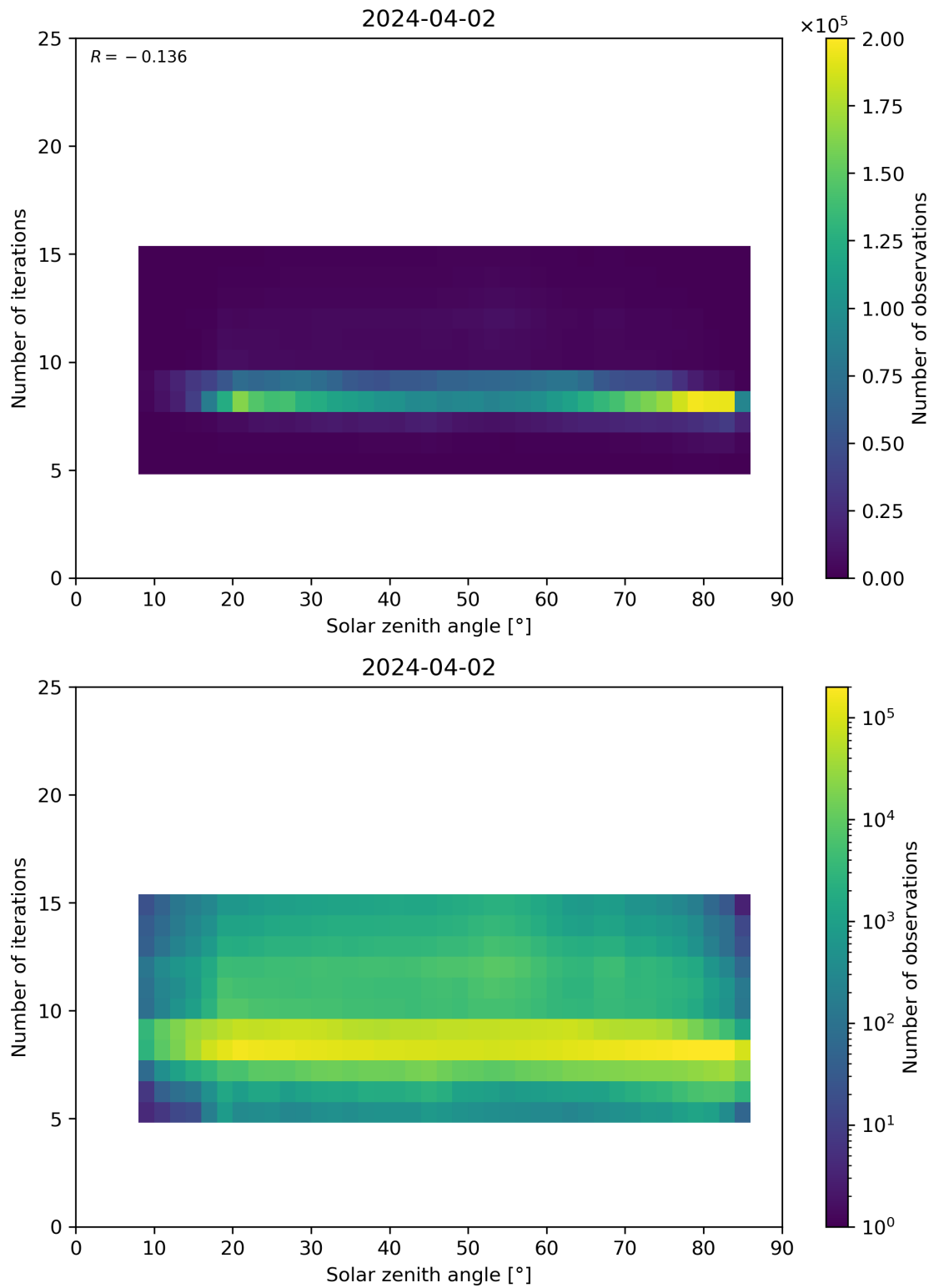
Figure 67: Scatter density plot of “Solar zenith angle” against “Number of iterations” for 2024-04-01 to 2024-04-03.
