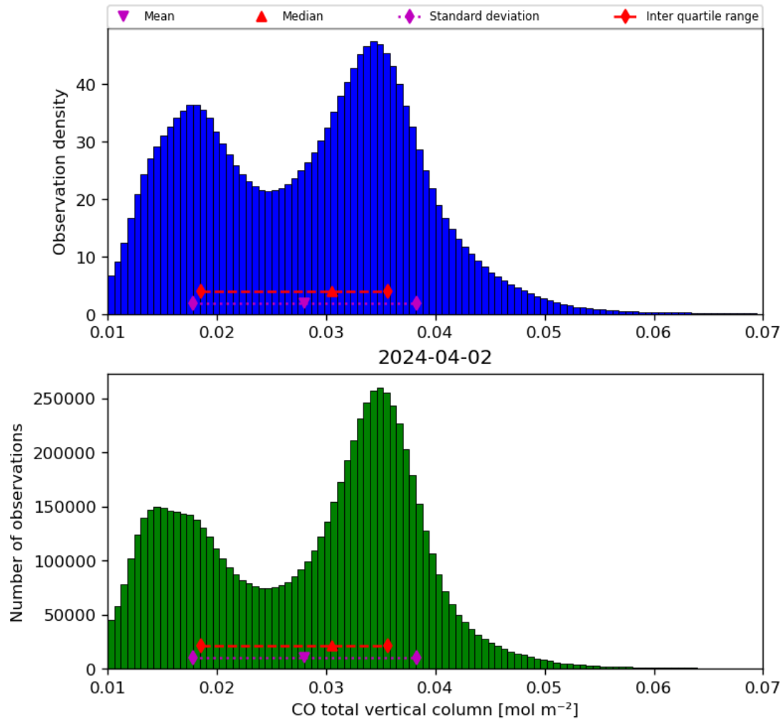
Figure 18: Histogram of “CO total vertical column” for 2024-04-01 to 2024-04-03
