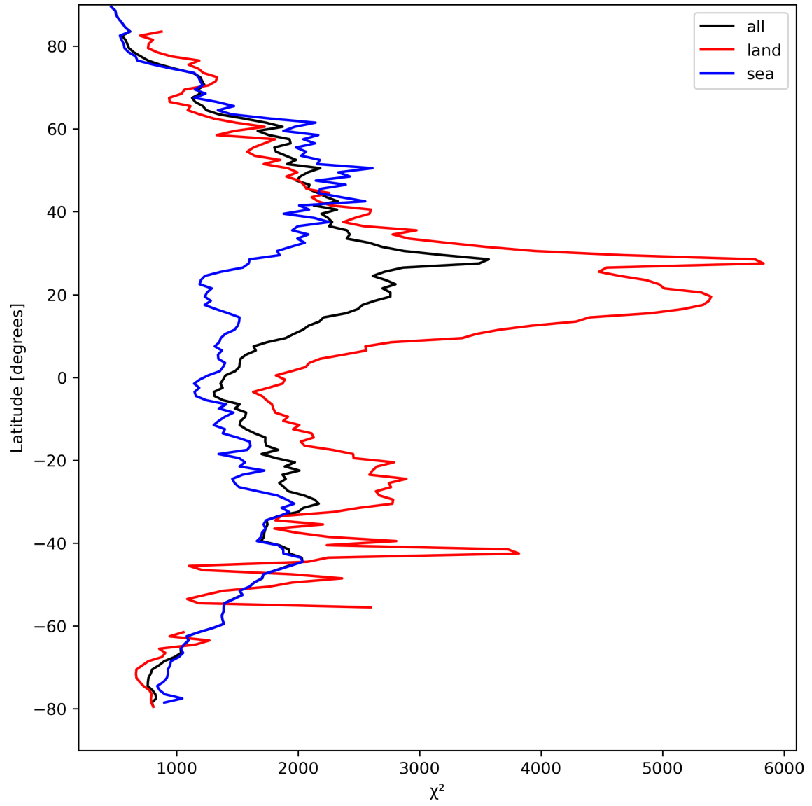
Figure 14: Zonal average of “ \chi^2 ” for 2024-04-01 to 2024-04-03.
