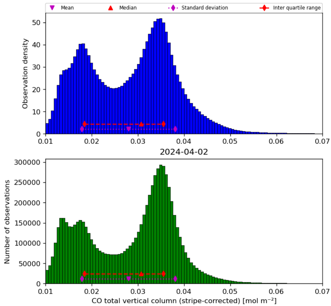
Figure 19: Histogram of “CO total vertical column (stripe-corrected)” for 2024-04-01 to 2024-04-03
