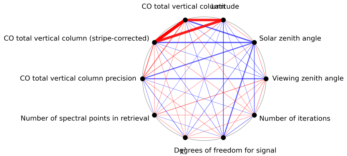
Figure 1: Map of correlation graph for 2024-04-01 to 2024-04-03.
