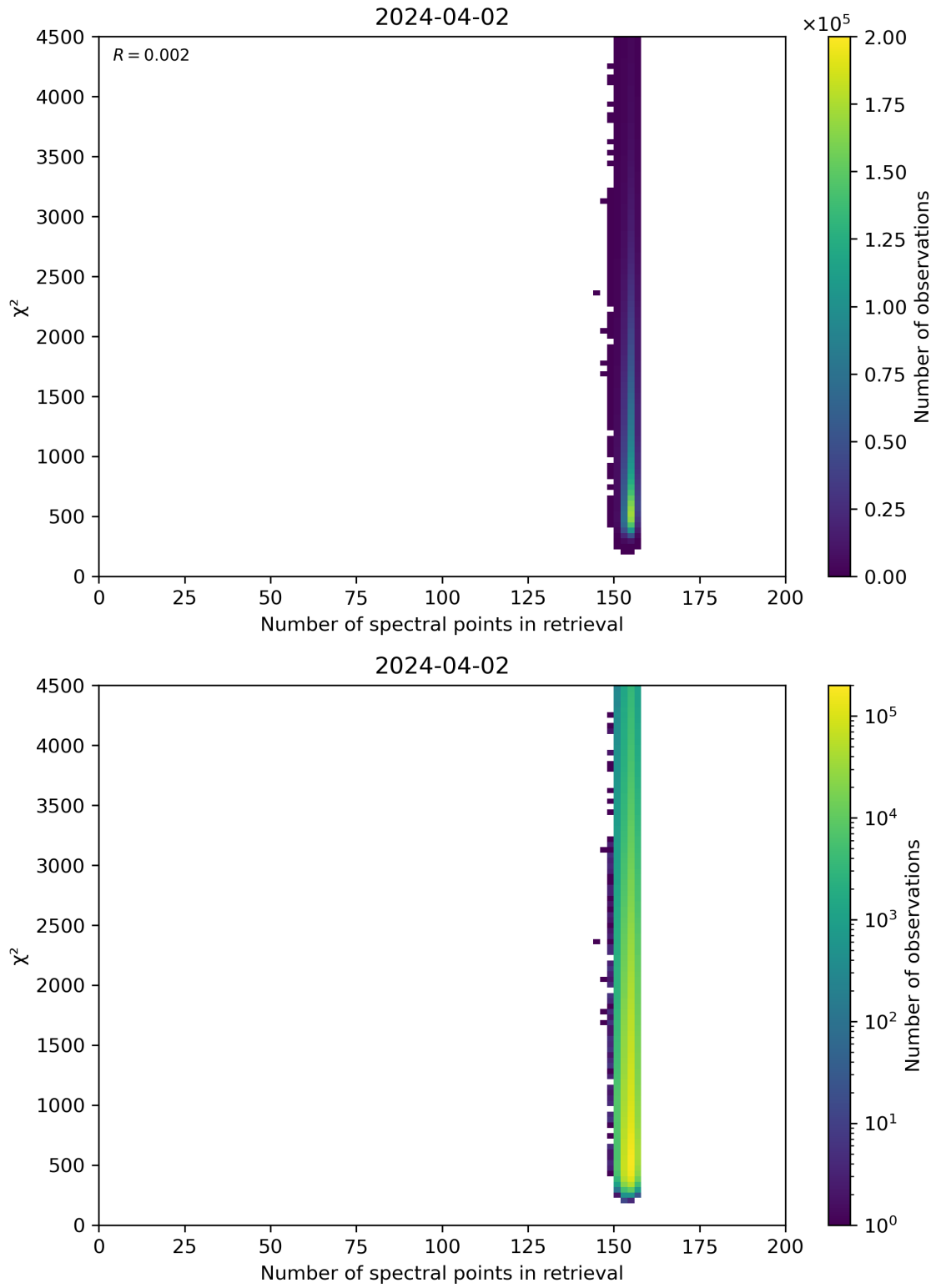
Figure 58: Scatter density plot of “Number of spectral points in retrieval” against “ \chi^2 ” for 2024-04-01 to 2024-04-03.
