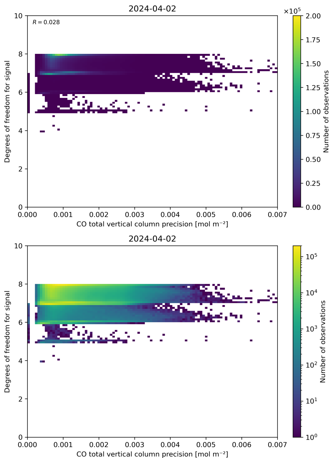
Figure 45: Scatter density plot of “CO total vertical column precision” against “Degrees of freedom for signal” for 2024-04-01 to 2024-04-03.
