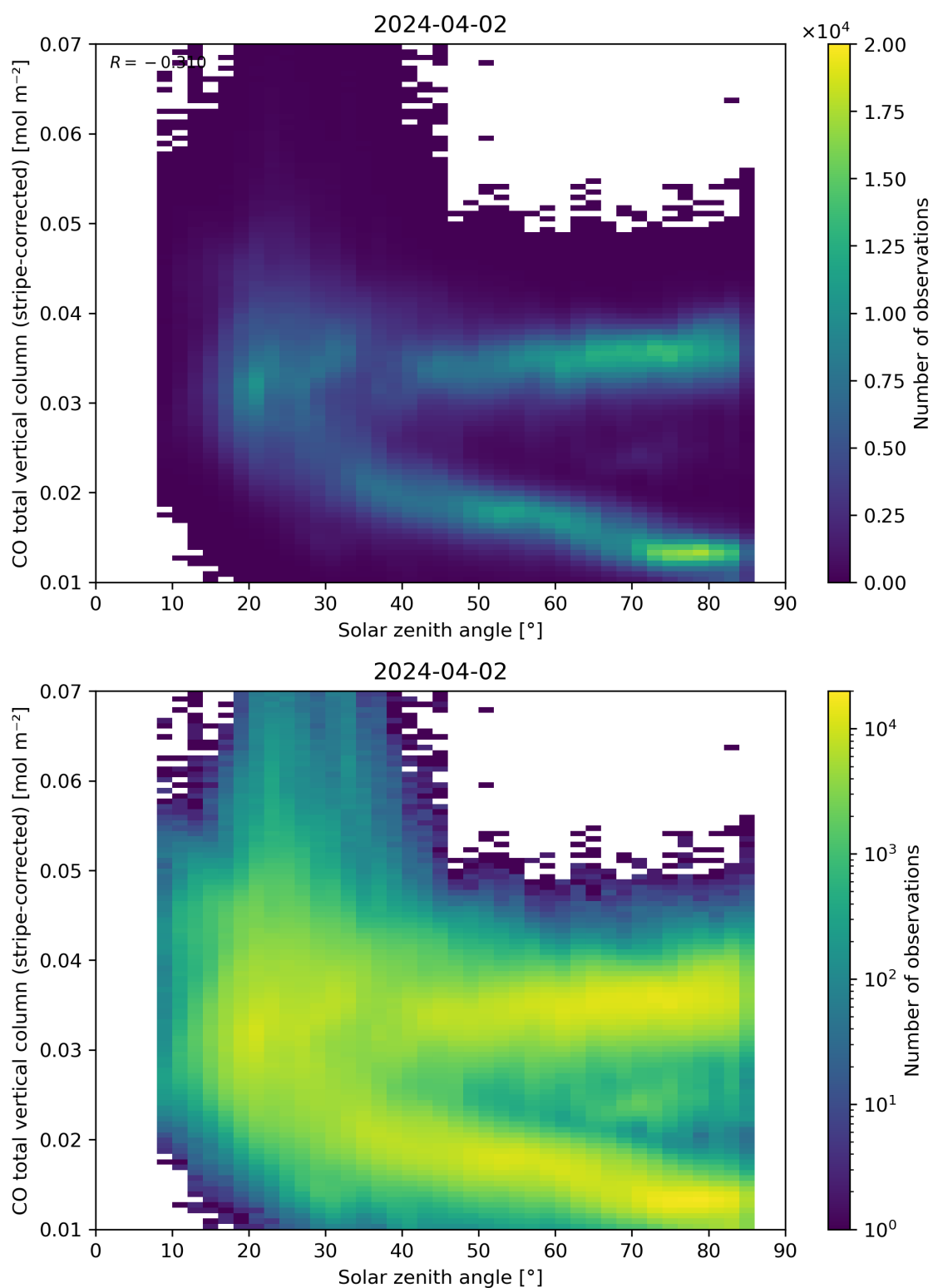
Figure 62: Scatter density plot of “Solar zenith angle” against “CO total vertical column (stripe-corrected)” for 2024-04-01 to 2024-04-03.
