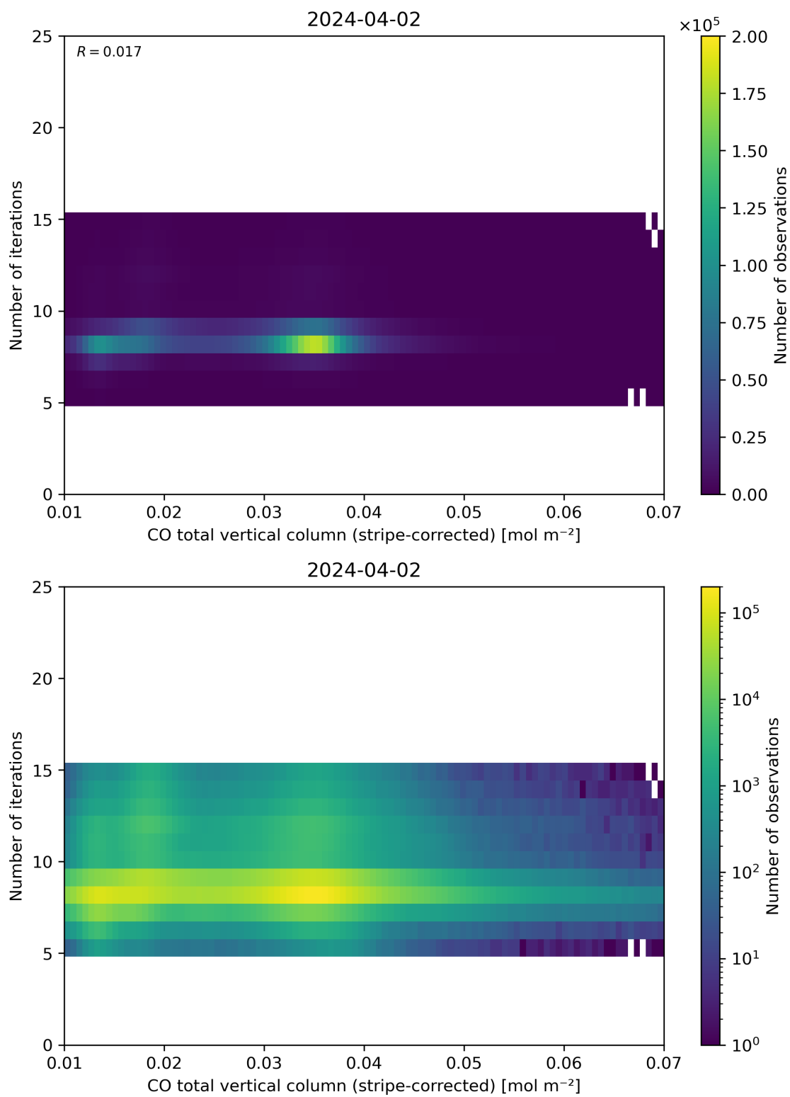
Figure 39: Scatter density plot of “CO total vertical column (stripe-corrected)” against “Number of iterations” for 2024-04-01 to 2024-04-03.
