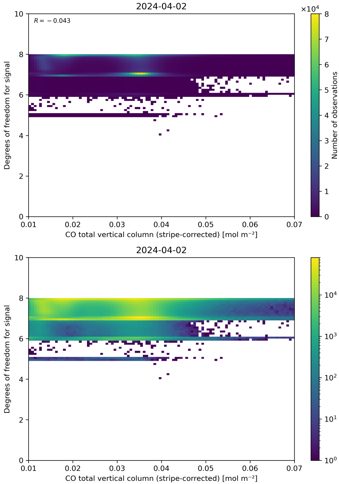
Figure 38: Scatter density plot of “CO total vertical column (stripe-corrected)” against “Degrees of freedom for signal” for 2024-04-01 to 2024-04-03.
