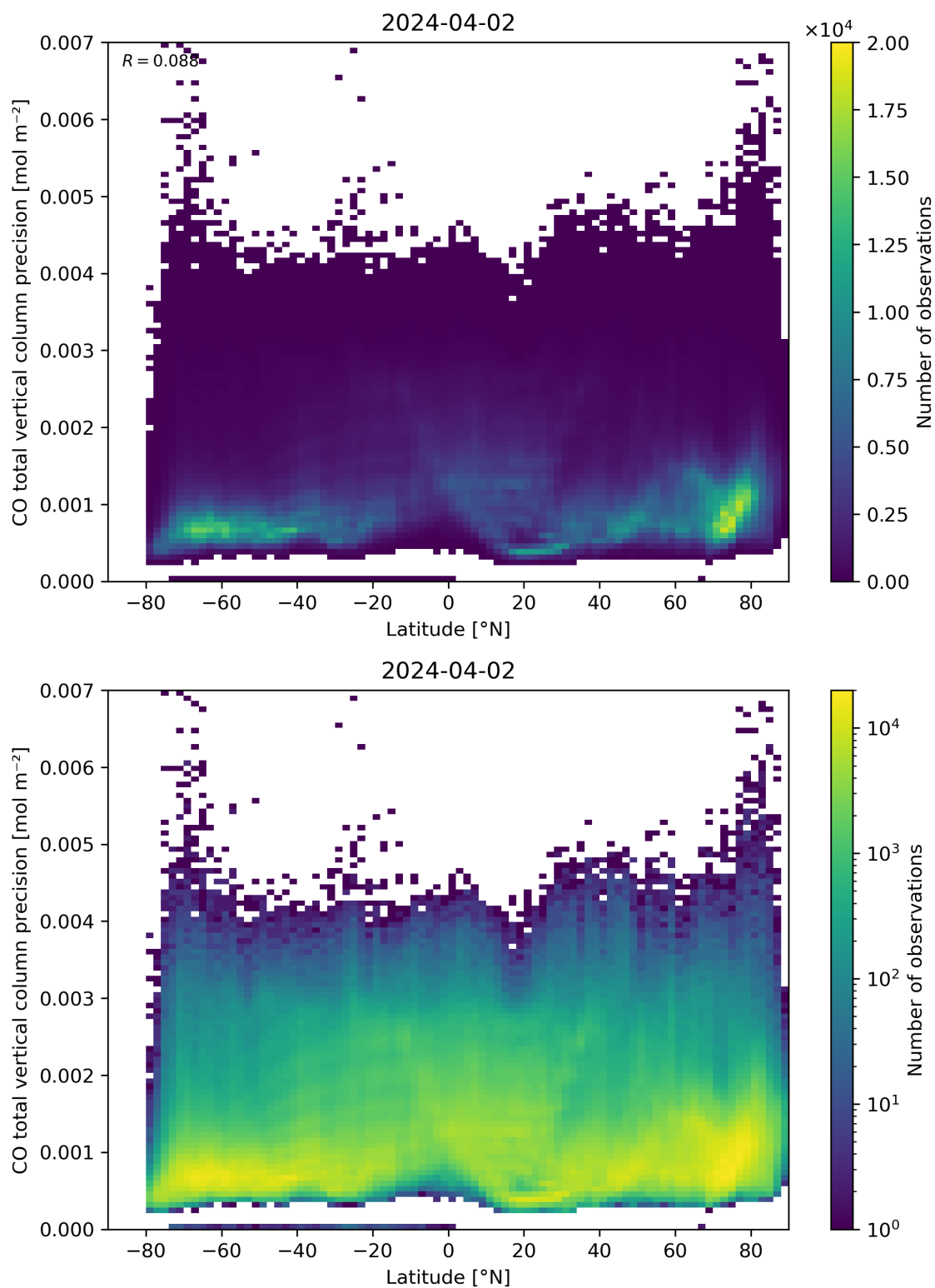
Figure 53: Scatter density plot of “Latitude” against “CO total vertical column precision” for 2024-04-01 to 2024-04-03.
