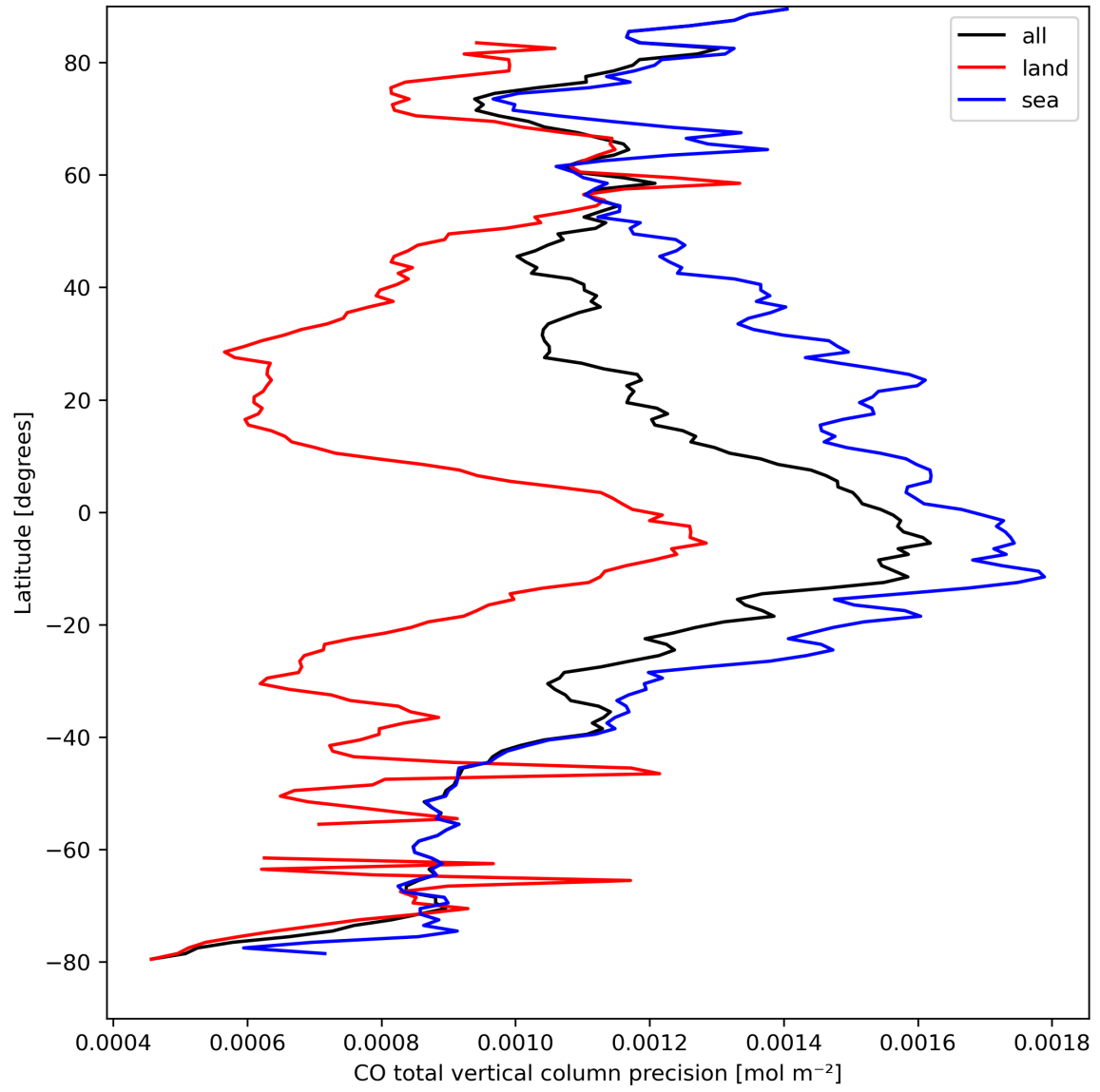
Figure 12: Zonal average of “CO total vertical column precision” for 2024-04-01 to 2024-04-03.
