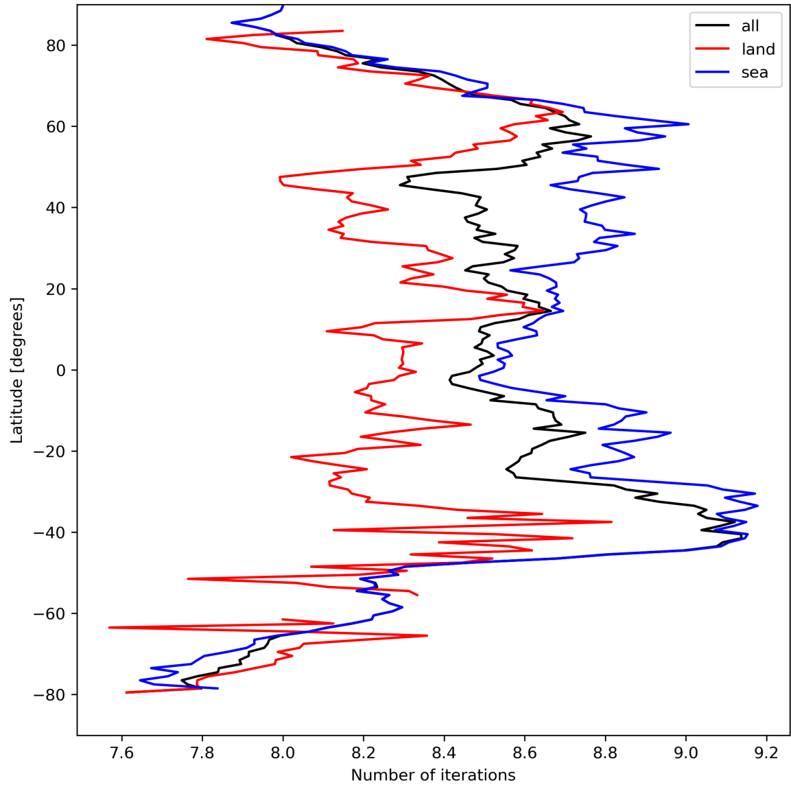
Figure 16: Zonal average of “Number of iterations” for 2024-04-01 to 2024-04-03.
