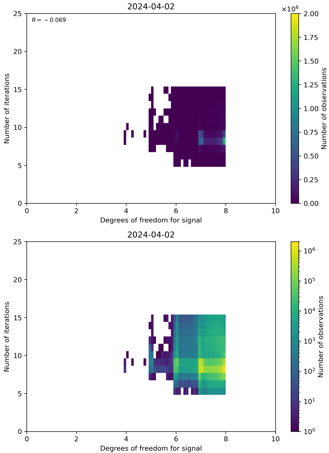
Figure 50: Scatter density plot of “Degrees of freedom for signal” against “Number of iterations” for 2024-04-01 to 2024-04-03.
