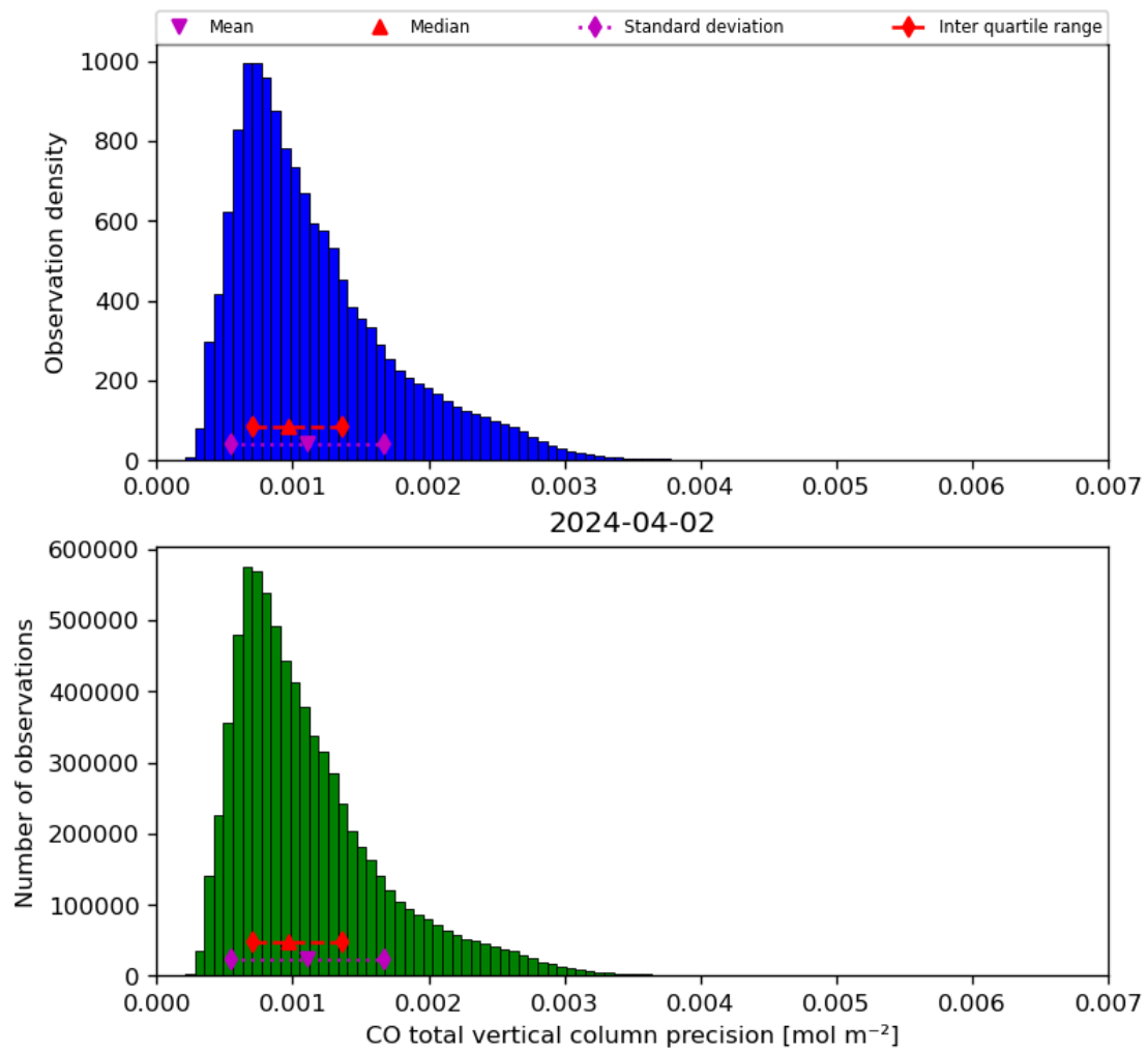
Figure 20: Histogram of “CO total vertical column precision” for 2024-04-01 to 2024-04-03
