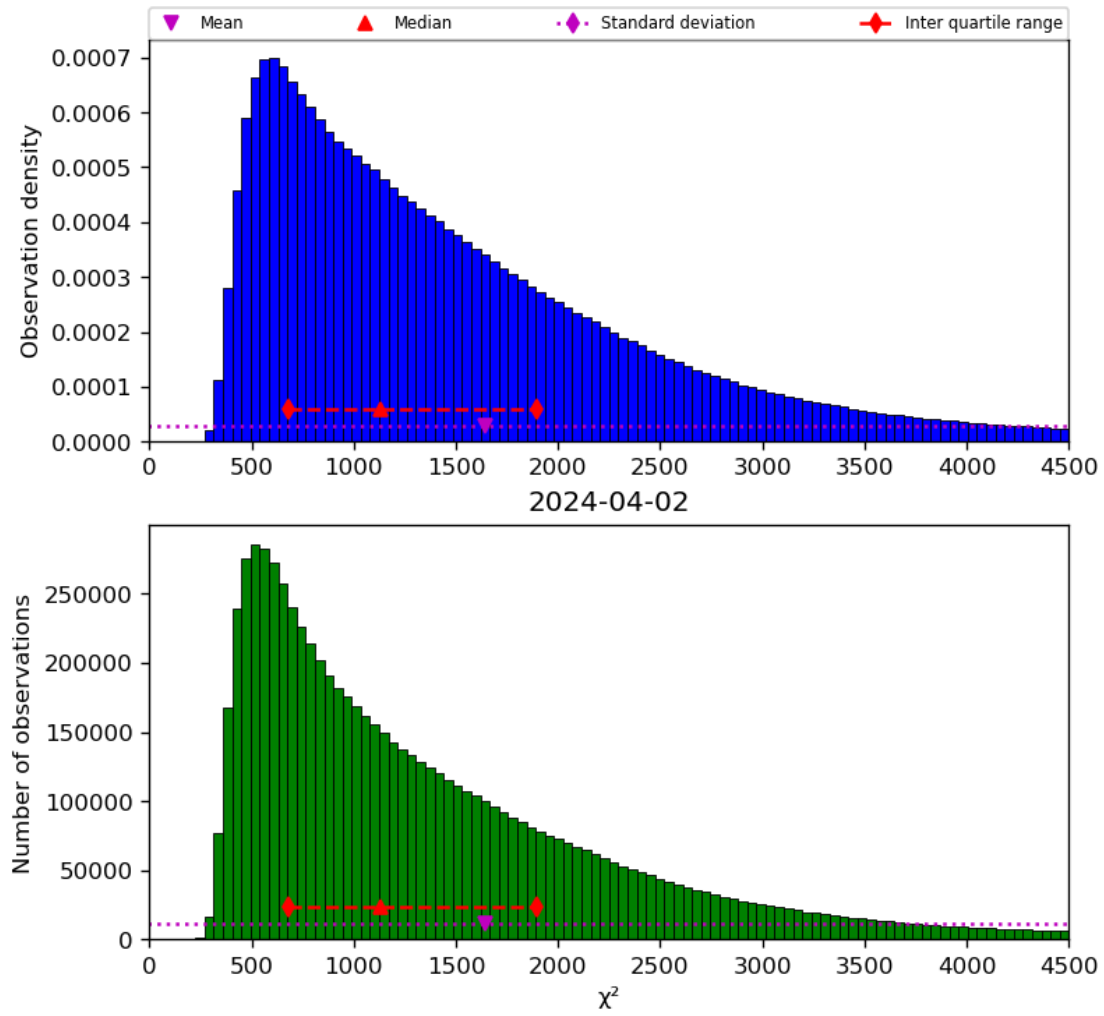
Figure 22: Histogram of " \chi^2 " for 2024-04-01 to 2024-04-03
