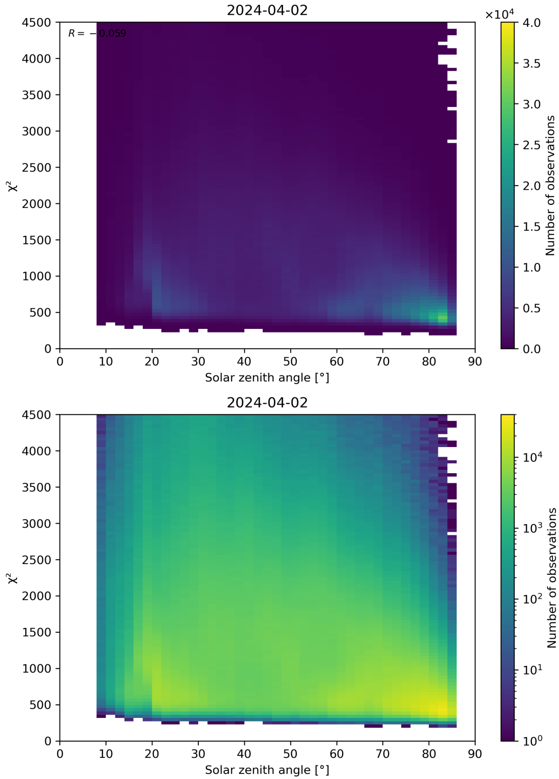
Figure 64: Scatter density plot of “Solar zenith angle” against “ \chi^2 ” for 2024-04-01 to 2024-04-03.
