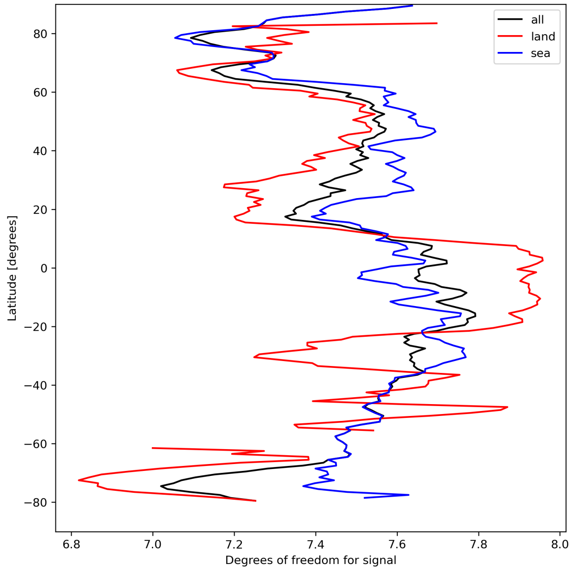
Figure 15: Zonal average of “Degrees of freedom for signal” for 2024-04-01 to 2024-04-03.
