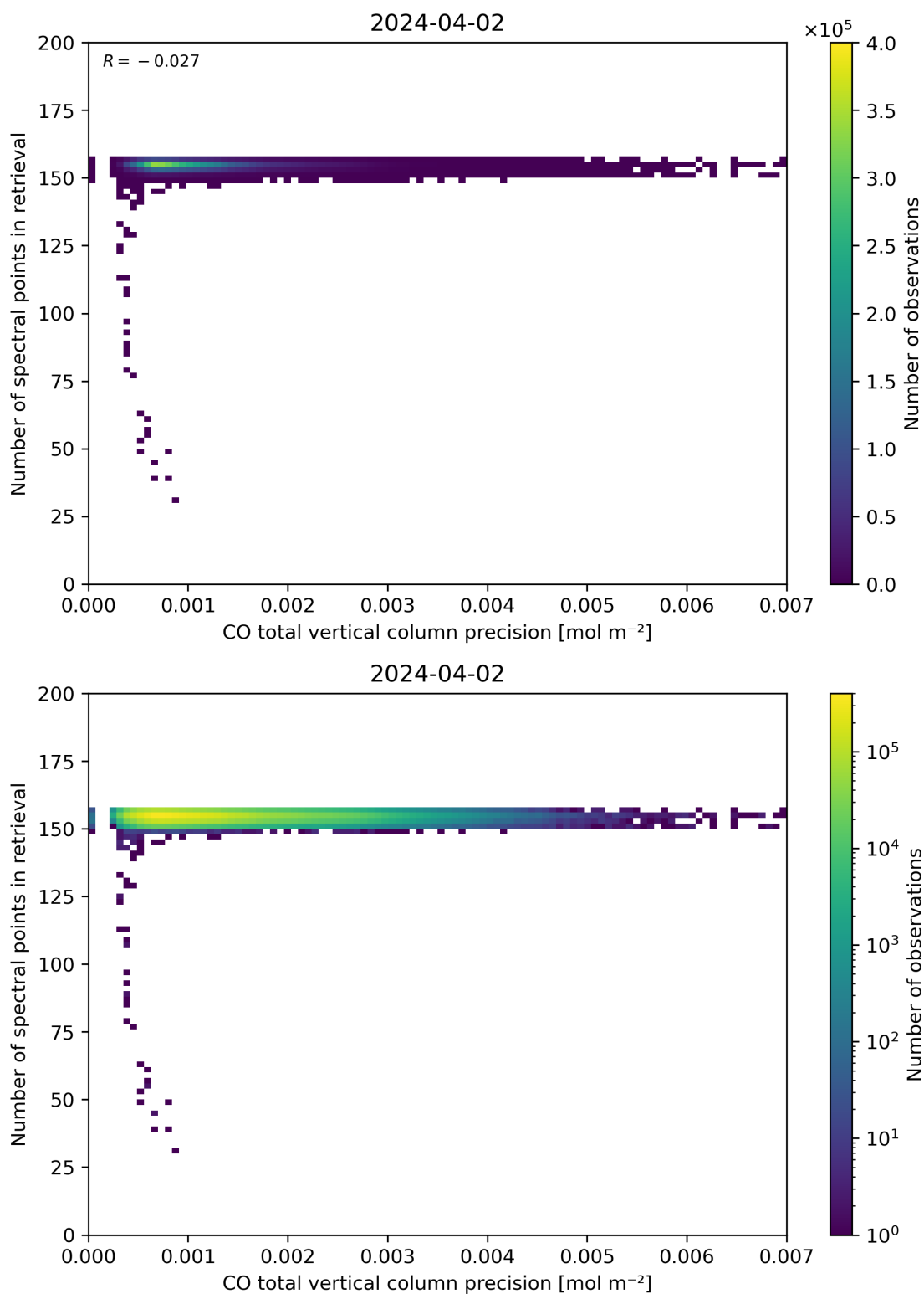
Figure 47: Scatter density plot of “CO total vertical column precision” against “Number of spectral points in retrieval” for 2024-04-01 to 2024-04-03.
