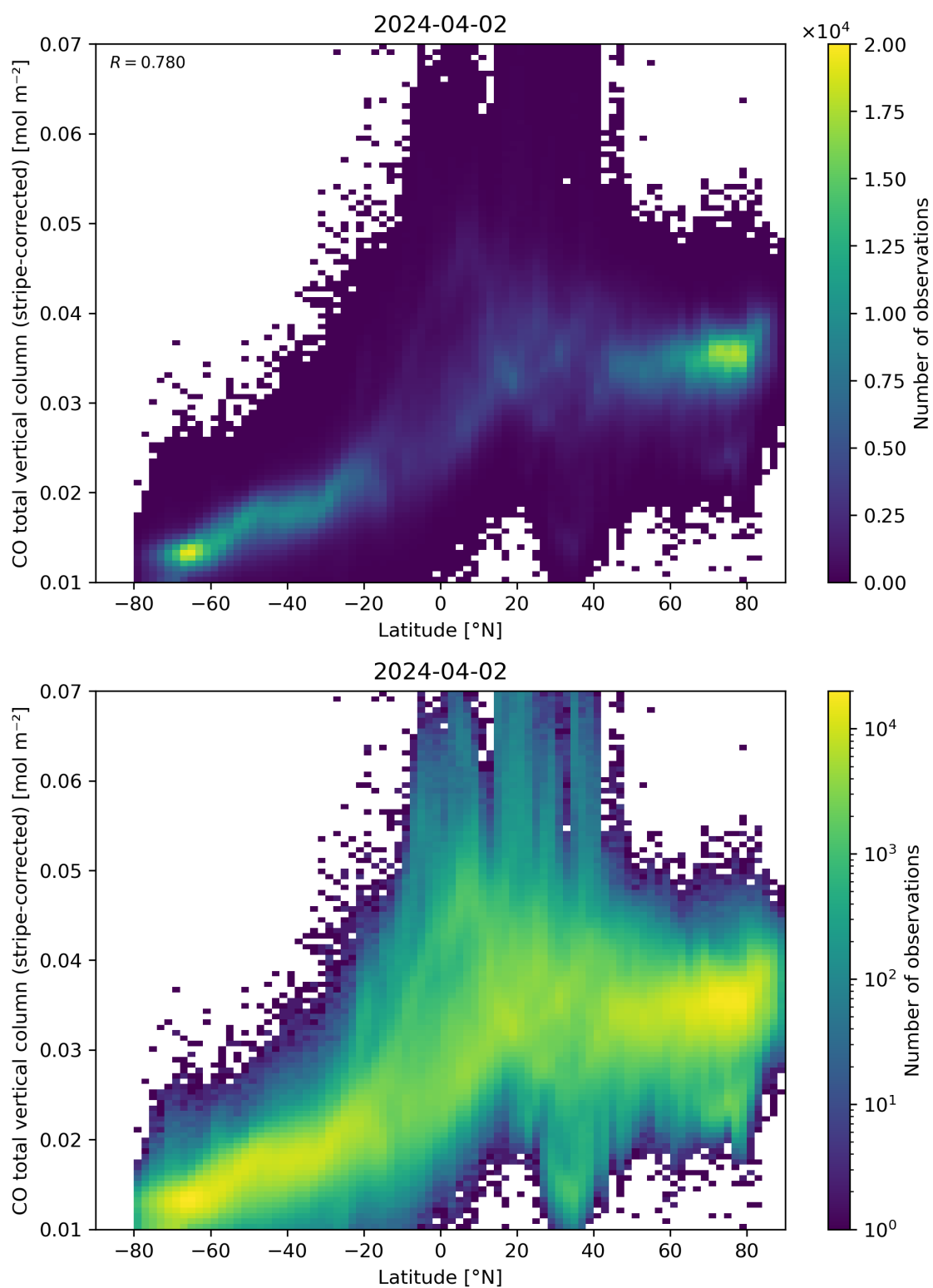
Figure 52: Scatter density plot of “Latitude” against “CO total vertical column (stripe-corrected)” for 2024-04-01 to 2024-04-03.
