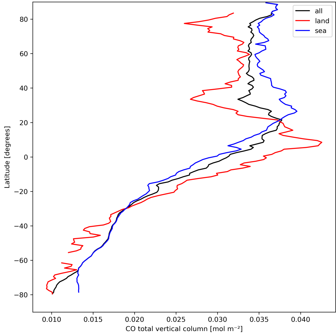
Figure 10: Zonal average of “CO total vertical column” for 2024-04-01 to 2024-04-03.
