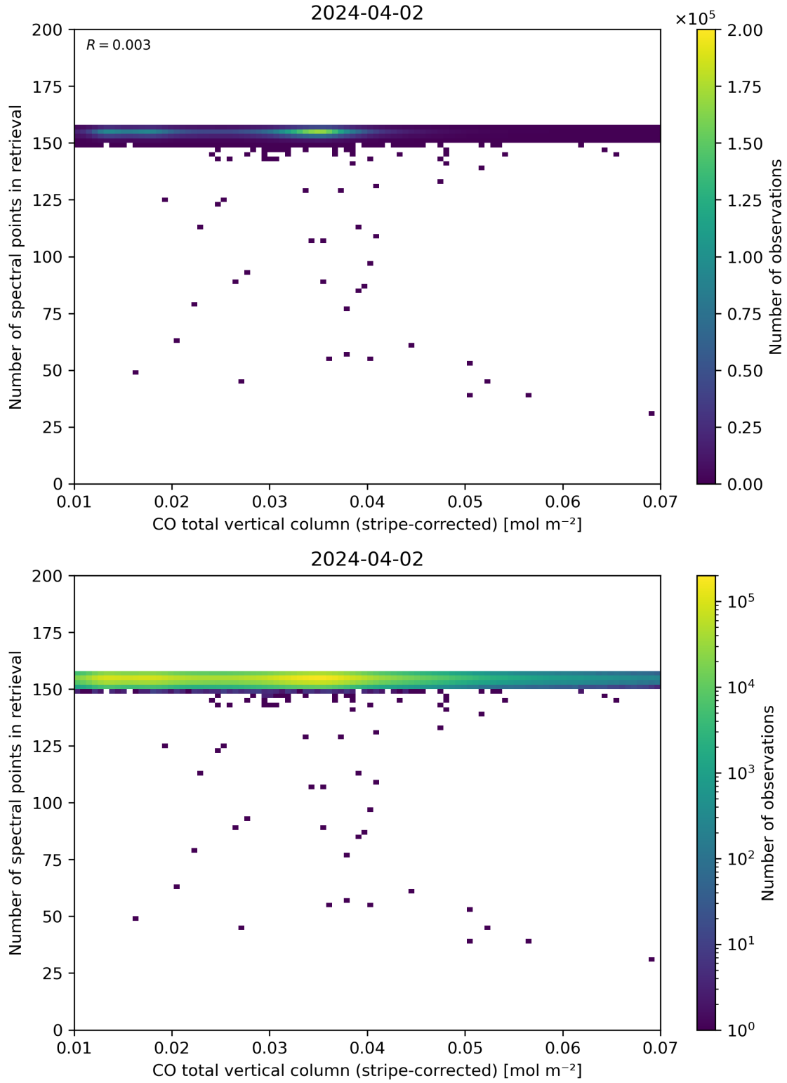
Figure 40: Scatter density plot of “CO total vertical column (stripe-corrected)” against “Number of spectral points in retrieval” for 2024-04-01 to 2024-04-03.
