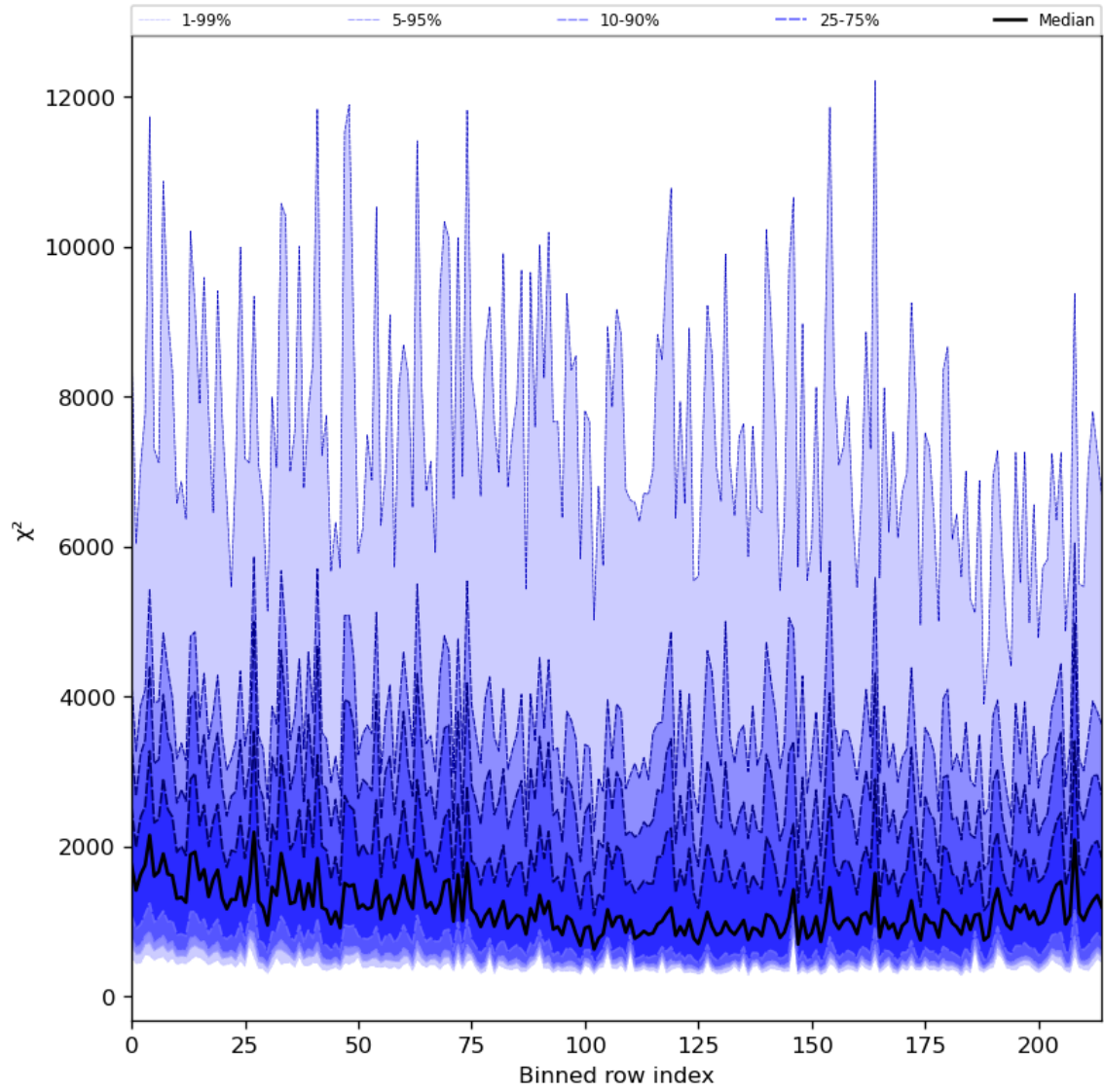
Figure 30: Along track statistics of “ \chi^2 ” for 2024-04-01 to 2024-04-03
