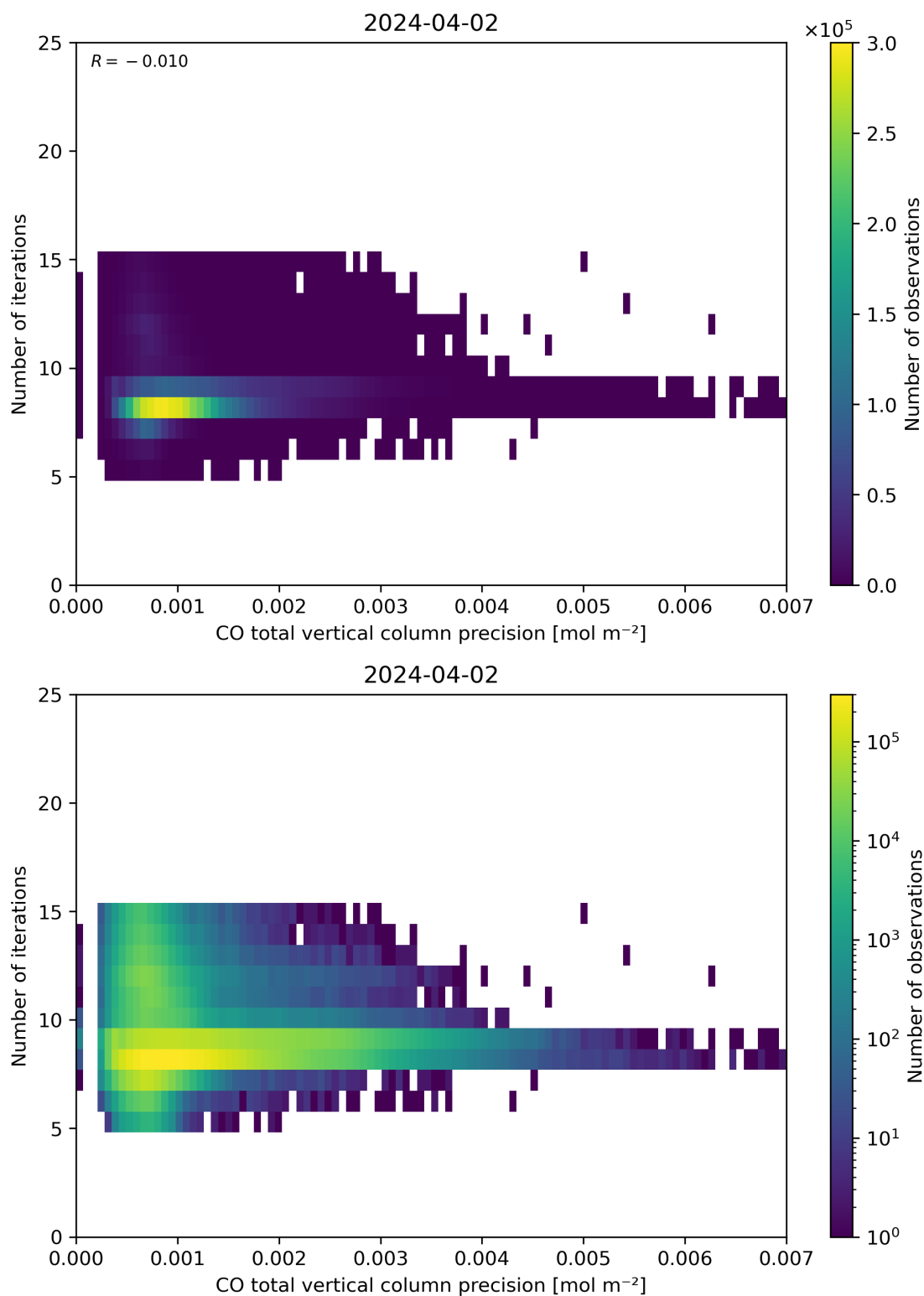
Figure 46: Scatter density plot of “CO total vertical column precision” against “Number of iterations” for 2024-04-01 to 2024-04-03.
