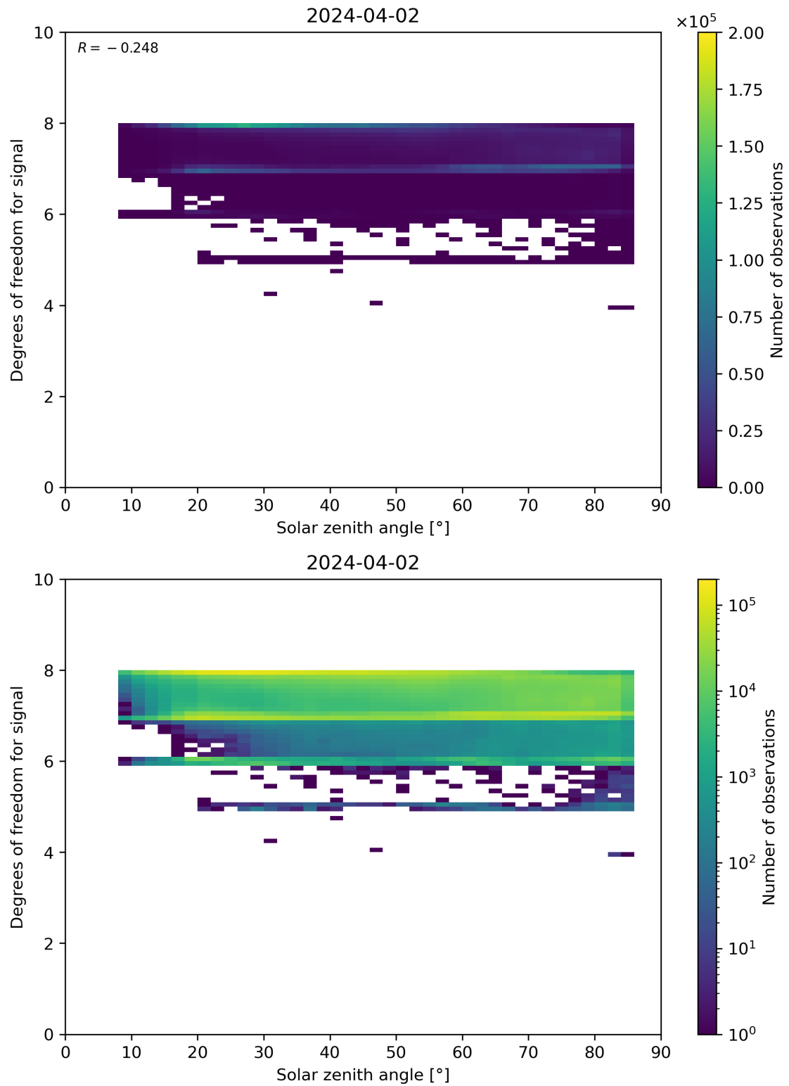
Figure 65: Scatter density plot of “Solar zenith angle” against “Degrees of freedom for signal” for 2024-04-01 to 2024-04-03.
