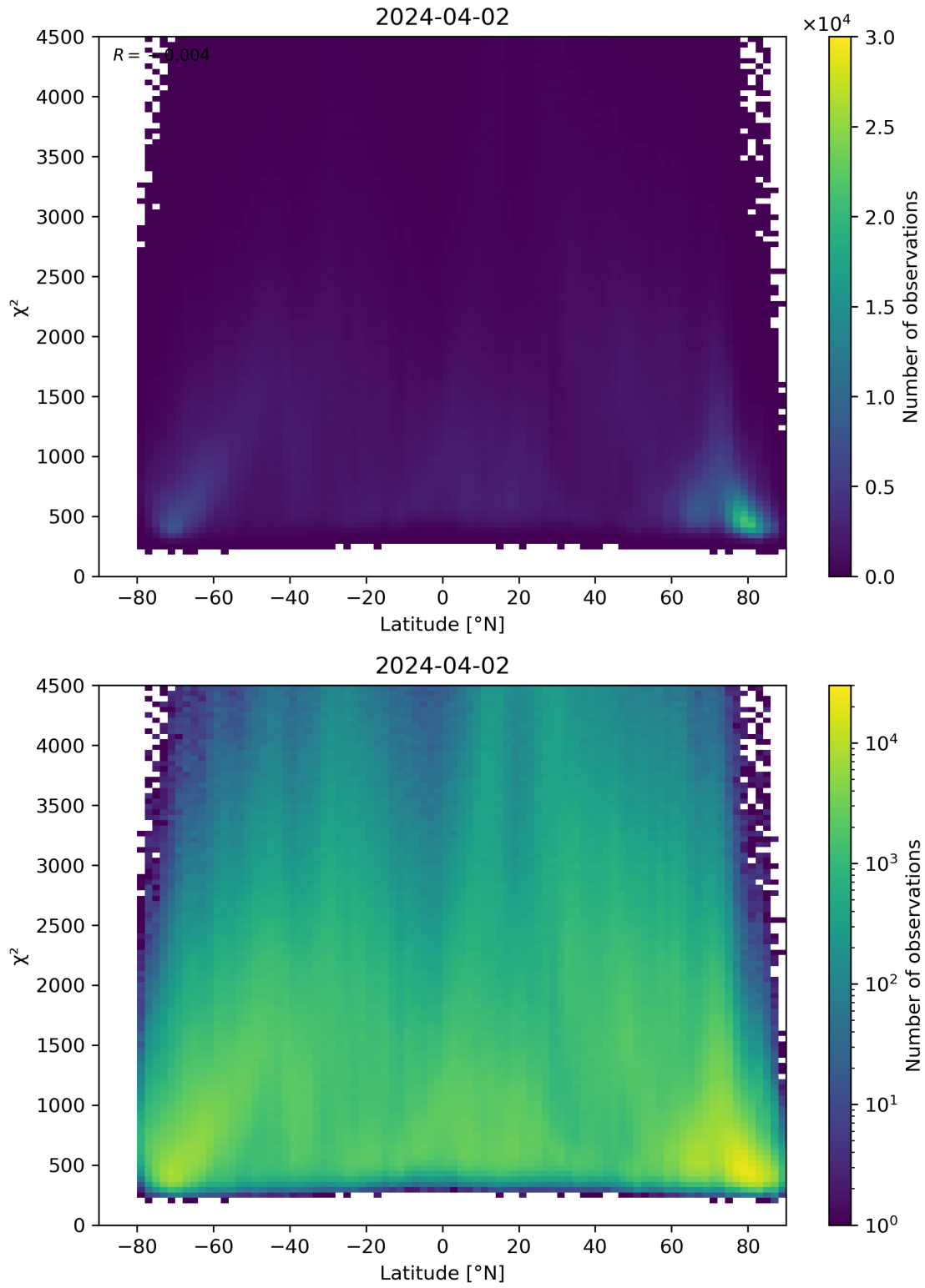
Figure 54: Scatter density plot of “Latitude” against “ \chi^2 ” for 2024-04-01 to 2024-04-03.
