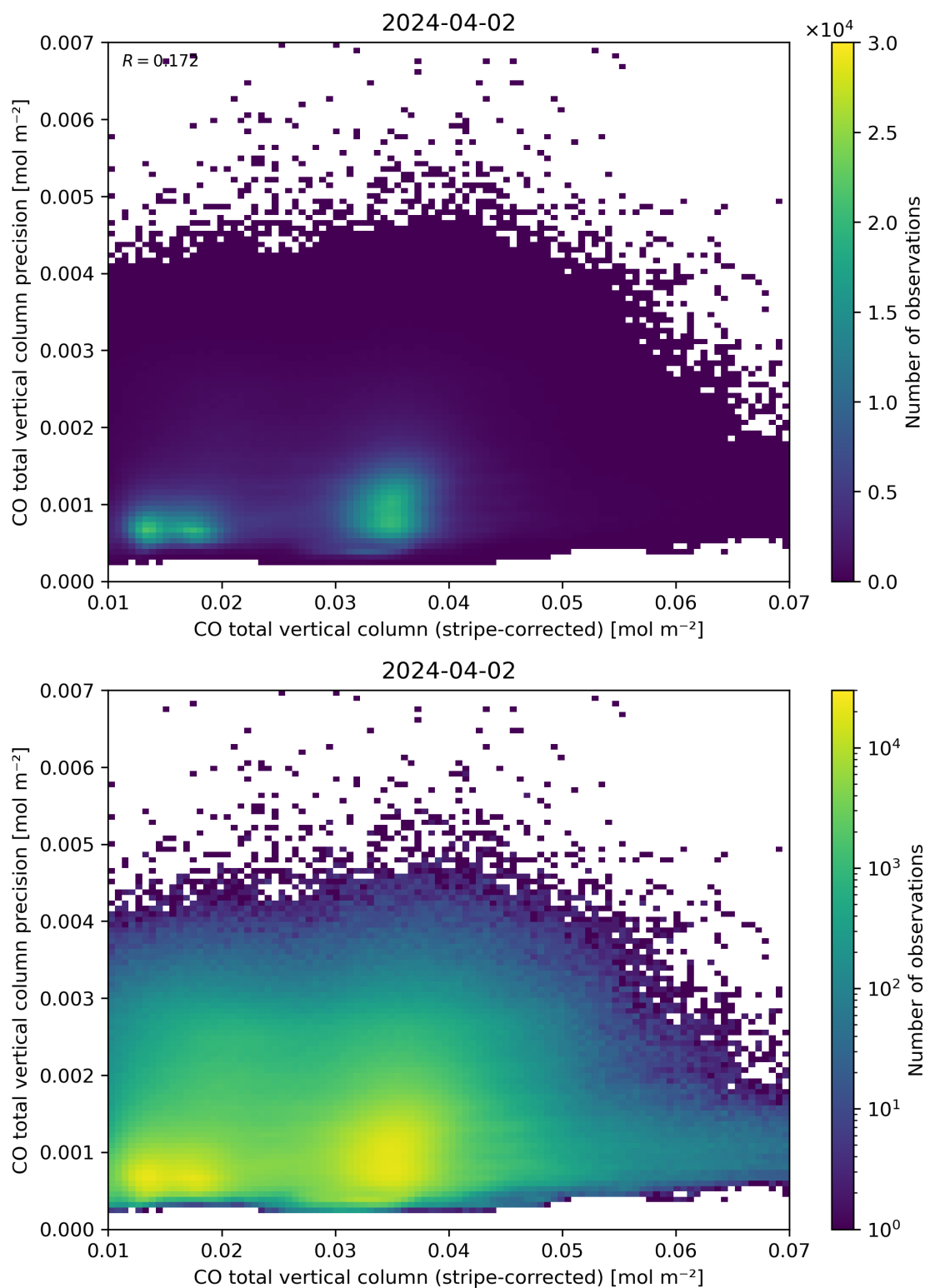
Figure 36: Scatter density plot of “CO total vertical column (stripe-corrected)” against “CO total vertical column precision” for 2024-04-01 to 2024-04-03.
