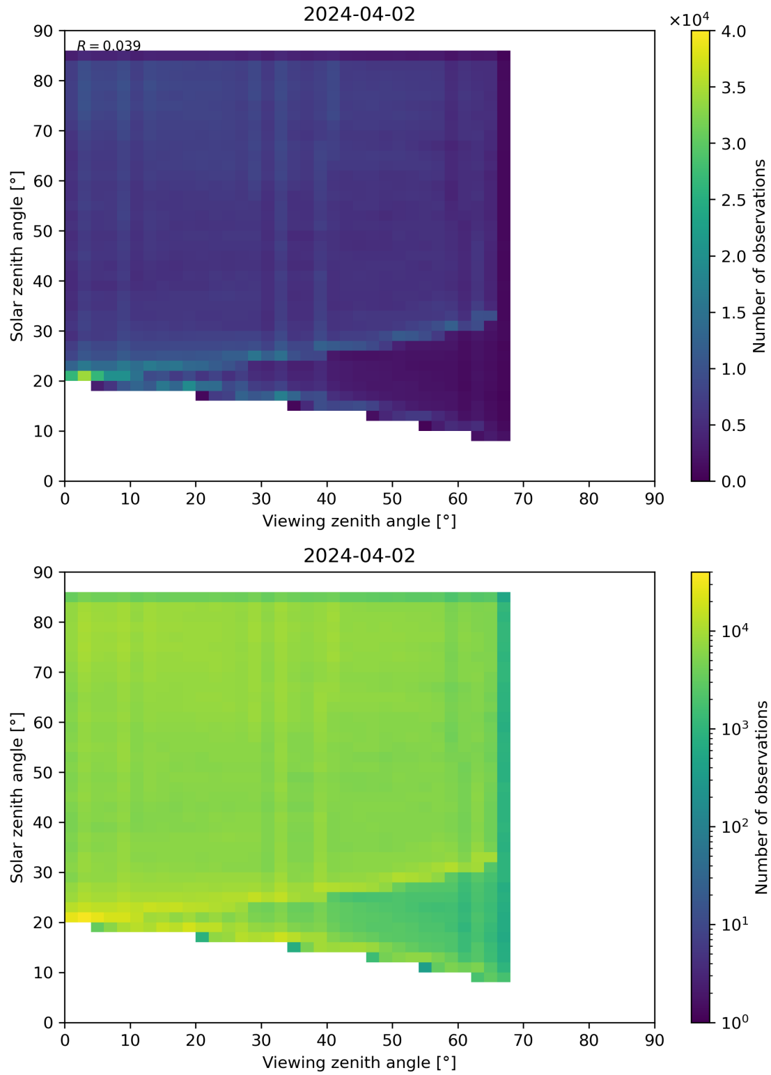
Figure 77: Scatter density plot of “Viewing zenith angle” against “Solar zenith angle” for 2024-04-01 to 2024-04-03.
