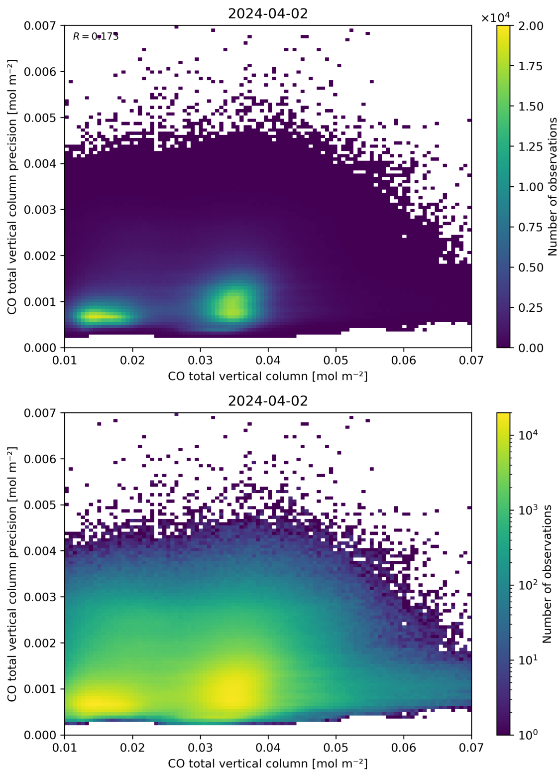
Figure 34: Scatter density plot of “CO total vertical column” against “CO total vertical column precision” for 2024-04-01 to 2024-04-03.
