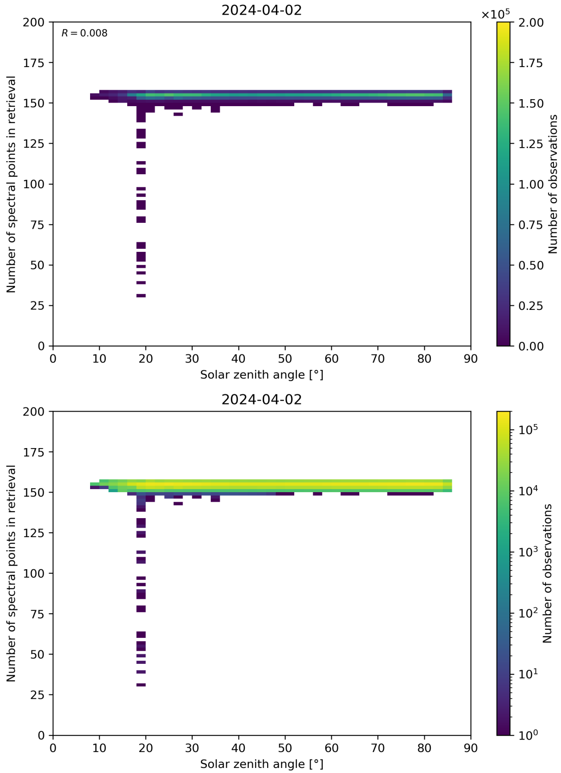
Figure 68: Scatter density plot of “Solar zenith angle” against “Number of spectral points in retrieval” for 2024-04-01 to 2024-04-03.
