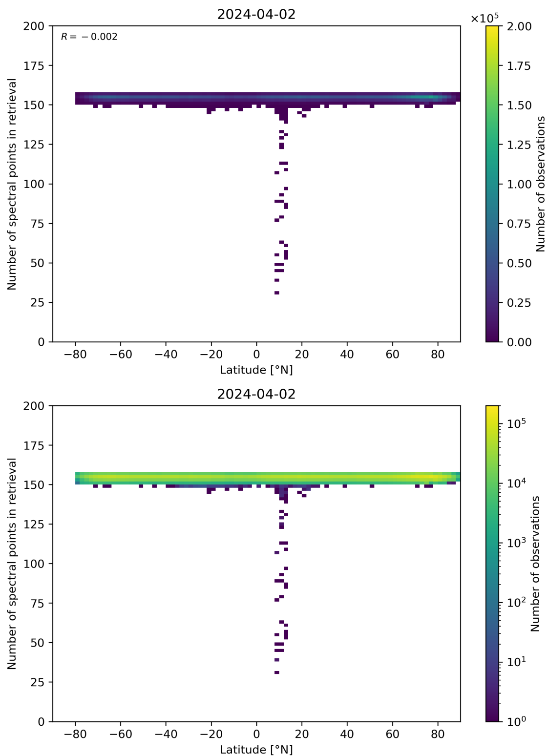
Figure 57: Scatter density plot of “Latitude” against “Number of spectral points in retrieval” for 2024-04-01 to 2024-04-03.
