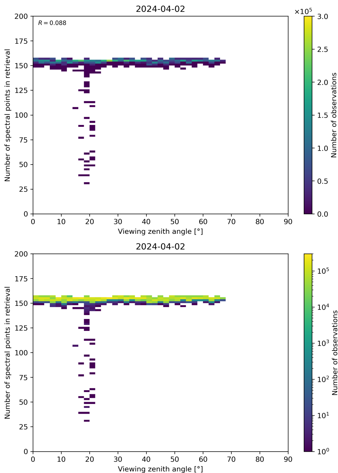
Figure 76: Scatter density plot of “Viewing zenith angle” against “Number of spectral points in retrieval” for 2024-04-01 to 2024-04-03.
