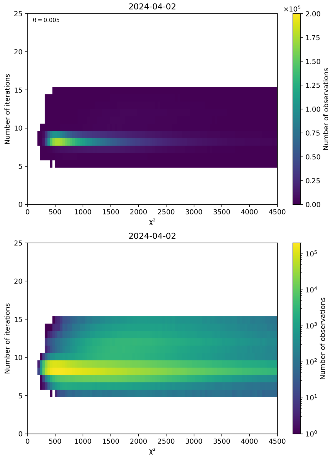
Figure 49: Scatter density plot of “ \chi^2 ” against “Number of iterations” for 2024-04-01 to 2024-04-03.
