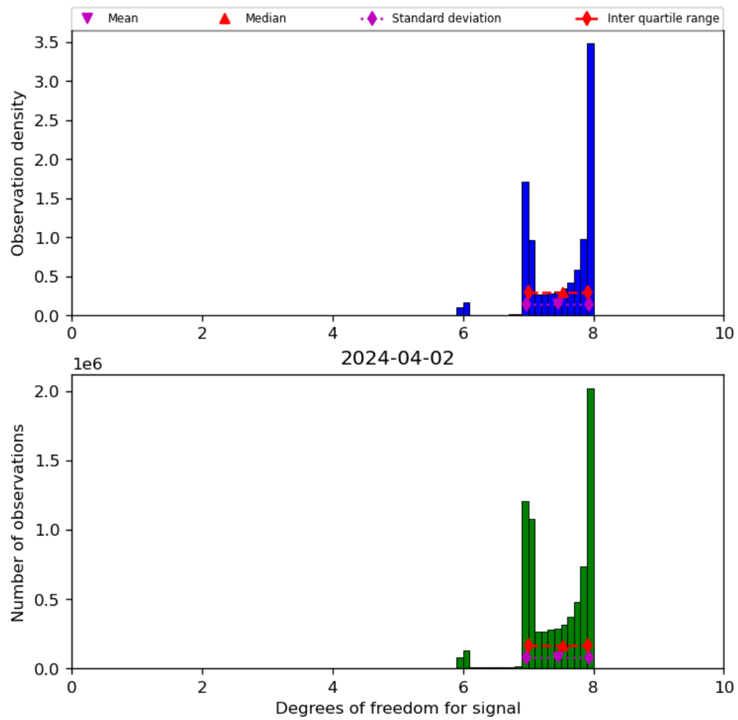
Figure 23: Histogram of “Degrees of freedom for signal” for 2024-04-01 to 2024-04-03
