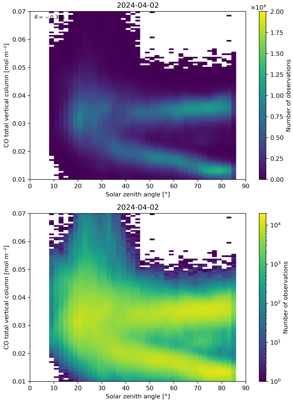
Figure 61: Scatter density plot of “Solar zenith angle” against “CO total vertical column” for 2024-04-01 to 2024-04-03.
