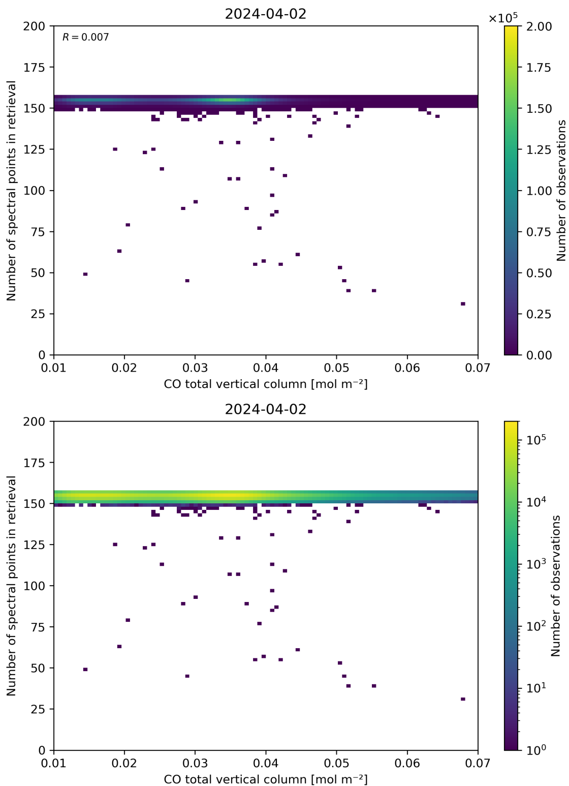
Figure 43: Scatter density plot of “CO total vertical column” against “Number of spectral points in retrieval” for 2024-04-01 to 2024-04-03.
