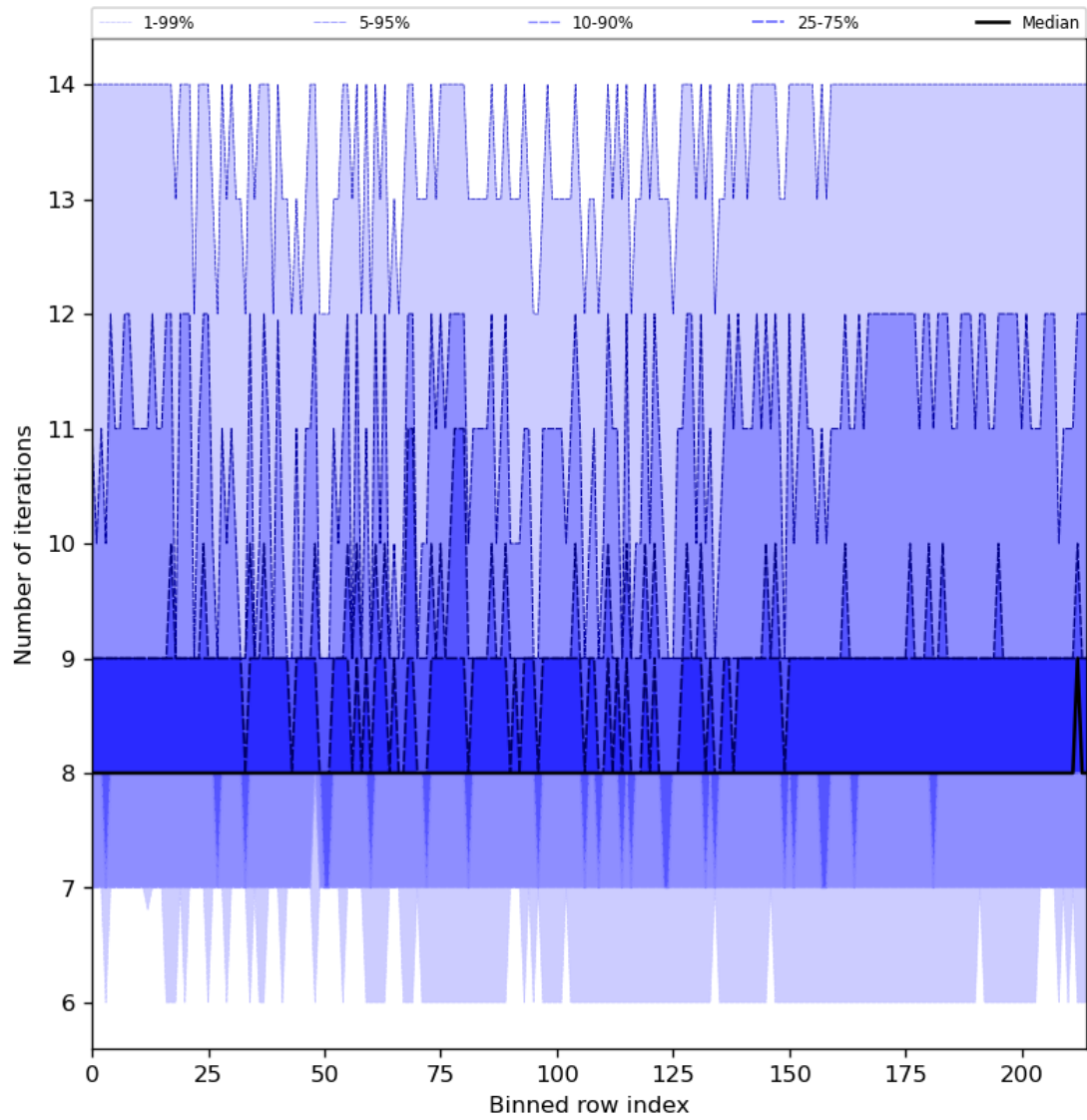
Figure 32: Along track statistics of “Number of iterations” for 2024-04-01 to 2024-04-03
