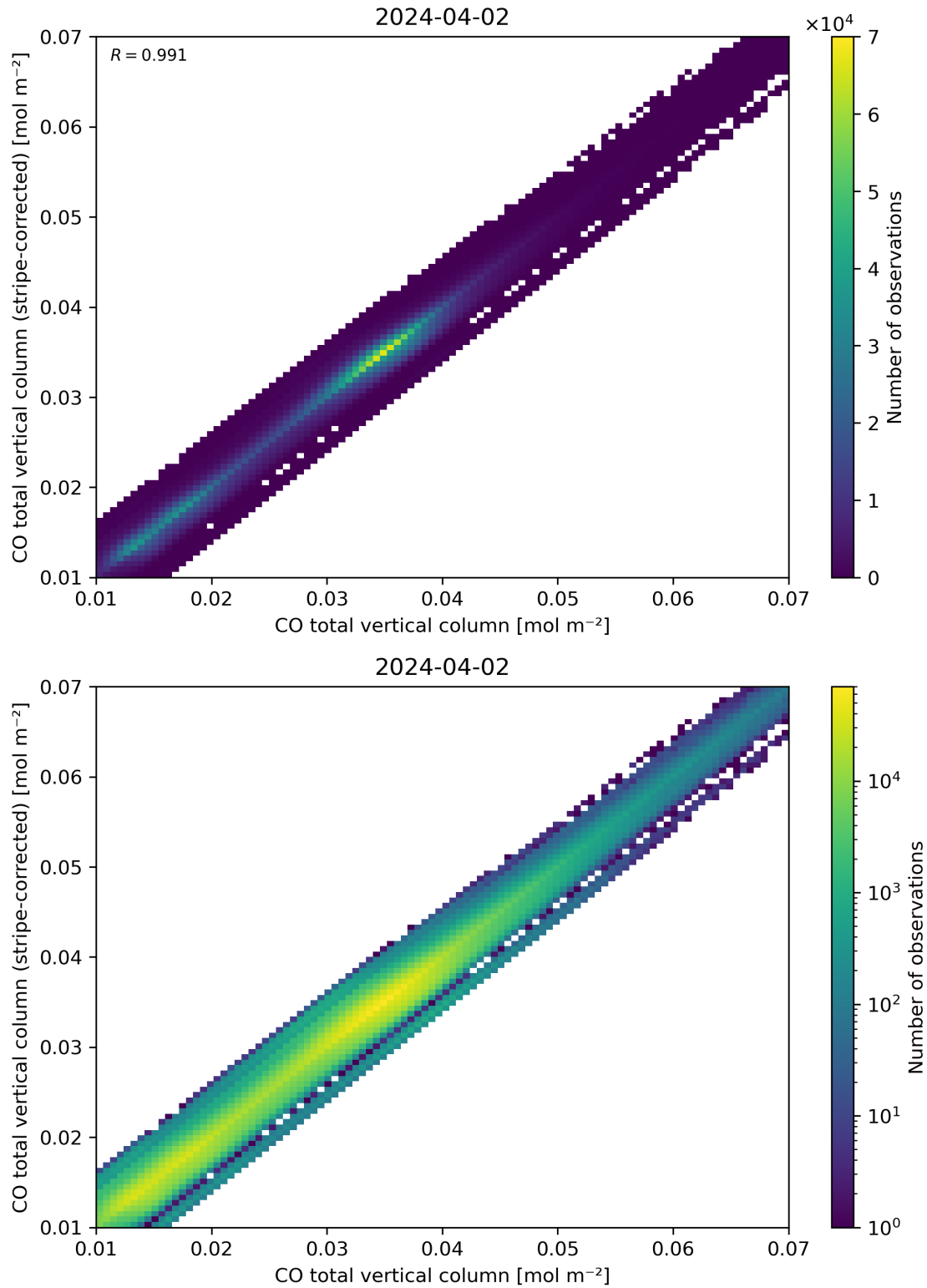
Figure 33: Scatter density plot of “CO total vertical column” against “CO total vertical column (stripe-corrected)” for 2024-04-01 to 2024-04-03.
