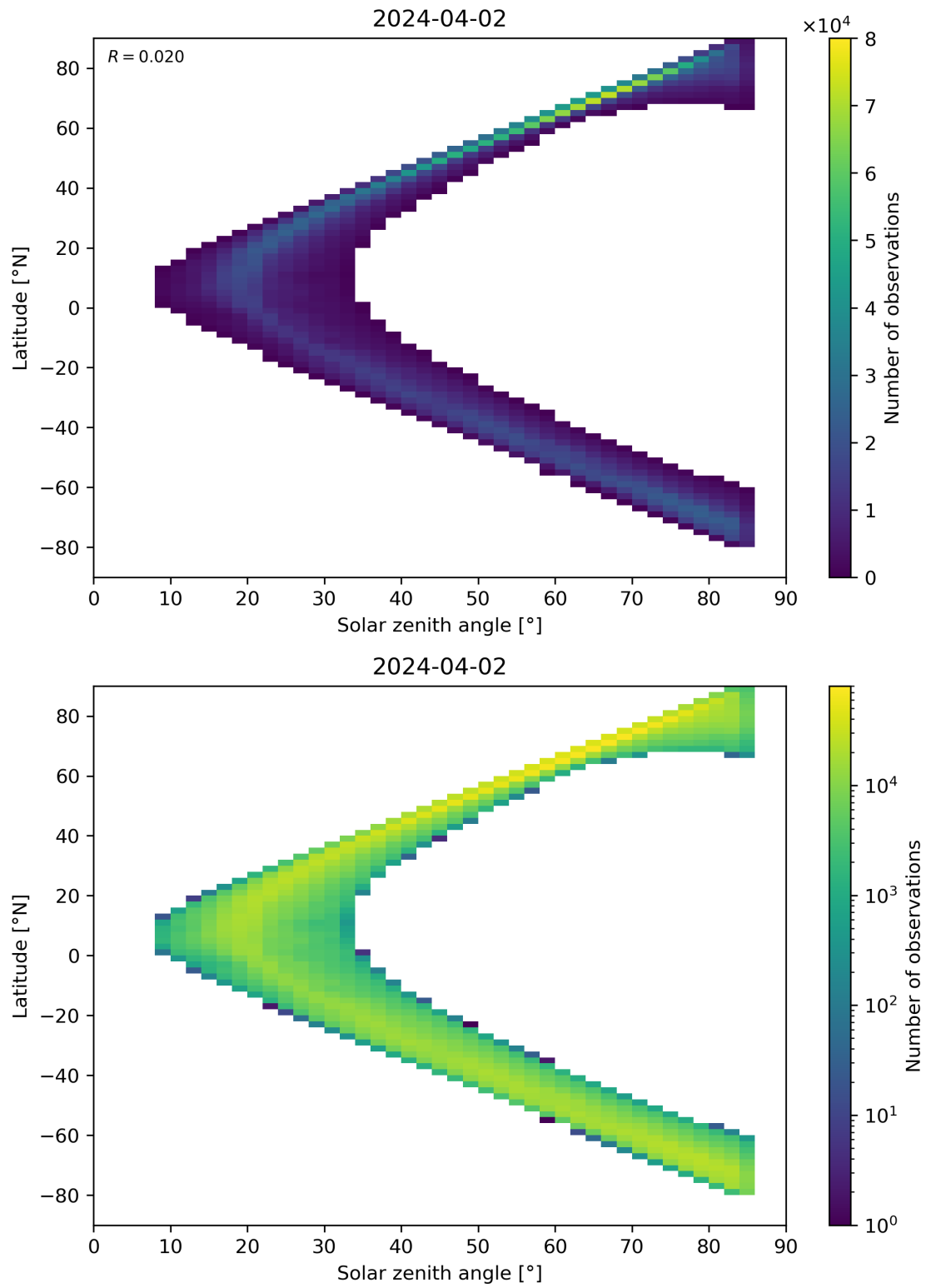
Figure 66: Scatter density plot of “Solar zenith angle” against “Latitude” for 2024-04-01 to 2024-04-03.
