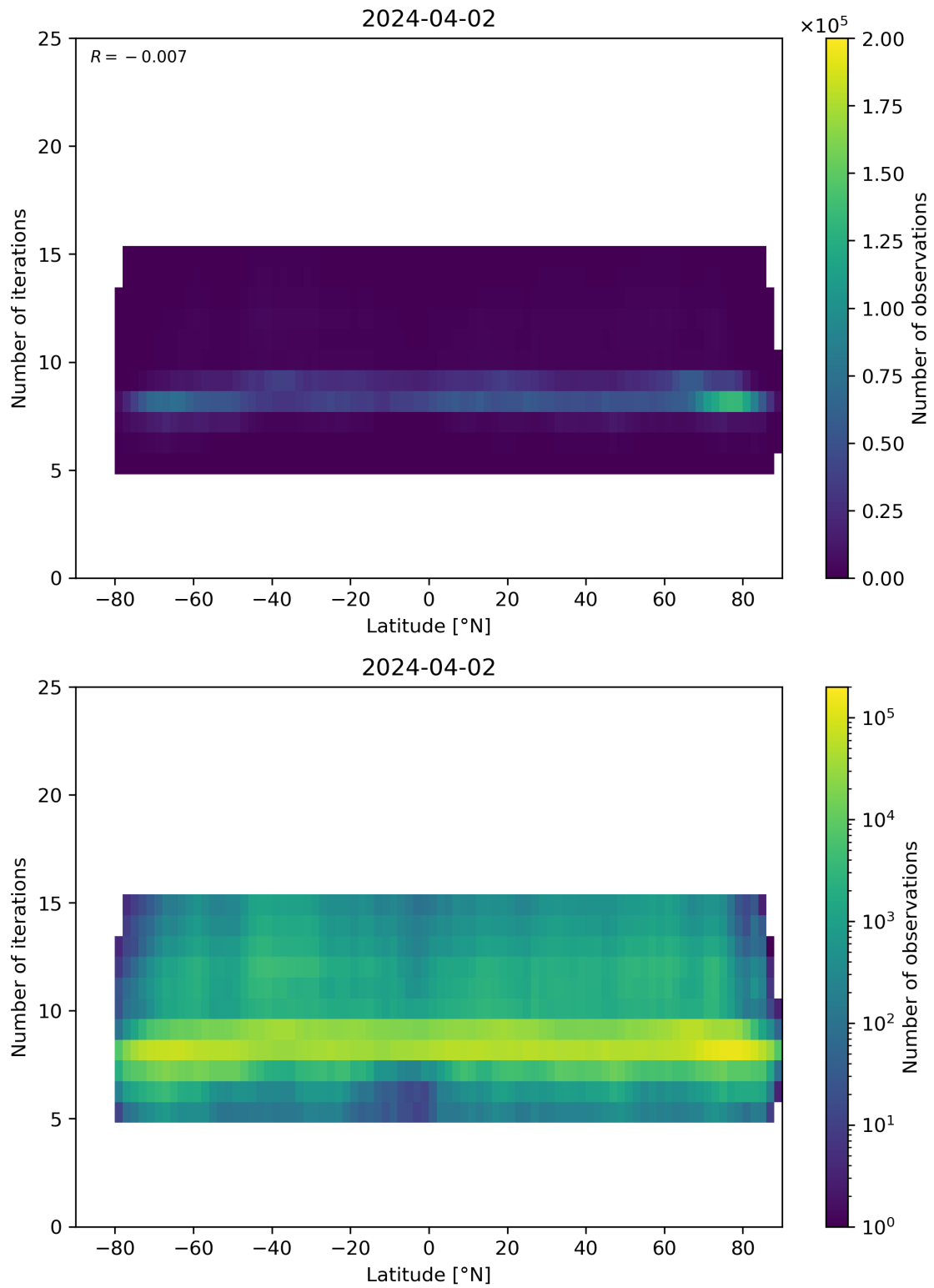
Figure 56: Scatter density plot of “Latitude” against “Number of iterations” for 2024-04-01 to 2024-04-03.
