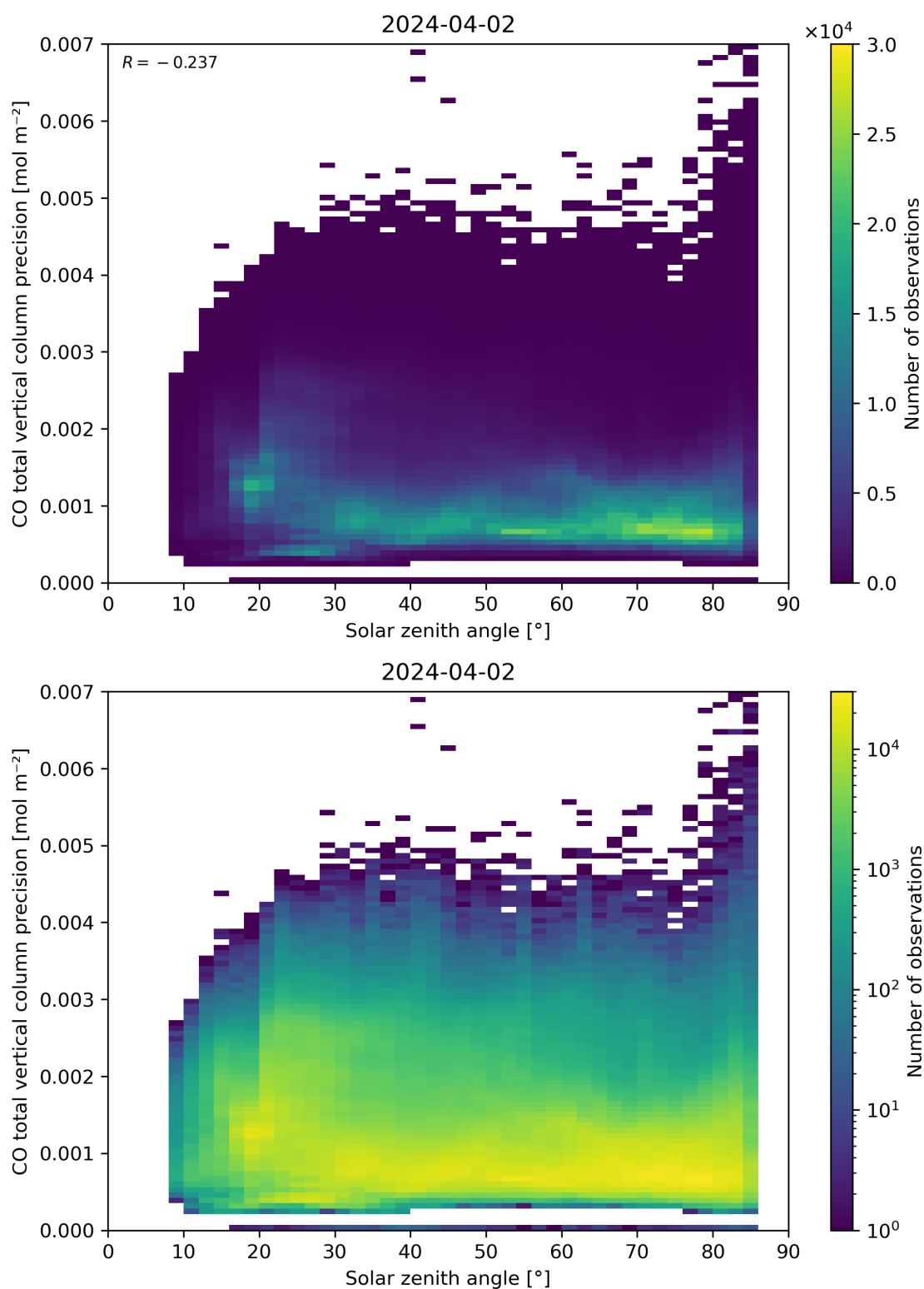
Figure 63: Scatter density plot of “Solar zenith angle” against “CO total vertical column precision” for 2024-04-01 to 2024-04-03.
