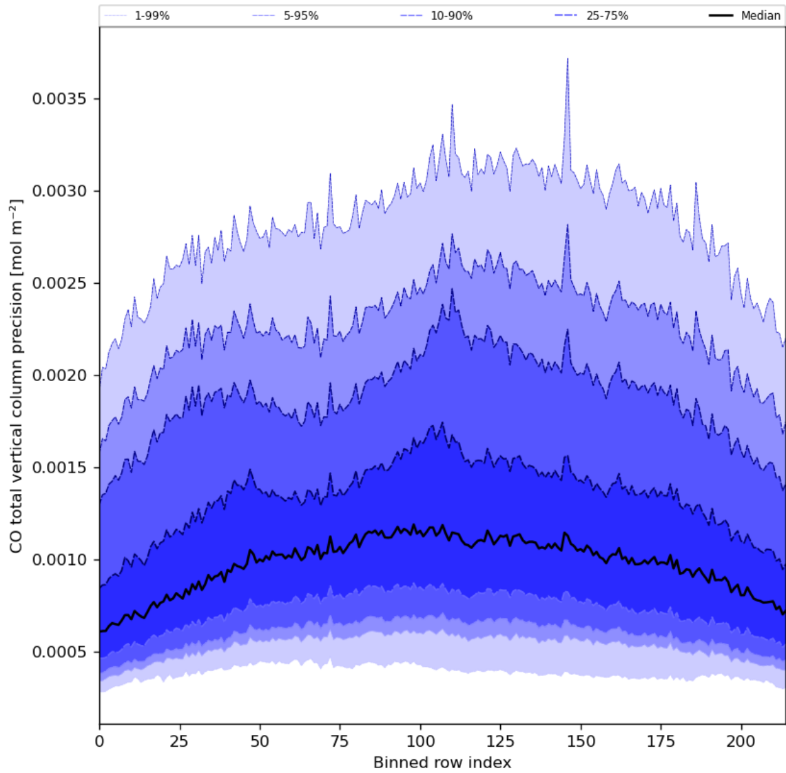
Figure 28: Along track statistics of “CO total vertical column precision” for 2024-04-01 to 2024-04-03
