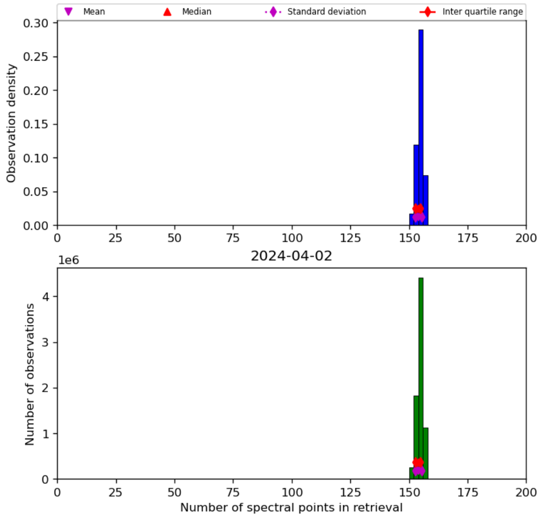
Figure 21: Histogram of “Number of spectral points in retrieval” for 2024-04-01 to 2024-04-03
