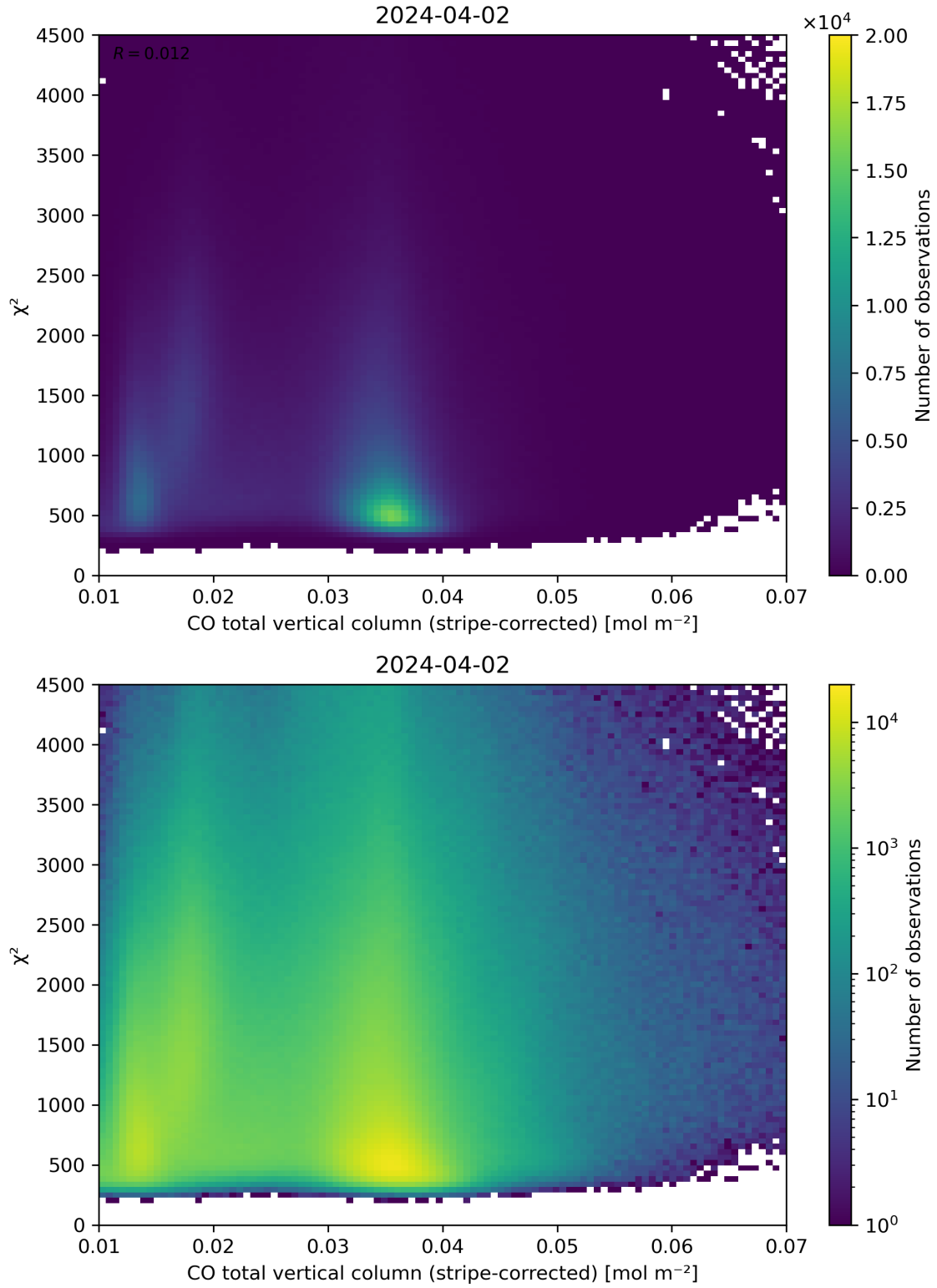
Figure 37: Scatter density plot of “CO total vertical column (stripe-corrected)” against “ \chi^2 ” for 2024-04-01 to 2024-04-03.
