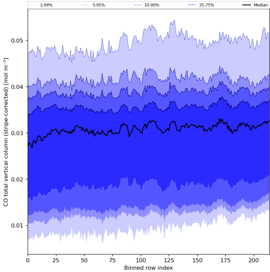
Figure 27: Along track statistics of “CO total vertical column (stripe-corrected)” for 2024-04-01 to 2024-04-03
