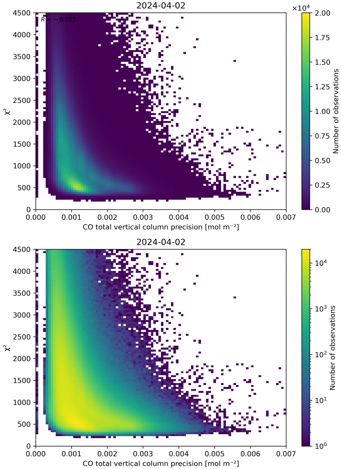
Figure 44: Scatter density plot of “CO total vertical column precision” against “ \chi^2 ” for 2024-04-01 to 2024-04-03.
