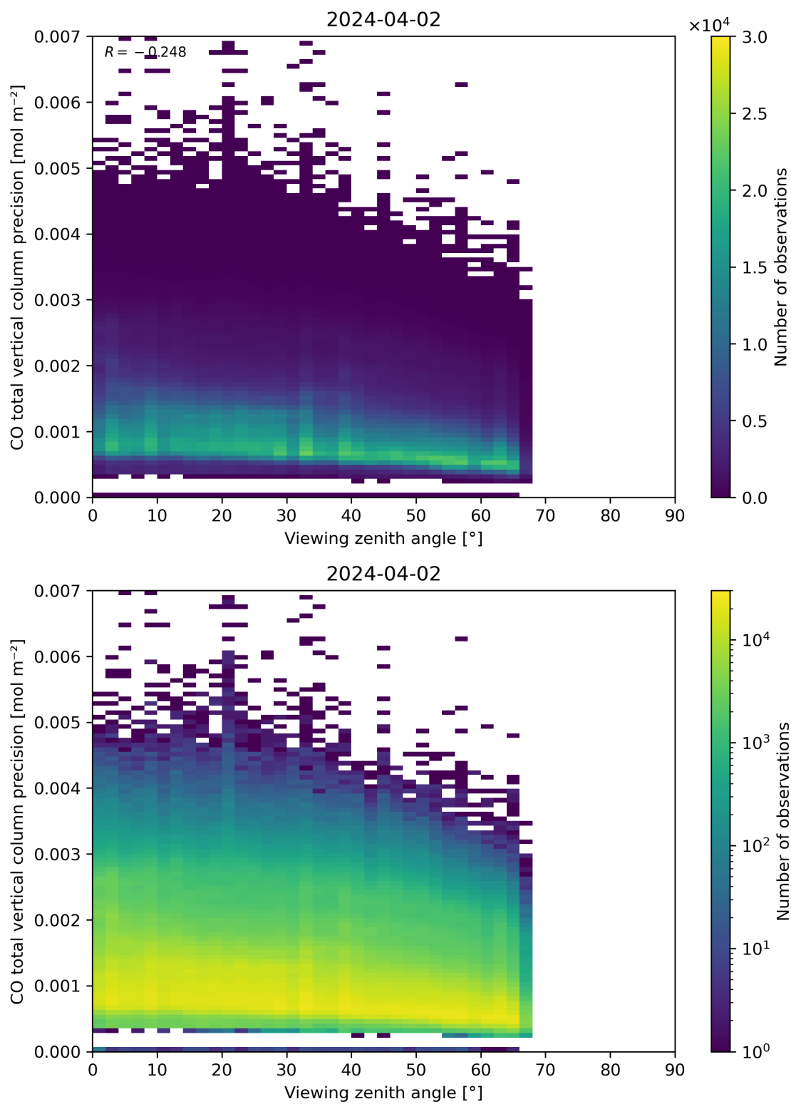
Figure 71: Scatter density plot of “Viewing zenith angle” against “CO total vertical column precision” for 2024-04-01 to 2024-04-03.
