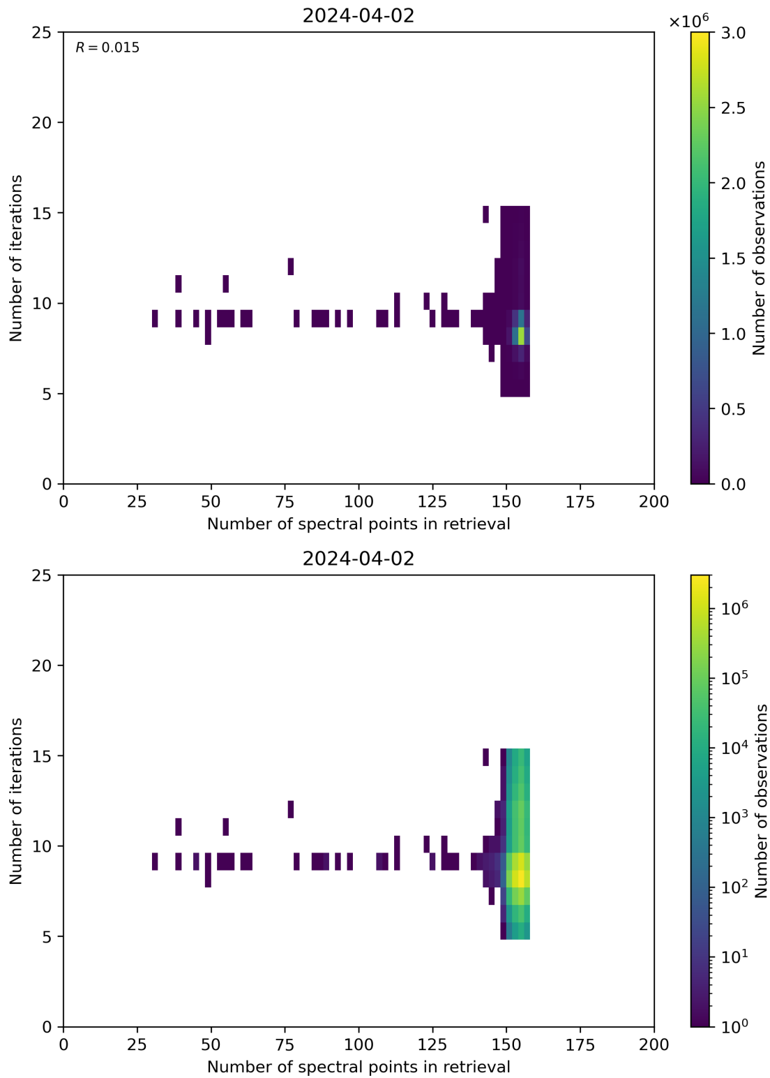
Figure 60: Scatter density plot of “Number of spectral points in retrieval” against “Number of iterations” for 2024-04-01 to 2024-04-03.
