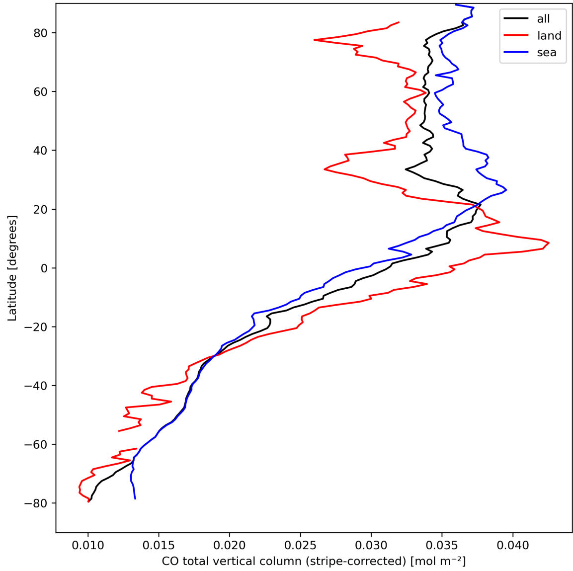
Figure 11: Zonal average of “CO total vertical column (stripe-corrected)” for 2024-04-01 to 2024-04-03.
