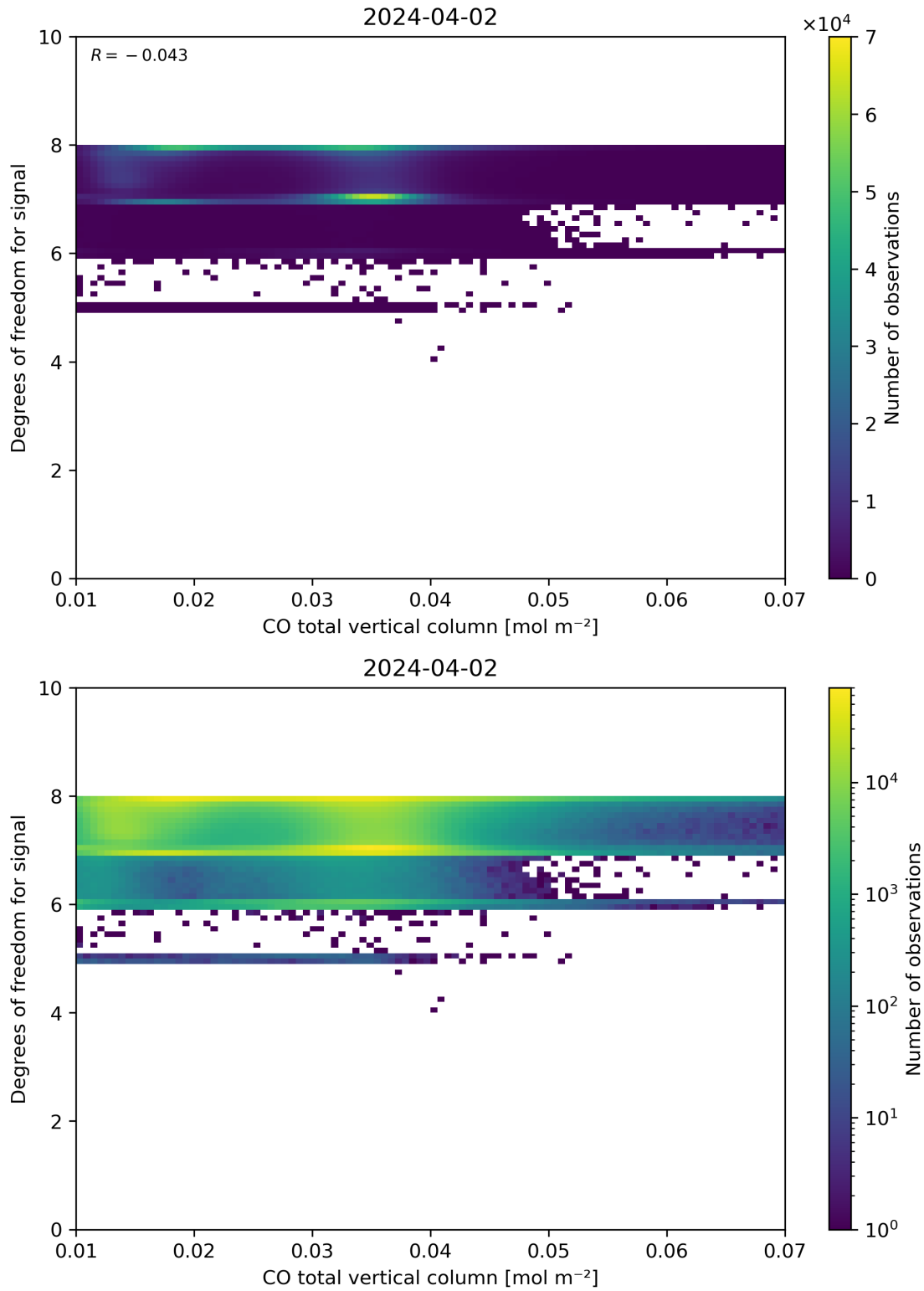
Figure 41: Scatter density plot of “CO total vertical column” against “Degrees of freedom for signal” for 2024-04-01 to 2024-04-03.
