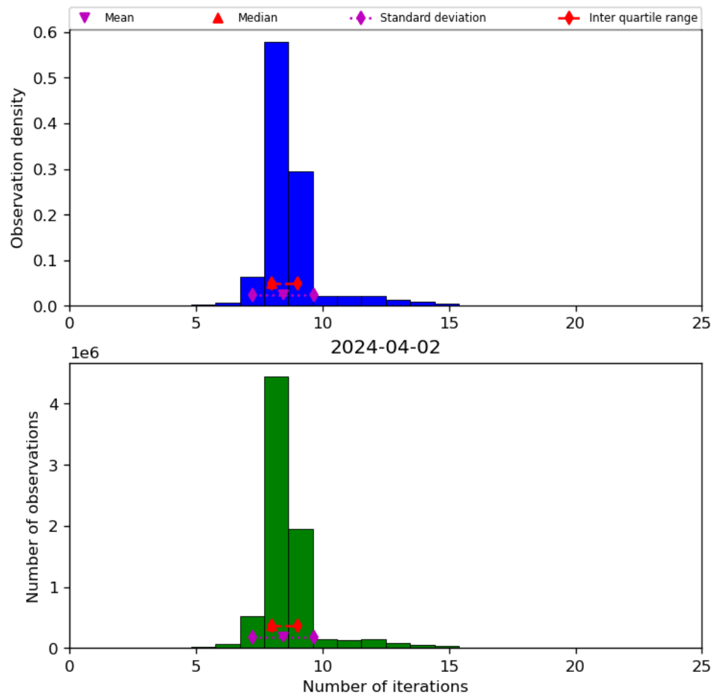
Figure 24: Histogram of “Number of iterations” for 2024-04-01 to 2024-04-03
