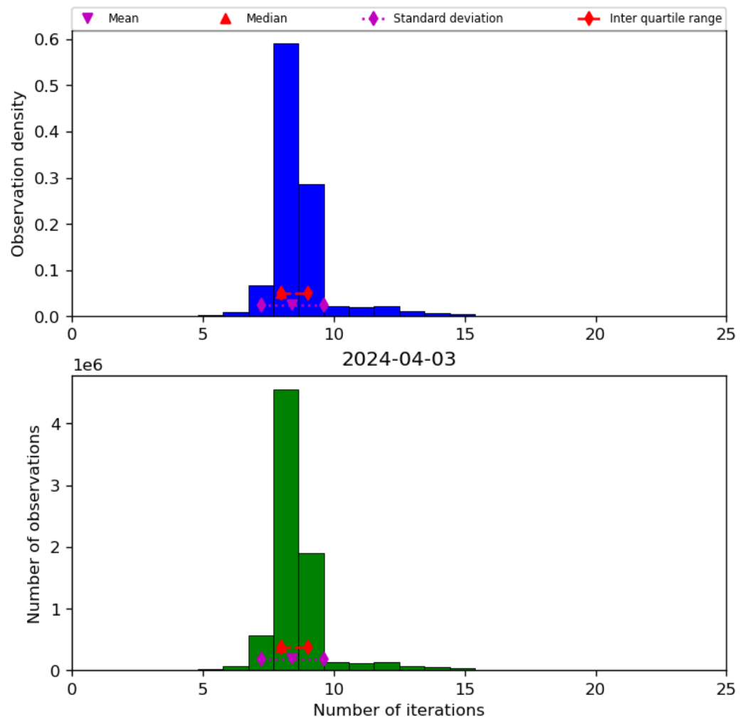
Figure 24: Histogram of “Number of iterations” for 2024-04-02 to 2024-04-04
