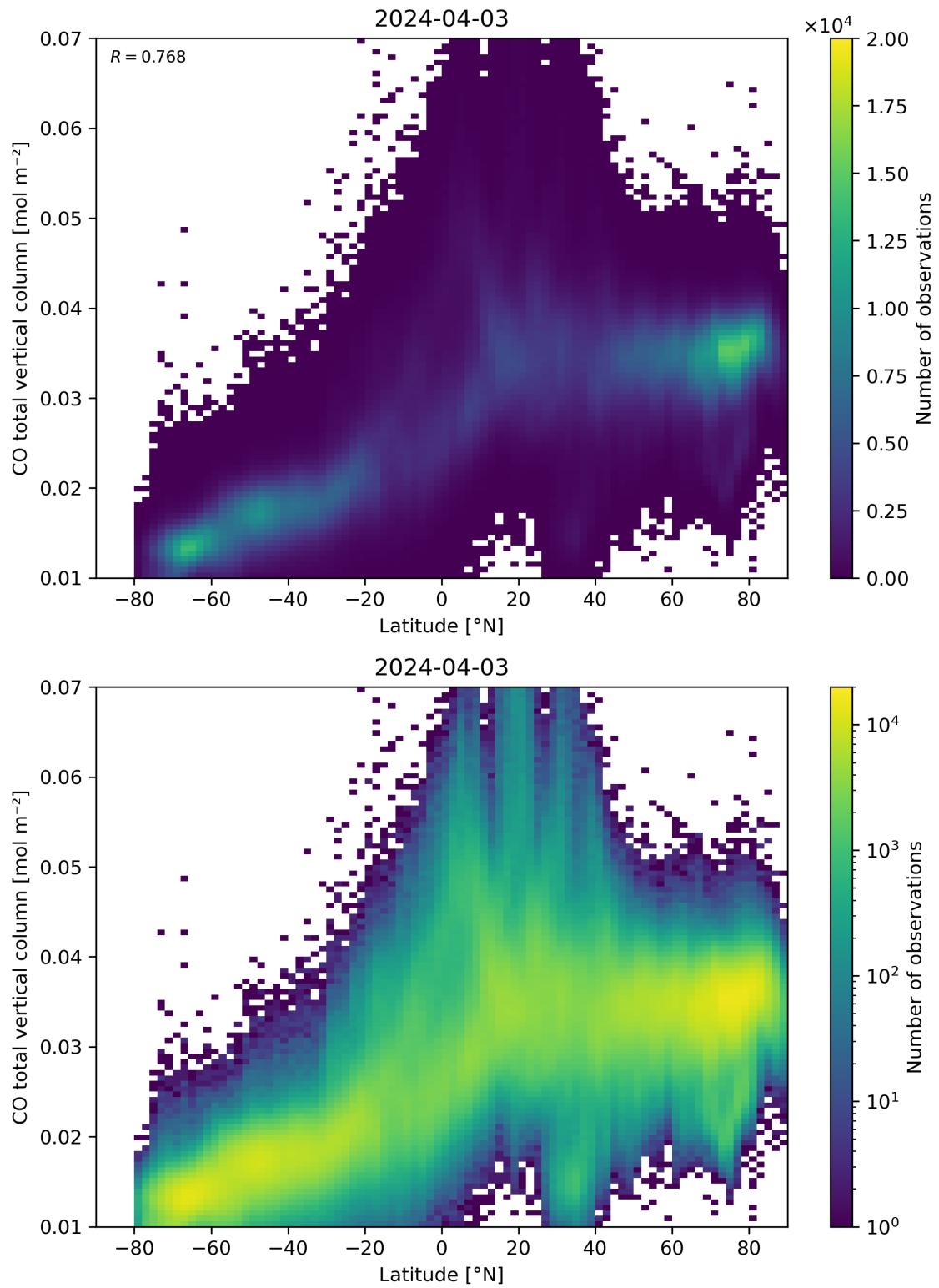
Figure 51: Scatter density plot of “Latitude” against “CO total vertical column” for 2024-04-02 to 2024-04-04.
