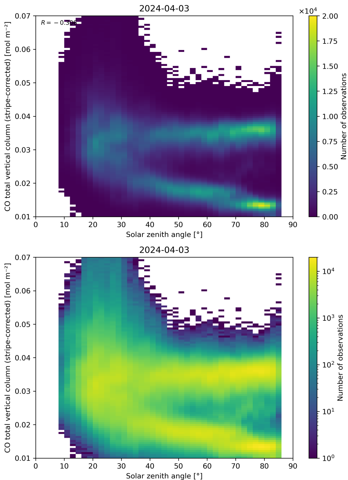
Figure 62: Scatter density plot of “Solar zenith angle” against “CO total vertical column (stripe-corrected)” for 2024-04-02 to 2024-04-04.
