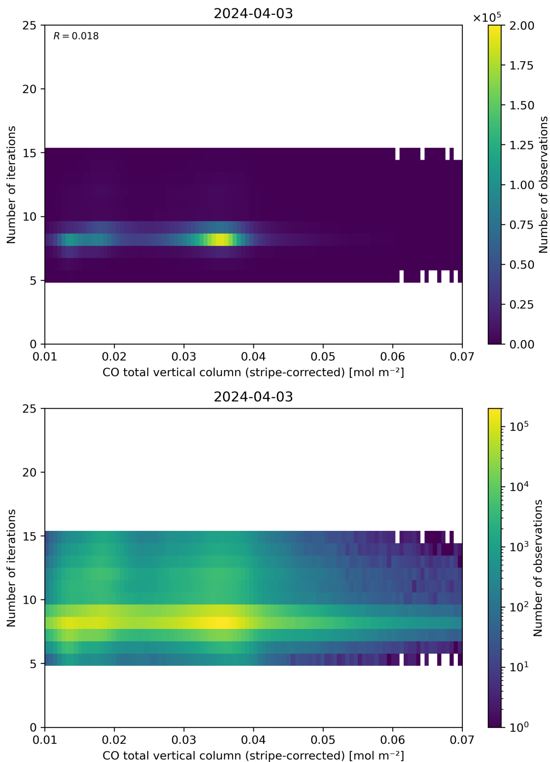
Figure 39: Scatter density plot of “CO total vertical column (stripe-corrected)” against “Number of iterations” for 2024-04-02 to 2024-04-04.
