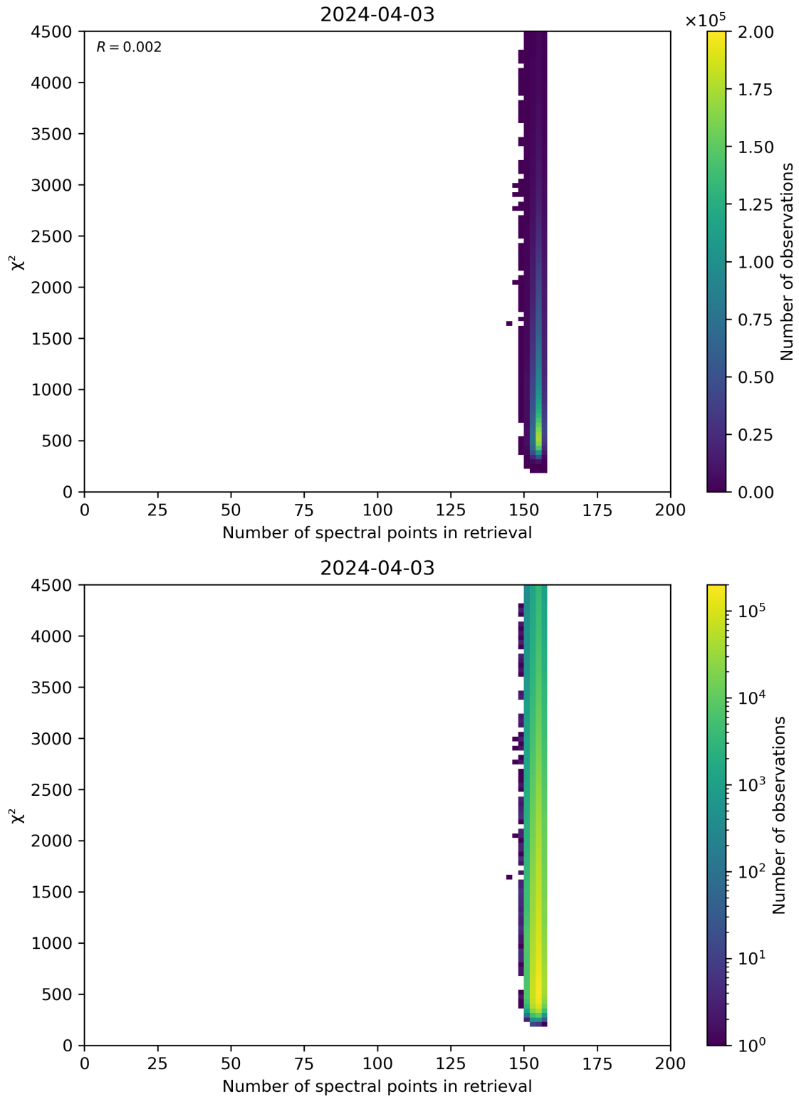
Figure 58: Scatter density plot of “Number of spectral points in retrieval” against “ \chi^2 ” for 2024-04-02 to 2024-04-04.
