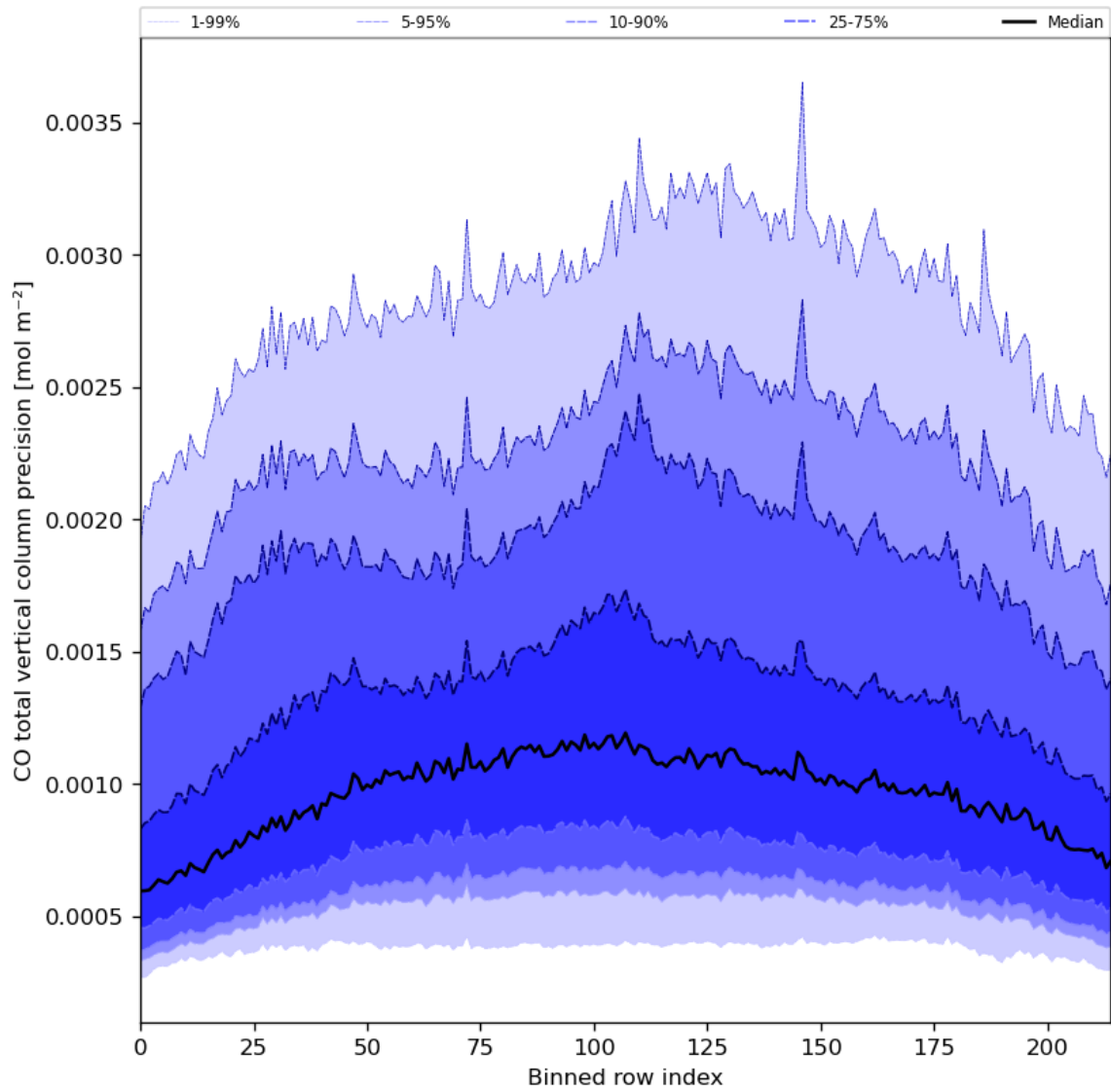
Figure 28: Along track statistics of “CO total vertical column precision” for 2024-04-02 to 2024-04-04
