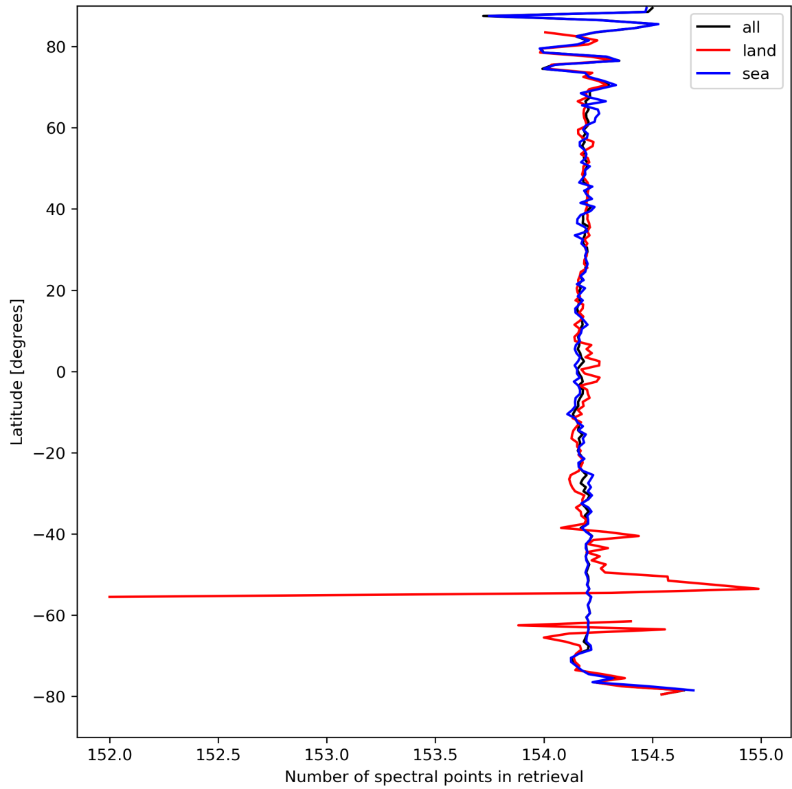
Figure 13: Zonal average of “Number of spectral points in retrieval” for 2024-04-02 to 2024-04-04.
