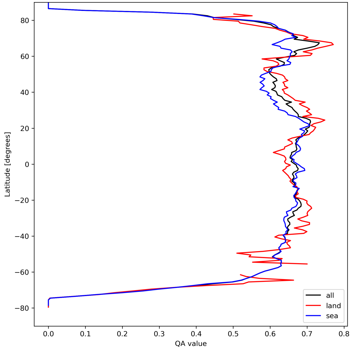
Figure 9: Zonal average of “QA value” for 2024-04-02 to 2024-04-04.
