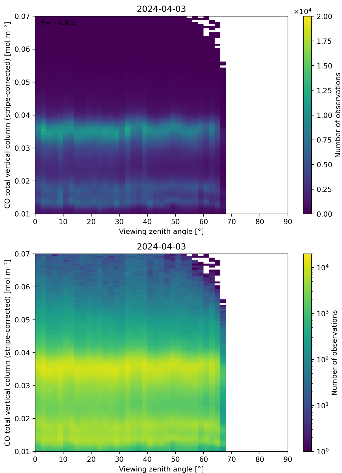
Figure 70: Scatter density plot of “Viewing zenith angle” against “CO total vertical column (stripe-corrected)” for 2024-04-02 to 2024-04-04.
