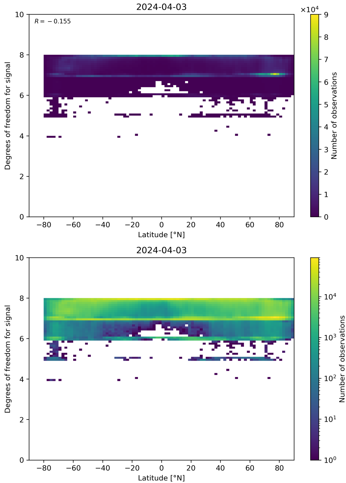
Figure 55: Scatter density plot of “Latitude” against “Degrees of freedom for signal” for 2024-04-02 to 2024-04-04.
