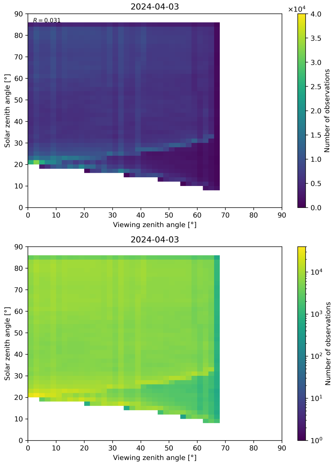
Figure 77: Scatter density plot of “Viewing zenith angle” against “Solar zenith angle” for 2024-04-02 to 2024-04-04.
