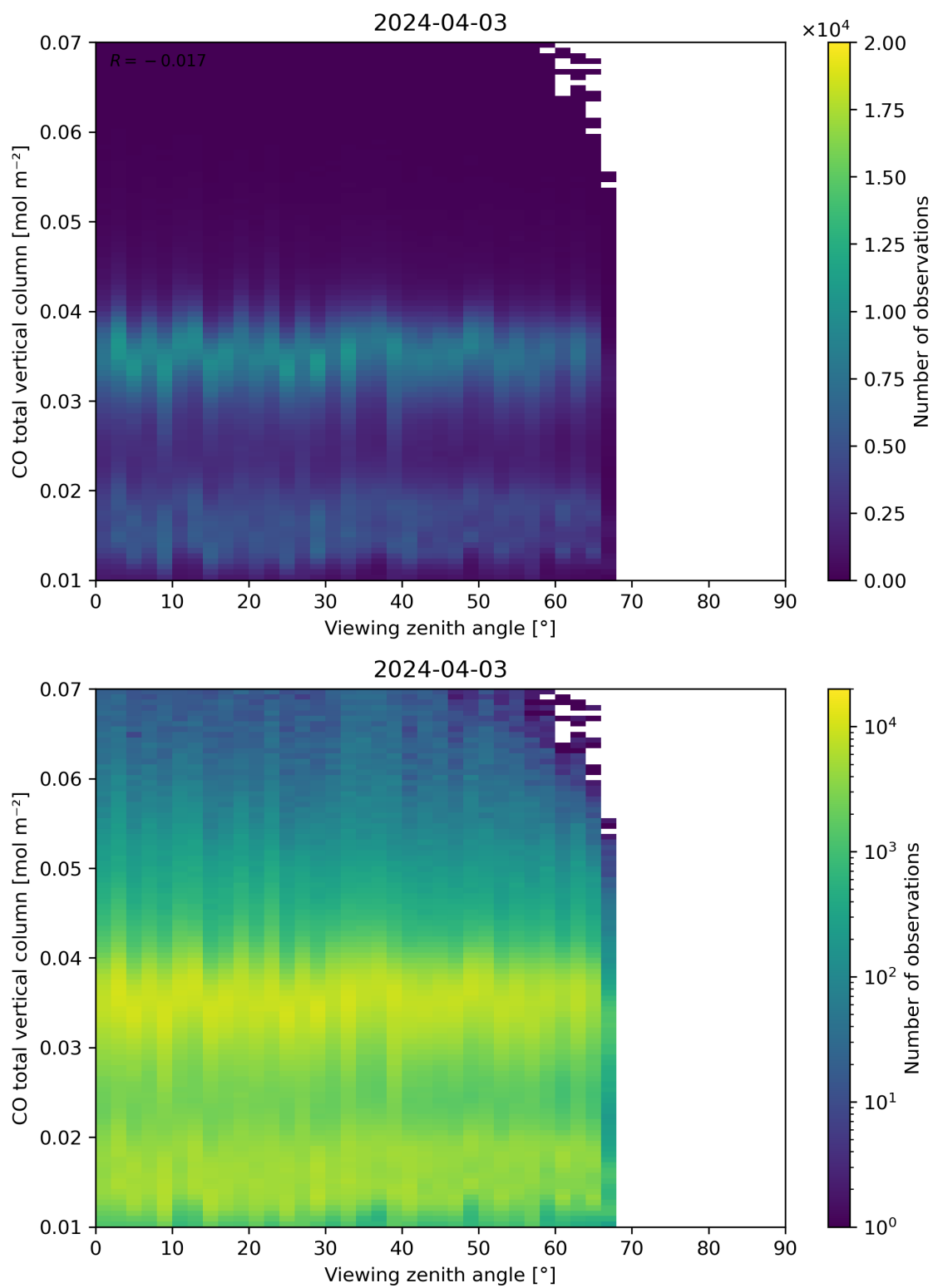
Figure 69: Scatter density plot of “Viewing zenith angle” against “CO total vertical column” for 2024-04-02 to 2024-04-04.
