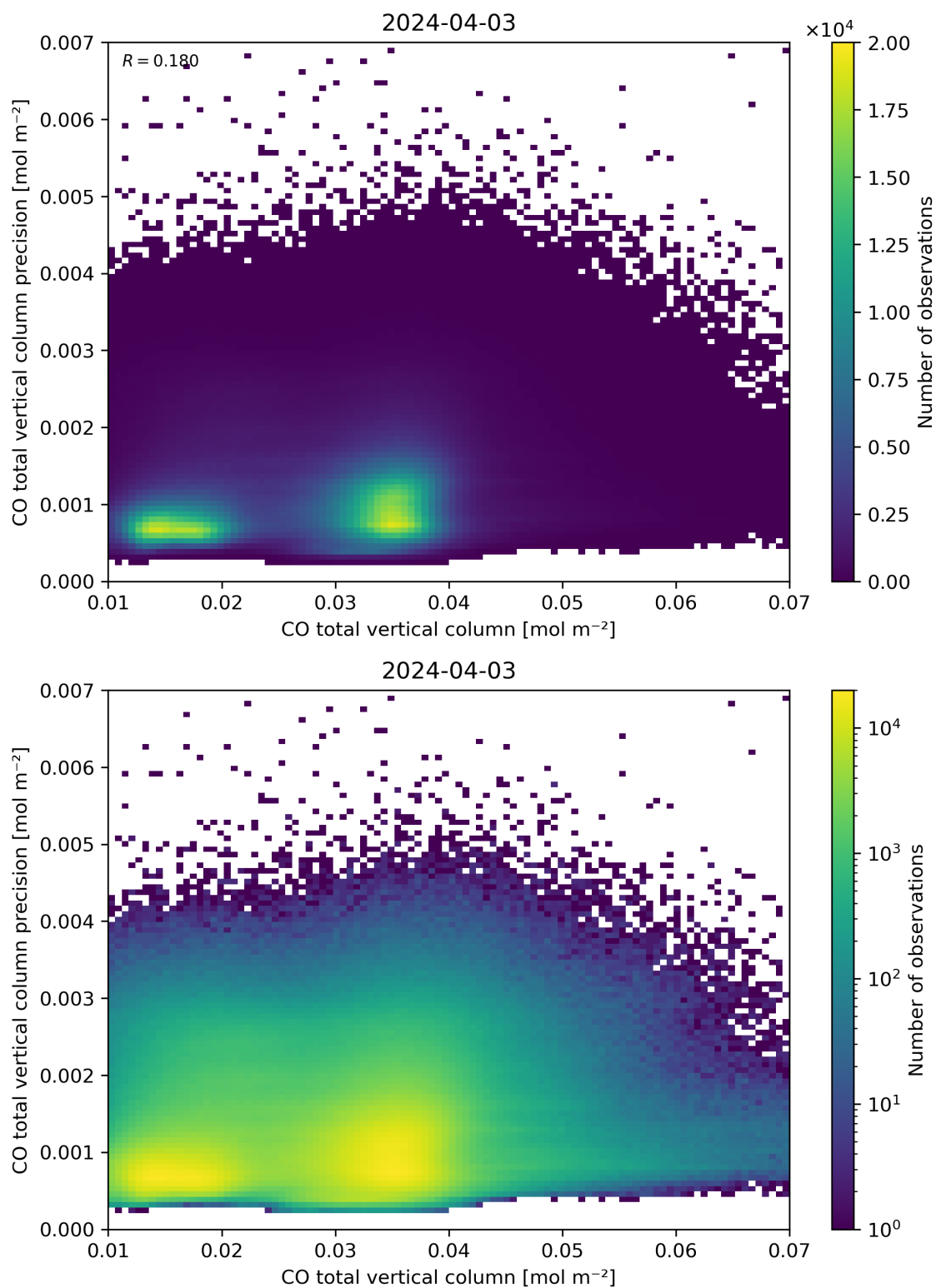
Figure 34: Scatter density plot of “CO total vertical column” against “CO total vertical column precision” for 2024-04-02 to 2024-04-04.
