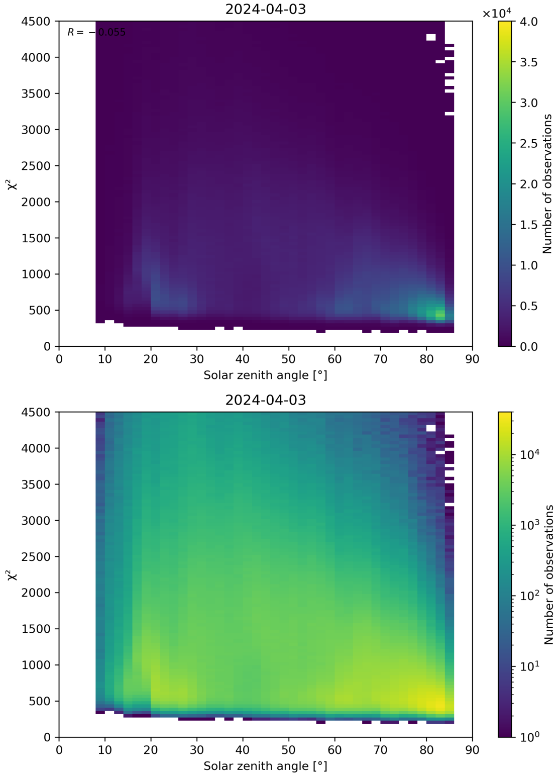
Figure 64: Scatter density plot of “Solar zenith angle” against “ \chi^2 ” for 2024-04-02 to 2024-04-04.
