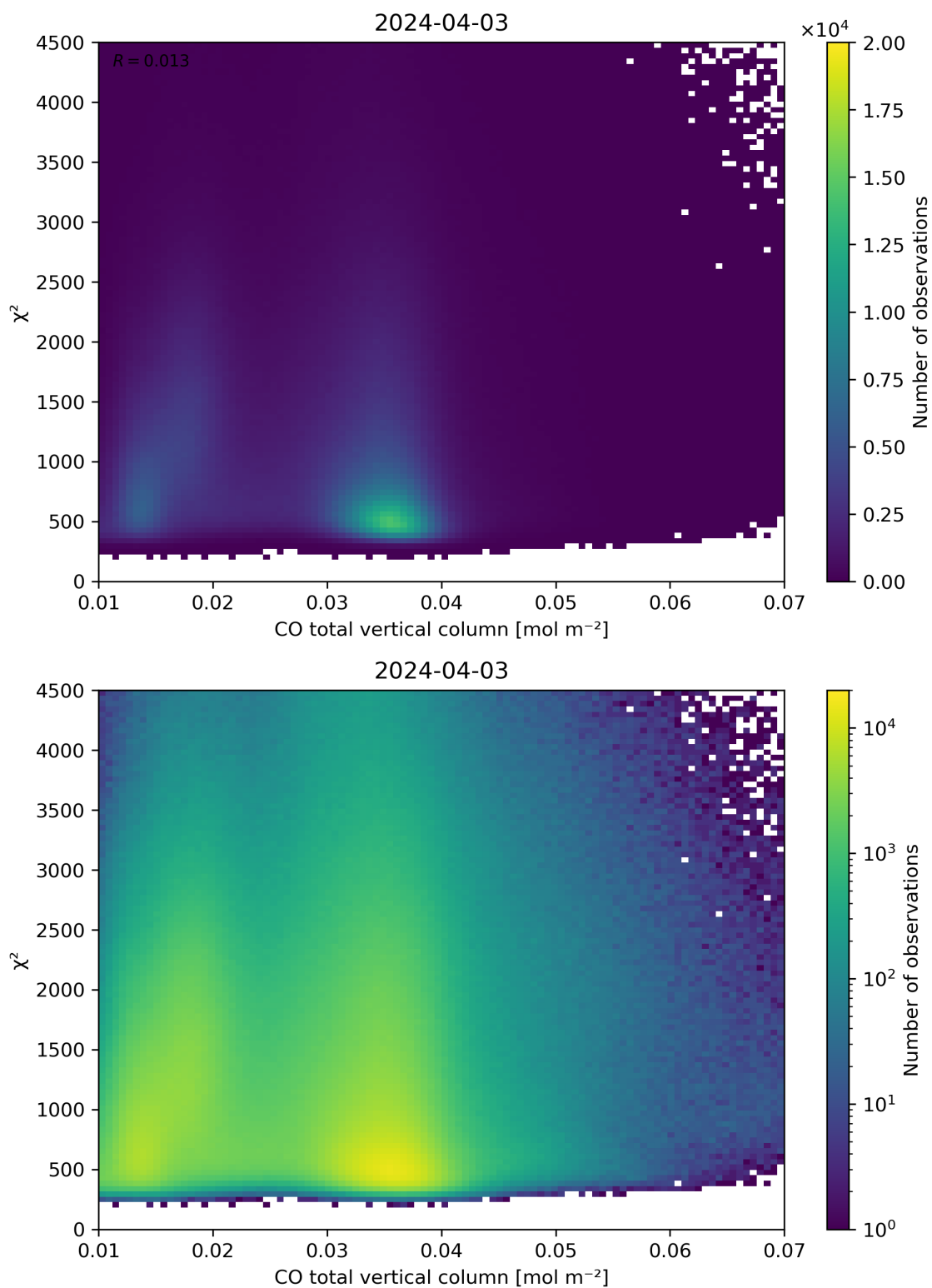
Figure 35: Scatter density plot of “CO total vertical column” against “ \chi^2 ” for 2024-04-02 to 2024-04-04.
