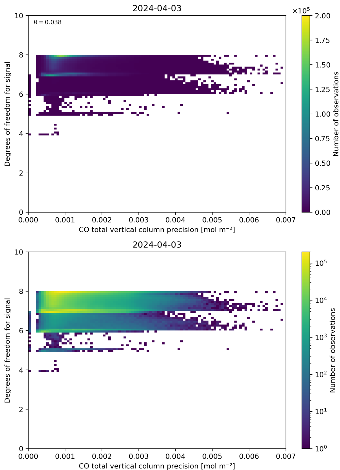
Figure 45: Scatter density plot of “CO total vertical column precision” against “Degrees of freedom for signal” for 2024-04-02 to 2024-04-04.
