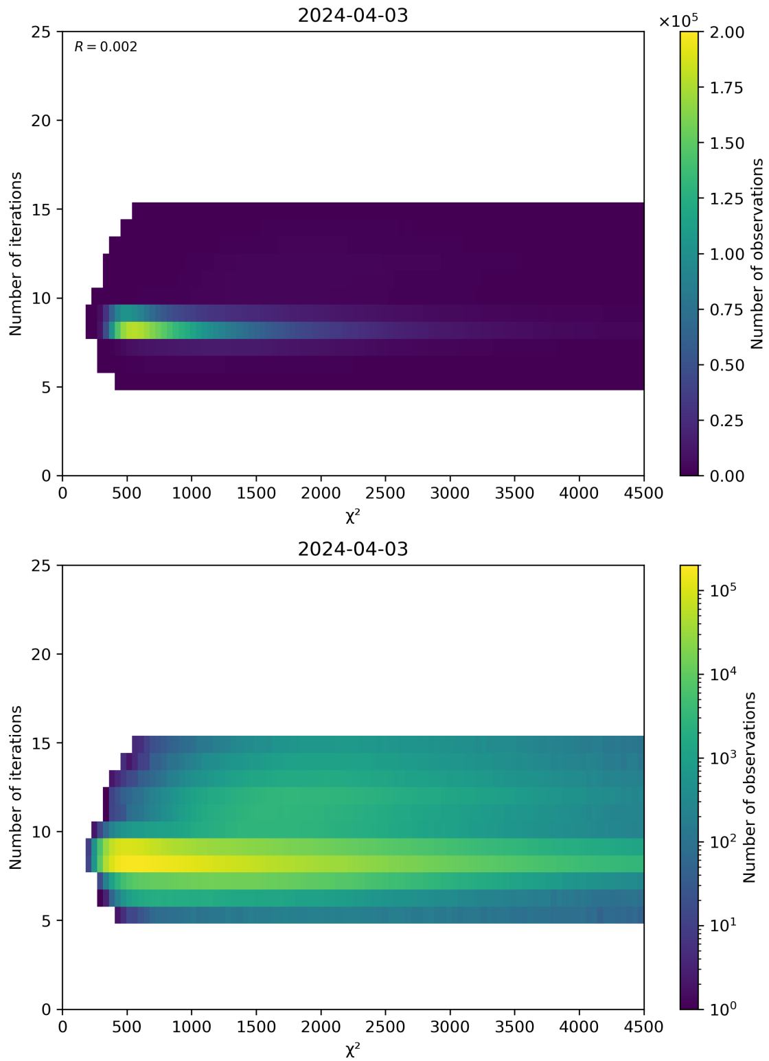
Figure 49: Scatter density plot of “ \chi^2 ” against “Number of iterations” for 2024-04-02 to 2024-04-04.
