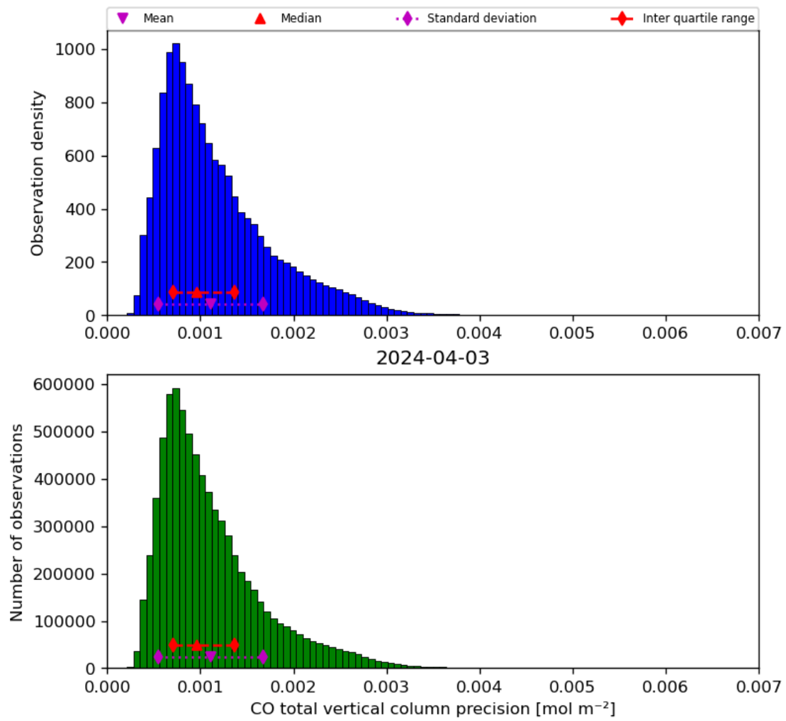
Figure 20: Histogram of “CO total vertical column precision” for 2024-04-02 to 2024-04-04
