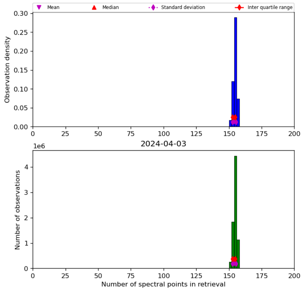
Figure 21: Histogram of “Number of spectral points in retrieval” for 2024-04-02 to 2024-04-04
