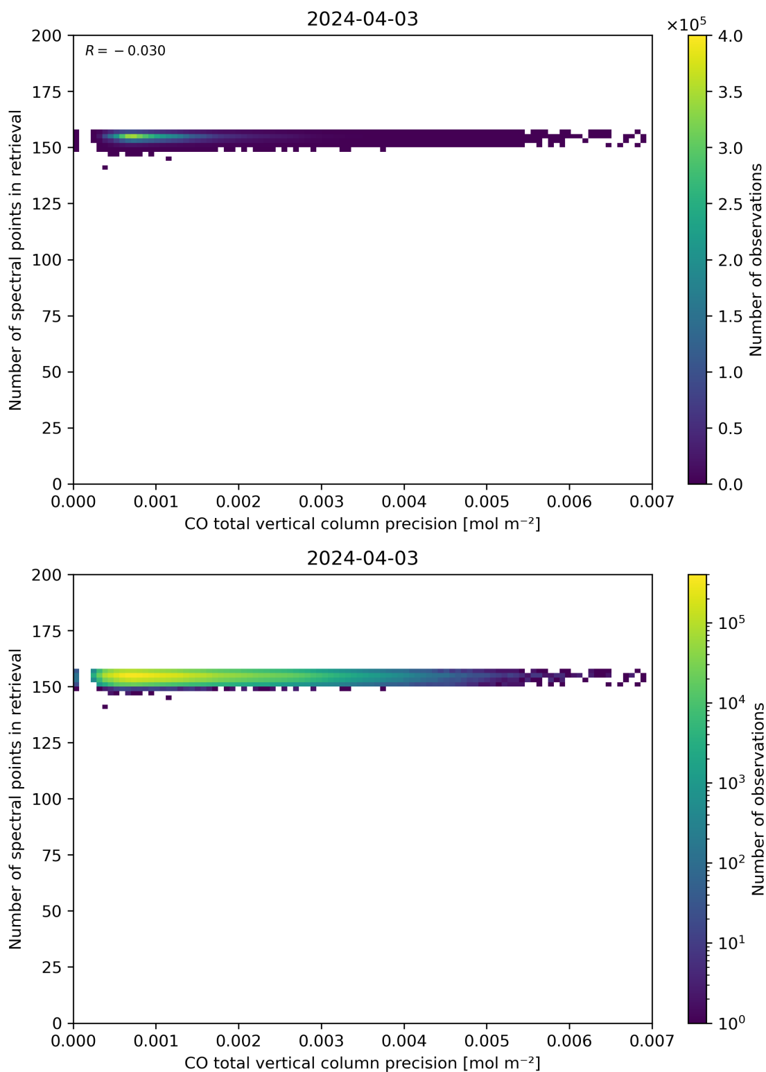
Figure 47: Scatter density plot of “CO total vertical column precision” against “Number of spectral points in retrieval” for 2024-04-02 to 2024-04-04.
