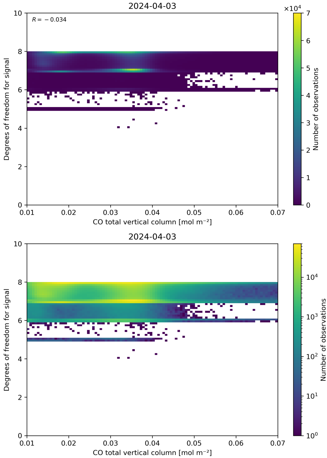
Figure 41: Scatter density plot of “CO total vertical column” against “Degrees of freedom for signal” for 2024-04-02 to 2024-04-04.
