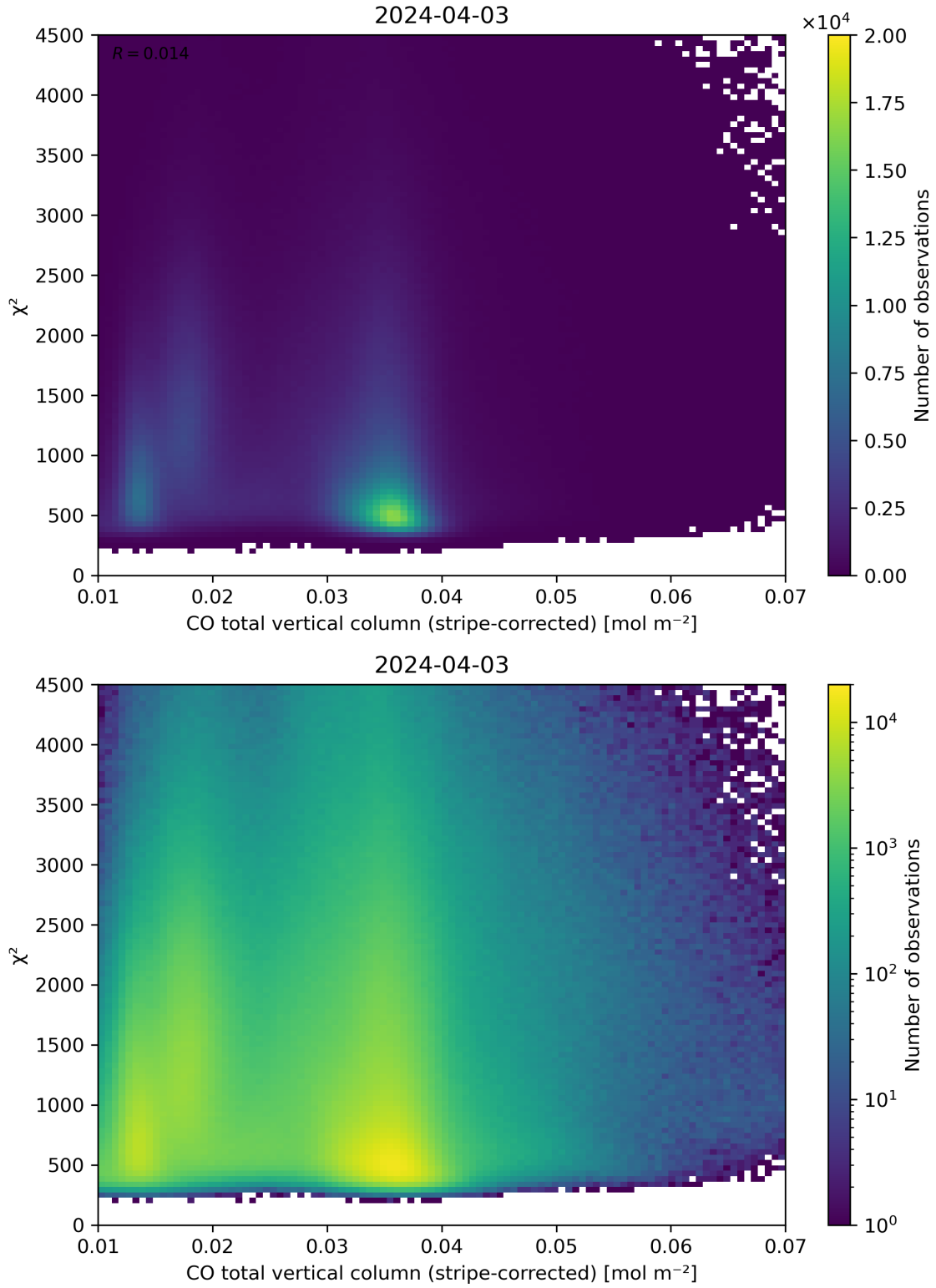
Figure 37: Scatter density plot of “CO total vertical column (stripe-corrected)” against “ \chi^2 ” for 2024-04-02 to 2024-04-04.
