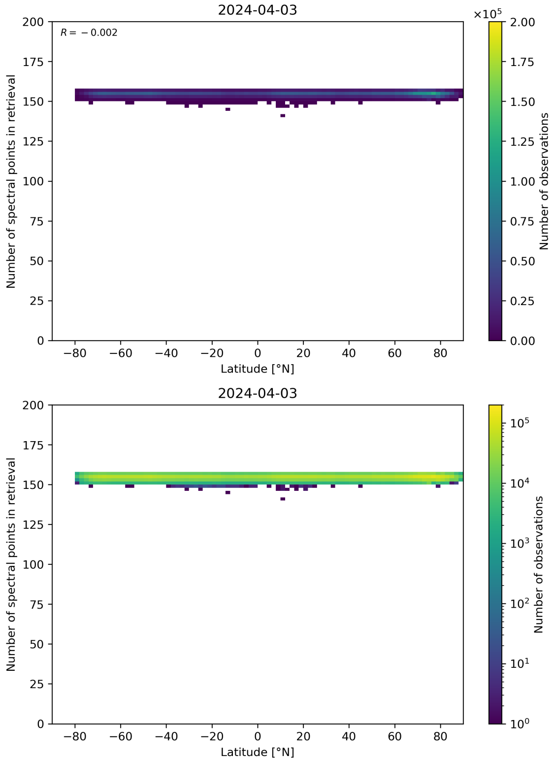
Figure 57: Scatter density plot of “Latitude” against “Number of spectral points in retrieval” for 2024-04-02 to 2024-04-04.
