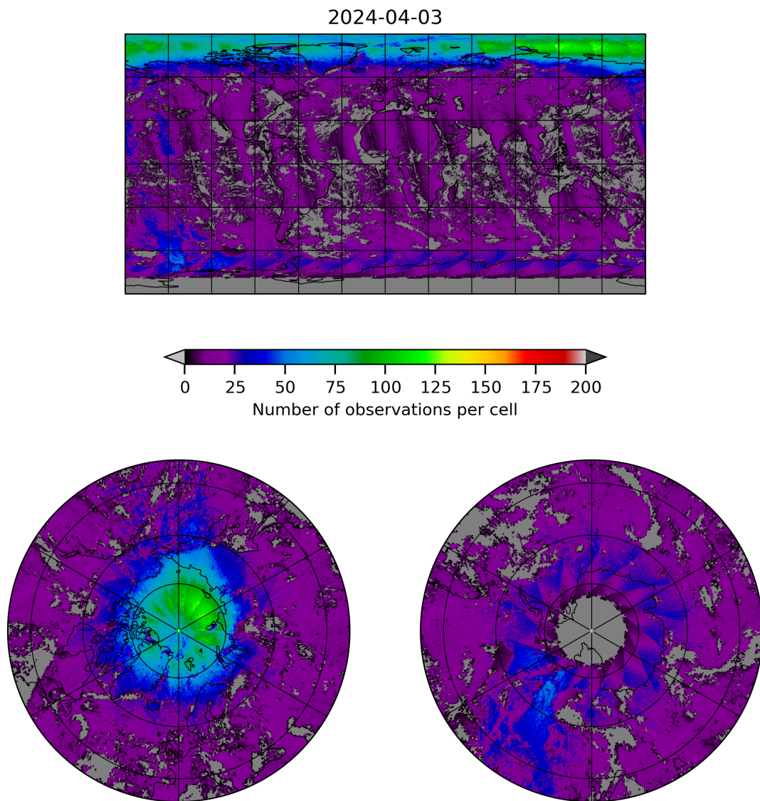
Figure 8: Map of the number of observations for 2024-04-02 to 2024-04-04
