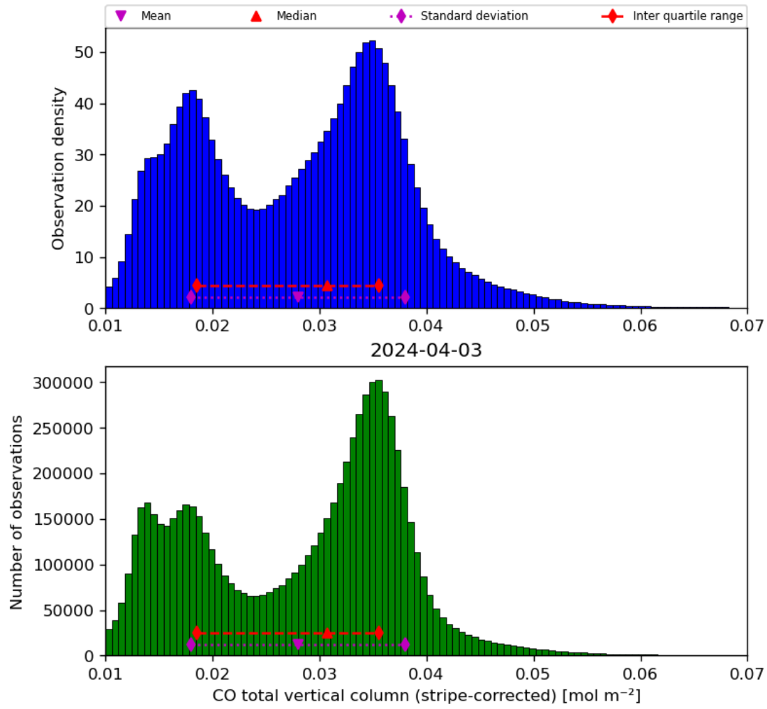
Figure 19: Histogram of “CO total vertical column (stripe-corrected)” for 2024-04-02 to 2024-04-04
