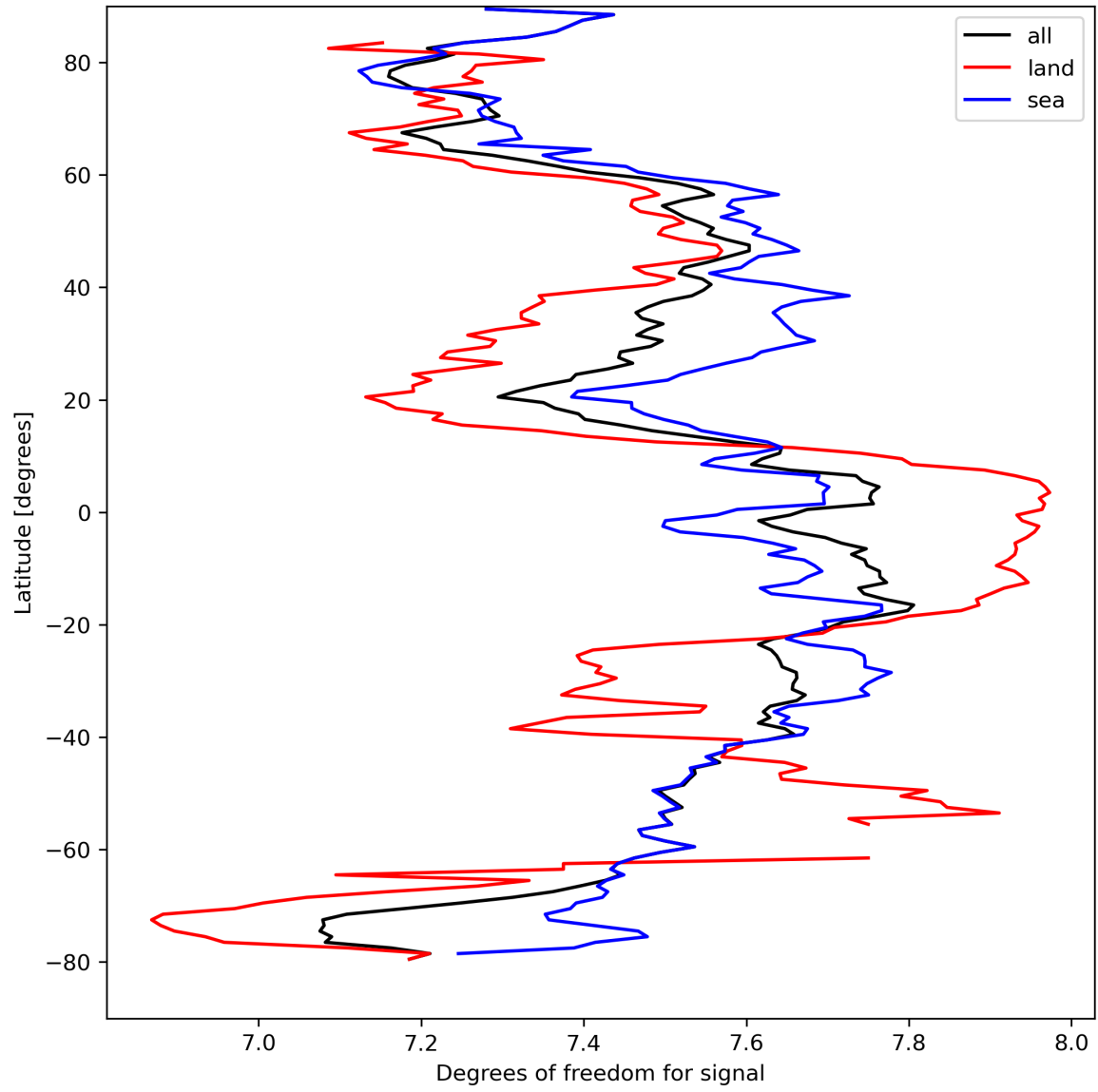
Figure 15: Zonal average of “Degrees of freedom for signal” for 2024-04-02 to 2024-04-04.
