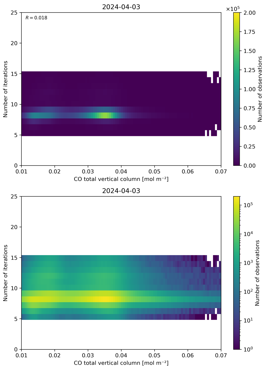
Figure 42: Scatter density plot of “CO total vertical column” against “Number of iterations” for 2024-04-02 to 2024-04-04.
