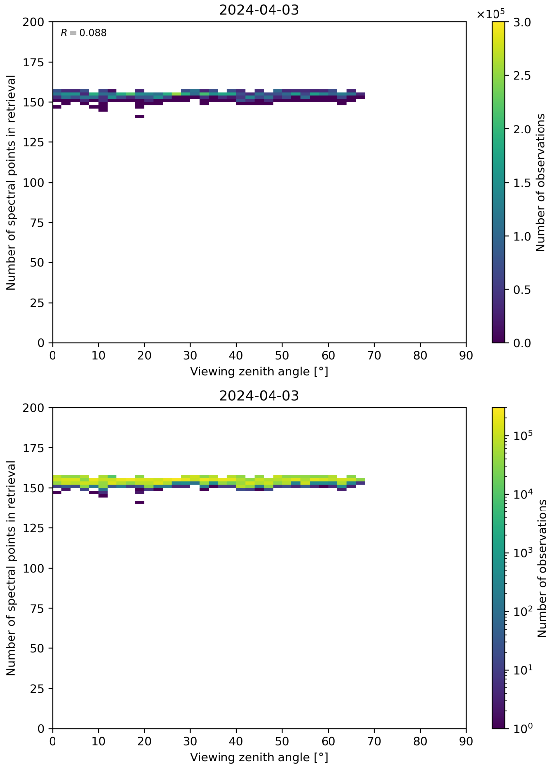
Figure 76: Scatter density plot of “Viewing zenith angle” against “Number of spectral points in retrieval” for 2024-04-02 to 2024-04-04.
