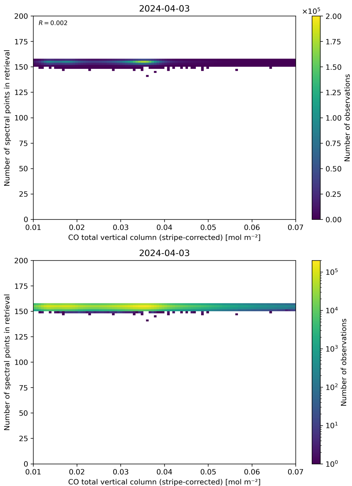
Figure 40: Scatter density plot of “CO total vertical column (stripe-corrected)” against “Number of spectral points in retrieval” for 2024-04-02 to 2024-04-04.
