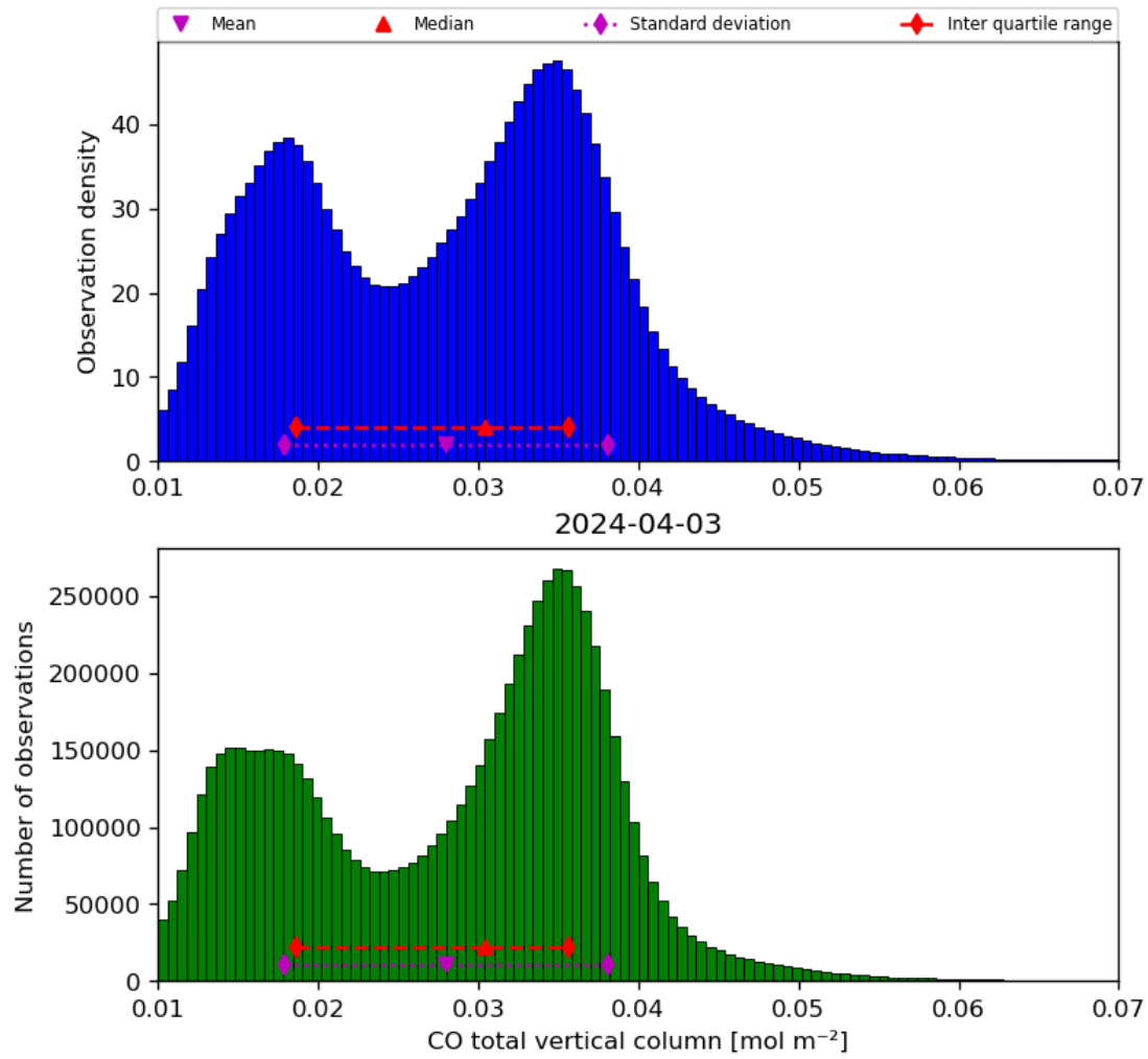
Figure 18: Histogram of “CO total vertical column” for 2024-04-02 to 2024-04-04
