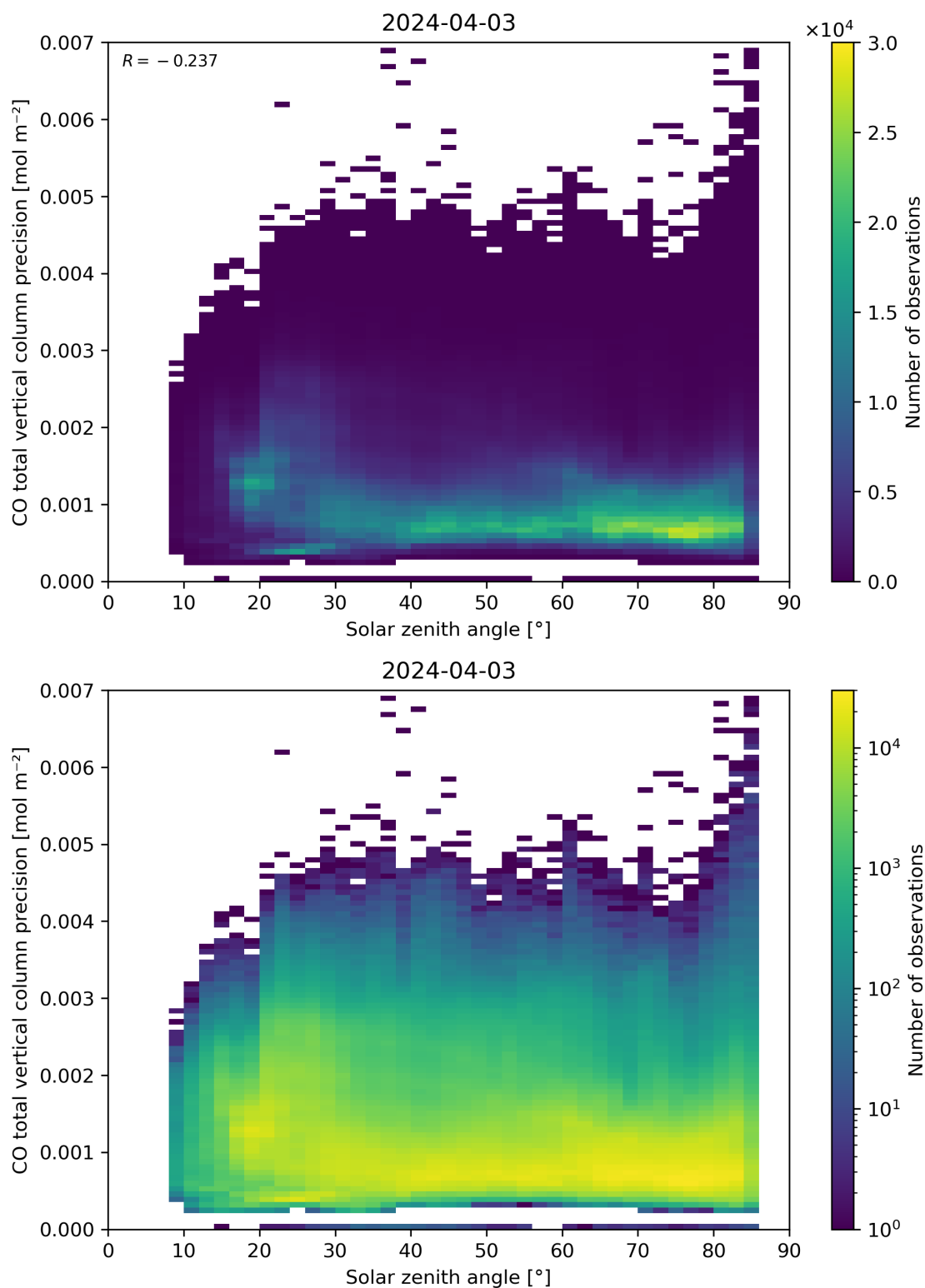
Figure 63: Scatter density plot of “Solar zenith angle” against “CO total vertical column precision” for 2024-04-02 to 2024-04-04.
