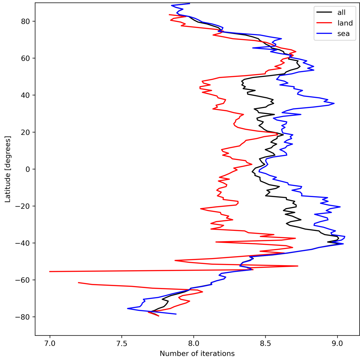
Figure 16: Zonal average of “Number of iterations” for 2024-04-02 to 2024-04-04.
