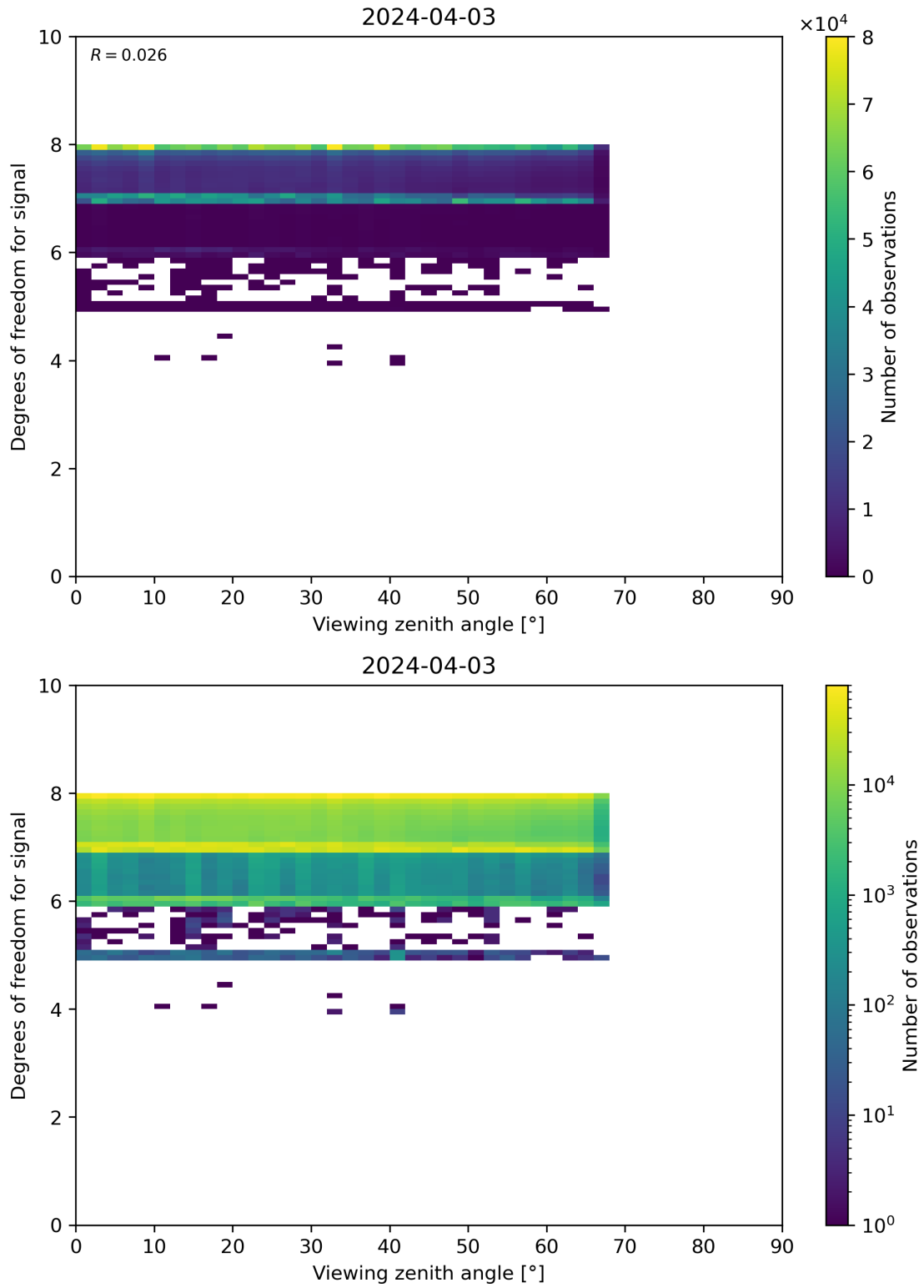
Figure 73: Scatter density plot of “Viewing zenith angle” against “Degrees of freedom for signal” for 2024-04-02 to 2024-04-04.
