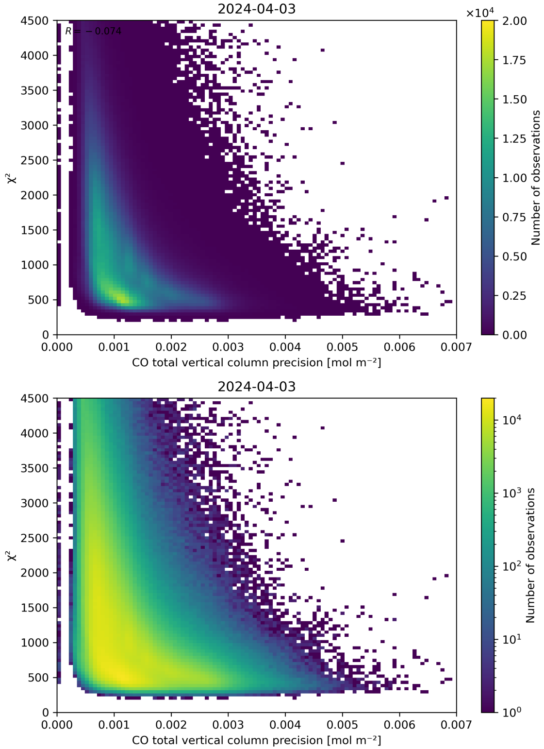
Figure 44: Scatter density plot of “CO total vertical column precision” against “ \chi^2 ” for 2024-04-02 to 2024-04-04.
