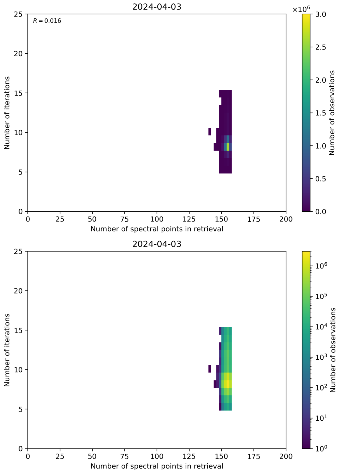
Figure 60: Scatter density plot of “Number of spectral points in retrieval” against “Number of iterations” for 2024-04-02 to 2024-04-04.
