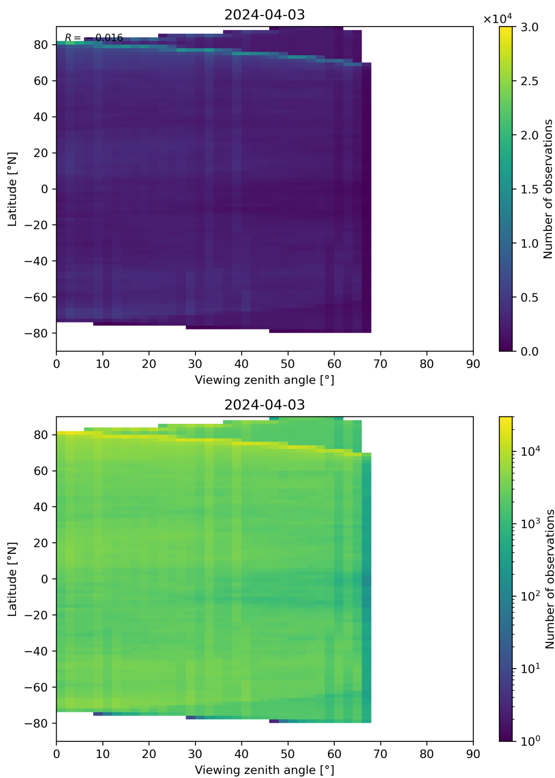
Figure 74: Scatter density plot of “Viewing zenith angle” against “Latitude” for 2024-04-02 to 2024-04-04.
