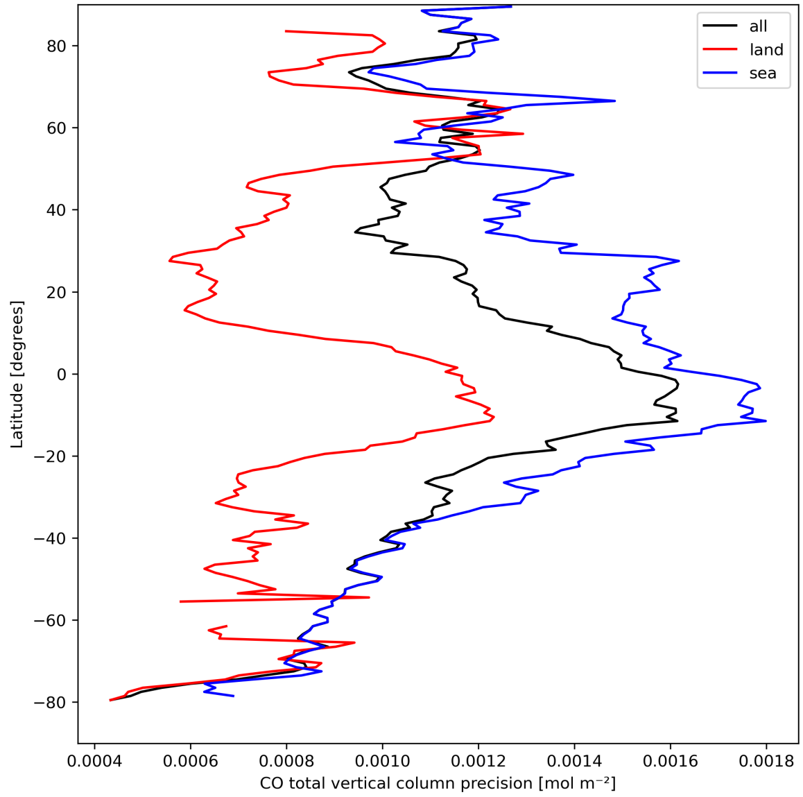
Figure 12: Zonal average of “CO total vertical column precision” for 2024-04-02 to 2024-04-04.
