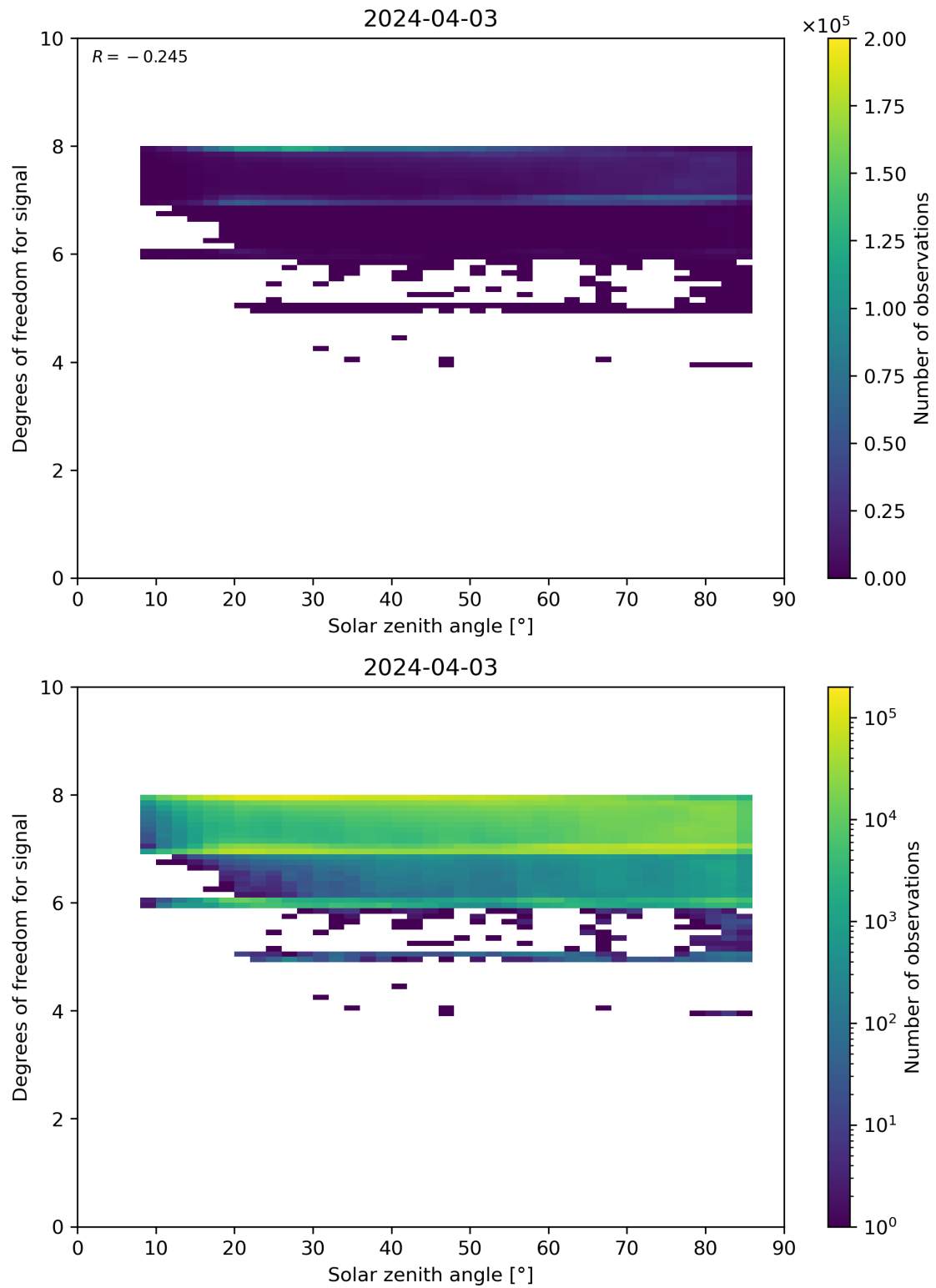
Figure 65: Scatter density plot of “Solar zenith angle” against “Degrees of freedom for signal” for 2024-04-02 to 2024-04-04.
