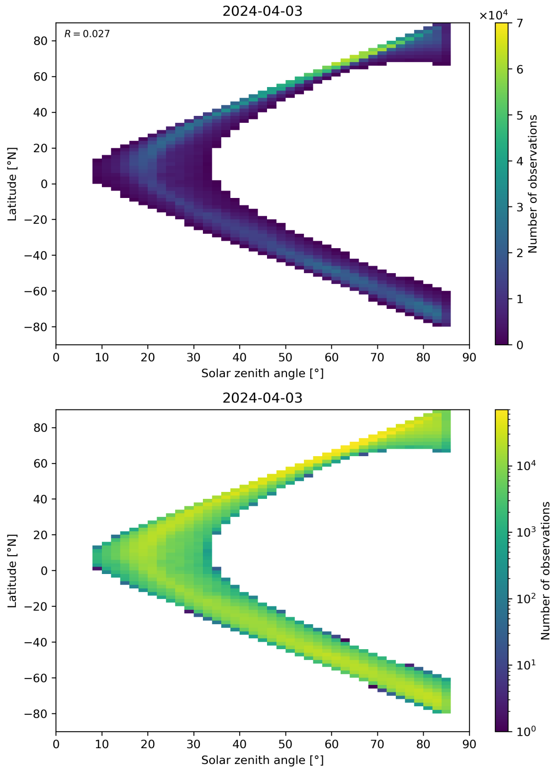
Figure 66: Scatter density plot of “Solar zenith angle” against “Latitude” for 2024-04-02 to 2024-04-04.
