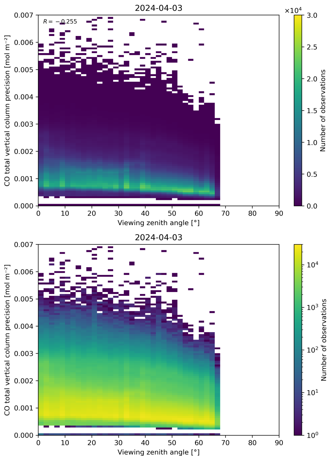
Figure 71: Scatter density plot of “Viewing zenith angle” against “CO total vertical column precision” for 2024-04-02 to 2024-04-04.
