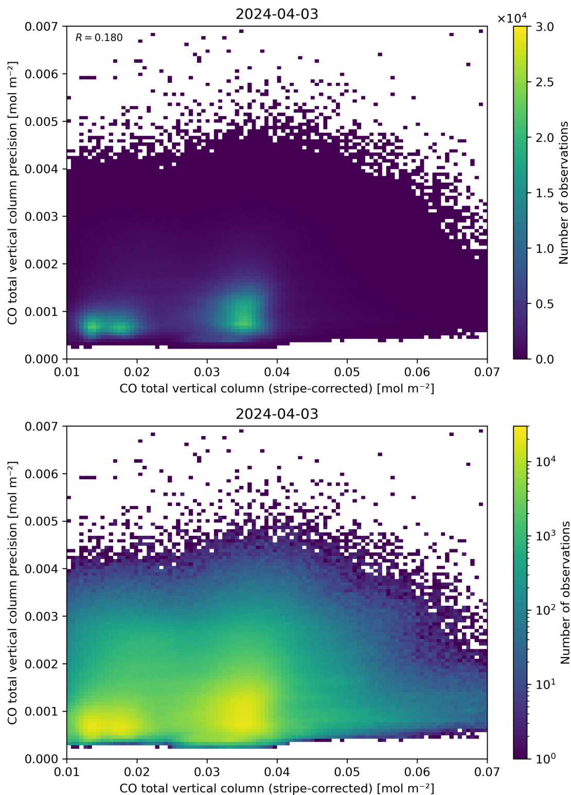
Figure 36: Scatter density plot of “CO total vertical column (stripe-corrected)” against “CO total vertical column precision” for 2024-04-02 to 2024-04-04.
