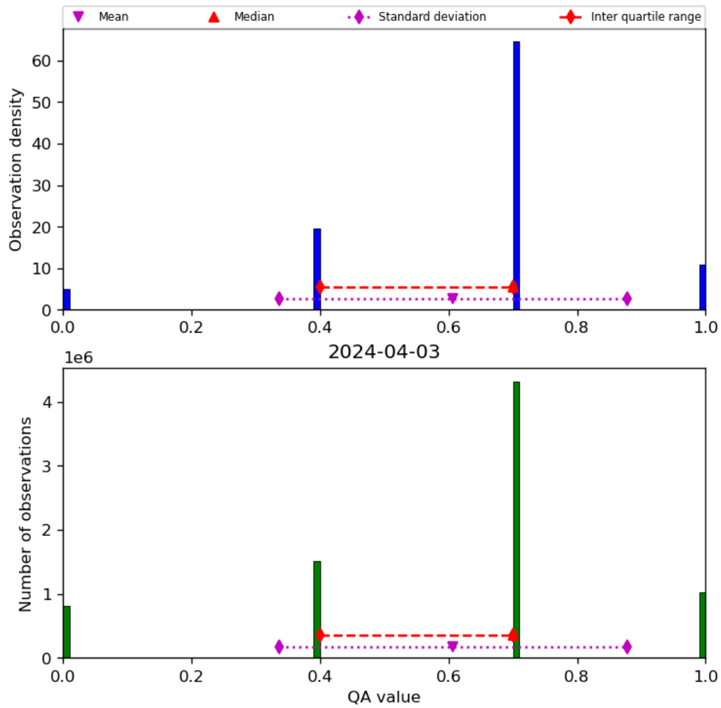
Figure 17: Histogram of “QA value” for 2024-04-02 to 2024-04-04
