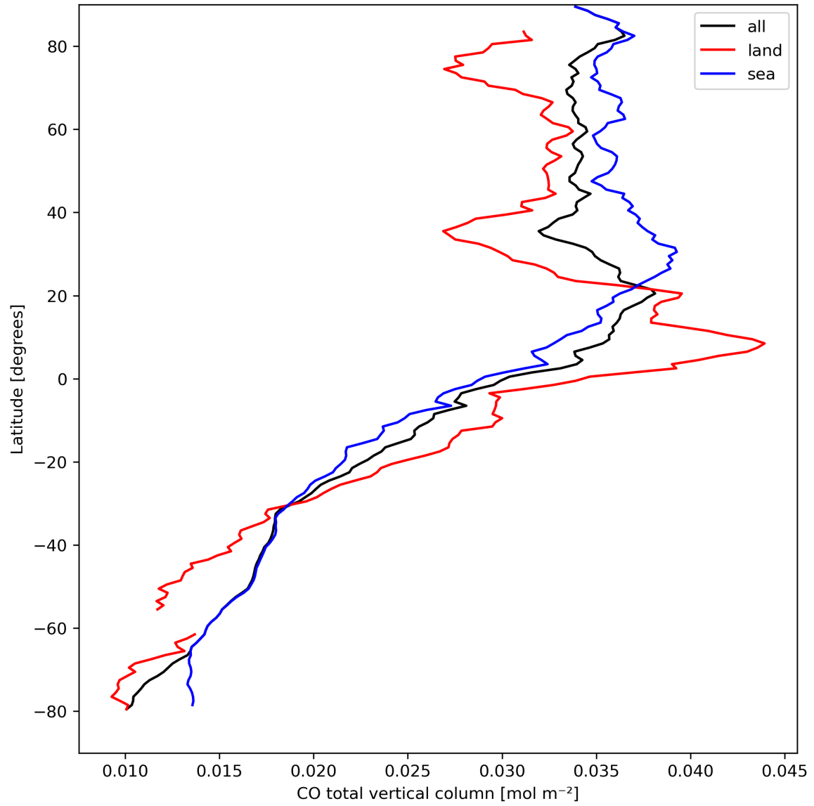
Figure 10: Zonal average of “CO total vertical column” for 2024-04-02 to 2024-04-04.
