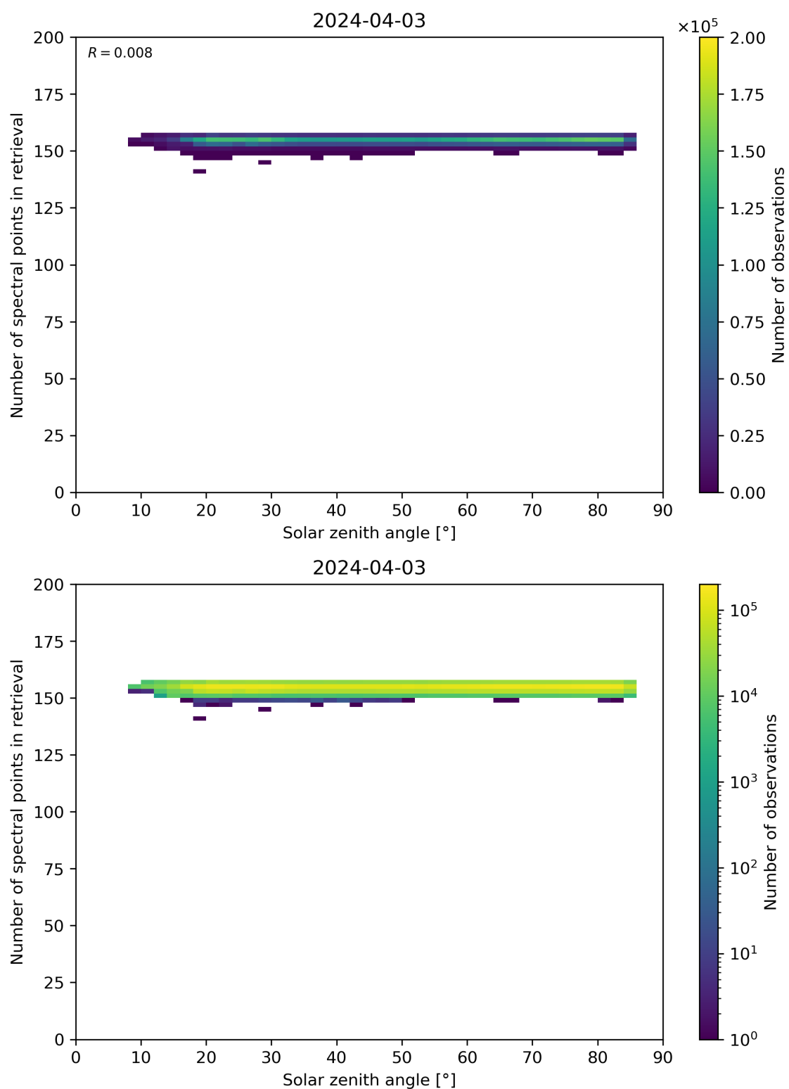
Figure 68: Scatter density plot of “Solar zenith angle” against “Number of spectral points in retrieval” for 2024-04-02 to 2024-04-04.
