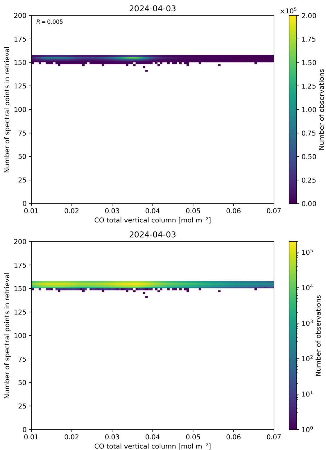
Figure 43: Scatter density plot of “CO total vertical column” against “Number of spectral points in retrieval” for 2024-04-02 to 2024-04-04.
