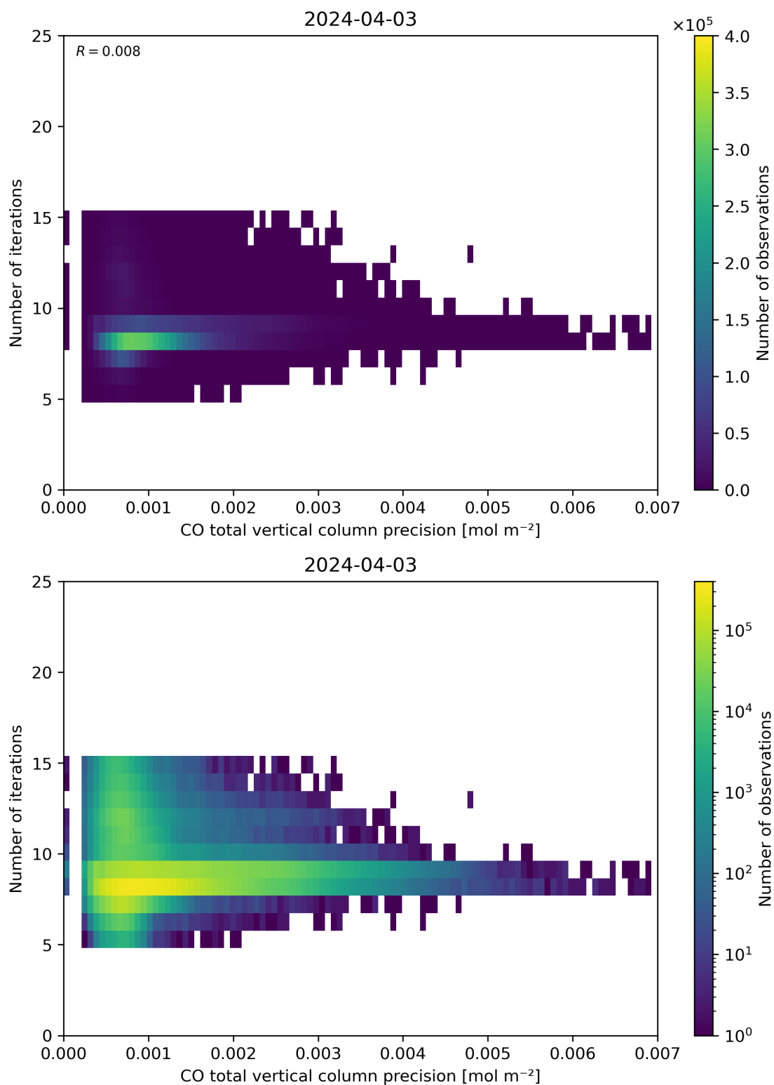
Figure 46: Scatter density plot of “CO total vertical column precision” against “Number of iterations” for 2024-04-02 to 2024-04-04.
