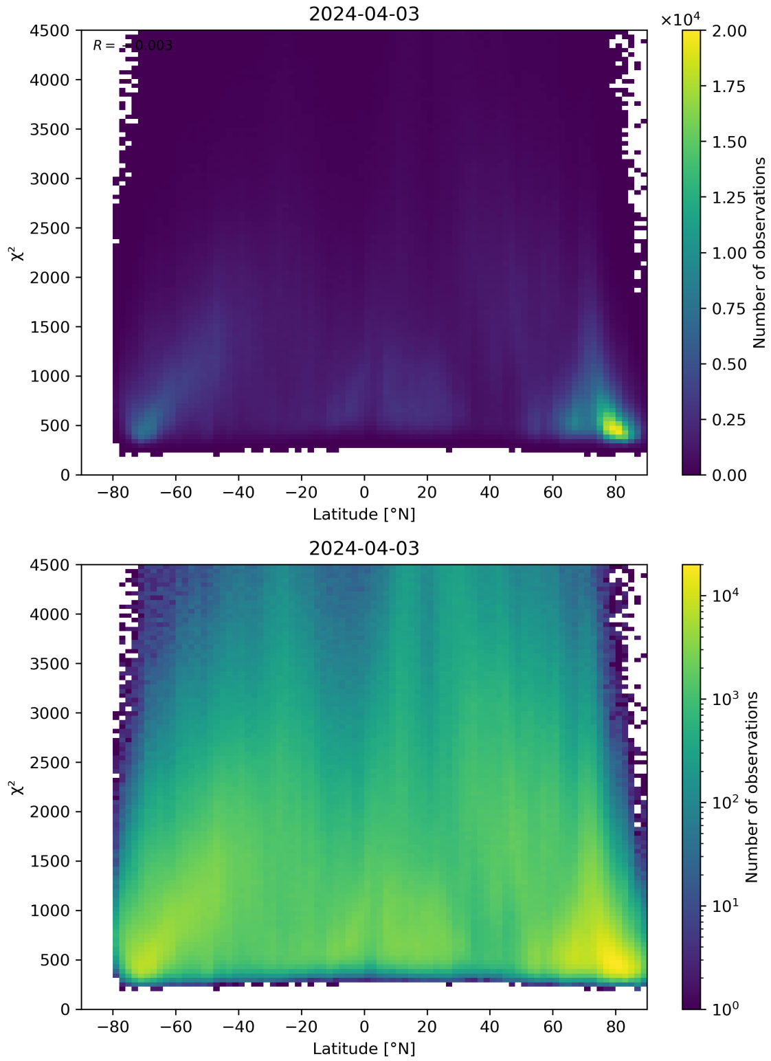
Figure 54: Scatter density plot of “Latitude” against “ \chi^2 ” for 2024-04-02 to 2024-04-04.
