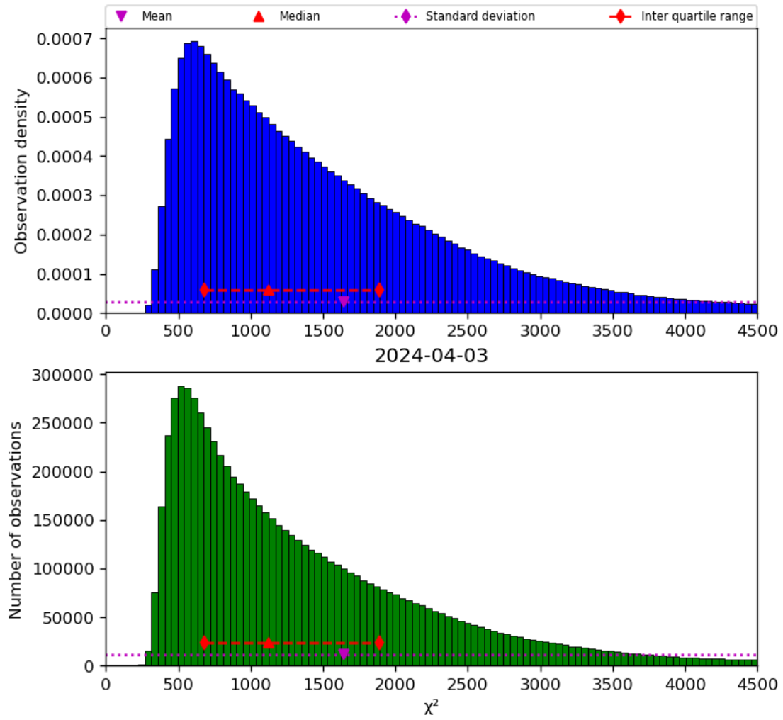
Figure 22: Histogram of “ \chi^2 ” for 2024-04-02 to 2024-04-04
