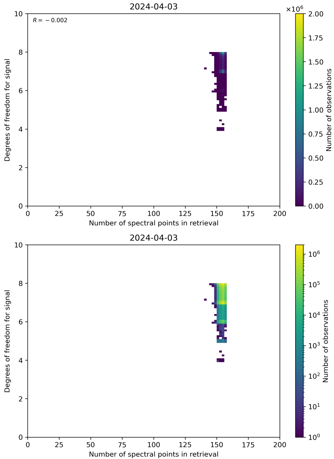
Figure 59: Scatter density plot of “Number of spectral points in retrieval” against “Degrees of freedom for signal” for 2024-04-02 to 2024-04-04.
