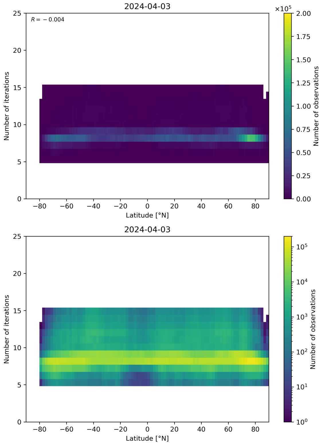
Figure 56: Scatter density plot of “Latitude” against “Number of iterations” for 2024-04-02 to 2024-04-04.
