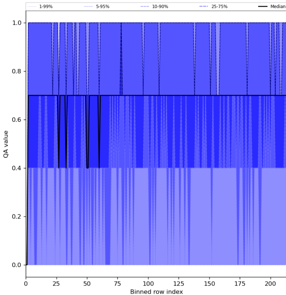
Figure 25: Along track statistics of “QA value” for 2024-04-02 to 2024-04-04
