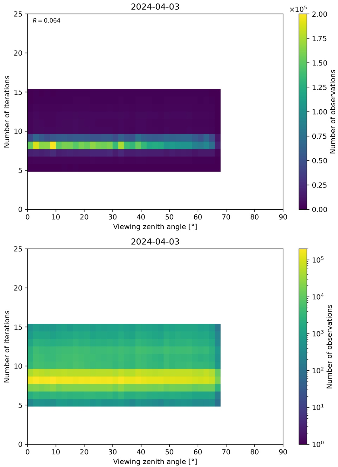
Figure 75: Scatter density plot of “Viewing zenith angle” against “Number of iterations” for 2024-04-02 to 2024-04-04.
