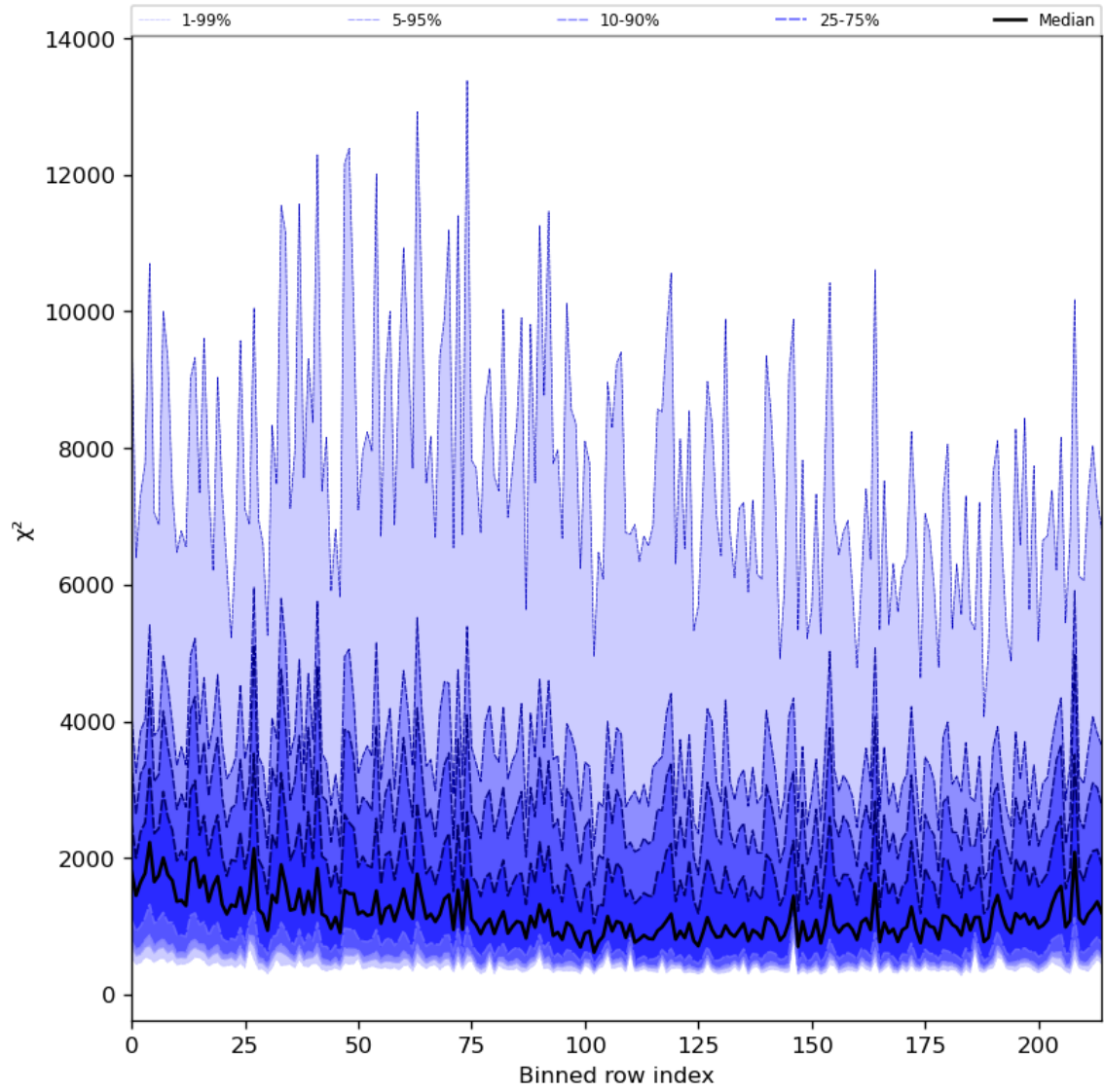
Figure 30: Along track statistics of “ \chi^2 ” for 2024-04-02 to 2024-04-04
