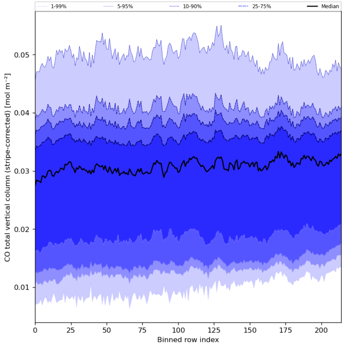
Figure 27: Along track statistics of “CO total vertical column (stripe-corrected)” for 2024-04-02 to 2024-04-04
