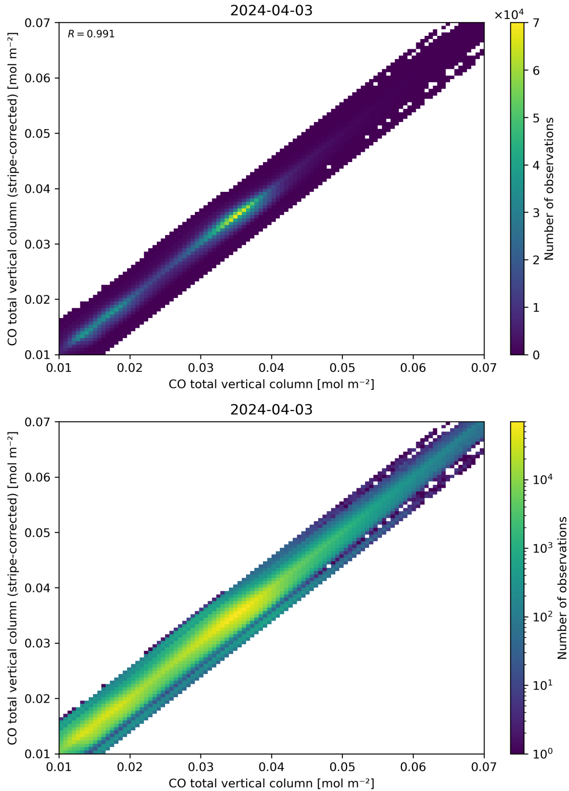
Figure 33: Scatter density plot of “CO total vertical column” against “CO total vertical column (stripe-corrected)” for 2024-04-02 to 2024-04-04.
