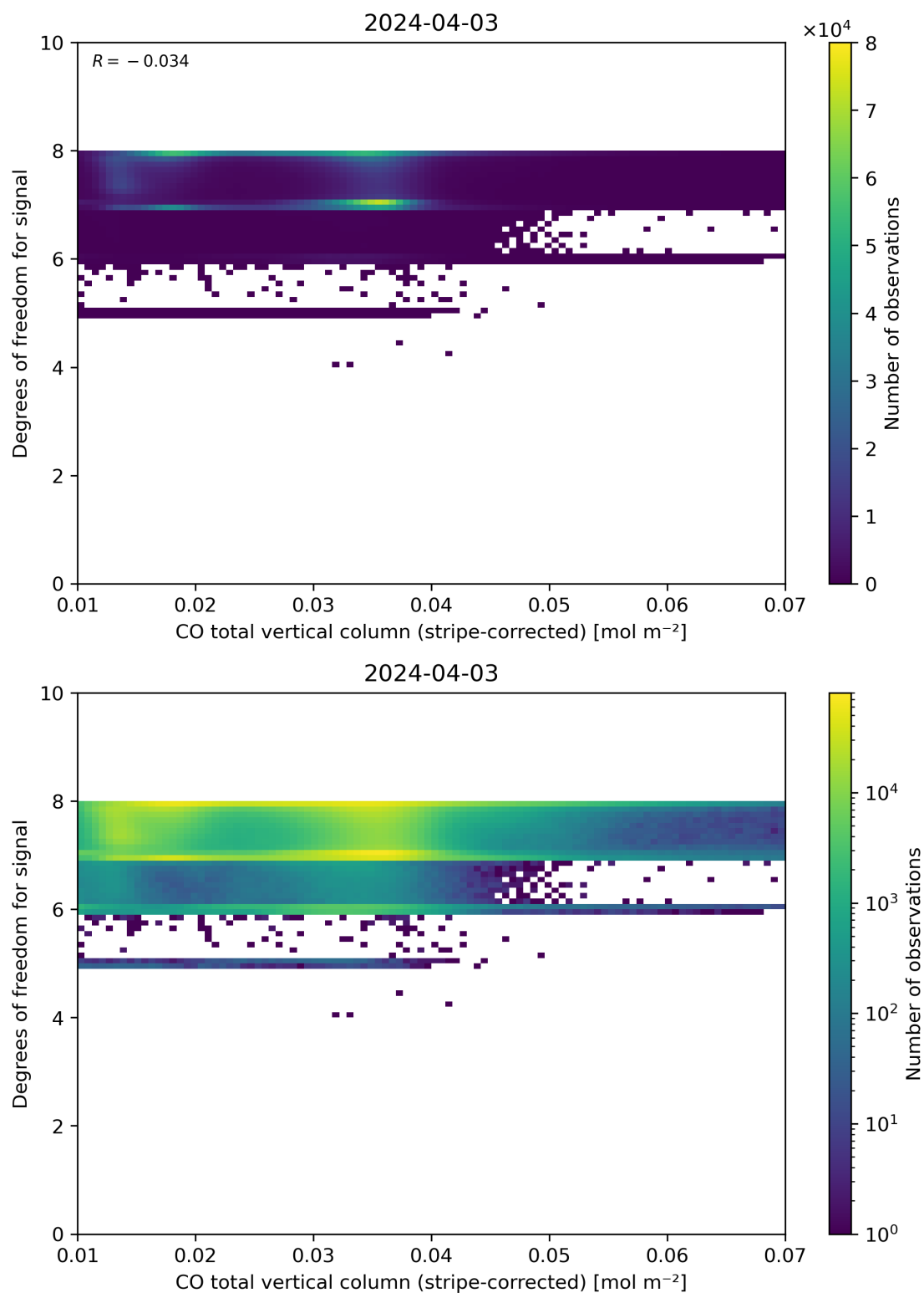
Figure 38: Scatter density plot of “CO total vertical column (stripe-corrected)” against “Degrees of freedom for signal” for 2024-04-02 to 2024-04-04.
