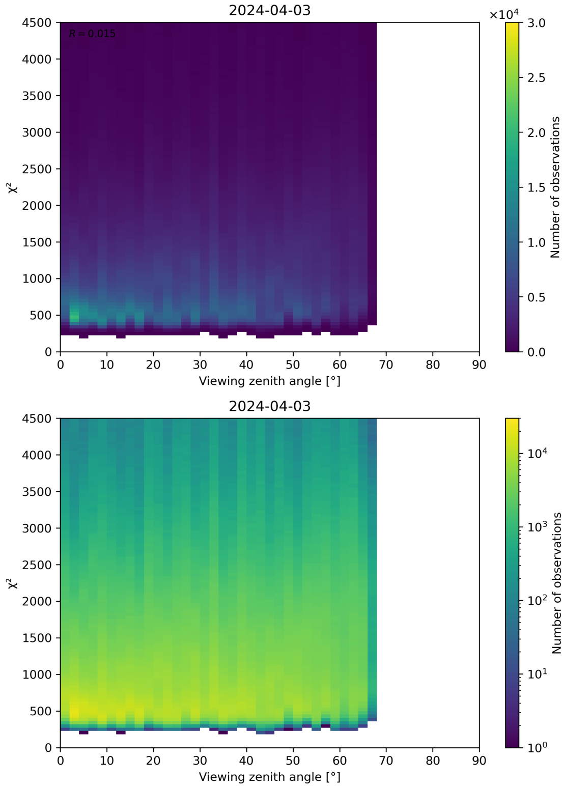
Figure 72: Scatter density plot of “Viewing zenith angle” against “ \chi^2 ” for 2024-04-02 to 2024-04-04.
