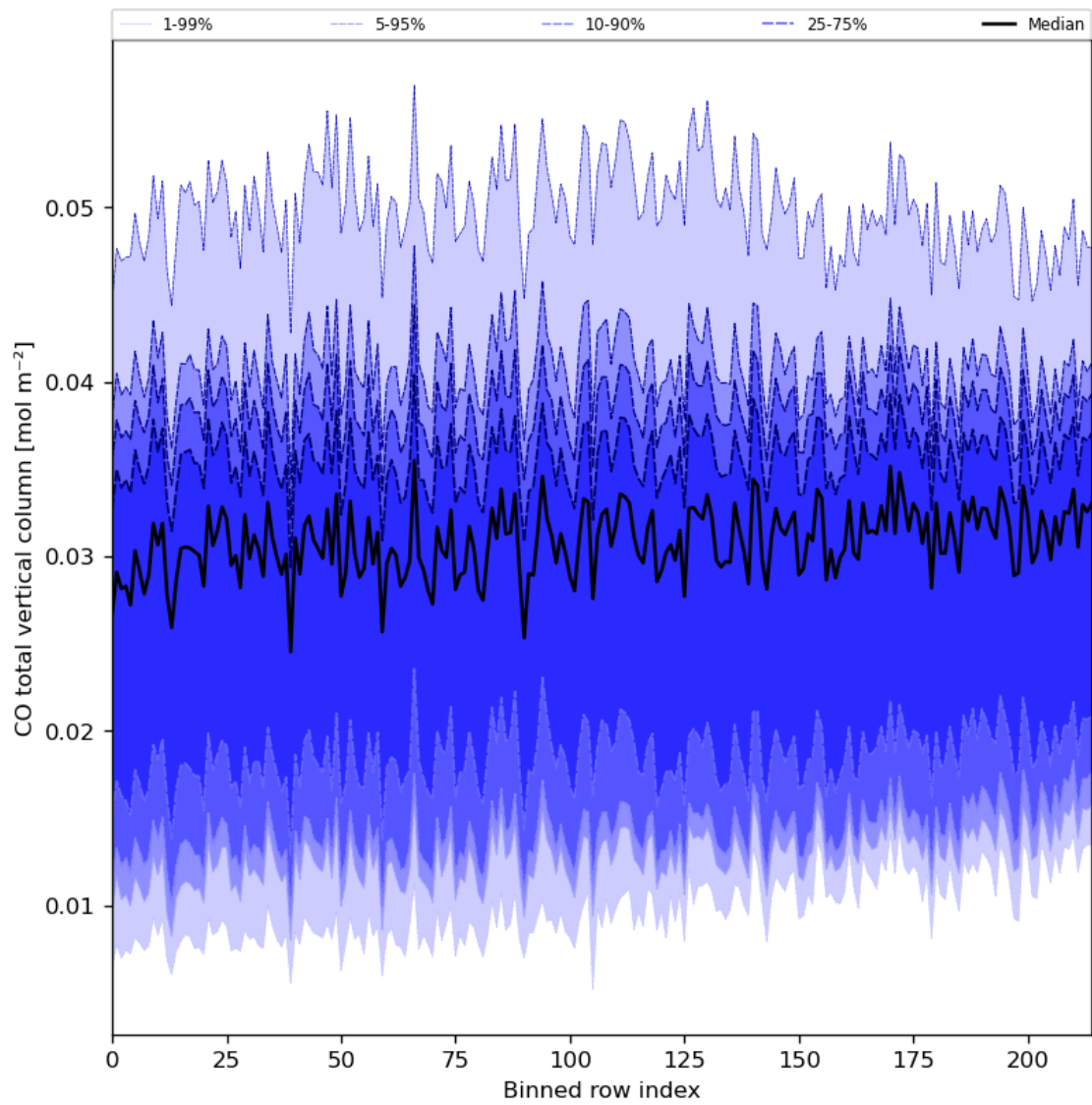
Figure 26: Along track statistics of "CO total vertical column" for 2024-04-02 to 2024-04-04
