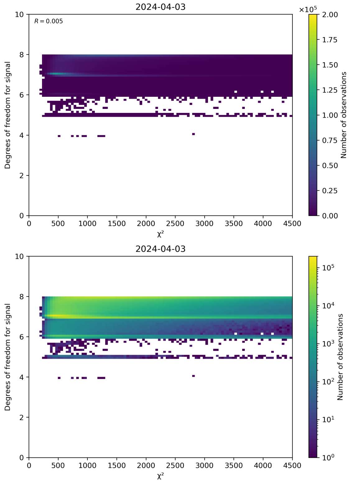
Figure 48: Scatter density plot of “ \chi^2 ” against “Degrees of freedom for signal” for 2024-04-02 to 2024-04-04.
