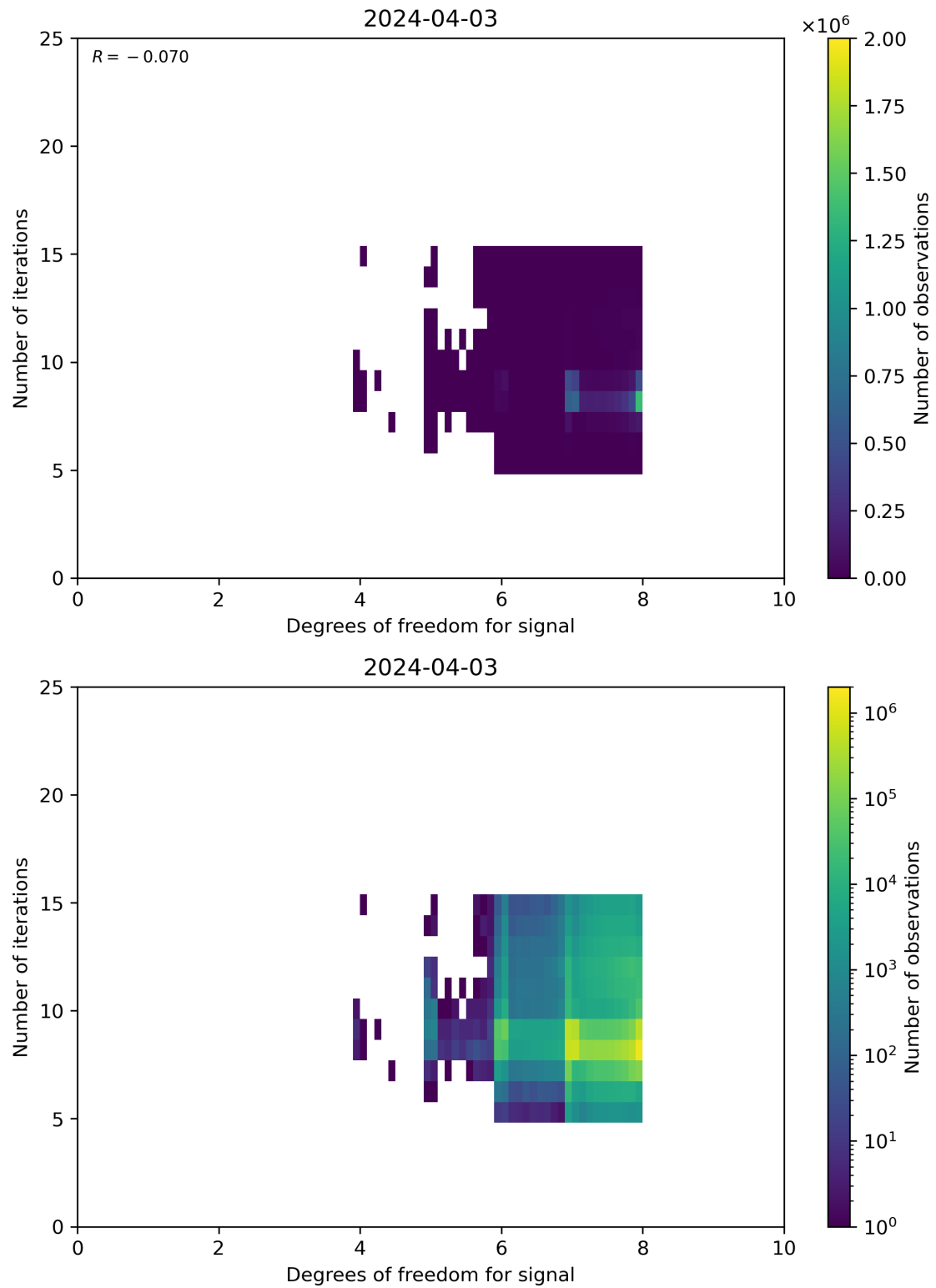
Figure 50: Scatter density plot of “Degrees of freedom for signal” against “Number of iterations” for 2024-04-02 to 2024-04-04.
