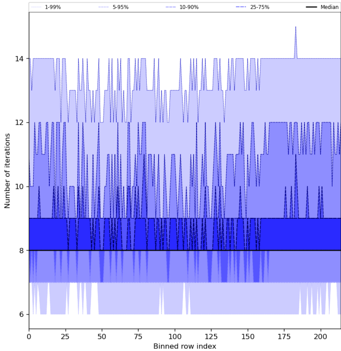
Figure 32: Along track statistics of “Number of iterations” for 2024-04-02 to 2024-04-04
