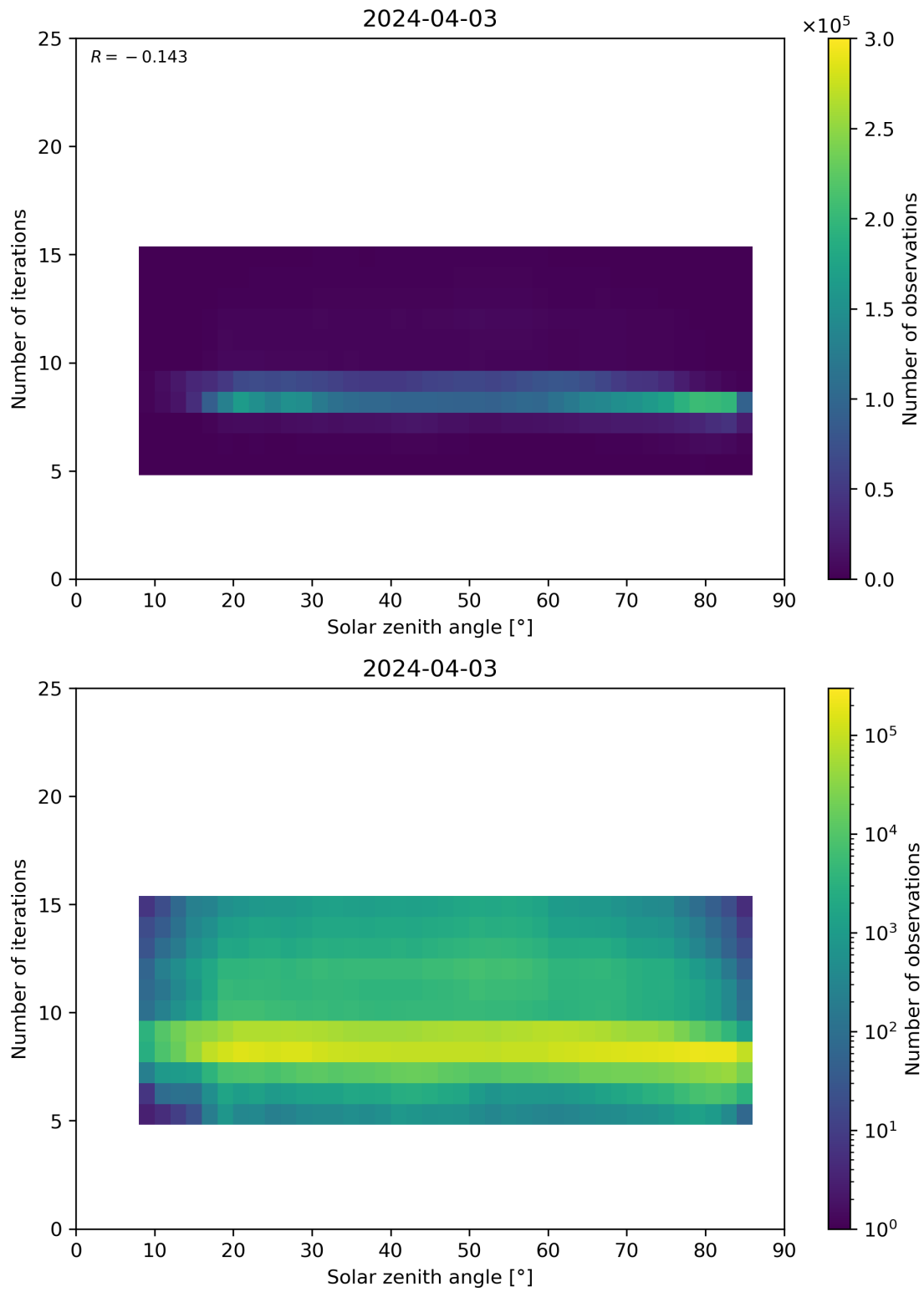
Figure 67: Scatter density plot of “Solar zenith angle” against “Number of iterations” for 2024-04-02 to 2024-04-04.
