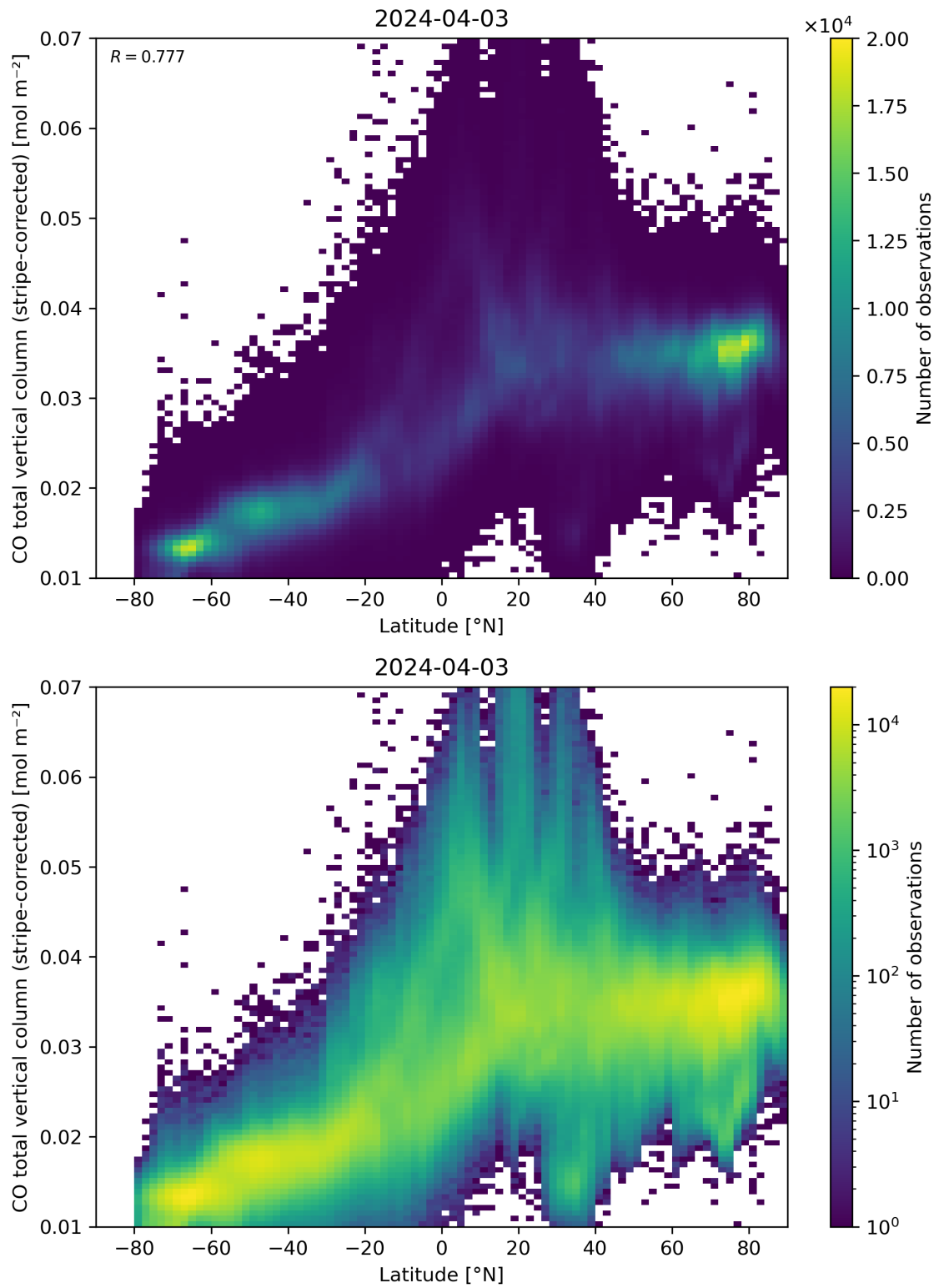
Figure 52: Scatter density plot of “Latitude” against “CO total vertical column (stripe-corrected)” for 2024-04-02 to 2024-04-04.
