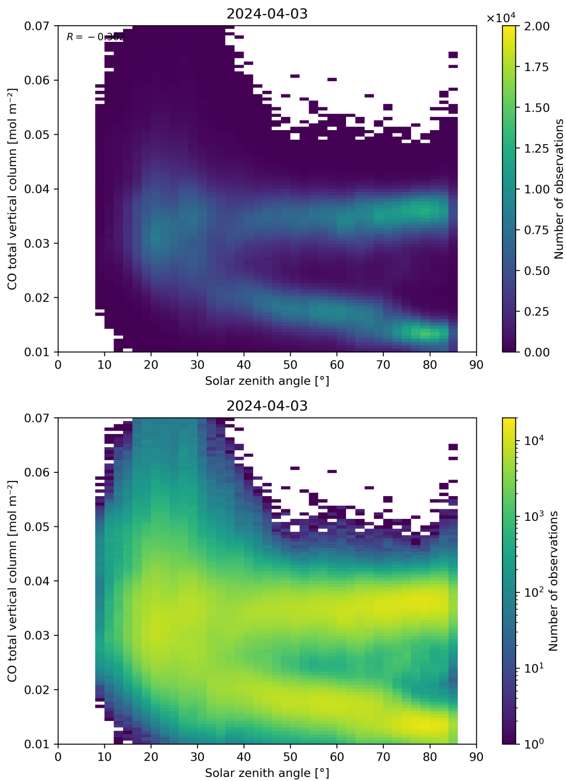
Figure 61: Scatter density plot of “Solar zenith angle” against “CO total vertical column” for 2024-04-02 to 2024-04-04.
