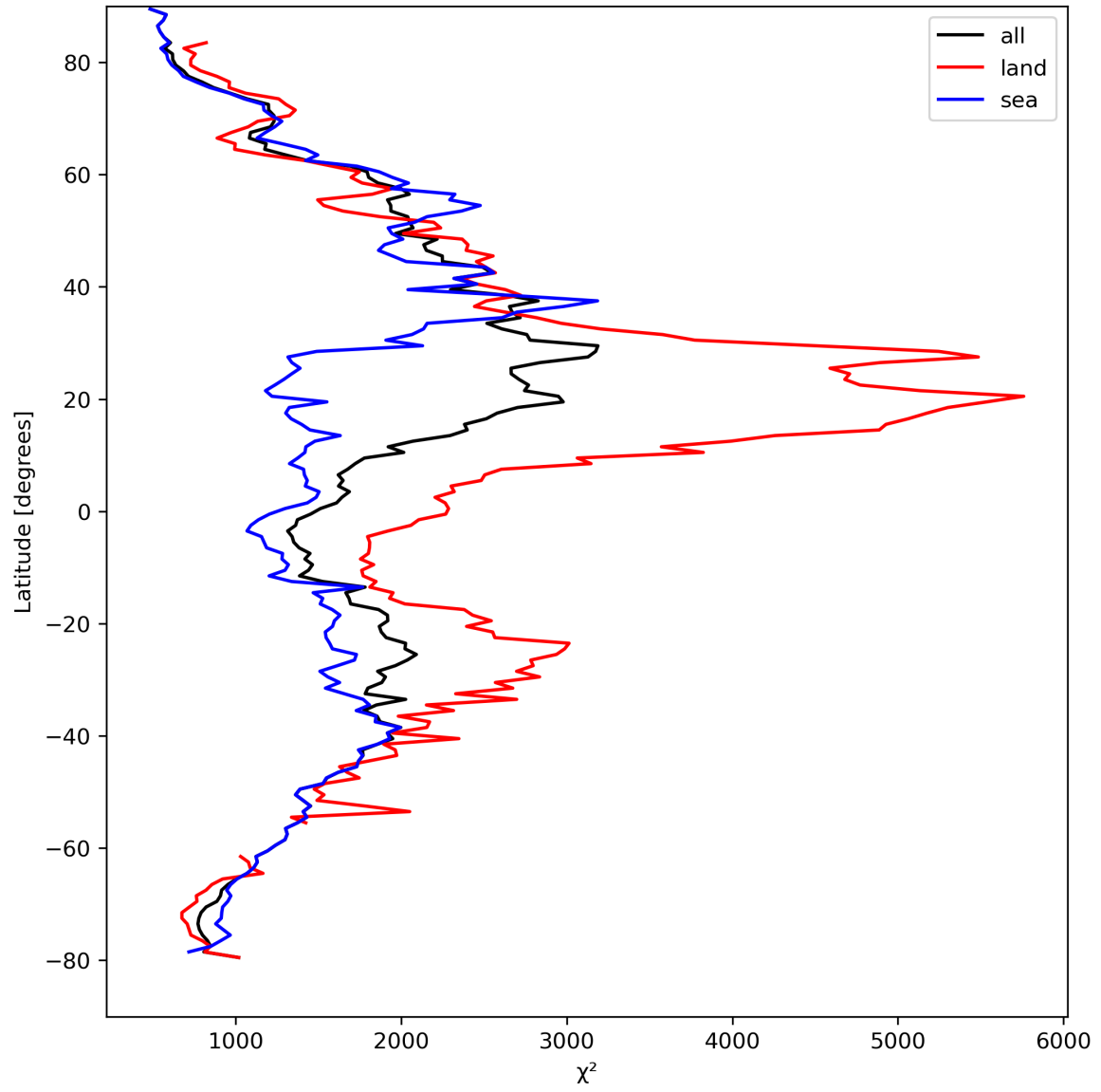
Figure 14: Zonal average of “ \chi^2 ” for 2024-04-02 to 2024-04-04.
