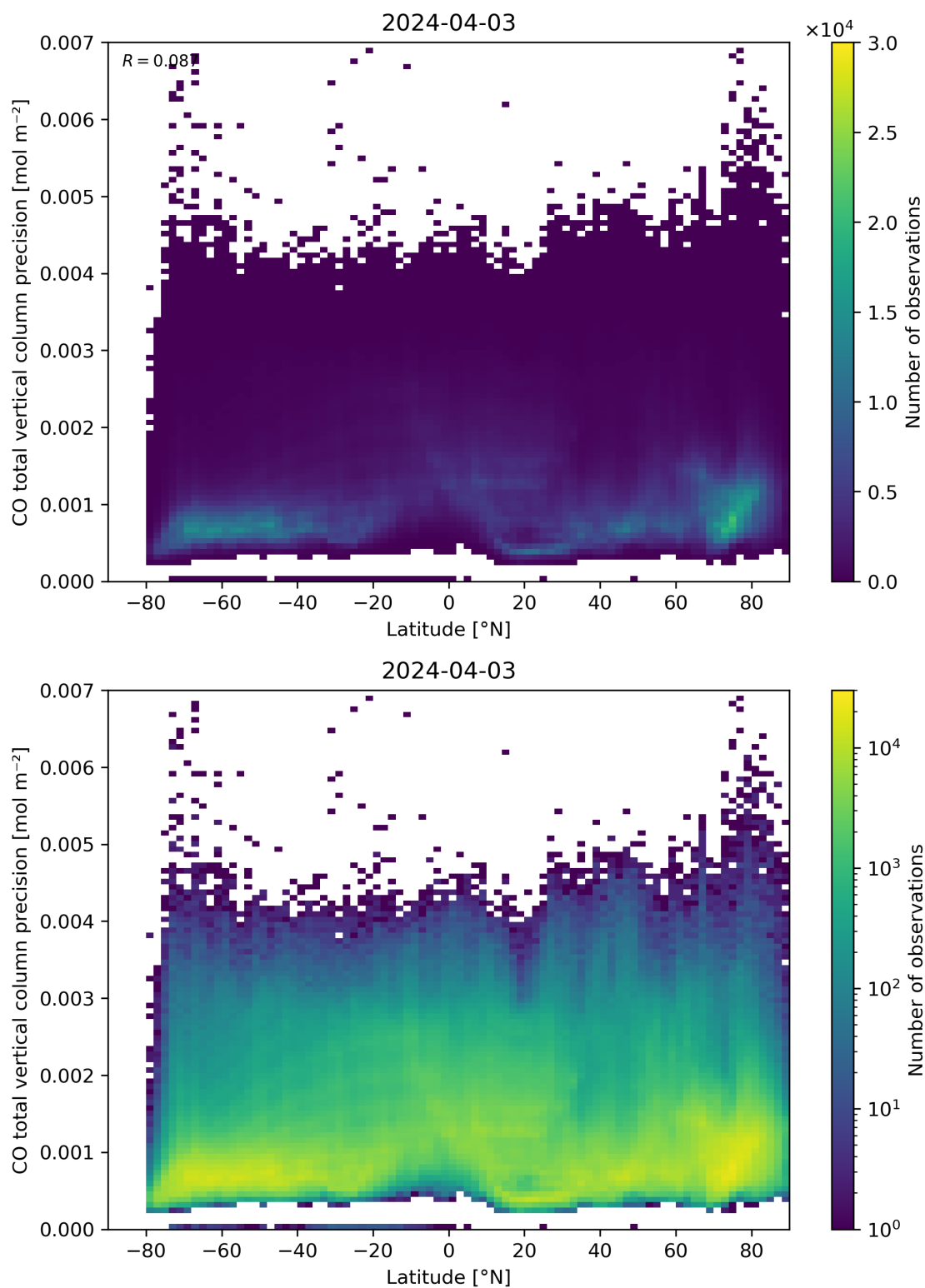
Figure 53: Scatter density plot of “Latitude” against “CO total vertical column precision” for 2024-04-02 to 2024-04-04.
