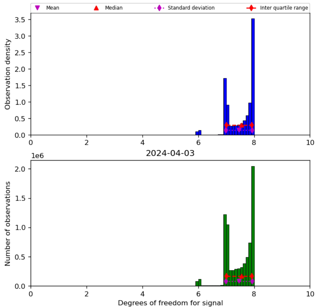
Figure 23: Histogram of “Degrees of freedom for signal” for 2024-04-02 to 2024-04-04
