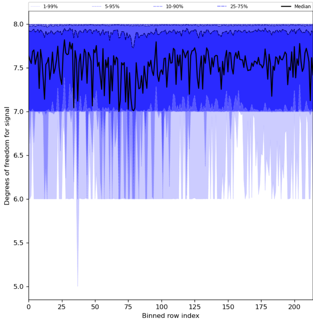
Figure 31: Along track statistics of “Degrees of freedom for signal” for 2024-04-02 to 2024-04-04
