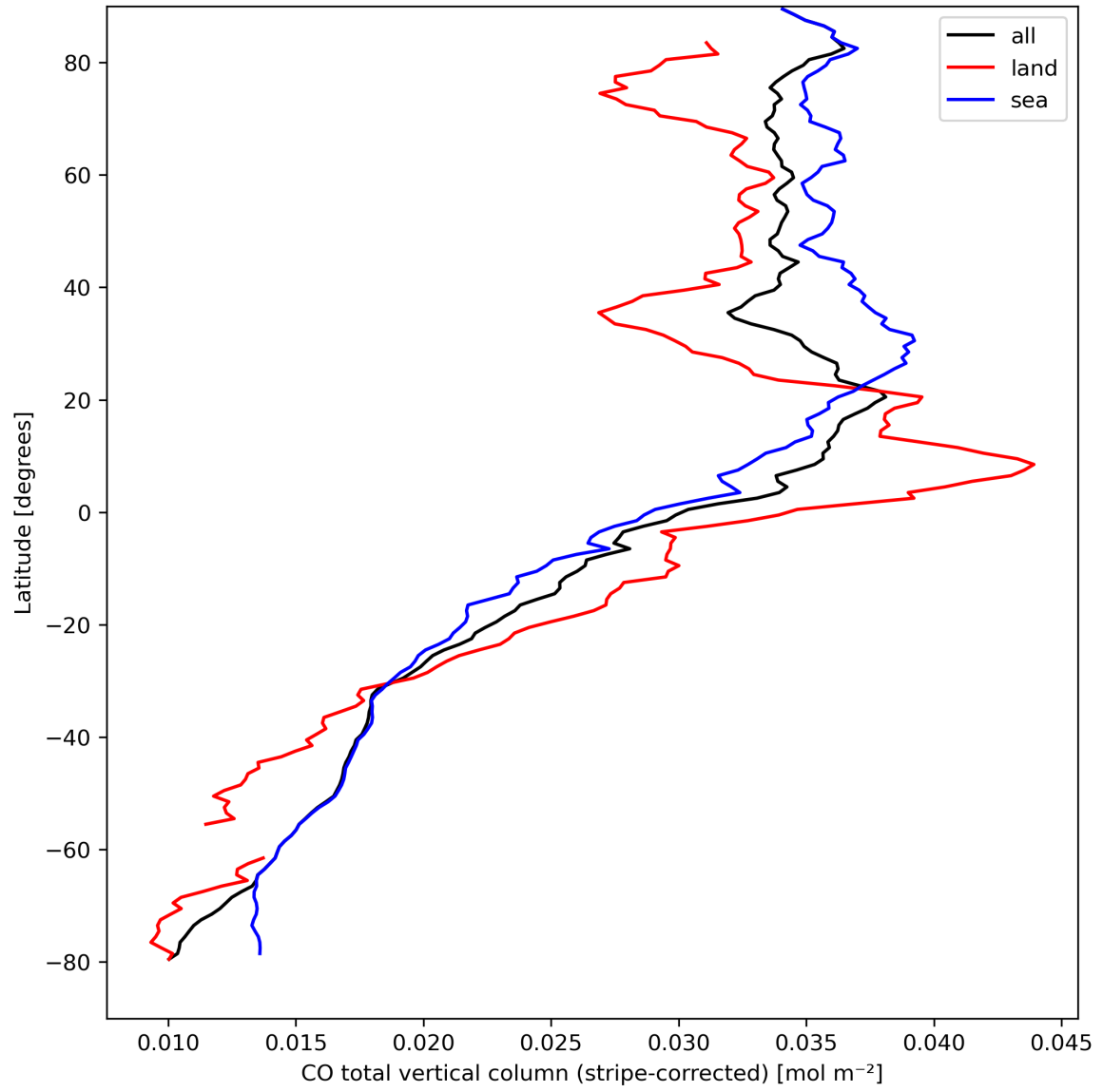
Figure 11: Zonal average of “CO total vertical column (stripe-corrected)” for 2024-04-02 to 2024-04-04.
